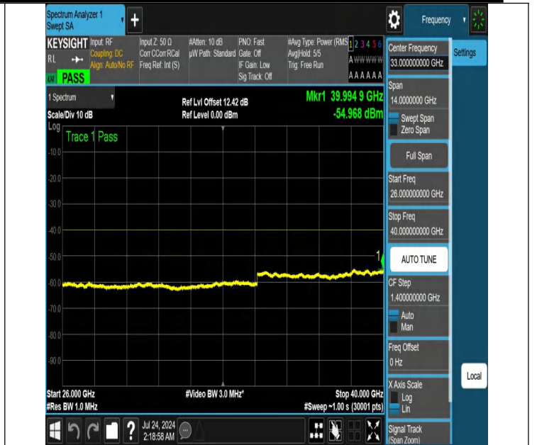
NTNV-N48-PC3-30-10-M-DFT-PI2BPSK-Edge_1RB_Right-26000-40000-Ant1-PASS
