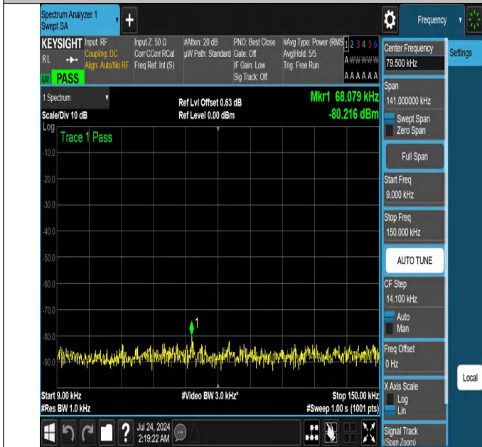
NTNV-N48-PC3-30-10-M-DFT-QPSK-Edge_1RB_Left-0.009-0.15-Ant1-PASS
