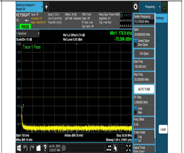
NTNV-N48-PC3-30-10-H-DFT-QPSK-Edge_1RB_Left-0.15-30-Ant1-PASS
