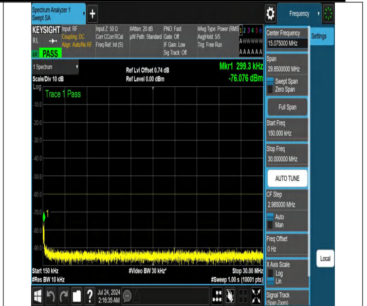
NTNV-N48-PC3-30-10-M-DFT-PI2BPSK-Edge_1RB_Left-0.15-30-Ant1-PASS
