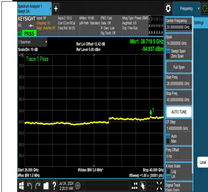
NTNV-N48-PC3-30-10-M-DFT-QPSK-Edge_1RB_Left-26000-40000-Ant1-PASS
