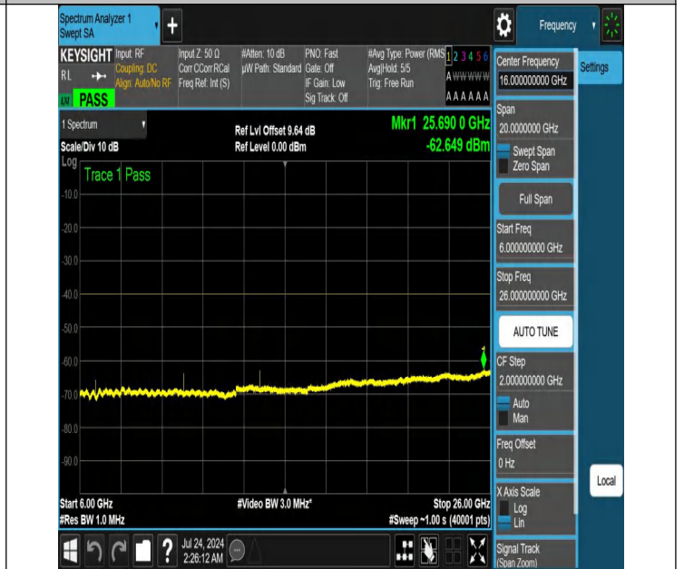
NTNV-N48-PC3-30-10-H-DFT-QPSK-Edge_1RB_Left-6000-26000 -Ant1-PASS
