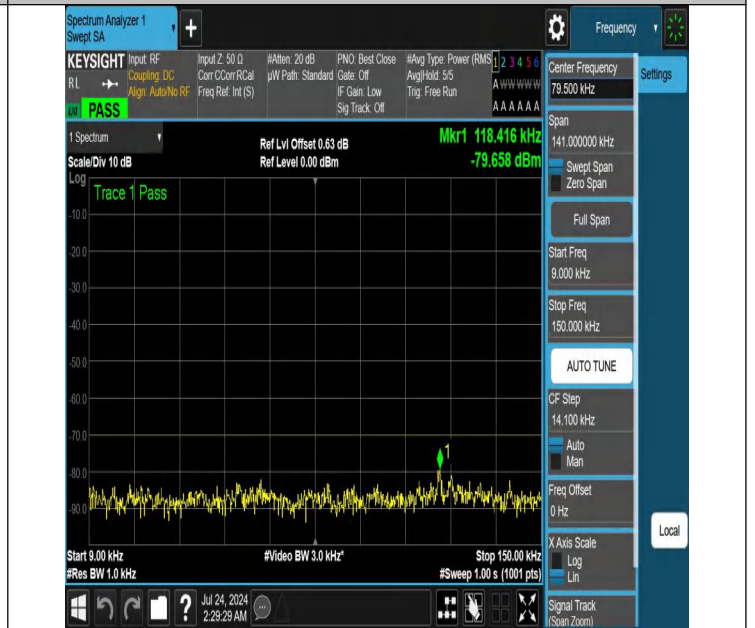
NTNV-N48-PC3-30-15-L-DFT-PI2BPSK-Edge_1RB_Right-0.009-0 .15-Ant1-PASS
