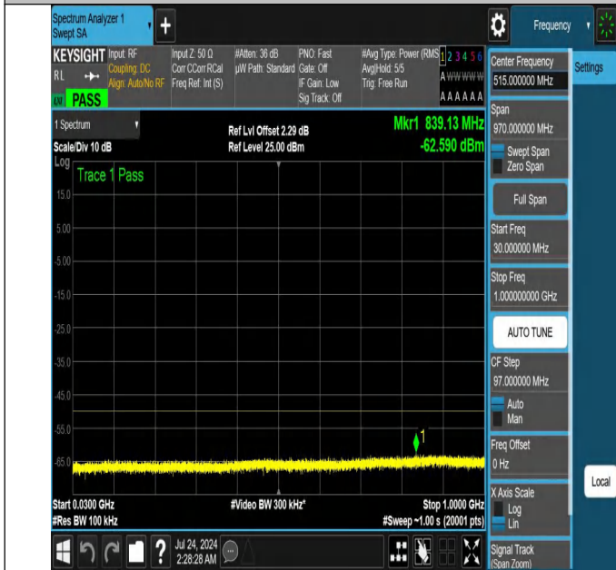
NTNV-N48-PC3-30-15-L-DFT-PI2BPSK-Edge_1RB_Left-30-1000-Ant1-PASS
