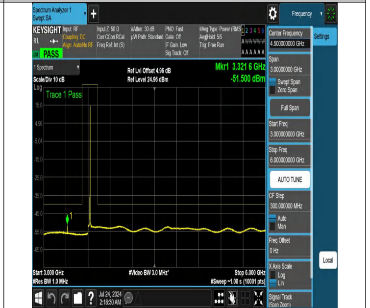
NTNV-N48-PC3-30-10-M-DFT-PI2BPSK-Edge_1RB_Right-3000-6000-Ant1-PASS
