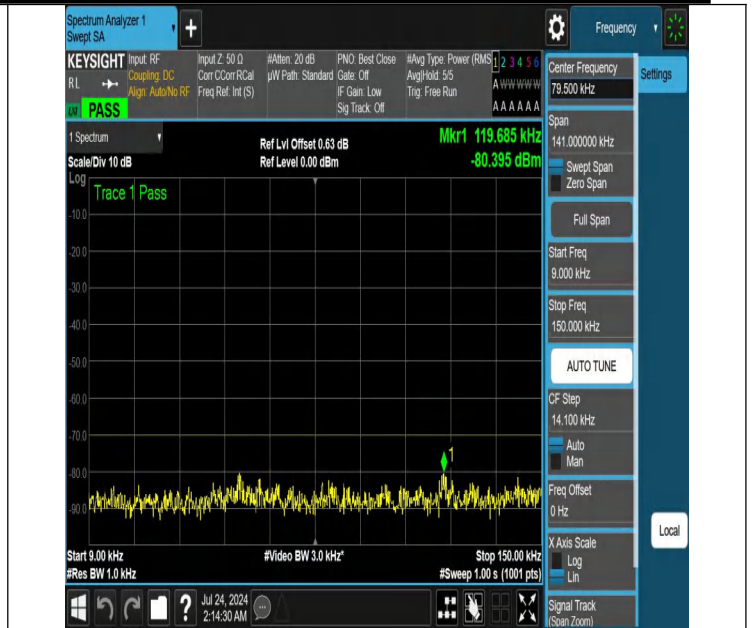
NTNV-N48-PC3-30-10-L-DFT-QPSK-Edge_1RB_Right-0.009-0.150-Ant1-PASS
