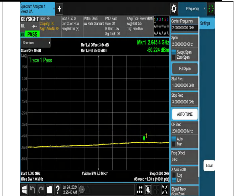
NTNV-N48-PC3-30-10-H-DFT-QPSK-Edge_1RB_Left-1000-3000-Ant1-PASS
