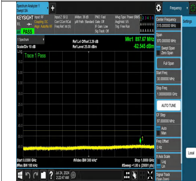
NTNV-N48-PC3-30-10-H-DFT-PI2BPSK-Edge_1RB_Left-30-1000-Ant1-PASS
