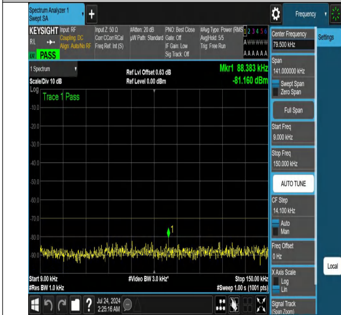
NTNV-N48-PC3-30-10-H-DFT-QPSK-Edge_1RB_Left-0.009-0.15-Ant1-PASS
