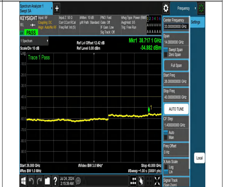
NTNV-N48-PC3-30-10-L-DFT-QPSK-Edge_1RB_Right-26000-400 00-Ant1-PASS
