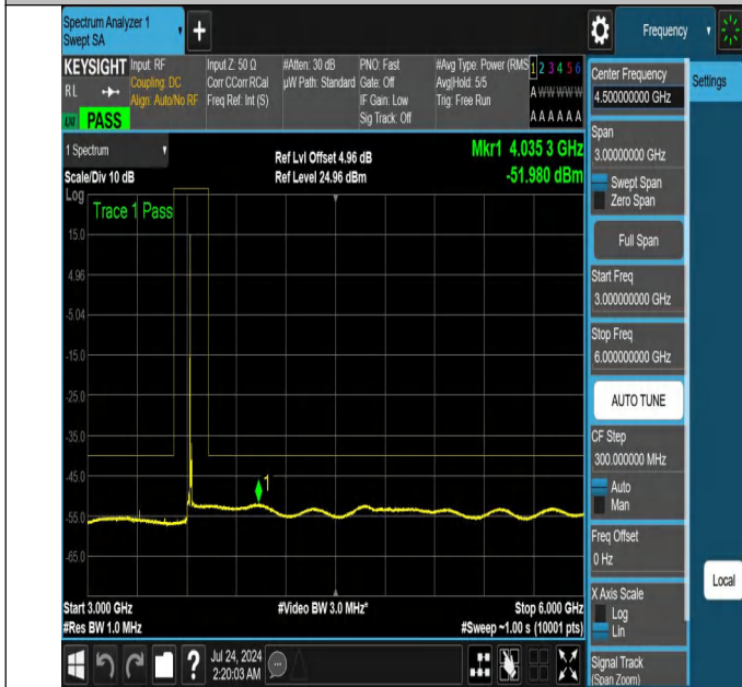
NTNV-N48-PC3-30-10-M-DFT-QPSK-Edge_1RB_Left-3000-6000-Ant1-PASS
