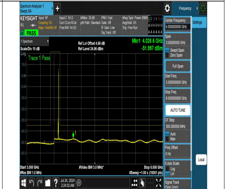
NTNV-N48-PC3-30-10-H-DFT-PI2BPSK-Edge_1RB_Right-3000-6000-Ant1-PASS
