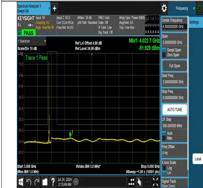
NTNV-N48-PC3-30-10-L-DFT-QPSK-Edge_1RB_Left-3000-6000-Ant1-PASS
