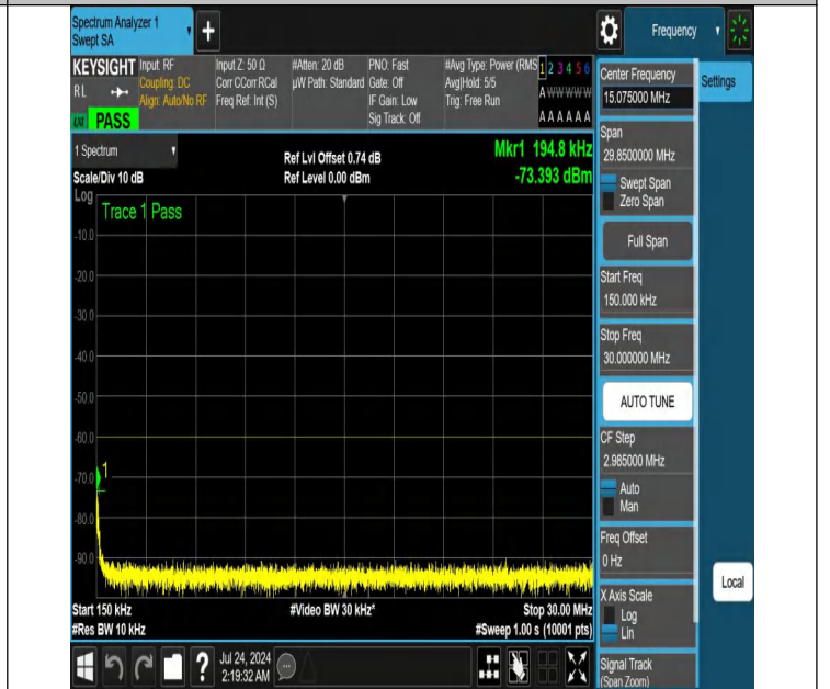
NTNV-N48-PC3-30-10-M-DFT-QPSK-Edge_1RB_Left-0.15-30-Ant1-PASS
