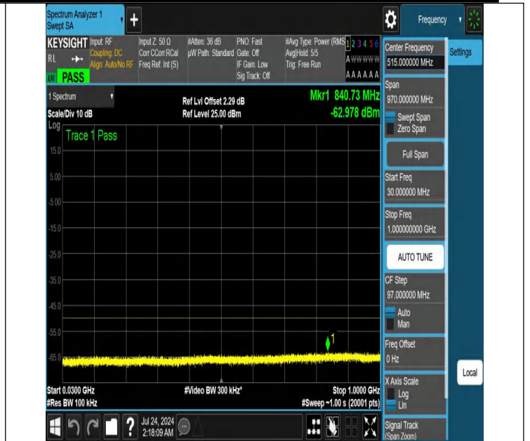
NTNV-N48-PC3-30-10-M-DFT-PI2BPSK-Edge_1RB_Right-30-100-0-Ant1-PASS
