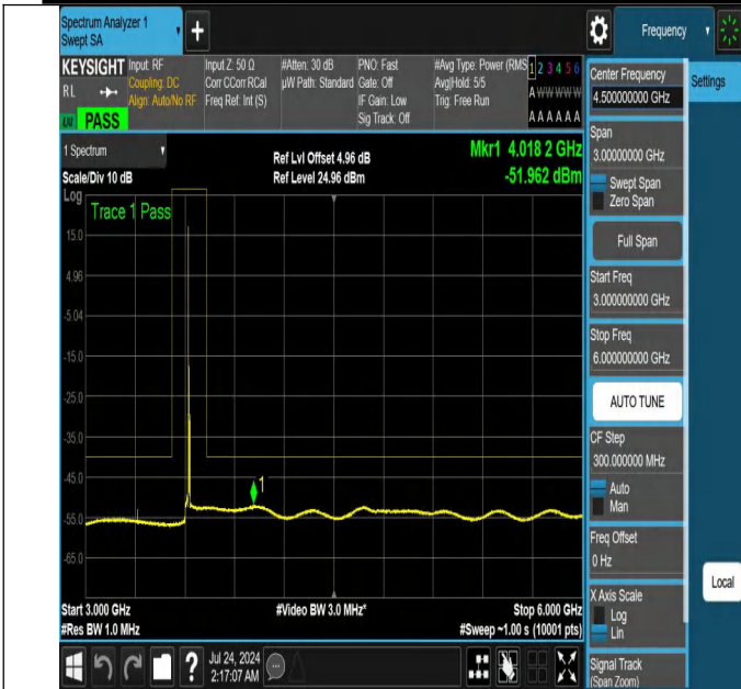
NTNV-N48-PC3-30-10-M-DFT-PI2BPSK-Edge_1RB_Left-3000-6000-Ant1-PASS
