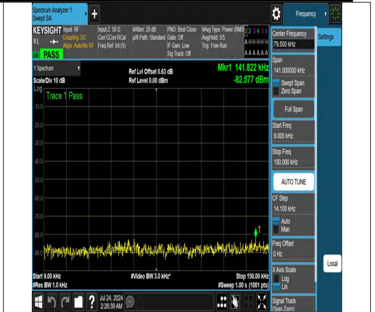
NTNV-N48-PC3-30-10-H-DFT-QPSK-Edge_1RB_Right-0.009-0.150-Ant1-PASS
