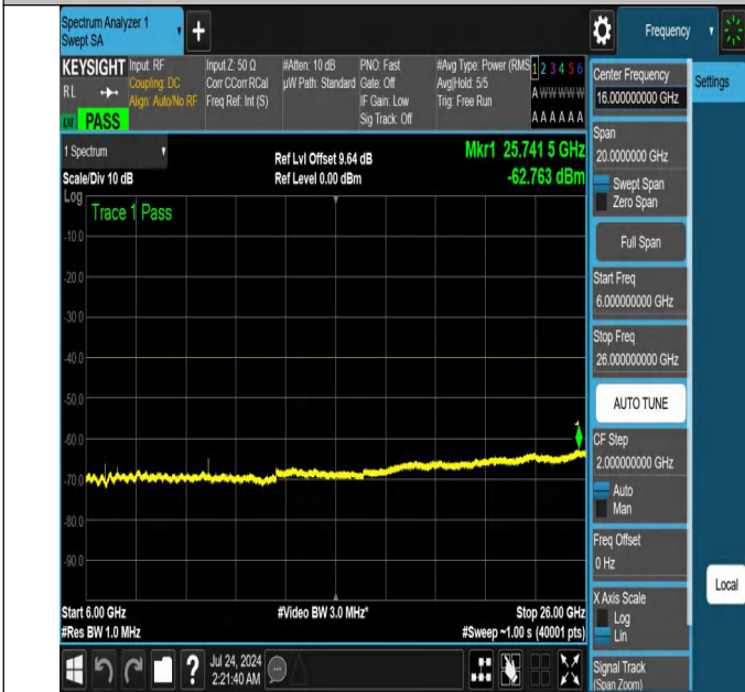
NTNV-N48-PC3-30-10-M-DFT-QPSK-Edge_1RB_Right-6000-26 000-Ant1-PASS
