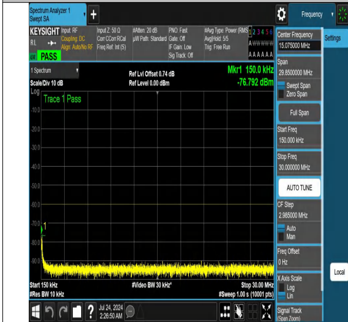
NTNV-N48-PC3-30-10-H-DFT-QPSK-Edge_1RB_Right-0.150-30.000-Ant1-PASS
