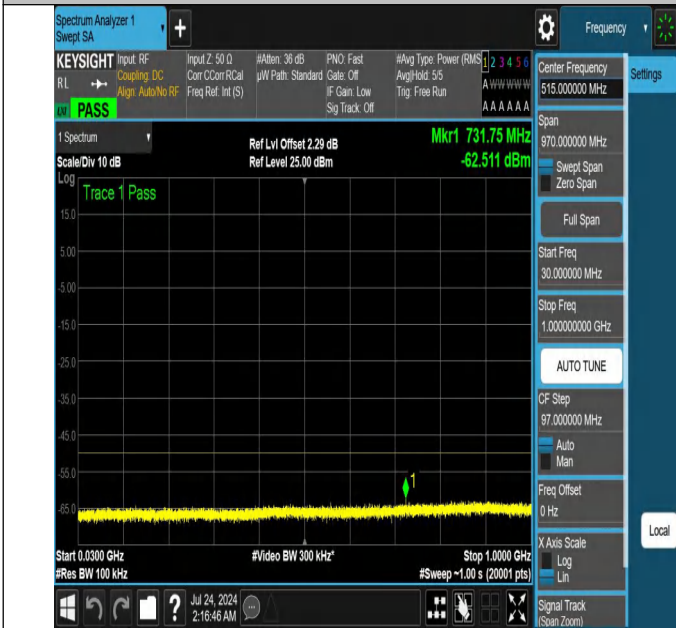
NTNV-N48-PC3-30-10-M-DFT-PI2BPSK-Edge_1RB_Left-30-100-0-Ant1-PASS
