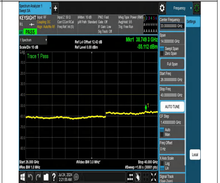
NTNV-N48-PC3-30-10-M-DFT-QPSK-Edge_1RB_Right-26000-40 000-Ant1-PASS
