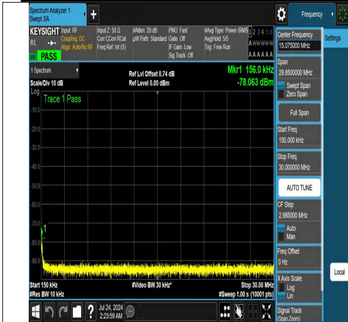
NTNV-N48-PC3-30-10-H-DFT-PI2BPSK-Edge_1RB_Right-0.15-3 0-Ant1-PASS
