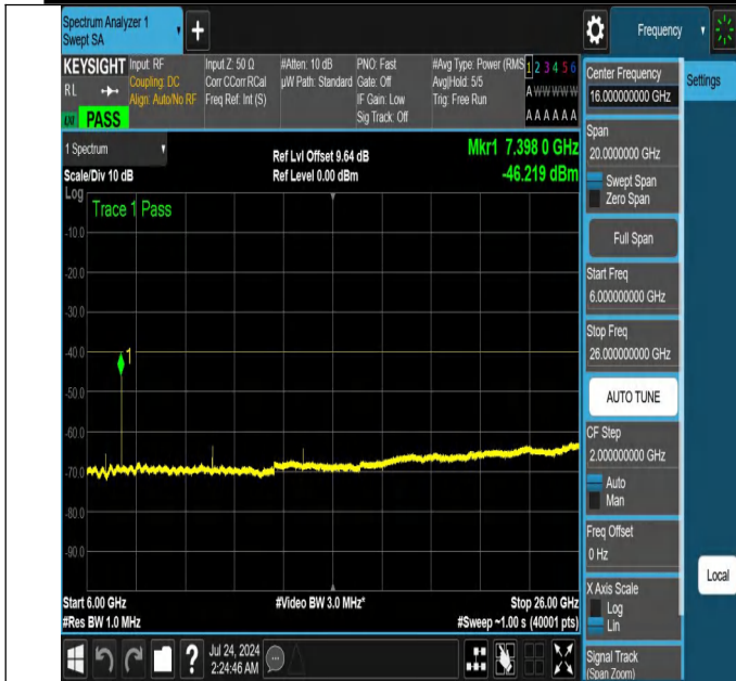
NTNV-N48-PC3-30-10-H-DFT-PI2BPSK-Edge_1RB_Right-6000-26000-Ant1-PASS
