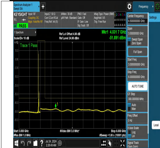
NTNV-N48-PC3-30-15-L-DFT-PI2BPSK-Edge_1RB_Left-3000-60 00-Ant1-PASS
