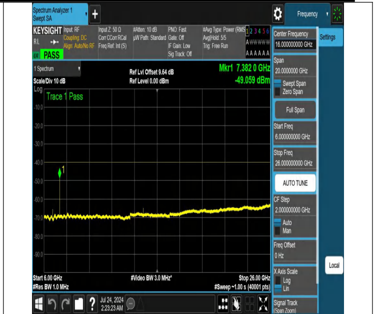
NTNV-N48-PC3-30-10-H-DFT-PI2BPSK-Edge_1RB_Left-6000-26000-Ant1-PASS
