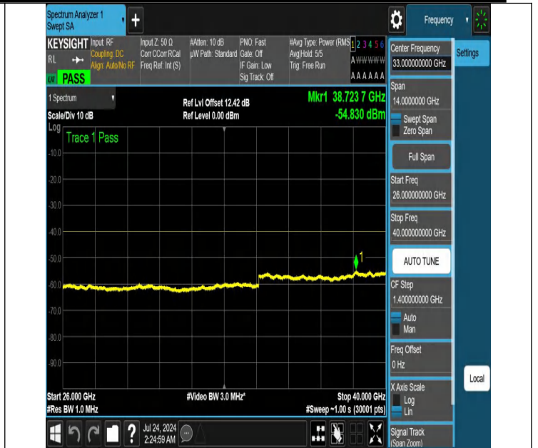
NTNV-N48-PC3-30-10-H-DFT-PI2BPSK-Edge_1RB_Right-26000-40000-Ant1-PASS
