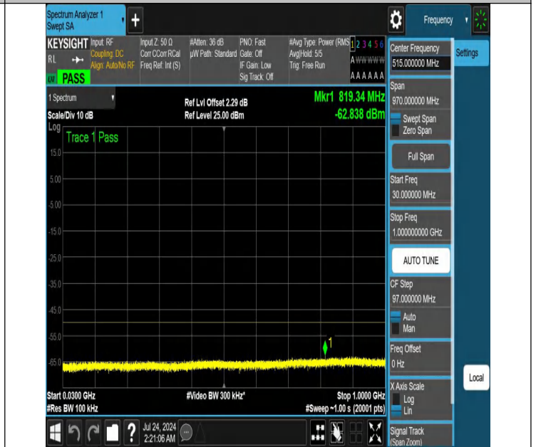
NTNV-N48-PC3-30-10-M-DFT-QPSK-Edge_1RB_Right-30-1000.000-Ant1-PASS
