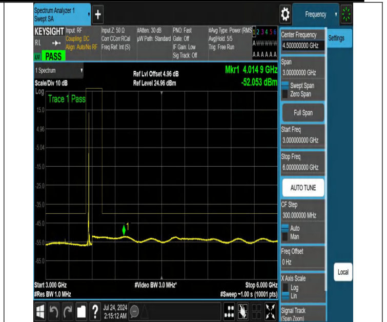
NTNV-N48-PC3-30-10-L-DFT-QPSK-Edge_1RB_Right-3000-6000 -Ant1-PASS
