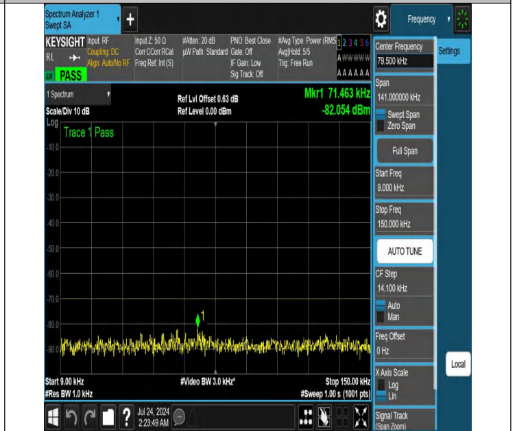
NTNV-N48-PC3-30-10-H-DFT-PI2BPSK-Edge_1RB_Right-0.009-0.15-Ant1-PASS
