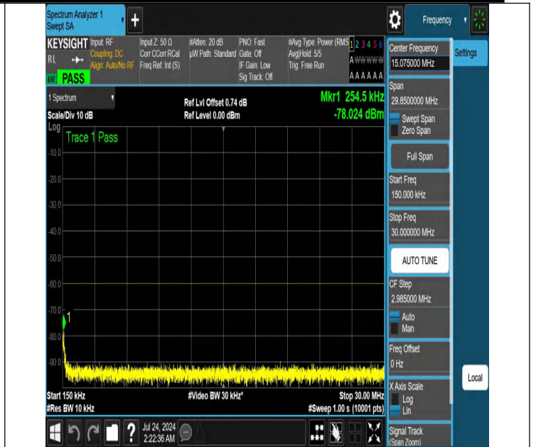
NTNV-N48-PC3-30-10-H-DFT-PI2BPSK-Edge_1RB_Left-0.15-30-Ant1-PASS
