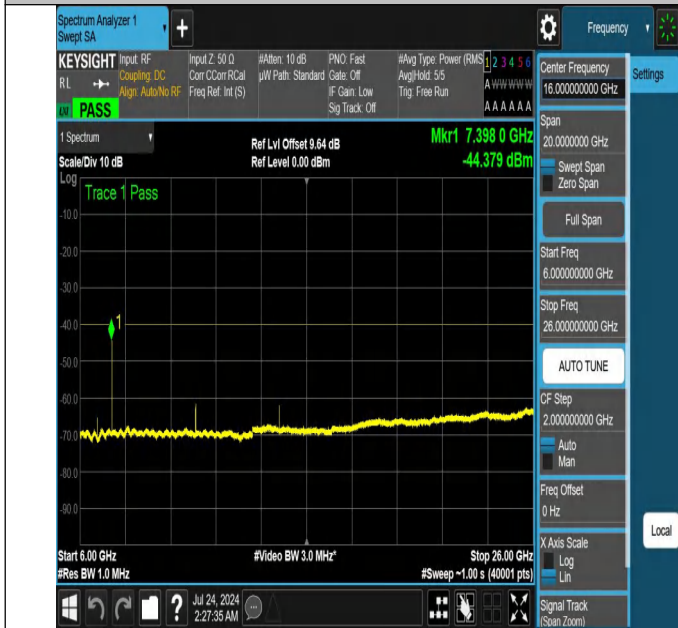
NTNV-N48-PC3-30-10-H-DFT-QPSK-Edge_1RB_Right-6000-260 00-Ant1-PASS
