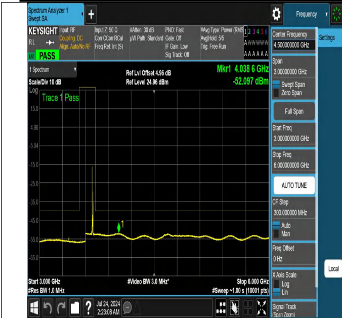
NTNV-N48-PC3-30-10-H-DFT-PI2BPSK-Edge_1RB_Left-3000-6000-Ant1-PASS
