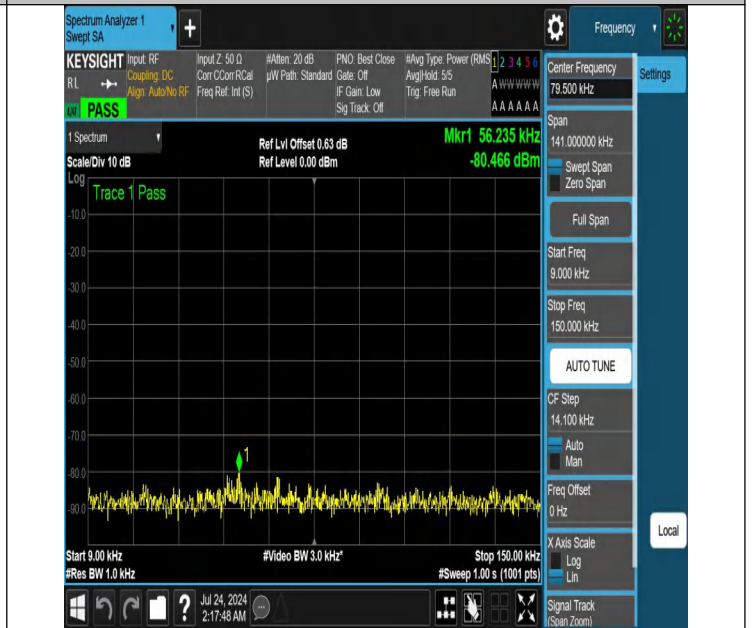
NTNV-N48-PC3-30-10-M-DFT-PI2BPSK-Edge_1RB_Right-0.009-0.15-Ant1-PASS
