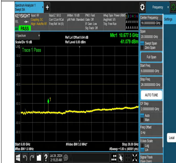
NTNV-N48-PC3-30-10-L-DFT-QPSK-Edge_1RB_Right-6000-260 00-Ant1-PASS
