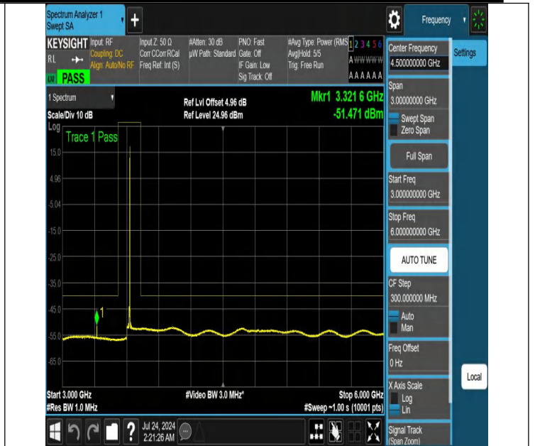
NTNV-N48-PC3-30-10-M-DFT-QPSK-Edge_1RB_Right-3000-600 0-Ant1-PASS
