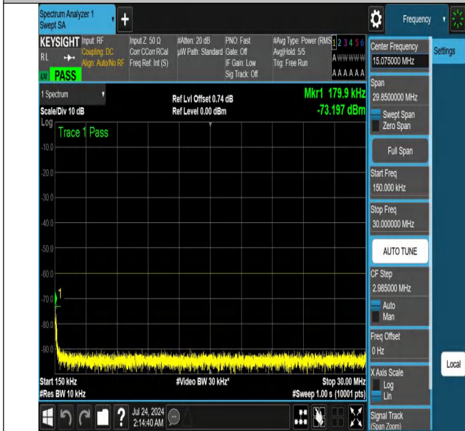
NTNV-N48-PC3-30-10-L-DFT-QPSK-Edge_1RB_Right-0.15-30-Ant1-PASS
