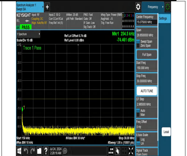
NTNV-N48-PC3-30-15-L-DFT-PI2BPSK-Edge_1RB_Left-0.15-30-Ant1-PASS
