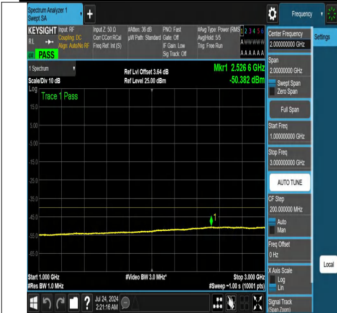
NTNV-N48-PC3-30-10-M-DFT-QPSK-Edge_1RB_Right-1000-30 00-Ant1-PASS
