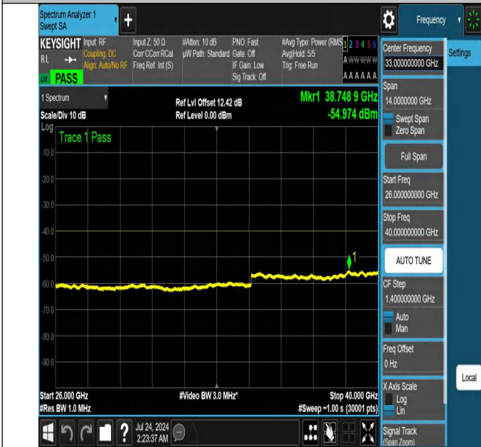
NTNV-N48-PC3-30-10-H-DFT-PI2BPSK-Edge_1RB_Left-26000-40000-Ant1-PASS
