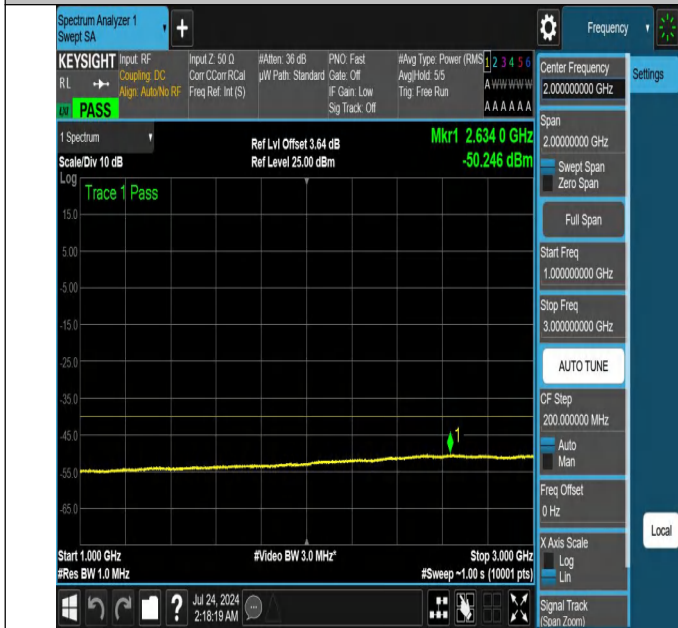
NTNV-N48-PC3-30-10-M-DFT-PI2BPSK-Edge_1RB_Right-1000-3000-Ant1-PASS
