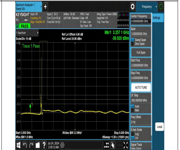
NTNV-N48-PC3-30-15-L-DFT-PI2BPSK-Edge_1RB_Right-3000-6000-Ant1-PASS
