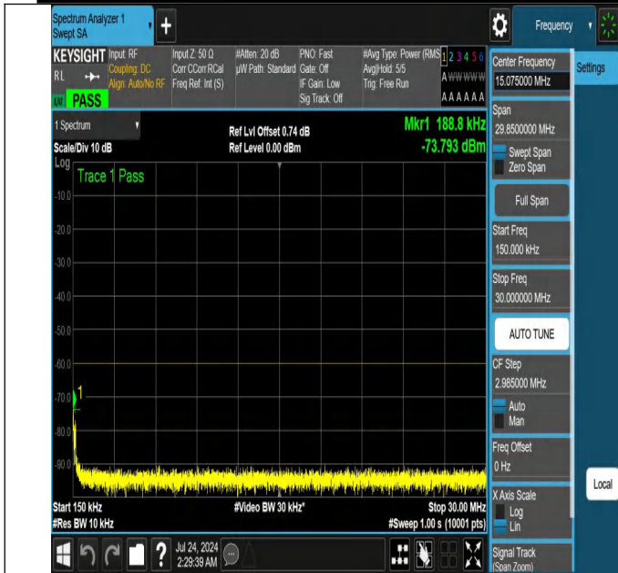
NTNV-N48-PC3-30-15-L-DFT-PI2BPSK-Edge_1RB_Right-0.15-3 0-Ant1-PASS
