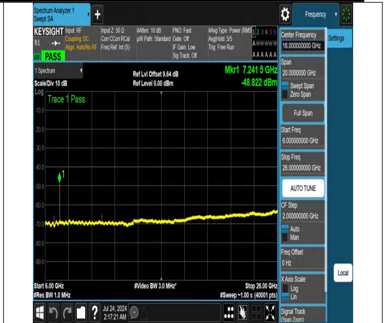
NTNV-N48-PC3-30-10-M-DFT-PI2BPSK-Edge_1RB_Left-6000-26000-Ant1-PASS
