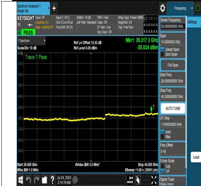
NTNV-N48-PC3-30-10-L-DFT-QPSK-Edge_1RB_Left-26000-40000-Ant1-PASS
