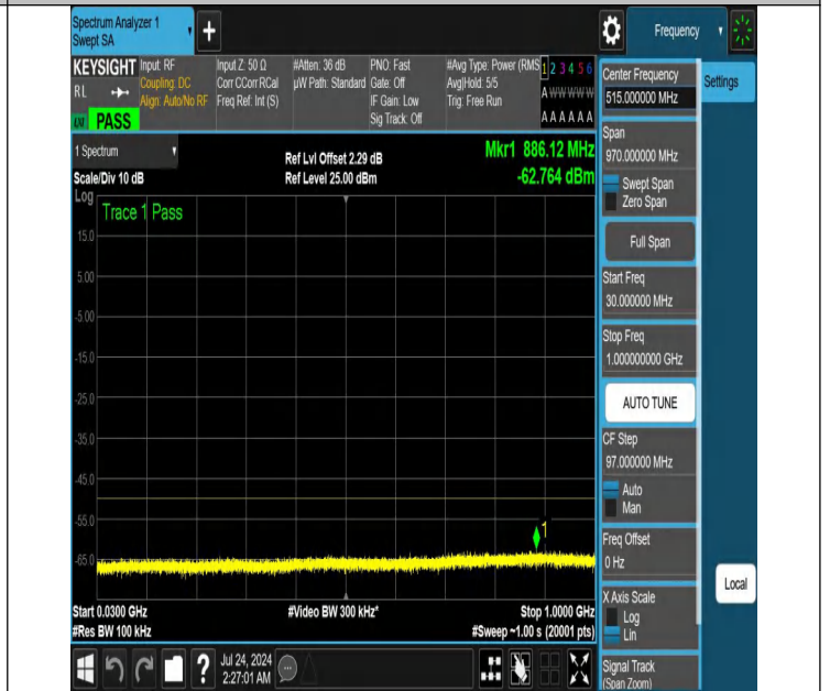
NTNV-N48-PC3-30-10-H-DFT-QPSK-Edge_1RB_Right-30-1000-Ant1-PASS
