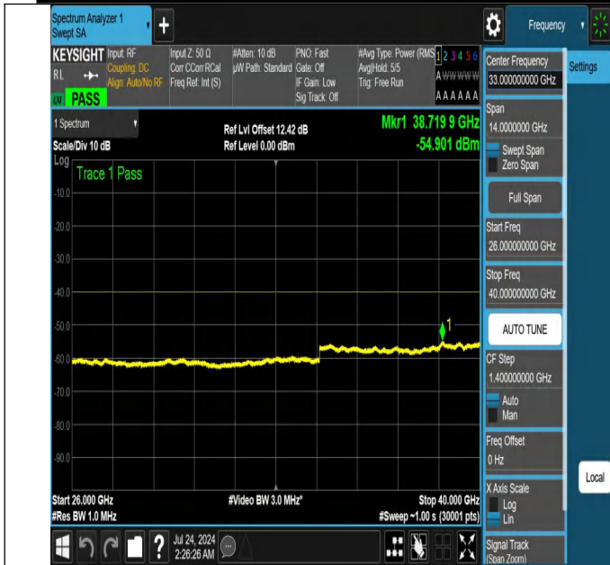
NTNV-N48-PC3-30-10-H-DFT-QPSK-Edge_1RB_Left-26000-40000-Ant1-PASS
