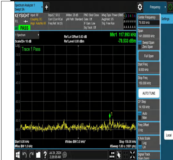
NTNV-N48-PC3-30-15-L-DFT-PI2BPSK-Edge_1RB_Left-0.009-0.15-Ant1-PASS
