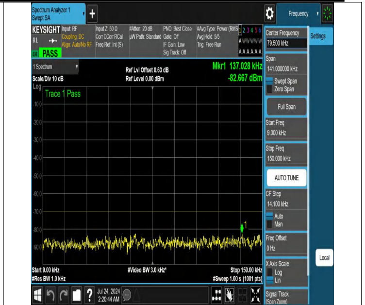
NTNV-N48-PC3-30-10-M-DFT-QPSK-Edge_1RB_Right-0.009-0.150-Ant1-PASS
