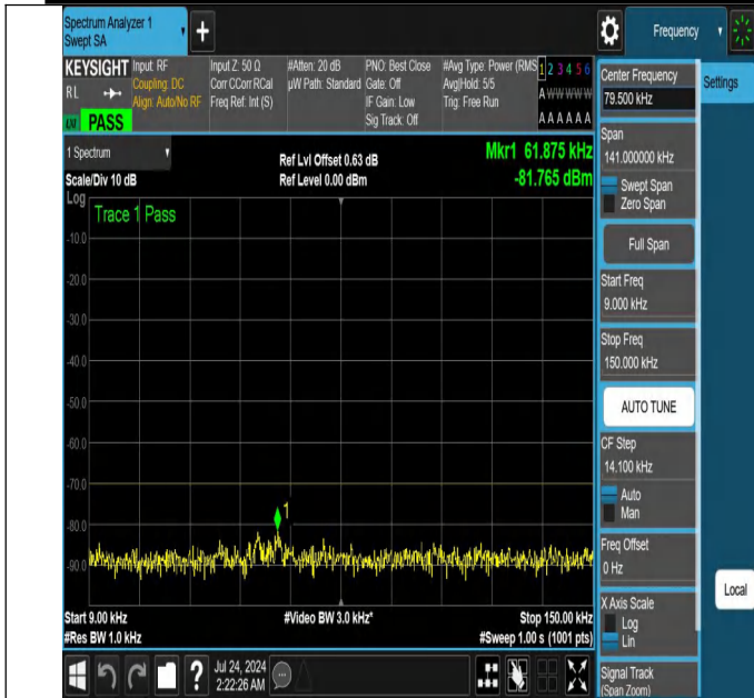
NTNV-N48-PC3-30-10-H-DFT-PI2BPSK-Edge_1RB_Left-0.009-0.15-Ant1-PASS
