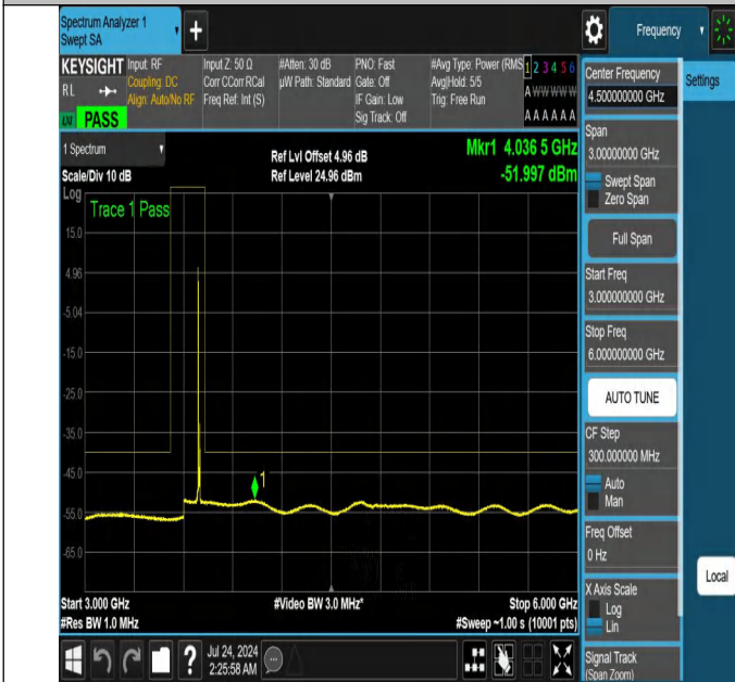
NTNV-N48-PC3-30-10-H-DFT-QPSK-Edge_1RB_Left-3000-6000 -Ant1-PASS
