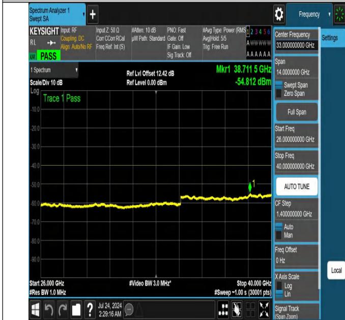
NTNV-N48-PC3-30-15-L-DFT-PI2BPSK-Edge_1RB_Left-26000-4 0000-Ant1-PASS
