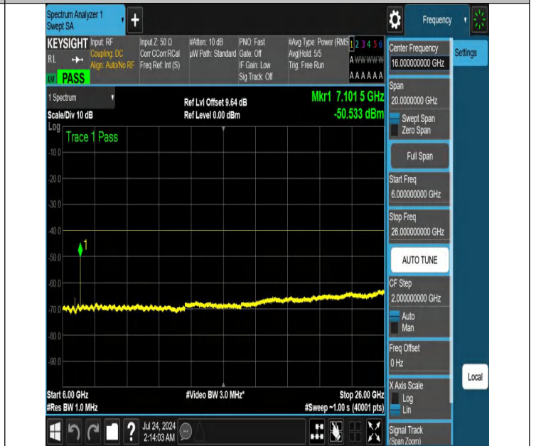
NTNV-N48-PC3-30-10-L-DFT-QPSK-Edge_1RB_Left-6000-26000-Ant1-PASS
