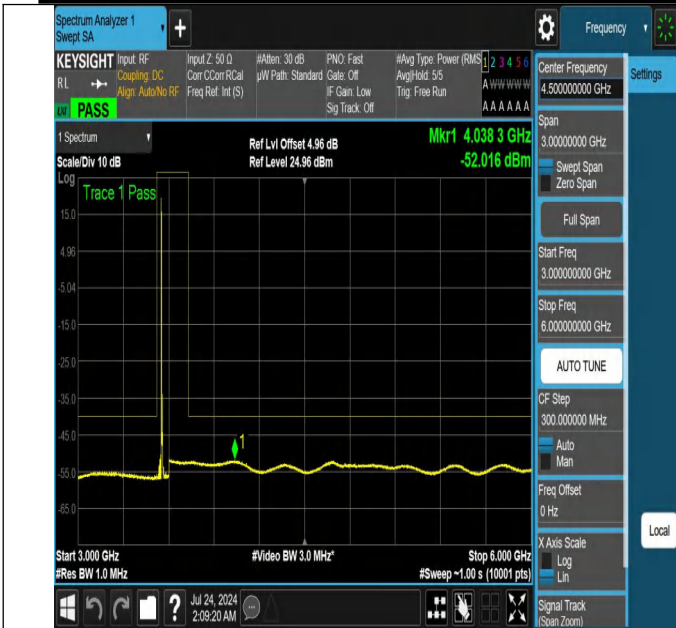
NTNV-N48-PC3-30-10-L-DFT-PI2BPSK-Edge_1RB_Left-3000-60 00-Ant1-PASS
