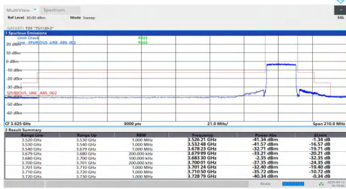
NTVN-n48-PC3-30-20-H-DFT-QPSK-Outer_Full-PASS
