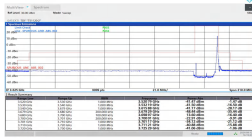
NTVN-n48-PC3-30-20-H-DFT-QPSK-Edge_1RB_Right-PASS
