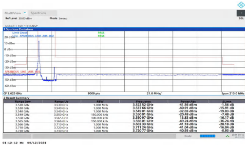
NTNV-n48-PC3-30-15-L-DFT-QPSK-Edge_1RB_Left-PASS
