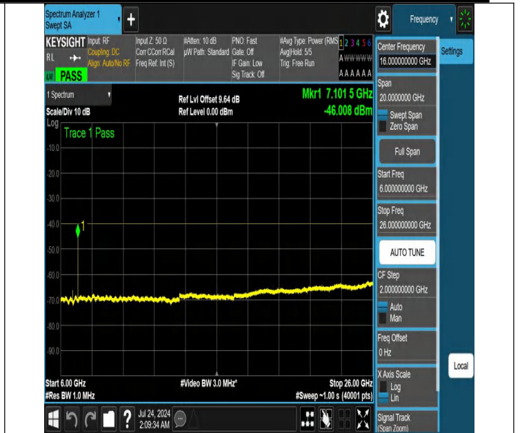
NTNV-N48-PC3-30-10-L-DFT-PI2BPSK-Edge_1RB_Left-6000-26 000-Ant1-PASS
