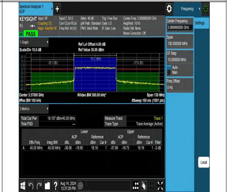
NTNV-N48-PC3-30-40-L-CP-64QAM-Outer_Full-Ant1-PASS
