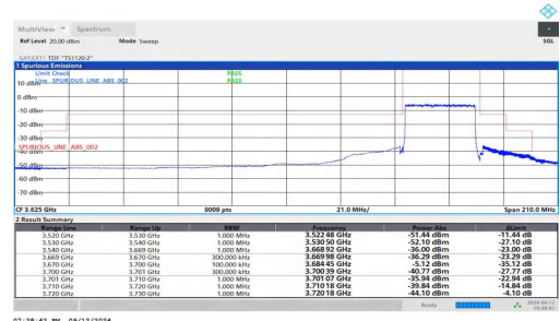
NTNV-n48-PC3-30-30-H-DFT-QPSK-Outer_Full-PASS
