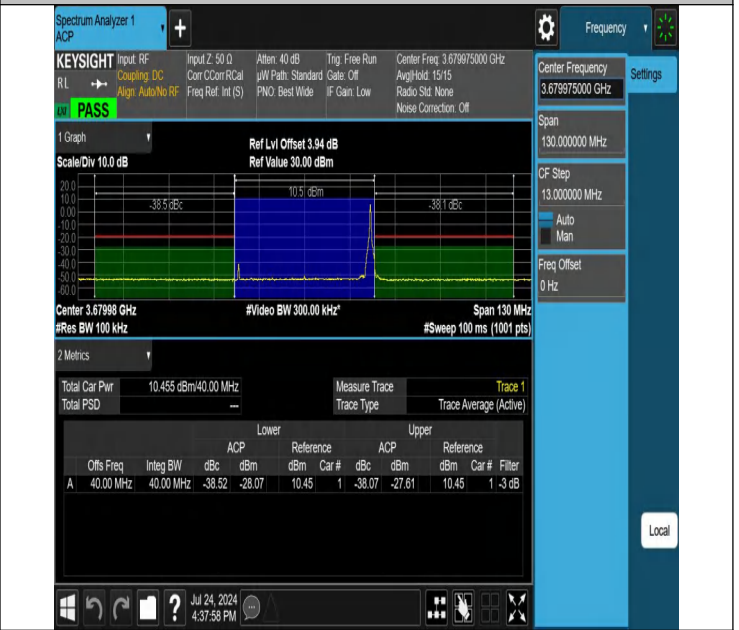
NTNV-N48-PC3-30-40-H-CP-64QAM-Edge_1RB_Right-Ant1-PAS
