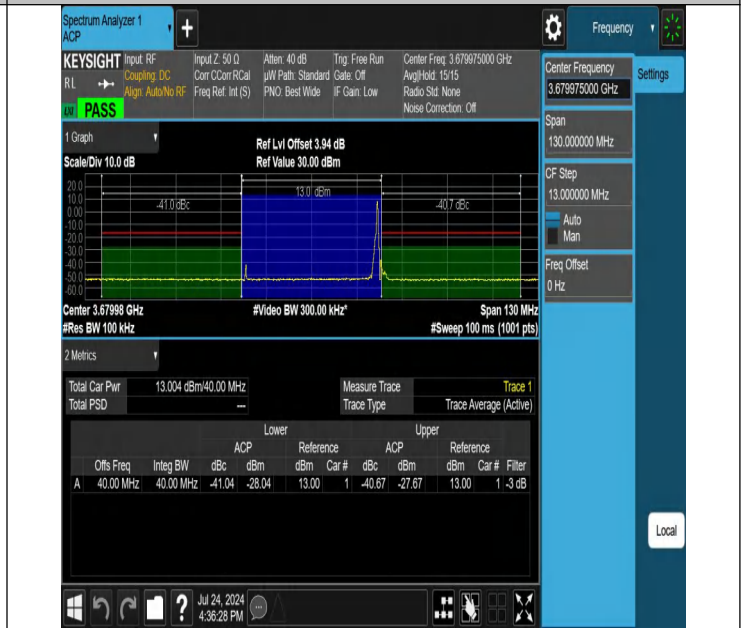
NTNV-N48-PC3-30-40-H-DFT-64QAM-Edge_1RB_Right-Ant1-PA SS
