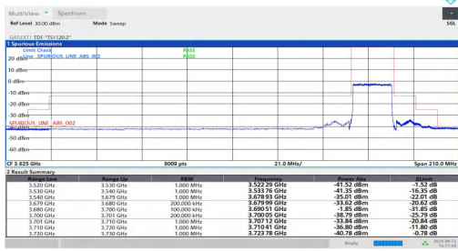
NTVN-n48-PC3-30-20-H-DFT-BPSK-Outer_Full-PASS
