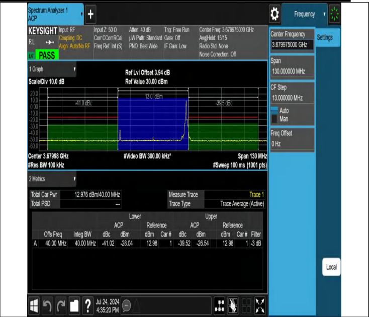
NTNV-N48-PC3-30-40-H-DFT-PI2BPSK-Edge_1RB_Right-Ant1-PASS
