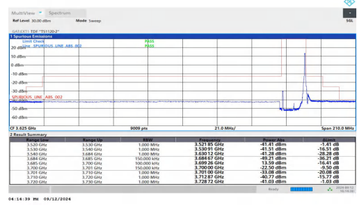
NTNV-n48-PC3-30-15-H-DFT-QPSK-Edge_1RB_Right-PASS
