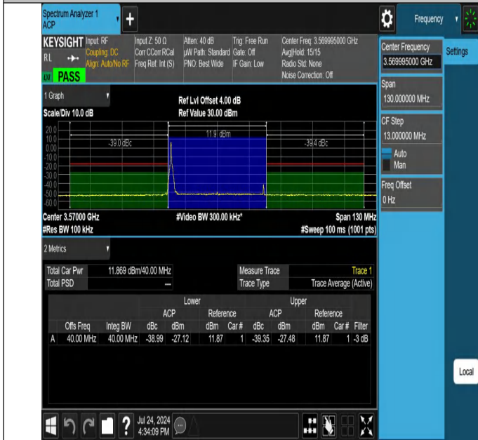
NTNV-N48-PC3-30-40-L-CP-16QAM-Edge_1RB_Left-Ant1-PASS
