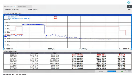
NTNV-n48-PC3-30-40-L-DFT-BPSK-Outer_Full-FAIL
