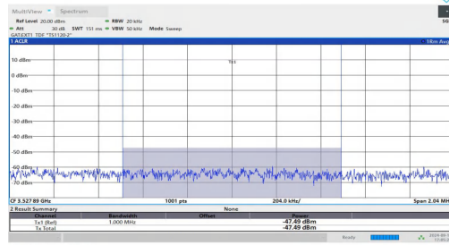
NTNV-n48-PC3-30-40-L-DFT-QPSK-Outer_Full-PASS
