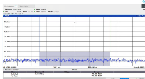
NTVN-n48-PC3-30-20-L-DFT-BPSK-Outter_Full-PASS_Final1
