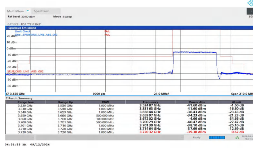
NTNV-n48-PC3-30-40-H-DFT-BPSK-Outer_Full-FAIL
