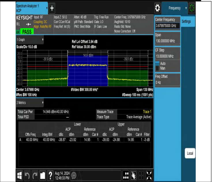
NTNV-N48-PC3-30-40-H-CP-256QAM-Outer_Full-Ant1-PASS
