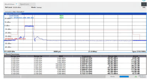
NTNV-n48-PC3-30-15-L-DFT-BPSK-Outer_Full-PASS
