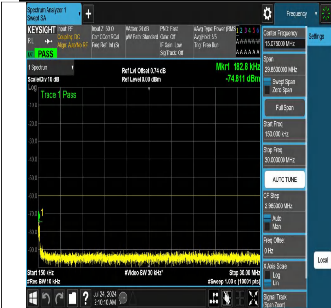
NTNV-N48-PC3-30-10-L-DFT-PI2BPSK-Edge_1RB_Right-0.15-3 0-Ant1-PASS
