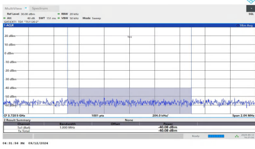
NTNV-n48-PC3-30-40-H-DFT-BPSK-Outer_Full-PASS_Final1
