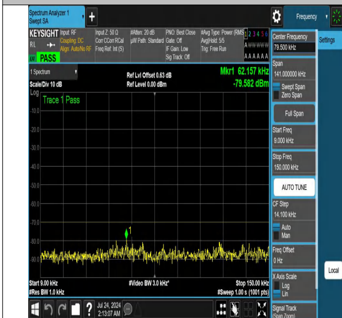
NTNV-N48-PC3-30-10-L-DFT-QPSK-Edge_1RB_Left-0.009-0.15-Ant1-PASS
