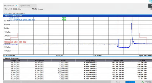
NTVN-n48-PC3-30-20-H-DFT-BPSK-Edge_1RB_Right-PASS
