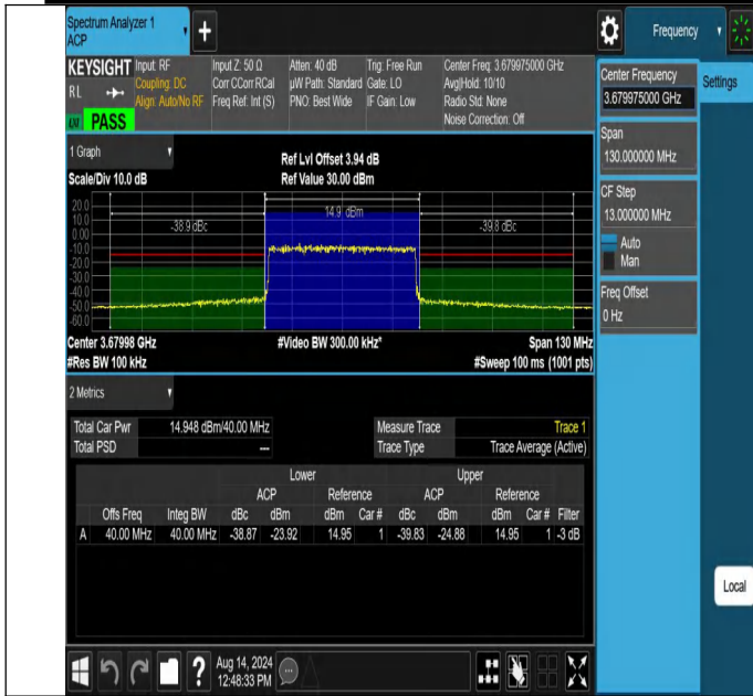
NTNV-N48-PC3-30-40-H-CP-256QAM-Outer_Full-Ant1-PASS
