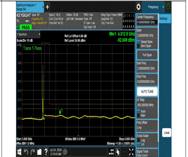
NTNV-N48-PC3-30-10-L-DFT-PI2BPSK-Edge_1RB_Right-3000-6000-Ant1-PASS
