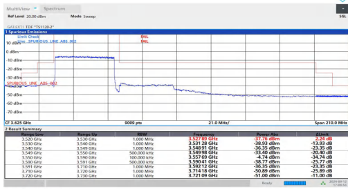
NTNV-n48-PC3-30-40-L-DFT-QPSK-Outer_Full-FAIL
