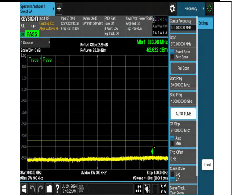
NTNV-N48-PC3-30-10-L-DFT-PI2BPSK-Edge_1RB_Right-30-100 0-Ant1-PASS
