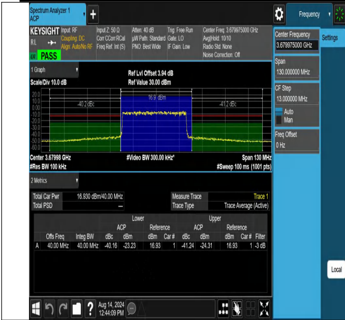
NTNV-N48-PC3-30-40-H-DFT-256QAM-Outer_Full-Ant1-PASS
