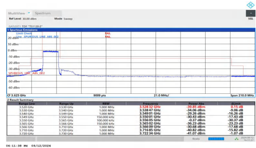
NTNV-n48-PC3-30-15-L-DFT-QPSK-Outer_Full-FAIL
