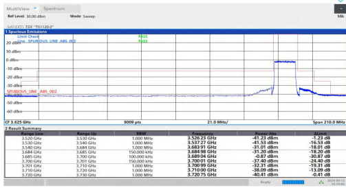
NTVN-n48-PC3-30-15-H-DFT-QPSK-Outter_Full-PASS
