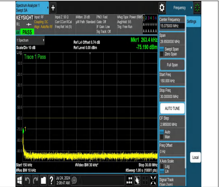
NTNV-N48-PC3-30-10-L-DFT-PI2BPSK-Edge_1RB_Left-0.15-30-Ant1-PASS
