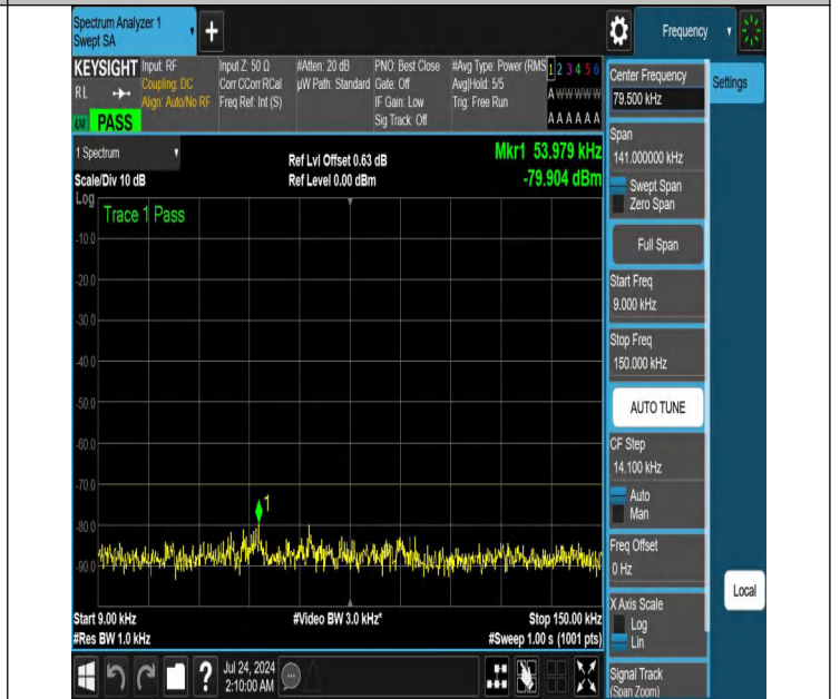
NTNV-N48-PC3-30-10-L-DFT-PI2BPSK-Edge_1RB_Right-0.009-0 .15-Ant1-PASS
