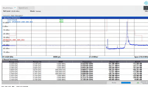
NTNV-n48-PC3-30-30-H-DFT-QPSK-Edge_1RB_Right-PASS
