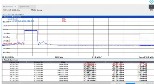
NTVN-n48-PC3-30-20-L-DFT-BPSK-Outter_Full-FAIL
