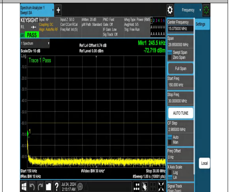
NTNV-N48-PC3-30-10-L-DFT-QPSK-Edge_1RB_Left-0.15-30-Ant1-PASS
