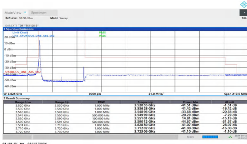
NTNV-n48-PC3-30-40-L-DFT-BPSK-Edge_1RB_Left-PASS
