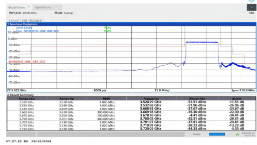
NTNV-n48-PC3-30-30-H-DFT-BPSK-Outer_Full-PASS
