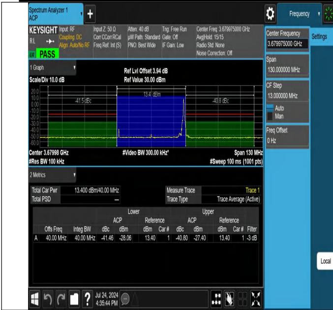
NTNV-N48-PC3-30-40-H-DFT-QPSK-Edge_1RB_Right-Ant1-PAS
