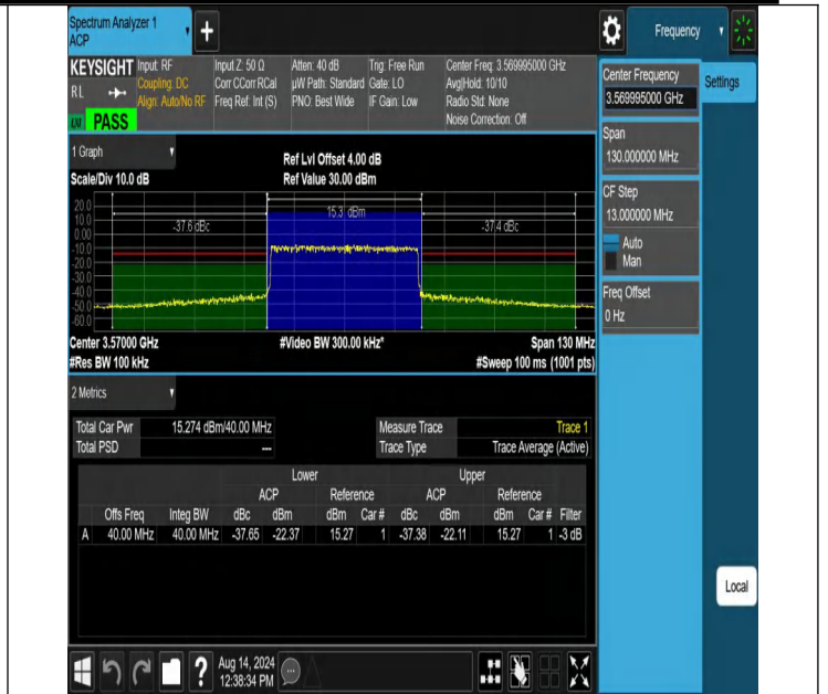
NTNV-N48-PC3-30-40-L-CP-256QAM-Outer_Full-Ant1-PASS
