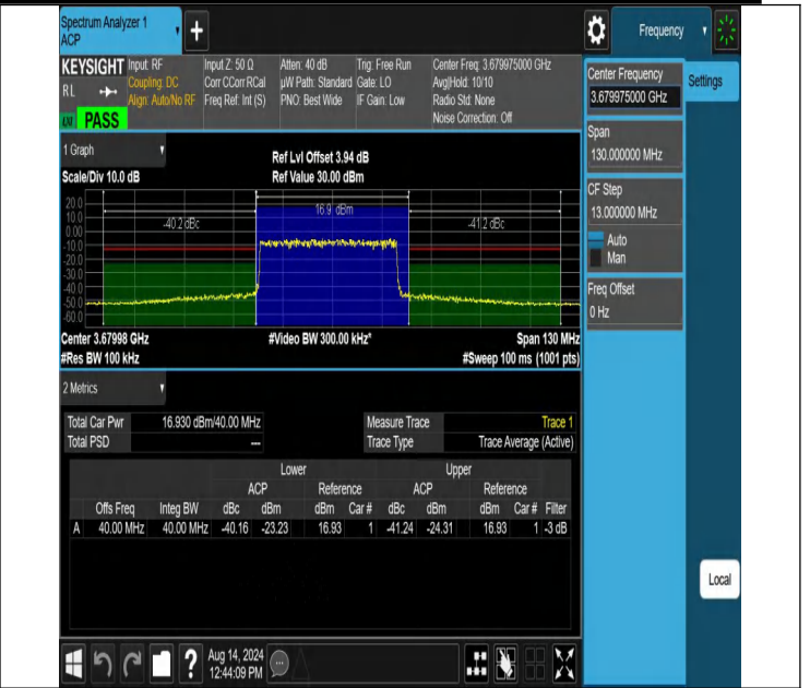
NTNV-N48-PC3-30-40-H-DFT-256QAM-Outer_Full-Ant1-PASS
