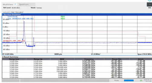
NTNV-n48-PC3-30-15-L-DFT-BPSK-Edge_1RB_Left-PASS
