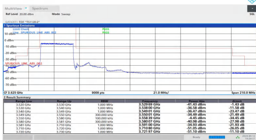
NTVN-n48-PC3-30-30-L-DFT-BPSK-Outer_Full-PASS
