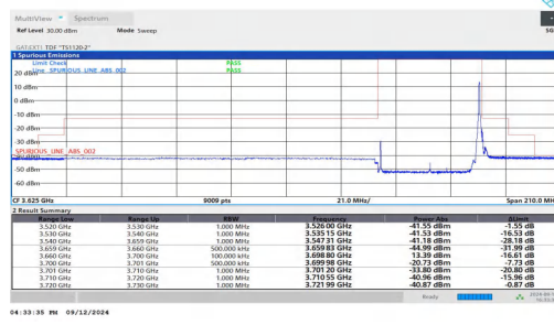
NTNV-n48-PC3-30-40-H-DFT-QPSK-Edge_1RB_Right-PASS
