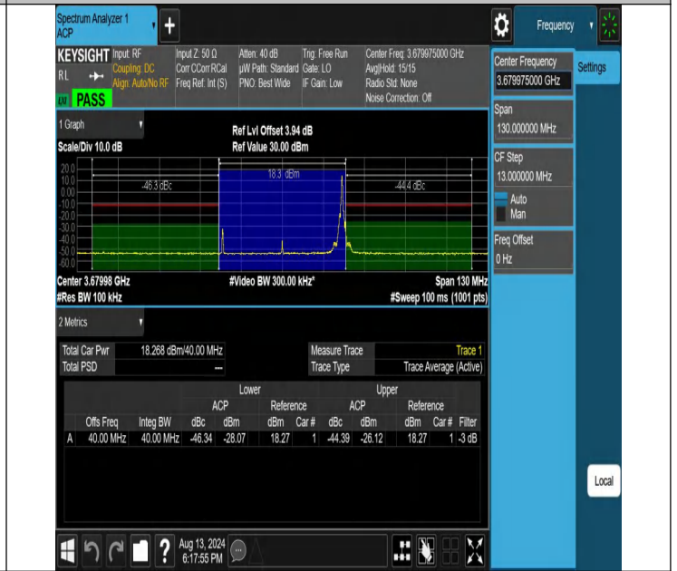
NTNV-N48-PC3-30-40-H-DFT-16QAM-Edge_1RB_Right-Ant1-PA
