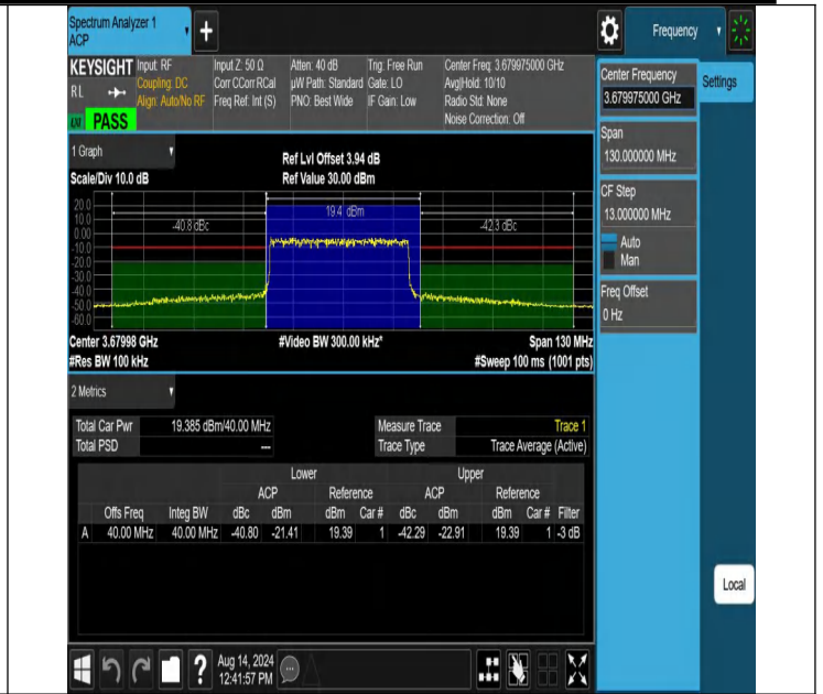
NTNV-N48-PC3-30-40-H-DFT-16QAM-Outer_Full-Ant1-PASS
