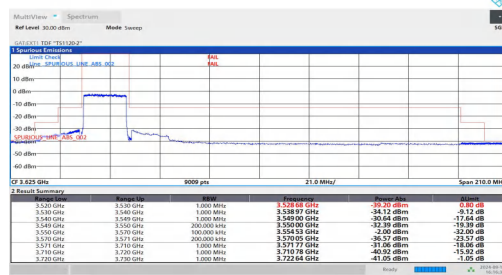
NTVN-n48-PC3-30-20-L-DFT-QPSK-Outter_Full-FAIL
