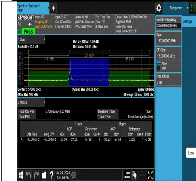
NTNV-N48-PC3-30-40-L-CP-256QAM-Edge_1RB_Left-Ant1-PAS
