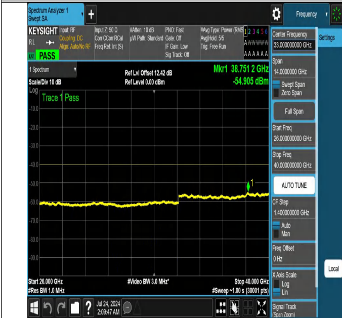
NTNV-N48-PC3-30-10-L-DFT-PI2BPSK-Edge_1RB_Left-26000-4 0000-Ant1-PASS
