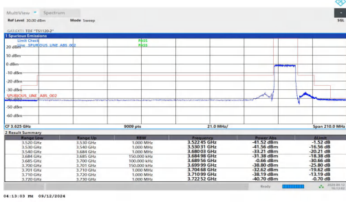
NTNV-n48-PC3-30-15-H-DFT-BPSK-Outer_Full-PASS
