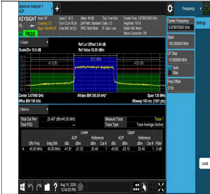
NTNV-N48-PC3-30-40-H-DFT-QPSK-Outer_Full-Ant1-PASS
