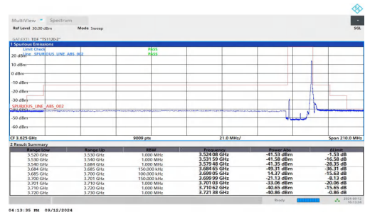
NTNV-n48-PC3-30-15-H-DFT-BPSK-Edge_1RB_Right-PASS
