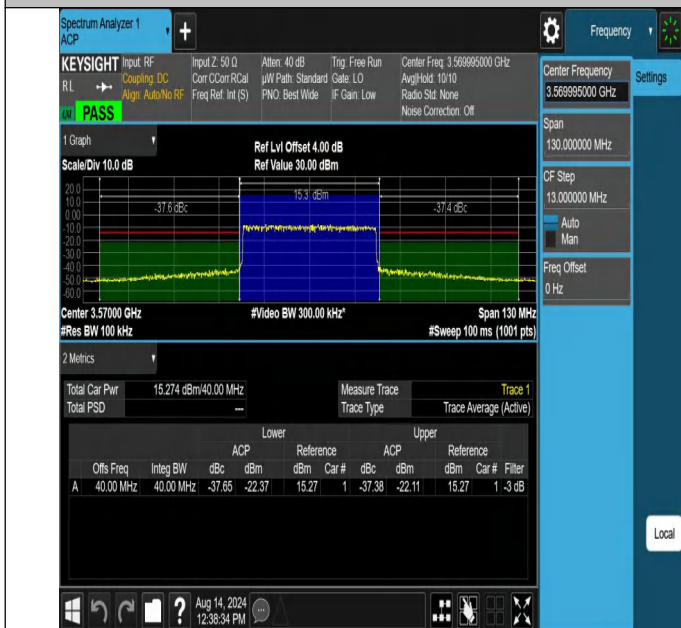
NTNV-N48-PC3-30-40-L-CP-256QAM-Outer_Full-Ant1-PASS
