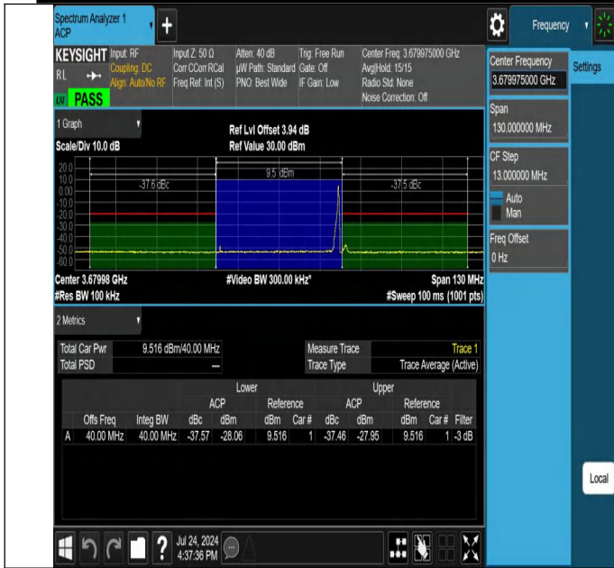
NTNV-N48-PC3-30-40-H-CP-16QAM-Edge_1RB_Right-Ant1-PAS
