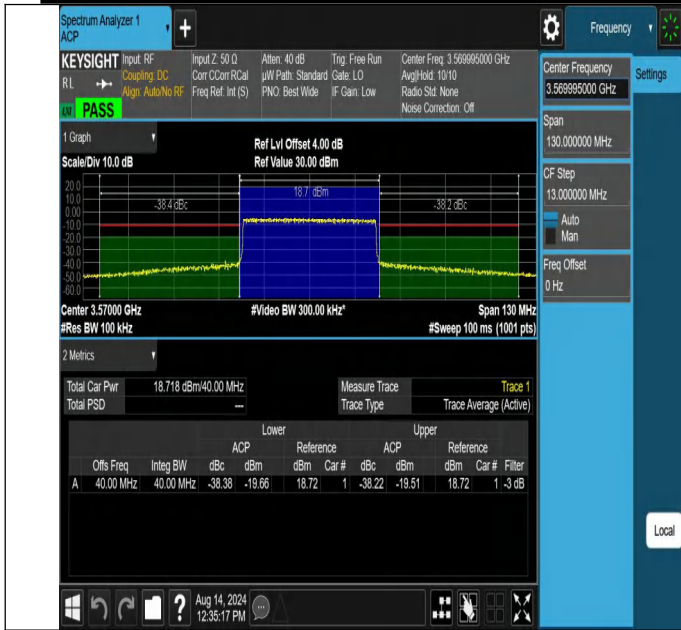
NTNV-N48-PC3-30-40-L-CP-QPSK-Outer_Full-Ant1-PASS
