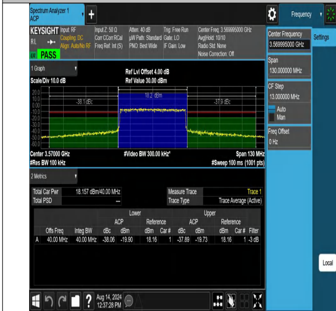
NTNV-N48-PC3-30-40-L-CP-64QAM-Outer_Full-Ant1-PASS
