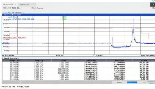
NTNV-n48-PC3-30-30-H-DFT-BPSK-Edge_1RB_Right-PASS
