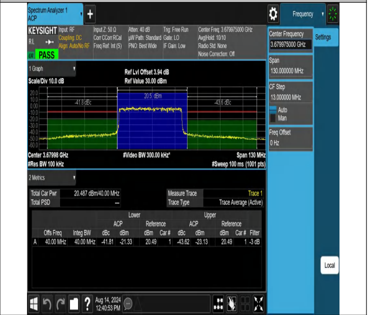
NTNV-N48-PC3-30-40-H-DFT-QPSK-Outer_Full-Ant1-PASS
