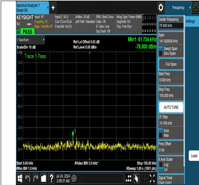
NTNV-N48-PC3-30-10-L-DFT-PI2BPSK-Edge_1RB_Left-0.009-0.15-Ant1-PASS
