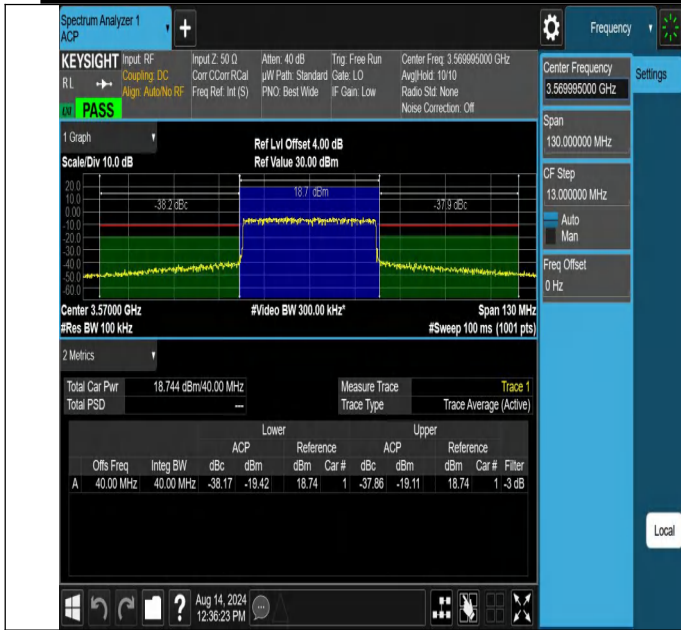
NTNV-N48-PC3-30-40-L-CP-16QAM-Outer_Full-Ant1-PASS
