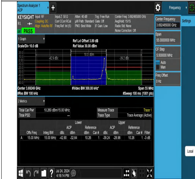
NTNV-N48-PC3-30-15-H-DFT-256QAM-Edge_1RB_Right-Ant1-PASS
