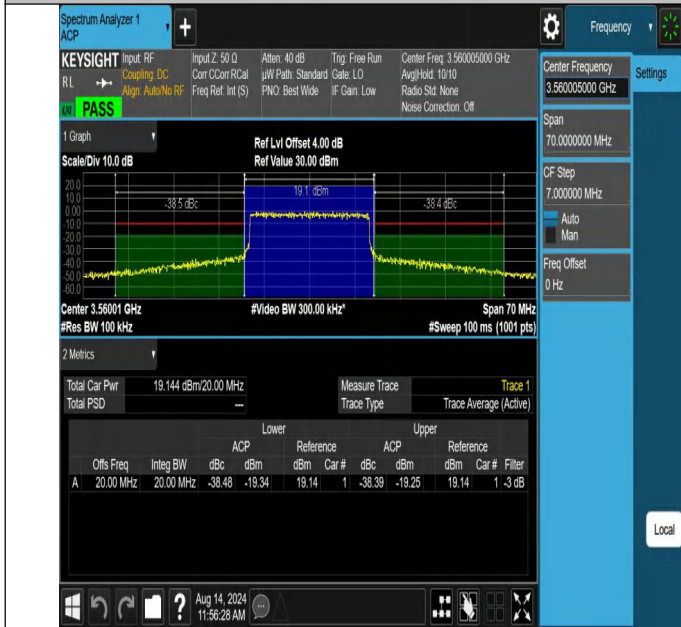
NTNV-N48-PC3-30-20-L-CP-16QAM-Outer_Full-Ant1-PASS
