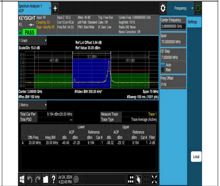
NTNV-N48-PC3-30-20-H-CP-QPSK-Edge_1RB_Right-Ant1-PASS
