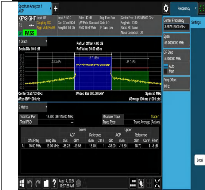
NTNV-N48-PC3-30-15-L-CP-64QAM-Outter_Full-Ant1-PASS
