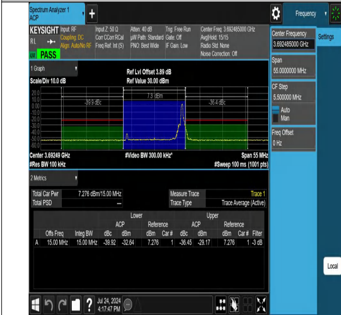
NTNV-N48-PC3-30-15-H-CP-256QAM-Edge_1RB_Right-Ant1-PA
