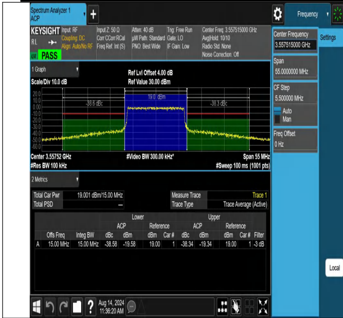
NTNV-N48-PC3-30-15-L-CP-16QAM-Outer_Full-Ant1-PASS
