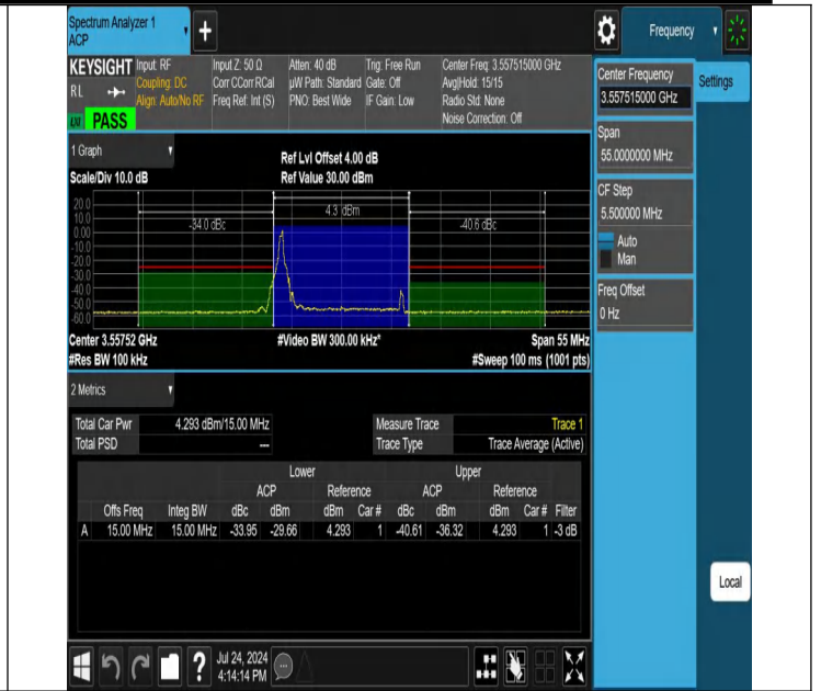
NTNV-N48-PC3-30-15-L-CP-256QAM-Edge_1RB_Left-Ant1-PASS
