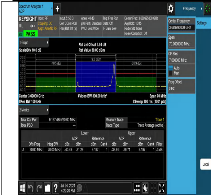
NTNV-N48-PC3-30-20-H-DFT-256QAM-Edge_1RB_Right-Ant1-PASS
