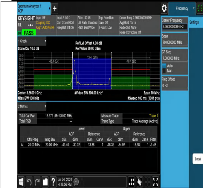
NTNV-N48-PC3-30-20-L-DFT-64QAM-Edge_1RB_Left-Ant1-PAS
