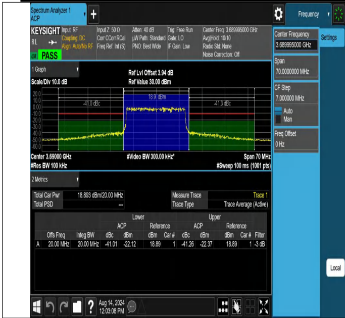
NTNV-N48-PC3-30-20-H-DFT-64QAM-Outer_Full-Ant1-PASS
