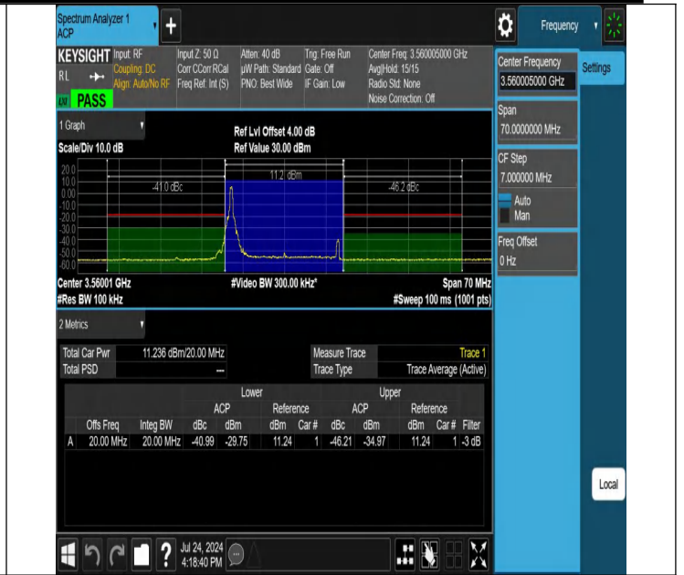
NTNV-N48-PC3-30-20-L-DFT-16QAM-Edge_1RB_Left-Ant1-PAS S
