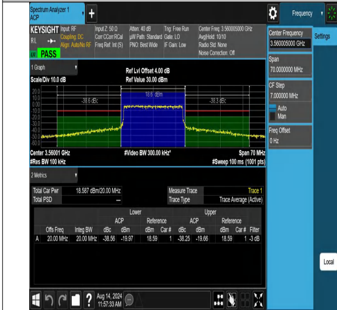
NTNV-N48-PC3-30-20-L-CP-64QAM-Outer_Full-Ant1-PASS
