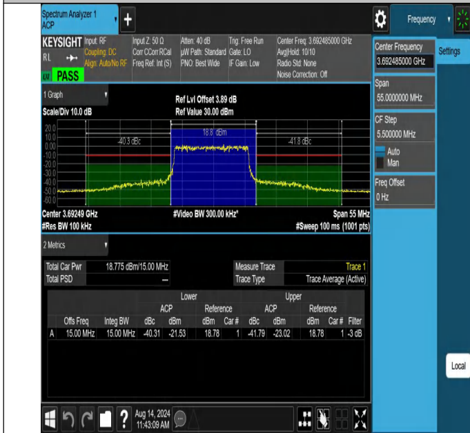
NTNV-N48-PC3-30-15-H-DFT-64QAM-Outer_Full-Ant1-PASS
