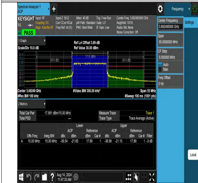
NTNV-N48-PC3-30-15-H-CP-64QAM-Outer_Full-Ant1-PASS
