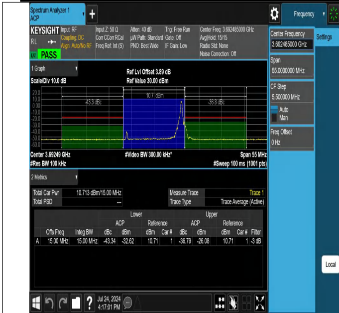
NTNV-N48-PC3-30-15-H-CP-16QAM-Edge_1RB_Right-Ant1-PAS
