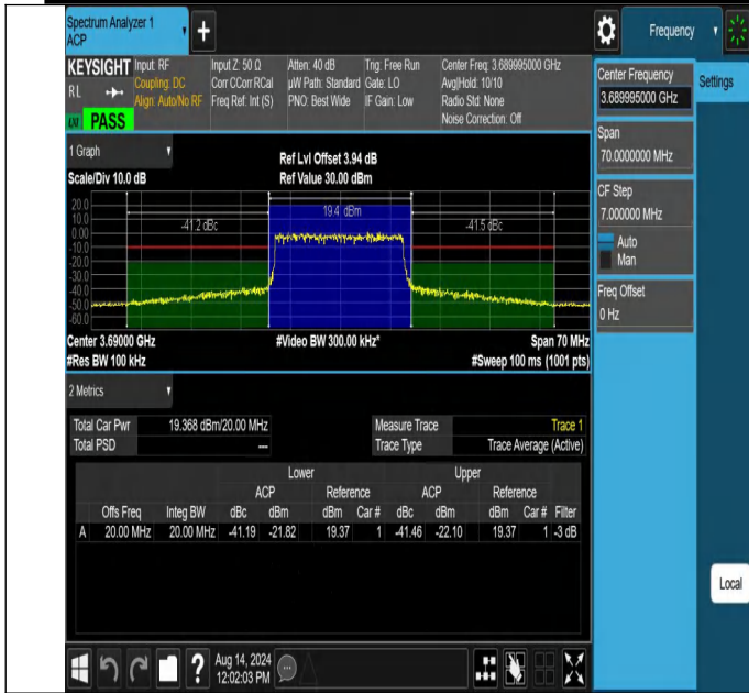
NTNV-N48-PC3-30-20-H-DFT-16QAM-Outer_Full-Ant1-PASS
