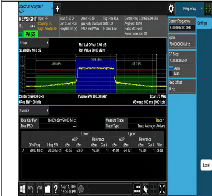
NTNV-N48-PC3-30-20-H-DFT-256QAM-Outer_Full-Ant1-PASS
