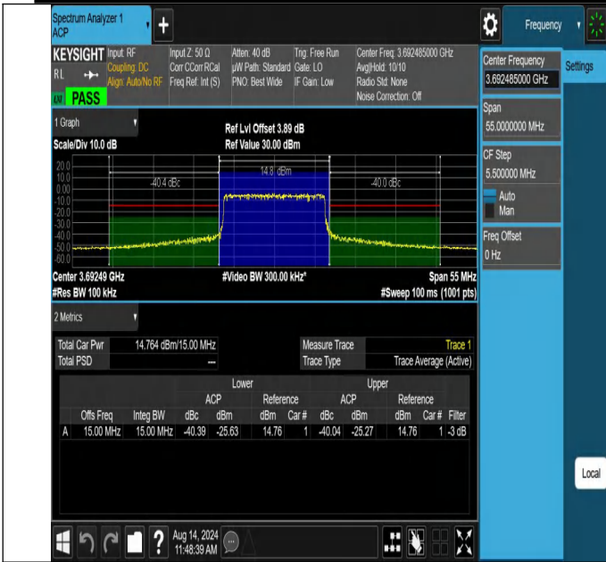
NTNV-N48-PC3-30-15-H-CP-256QAM-Outer_Full-Ant1-PASS
