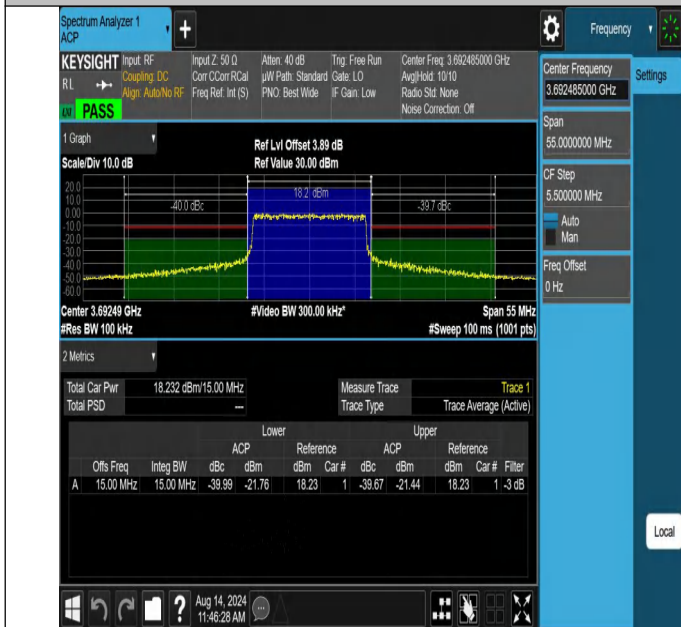
NTNV-N48-PC3-30-15-H-CP-16QAM-Outer_Full-Ant1-PASS
