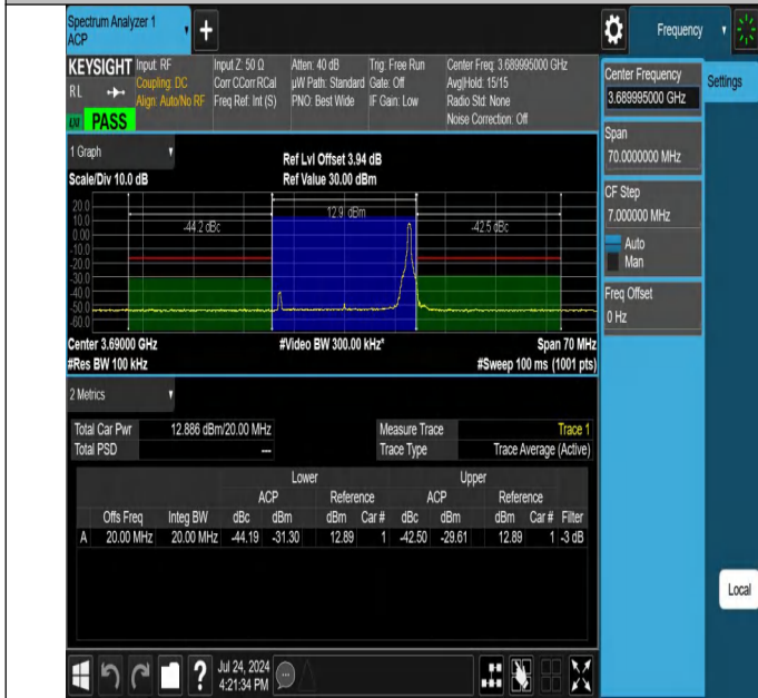
NTNV-N48-PC3-30-20-H-DFT-16QAM-Edge_1RB_Right-Ant1-PA SS
