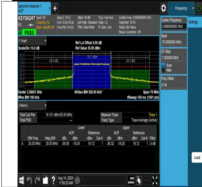
NTNV-N48-PC3-30-20-L-CP-QPSK-Outer_Full-Ant1-PASS
