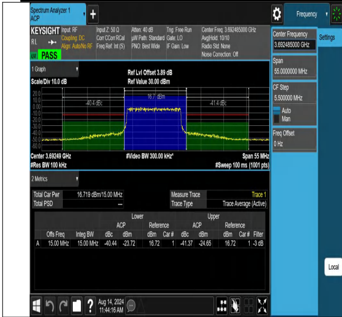
NTNV-N48-PC3-30-15-H-DFT-256QAM-Outer_Full-Ant1-PASS
