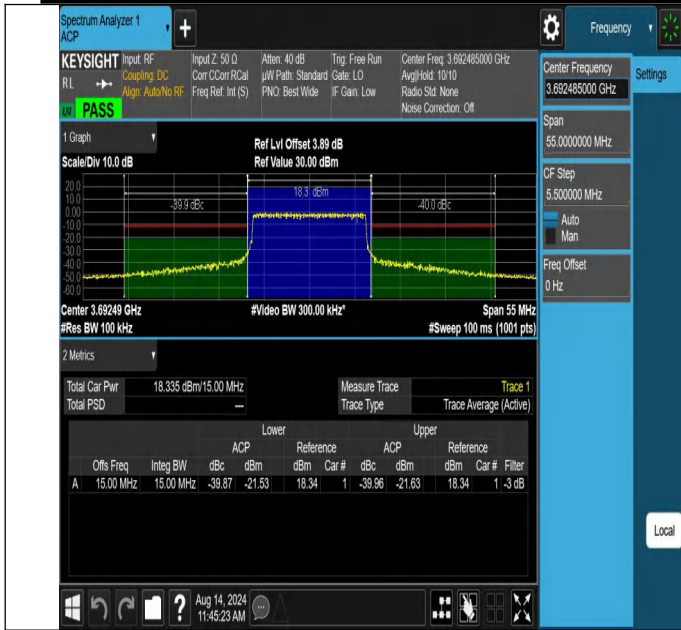
NTNV-N48-PC3-30-15-H-CP-QPSK-Outer_Full-Ant1-PASS
