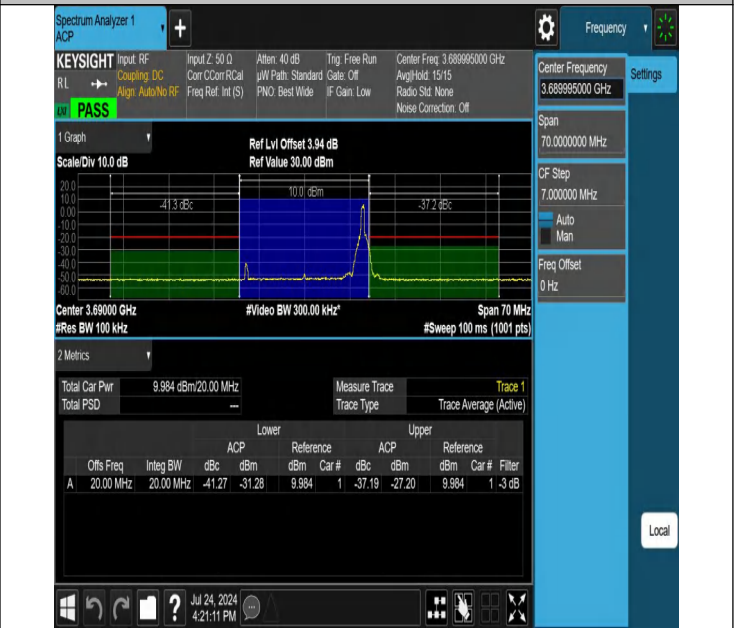
NTNV-N48-PC3-30-20-H-DFT-QPSK-Edge_1RB_Right-Ant1-PAS S
