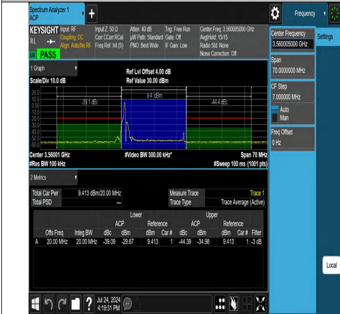
NTVN-N48-PC3-30-20-L-CP-QPSK-Edge_1RB_Left-Ant1-PASS
