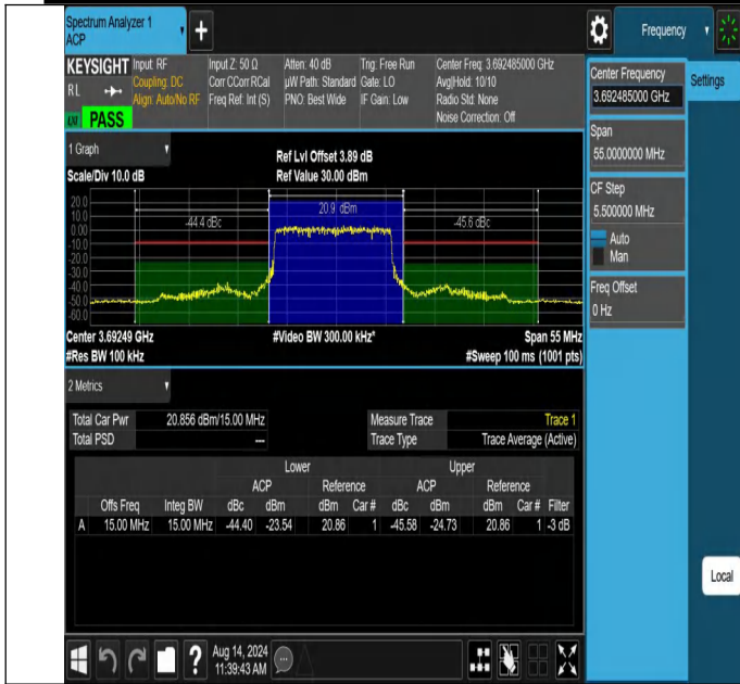
NTNV-N48-PC3-30-15-H-DFT-PI2BPSK-Outer_Full-Ant1-PASS
