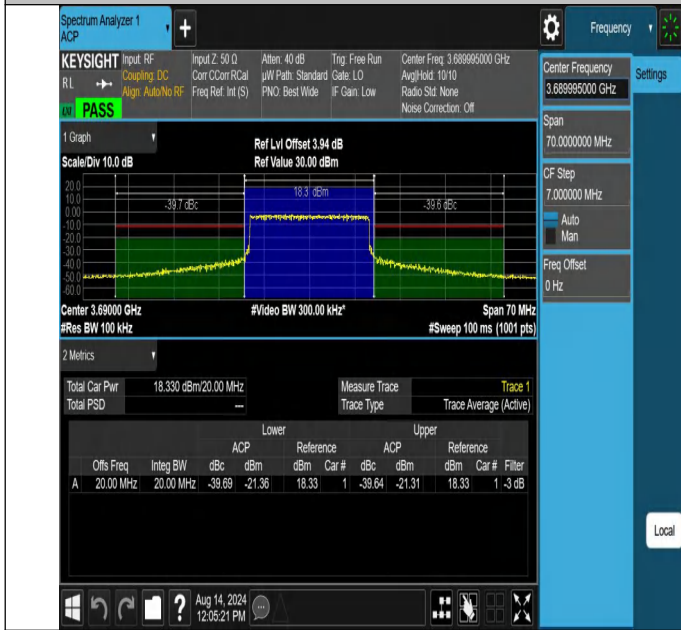
NTNV-N48-PC3-30-20-H-CP-QPSK-Outer_Full-Ant1-PASS
