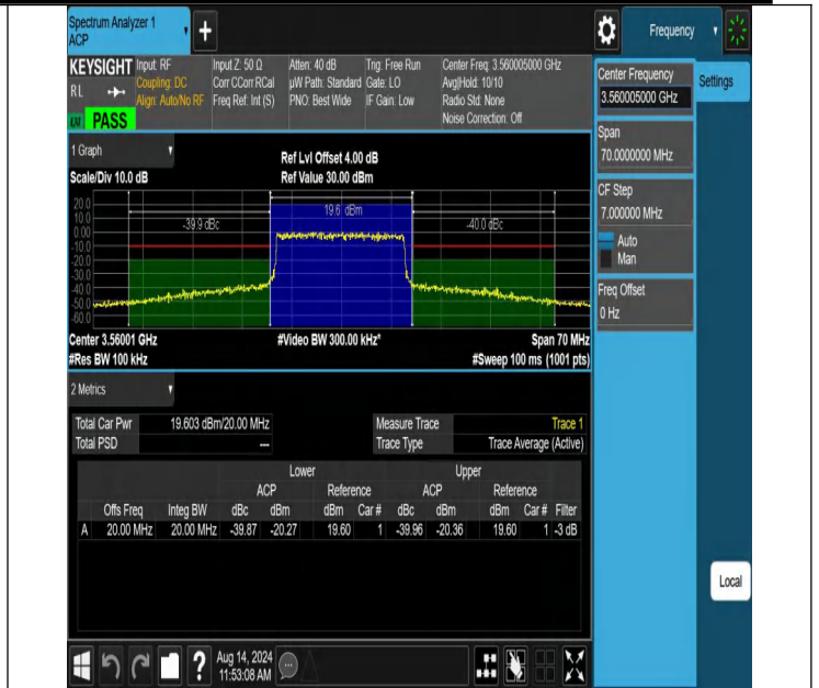
NTNV-N48-PC3-30-20-L-DFT-64QAM-Outer_Full-Ant1-PASS
