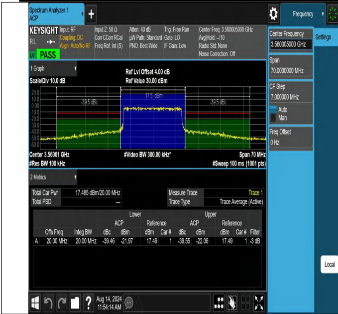
NTVN-N48-PC3-30-20-L-DFT-256QAM-Outer_Full-Ant1-PASS
