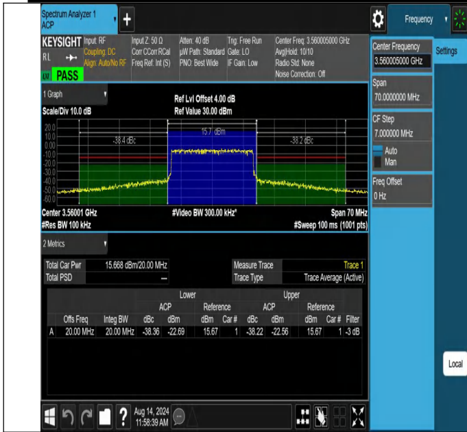
NTVN-N48-PC3-30-20-L-CP-256QAM-Outer_Full-Ant1-PASS
