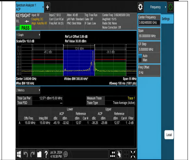
NTNV-N48-PC3-30-15-H-CP-QPSK-Edge_1RB_Right-Ant1-PASS
