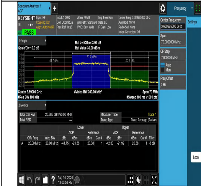
NTNV-N48-PC3-30-20-H-DFT-QPSK-Outer_Full-Ant1-PASS
