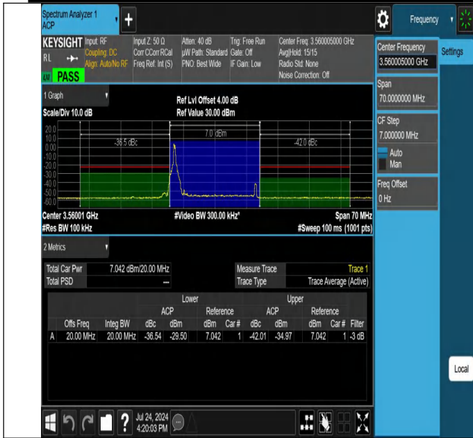
NTNV-N48-PC3-30-20-L-CP-64QAM-Edge_1RB_Left-Ant1-PASS
