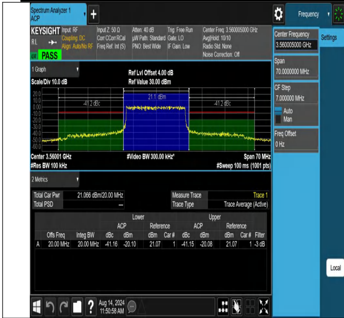
NTNV-N48-PC3-30-20-L-DFT-QPSK-Outet_Full-Ant1-PASS
