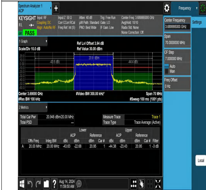
NTVN-N48-PC3-30-20-H-DFT-PI2BPSK-Outer_Full-Ant1-PASS
