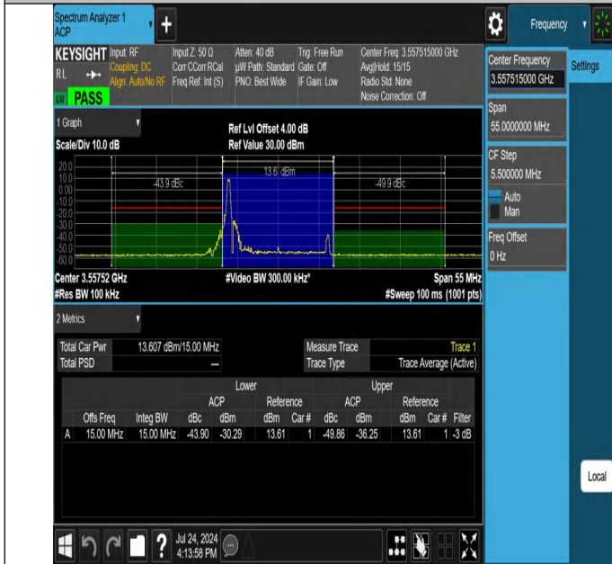
NTNV-N48-PC3-30-15-L-CP-64QAM-Edge_1RB_Left-Ant1-PASS
