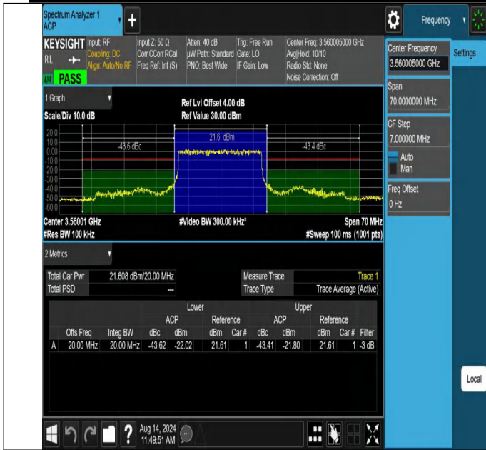
NTNV-N48-PC3-30-20-L-DFT-PI2BPSK-Outer_Full-Ant1-PASS
