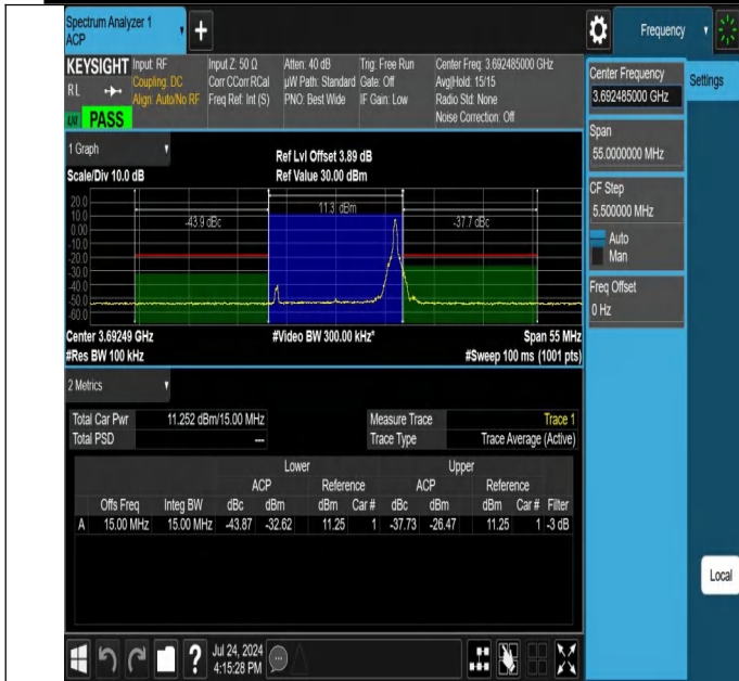
NTNV-N48-PC3-30-15-H-DFT-16QAM-Edge_1RB_Right-Ant1-PA SS
