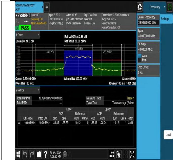
NTNV-N48-PC3-30-10-H-CP-64QAM-Outer_Full-Ant1-PASS
