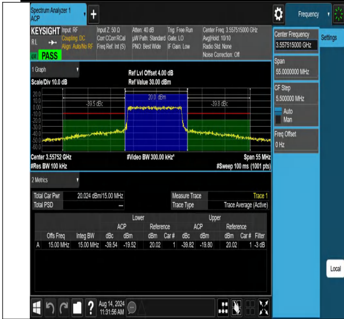
NTNV-N48-PC3-30-15-L-DFT-16QAM-Outer_Full-Ant1-PASS
