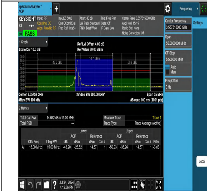
NTNV-N48-PC3-30-15-L-DFT-16QAM-Edge_1RB_Left-Ant1-PAS
