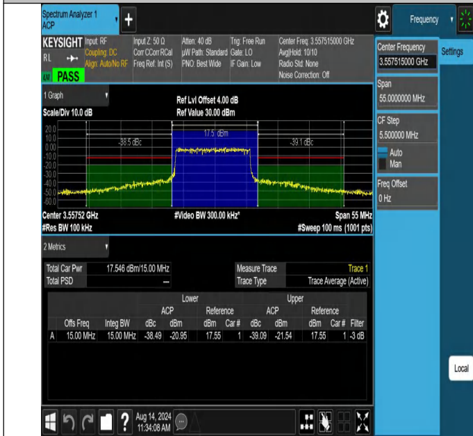
NTNV-N48-PC3-30-15-L-DFT-256QAM-Outer_Full-Ant1-PASS
