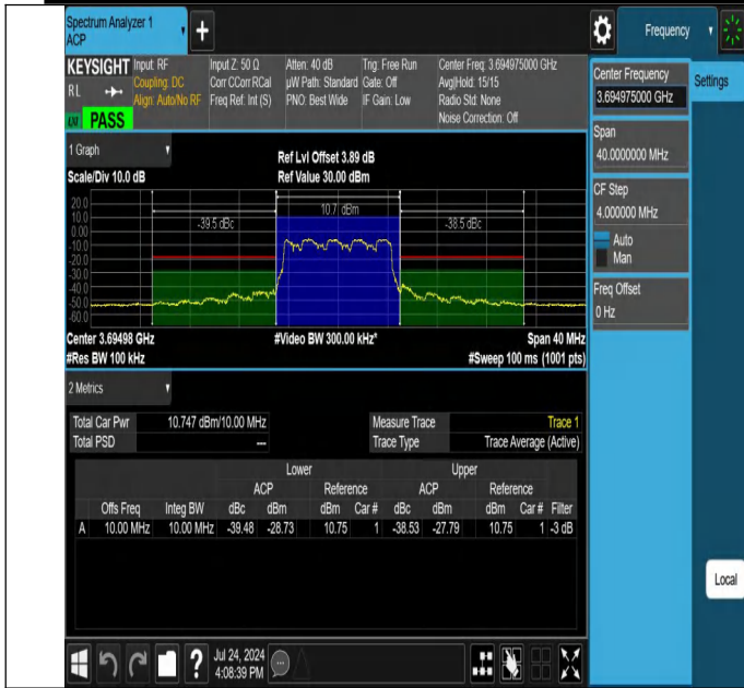
NTNV-N48-PC3-30-10-H-CP-QPSK-Outer_Full-Ant1-PASS
