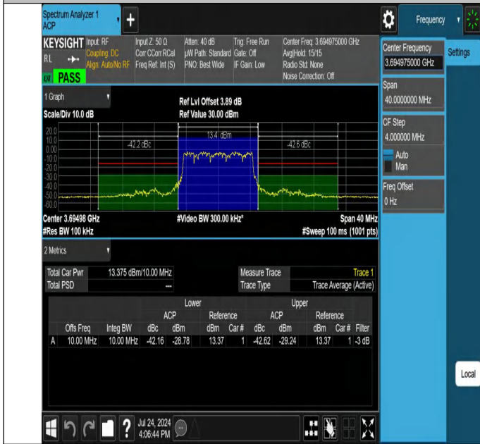
NTNV-N48-PC3-30-10-H-DFT-PI2BPSK-Outer_Full-Ant1-PASS
