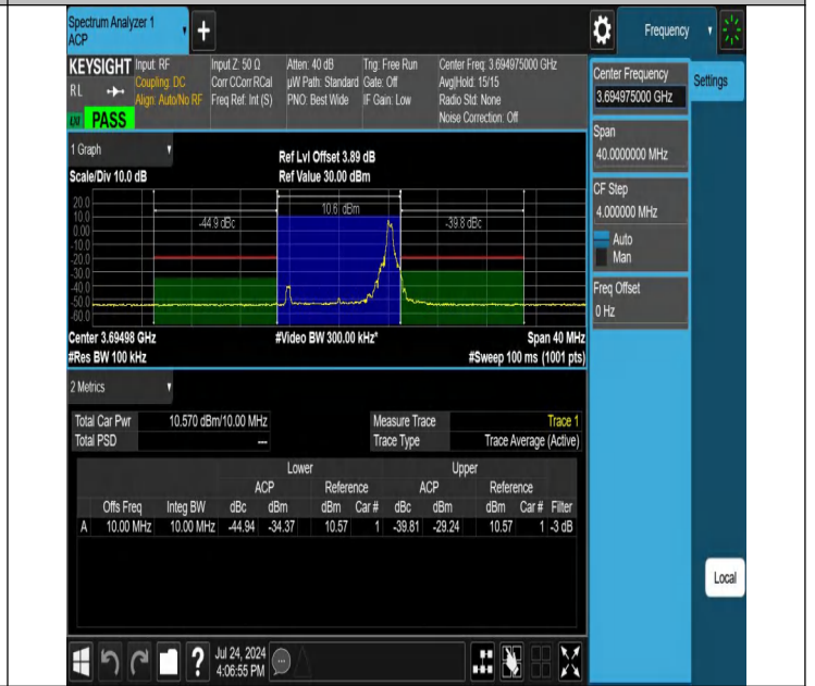
NTNV-N48-PC3-30-10-H-DFT-PI2BPSK-Edge_1RB_Right-Ant1-PASS
