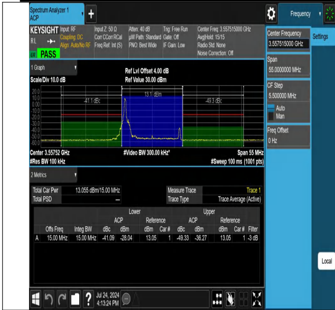
NTVN-N48-PC3-30-15-L-CP-QPSK-Edge_1RB_Left-Ant1-PASS
