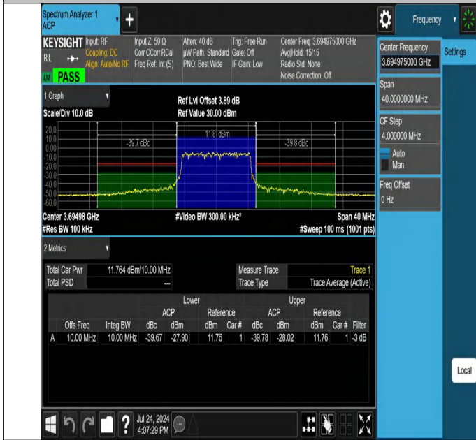
NTNV-N48-PC3-30-10-H-DFT-16QAM-Outer_Full-Ant1-PASS
