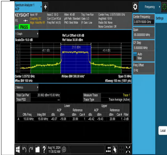
NTNV-N48-PC3-30-15-L-DFT-QPSK-Outer_Full-Ant1-PASS
