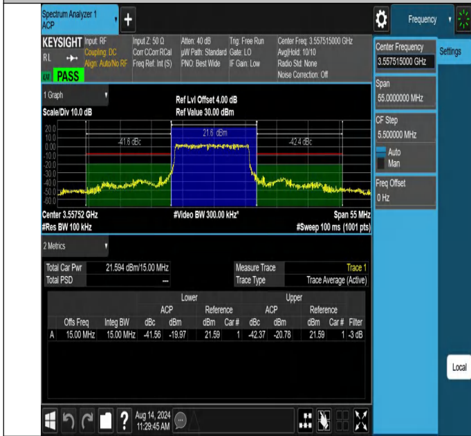
NTNV-N48-PC3-30-15-L-DFT-PI2BPSK-Outer_Full-Ant1-PASS
