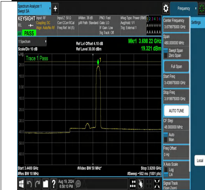
NTNV-N48-PC3-30-40-H-DFT-64QAM-Edge_1RB_Right-3439.97 5-3919.975-Ant1-PASS
