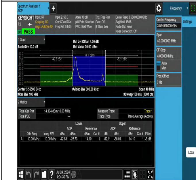
NTNV-N48-PC3-30-10-L-DFT-QPSK-Edge_1RB_Left-Ant1-PASS
