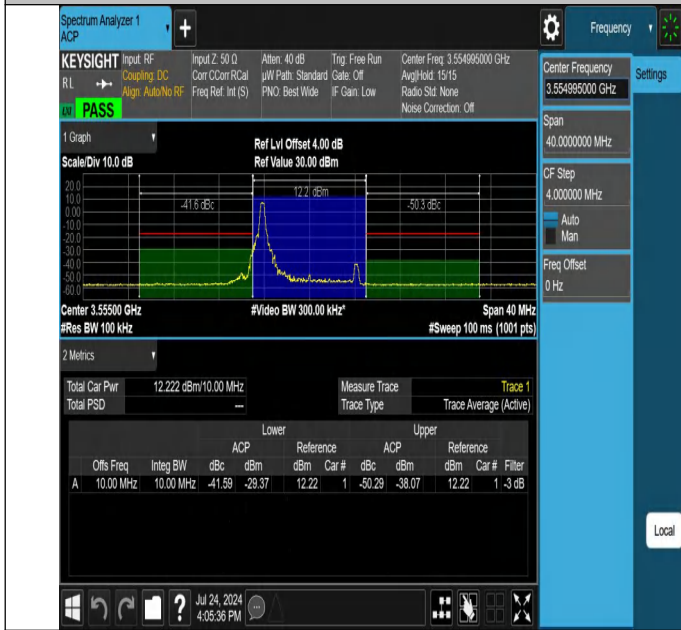
NTNV-N48-PC3-30-10-L-CP-QPSK-Edge_1RB_Left-Ant1-PASS
