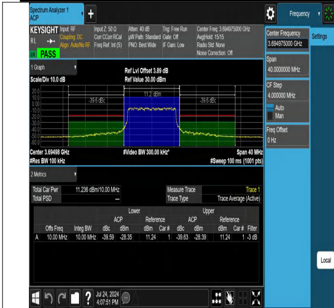
NTNV-N48-PC3-30-10-H-DFT-64QAM-Outer_Full-Ant1-PASS
