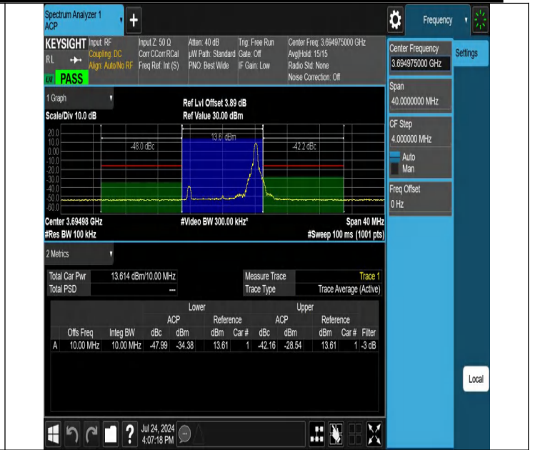
NTNV-N48-PC3-30-10-H-DFT-QPSK-Edge_1RB_Right-Ant1-PASS S
