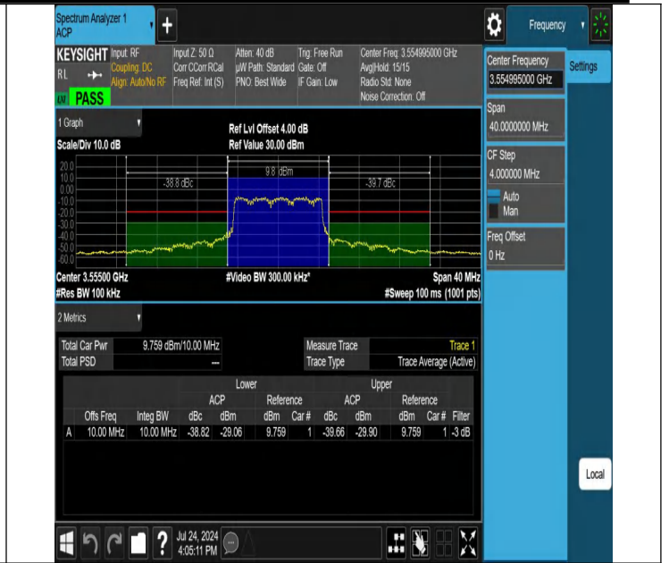
NTNV-N48-PC3-30-10-L-DFT-256QAM-Outer_Full-Ant1-PASS
