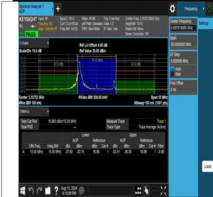
NTNV-N48-PC3-30-15-L-DFT-256QAM-Edge_1RB_Left-Ant1-PA
