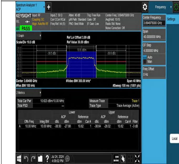
NTNV-N48-PC3-30-10-H-CP-16QAM-Outer_Full-Ant1-PASS
