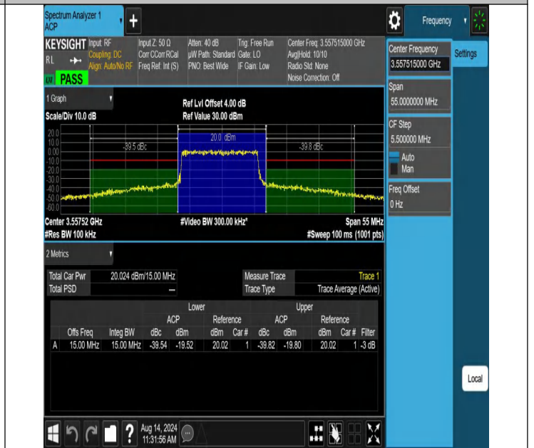
NTNV-N48-PC3-30-15-L-DFT-QPSK-Outer_Full-Ant1-PASS
