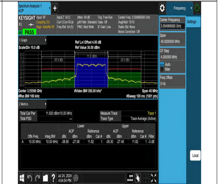
NTNV-N48-PC3-30-10-L-DFT-64QAM-Outer_Full-Ant1-PASS
