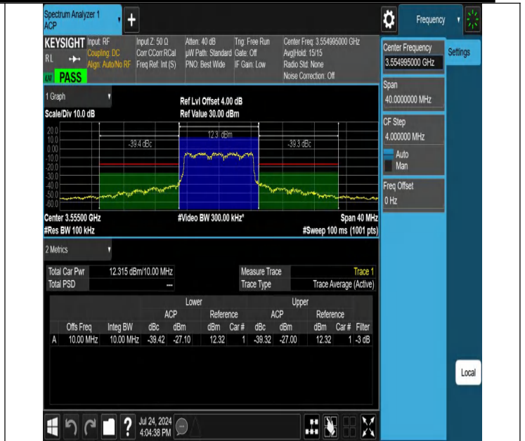
NTNV-N48-PC3-30-10-L-DFT-16QAM-Outer_Full-Ant1-PASS
