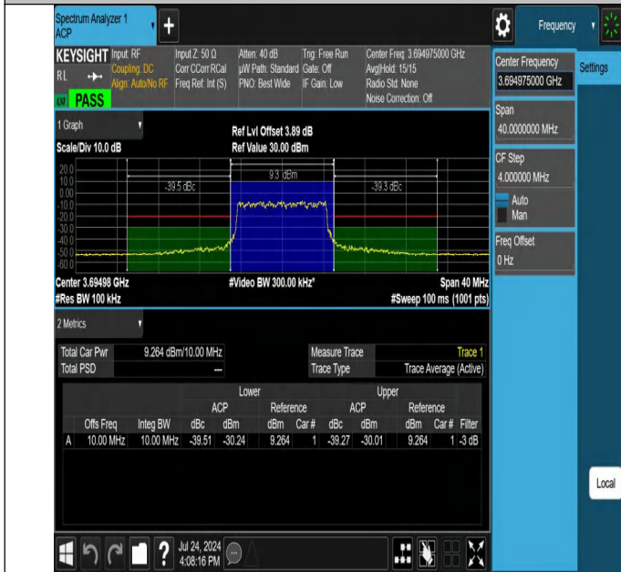
NTNV-N48-PC3-30-10-H-DFT-256QAM-Outer_Full-Ant1-PASS
