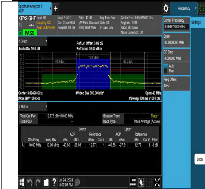
NTNV-N48-PC3-30-10-H-DFT-QPSK-Outer_Full-Ant1-PASS
