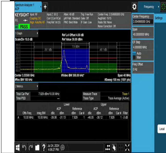
NTNV-N48-PC3-30-10-L-CP-256QAM-Edge_1RB_Left-Ant1-PAS
