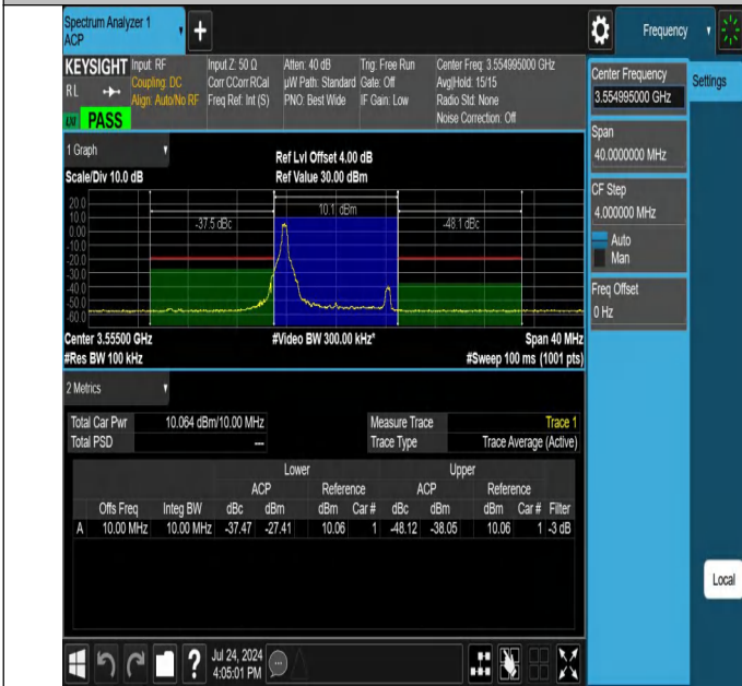
NTNV-N48-PC3-30-10-L-DFT-64QAM-Edge_1RB_Left-Ant1-PAS
