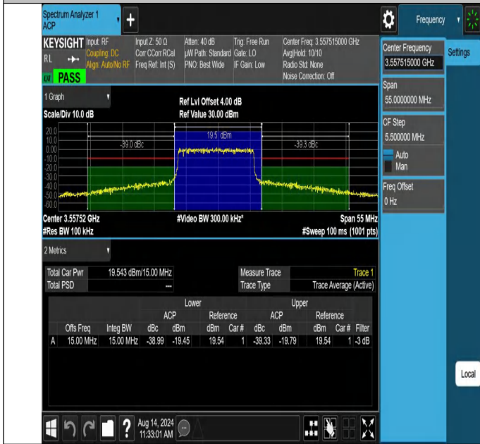
NTNV-N48-PC3-30-15-L-DFT-64QAM-Outer_Full-Ant1-PASS
