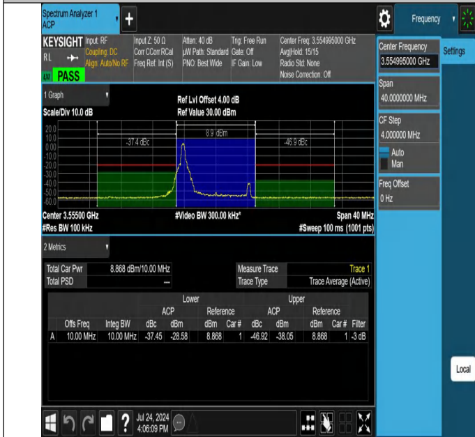
NTNV-N48-PC3-30-10-L-CP-64QAM-Edge_1RB_Left-Ant1-PASS
