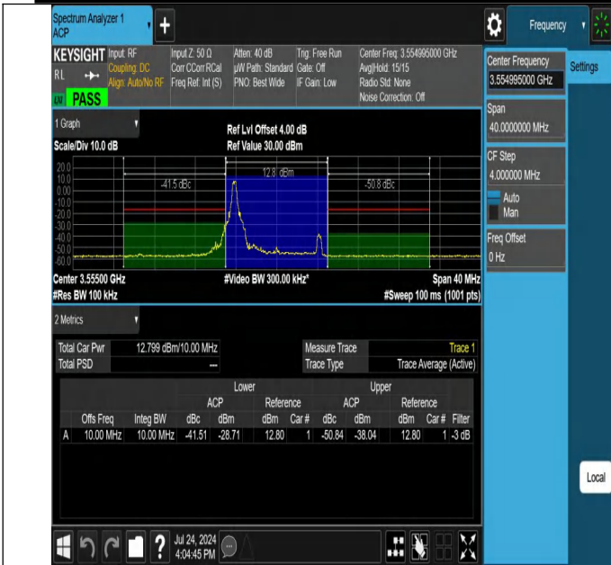
NTNV-N48-PC3-30-10-L-DFT-16QAM-Edge_1RB_Left-Ant1-PAS
