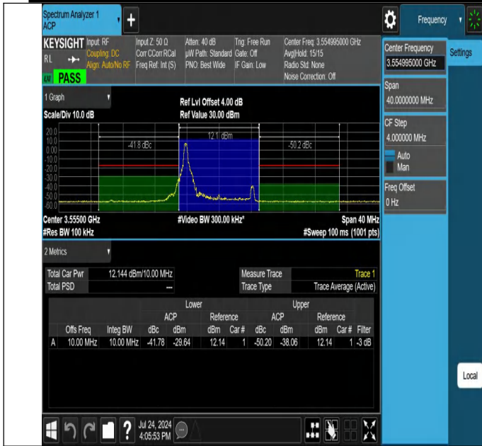
NTNV-N48-PC3-30-10-L-CP-16QAM-Edge_1RB_Left-Ant1-PASS
