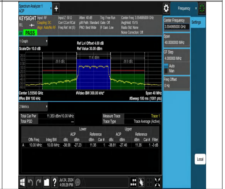
NTNV-N48-PC3-30-10-L-CP-QPSK-Outer_Full-Ant1-PASS
