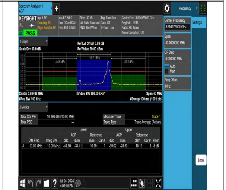
NTNV-N48-PC3-30-10-H-DFT-16QAM-Edge_1RB_Right-Ant1-PASS SS
