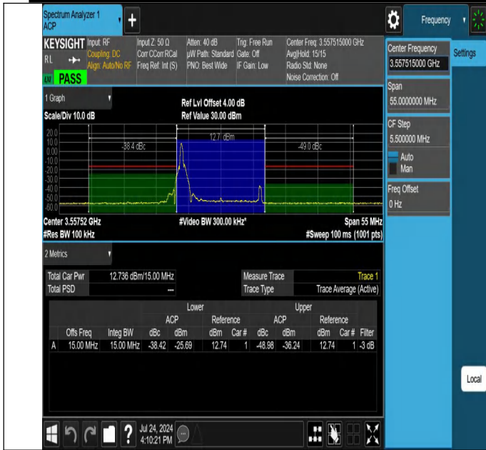
NTNV-N48-PC3-30-15-L-DFT-PI2BPSK-Edge_1RB_Left-Ant1-PA SS
