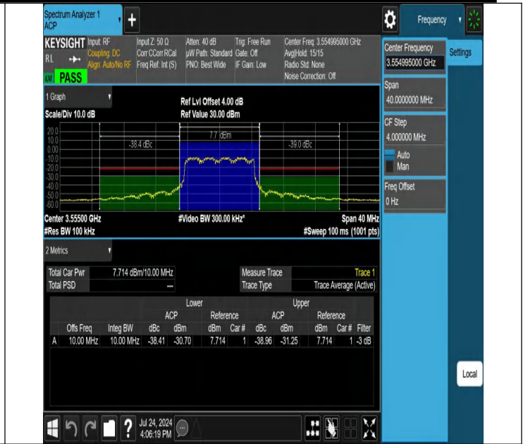
NTNV-N48-PC3-30-10-L-CP-256QAM-Outer_Full-Ant1-PASS
