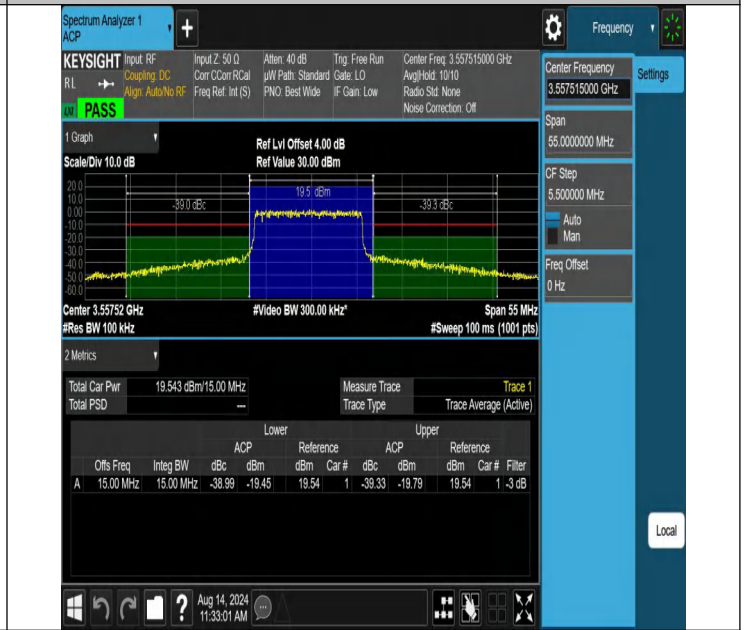
NTNV-N48-PC3-30-15-L-DFT-64QAM-Outer_Full-Ant1-PASS
