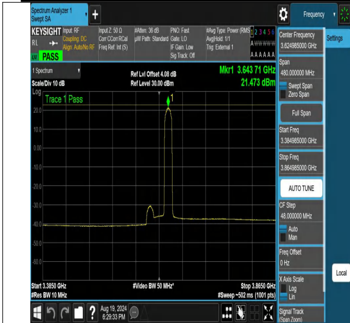
NTNV-N48-PC3-30-40-M-DFT-BPSK-Edge_1RB_Right-3384.985-3864.985-Ant1-PASS
