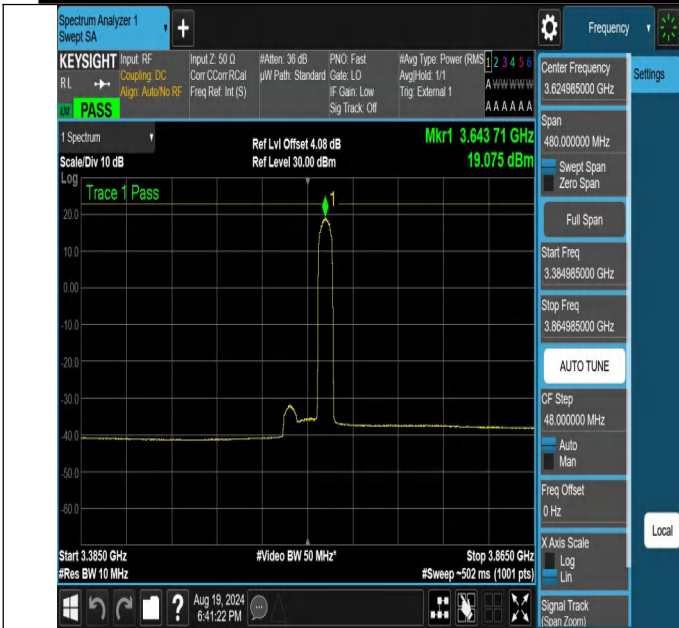
NTNV-N48-PC3-30-40-M-CP-QPSK-Edge_1RB_Right-3384.985-3864.985-Ant1-PASS
