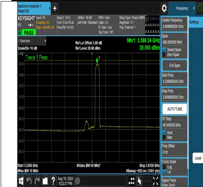
NTNV-N48-PC3-30-40-L-CP-16QAM-Edge_1RB_Right-3329.995-3809.995-Ant1-PASS
