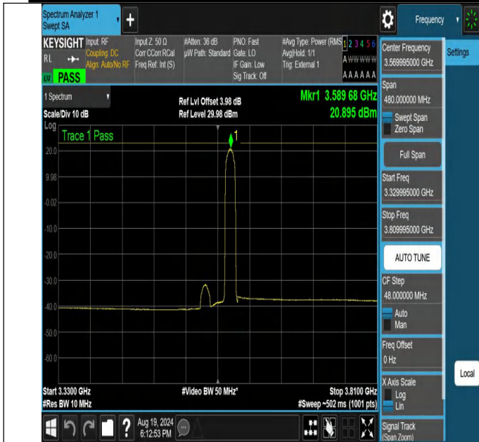
NTNV-N48-PC3-30-40-L-DFT-16QAM-Edge_1RB_Right-3329.995-3809.995-Ant1-PASS
