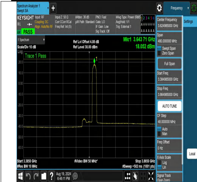
NTNV-N48-PC3-30-40-M-CP-64QAM-Edge_1RB_Right-3384.985-3864.985-Ant1-PASS
