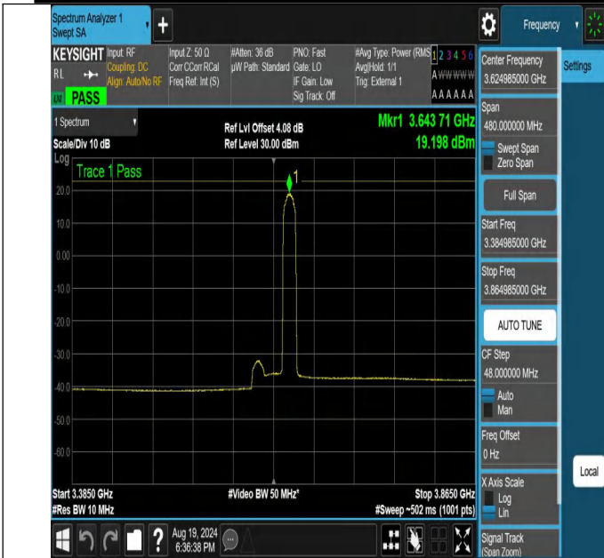
NTNV-N48-PC3-30-40-M-DFT-64QAM-Edge_1RB_Right-3384.98 5-3864.985-Ant1-PASS
