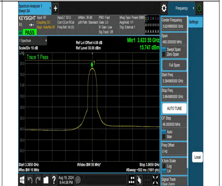
NTNV-N48-PC3-30-40-M-CP-64QAM-Inner_Full-3384.985-3864.985-Ant1-PASS
