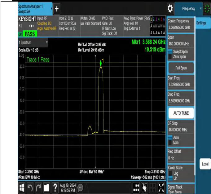
NTNV-N48-PC3-30-40-L-CP-QPSK-Edge_1RB_Right-3329.995-3 809.995-Ant1-PASS
