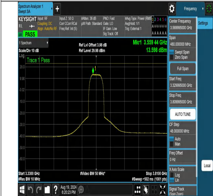
NTNV-N48-PC3-30-40-L-CP-16QAM-Outer_Full-3329.995-3809.9 95-Ant1-PASS
