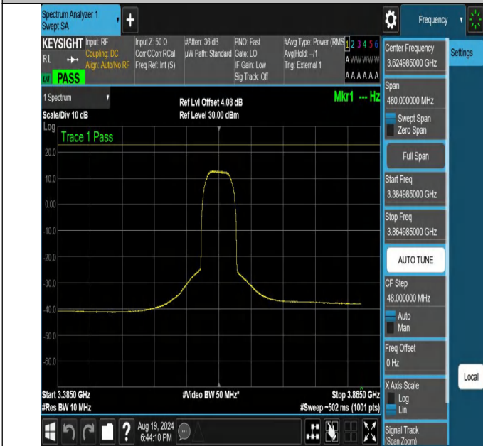
NTNV-N48-PC3-30-40-M-CP-64QAM-Outer_Full-3384.985-3864.985-Ant1-PASS
