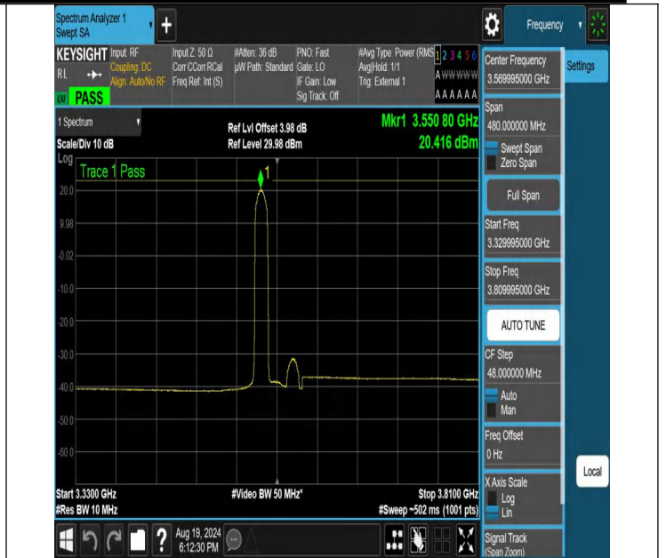
NTNV-N48-PC3-30-40-L-DFT-16QAM-Edge_1RB_Left-3329.995-3809.995-Ant1-PASS
