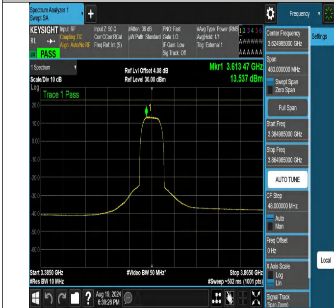
NTNV-N48-PC3-30-40-M-CP-QPSK-Outer_Full-3384.985-3864.9-85-Ant1-PASS
