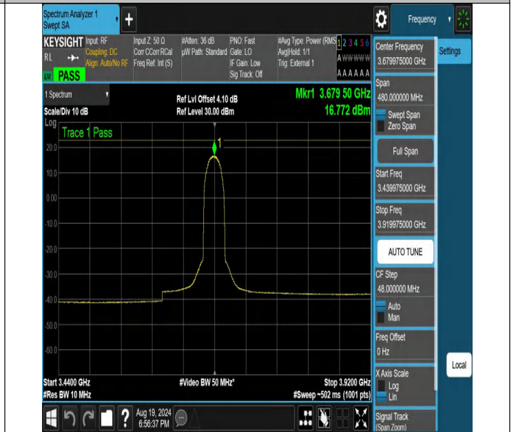
NTNV-N48-PC3-30-40-H-DFT-64QAM-Inner_Full-3439.975-3919.975-Ant1-PASS
