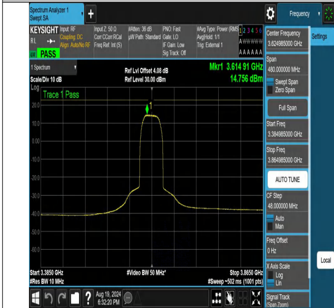
NTNV-N48-PC3-30-40-M-DFT-16QAM-Outer_Full-3384.985-3864.985-Ant1-PASS
