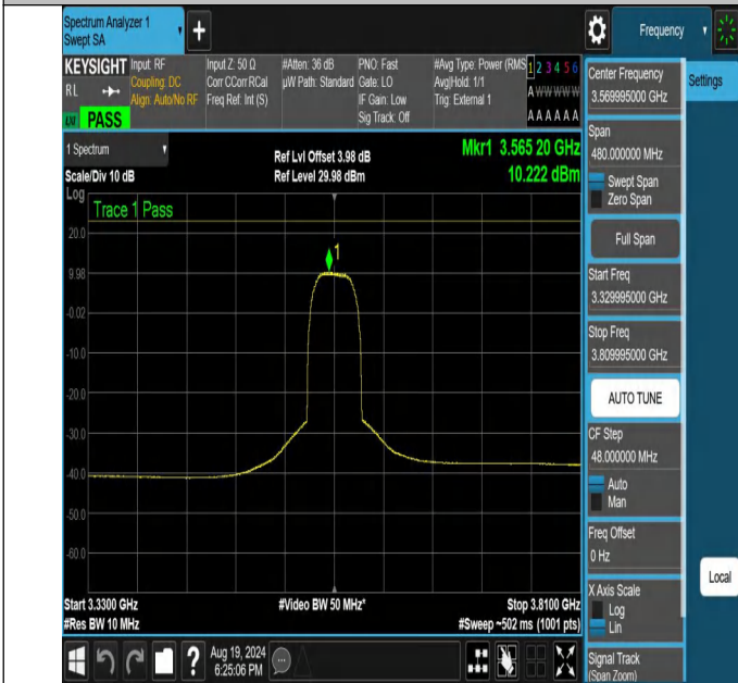
NTNV-N48-PC3-30-40-L-CP-256QAM-Outer_Full-3329.995-3809.995-Ant1-PASS
