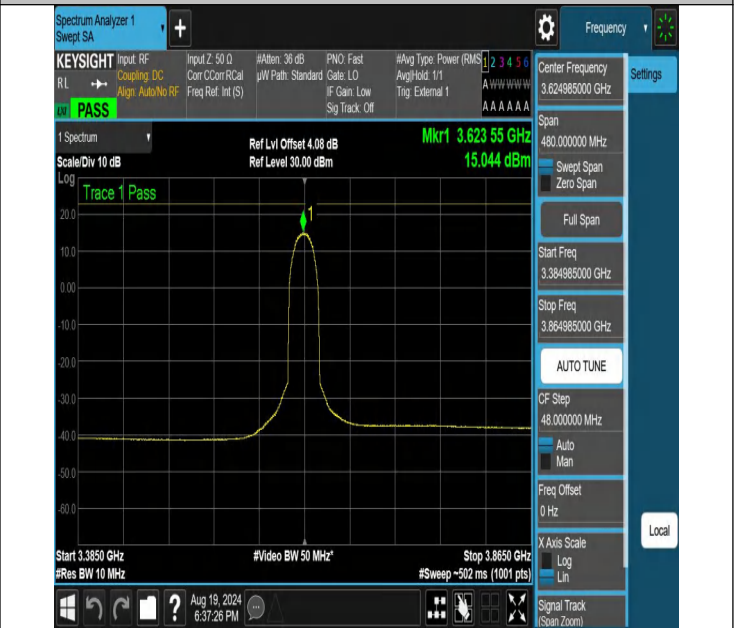
NTNV-N48-PC3-30-40-M-DFT-256QAM-Inner_Full-3384.985-386 4.985-Ant1-PASS
