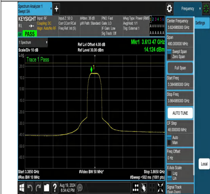
NTNV-N48-PC3-30-40-M-DFT-64QAM-Outer_Full-3384.985-3864.985-Ant1-PASS
