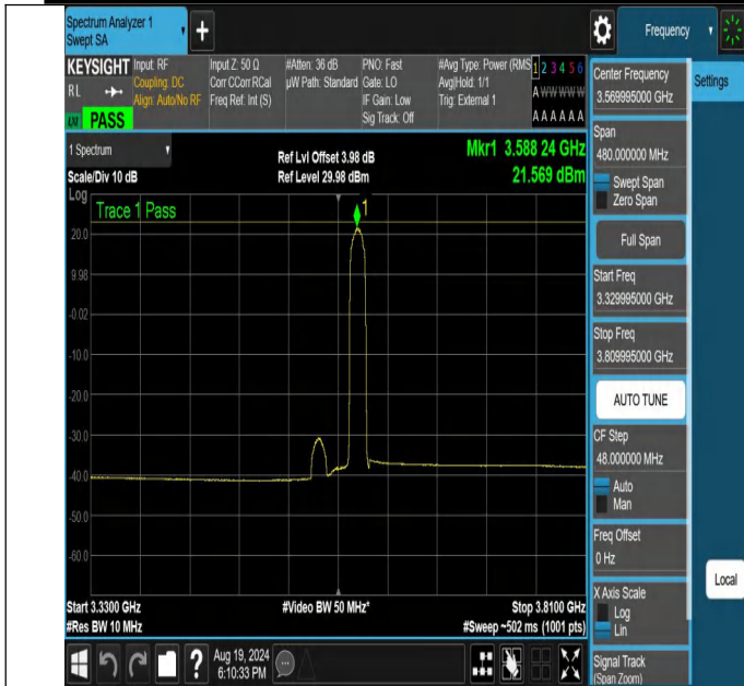
NTNV-N48-PC3-30-40-L-DFT-QPSK-Edge_1RB_Right-3329.995-3809.995-Ant1-PASS
