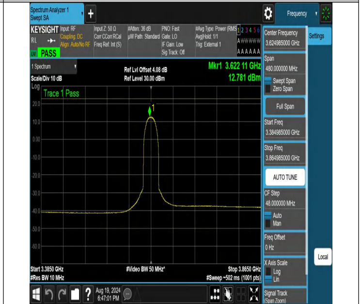
NTNV-N48-PC3-30-40-M-CP-256QAM-Inner_Full-3384.985-3864.985-Ant1-PASS
