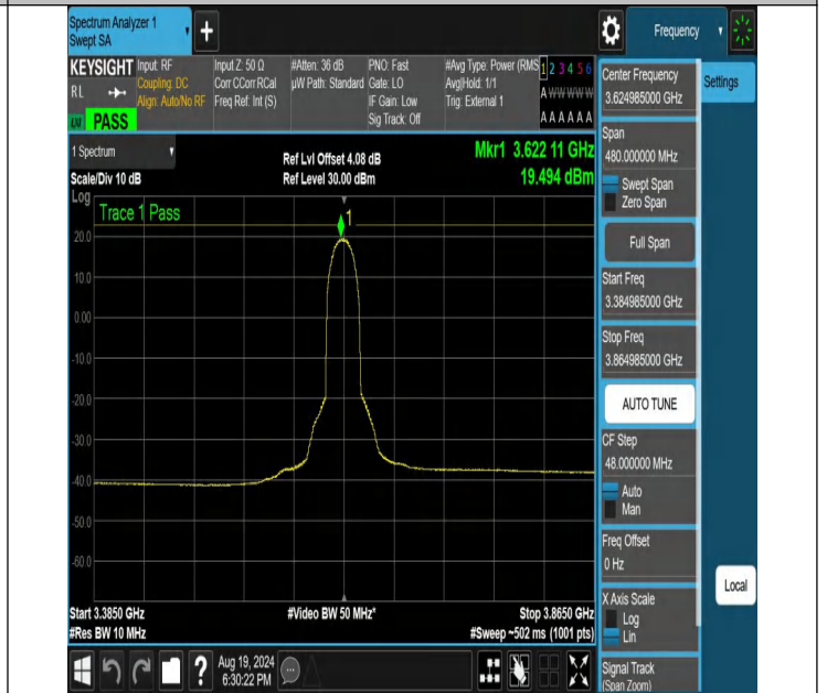
NTNV-N48-PC3-30-40-M-DFT-QPSK-Inner_Full-3384.985-3864.985-Ant1-PASS
