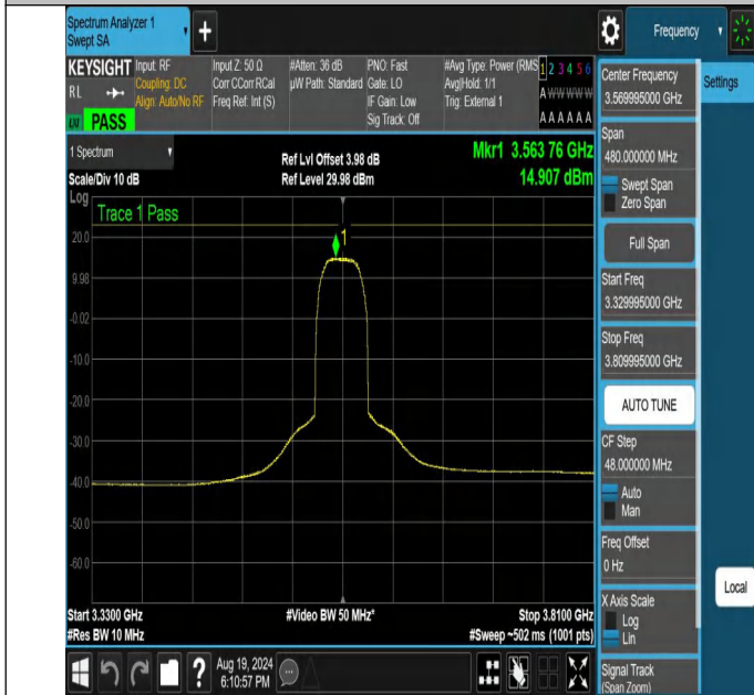
NTNV-N48-PC3-30-40-L-DFT-16QAM-Outer_Full-3329.995-3809.995-Ant1-PASS
