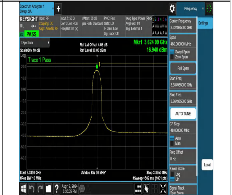
NTNV-N48-PC3-30-40-M-DFT-64QAM-Inner_Full-3384.985-3864.985-Ant1-PASS
