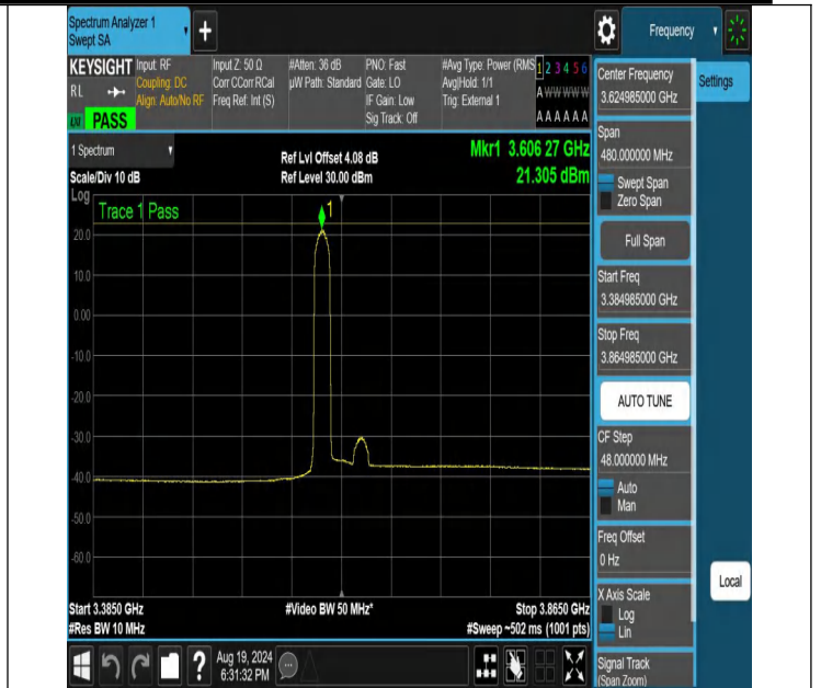
NTNV-N48-PC3-30-40-M-DFT-QPSK-Edge_1RB_Left-3384.985-3864.985-Ant1-PASS
