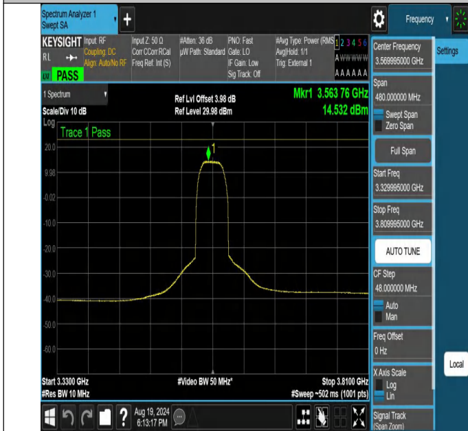
NTNV-N48-PC3-30-40-L-DFT-64QAM-Outer_Full-3329.995-3809.995-Ant1-PASS
