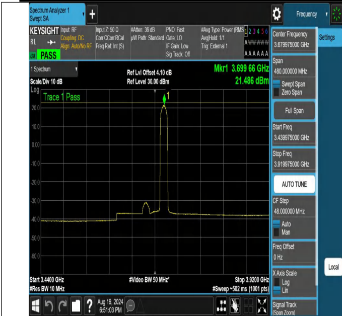
NTNV-N48-PC3-30-40-H-DFT-BPSK-Edge_1RB_Right-3439.975-3919.975-Ant1-PASS
