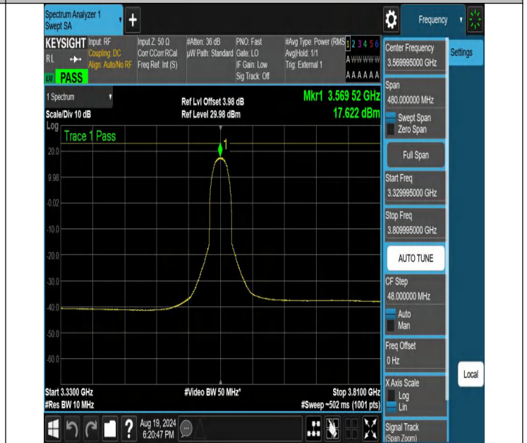
NTNV-N48-PC3-30-40-L-CP-16QAM-Inner_Full-3329.995-3809.9 95-Ant1-PASS
