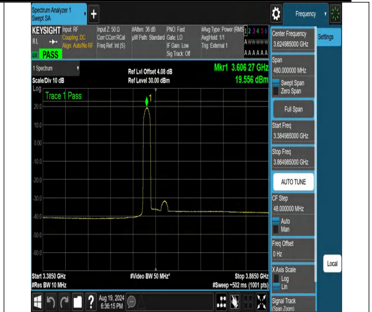
NTNV-N48-PC3-30-40-M-DFT-64QAM-Edge_1RB_Left-3384.985-3864.985-Ant1-PASS
