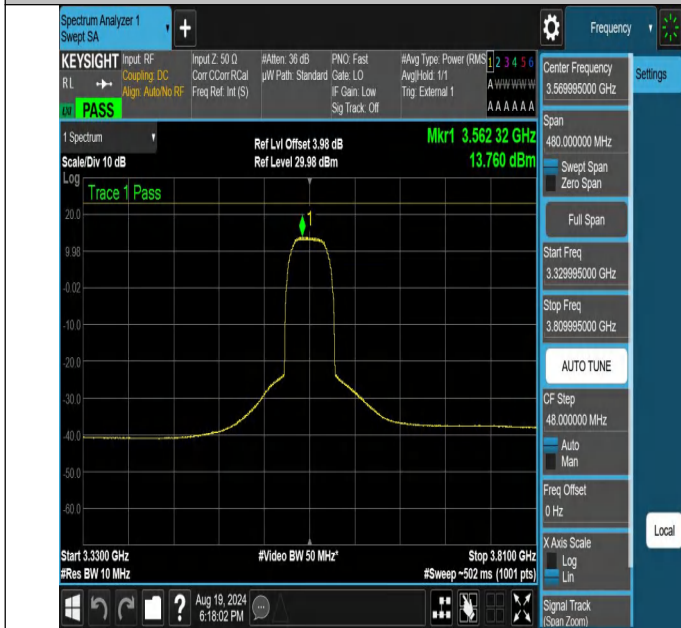
NTNV-N48-PC3-30-40-L-CP-QPSK-Outer_Full-3329.995-3809.995-Ant1-PASS
