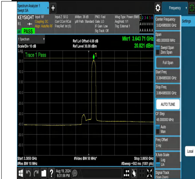
NTNV-N48-PC3-30-40-M-DFT-QPSK-Edge_1RB_Right-3384.985-3864.985-Ant1-PASS
