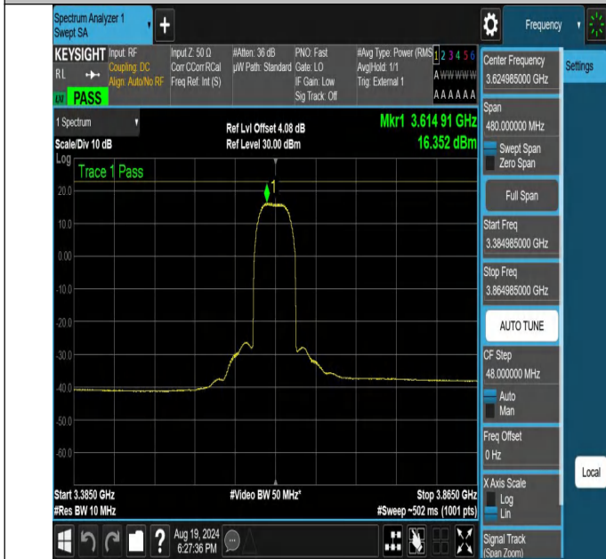
NTNV-N48-PC3-30-40-M-DFT-BPSK-Outer_Full-3384.985-3864.985-Ant1-PASS
