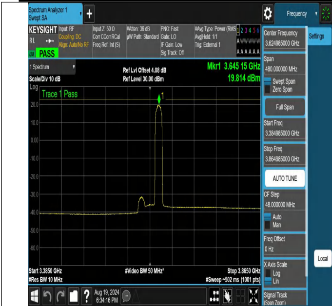
NTNV-N48-PC3-30-40-M-DFT-16QAM-Edge_1RB_Right-3384.985-3864.985-Ant1-PASS
