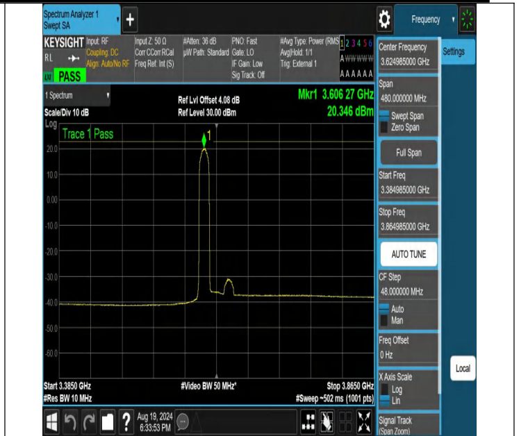
NTNV-N48-PC3-30-40-M-DFT-16QAM-Edge_1RB_Left-3384.985-3864.985-Ant1-PASS
