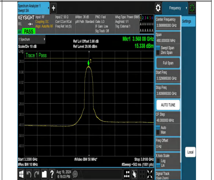
NTNV-N48-PC3-30-40-L-DFT-256QAM-Inner_Full-3329.995-3809.995-Ant1-PASS
