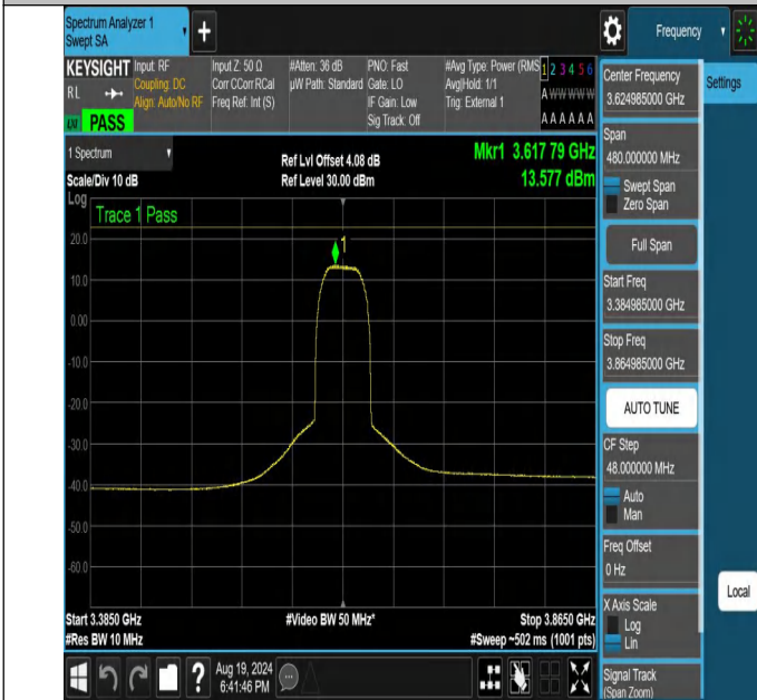
NTNV-N48-PC3-30-40-M-CP-16QAM-Outer_Full-3384.985-3864.985-Ant1-PASS
