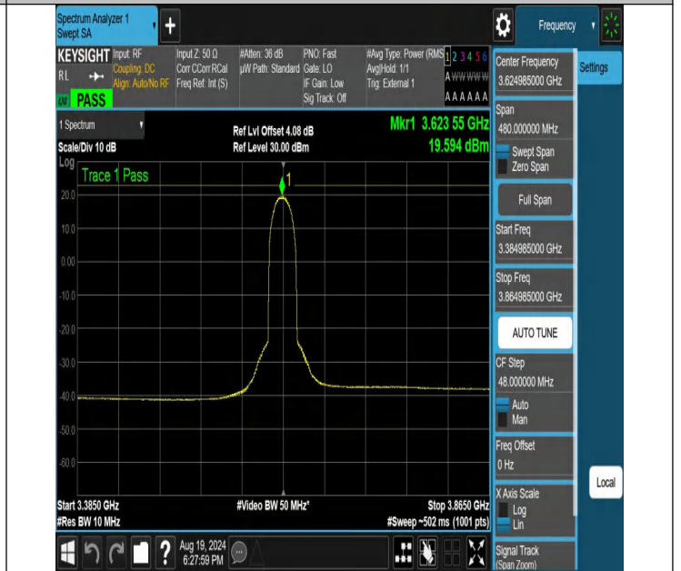
NTNV-N48-PC3-30-40-M-DFT-BPSK-Inner_Full-3384.985-3864.985-Ant1-PASS
