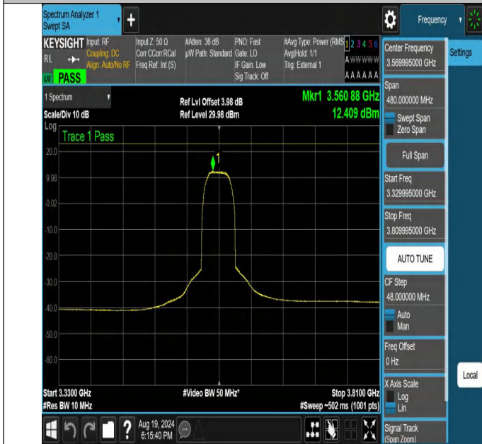
NTNV-N48-PC3-30-40-L-DFT-256QAM-Outer_Full-3329.995-3809.995-Ant1-PASS
