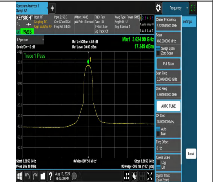
NTNV-N48-PC3-30-40-M-CP-16QAM-Inner_Full-3384.985-3864.985-Ant1-PASS
