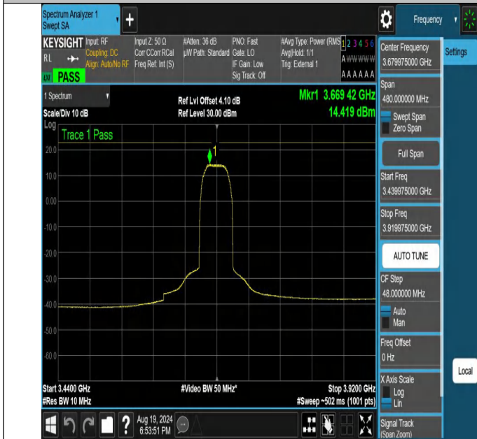
NTNV-N48-PC3-30-40-H-DFT-16QAM-Outer_Full-3439.975-3919.975-Ant1-PASS
