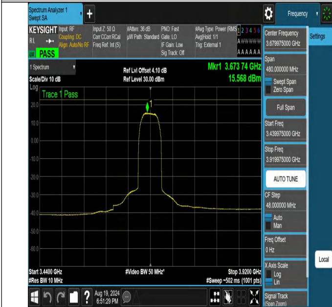
NTNV-N48-PC3-30-40-H-DFT-QPSK-Outer_Full-3439.975-3919.975-75-Ant1-PASS
