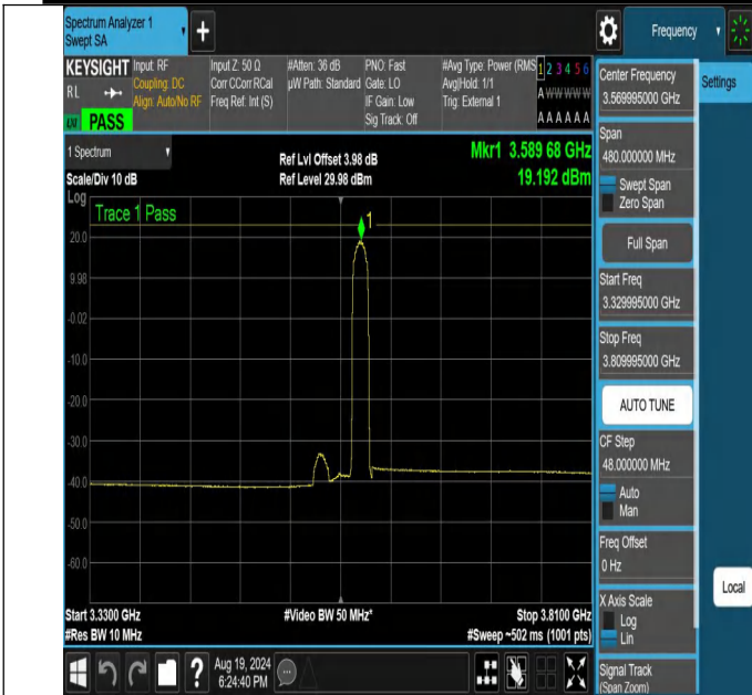
NTNV-N48-PC3-30-40-L-CP-64QAM-Edge_1RB_Right-3329.995-3809.995-Ant1-PASS
