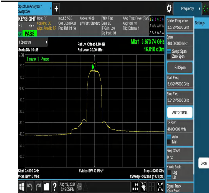
NTNV-N48-PC3-30-40-H-DFT-BPSK-Outer_Full-3439.975-3919.9 75-Ant1-PASS
