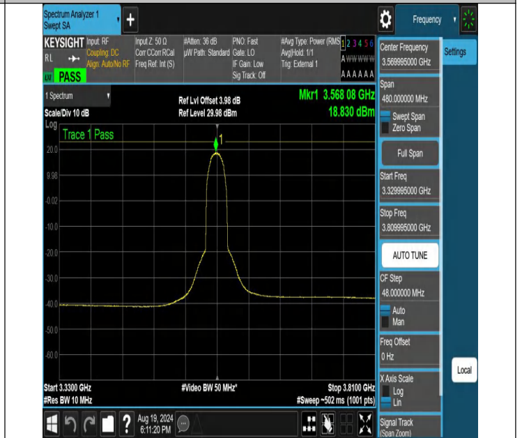
NTNV-N48-PC3-30-40-L-DFT-16QAM-Inner_Full-3329.995-3809.995-Ant1-PASS
