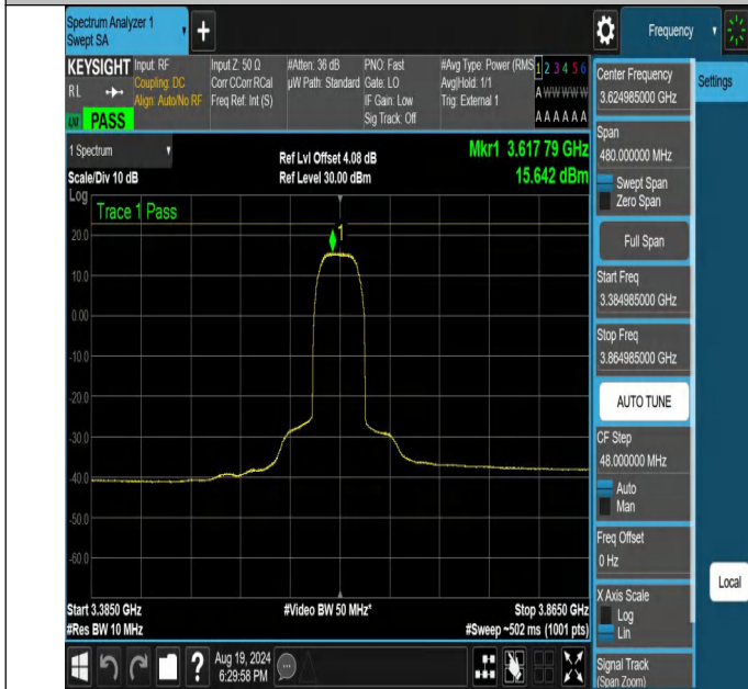
NTNV-N48-PC3-30-40-M-DFT-QPSK-Outer_Full-3384.985-3864.985-Ant1-PASS
