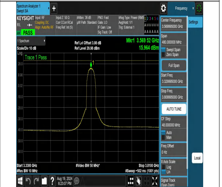
NTNV-N48-PC3-30-40-L-CP-64QAM-Inner_Full-3329.995-3809.995-Ant1-PASS
