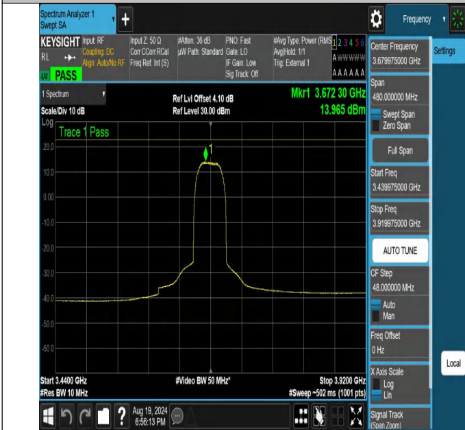
NTNV-N48-PC3-30-40-H-DFT-64QAM-Outer_Full-3439.975-3919.975-Ant1-PASS
