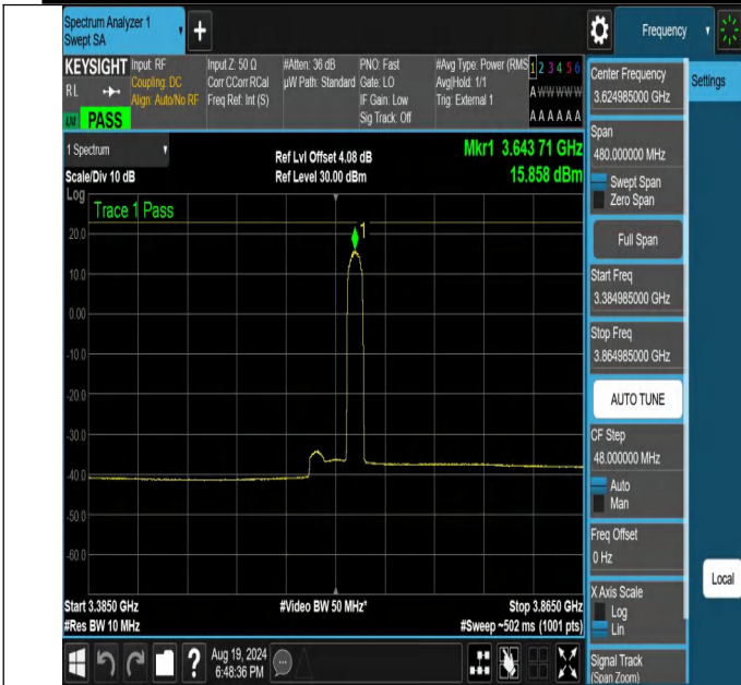
NTNV-N48-PC3-30-40-M-CP-256QAM-Edge_1RB_Right-3384.98 5-3864.985-Ant1-PASS
