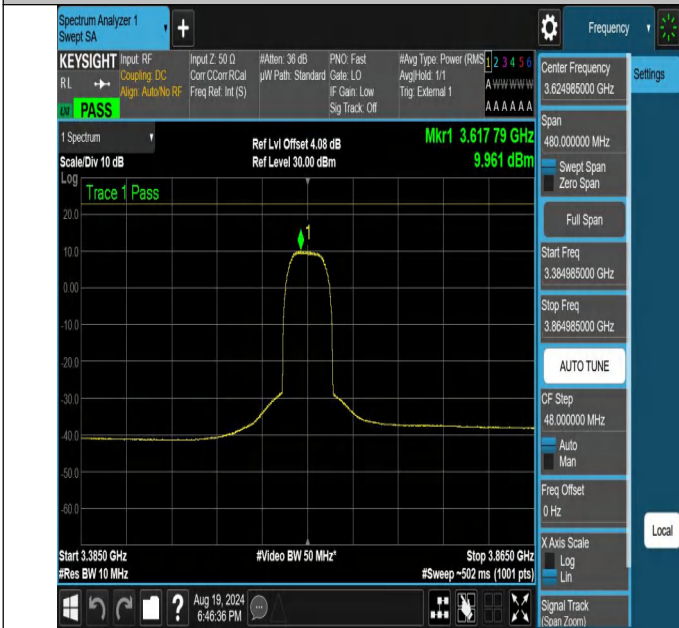
NTNV-N48-PC3-30-40-M-CP-256QAM-Outer_Full-3384.985-3864.985-Ant1-PASS
