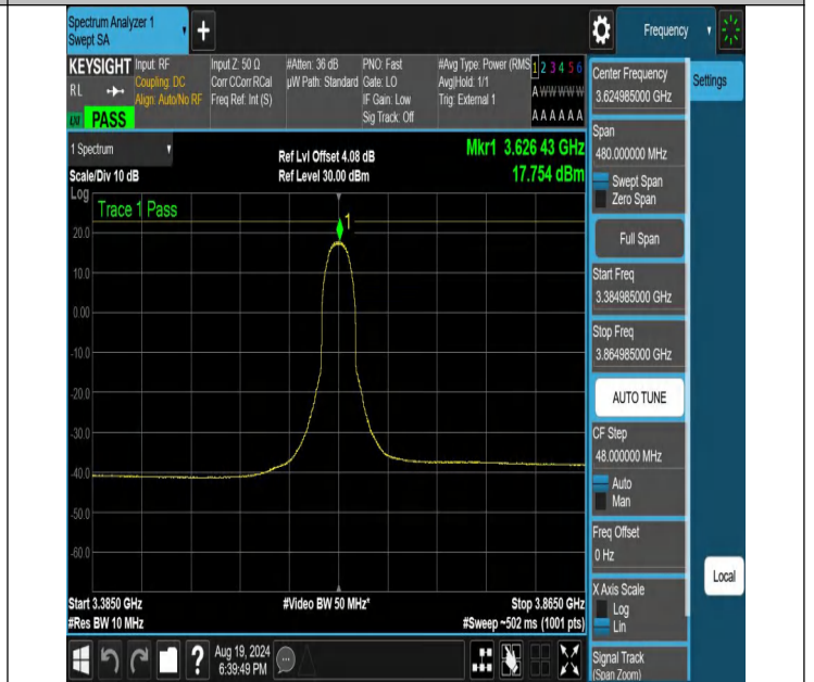
NTNV-N48-PC3-30-40-M-CP-QPSK-Inner_Full-3384.985-3864.98-5-Ant1-PASS
