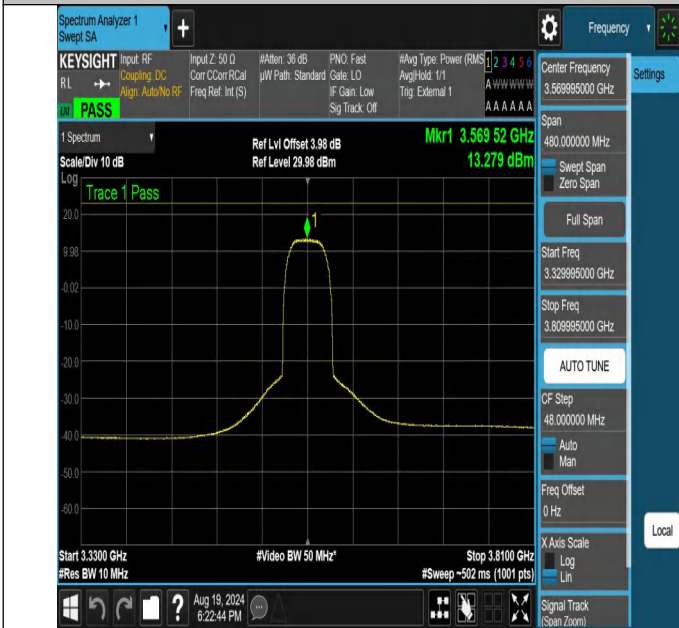
NTNV-N48-PC3-30-40-L-CP-64QAM-Outer_Full-3329.995-3809.995-Ant1-PASS
