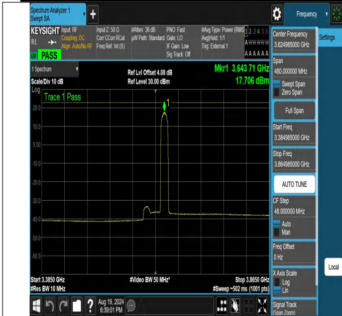
NTNV-N48-PC3-30-40-M-DFT-256QAM-Edge_1RB_Right-3384.9-85-3864.985-Ant1-PASS
