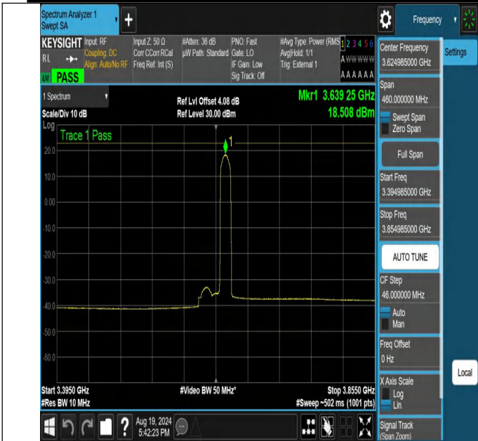
NTNV-N48-PC3-30-30-M-CP-64QAM-Edge_1RB_Right-3394.985-3854.985-Ant1-PASS
