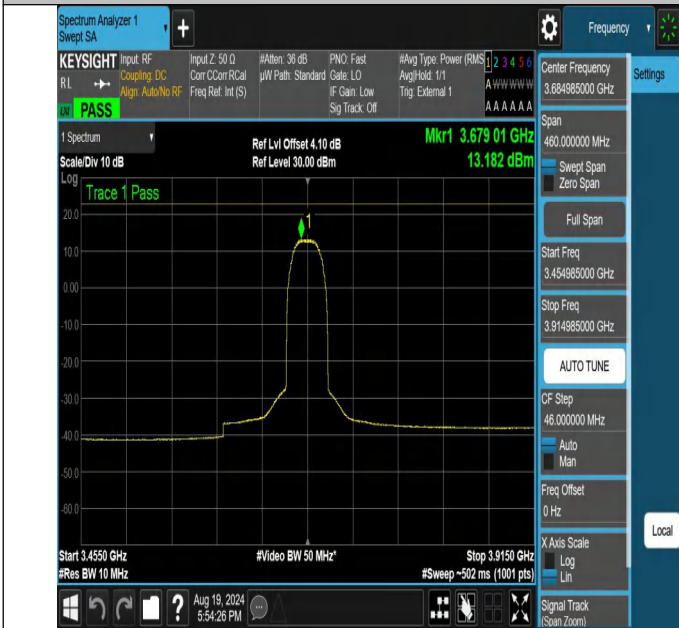
NTNV-N48-PC3-30-30-H-DFT-256QAM-Outer_Full-3454.985-391 4.985-Ant1-PASS
