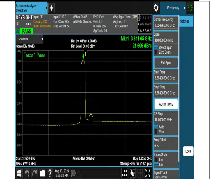
NTNV-N48-PC3-30-30-M-DFT-BPSK-Edge_1RB_Left-3394.985-3 854.985-Ant1-PASS
