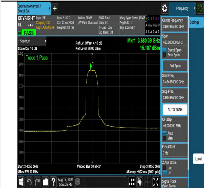
NTNV-N48-PC3-30-30-H-DFT-64QAM-Outer_Full-3454.985-3914.985-Ant1-PASS
