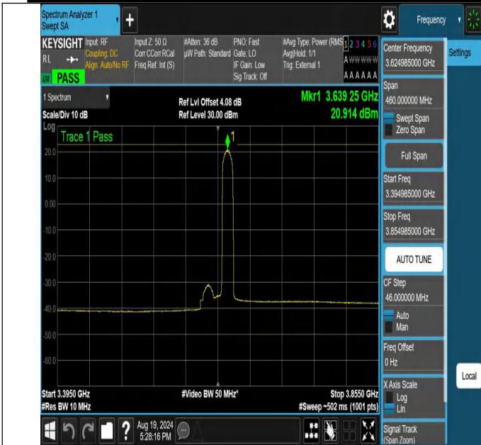
NTNV-N48-PC3-30-30-M-DFT-QPSK-Edge_1RB_Right-3394.985-3854.985-Ant1-PASS
