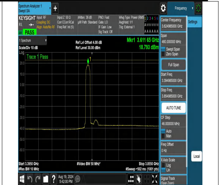
NTNV-N48-PC3-30-30-M-CP-64QAM-Edge_1RB_Left-3394.985-3854.985-Ant1-PASS
