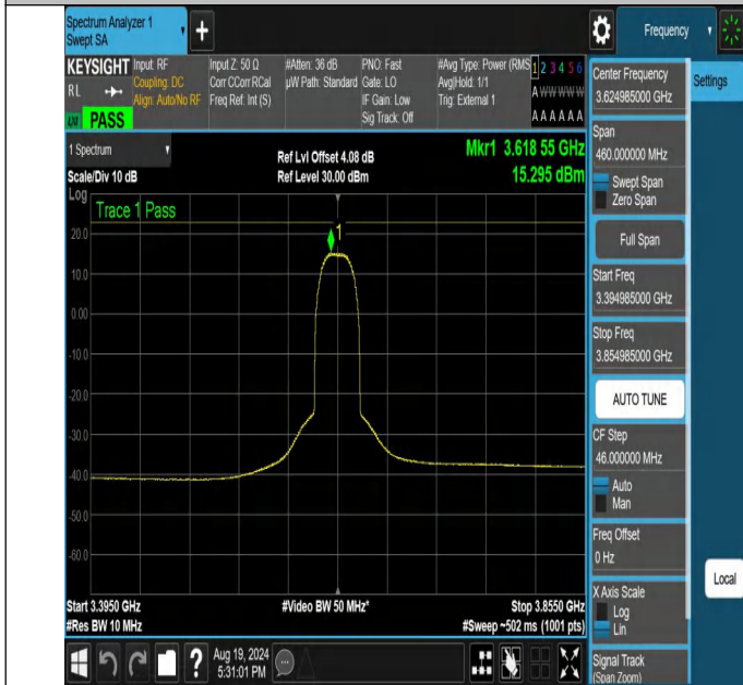
NTNV-N48-PC3-30-30-M-DFT-64QAM-Outer_Full-3394.985-3854.985-Ant1-PASS
