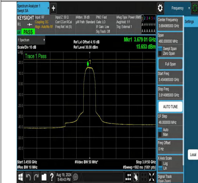
NTNV-N48-PC3-30-30-H-DFT-16QAM-Outer_Full-3454.985-3914.985-Ant1-PASS
