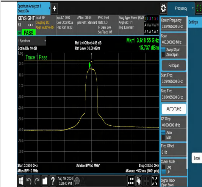
NTNV-N48-PC3-30-30-M-DFT-16QAM-Outer_Full-3394.985-3854.985-Ant1-PASS
