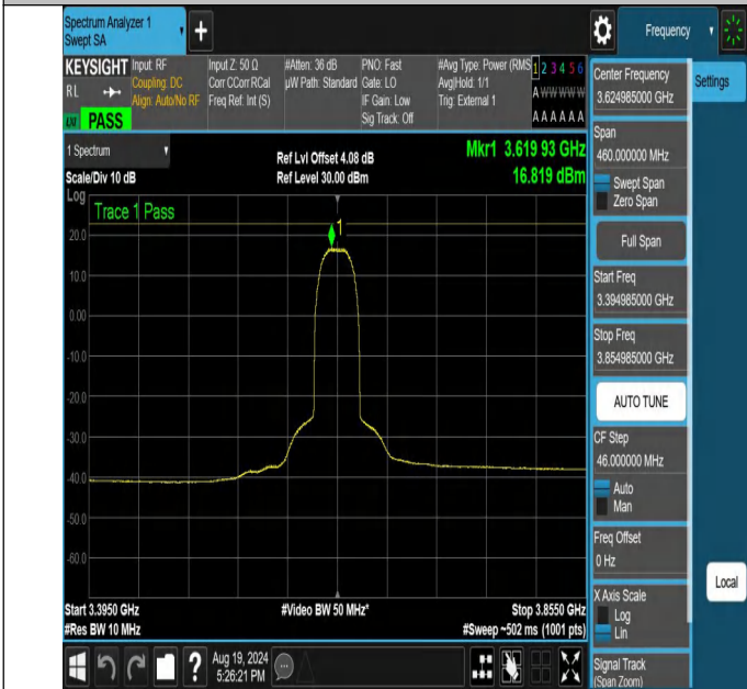
NTNV-N48-PC3-30-30-M-DFT-QPSK-Outer_Full-3394.985-3854.985-Ant1-PASS
