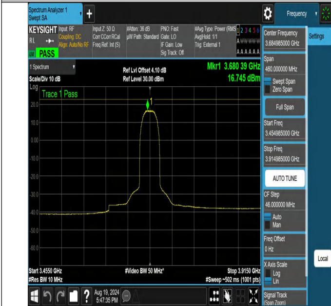
NTNV-N48-PC3-30-30-H-DFT-QPSK-Outer_Full-3454.985-3914.985-85-Ant1-PASS
