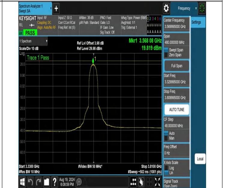
NTNV-N48-PC3-30-40-L-DFT-QPSK-Inner_Full-3329.995-3809.995-Ant1-PASS
