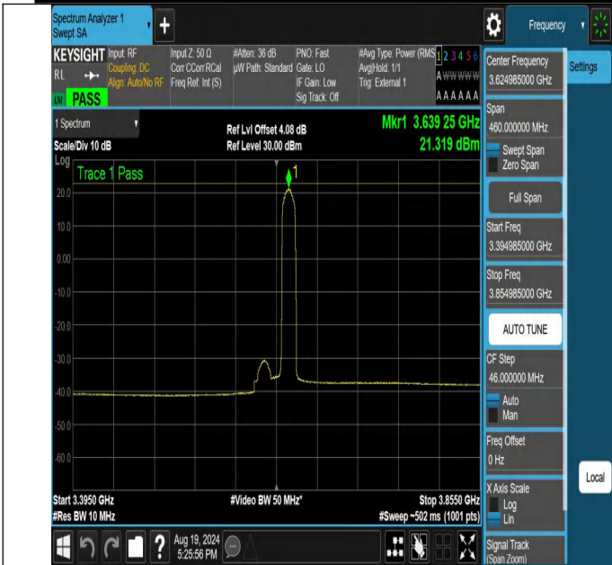
NTNV-N48-PC3-30-30-M-DFT-BPSK-Edge_1RB_Right-3394.985-3854.985-Ant1-PASS
