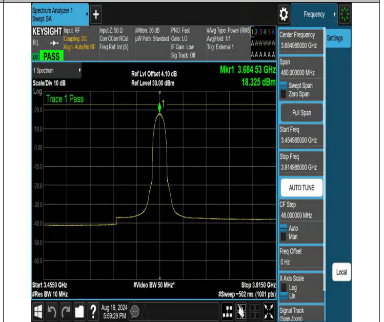
NTNV-N48-PC3-30-30-H-CP-16QAM-Inner_Full-3454.985-3914.985-Ant1-PASS
