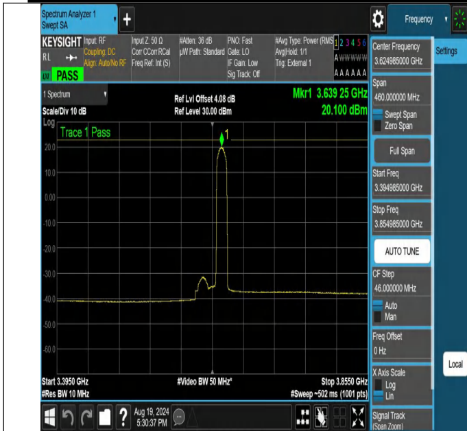
NTNV-N48-PC3-30-30-M-DFT-16QAM-Edge_1RB_Right-3394.985-3854.985-Ant1-PASS
