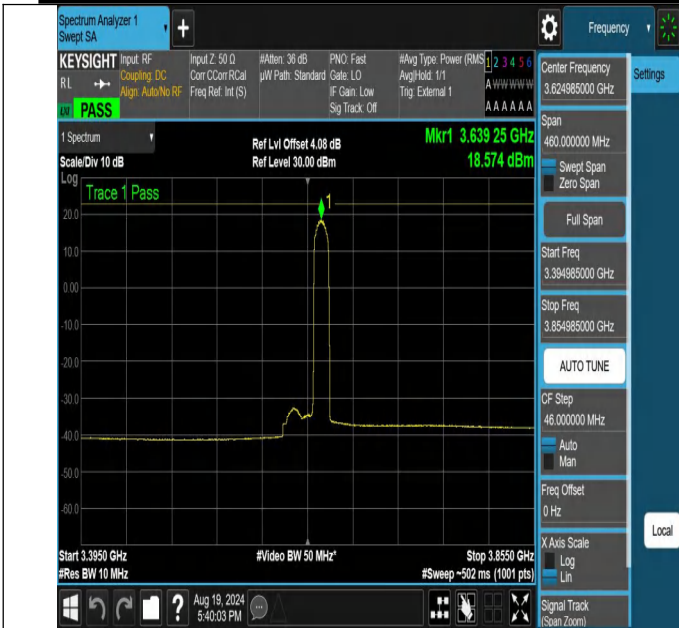
NTNV-N48-PC3-30-30-M-CP-16QAM-Edge_1RB_Right-3394.985-3854.985-Ant1-PASS
