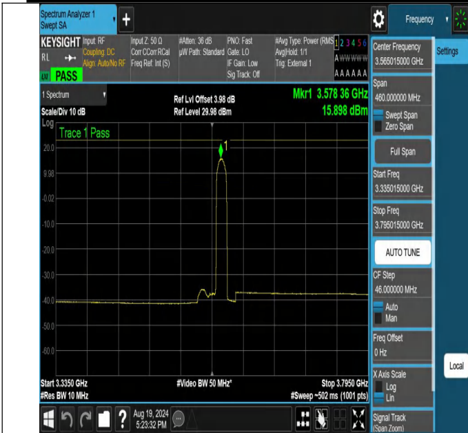
NTNV-N48-PC3-30-30-L-CP-256QAM-Edge_1RB_Right-3335.01 5-3795.015-Ant1-PASS
