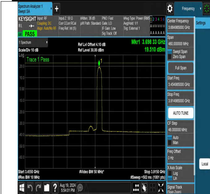
NTNV-N48-PC3-30-30-H-DFT-64QAM-Edge_1RB_Right-3454.98 5-3914.985-Ant1-PASS
