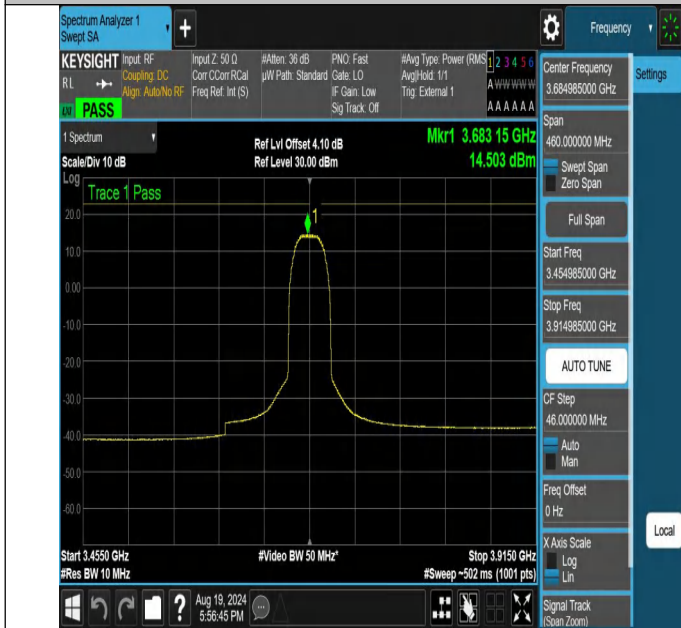
NTNV-N48-PC3-30-30-H-CP-QPSK-Outer_Full-3454.985-3914.9 85-Ant1-PASS
