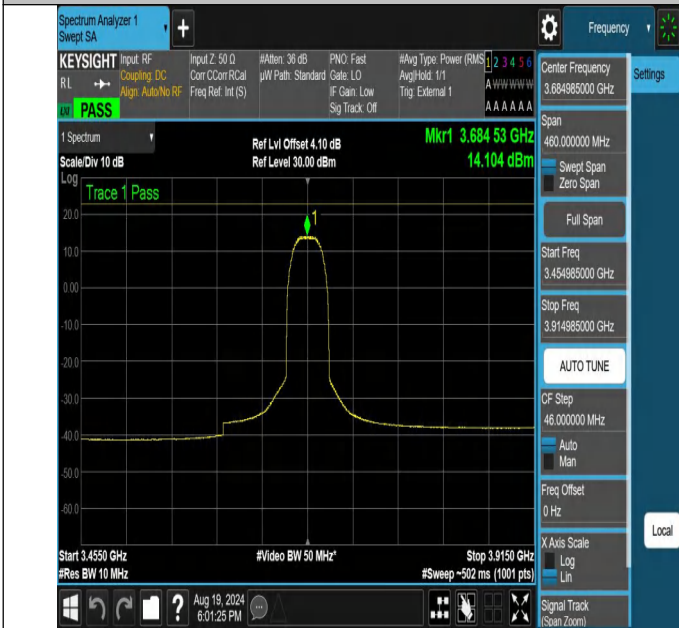
NTNV-N48-PC3-30-30-H-CP-64QAM-Outer_Full-3454.985-3914.985-Ant1-PASS
