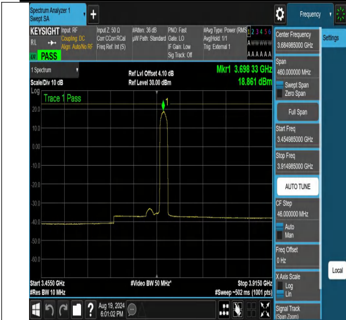
NTNV-N48-PC3-30-30-H-CP-16QAM-Edge_1RB_Right-3454.985-3914.985-Ant1-PASS
