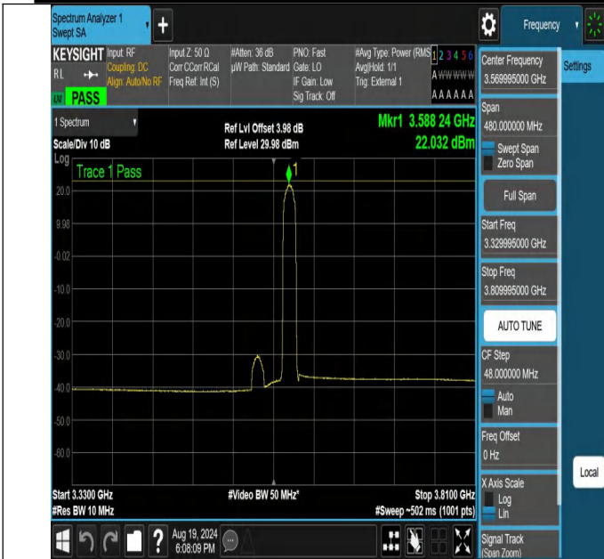
NTNV-N48-PC3-30-40-L-DFT-BPSK-Edge_1RB_Right-3329.995-3809.995-Ant1-PASS
