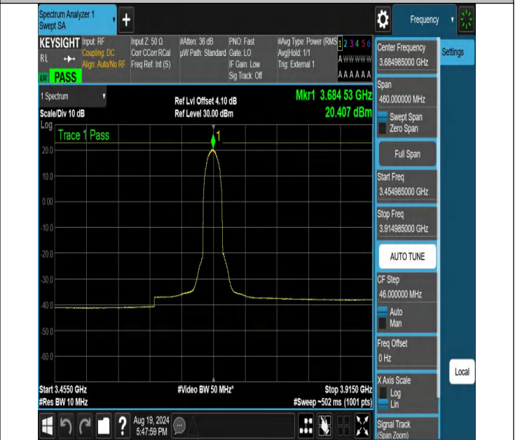
NTNV-N48-PC3-30-30-H-DFT-QPSK-Inner_Full-3454.985-3914.985-85-Ant1-PASS
