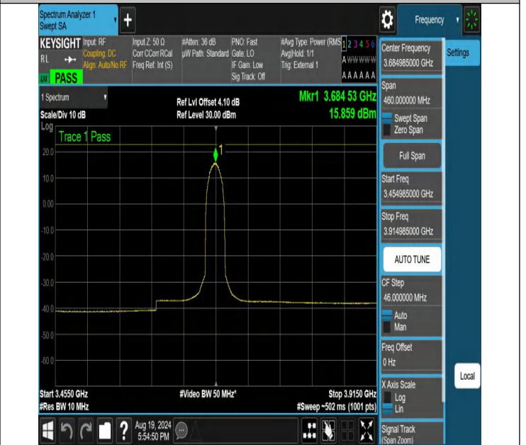
NTNV-N48-PC3-30-30-H-DFT-256QAM-Inner_Full-3454.985-391 4.985-Ant1-PASS
