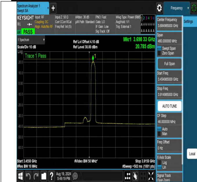
NTNV-N48-PC3-30-30-H-DFT-QPSK-Edge_1RB_Right-3454.985-3914.985-Ant1-PASS
