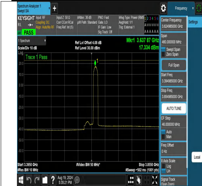
NTNV-N48-PC3-30-30-M-DFT-256QAM-Edge_1RB_Right-3394.9-85-3854.985-Ant1-PASS
