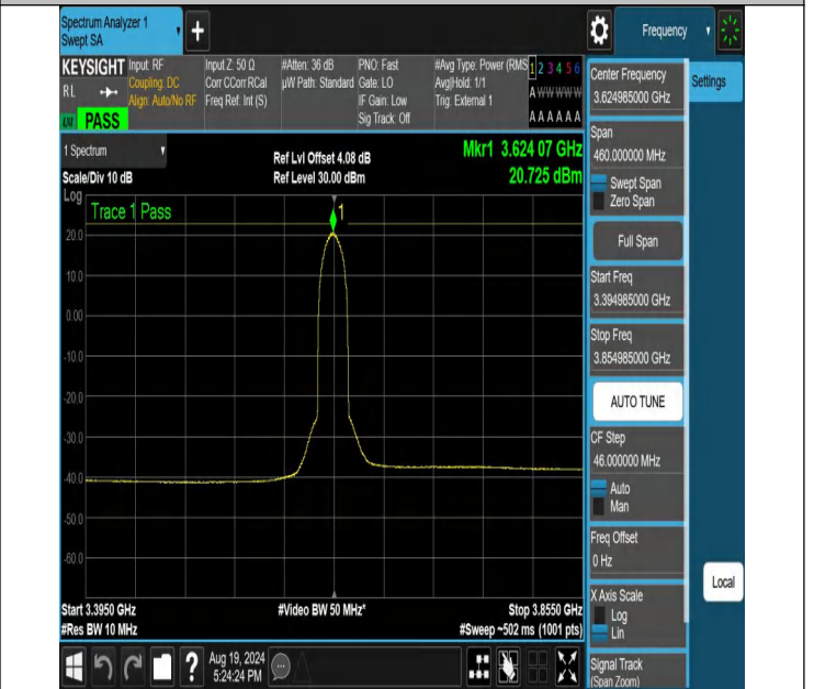
NTNV-N48-PC3-30-30-M-DFT-BPSK-Inner_Full-3394.985-3854.9 85-Ant1-PASS
