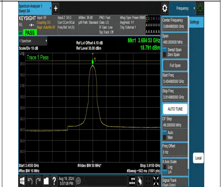
NTNV-N48-PC3-30-30-H-CP-QPSK-Inner_Full-3454.985-3914.98 5-Ant1-PASS
