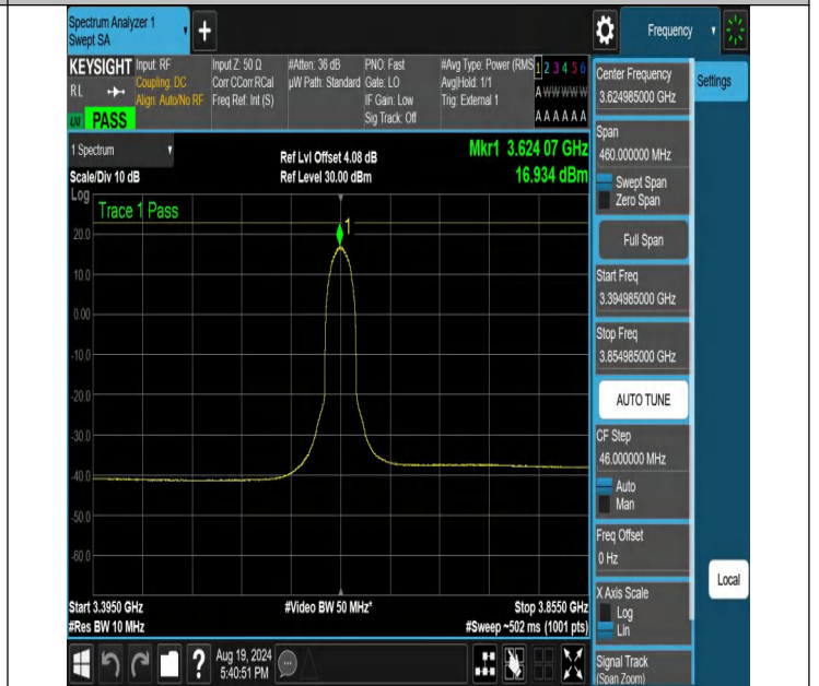
NTNV-N48-PC3-30-30-M-CP-64QAM-Inner_Full-3394.985-3854.985-Ant1-PASS
