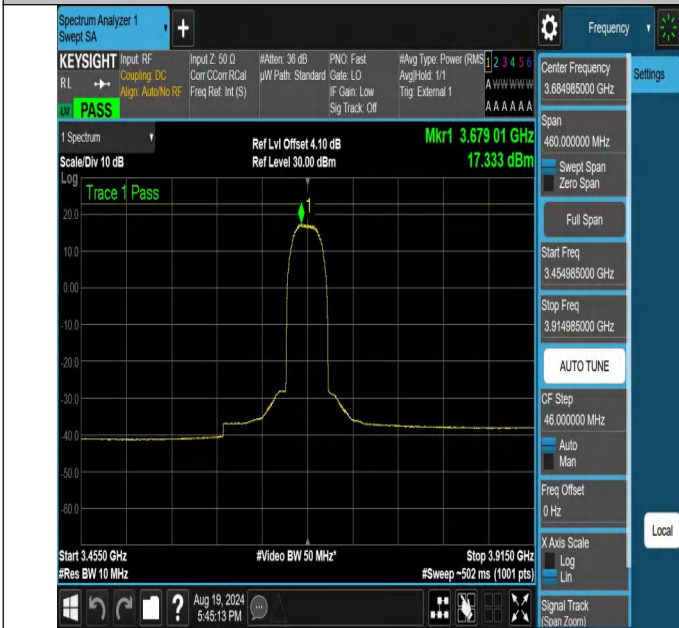
NTNV-N48-PC3-30-30-H-DFT-BPSK-Outer_Full-3454.985-3914.985-Ant1-PASS
