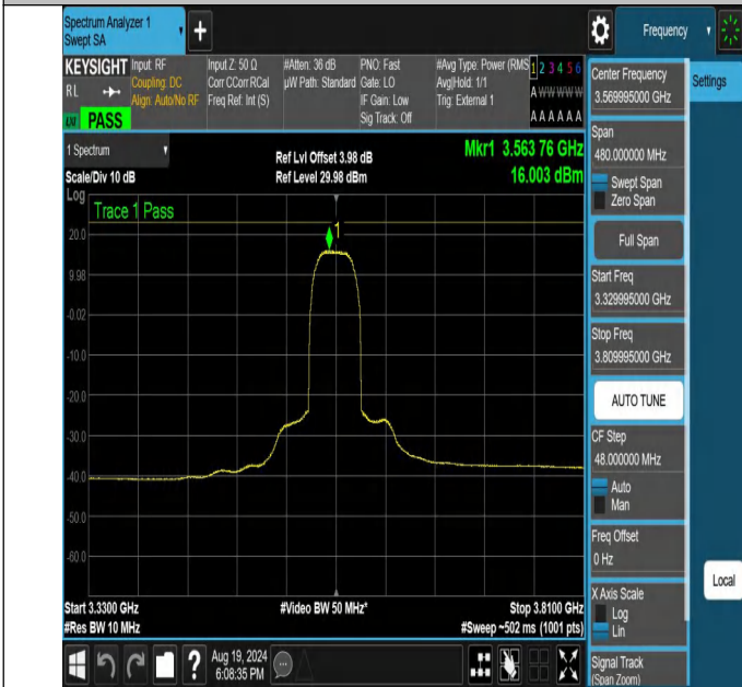
NTNV-N48-PC3-30-40-L-DFT-QPSK-Outer_Full-3329.995-3809.995-Ant1-PASS
