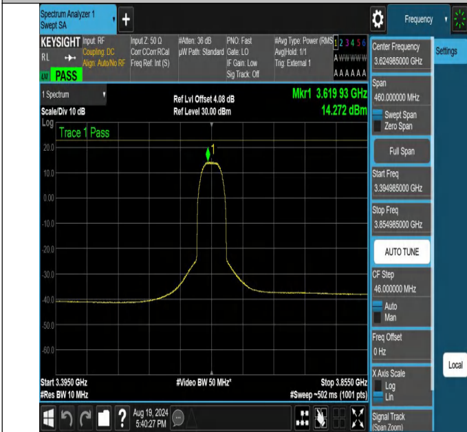
NTNV-N48-PC3-30-30-M-CP-64QAM-Outer_Full-3394.985-3854.985-Ant1-PASS
