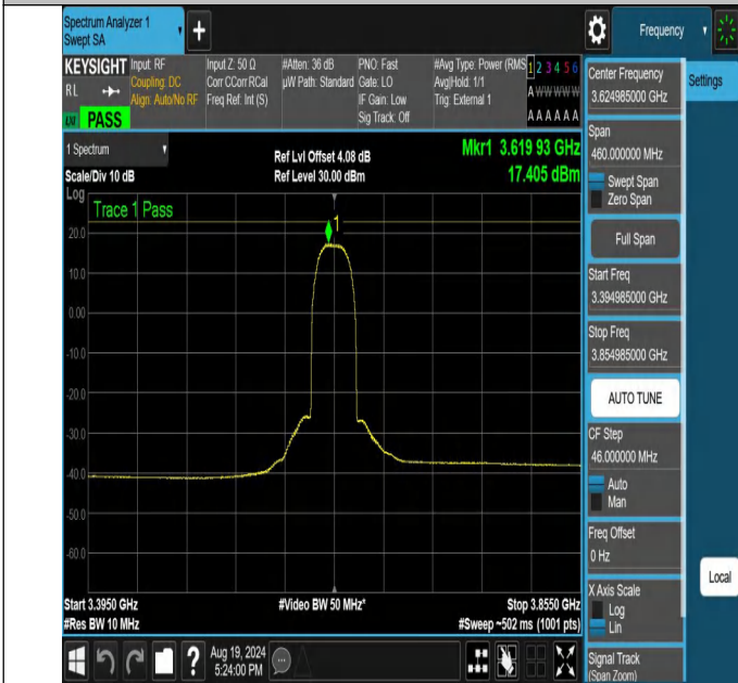
NTNV-N48-PC3-30-30-M-DFT-BPSK-Outer_Full-3394.985-3854.9 85-Ant1-PASS
