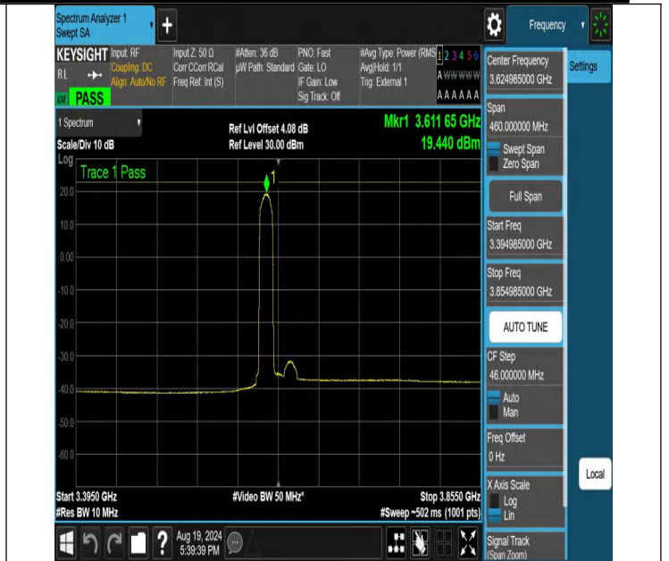
NTNV-N48-PC3-30-30-M-CP-16QAM-Edge_1RB_Left-3394.985-3854.985-Ant1-PASS
