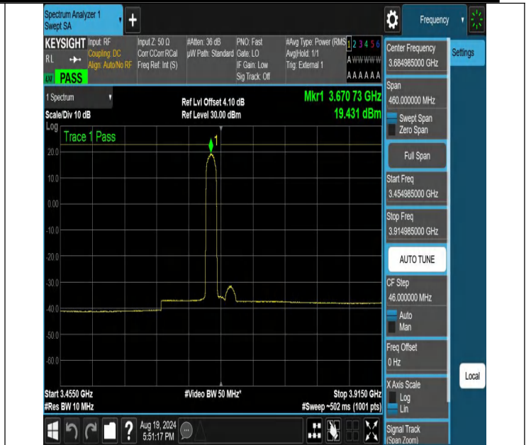
NTNV-N48-PC3-30-30-H-DFT-16QAM-Edge_1RB_Left-3454.985-3914.985-Ant1-PASS
