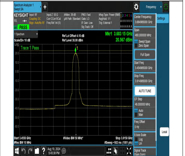
NTNV-N48-PC3-30-30-H-DFT-BPSK-Inner_Full-3454.985-3914.985-Ant1-PASS
