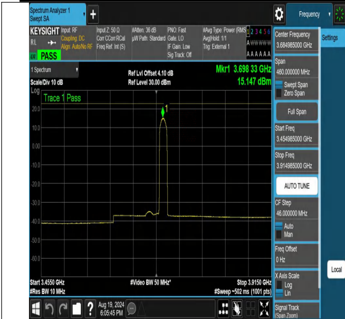
NTNV-N48-PC3-30-30-H-CP-256QAM-Edge_1RB_Right-3454.98-5-3914.985-Ant1-PASS
