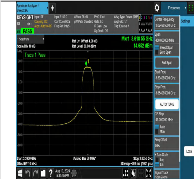
NTNV-N48-PC3-30-30-M-CP-QPSK-Outer_Full-3394.985-3854.985-Ant1-PASS
