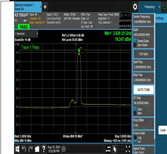
NTNV-N48-PC3-30-30-M-DFT-64QAM-Edge_1RB_Right-3394.98 5-3854.985-Ant1-PASS
