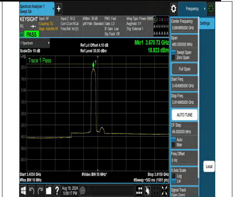
NTNV-N48-PC3-30-30-H-CP-QPSK-Edge_1RB_Left-3454.985-39 14.985-Ant1-PASS
