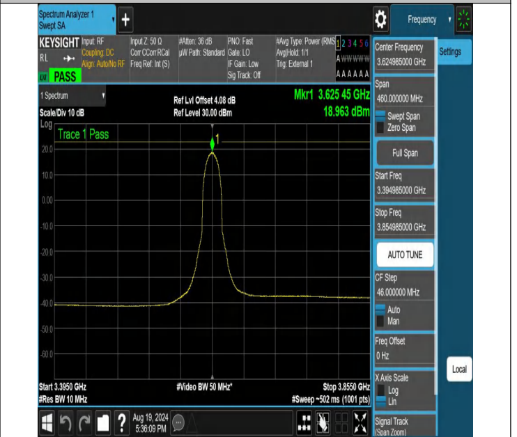
NTNV-N48-PC3-30-30-M-CP-QPSK-Inner_Full-3394.985-3854.985-Ant1-PASS
