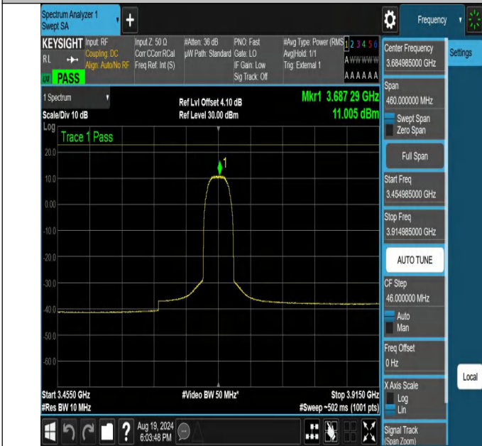
NTNV-N48-PC3-30-30-H-CP-256QAM-Outer_Full-3454.985-3914.985-Ant1-PASS
