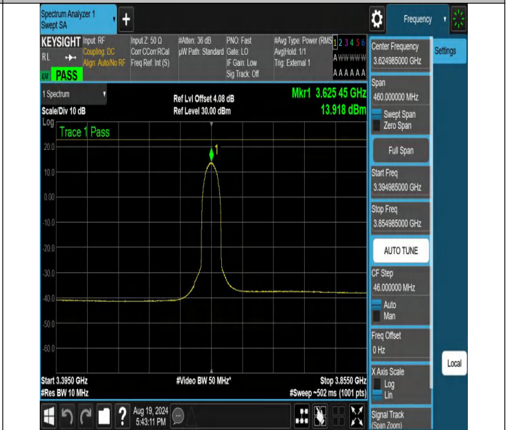
NTNV-N48-PC3-30-30-M-CP-256QAM-Inner_Full-3394.985-3854.985-Ant1-PASS
