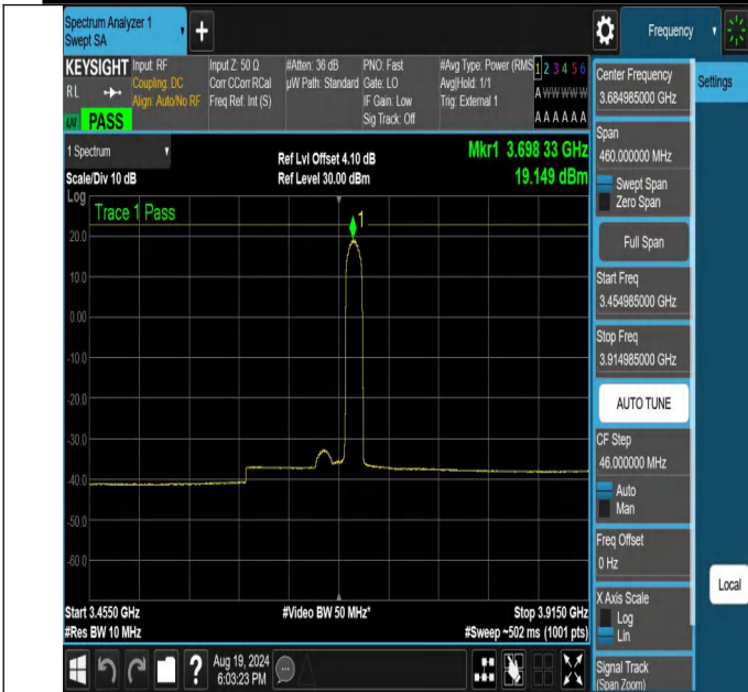
NTNV-N48-PC3-30-30-H-CP-64QAM-Edge_1RB_Right-3454.985-3914.985-Ant1-PASS
