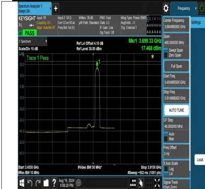
NTNV-N48-PC3-30-30-H-DFT-256QAM-Edge_1RB_Right-3454.9 85-3914.985-Ant1-PASS
