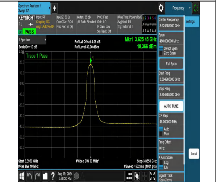
NTNV-N48-PC3-30-30-M-CP-16QAM-Inner_Full-3394.985-3854.985-Ant1-PASS
