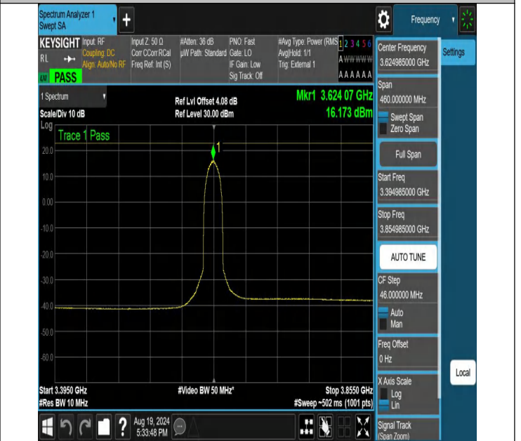
NTNV-N48-PC3-30-30-M-DFT-256QAM-Inner_Full-3394.985-385 4.985-Ant1-PASS
