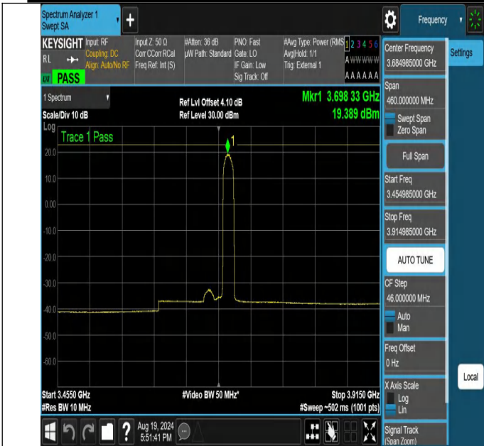
NTNV-N48-PC3-30-30-H-DFT-16QAM-Edge_1RB_Right-3454.985-3914.985-Ant1-PASS
