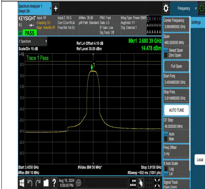
NTNV-N48-PC3-30-30-H-CP-16QAM-Outer_Full-3454.985-3914.985-Ant1-PASS
