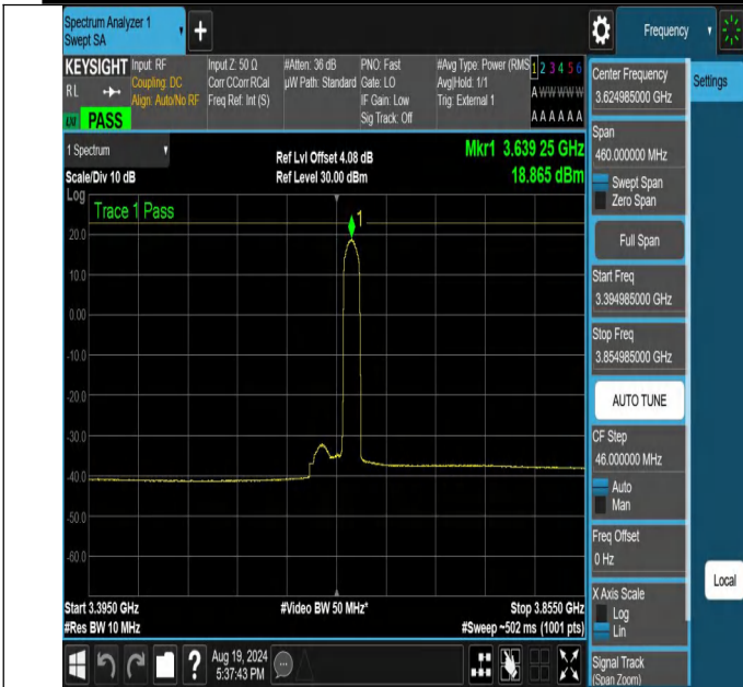
NTNV-N48-PC3-30-30-M-CP-QPSK-Edge_1RB_Right-3394.985-3854.985-Ant1-PASS
