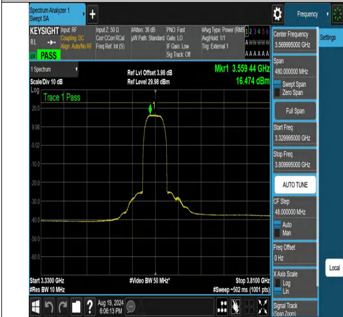
NTNV-N48-PC3-30-40-L-DFT-BPSK-Outer_Full-3329.995-3809.9-95-Ant1-PASS
