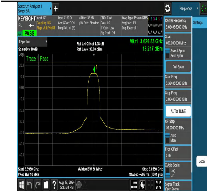
NTNV-N48-PC3-30-30-M-DFT-256QAM-Outer_Full-3394.985-385 4.985-Ant1-PASS
