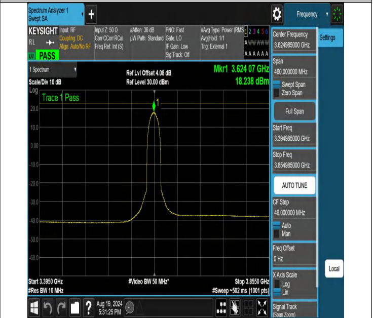
NTNV-N48-PC3-30-30-M-DFT-64QAM-Inner_Full-3394.985-3854.985-Ant1-PASS
