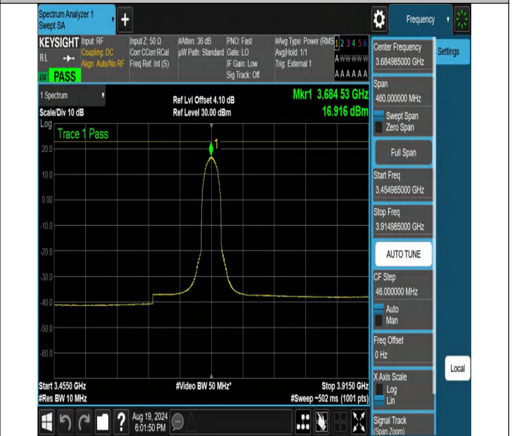
NTNV-N48-PC3-30-30-H-CP-64QAM-Inner_Full-3454.985-3914.985-Ant1-PASS
