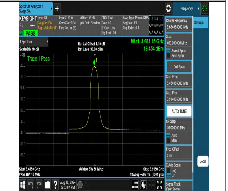
NTNV-N48-PC3-30-30-H-DFT-16QAM-Inner_Full-3454.985-3914.985-Ant1-PASS
