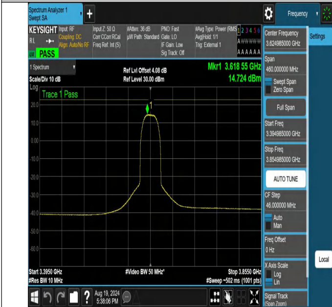
NTNV-N48-PC3-30-30-M-CP-16QAM-Outer_Full-3394.985-3854.985-Ant1-PASS
