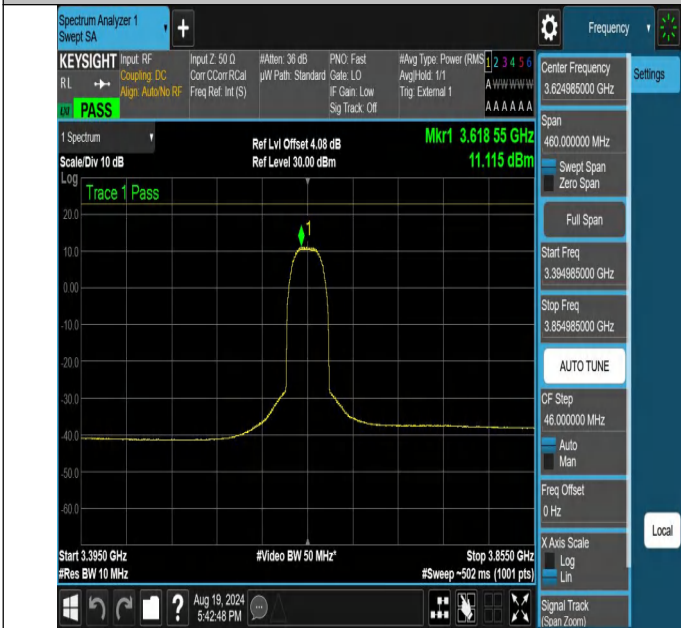
NTNV-N48-PC3-30-30-M-CP-256QAM-Outer_Full-3394.985-3854.985-Ant1-PASS
