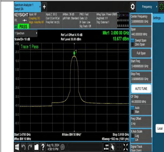
NTNV-N48-PC3-30-20-H-CP-64QAM-Outer_Full-3469.995-3909.995-Ant1-PASS
