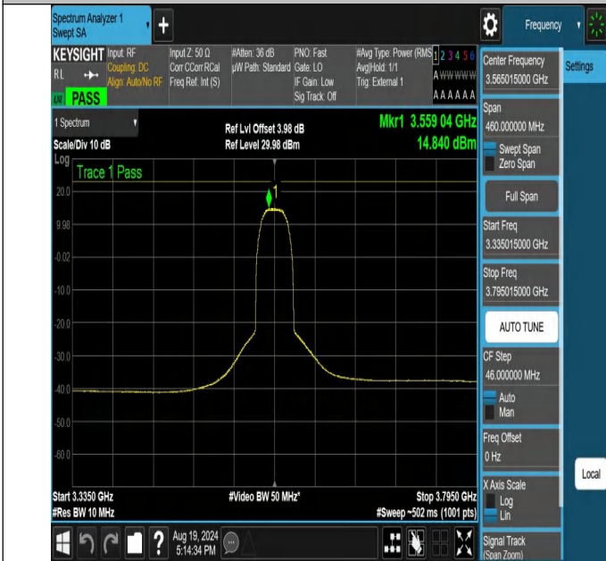
NTNV-N48-PC3-30-30-L-CP-QPSK-Outer_Full-3335.015-3795.015-Ant1-PASS
