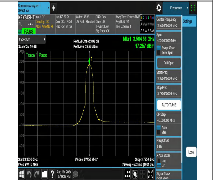
NTNV-N48-PC3-30-30-L-CP-64QAM-Inner_Full-3335.015-3795.015-15-Ant1-PASS
