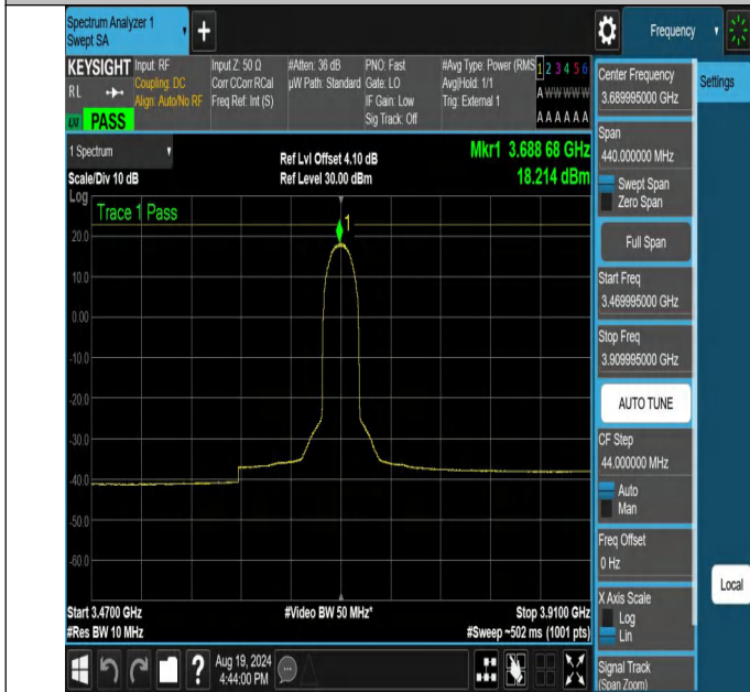
NTNV-N48-PC3-30-20-H-DFT-QPSK-Outer_Full-3469.995-3909.995-Ant1-PASS
