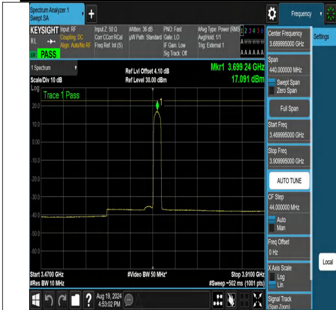
NTNV-N48-PC3-30-20-H-DFT-256QAM-Edge_1RB_Right-3469.9 95-3909.995-Ant1-PASS
