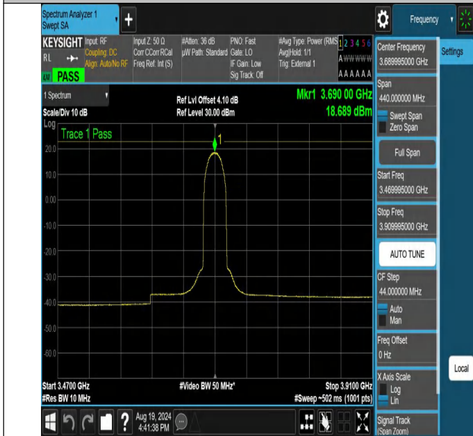
NTNV-N48-PC3-30-20-H-DFT-BPSK-Outer_Full-3469.995-3909.995-Ant1-PASS
