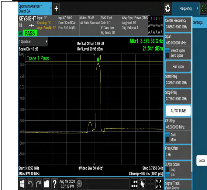
NTNV-N48-PC3-30-30-L-DFT-QPSK-Edge_1RB_Right-3335.015-3795.015-Ant1-PASS
