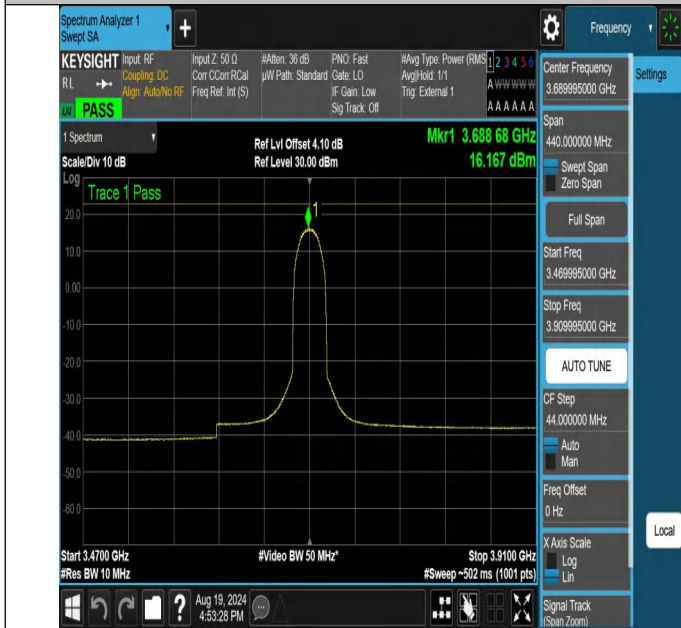
NTNV-N48-PC3-30-20-H-CP-QPSK-Outer_Full-3469.995-3909.995-Ant1-PASS
