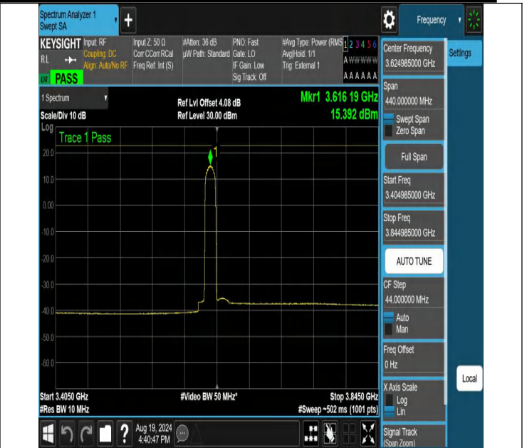
NTNV-N48-PC3-30-20-M-CP-256QAM-Edge_1RB_Left-3404.985-3844.985-Ant1-PASS
