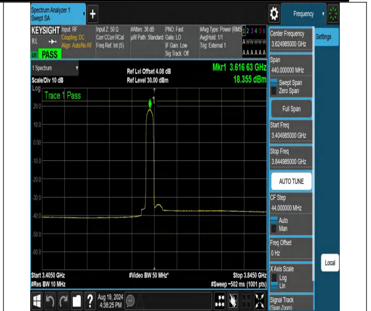
NTNV-N48-PC3-30-20-M-CP-64QAM-Edge_1RB_Left-3404.985-3844.985-Ant1-PASS
