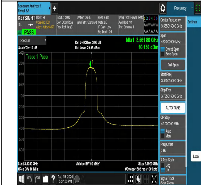
NTNV-N48-PC3-30-30-L-DFT-16QAM-Outer_Full-3335.015-3795.015-Ant1-PASS
