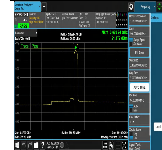
NTNV-N48-PC3-30-20-H-DFT-BPSK-Edge_1RB_Right-3469.995-3909.995-Ant1-PASS
