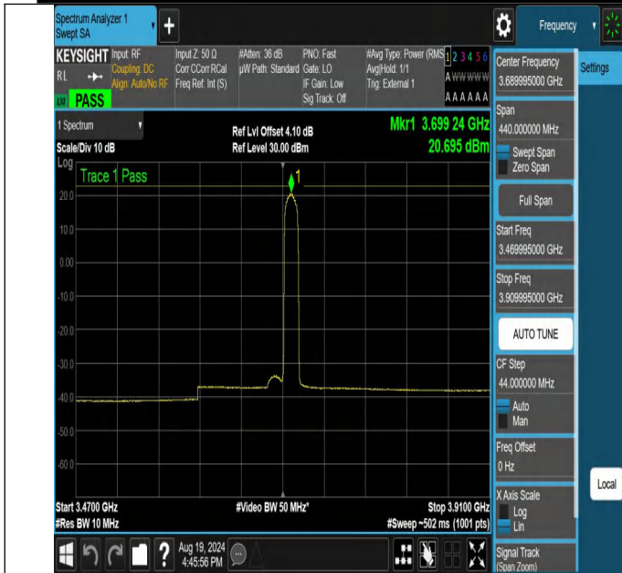
NTNV-N48-PC3-30-20-H-DFT-QPSK-Edge_1RB_Right-3469.995-3909.995-Ant1-PASS
