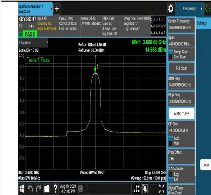
NTNV-N48-PC3-30-20-H-DFT-256QAM-Outer_Full-3469.995-390 9.995-Ant1-PASS
