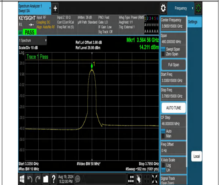
NTNV-N48-PC3-30-30-L-CP-256QAM-Inner_Full-3335.015-3795.015-Ant1-PASS
