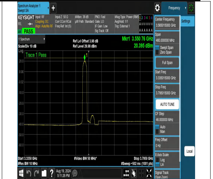
NTNV-N48-PC3-30-30-L-DFT-64QAM-Edge_1RB_Left-3335.015-3795.015-Ant1-PASS
