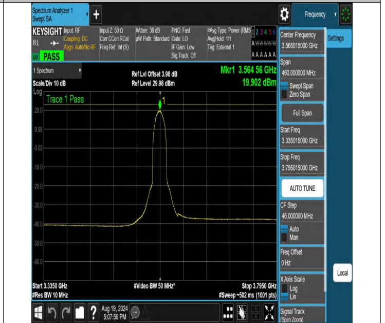
NTNV-N48-PC3-30-30-L-DFT-16QAM-Inner_Full-3335.015-3795.015-Ant1-PASS
