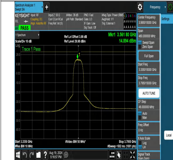
NTNV-N48-PC3-30-30-L-CP-16QAM-Outer_Full-3335.015-3795.015-15-Ant1-PASS
