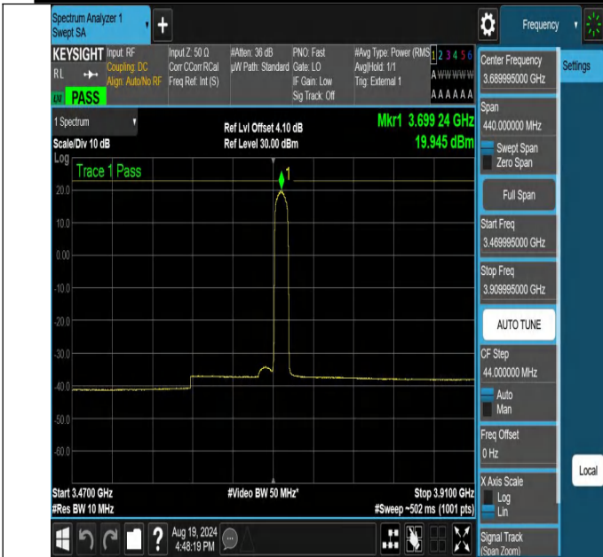
NTNV-N48-PC3-30-20-H-DFT-16QAM-Edge_1RB_Right-3469.995-3909.995-Ant1-PASS
