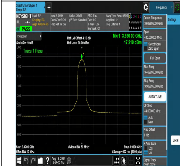
NTNV-N48-PC3-30-20-H-DFT-16QAM-Outer_Full-3469.995-3909.995-Ant1-PASS
