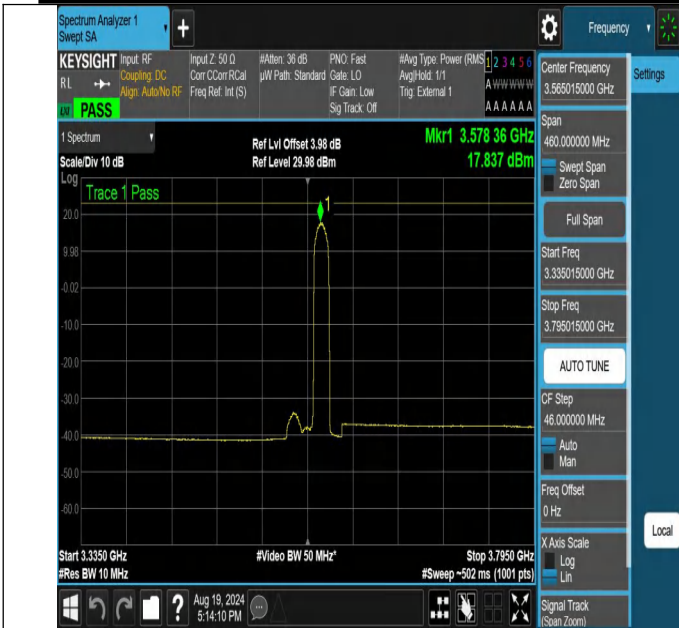
NTNV-N48-PC3-30-30-L-DFT-256QAM-Edge_1RB_Right-3335.015-3795.015-Ant1-PASS
