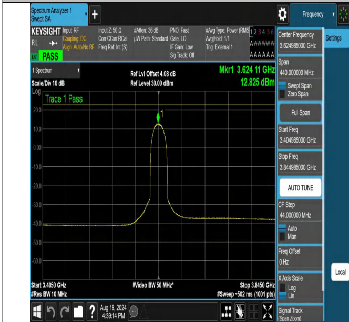
NTNV-N48-PC3-30-20-M-CP-256QAM-Outer_Full-3404.985-3844.985-Ant1-PASS
