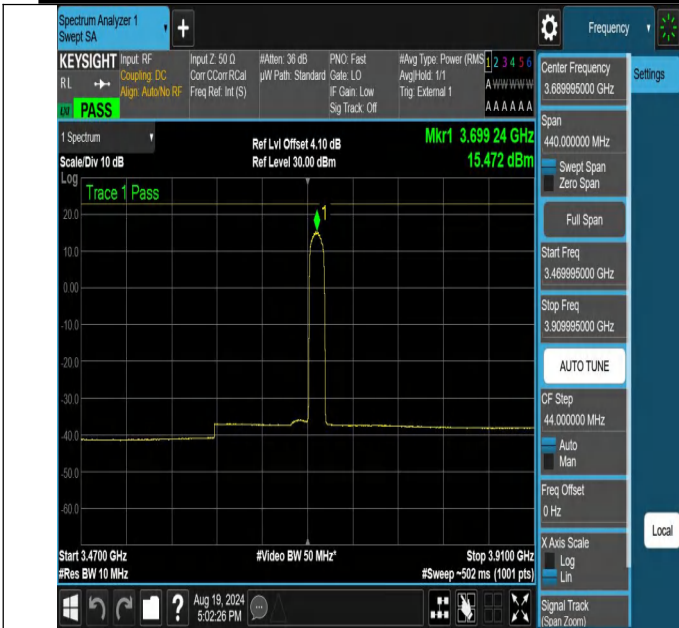
NTNV-N48-PC3-30-20-H-CP-256QAM-Edge_1RB_Right-3469.99 5-3909.995-Ant1-PASS
