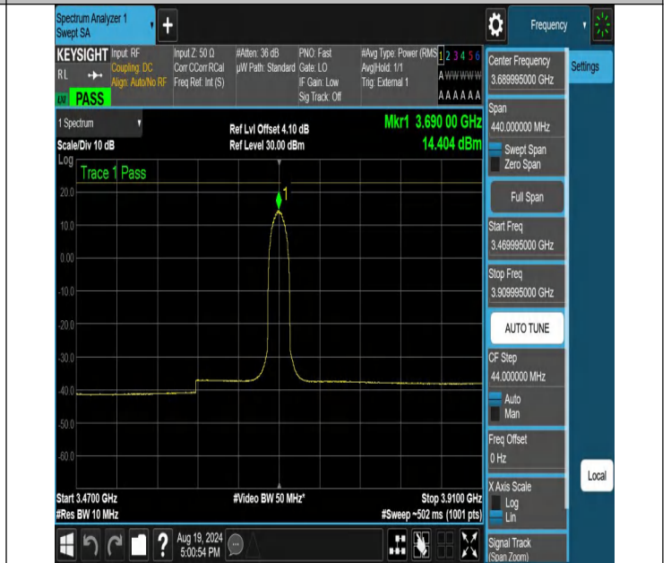
NTNV-N48-PC3-30-20-H-CP-256QAM-Inner_Full-3469.995-3909.995-Ant1-PASS
