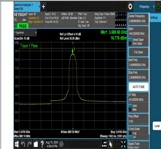
NTNV-N48-PC3-30-20-H-DFT-64QAM-Outer_Full-3469.995-3909.995-Ant1-PASS
