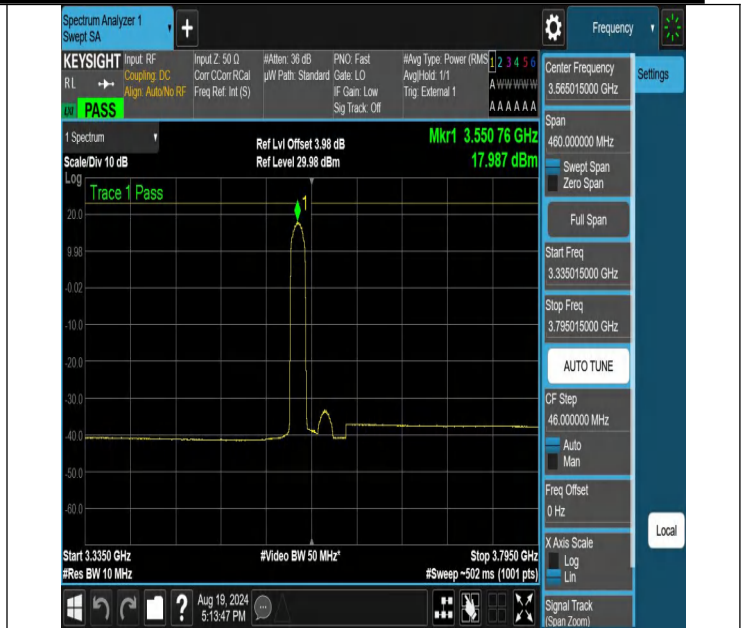
NTNV-N48-PC3-30-30-L-DFT-256QAM-Edge_1RB_Left-3335.015 -3795.015-Ant1-PASS
