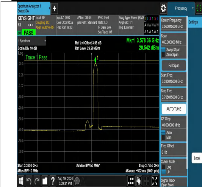
NTNV-N48-PC3-30-30-L-DFT-16QAM-Edge_1RB_Right-3335.015-3795.015-Ant1-PASS
