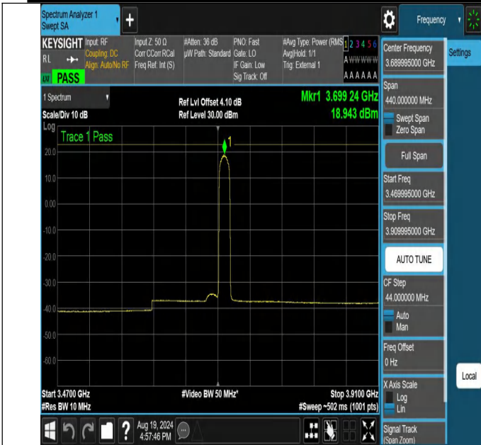
NTNV-N48-PC3-30-20-H-CP-16QAM-Edge_1RB_Right-3469.995-3909.995-Ant1-PASS
