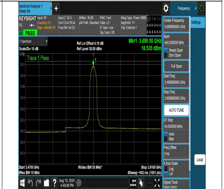
NTNV-N48-PC3-30-20-H-DFT-64QAM-Inner_Full-3469.995-3909.995-Ant1-PASS
