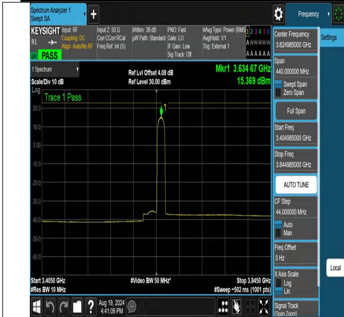
NTNV-N48-PC3-30-20-M-CP-256QAM-Edge_1RB_Right-3404.985-3844.985-Ant1-PASS
