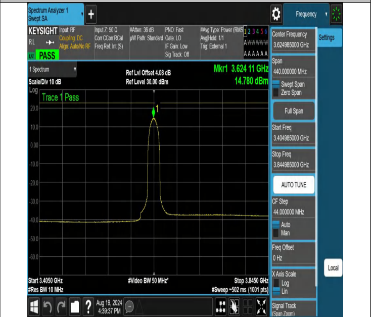
NTNV-N48-PC3-30-20-M-CP-256QAM-Inner_Full-3404.985-3844.985-Ant1-PASS
