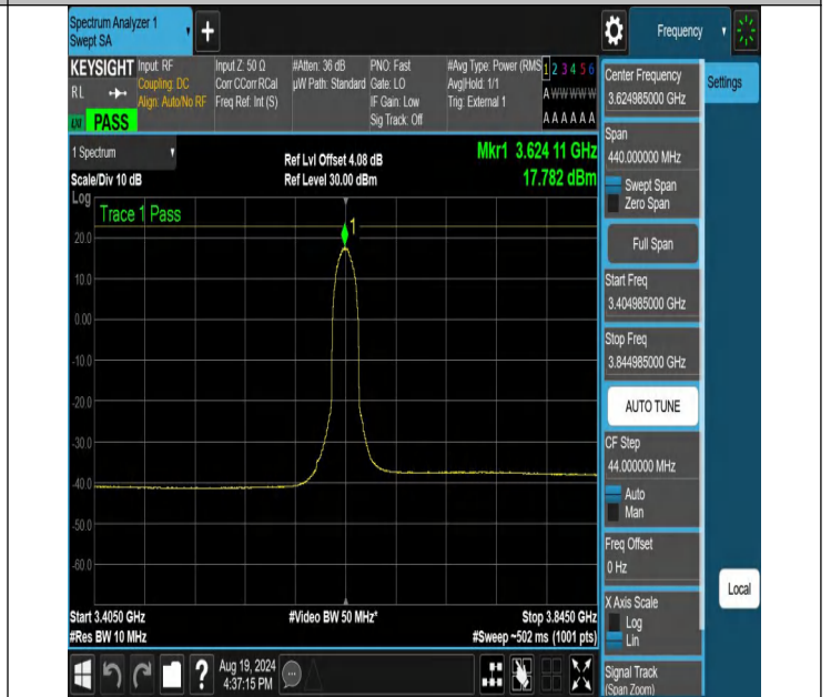
NTNV-N48-PC3-30-20-M-CP-64QAM-Inner_Full-3404.985-3844.985-Ant1-PASS
