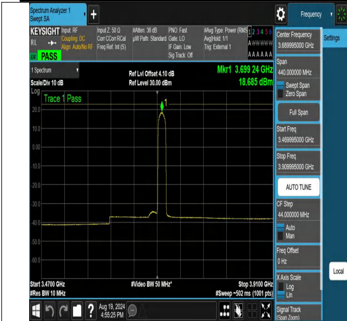
NTNV-N48-PC3-30-20-H-CP-QPSK-Edge_1RB_Right-3469.995-3909.995-Ant1-PASS
