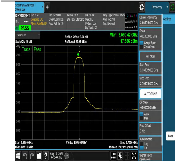
NTNV-N48-PC3-30-30-L-DFT-BPSK-Outer_Full-3335.015-3795.015-Ant1-PASS
