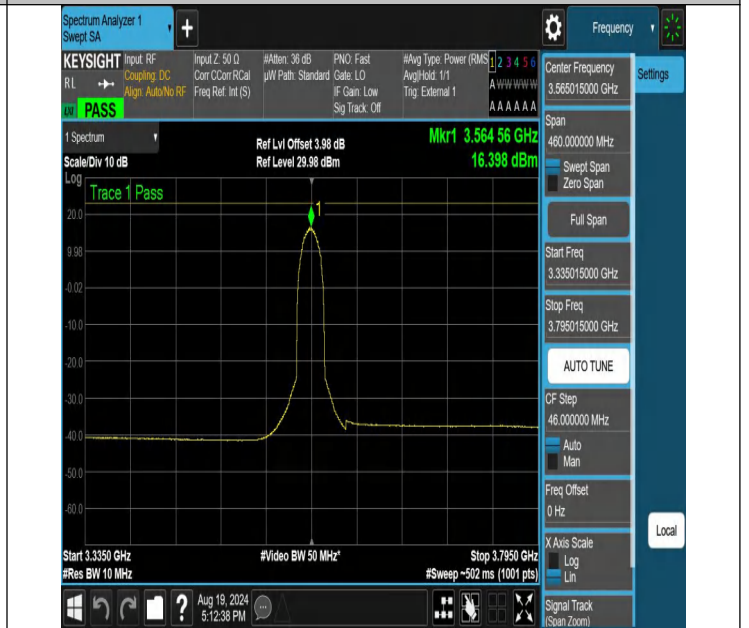
NTNV-N48-PC3-30-30-L-DFT-256QAM-Inner_Full-3335.015-3795.015-Ant1-PASS
