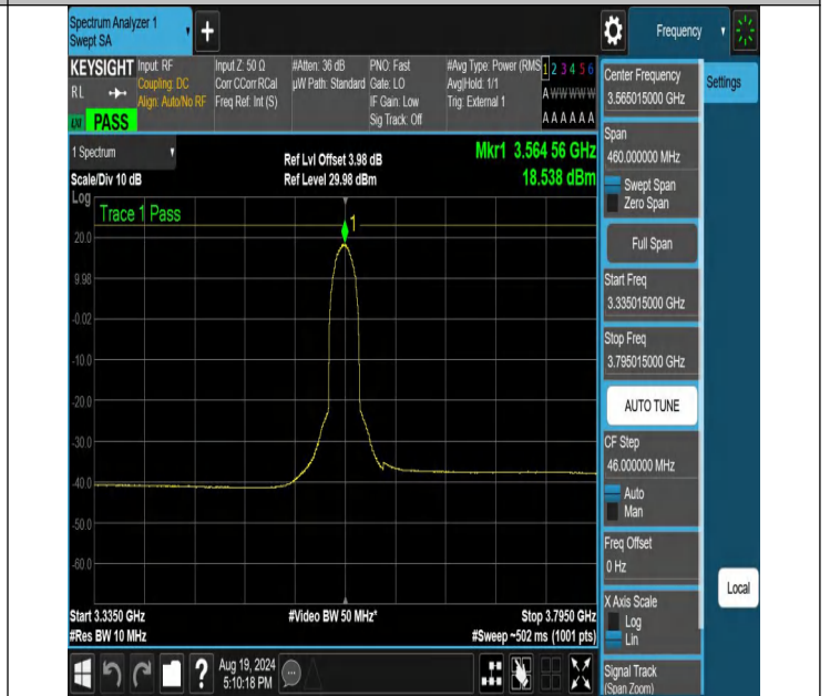
NTNV-N48-PC3-30-30-L-DFT-64QAM-Inner_Full-3335.015-3795.015-Ant1-PASS
