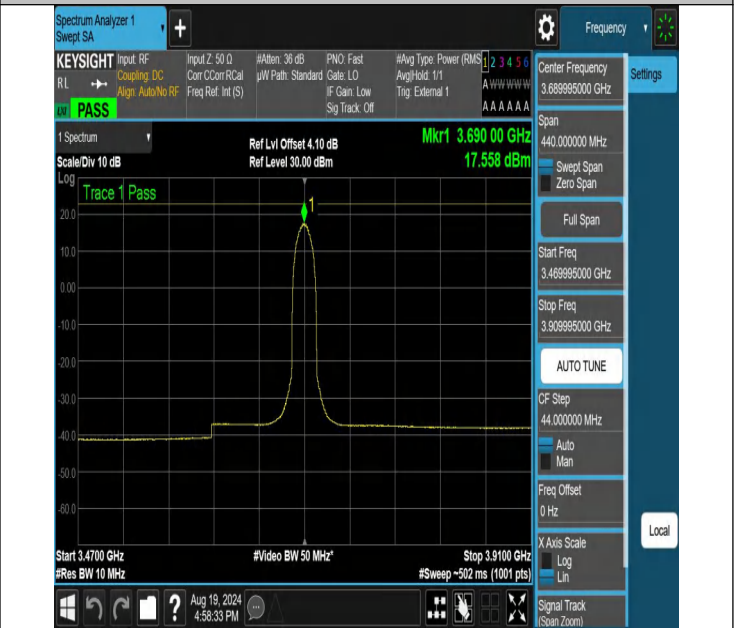
NTNV-N48-PC3-30-20-H-CP-64QAM-Inner_Full-3469.995-3909.995-Ant1-PASS
