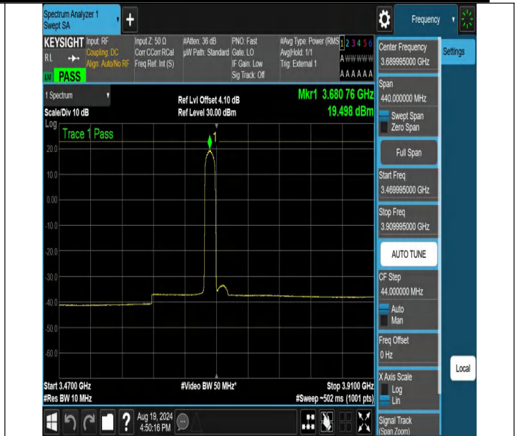
NTNV-N48-PC3-30-20-H-DFT-64QAM-Edge_1RB_Left-3469.995-3909.995-Ant1-PASS
