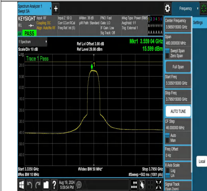
NTNV-N48-PC3-30-30-L-DFT-64QAM-Outer_Full-3335.015-3795.015-Ant1-PASS
