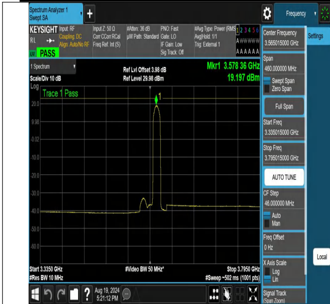
NTNV-N48-PC3-30-30-L-CP-64QAM-Edge_1RB_Right-3335.015-3795.015-Ant1-PASS
