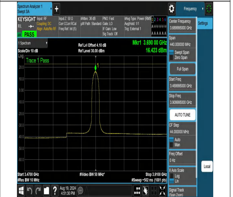
NTNV-N48-PC3-30-20-H-DFT-256QAM-Inner_Full-3469.995-390 9.995-Ant1-PASS
