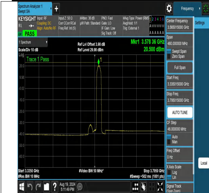
NTNV-N48-PC3-30-30-L-DFT-64QAM-Edge_1RB_Right-3335.01 5-3795.015-Ant1-PASS
