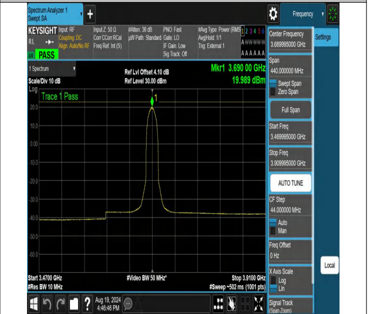
NTNV-N48-PC3-30-20-H-DFT-16QAM-Inner_Full-3469.995-3909.995-Ant1-PASS
