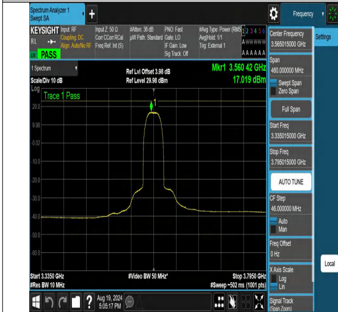
NTNV-N48-PC3-30-30-L-DFT-QPSK-Outer_Full-3335.015-3795.015-Ant1-PASS
