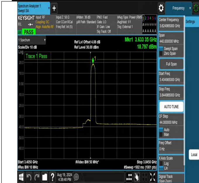
NTNV-N48-PC3-30-20-M-CP-64QAM-Edge_1RB_Right-3404.985-3844.985-Ant1-PASS
