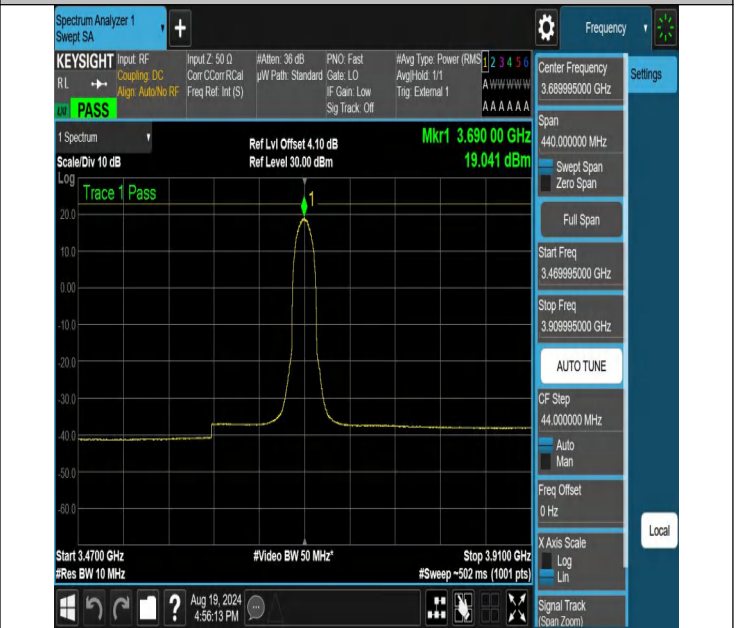
NTNV-N48-PC3-30-20-H-CP-16QAM-Inner_Full-3469.995-3909.995-Ant1-PASS
