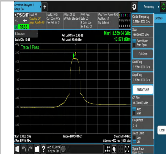
NTNV-N48-PC3-30-30-L-DFT-256QAM-Outer_Full-3335.015-3795.015-Ant1-PASS
