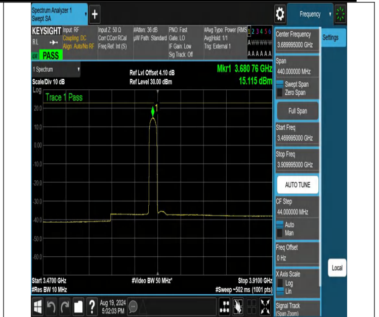
NTNV-N48-PC3-30-20-H-CP-256QAM-Edge_1RB_Left-3469.995-3909.995-Ant1-PASS
