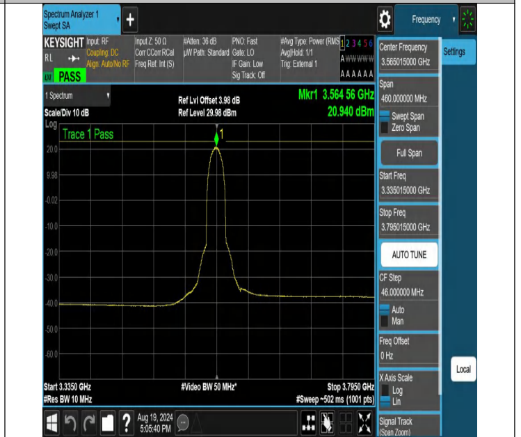
NTNV-N48-PC3-30-30-L-DFT-QPSK-Inner_Full-3335.015-3795.015-Ant1-PASS
