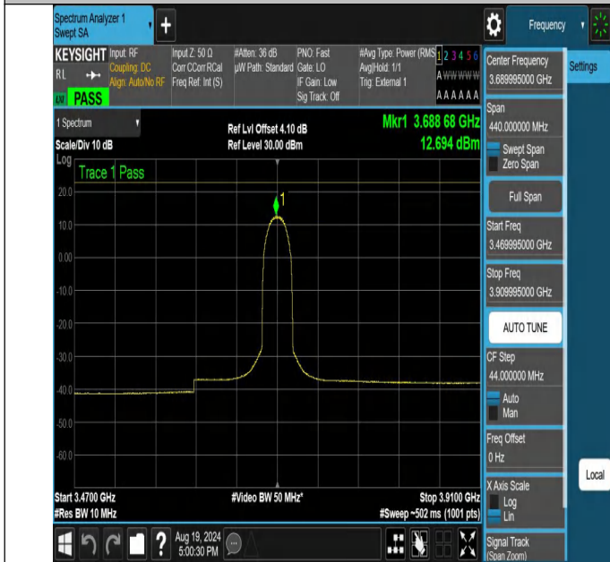
NTNV-N48-PC3-30-20-H-CP-256QAM-Outer_Full-3469.995-3909.995-Ant1-PASS
