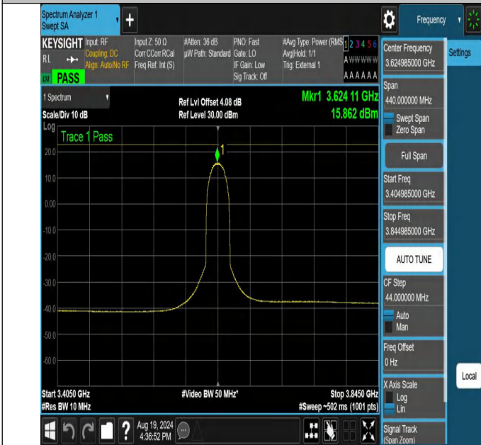
NTNV-N48-PC3-30-20-M-CP-64QAM-Outer_Full-3404.985-3844.985-Ant1-PASS
