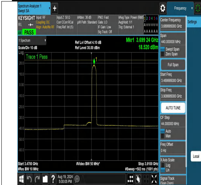
NTNV-N48-PC3-30-20-H-CP-64QAM-Edge_1RB_Right-3469.995-3909.995-Ant1-PASS
