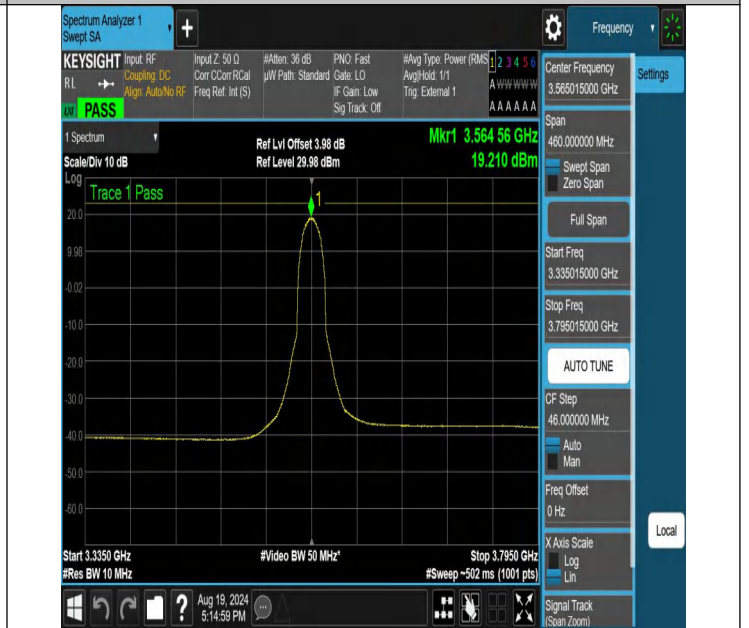
NTNV-N48-PC3-30-30-L-CP-QPSK-Inner_Full-3335.015-3795.015-Ant1-PASS
