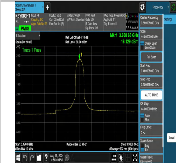
NTNV-N48-PC3-30-20-H-CP-16QAM-Outer_Full-3469.995-3909.995-Ant1-PASS
