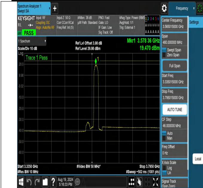
NTNV-N48-PC3-30-30-L-CP-QPSK-Edge_1RB_Right-3335.015-3795.015-Ant1-PASS
