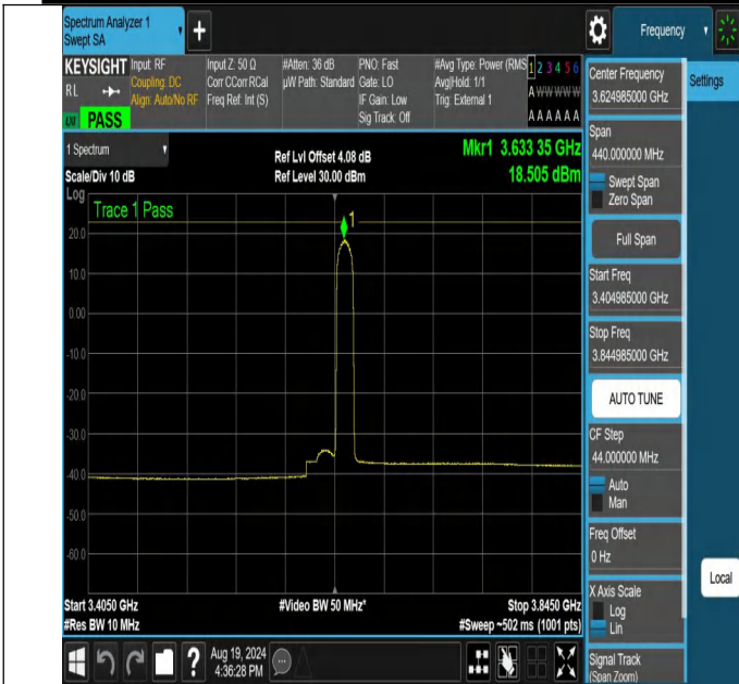
NTNV-N48-PC3-30-20-M-CP-16QAM-Edge_1RB_Right-3404.985-3844.985-Ant1-PASS
