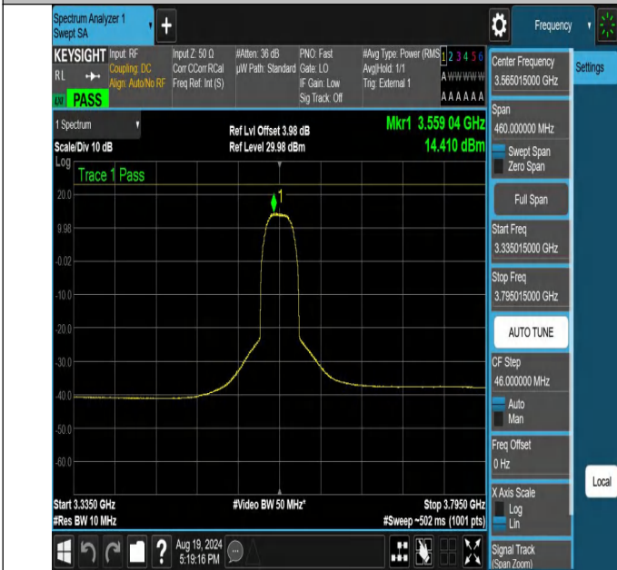
NTNV-N48-PC3-30-30-L-CP-64QAM-Outer_Full-3335.015-3795.015-15-Ant1-PASS
