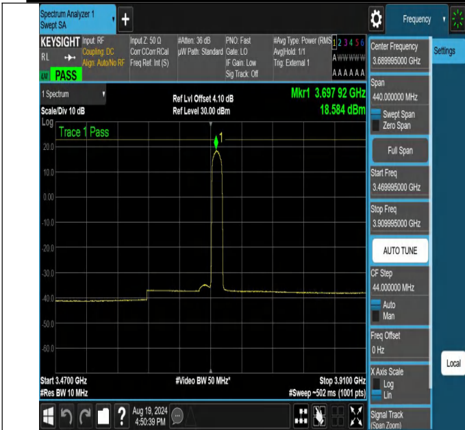
NTNV-N48-PC3-30-20-H-DFT-64QAM-Edge_1RB_Right-3469.99 5-3909.995-Ant1-PASS
