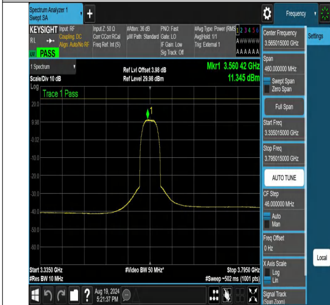
NTNV-N48-PC3-30-30-L-CP-256QAM-Outer_Full-3335.015-3795.015-Ant1-PASS
