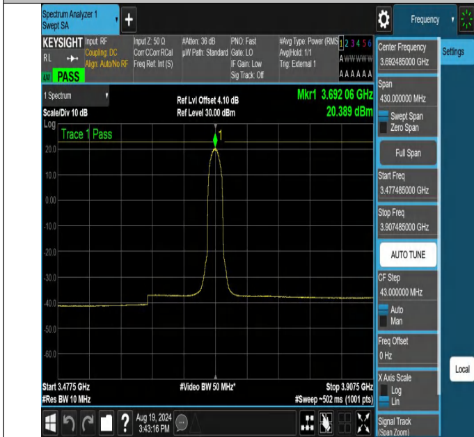
NTNV-N48-PC3-30-15-H-DFT-16QAM-Inner_Full-3477.485-3907.485-Ant1-PASS
