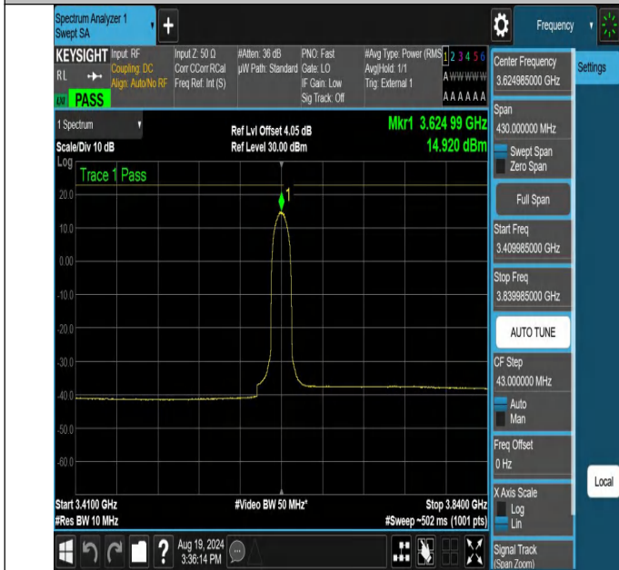
NTNV-N48-PC3-30-15-M-CP-256QAM-Inner_Full-3409.985-3839.985-Ant1-PASS
