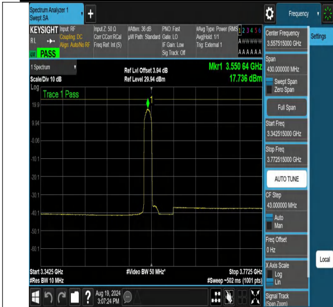
NTNV-N48-PC3-30-15-L-DFT-256QAM-Edge_1RB_Left-3342.515-3772.515-Ant1-PASS
