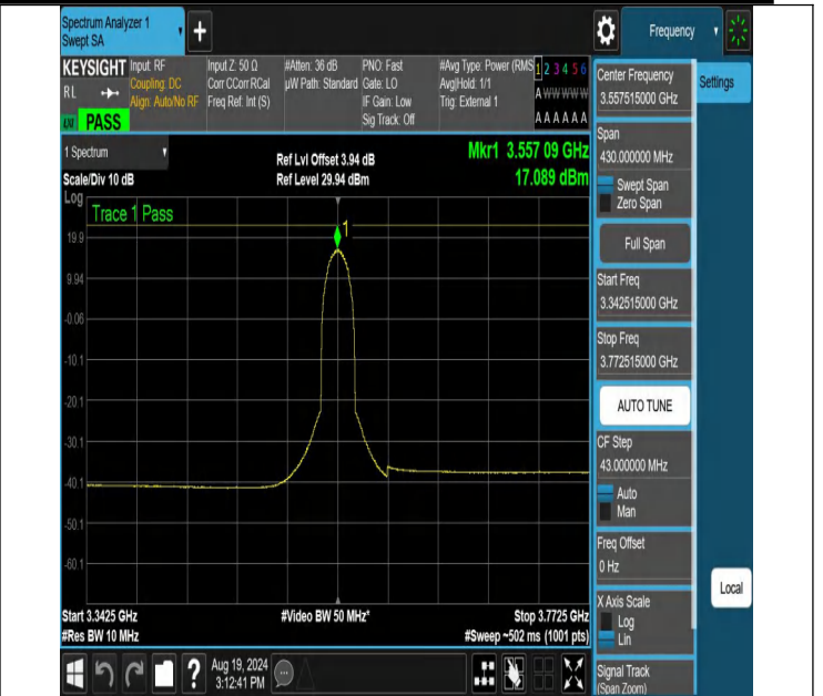
NTNV-N48-PC3-30-15-L-CP-64QAM-Outer_Full-3342.515-3772.515-15-Ant1-PASS
