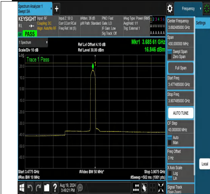
NTNV-N48-PC3-30-15-H-DFT-256QAM-Edge_1RB_Left-3477.485-3907.485-Ant1-PASS
