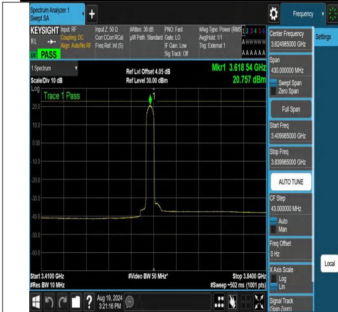
NTNV-N48-PC3-30-15-M-DFT-QPSK-Edge_1RB_Left-3409.985-3839.985-Ant1-PASS
