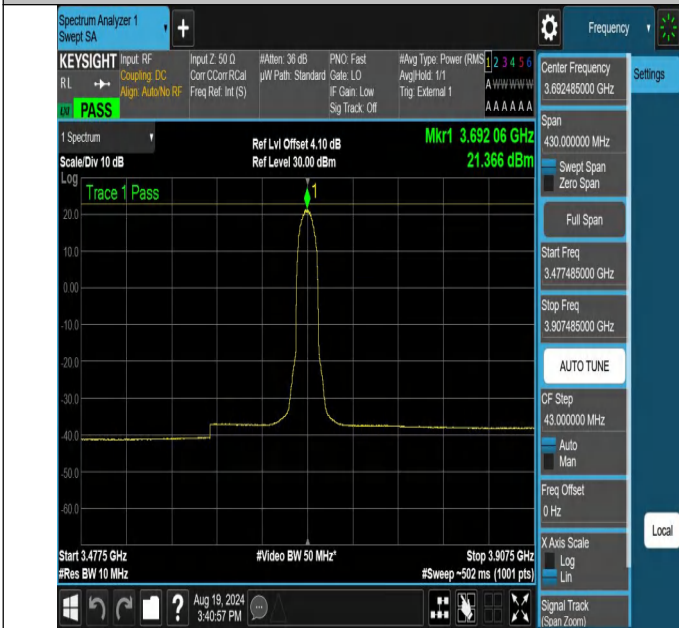
NTNV-N48-PC3-30-15-H-DFT-QPSK-Inner_Full-3477.485-3907.485-Ant1-PASS
