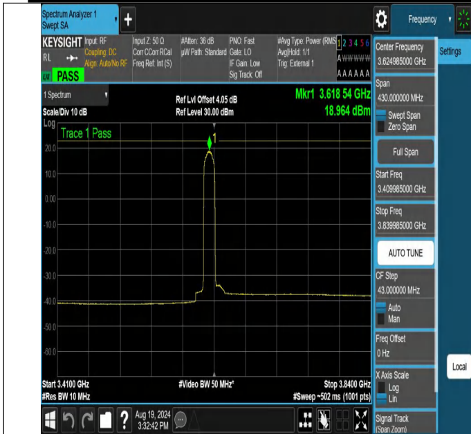
NTNV-N48-PC3-30-15-M-CP-16QAM-Edge_1RB_Left-3409.985-3839.985-Ant1-PASS
