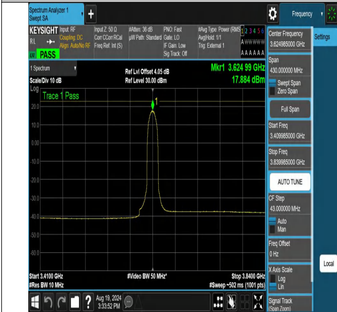
NTNV-N48-PC3-30-15-M-CP-64QAM-Inner_Full-3409.985-3839.985-85-Ant1-PASS
