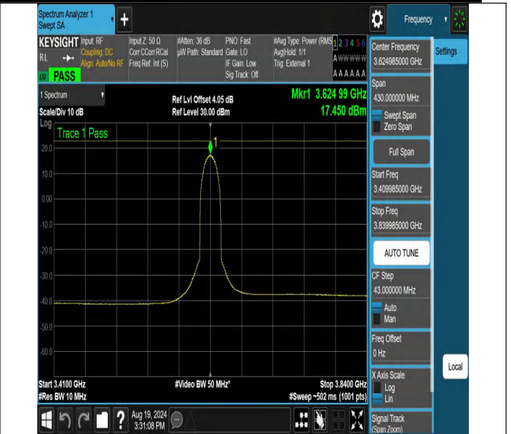
NTNV-N48-PC3-30-15-M-CP-16QAM-Outer_Full-3409.985-3839.985-Ant1-PASS
