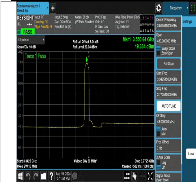
NTNV-N48-PC3-30-15-L-CP-16QAM-Edge_1RB_Left-3342.515-3772.515-Ant1-PASS
