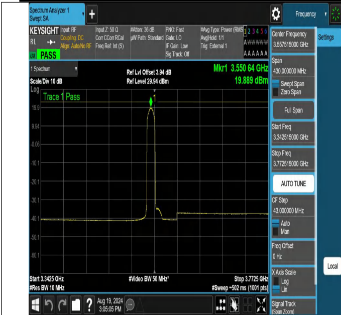
NTNV-N48-PC3-30-15-L-DFT-64QAM-Edge_1RB_Left-3342.515-3772.515-Ant1-PASS
