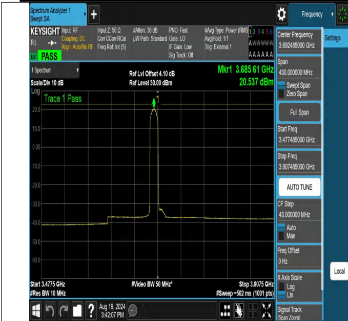
NTNV-N48-PC3-30-15-H-DFT-QPSK-Edge_1RB_Left-3477.485-3907.485-Ant1-PASS
