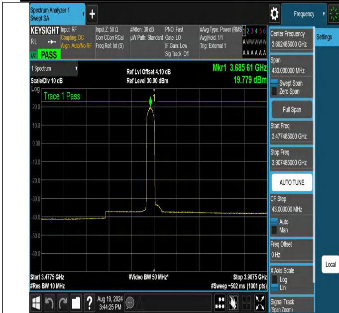
NTNV-N48-PC3-30-15-H-DFT-16QAM-Edge_1RB_Left-3477.485-3907.485-Ant1-PASS
