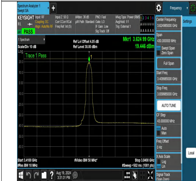
NTNV-N48-PC3-30-15-M-CP-16QAM-Inner_Full-3409.985-3839.985-85-Ant1-PASS
