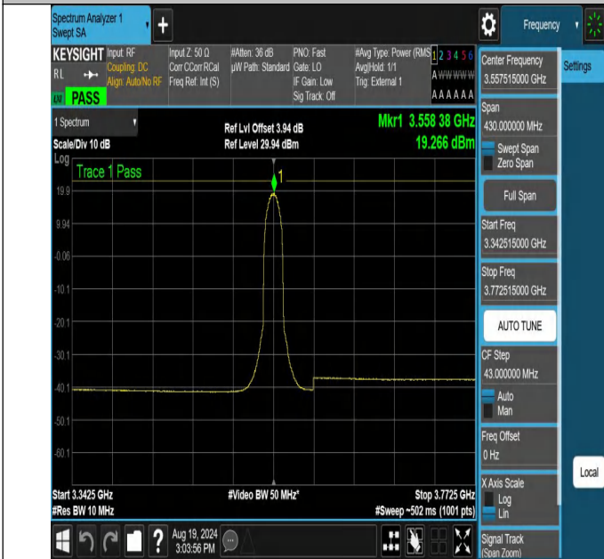
NTNV-N48-PC3-30-15-L-DFT-64QAM-Inner_Full-3342.515-3772.515-Ant1-PASS
