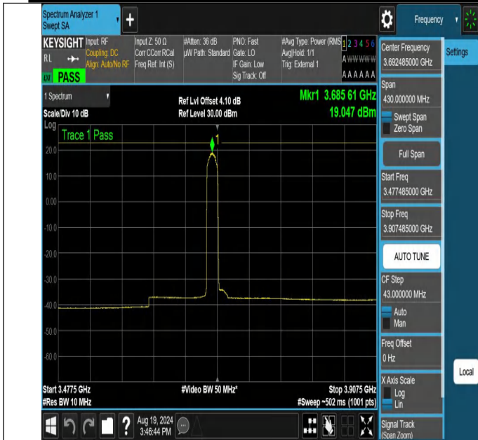
NTNV-N48-PC3-30-15-H-DFT-64QAM-Edge_1RB_Left-3477.485-3907.485-Ant1-PASS
