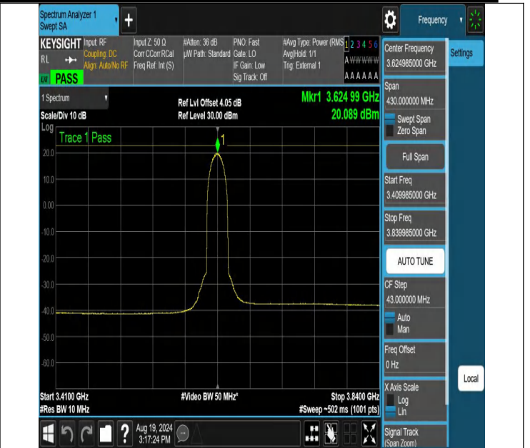
NTNV-N48-PC3-30-15-M-DFT-BPSK-Outer_Full-3409.985-3839.985-Ant1-PASS
