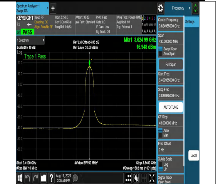
NTNV-N48-PC3-30-15-M-CP-64QAM-Outer_Full-3409.985-3839.985-Ant1-PASS
