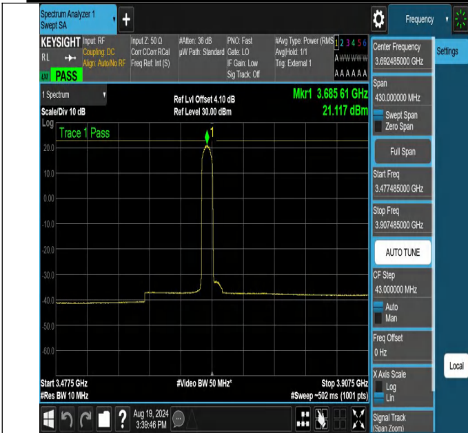
NTNV-N48-PC3-30-15-H-DFT-BPSK-Edge_1RB_Left-3477.485-3907.485-Ant1-PASS
