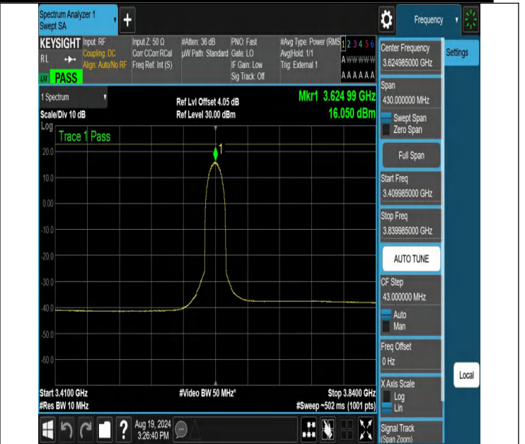
NTNV-N48-PC3-30-15-M-DFT-256QAM-Outer_Full-3409.985-3839.985-Ant1-PASS
