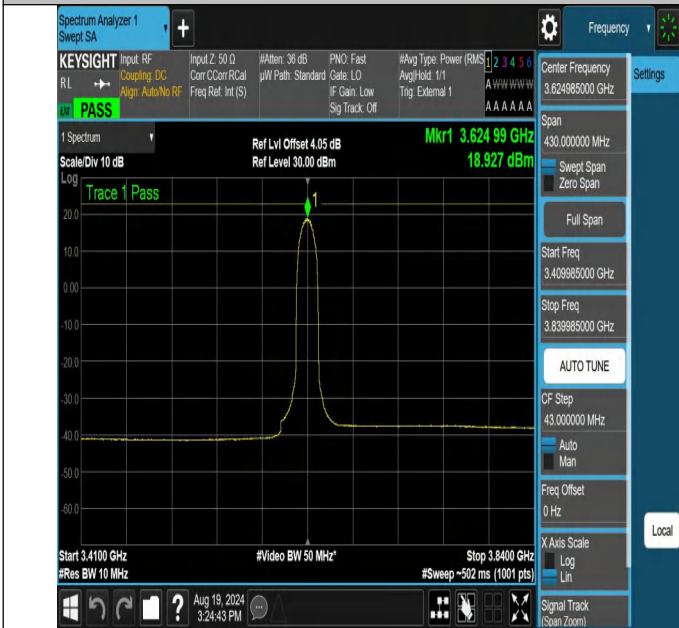
NTNV-N48-PC3-30-15-M-DFT-64QAM-Inner_Full-3409.985-3839.985-Ant1-PASS
