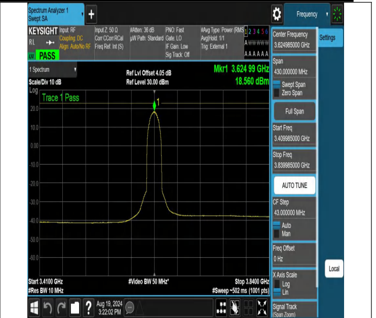
NTNV-N48-PC3-30-15-M-DFT-16QAM-Outer_Full-3409.985-3839.985-Ant1-PASS
