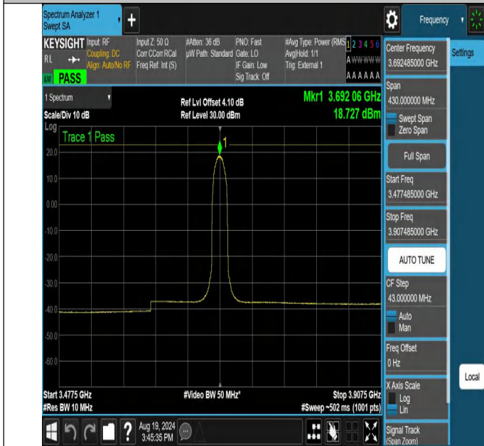
NTNV-N48-PC3-30-15-H-DFT-64QAM-Inner_Full-3477.485-3907.485-Ant1-PASS
