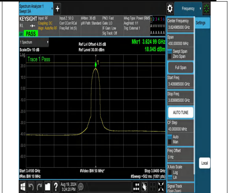
NTNV-N48-PC3-30-15-M-DFT-64QAM-Outer_Full-3409.985-3839.985-Ant1-PASS
