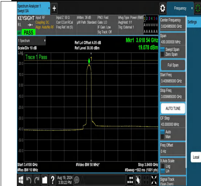
NTNV-N48-PC3-30-15-M-CP-QPSK-Edge_1RB_Left-3409.985-389.985-Ant1-PASS
