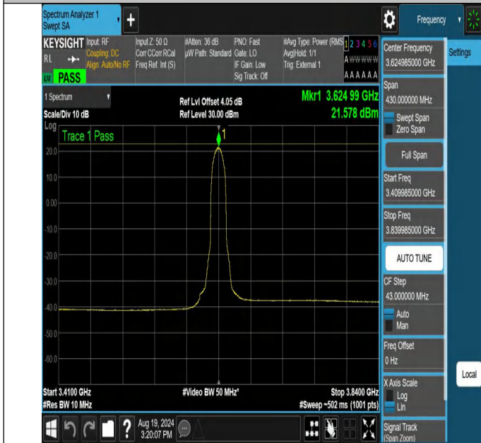
NTNV-N48-PC3-30-15-M-DFT-QPSK-Inner_Full-3409.985-3839.985-Ant1-PASS
