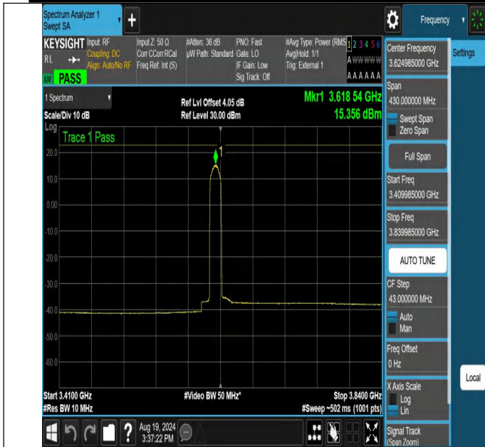
NTNV-N48-PC3-30-15-M-CP-256QAM-Edge_1RB_Left-3409.985-3839.985-Ant1-PASS
