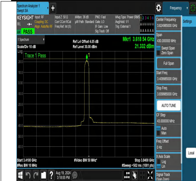
NTNV-N48-PC3-30-15-M-DFT-BPSK-Edge_1RB_Left-3409.985-389.985-Ant1-PASS
