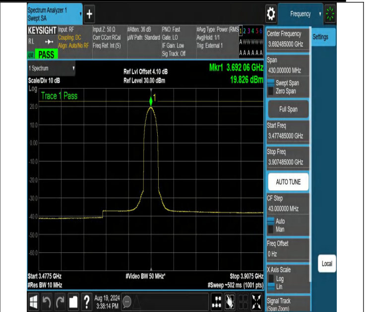
NTNV-N48-PC3-30-15-H-DFT-BPSK-Outer_Full-3477.485-3907.485-Ant1-PASS
