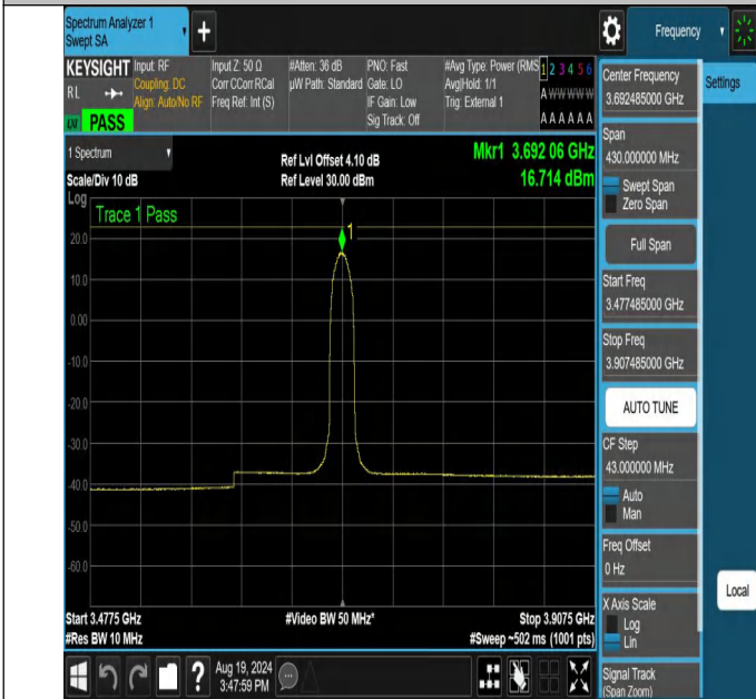
NTNV-N48-PC3-30-15-H-DFT-256QAM-Inner_Full-3477.485-3907.485-Ant1-PASS
