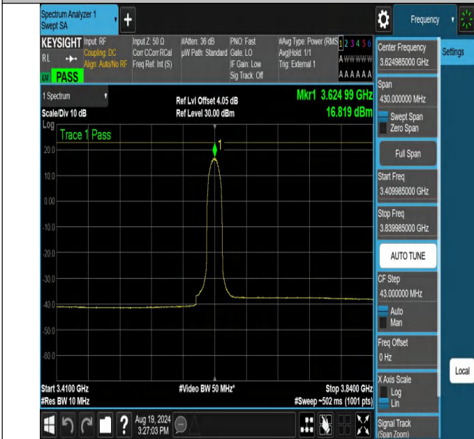
NTNV-N48-PC3-30-15-M-DFT-256QAM-Inner_Full-3409.985-3839.985-Ant1-PASS
