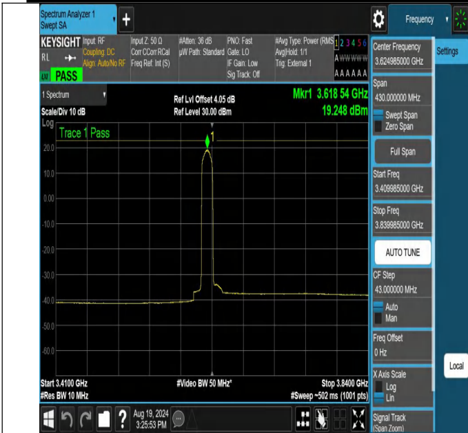
NTNV-N48-PC3-30-15-M-DFT-64QAM-Edge_1RB_Left-3409.985-3839.985-Ant1-PASS
