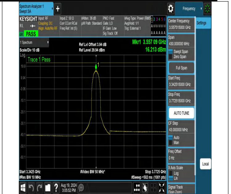
NTNV-N48-PC3-30-15-L-DFT-256QAM-Outer_Full-3342.515-3772.515-Ant1-PASS
