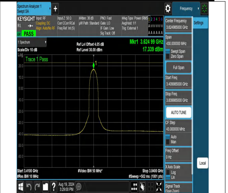
NTNV-N48-PC3-30-15-M-CP-QPSK-Outer_Full-3409.985-3839.985-Ant1-PASS
