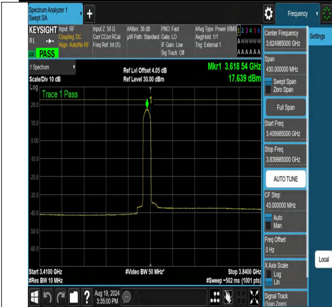
NTNV-N48-PC3-30-15-M-CP-64QAM-Edge_1RB_Left-3409.985-3839.985-Ant1-PASS
