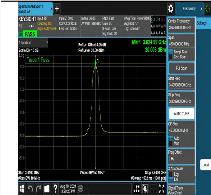
NTNV-N48-PC3-30-15-M-CP-QPSK-Inner_Full-3409.985-3839.985-Ant1-PASS
