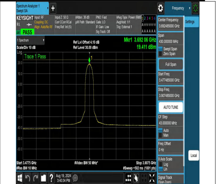
NTNV-N48-PC3-30-15-H-DFT-QPSK-Outer_Full-3477.485-3907.485-Ant1-PASS
