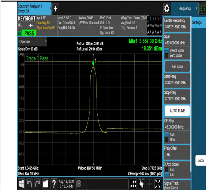
NTNV-N48-PC3-30-15-L-CP-64QAM-Inner_Full-3342.515-3772.515-15-Ant1-PASS
