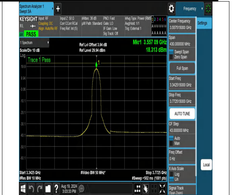
NTNV-N48-PC3-30-15-L-DFT-64QAM-Outer_Full-3342.515-3772.515-Ant1-PASS
