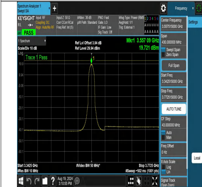
NTNV-N48-PC3-30-15-L-CP-16QAM-Inner_Full-3342.515-3772.515-Ant1-PASS
