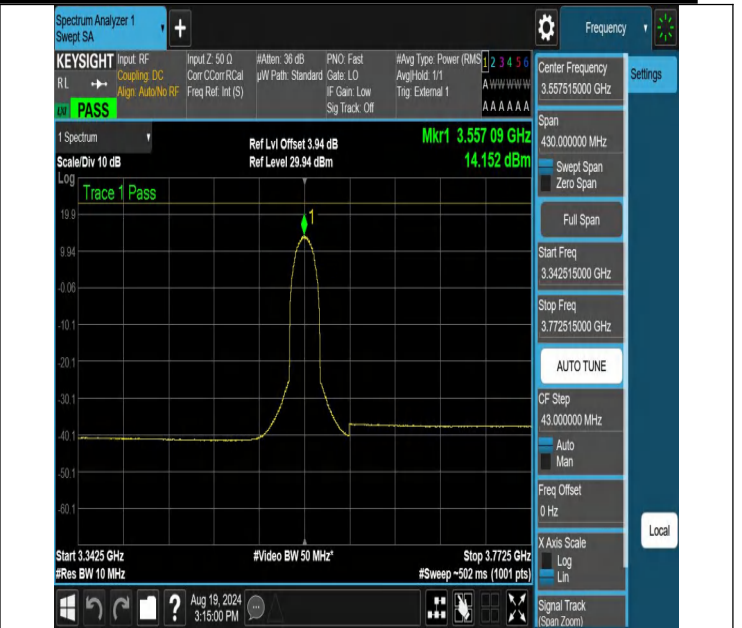
NTNV-N48-PC3-30-15-L-CP-256QAM-Outer_Full-3342.515-3772.515-Ant1-PASS
