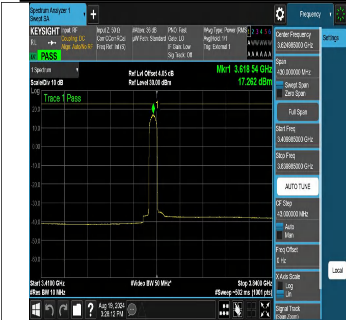
NTNV-N48-PC3-30-15-M-DFT-256QAM-Edge_1RB_Left-3409.985-3839.985-Ant1-PASS
