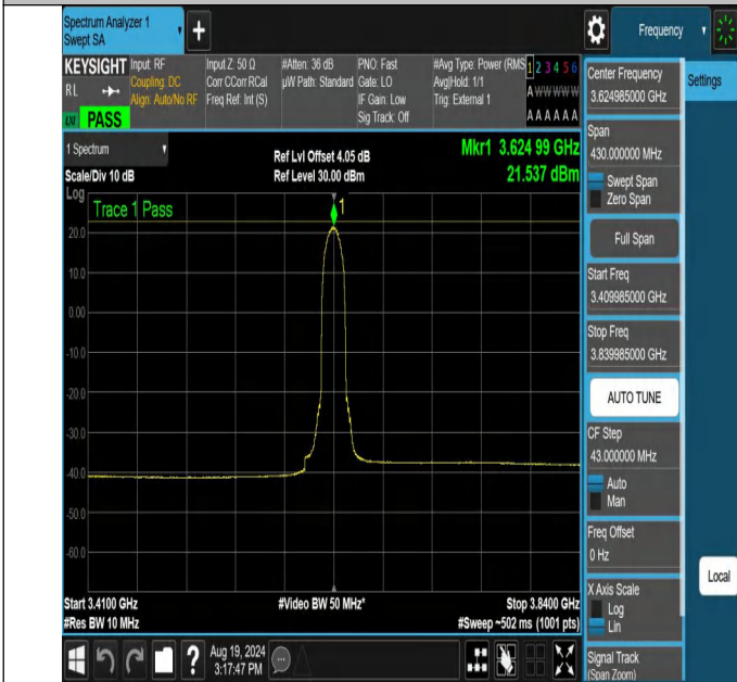
NTNV-N48-PC3-30-15-M-DFT-BPSK-Inner_Full-3409.985-3839.985-Ant1-PASS
