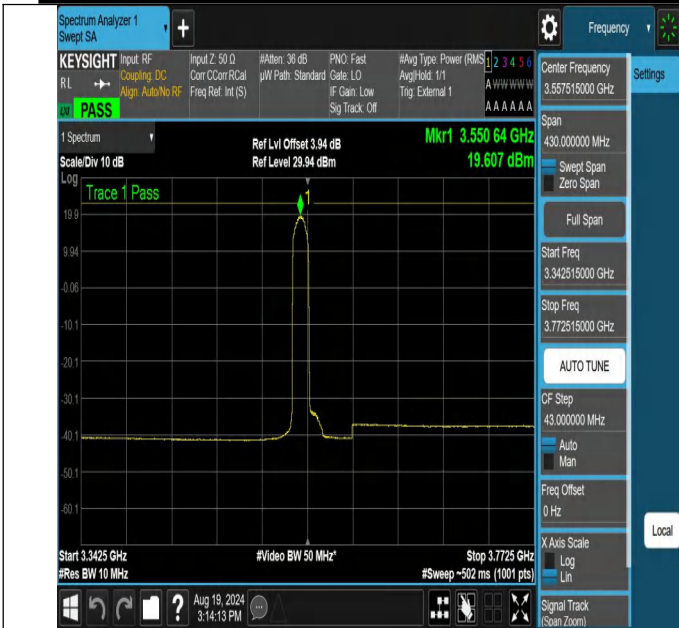
NTNV-N48-PC3-30-15-L-CP-64QAM-Edge_1RB_Left-3342.515-772.515-Ant1-PASS
