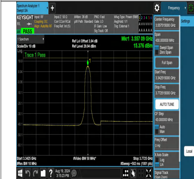
NTNV-N48-PC3-30-15-L-CP-256QAM-Inner_Full-3342.515-3772.515-Ant1-PASS
