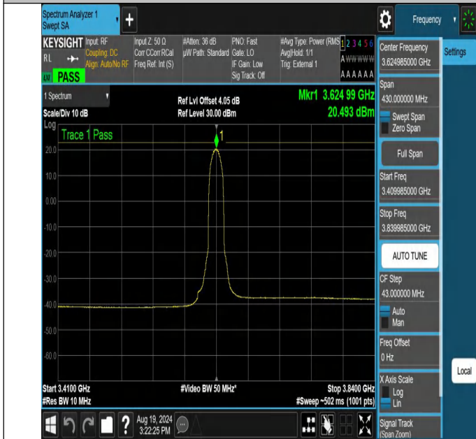
NTNV-N48-PC3-30-15-M-DFT-16QAM-Inner_Full-3409.985-3839.985-Ant1-PASS
