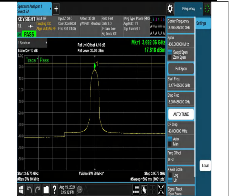
NTNV-N48-PC3-30-15-H-DFT-64QAM-Outer_Full-3477.485-3907.485-Ant1-PASS
