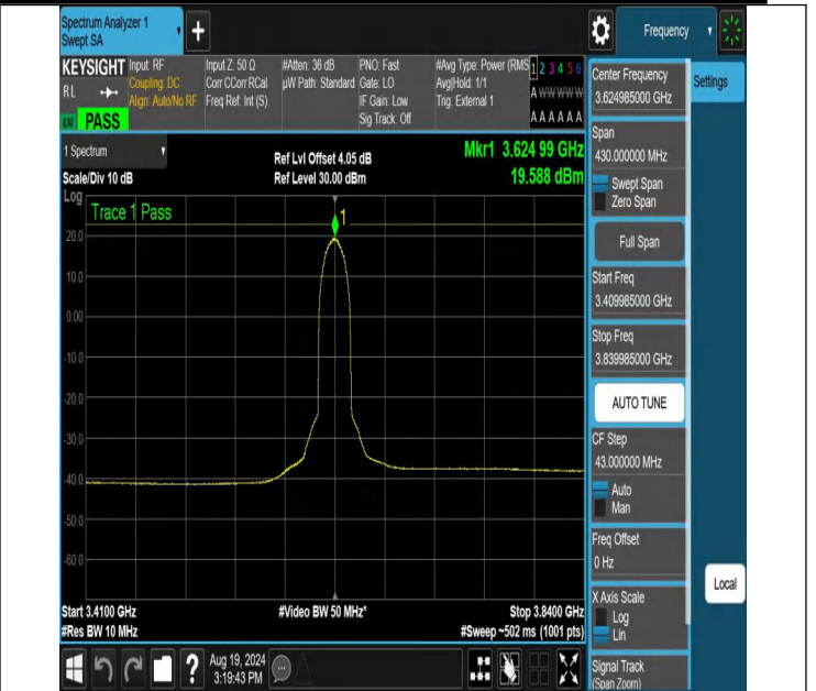
NTNV-N48-PC3-30-15-M-DFT-QPSK-Outer_Full-3409.985-3839.985-Ant1-PASS
