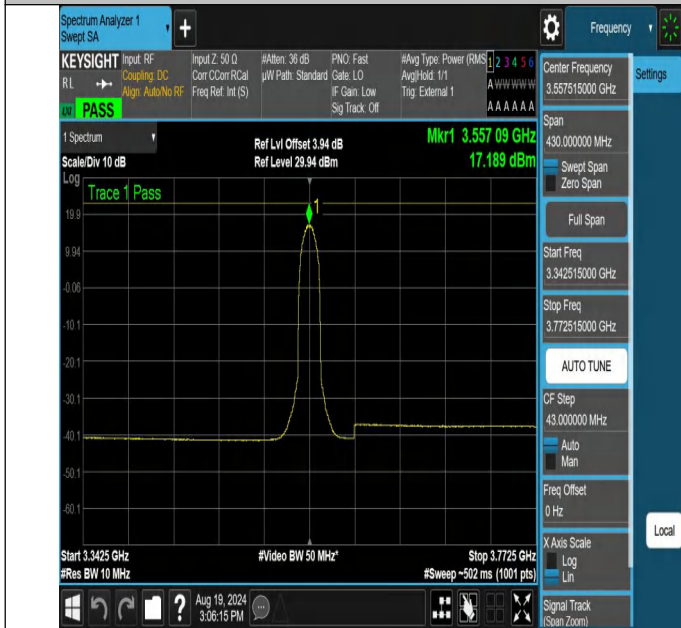
NTNV-N48-PC3-30-15-L-DFT-256QAM-Inner_Full-3342.515-3772.515-Ant1-PASS
