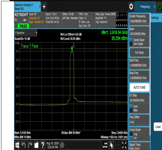
NTNV-N48-PC3-30-15-M-DFT-16QAM-Edge_1RB_Left-3409.985-3839.985-Ant1-PASS
