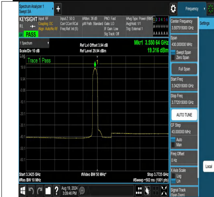
NTNV-N48-PC3-30-15-L-CP-QPSK-Edge_1RB_Left-3342.515-3772.515-Ant1-PASS
