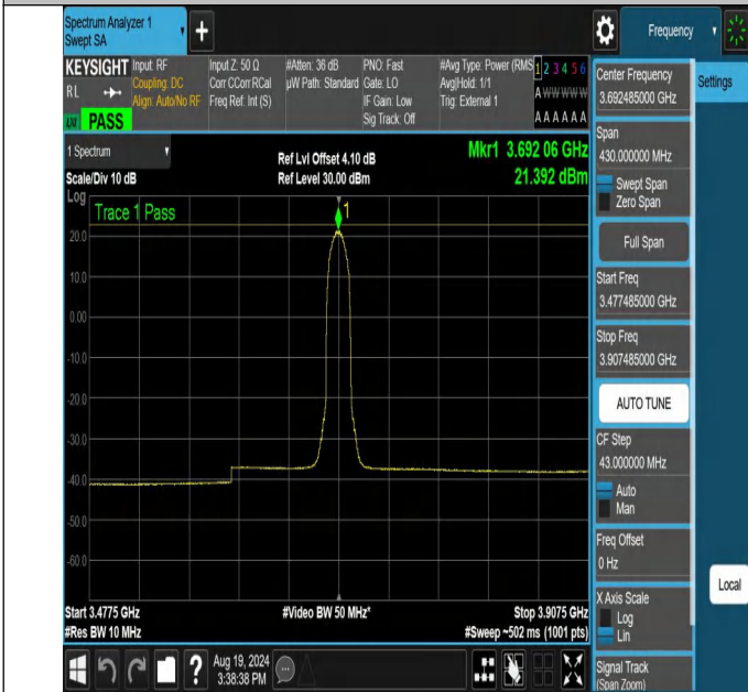
NTNV-N48-PC3-30-15-H-DFT-BPSK-Inner_Full-3477.485-3907.485-Ant1-PASS
