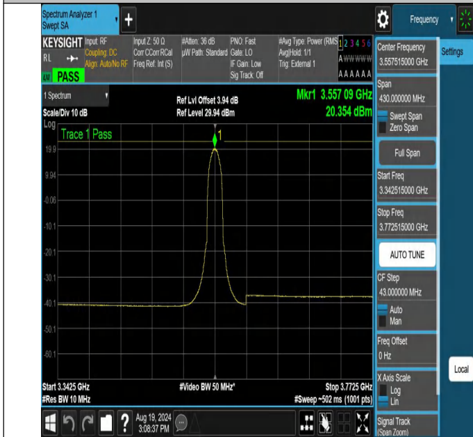
NTNV-N48-PC3-30-15-L-CP-QPSK-Inner_Full-3342.515-3772.515-Ant1-PASS
