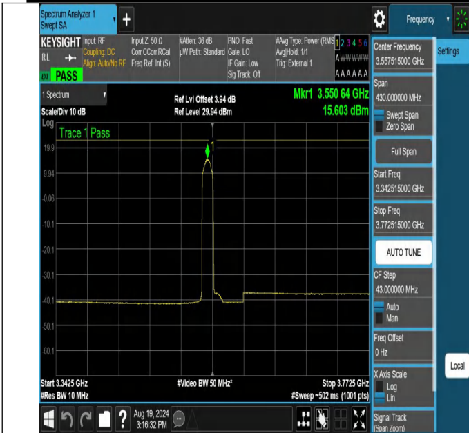
NTNV-N48-PC3-30-15-L-CP-256QAM-Edge_1RB_Left-3342.515-3772.515-Ant1-PASS
