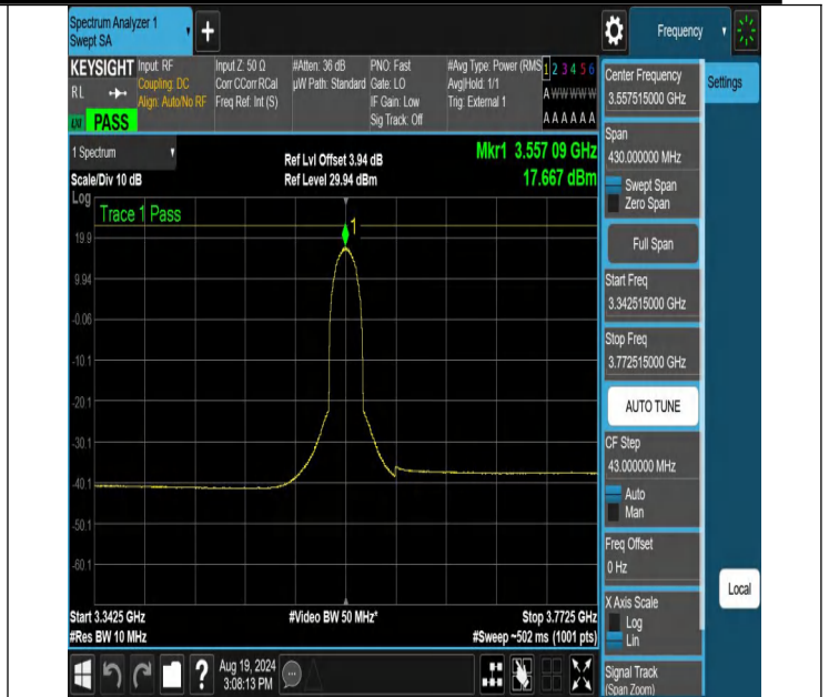
NTNV-N48-PC3-30-15-L-CP-QPSK-Outer_Full-3342.515-3772.515-Ant1-PASS
