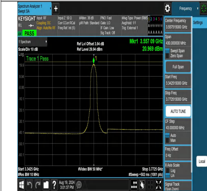
NTNV-N48-PC3-30-15-L-DFT-16QAM-Inner_Full-3342.515-3772.515-Ant1-PASS
