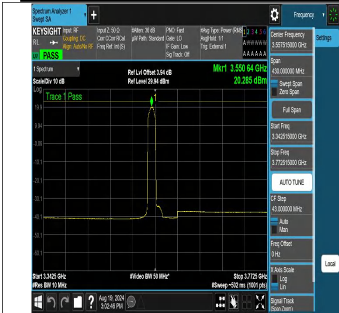
NTNV-N48-PC3-30-15-L-DFT-BPSK-Edge_1RB_Left-3342.515-3772.515-Ant1-PASS
