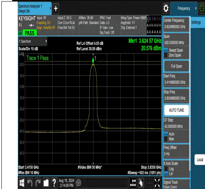
NTNV-N48-PC3-30-10-M-DFT-BPSK-Outter_Full-3414.985-3834.9 85-Ant1-PASS
