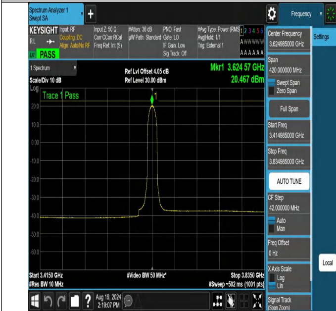
NTNV-N48-PC3-30-10-M-DFT-16QAM-Inner_Full-3414.985-3834.985-Ant1-PASS
