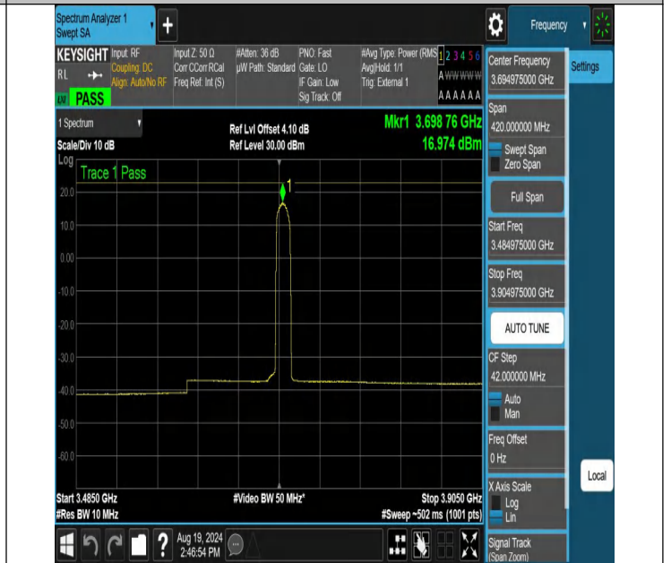
NTNV-N48-PC3-30-10-H-DFT-256QAM-Edge_1RB_Right-3484.975-3904.975-Ant1-PASS
