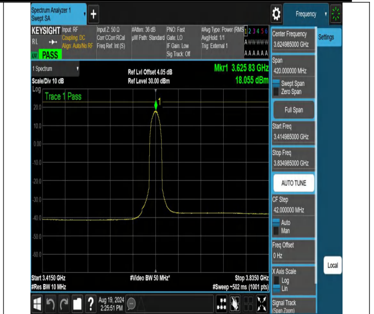
NTNV-N48-PC3-30-10-M-CP-QPSK-Outer_Full-3414.985-3834.985-85-Ant1-PASS
