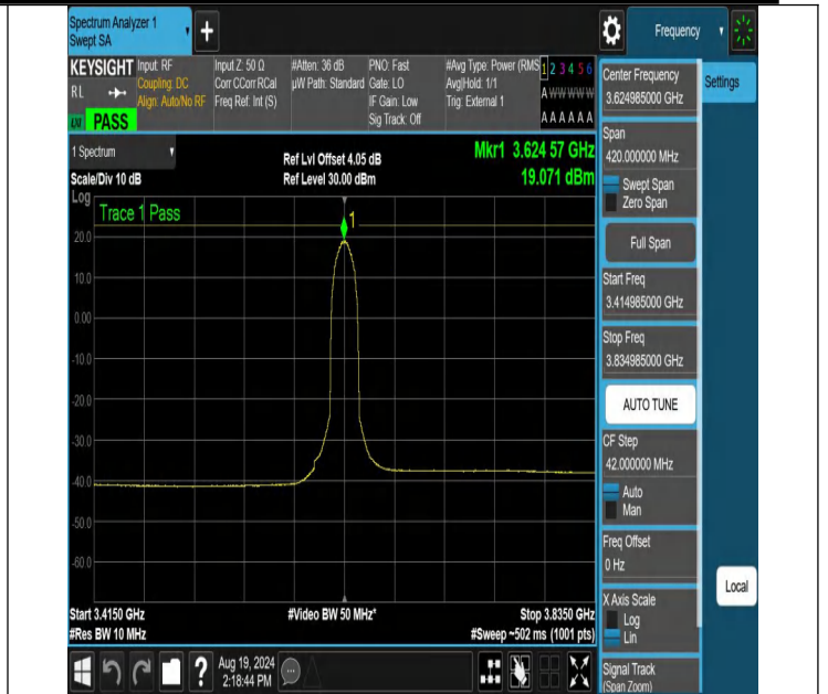
NTNV-N48-PC3-30-10-M-DFT-16QAM-Outer_Full-3414.985-3834.985-Ant1-PASS
