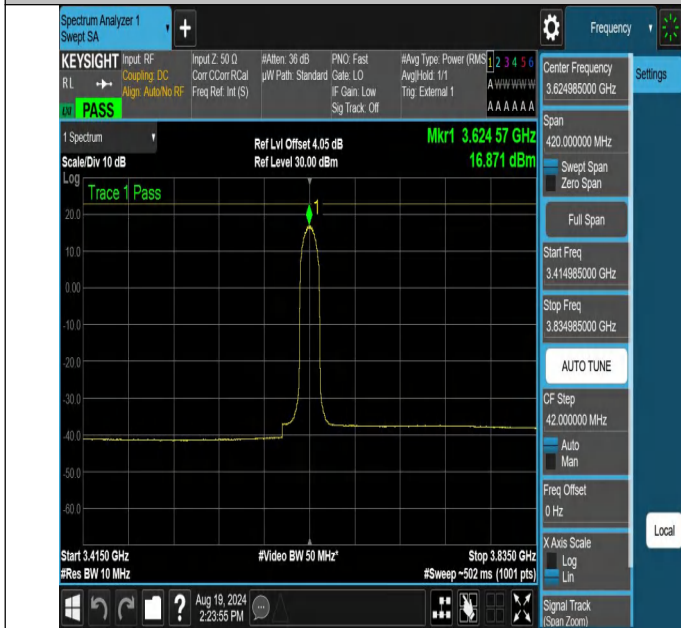
NTNV-N48-PC3-30-10-M-DFT-256QAM-Inner_Full-3414.985-3834.985-Ant1-PASS
