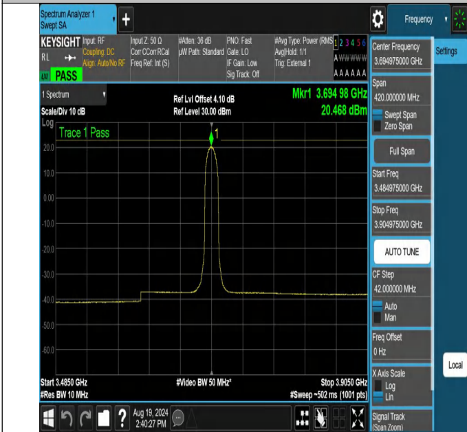
NTNV-N48-PC3-30-10-H-DFT-16QAM-Inner_Full-3484.975-3904.975-Ant1-PASS
