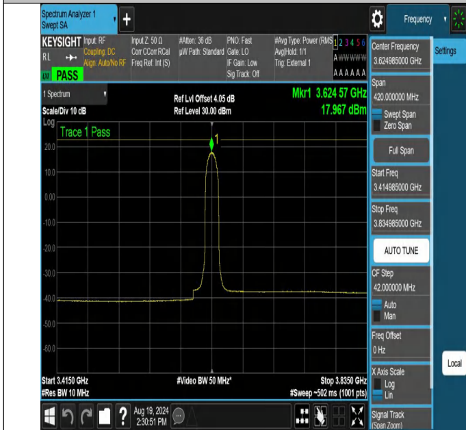
NTNV-N48-PC3-30-10-M-CP-64QAM-Inner_Full-3414.985-3834.985-85-Ant1-PASS
