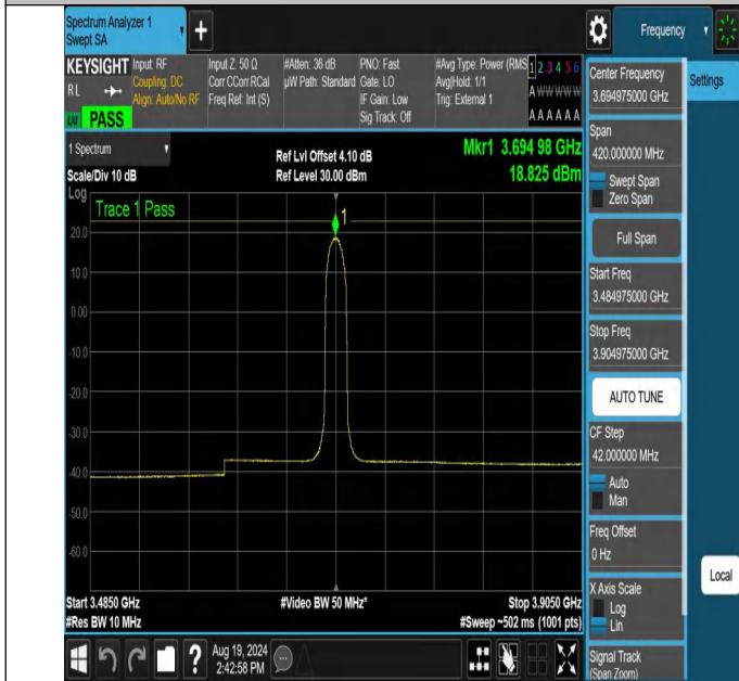
NTNV-N48-PC3-30-10-H-DFT-64QAM-Inner_Full-3484.975-3904.975-Ant1-PASS
