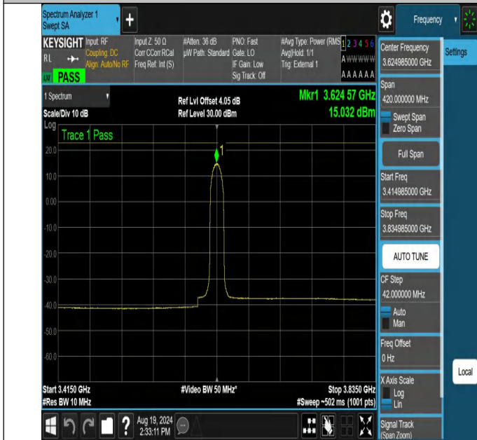
NTNV-N48-PC3-30-10-M-CP-256QAM-Inner_Full-3414.985-3834.985-Ant1-PASS
