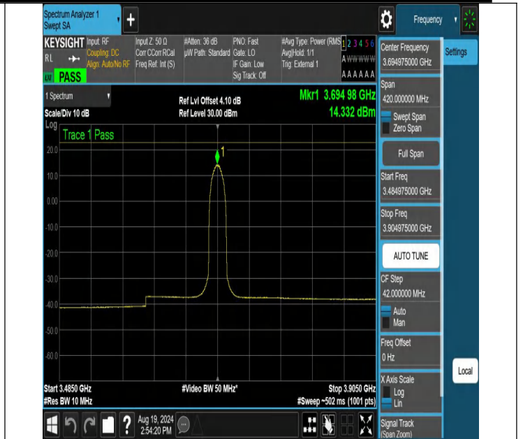
NTNV-N48-PC3-30-10-H-CP-256QAM-Outer_Full-3484.975-3904.975-Ant1-PASS
