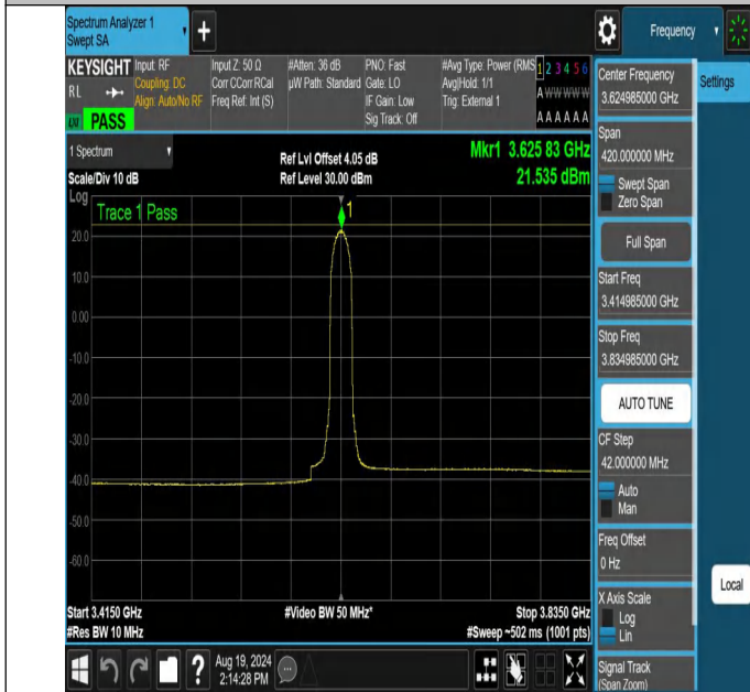
NTNV-N48-PC3-30-10-M-DFT-BPSK-Inner_Full-3414.985-3834.9 85-Ant1-PASS
