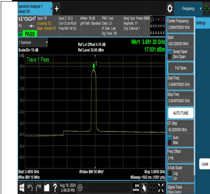
NTNV-N48-PC3-30-10-H-DFT-256QAM-Edge_1RB_Left-3484.975-3904.975-Ant1-PASS
