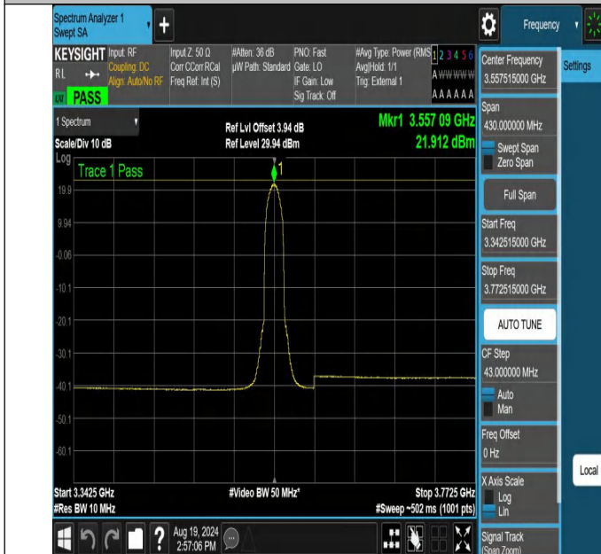
NTNV-N48-PC3-30-15-L-DFT-BPSK-Inner_Full-3342.515-3772.515-Ant1-PASS
