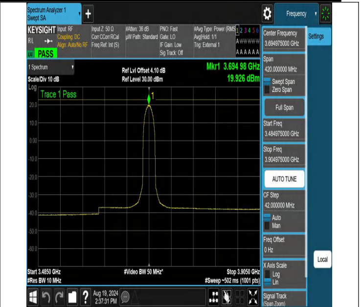
NTNV-N48-PC3-30-10-H-DFT-QPSK-Outer_Full-3484.975-3904.975-Ant1-PASS
