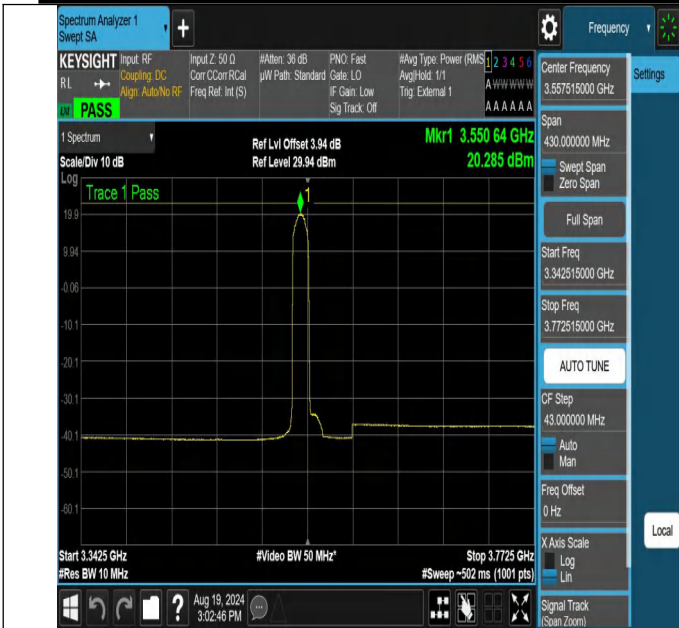
NTNV-N48-PC3-30-15-L-DFT-16QAM-Edge_1RB_Left-3342.515-3772.515-Ant1-PASS
