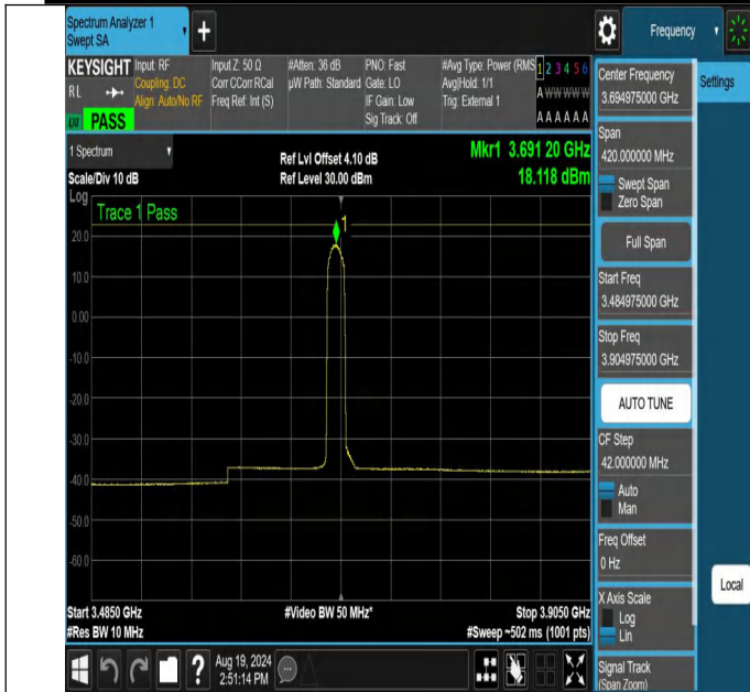
NTNV-N48-PC3-30-10-H-CP-16QAM-Edge_1RB_Left-3484.975-3904.975-Ant1-PASS
