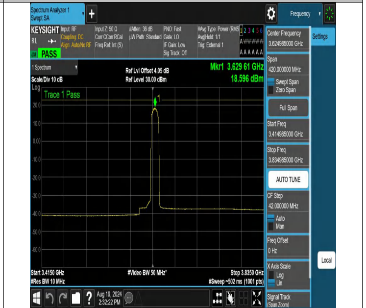
NTNV-N48-PC3-30-10-M-CP-64QAM-Edge_1RB_Right-3414.985-3834.985-Ant1-PASS
