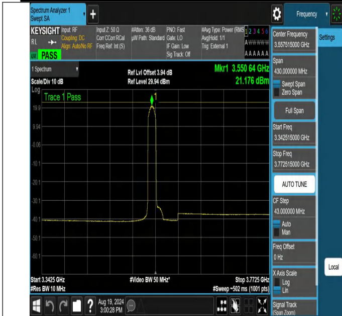
NTNV-N48-PC3-30-15-L-DFT-QPSK-Edge_1RB_Left-3342.515-3772.515-Ant1-PASS
