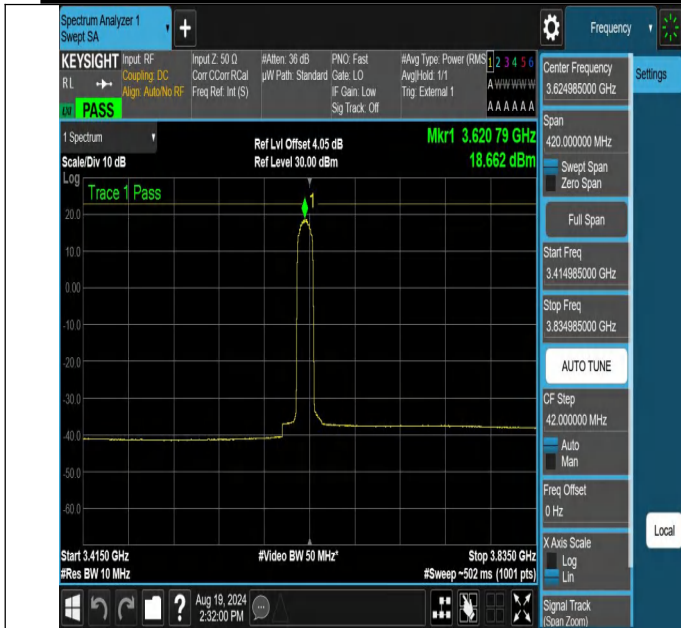
NTNV-N48-PC3-30-10-M-CP-64QAM-Edge_1RB_Left-3414.985-3834.985-Ant1-PASS
