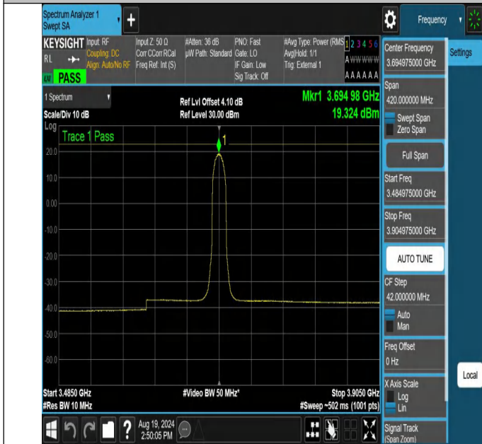
NTNV-N48-PC3-30-10-H-CP-16QAM-Inner_Full-3484.975-3904.975-75-Ant1-PASS
