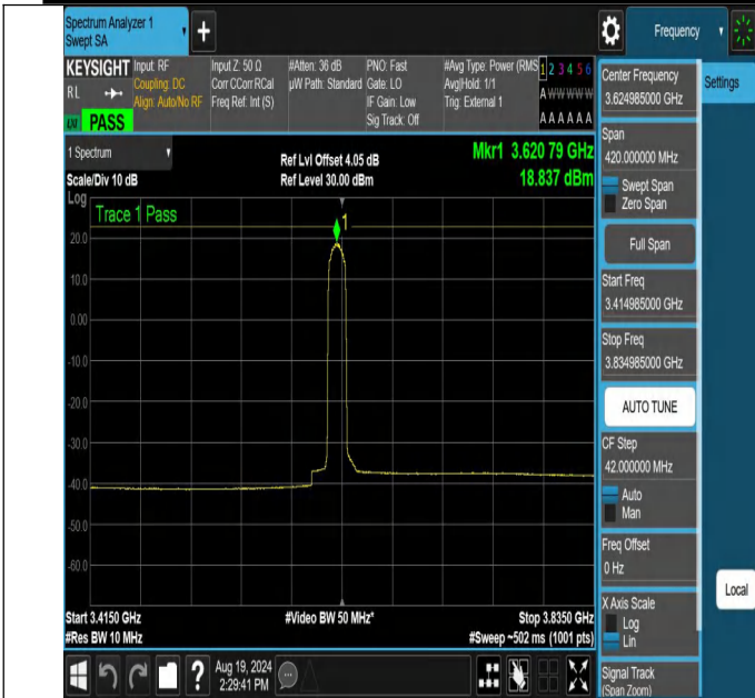
NTNV-N48-PC3-30-10-M-CP-16QAM-Edge_1RB_Left-3414.985-3834.985-Ant1-PASS
