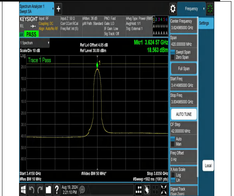
NTNV-N48-PC3-30-10-M-DFT-64QAM-Outer_Full-3414.985-3834.985-Ant1-PASS
