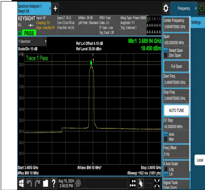
NTNV-N48-PC3-30-10-H-CP-QPSK-Edge_1RB_Left-3484.975-3904.975-Ant1-PASS
