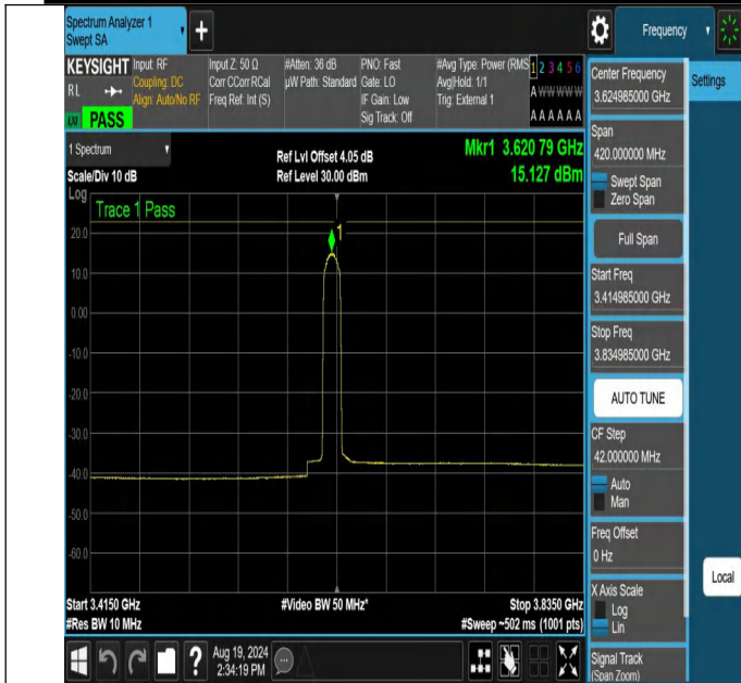
NTNV-N48-PC3-30-10-M-CP-256QAM-Edge_1RB_Left-3414.985-3834.985-Ant1-PASS
