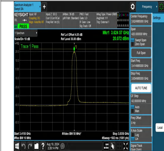
NTNV-N48-PC3-30-10-M-CP-QPSK-Inner_Full-3414.985-3834.985-5-Ant1-PASS
