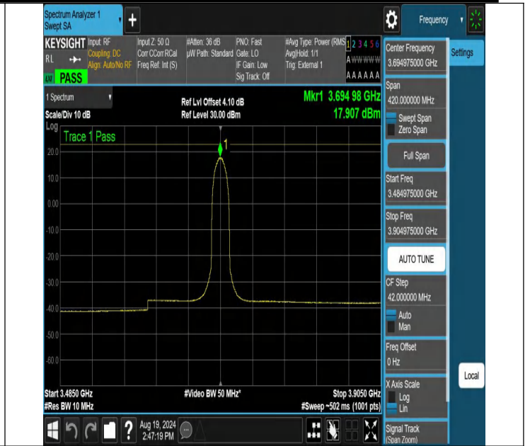
NTNV-N48-PC3-30-10-H-CP-QPSK-Outer_Full-3484.975-3904.975-Ant1-PASS
