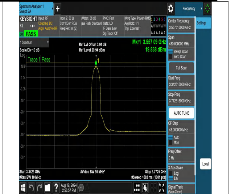
NTNV-N48-PC3-30-15-L-DFT-QPSK-Outer_Full-3342.515-3772.515-Ant1-PASS
