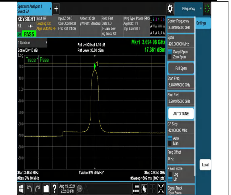
NTNV-N48-PC3-30-10-H-CP-64QAM-Outer_Full-3484.975-3904.975-Ant1-PASS
