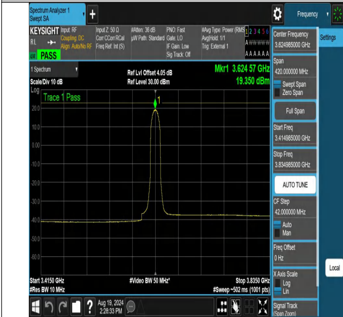
NTNV-N48-PC3-30-10-M-CP-16QAM-Inner_Full-3414.985-3834.985-85-Ant1-PASS
