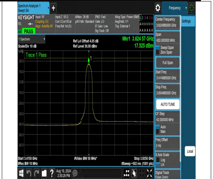
NTNV-N48-PC3-30-10-M-CP-64QAM-Outer_Full-3414.985-3834.985-Ant1-PASS
