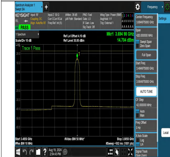
NTNV-N48-PC3-30-10-H-CP-256QAM-Inner_Full-3484.975-3904.975-Ant1-PASS
