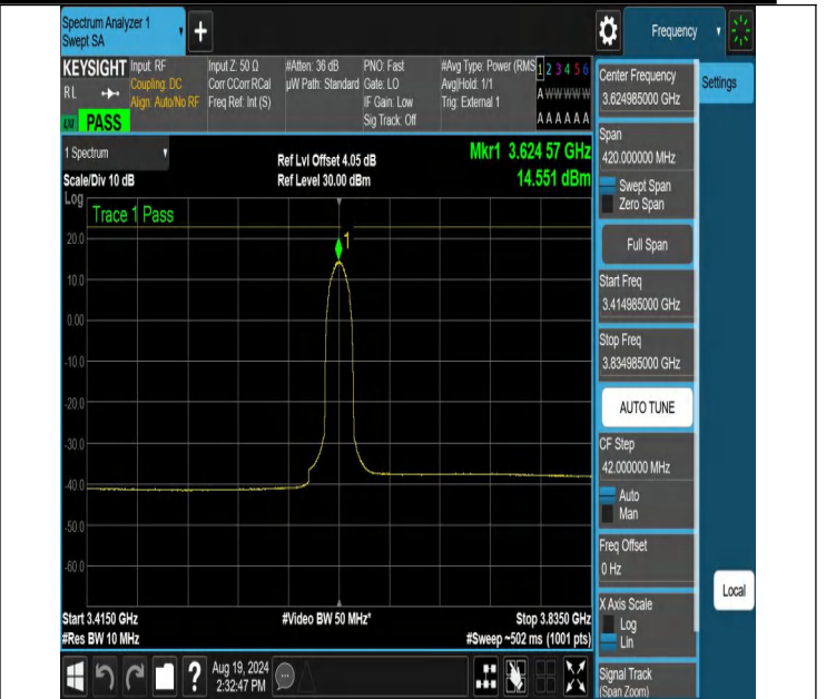
NTNV-N48-PC3-30-10-M-CP-256QAM-Outer_Full-3414.985-3834.985-Ant1-PASS
