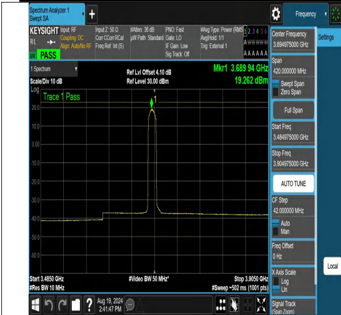
NTNV-N48-PC3-30-10-H-DFT-16QAM-Edge_1RB_Left-3484.975-3904.975-Ant1-PASS
