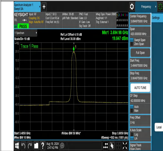
NTNV-N48-PC3-30-10-H-CP-QPSK-Inner_Full-3484.975-3904.975-Ant1-PASS
