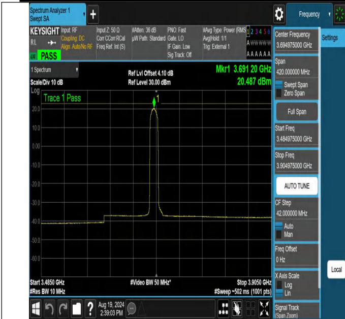
NTNV-N48-PC3-30-10-H-DFT-QPSK-Edge_1RB_Left-3484.975-3904.975-Ant1-PASS
