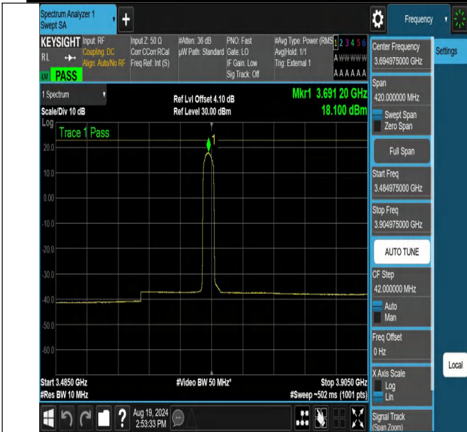
NTNV-N48-PC3-30-10-H-CP-64QAM-Edge_1RB_Left-3484.975-3904.975-Ant1-PASS
