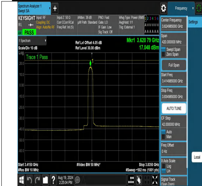
NTNV-N48-PC3-30-10-M-DFT-256QAM-Edge_1RB_Left-3414.985-3834.985-Ant1-PASS
