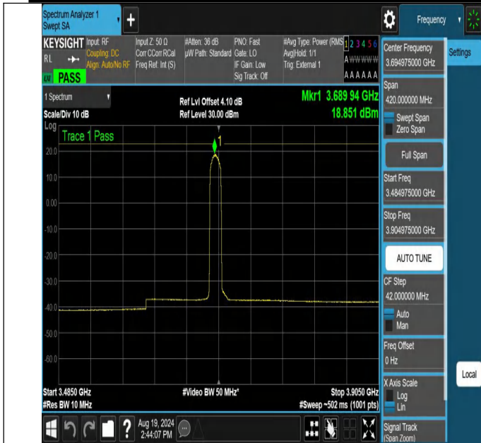
NTNV-N48-PC3-30-10-H-DFT-64QAM-Edge_1RB_Left-3484.975-3904.975-Ant1-PASS
