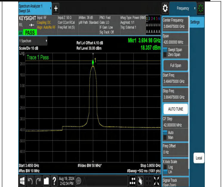
NTNV-N48-PC3-30-10-H-DFT-64QAM-Outer_Full-3484.975-3904.975-Ant1-PASS
