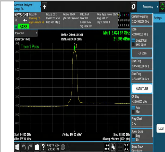
NTNV-N48-PC3-30-10-M-DFT-QPSK-Inner_Full-3414.985-3834.985-Ant1-PASS
