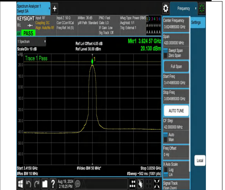
NTNV-N48-PC3-30-10-M-DFT-QPSK-Outer_Full-3414.985-3834.985-Ant1-PASS
