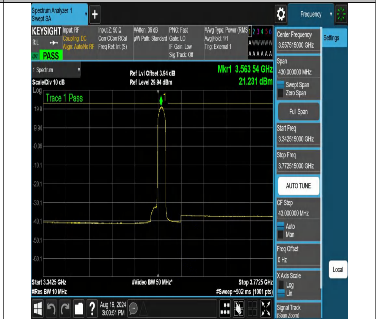
NTNV-N48-PC3-30-15-L-DFT-QPSK-Edge_1RB_Right-3342.515-3772.515-Ant1-PASS
