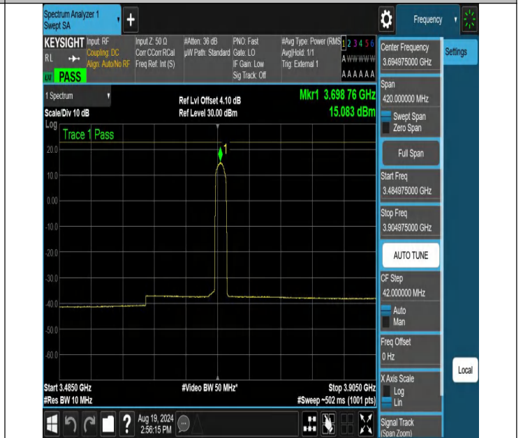
NTNV-N48-PC3-30-10-H-CP-256QAM-Edge_1RB_Right-3484.975-3904.975-Ant1-PASS
