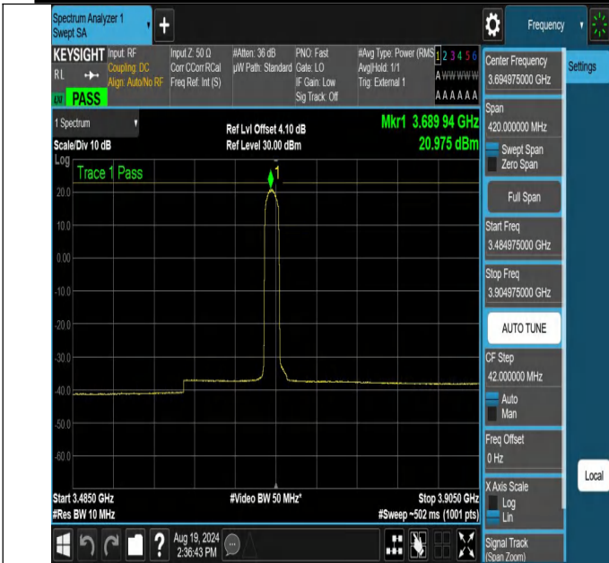
NTNV-N48-PC3-30-10-H-DFT-BPSK-Edge_1RB_Left-3484.975-3904.975-Ant1-PASS
