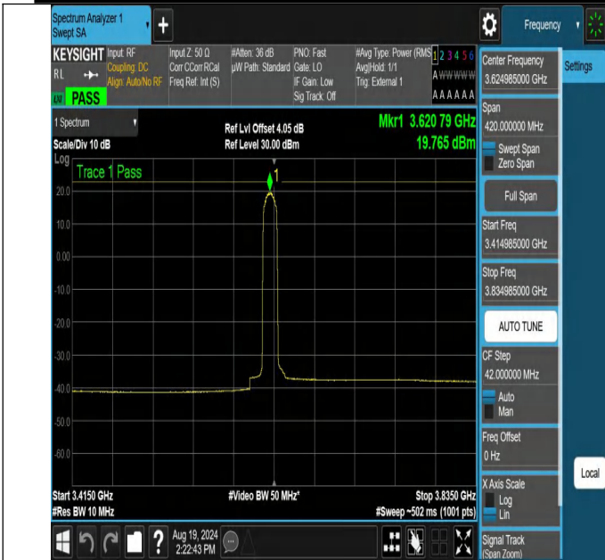
NTNV-N48-PC3-30-10-M-DFT-64QAM-Edge_1RB_Left-3414.985-3834.985-Ant1-PASS
