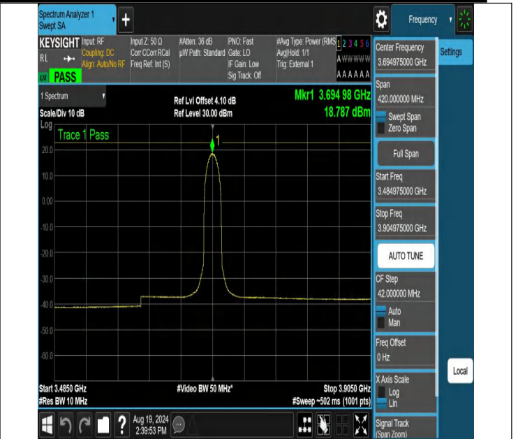
NTNV-N48-PC3-30-10-H-DFT-16QAM-Outer_Full-3484.975-3904.975-Ant1-PASS
