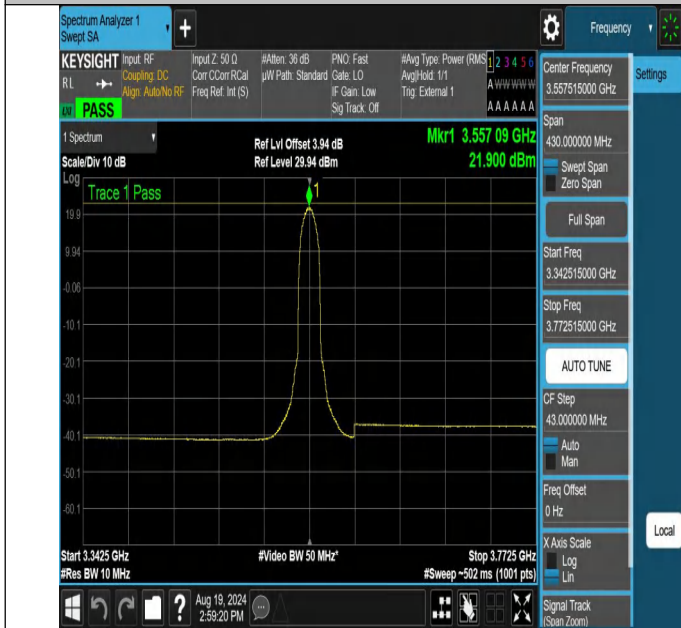
NTNV-N48-PC3-30-15-L-DFT-QPSK-Inner_Full-3342.515-3772.515-Ant1-PASS
