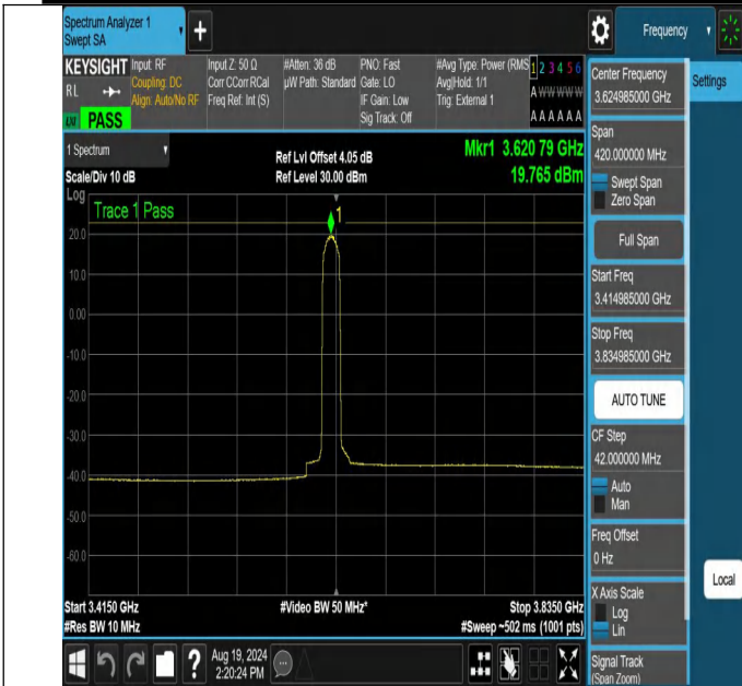
NTNV-N48-PC3-30-10-M-DFT-16QAM-Edge_1RB_Left-3414.985-3834.985-Ant1-PASS
