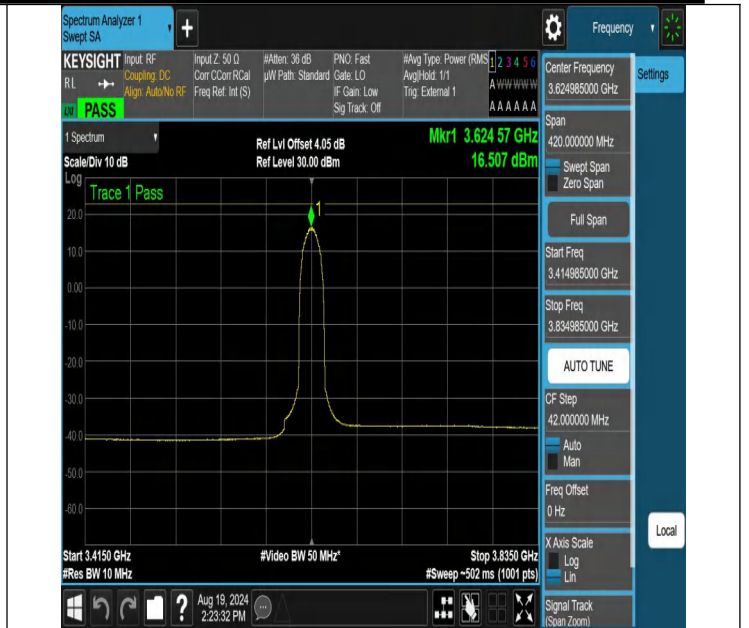
NTNV-N48-PC3-30-10-M-DFT-256QAM-Outer_Full-3414.985-3834.985-Ant1-PASS
