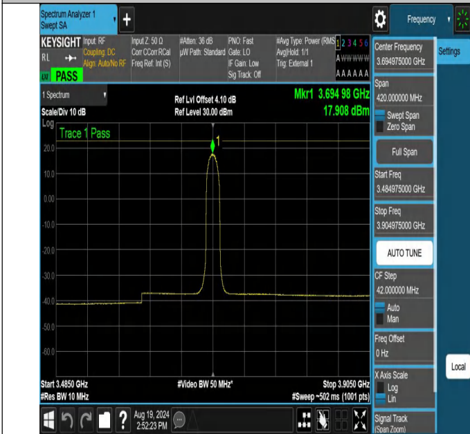
NTNV-N48-PC3-30-10-H-CP-64QAM-Inner_Full-3484.975-3904.975-75-Ant1-PASS
