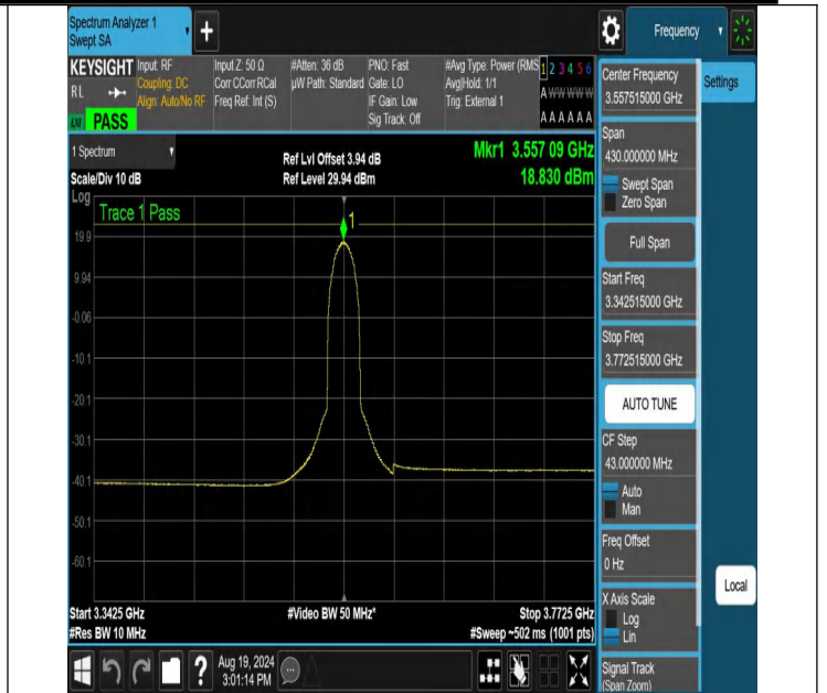
NTNV-N48-PC3-30-15-L-DFT-16QAM-Outer_Full-3342.515-3772.515-Ant1-PASS
