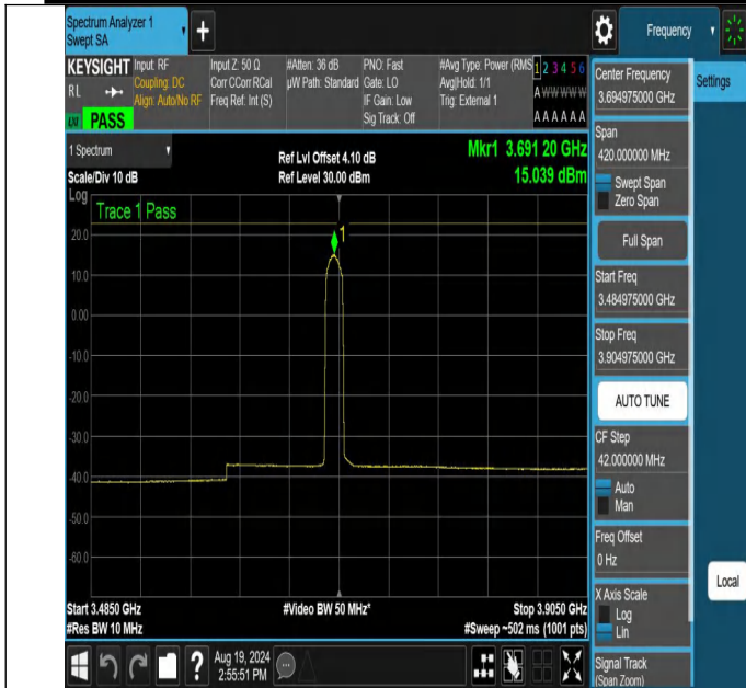
NTNV-N48-PC3-30-10-H-CP-256QAM-Edge_1RB_Left-3484.975-3904.975-Ant1-PASS
