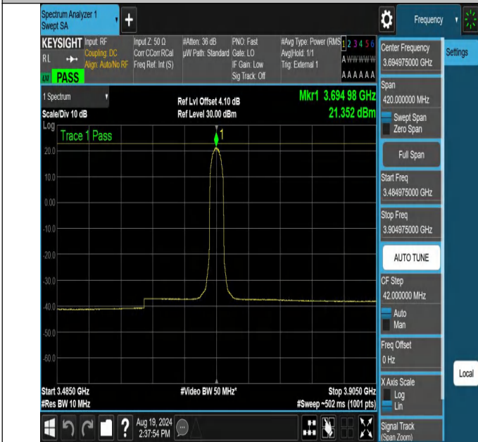
NTNV-N48-PC3-30-10-H-DFT-QPSK-Inner_Full-3484.975-3904.975-Ant1-PASS
