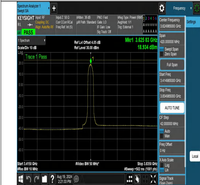
NTNV-N48-PC3-30-10-M-DFT-64QAM-Inner_Full-3414.985-3834.985-Ant1-PASS
