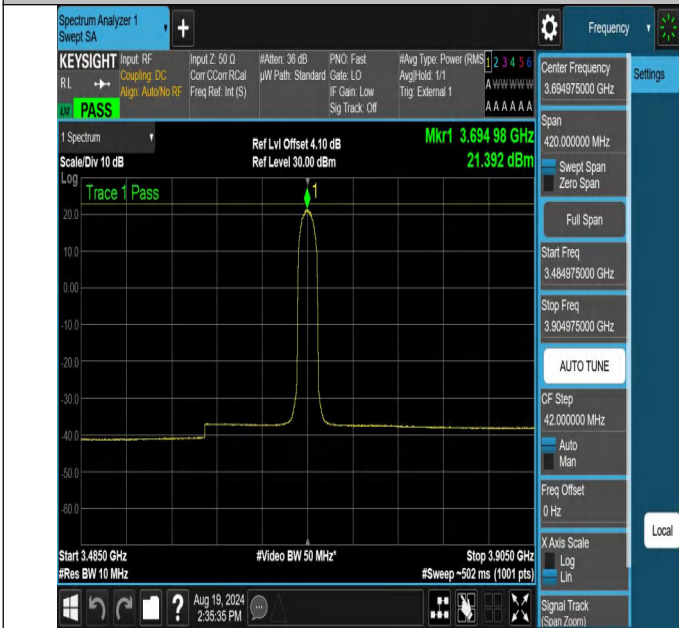
NTNV-N48-PC3-30-10-H-DFT-BPSK-Inner_Full-3484.975-3904.975-Ant1-PASS
