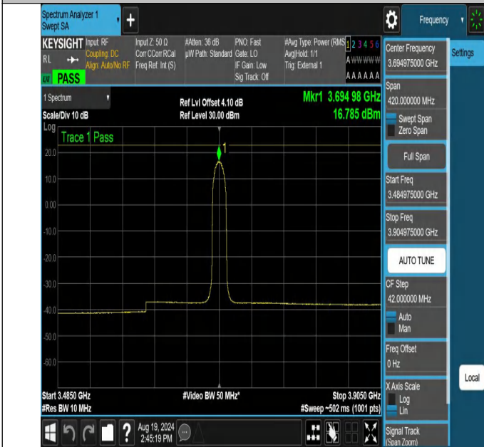
NTNV-N48-PC3-30-10-H-DFT-256QAM-Inner_Full-3484.975-3904.975-Ant1-PASS
