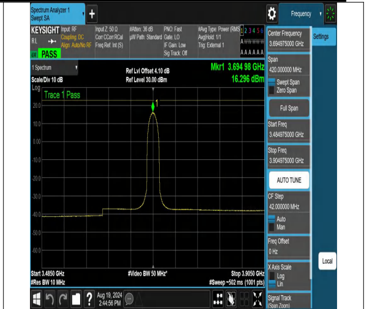
NTNV-N48-PC3-30-10-H-DFT-256QAM-Outer_Full-3484.975-3904.975-Ant1-PASS
