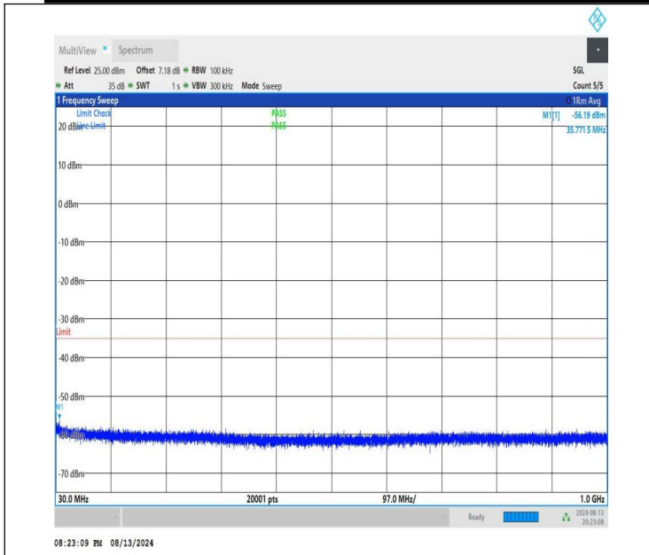
NTNV-n41-PC1.5-30-70-M-CP-QPSK-Edge_1RB_Right-30-1000-PASS
