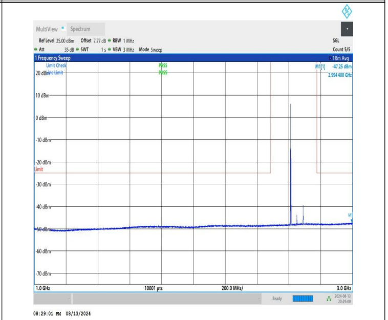
NTNV-n41-PC1.5-30-80-H-CP-QPSK-Edge_1RB_Left-1000-3000-PASS
