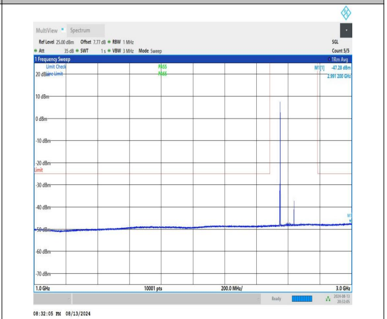
NTNV-n41-PC1.5-30-90-M-CP-QPSK-Edge_1RB_Left-1000-3000-P PASS
