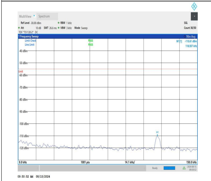
NTVN-n41-PC1.5-30-80-L-CP-QPSK-Edge_1RB_Right-0.009-0.1 5-PASS
