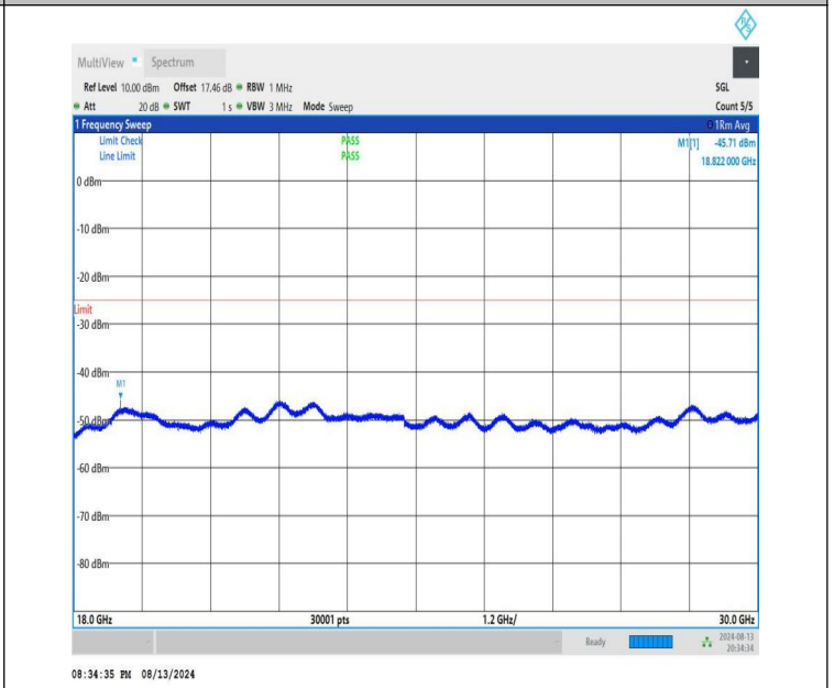
NTNV-n41-PC1.5-30-90-H-CP-QPSK-Edge_1RB_Right-18000-30000-PASS
