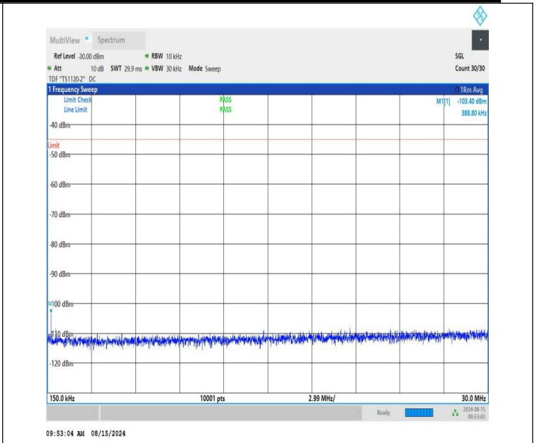
NTNV-n41-PC1.5-30-100-L-CP-QPSK-Edge_1RB_Left-0.15-30-PA SS
