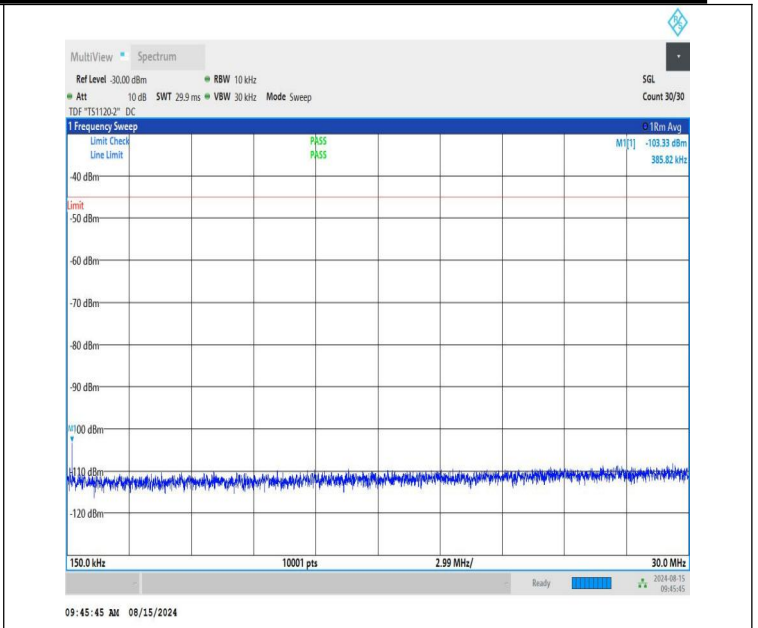
NTNV-n41-PC1.5-30-30-H-CP-QPSK-Edge_1RB_Left-0.15-30-PASS
