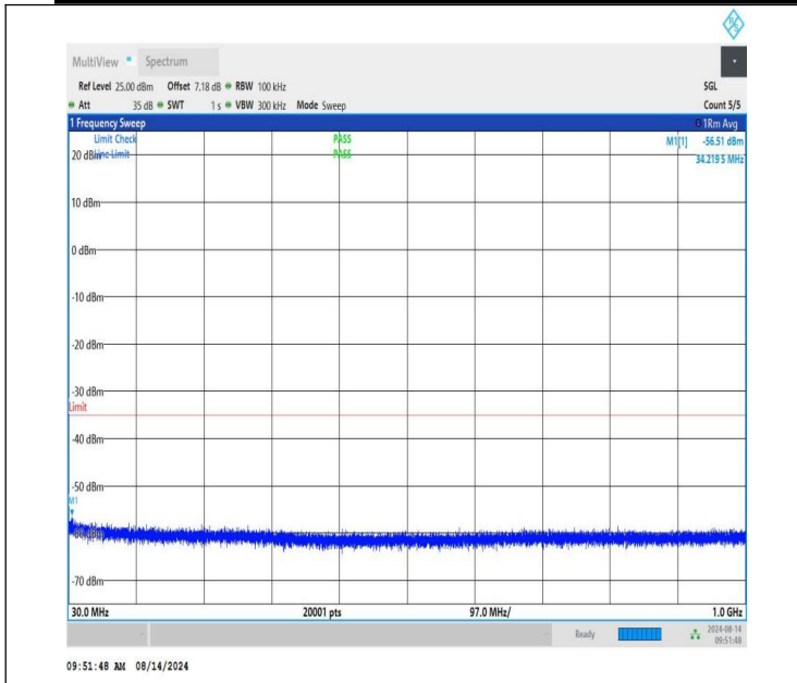
NTNV-n41-PC1.5-30-30-H-CP-QPSK-Edge_1RB_Right-30-1000-PASS
