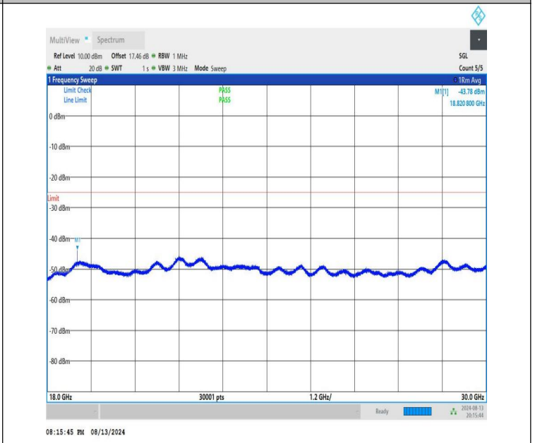
NTNV-n41-PC1.5-30-50-H-CP-QPSK-Edge_1RB_Right-18000-30000-PASS
