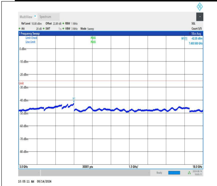
NTNV-n41-PC1.5-30-40-H-CP-QPSK-Edge_1RB_Left-3000-1800 0-PASS
