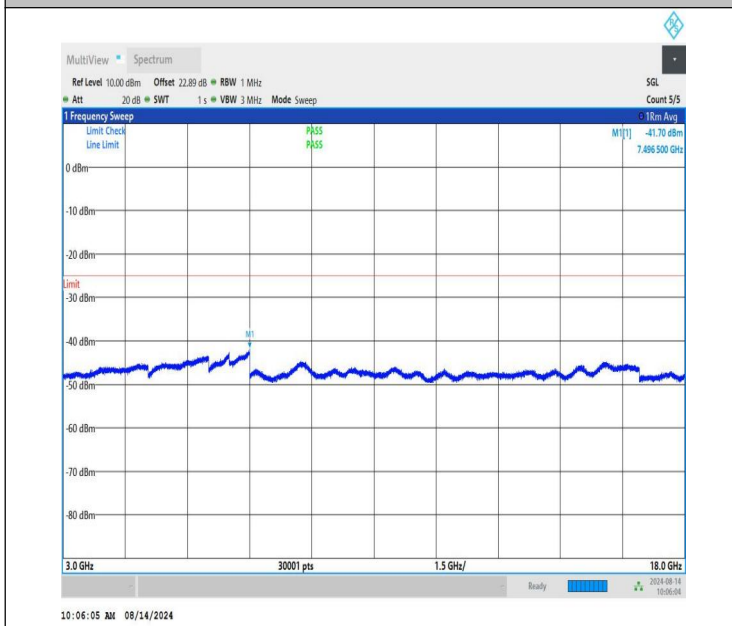
NTNV-n41-PC1.5-30-50-L-CP-QPSK-Edge_1RB_Right-3000-180 00-PASS
