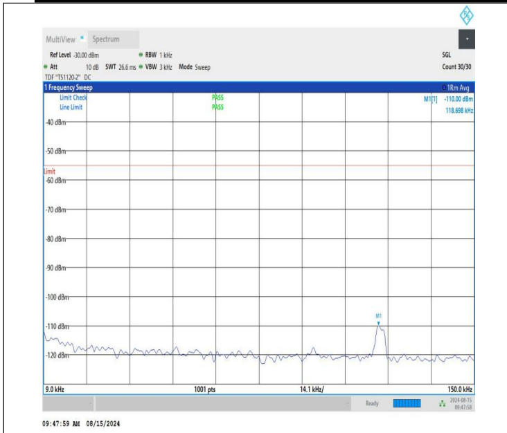
NTNV-n41-PC1.5-30-50-H-CP-QPSK-Edge_1RB_Left-0.09-0.15-PASS
