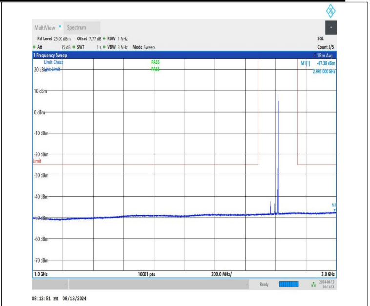
NTNV-n41-PC1.5-30-50-M-CP-QPSK-Edge_1RB_Right-1000-3000-PASS
