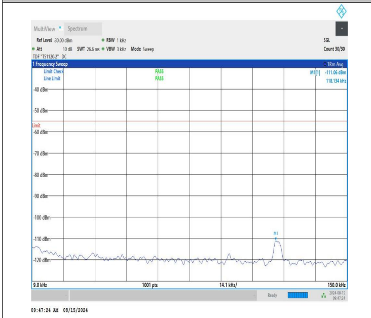
NTVN-n41-PC1.5-30-50-L-CP-QPSK-Edge_1RB_Right-0.009-0.1 5-PASS
