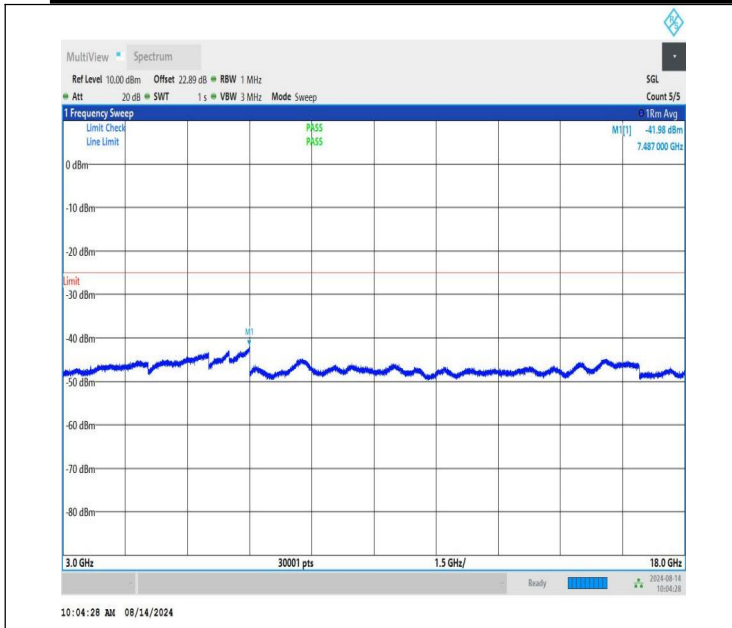
NTNV-n41-PC1.5-30-40-M-CP-QPSK-Edge_1RB_Left-3000-1800 0-PASS
