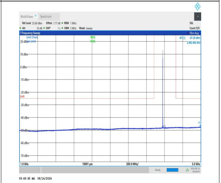
NTNV-n41-PC1.5-30-30-M-CP-QPSK-Edge_1RB_Left-1000-3000-P PASS
