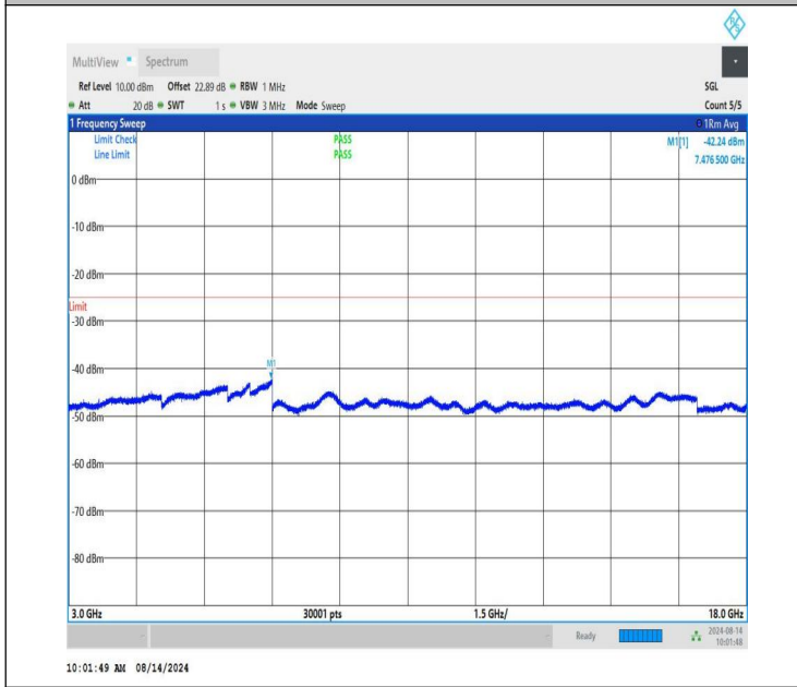
NTNV-n41-PC1.5-30-30-L-CP-QPSK-Edge_1RB_Right-3000-180 00-PASS
