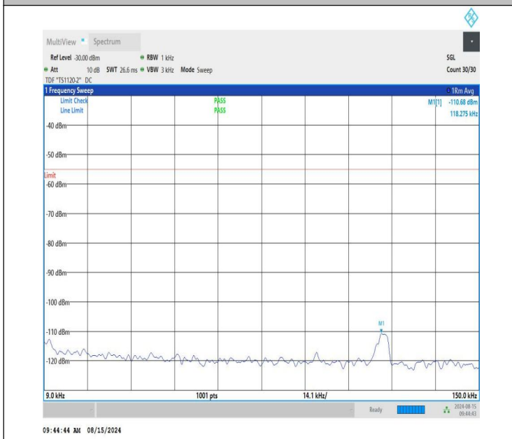
NTNV-n41-PC1.5-30-20-H-CP-QPSK-Edge_1RB_Right-0.009-0.1 5-PASS
