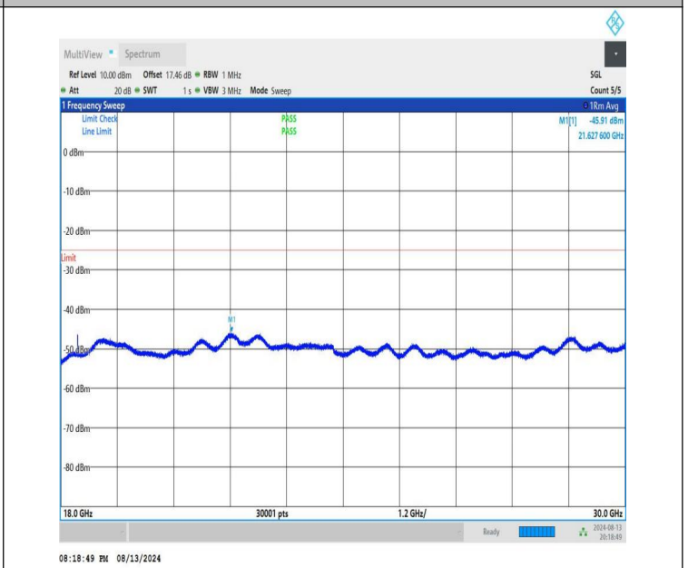
NTNV-n41-PC1.5-30-60-M-CP-QPSK-Edge_1RB_Right-18000-30000-PASS
