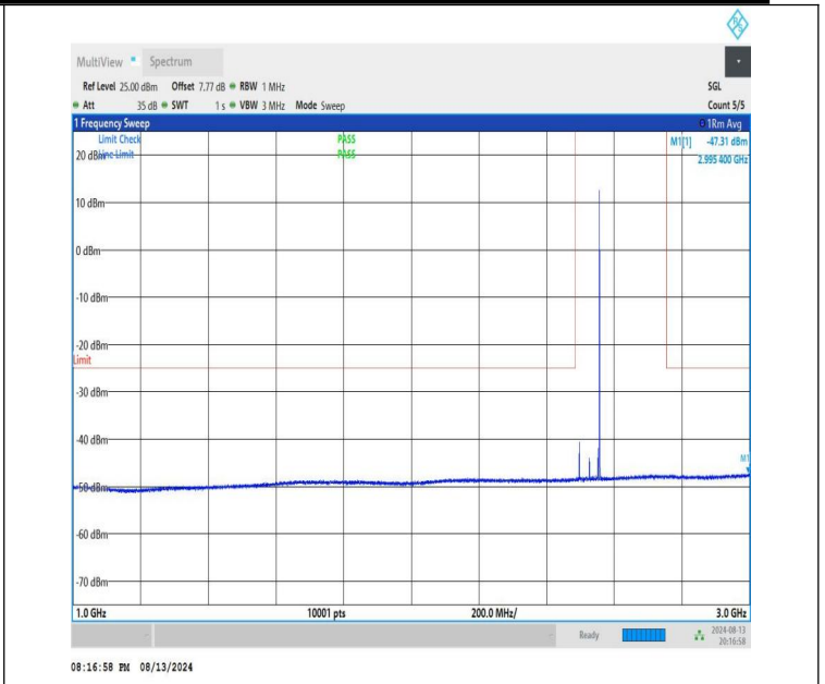
NTNV-n41-PC1.5-30-60-L-CP-QPSK-Edge_1RB_Right-1000-3000- PASS
