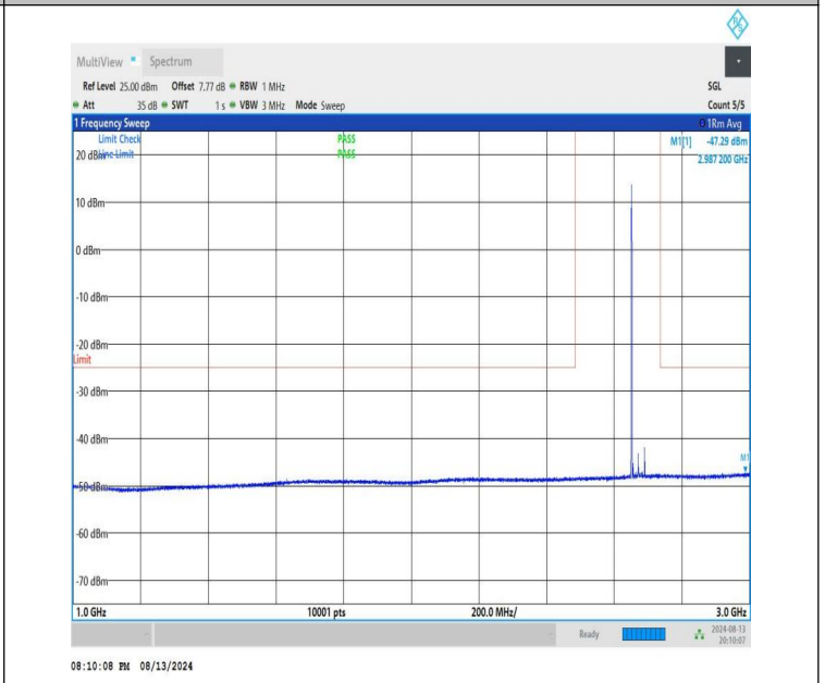
NTNV-n41-PC1.5-30-40-H-CP-QPSK-Edge_1RB_Left-1000-3000-PASS
