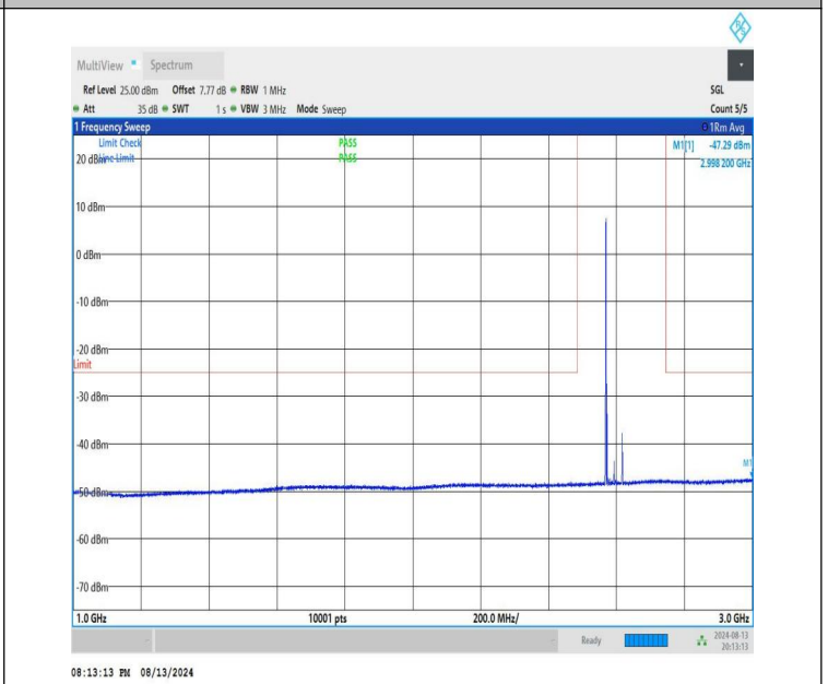
NTNV-n41-PC1.5-30-50-M-CP-QPSK-Edge_1RB_Left-1000-3000-P PASS
