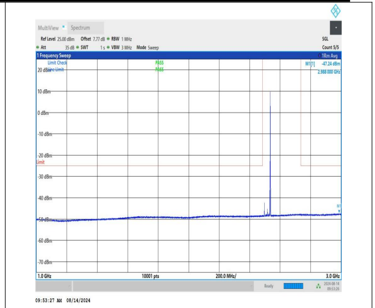
NTNV-n41-PC1.5-30-40-L-CP-QPSK-Edge_1RB_Right-1000-3000- PASS
