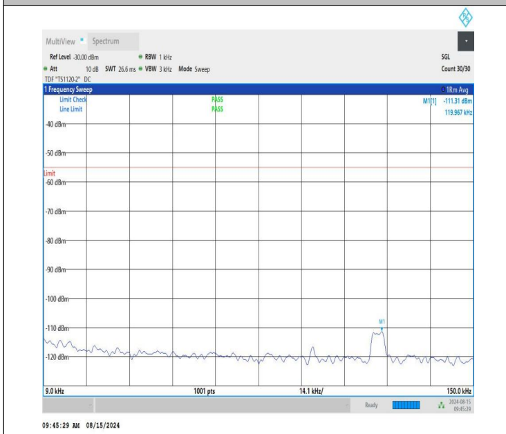
NTNV-n41-PC1.5-30-30-M-CP-QPSK-Edge_1RB_Right-0.009-0.1 5-PASS
