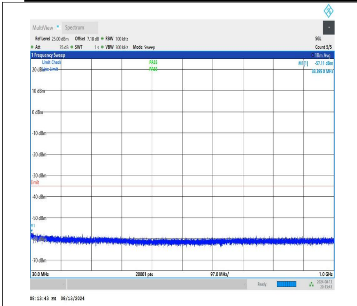
NTNV-n41-PC1.5-30-50-M-CP-QPSK-Edge_1RB_Right-30-1000-PASS
