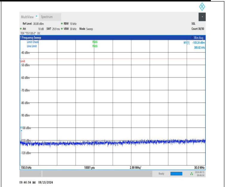
NTNV-n41-PC1.5-30-40-H-CP-QPSK-Edge_1RB_Left-0.15-30-PASS
