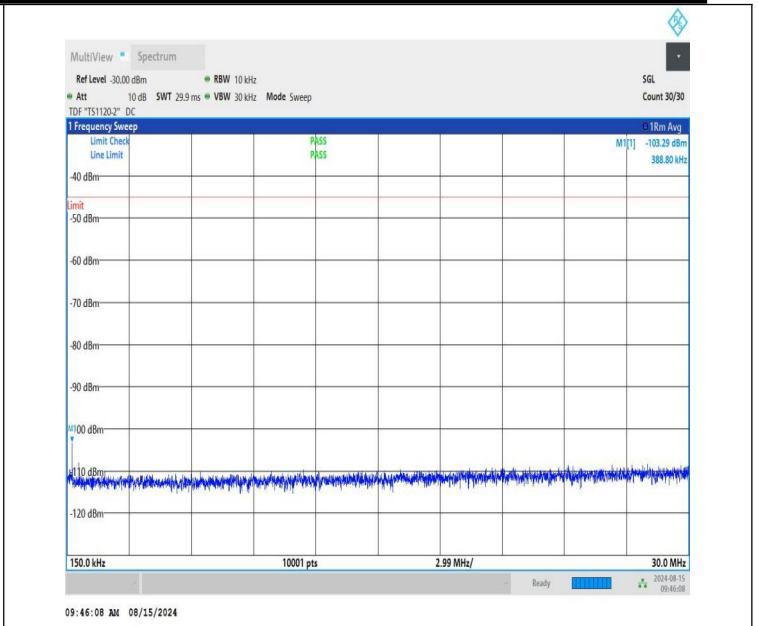
NTNV-n41-PC1.5-30-40-L-CP-QPSK-Edge_1RB_Left-0.15-30-PASS
