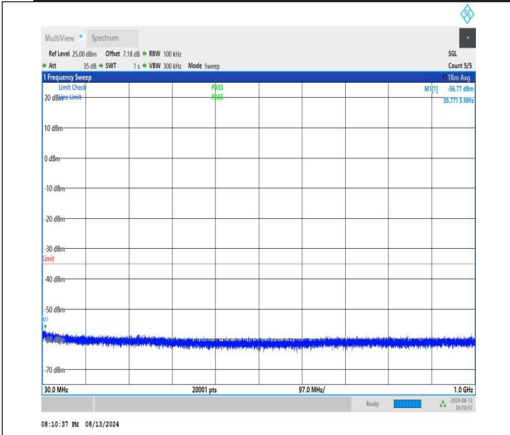
NTNV-n41-PC1.5-30-40-H-CP-QPSK-Edge_1RB_Right-30-1000-PASS
