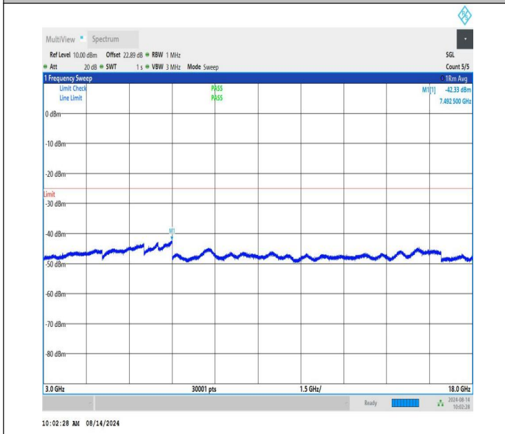
NTNV-n41-PC1.5-30-30-M-CP-QPSK-Edge_1RB_Right-3000-18000-PASS
