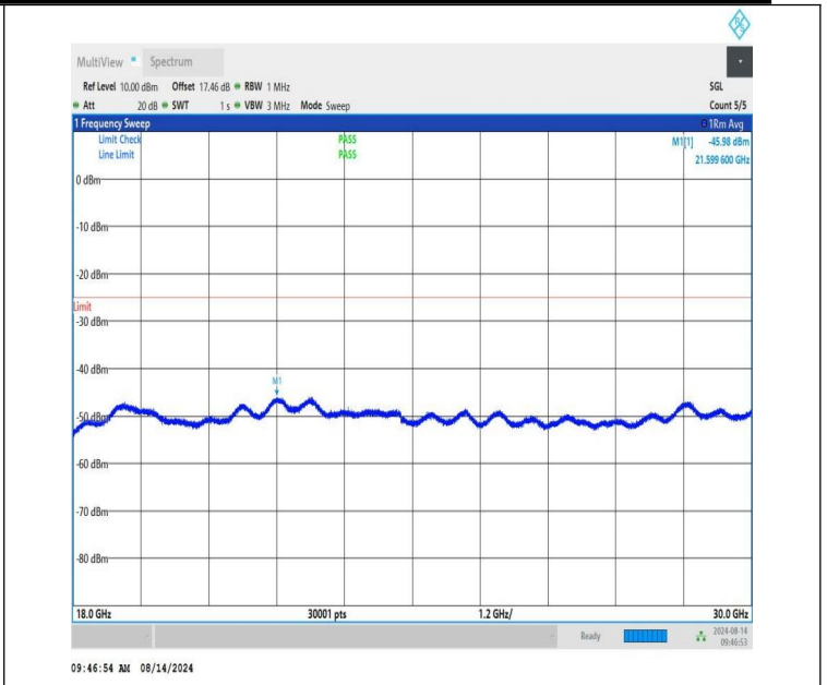
NTNV-n41-PC1.5-30-20-H-CP-QPSK-Edge_1RB_Left-18000-3000 0-PASS
