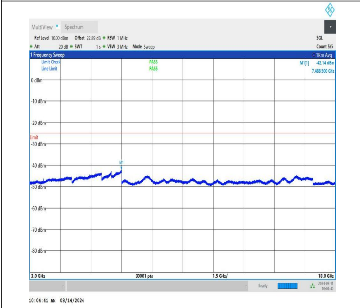
NTNV-n41-PC1.5-30-40-M-CP-QPSK-Edge_1RB_Right-3000-18000-PASS
