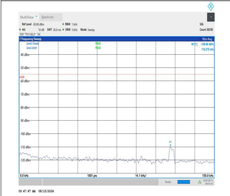
NTNV-n41-PC1.5-30-50-M-CP-QPSK-Edge_1RB_Right-0.009-0.1 5-PASS
