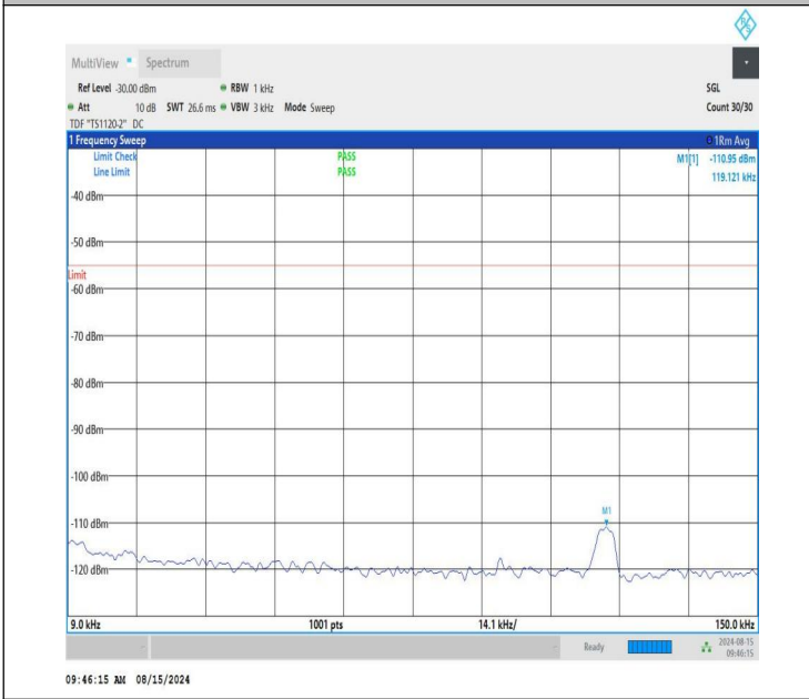
NTVN-n41-PC1.5-30-40-L-CP-QPSK-Edge_1RB_Right-0.009-0.1 5-PASS
