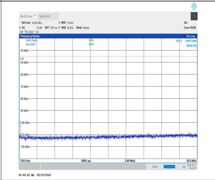
NTVN-n41-PC1.5-30-40-L-CP-QPSK-Edge_1RB_Right-0.15-30-PA SS
