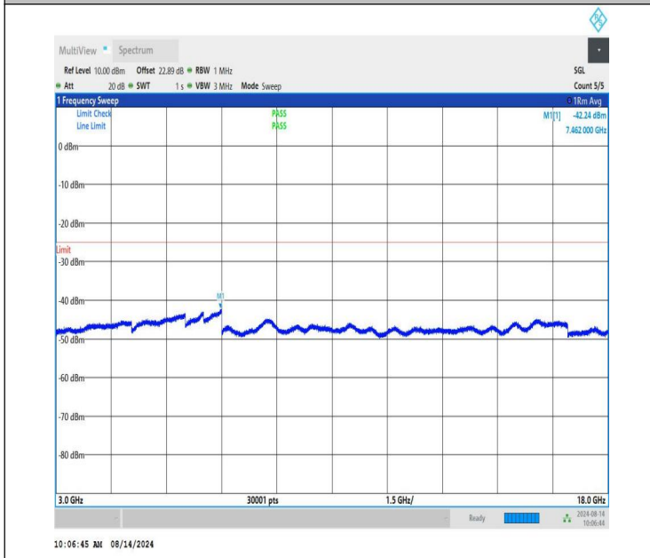
NTNV-n41-PC1.5-30-50-M-CP-QPSK-Edge_1RB_Right-3000-18000-PASS
