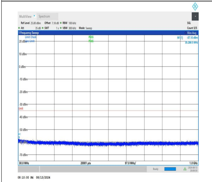
NTNV-n41-PC1.5-30-40-H-CP-QPSK-Edge_1RB_Left-30-1000-PASS
