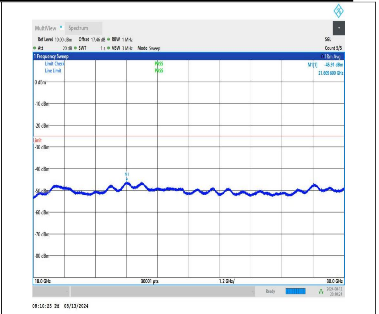
NTNV-n41-PC1.5-30-40-H-CP-QPSK-Edge_1RB_Left-18000-3000 0-PASS
