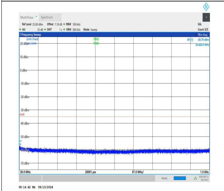
NTNV-n41-PC1.5-30-50-H-CP-QPSK-Edge_1RB_Left-30-1000-PASS
