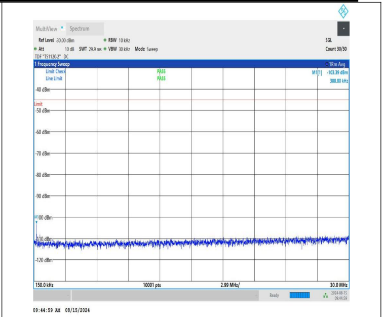
NTNV-n41-PC1.5-30-30-L-CP-QPSK-Edge_1RB_Left-0.15-30-PASS
