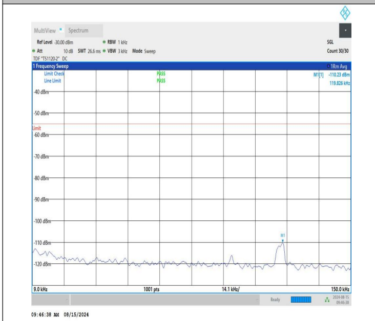
NTNV-n41-PC1.5-30-40-M-CP-QPSK-Edge_1RB_Right-0.009-0.1 5-PASS
