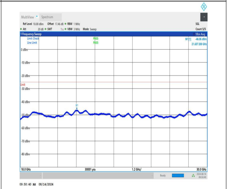
NTNV-n41-PC1.5-30-30-M-CP-QPSK-Edge_1RB_Right-18000-30000-PASS
