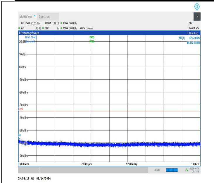
NTNV-n41-PC1.5-30-40-L-CP-QPSK-Edge_1RB_Right-30-1000-P ASS
