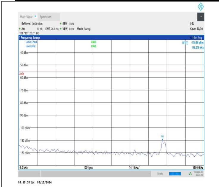
NTNV-n41-PC1.5-30-60-H-CP-QPSK-Edge_1RB_Left-0.09-0.15-PASS
