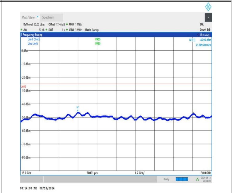
NTNV-n41-PC1.5-30-50-M-CP-QPSK-Edge_1RB_Right-18000-30000-PASS
