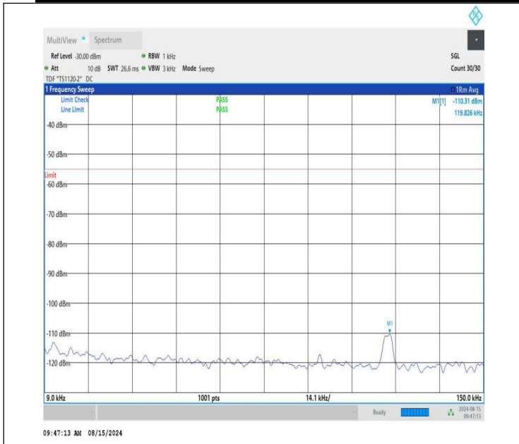
NTNV-n41-PC1.5-30-50-L-CP-QPSK-Edge_1RB_Left-0.009-0.15-PASS
