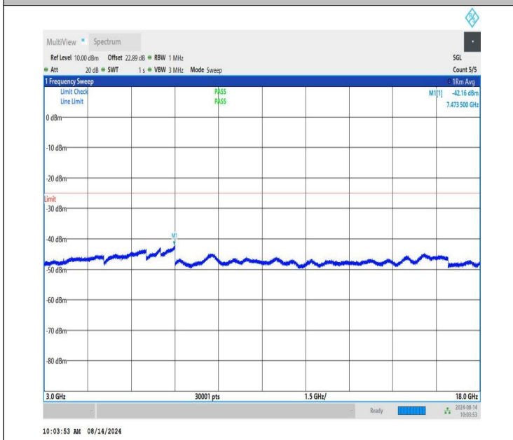
NTNV-n41-PC1.5-30-40-L-CP-QPSK-Edge_1RB_Right-3000-180 00-PASS
