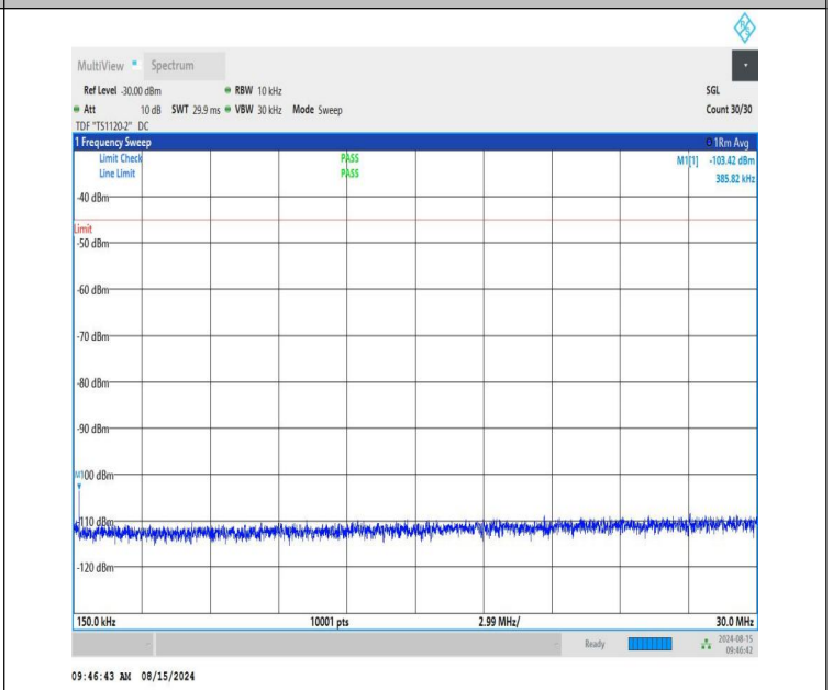
NTNV-n41-PC1.5-30-40-M-CP-QPSK-Edge_1RB_Right-0.15-30-P ASS
