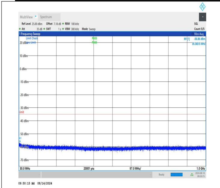
NTNV-n41-PC1.5-30-30-M-CP-QPSK-Edge_1RB_Right-30-1000-PASS
