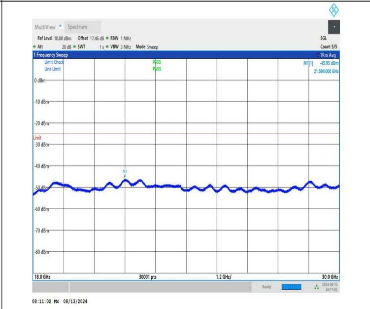
NTNV-n41-PC1.5-30-40-H-CP-QPSK-Edge_1RB_Right-18000-3000-PASS
