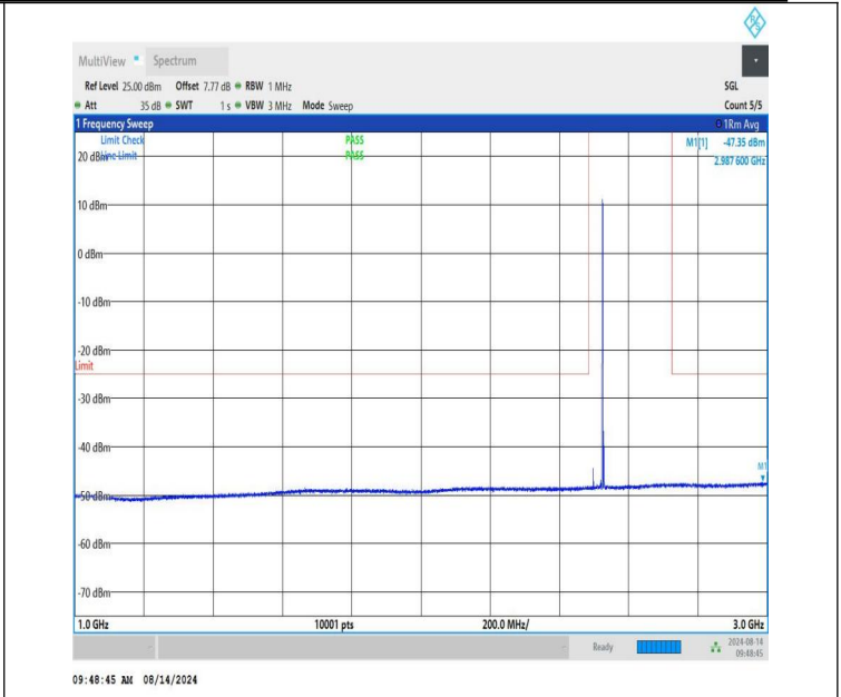
NTNV-n41-PC1.5-30-30-L-CP-QPSK-Edge_1RB_Right-1000-3000- PASS
