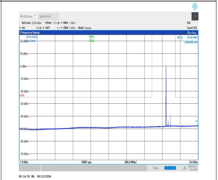
NTNV-n41-PC1.5-30-50-H-CP-QPSK-Edge_1RB_Left-1000-3000-PASS
