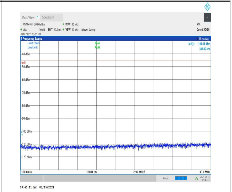
NTVN-n41-PC1.5-30-30-L-CP-QPSK-Edge_1RB_Right-0.15-30-PA SS
