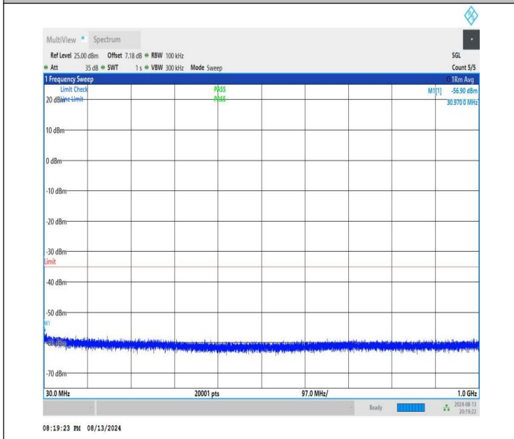
NTNV-n41-PC1.5-30-60-H-CP-QPSK-Edge_1RB_Left-30-1000-PASS
