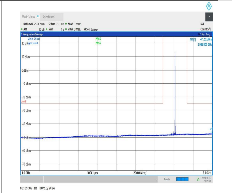
NTNV-n41-PC1.5-30-40-M-CP-QPSK-Edge_1RB_Right-1000-3000-PASS
