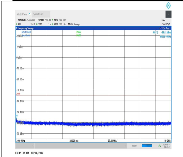
NTNV-n41-PC1.5-30-20-H-CP-QPSK-Edge_1RB_Right-30-1000-PASS
