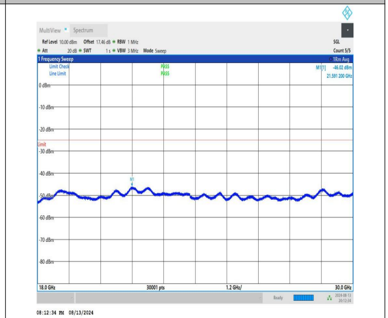
NTNV-n41-PC1.5-30-50-L-CP-QPSK-Edge_1RB_Right-18000-300 00-PASS
