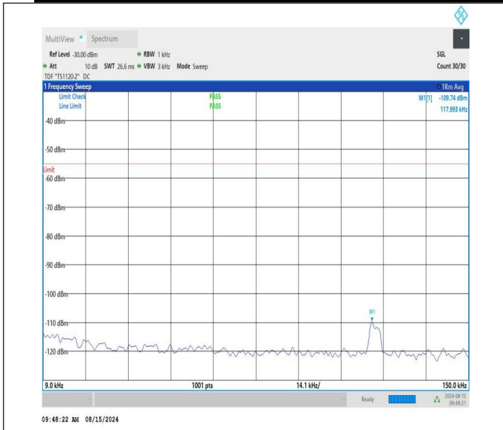
NTNV-n41-PC1.5-30-60-L-CP-QPSK-Edge_1RB_Left-0.009-0.15-PASS
