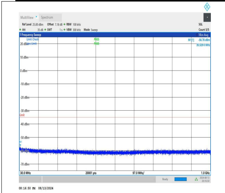
NTNV-n41-PC1.5-30-60-L-CP-QPSK-Edge_1RB_Right-30-1000-P ASS
