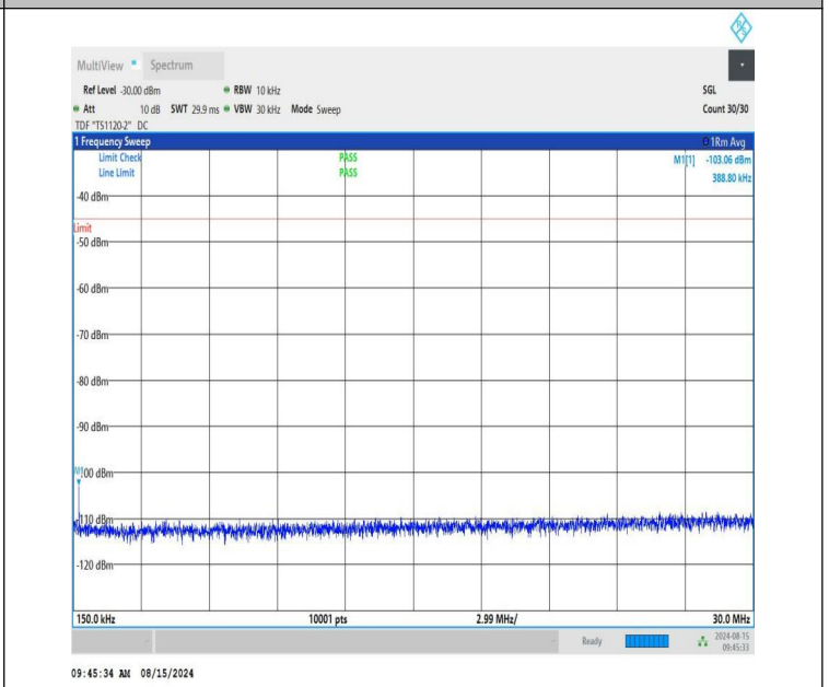
NTNV-n41-PC1.5-30-30-M-CP-QPSK-Edge_1RB_Right-0.15-30-P ASS
