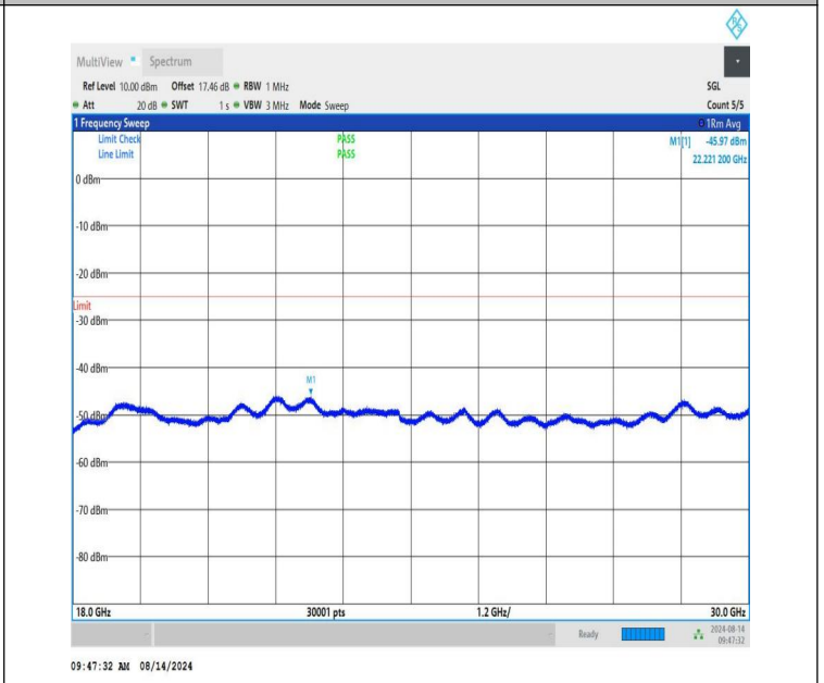
NTNV-n41-PC1.5-30-20-H-CP-QPSK-Edge_1RB_Right-18000-30000-PASS
