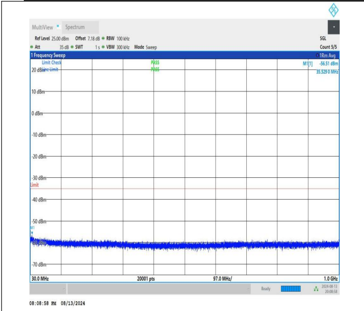
NTNV-n41-PC1.5-30-40-M-CP-QPSK-Edge_1RB_Right-30-1000-PASS
