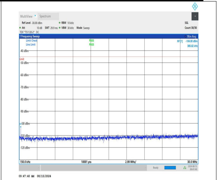
NTNV-n41-PC1.5-30-50-M-CP-QPSK-Edge_1RB_Left-0.15-30-PA SS
