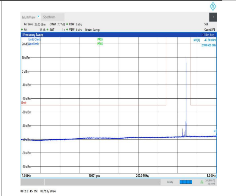
NTNV-n41-PC1.5-30-40-H-CP-QPSK-Edge_1RB_Right-1000-3000-PASS
