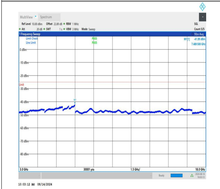
NTNV-n41-PC1.5-30-30-H-CP-QPSK-Edge_1RB_Right-3000-18000-PASS
