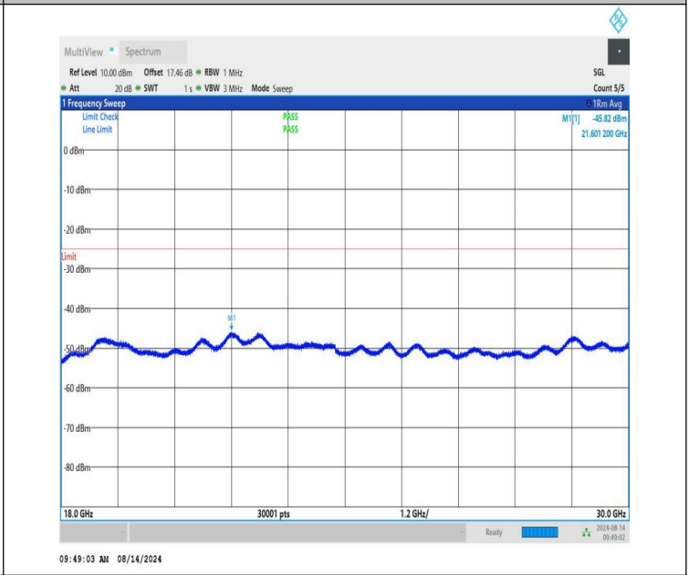
NTNV-n41-PC1.5-30-30-L-CP-QPSK-Edge_1RB_Right-18000-300 00-PASS
