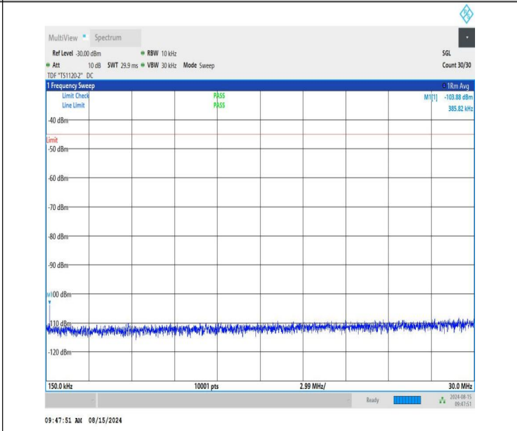
NTNV-n41-PC1.5-30-50-M-CP-QPSK-Edge_1RB_Right-0.15-30-P ASS
