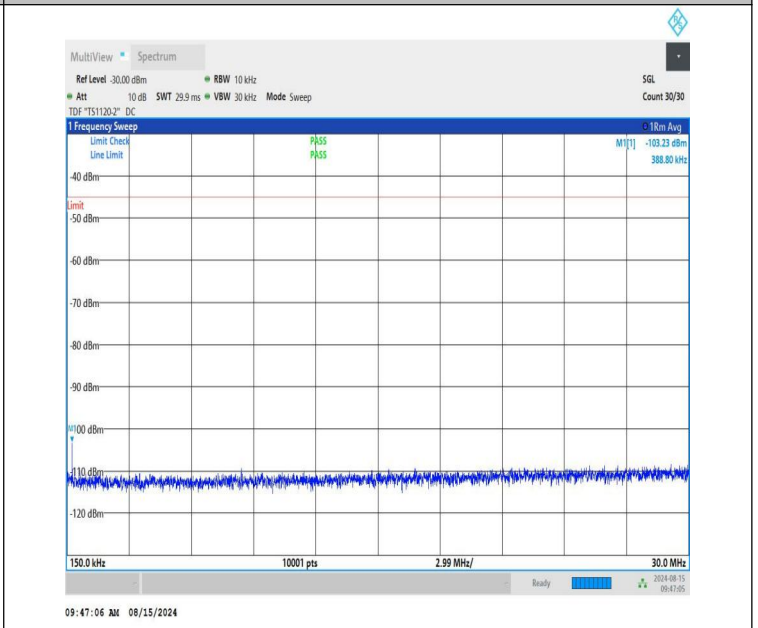
NTNV-n41-PC1.5-30-40-H-CP-QPSK-Edge_1RB_Right-0.15-30-PA SS
