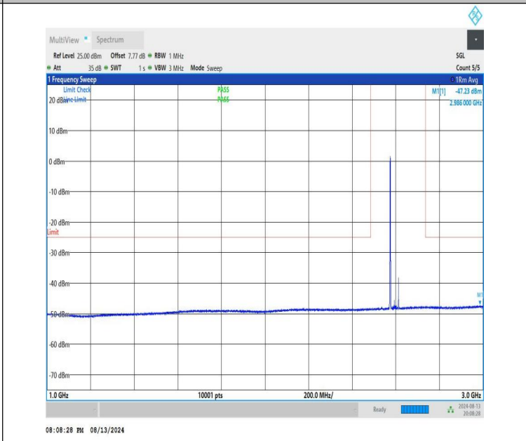
NTNV-n41-PC1.5-30-40-M-CP-QPSK-Edge_1RB_Left-1000-3000-P PASS
