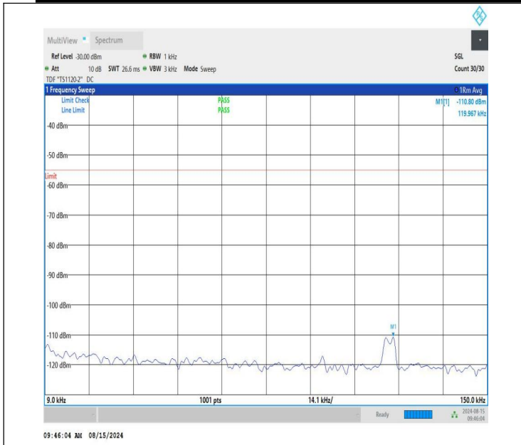
NTNV-n41-PC1.5-30-40-L-CP-QPSK-Edge_1RB_Left-0.009-0.15-PASS
