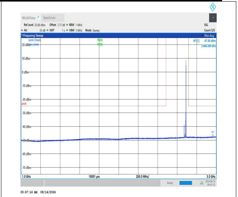
NTNV-n41-PC1.5-30-20-H-CP-QPSK-Edge_1RB_Right-1000-3000-PASS
