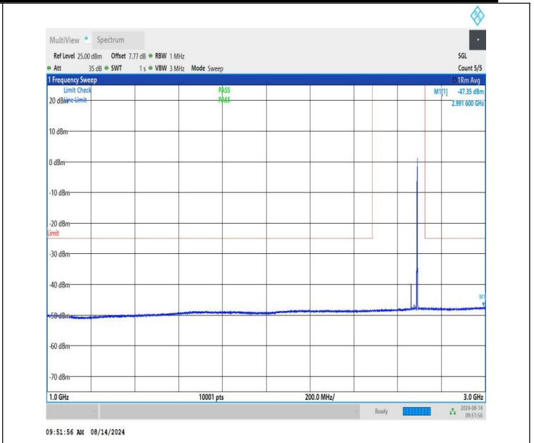
NTNV-n41-PC1.5-30-30-H-CP-QPSK-Edge_1RB_Right-1000-3000-PASS
