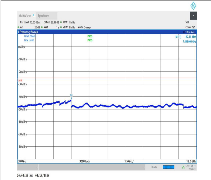
NTNV-n41-PC1.5-30-40-H-CP-QPSK-Edge_1RB_Right-3000-18000-PASS
