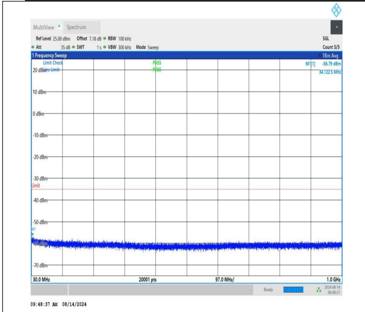
NTNV-n41-PC1.5-30-30-L-CP-QPSK-Edge_1RB_Right-30-1000-P ASS
