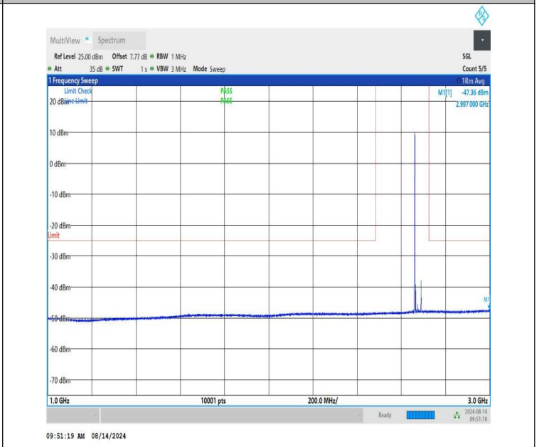
NTNV-n41-PC1.5-30-30-H-CP-QPSK-Edge_1RB_Left-1000-3000-PASS
