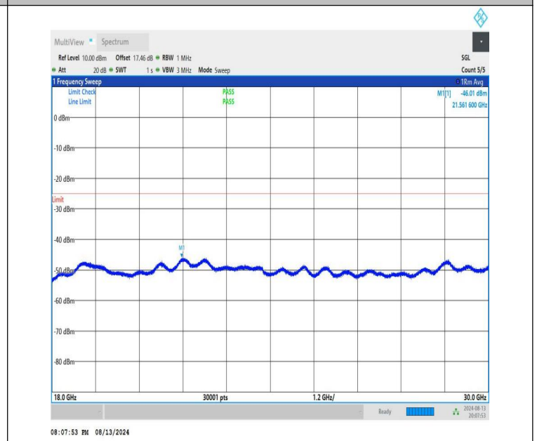
NTNV-n41-PC1.5-30-40-L-CP-QPSK-Edge_1RB_Right-18000-300 00-PASS
