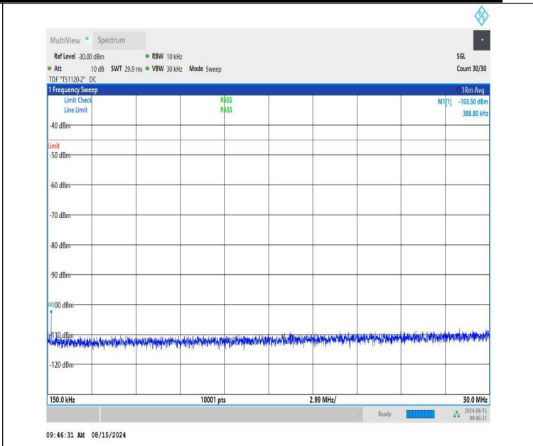
NTNV-n41-PC1.5-30-40-M-CP-QPSK-Edge_1RB_Left-0.15-30-PA SS
