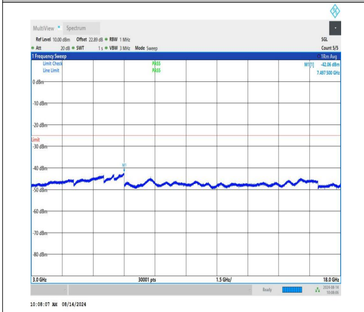
NTNV-n41-PC1.5-30-60-L-CP-QPSK-Edge_1RB_Right-3000-180 00-PASS
