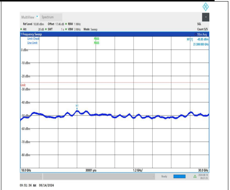
NTNV-n41-PC1.5-30-30-H-CP-QPSK-Edge_1RB_Left-18000-3000 0-PASS
