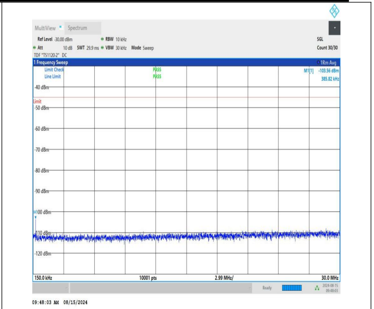
NTNV-n41-PC1.5-30-50-H-CP-QPSK-Edge_1RB_Left-0.15-30-PASS
