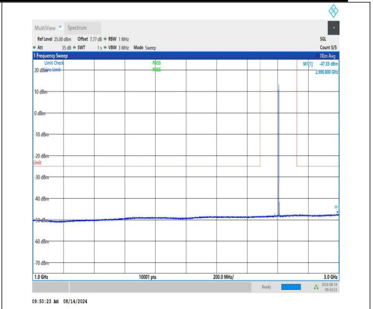
NTNV-n41-PC1.5-30-30-M-CP-QPSK-Edge_1RB_Right-1000-3000-PASS
