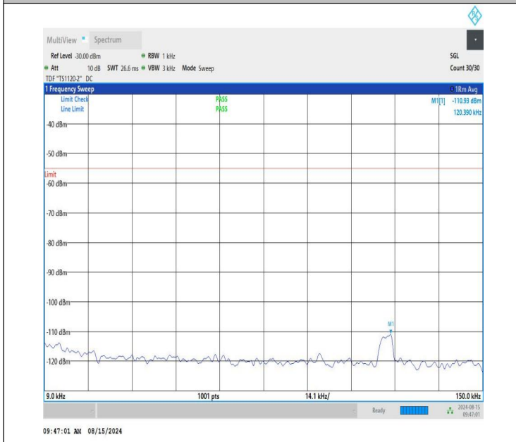
NTNV-n41-PC1.5-30-40-H-CP-QPSK-Edge_1RB_Right-0.009-0.1 5-PASS
