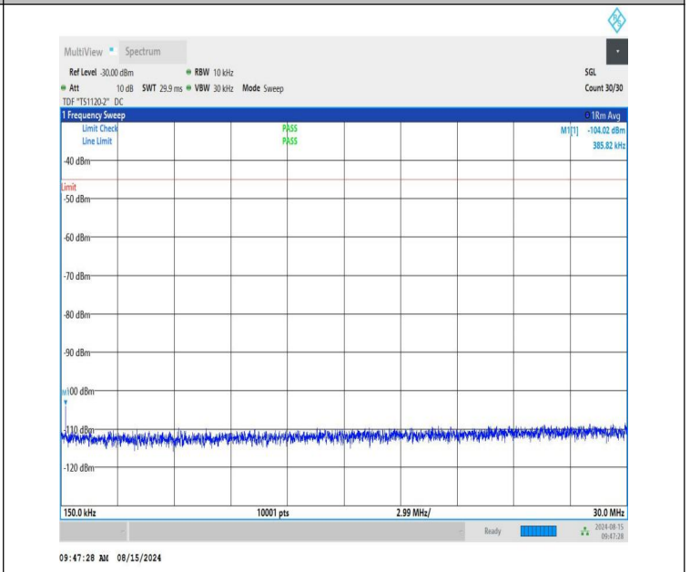
NTVN-n41-PC1.5-30-50-L-CP-QPSK-Edge_1RB_Right-0.15-30-PA SS
