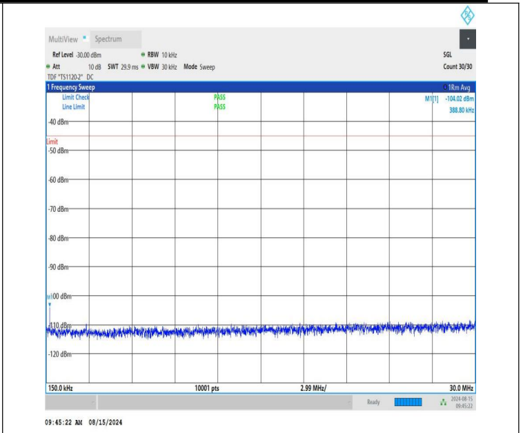
NTNV-n41-PC1.5-30-30-M-CP-QPSK-Edge_1RB_Left-0.15-30-PA SS
