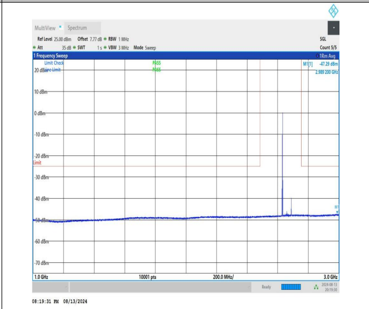
NTNV-n41-PC1.5-30-60-H-CP-QPSK-Edge_1RB_Left-1000-3000-PASS
