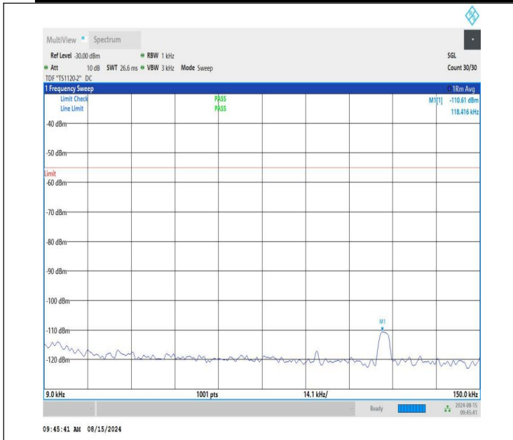
NTNV-n41-PC1.5-30-30-H-CP-QPSK-Edge_1RB_Left-0.009-0.15-PASS
