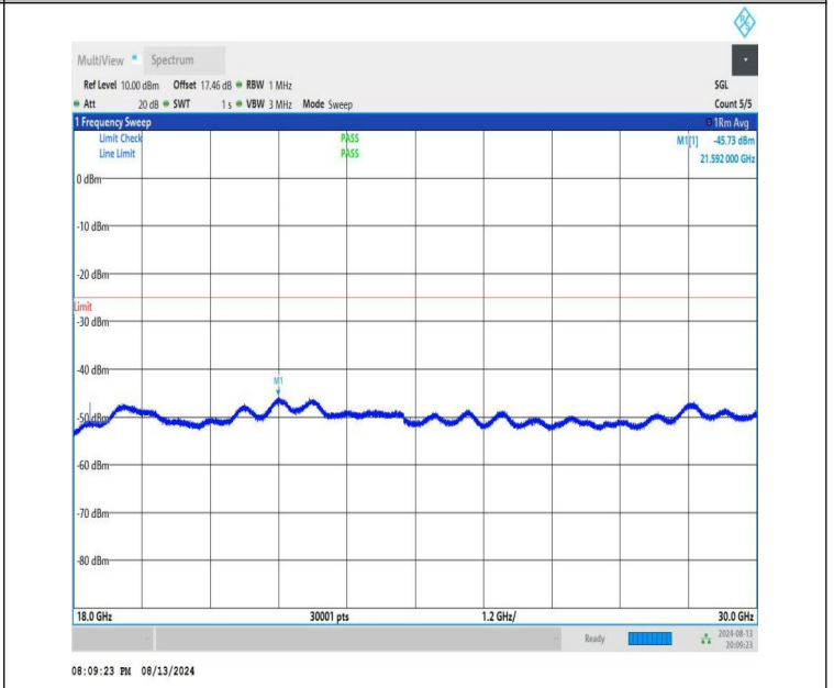
NTNV-n41-PC1.5-30-40-M-CP-QPSK-Edge_1RB_Right-18000-3000-PASS
