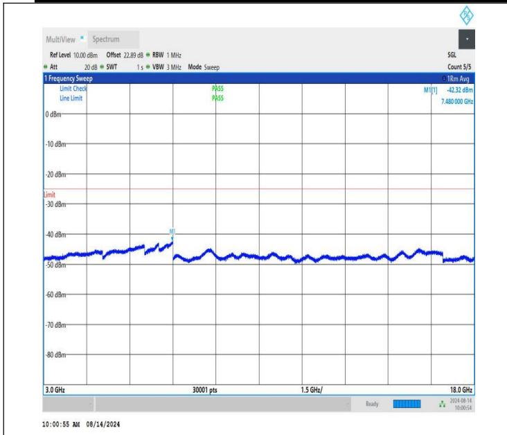
NTNV-n41-PC1.5-30-20-H-CP-QPSK-Edge_1RB_Left-3000-1800 0-PASS
