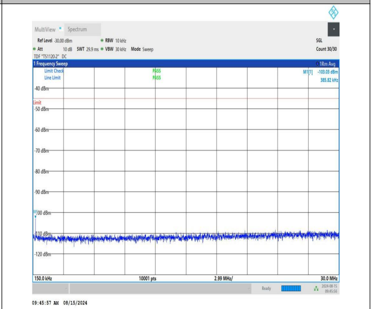
NTNV-n41-PC1.5-30-30-H-CP-QPSK-Edge_1RB_Right-0.15-30-PA SS
