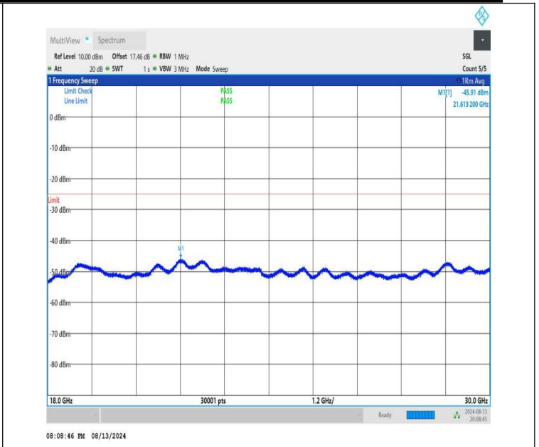
NTNV-n41-PC1.5-30-40-M-CP-QPSK-Edge_1RB_Left-18000-3000 0-PASS
