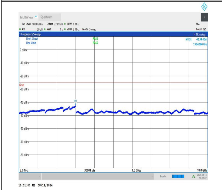
NTNV-n41-PC1.5-30-20-H-CP-QPSK-Edge_1RB_Right-3000-18000-PASS
