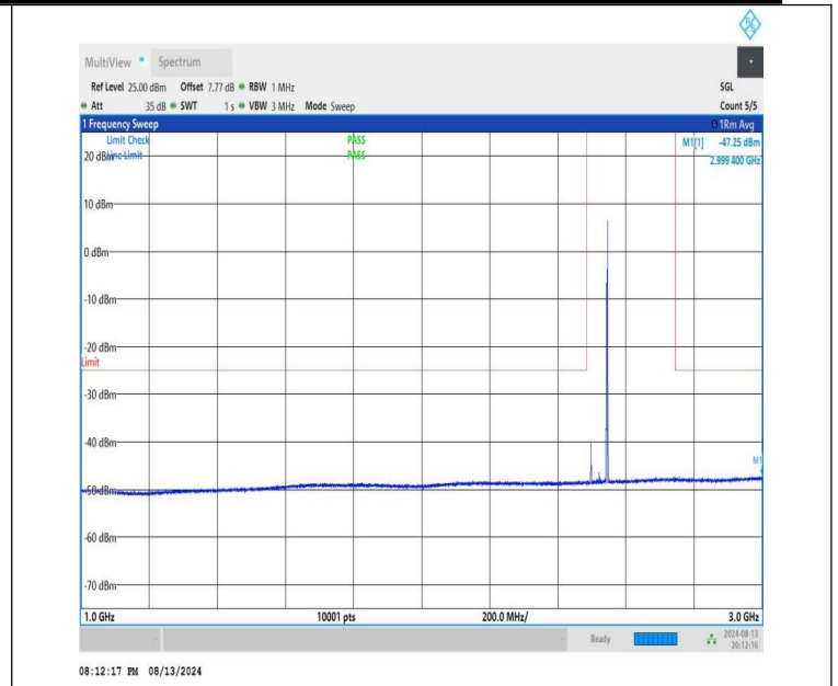
NTNV-n41-PC1.5-30-50-L-CP-QPSK-Edge_1RB_Right-1000-3000- PASS
