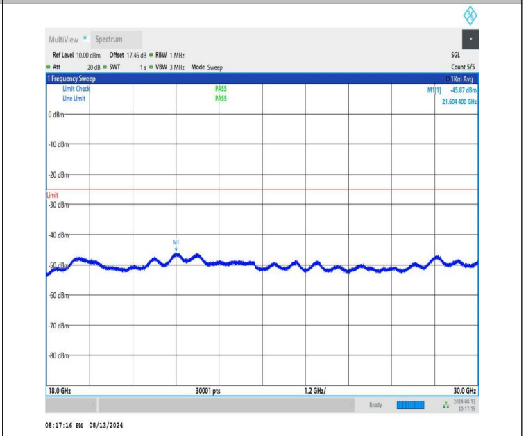
NTNV-n41-PC1.5-30-60-L-CP-QPSK-Edge_1RB_Right-18000-300 00-PASS
