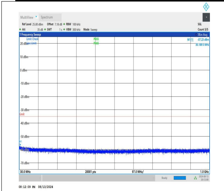
NTNV-n41-PC1.5-30-50-L-CP-QPSK-Edge_1RB_Right-30-1000-P ASS
