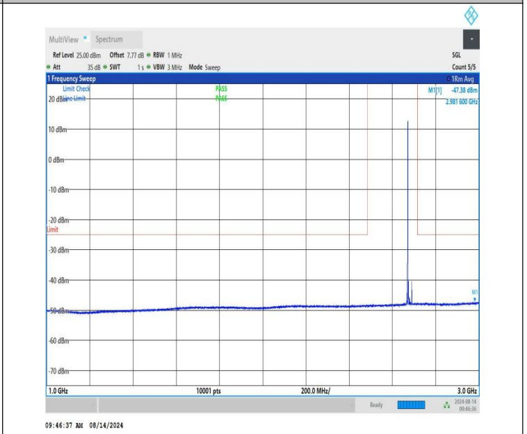
NTNV-n41-PC1.5-30-20-H-CP-QPSK-Edge_1RB_Left-1000-3000-PASS
