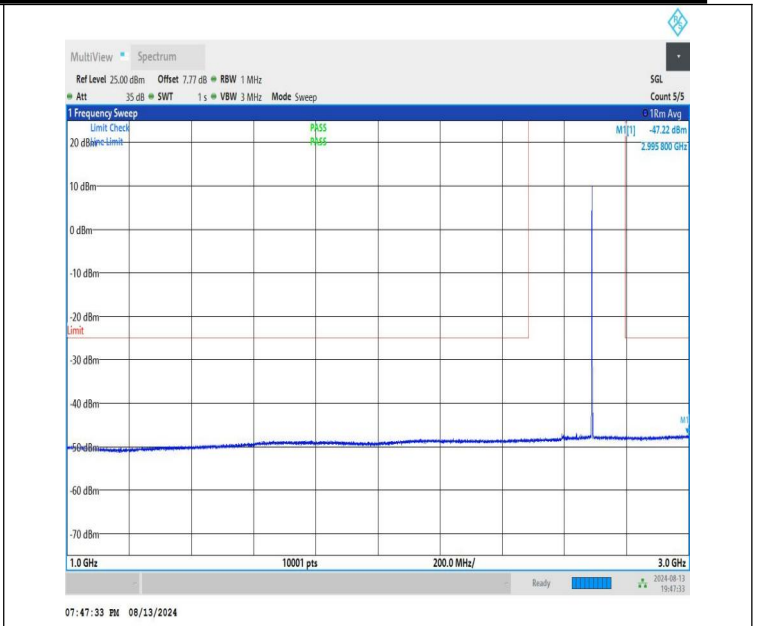
NTNV-n41-PC1.5-30-100-H-CP-QPSK-Edge_1RB_Right-1000-300 0-PASS
