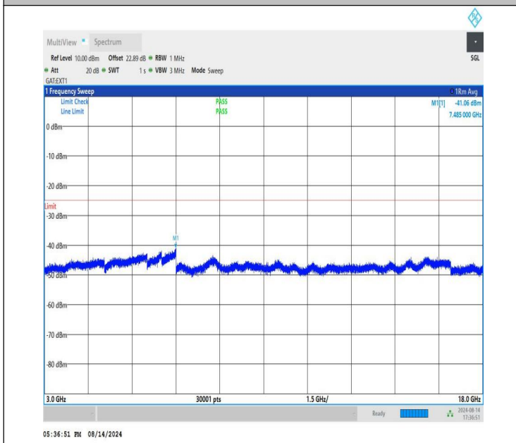
NTNV-n41-PC1.5-30-90-H-CP-QPSK-Edge_1RB_Right-3000-18000-PASS
