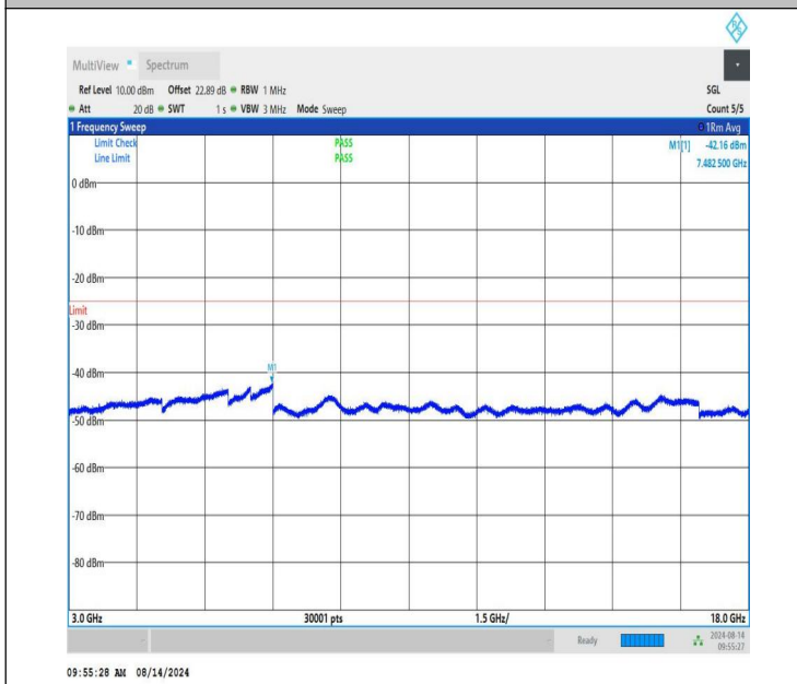
NTNV-n41-PC1.5-30-10-L-CP-QPSK-Edge_1RB_Right-3000-180 00-PASS
