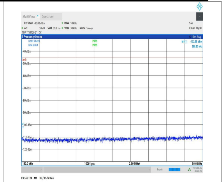
NTNV-n41-PC1.5-30-100-L-CP-QPSK-Edge_1RB_Left-0.15-30-PA SS
