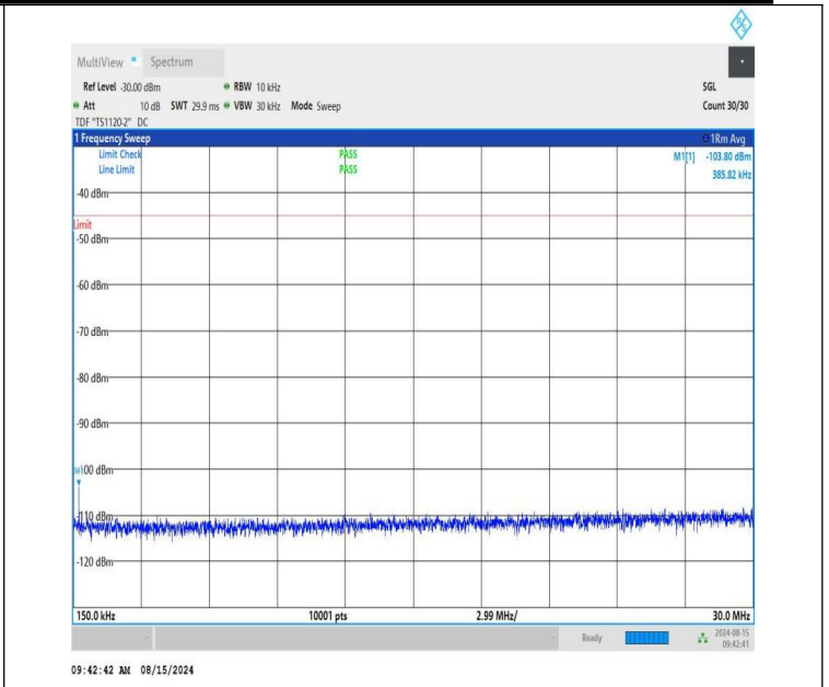
NTNV-n41-PC1.5-30-15-L-CP-QPSK-Edge_1RB_Left-0.15-30-PASS
