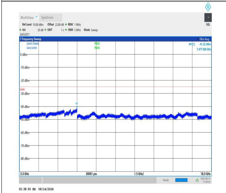
NTNV-n41-PC1.5-30-100-M-CP-QPSK-Edge_1RB_Right-3000-18000 000-PASS
