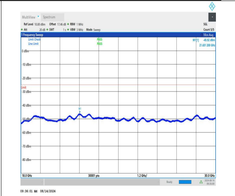
NTNV-n41-PC1.5-30-10-M-CP-QPSK-Edge_1RB_Left-18000-3000 0-PASS
