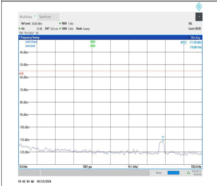
NTVN-n41-PC1.5-30-15-L-CP-QPSK-Edge_1RB_Right-0.009-0.1 5-PASS
