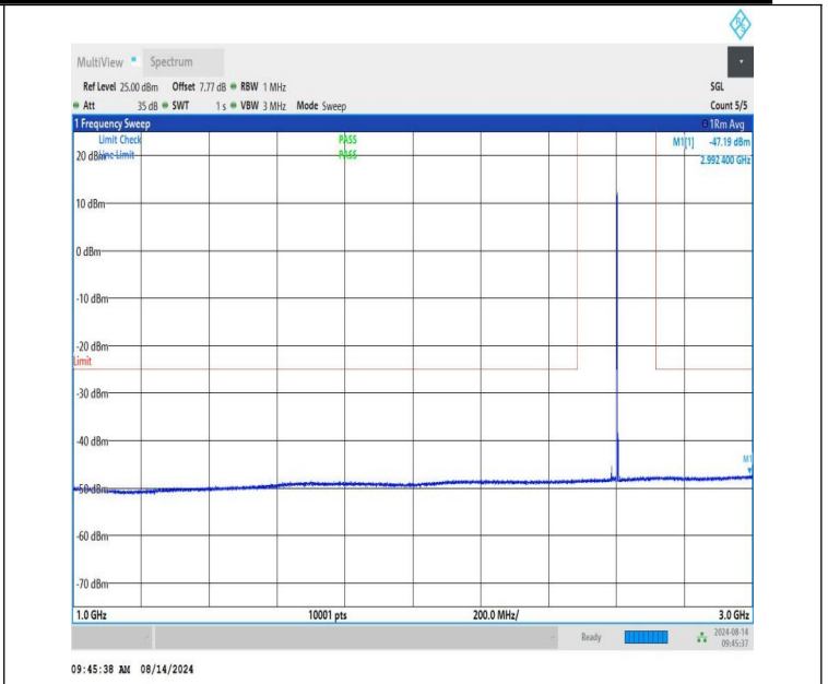
NTNV-n41-PC1.5-30-20-M-CP-QPSK-Edge_1RB_Right-1000-3000-PASS
