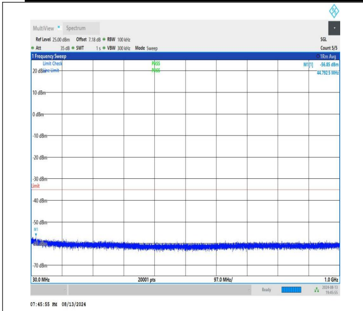
NTNV-n41-PC1.5-30-100-M-CP-QPSK-Edge_1RB_Right-30-1000 -PASS
