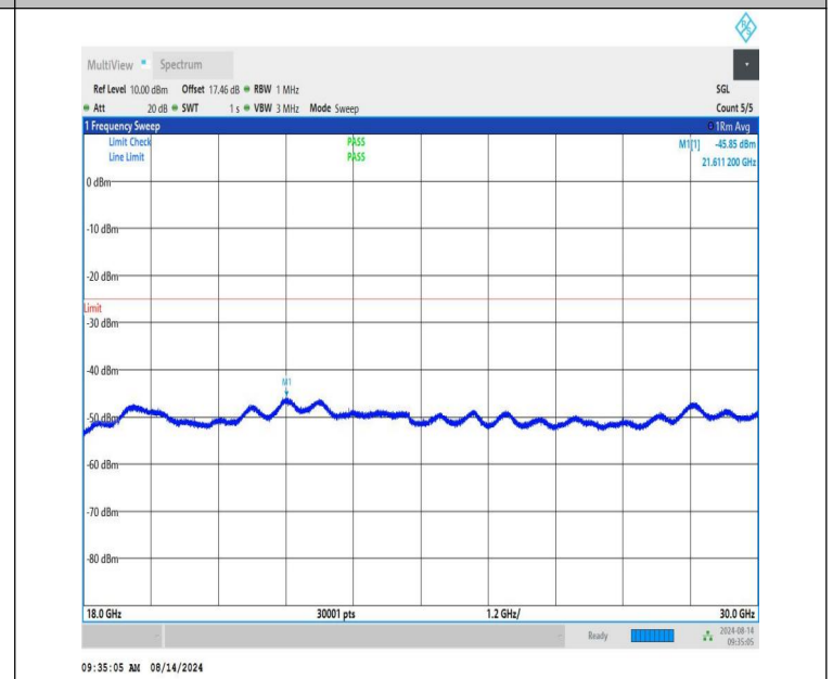
NTNV-n41-PC1.5-30-10-L-CP-QPSK-Edge_1RB_Right-18000-300 00-PASS
