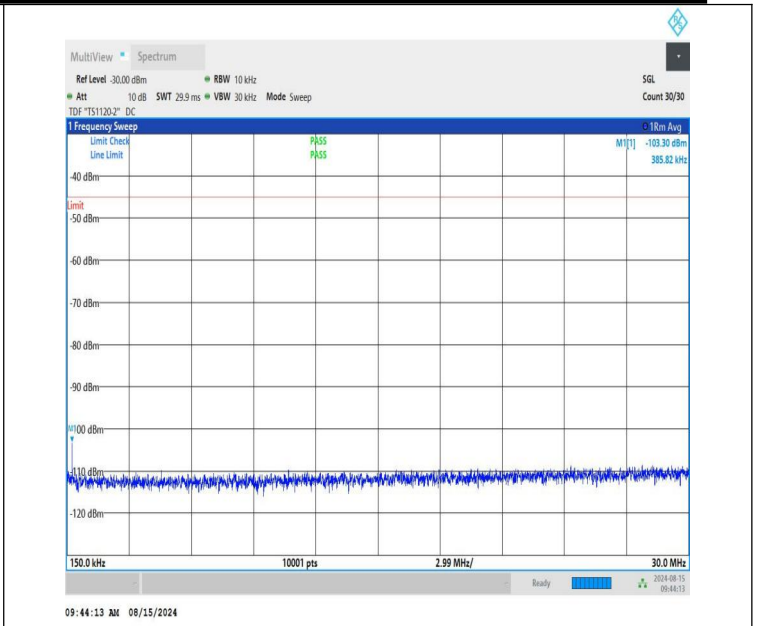
NTNV-n41-PC1.5-30-20-M-CP-QPSK-Edge_1RB_Left-0.15-30-PA SS
