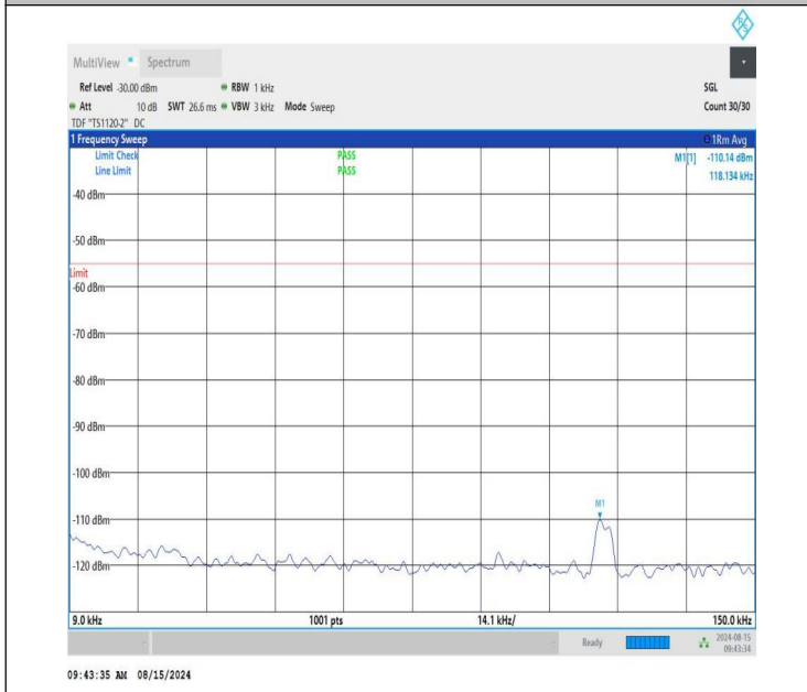
NTNV-n41-PC1.5-30-15-H-CP-QPSK-Edge_1RB_Right-0.009-0.1 5-PASS
