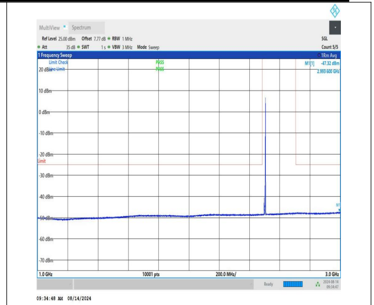
NTNV-n41-PC1.5-30-10-L-CP-QPSK-Edge_1RB_Right-1000-3000- PASS
