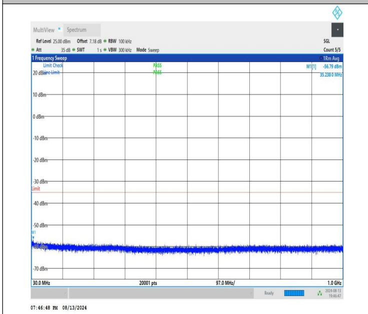
NTNV-n41-PC1.5-30-100-H-CP-QPSK-Edge_1RB_Left-30-1000-P ASS
