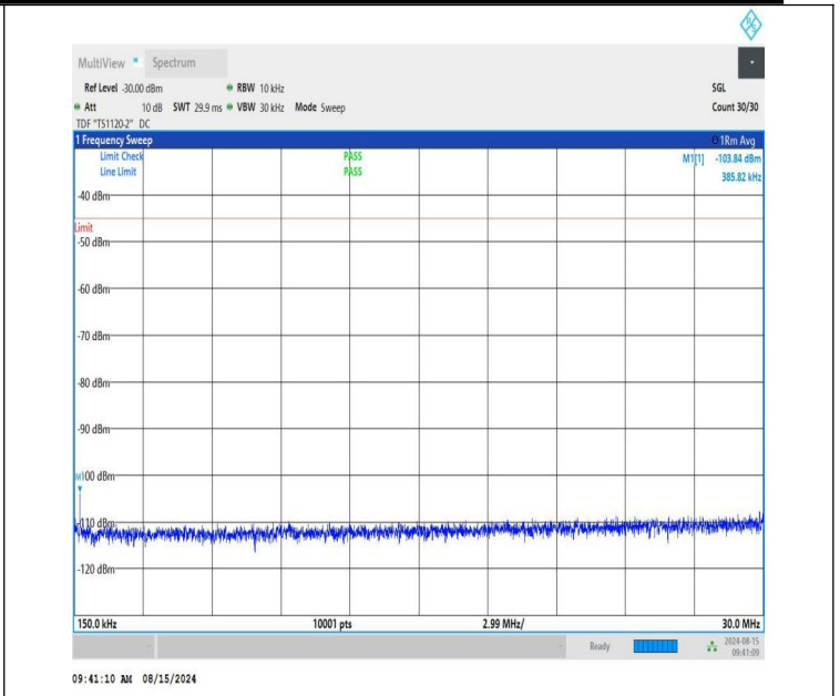
NTNV-n41-PC1.5-30-100-H-CP-QPSK-Edge_1RB_Left-0.15-30-PA SS
