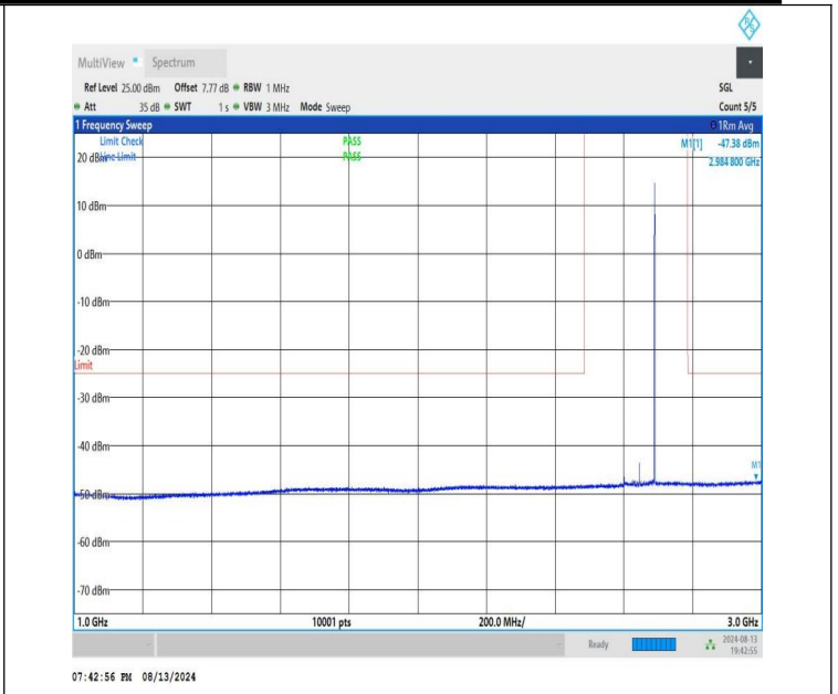
NTNV-n41-PC1.5-30-90-H-CP-QPSK-Edge_1RB_Right-1000-3000-PASS
