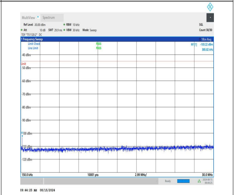
NTNV-n41-PC1.5-30-20-M-CP-QPSK-Edge_1RB_Right-0.15-30-P ASS
