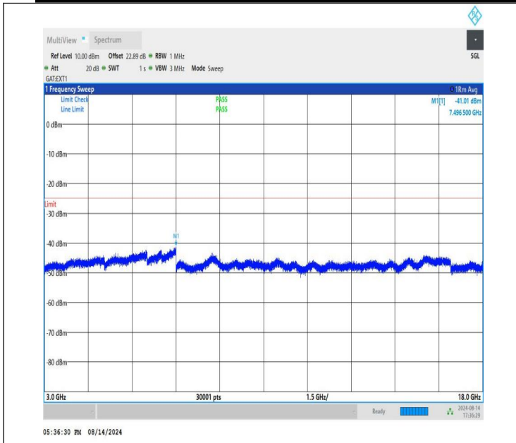
NTNV-n41-PC1.5-30-90-H-CP-QPSK-Edge_1RB_Left-3000-1800 0-PASS
