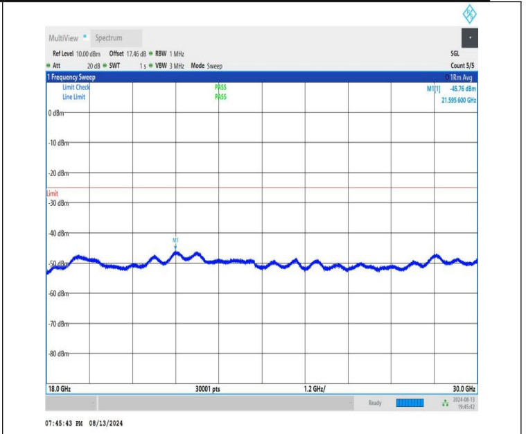
NTNV-n41-PC1.5-30-100-M-CP-QPSK-Edge_1RB_Left-18000-300 00-PASS
