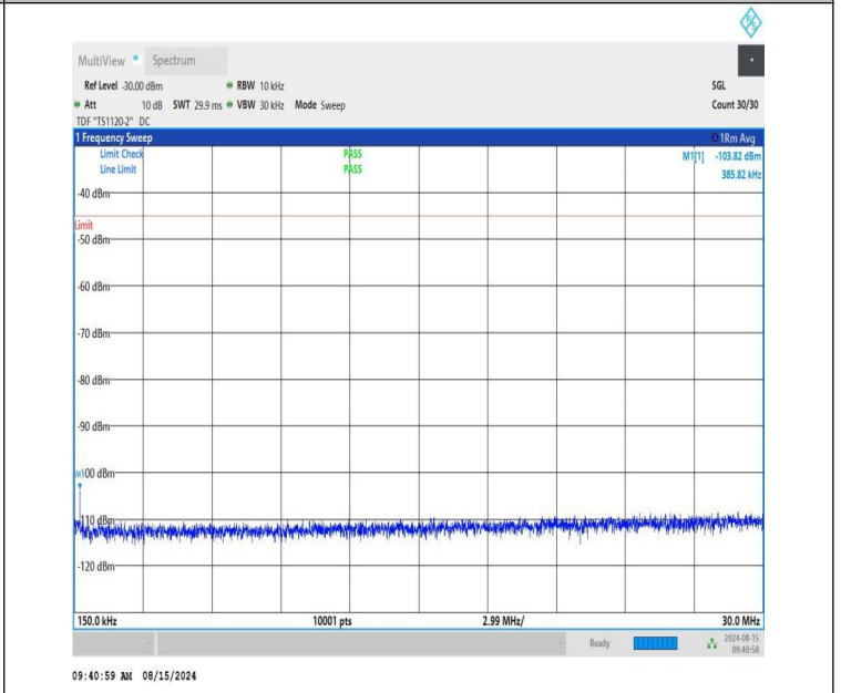
NTNV-n41-PC1.5-30-100-M-CP-QPSK-Edge_1RB_Right-0.15-30-P ASS
