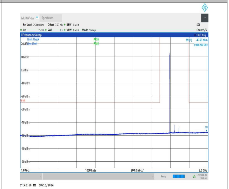
NTNV-n41-PC1.5-30-100-H-CP-QPSK-Edge_1RB_Left-1000-3000-P PASS
