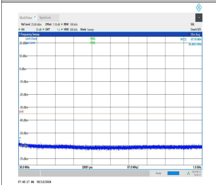
NTNV-n41-PC1.5-30-100-M-CP-QPSK-Edge_1RB_Left-30-1000- PASS
