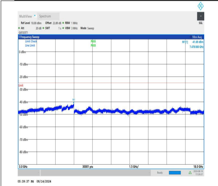
NTNV-n41-PC1.5-30-100-H-CP-QPSK-Edge_1RB_Left-3000-180 00-PASS
