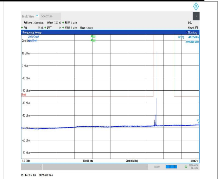
NTNV-n41-PC1.5-30-20-L-CP-QPSK-Edge_1RB_Right-1000-3000- PASS
