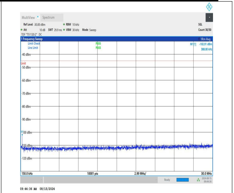
NTNV-n41-PC1.5-30-20-H-CP-QPSK-Edge_1RB_Left-0.15-30-PASS
