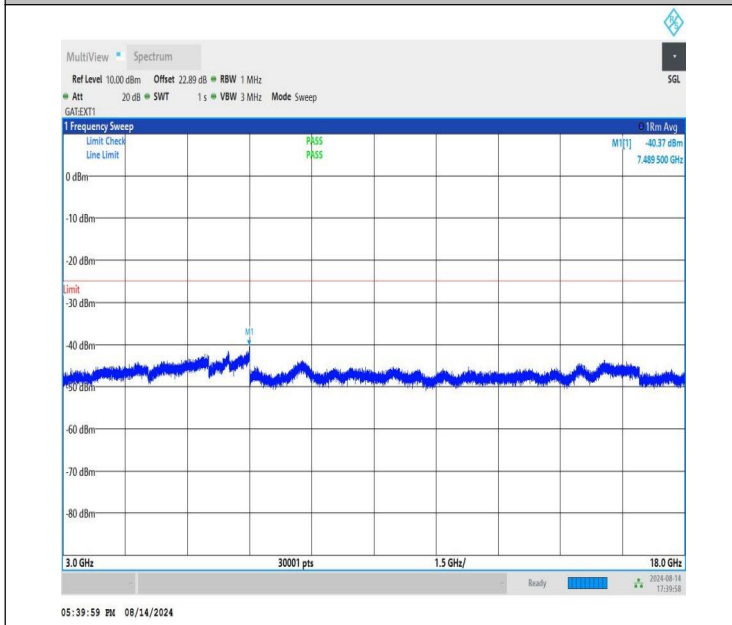
NTNV-n41-PC1.5-30-100-H-CP-QPSK-Edge_1RB_Right-3000-18000-30 000-PASS
