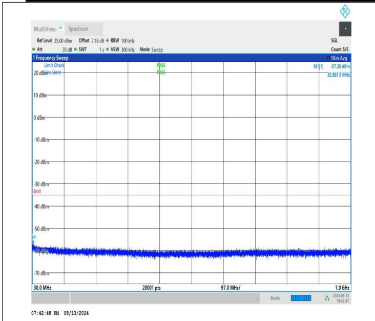
NTNV-n41-PC1.5-30-90-H-CP-QPSK-Edge_1RB_Right-30-1000-PASS
