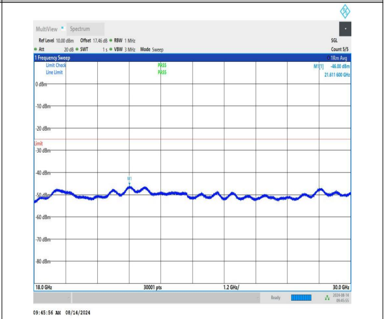
NTNV-n41-PC1.5-30-20-M-CP-QPSK-Edge_1RB_Right-18000-30000-PASS
