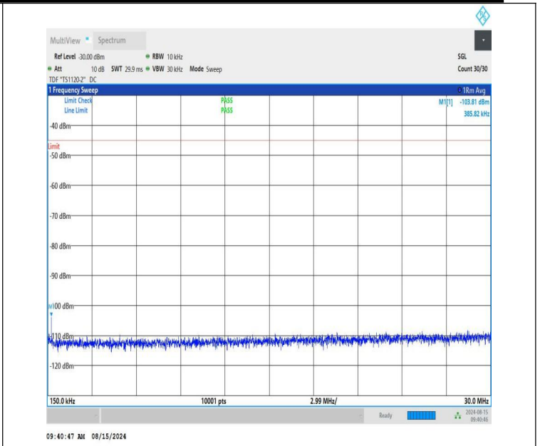
NTNV-n41-PC1.5-30-100-M-CP-QPSK-Edge_1RB_Left-0.15-30-PA SS
