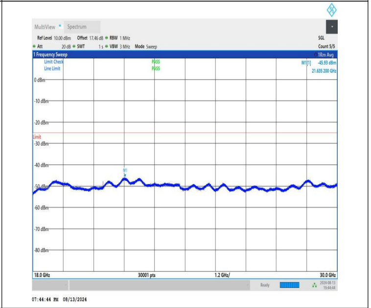
NTNV-n41-PC1.5-30-100-L-CP-QPSK-Edge_1RB_Right-18000-30000-PASS
