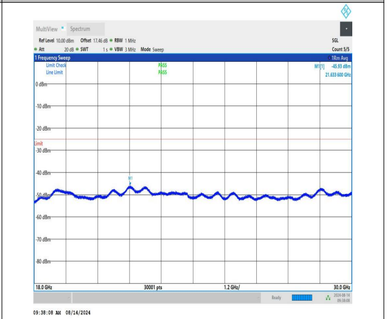
NTNV-n41-PC1.5-30-10-H-CP-QPSK-Edge_1RB_Right-18000-30000-PASS
