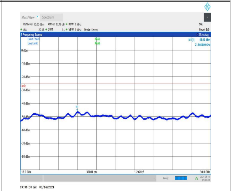
NTNV-n41-PC1.5-30-10-M-CP-QPSK-Edge_1RB_Right-18000-30000-PASS
