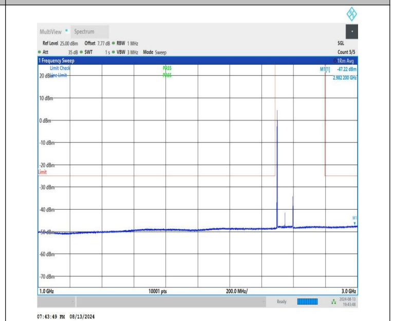
NTNV-n41-PC1.5-30-100-L-CP-QPSK-Edge_1RB_Left-1000-3000-P PASS
