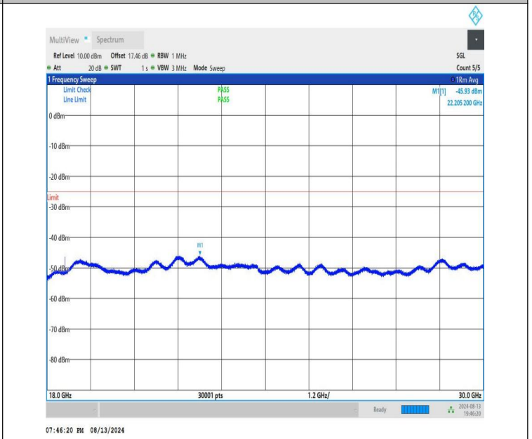
NTNV-n41-PC1.5-30-100-M-CP-QPSK-Edge_1RB_Right-18000-30000 000-PASS
