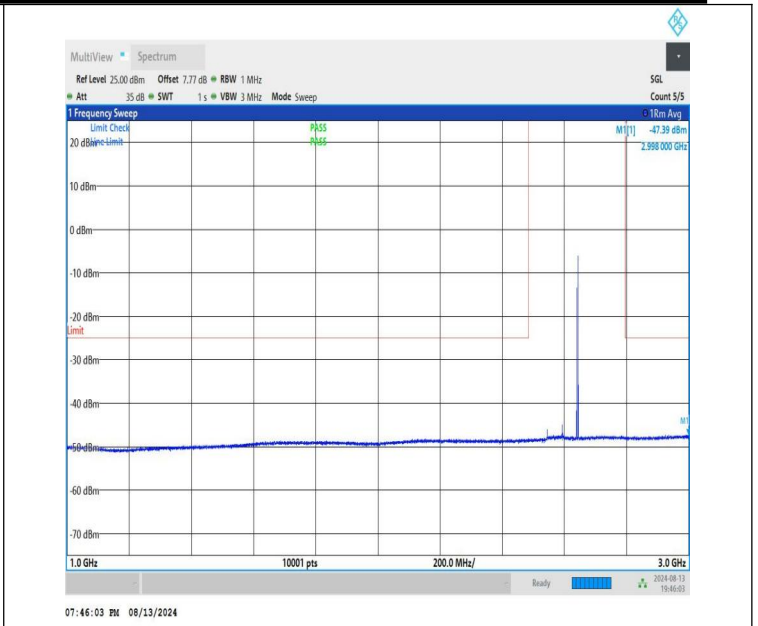
NTNV-n41-PC1.5-30-100-M-CP-QPSK-Edge_1RB_Right-1000-300 0-PASS
