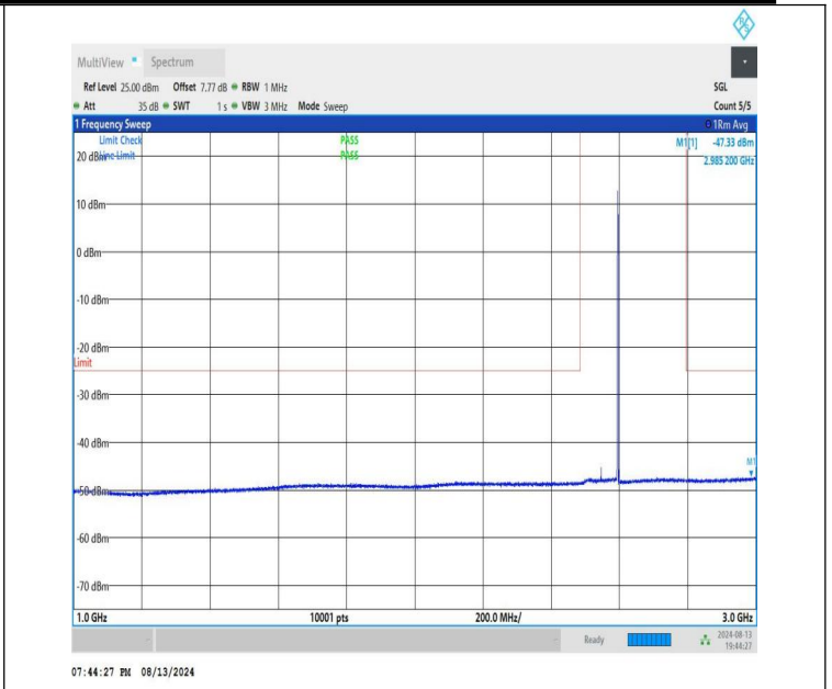
NTNV-n41-PC1.5-30-100-L-CP-QPSK-Edge_1RB_Right-1000-300-0-PASS
