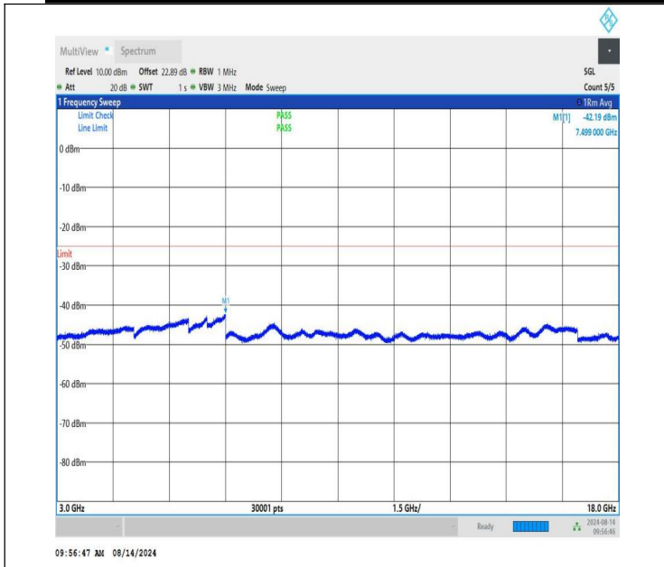
NTNV-n41-PC1.5-30-10-H-CP-QPSK-Edge_1RB_Left-3000-1800 0-PASS
