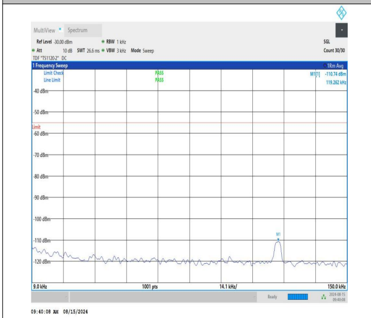
NTNV-n41-PC1.5-30-90-H-CP-QPSK-Edge_1RB_Right-0.009-0.1 5-PASS
