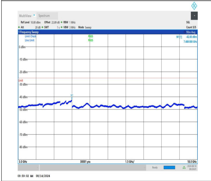
NTNV-n41-PC1.5-30-15-H-CP-QPSK-Edge_1RB_Right-3000-18000-PASS
