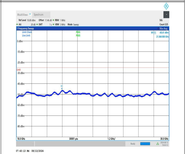
NTNV-n41-PC1.5-30-90-H-CP-QPSK-Edge_1RB_Right-18000-30000-PASS
