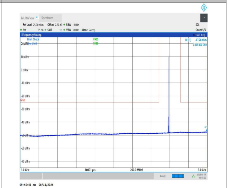
NTNV-n41-PC1.5-30-20-M-CP-QPSK-Edge_1RB_Left-1000-3000-P PASS
