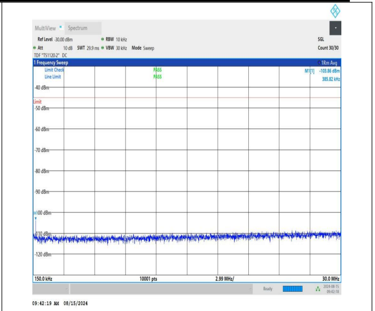
NTNV-n41-PC1.5-30-10-H-CP-QPSK-Edge_1RB_Left-0.15-30-PASS
