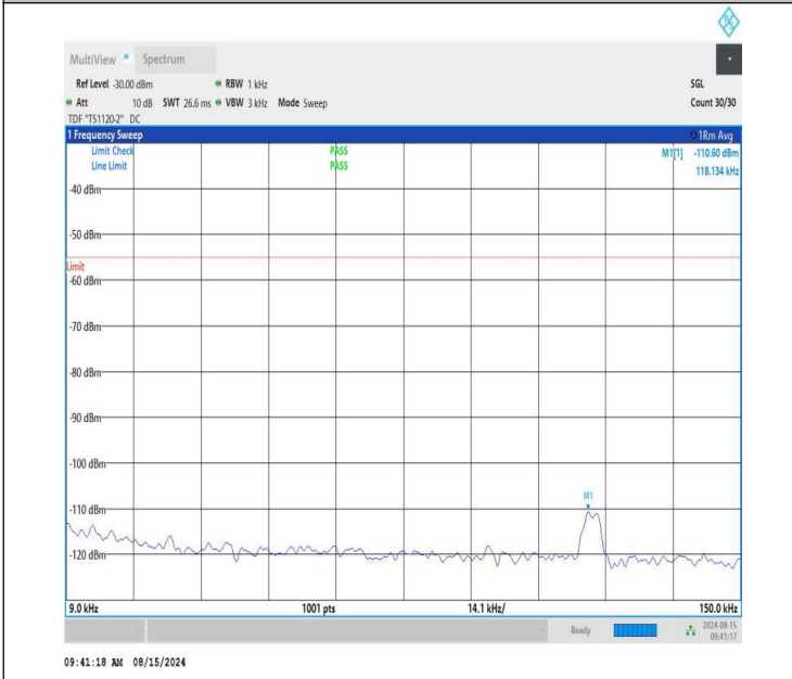
NTNV-n41-PC1.5-30-100-H-CP-QPSK-Edge_1RB_Right-0.009-0. 15-PASS
