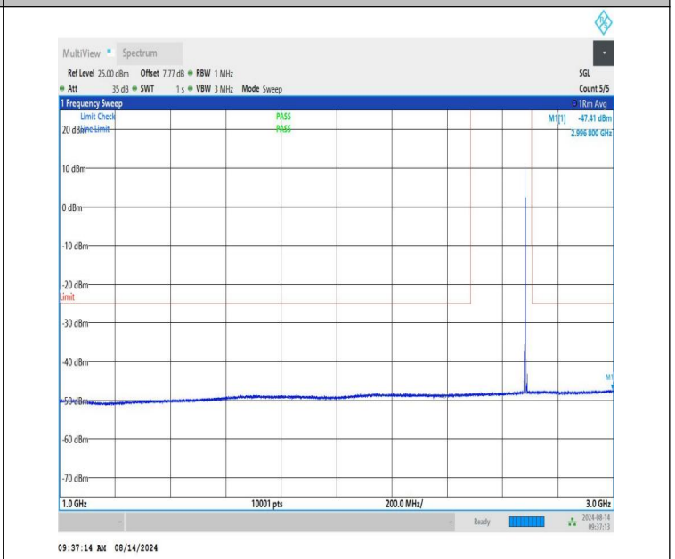
NTNV-n41-PC1.5-30-10-H-CP-QPSK-Edge_1RB_Left-1000-3000-PASS
