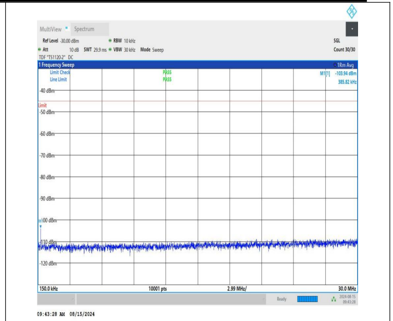
NTNV-n41-PC1.5-30-15-H-CP-QPSK-Edge_1RB_Left-0.15-30-PASS
