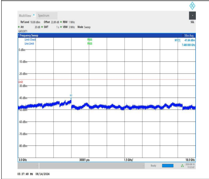
NTNV-n41-PC1.5-30-100-L-CP-QPSK-Edge_1RB_Right-3000-18000-PASS
