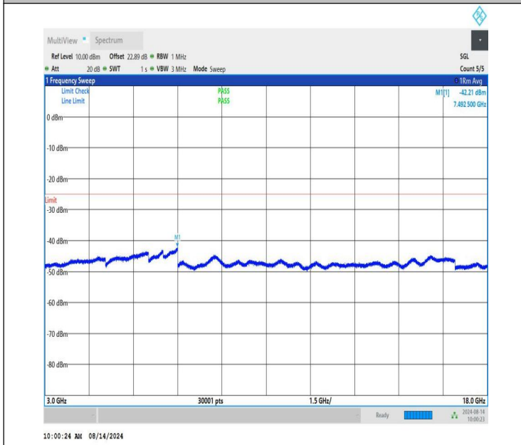
NTNV-n41-PC1.5-30-20-M-CP-QPSK-Edge_1RB_Right-3000-18000-PASS
