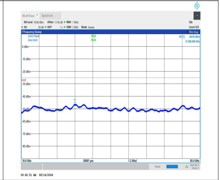
NTNV-n41-PC1.5-30-15-H-CP-QPSK-Edge_1RB_Right-18000-30000-PASS
