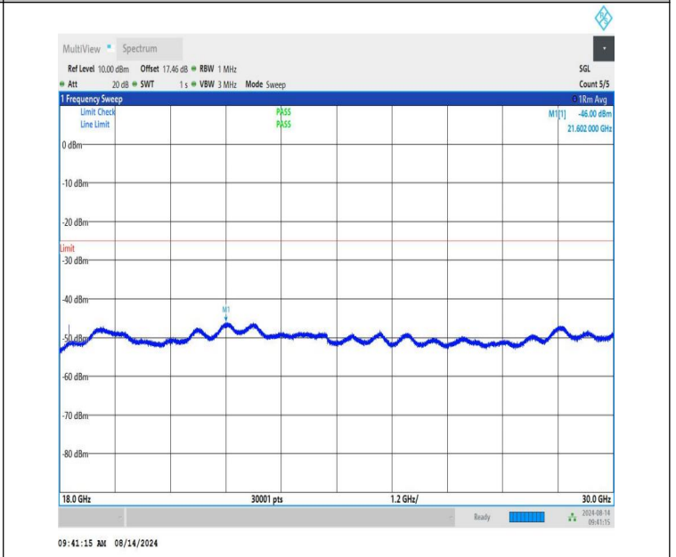
NTNV-n41-PC1.5-30-15-M-CP-QPSK-Edge_1RB_Right-18000-300-PASS
