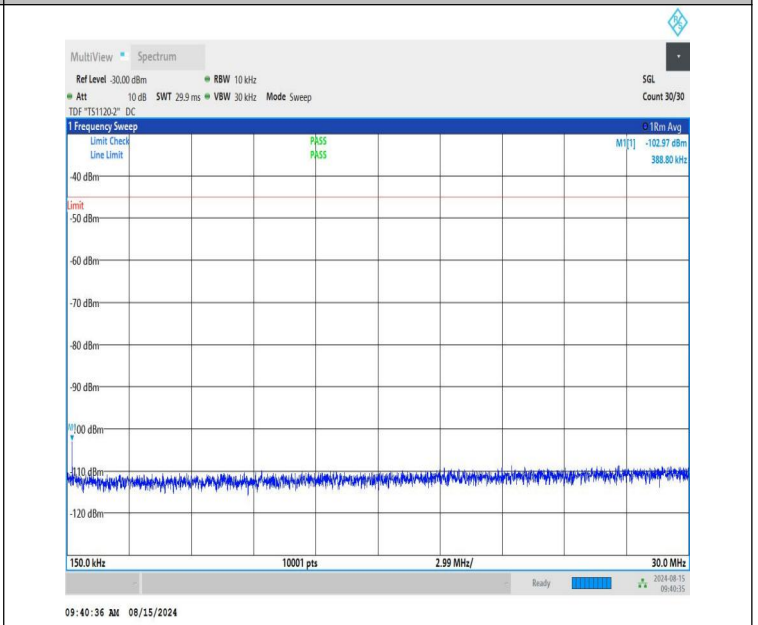
NTVN-n41-PC1.5-30-100-L-CP-QPSK-Edge_1RB_Right-0.15-30-P ASS
