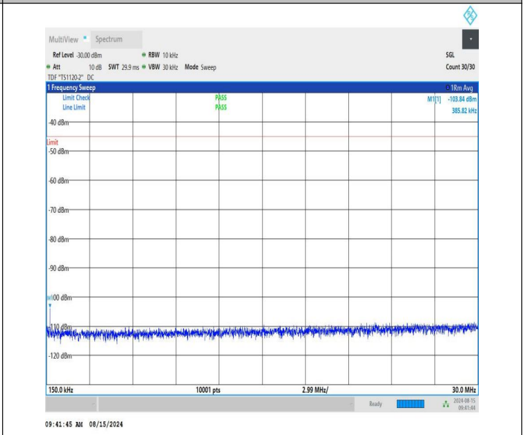
NTVN-n41-PC1.5-30-10-L-CP-QPSK-Edge_1RB_Right-0.15-30-PA SS
