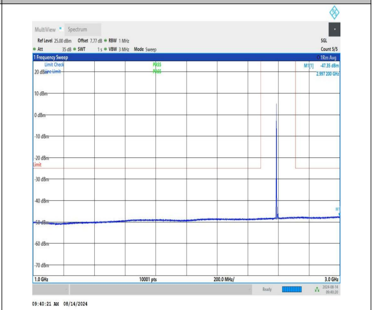
NTNV-n41-PC1.5-30-15-M-CP-QPSK-Edge_1RB_Left-1000-3000-P PASS
