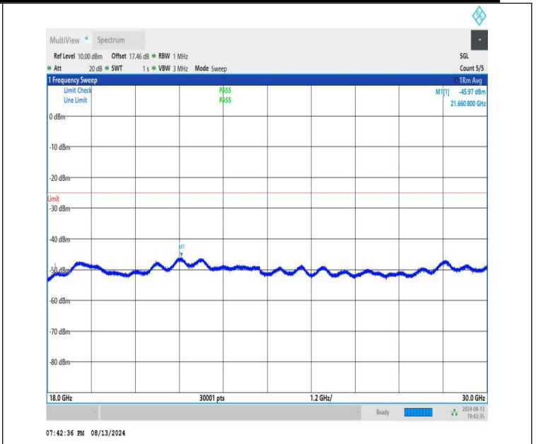
NTNV-n41-PC1.5-30-90-H-CP-QPSK-Edge_1RB_Left-18000-3000 0-PASS
