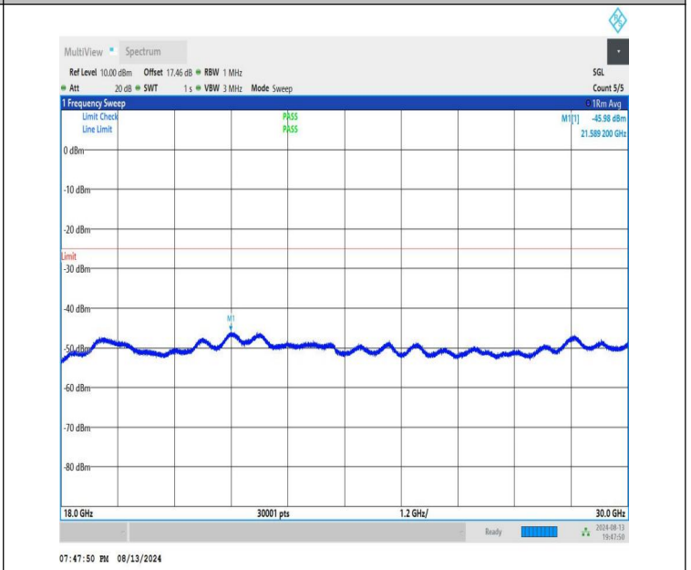
NTNV-n41-PC1.5-30-100-H-CP-QPSK-Edge_1RB_Right-18000-30000-30 000-PASS
