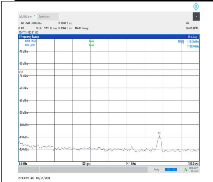
NTNV-n41-PC1.5-30-15-H-CP-QPSK-Edge_1RB_Left-0.009-0.15-PASS
