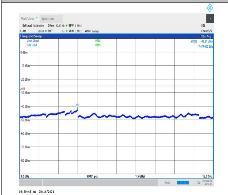
NTNV-n41-PC1.5-30-20-L-CP-QPSK-Edge_1RB_Right-3000-180 00-PASS
