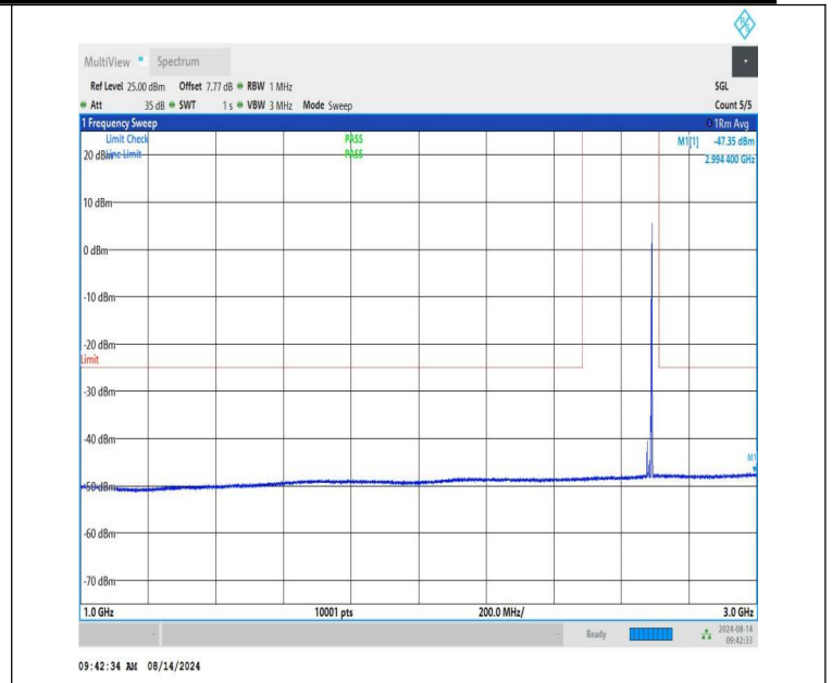
NTNV-n41-PC1.5-30-15-H-CP-QPSK-Edge_1RB_Right-1000-3000-PASS
