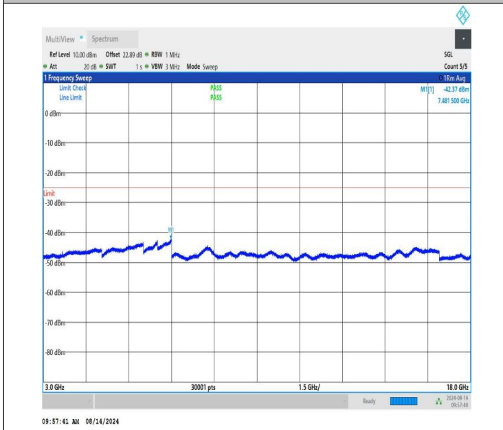
NTNV-n41-PC1.5-30-15-L-CP-QPSK-Edge_1RB_Right-3000-180 00-PASS
