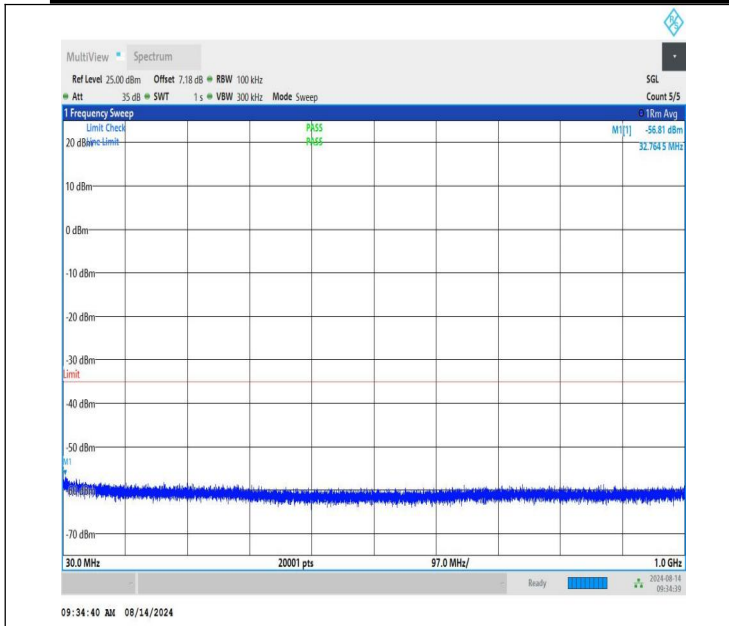
NTNV-n41-PC1.5-30-10-L-CP-QPSK-Edge_1RB_Right-30-1000-P ASS
