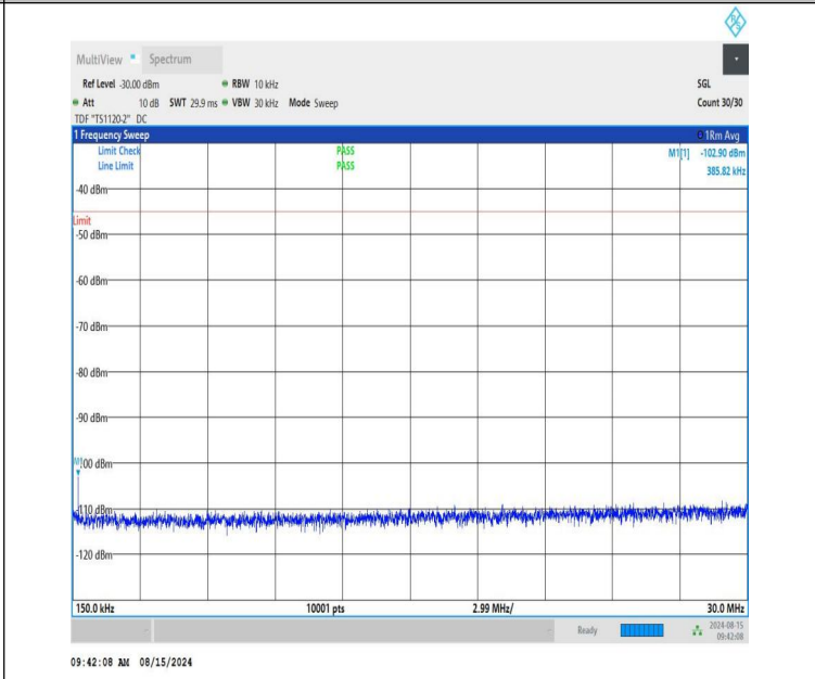
NTNV-n41-PC1.5-30-10-M-CP-QPSK-Edge_1RB_Right-0.15-30-P ASS
