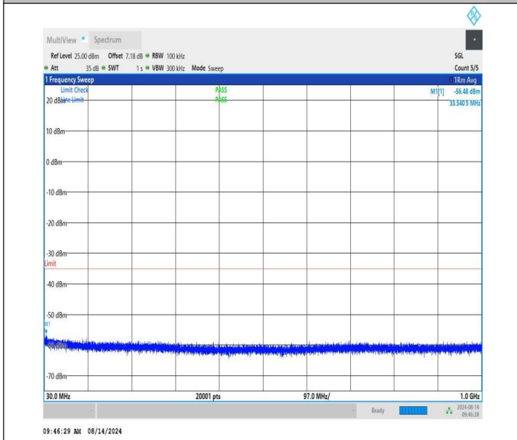
NTNV-n41-PC1.5-30-20-H-CP-QPSK-Edge_1RB_Left-30-1000-PASS
