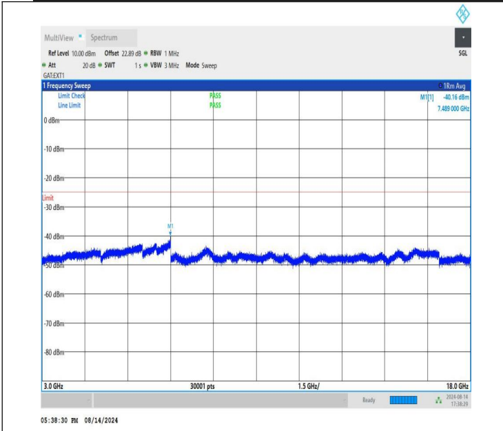
NTNV-n41-PC1.5-30-100-M-CP-QPSK-Edge_1RB_Left-3000-180 00-PASS
