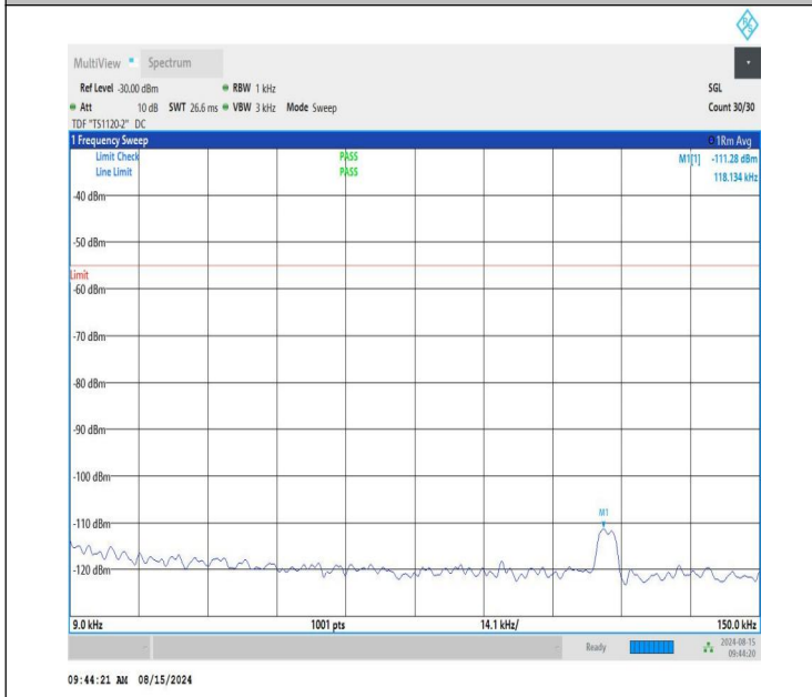
NTNV-n41-PC1.5-30-20-M-CP-QPSK-Edge_1RB_Right-0.009-0.1 5-PASS
