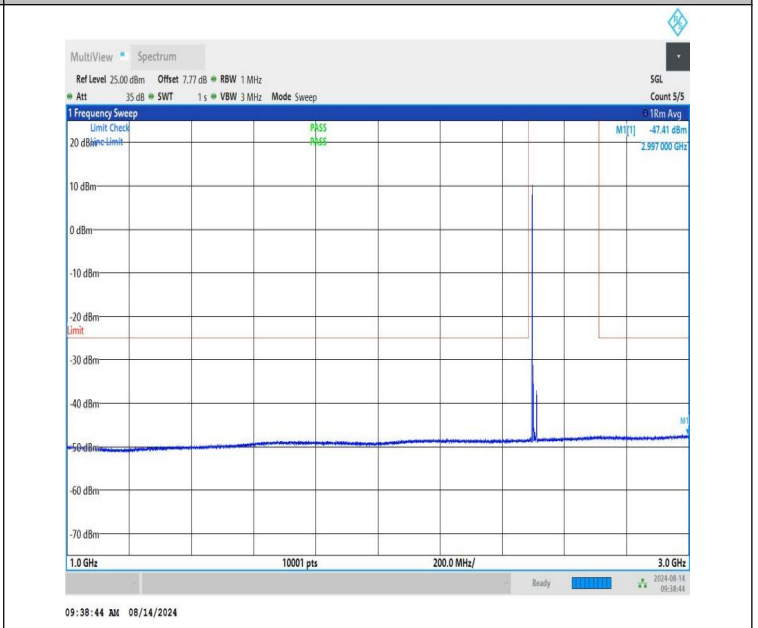
NTNV-n41-PC1.5-30-15-L-CP-QPSK-Edge_1RB_Left-1000-3000-PASS
