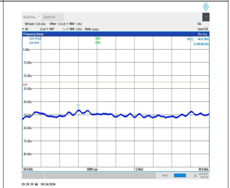
NTNV-n41-PC1.5-30-15-L-CP-QPSK-Edge_1RB_Right-18000-300 00-PASS
