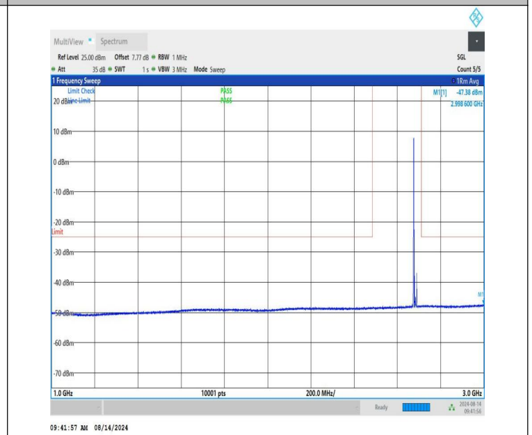
NTNV-n41-PC1.5-30-15-H-CP-QPSK-Edge_1RB_Left-1000-3000-PASS
