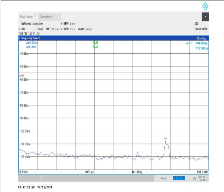
NTVN-n41-PC1.5-30-20-L-CP-QPSK-Edge_1RB_Right-0.009-0.1 5-PASS
