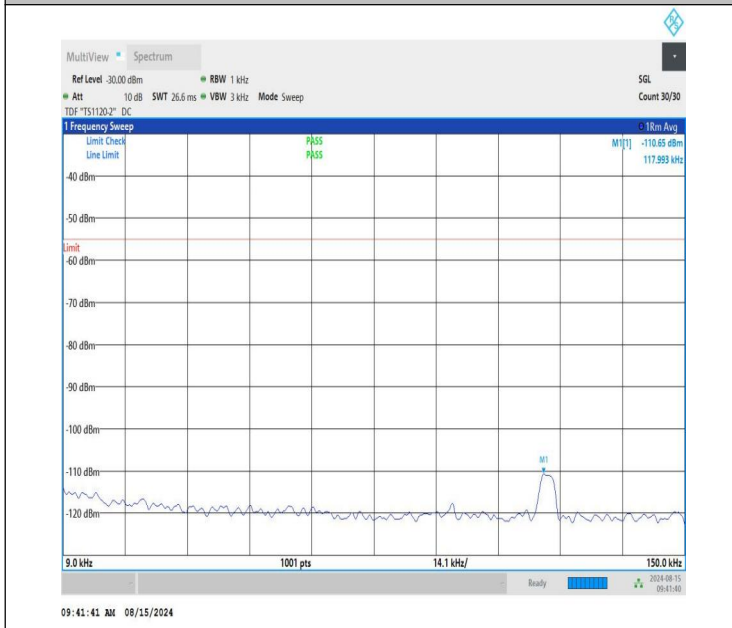
NTVN-n41-PC1.5-30-10-L-CP-QPSK-Edge_1RB_Right-0.009-0.1 5-PASS
