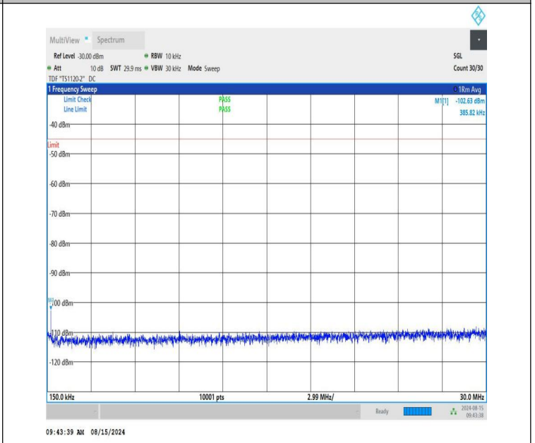
NTNV-n41-PC1.5-30-15-H-CP-QPSK-Edge_1RB_Right-0.15-30-PA SS
