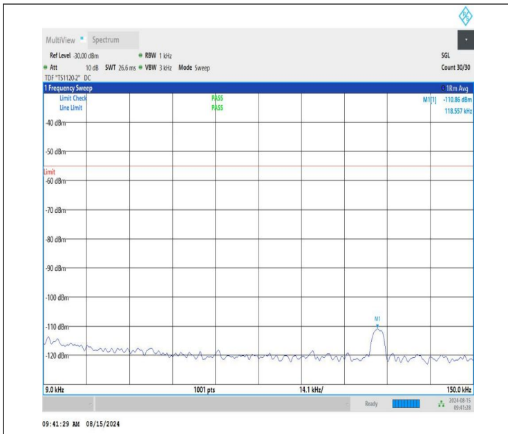
NTNV-n41-PC1.5-30-10-L-CP-QPSK-Edge_1RB_Left-0.009-0.15-PASS
