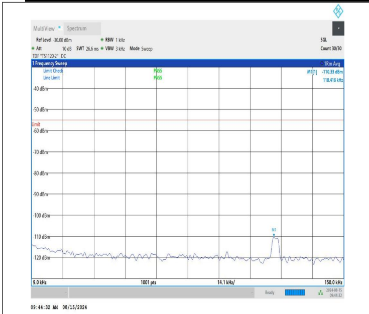
NTNV-n41-PC1.5-30-20-H-CP-QPSK-Edge_1RB_Left-0.009-0.15-PASS
