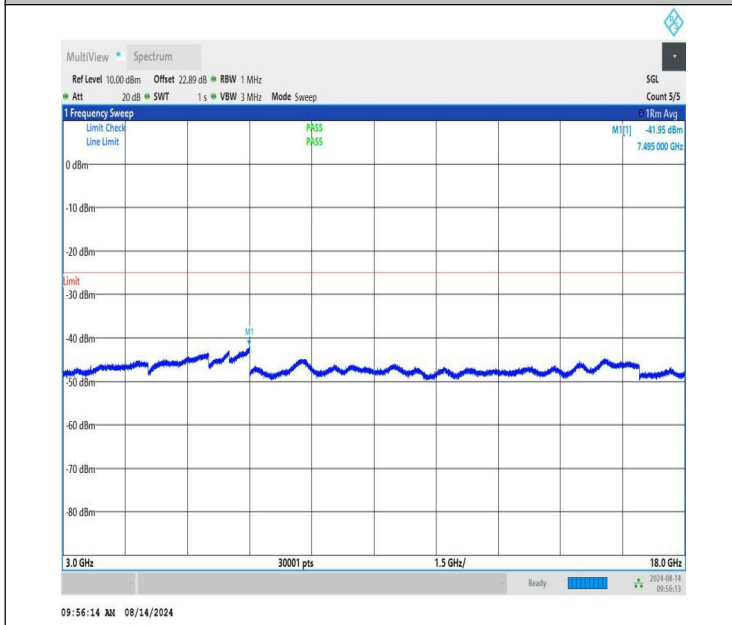
NTNV-n41-PC1.5-30-10-M-CP-QPSK-Edge_1RB_Right-3000-18000-PASS
