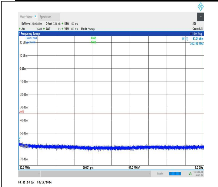
NTNV-n41-PC1.5-30-15-H-CP-QPSK-Edge_1RB_Right-30-1000-PASS
