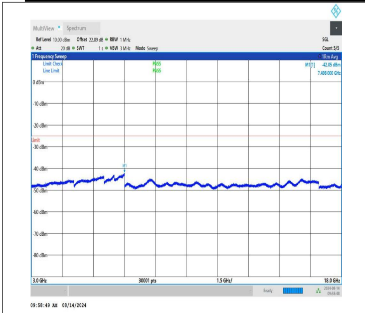
NTNV-n41-PC1.5-30-15-H-CP-QPSK-Edge_1RB_Left-3000-1800 0-PASS
