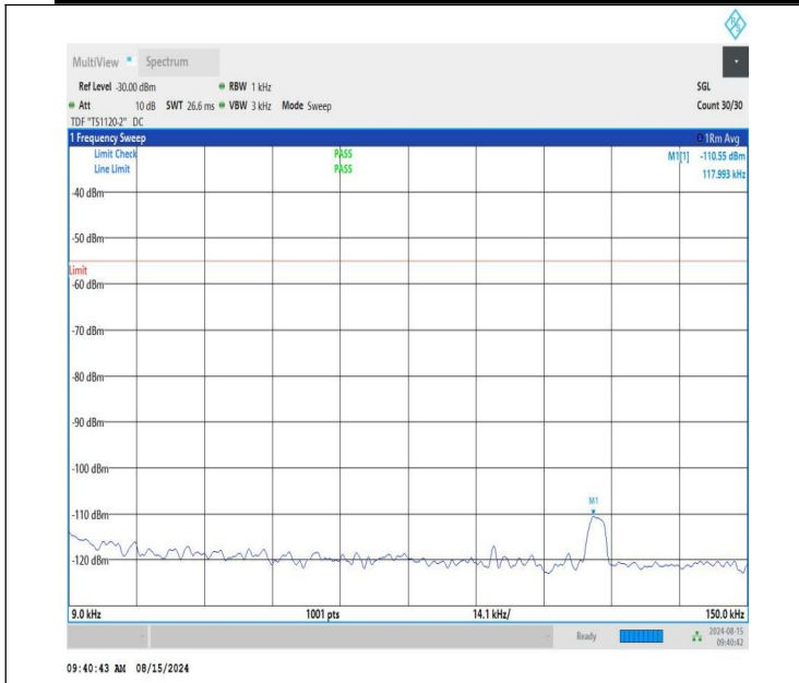
NTNV-n41-PC1.5-30-100-M-CP-QPSK-Edge_1RB_Left-0.009-0.1 5-PASS
