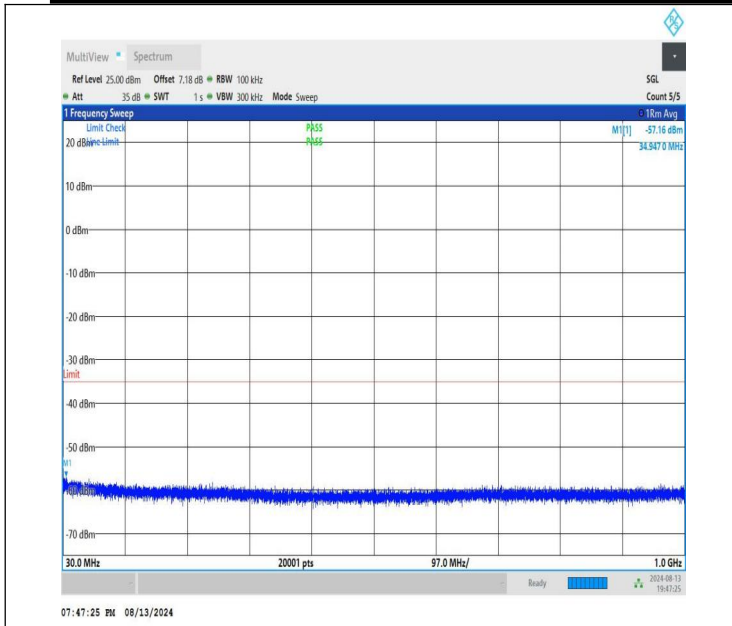
NTNV-n41-PC1.5-30-100-H-CP-QPSK-Edge_1RB_Right-30-1000 -PASS
