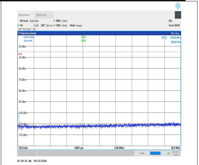
NTNV-n41-PC1.5-30-80-H-CP-QPSK-Edge_1RB_Left-0.15-30-PASS
