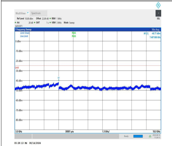
NTNV-n41-PC1.5-30-60-H-CP-QPSK-Edge_1RB_Right-3000-18000-PASS
