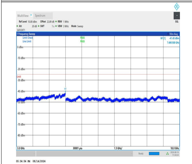
NTNV-n41-PC1.5-30-90-L-CP-QPSK-Edge_1RB_Right-3000-180 00-PASS
