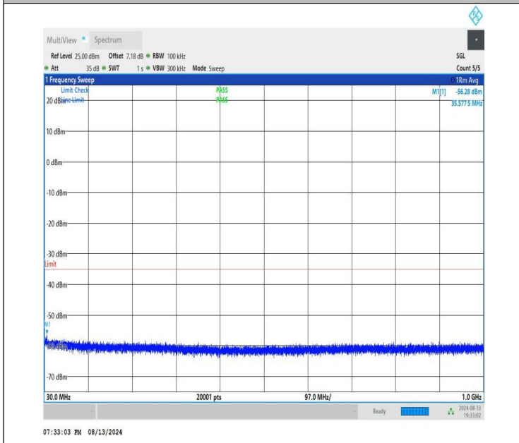
NTNV-n41-PC1.5-30-70-H-CP-QPSK-Edge_1RB_Left-30-1000-PASS
