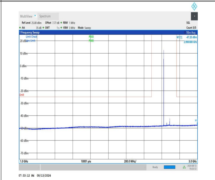
NTNV-n41-PC1.5-30-70-H-CP-QPSK-Edge_1RB_Left-1000-3000-PASS
