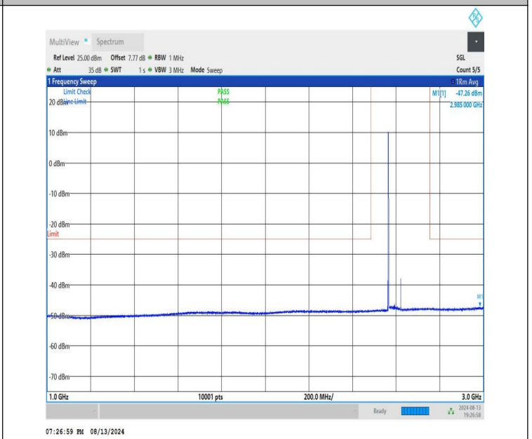
NTNV-n41-PC1.5-30-60-M-CP-QPSK-Edge_1RB_Left-1000-3000-P PASS
