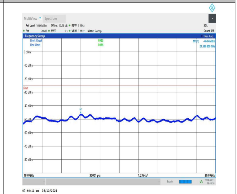
NTNV-n41-PC1.5-30-90-L-CP-QPSK-Edge_1RB_Right-18000-300 00-PASS
