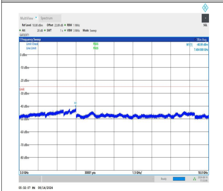
NTNV-n41-PC1.5-30-80-L-CP-QPSK-Edge_1RB_Right-3000-180 00-PASS
