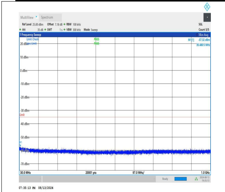
NTNV-n41-PC1.5-30-80-L-CP-QPSK-Edge_1RB_Right-30-1000-P ASS
