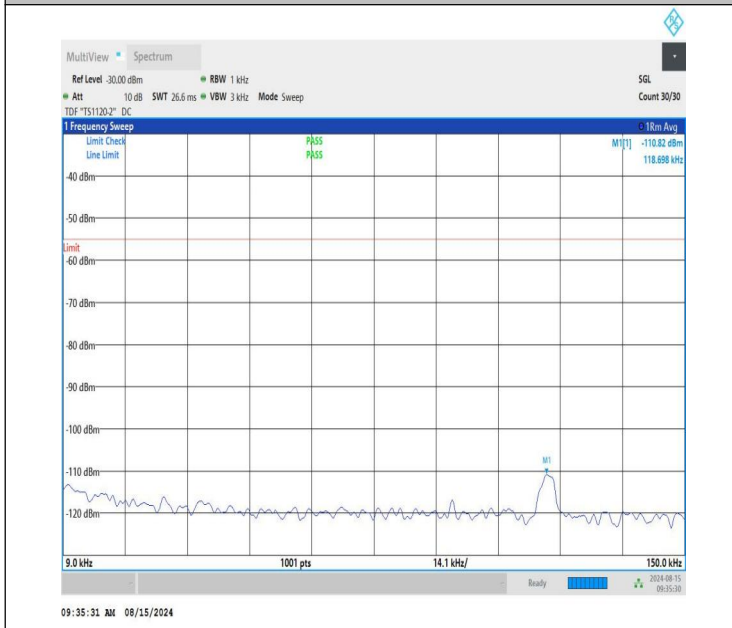
NTNV-n41-PC1.5-30-50-H-CP-QPSK-Edge_1RB_Right-0.009-0.1 5-PASS
