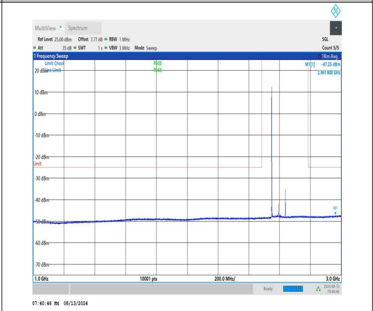
NTNV-n41-PC1.5-30-90-M-CP-QPSK-Edge_1RB_Left-1000-3000-P PASS
