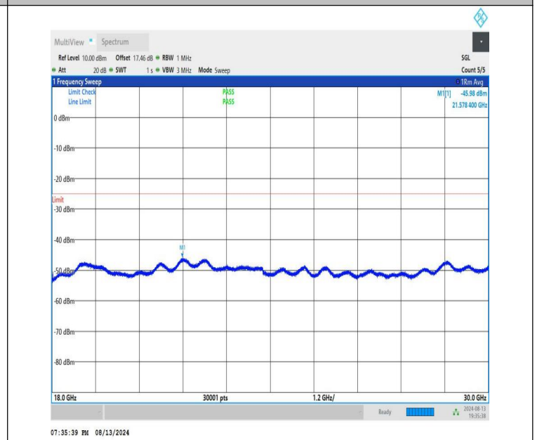
NTNV-n41-PC1.5-30-80-L-CP-QPSK-Edge_1RB_Right-18000-300 00-PASS
