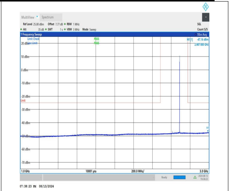
NTNV-n41-PC1.5-30-80-H-CP-QPSK-Edge_1RB_Right-1000-3000-PASS
