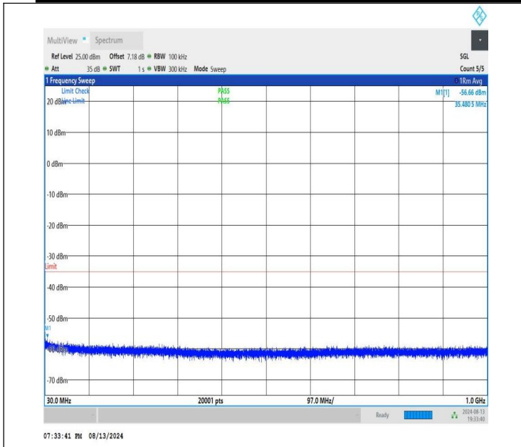
NTNV-n41-PC1.5-30-70-H-CP-QPSK-Edge_1RB_Right-30-1000-PASS
