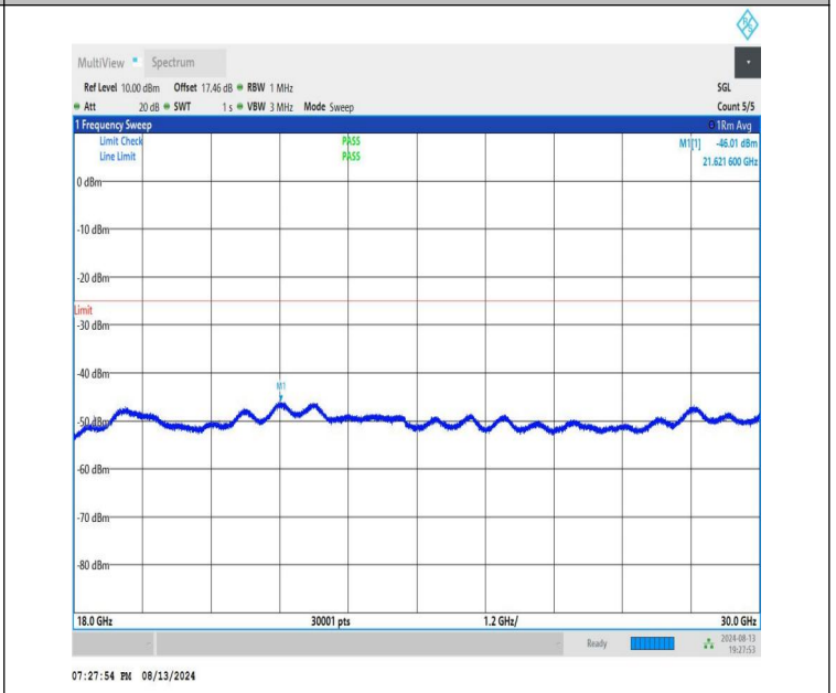
NTNV-n41-PC1.5-30-60-M-CP-QPSK-Edge_1RB_Right-18000-3000-PASS
