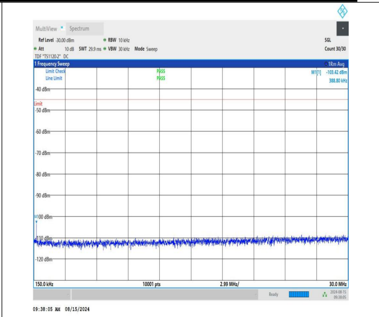
NTNV-n41-PC1.5-30-80-L-CP-QPSK-Edge_1RB_Left-0.15-30-PASS
