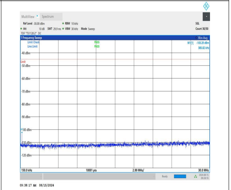
NTVN-n41-PC1.5-30-80-L-CP-QPSK-Edge_1RB_Right-0.15-30-PA SS
