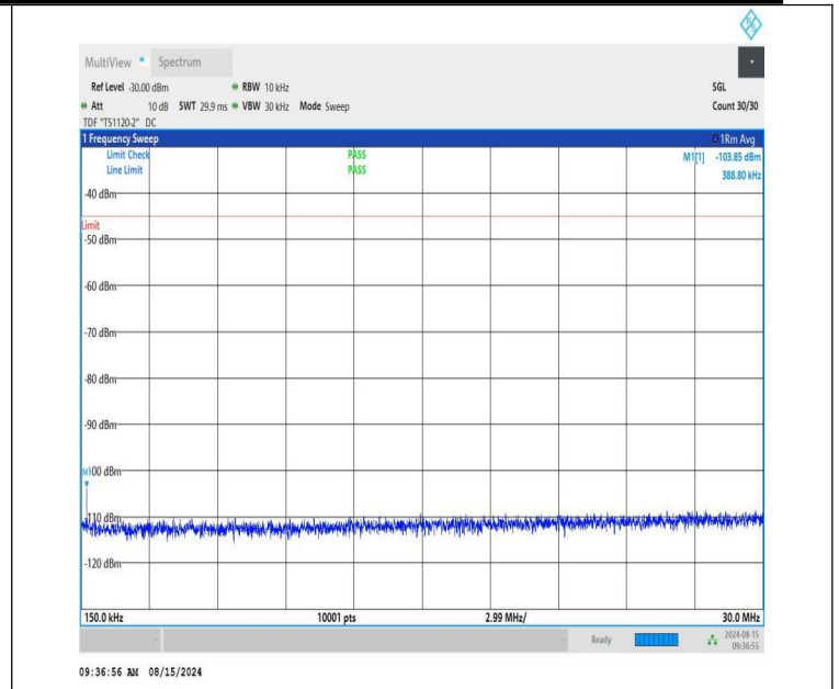
NTNV-n41-PC1.5-30-70-L-CP-QPSK-Edge_1RB_Left-0.15-30-PASS
