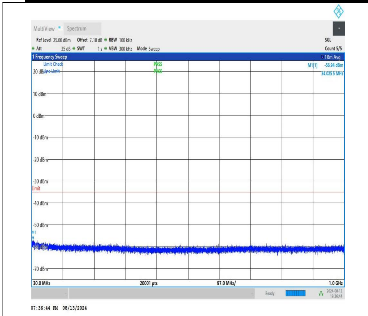
NTNV-n41-PC1.5-30-80-M-CP-QPSK-Edge_1RB_Right-30-1000-PASS
