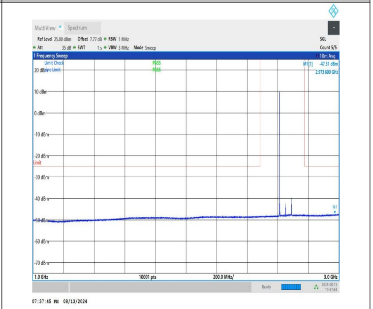
NTNV-n41-PC1.5-30-80-H-CP-QPSK-Edge_1RB_Left-1000-3000-PASS
