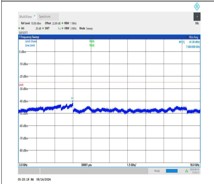
NTNV-n41-PC1.5-30-50-H-CP-QPSK-Edge_1RB_Right-3000-18000-PASS
