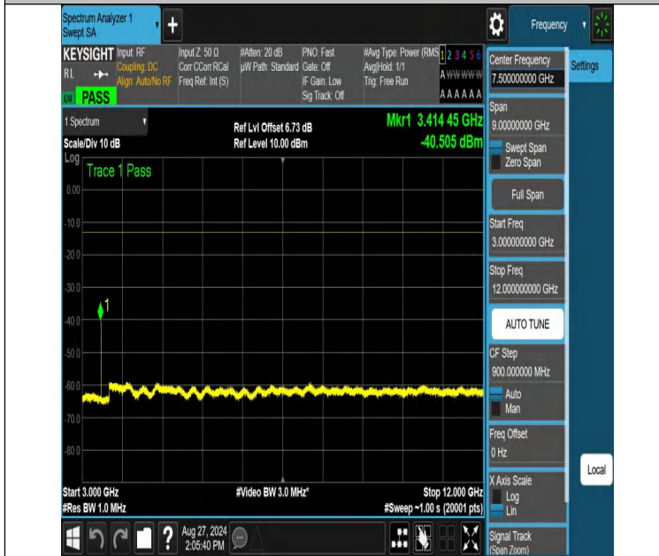
NTNV-n70-PC3-15-10-M-DFT-16QAM-Edge_1RB_Right-3000-12000-PASS
