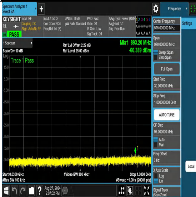
NTNV-n70-PC3-15-10-M-DFT-64QAM-Edge_1RB_Right-30-1000-P ASS
