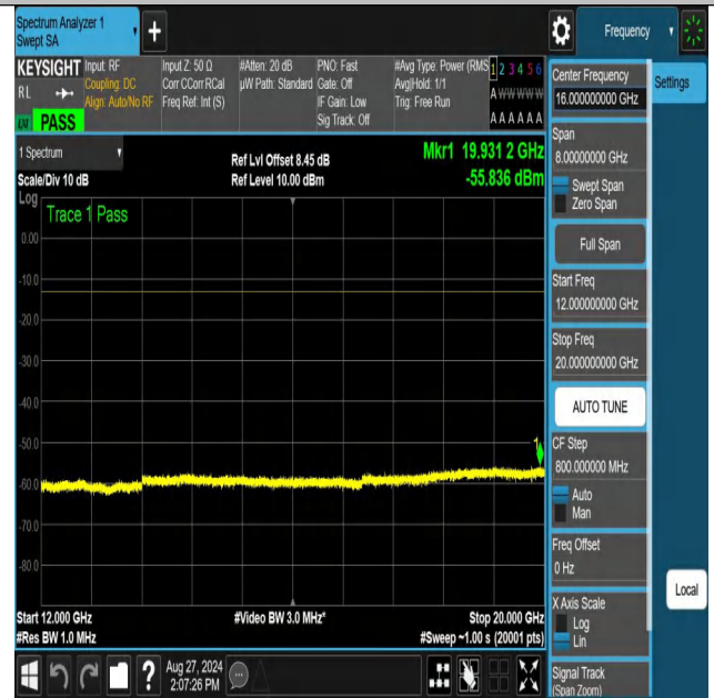
NTNV-n70-PC3-15-10-M-DFT-64QAM-Edge_1RB_Right-12000-200 00-PASS
