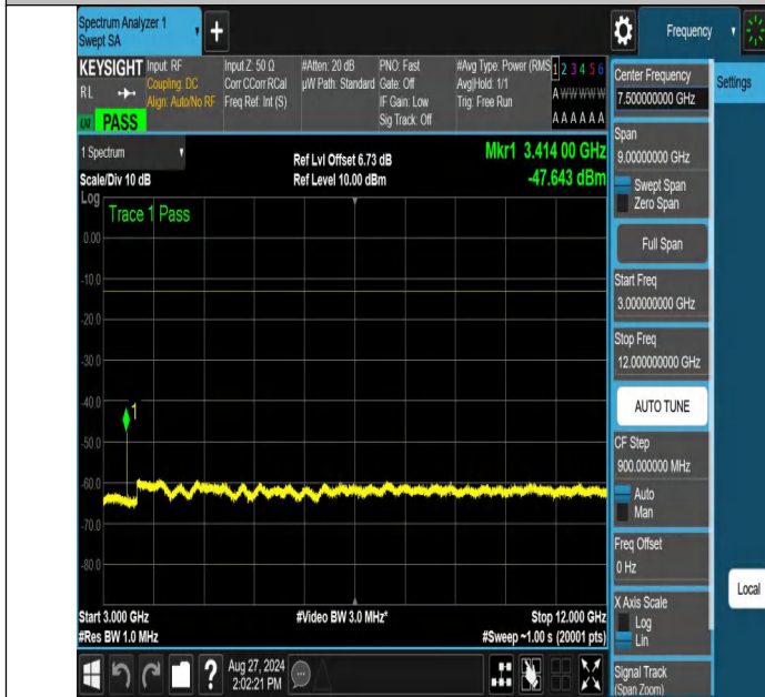
NTNV-n70-PC3-15-10-M-DFT-BPSK-Edge_1RB_Right-3000-12000 -PASS
