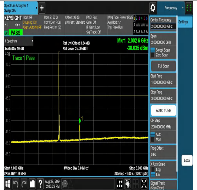
NTNV-n70-PC3-15-10-M-DFT-64QAM-Edge_1RB_Left-1000-3000-P
