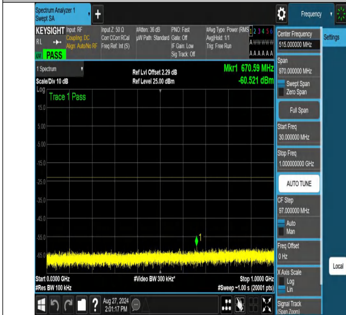
NTNV-n70-PC3-15-10-M-DFT-BPSK-Edge_1RB_Left-30-1000-PAS S
