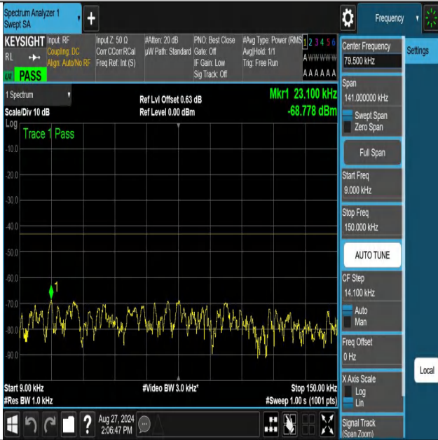
NTNV-n70-PC3-15-10-M-DFT-64QAM-Edge_1RB_Right-0.009-0.1 5-PASS
