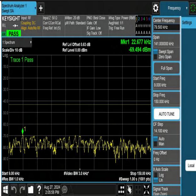
NTNV-n70-PC3-15-10-M-DFT-64QAM-Edge_1RB_Left-0.009-0.15-PASS
