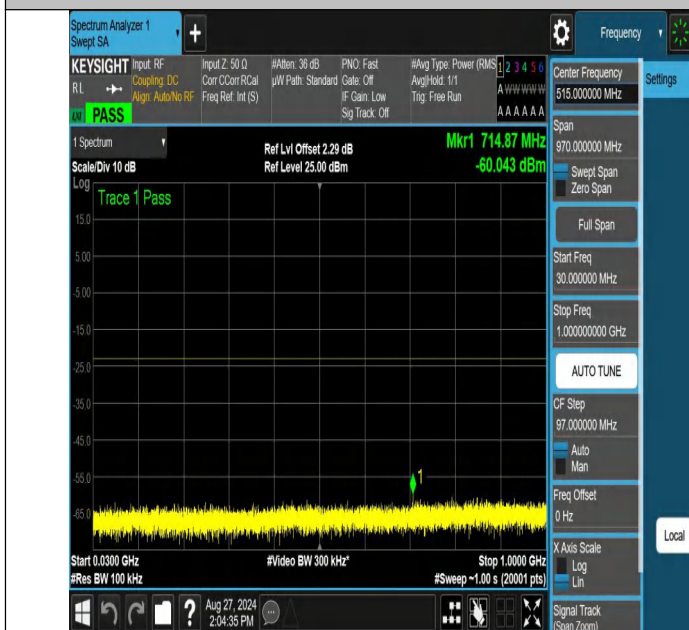
NTNV-n70-PC3-15-10-M-DFT-16QAM-Edge_1RB_Left-30-1000-PA
