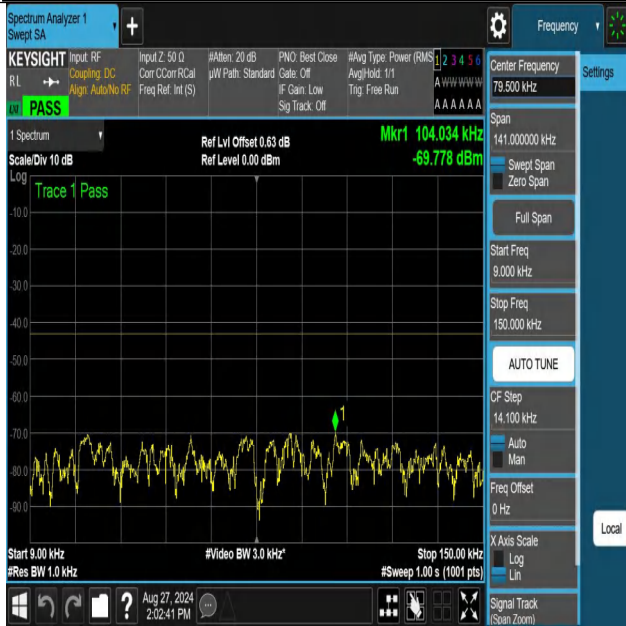
NTNV-n70-PC3-15-10-M-DFT-QPSK-Edge_1RB_Left-0.009-0.15-P ASS
