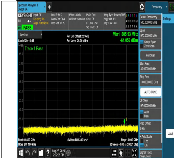
NTNV-n70-PC3-15-10-M-DFT-BPSK-Edge_1RB_Right-30-1000-PA SS
