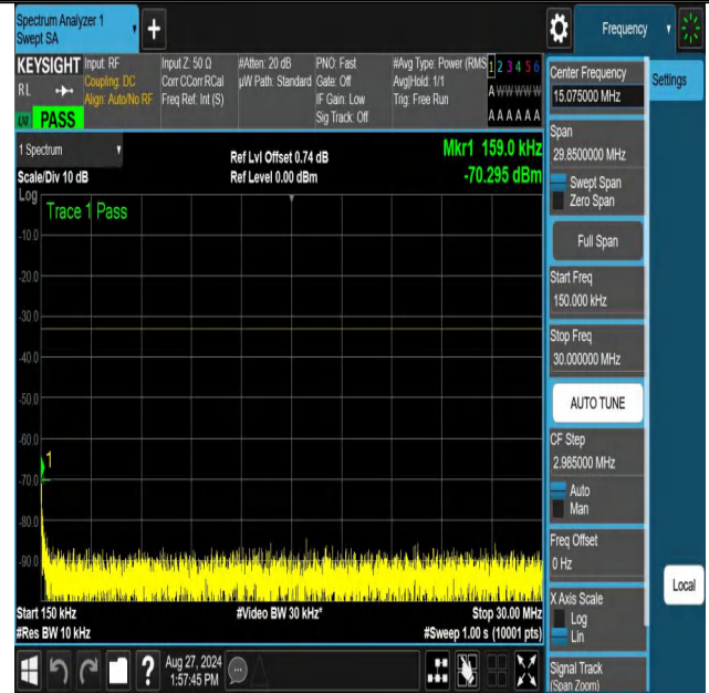
NTNV-n70-PC3-15-5-M-DFT-64QAM-Edge_1RB_Left-0.15-30-PASS
