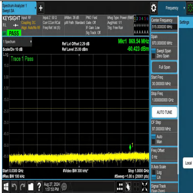
NTNV-n70-PC3-15-5-M-DFT-64QAM-Edge_1RB_Left-30-1000-PAS S
