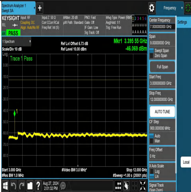
NTNV-n70-PC3-15-10-M-DFT-BPSK-Edge_1RB_Left-3000-12000- PASS
