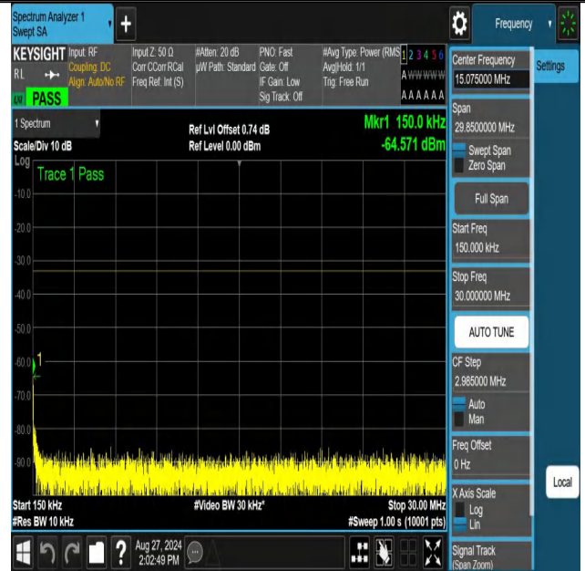
NTNV-n70-PC3-15-10-M-DFT-QPSK-Edge_1RB_Left-0.15-30-PASS
