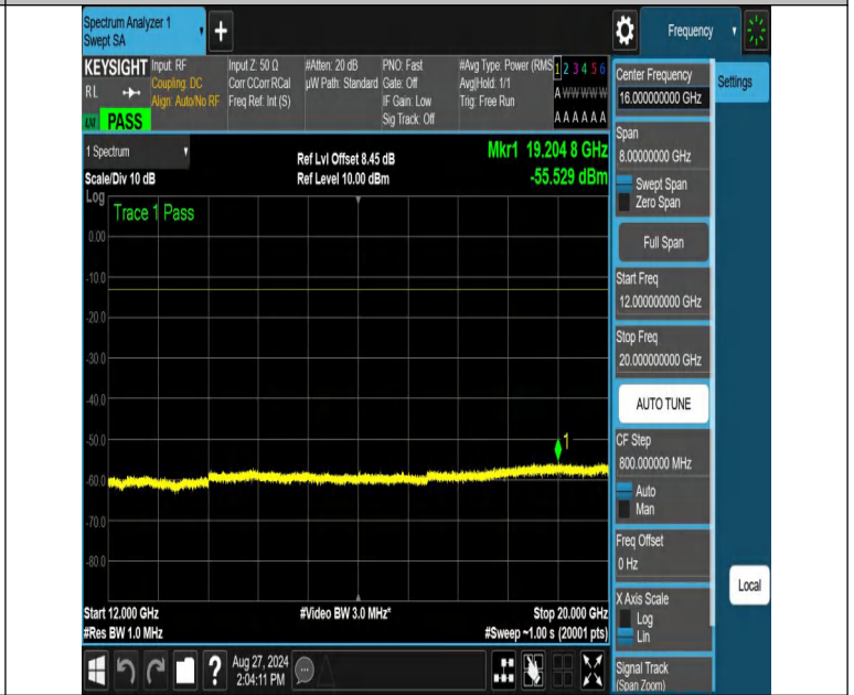
NTNV-n70-PC3-15-10-M-DFT-QPSK-Edge_1RB_Right-12000-2000 0-PASS
