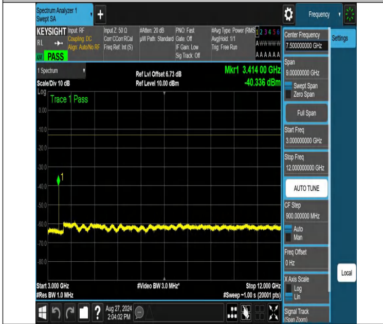
NTNV-n70-PC3-15-10-M-DFT-QPSK-Edge_1RB_Right-3000-12000 -PASS
