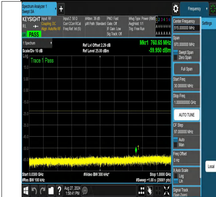
NTNV-n70-PC3-15-5-M-DFT-64QAM-Edge_1RB_Right-30-1000-PA SS
