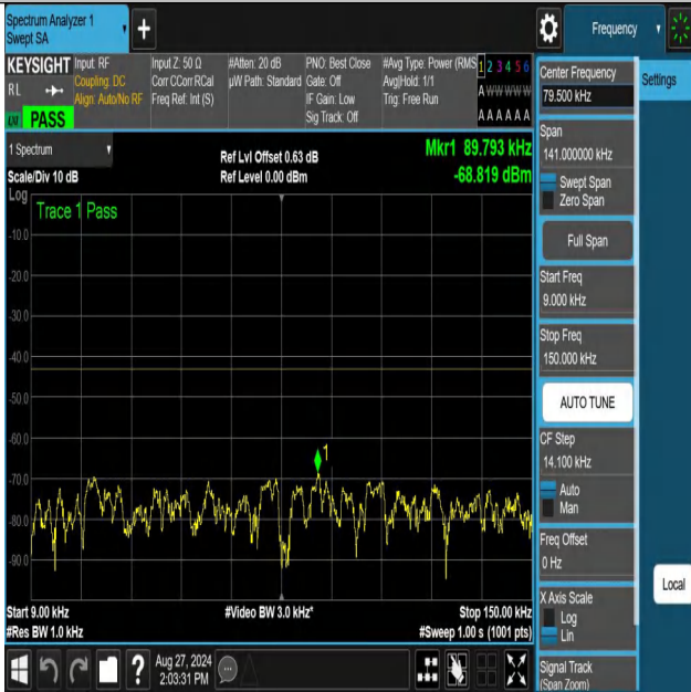
NTNV-n70-PC3-15-10-M-DFT-QPSK-Edge_1RB_Right-0.009-0.15- PASS
