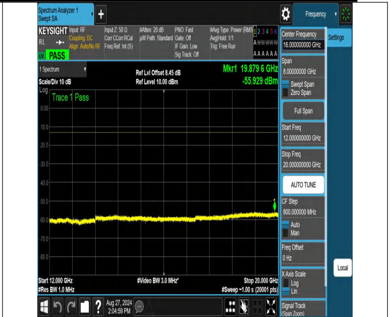
NTNV-n70-PC3-15-10-M-DFT-16QAM-Edge_1RB_Left-12000-20000 -PASS
