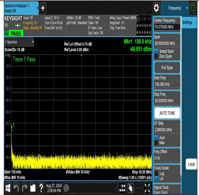
NTNV-n70-PC3-15-10-M-DFT-64QAM-Edge_1RB_Right-0.15-30-PA SS
