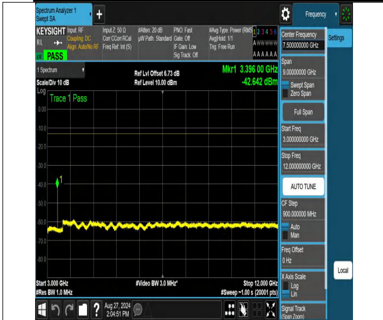
NTNV-n70-PC3-15-10-M-DFT-16QAM-Edge_1RB_Left-3000-12000 -PASS
