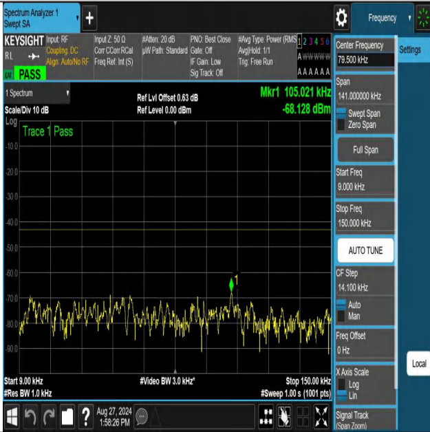
NTNV-n70-PC3-15-5-M-DFT-64QAM-Edge_1RB_Right-0.009-0.15- PASS
