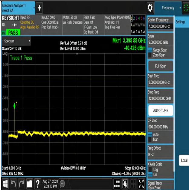
NTNV-n70-PC3-15-10-M-DFT-QPSK-Edge_1RB_Left-3000-12000- PASS
