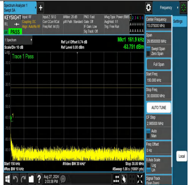
NTNV-n70-PC3-15-10-M-DFT-QPSK-Edge_1RB_Right-0.15-30-PAS S
