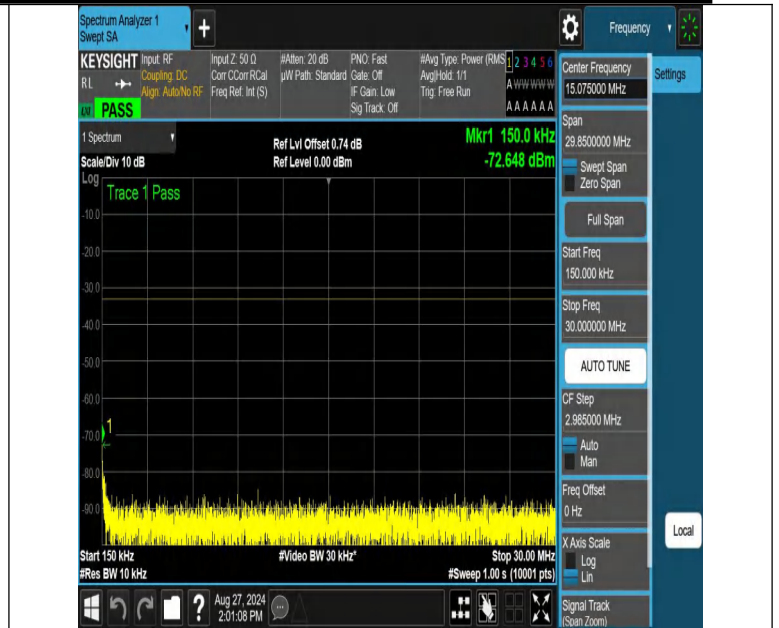
NTNV-n70-PC3-15-10-M-DFT-BPSK-Edge_1RB_Left-0.15-30-PASS
