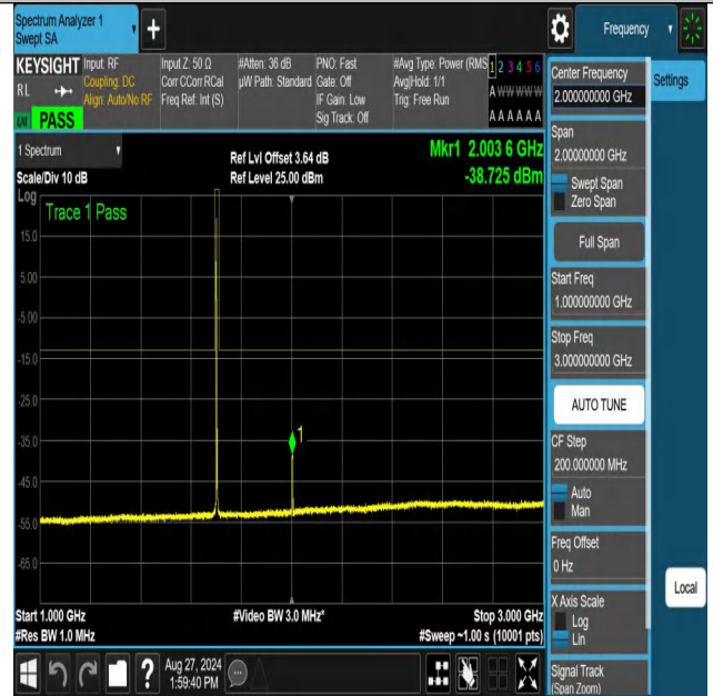
NTNV-n70-PC3-15-5-M-DFT-256QAM-Edge_1RB_Left-1000-3000-PASS
