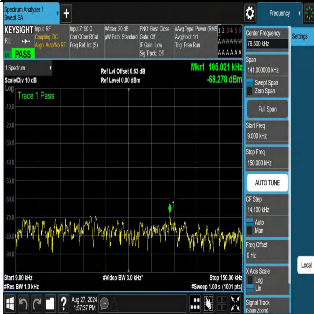
NTNV-n70-PC3-15-5-M-DFT-64QAM-Edge_1RB_Left-0.009-0.15-P ASS
