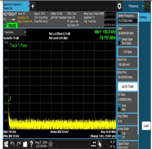
NTNV-n70-PC3-15-10-M-DFT-BPSK-Edge_1RB_Right-0.15-30-PAS S
