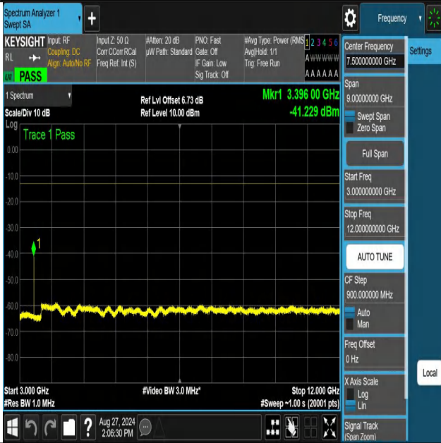
NTNV-n70-PC3-15-10-M-DFT-64QAM-Edge_1RB_Left-3000-12000 -PASS
