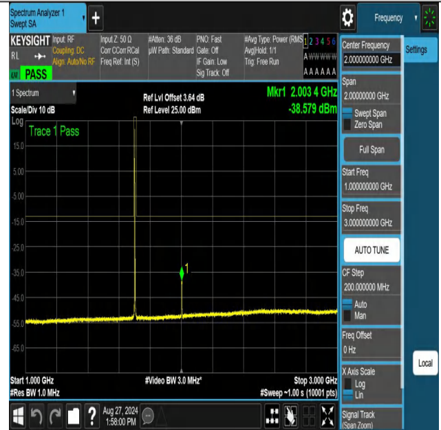
NTNV-n70-PC3-15-5-M-DFT-64QAM-Edge_1RB_Left-1000-3000-PA SS
