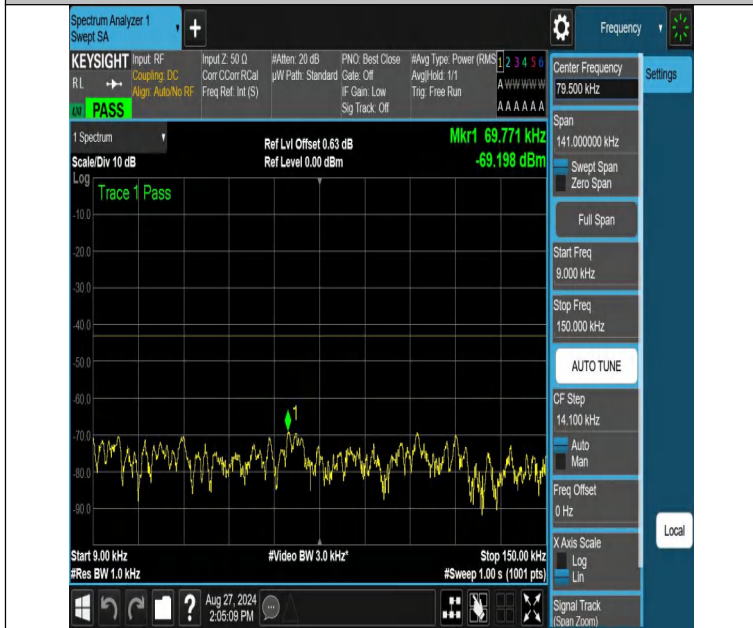
NTNV-n70-PC3-15-10-M-DFT-16QAM-Edge_1RB_Right-0.009-0.1 5-PASS
