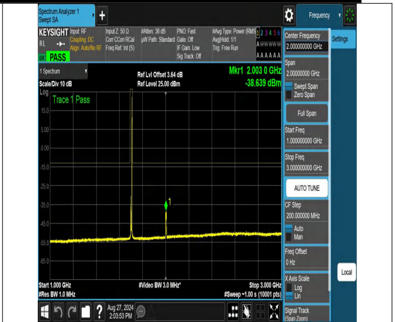
NTNV-n70-PC3-15-10-M-DFT-QPSK-Edge_1RB_Right-1000-3000-P ASS
