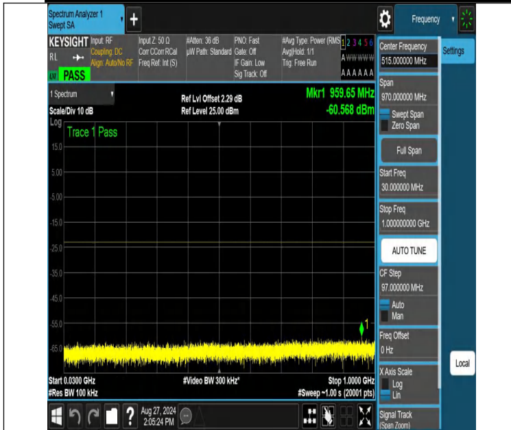
NTNV-n70-PC3-15-10-M-DFT-16QAM-Edge_1RB_Right-30-1000-P ASS
