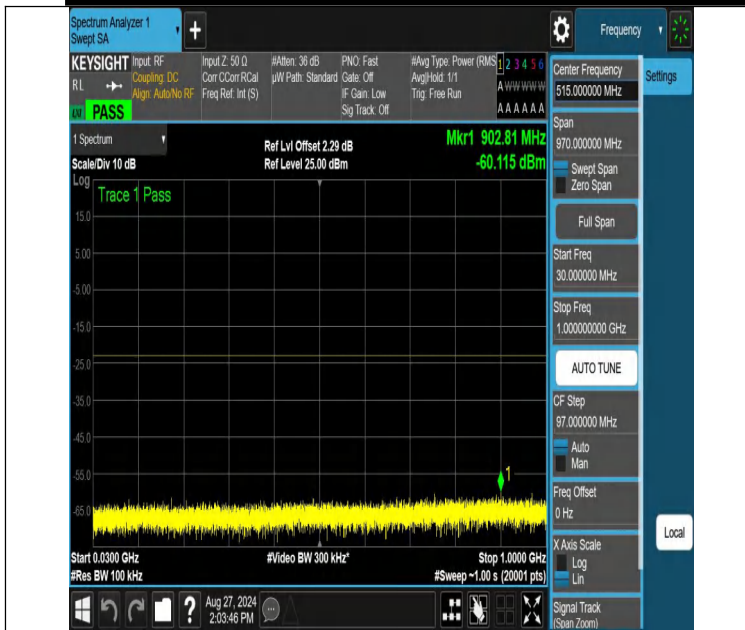
NTNV-n70-PC3-15-10-M-DFT-QPSK-Edge_1RB_Right-30-1000-PA SS
