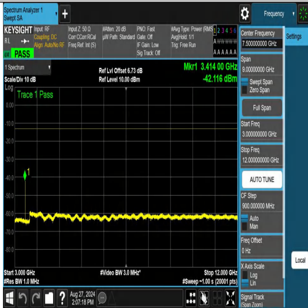
NTNV-n70-PC3-15-10-M-DFT-64QAM-Edge_1RB_Right-3000-120 00-PASS
