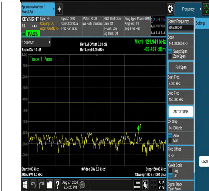
NTNV-n70-PC3-15-10-M-DFT-16QAM-Edge_1RB_Left-0.009-0.15-PASS
