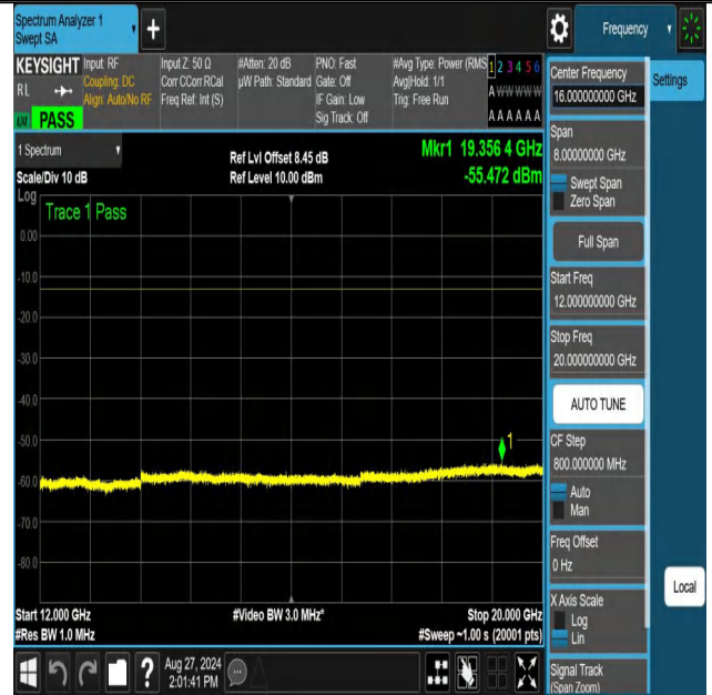
NTNV-n70-PC3-15-10-M-DFT-BPSK-Edge_1RB_Left-12000-20000- PASS
