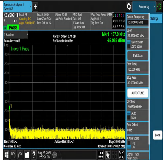
NTNV-n70-PC3-15-5-M-DFT-256QAM-Edge_1RB_Left-0.15-30-PASS
