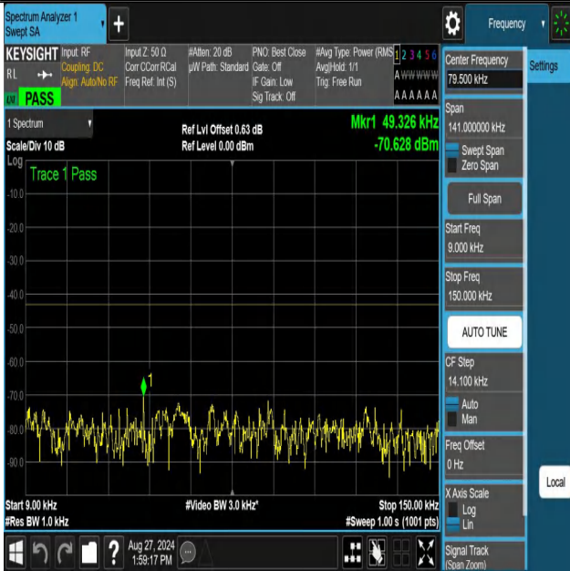
NTNV-n70-PC3-15-5-M-DFT-256QAM-Edge_1RB_Left-0.009-0.15-PASS
