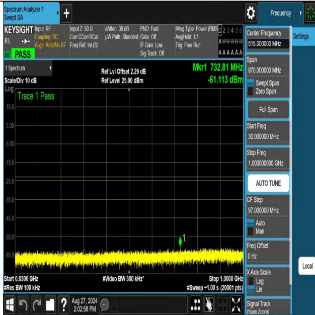
NTNV-n70-PC3-15-10-M-DFT-QPSK-Edge_1RB_Left-30-1000-PAS S
