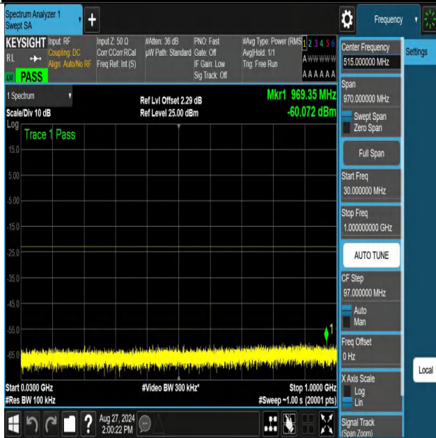
NTVN-n70-PC3-15-5-M-DFT-256QAM-Edge_1RB_Right-30-1000-P ASS
