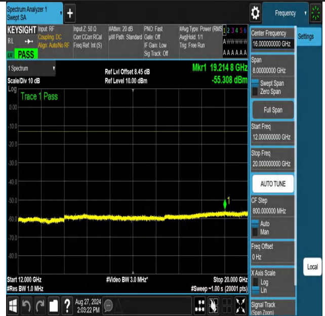
NTNV-n70-PC3-15-10-M-DFT-QPSK-Edge_1RB_Left-12000-20000- PASS
