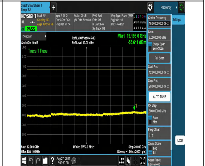
NTNV-n70-PC3-15-10-M-DFT-BPSK-Edge_1RB_Right-12000-20000 -PASS
