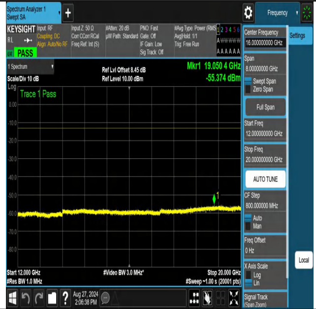
NTNV-n70-PC3-15-10-M-DFT-64QAM-Edge_1RB_Left-12000-20000 -PASS
