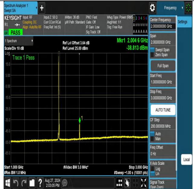
NTNV-n70-PC3-15-10-M-DFT-QPSK-Edge_1RB_Left-1000-3000-PA SS
