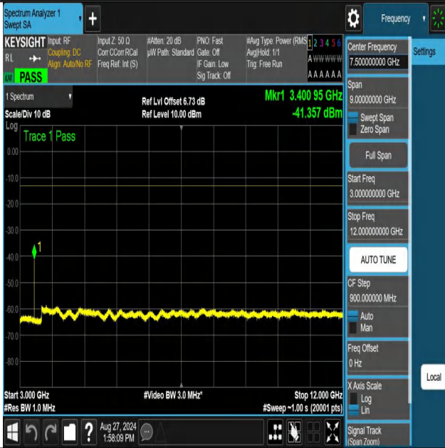
NTNV-n70-PC3-15-5-M-DFT-64QAM-Edge_1RB_Left-3000-12000- PASS
