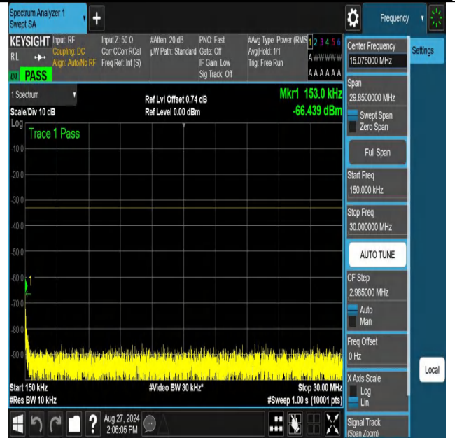
NTNV-n70-PC3-15-10-M-DFT-64QAM-Edge_1RB_Left-0.15-30-PASS
