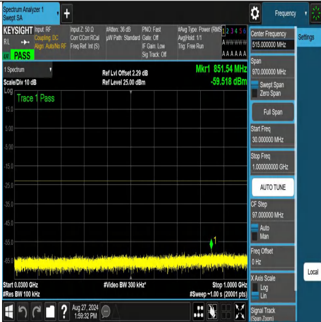
NTNV-n70-PC3-15-5-M-DFT-256QAM-Edge_1RB_Left-30-1000-PASS
