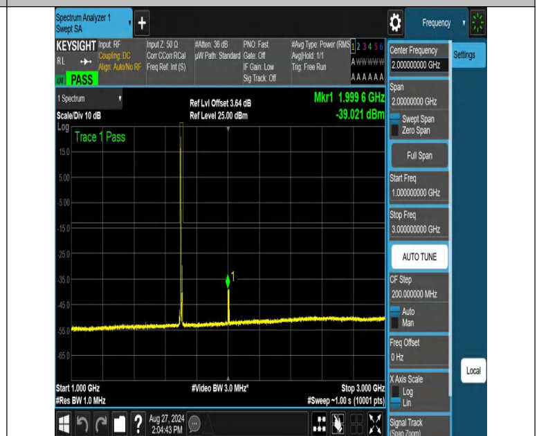
NTNV-n70-PC3-15-10-M-DFT-16QAM-Edge_1RB_Left-1000-3000-P
