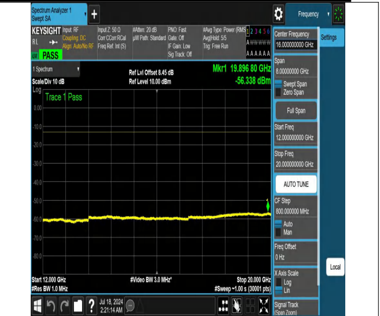
NTNV-DC_12A_n66A-PC3-15-5+40-M+M-N/A-N/A-DFT-QPSK-Edge_1RB_Left-12000-20000-PASS
