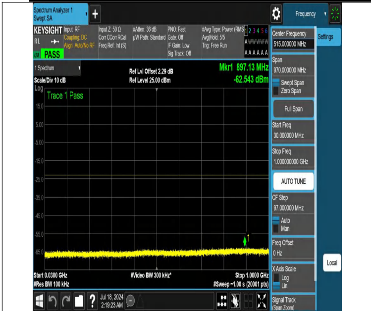
NTNV-DC_12A_n66A-PC3-15-5+40-M+M-N/A-N/A-DFT-PI2BPSK- Edge_1RB_Right-30-1000-PASS
