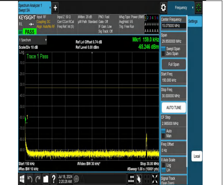
NTNV-DC_12A_n66A-PC3-15-5+40-M+M-N/A-N/A-DFT-QPSK-Edge_1RB_Left-0.15-30-PASS
