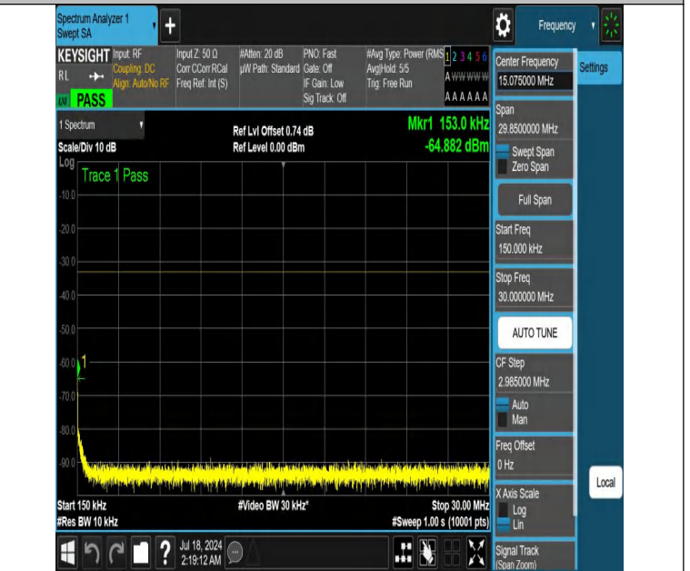
NTNV-DC_12A_n66A-PC3-15-5+40-M+M-N/A-N/A-DFT-PI2BPSK-E dge_1RB_Right-0.15-30-PASS
