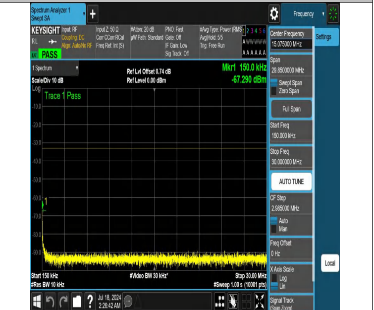
NTNV-DC_12A_n66A-PC3-15-5+40-M+H-N/A-N/A-DFT-QPSK-Edge e_1RB_Right-0.15-30-PASS
