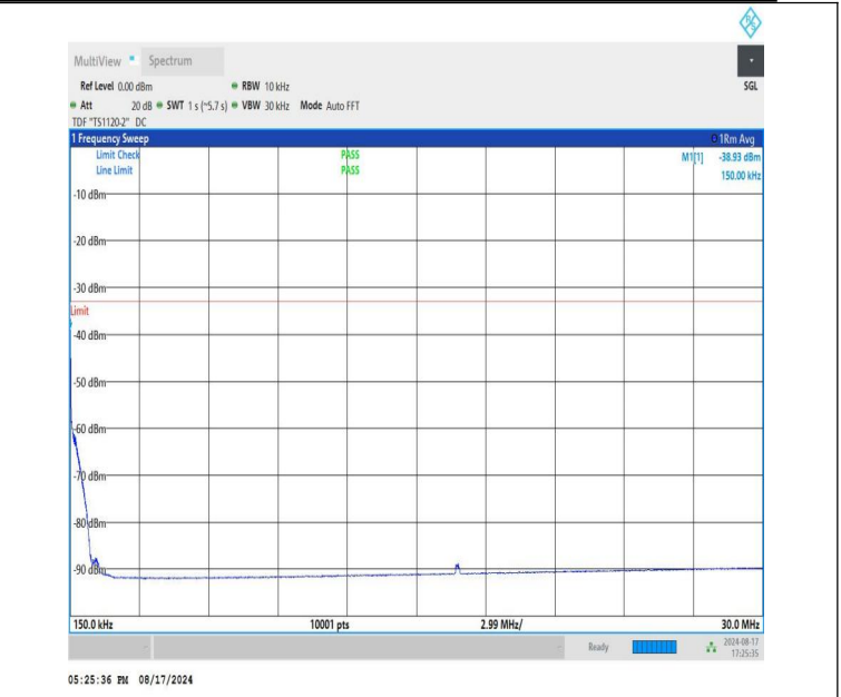
NTNV-DC_12A-n66A-PC3-15-5+35-M+L-QPSK-IDLE-DFT-QPSK-E dge_1RB_Left-0.15-30-PASS
