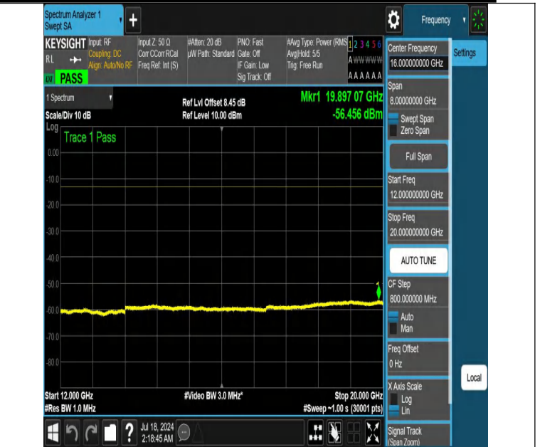
NTNV-DC_12A_n66A-PC3-15-5+40-M+M-N/A-N/A-DFT-PI2BPSK-E dge_1RB_Left-12000-20000-PASS
