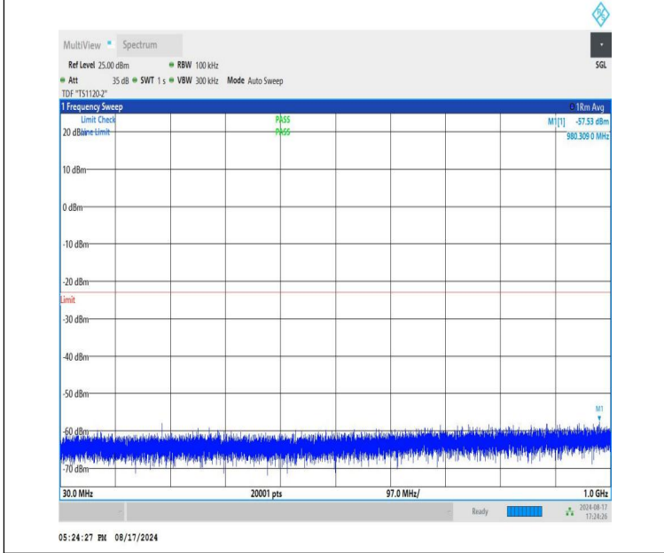
NTNV-DC_12A-n66A-PC3-15-5+35-M+L-QPSK-IDLE-DFT-BPSK-Edge_1RB_Left-30-1000-PASS
