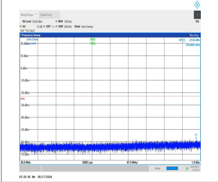
NTNV-DC_12A-n66A-PC3-15-5+35-M+L-QPSK-IDLE-DFT-QPSK-Edge_1RB_Left-30-1000-PASS
