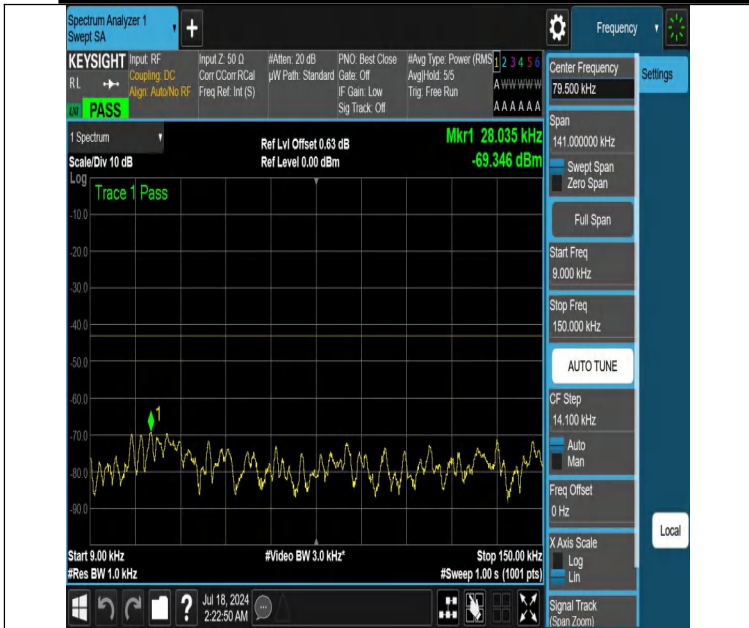
NTNV-DC_12A_n66A-PC3-15-5+40-M+H-N/A-N/A-DFT-PI2BPSK-Edge_1RB_Left-0.009-0.15-PASS
