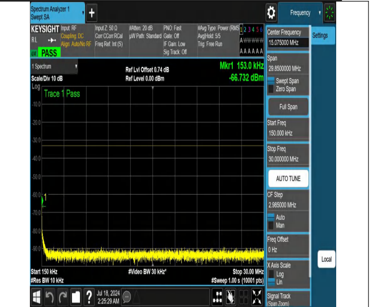
NTNV-DC_12A_n66A-PC3-15-5+40-M+H-N/A-N/A-DFT-QPSK-Edge e_1RB_Left-0.15-30-PASS
