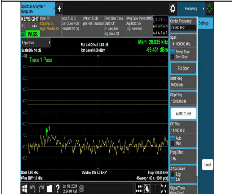
NTNV-DC_12A_n66A-PC3-15-5+40-M+H-N/A-N/A-DFT-PI2BPSK-Edge_1RB_Right-0.009-0.15-PASS
