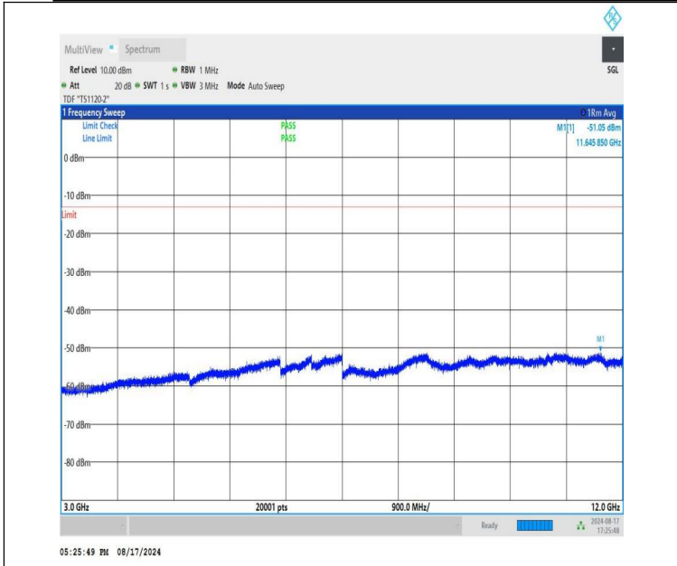
NTNV-DC_12A-n66A-PC3-15-5+35-M+L-QPSK-IDLE-DFT-QPSK-Edge_1RB_Left-3000-12000-PASS
