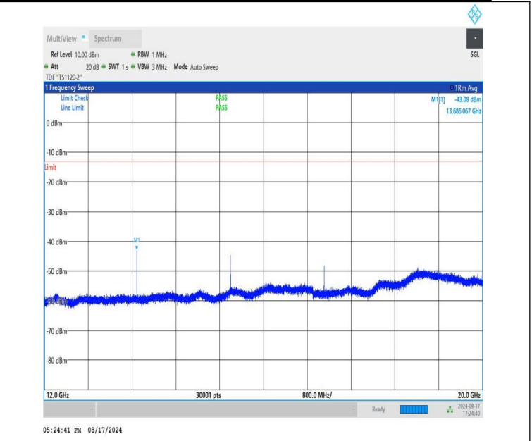
NTNV-DC_12A-n66A-PC3-15-5+35-M+L-QPSK-IDLE-DFT-BPSK-E dge_1RB_Left-12000-20000-PASS
