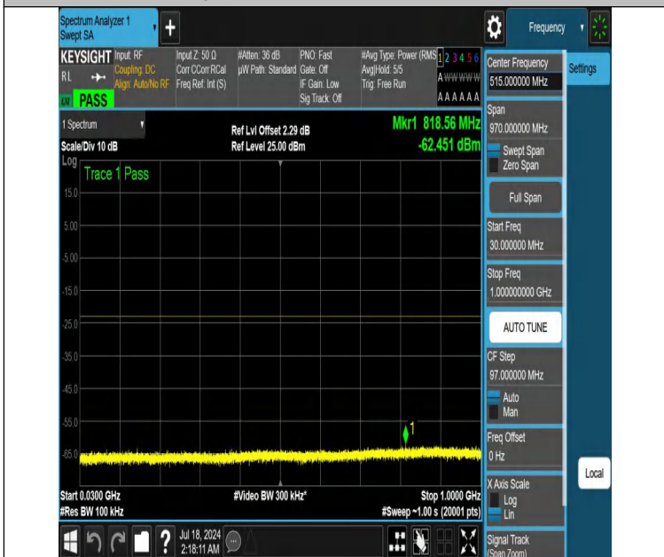
NTNV-DC_12A_n66A-PC3-15-5+40-M+M-N/A-N/A-DFT-PI2BPSK-Edge_1RB_Left-30-1000-PASS
