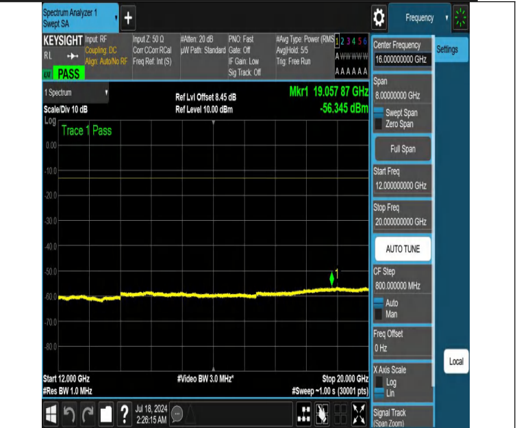
NTNV-DC_12A_n66A-PC3-15-5+40-M+H-N/A-N/A-DFT-QPSK-Edge e_1RB_Left-12000-20000-PASS
