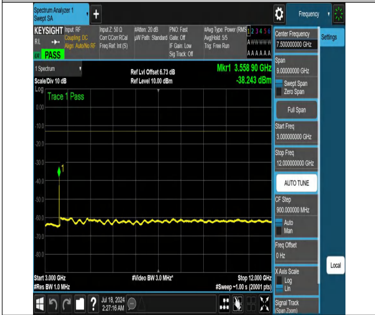
NTNV-DC_12A_n66A-PC3-15-5+40-M+H-N/A-N/A-DFT-QPSK-Edge e_1RB_Right-3000-12000-PASS
