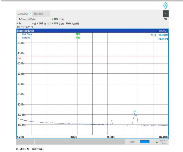
NTNV-DC_12A-n66A-PC3-15-5+35-M+L-QPSK-IDLE-DFT-QPSK-Edge_1RB_Right-0.009-0.15-PASS
