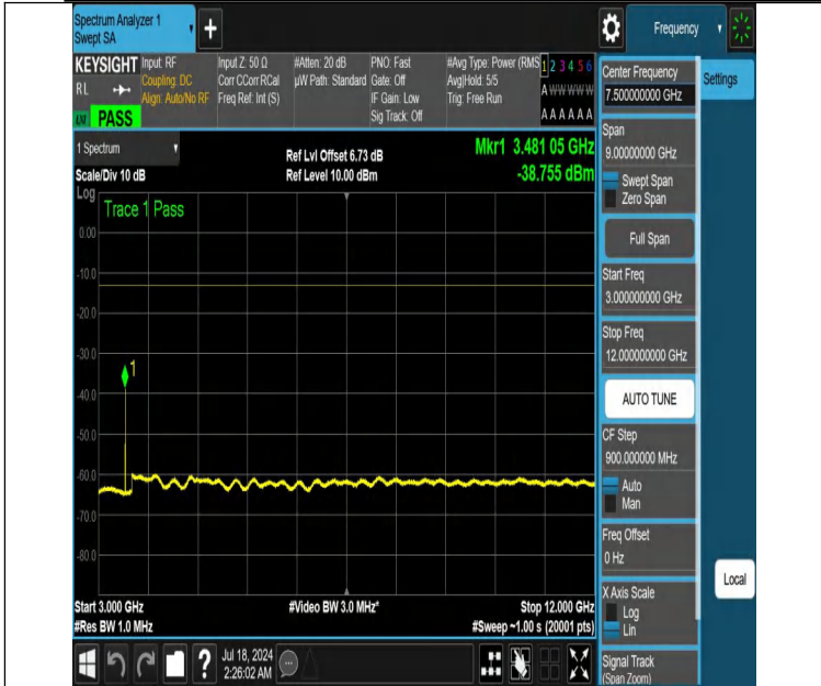
NTNV-DC_12A_n66A-PC3-15-5+40-M+H-N/A-N/A-DFT-QPSK-Edge e_1RB_Left-3000-12000-PASS
