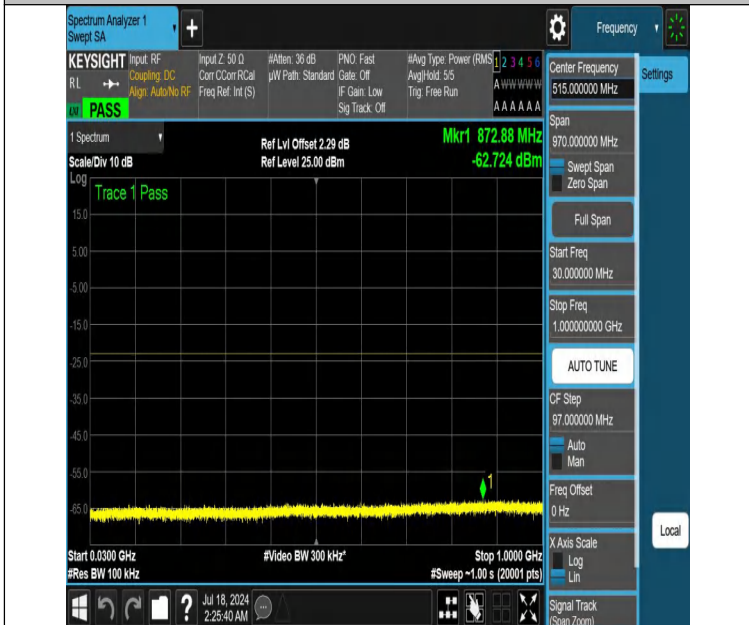
NTNV-DC_12A_n66A-PC3-15-5+40-M+H-N/A-N/A-DFT-QPSK-Edge e_1RB_Left-30-1000-PASS
