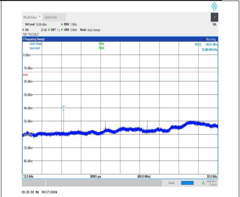
NTNV-DC_12A-n66A-PC3-15-5+35-M+L-QPSK-IDLE-DFT-QPSK-E dge_1RB_Left-12000-20000-PASS
