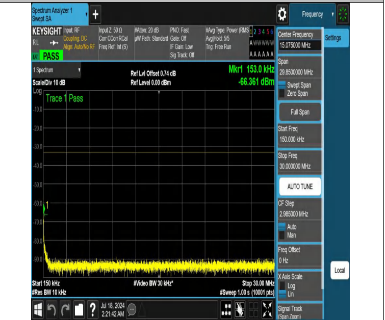
NTNV-DC_12A_n66A-PC3-15-5+40-M+M-N/A-N/A-DFT-QPSK-Edge_1RB_Right-0.15-30-PASS
