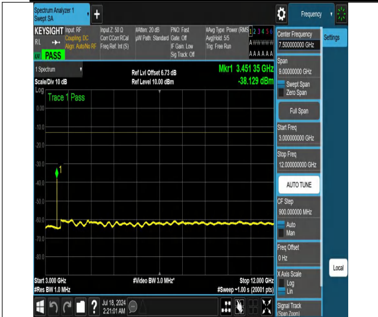
NTNV-DC_12A_n66A-PC3-15-5+40-M+M-N/A-N/A-DFT-QPSK-Edge_1RB_Left-3000-12000-PASS
