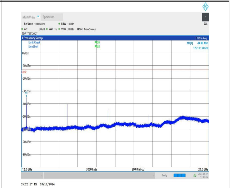
NTNV-DC_12A-n66A-PC3-15-5+35-M+L-QPSK-IDLE-DFT-BPSK-Edge_1RB_Right-12000-20000-PASS
