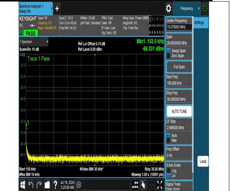
NTNV-DC_12A_n66A-PC3-15-5+40-M+H-N/A-N/A-DFT-PI2BPSK-E dge_1RB_Left-0.15-30-PASS
