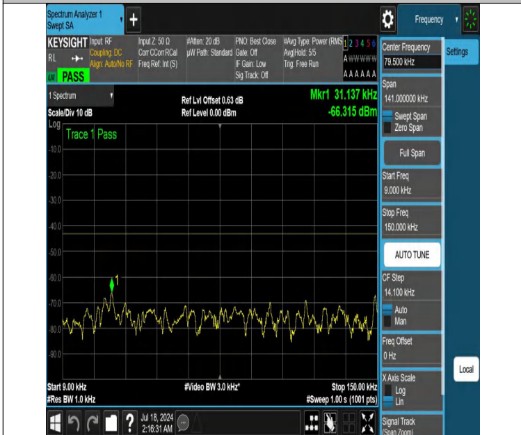
NTNV-DC_12A_n66A-PC3-15-5+40-M+L-N/A-N/A-DFT-QPSK-Edge e_1RB_Right-0.009-0.15-PASS
