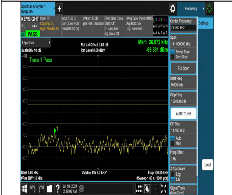
NTNV-DC_12A_n66A-PC3-15-5+40-M+M-N/A-N/A-DFT-PI2BPSK-Edge_1RB_Right-0.009-0.15-PASS
