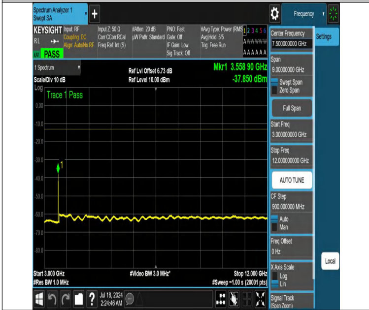
NTNV-DC_12A_n66A-PC3-15-5+40-M+H-N/A-N/A-DFT-PI2BPSK-Edge_1RB_Right-3000-12000-PASS
