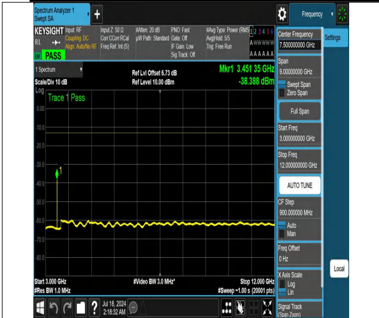
NTNV-DC_12A_n66A-PC3-15-5+40-M+M-N/A-N/A-DFT-PI2BPSK-Edge_1RB_Left-3000-12000-PASS
