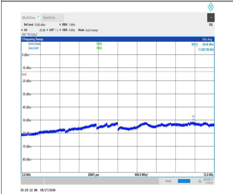
NTNV-DC_12A-n66A-PC3-15-5+35-M+L-QPSK-IDLE-DFT-BPSK-Edge_1RB_Right-3000-12000-PASS
