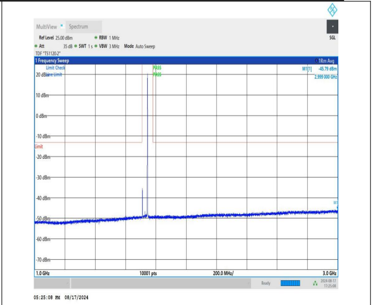
NTNV-DC_12A-n66A-PC3-15-5+35-M+L-QPSK-IDLE-DFT-BPSK-Edge_1RB_Right-1000-3000-PASS
