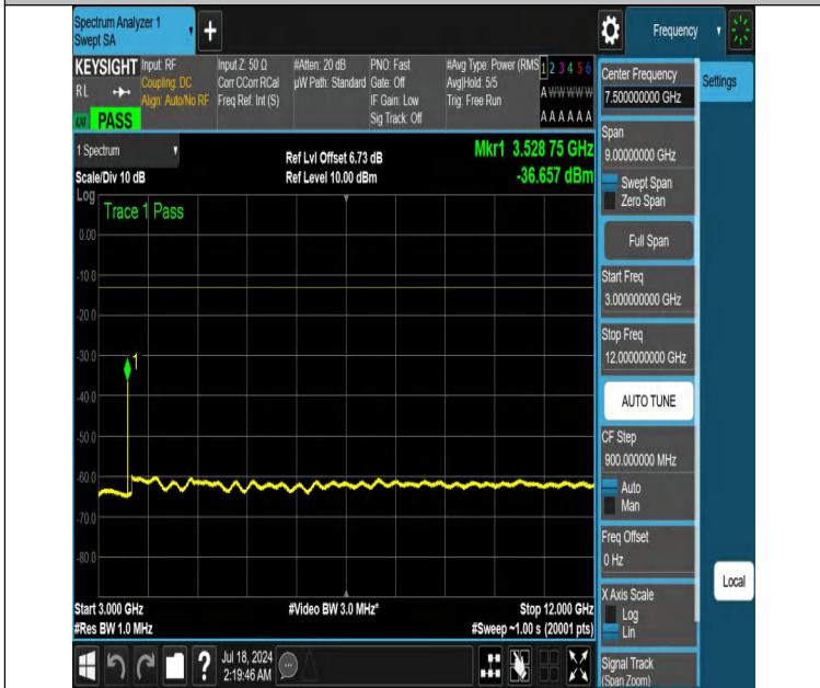
NTNV-DC_12A_n66A-PC3-15-5+40-M+M-N/A-N/A-DFT-PI2BPSK- Edge_1RB_Right-3000-12000-PASS
