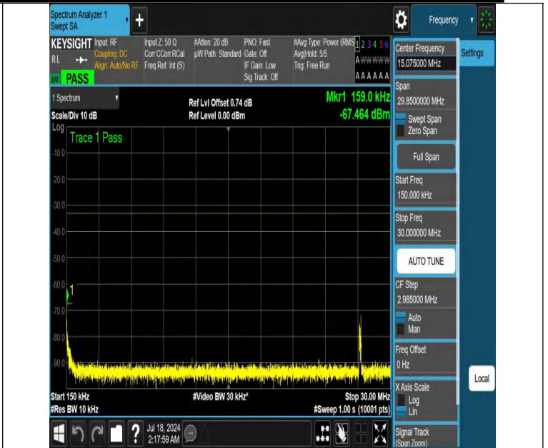
NTNV-DC_12A_n66A-PC3-15-5+40-M+M-N/A-N/A-DFT-PI2BPSK-E dge_1RB_Left-0.15-30-PASS
