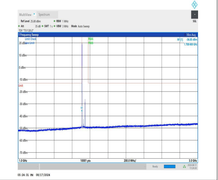
NTNV-DC_12A-n66A-PC3-15-5+35-M+L-QPSK-IDLE-DFT-BPSK-E dge_1RB_Left-1000-3000-PASS
