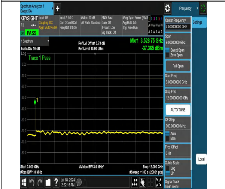
NTNV-DC_12A_n66A-PC3-15-5+40-M+M-N/A-N/A-DFT-QPSK-Edge_1RB_Right-3000-12000-PASS
