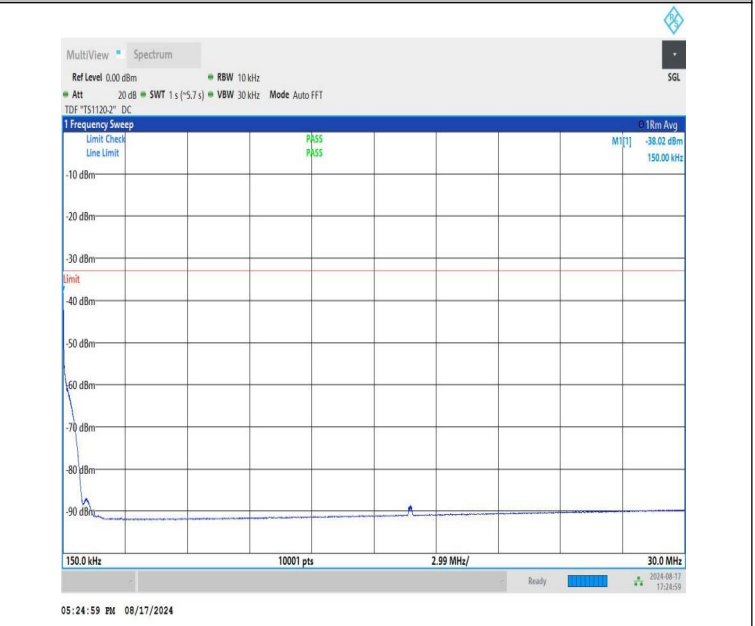
NTNV-DC_12A-n66A-PC3-15-5+35-M+L-QPSK-IDLE-DFT-BPSK-E dge_1RB_Right-0.15-30-PASS
