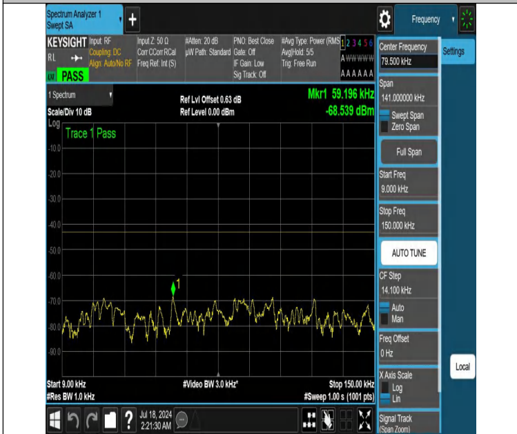
NTNV-DC_12A_n66A-PC3-15-5+40-M+M-N/A-N/A-DFT-QPSK-Edge_1RB_Right-0.009-0.15-PASS
