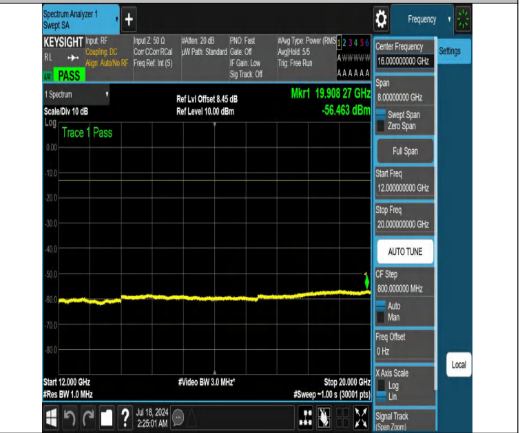
NTNV-DC_12A_n66A-PC3-15-5+40-M+H-N/A-N/A-DFT-PI2BPSK-E dge_1RB_Right-12000-20000-PASS
