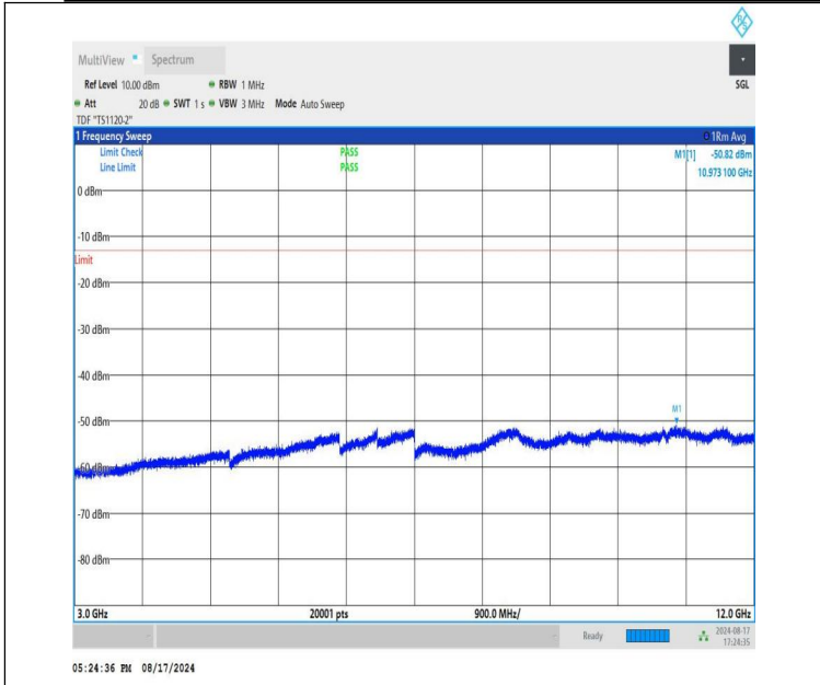
NTNV-DC_12A-n66A-PC3-15-5+35-M+L-QPSK-IDLE-DFT-BPSK-Edge_1RB_Left-3000-12000-PASS
