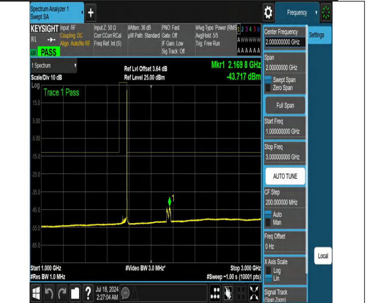
NTNV-DC_12A_n66A-PC3-15-5+40-M+H-N/A-N/A-DFT-QPSK-Edge e_1RB_Right-1000-3000-PASS
