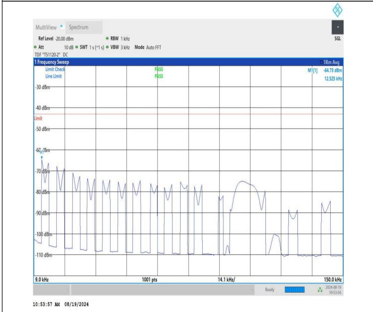
NTNV-DC_12A-n66A-PC3-15-5+35-M+L-QPSK-IDLE-DFT-BPSK-Edge_1RB_Right-0.009-0.15-PASS
