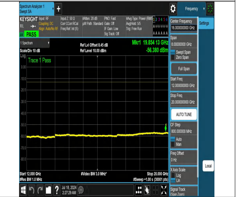
NTNV-DC_12A_n66A-PC3-15-5+40-M+H-N/A-N/A-DFT-QPSK-Edge e_1RB_Right-12000-20000-PASS
