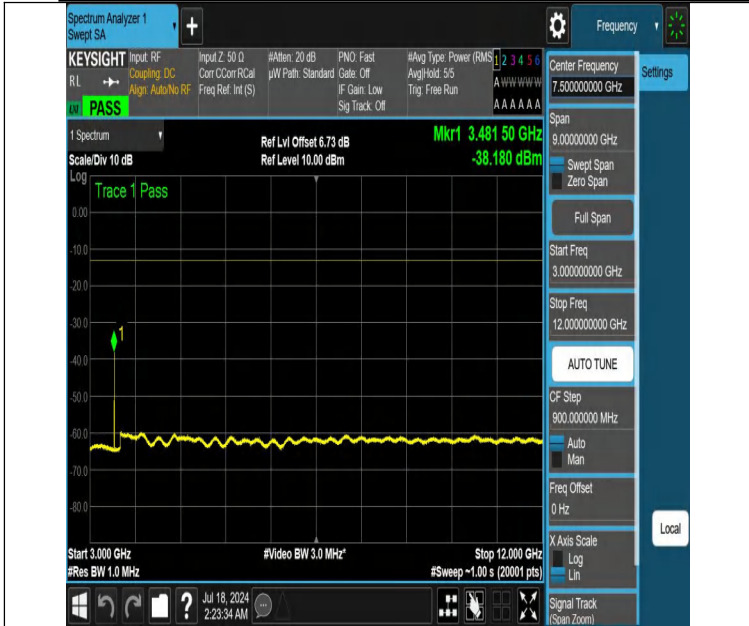
NTNV-DC_12A_n66A-PC3-15-5+40-M+H-N/A-N/A-DFT-PI2BPSK-Edge_1RB_Left-3000-12000-PASS
