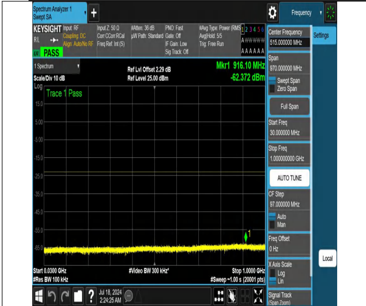
NTNV-DC_12A_n66A-PC3-15-5+40-M+H-N/A-N/A-DFT-PI2BPSK-Edge_1RB_Right-30-1000-PASS
