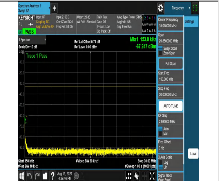
NTNV-DC_12A_n66A-PC3-15-5+25-M+H-N/A-N/A-DFT-QPSK-Edge e_1RB_Right-0.15-30-PASS
