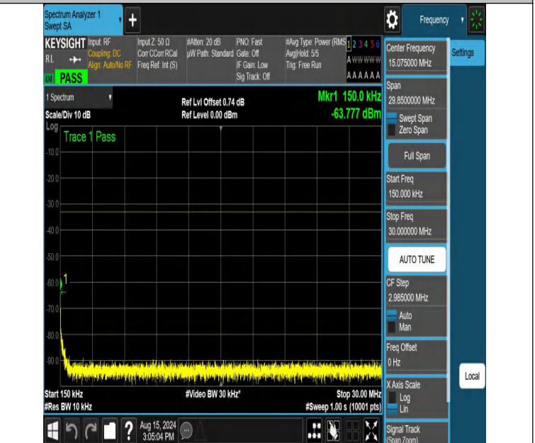
NTNV-DC_12A_n66A-PC3-15-5+30-M+H-N/A-N/A-DFT-QPSK-Edge_1RB_Right-0.15-30-PASS
