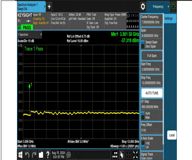
NTNV-DC_12A_n66A-PC3-15-5+30-M+H-N/A-N/A-DFT-PI2BPSK-Edge_1RB_Left-3000-12000-PASS
