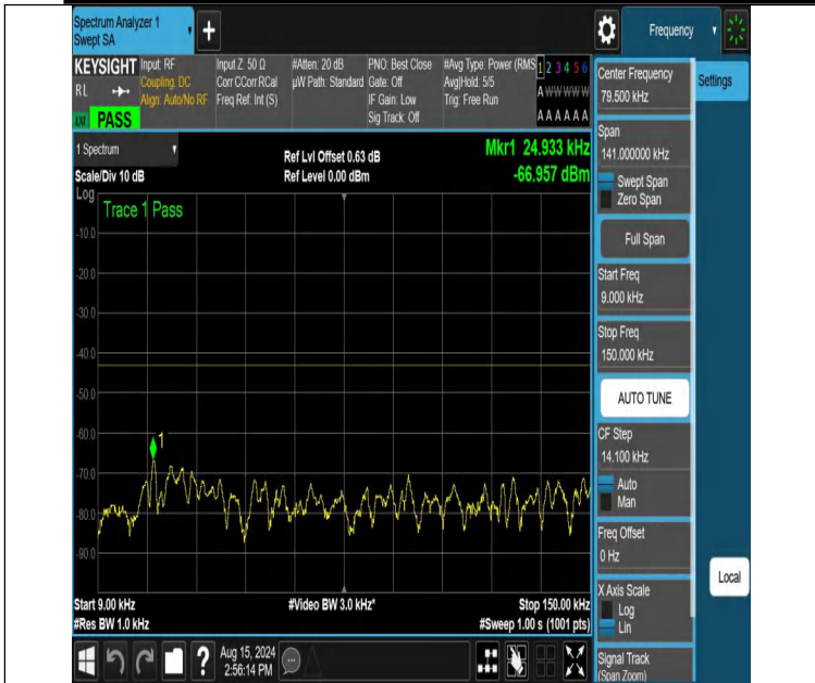
NTNV-DC_12A_n66A-PC3-15-5+30-M+M-N/A-N/A-DFT-PI2BPSK-Edge_1RB_Left-0.009-0.15-PASS
