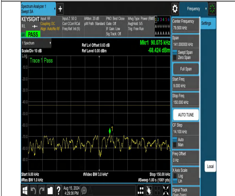
NTNV-DC_12A_n66A-PC3-15-5+25-M+H-N/A-N/A-DFT-QPSK-Edge e_1RB_Right-0.009-0.15-PASS
