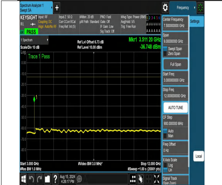
NTNV-DC_12A_n66A-PC3-15-5+25-M+H-N/A-N/A-DFT-PI2BPSK-Edge_1RB_Left-3000-12000-PASS
