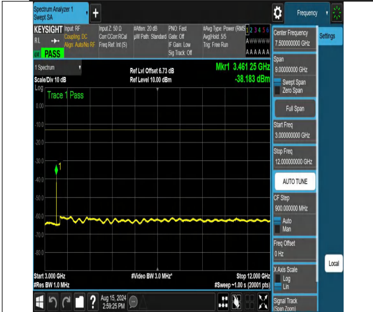
NTNV-DC_12A_n66A-PC3-15-5+30-M+M-N/A-N/A-DFT-QPSK-Edge_1RB_Left-3000-12000-PASS
