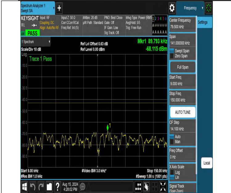
NTNV-DC_12A_n66A-PC3-15-5+25-M+H-N/A-N/A-DFT-QPSK-Edge e_1RB_Left-0.009-0.15-PASS
