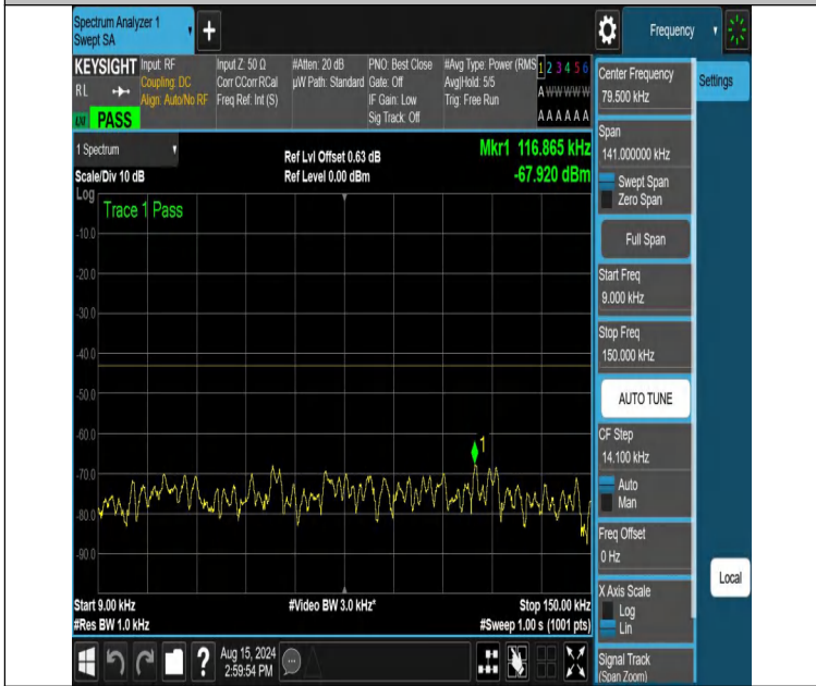
NTNV-DC_12A_n66A-PC3-15-5+30-M+M-N/A-N/A-DFT-QPSK-Edge_1RB_Right-0.009-0.15-PASS
