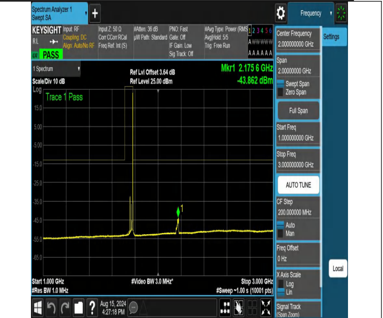
NTNV-DC_12A_n66A-PC3-15-5+25-M+H-N/A-N/A-DFT-PI2BPSK-E dge_1RB_Right-1000-3000-PASS
