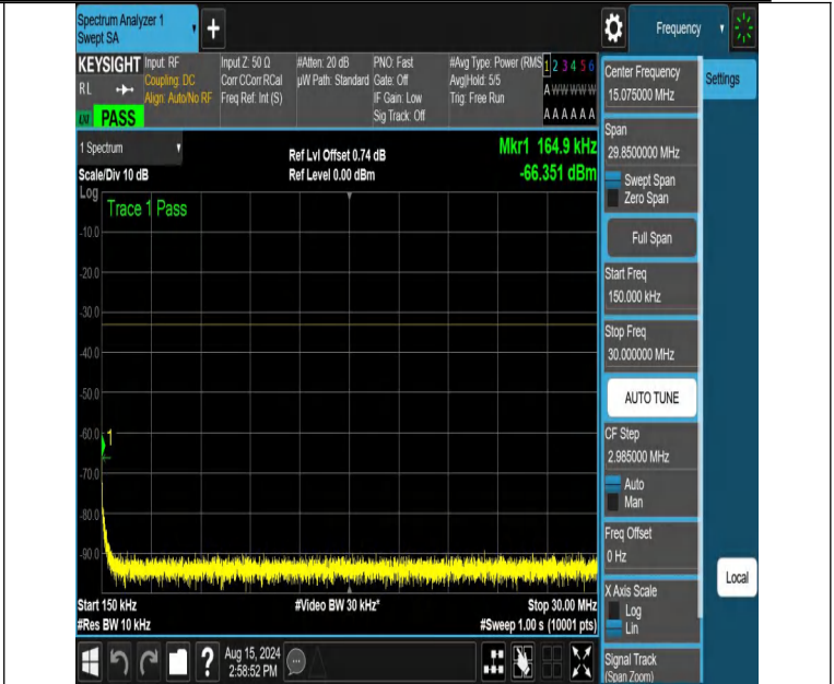
NTNV-DC_12A_n66A-PC3-15-5+30-M+M-N/A-N/A-DFT-QPSK-Edge_1RB_Left-0.15-30-PASS
