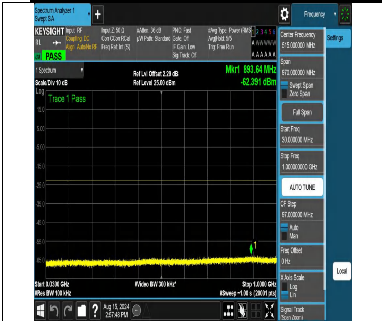
NTNV-DC_12A_n66A-PC3-15-5+30-M+M-N/A-N/A-DFT-PI2BPSK-Edge_1RB_Right-30-1000-PASS
