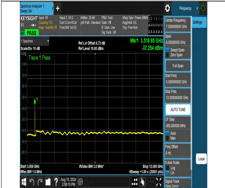
NTNV-DC_12A_n66A-PC3-15-5+30-M+M-N/A-N/A-DFT-PI2BPSK-Edge_1RB_Right-3000-12000-PASS
