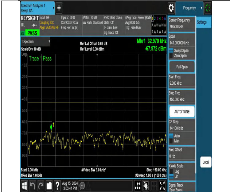
NTNV-DC_12A_n66A-PC3-15-5+30-M+H-N/A-N/A-DFT-QPSK-Edge e_1RB_Left-0.009-0.15-PASS
