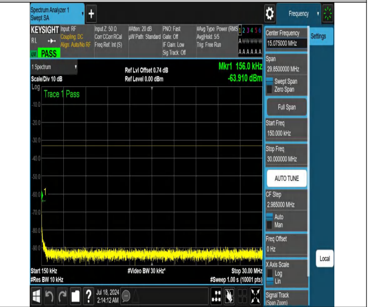
NTNV-DC_12A_n66A-PC3-15-5+40-M+L-N/A-N/A-DFT-PI2BPSK-E_dge_1RB_Right-0.15-30-PASS
