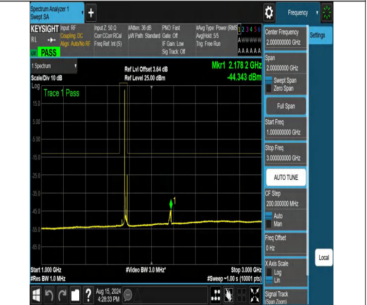
NTNV-DC_12A_n66A-PC3-15-5+25-M+H-N/A-N/A-DFT-QPSK-Edge e_1RB_Left-1000-3000-PASS
