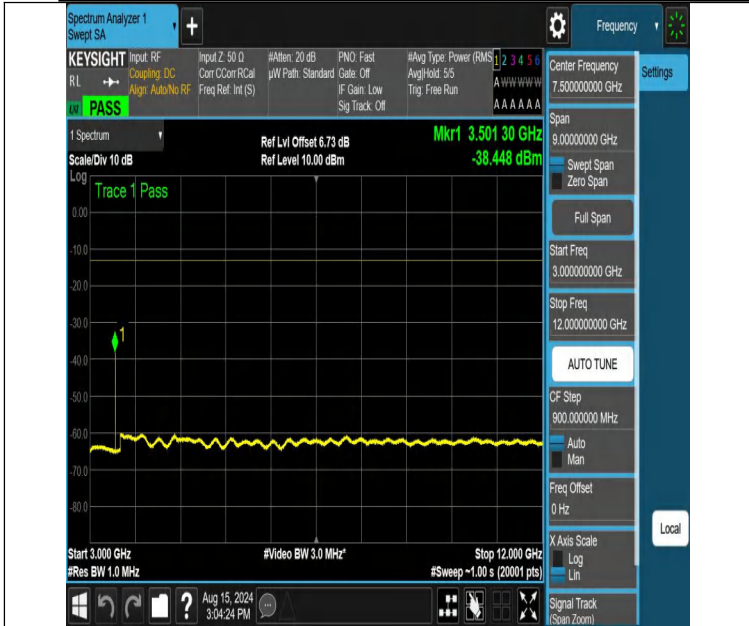
NTNV-DC_12A_n66A-PC3-15-5+30-M+H-N/A-N/A-DFT-QPSK-Edge_1RB_Left-3000-12000-PASS
