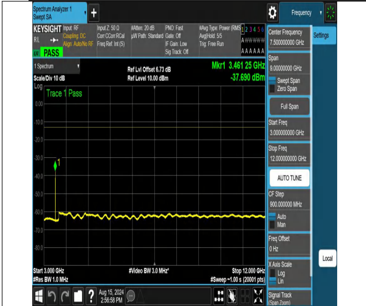
NTNV-DC_12A_n66A-PC3-15-5+30-M+M-N/A-N/A-DFT-PI2BPSK-Edge_1RB_Left-3000-12000-PASS
