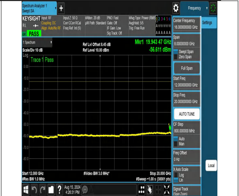
NTNV-DC_12A_n66A-PC3-15-5+25-M+H-N/A-N/A-DFT-PI2BPSK-E_dge_1RB_Left-12000-20000-PASS
