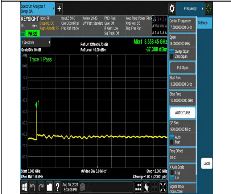
NTNV-DC_12A_n66A-PC3-15-5+30-M+H-N/A-N/A-DFT-PI2BPSK-Edge_1RB_Right-3000-12000-PASS
