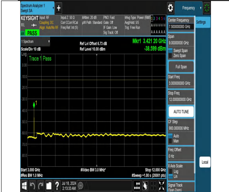
NTNV-DC_12A_n66A-PC3-15-5+40-M+L-N/A-N/A-DFT-PI2BPSK-Edge_1RB_Left-3000-12000-PASS
