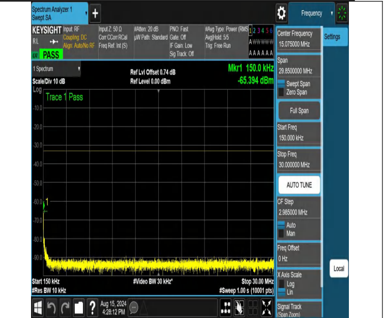
NTNV-DC_12A_n66A-PC3-15-5+25-M+H-N/A-N/A-DFT-QPSK-Edge e_1RB_Left-0.15-30-PASS
