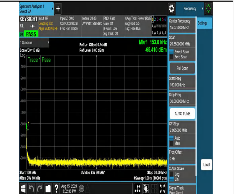
NTNV-DC_12A_n66A-PC3-15-5+30-M+H-N/A-N/A-DFT-PI2BPSK-E dge_1RB_Right-0.15-30-PASS
