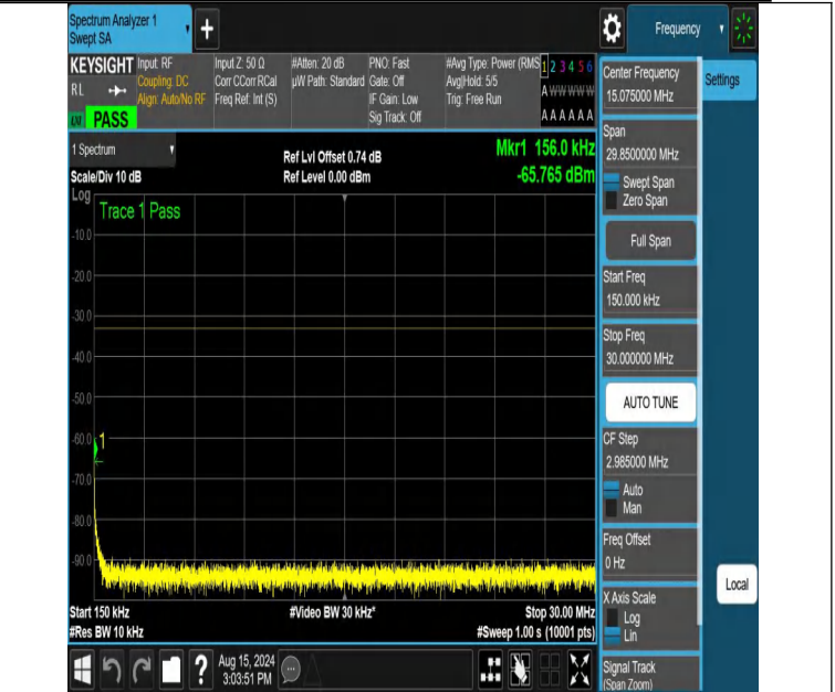
NTNV-DC_12A_n66A-PC3-15-5+30-M+H-N/A-N/A-DFT-QPSK-Edge e_1RB_Left-0.15-30-PASS
