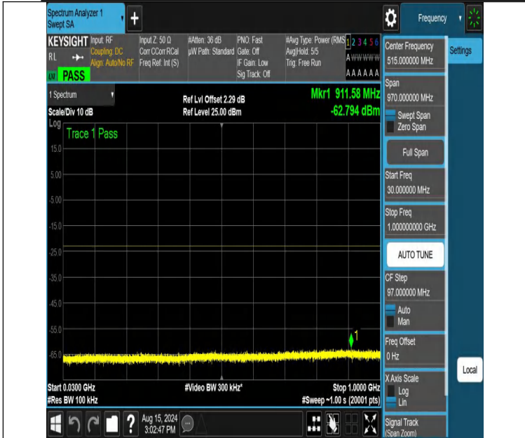
NTNV-DC_12A_n66A-PC3-15-5+30-M+H-N/A-N/A-DFT-PI2BPSK-Edge_1RB_Right-30-1000-PASS
