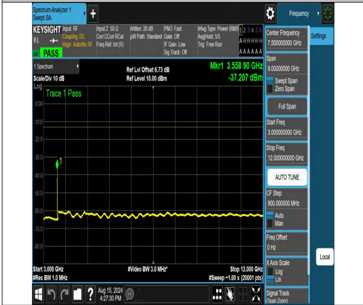
NTNV-DC_12A_n66A-PC3-15-5+25-M+H-N/A-N/A-DFT-PI2BPSK-Edge_1RB_Right-3000-12000-PASS
