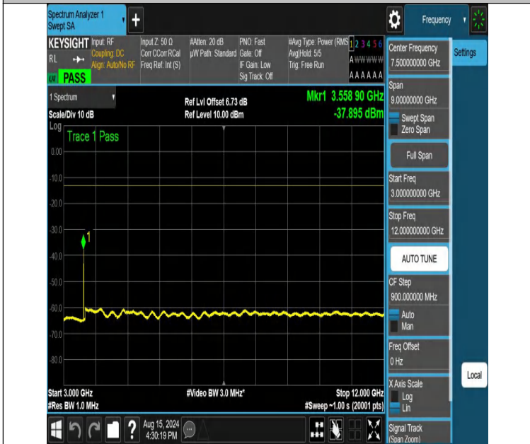
NTNV-DC_12A_n66A-PC3-15-5+25-M+H-N/A-N/A-DFT-QPSK-Edge e_1RB_Right-3000-12000-PASS
