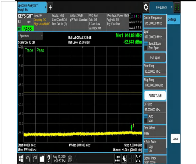
NTNV-DC_12A_n66A-PC3-15-5+25-M+H-N/A-N/A-DFT-QPSK-Edge e_1RB_Right-30-1000-PASS
