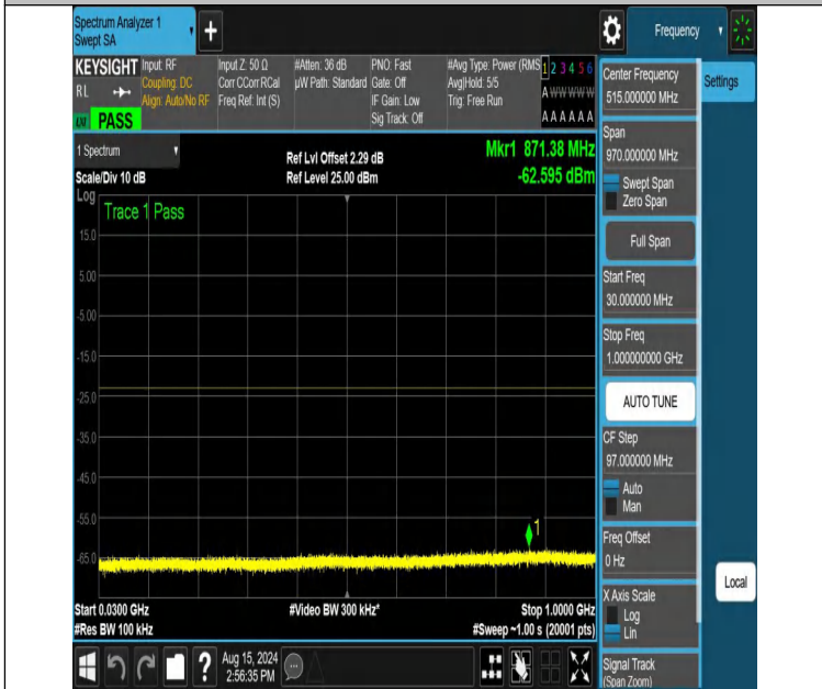
NTNV-DC_12A_n66A-PC3-15-5+30-M+M-N/A-N/A-DFT-PI2BPSK-Edge_1RB_Left-30-1000-PASS
