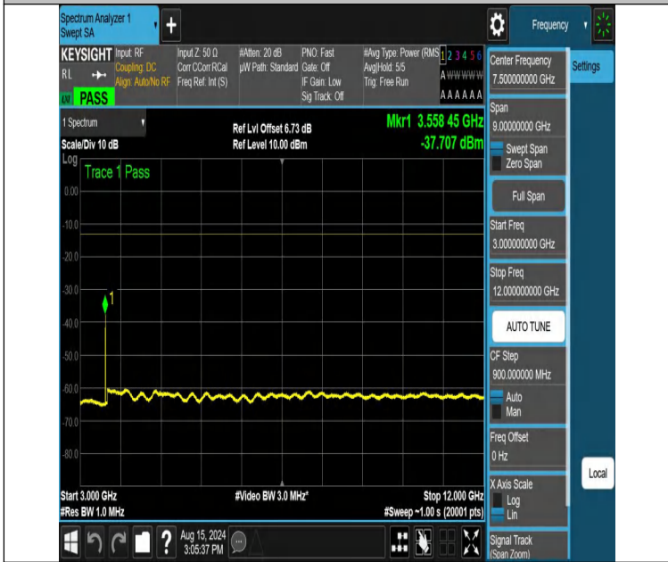
NTNV-DC_12A_n66A-PC3-15-5+30-M+H-N/A-N/A-DFT-QPSK-Edge e_1RB_Right-3000-12000-PASS
