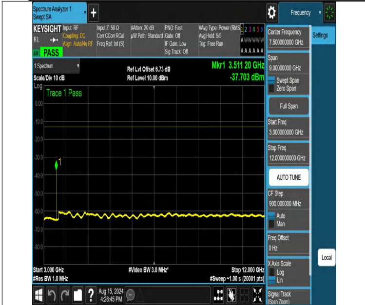
NTNV-DC_12A_n66A-PC3-15-5+25-M+H-N/A-N/A-DFT-QPSK-Edge e_1RB_Left-3000-12000-PASS
