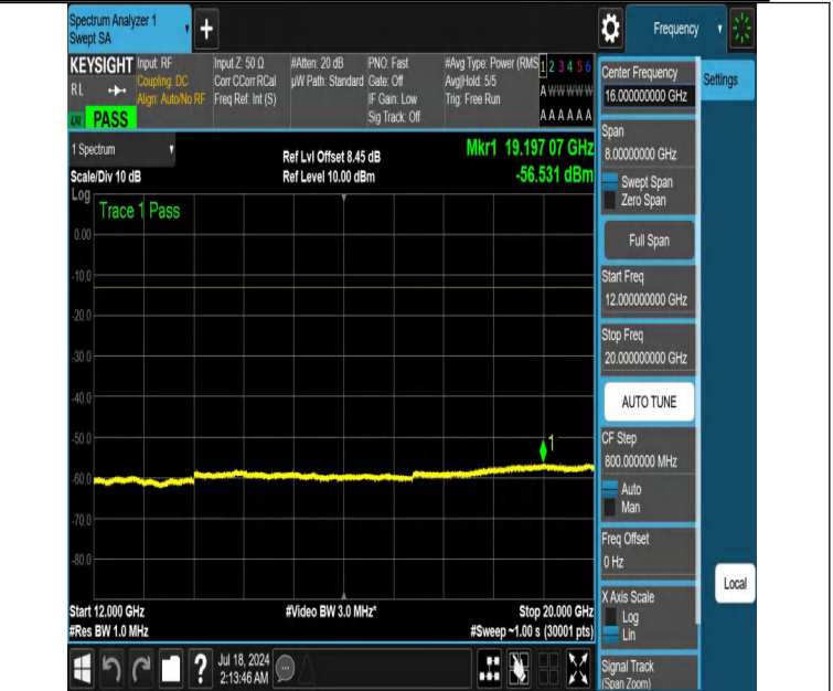
NTNV-DC_12A_n66A-PC3-15-5+40-M+L-N/A-N/A-DFT-PI2BPSK-E_dge_1RB_Left-12000-20000-PASS
