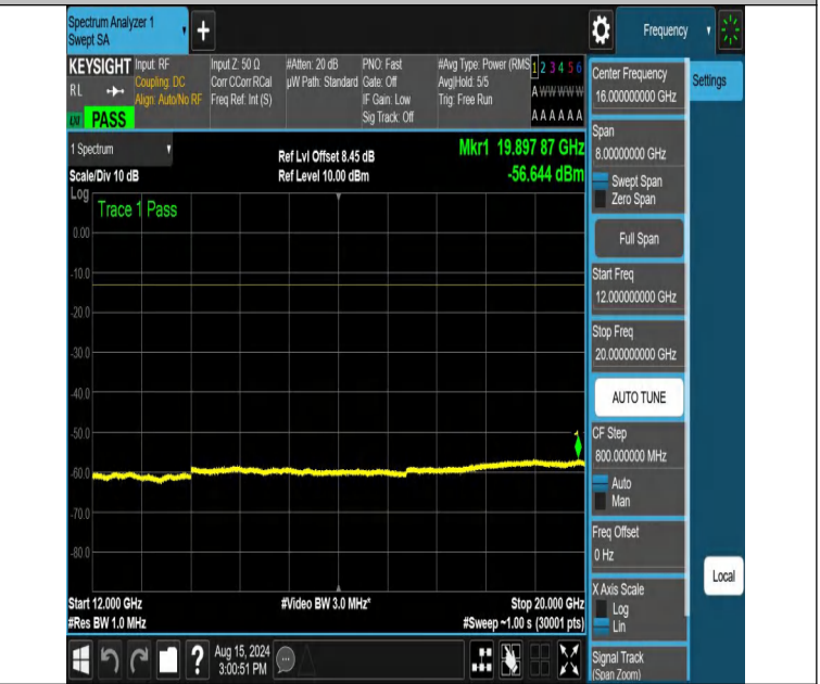
NTNV-DC_12A_n66A-PC3-15-5+30-M+M-N/A-N/A-DFT-QPSK-Edge_1RB_Right-12000-20000-PASS
