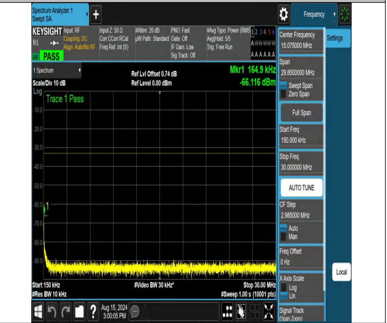
NTNV-DC_12A_n66A-PC3-15-5+30-M+M-N/A-N/A-DFT-QPSK-Edge_1RB_Right-0.15-30-PASS
