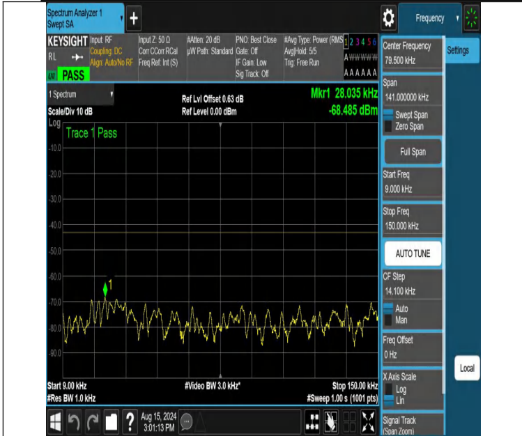
NTNV-DC_12A_n66A-PC3-15-5+30-M+H-N/A-N/A-DFT-PI2BPSK-Edge_1RB_Left-0.009-0.15-PASS
