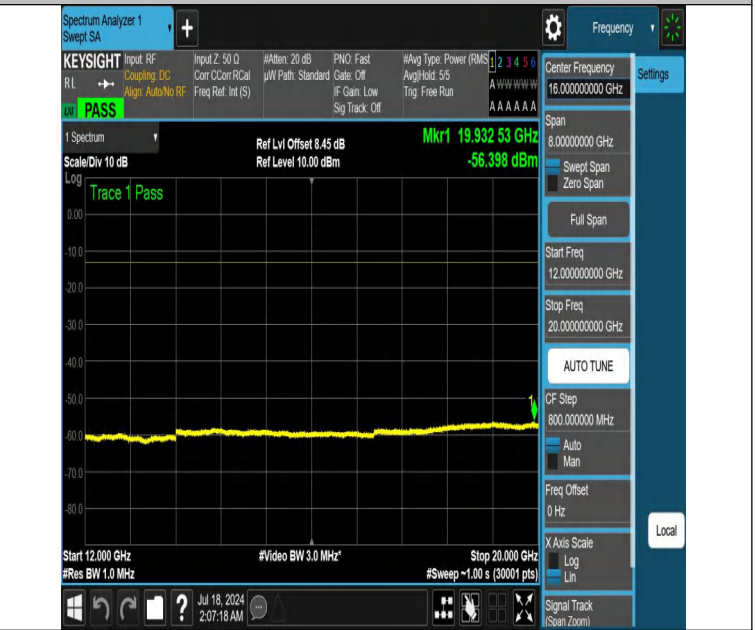
NTNV-DC_12A_n66A-PC3-15-5+20-M+M-N/A-N/A-DFT-QPSK-Edge_1RB_Right-12000-20000-PASS
