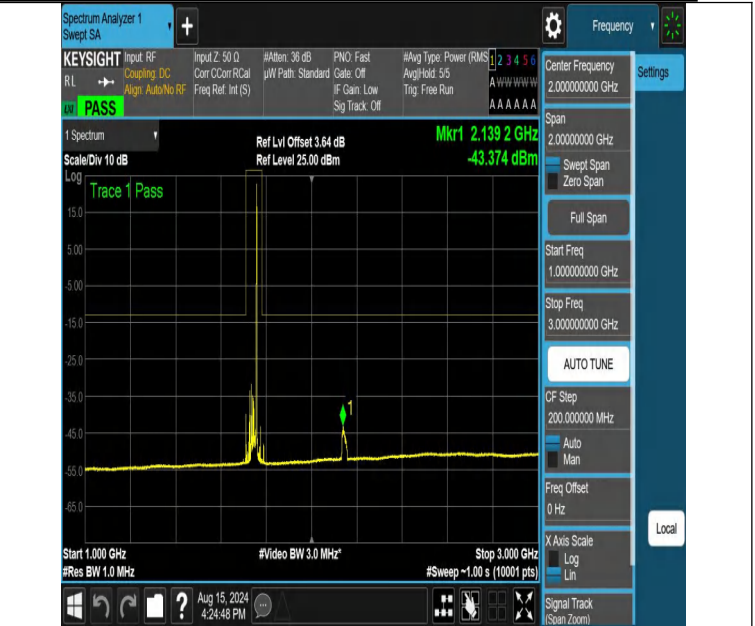
NTNV-DC_12A_n66A-PC3-15-5+25-M+M-N/A-N/A-DFT-QPSK-Edge_1RB_Right-1000-3000-PASS
