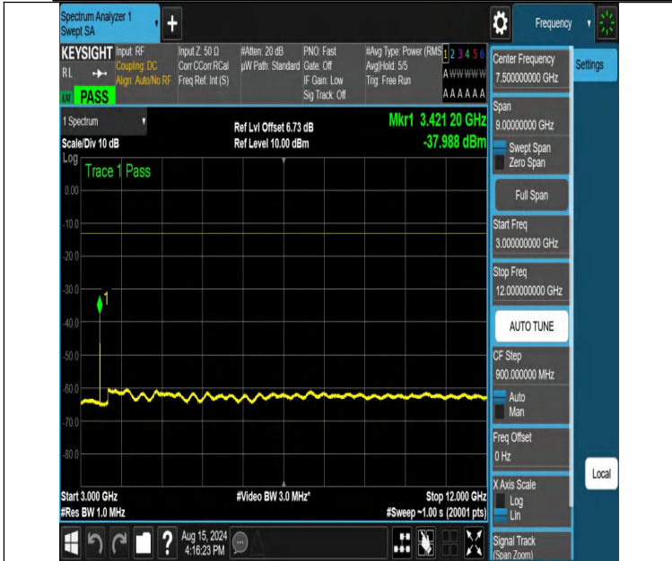
NTNV-DC_12A_n66A-PC3-15-5+25-M+L-N/A-N/A-DFT-PI2BPSK-Edge_1RB_Left-3000-12000-PASS
