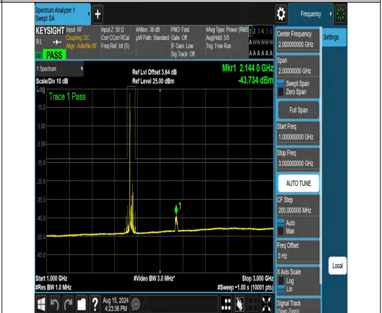
NTNV-DC_12A_n66A-PC3-15-5+25-M+M-N/A-N/A-DFT-QPSK-Edge_1RB_Left-1000-3000-PASS
