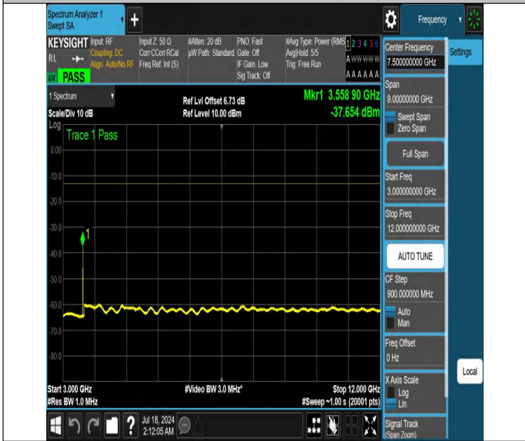
NTNV-DC_12A_n66A-PC3-15-5+20-M+H-N/A-N/A-DFT-QPSK-Edge e_1RB_Right-3000-12000-PASS
