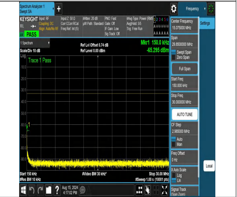
NTNV-DC_12A_n66A-PC3-15-5+25-M+L-N/A-N/A-DFT-PI2BPSK-E dge_1RB_Right-0.15-30-PASS
