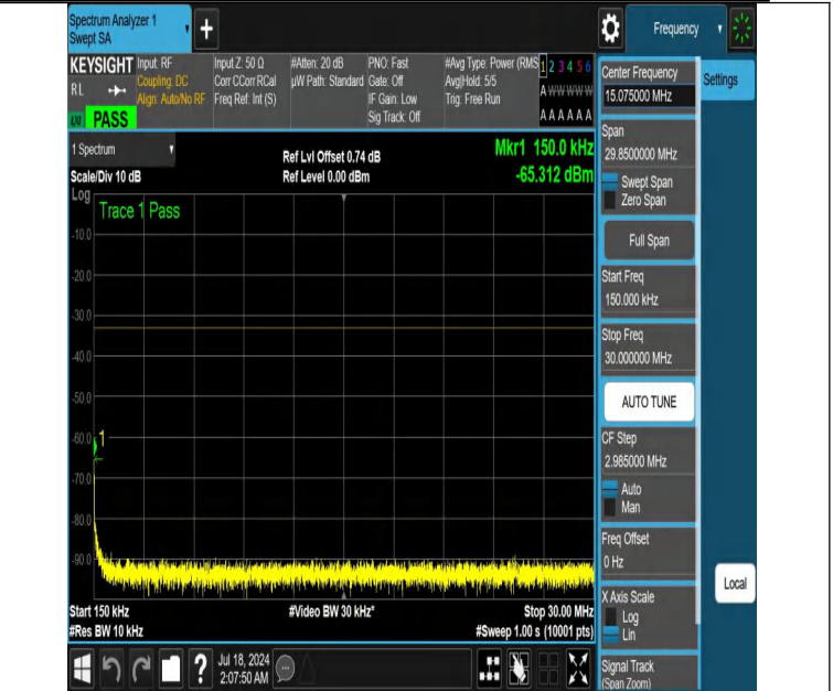
NTNV-DC_12A_n66A-PC3-15-5+20-M+H-N/A-N/A-DFT-PI2BPSK-E dge_1RB_Left-0.15-30-PASS
