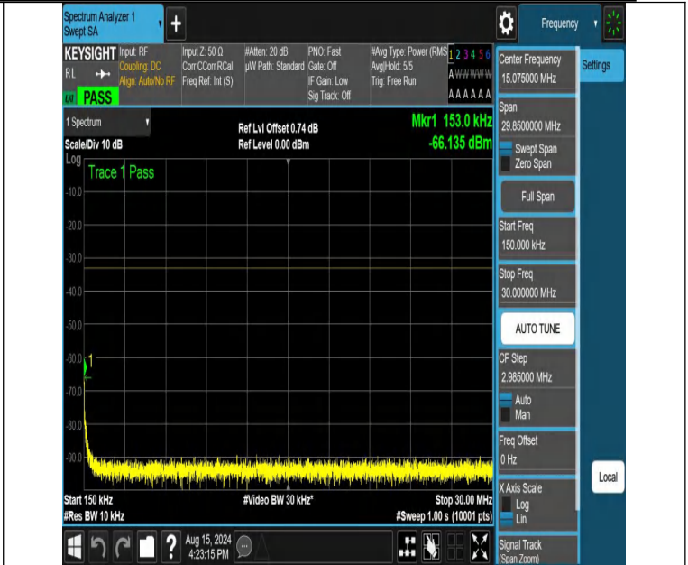
NTNV-DC_12A_n66A-PC3-15-5+25-M+M-N/A-N/A-DFT-QPSK-Edge_1RB_Left-0.15-30-PASS
