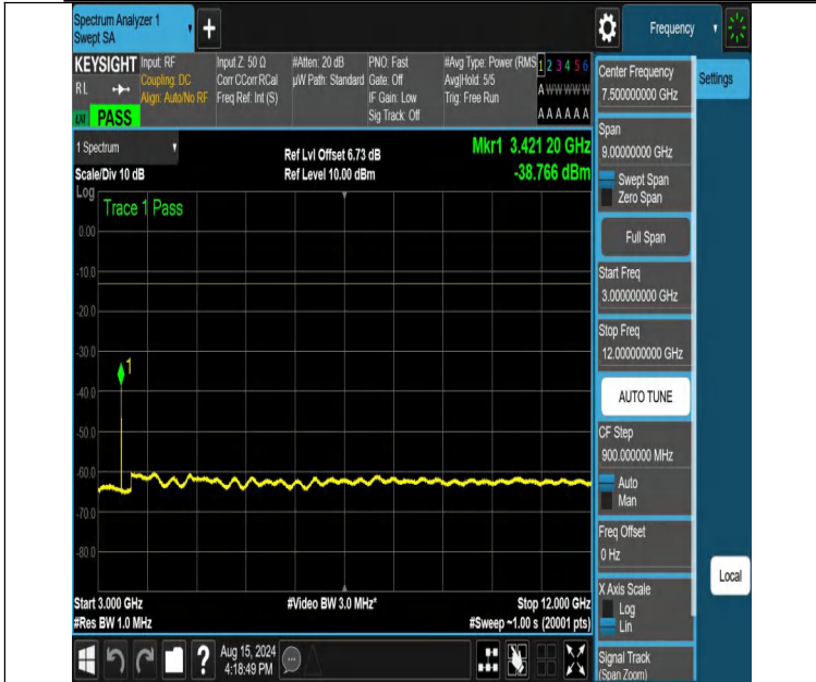
NTNV-DC_12A_n66A-PC3-15-5+25-M+L-N/A-N/A-DFT-QPSK-Edge e_1RB_Left-3000-12000-PASS
