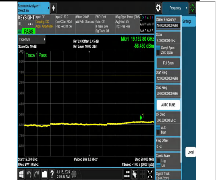
NTNV-DC_12A_n66A-PC3-15-5+20-M+H-N/A-N/A-DFT-PI2BPSK-E dge_1RB_Left-12000-20000-PASS
