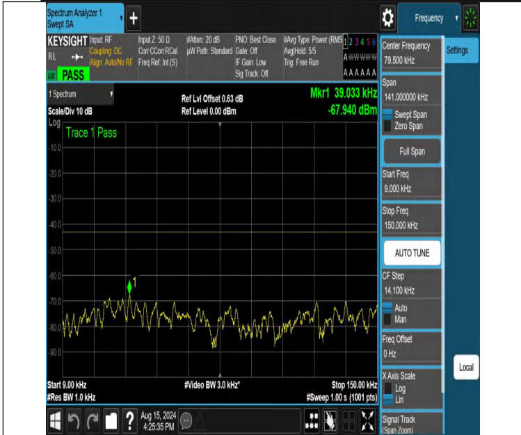
NTNV-DC_12A_n66A-PC3-15-5+25-M+H-N/A-N/A-DFT-PI2BPSK-Edge_1RB_Left-0.009-0.15-PASS
