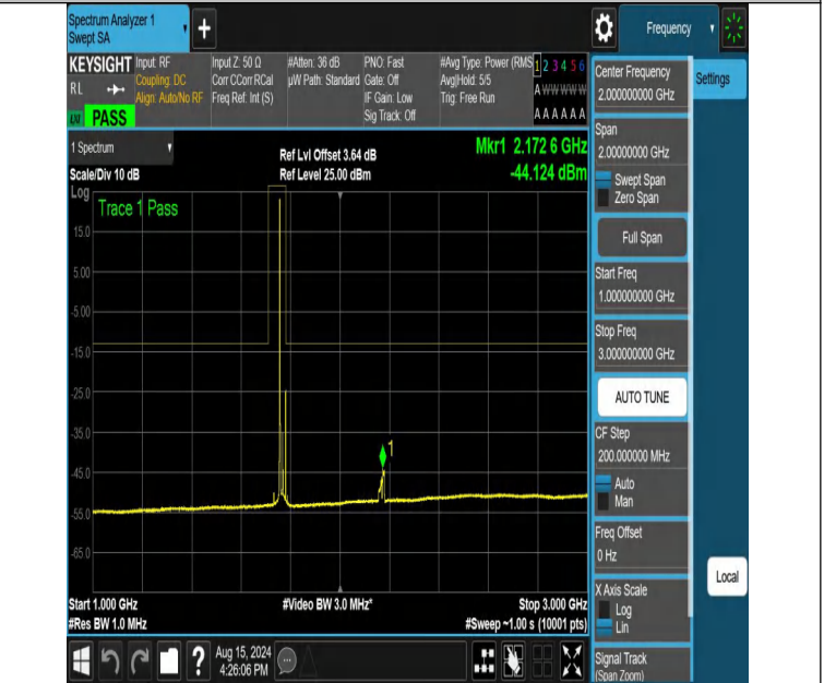
NTNV-DC_12A_n66A-PC3-15-5+25-M+H-N/A-N/A-DFT-PI2BPSK-E dge_1RB_Left-1000-3000-PASS
