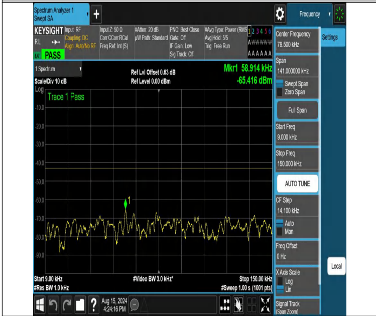
NTNV-DC_12A_n66A-PC3-15-5+25-M+M-N/A-N/A-DFT-QPSK-Edge_1RB_Right-0.009-0.15-PASS
