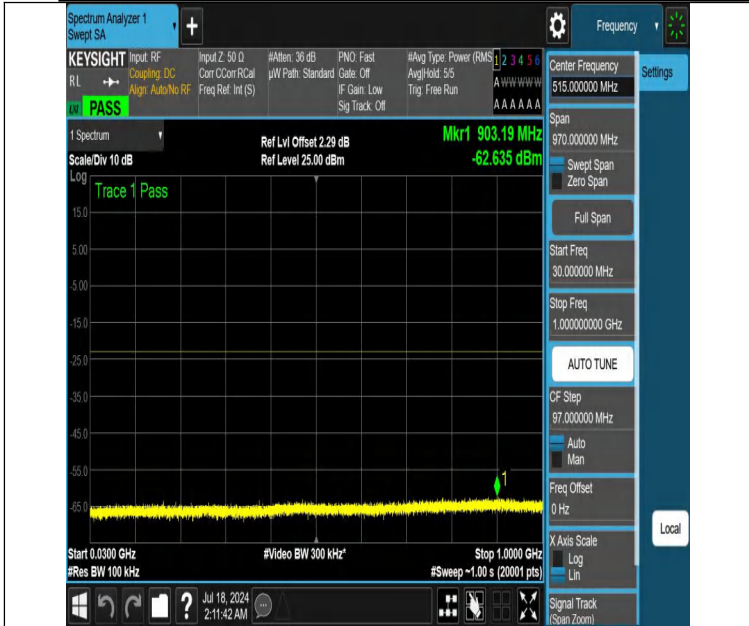
NTNV-DC_12A_n66A-PC3-15-5+20-M+H-N/A-N/A-DFT-QPSK-Edge e_1RB_Right-30-1000-PASS
