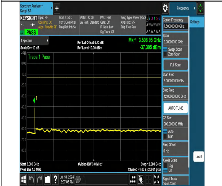
NTNV-DC_12A_n66A-PC3-15-5+20-M+M-N/A-N/A-DFT-QPSK-Edge_1RB_Right-3000-12000-PASS
