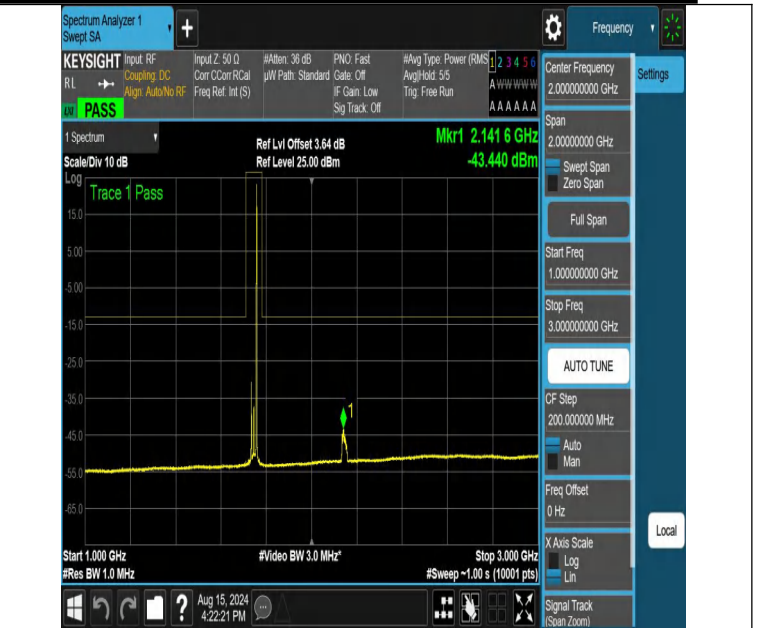
NTNV-DC_12A_n66A-PC3-15-5+25-M+M-N/A-N/A-DFT-PI2BPSK-E dge_1RB_Right-1000-3000-PASS
