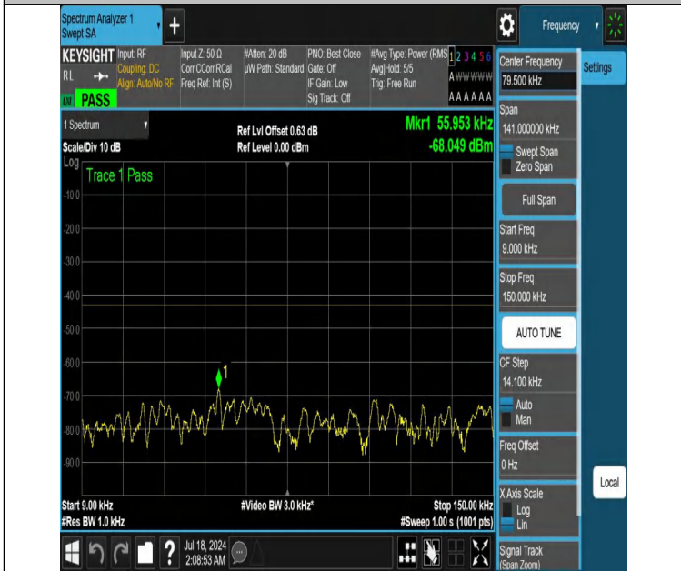
NTNV-DC_12A_n66A-PC3-15-5+20-M+H-N/A-N/A-DFT-PI2BPSK-Edge_1RB_Right-0.009-0.15-PASS
