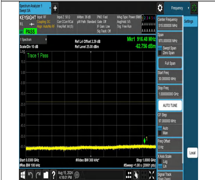
NTNV-DC_12A_n66A-PC3-15-5+25-M+L-N/A-N/A-DFT-PI2BPSK-Edge_1RB_Left-30-1000-PASS
