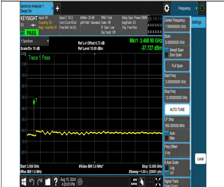
NTNV-DC_12A_n66A-PC3-15-5+25-M+L-N/A-N/A-DFT-QPSK-Edge e_1RB_Right-3000-12000-PASS
