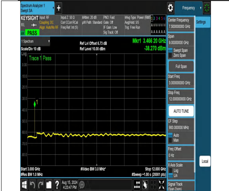
NTNV-DC_12A_n66A-PC3-15-5+25-M+M-N/A-N/A-DFT-QPSK-Edge_1RB_Left-3000-12000-PASS
