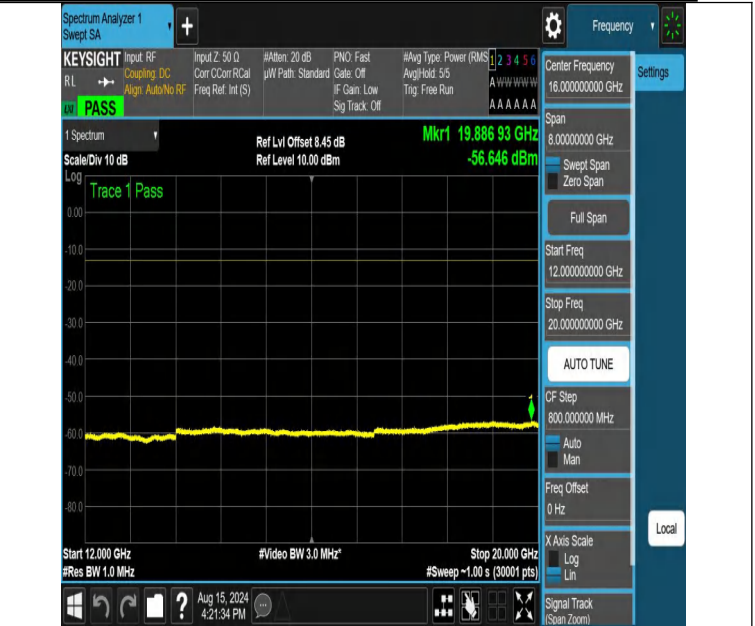
NTNV-DC_12A_n66A-PC3-15-5+25-M+M-N/A-N/A-DFT-PI2BPSK-E dge_1RB_Left-12000-20000-PASS
