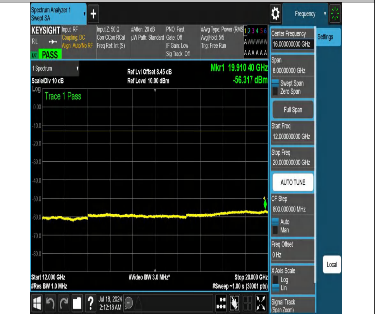
NTNV-DC_12A_n66A-PC3-15-5+20-M+H-N/A-N/A-DFT-QPSK-Edge e_1RB_Right-12000-20000-PASS
