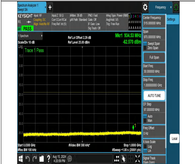
NTNV-DC_12A_n66A-PC3-15-5+25-M+M-N/A-N/A-DFT-PI2BPSK-Edge_1RB_Left-30-1000-PASS
