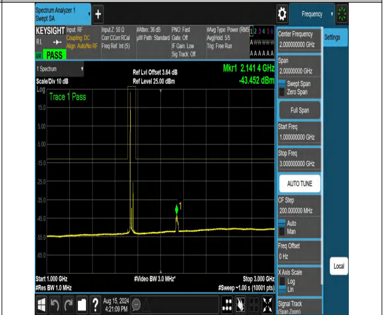
NTNV-DC_12A_n66A-PC3-15-5+25-M+M-N/A-N/A-DFT-PI2BPSK-E dge_1RB_Left-1000-3000-PASS
