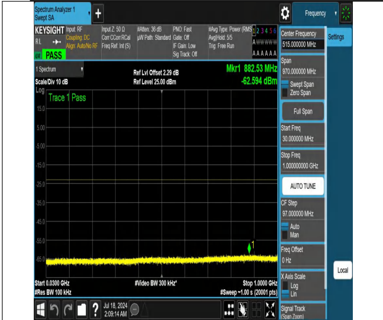
NTNV-DC_12A_n66A-PC3-15-5+20-M+H-N/A-N/A-DFT-PI2BPSK-Edge_1RB_Right-30-1000-PASS
