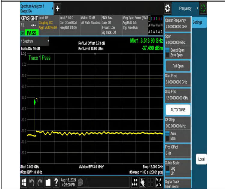
NTNV-DC_12A_n66A-PC3-15-5+25-M+M-N/A-N/A-DFT-QPSK-Edge_1RB_Right-3000-12000-PASS
