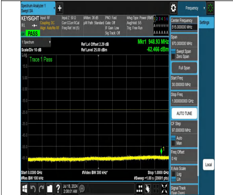
NTNV-DC_12A_n66A-PC3-15-5+20-M+H-N/A-N/A-DFT-PI2BPSK-Edge_1RB_Left-30-1000-PASS
