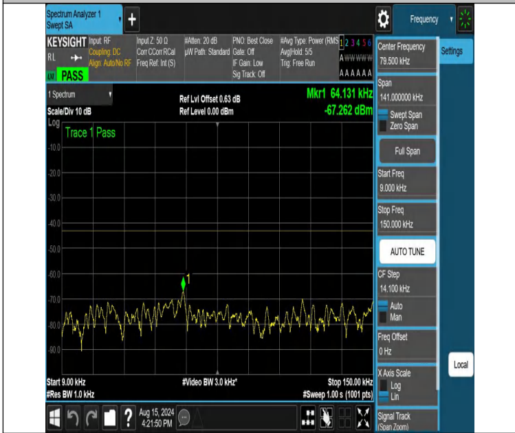
NTNV-DC_12A_n66A-PC3-15-5+25-M+M-N/A-N/A-DFT-PI2BPSK-Edge_1RB_Right-0.009-0.15-PASS
