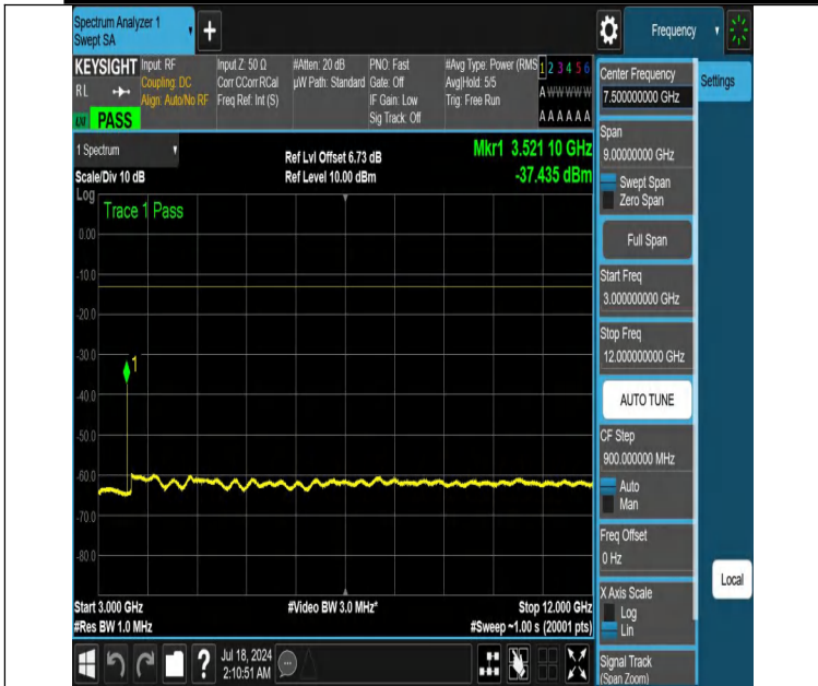
NTNV-DC_12A_n66A-PC3-15-5+20-M+H-N/A-N/A-DFT-QPSK-Edge e_1RB_Left-3000-12000-PASS
