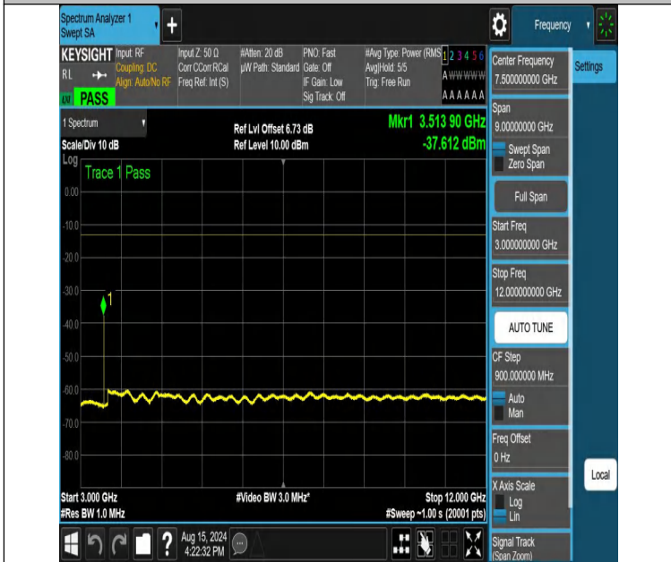
NTNV-DC_12A_n66A-PC3-15-5+25-M+M-N/A-N/A-DFT-PI2BPSK-Edge_1RB_Right-3000-12000-PASS
