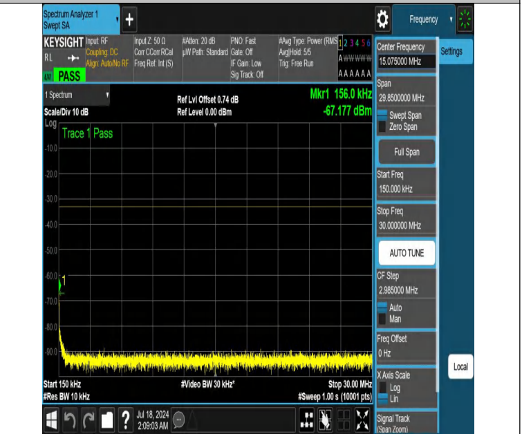
NTNV-DC_12A_n66A-PC3-15-5+20-M+H-N/A-N/A-DFT-PI2BPSK-E dge_1RB_Right-0.15-30-PASS
