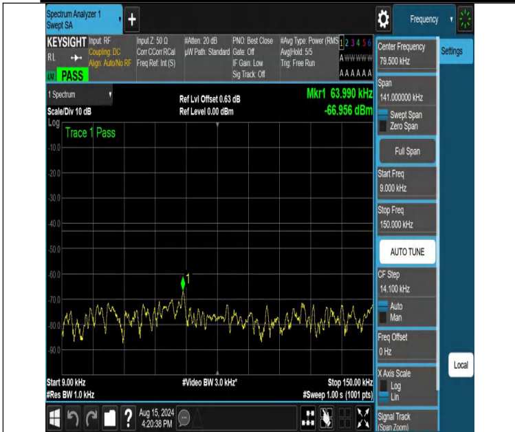
NTNV-DC_12A_n66A-PC3-15-5+25-M+M-N/A-N/A-DFT-PI2BPSK-Edge_1RB_Left-0.009-0.15-PASS
