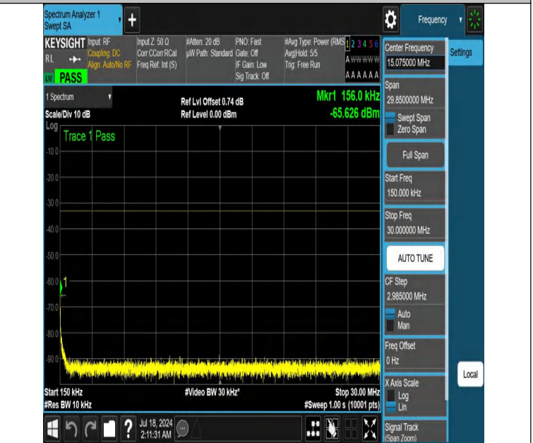
NTNV-DC_12A_n66A-PC3-15-5+20-M+H-N/A-N/A-DFT-QPSK-Edge e_1RB_Right-0.15-30-PASS
