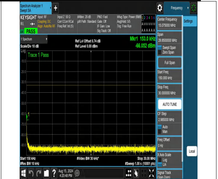
NTNV-DC_12A_n66A-PC3-15-5+25-M+M-N/A-N/A-DFT-PI2BPSK-E dge_1RB_Left-0.15-30-PASS
