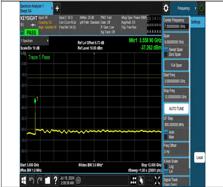
NTNV-DC_12A_n66A-PC3-15-5+20-M+H-N/A-N/A-DFT-PI2BPSK-Edge_1RB_Right-3000-12000-PASS
