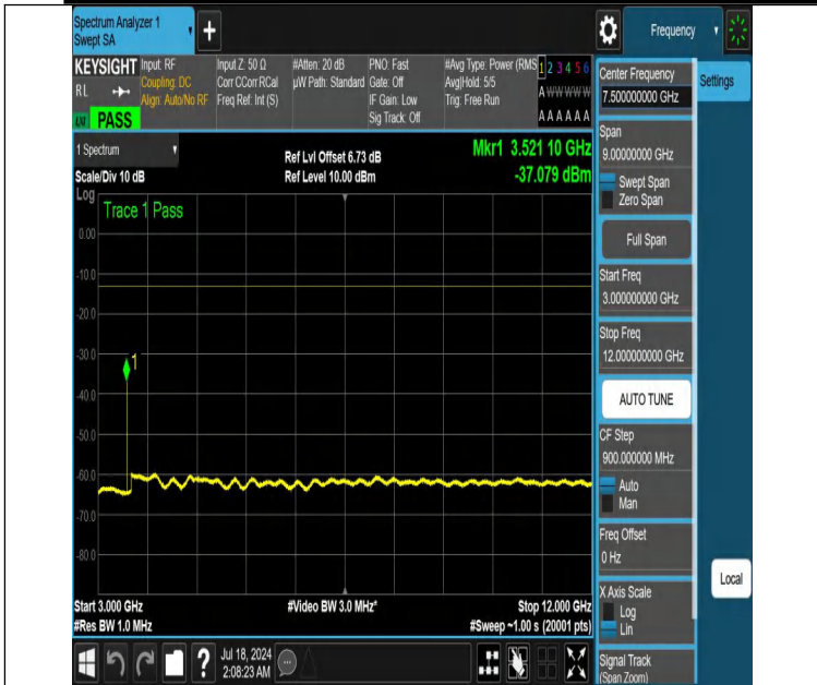
NTNV-DC_12A_n66A-PC3-15-5+20-M+H-N/A-N/A-DFT-PI2BPSK-Edge_1RB_Left-3000-12000-PASS
