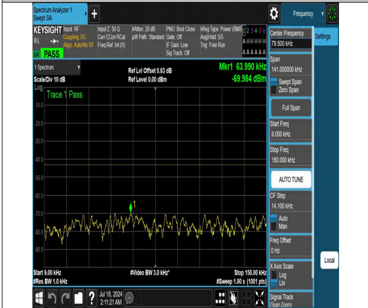
NTNV-DC_12A_n66A-PC3-15-5+20-M+H-N/A-N/A-DFT-QPSK-Edge e_1RB_Right-0.009-0.15-PASS
