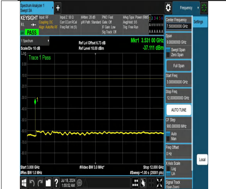
NTNV-DC_12A_n66A-PC3-15-5+15-M+H-N/A-N/A-DFT-QPSK-Edge e_1RB_Left-3000-12000-PASS
