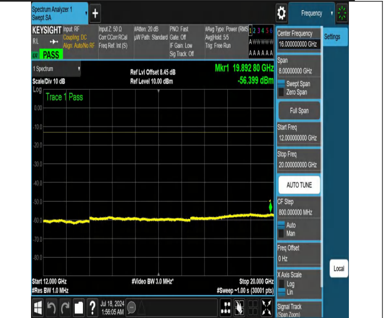
NTNV-DC_12A_n66A-PC3-15-5+15-M+H-N/A-N/A-DFT-QPSK-Edge e_1RB_Left-12000-20000-PASS
