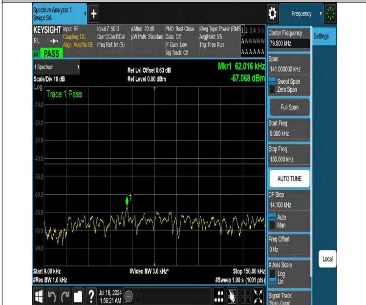
NTNV-DC_12A_n66A-PC3-15-5+15-M+H-N/A-N/A-DFT-QPSK-Edge e_1RB_Right-0.009-0.15-PASS
