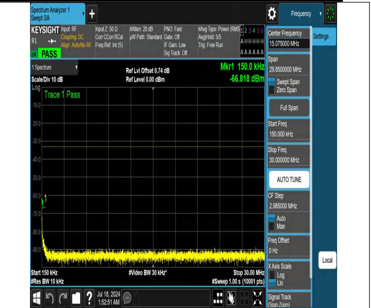
NTNV-DC_12A_n66A-PC3-15-5+15-M+H-N/A-N/A-DFT-PI2BPSK-E dge_1RB_Left-0.15-30-PASS
