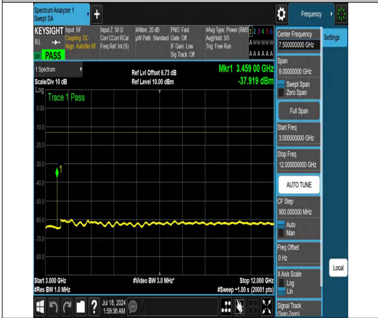
NTNV-DC_12A_n66A-PC3-15-5+20-M+L-N/A-N/A-DFT-PI2BPSK-Edge_1RB_Right-3000-12000-PASS
