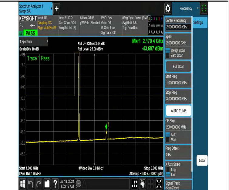
NTNV-DC_12A_n66A-PC3-15-5+15-M+H-N/A-N/A-DFT-PI2BPSK-E dge_1RB_Left-1000-3000-PASS
