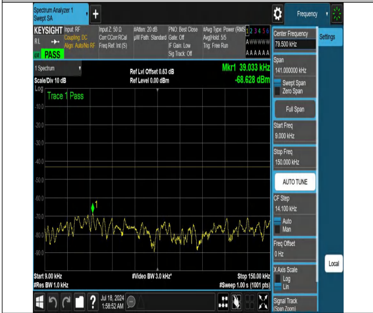
NTNV-DC_12A_n66A-PC3-15-5+20-M+L-N/A-N/A-DFT-PI2BPSK-Edge_1RB_Right-0.009-0.15-PASS
