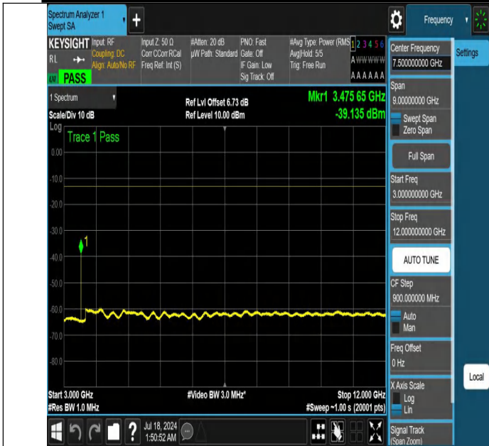
NTNV-DC_12A_n66A-PC3-15-5+15-M+M-N/A-N/A-DFT-QPSK-Edge_1RB_Left-3000-12000-PASS
