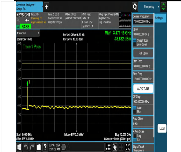
NTNV-DC_12A_n66A-PC3-15-5+20-M+M-N/A-N/A-DFT-QPSK-Edge_1RB_Left-3000-12000-PASS
