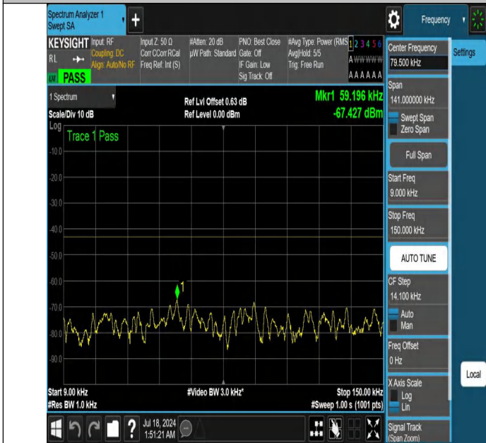
NTNV-DC_12A_n66A-PC3-15-5+15-M+M-N/A-N/A-DFT-QPSK-Edge_1RB_Right-0.009-0.15-PASS
