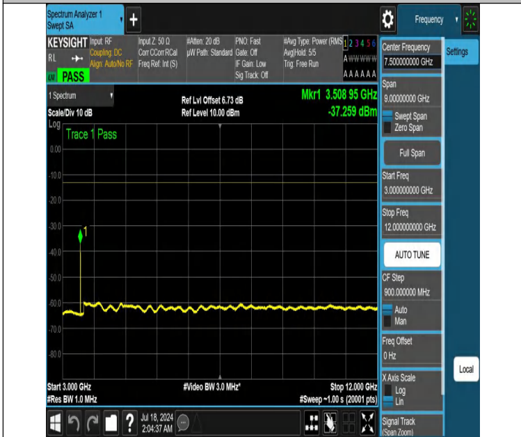
NTNV-DC_12A_n66A-PC3-15-5+20-M+M-N/A-N/A-DFT-PI2BPSK-Edge_1RB_Right-3000-12000-PASS
