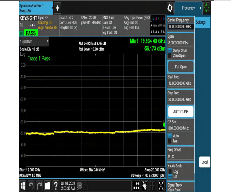
NTNV-DC_12A_n66A-PC3-15-5+20-M+M-N/A-N/A-DFT-PI2BPSK-E dge_1RB_Left-12000-20000-PASS
