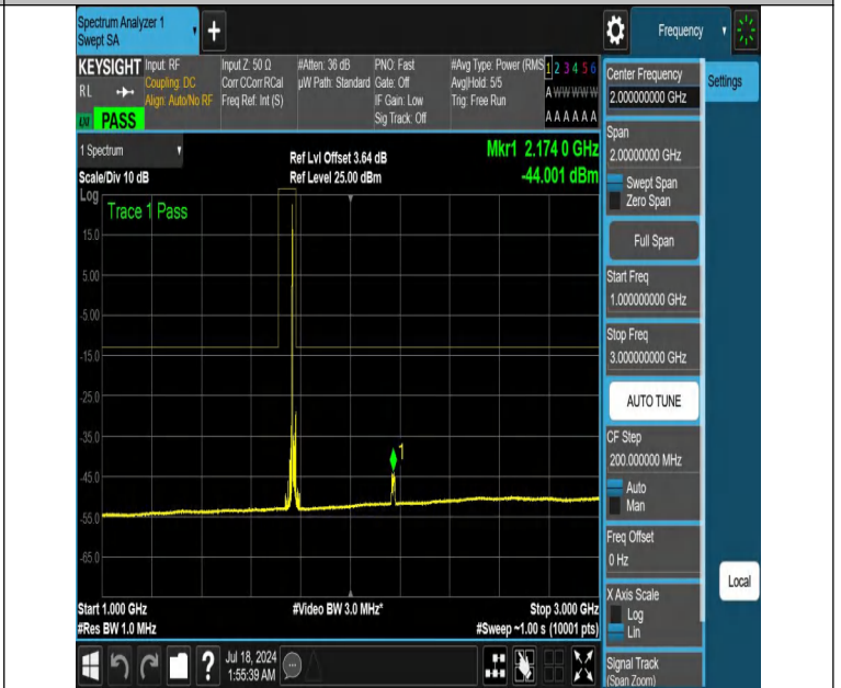
NTNV-DC_12A_n66A-PC3-15-5+15-M+H-N/A-N/A-DFT-QPSK-Edge e_1RB_Left-1000-3000-PASS
