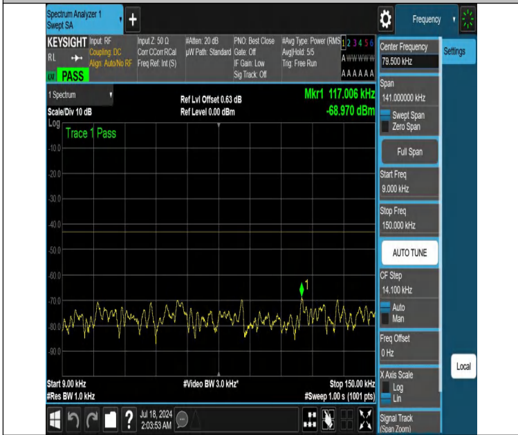
NTNV-DC_12A_n66A-PC3-15-5+20-M+M-N/A-N/A-DFT-PI2BPSK-Edge_1RB_Right-0.009-0.15-PASS
