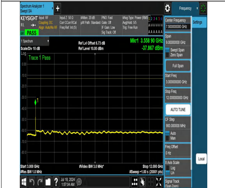
NTNV-DC_12A_n66A-PC3-15-5+15-M+H-N/A-N/A-DFT-QPSK-Edge e_1RB_Right-3000-12000-PASS
