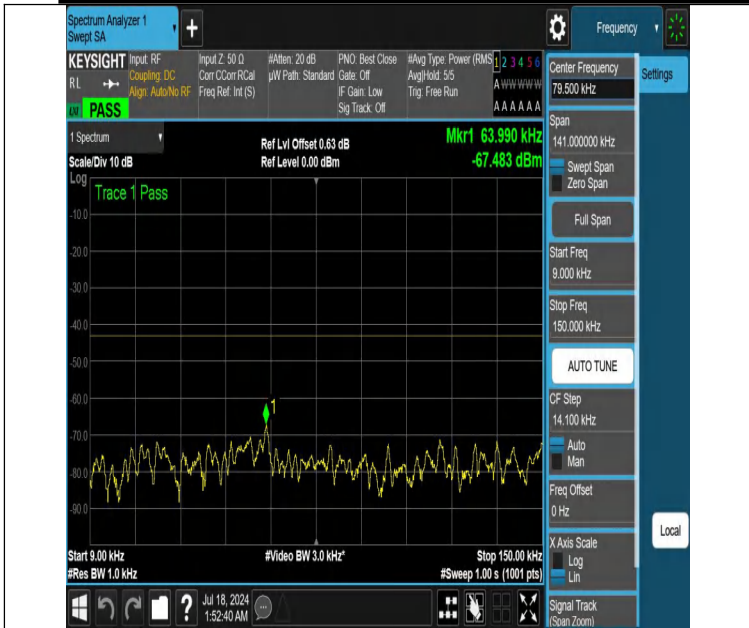
NTNV-DC_12A_n66A-PC3-15-5+15-M+H-N/A-N/A-DFT-PI2BPSK-Edge_1RB_Left-0.009-0.15-PASS
