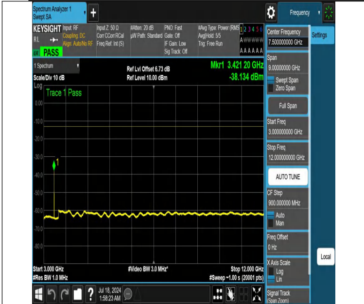
NTNV-DC_12A_n66A-PC3-15-5+20-M+L-N/A-N/A-DFT-PI2BPSK-Edge_1RB_Left-3000-12000-PASS
