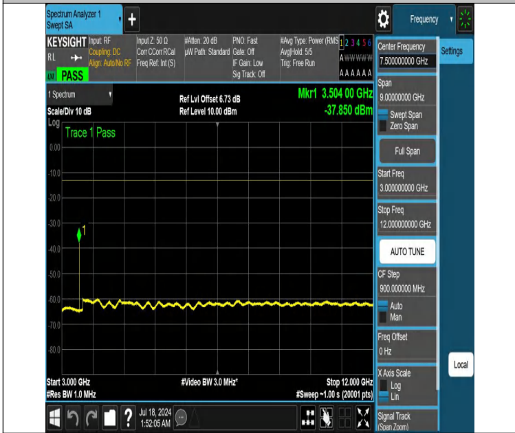
NTNV-DC_12A_n66A-PC3-15-5+15-M+M-N/A-N/A-DFT-QPSK-Edge_1RB_Right-3000-12000-PASS
