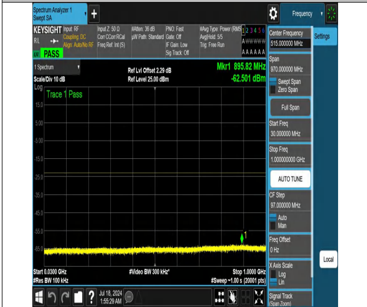
NTNV-DC_12A_n66A-PC3-15-5+15-M+H-N/A-N/A-DFT-QPSK-Edge e_1RB_Left-30-1000-PASS
