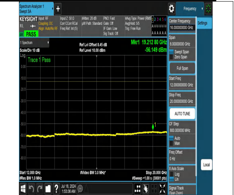
NTNV-DC_12A_n66A-PC3-15-5+15-M+H-N/A-N/A-DFT-PI2BPSK-E dge_1RB_Left-12000-20000-PASS
