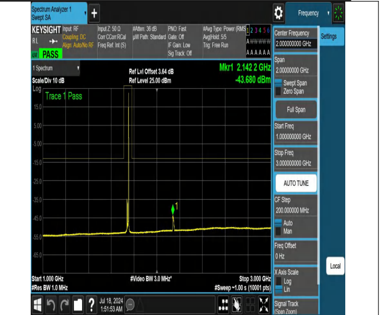
NTNV-DC_12A_n66A-PC3-15-5+15-M+M-N/A-N/A-DFT-QPSK-Edge_1RB_Right-1000-3000-PASS
