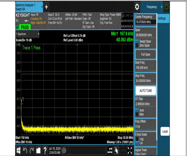
NTNV-DC_12A_n66A-PC3-15-5+20-M+M-N/A-N/A-DFT-PI2BPSK-E dge_1RB_Right-0.15-30-PASS
