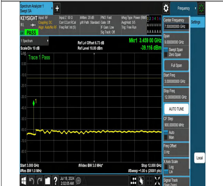
NTNV-DC_12A_n66A-PC3-15-5+20-M+L-N/A-N/A-DFT-QPSK-Edge e_1RB_Right-3000-12000-PASS
