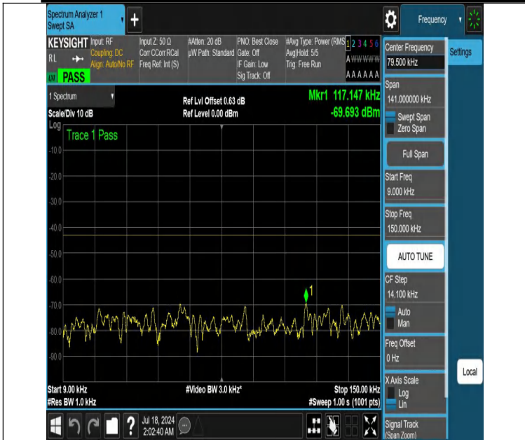
NTNV-DC_12A_n66A-PC3-15-5+20-M+M-N/A-N/A-DFT-PI2BPSK-Edge_1RB_Left-0.009-0.15-PASS
