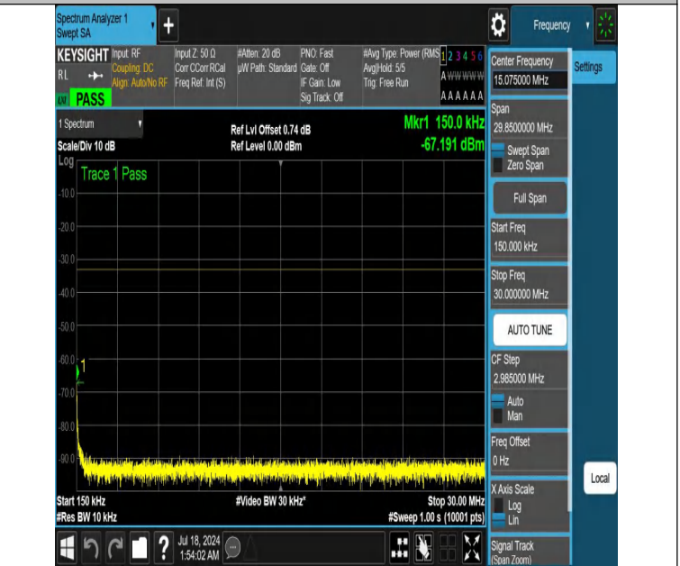
NTNV-DC_12A_n66A-PC3-15-5+15-M+H-N/A-N/A-DFT-PI2BPSK-E dge_1RB_Right-0.15-30-PASS
