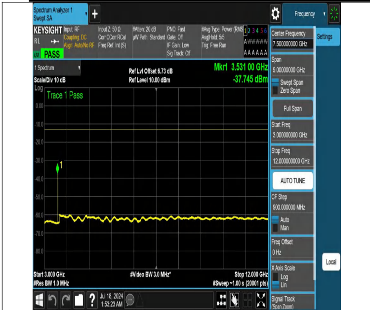
NTNV-DC_12A_n66A-PC3-15-5+15-M+H-N/A-N/A-DFT-PI2BPSK-Edge_1RB_Left-3000-12000-PASS
