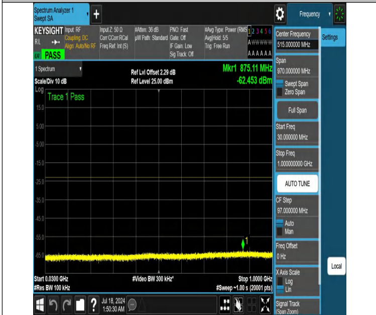
NTNV-DC_12A_n66A-PC3-15-5+15-M+M-N/A-N/A-DFT-QPSK-Edge_1RB_Left-30-1000-PASS
