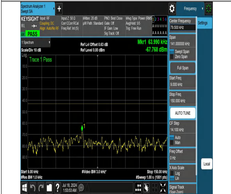
NTNV-DC_12A_n66A-PC3-15-5+15-M+H-N/A-N/A-DFT-PI2BPSK-Edge_1RB_Right-0.009-0.15-PASS
