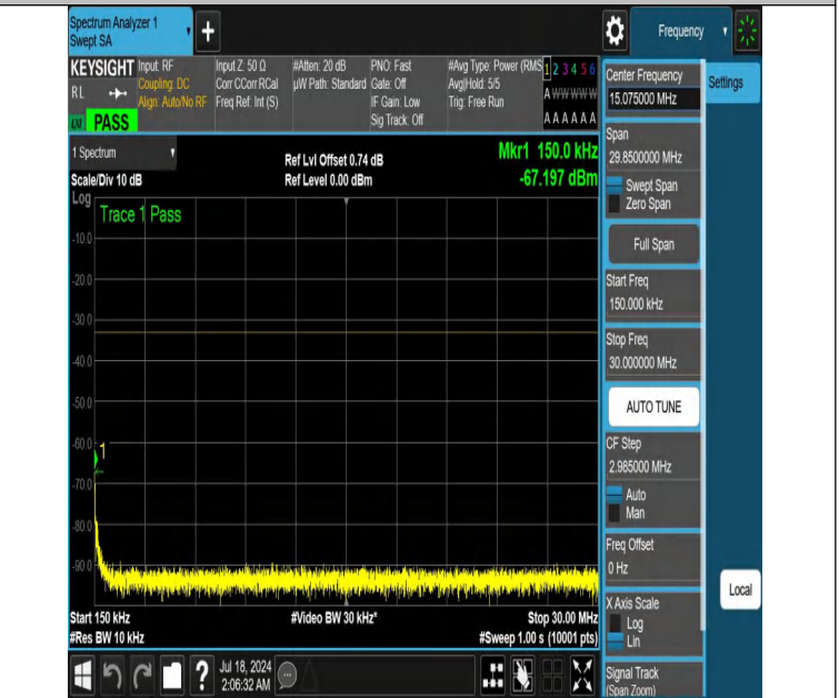
NTNV-DC_12A_n66A-PC3-15-5+20-M+M-N/A-N/A-DFT-QPSK-Edge_1RB_Right-0.15-30-PASS
