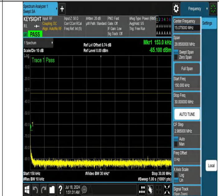
NTNV-DC_12A_n66A-PC3-15-5+15-M+M-N/A-N/A-DFT-QPSK-Edge_1RB_Right-0.15-30-PASS
