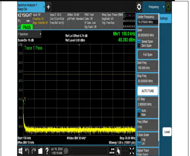
NTNV-DC_12A_n66A-PC3-15-5+15-M+H-N/A-N/A-DFT-QPSK-Edge e_1RB_Left-0.15-30-PASS
