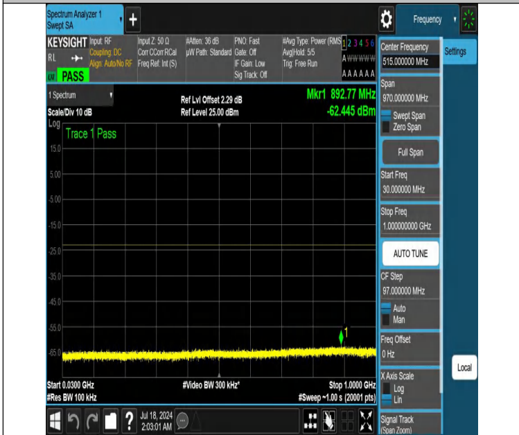
NTNV-DC_12A_n66A-PC3-15-5+20-M+M-N/A-N/A-DFT-PI2BPSK-Edge_1RB_Left-30-1000-PASS
