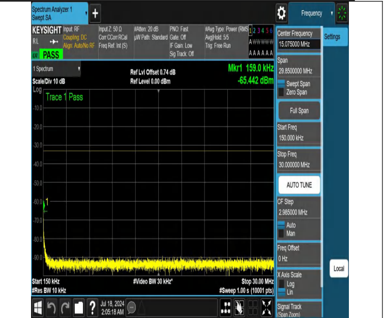
NTNV-DC_12A_n66A-PC3-15-5+20-M+M-N/A-N/A-DFT-QPSK-Edge_1RB_Left-0.15-30-PASS
