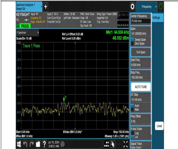
NTNV-DC_12A_n66A-PC3-15-5+20-M+M-N/A-N/A-DFT-QPSK-Edge_1RB_Right-0.009-0.15-PASS
