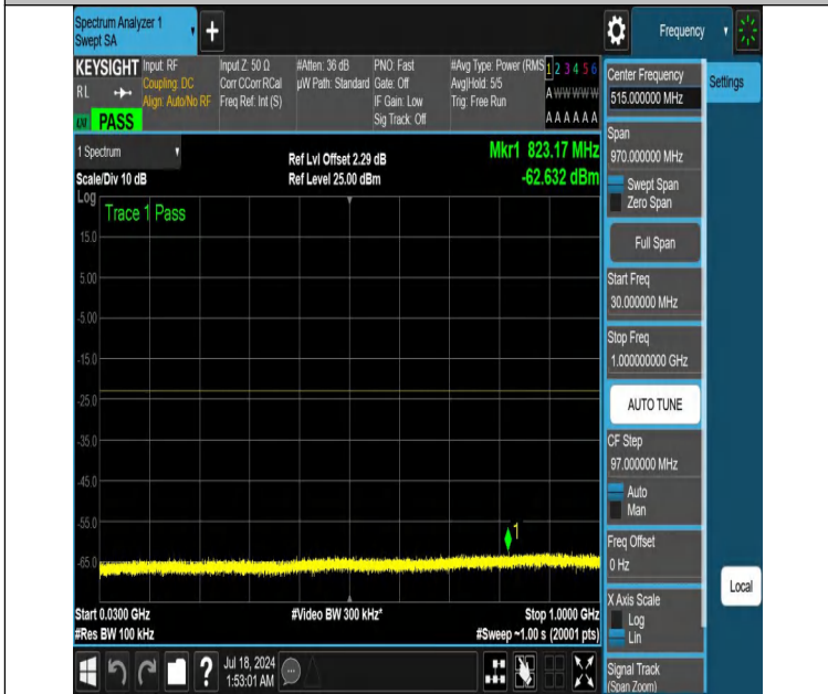
NTNV-DC_12A_n66A-PC3-15-5+15-M+H-N/A-N/A-DFT-PI2BPSK-Edge_1RB_Left-30-1000-PASS
