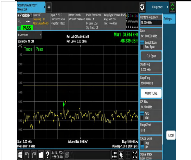
NTNV-DC_12A_n66A-PC3-15-5+15-M+H-N/A-N/A-DFT-QPSK-Edge e_1RB_Left-0.009-0.15-PASS
