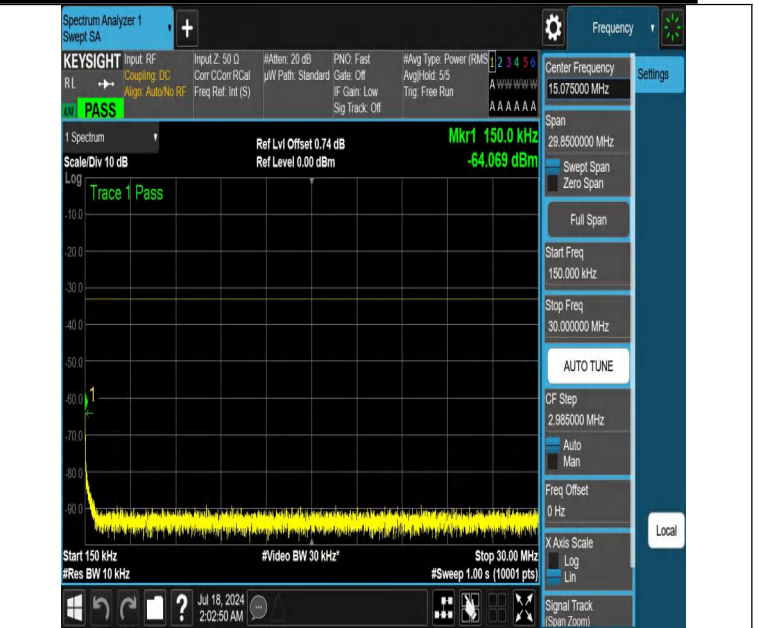
NTNV-DC_12A_n66A-PC3-15-5+20-M+M-N/A-N/A-DFT-PI2BPSK-E dge_1RB_Left-0.15-30-PASS
