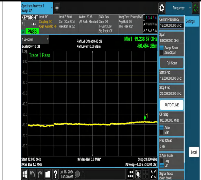
NTNV-DC_12A_n66A-PC3-15-5+15-M+M-N/A-N/A-DFT-QPSK-Edge_1RB_Left-12000-20000-PASS
