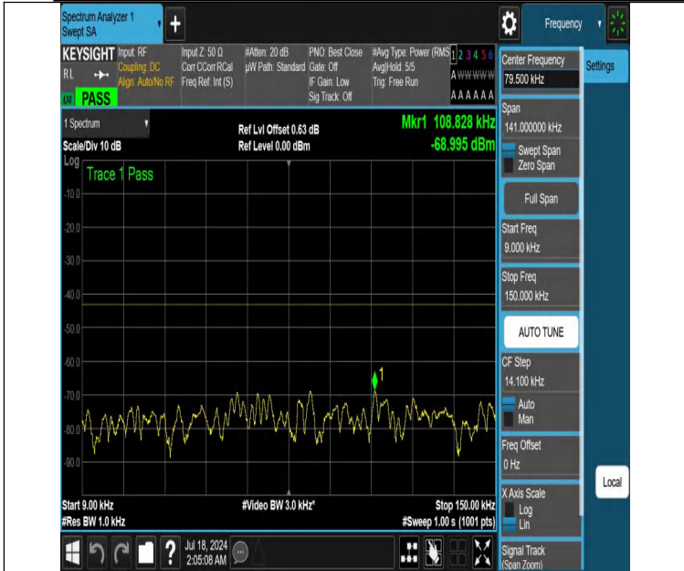
NTNV-DC_12A_n66A-PC3-15-5+20-M+M-N/A-N/A-DFT-QPSK-Edge_1RB_Left-0.009-0.15-PASS
