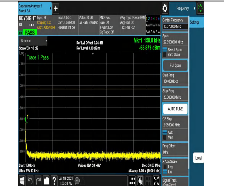
NTNV-DC_12A_n66A-PC3-15-5+15-M+H-N/A-N/A-DFT-QPSK-Edge e_1RB_Right-0.15-30-PASS
