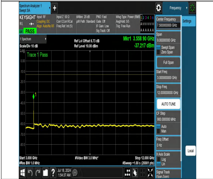
NTNV-DC_12A_n66A-PC3-15-5+15-M+H-N/A-N/A-DFT-PI2BPSK-Edge_1RB_Right-3000-12000-PASS
