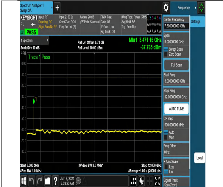
NTNV-DC_12A_n66A-PC3-15-5+20-M+M-N/A-N/A-DFT-PI2BPSK-Edge_1RB_Left-3000-12000-PASS
