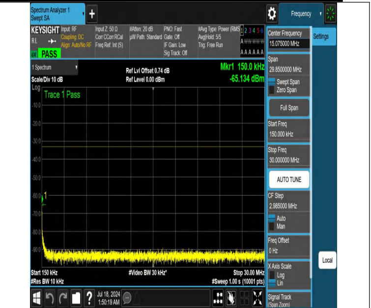
NTNV-DC_12A_n66A-PC3-15-5+15-M+M-N/A-N/A-DFT-QPSK-Edge_1RB_Left-0.15-30-PASS
