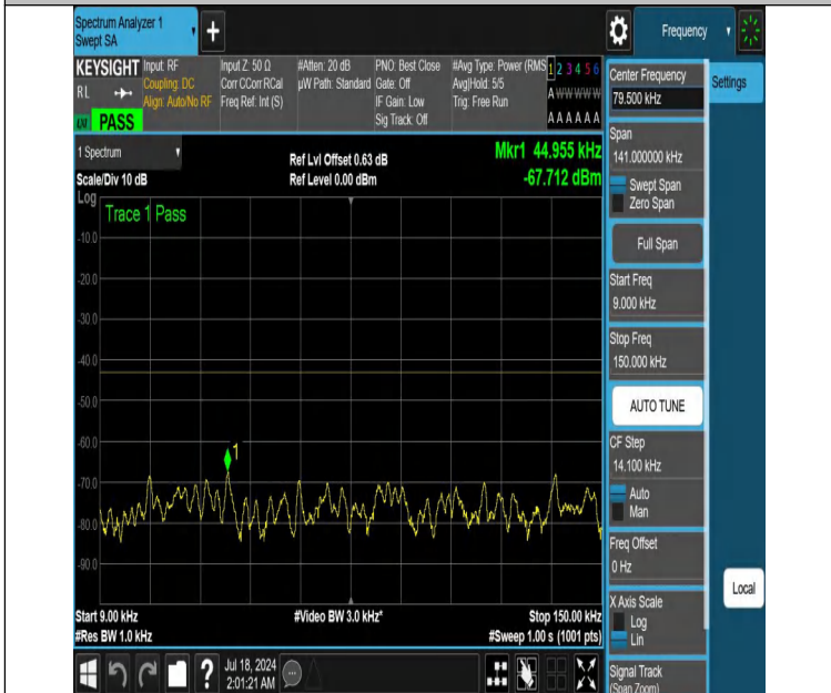
NTNV-DC_12A_n66A-PC3-15-5+20-M+L-N/A-N/A-DFT-QPSK-Edge e_1RB_Right-0.009-0.15-PASS
