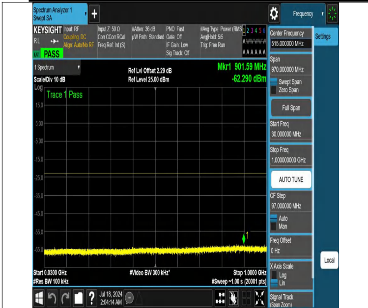
NTNV-DC_12A_n66A-PC3-15-5+20-M+M-N/A-N/A-DFT-PI2BPSK-Edge_1RB_Right-30-1000-PASS
