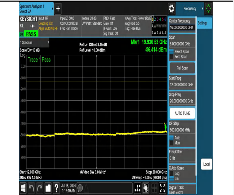
NTNV-DC_12A_n66A-PC3-15-5+5-M+L-N/A-N/A-DFT-QPSK-Edge_1RB_Right-12000-20000-PASS
