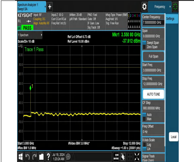
NTNV-DC_12A_n66A-PC3-15-5+5-M+H-N/A-N/A-DFT-PI2BPSK-E dge_1RB_Left-3000-12000-PASS
