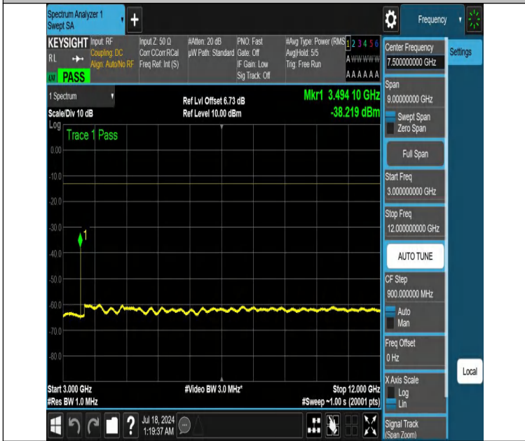
NTNV-DC_12A_n66A-PC3-15-5+5-M+M-N/A-N/A-DFT-PI2BPSK-E dge_1RB_Right-3000-12000-PASS
