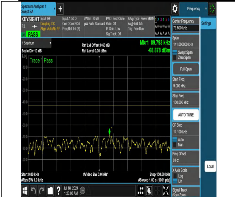
NTNV-DC_12A_n66A-PC3-15-5+5-M+M-N/A-N/A-DFT-QPSK-Edge e_1RB_Left-0.009-0.15-PASS
