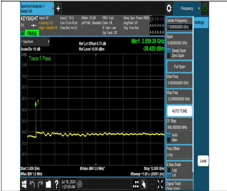
NTNV-DC_12A_n66A-PC3-15-5+5-M+H-N/A-N/A-DFT-QPSK-Edge _1RB_Right-3000-12000-PASS
