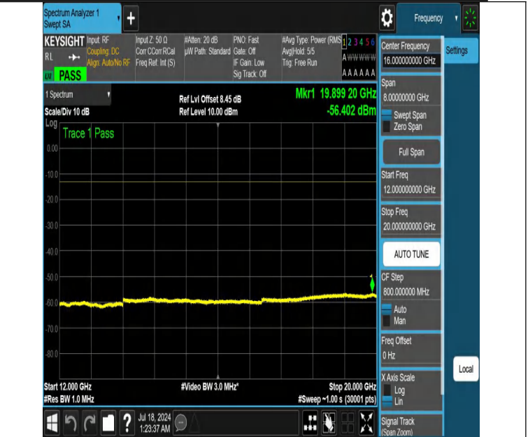
NTNV-DC_12A_n66A-PC3-15-5+5-M+H-N/A-N/A-DFT-PI2BPSK-Ed ge_1RB_Left-12000-20000-PASS
