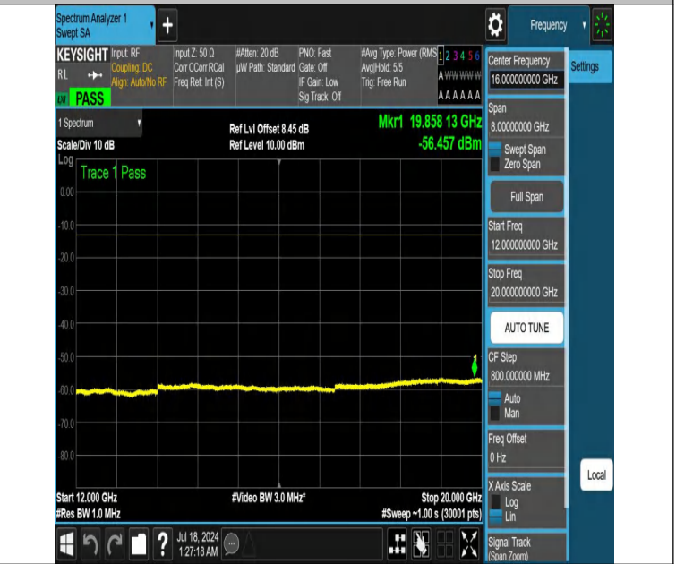
NTNV-DC_12A_n66A-PC3-15-5+5-M+H-N/A-N/A-DFT-QPSK-Edge _1RB_Right-12000-20000-PASS
