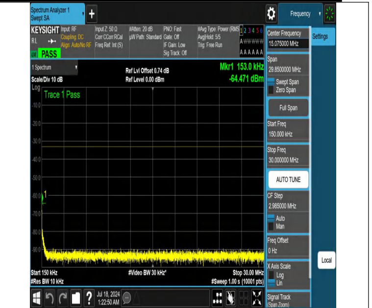
NTNV-DC_12A_n66A-PC3-15-5+5-M+H-N/A-N/A-DFT-PI2BPSK-Ed ge_1RB_Left-0.15-30-PASS
