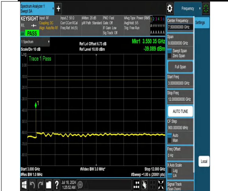
NTNV-DC_12A_n66A-PC3-15-5+5-M+H-N/A-N/A-DFT-QPSK-Edge _1RB_Left-3000-12000-PASS
