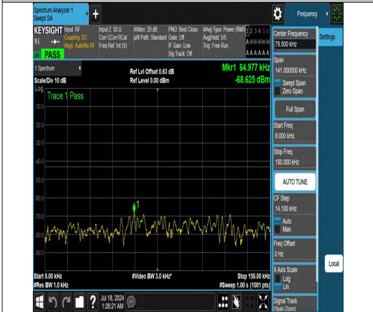
NTNV-DC_12A_n66A-PC3-15-5+5-M+H-N/A-N/A-DFT-QPSK-Edge _1RB_Right-0.009-0.15-PASS
