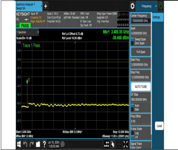
NTNV-DC_12A_n66A-PC3-15-5+5-M+M-N/A-N/A-DFT-QPSK-Edge e_1RB_Left-3000-12000-PASS
