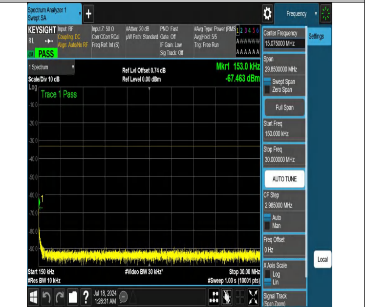
NTNV-DC_12A_n66A-PC3-15-5+5-M+H-N/A-N/A-DFT-QPSK-Edge _1RB_Right-0.15-30-PASS
