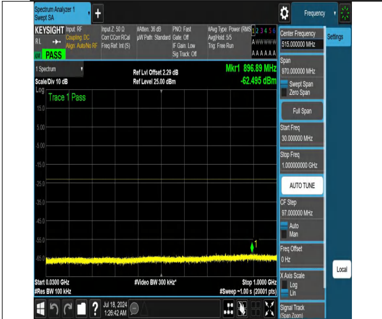
NTNV-DC_12A_n66A-PC3-15-5+5-M+H-N/A-N/A-DFT-QPSK-Edge _1RB_Right-30-1000-PASS
