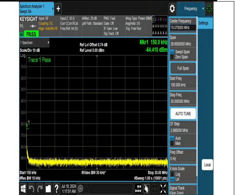
NTNV-DC_12A_n66A-PC3-15-5+5-M+M-N/A-N/A-DFT-PI2BPSK-Ed ge_1RB_Left-0.15-30-PASS
