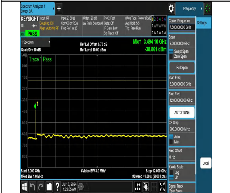
NTNV-DC_12A_n66A-PC3-15-5+5-M+M-N/A-N/A-DFT-QPSK-Edge e_1RB_Right-3000-12000-PASS
