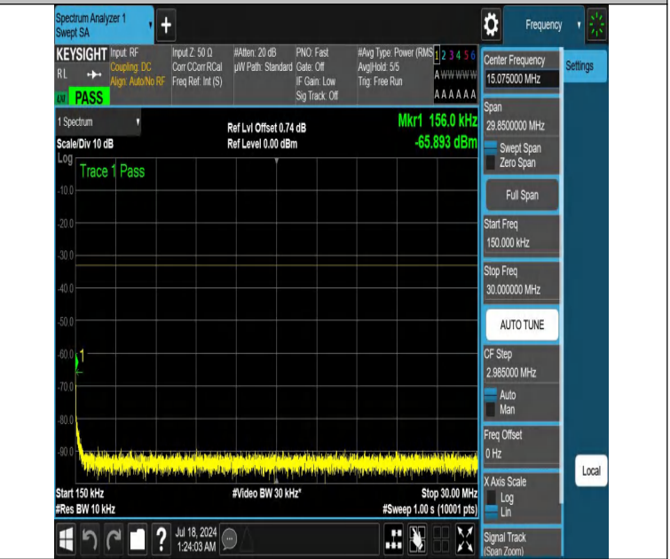
NTNV-DC_12A_n66A-PC3-15-5+5-M+H-N/A-N/A-DFT-PI2BPSK-Ed ge_1RB_Right-0.15-30-PASS
