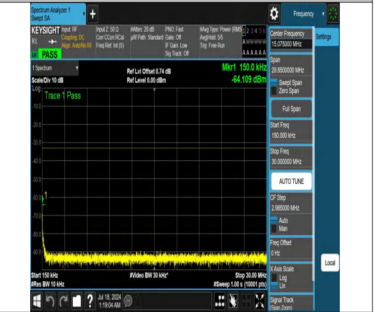
NTNV-DC_12A_n66A-PC3-15-5+5-M+M-N/A-N/A-DFT-PI2BPSK-Ed ge_1RB_Right-0.15-30-PASS
