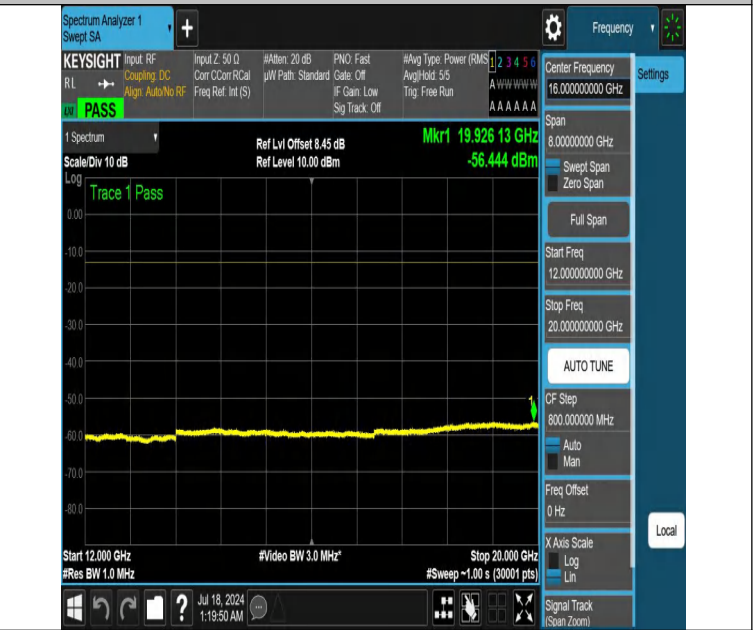
NTNV-DC_12A_n66A-PC3-15-5+5-M+M-N/A-N/A-DFT-PI2BPSK-Ed ge_1RB_Right-12000-20000-PASS
