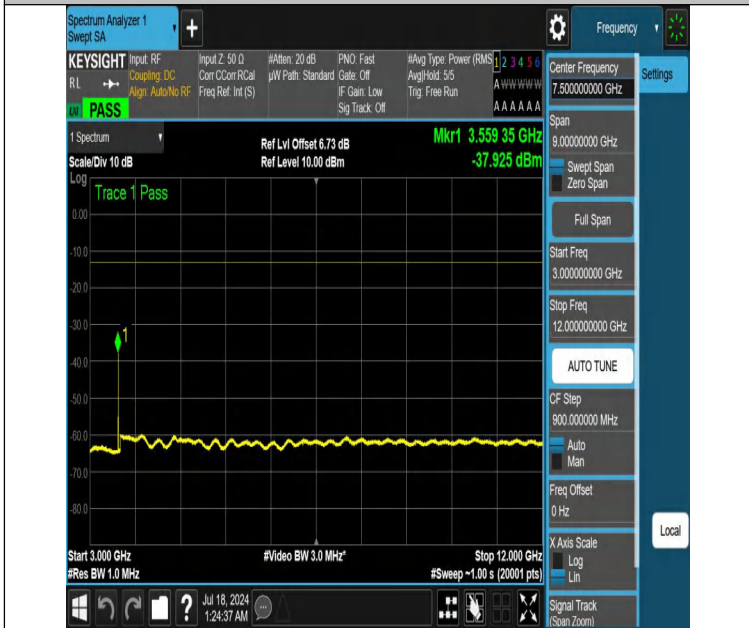
NTNV-DC_12A_n66A-PC3-15-5+5-M+H-N/A-N/A-DFT-PI2BPSK-E dge_1RB_Right-3000-12000-PASS
