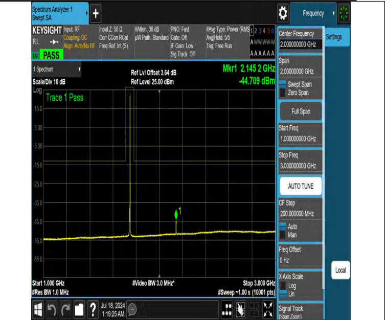
NTNV-DC_12A_n66A-PC3-15-5+5-M+M-N/A-N/A-DFT-PI2BPSK-Ed ge_1RB_Right-1000-3000-PASS
