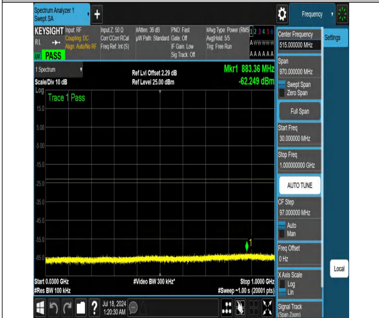
NTNV-DC_12A_n66A-PC3-15-5+5-M+M-N/A-N/A-DFT-QPSK-Edge e_1RB_Left-30-1000-PASS
