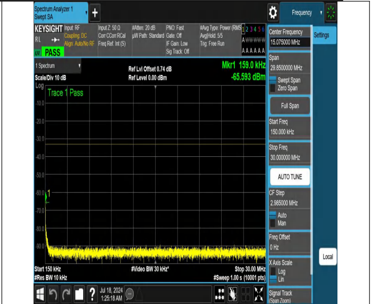
NTNV-DC_12A_n66A-PC3-15-5+5-M+H-N/A-N/A-DFT-QPSK-Edge _1RB_Left-0.15-30-PASS
