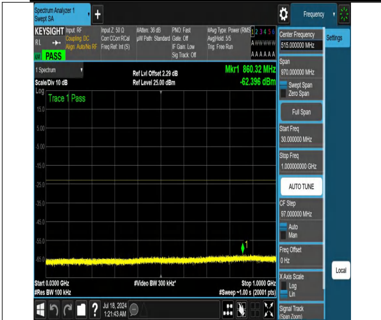
NTNV-DC_12A_n66A-PC3-15-5+5-M+M-N/A-N/A-DFT-QPSK-Edge e_1RB_Right-30-1000-PASS
