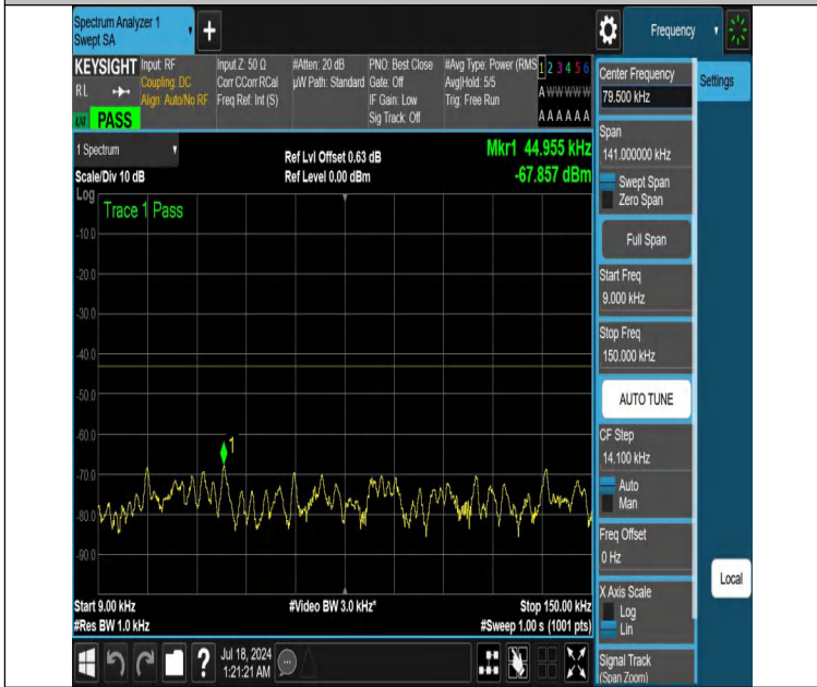
NTNV-DC_12A_n66A-PC3-15-5+5-M+M-N/A-N/A-DFT-QPSK-Edge e_1RB_Right-0.009-0.15-PASS
