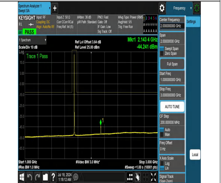
NTNV-DC_12A_n66A-PC3-15-5+5-M+M-N/A-N/A-DFT-PI2BPSK-Ed ge_1RB_Left-1000-3000-PASS
