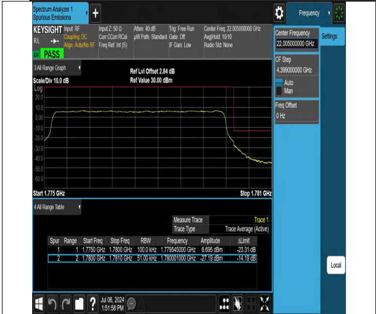
NTNV-DC_12A_n66A-PC3-15-5+5-M+H-N/A-N/A-DFT-PI2BPSK-Outer_Full-PASS
