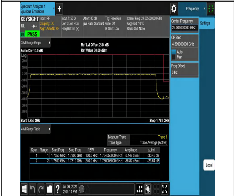
NTNV-DC_12A_n66A-PC3-15-5+25-M+H-N/A-N/A-DFT-QPSK-Outter_Full-PASS
