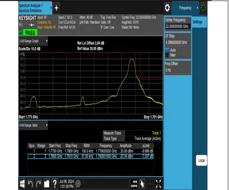
NTNV-DC_12A_n66A-PC3-15-5+5-M+H-N/A-N/A-DFT-PI2BPSK-Edge_1RB_Right-PASS
