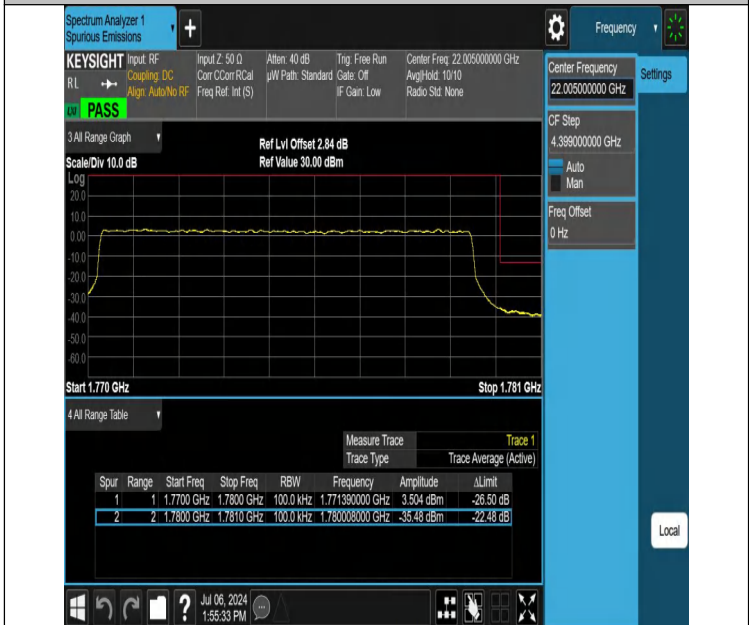
NTNV-DC_12A_n66A-PC3-15-5+10-M+H-N/A-N/A-DFT-QPSK-Outter_Full-PASS
