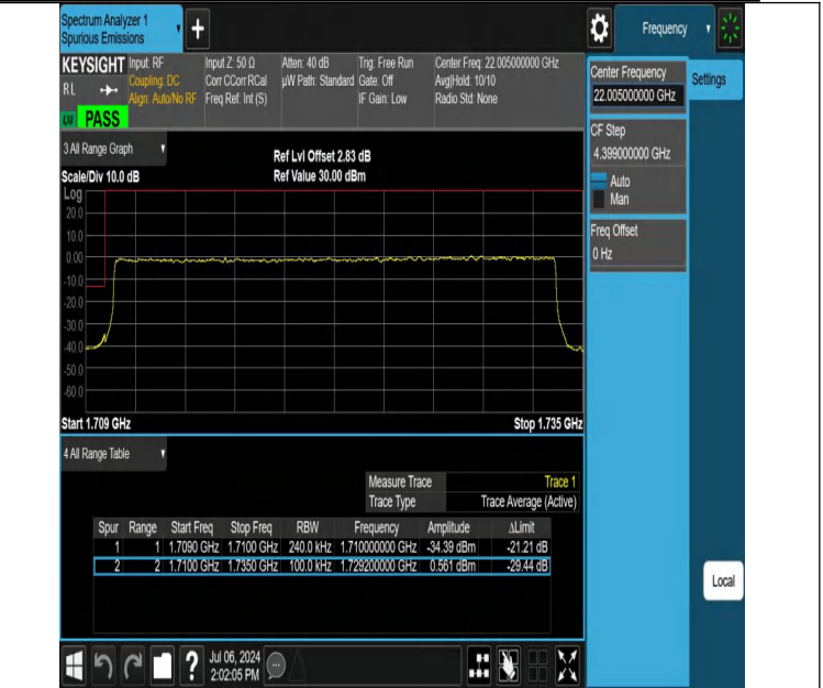
NTVN-DC_12A_n66A-PC3-15-5+25-M+L-N/A-N/A-DFT-PI2BPSK-Outer_Full-PASS
