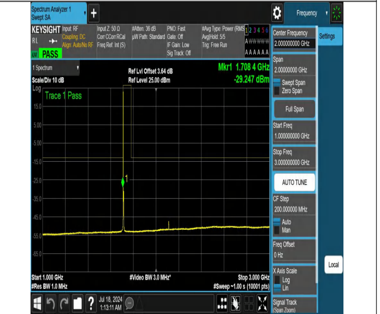
NTNV-DC_12A_n66A-PC3-15-5+5-M+L-N/A-N/A-DFT-PI2BPSK-Ed ge_1RB_Left-1000-3000-PASS
