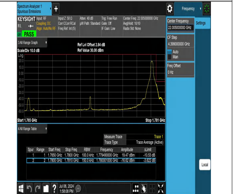
NTNV-DC_12A_n66A-PC3-15-5+15-M+H-N/A-N/A-DFT-QPSK-Edge_1RB_Right-PASS
