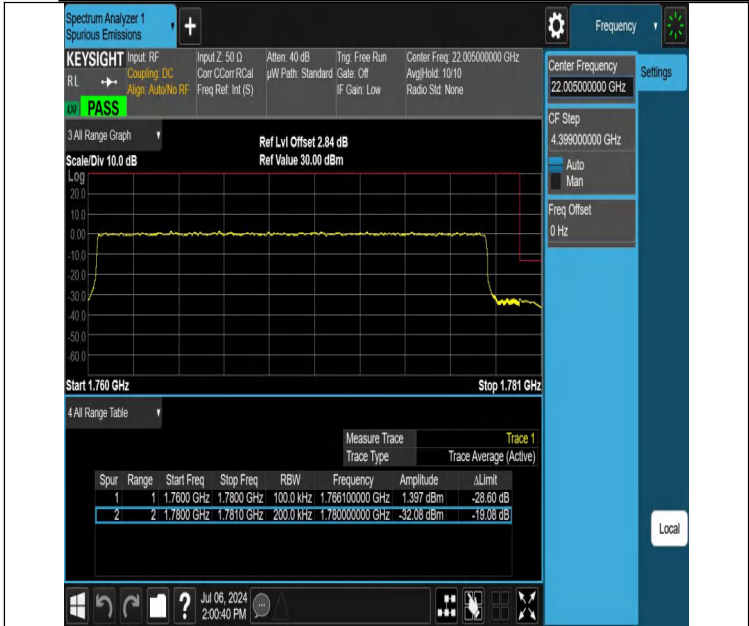
NTNV-DC_12A_n66A-PC3-15-5+20-M+H-N/A-N/A-DFT-PI2BPSK-Outter_Full-PASS
