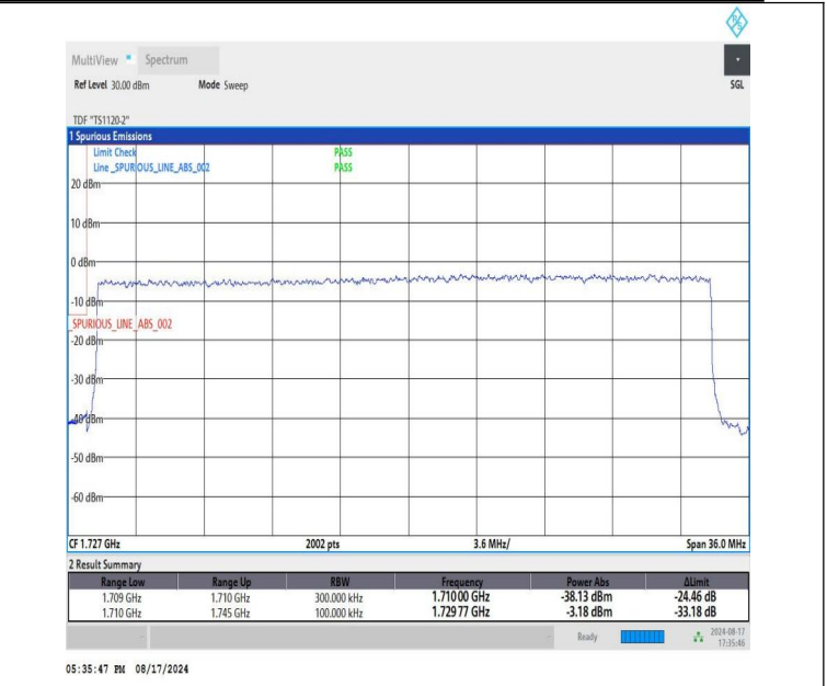
NTNV-DC_12A-n66A-PC3-15-5+35-M+L-QPSK-IDLE-DFT-BPSK-Outer_Full-PASS
