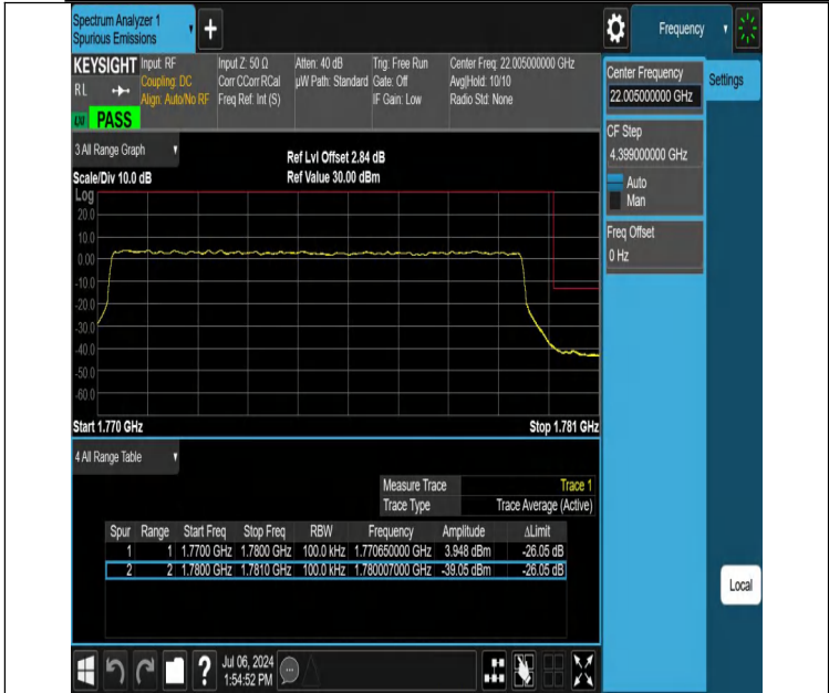
NTNV-DC_12A_n66A-PC3-15-5+10-M+H-N/A-N/A-DFT-PI2BPSK-Outter_Full-PASS
