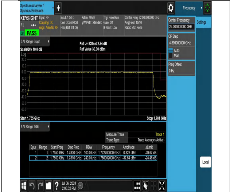
NTNV-DC_12A_n66A-PC3-15-5+25-M+H-N/A-N/A-DFT-PI2BPSK-Outter_Full-PASS
