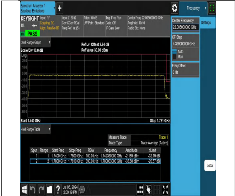
NTVN-DC_12A_n66A-PC3-15-5+40-M+H-N/A-N/A-DFT-PI2BPSK-Outter_Full-PASS
