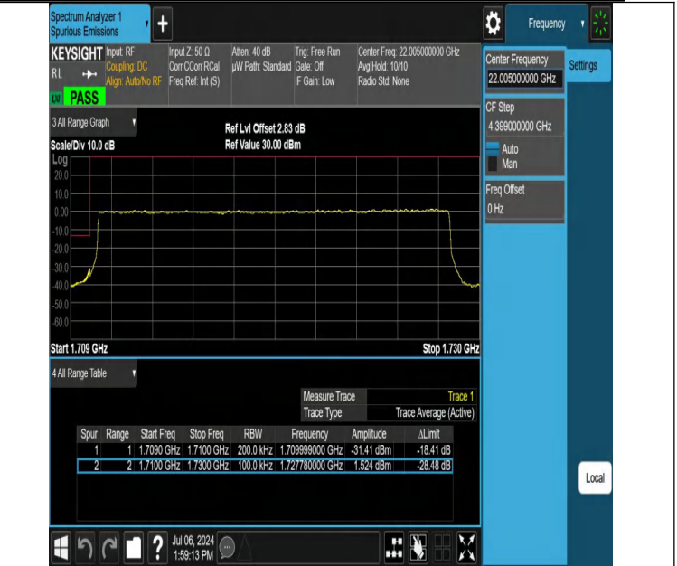
NTVN-DC_12A_n66A-PC3-15-5+20-M+L-N/A-N/A-DFT-PI2BPSK-Outer_Full-PASS
