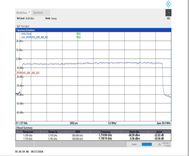
NTNV-DC_12A-n66A-PC3-15-5+35-M+L-QPSK-IDLE-DFT-QPSK-Outer_Full-PASS
