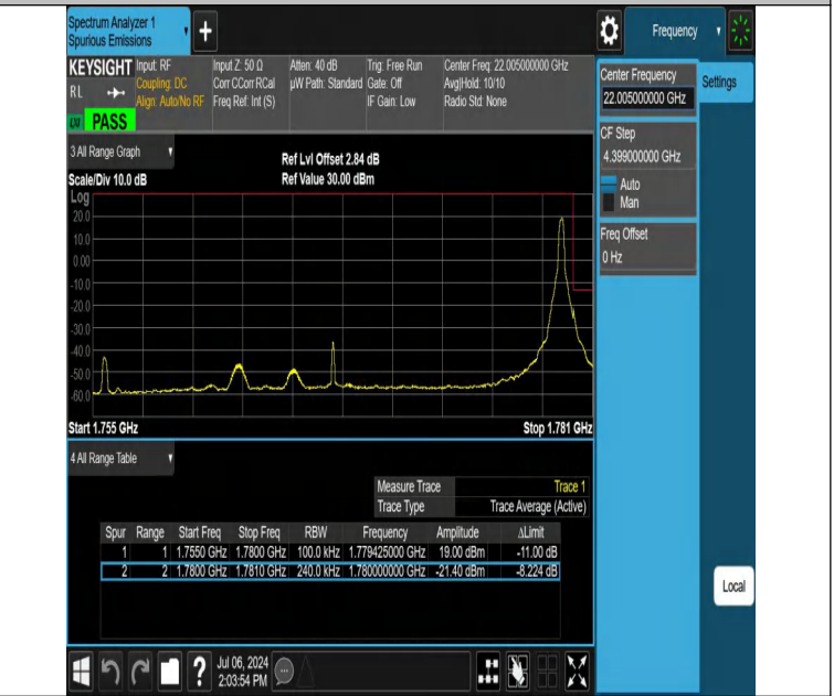
NTNV-DC_12A_n66A-PC3-15-5+25-M+H-N/A-N/A-DFT-QPSK-Edge_1RB_Right-PASS
