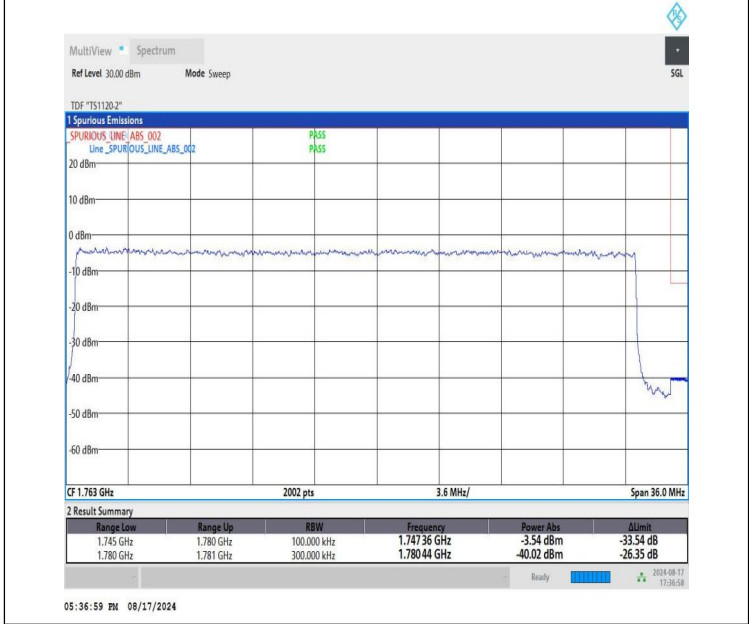
NTVN-DC_12A-n66A-PC3-15-5+35-M+H-QPSK-IDLE-DFT-QPSK-Outer_Full-PASS
