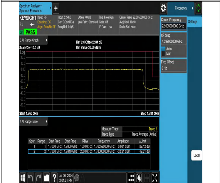
NTNV-DC_12A_n66A-PC3-15-5+20-M+H-N/A-N/A-DFT-QPSK-Outter_Full-PASS
