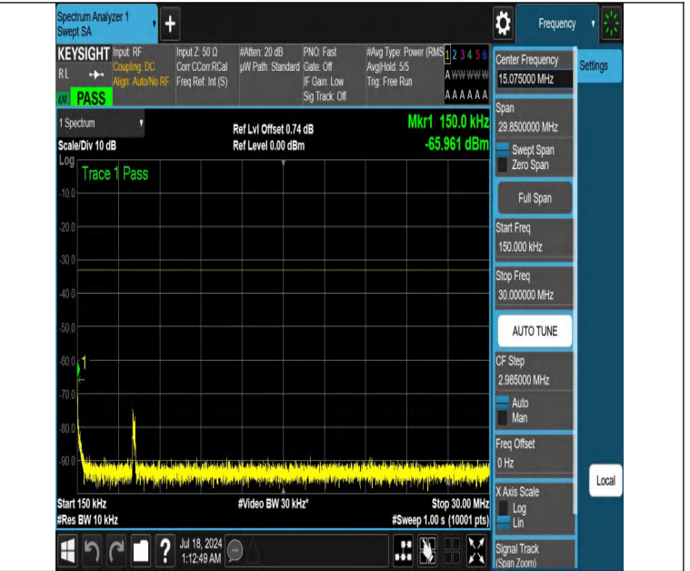
NTNV-DC_12A_n66A-PC3-15-5+5-M+L-N/A-N/A-DFT-PI2BPSK-Ed ge_1RB_Left-0.15-30-PASS
