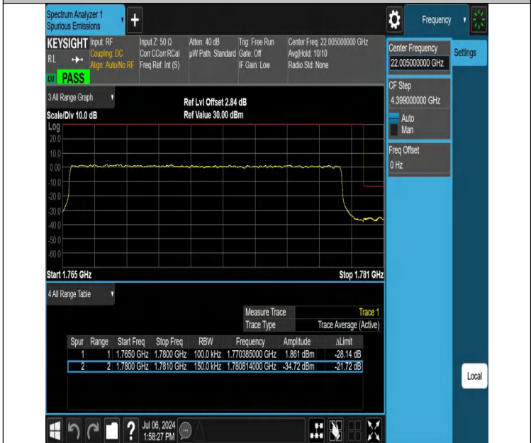
NTNV-DC_12A_n66A-PC3-15-5+15-M+H-N/A-N/A-DFT-QPSK-Outter_Full-PASS
