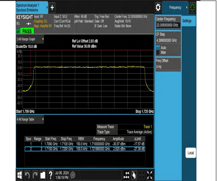
NTVN-DC_12A_n66A-PC3-15-5+15-M+L-N/A-N/A-DFT-PI2BPSK-Outer_Full-PASS
