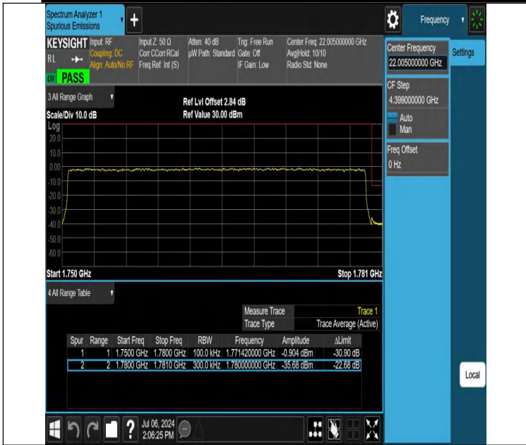
NTNV-DC_12A_n66A-PC3-15-5+30-M+H-N/A-N/A-DFT-PI2BPSK-Outter_Full-PASS
