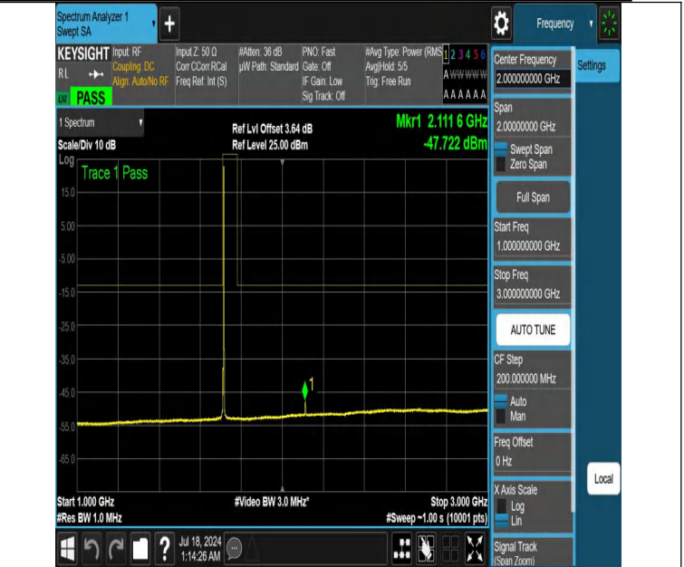
NTNV-DC_12A_n66A-PC3-15-5+5-M+L-N/A-N/A-DFT-PI2BPSK-Ed ge_1RB_Right-1000-3000-PASS
