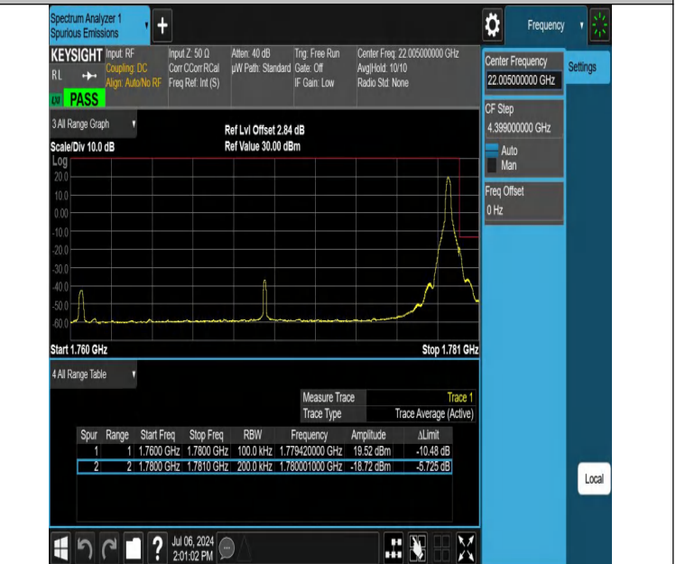
NTNV-DC_12A_n66A-PC3-15-5+20-M+H-N/A-N/A-DFT-QPSK-Edge_1RB_Right-PASS
