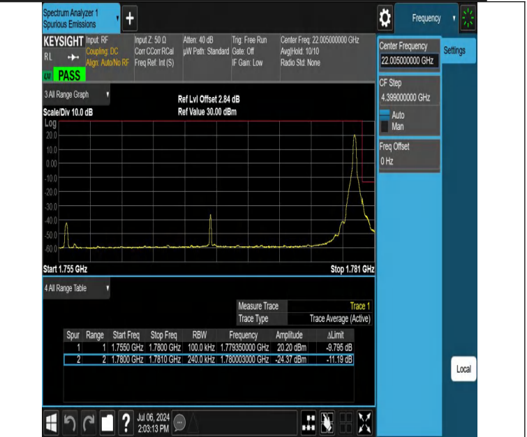
NTNV-DC_12A_n66A-PC3-15-5+25-M+H-N/A-N/A-DFT-PI2BPSK-E dge_1RB_Right-PASS
