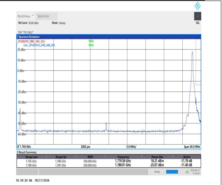
NTVN-DC_12A-n66A-PC3-15-5+35-M+H-QPSK-IDLE-DFT-BPSK-E dge_1RB_Right-PASS
