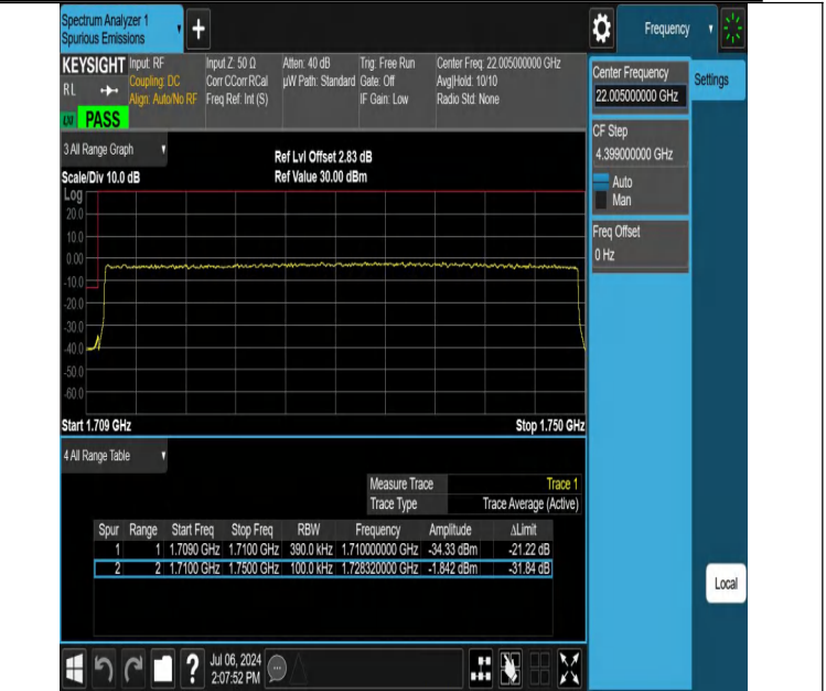
NTVN-DC_12A_n66A-PC3-15-5+40-M+L-N/A-N/A-DFT-PI2BPSK-Outer_Full-PASS
