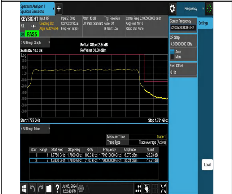
NTNV-DC_12A_n66A-PC3-15-5+5-M+H-N/A-N/A-DFT-QPSK-Outer_Full-PASS
