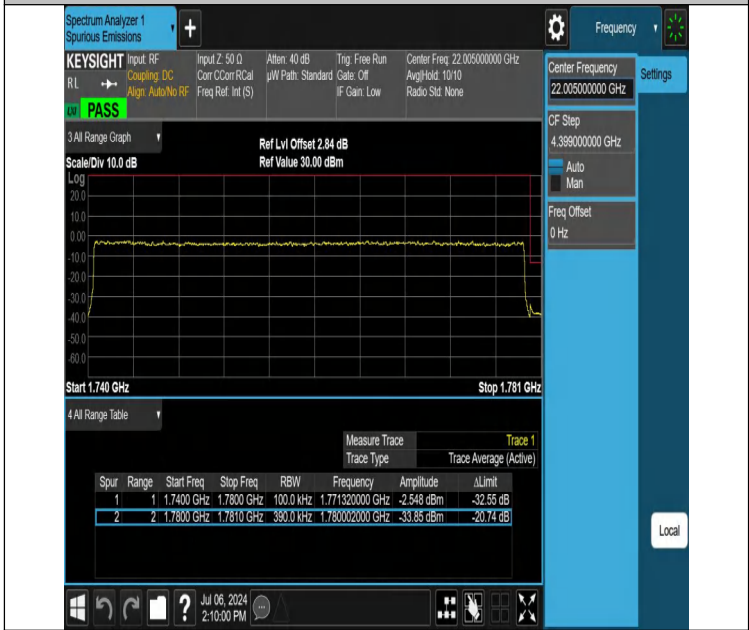
NTVN-DC_12A_n66A-PC3-15-5+40-M+H-N/A-N/A-DFT-QPSK-Out er_Full-PASS
