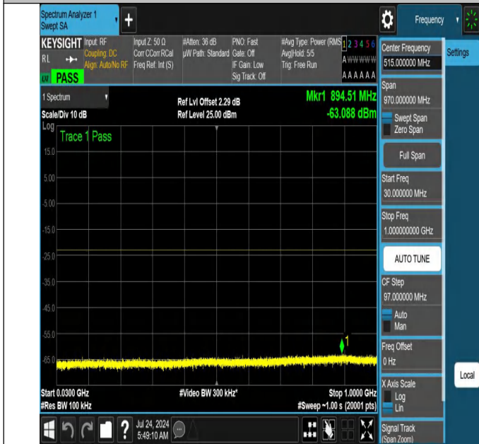
NTNV-N66-PC3-15-40-H-DFT-PI2BPSK-Edge_1RB_Left-30-1000-Ant1-PASS
