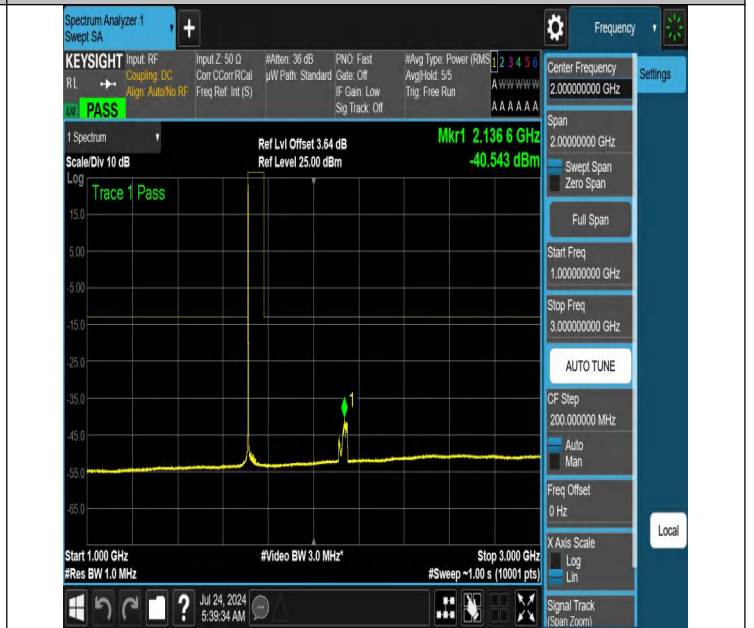
NTNV-N66-PC3-15-40-L-DFT-PI2BPSK-Edge_1RB_Left-1000-3000-Ant1-PASS
