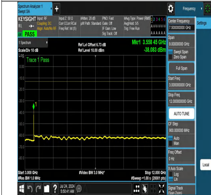
NTNV-N66-PC3-15-40-H-DFT-PI2BPSK-Edge_1RB_Right-3000-12000-Ant1-PASS
