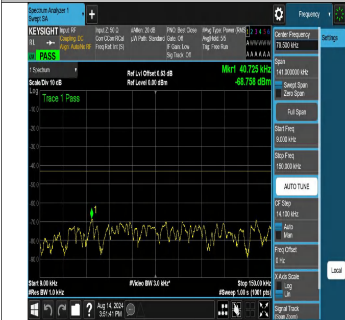
NTNV-N66-PC3-15-30-H-DFT-QPSK-Edge_1RB_Right-0.009-0.1 5-Ant1-PASS
