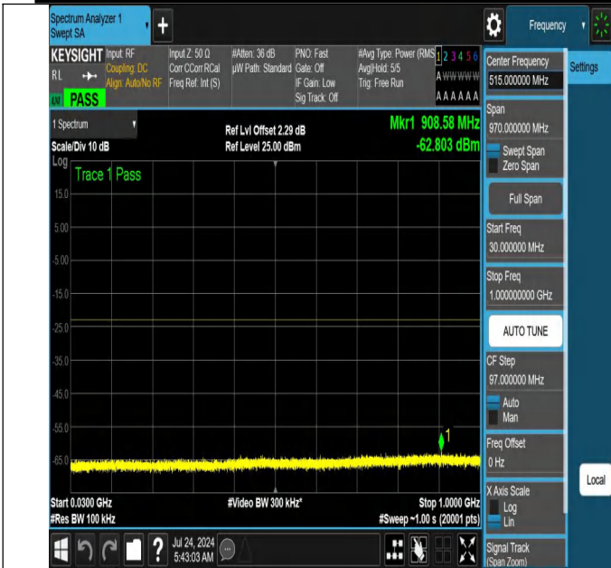
NTNV-N66-PC3-15-40-L-DFT-QPSK-Edge_1RB_Right-30-1000-Ant1-PASS
