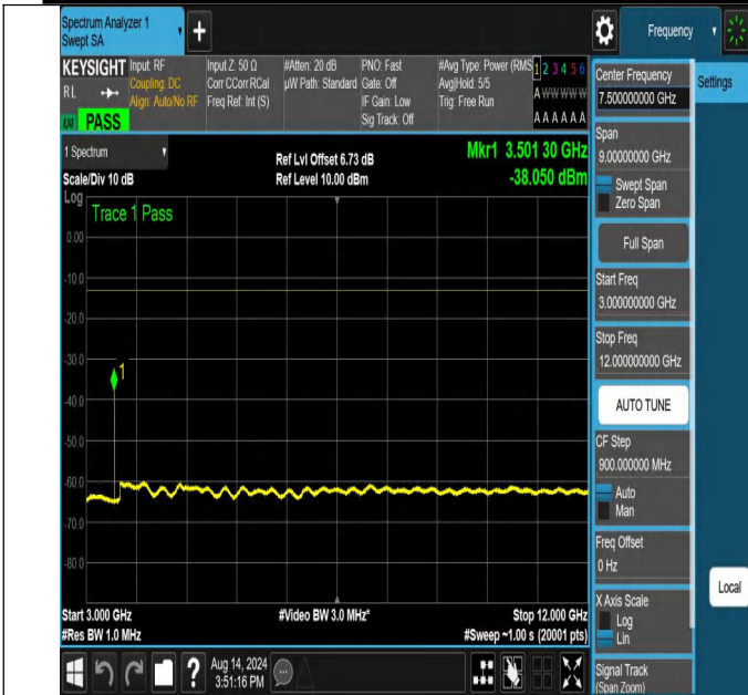
NTNV-N66-PC3-15-30-H-DFT-QPSK-Edge_1RB_Left-3000-1200 0-Ant1-PASS
