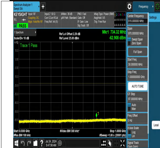
NTNV-N66-PC3-15-40-M-DFT-QPSK-Edge_1RB_Right-30-1000-Ant1-PASS
