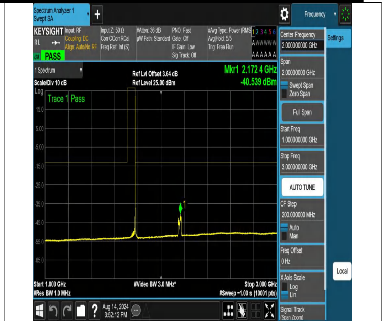
NTNV-N66-PC3-15-30-H-DFT-QPSK-Edge_1RB_Right-1000-300-0-Ant1-PASS
