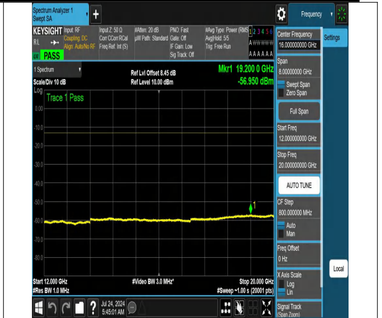
NTNV-N66-PC3-15-40-M-DFT-PI2BPSK-Edge_1RB_Left-12000-2 0000-Ant1-PASS
