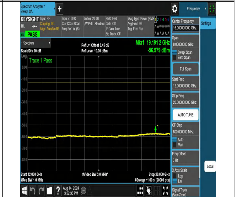
NTNV-N66-PC3-15-30-H-DFT-QPSK-Edge_1RB_Right-12000-2000-000-Ant1-PASS
