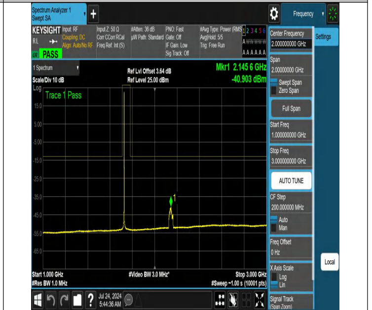
NTNV-N66-PC3-15-40-M-DFT-PI2BPSK-Edge_1RB_Left-1000-3000-Ant1-PASS
