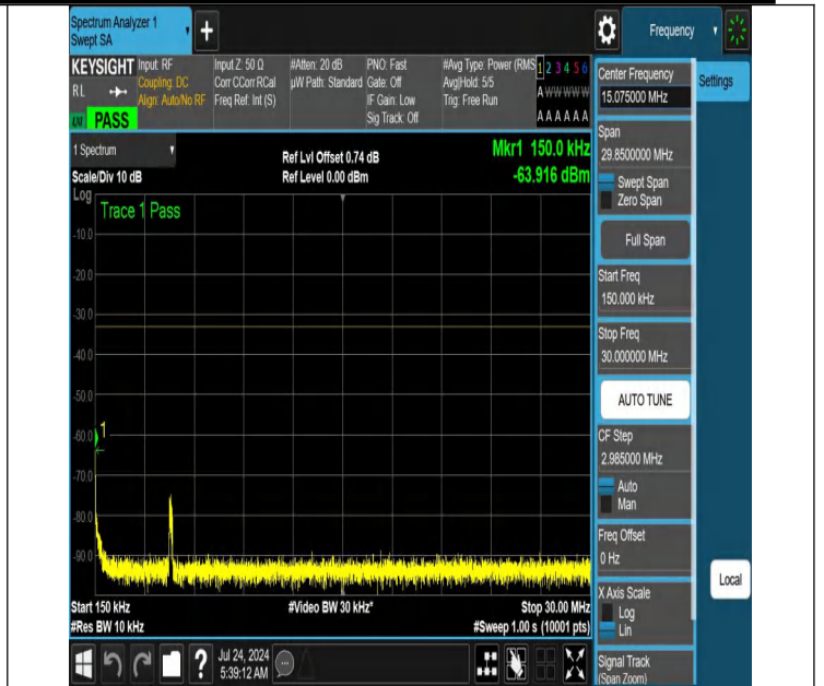
NTNV-N66-PC3-15-40-L-DFT-PI2BPSK-Edge_1RB_Left-0.15-30-Ant1-PASS
