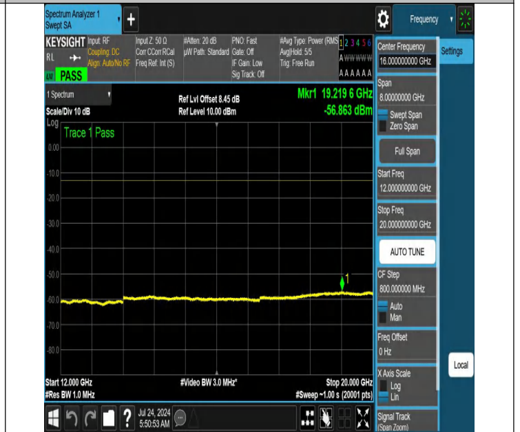
NTNV-N66-PC3-15-40-H-DFT-PI2BPSK-Edge_1RB_Right-12000-20000-Ant1-PASS
