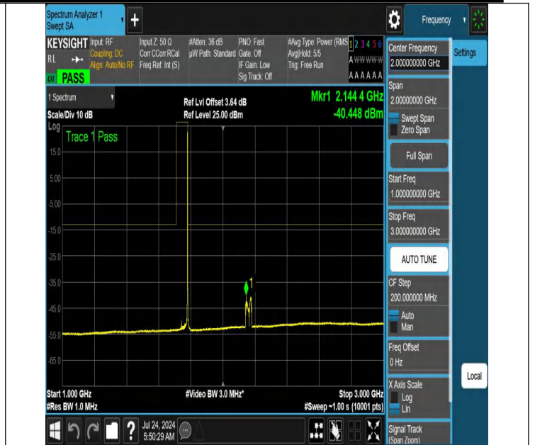
NTNV-N66-PC3-15-40-H-DFT-PI2BPSK-Edge_1RB_Right-1000-3000-Ant1-PASS
