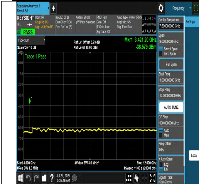
NTNV-N66-PC3-15-40-L-DFT-PI2BPSK-Edge_1RB_Left-3000-12000-Ant1-PASS
