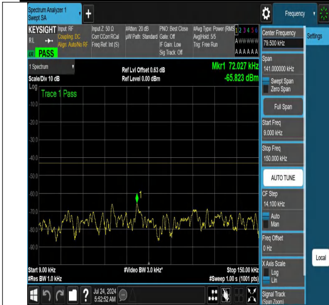
NTNV-N66-PC3-15-40-H-DFT-QPSK-Edge_1RB_Left-0.009-0.15 -Ant1-PASS
