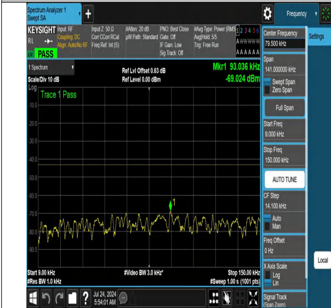
NTNV-N66-PC3-15-40-H-DFT-QPSK-Edge_1RB_Right-0.009-0.1 5-Ant1-PASS
