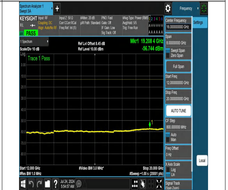
NTNV-N66-PC3-15-40-H-DFT-QPSK-Edge_1RB_Right-12000-20000-Ant1-PASS
