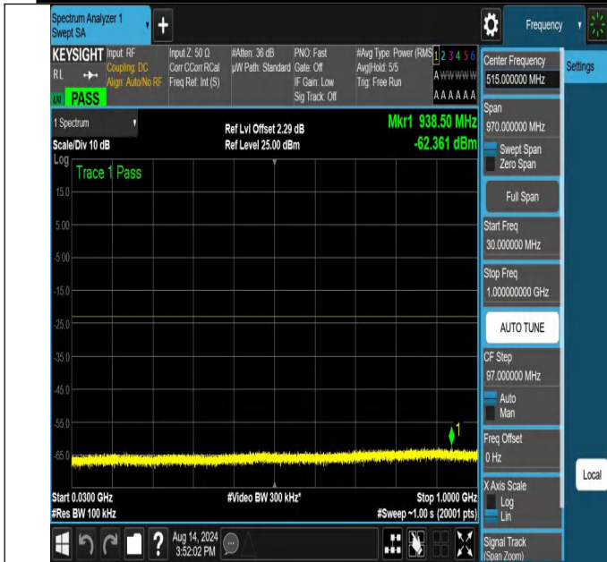
NTNV-N66-PC3-15-30-H-DFT-QPSK-Edge_1RB_Right-30-1000-Ant1-PASS
