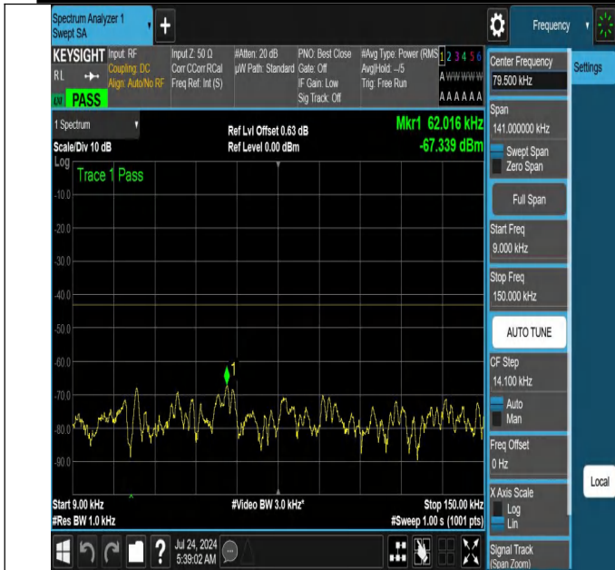
NTNV-N66-PC3-15-40-L-DFT-PI2BPSK-Edge_1RB_Left-0.009-0.15-Ant1-PASS
