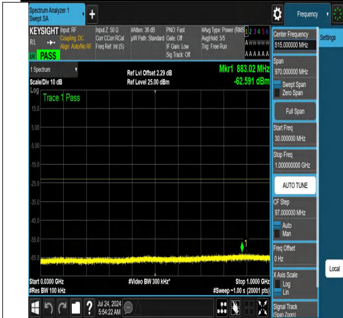
NTNV-N66-PC3-15-40-H-DFT-QPSK-Edge_1RB_Right-30-1000-Ant1-PASS
