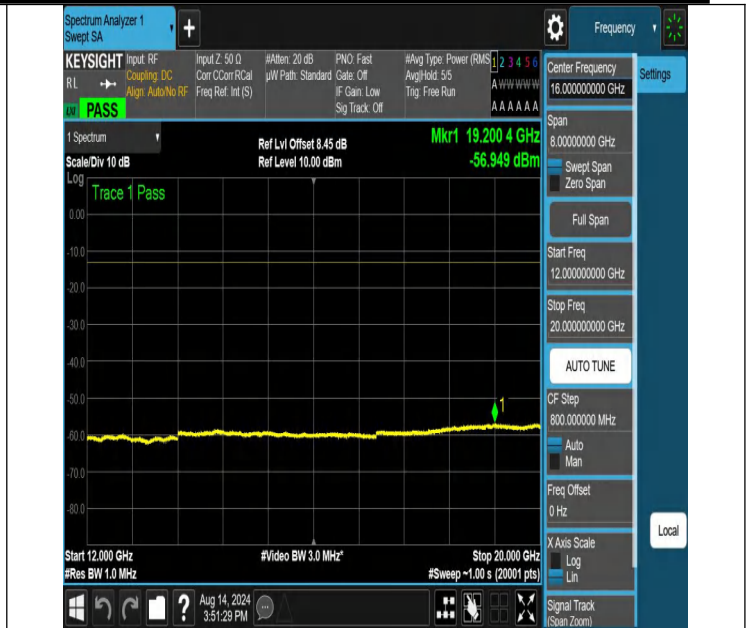
NTNV-N66-PC3-15-30-H-DFT-QPSK-Edge_1RB_Left-12000-2000 0-Ant1-PASS
