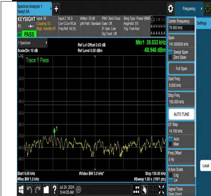
NTNV-N66-PC3-15-40-M-DFT-PI2BPSK-Edge_1RB_Left-0.009-0.15-Ant1-PASS
