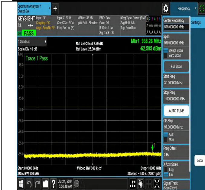
NTNV-N66-PC3-15-40-H-DFT-PI2BPSK-Edge_1RB_Right-30-1000-Ant1-PASS
