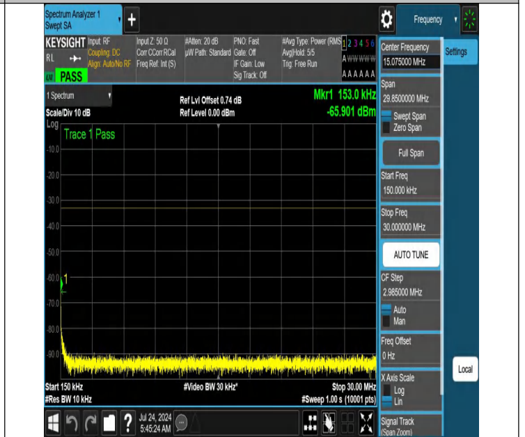
NTNV-N66-PC3-15-40-M-DFT-PI2BPSK-Edge_1RB_Right-0.15-3 0-Ant1-PASS
