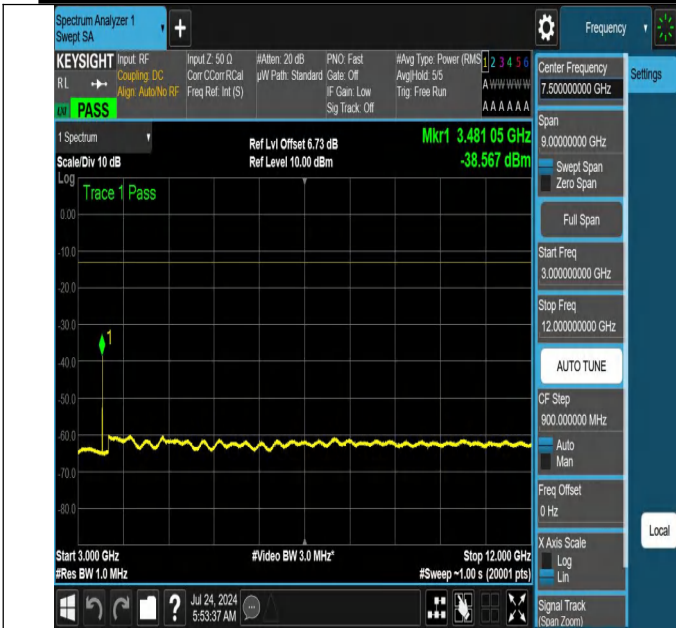
NTNV-N66-PC3-15-40-H-DFT-QPSK-Edge_1RB_Left-3000-1200 0-Ant1-PASS
