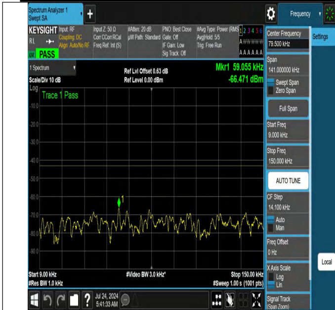
NTNV-N66-PC3-15-40-L-DFT-QPSK-Edge_1RB_Left-0.009-0.15-Ant1-PASS
