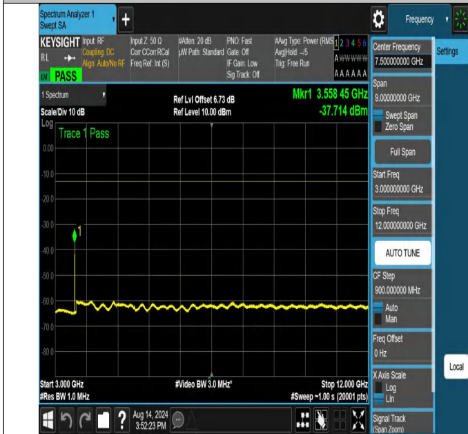
NTNV-N66-PC3-15-30-H-DFT-QPSK-Edge_1RB_Right-3000-1200-00-Ant1-PASS
