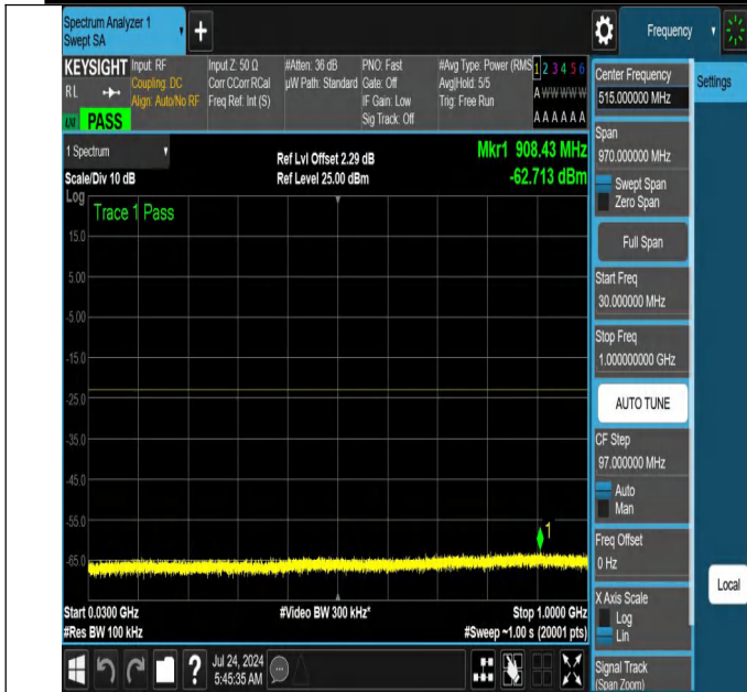
NTNV-N66-PC3-15-40-M-DFT-PI2BPSK-Edge_1RB_Right-30-1000-Ant1-PASS
