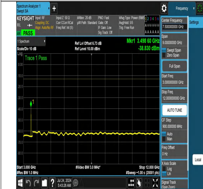
NTNV-N66-PC3-15-40-L-DFT-QPSK-Edge_1RB_Right-3000-12000-Ant1-PASS
