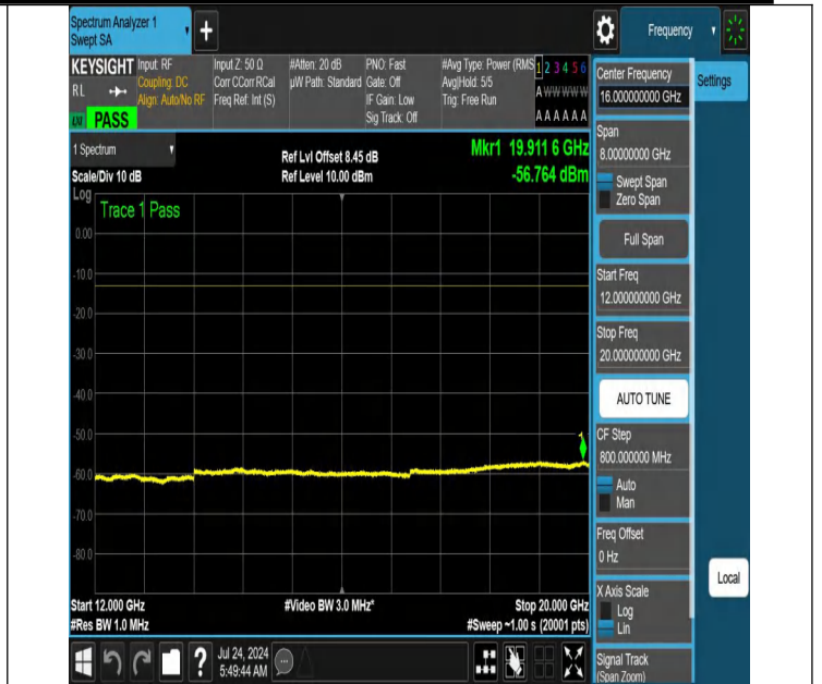
NTNV-N66-PC3-15-40-H-DFT-PI2BPSK-Edge_1RB_Left-12000-2 0000-Ant1-PASS
