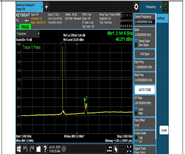
NTNV-N66-PC3-15-40-H-DFT-QPSK-Edge_1RB_Left-1000-3000- Ant1-PASS
