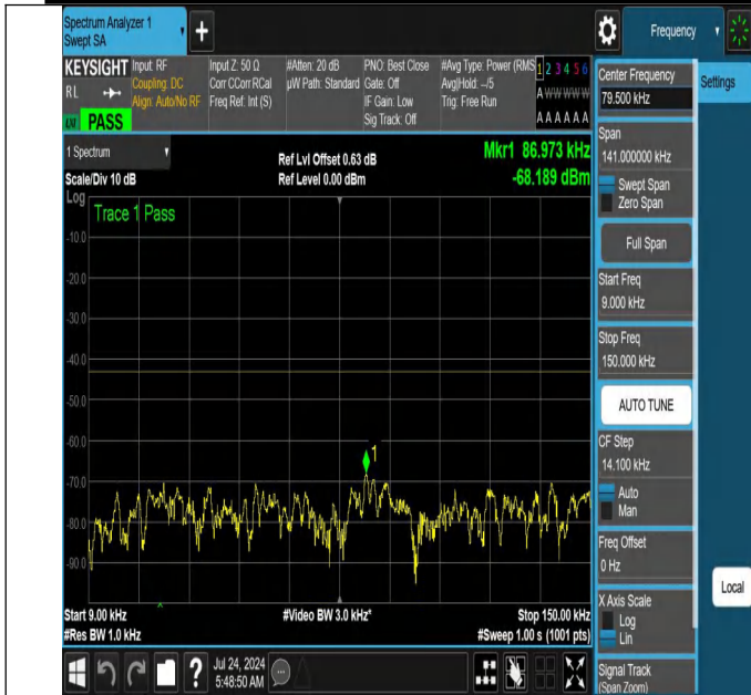
NTNV-N66-PC3-15-40-H-DFT-PI2BPSK-Edge_1RB_Left-0.009-0.15-Ant1-PASS
