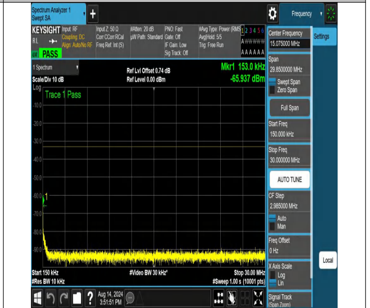
NTNV-N66-PC3-15-30-H-DFT-QPSK-Edge_1RB_Right-0.15-30-A nt1-PASS
