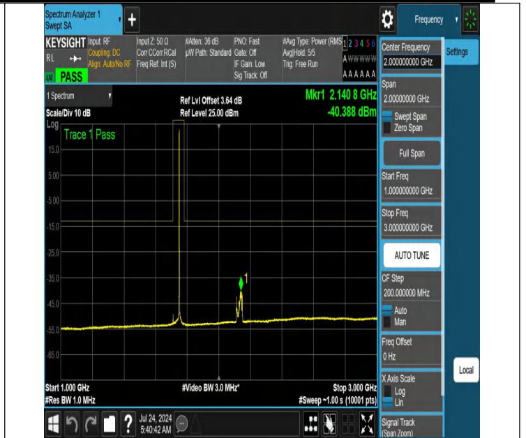
NTNV-N66-PC3-15-40-L-DFT-PI2BPSK-Edge_1RB_Right-1000-3000-Ant1-PASS
