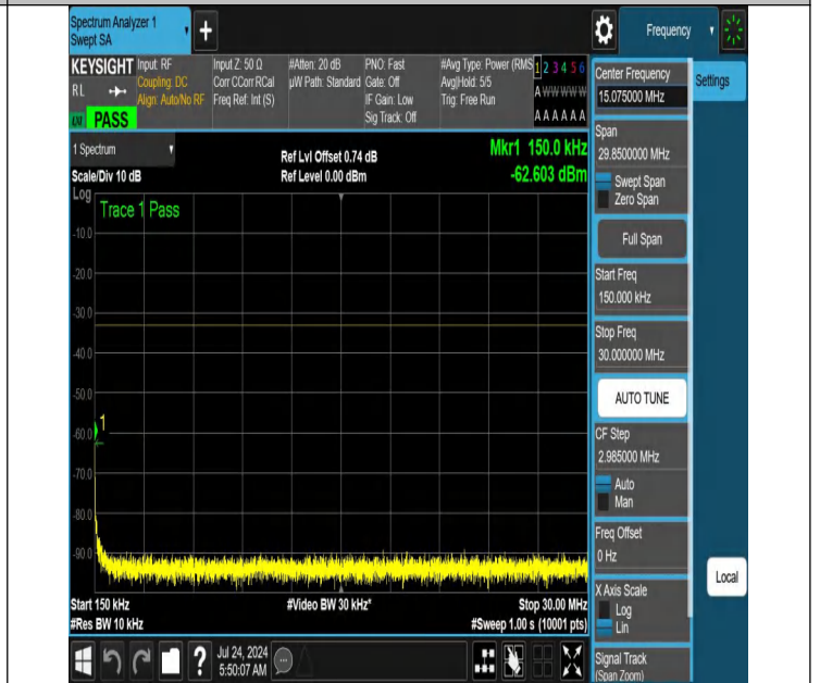
NTNV-N66-PC3-15-40-H-DFT-PI2BPSK-Edge_1RB_Right-0.15-3 0-Ant1-PASS
