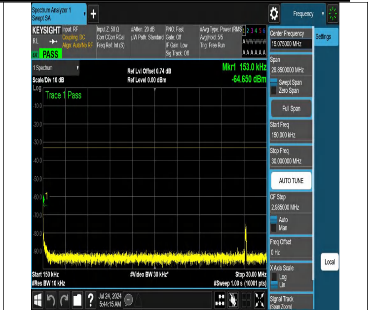
NTNV-N66-PC3-15-40-M-DFT-PI2BPSK-Edge_1RB_Left-0.15-30-Ant1-PASS
