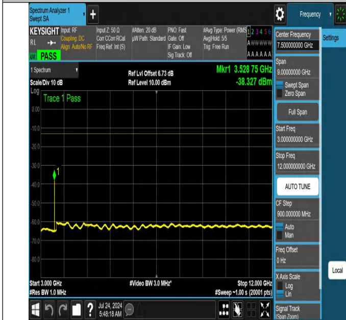
NTNV-N66-PC3-15-40-M-DFT-QPSK-Edge_1RB_Right-3000-12000-Ant1-PASS
