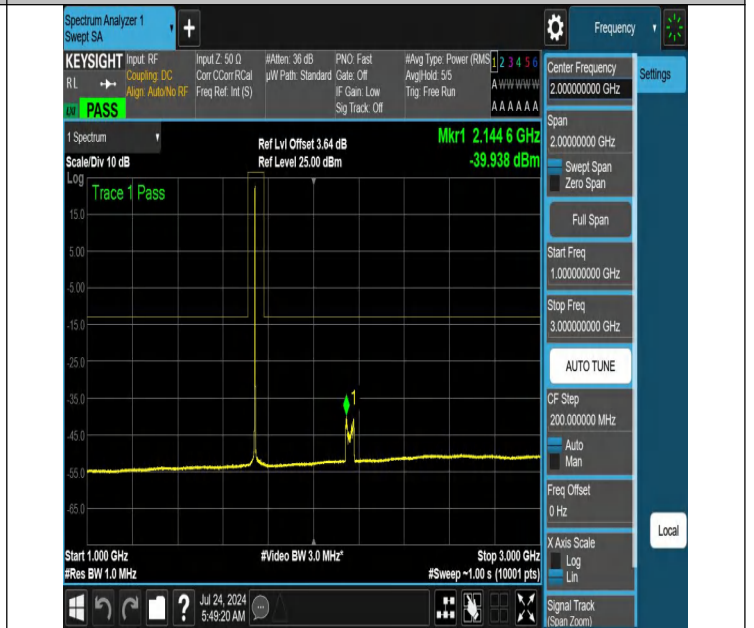
NTNV-N66-PC3-15-40-H-DFT-PI2BPSK-Edge_1RB_Left-1000-3000-Ant1-PASS
