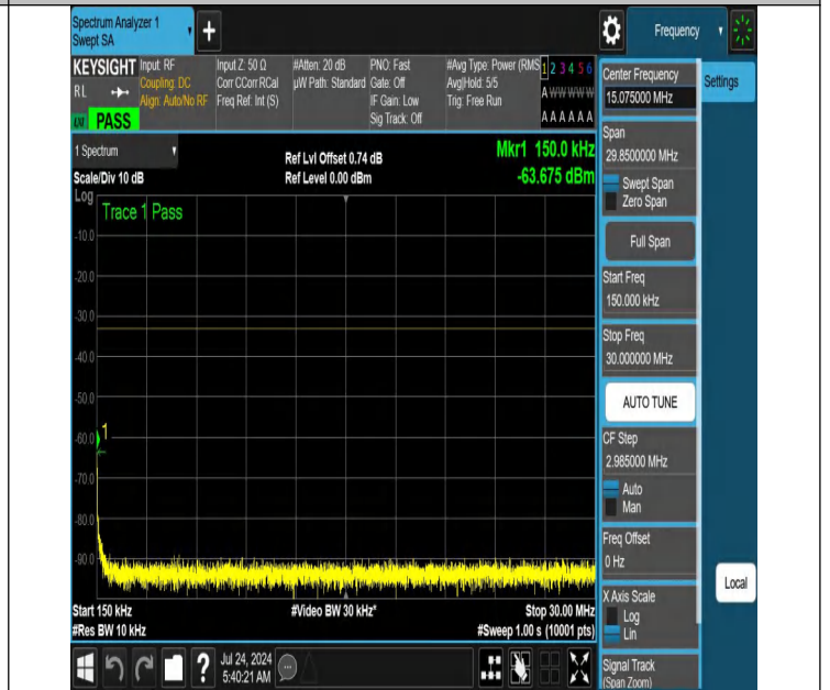
NTNV-N66-PC3-15-40-L-DFT-PI2BPSK-Edge_1RB_Right-0.15-30-Ant1-PASS
