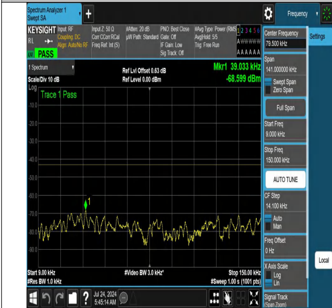
NTNV-N66-PC3-15-40-M-DFT-PI2BPSK-Edge_1RB_Right-0.009 -0.15-Ant1-PASS
