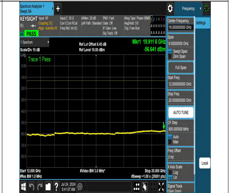
NTNV-N66-PC3-15-40-L-DFT-PI2BPSK-Edge_1RB_Right-12000-20000-Ant1-PASS
