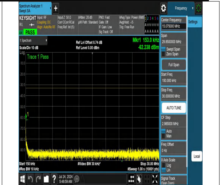
NTNV-N66-PC3-15-40-H-DFT-PI2BPSK-Edge_1RB_Left-0.15-30-Ant1-PASS
