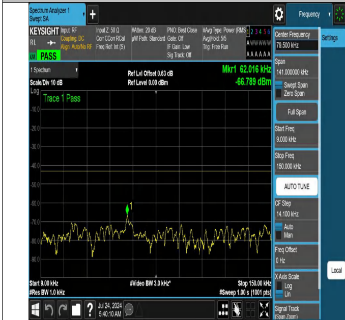
NTNV-N66-PC3-15-40-L-DFT-PI2BPSK-Edge_1RB_Right-0.009-0.15-Ant1-PASS
