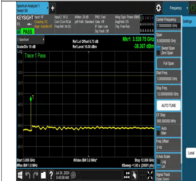
NTNV-N66-PC3-15-40-M-DFT-PI2BPSK-Edge_1RB_Right-3000-12000-Ant1-PASS
