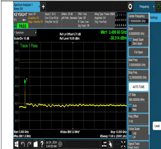
NTNV-N66-PC3-15-40-L-DFT-PI2BPSK-Edge_1RB_Right-3000-12000-Ant1-PASS
