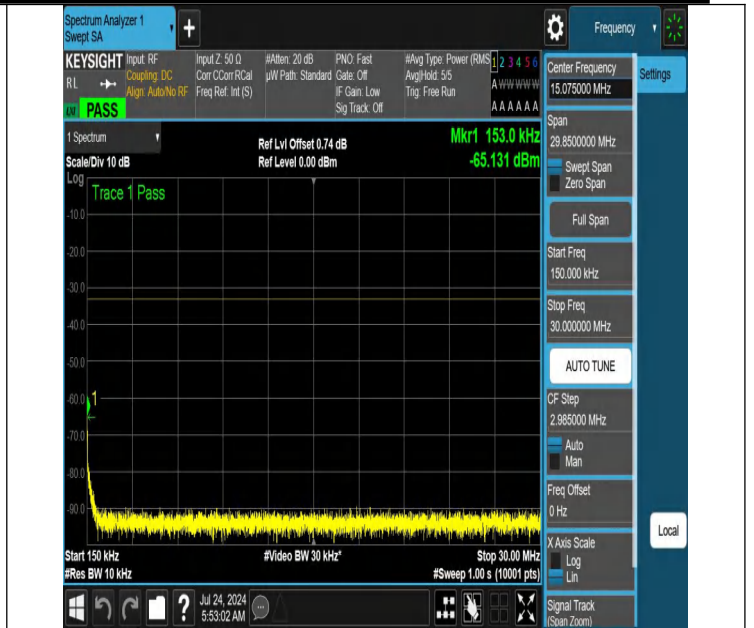
NTNV-N66-PC3-15-40-H-DFT-QPSK-Edge_1RB_Left-0.15-30-Ant 1-PASS
