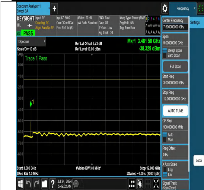
NTNV-N66-PC3-15-40-H-DFT-PI2BPSK-Edge_1RB_Left-3000-1 2000-Ant1-PASS
