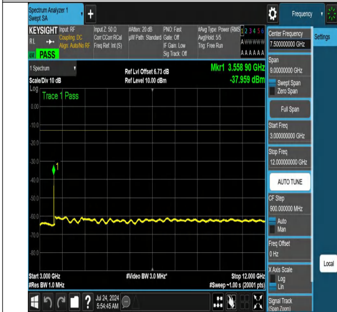
NTNV-N66-PC3-15-40-H-DFT-QPSK-Edge_1RB_Right-3000-12000-Ant1-PASS
