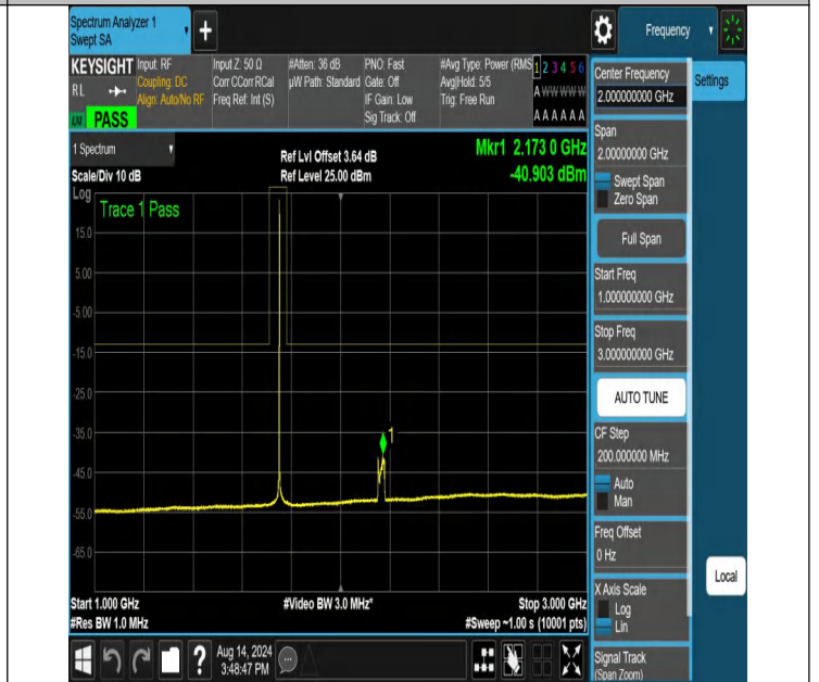
NTNV-N66-PC3-15-30-H-DFT-PI2BPSK-Edge_1RB_Left-1000-3000-Ant1-PASS
