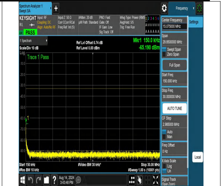
NTNV-N66-PC3-15-30-M-DFT-PI2BPSK-Edge_1RB_Left-0.15-30-Ant1-PASS
