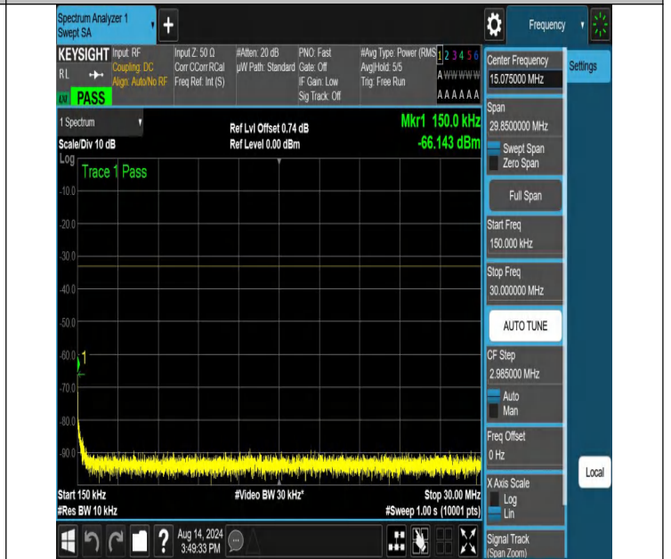
NTNV-N66-PC3-15-30-H-DFT-PI2BPSK-Edge_1RB_Right-0.15-3 0-Ant1-PASS
