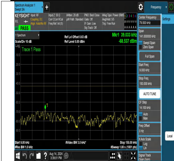
NTNV-N66-PC3-15-30-L-DFT-PI2BPSK-Edge_1RB_Left-0.009-0.15-Ant1-PASS
