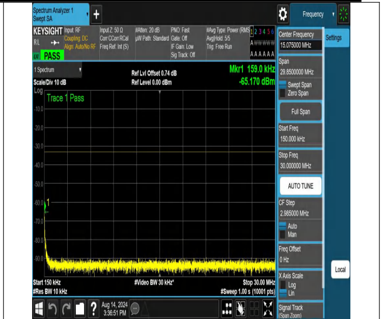
NTNV-N66-PC3-15-25-H-DFT-QPSK-Edge_1RB_Left-0.15-30-Ant 1-PASS
