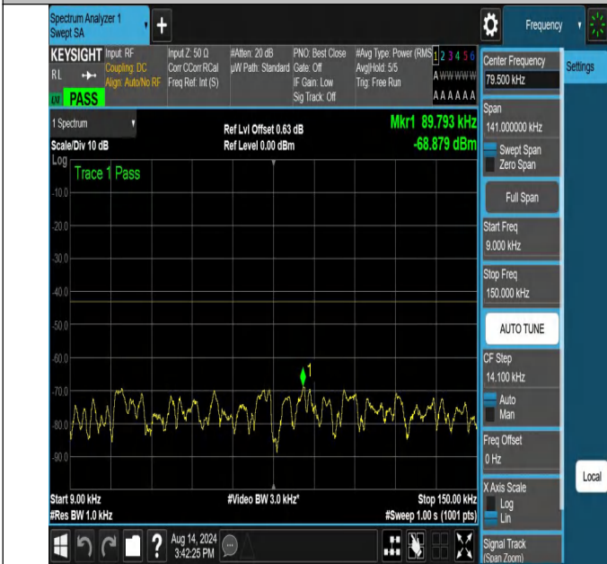
NTNV-N66-PC3-15-30-L-DFT-QPSK-Edge_1RB_Right-0.009-0.1 5-Ant1-PASS
