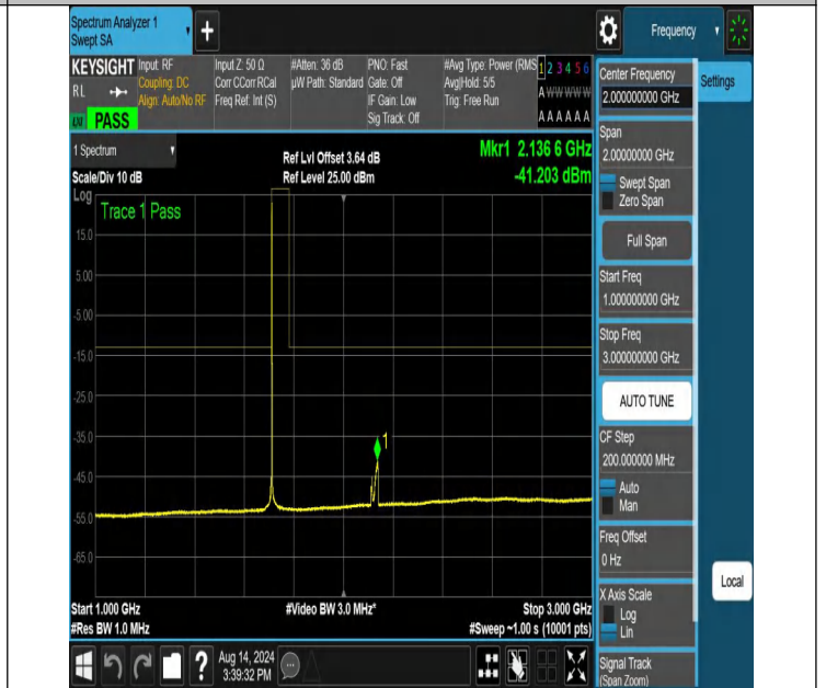
NTNV-N66-PC3-15-30-L-DFT-PI2BPSK-Edge_1RB_Left-1000-3000-Ant1-PASS
