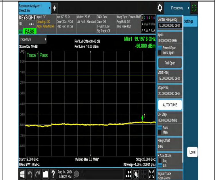
NTNV-N66-PC3-15-25-H-DFT-PI2BPSK-Edge_1RB_Right-12000-20000-Ant1-PASS
