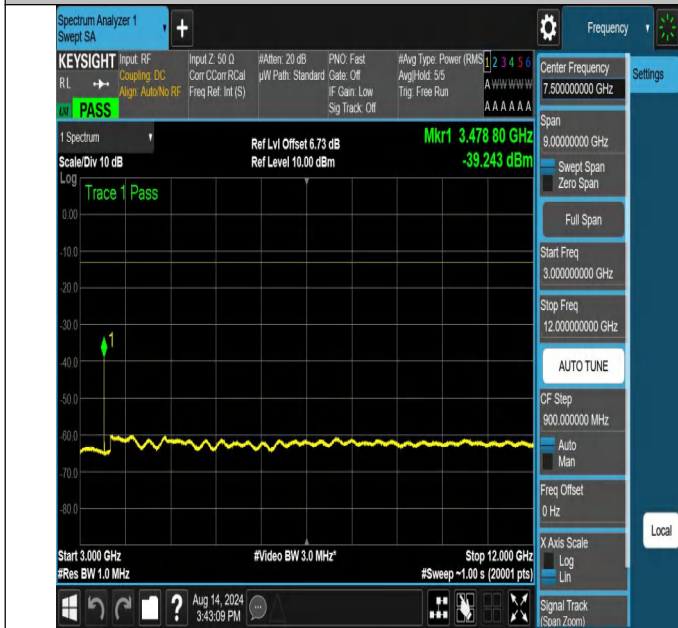
NTNV-N66-PC3-15-30-L-DFT-QPSK-Edge_1RB_Right-3000-12000-Ant1-PASS
