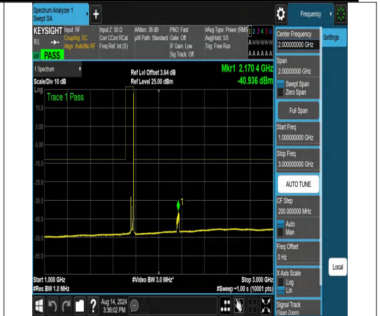
NTNV-N66-PC3-15-25-H-DFT-PI2BPSK-Edge_1RB_Right-1000-3000-Ant1-PASS
