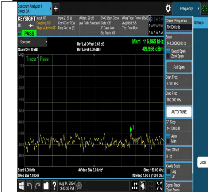
NTNV-N66-PC3-15-30-M-DFT-PI2BPSK-Edge_1RB_Left-0.009-0.15-Ant1-PASS
