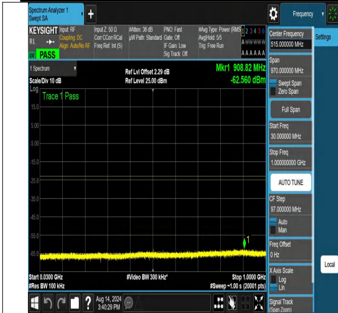
NTNV-N66-PC3-15-30-L-DFT-PI2BPSK-Edge_1RB_Right-30-1000-Ant1-PASS
