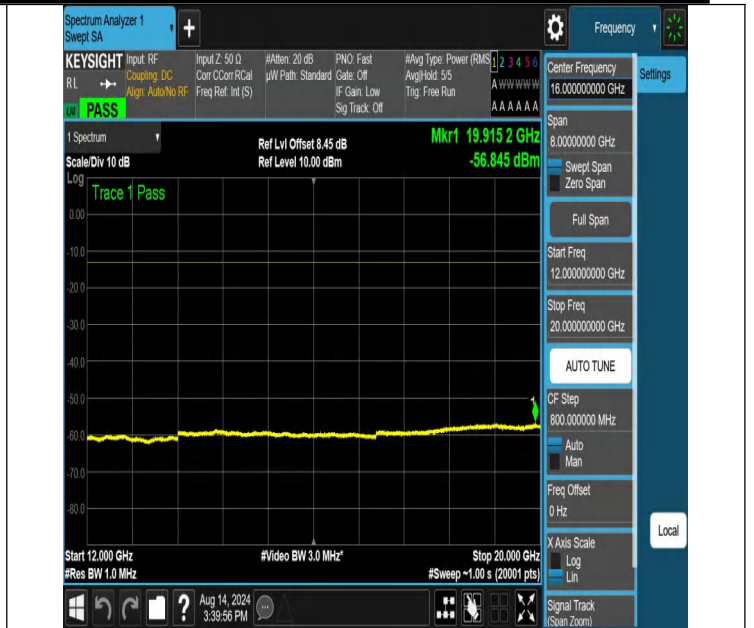
NTNV-N66-PC3-15-30-L-DFT-PI2BPSK-Edge_1RB_Left-12000-20000-Ant1-PASS
