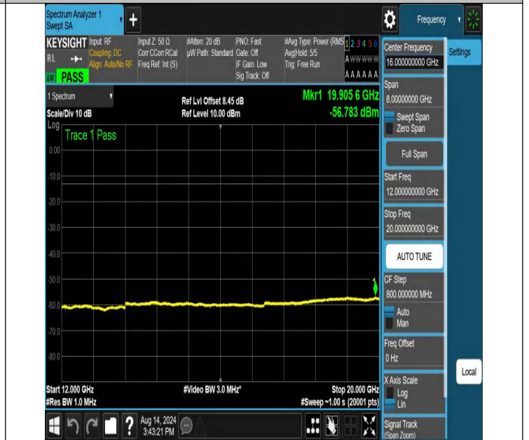
NTNV-N66-PC3-15-30-L-DFT-QPSK-Edge_1RB_Right-12000-20000-Ant1-PASS
