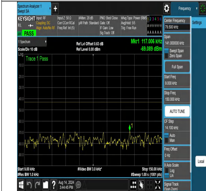
NTNV-N66-PC3-15-30-M-DFT-PI2BPSK-Edge_1RB_Right-0.009 -0.15-Ant1-PASS
