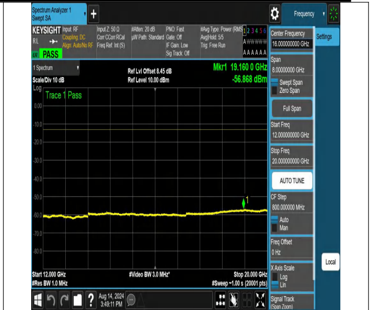
NTNV-N66-PC3-15-30-H-DFT-PI2BPSK-Edge_1RB_Left-12000-2 0000-Ant1-PASS
