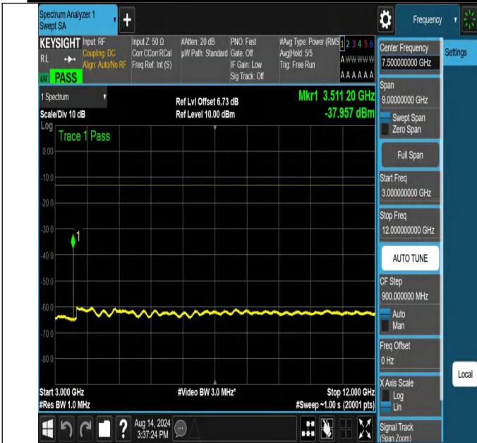
NTNV-N66-PC3-15-25-H-DFT-QPSK-Edge_1RB_Left-3000-1200 0-Ant1-PASS
