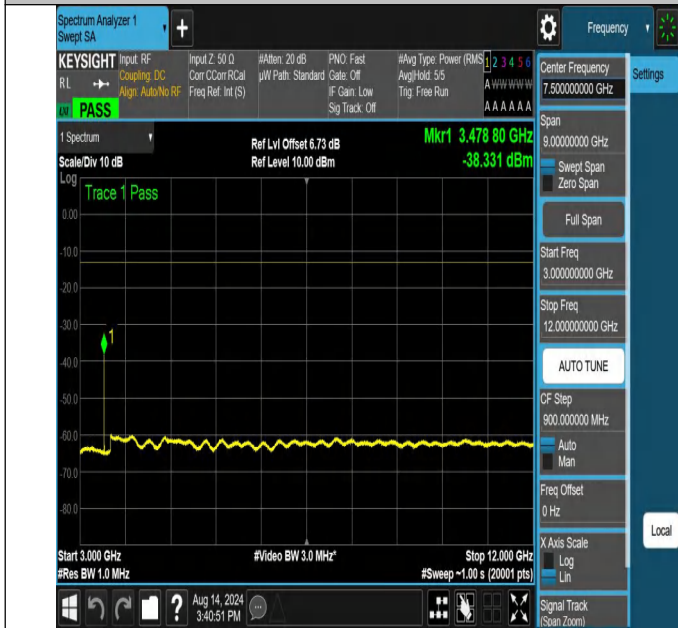
NTNV-N66-PC3-15-30-L-DFT-PI2BPSK-Edge_1RB_Right-3000-12000-Ant1-PASS
