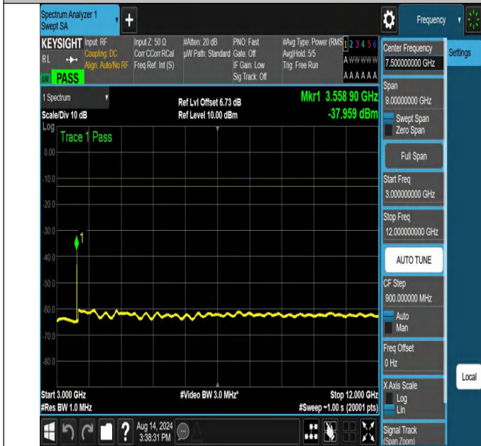
NTNV-N66-PC3-15-25-H-DFT-QPSK-Edge_1RB_Right-3000-12000-Ant1-PASS
