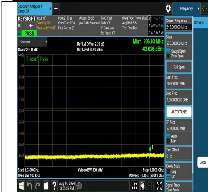
NTNV-N66-PC3-15-25-H-DFT-PI2BPSK-Edge_1RB_Right-30-1000-Ant1-PASS
