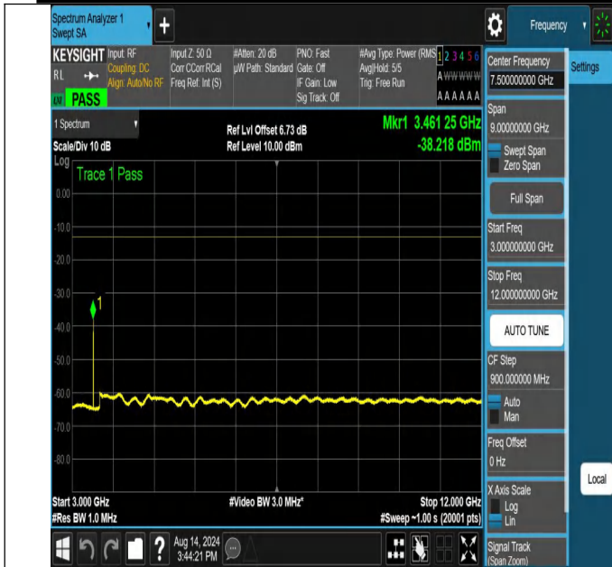
NTNV-N66-PC3-15-30-M-DFT-PI2BPSK-Edge_1RB_Left-3000-1 2000-Ant1-PASS
