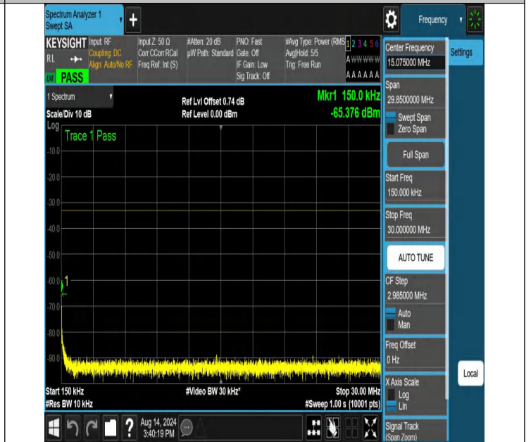
NTNV-N66-PC3-15-30-L-DFT-PI2BPSK-Edge_1RB_Right-0.15-30-Ant1-PASS
