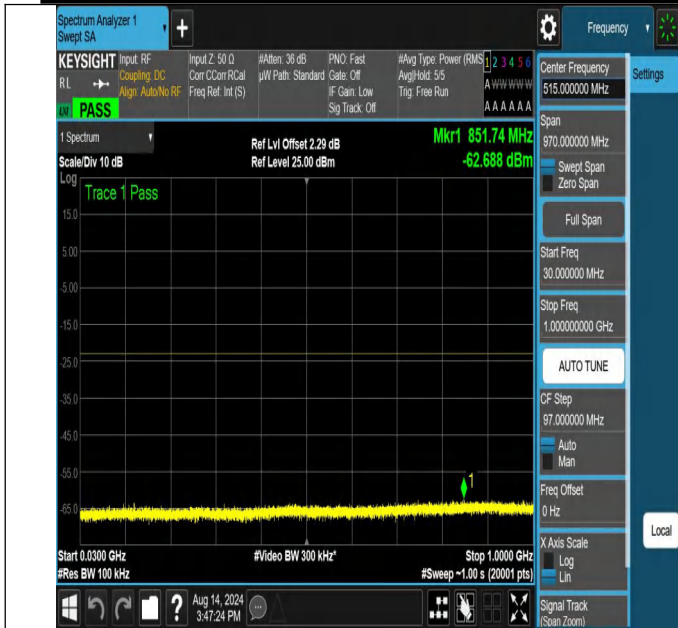
NTNV-N66-PC3-15-30-M-DFT-QPSK-Edge_1RB_Right-30-1000-Ant1-PASS
