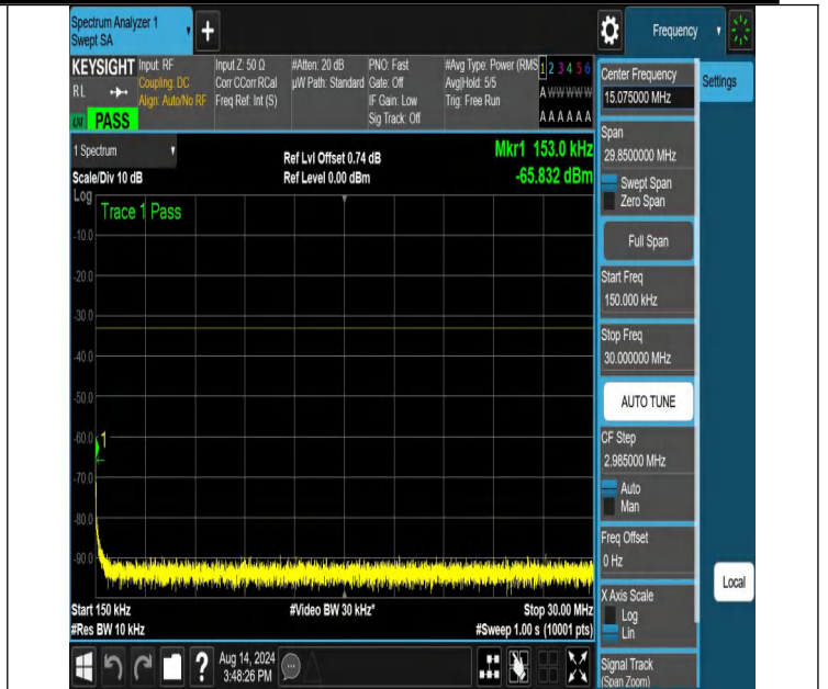
NTNV-N66-PC3-15-30-H-DFT-PI2BPSK-Edge_1RB_Left-0.15-30-Ant1-PASS
