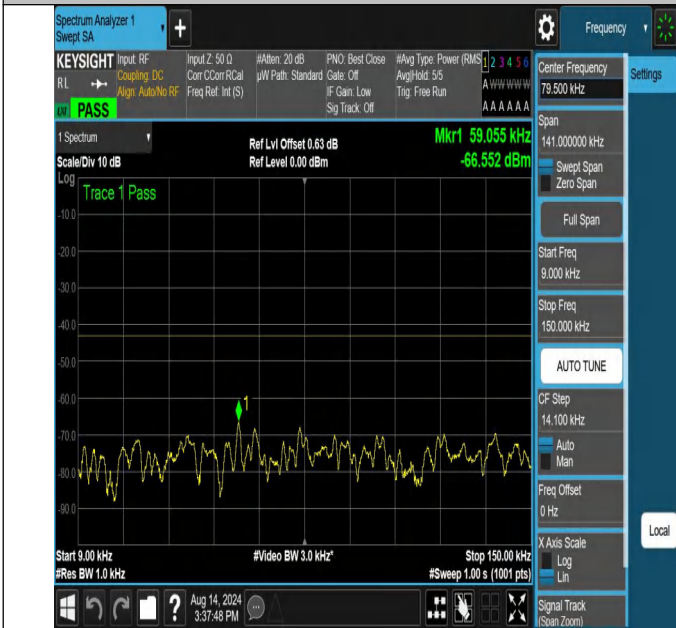
NTNV-N66-PC3-15-25-H-DFT-QPSK-Edge_1RB_Right-0.009-0.1 5-Ant1-PASS
