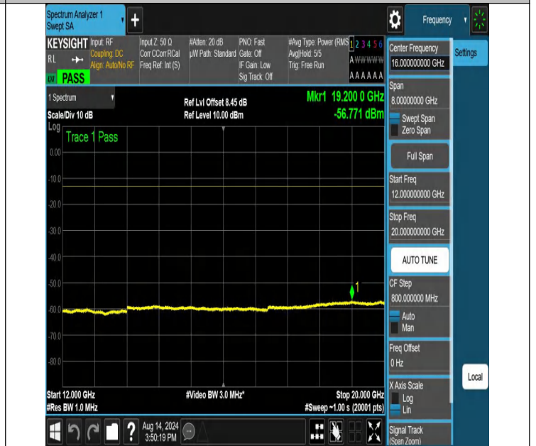
NTNV-N66-PC3-15-30-H-DFT-PI2BPSK-Edge_1RB_Right-12000-20000-Ant1-PASS
