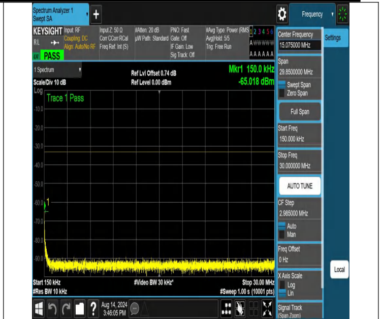
NTNV-N66-PC3-15-30-M-DFT-QPSK-Edge_1RB_Left-0.15-30-Ant 1-PASS
