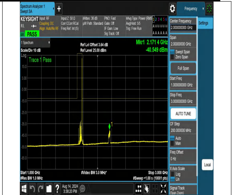
NTNV-N66-PC3-15-25-H-DFT-QPSK-Edge_1RB_Right-1000-300-0-Ant1-PASS
