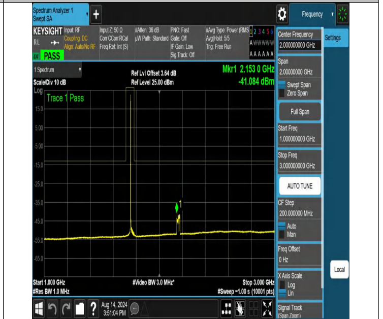
NTNV-N66-PC3-15-30-H-DFT-QPSK-Edge_1RB_Left-1000-3000-Ant1-PASS
