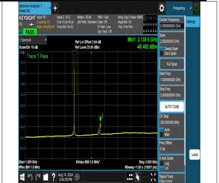
NTNV-N66-PC3-15-30-L-DFT-PI2BPSK-Edge_1RB_Right-1000-3000-Ant1-PASS
