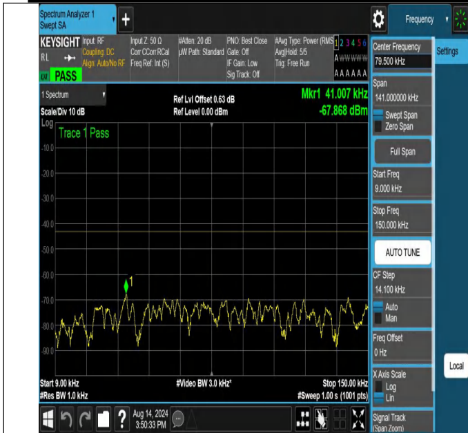
NTNV-N66-PC3-15-30-H-DFT-QPSK-Edge_1RB_Left-0.009-0.15 -Ant1-PASS
