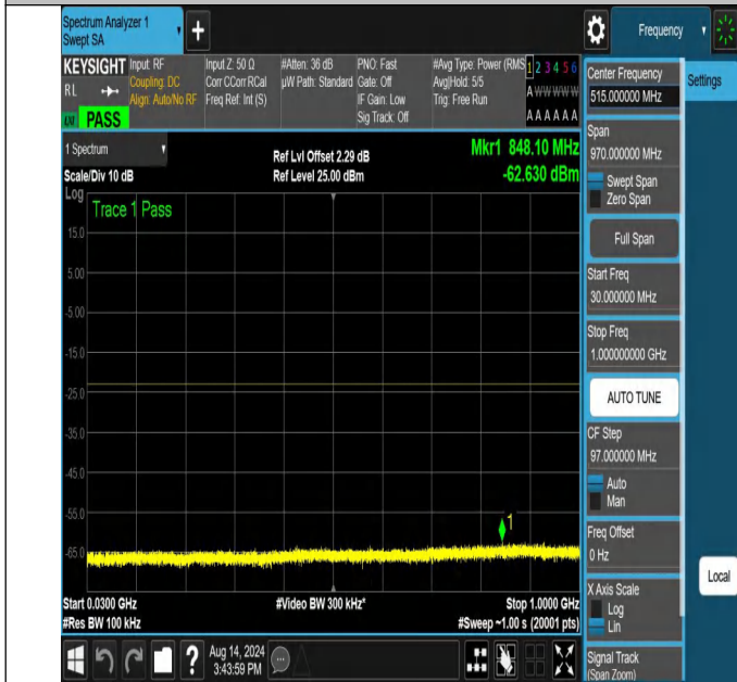
NTNV-N66-PC3-15-30-M-DFT-PI2BPSK-Edge_1RB_Left-30-1000-Ant1-PASS
