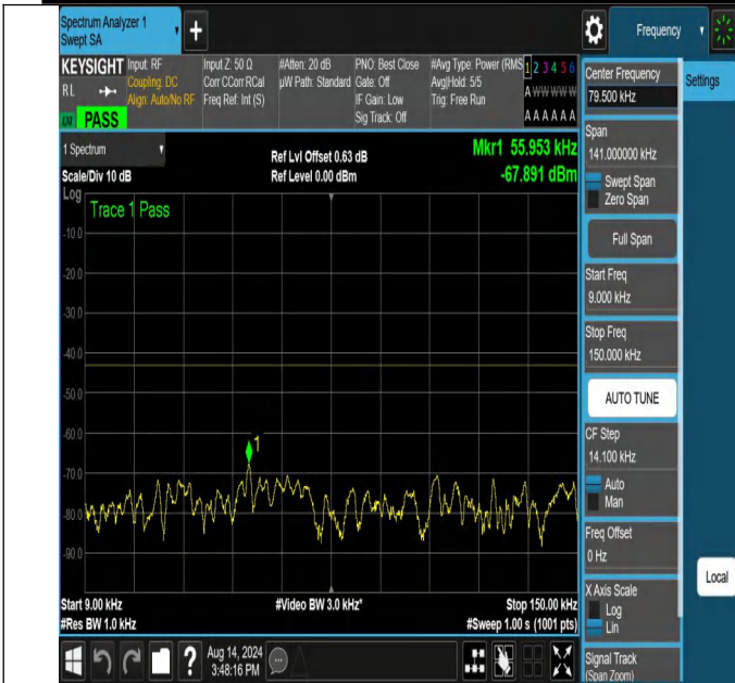
NTNV-N66-PC3-15-30-H-DFT-PI2BPSK-Edge_1RB_Left-0.009-0.15-Ant1-PASS
