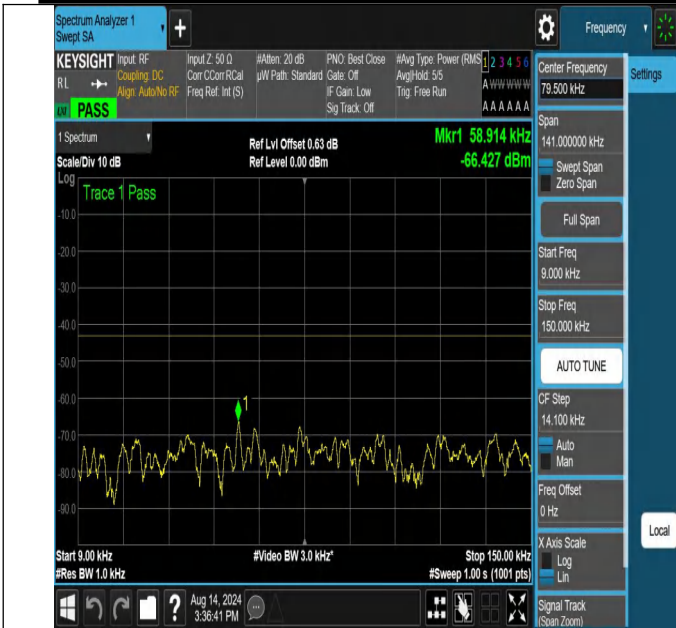
NTNV-N66-PC3-15-25-H-DFT-QPSK-Edge_1RB_Left-0.009-0.15 -Ant1-PASS
