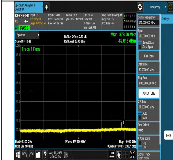
NTNV-N66-PC3-15-30-L-DFT-PI2BPSK-Edge_1RB_Left-30-1000-Ant1-PASS
