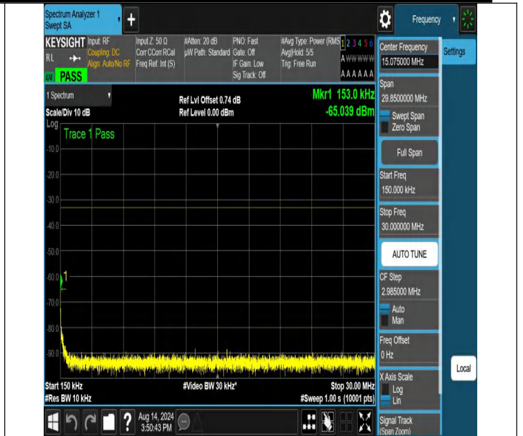
NTNV-N66-PC3-15-30-H-DFT-QPSK-Edge_1RB_Left-0.15-30-Ant 1-PASS
