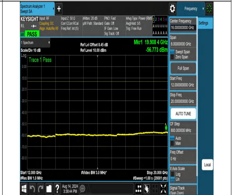
NTNV-N66-PC3-15-25-H-DFT-QPSK-Edge_1RB_Right-12000-20000-Ant1-PASS
