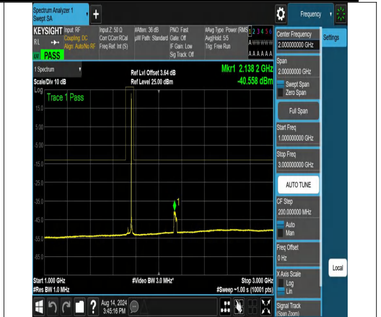
NTNV-N66-PC3-15-30-M-DFT-PI2BPSK-Edge_1RB_Right-1000-3000-Ant1-PASS
