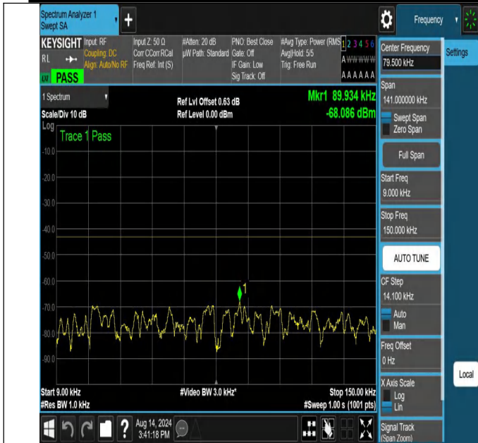
NTNV-N66-PC3-15-30-L-DFT-QPSK-Edge_1RB_Left-0.009-0.15-Ant1-PASS
