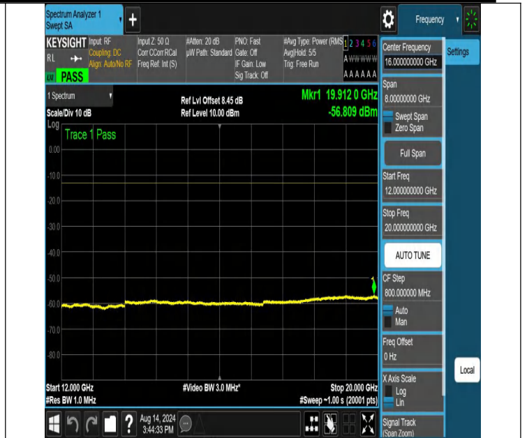
NTNV-N66-PC3-15-30-M-DFT-PI2BPSK-Edge_1RB_Left-12000-2 0000-Ant1-PASS
