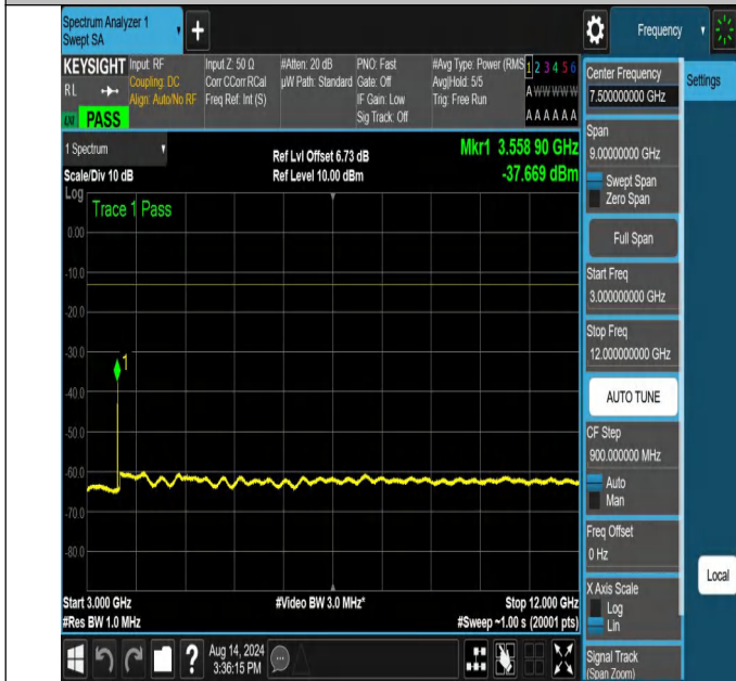
NTNV-N66-PC3-15-25-H-DFT-PI2BPSK-Edge_1RB_Right-3000-12000-Ant1-PASS
