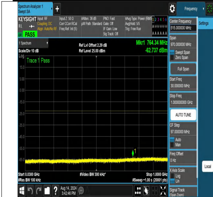
NTNV-N66-PC3-15-30-L-DFT-QPSK-Edge_1RB_Right-30-1000-Ant1-PASS
