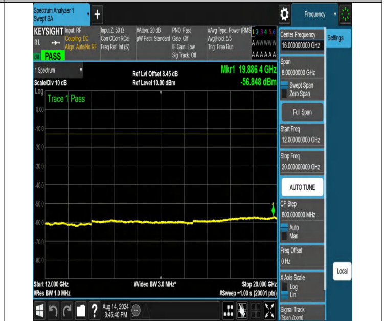
NTNV-N66-PC3-15-30-M-DFT-PI2BPSK-Edge_1RB_Right-12000-20000-Ant1-PASS
