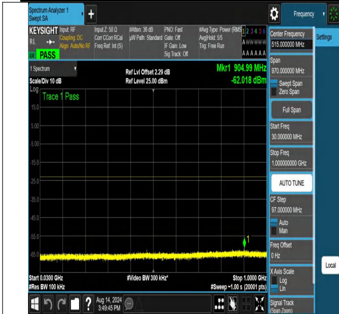
NTNV-N66-PC3-15-30-H-DFT-PI2BPSK-Edge_1RB_Right-30-1000-Ant1-PASS
