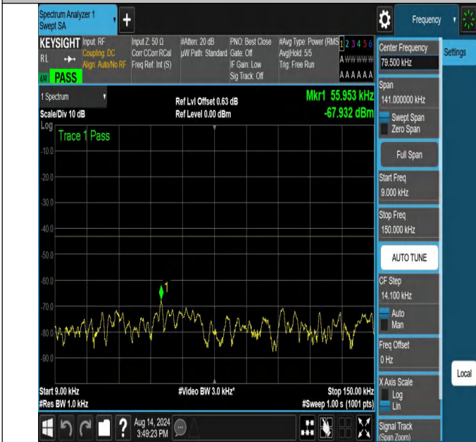
NTNV-N66-PC3-15-30-H-DFT-PI2BPSK-Edge_1RB_Right-0.009- 0.15-Ant1-PASS
