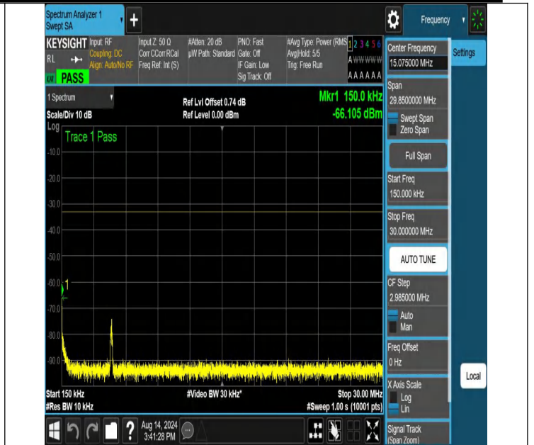
NTNV-N66-PC3-15-30-L-DFT-QPSK-Edge_1RB_Left-0.15-30-Ant 1-PASS
