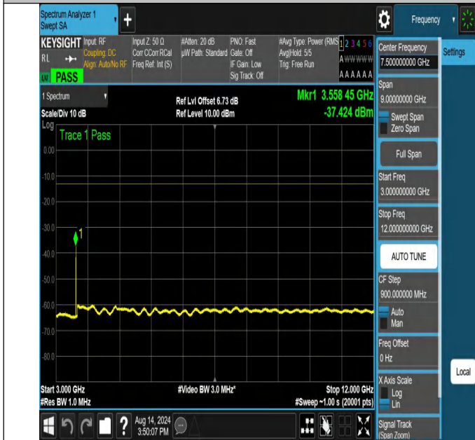
NTNV-N66-PC3-15-30-H-DFT-PI2BPSK-Edge_1RB_Right-3000-12000-Ant1-PASS
