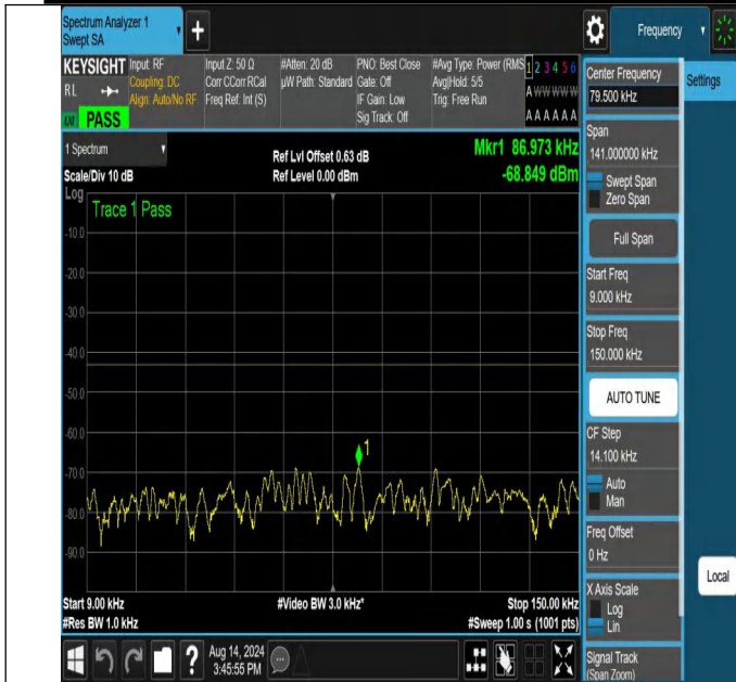
NTNV-N66-PC3-15-30-M-DFT-QPSK-Edge_1RB_Left-0.009-0.15 -Ant1-PASS
