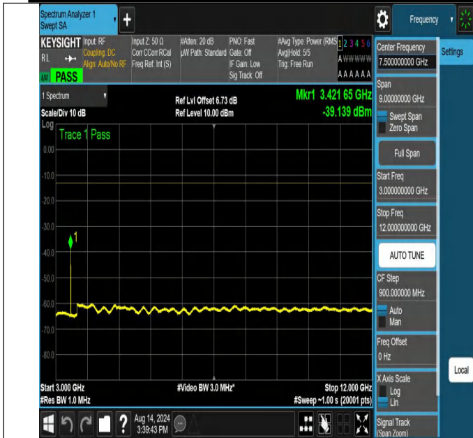
NTNV-N66-PC3-15-30-L-DFT-PI2BPSK-Edge_1RB_Left-3000-12000-Ant1-PASS
