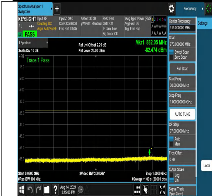
NTNV-N66-PC3-15-30-M-DFT-PI2BPSK-Edge_1RB_Right-30-1000-Ant1-PASS
