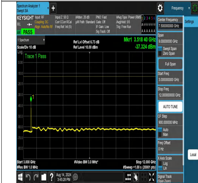
NTNV-N66-PC3-15-30-M-DFT-PI2BPSK-Edge_1RB_Right-3000-12000-Ant1-PASS
