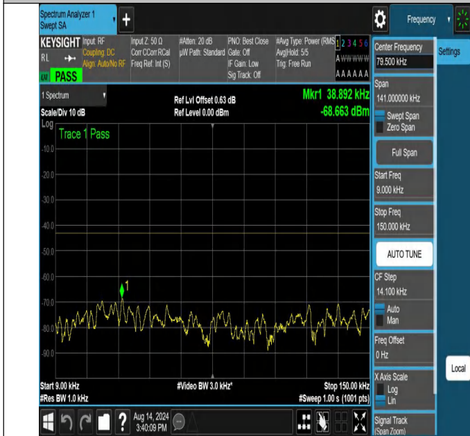
NTNV-N66-PC3-15-30-L-DFT-PI2BPSK-Edge_1RB_Right-0.009-0.15-Ant1-PASS
