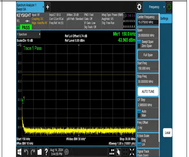
NTNV-N66-PC3-15-30-M-DFT-PI2BPSK-Edge_1RB_Right-0.15-3 0-Ant1-PASS
