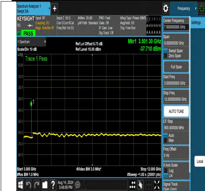
NTNV-N66-PC3-15-30-H-DFT-PI2BPSK-Edge_1RB_Left-3000-1 2000-Ant1-PASS
