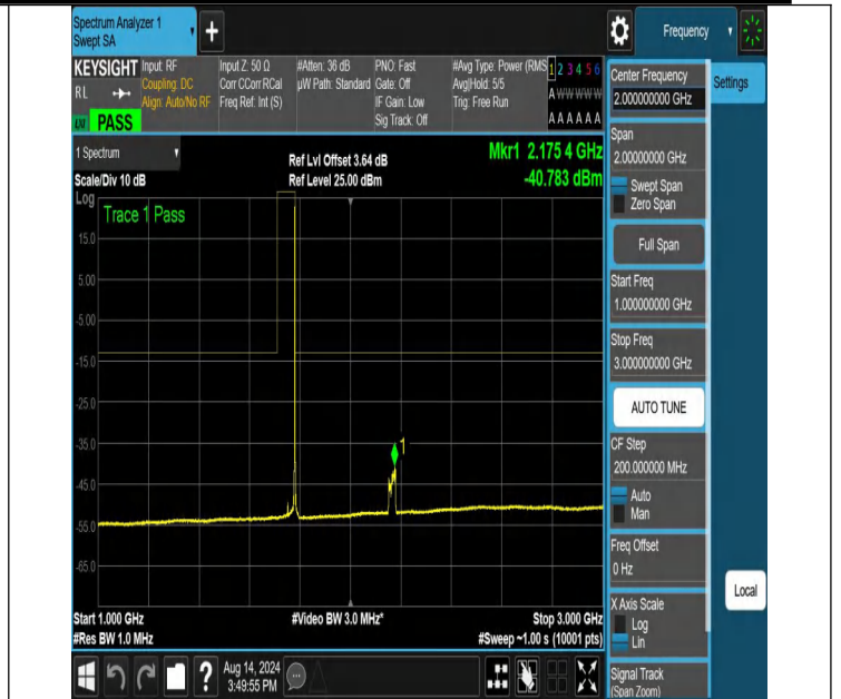
NTNV-N66-PC3-15-30-H-DFT-PI2BPSK-Edge_1RB_Right-1000-3000-Ant1-PASS
