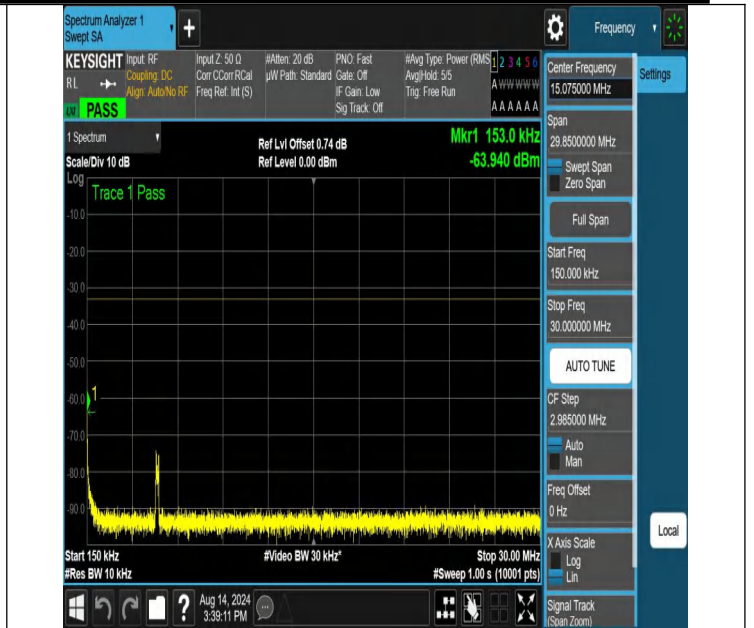
NTNV-N66-PC3-15-30-L-DFT-PI2BPSK-Edge_1RB_Left-0.15-30-Ant1-PASS
