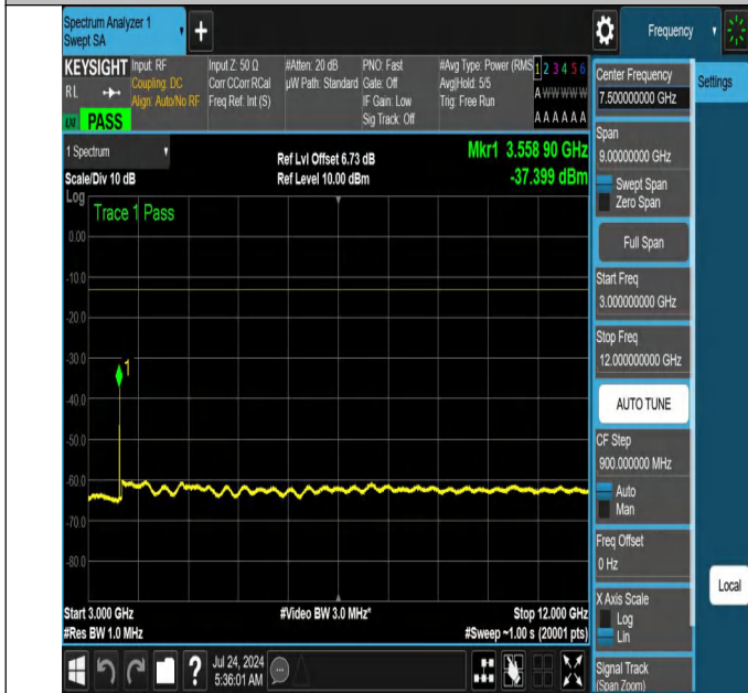
NTNV-N66-PC3-15-20-H-DFT-PI2BPSK-Edge_1RB_Right-3000-12000-Ant1-PASS
