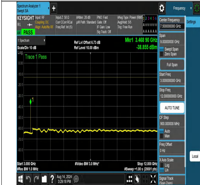
NTNV-N66-PC3-15-25-L-DFT-QPSK-Edge_1RB_Right-3000-12000-Ant1-PASS
