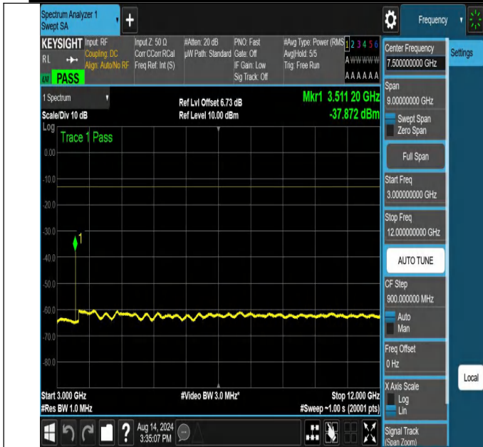
NTNV-N66-PC3-15-25-H-DFT-PI2BPSK-Edge_1RB_Left-3000-1 2000-Ant1-PASS
