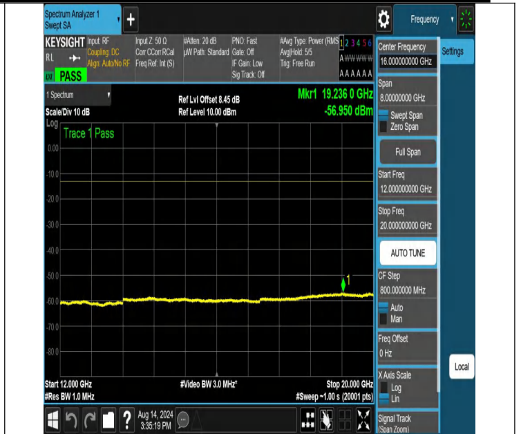
NTNV-N66-PC3-15-25-H-DFT-PI2BPSK-Edge_1RB_Left-12000-2 0000-Ant1-PASS
