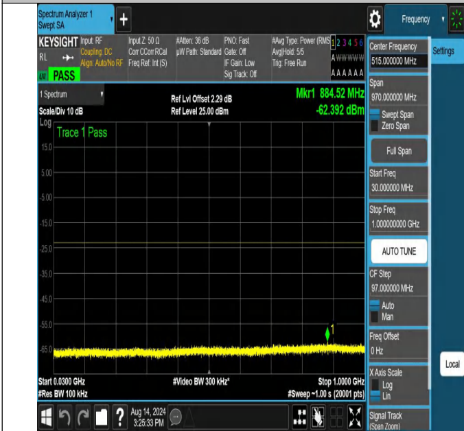
NTNV-N66-PC3-15-25-L-DFT-PI2BPSK-Edge_1RB_Left-30-1000-Ant1-PASS
