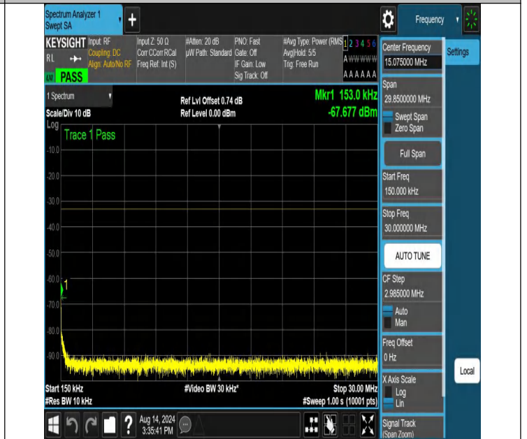
NTNV-N66-PC3-15-25-H-DFT-PI2BPSK-Edge_1RB_Right-0.15-3 0-Ant1-PASS
