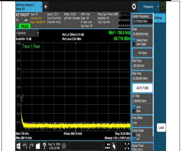
NTNV-N66-PC3-15-25-H-DFT-PI2BPSK-Edge_1RB_Left-0.15-30-Ant1-PASS
