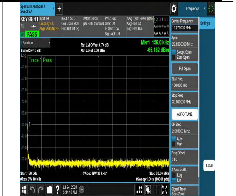
NTNV-N66-PC3-15-20-H-DFT-PI2BPSK-Edge_1RB_Left-0.15-30-Ant1-PASS
