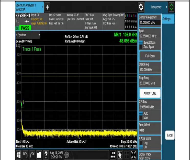
NTNV-N66-PC3-15-25-L-DFT-PI2BPSK-Edge_1RB_Right-0.15-30-Ant1-PASS
