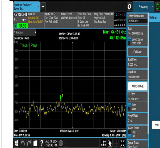
NTNV-N66-PC3-15-25-M-DFT-PI2BPSK-Edge_1RB_Left-0.009-0.15-Ant1-PASS
