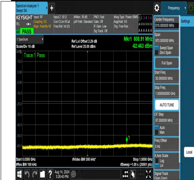
NTNV-N66-PC3-15-25-L-DFT-PI2BPSK-Edge_1RB_Right-30-1000-Ant1-PASS
