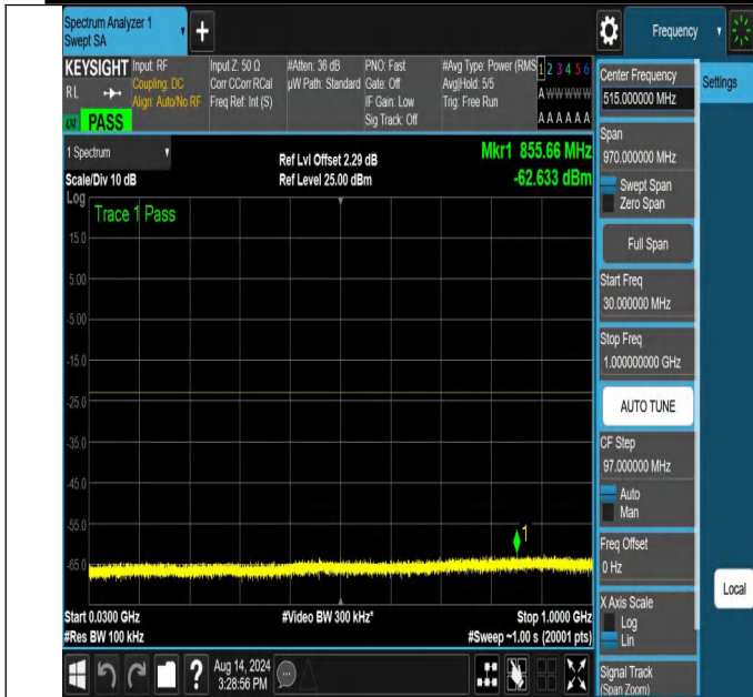
NTNV-N66-PC3-15-25-L-DFT-QPSK-Edge_1RB_Right-30-1000-Ant1-PASS
