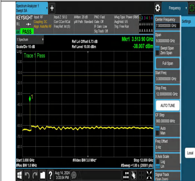
NTNV-N66-PC3-15-25-M-DFT-QPSK-Edge_1RB_Right-3000-12000-Ant1-PASS
