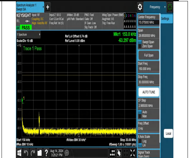
NTNV-N66-PC3-15-25-L-DFT-PI2BPSK-Edge_1RB_Left-0.15-30-Ant1-PASS
