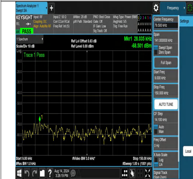
NTNV-N66-PC3-15-25-L-DFT-PI2BPSK-Edge_1RB_Right-0.009-0.15-Ant1-PASS
