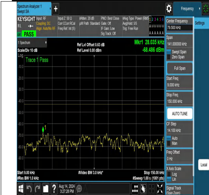
NTNV-N66-PC3-15-25-L-DFT-QPSK-Edge_1RB_Left-0.009-0.15-Ant1-PASS
