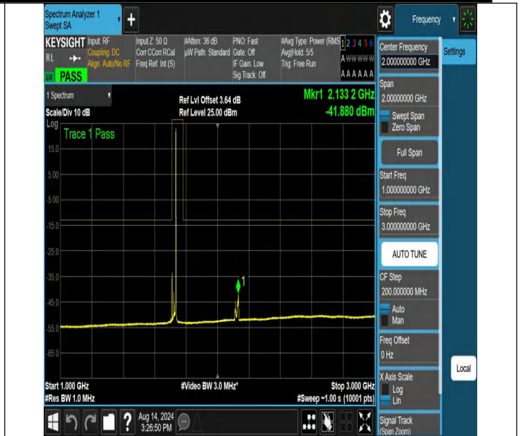
NTNV-N66-PC3-15-25-L-DFT-PI2BPSK-Edge_1RB_Right-1000-3000-Ant1-PASS
