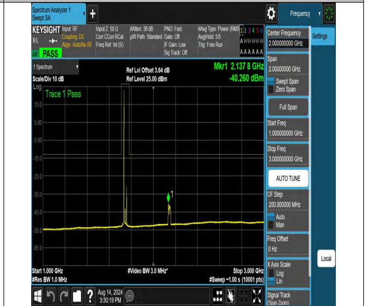
NTNV-N66-PC3-15-25-M-DFT-PI2BPSK-Edge_1RB_Left-1000-3000-Ant1-PASS
