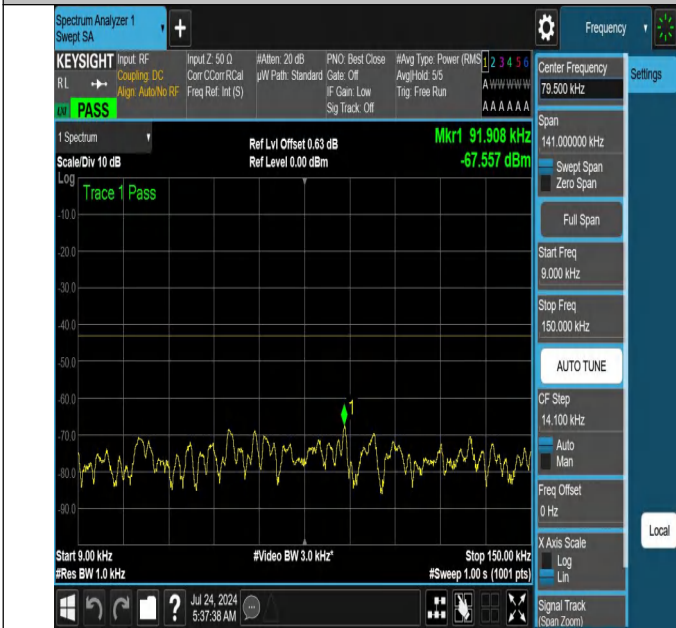
NTNV-N66-PC3-15-20-H-DFT-QPSK-Edge_1RB_Right-0.009-0.1 5-Ant1-PASS
