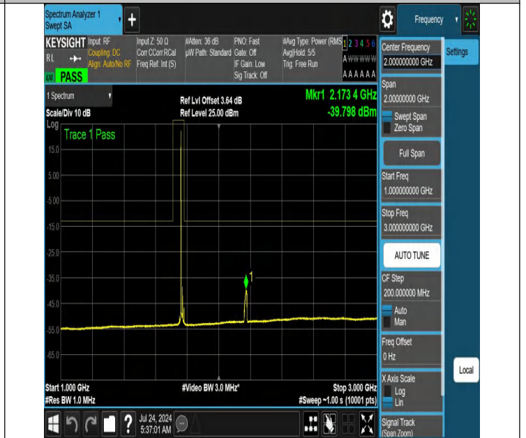
NTNV-N66-PC3-15-20-H-DFT-QPSK-Edge_1RB_Left-1000-3000- Ant1-PASS
