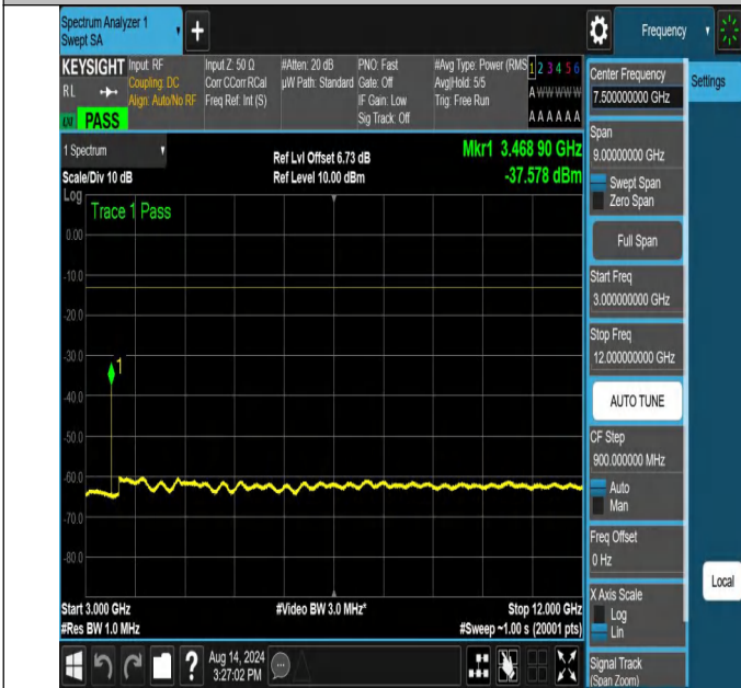
NTNV-N66-PC3-15-25-L-DFT-PI2BPSK-Edge_1RB_Right-3000-12000-Ant1-PASS
