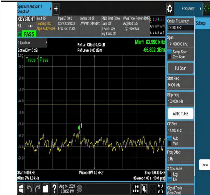
NTNV-N66-PC3-15-25-M-DFT-PI2BPSK-Edge_1RB_Right-0.009 -0.15-Ant1-PASS
