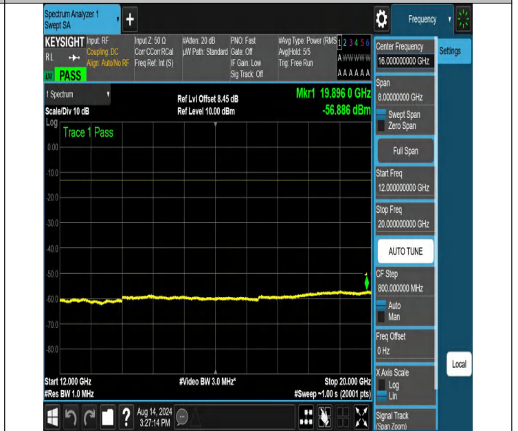
NTNV-N66-PC3-15-25-L-DFT-PI2BPSK-Edge_1RB_Right-12000-20000-Ant1-PASS
