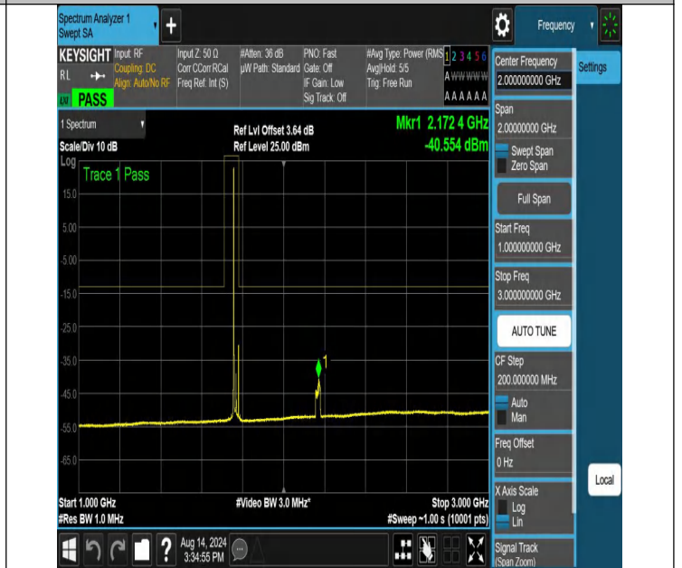
NTNV-N66-PC3-15-25-H-DFT-PI2BPSK-Edge_1RB_Left-1000-3000-Ant1-PASS
