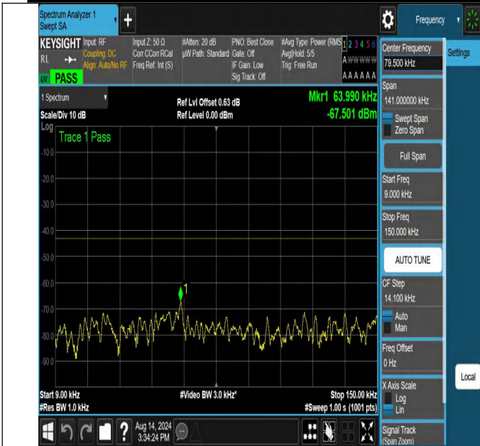
NTNV-N66-PC3-15-25-H-DFT-PI2BPSK-Edge_1RB_Left-0.009-0.15-Ant1-PASS
