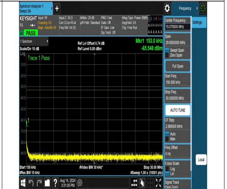
NTNV-N66-PC3-15-25-M-DFT-PI2BPSK-Edge_1RB_Right-0.15-3 0-Ant1-PASS
