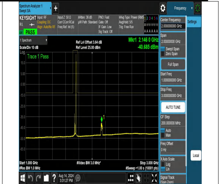
NTNV-N66-PC3-15-25-M-DFT-PI2BPSK-Edge_1RB_Right-1000-3000-Ant1-PASS
