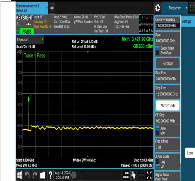
NTNV-N66-PC3-15-25-L-DFT-PI2BPSK-Edge_1RB_Left-3000-12000-Ant1-PASS
