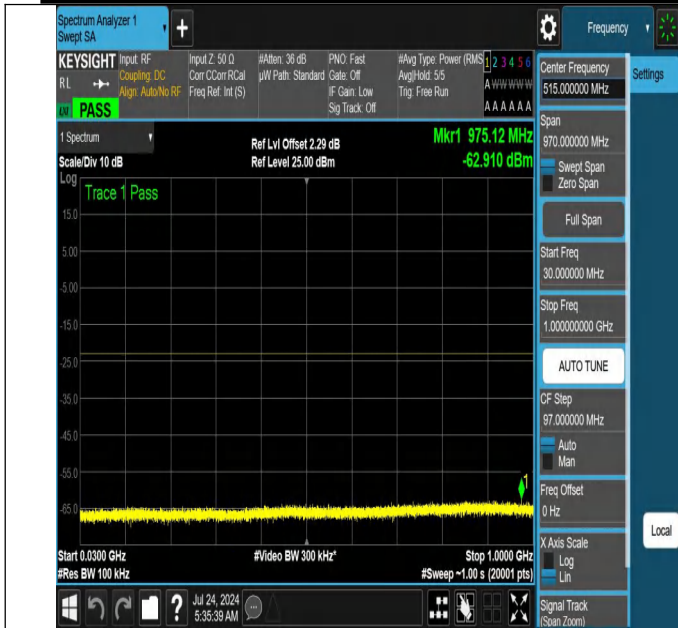
NTNV-N66-PC3-15-20-H-DFT-PI2BPSK-Edge_1RB_Right-30-1000-Ant1-PASS
