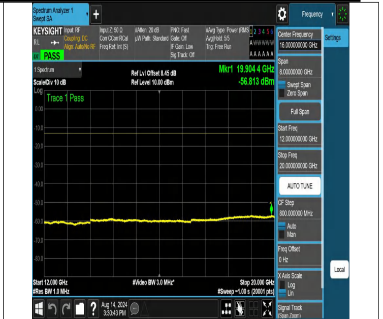
NTNV-N66-PC3-15-25-M-DFT-PI2BPSK-Edge_1RB_Left-12000-2 0000-Ant1-PASS
