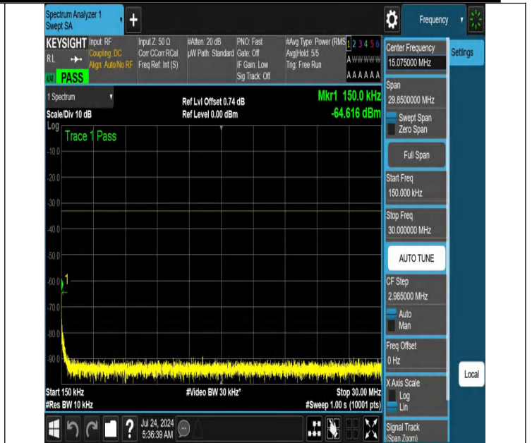
NTNV-N66-PC3-15-20-H-DFT-QPSK-Edge_1RB_Left-0.15-30-Ant 1-PASS
