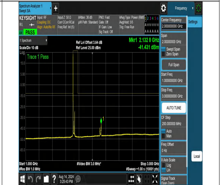
NTNV-N66-PC3-15-25-L-DFT-PI2BPSK-Edge_1RB_Left-1000-3000-Ant1-PASS
