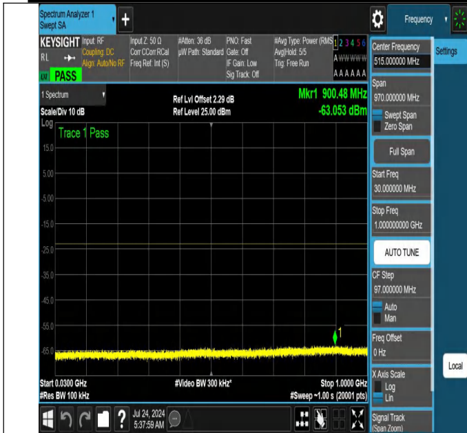
NTNV-N66-PC3-15-20-H-DFT-QPSK-Edge_1RB_Right-30-1000-Ant1-PASS
