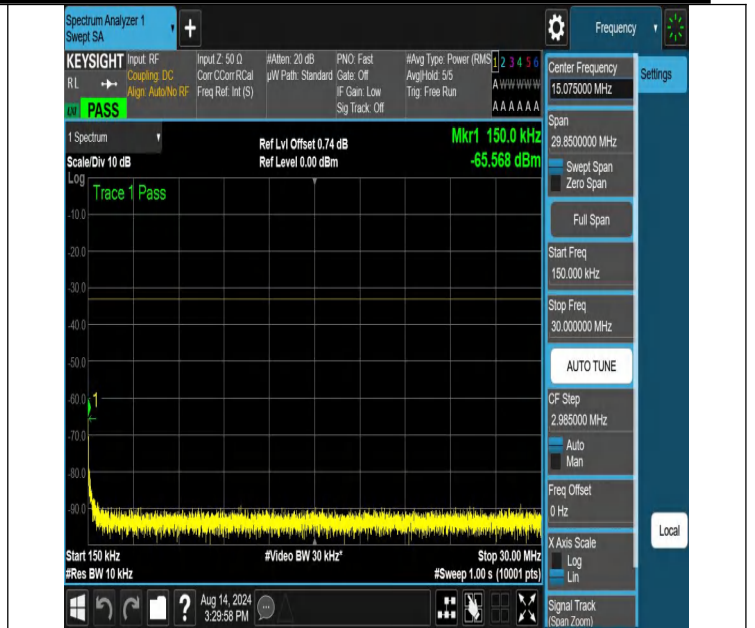
NTNV-N66-PC3-15-25-M-DFT-PI2BPSK-Edge_1RB_Left-0.15-30-Ant1-PASS
