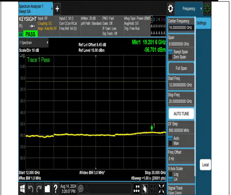
NTNV-N66-PC3-15-25-L-DFT-PI2BPSK-Edge_1RB_Left-12000-20000-Ant1-PASS
