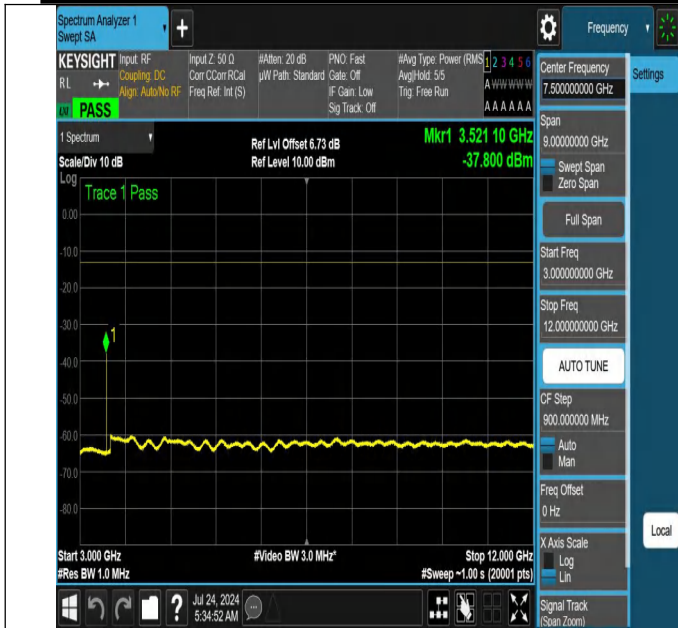
NTNV-N66-PC3-15-20-H-DFT-PI2BPSK-Edge_1RB_Left-3000-1 2000-Ant1-PASS
