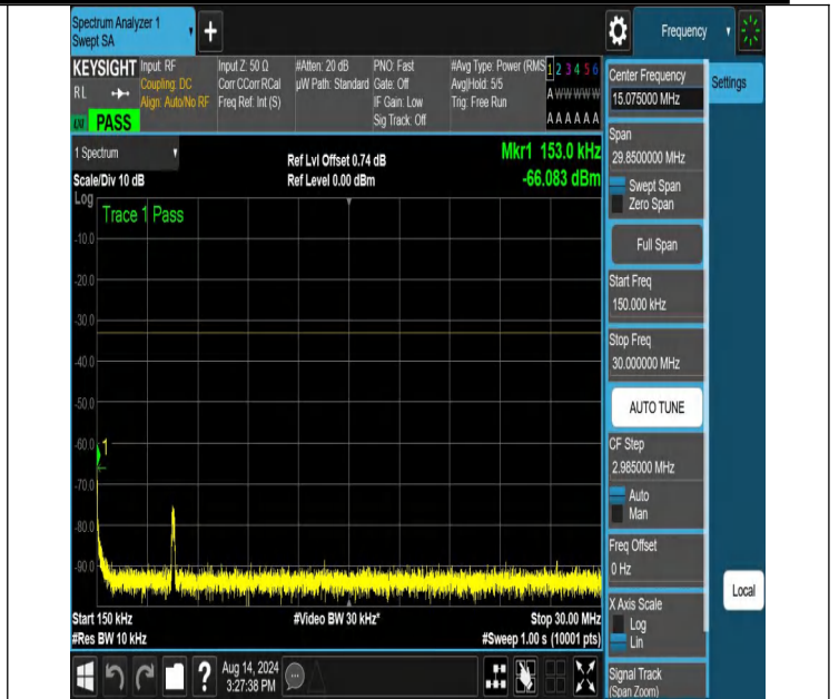
NTNV-N66-PC3-15-25-L-DFT-QPSK-Edge_1RB_Left-0.15-30-Ant 1-PASS
