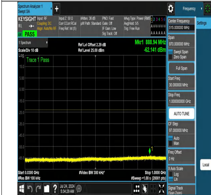
NTNV-N66-PC3-15-20-H-DFT-PI2BPSK-Edge_1RB_Left-30-1000-Ant1-PASS
