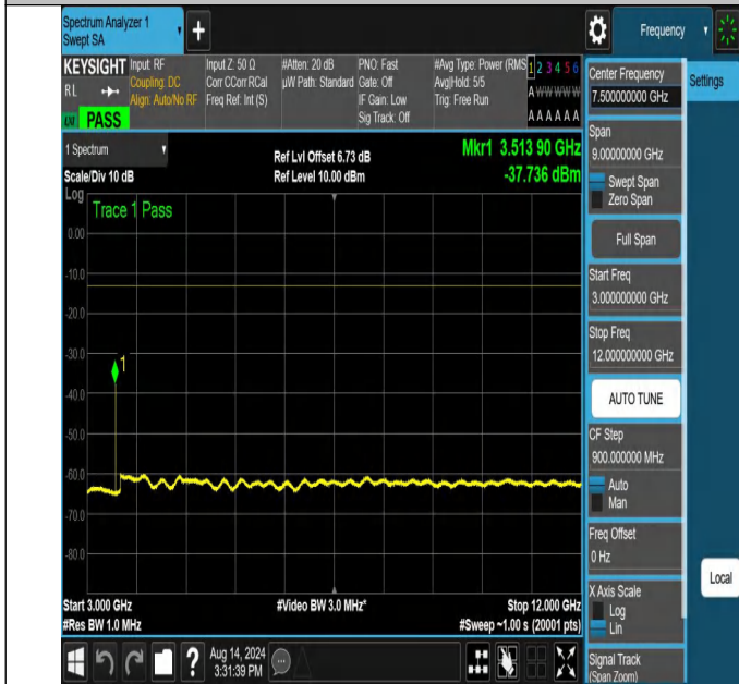
NTNV-N66-PC3-15-25-M-DFT-PI2BPSK-Edge_1RB_Right-3000-12000-Ant1-PASS
