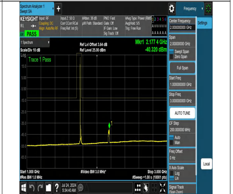
NTNV-N66-PC3-15-20-H-DFT-PI2BPSK-Edge_1RB_Left-1000-3000-Ant1-PASS
