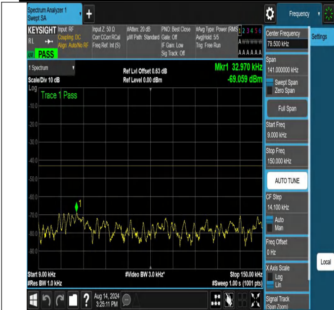
NTNV-N66-PC3-15-25-L-DFT-PI2BPSK-Edge_1RB_Left-0.009-0.15-Ant1-PASS
