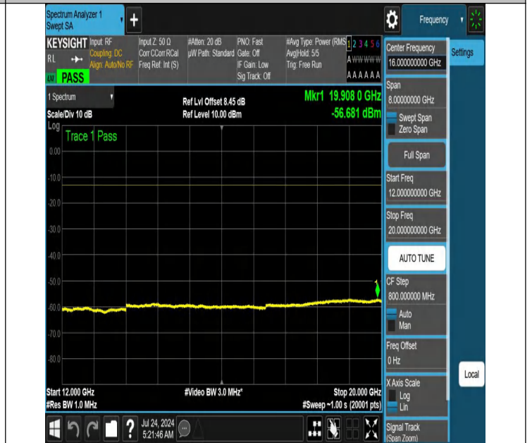
NTNV-N66-PC3-15-15-H-DFT-PI2BPSK-Edge_1RB_Right-12000-20000-Ant1-PASS
