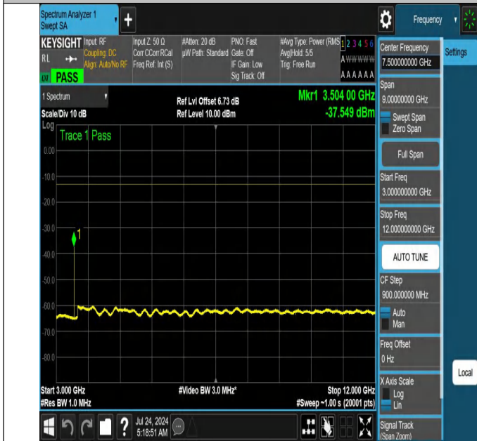
NTNV-N66-PC3-15-15-M-DFT-QPSK-Edge_1RB_Right-3000-12000-Ant1-PASS
