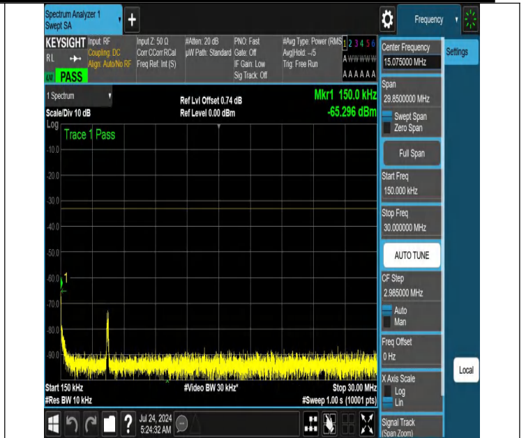
NTNV-N66-PC3-15-20-L-DFT-PI2BPSK-Edge_1RB_Left-0.15-30-Ant1-PASS
