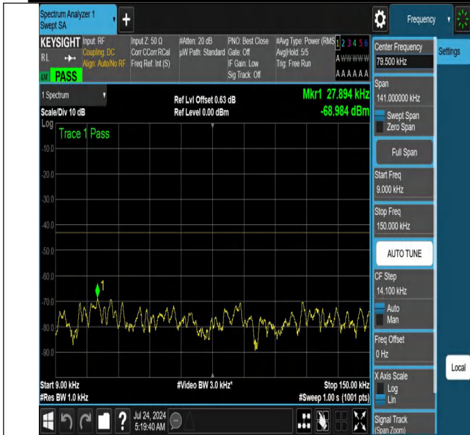
NTNV-N66-PC3-15-15-H-DFT-PI2BPSK-Edge_1RB_Left-0.009-0.15-Ant1-PASS
