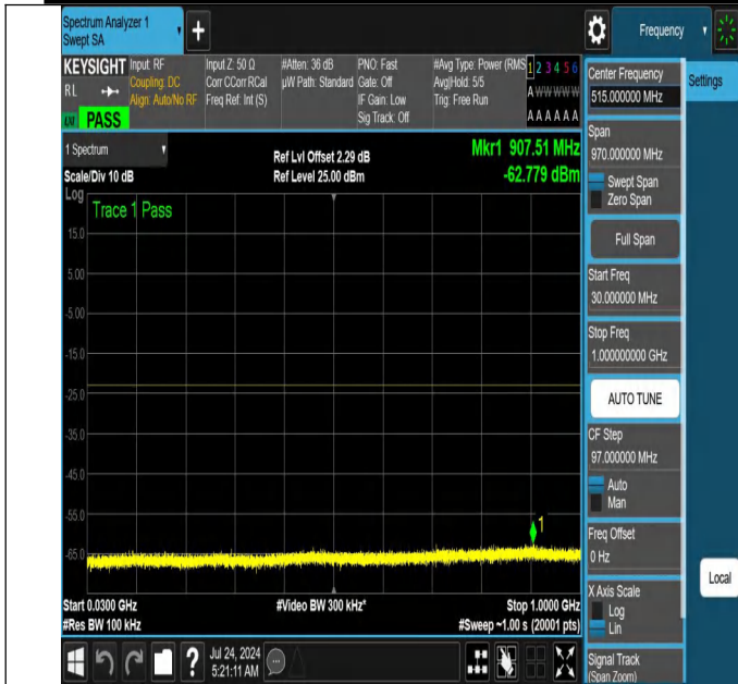
NTNV-N66-PC3-15-15-H-DFT-PI2BPSK-Edge_1RB_Right-30-1000-Ant1-PASS
