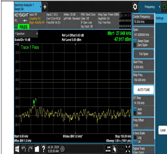
NTNV-N66-PC3-15-20-L-DFT-PI2BPSK-Edge_1RB_Right-0.009-0.15-Ant1-PASS
