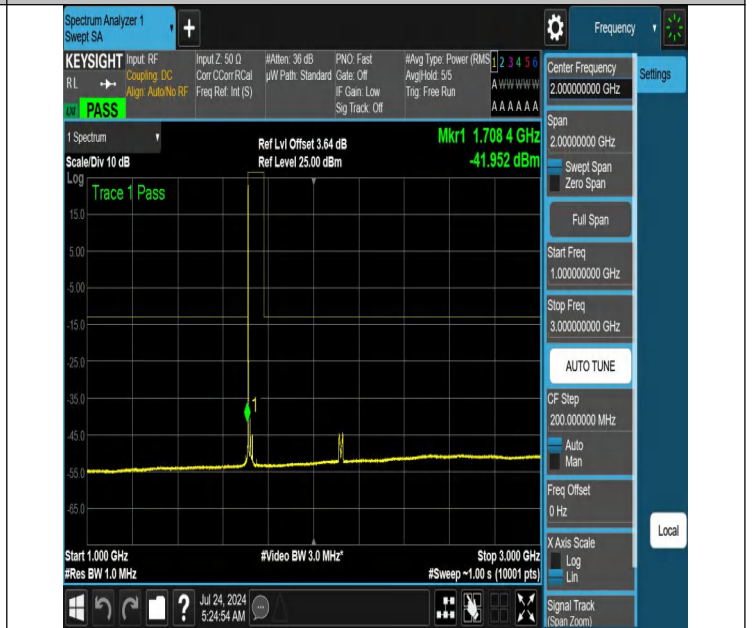
NTNV-N66-PC3-15-20-L-DFT-PI2BPSK-Edge_1RB_Left-1000-3000-Ant1-PASS
