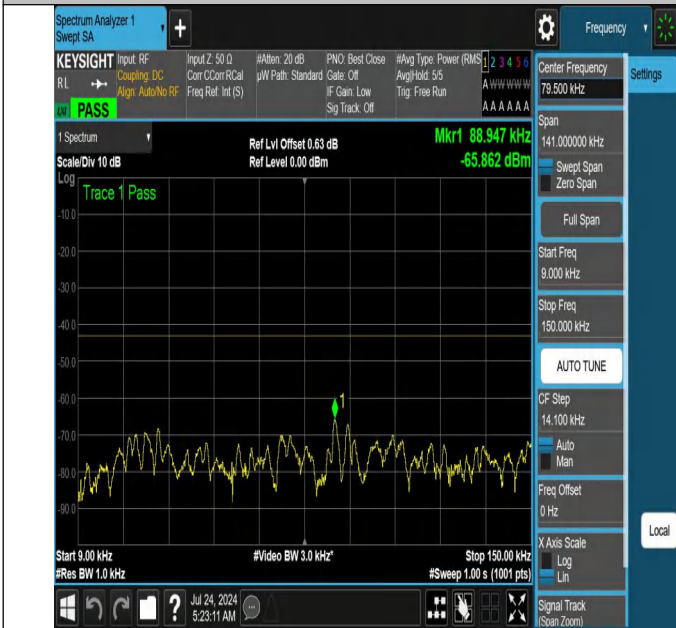
NTNV-N66-PC3-15-15-H-DFT-QPSK-Edge_1RB_Right-0.009-0.1 5-Ant1-PASS
