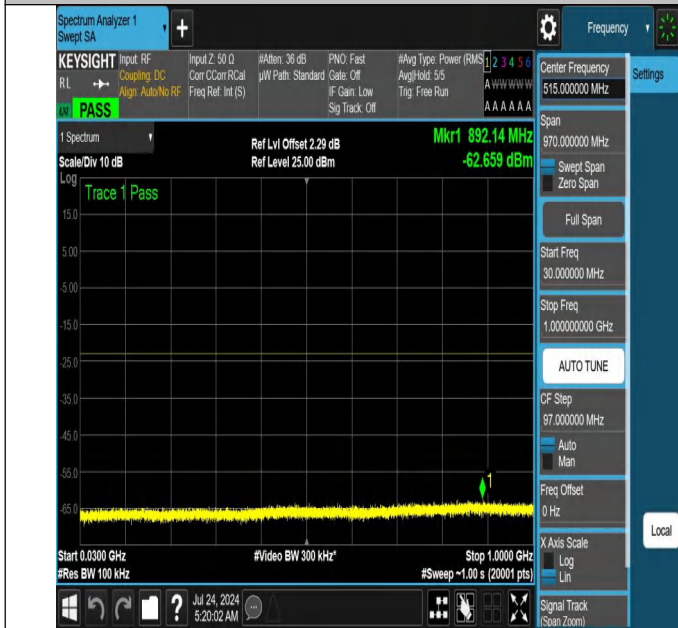
NTNV-N66-PC3-15-15-H-DFT-PI2BPSK-Edge_1RB_Left-30-1000-Ant1-PASS
