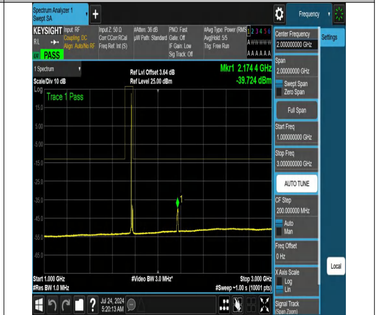
NTNV-N66-PC3-15-15-H-DFT-PI2BPSK-Edge_1RB_Left-1000-3000-Ant1-PASS
