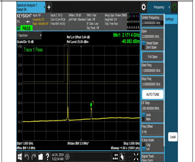
NTNV-N66-PC3-15-15-H-DFT-QPSK-Edge_1RB_Left-1000-3000- Ant1-PASS
