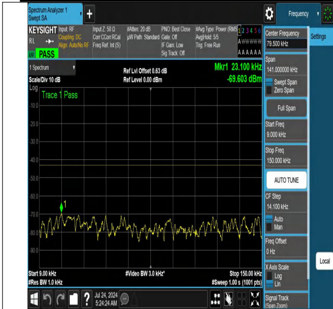
NTNV-N66-PC3-15-20-L-DFT-PI2BPSK-Edge_1RB_Left-0.009-0.15-Ant1-PASS
