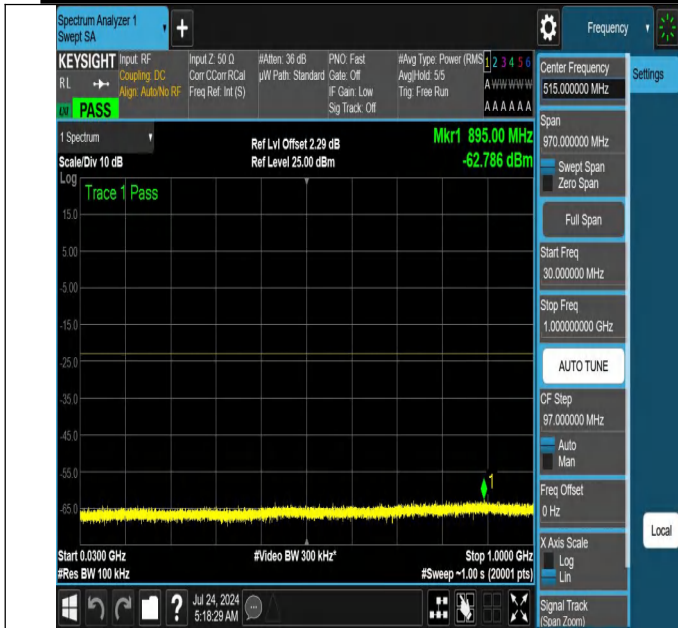
NTNV-N66-PC3-15-15-M-DFT-QPSK-Edge_1RB_Right-30-1000-Ant1-PASS
