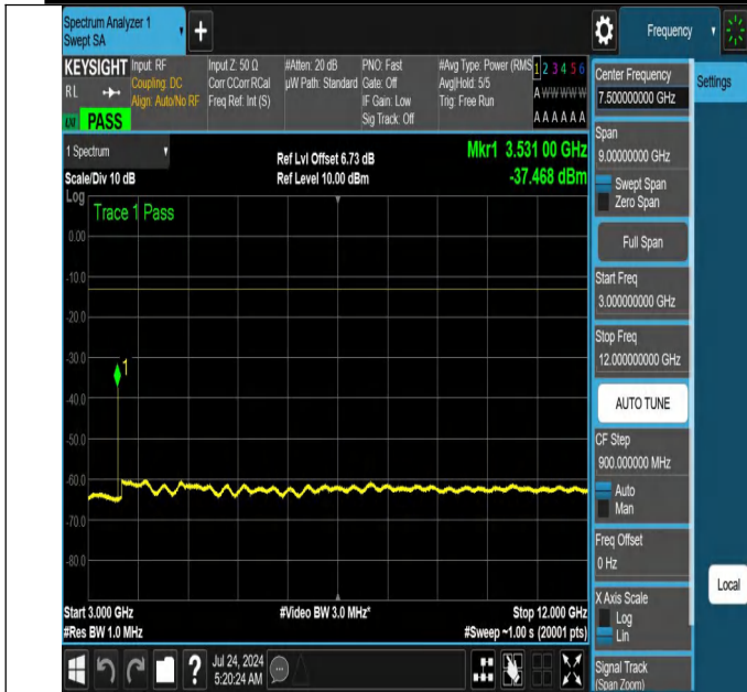
NTNV-N66-PC3-15-15-H-DFT-PI2BPSK-Edge_1RB_Left-3000-1 2000-Ant1-PASS
