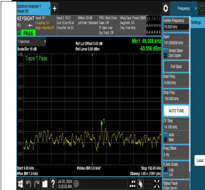
NTNV-N66-PC3-15-15-H-DFT-QPSK-Edge_1RB_Left-0.009-0.15 -Ant1-PASS
