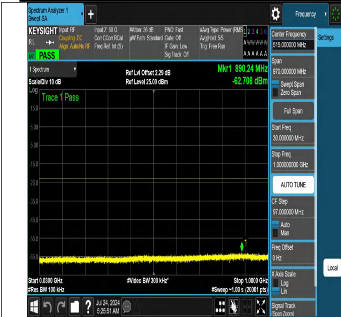
NTNV-N66-PC3-15-20-L-DFT-PI2BPSK-Edge_1RB_Right-30-1000-Ant1-PASS
