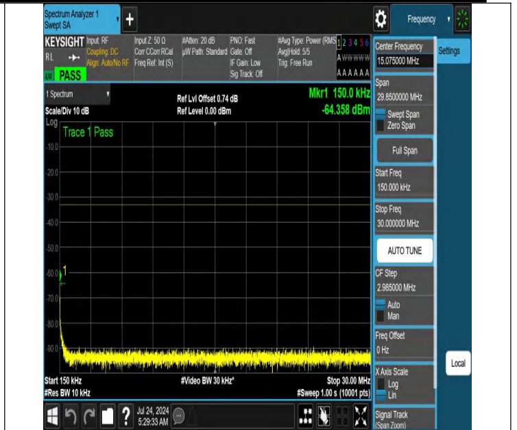
NTNV-N66-PC3-15-20-M-DFT-PI2BPSK-Edge_1RB_Left-0.15-30-Ant1-PASS
