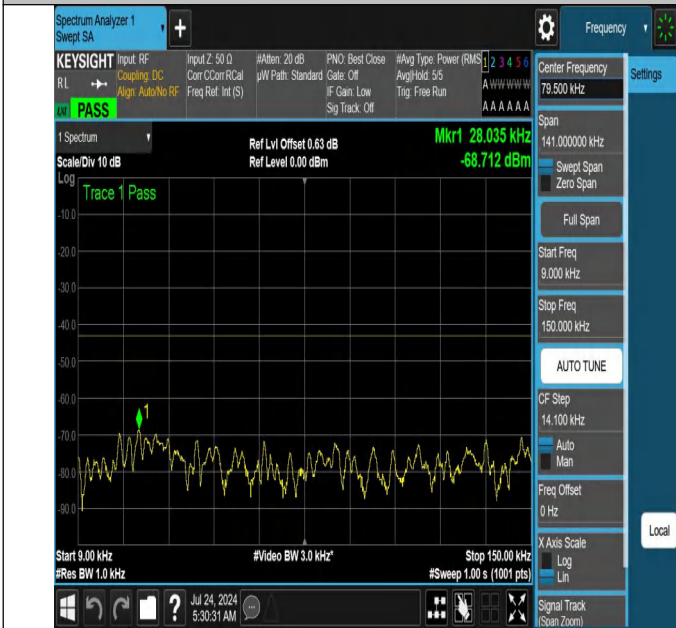
NTNV-N66-PC3-15-20-M-DFT-PI2BPSK-Edge_1RB_Right-0.009 -0.15-Ant1-PASS
