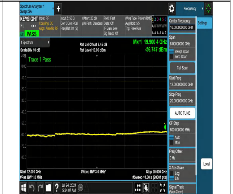
NTNV-N66-PC3-15-15-H-DFT-QPSK-Edge_1RB_Right-12000-20000-Ant1-PASS
