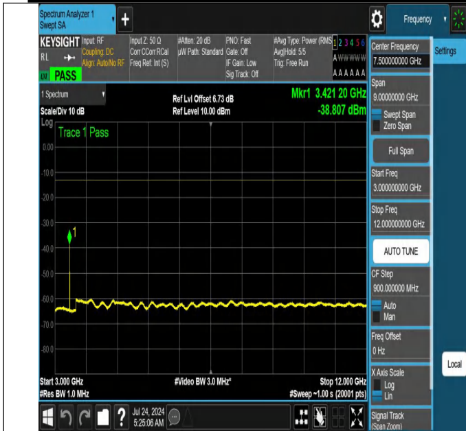
NTNV-N66-PC3-15-20-L-DFT-PI2BPSK-Edge_1RB_Left-3000-12000-Ant1-PASS
