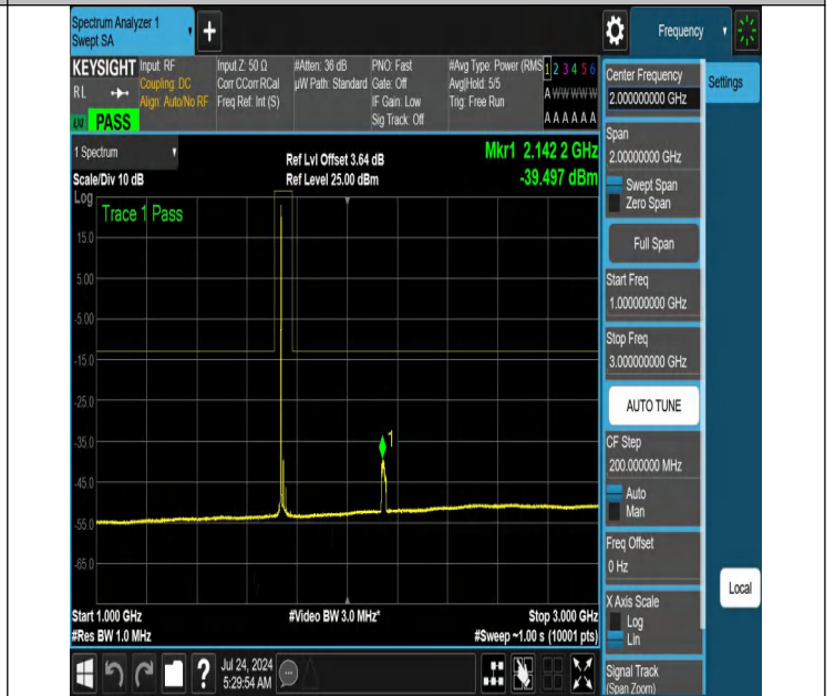
NTNV-N66-PC3-15-20-M-DFT-PI2BPSK-Edge_1RB_Left-1000-3000-Ant1-PASS
