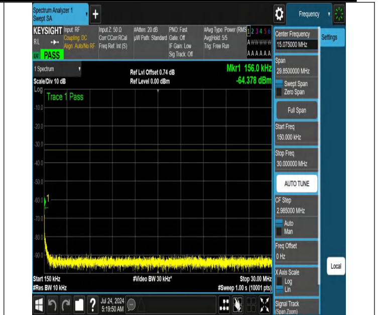
NTNV-N66-PC3-15-15-H-DFT-PI2BPSK-Edge_1RB_Left-0.15-30-Ant1-PASS
