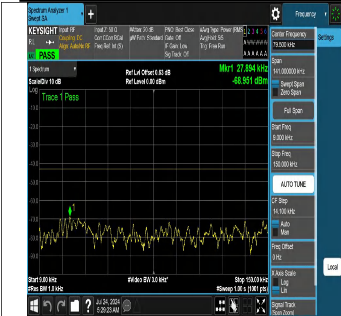
NTNV-N66-PC3-15-20-M-DFT-PI2BPSK-Edge_1RB_Left-0.009-0.15-Ant1-PASS
