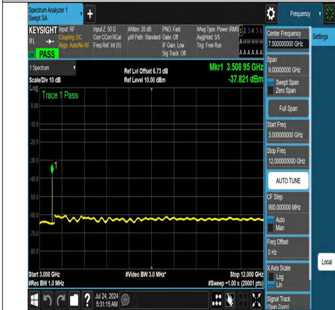
NTNV-N66-PC3-15-20-M-DFT-PI2BPSK-Edge_1RB_Right-3000-12000-Ant1-PASS
