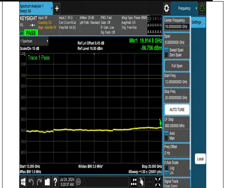
NTNV-N66-PC3-15-15-H-DFT-PI2BPSK-Edge_1RB_Left-12000-2 0000-Ant1-PASS
