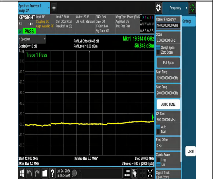
NTNV-N66-PC3-15-15-M-DFT-QPSK-Edge_1RB_Right-12000-20000-Ant1-PASS
