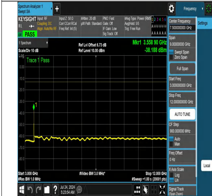
NTNV-N66-PC3-15-15-H-DFT-QPSK-Edge_1RB_Right-3000-12000-Ant1-PASS
