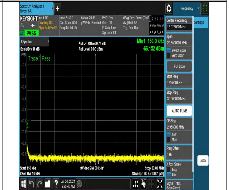
NTNV-N66-PC3-15-20-L-DFT-PI2BPSK-Edge_1RB_Right-0.15-30-Ant1-PASS
