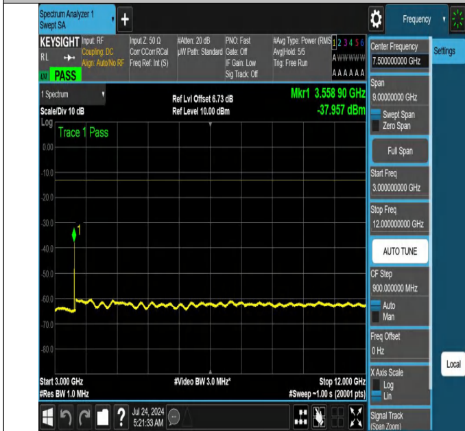
NTNV-N66-PC3-15-15-H-DFT-PI2BPSK-Edge_1RB_Right-3000-12000-Ant1-PASS
