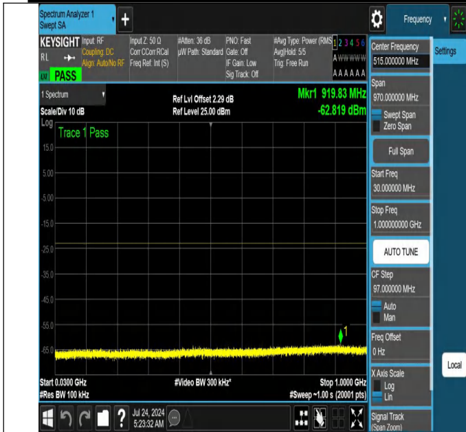
NTNV-N66-PC3-15-15-H-DFT-QPSK-Edge_1RB_Right-30-1000-Ant1-PASS
