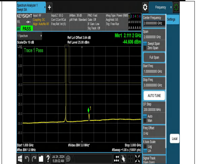
NTNV-N66-PC3-15-20-L-DFT-PI2BPSK-Edge_1RB_Right-1000-3000-Ant1-PASS
