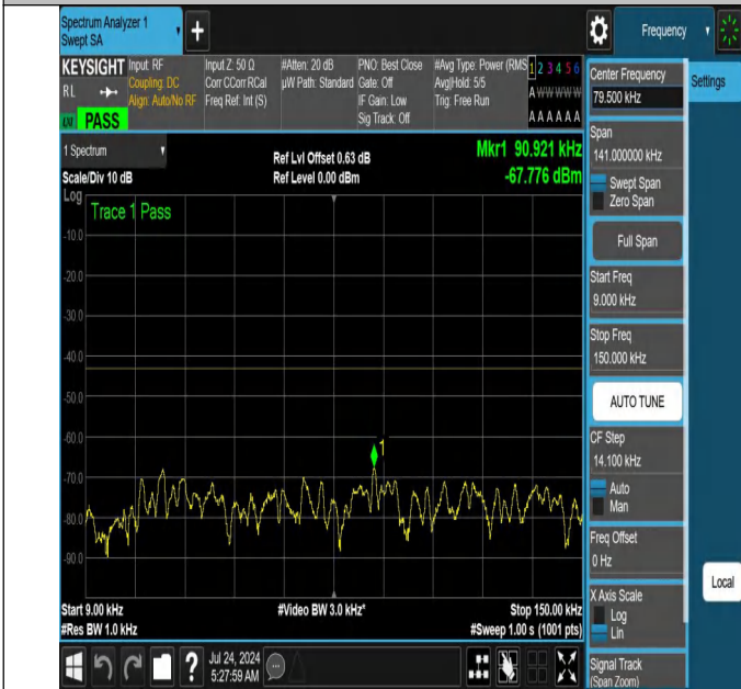
NTNV-N66-PC3-15-20-L-DFT-QPSK-Edge_1RB_Right-0.009-0.1 5-Ant1-PASS
