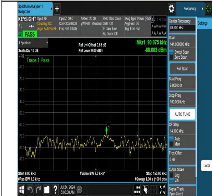
NTNV-N66-PC3-15-10-H-DFT-QPSK-Edge_1RB_Right-0.009-0.1 5-Ant1-PASS
