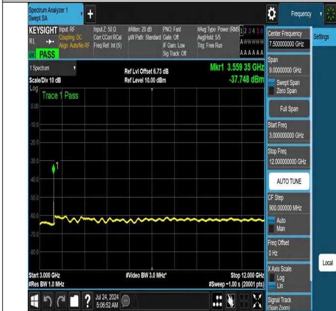
NTNV-N66-PC3-15-10-H-DFT-PI2BPSK-Edge_1RB_Right-3000-12000-Ant1-PASS
