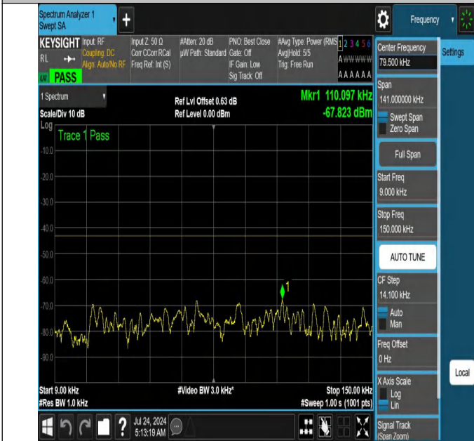
NTNV-N66-PC3-15-15-L-DFT-QPSK-Edge_1RB_Right-0.009-0.1 5-Ant1-PASS
