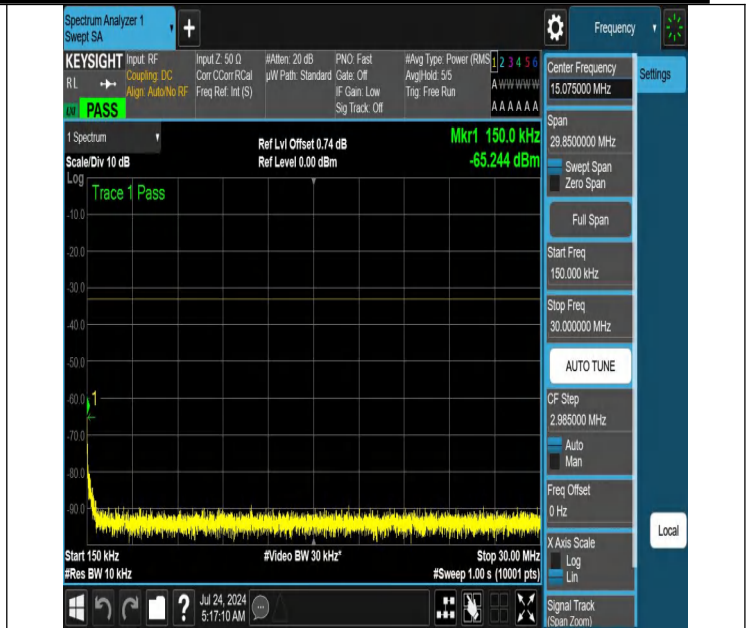
NTNV-N66-PC3-15-15-M-DFT-QPSK-Edge_1RB_Left-0.15-30-Ant 1-PASS
