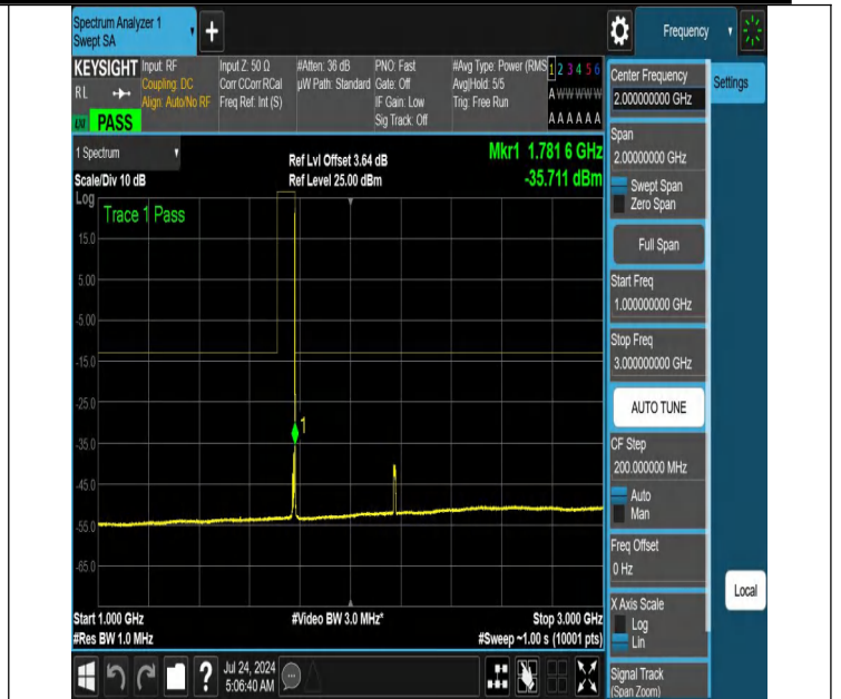
NTNV-N66-PC3-15-10-H-DFT-PI2BPSK-Edge_1RB_Right-1000-3000-Ant1-PASS
