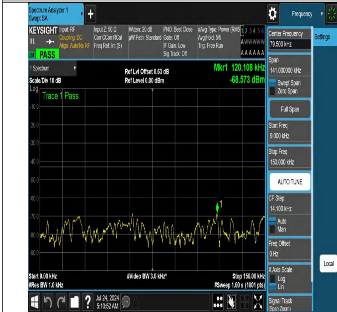
NTNV-N66-PC3-15-15-L-DFT-PI2BPSK-Edge_1RB_Right-0.009-0.15-Ant1-PASS
