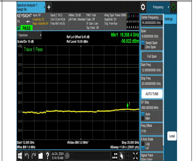
NTNV-N66-PC3-15-15-L-DFT-QPSK-Edge_1RB_Right-12000-20000-Ant1-PASS
