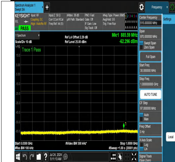
NTNV-N66-PC3-15-15-L-DFT-PI2BPSK-Edge_1RB_Right-30-1000-Ant1-PASS
