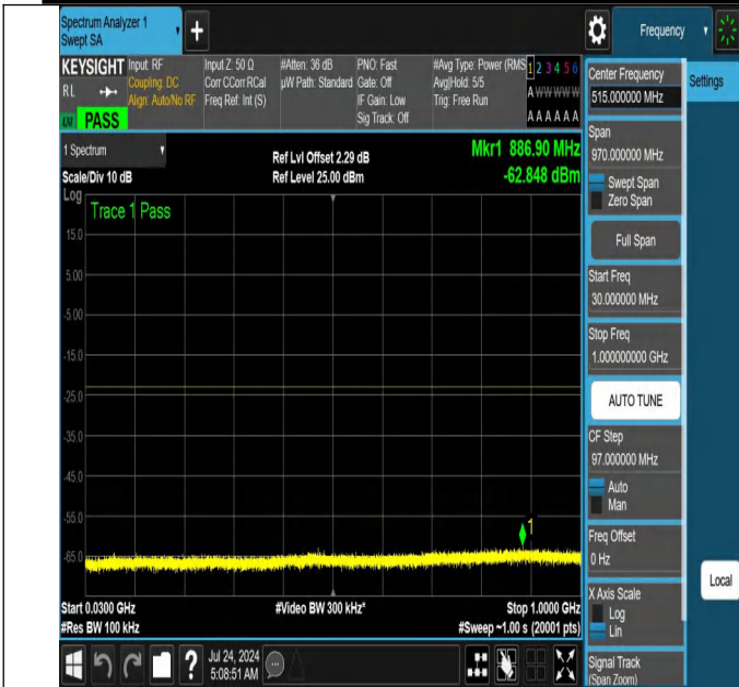
NTNV-N66-PC3-15-10-H-DFT-QPSK-Edge_1RB_Right-30-1000-Ant1-PASS
