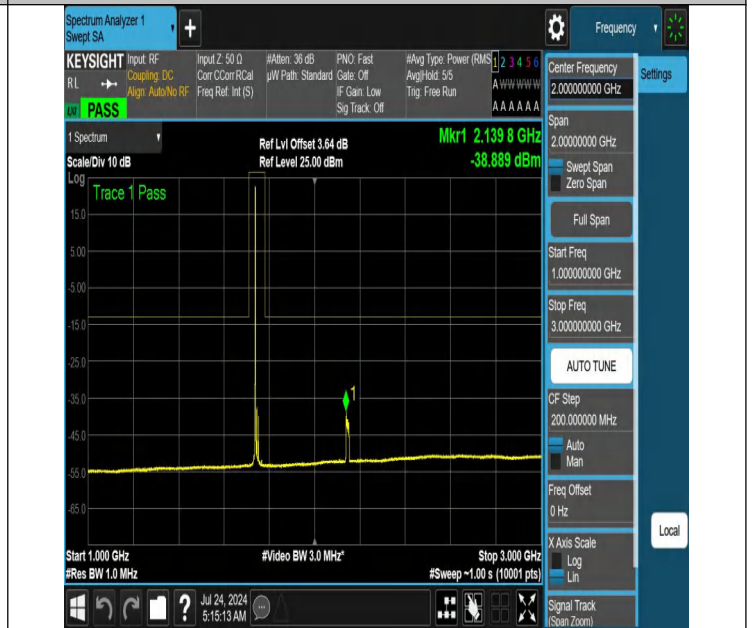
NTNV-N66-PC3-15-15-M-DFT-PI2BPSK-Edge_1RB_Left-1000-3000-Ant1-PASS
