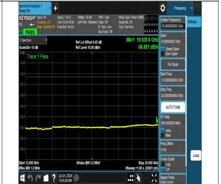
NTNV-N66-PC3-15-10-M-DFT-QPSK-Edge_1RB_Right-12000-20000-Ant1-PASS
