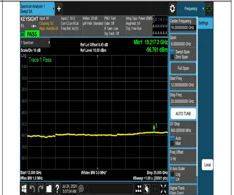
NTNV-N66-PC3-15-10-H-DFT-PI2BPSK-Edge_1RB_Right-12000-20000-Ant1-PASS
