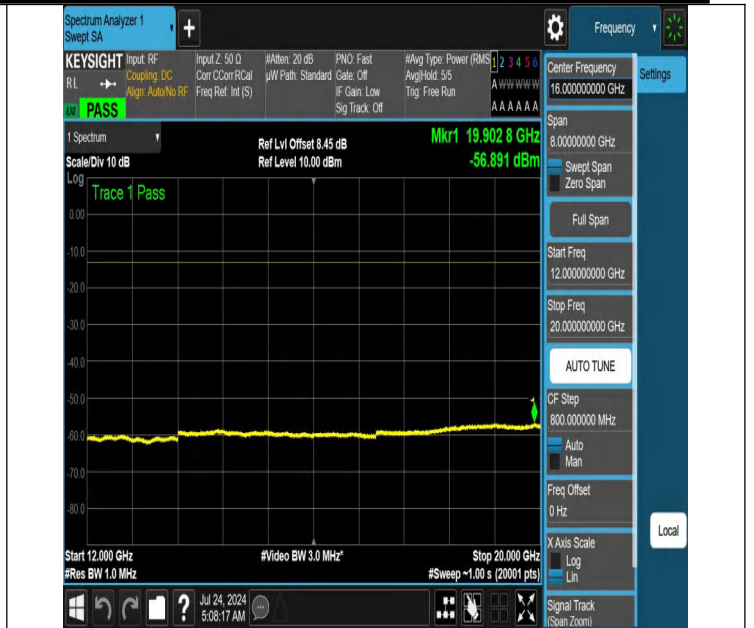
NTNV-N66-PC3-15-10-H-DFT-QPSK-Edge_1RB_Left-12000-2000 0-Ant1-PASS
