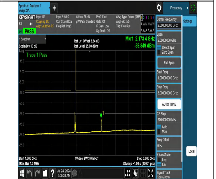
NTNV-N66-PC3-15-10-H-DFT-PI2BPSK-Edge_1RB_Left-1000-3000-Ant1-PASS
