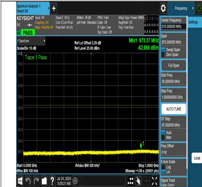
NTNV-N66-PC3-15-10-H-DFT-PI2BPSK-Edge_1RB_Left-30-1000-Ant1-PASS
