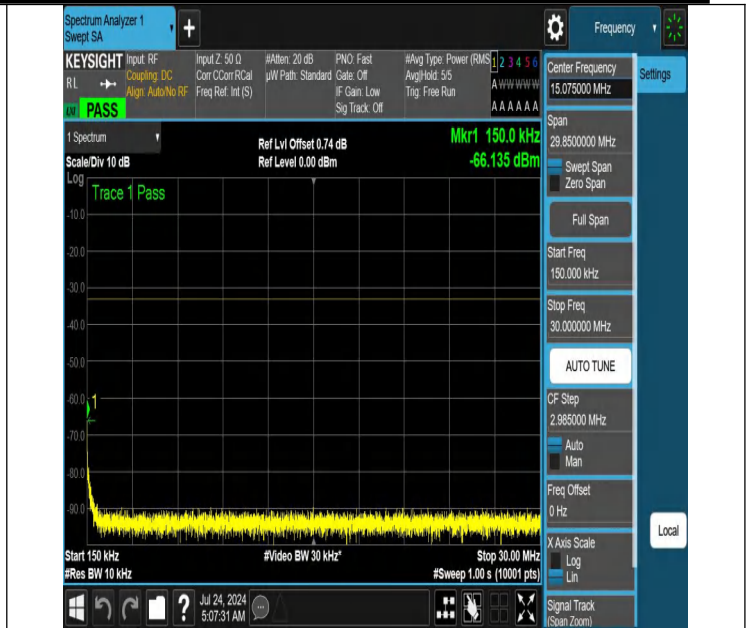
NTNV-N66-PC3-15-10-H-DFT-QPSK-Edge_1RB_Left-0.15-30-Ant 1-PASS
