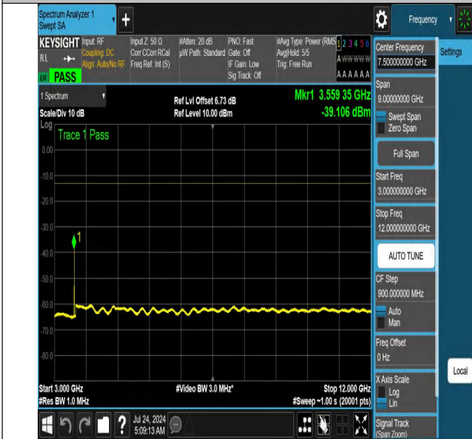
NTNV-N66-PC3-15-10-H-DFT-QPSK-Edge_1RB_Right-3000-12000-Ant1-PASS
