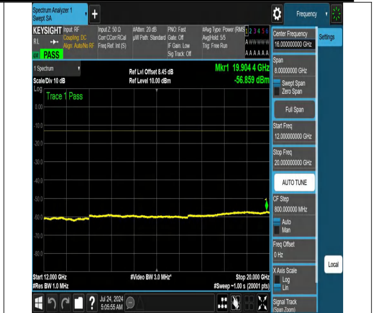
NTNV-N66-PC3-15-10-H-DFT-PI2BPSK-Edge_1RB_Left-12000-2 0000-Ant1-PASS
