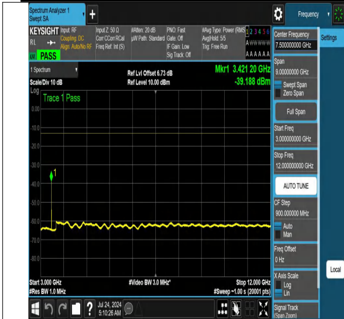
NTNV-N66-PC3-15-15-L-DFT-PI2BPSK-Edge_1RB_Left-3000-12000-Ant1-PASS
