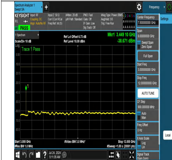
NTNV-N66-PC3-15-15-L-DFT-PI2BPSK-Edge_1RB_Right-3000-12000-Ant1-PASS
