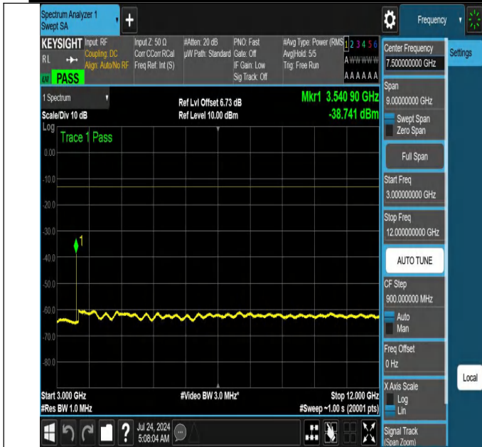
NTNV-N66-PC3-15-10-H-DFT-QPSK-Edge_1RB_Left-3000-1200 0-Ant1-PASS
