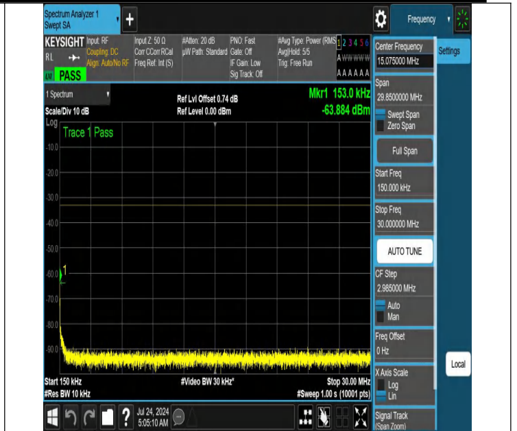
NTNV-N66-PC3-15-10-H-DFT-PI2BPSK-Edge_1RB_Left-0.15-30-Ant1-PASS
