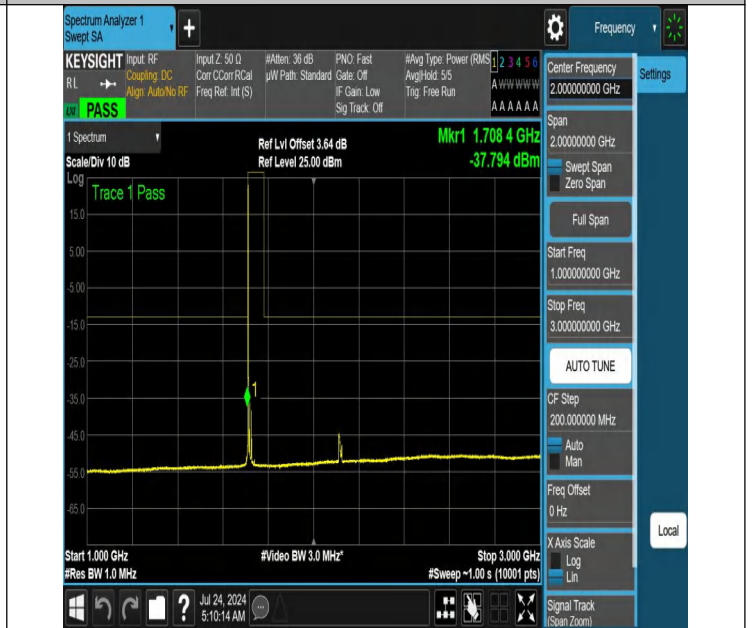
NTNV-N66-PC3-15-15-L-DFT-PI2BPSK-Edge_1RB_Left-1000-3000-Ant1-PASS
