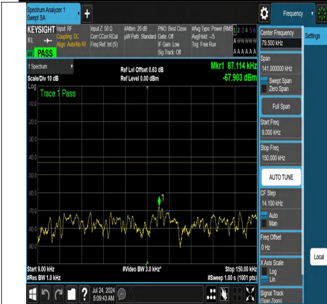
NTNV-N66-PC3-15-15-L-DFT-PI2BPSK-Edge_1RB_Left-0.009-0.15-Ant1-PASS
