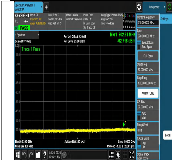
NTNV-N66-PC3-15-15-M-DFT-PI2BPSK-Edge_1RB_Right-30-1000-Ant1-PASS
