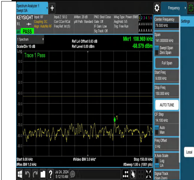
NTNV-N66-PC3-15-15-L-DFT-QPSK-Edge_1RB_Left-0.009-0.15-Ant1-PASS
