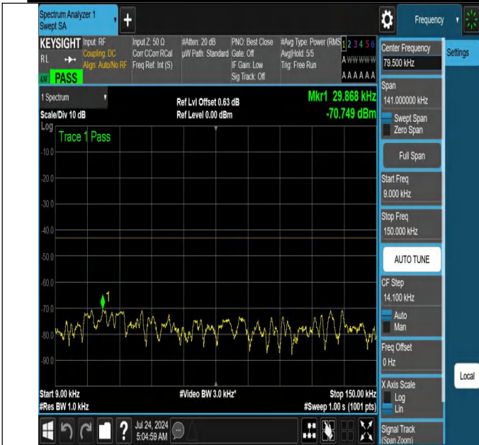
NTNV-N66-PC3-15-10-H-DFT-PI2BPSK-Edge_1RB_Left-0.009-0.15-Ant1-PASS
