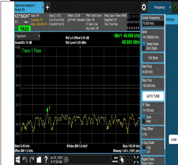
NTNV-N66-PC3-15-15-M-DFT-QPSK-Edge_1RB_Left-0.009-0.15 -Ant1-PASS
