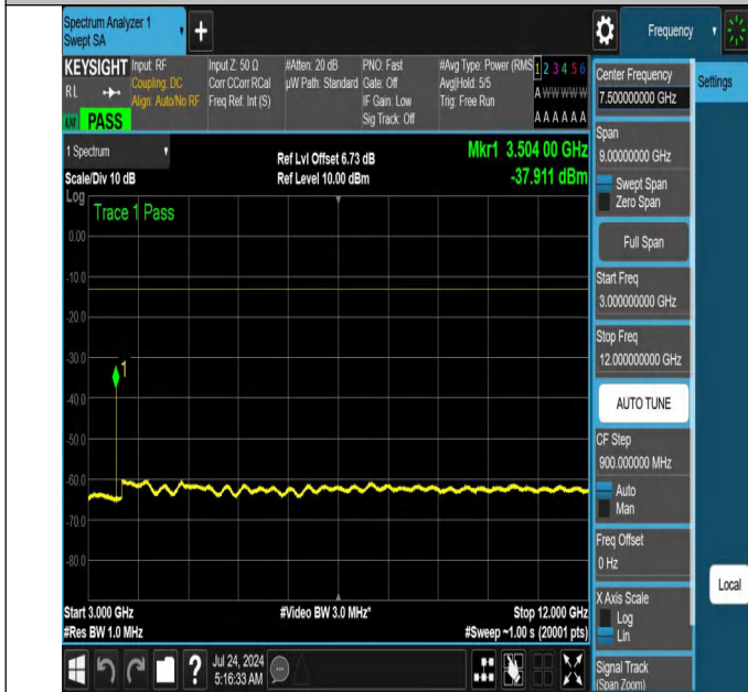
NTNV-N66-PC3-15-15-M-DFT-PI2BPSK-Edge_1RB_Right-3000-12000-Ant1-PASS
