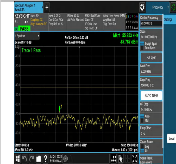
NTNV-N66-PC3-15-15-M-DFT-PI2BPSK-Edge_1RB_Right-0.009 -0.15-Ant1-PASS
