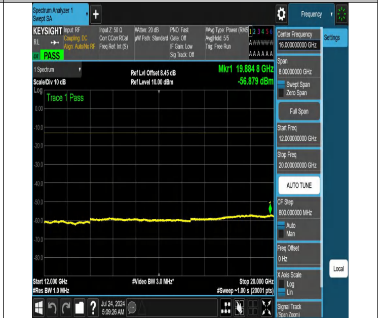
NTNV-N66-PC3-15-10-H-DFT-QPSK-Edge_1RB_Right-12000-20000-Ant1-PASS
