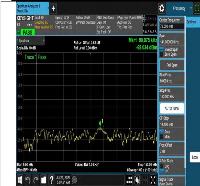
NTNV-N66-PC3-15-10-H-DFT-QPSK-Edge_1RB_Left-0.009-0.15 -Ant1-PASS
