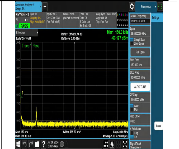
NTNV-N66-PC3-15-15-L-DFT-PI2BPSK-Edge_1RB_Left-0.15-30-Ant1-PASS
