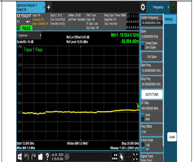
NTNV-N66-PC3-15-15-M-DFT-PI2BPSK-Edge_1RB_Right-12000-20000-Ant1-PASS
