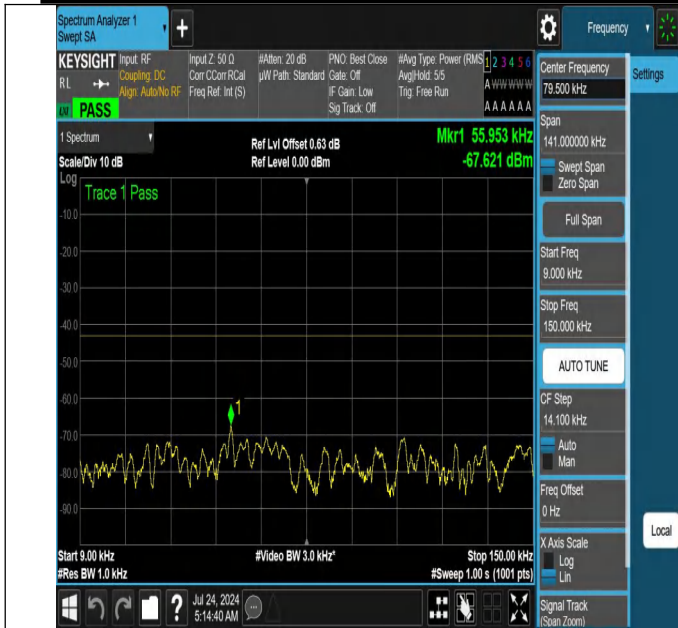
NTNV-N66-PC3-15-15-M-DFT-PI2BPSK-Edge_1RB_Left-0.009-0.15-Ant1-PASS
