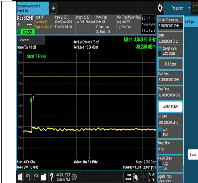
NTNV-N66-PC3-15-10-H-DFT-PI2BPSK-Edge_1RB_Left-3000-1 2000-Ant1-PASS
