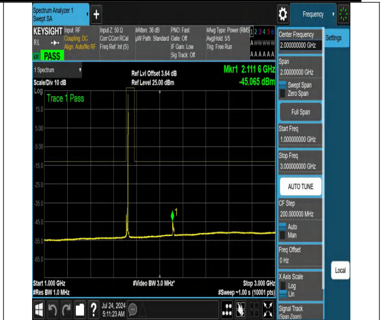
NTNV-N66-PC3-15-15-L-DFT-PI2BPSK-Edge_1RB_Right-1000-3000-Ant1-PASS
