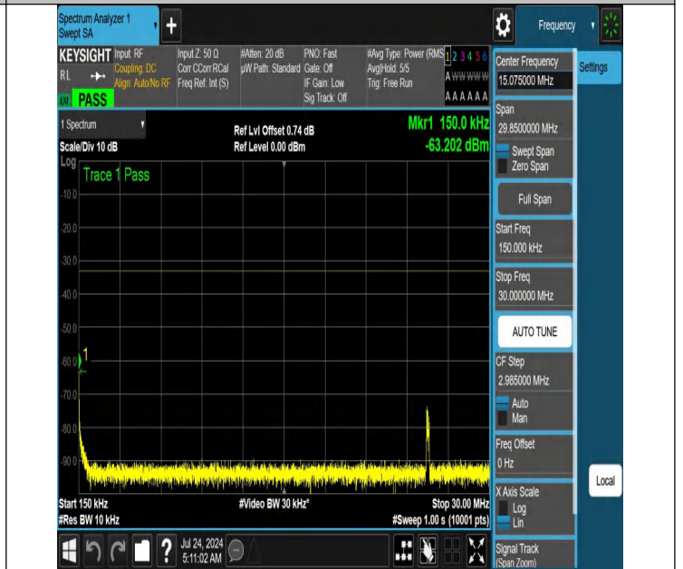
NTNV-N66-PC3-15-15-L-DFT-PI2BPSK-Edge_1RB_Right-0.15-30-Ant1-PASS
