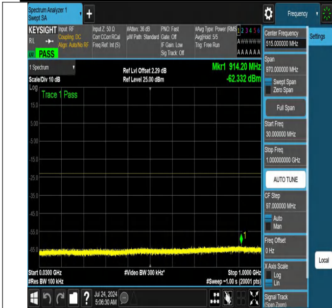
NTNV-N66-PC3-15-10-H-DFT-PI2BPSK-Edge_1RB_Right-30-1000-Ant1-PASS
