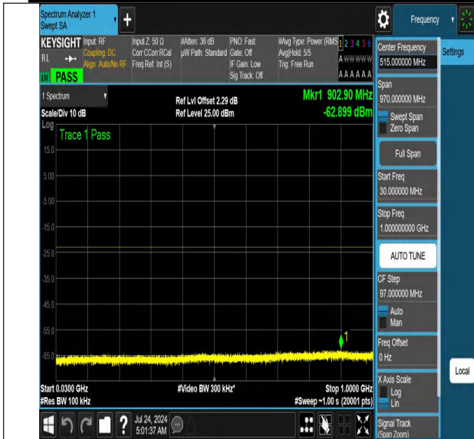
NTNV-N66-PC3-15-10-M-DFT-PI2BPSK-Edge_1RB_Right-30-1000-Ant1-PASS
