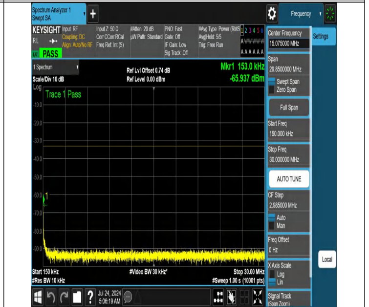
NTNV-N66-PC3-15-10-H-DFT-PI2BPSK-Edge_1RB_Right-0.15-3 0-Ant1-PASS
