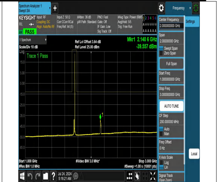
NTNV-N66-PC3-15-15-M-DFT-PI2BPSK-Edge_1RB_Right-1000-3000-Ant1-PASS
