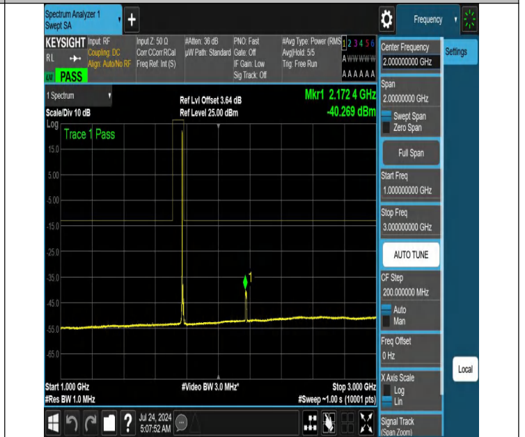
NTNV-N66-PC3-15-10-H-DFT-QPSK-Edge_1RB_Left-1000-3000- Ant1-PASS
