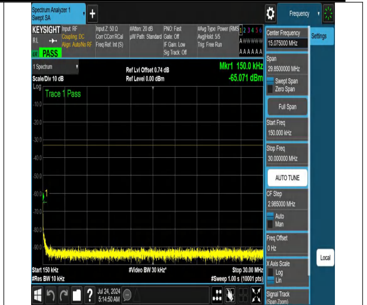
NTNV-N66-PC3-15-15-M-DFT-PI2BPSK-Edge_1RB_Left-0.15-30-Ant1-PASS
