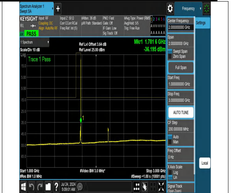
NTNV-N66-PC3-15-10-H-DFT-QPSK-Edge_1RB_Right-1000-300-0-Ant1-PASS
