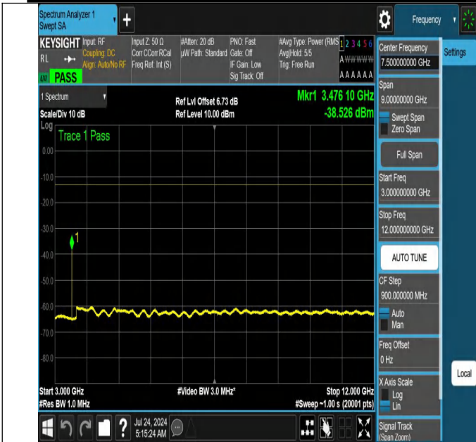
NTNV-N66-PC3-15-15-M-DFT-PI2BPSK-Edge_1RB_Left-3000-1 2000-Ant1-PASS
