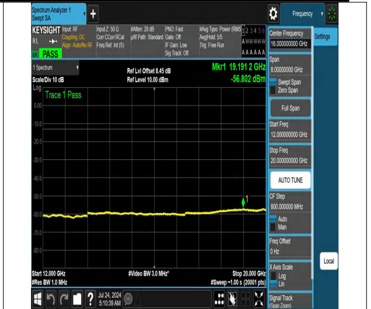
NTNV-N66-PC3-15-15-L-DFT-PI2BPSK-Edge_1RB_Left-12000-20000-Ant1-PASS
