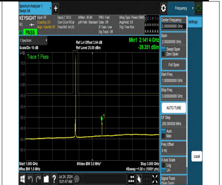
NTNV-N66-PC3-15-10-M-DFT-PI2BPSK-Edge_1RB_Right-1000-3000-Ant1-PASS
