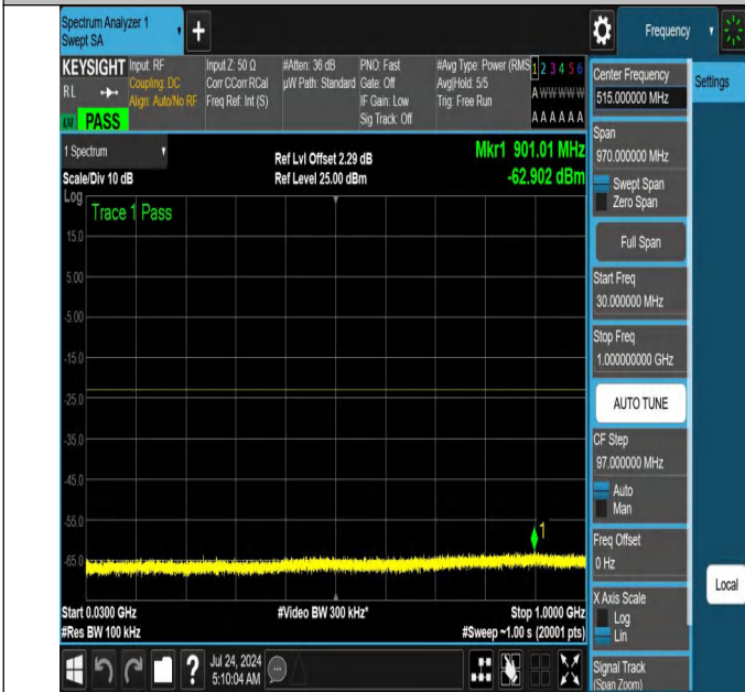
NTNV-N66-PC3-15-15-L-DFT-PI2BPSK-Edge_1RB_Left-30-1000-Ant1-PASS
