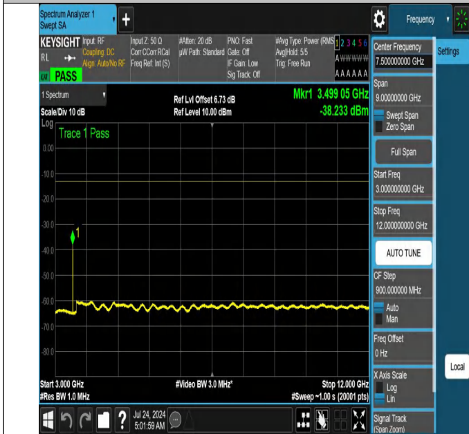
NTNV-N66-PC3-15-10-M-DFT-PI2BPSK-Edge_1RB_Right-3000-12000-Ant1-PASS
