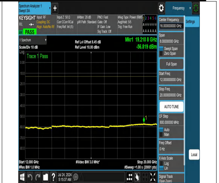
NTNV-N66-PC3-15-15-M-DFT-PI2BPSK-Edge_1RB_Left-12000-2 0000-Ant1-PASS
