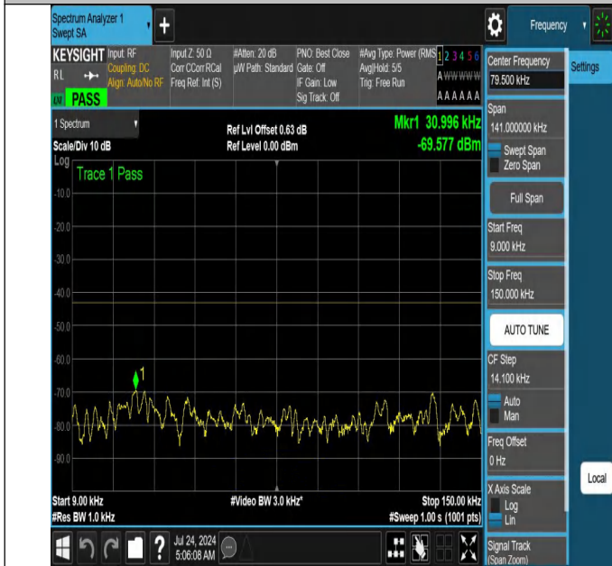
NTNV-N66-PC3-15-10-H-DFT-PI2BPSK-Edge_1RB_Right-0.009- 0.15-Ant1-PASS
