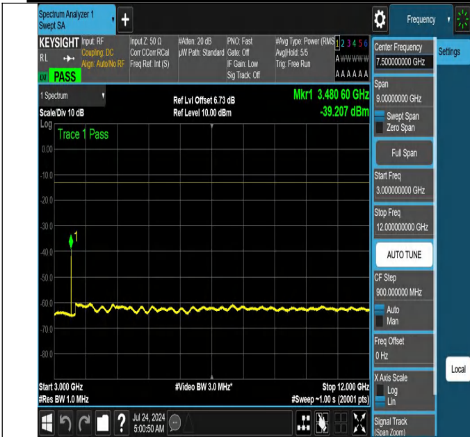
NTNV-N66-PC3-15-10-M-DFT-PI2BPSK-Edge_1RB_Left-3000-1 2000-Ant1-PASS
