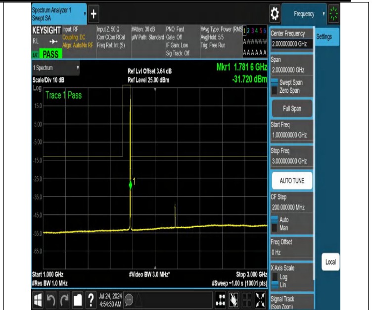
NTNV-N66-PC3-15-5-H-DFT-QPSK-Edge_1RB_Right-1000-3000- Ant1-PASS
