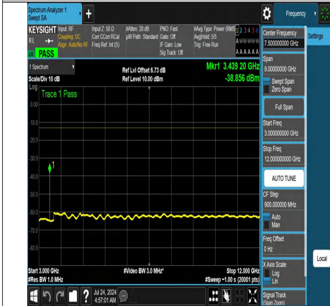
NTNV-N66-PC3-15-10-L-DFT-PI2BPSK-Edge_1RB_Right-3000-12000-Ant1-PASS
