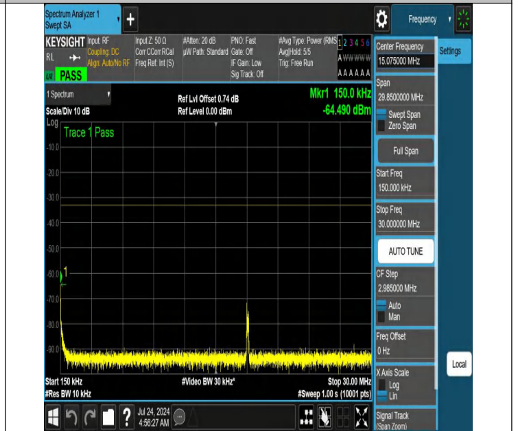
NTNV-N66-PC3-15-10-L-DFT-PI2BPSK-Edge_1RB_Right-0.15-30-Ant1-PASS
