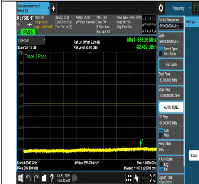
NTNV-N66-PC3-15-5-H-DFT-QPSK-Edge_1RB_Left-30-1000-Ant1-PASS
