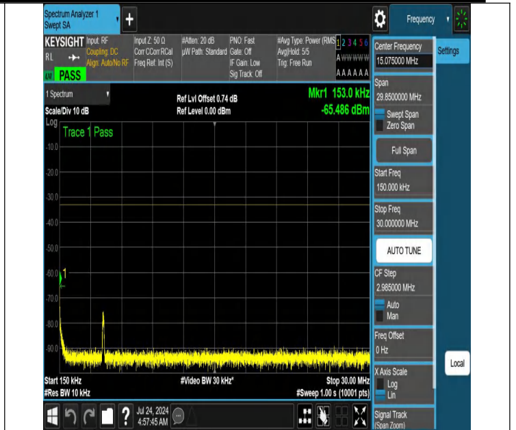
NTNV-N66-PC3-15-10-L-DFT-QPSK-Edge_1RB_Left-0.15-30-Ant 1-PASS
