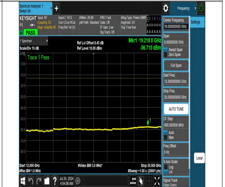
NTNV-N66-PC3-15-5-H-DFT-QPSK-Edge_1RB_Right-12000-200 00-Ant1-PASS
