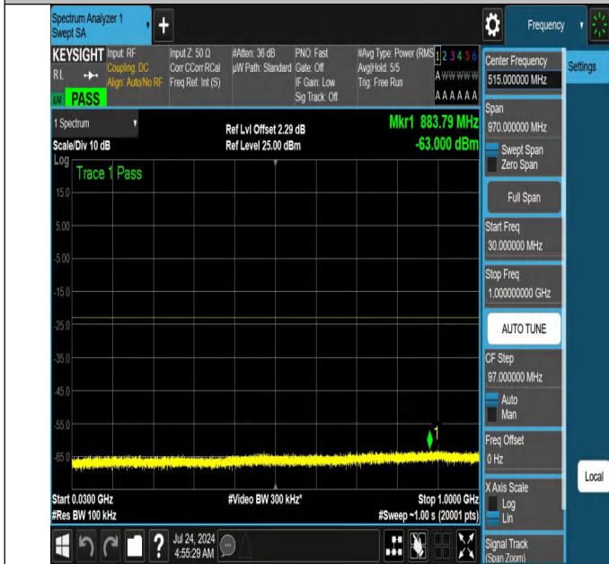
NTNV-N66-PC3-15-10-L-DFT-PI2BPSK-Edge_1RB_Left-30-1000-Ant1-PASS
