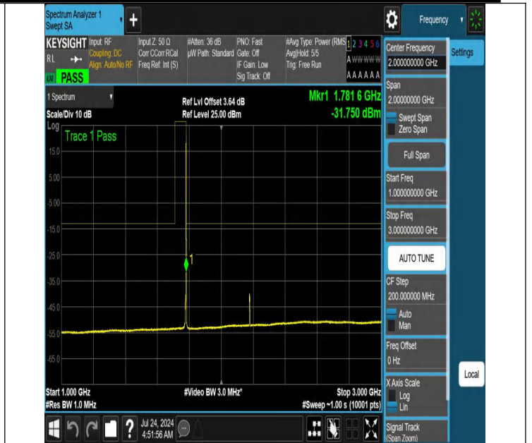
NTNV-N66-PC3-15-5-H-DFT-PI2BPSK-Edge_1RB_Right-1000-30 00-Ant1-PASS
