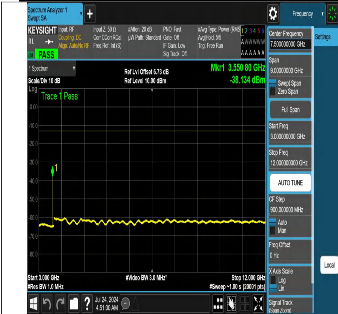
NTNV-N66-PC3-15-5-H-DFT-PI2BPSK-Edge_1RB_Left-3000-12000-Ant1-PASS
