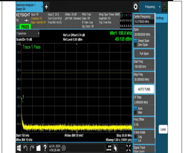
NTNV-N66-PC3-15-5-H-DFT-PI2BPSK-Edge_1RB_Left-0.15-30-Ant1-PASS
