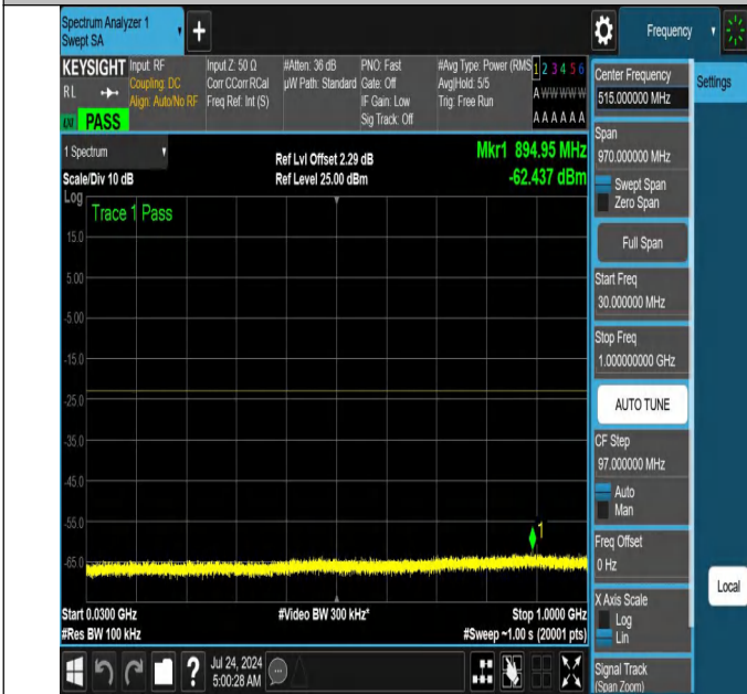
NTNV-N66-PC3-15-10-M-DFT-PI2BPSK-Edge_1RB_Left-30-1000-Ant1-PASS
