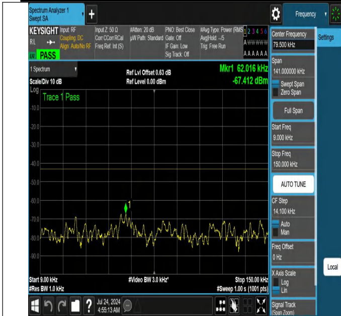
NTNV-N66-PC3-15-10-L-DFT-PI2BPSK-Edge_1RB_Left-0.009-0.15-Ant1-PASS
