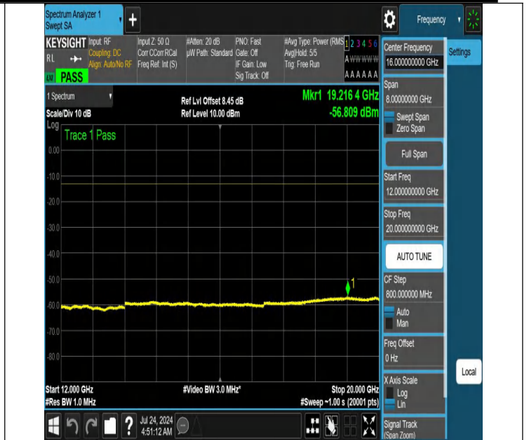
NTNV-N66-PC3-15-5-H-DFT-PI2BPSK-Edge_1RB_Left-12000-20000-Ant1-PASS
