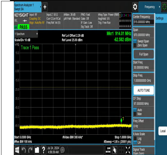
NTNV-N66-PC3-15-10-L-DFT-PI2BPSK-Edge_1RB_Right-30-1000-Ant1-PASS
