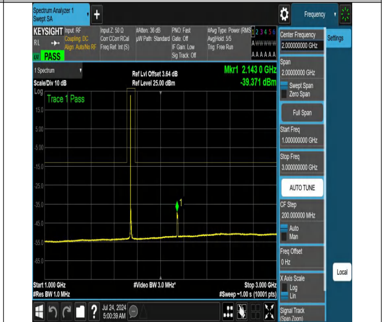
NTNV-N66-PC3-15-10-M-DFT-PI2BPSK-Edge_1RB_Left-1000-3000-Ant1-PASS
