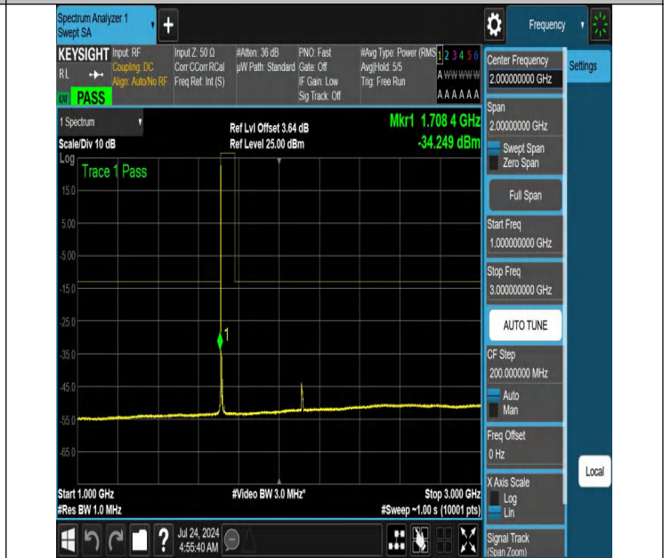
NTNV-N66-PC3-15-10-L-DFT-PI2BPSK-Edge_1RB_Left-1000-3000-Ant1-PASS
