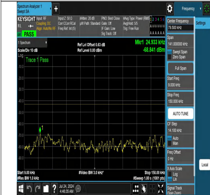
NTNV-N66-PC3-15-5-M-DFT-PI2BPSK-Edge_1RB_Right-0.009-0.15-Ant1-PASS
