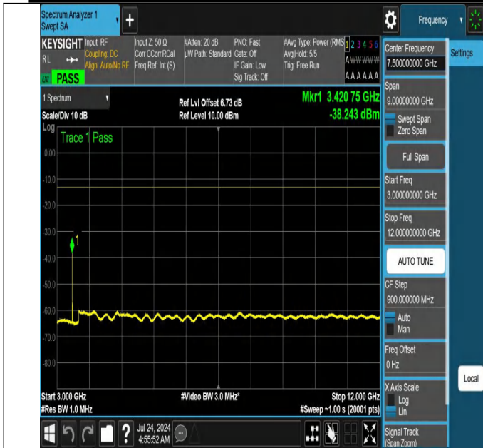
NTNV-N66-PC3-15-10-L-DFT-PI2BPSK-Edge_1RB_Left-3000-12000-Ant1-PASS
