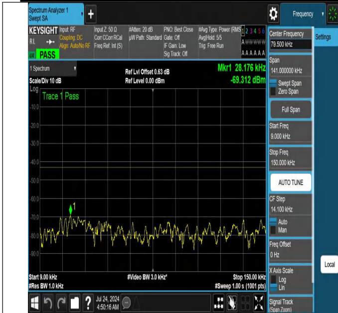
NTNV-N66-PC3-15-5-H-DFT-PI2BPSK-Edge_1RB_Left-0.009-0.15-Ant1-PASS
