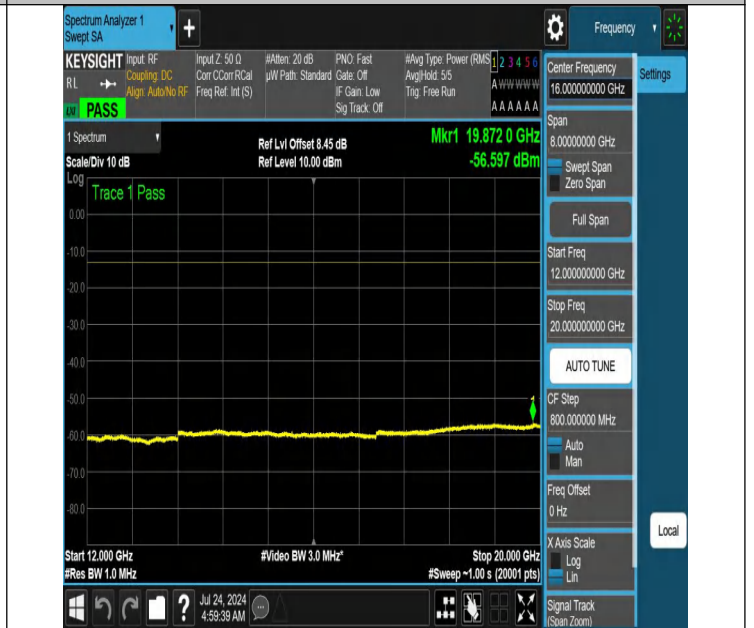
NTNV-N66-PC3-15-10-L-DFT-QPSK-Edge_1RB_Right-12000-20000-Ant1-PASS
