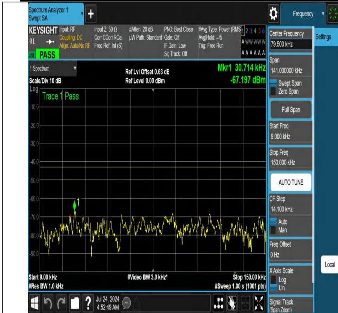
NTNV-N66-PC3-15-5-H-DFT-QPSK-Edge_1RB_Left-0.009-0.15-Ant1-PASS
