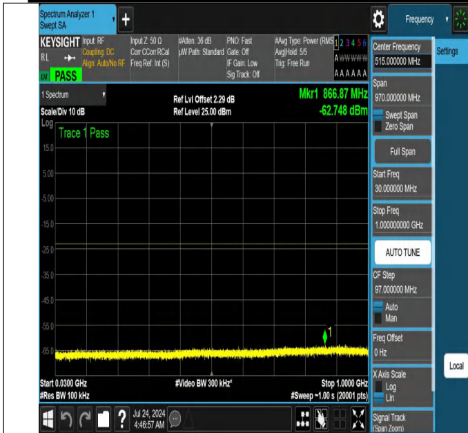
NTNV-N66-PC3-15-5-M-DFT-PI2BPSK-Edge_1RB_Right-30-100 0-Ant1-PASS
