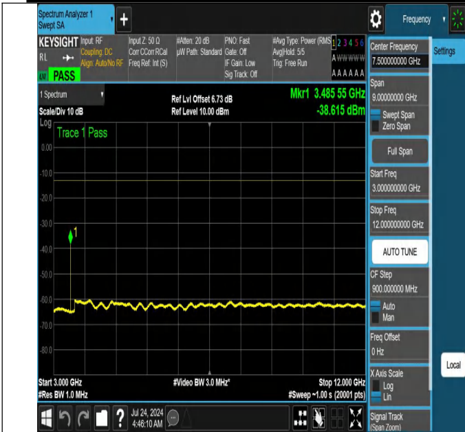
NTNV-N66-PC3-15-5-M-DFT-PI2BPSK-Edge_1RB_Left-3000-12000-Ant1-PASS
