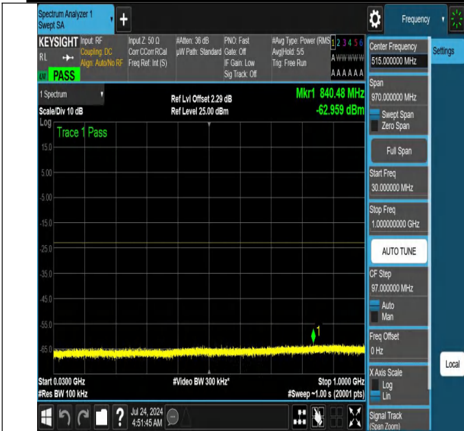
NTNV-N66-PC3-15-5-H-DFT-PI2BPSK-Edge_1RB_Right-30-100 0-Ant1-PASS
