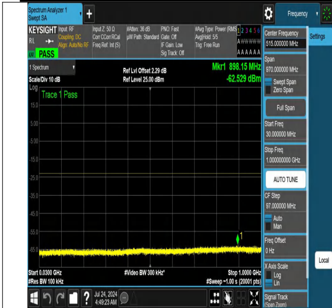
NTNV-N66-PC3-15-5-M-DFT-QPSK-Edge_1RB_Right-30-1000-A-nt1-PASS
