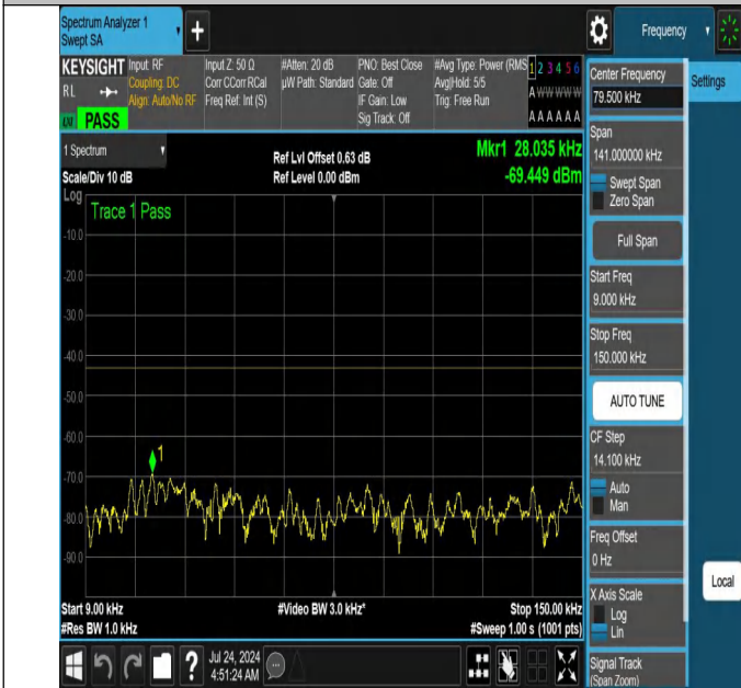
NTNV-N66-PC3-15-5-H-DFT-PI2BPSK-Edge_1RB_Right-0.009-0.15-Ant1-PASS
