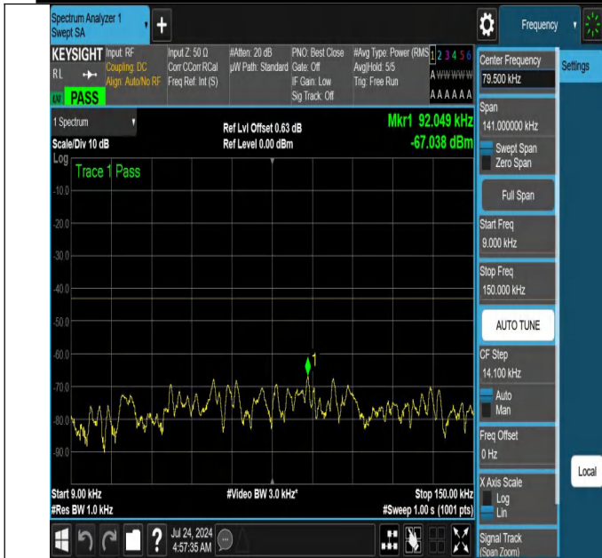
NTNV-N66-PC3-15-10-L-DFT-QPSK-Edge_1RB_Left-0.009-0.15-Ant1-PASS
