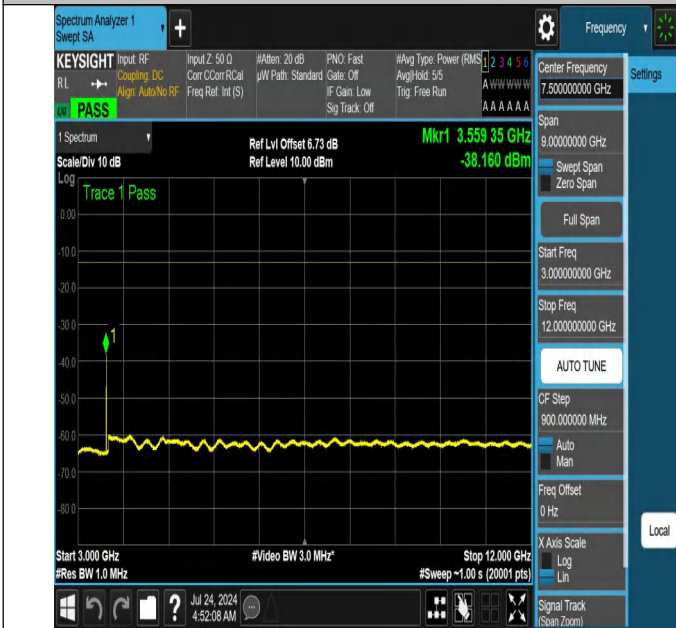
NTNV-N66-PC3-15-5-H-DFT-PI2BPSK-Edge_1RB_Right-3000-1 2000-Ant1-PASS
