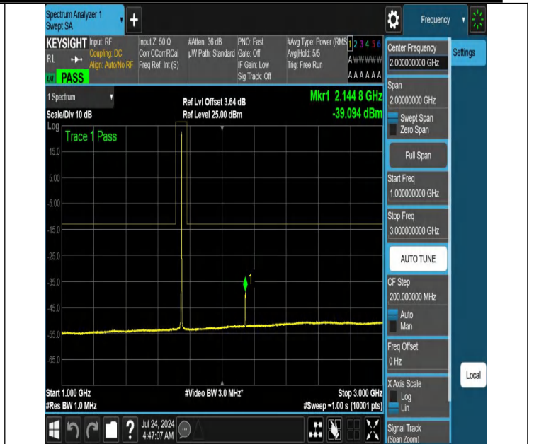
NTNV-N66-PC3-15-5-M-DFT-PI2BPSK-Edge_1RB_Right-1000-30 00-Ant1-PASS
