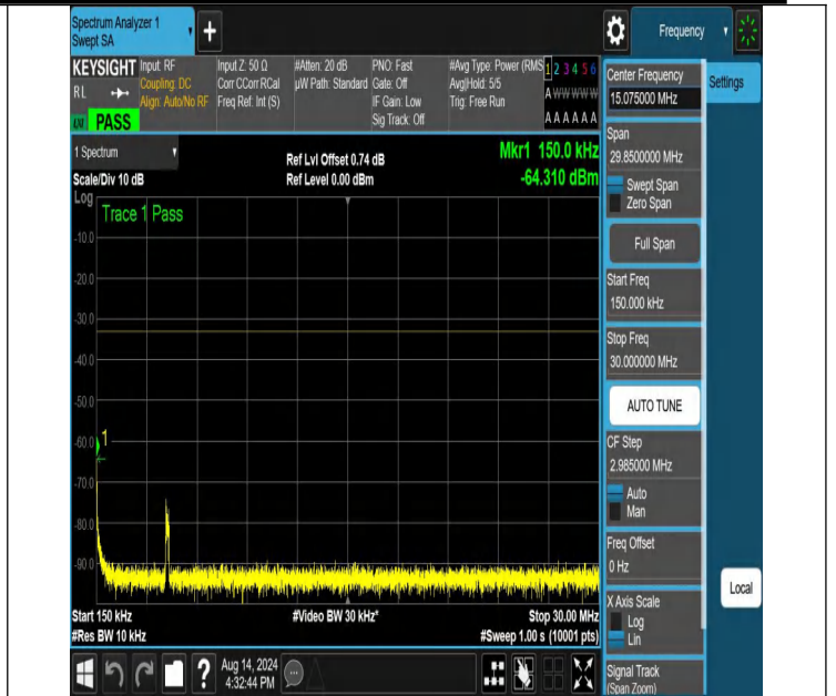
NTNV-N66-PC3-15-10-L-DFT-PI2BPSK-Edge_1RB_Left-0.15-30-Ant1-PASS
