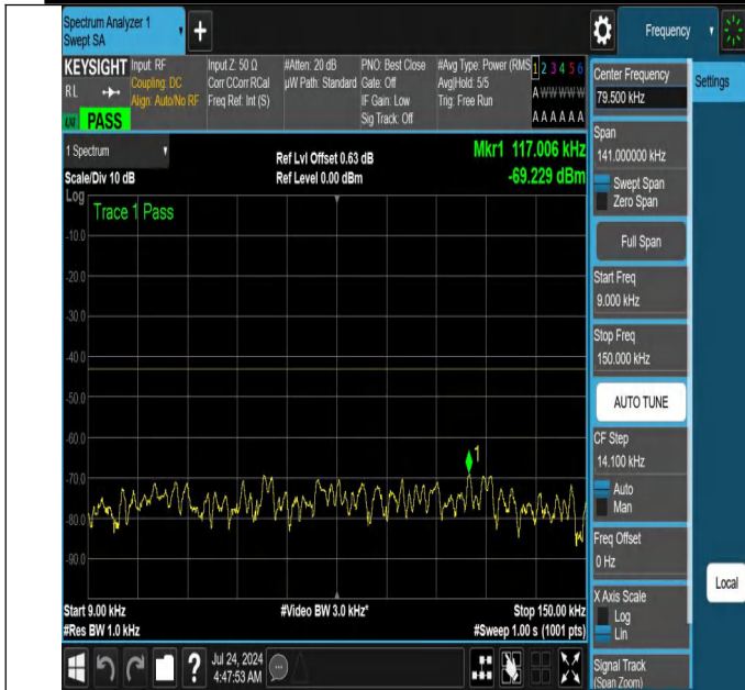
NTNV-N66-PC3-15-5-M-DFT-QPSK-Edge_1RB_Left-0.009-0.15-Ant1-PASS
