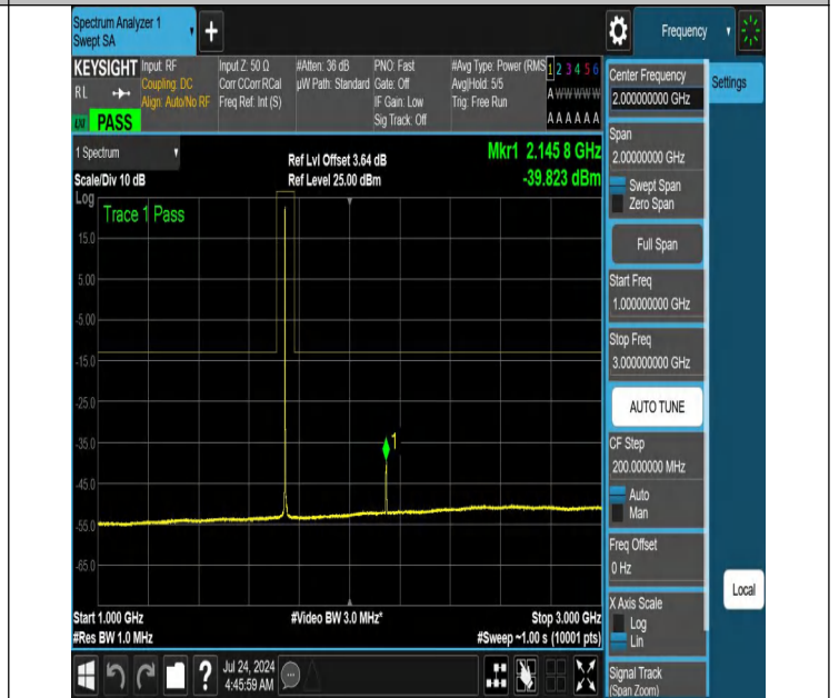
NTNV-N66-PC3-15-5-M-DFT-PI2BPSK-Edge_1RB_Left-1000-3000-Ant1-PASS
