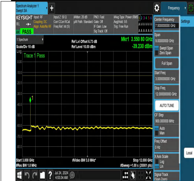
NTNV-N66-PC3-15-5-H-DFT-QPSK-Edge_1RB_Left-3000-12000 -Ant1-PASS
