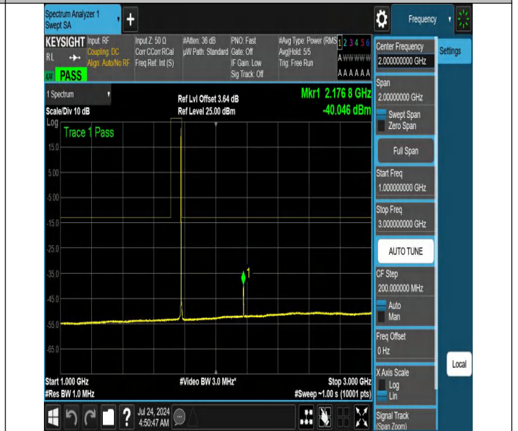
NTNV-N66-PC3-15-5-H-DFT-PI2BPSK-Edge_1RB_Left-1000-3000-Ant1-PASS
