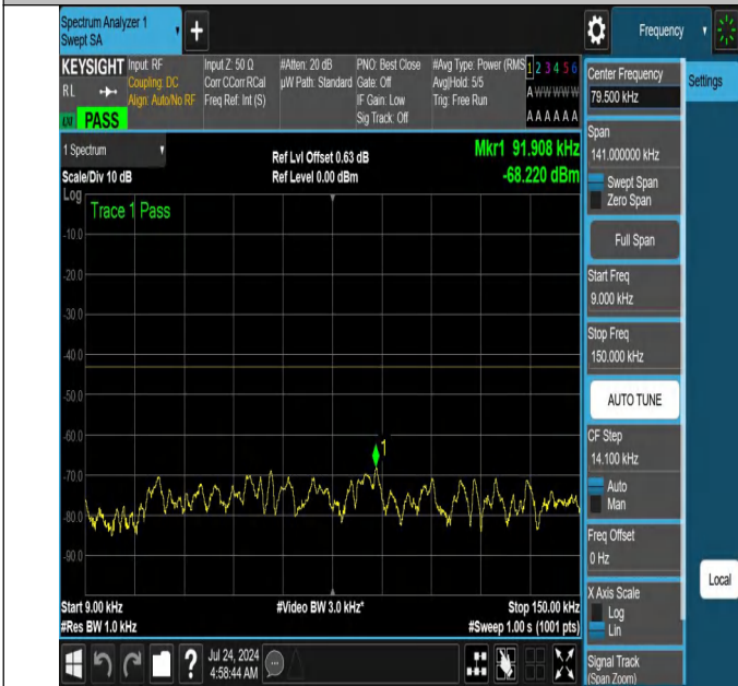
NTNV-N66-PC3-15-10-L-DFT-QPSK-Edge_1RB_Right-0.009-0.1 5-Ant1-PASS
