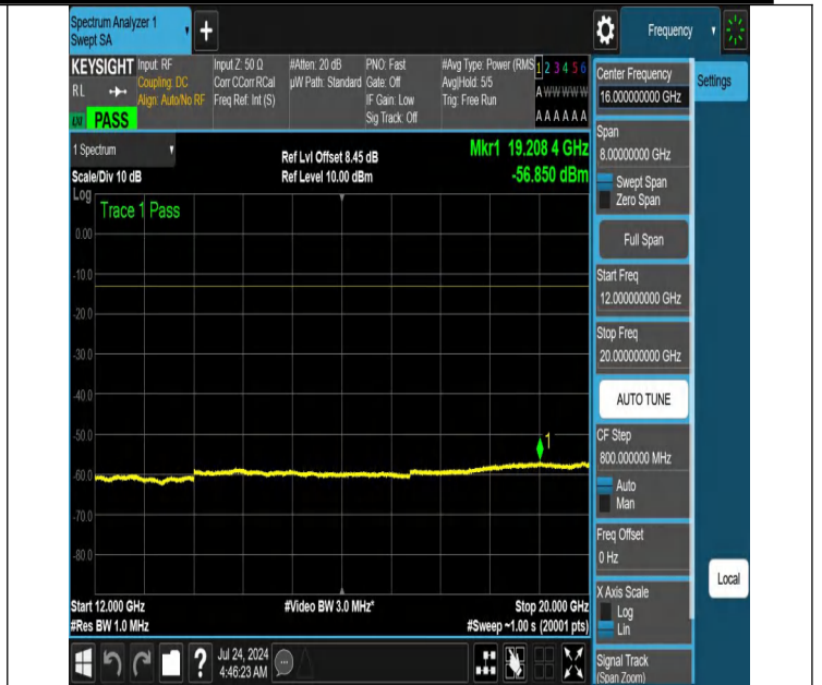
NTNV-N66-PC3-15-5-M-DFT-PI2BPSK-Edge_1RB_Left-12000-20000-Ant1-PASS
