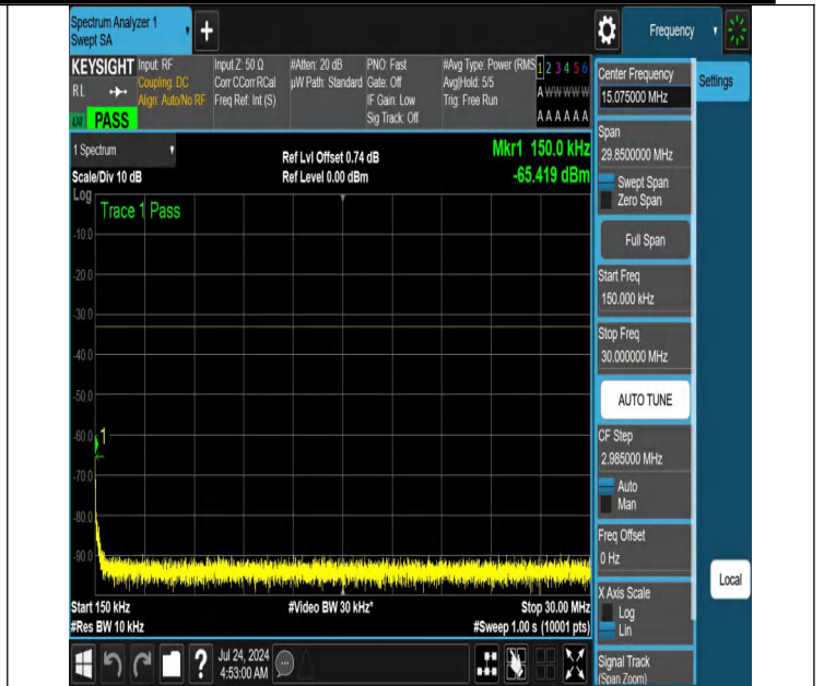
NTNV-N66-PC3-15-5-H-DFT-QPSK-Edge_1RB_Left-0.15-30-Ant1-PASS
