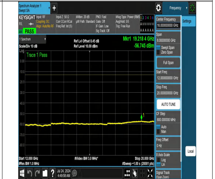
NTNV-N66-PC3-15-5-M-DFT-QPSK-Edge_1RB_Right-12000-20000-Ant1-PASS
