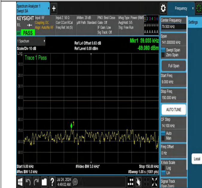
NTNV-N66-PC3-15-5-M-DFT-QPSK-Edge_1RB_Right-0.009-0.1 5-Ant1-PASS
