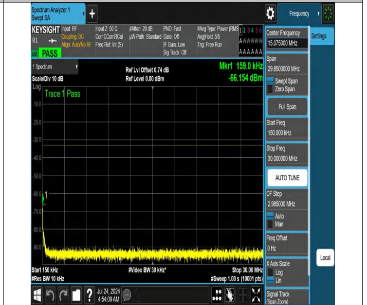
NTNV-N66-PC3-15-5-H-DFT-QPSK-Edge_1RB_Right-0.15-30-Ant 1-PASS
