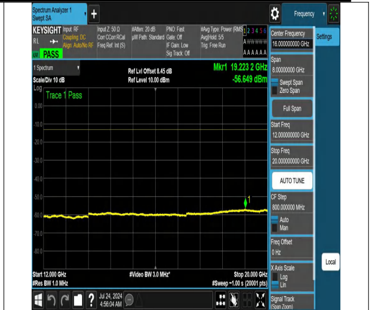
NTNV-N66-PC3-15-10-L-DFT-PI2BPSK-Edge_1RB_Left-12000-20000-Ant1-PASS
