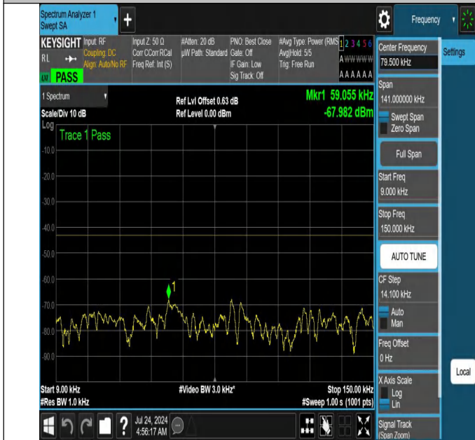
NTNV-N66-PC3-15-10-L-DFT-PI2BPSK-Edge_1RB_Right-0.009-0.15-Ant1-PASS
