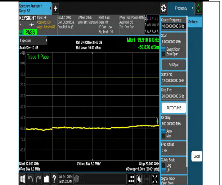
NTNV-N66-PC3-15-10-M-DFT-PI2BPSK-Edge_1RB_Left-12000-2 0000-Ant1-PASS
