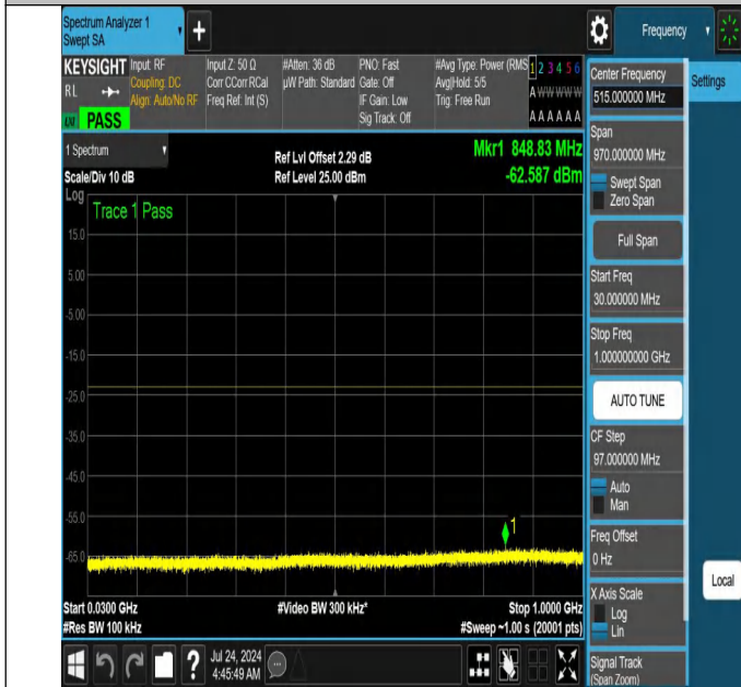
NTNV-N66-PC3-15-5-M-DFT-PI2BPSK-Edge_1RB_Left-30-1000-Ant1-PASS
