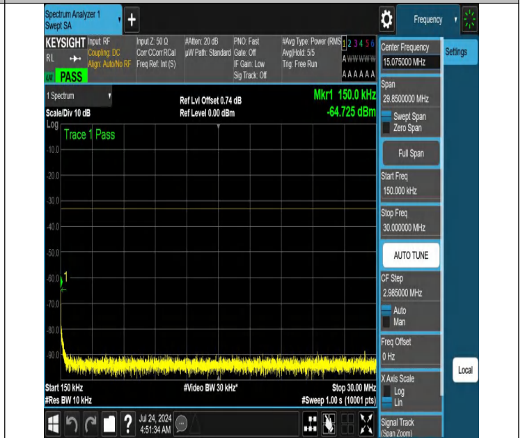
NTNV-N66-PC3-15-5-H-DFT-PI2BPSK-Edge_1RB_Right-0.15-30-Ant1-PASS
