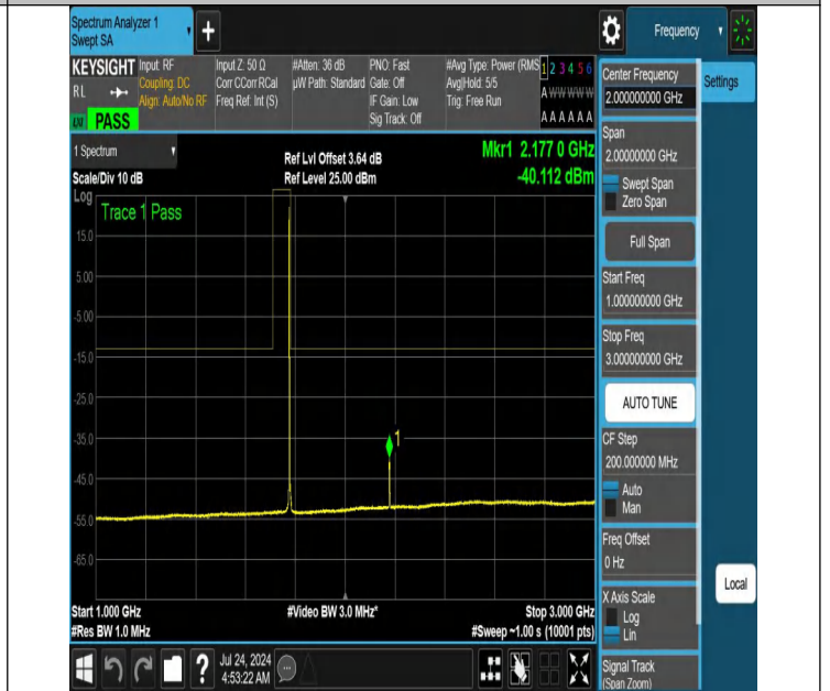
NTNV-N66-PC3-15-5-H-DFT-QPSK-Edge_1RB_Left-1000-3000-Ant1-PASS
