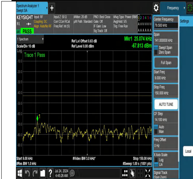
NTNV-N66-PC3-15-5-M-DFT-PI2BPSK-Edge_1RB_Left-0.009-0.15-Ant1-PASS
