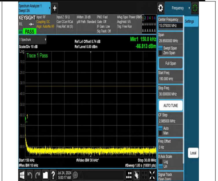
NTNV-N66-PC3-15-10-M-DFT-PI2BPSK-Edge_1RB_Left-0.15-30-Ant1-PASS
