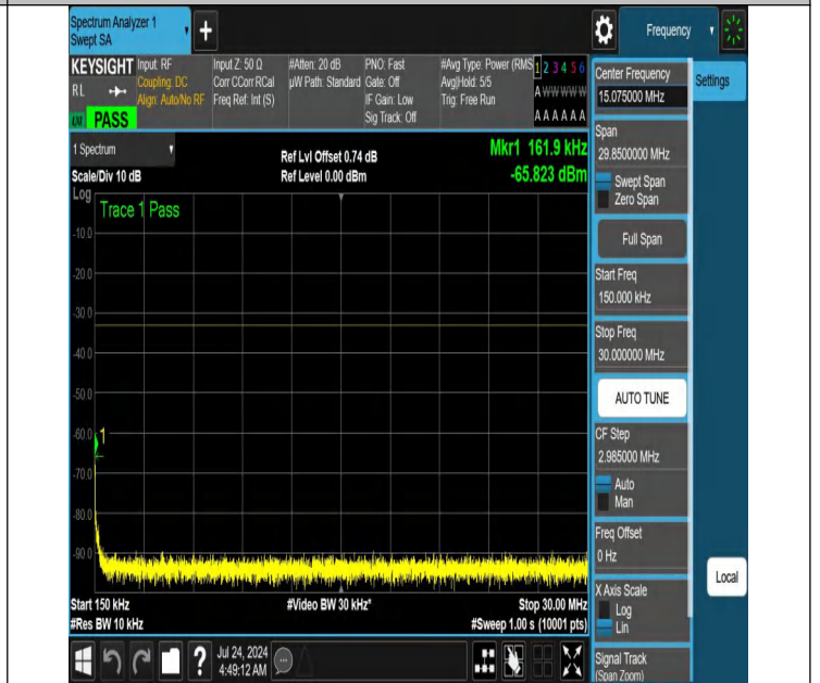
NTNV-N66-PC3-15-5-M-DFT-QPSK-Edge_1RB_Right-0.15-30-An t1-PASS
