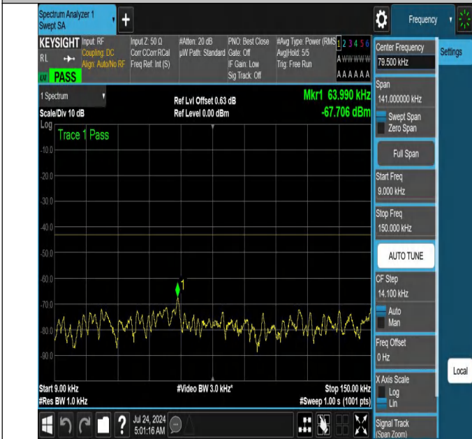
NTNV-N66-PC3-15-10-M-DFT-PI2BPSK-Edge_1RB_Right-0.009 -0.15-Ant1-PASS
