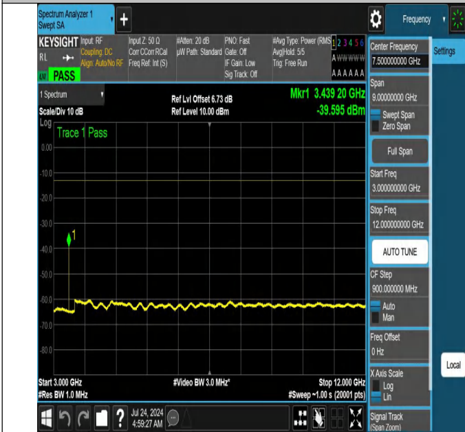
NTNV-N66-PC3-15-10-L-DFT-QPSK-Edge_1RB_Right-3000-12000-Ant1-PASS
