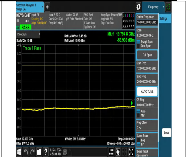
NTNV-N66-PC3-15-5-H-DFT-QPSK-Edge_1RB_Left-12000-20000 -Ant1-PASS
