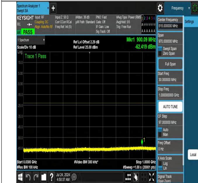
NTNV-N66-PC3-15-5-H-DFT-PI2BPSK-Edge_1RB_Left-30-1000-Ant1-PASS
