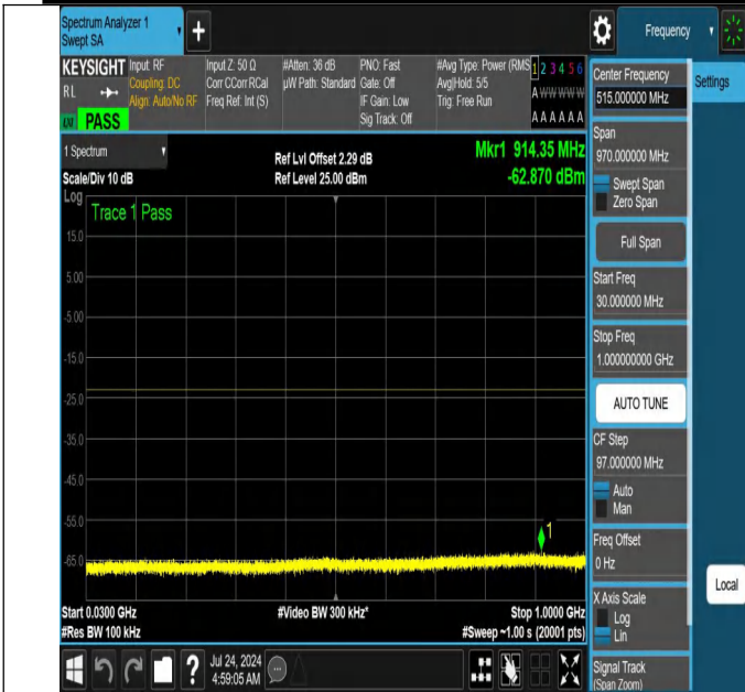
NTNV-N66-PC3-15-10-L-DFT-QPSK-Edge_1RB_Right-30-1000-Ant1-PASS
