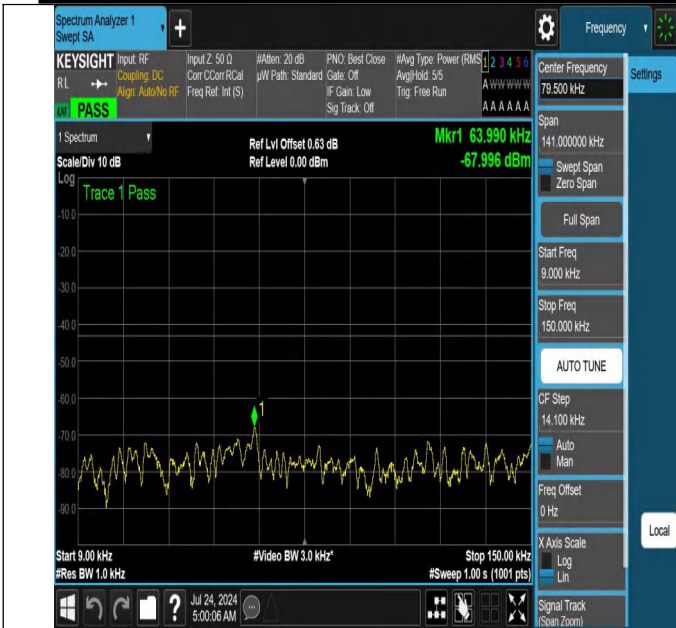
NTNV-N66-PC3-15-10-M-DFT-PI2BPSK-Edge_1RB_Left-0.009-0.15-Ant1-PASS
