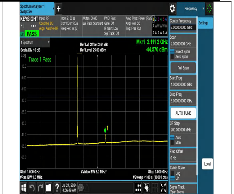
NTNV-N66-PC3-15-10-L-DFT-PI2BPSK-Edge_1RB_Right-1000-3000-Ant1-PASS
