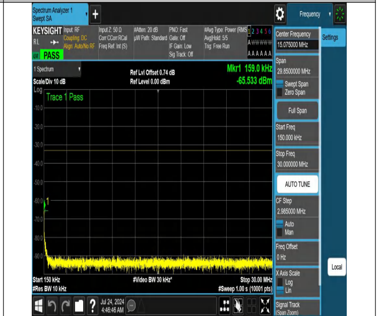
NTNV-N66-PC3-15-5-M-DFT-PI2BPSK-Edge_1RB_Right-0.15-30-Ant1-PASS
