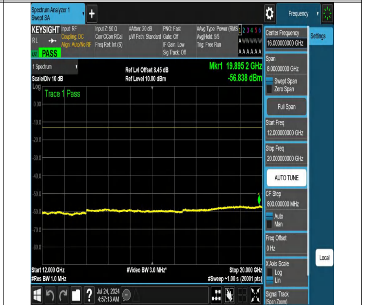
NTNV-N66-PC3-15-10-L-DFT-PI2BPSK-Edge_1RB_Right-12000-20000-Ant1-PASS
