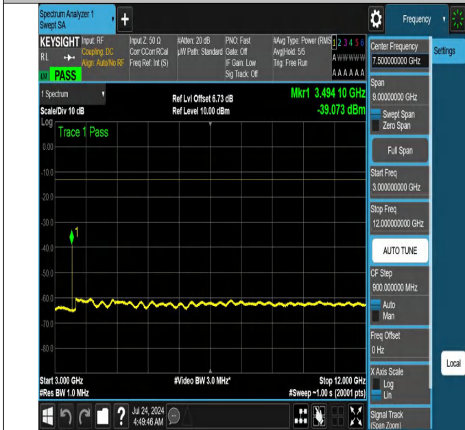
NTNV-N66-PC3-15-5-M-DFT-QPSK-Edge_1RB_Right-3000-12000-Ant1-PASS
