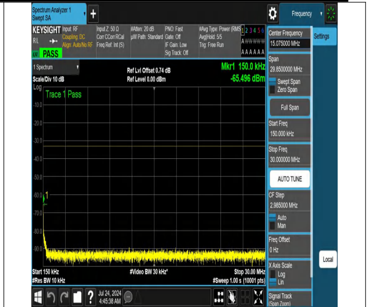
NTNV-N66-PC3-15-5-M-DFT-PI2BPSK-Edge_1RB_Left-0.15-30-Ant1-PASS
