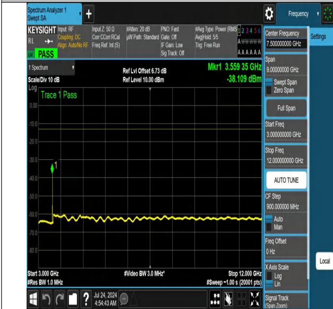
NTNV-N66-PC3-15-5-H-DFT-QPSK-Edge_1RB_Right-3000-1200 0-Ant1-PASS
