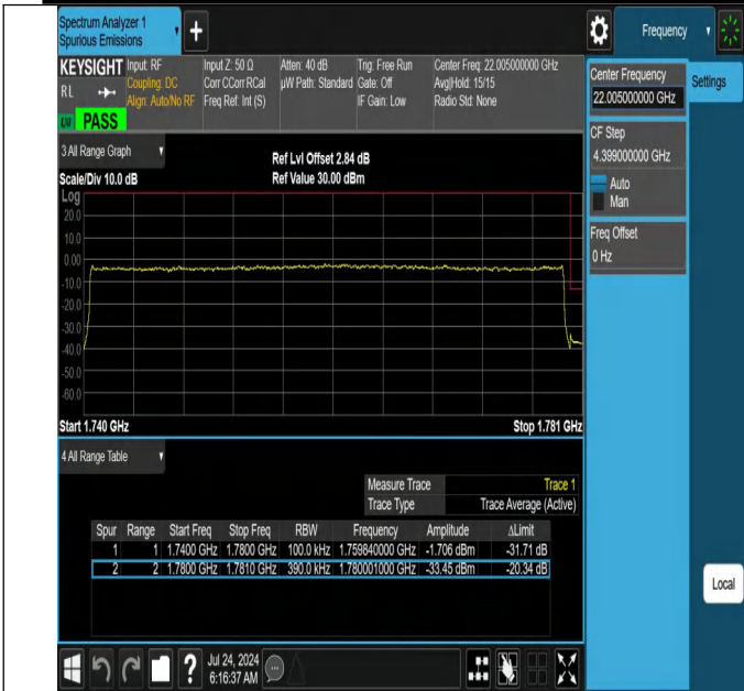
NTNV-N66-PC3-15-40-H-DFT-PI2BPSK-Outter_Full-Ant1-PASS
