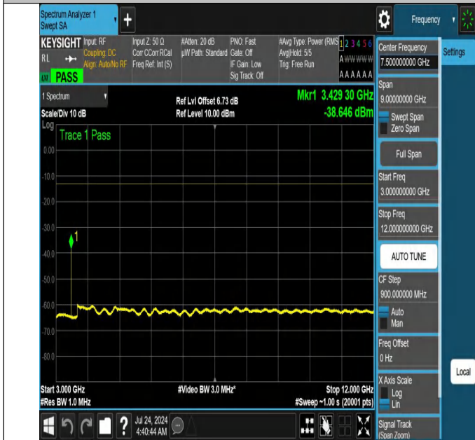
NTNV-N66-PC3-15-5-L-DFT-PI2BPSK-Edge_1RB_Right-3000-1 2000-Ant1-PASS
