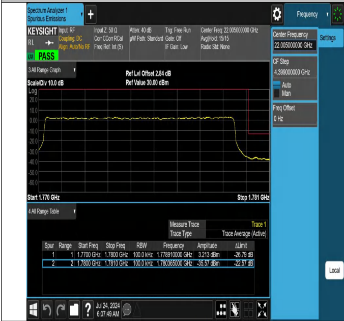
NTNV-N66-PC3-15-10-H-DFT-QPSK-Outer_Full-Ant1-PASS
