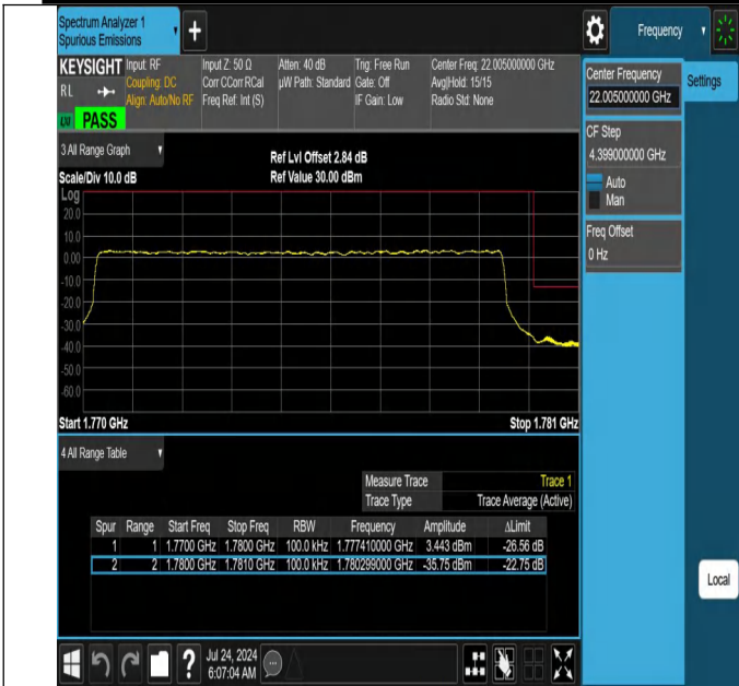
NTNV-N66-PC3-15-10-H-DFT-PI2BPSK-Outer_Full-Ant1-PASS
