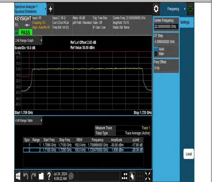
NTNV-N66-PC3-15-15-L-DFT-QPSK-Outer_Full-Ant1-PASS
