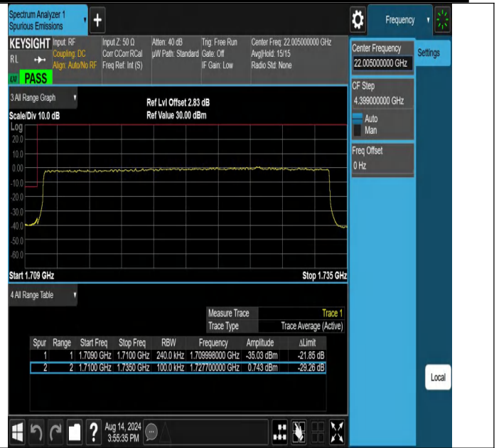
NTNV-N66-PC3-15-25-L-DFT-PI2BPSK-Outer_Full-Ant1-PASS
