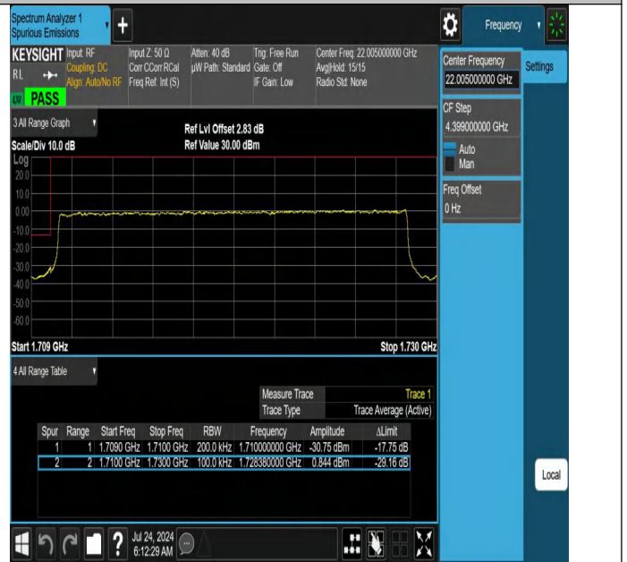
NTNV-N66-PC3-15-20-L-DFT-QPSK-Outer_Full-Ant1-PASS
