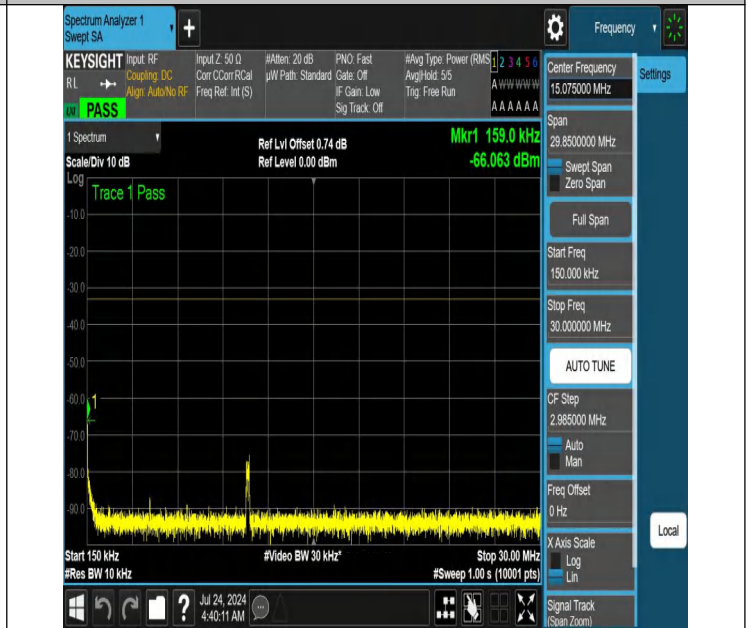
NTNV-N66-PC3-15-5-L-DFT-PI2BPSK-Edge_1RB_Right-0.15-30-Ant1-PASS
