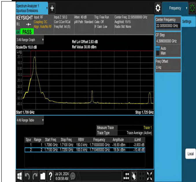
NTNV-N66-PC3-15-15-L-DFT-PI2BPSK-Edge_1RB_Left-Ant1-P ASS
