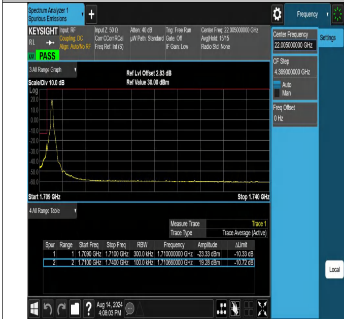
NTNV-N66-PC3-15-30-L-DFT-QPSK-Edge_1RB_Left-Ant1-PAS S
