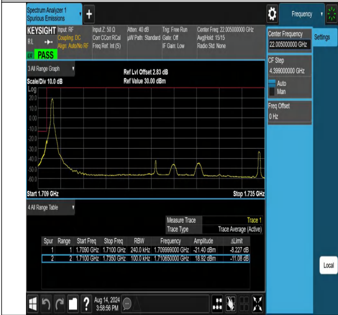
NTNV-N66-PC3-15-25-L-DFT-QPSK-Edge_1RB_Left-Ant1-PAS S
