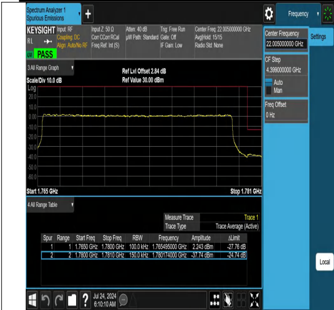
NTNV-N66-PC3-15-15-H-DFT-PI2BPSK-Outer_Full-Ant1-PASS
