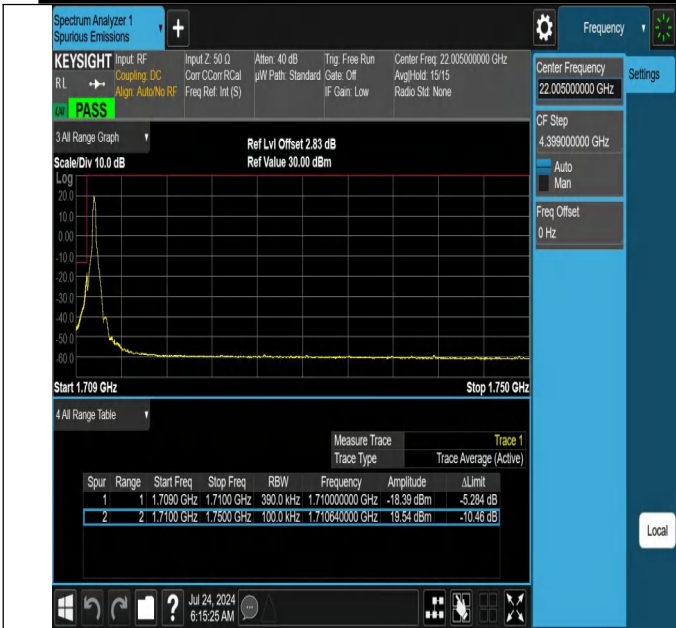
NTNV-N66-PC3-15-40-L-DFT-PI2BPSK-Edge_1RB_Left-Ant1-P ASS
