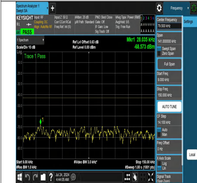
NTNV-N66-PC3-15-5-L-DFT-QPSK-Edge_1RB_Right-0.009-0.15 -Ant1-PASS
