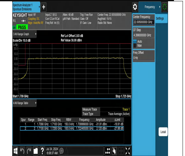
NTNV-N66-PC3-15-15-L-DFT-PI2BPSK-Outer_Full-Ant1-PASS
