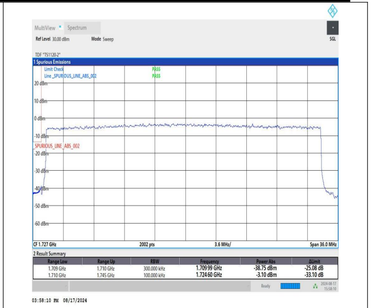
NTFN-n66-PC3-15-35-L-DFT-BPSK-Outer_Full-PASS
