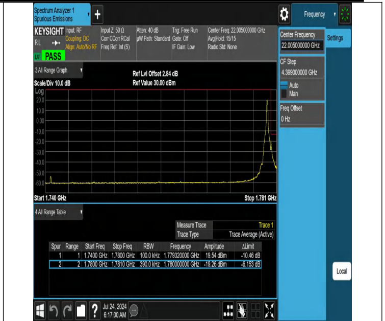
NTN-N66-PC3-15-40-H-DFT-PI2BPSK-Edge_1RB_Right-Ant1-PASS
