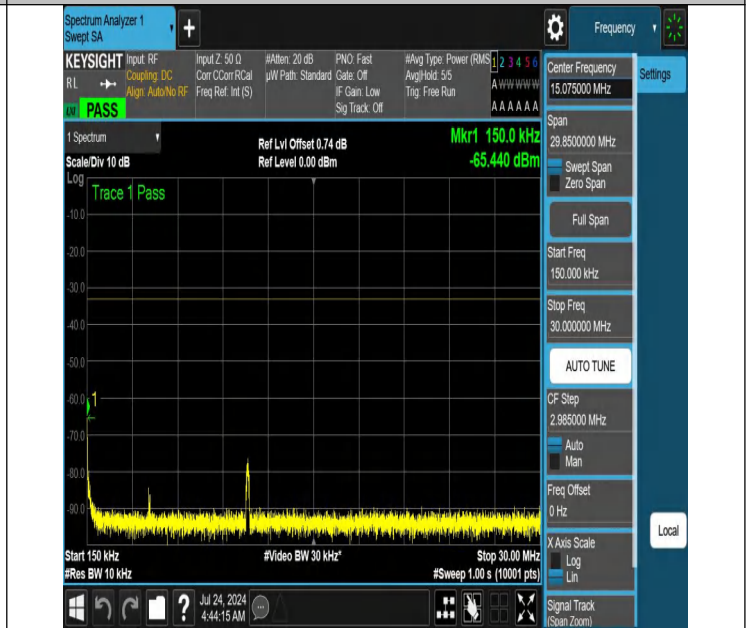
NTNV-N66-PC3-15-5-L-DFT-QPSK-Edge_1RB_Right-0.15-30-Ant 1-PASS
