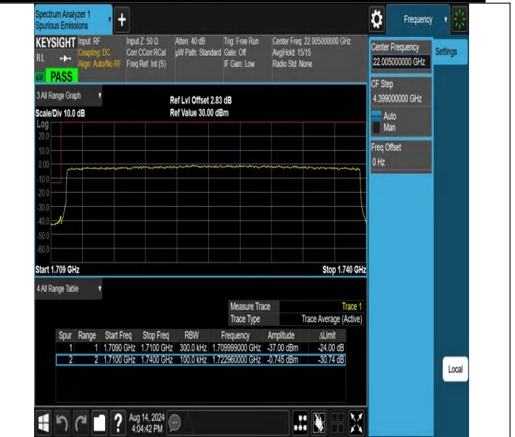
NTNV-N66-PC3-15-30-L-DFT-PI2BPSK-Outer_Full-Ant1-PASS
