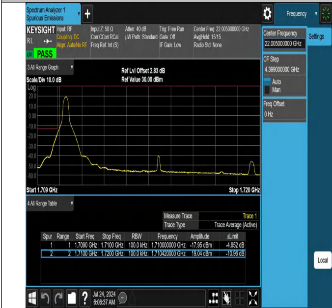
NTNV-N66-PC3-15-10-L-DFT-QPSK-Edge_1RB_Left-Ant1-PAS S
