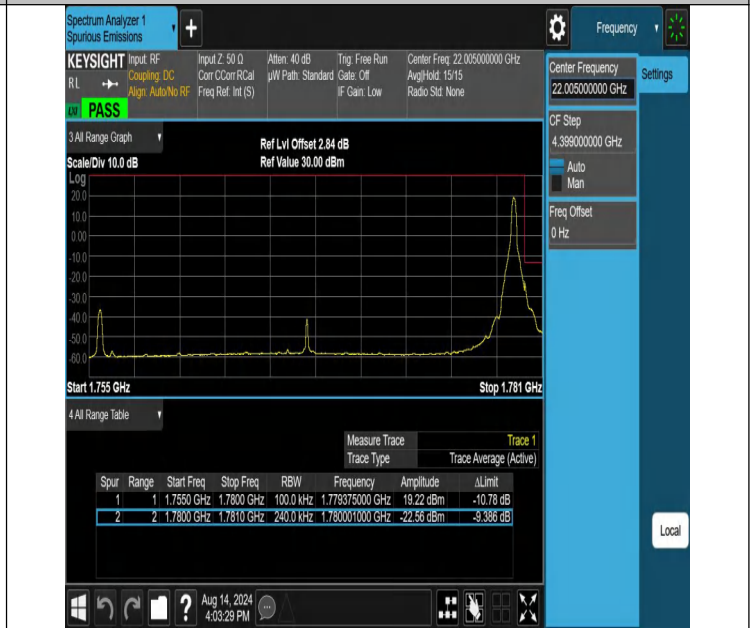
NTNV-N66-PC3-15-25-H-DFT-QPSK-Edge_1RB_Right-Ant1-PAS S
