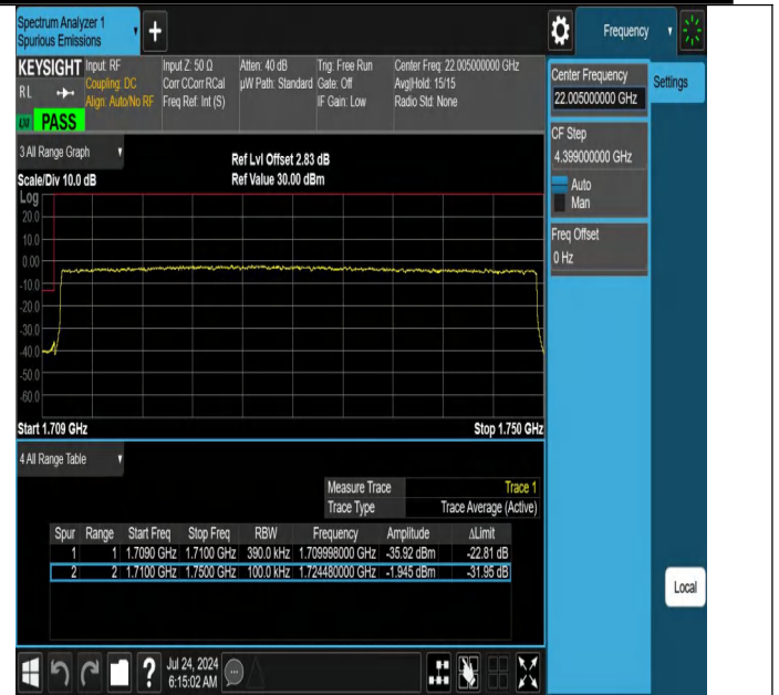
NTNV-N66-PC3-15-40-L-DFT-PI2BPSK-Outer_Full-Ant1-PASS
