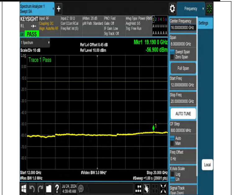
NTNV-N66-PC3-15-5-L-DFT-PI2BPSK-Edge_1RB_Left-12000-20000-Ant1-PASS
