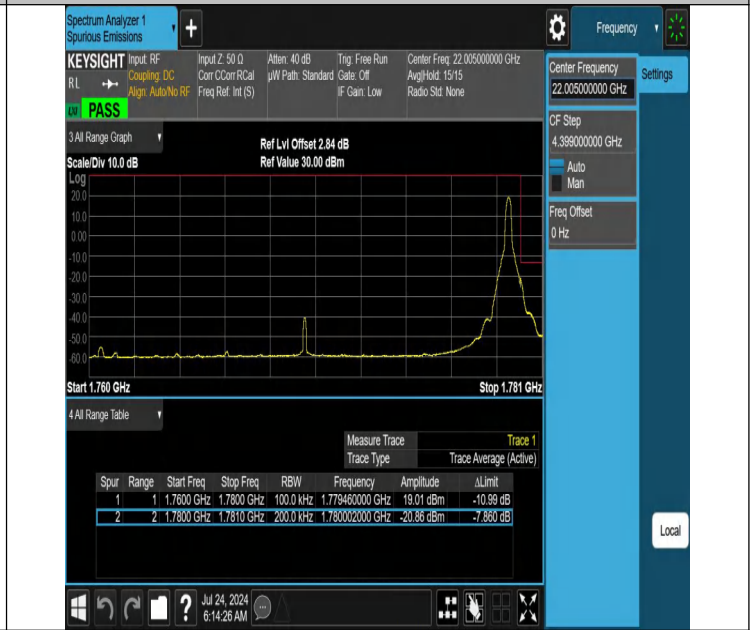
NTN-N66-PC3-15-20-H-DFT-QPSK-Edge_1RB_Right-Ant1-PASS
