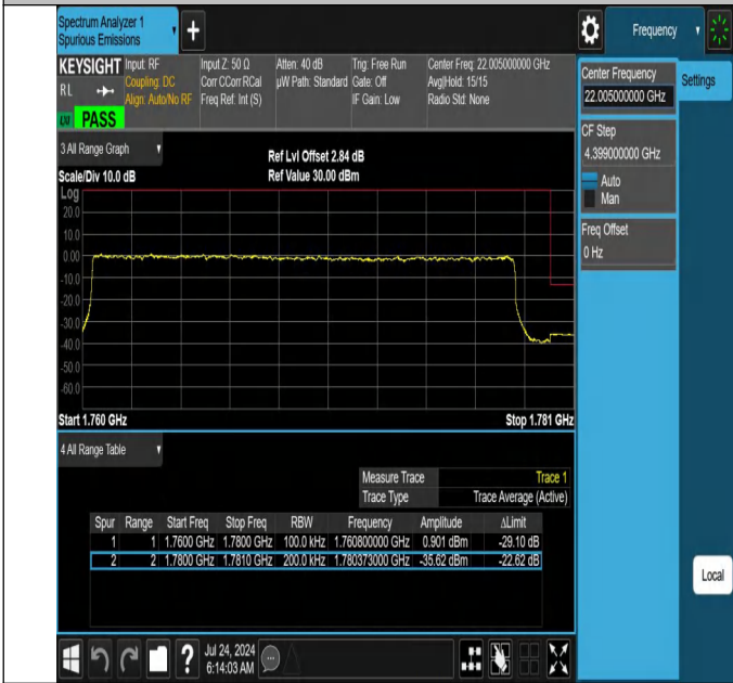
NTNV-N66-PC3-15-20-H-DFT-QPSK-Outer_Full-Ant1-PASS
