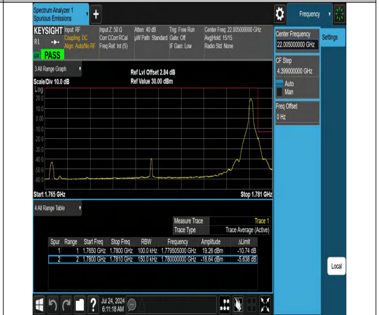
NTN-N66-PC3-15-15-H-DFT-QPSK-Edge_1RB_Right-Ant1-PASS
