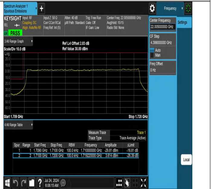
NTNV-N66-PC3-15-10-L-DFT-QPSK-Outer_Full-Ant1-PASS
