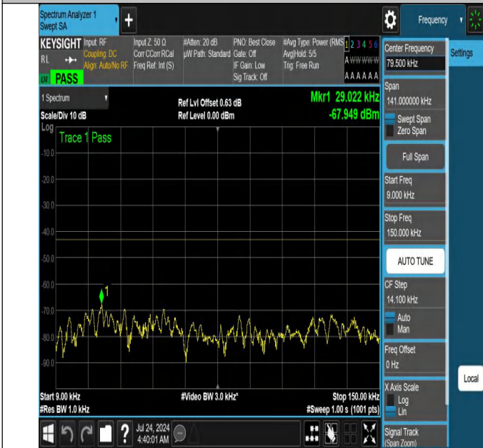
NTNV-N66-PC3-15-5-L-DFT-PI2BPSK-Edge_1RB_Right-0.009-0.15-Ant1-PASS
