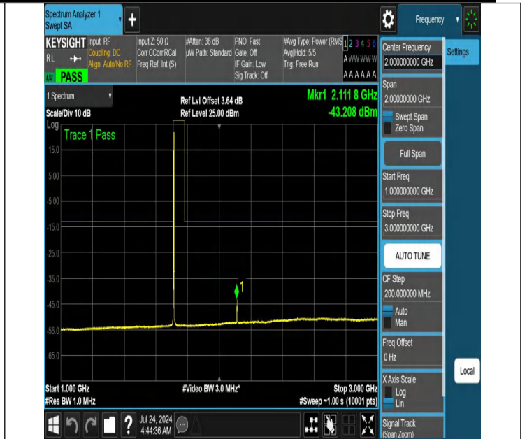
NTNV-N66-PC3-15-5-L-DFT-QPSK-Edge_1RB_Right-1000-3000- Ant1-PASS
