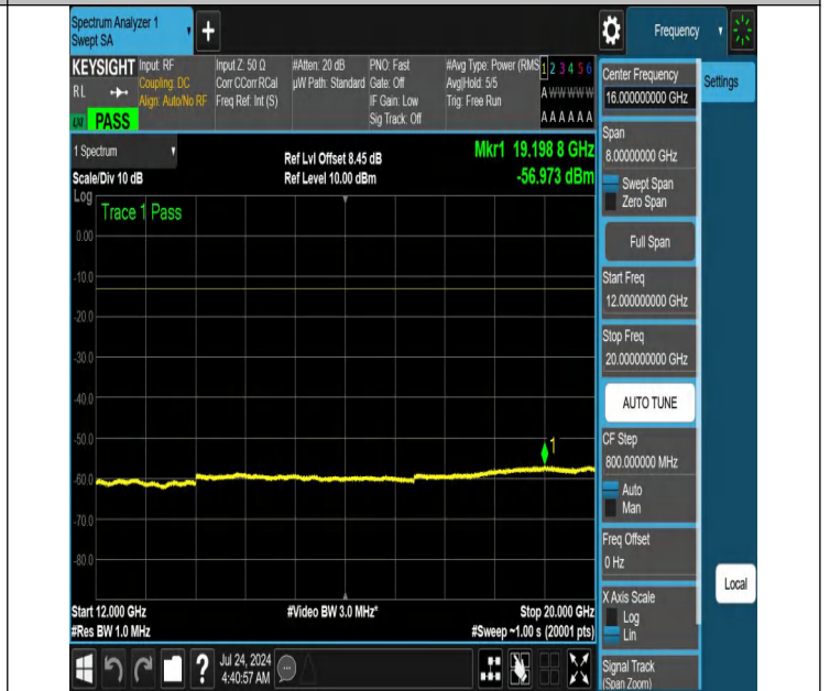
NTNV-N66-PC3-15-5-L-DFT-PI2BPSK-Edge_1RB_Right-12000-2 0000-Ant1-PASS
