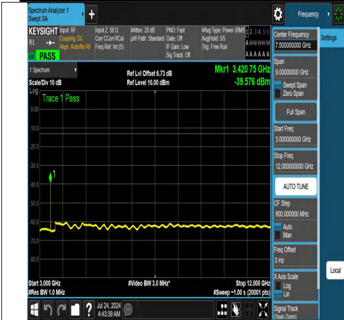
NTNV-N66-PC3-15-5-L-DFT-QPSK-Edge_1RB_Left-3000-12000- Ant1-PASS
