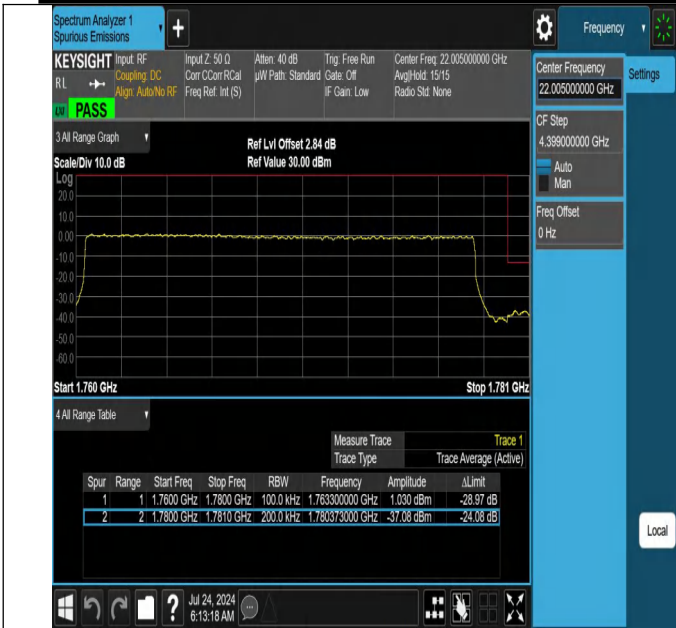
NTNV-N66-PC3-15-20-H-DFT-PI2BPSK-Outer_Full-Ant1-PASS
