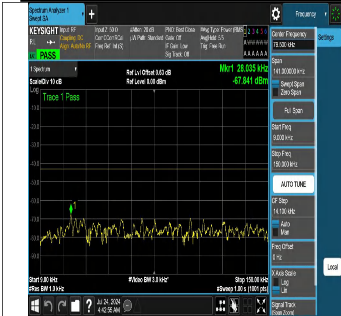
NTNV-N66-PC3-15-5-L-DFT-QPSK-Edge_1RB_Left-0.009-0.15-Ant1-PASS
