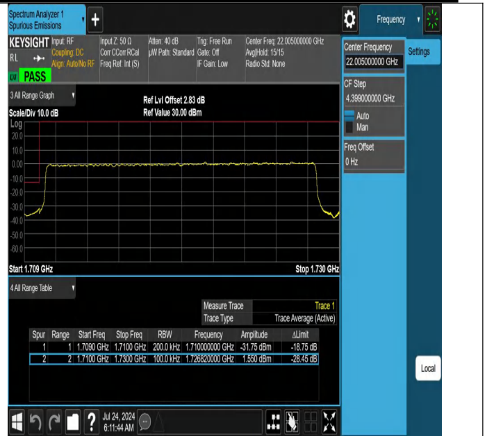
NTNV-N66-PC3-15-20-L-DFT-PI2BPSK-Outer_Full-Ant1-PASS
