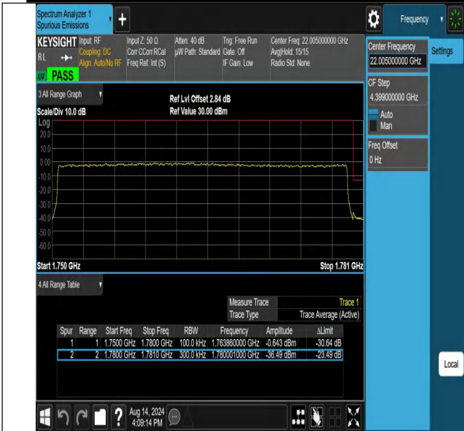
NTNV-N66-PC3-15-30-H-DFT-PI2BPSK-Outer_Full-Ant1-PASS
