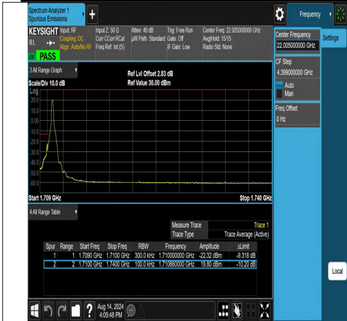
NTNV-N66-PC3-15-30-L-DFT-PI2BPSK-Edge_1RB_Left-Ant1-P ASS
