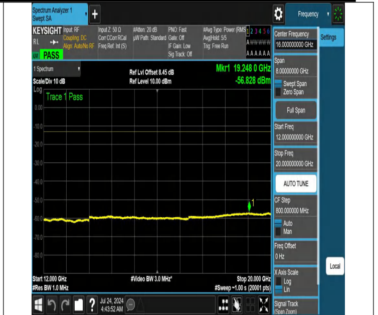
NTNV-N66-PC3-15-5-L-DFT-QPSK-Edge_1RB_Left-12000-20000 -Ant1-PASS
