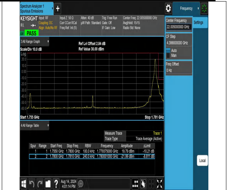
NTNV-N66-PC3-15-25-H-DFT-PI2BPSK-Edge_1RB_Right-Ant1-P ASS
