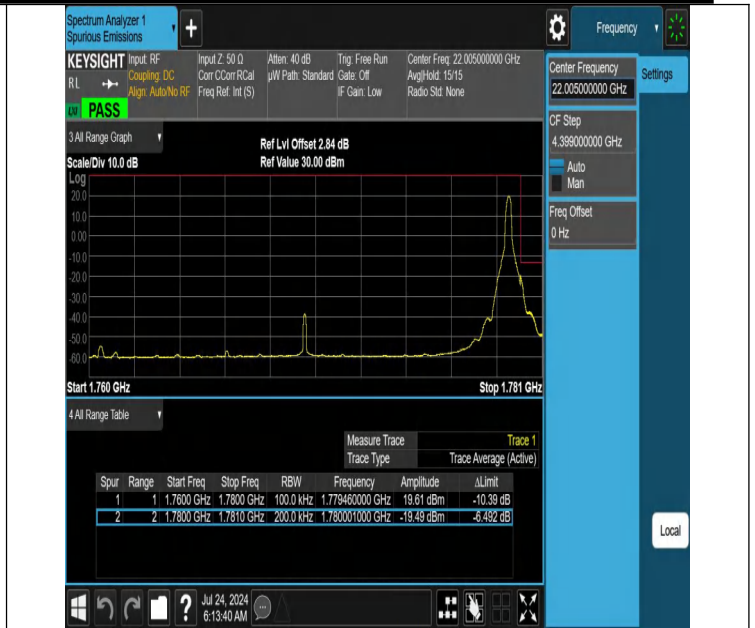
NTN-N66-PC3-15-20-H-DFT-PI2BPSK-Edge_1RB_Right-Ant1-PASS
