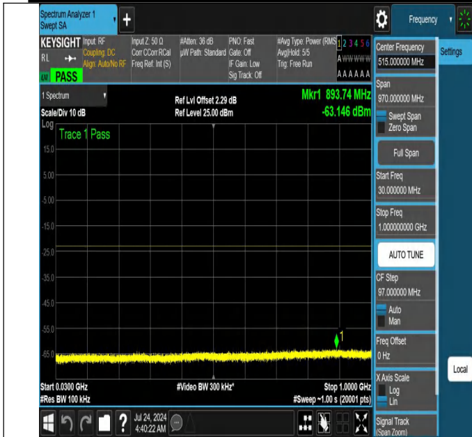
NTNV-N66-PC3-15-5-L-DFT-PI2BPSK-Edge_1RB_Right-30-100 0-Ant1-PASS
