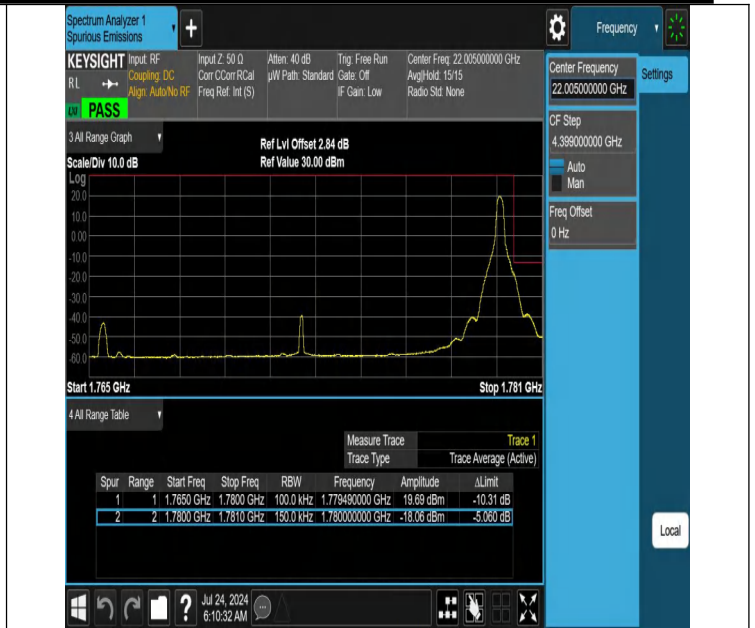
NTN-N66-PC3-15-15-H-DFT-PI2BPSK-Edge_1RB_Right-Ant1-PASS
