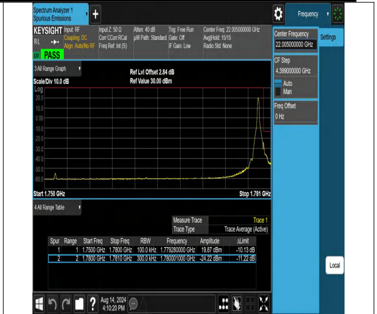
NTNV-N66-PC3-15-30-H-DFT-PI2BPSK-Edge_1RB_Right-Ant1-PASS
