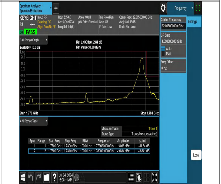
NTNV-N66-PC3-15-10-H-DFT-QPSK-Edge_1RB_Right-Ant1-PASS
