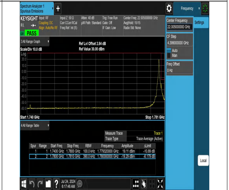
NTN-N66-PC3-15-40-H-DFT-QPSK-Edge_1RB_Right-Ant1-PASS
