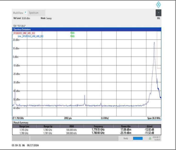
NNTV-n66-PC3-15-35-H-DFT-QPSK-Edge_1RB_Right-PASS
