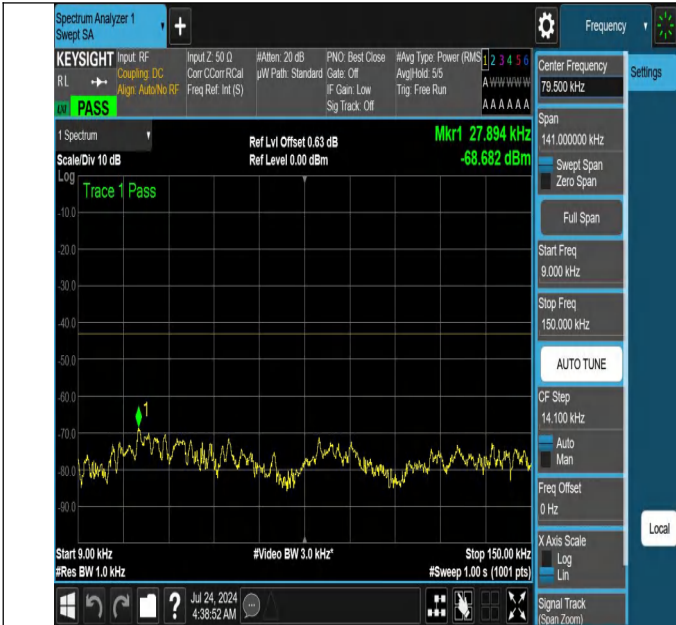
NTNV-N66-PC3-15-5-L-DFT-PI2BPSK-Edge_1RB_Left-0.009-0.1 5-Ant1-PASS
