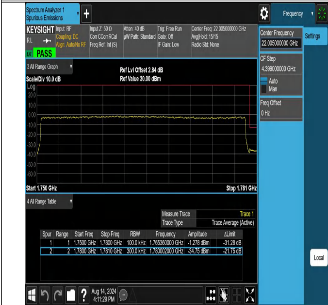
NTNV-N66-PC3-15-30-H-DFT-QPSK-Outer_Full-Ant1-PASS
