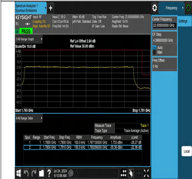
NTNV-N66-PC3-15-15-H-DFT-QPSK-Outer_Full-Ant1-PASS
