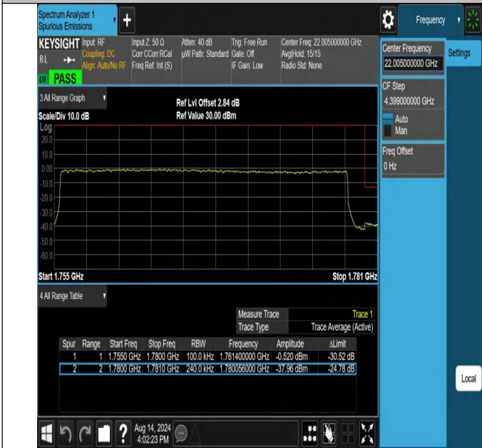
NTNV-N66-PC3-15-25-H-DFT-QPSK-Outter_Full-Ant1-PASS
