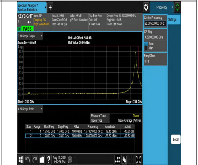
NTNV-N66-PC3-15-30-H-DFT-QPSK-Edge_1RB_Right-Ant1-PASS
