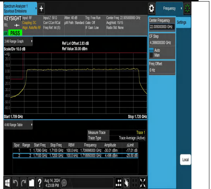
NTNV-N66-PC3-15-10-L-DFT-PI2BPSK-Outer_Full-Ant1-PASS
