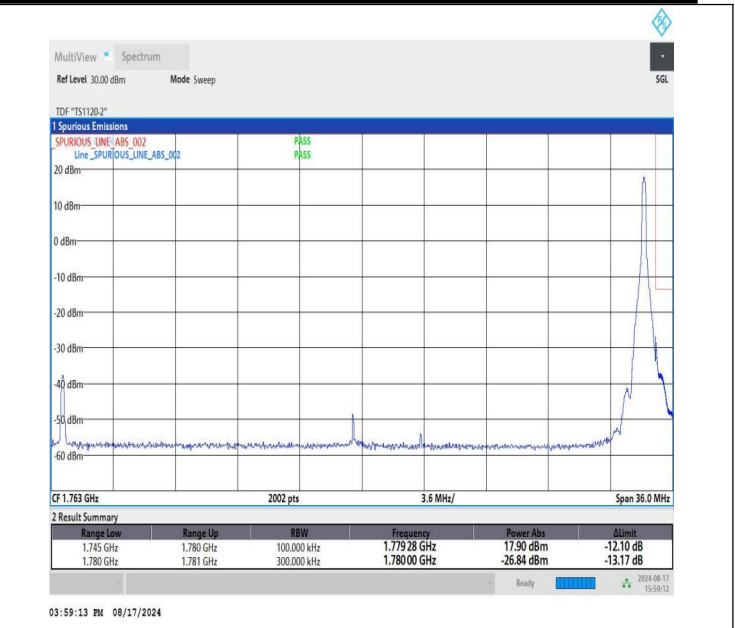
NNTV-n66-PC3-15-35-H-DFT-BPSK-Edge_1RB_Right-PASS
