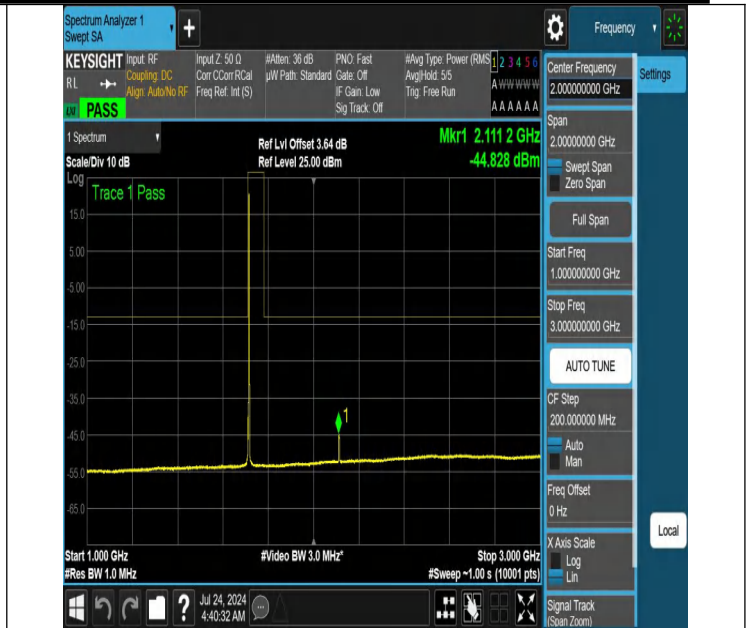
NTNV-N66-PC3-15-5-L-DFT-PI2BPSK-Edge_1RB_Right-1000-30 00-Ant1-PASS
