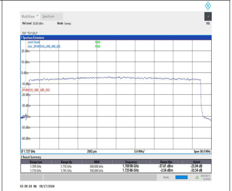
NTFN-n66-PC3-15-35-L-DFT-QPSK-Outer_Full-PASS
