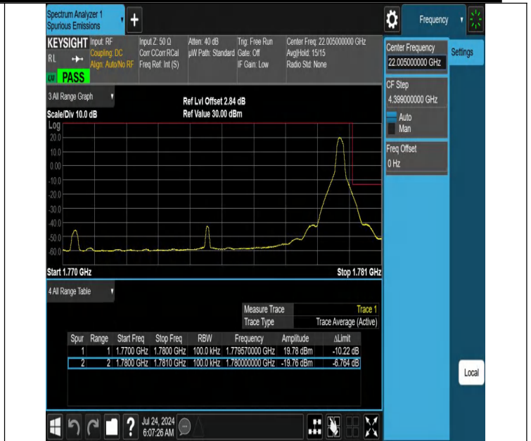
NTNV-N66-PC3-15-10-H-DFT-PI2BPSK-Edge_1RB_Right-Ant1-PASS
