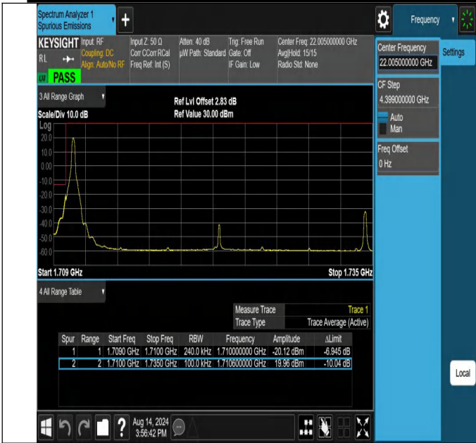
NTNV-N66-PC3-15-25-L-DFT-PI2BPSK-Edge_1RB_Left-Ant1-P ASS
