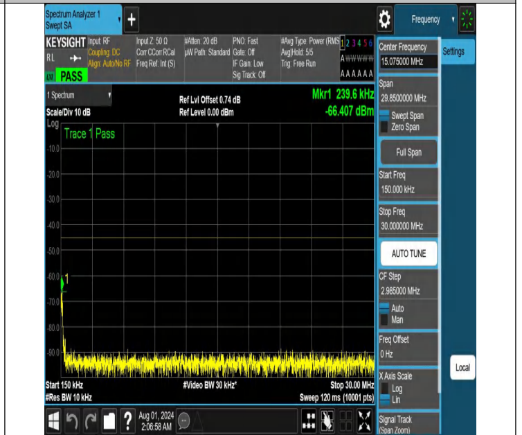
NTNV-N41-PC2-30-60-H-DFT-QPSK-Edge_1RB_Right-0.15-30-A nt1-PASS
