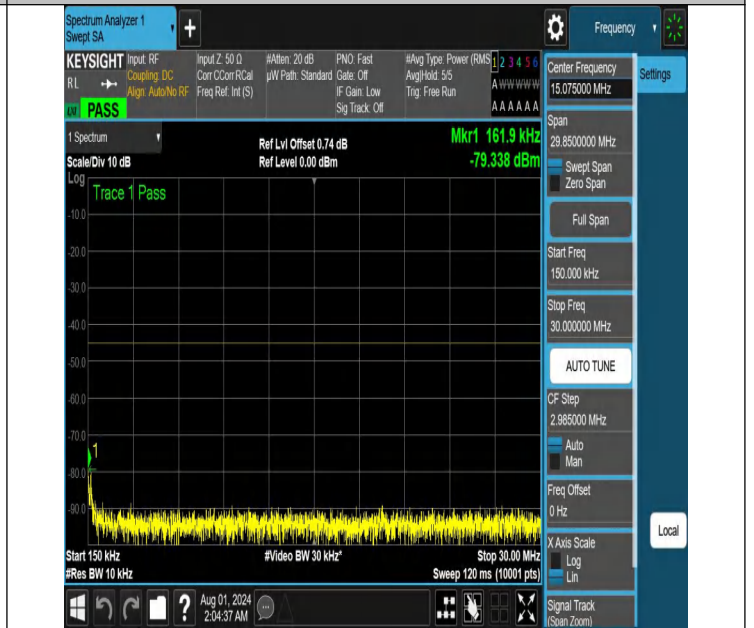
NTNV-N41-PC2-30-60-H-DFT-PI2BPSK-Edge_1RB_Right-0.15-3 0-Ant1-PASS
