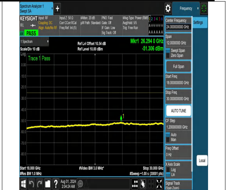
NTNV-N41-PC2-30-60-H-DFT-PI2BPSK-Edge_1RB_Left-18000-3 0000-Ant1-PASS
