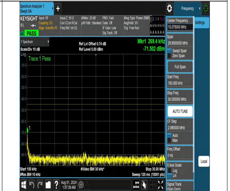
NTNV-N41-PC2-30-60-L-DFT-QPSK-Edge_1RB_Right-0.15-30-A nt1-PASS
