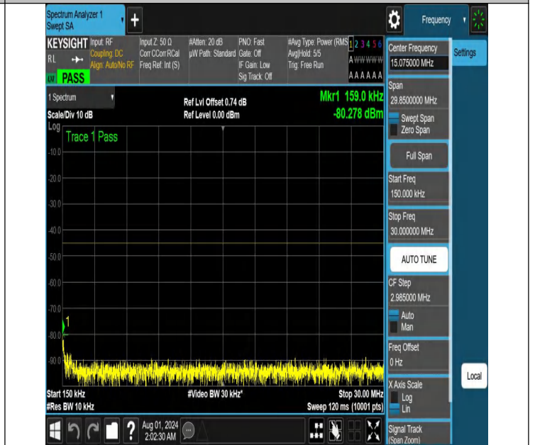
NTNV-N41-PC2-30-60-M-DFT-QPSK-Edge_1RB_Right-0.15-30-A nt1-PASS
