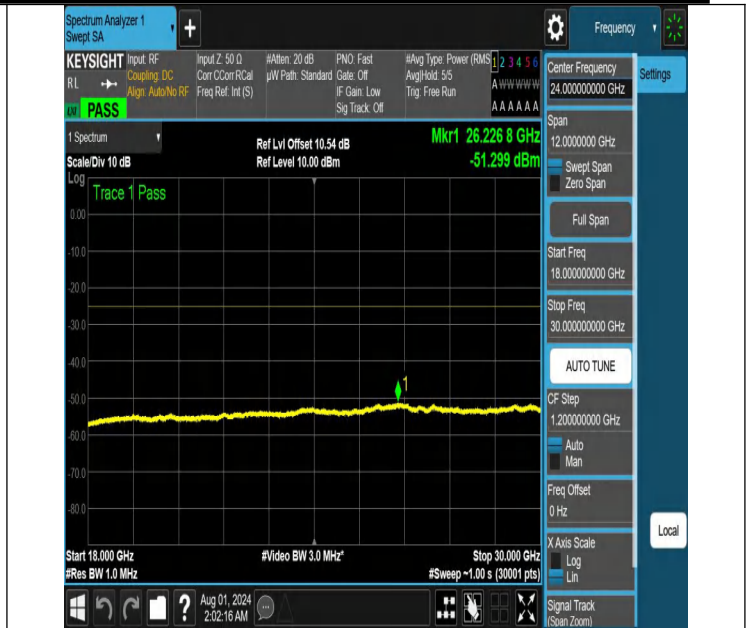
NTNV-N41-PC2-30-60-M-DFT-QPSK-Edge_1RB_Left-18000-300 00-Ant1-PASS
