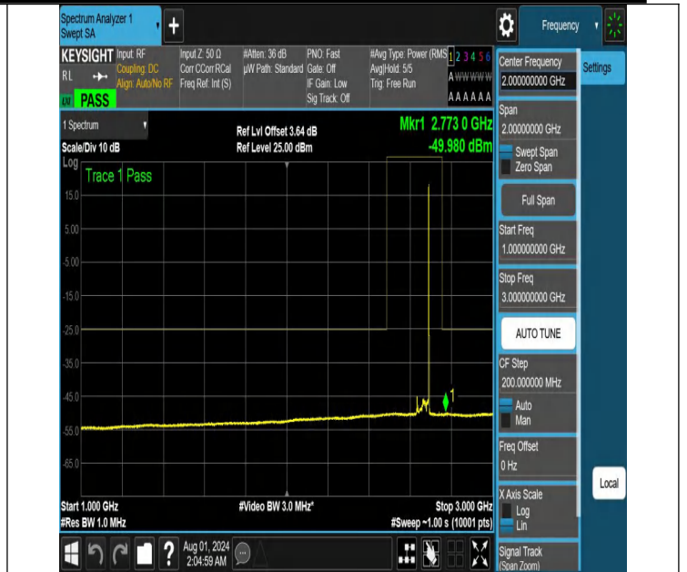
NTNV-N41-PC2-30-60-H-DFT-PI2BPSK-Edge_1RB_Right-1000-3000-Ant1-PASS
