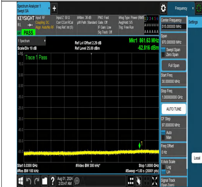
NTNV-N41-PC2-30-60-H-DFT-PI2BPSK-Edge_1RB_Left-30-1000-Ant1-PASS
