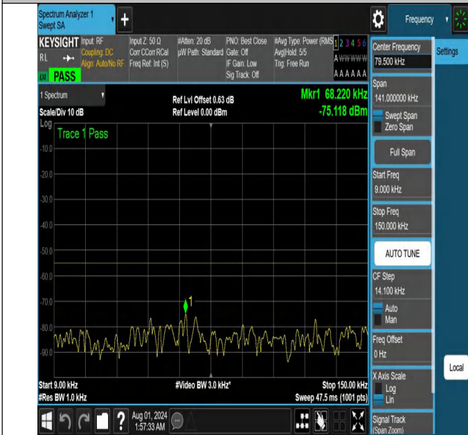
NTNV-N41-PC2-30-60-L-DFT-QPSK-Edge_1RB_Right-0.009-0.1 5-Ant1-PASS
