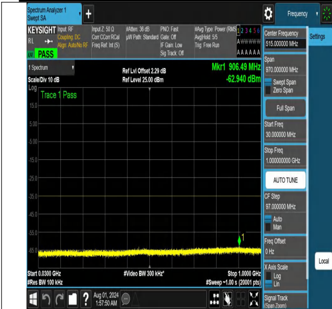
NTNV-N41-PC2-30-60-L-DFT-QPSK-Edge_1RB_Right-30-1000-Ant1-PASS
