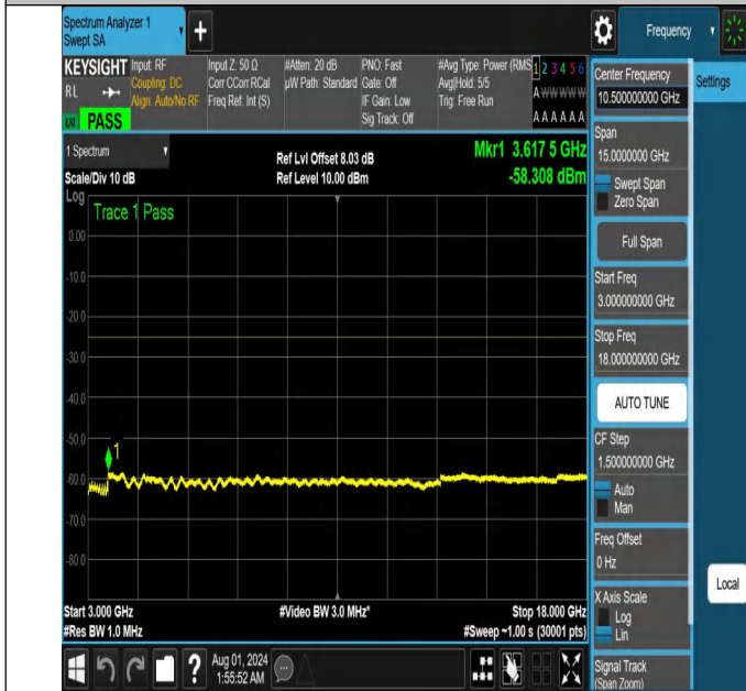
NTNV-N41-PC2-30-60-L-DFT-PI2BPSK-Edge_1RB_Right-3000-18000-Ant1-PASS
