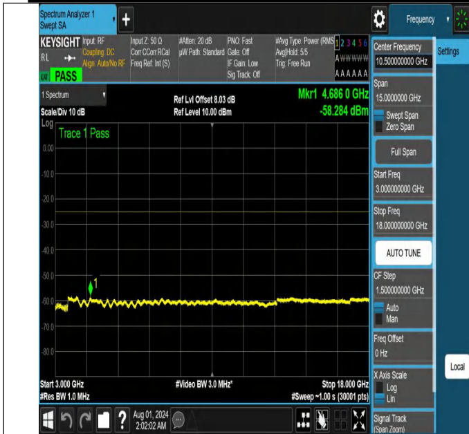
NTNV-N41-PC2-30-60-M-DFT-QPSK-Edge_1RB_Left-3000-1800 0-Ant1-PASS
