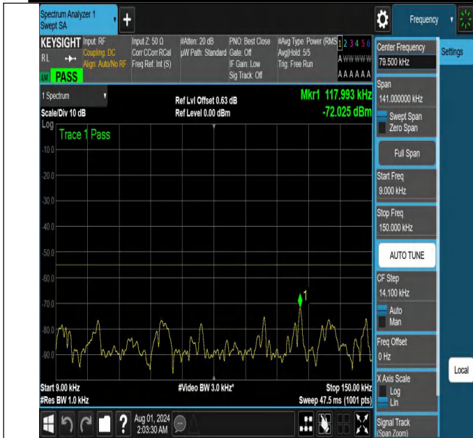
NTNV-N41-PC2-30-60-H-DFT-PI2BPSK-Edge_1RB_Left-0.009-0.15-Ant1-PASS
