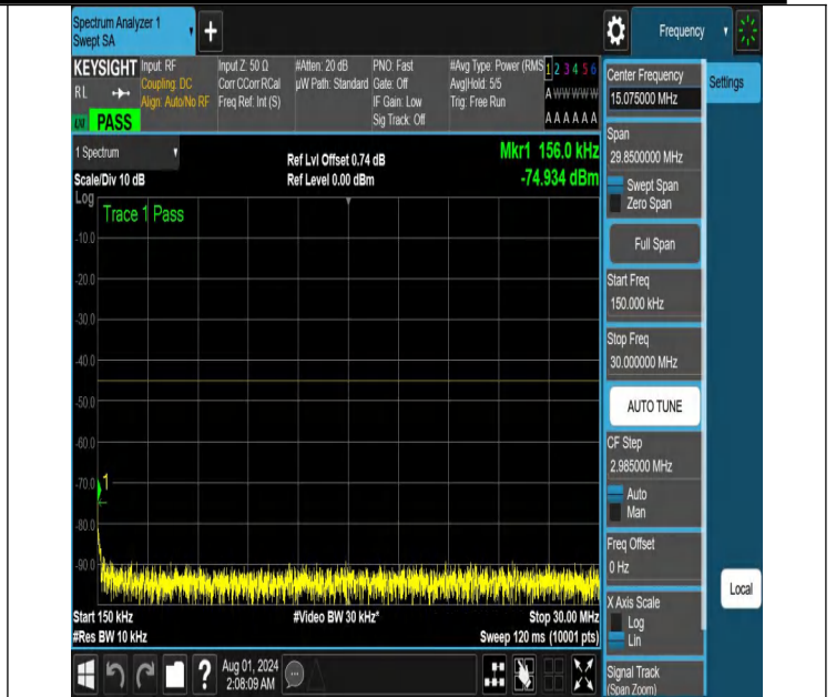
NTNV-N41-PC2-30-70-L-DFT-PI2BPSK-Edge_1RB_Left-0.15-30-Ant1-PASS
