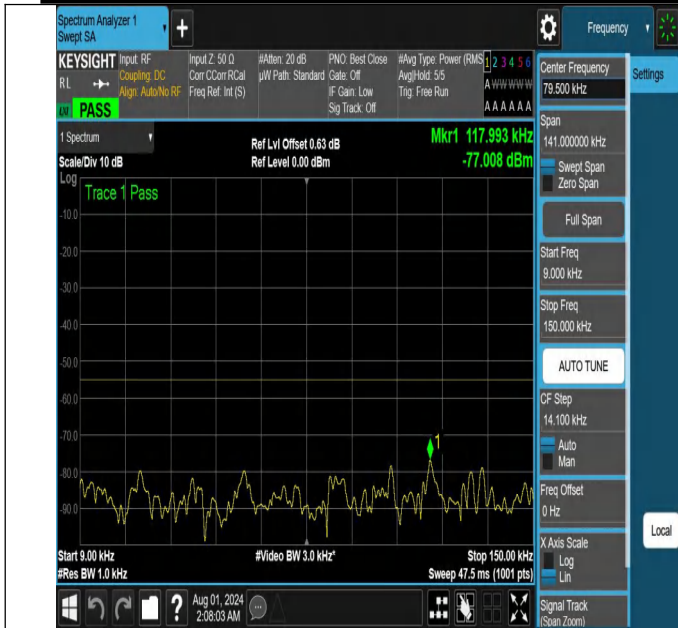
NTNV-N41-PC2-30-70-L-DFT-PI2BPSK-Edge_1RB_Left-0.009-0.15-Ant1-PASS
