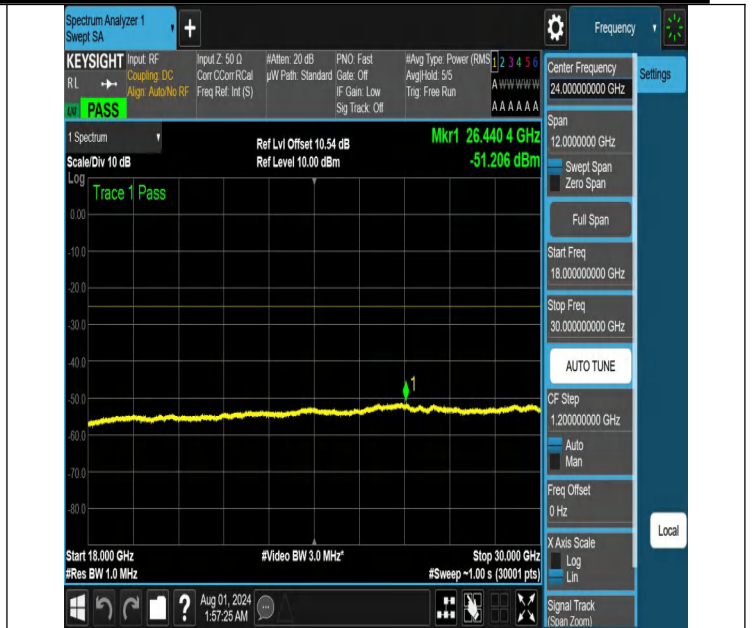
NTNV-N41-PC2-30-60-L-DFT-QPSK-Edge_1RB_Left-18000-3000 0-Ant1-PASS
