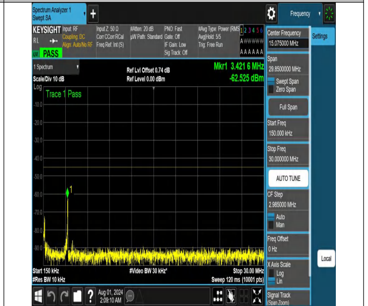
NTNV-N41-PC2-30-70-L-DFT-PI2BPSK-Edge_1RB_Right-0.15-30.0-Ant1-PASS
