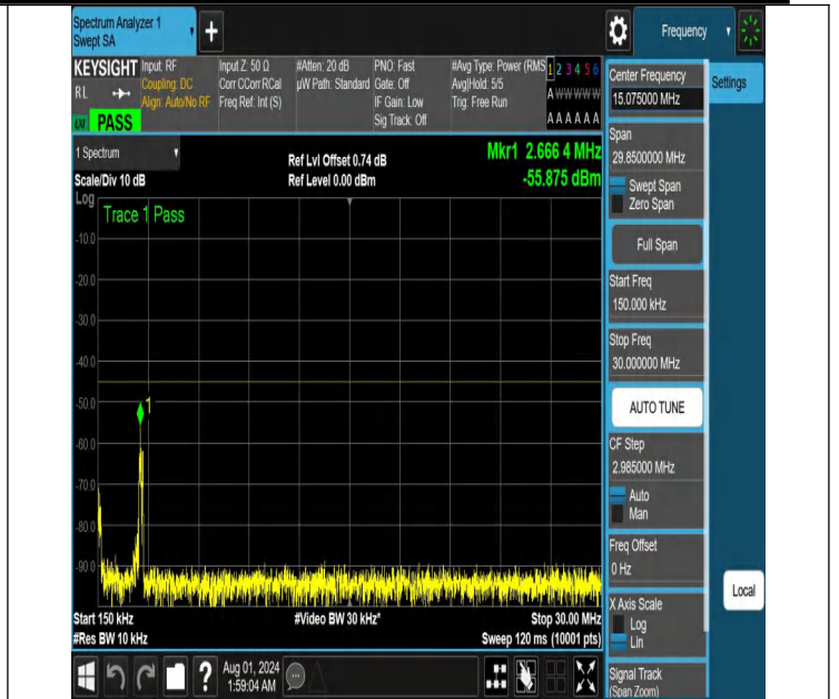
NTNV-N41-PC2-30-60-M-DFT-PI2BPSK-Edge_1RB_Left-0.15-30-Ant1-PASS
