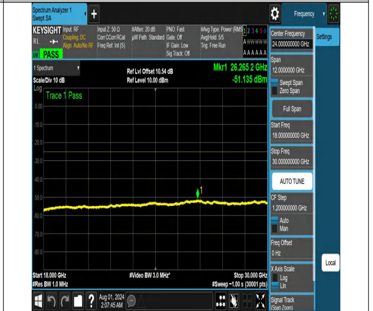
NTNV-N41-PC2-30-60-H-DFT-QPSK-Edge_1RB_Right-18000-30-000-Ant1-PASS
