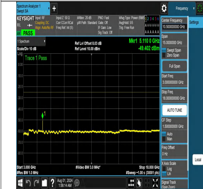
NTNV-N41-PC2-30-60-L-DFT-QPSK-Edge_1RB_Right-3000-18000-Ant1-PASS
