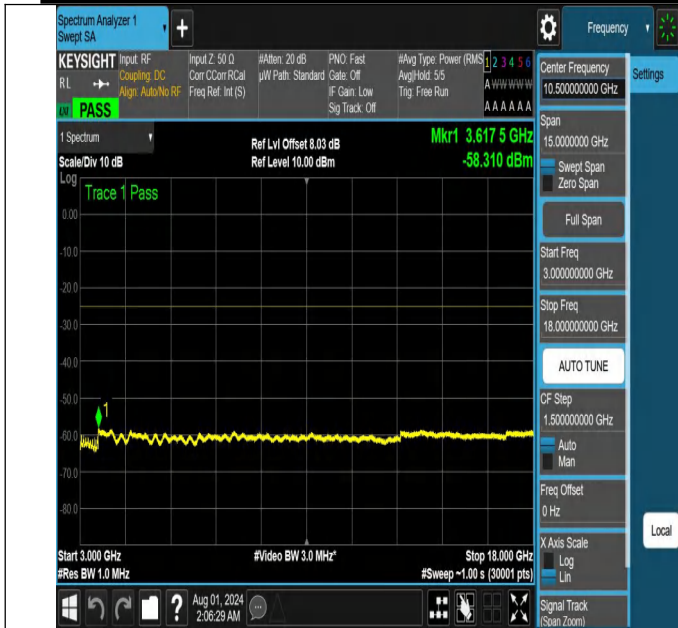
NTNV-N41-PC2-30-60-H-DFT-QPSK-Edge_1RB_Left-3000-1800 0-Ant1-PASS
