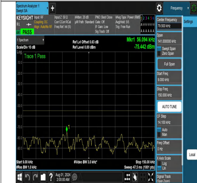
NTNV-N41-PC2-30-60-M-DFT-PI2BPSK-Edge_1RB_Right-0.009 -0.15-Ant1-PASS
