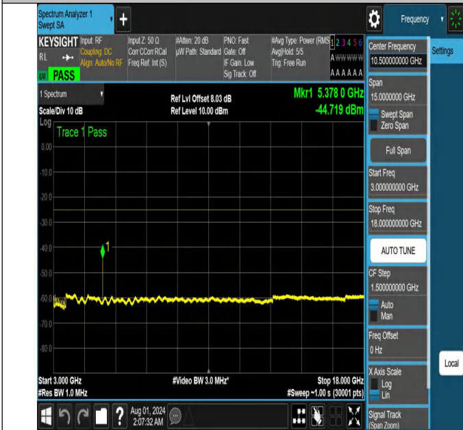
NTNV-N41-PC2-30-60-H-DFT-QPSK-Edge_1RB_Right-3000-180-00-Ant1-PASS
