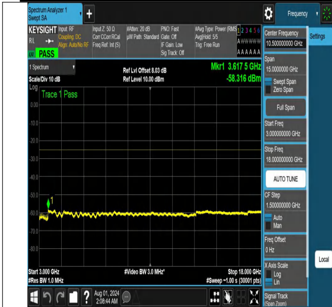
NTNV-N41-PC2-30-70-L-DFT-PI2BPSK-Edge_1RB_Left-3000-18000-Ant1-PASS
