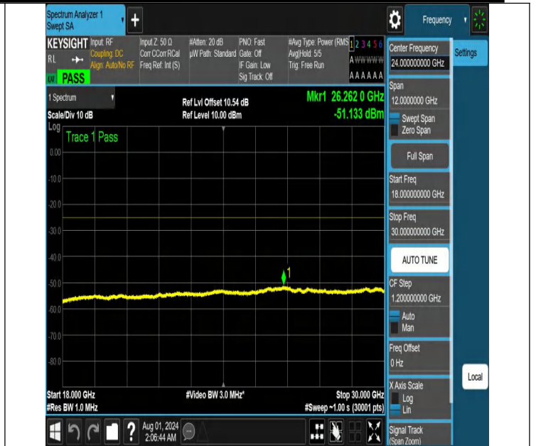
NTNV-N41-PC2-30-60-H-DFT-QPSK-Edge_1RB_Left-1800-3000 0-Ant1-PASS
