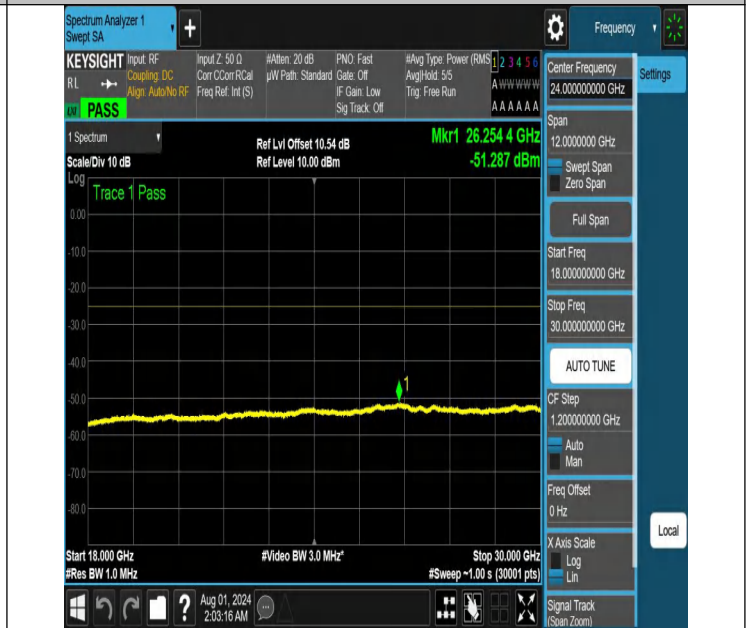
NTNV-N41-PC2-30-60-M-DFT-QPSK-Edge_1RB_Right-18000-3000-Ant1-PASS
