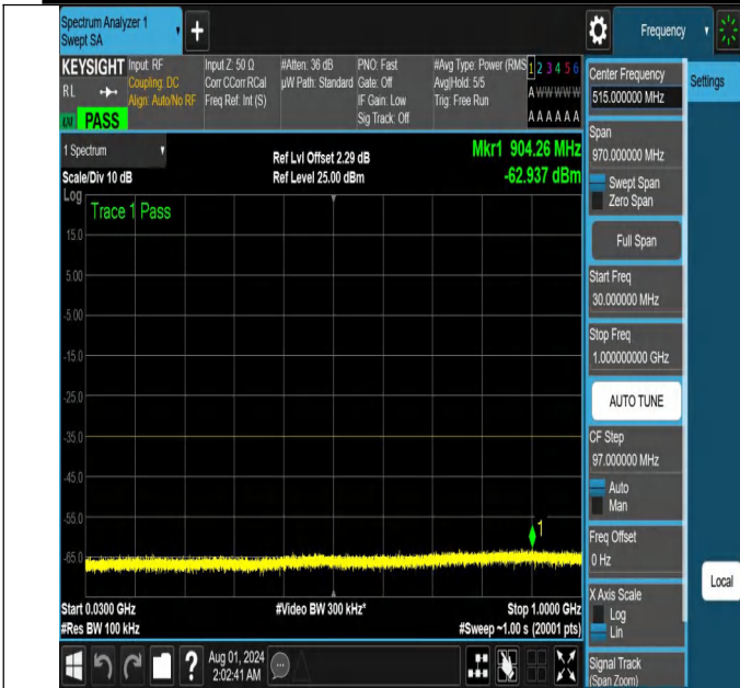
NTNV-N41-PC2-30-60-M-DFT-QPSK-Edge_1RB_Right-30-1000-Ant1-PASS
