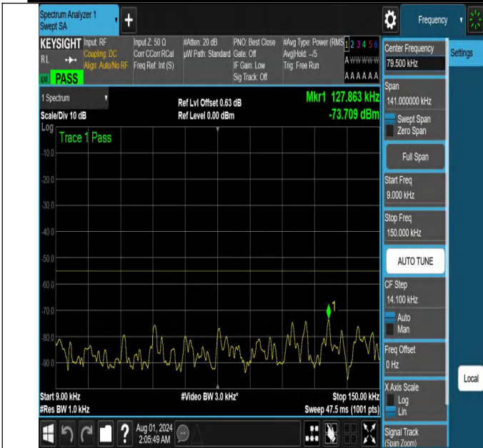
NTNV-N41-PC2-30-60-H-DFT-QPSK-Edge_1RB_Left-0.009-0.15 -Ant1-PASS
