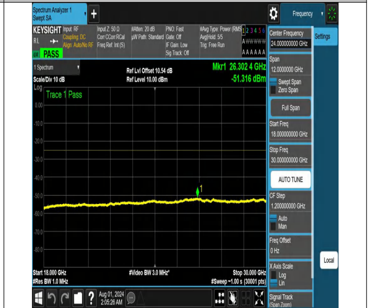
NTNV-N41-PC2-30-60-H-DFT-PI2BPSK-Edge_1RB_Right-18000-30000-Ant1-PASS
