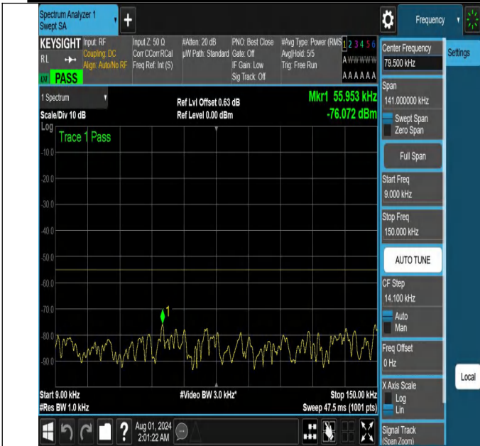
NTNV-N41-PC2-30-60-M-DFT-QPSK-Edge_1RB_Left-0.009-0.15 -Ant1-PASS
