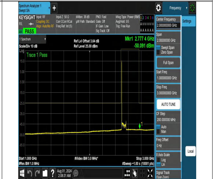
NTNV-N41-PC2-30-70-L-DFT-PI2BPSK-Edge_1RB_Left-1000-3000-Ant1-PASS
