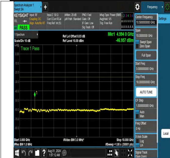
NTNV-N41-PC2-30-60-L-DFT-QPSK-Edge_1RB_Left-3000-1800 0-Ant1-PASS
