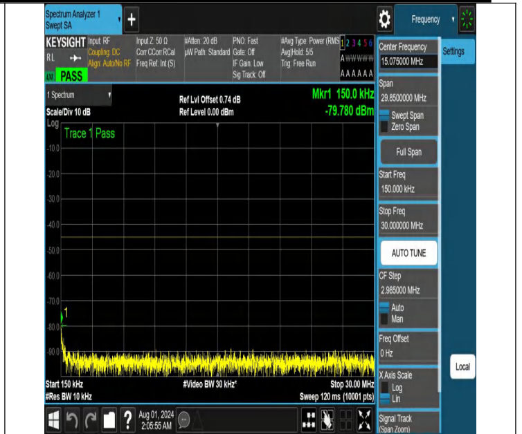
NTNV-N41-PC2-30-60-H-DFT-QPSK-Edge_1RB_Left-0.15-30-Ant 1-PASS
