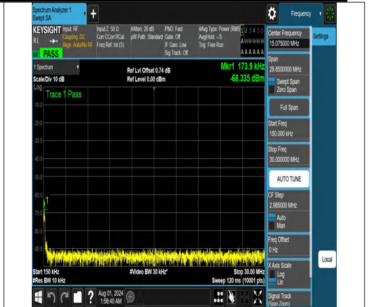
NTNV-N41-PC2-30-60-L-DFT-QPSK-Edge_1RB_Left-0.15-30-Ant 1-PASS
