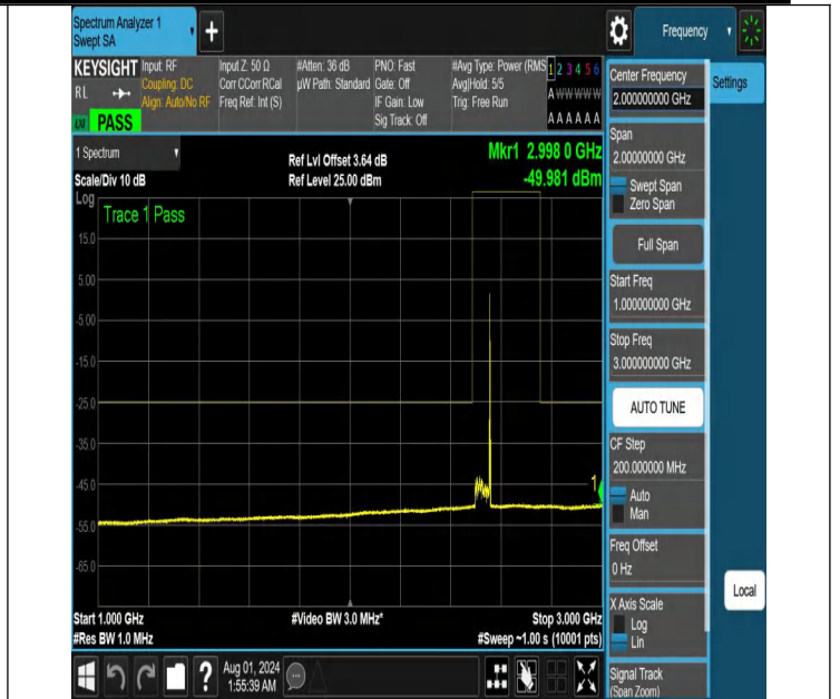
NTNV-N41-PC2-30-60-L-DFT-PI2BPSK-Edge_1RB_Right-1000-3000-Ant1-PASS
