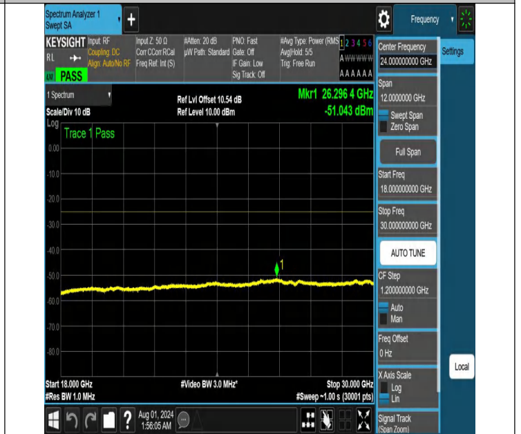
NTNV-N41-PC2-30-60-L-DFT-PI2BPSK-Edge_1RB_Right-18000-30000-Ant1-PASS
