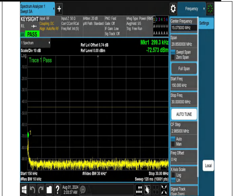
NTNV-N41-PC2-30-60-H-DFT-PI2BPSK-Edge_1RB_Left-0.15-30-Ant1-PASS
