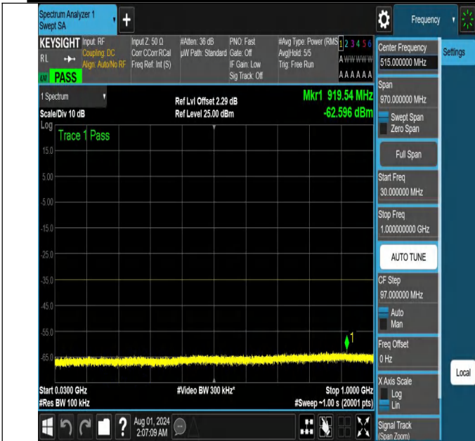
NTNV-N41-PC2-30-60-H-DFT-QPSK-Edge_1RB_Right-30-1000-Ant1-PASS
