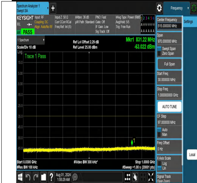
NTNV-N41-PC2-30-60-L-DFT-PI2BPSK-Edge_1RB_Right-30-1000-Ant1-PASS
