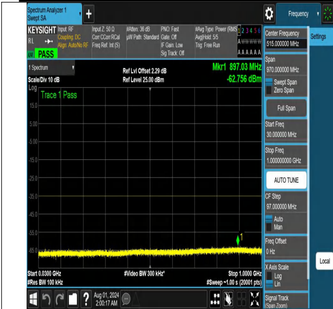
NTNV-N41-PC2-30-60-M-DFT-PI2BPSK-Edge_1RB_Right-30-1000-Ant1-PASS
