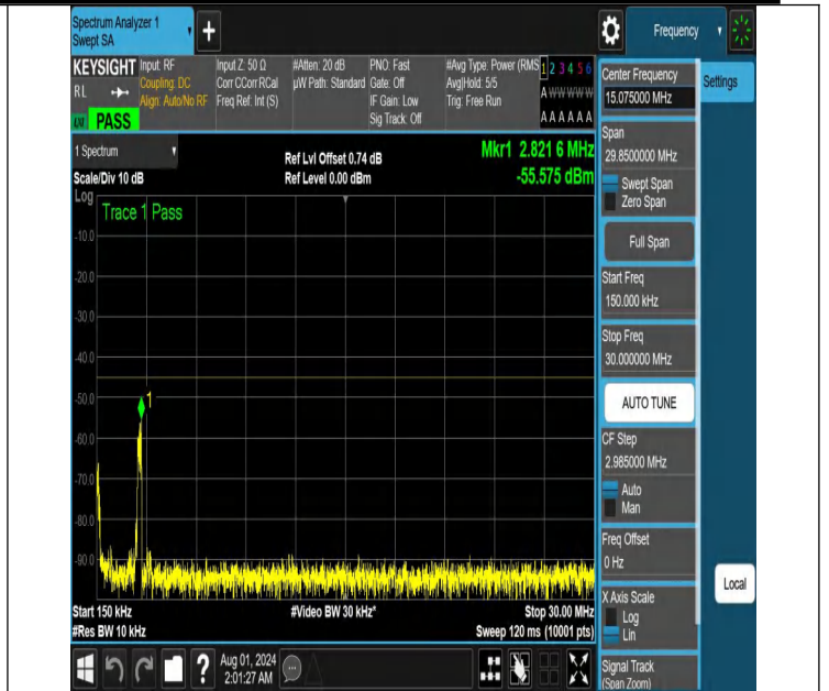
NTNV-N41-PC2-30-60-M-DFT-QPSK-Edge_1RB_Left-0.15-30-Ant 1-PASS
