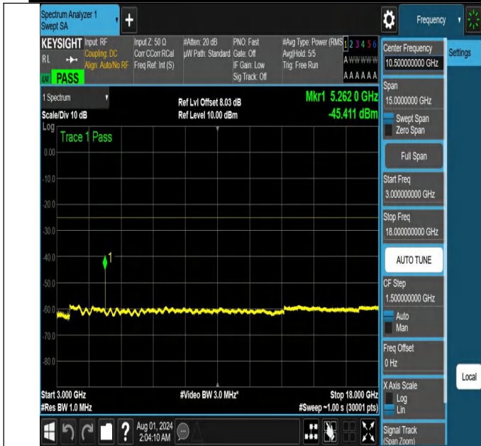
NTNV-N41-PC2-30-60-H-DFT-PI2BPSK-Edge_1RB_Left-3000-1 8000-Ant1-PASS
