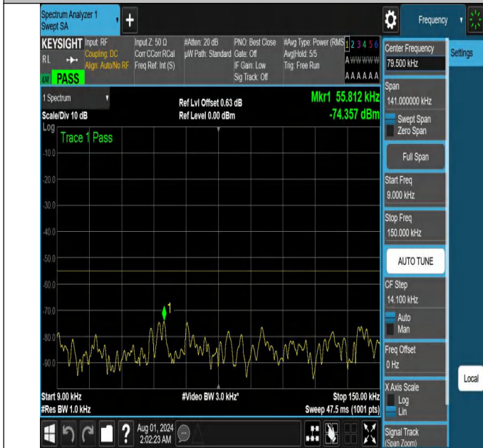
NTNV-N41-PC2-30-60-M-DFT-QPSK-Edge_1RB_Right-0.009-0. 15-Ant1-PASS
