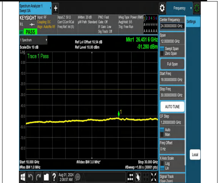
NTNV-N41-PC2-30-70-L-DFT-PI2BPSK-Edge_1RB_Left-18000-30000-Ant1-PASS
