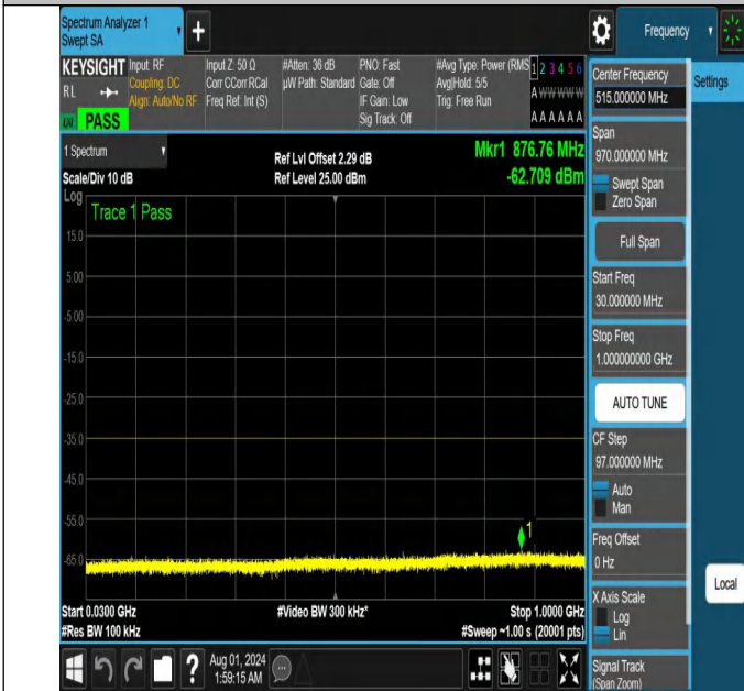
NTNV-N41-PC2-30-60-M-DFT-PI2BPSK-Edge_1RB_Left-30-1000-Ant1-PASS
