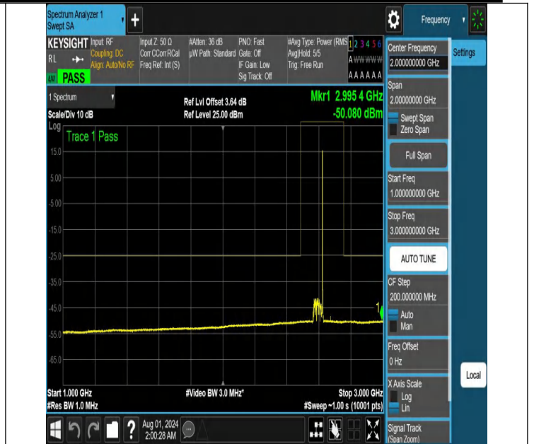
NTNV-N41-PC2-30-60-M-DFT-PI2BPSK-Edge_1RB_Right-1000-3000-Ant1-PASS
