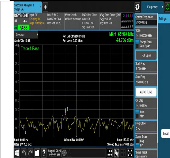
NTNV-N41-PC2-30-60-M-DFT-PI2BPSK-Edge_1RB_Left-0.009-0.15-Ant1-PASS
