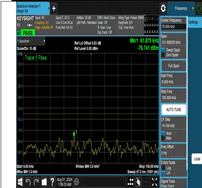
NTNV-N41-PC2-30-60-L-DFT-QPSK-Edge_1RB_Left-0.009-0.15-Ant1-PASS
