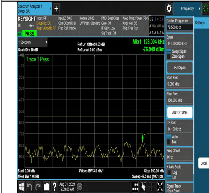
NTNV-N41-PC2-30-70-L-DFT-PI2BPSK-Edge_1RB_Right-0.009-150.0-Ant1-PASS
