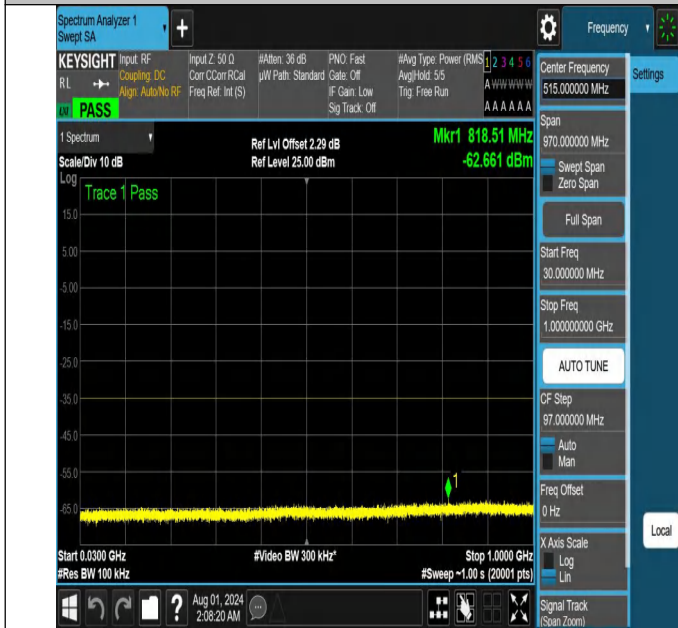
NTNV-N41-PC2-30-70-L-DFT-PI2BPSK-Edge_1RB_Left-30-1000-Ant1-PASS
