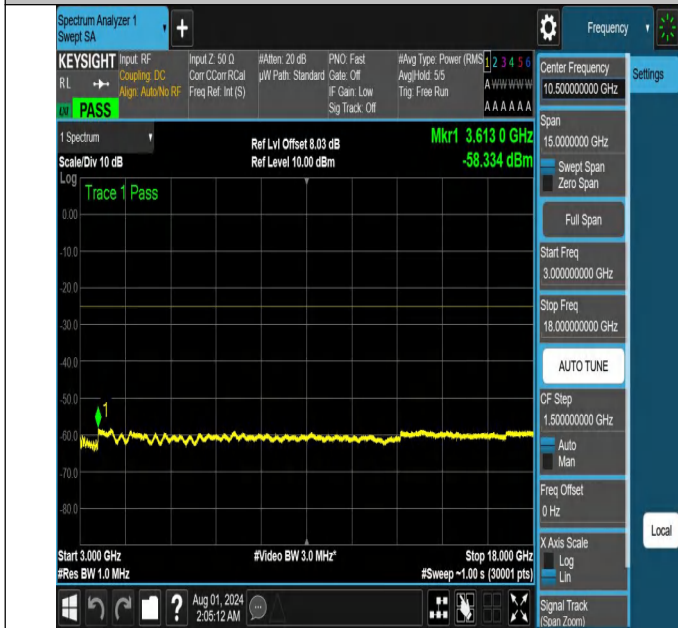
NTNV-N41-PC2-30-60-H-DFT-PI2BPSK-Edge_1RB_Right-3000-18000-Ant1-PASS
