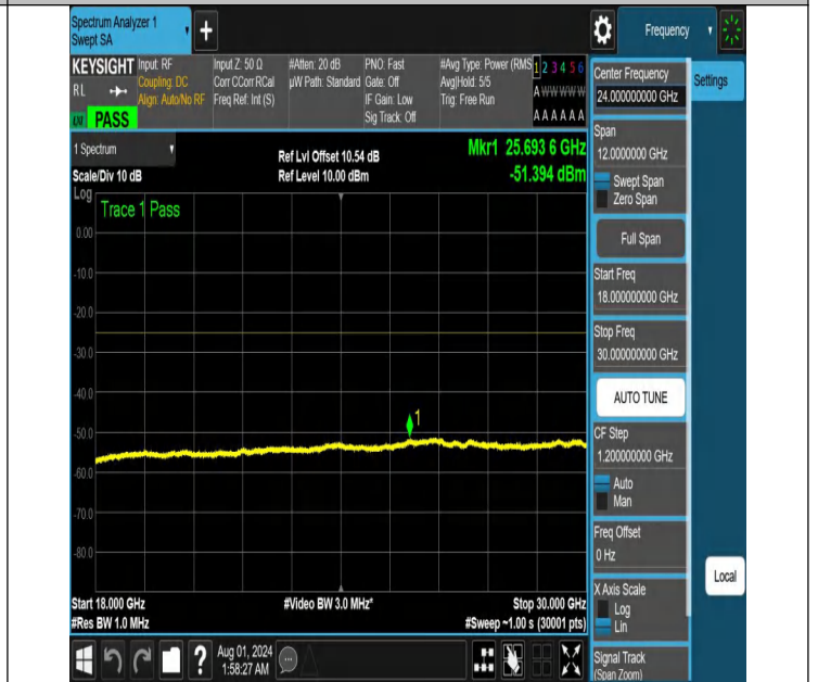
NTNV-N41-PC2-30-60-L-DFT-QPSK-Edge_1RB_Right-18000-30000-Ant1-PASS
