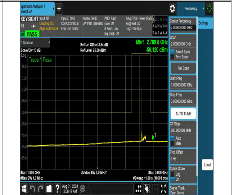
NTNV-N41-PC2-30-60-H-DFT-QPSK-Edge_1RB_Left-1000-3000- Ant1-PASS
