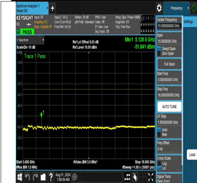
NTNV-N41-PC2-30-60-M-DFT-PI2BPSK-Edge_1RB_Left-3000-1 8000-Ant1-PASS
