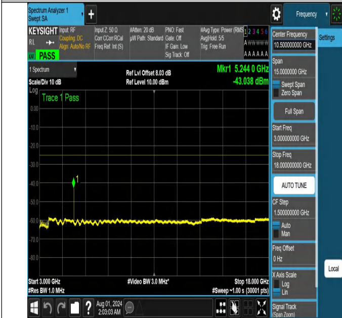
NTNV-N41-PC2-30-60-M-DFT-QPSK-Edge_1RB_Right-3000-1800-Ant1-PASS
