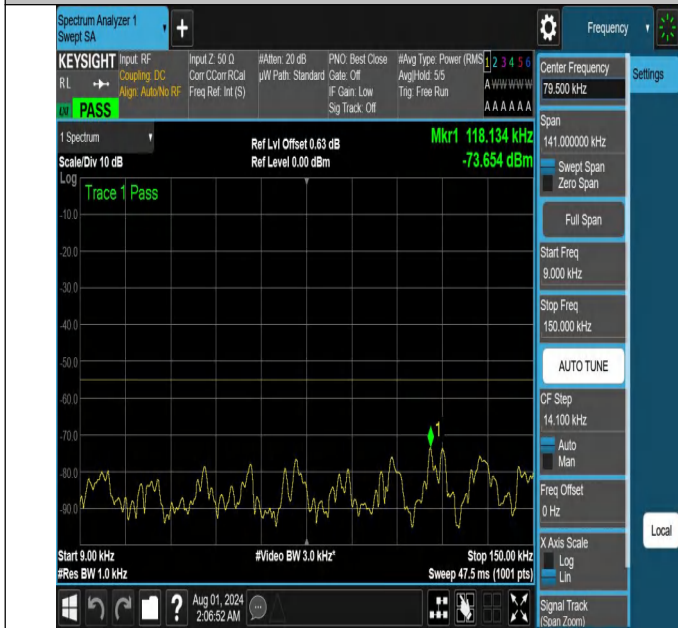
NTNV-N41-PC2-30-60-H-DFT-QPSK-Edge_1RB_Right-0.009-0.1 5-Ant1-PASS
