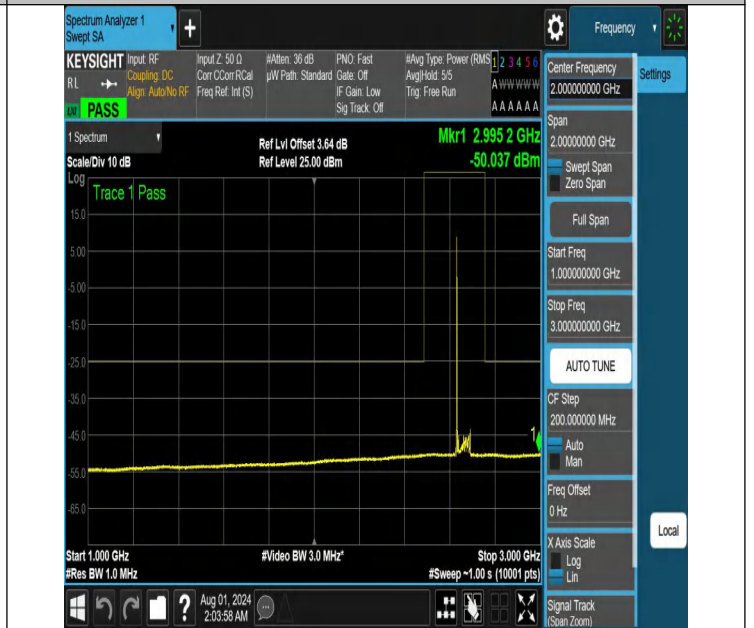
NTNV-N41-PC2-30-60-H-DFT-PI2BPSK-Edge_1RB_Left-1000-3000-Ant1-PASS
