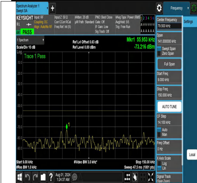
NTNV-N41-PC2-30-30-H-DFT-QPSK-Edge_1RB_Left-0.009-0.15 -Ant1-PASS
