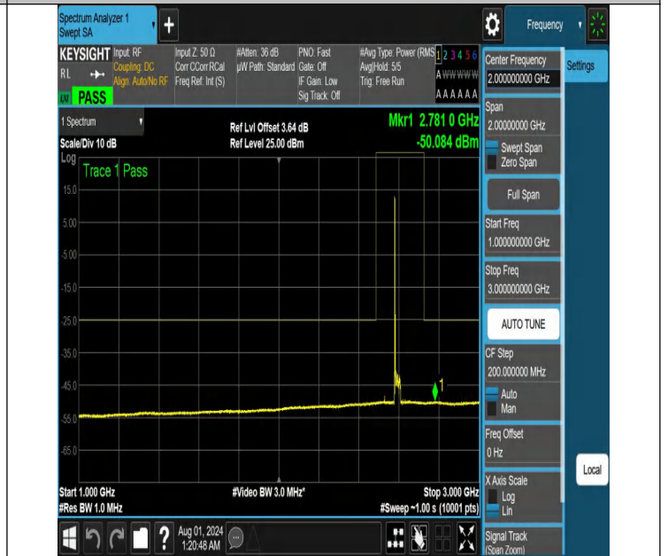
NTNV-N41-PC2-30-30-M-DFT-QPSK-Edge_1RB_Left-1000-3000-Ant1-PASS
