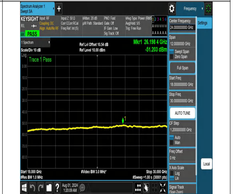
NTNV-N41-PC2-30-30-M-DFT-PI2BPSK-Edge_1RB_Right-18000-30000-Ant1-PASS
