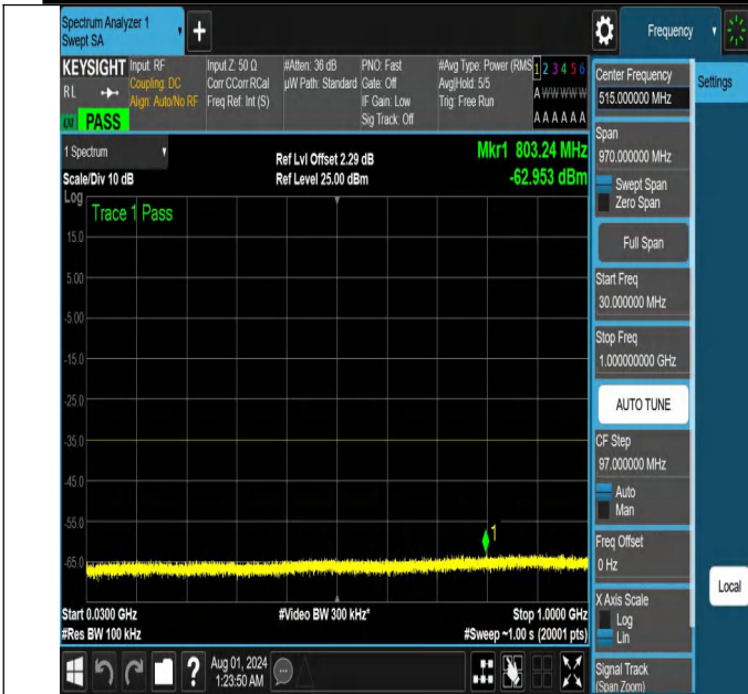
NTNV-N41-PC2-30-30-H-DFT-PI2BPSK-Edge_1RB_Right-30-1000-Ant1-PASS
