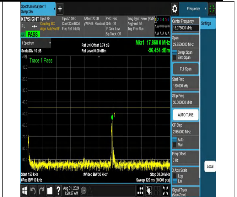
NTNV-N41-PC2-30-30-M-DFT-QPSK-Edge_1RB_Left-0.15-30-Ant 1-PASS
