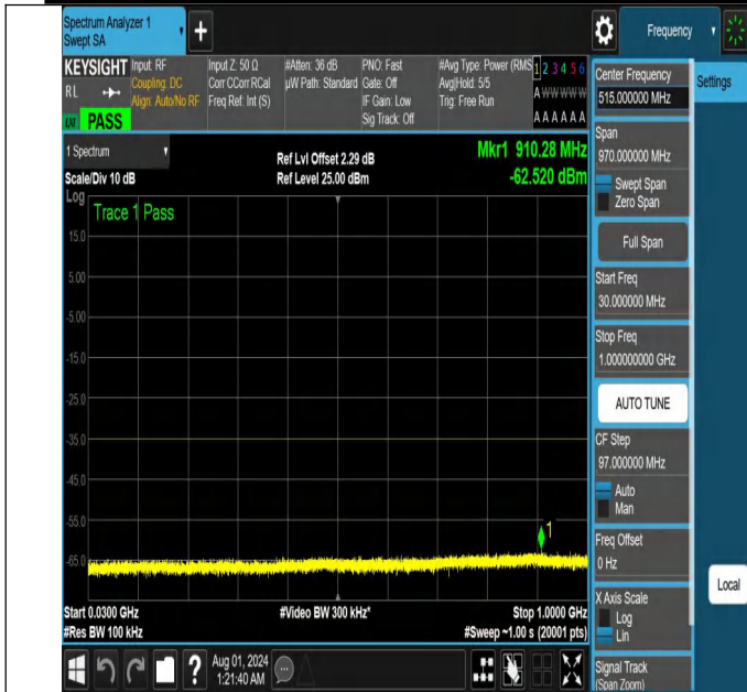
NTNV-N41-PC2-30-30-M-DFT-QPSK-Edge_1RB_Right-30-1000-Ant1-PASS
