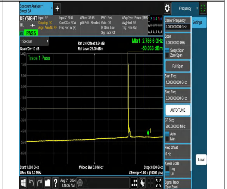
NTNV-N41-PC2-30-30-L-DFT-QPSK-Edge_1RB_Left-1000-3000-Ant1-PASS
