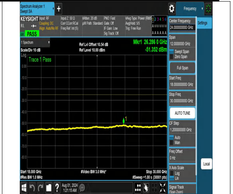
NTNV-N41-PC2-30-30-M-DFT-QPSK-Edge_1RB_Left-18000-300 00-Ant1-PASS
