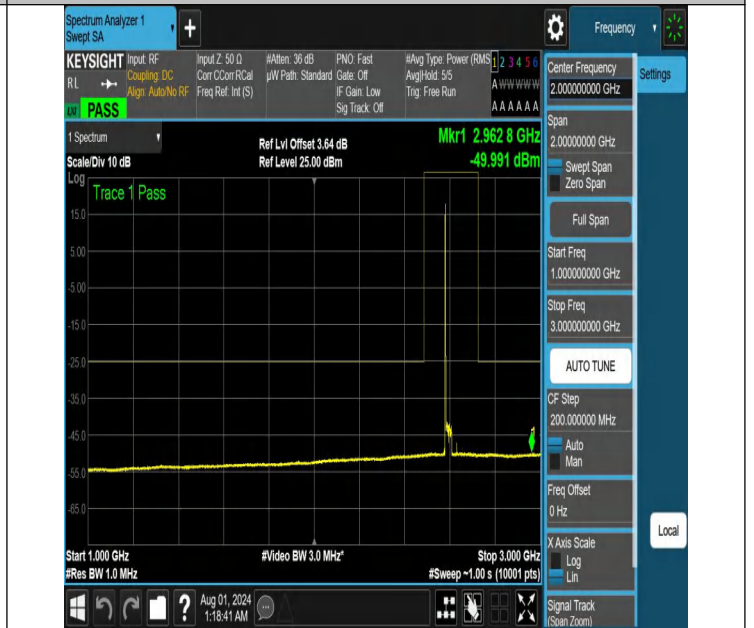
NTNV-N41-PC2-30-30-M-DFT-PI2BPSK-Edge_1RB_Left-1000-3000-Ant1-PASS
