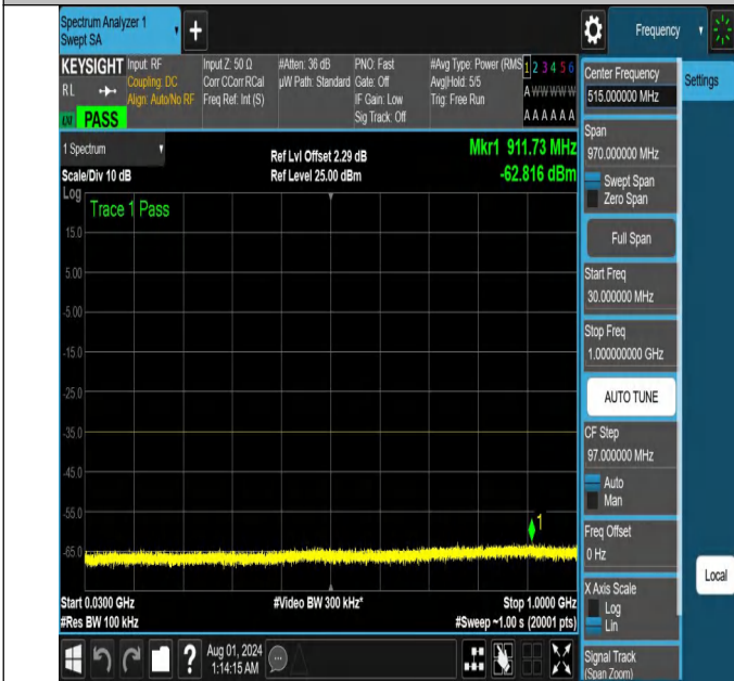
NTNV-N41-PC2-30-30-L-DFT-PI2BPSK-Edge_1RB_Left-30-1000-Ant1-PASS
