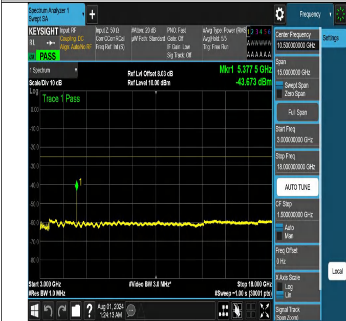
NTNV-N41-PC2-30-30-H-DFT-PI2BPSK-Edge_1RB_Right-3000-18000-Ant1-PASS
