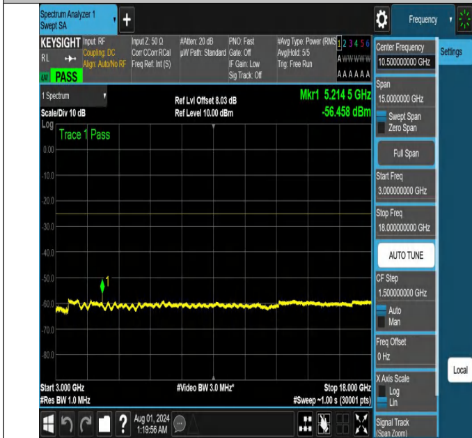
NTNV-N41-PC2-30-30-M-DFT-PI2BPSK-Edge_1RB_Right-3000-18000-Ant1-PASS
