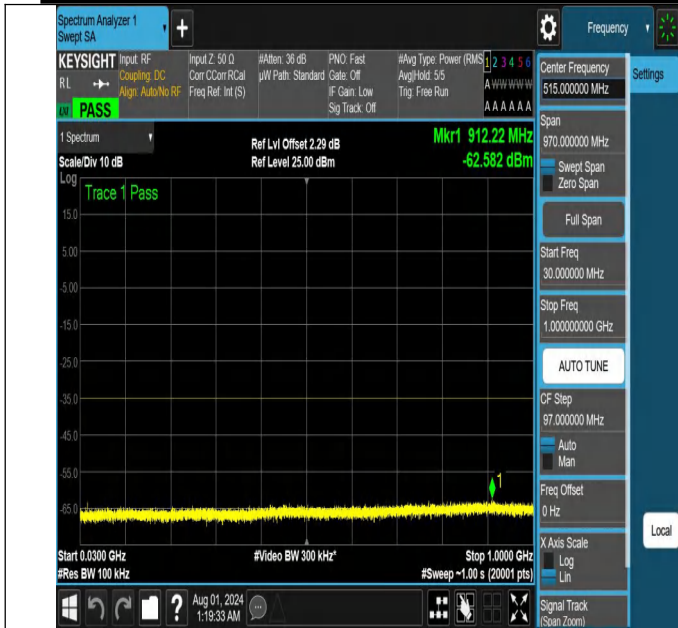
NTNV-N41-PC2-30-30-M-DFT-PI2BPSK-Edge_1RB_Right-30-1000-Ant1-PASS
