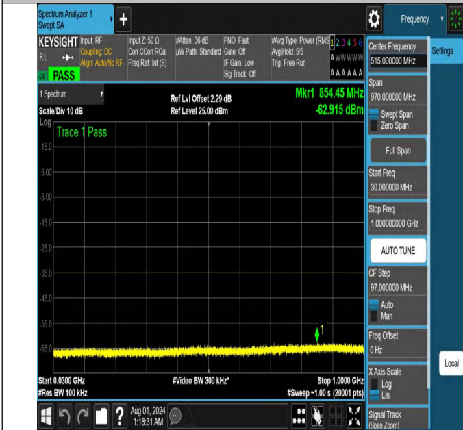
NTNV-N41-PC2-30-30-M-DFT-PI2BPSK-Edge_1RB_Left-30-1000-Ant1-PASS
