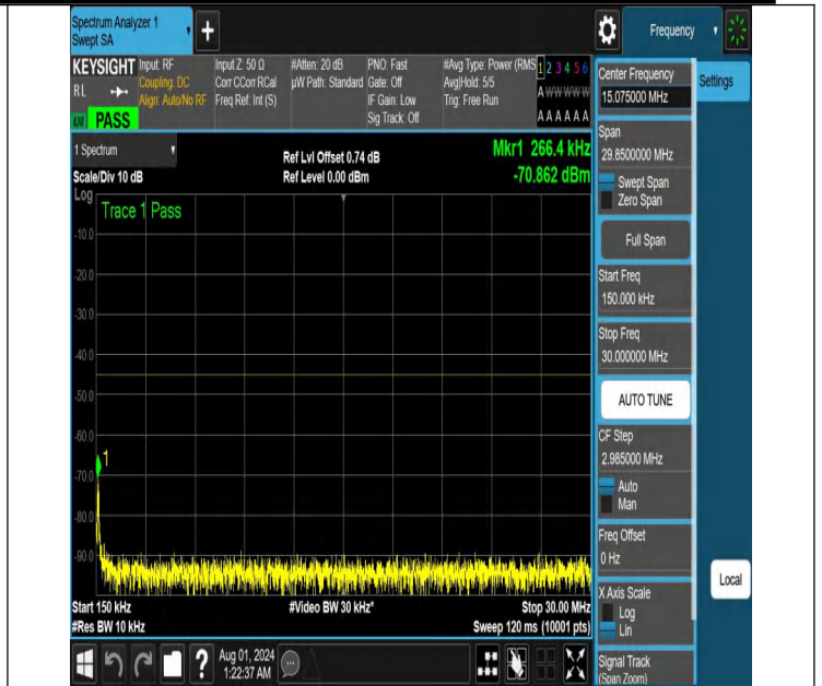
NTNV-N41-PC2-30-30-H-DFT-PI2BPSK-Edge_1RB_Left-0.15-30-Ant1-PASS
