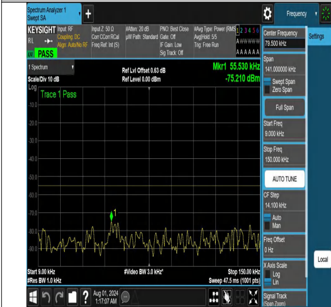
NTNV-N41-PC2-30-30-L-DFT-QPSK-Edge_1RB_Right-0.009-0.1 5-Ant1-PASS
