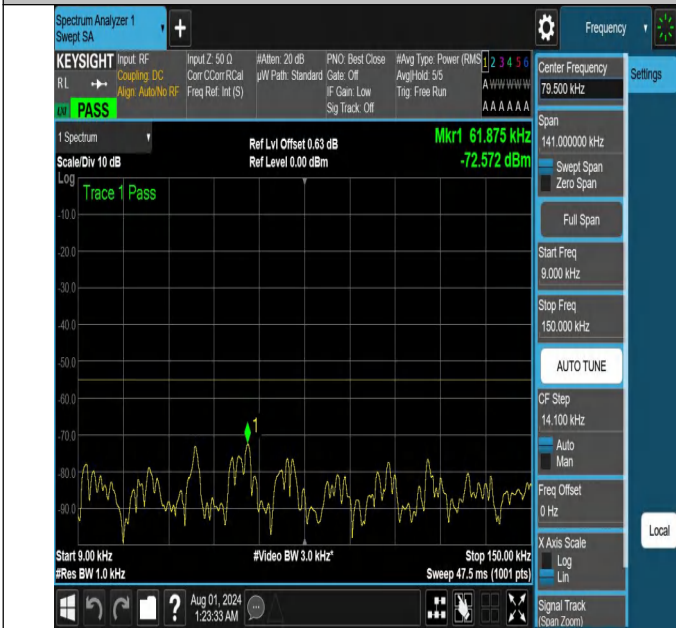
NTNV-N41-PC2-30-30-H-DFT-PI2BPSK-Edge_1RB_Right-0.009- 0.15-Ant1-PASS
