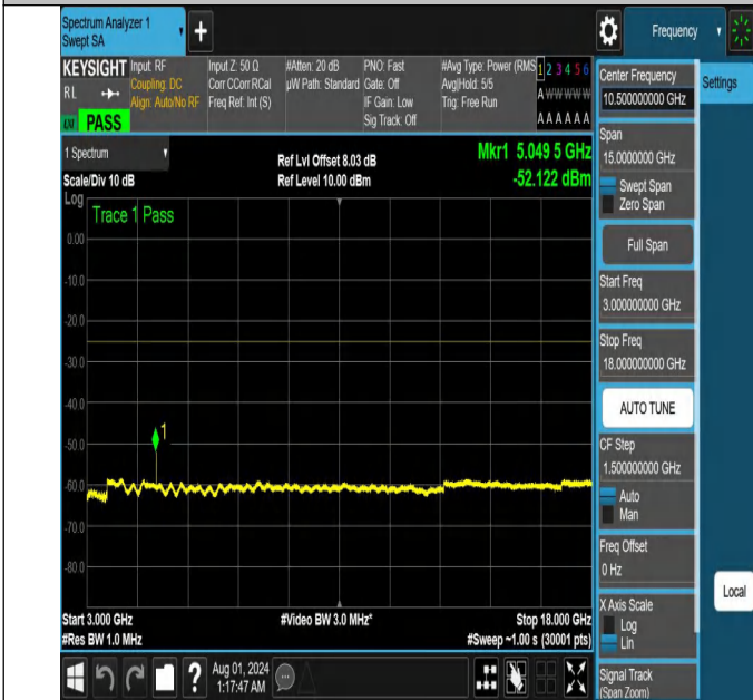
NTNV-N41-PC2-30-30-L-DFT-QPSK-Edge_1RB_Right-3000-18000-Ant1-PASS
