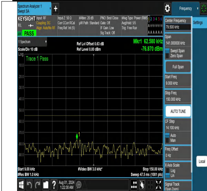
NTNV-N41-PC2-30-30-H-DFT-PI2BPSK-Edge_1RB_Left-0.009-0.15-Ant1-PASS
