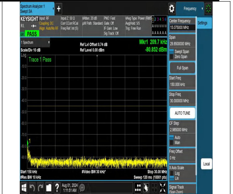
NTNV-N41-PC2-30-20-H-DFT-QPSK-Edge_1RB_Left-0.15-30-Ant 1-PASS
