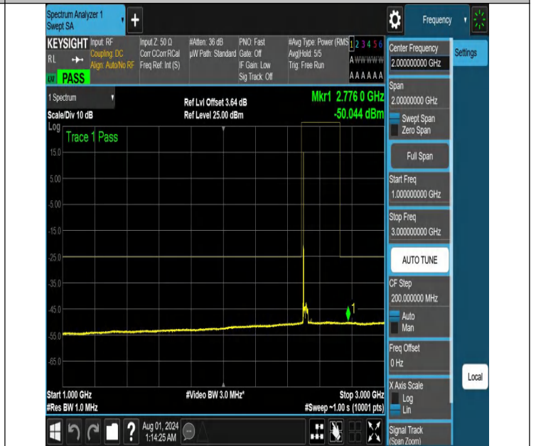
NTNV-N41-PC2-30-30-L-DFT-PI2BPSK-Edge_1RB_Left-1000-3000-Ant1-PASS
