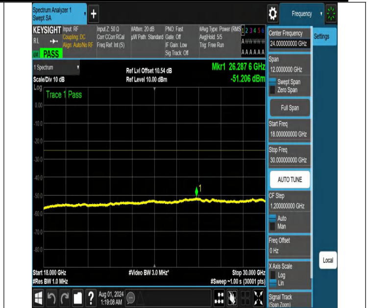
NTNV-N41-PC2-30-30-M-DFT-PI2BPSK-Edge_1RB_Left-18000-3 0000-Ant1-PASS
