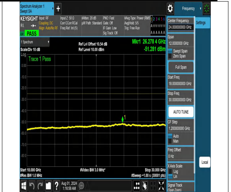
NTNV-N41-PC2-30-30-L-DFT-QPSK-Edge_1RB_Left-18000-3000 0-Ant1-PASS
