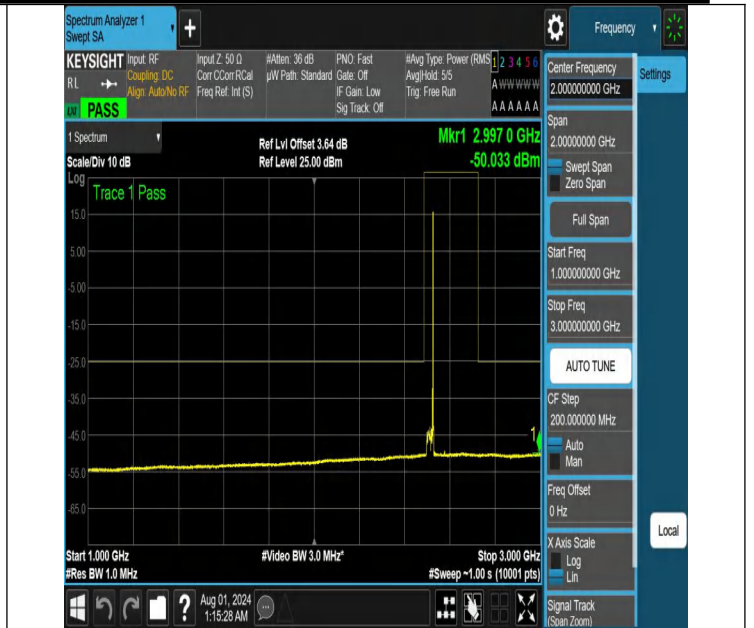
NTNV-N41-PC2-30-30-L-DFT-PI2BPSK-Edge_1RB_Right-1000-3000-Ant1-PASS
