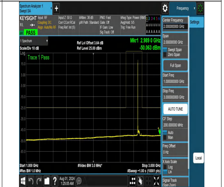
NTNV-N41-PC2-30-30-H-DFT-QPSK-Edge_1RB_Left-1000-3000- Ant1-PASS
