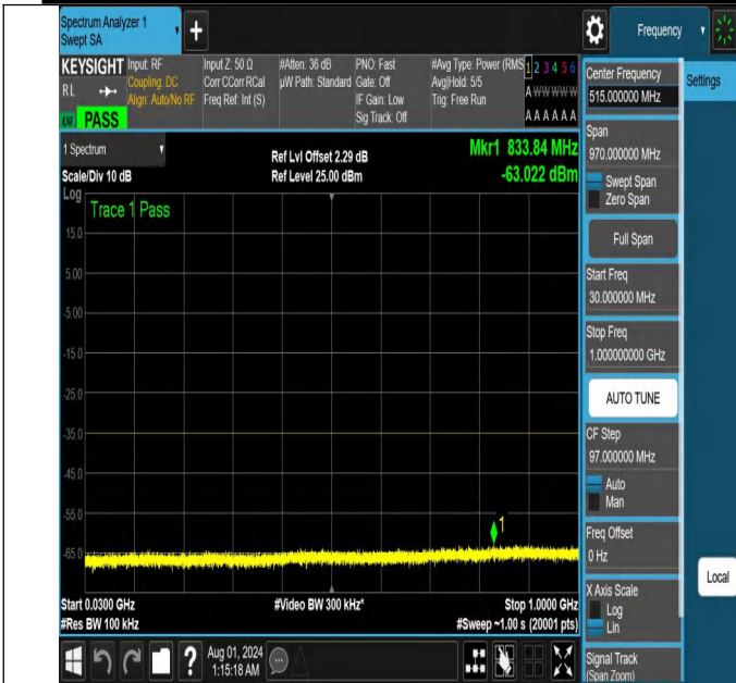
NTNV-N41-PC2-30-30-L-DFT-PI2BPSK-Edge_1RB_Right-30-1000-Ant1-PASS
