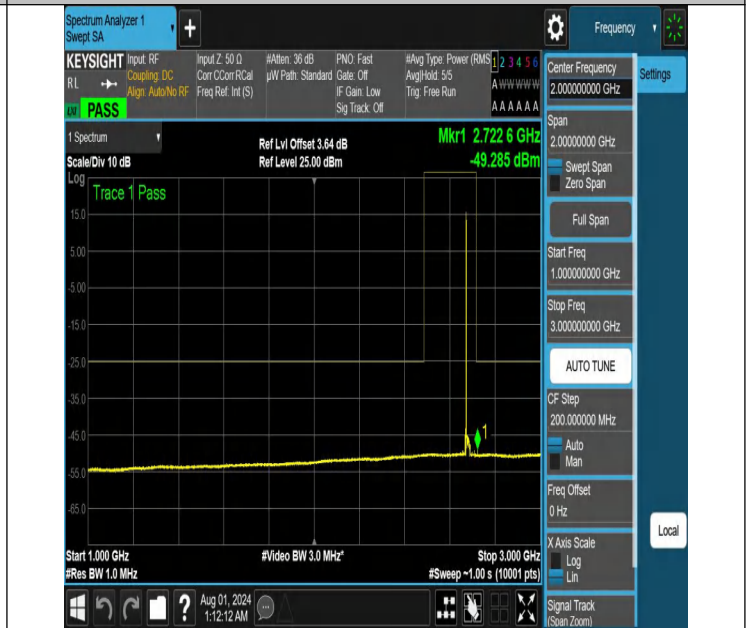
NTNV-N41-PC2-30-20-H-DFT-QPSK-Edge_1RB_Left-1000-3000- Ant1-PASS
