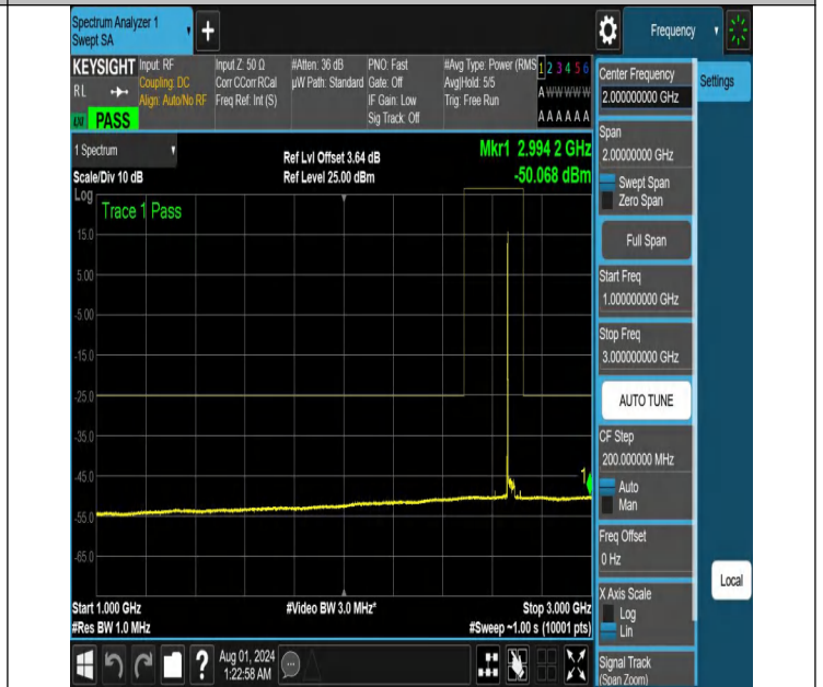
NTNV-N41-PC2-30-30-H-DFT-PI2BPSK-Edge_1RB_Left-1000-3000-Ant1-PASS
