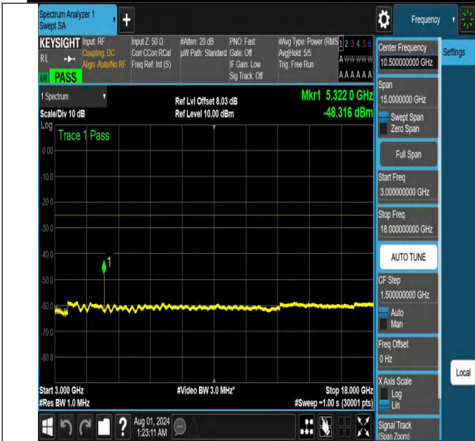
NTNV-N41-PC2-30-30-H-DFT-PI2BPSK-Edge_1RB_Left-3000-1 8000-Ant1-PASS
