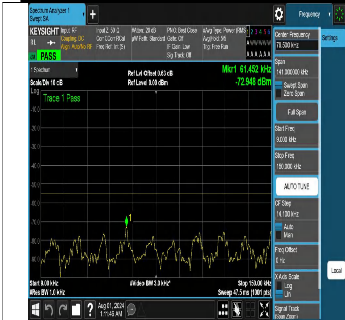
NTNV-N41-PC2-30-20-H-DFT-QPSK-Edge_1RB_Left-0.009-0.15 -Ant1-PASS
