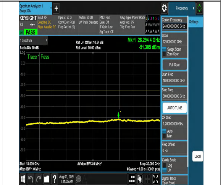
NTNV-N41-PC2-30-20-H-DFT-PI2BPSK-Edge_1RB_Right-18000-30000-Ant1-PASS
