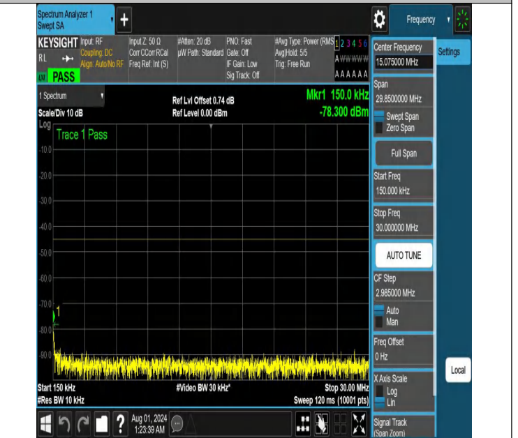
NTNV-N41-PC2-30-30-H-DFT-PI2BPSK-Edge_1RB_Right-0.15-3 0-Ant1-PASS
