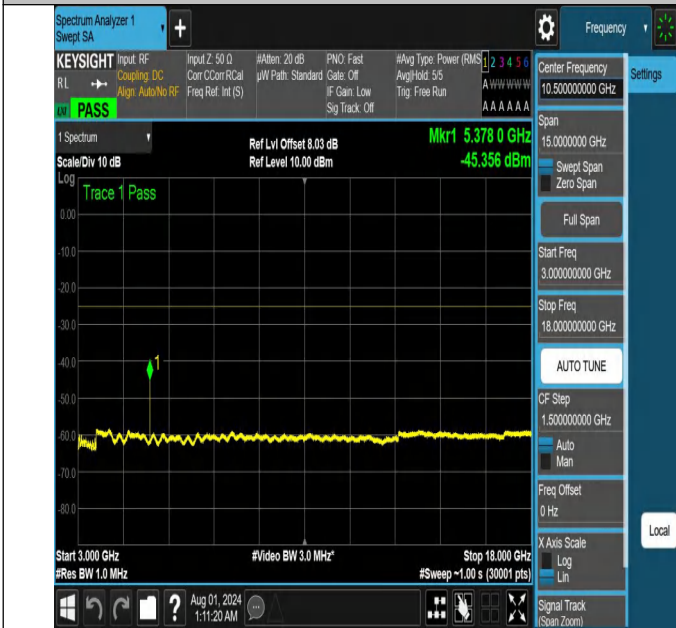
NTNV-N41-PC2-30-20-H-DFT-PI2BPSK-Edge_1RB_Right-3000-18000-Ant1-PASS
