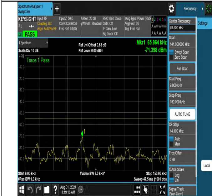
NTNV-N41-PC2-30-30-M-DFT-PI2BPSK-Edge_1RB_Right-0.009 -0.15-Ant1-PASS
