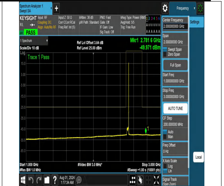
NTNV-N41-PC2-30-30-L-DFT-QPSK-Edge_1RB_Right-1000-3000-Ant1-PASS
