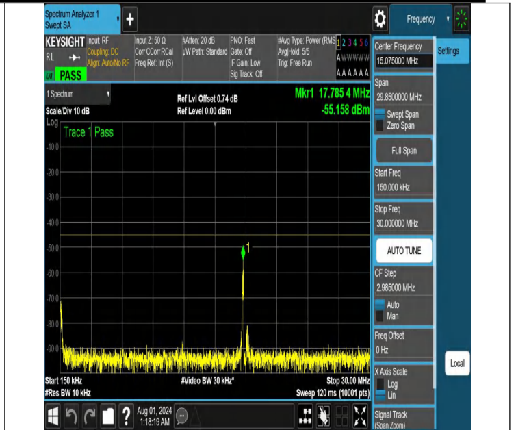
NTNV-N41-PC2-30-30-M-DFT-PI2BPSK-Edge_1RB_Left-0.15-30-Ant1-PASS
