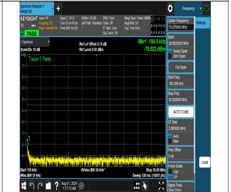
NTNV-N41-PC2-30-30-L-DFT-QPSK-Edge_1RB_Right-0.15-30-A nt1-PASS
