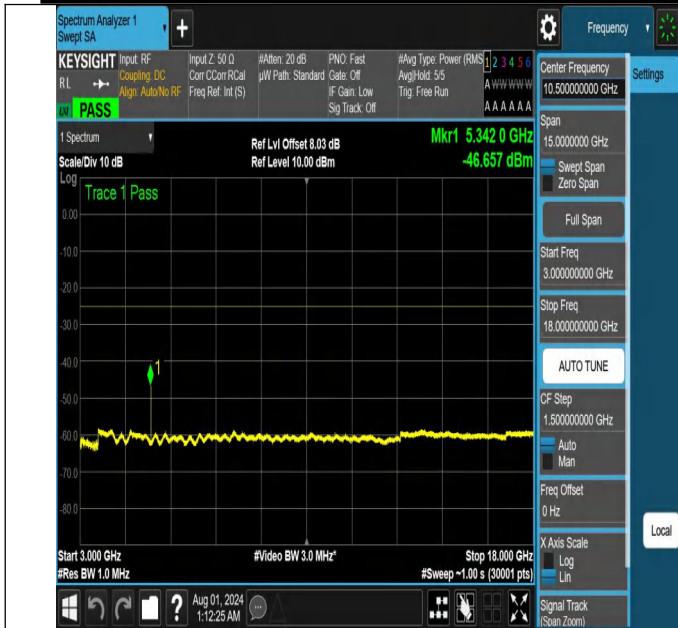
NTNV-N41-PC2-30-20-H-DFT-QPSK-Edge_1RB_Left-3000-1800 0-Ant1-PASS
