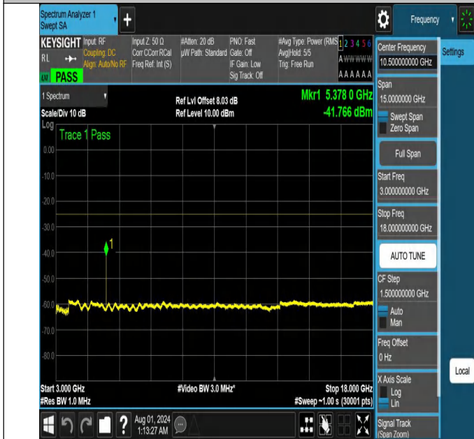
NTNV-N41-PC2-30-20-H-DFT-QPSK-Edge_1RB_Right-3000-180-00-Ant1-PASS
