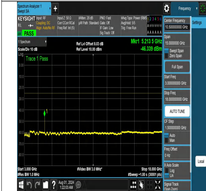
NTNV-N41-PC2-30-30-M-DFT-QPSK-Edge_1RB_Right-3000-1800-Ant1-PASS
