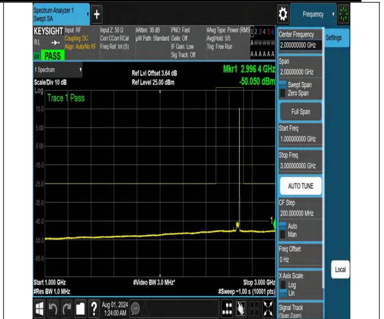
NTNV-N41-PC2-30-30-H-DFT-PI2BPSK-Edge_1RB_Right-1000-3000-Ant1-PASS
