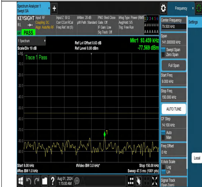
NTNV-N41-PC2-30-30-L-DFT-PI2BPSK-Edge_1RB_Right-0.009-0.15-Ant1-PASS
