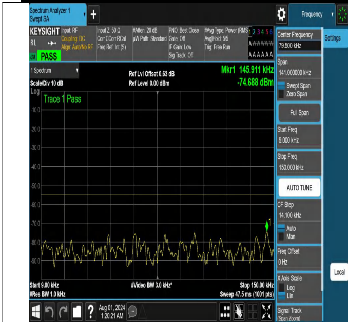
NTNV-N41-PC2-30-30-M-DFT-QPSK-Edge_1RB_Left-0.009-0.15 -Ant1-PASS
