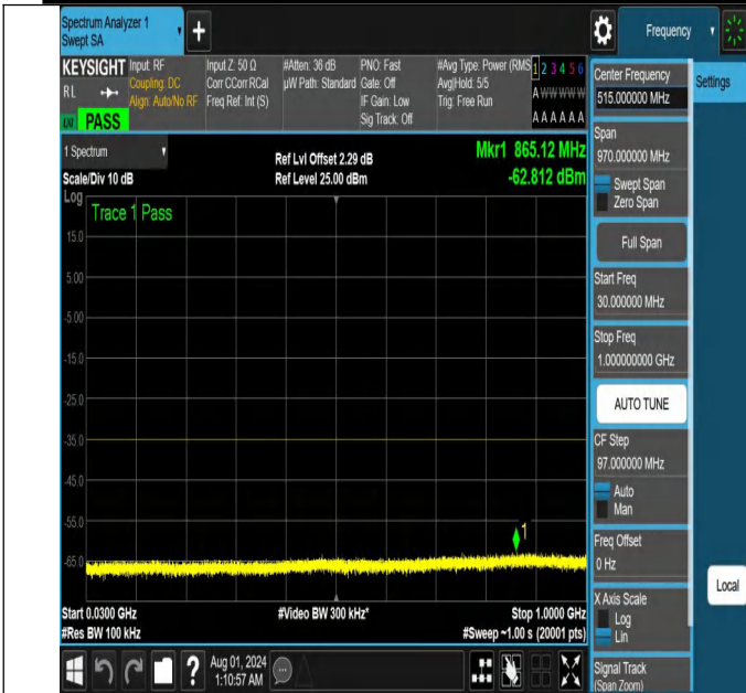
NTNV-N41-PC2-30-20-H-DFT-PI2BPSK-Edge_1RB_Right-30-1000-Ant1-PASS
