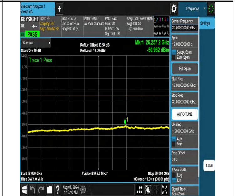
NTNV-N41-PC2-30-20-H-DFT-QPSK-Edge_1RB_Right-18000-30-000-Ant1-PASS
