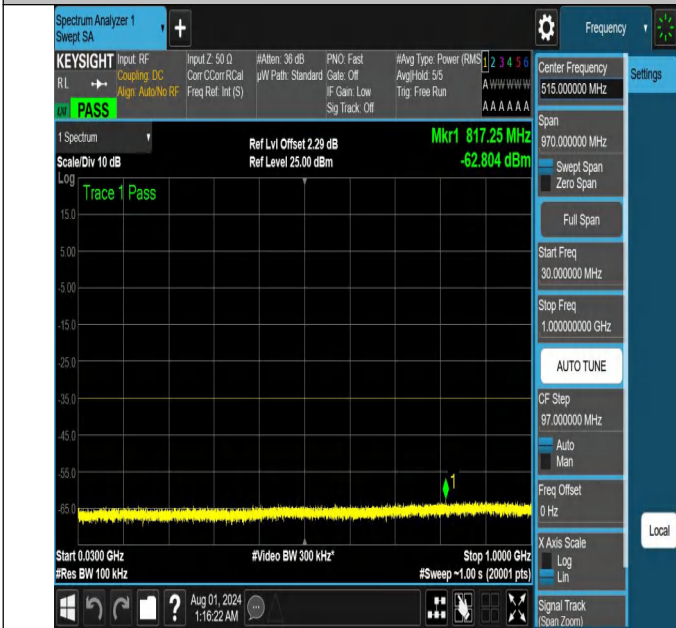
NTNV-N41-PC2-30-30-L-DFT-QPSK-Edge_1RB_Left-30-1000-Ant1-PASS
