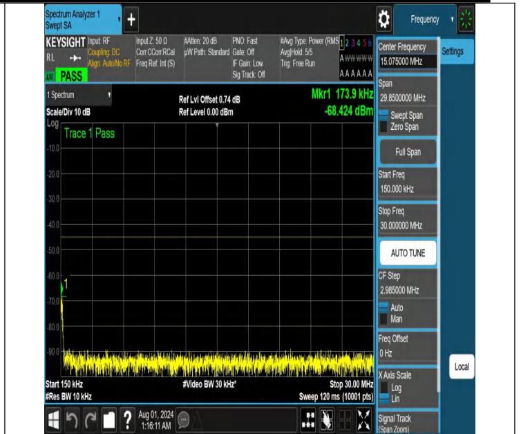
NTNV-N41-PC2-30-30-L-DFT-QPSK-Edge_1RB_Left-0.15-30-Ant 1-PASS
