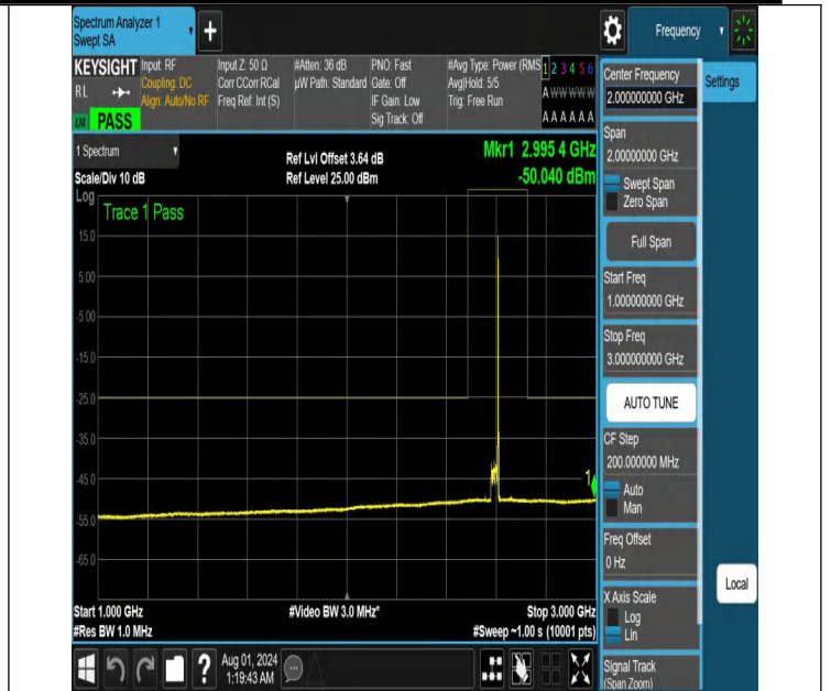
NTNV-N41-PC2-30-30-M-DFT-PI2BPSK-Edge_1RB_Right-1000-3000-Ant1-PASS
