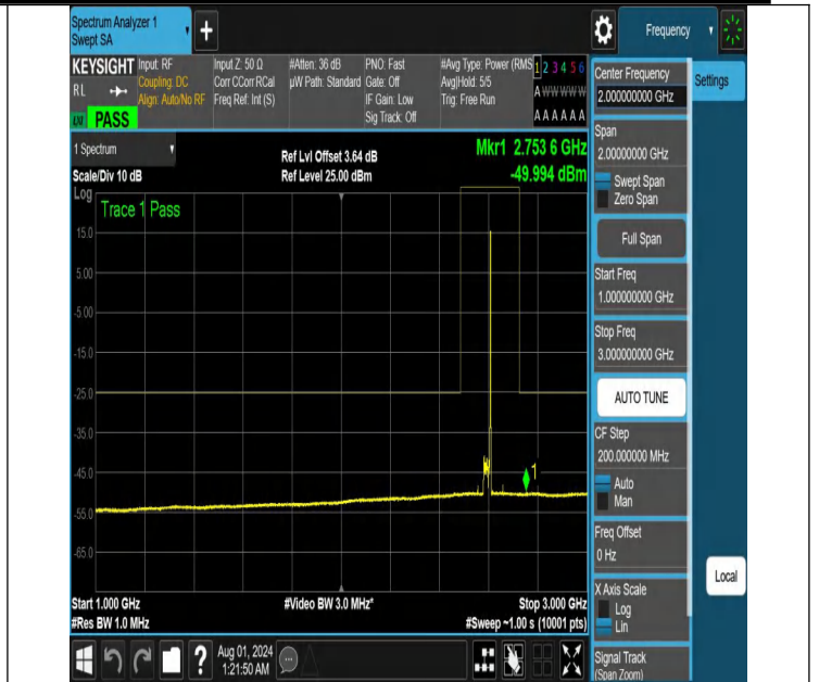
NTNV-N41-PC2-30-30-M-DFT-QPSK-Edge_1RB_Right-1000-300-Ant1-PASS
