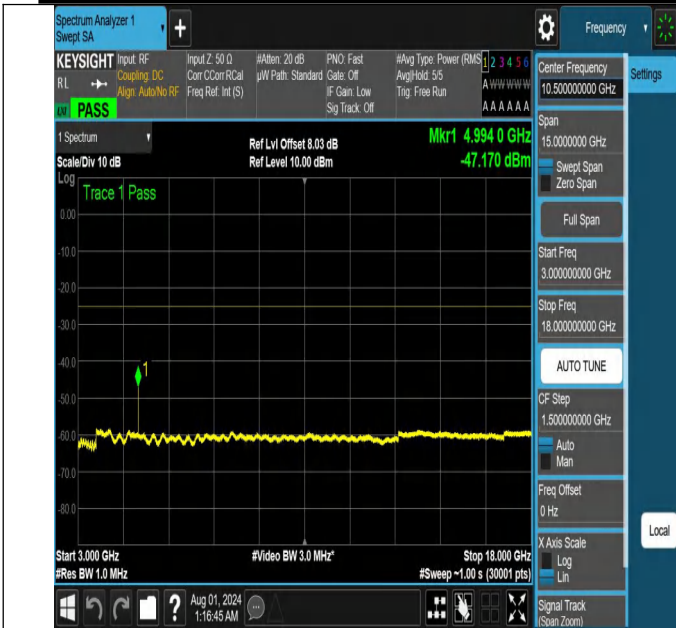
NTNV-N41-PC2-30-30-L-DFT-QPSK-Edge_1RB_Left-3000-1800 0-Ant1-PASS
