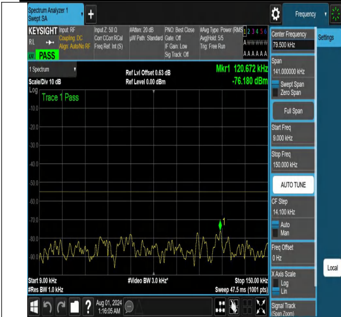
NTNV-N41-PC2-30-30-L-DFT-QPSK-Edge_1RB_Left-0.009-0.15-Ant1-PASS
