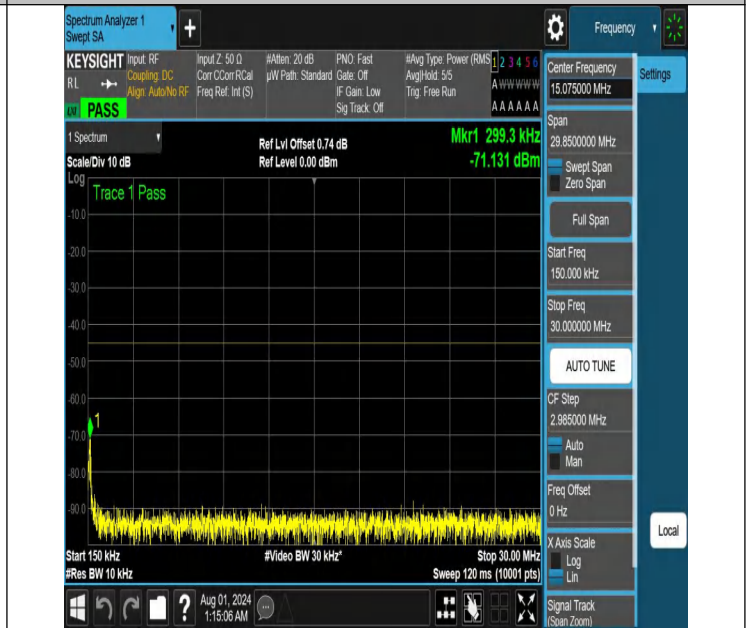
NTNV-N41-PC2-30-30-L-DFT-PI2BPSK-Edge_1RB_Right-0.15-300000000-Ant1-PASS
