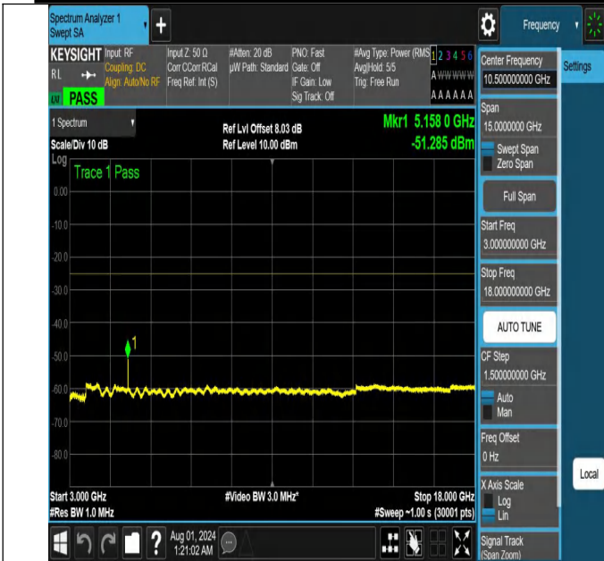
NTNV-N41-PC2-30-30-M-DFT-QPSK-Edge_1RB_Left-3000-1800 0-Ant1-PASS
