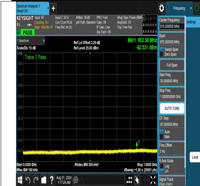
NTNV-N41-PC2-30-30-L-DFT-QPSK-Edge_1RB_Right-30-1000-Ant1-PASS
