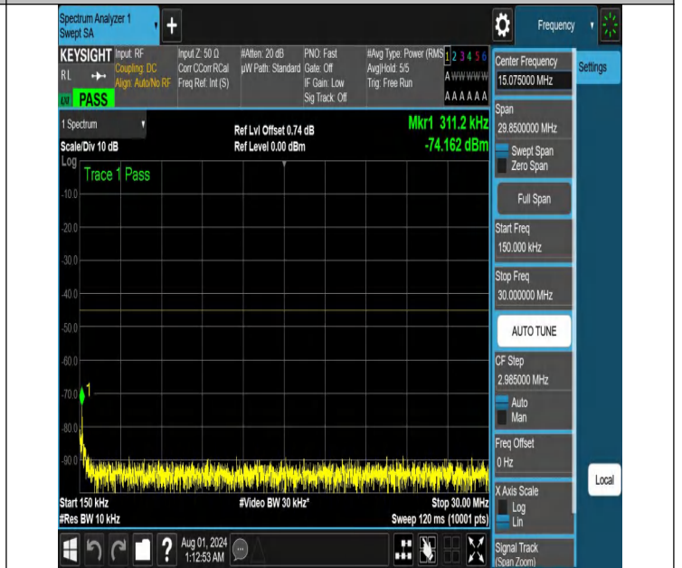
NTNV-N41-PC2-30-20-H-DFT-QPSK-Edge_1RB_Right-0.15-30-A nt1-PASS
