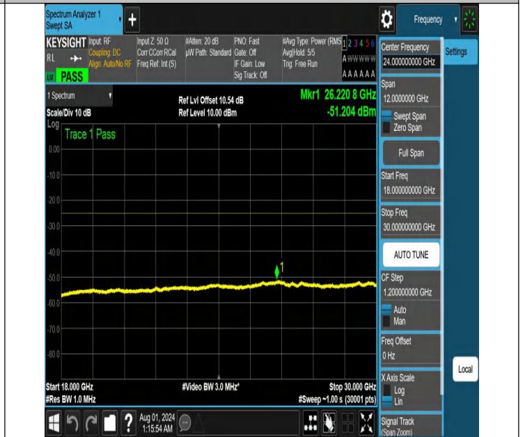
NTNV-N41-PC2-30-30-L-DFT-PI2BPSK-Edge_1RB_Right-18000-30000-Ant1-PASS
