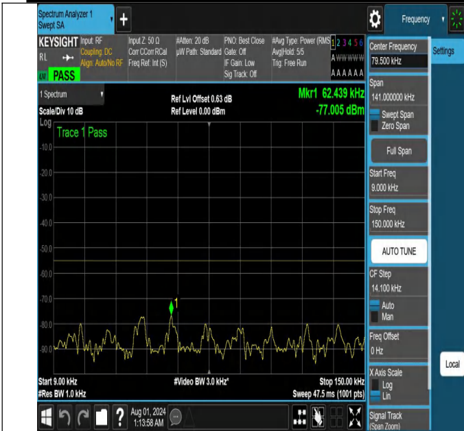
NTNV-N41-PC2-30-30-L-DFT-PI2BPSK-Edge_1RB_Left-0.009-0.15-Ant1-PASS
