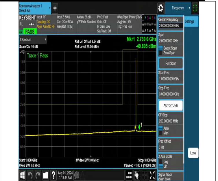
NTNV-N41-PC2-30-20-H-DFT-QPSK-Edge_1RB_Right-1000-300-0-Ant1-PASS
