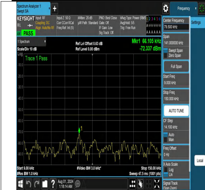
NTNV-N41-PC2-30-30-M-DFT-PI2BPSK-Edge_1RB_Left-0.009-0.15-Ant1-PASS
