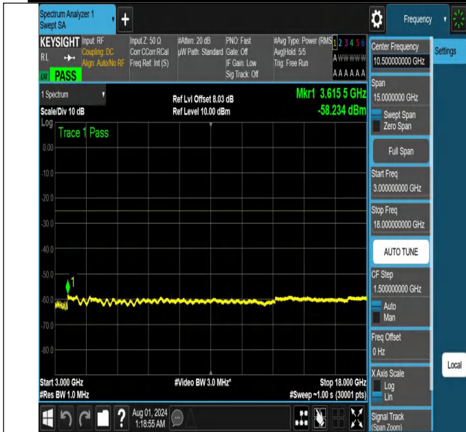
NTNV-N41-PC2-30-30-M-DFT-PI2BPSK-Edge_1RB_Left-3000-1 8000-Ant1-PASS
