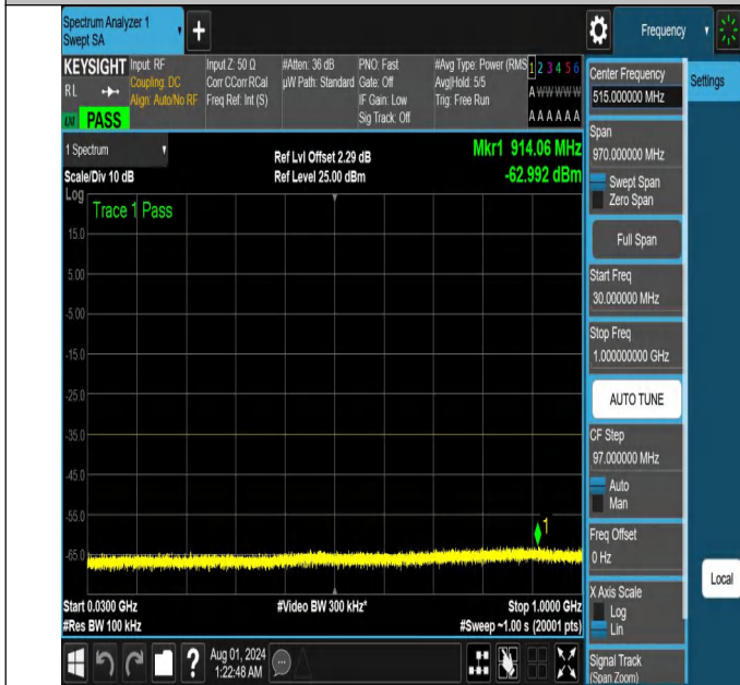
NTNV-N41-PC2-30-30-H-DFT-PI2BPSK-Edge_1RB_Left-30-1000-Ant1-PASS
