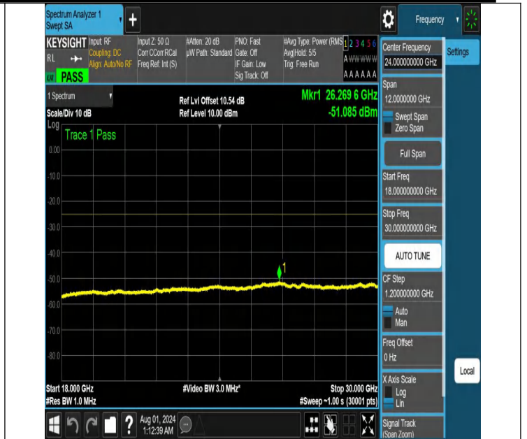
NTNV-N41-PC2-30-20-H-DFT-QPSK-Edge_1RB_Left-1800-3000 0-Ant1-PASS
