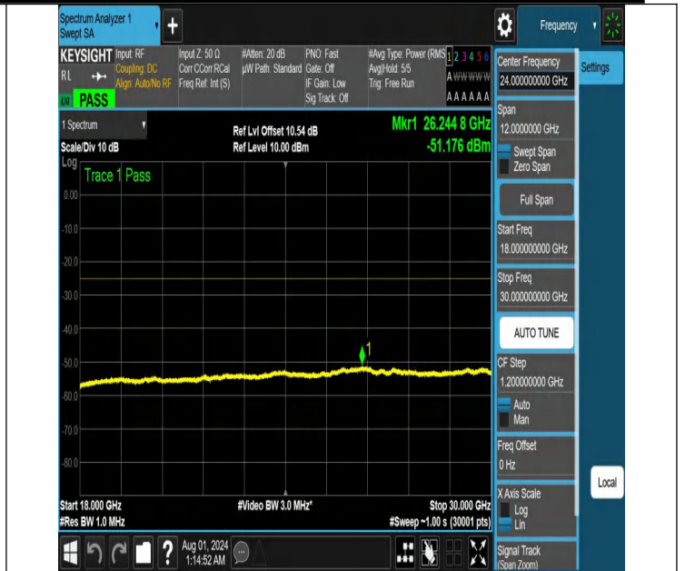
NTNV-N41-PC2-30-30-L-DFT-PI2BPSK-Edge_1RB_Left-18000-30000-Ant1-PASS
