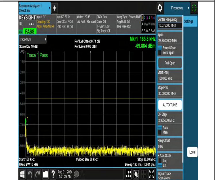
NTNV-N41-PC2-30-30-M-DFT-QPSK-Edge_1RB_Right-0.15-30-A nt1-PASS
