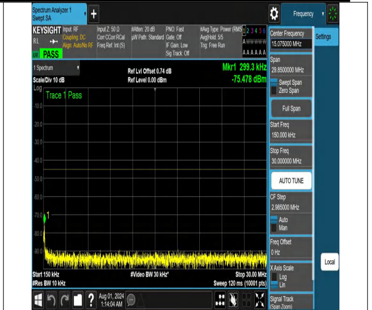
NTNV-N41-PC2-30-30-L-DFT-PI2BPSK-Edge_1RB_Left-0.15-30-Ant1-PASS
