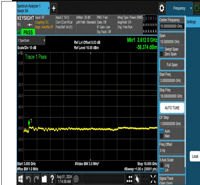
NTNV-N41-PC2-30-30-L-DFT-PI2BPSK-Edge_1RB_Left-3000-18000-Ant1-PASS
