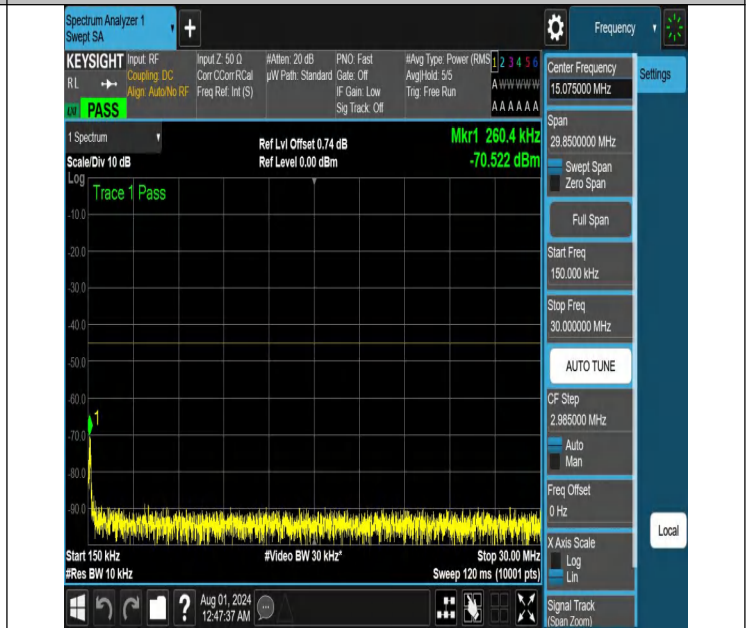
NTNV-N41-PC2-30-15-L-DFT-PI2BPSK-Edge_1RB_Right-0.15-30.000-Ant1-PASS
