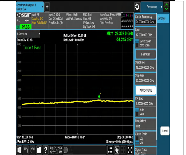
NTNV-N41-PC2-30-15-L-DFT-QPSK-Edge_1RB_Left-18000-3000 0-Ant1-PASS
