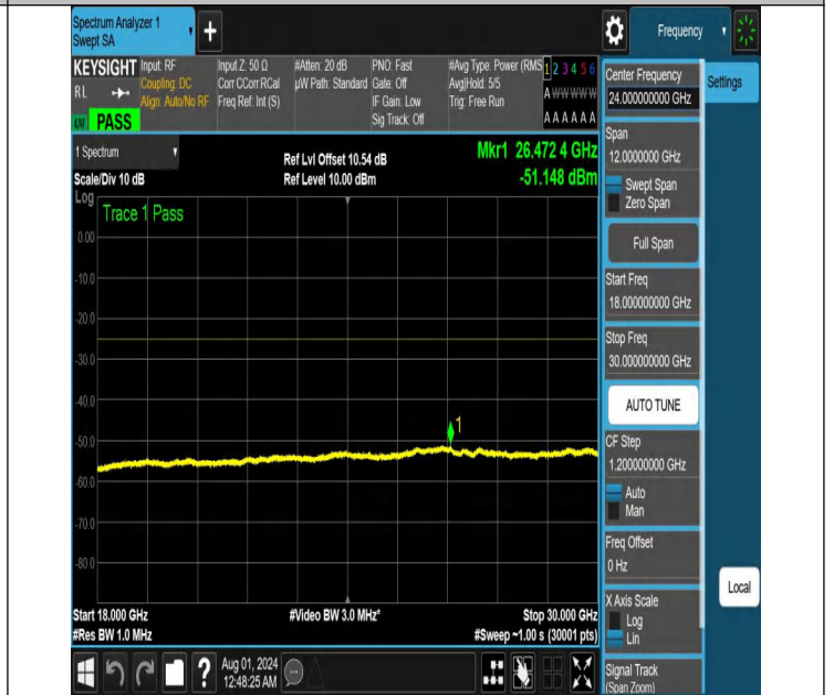
NTNV-N41-PC2-30-15-L-DFT-PI2BPSK-Edge_1RB_Right-18000-30000-Ant1-PASS
