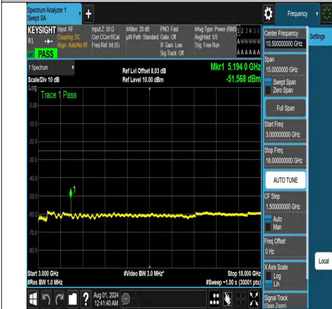
NTNV-N41-PC2-30-10-M-DFT-QPSK-Edge_1RB_Right-3000-18000-Ant1-PASS
