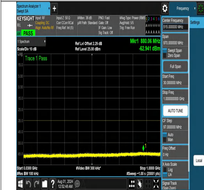
NTNV-N41-PC2-30-15-M-DFT-PI2BPSK-Edge_1RB_Left-30-1000-Ant1-PASS
