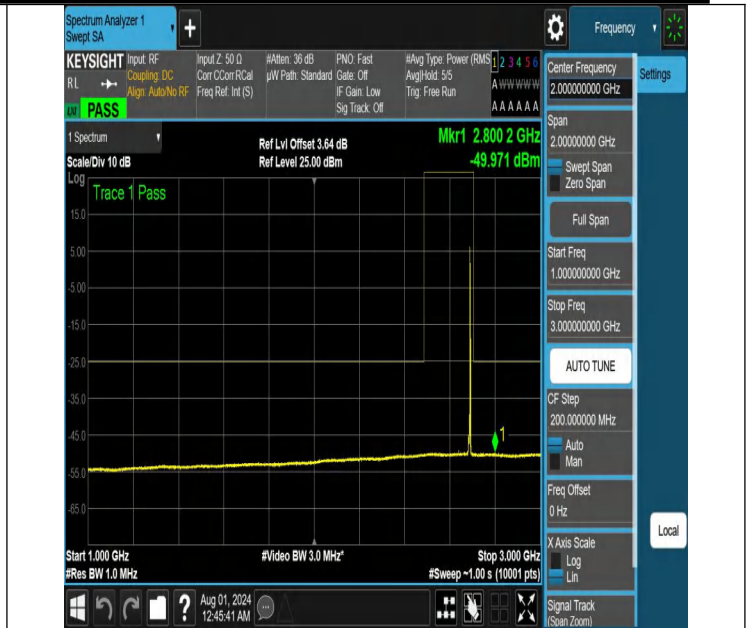
NTNV-N41-PC2-30-10-H-DFT-QPSK-Edge_1RB_Right-1000-300-0-Ant1-PASS
