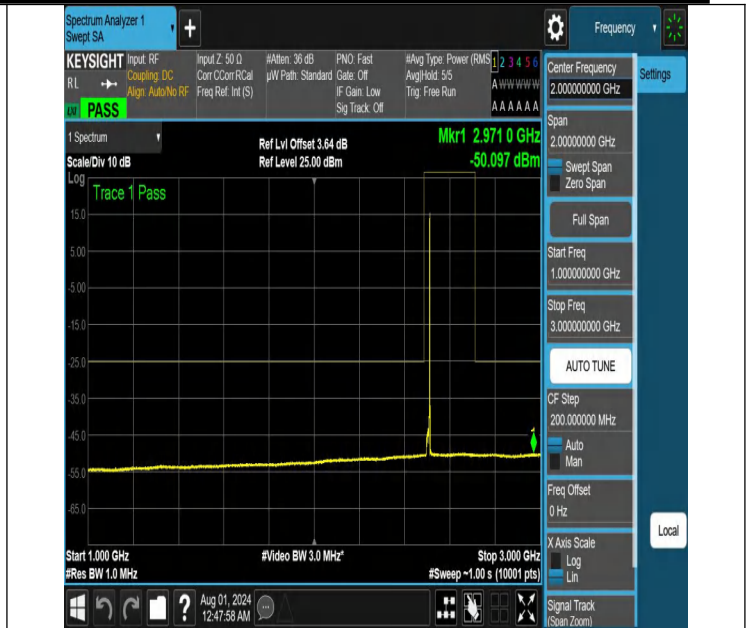
NTNV-N41-PC2-30-15-L-DFT-PI2BPSK-Edge_1RB_Right-1000-3000-Ant1-PASS
