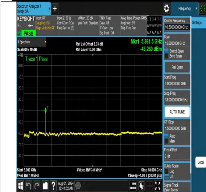
NTNV-N41-PC2-30-10-H-DFT-QPSK-Edge_1RB_Left-3000-1800 0-Ant1-PASS
