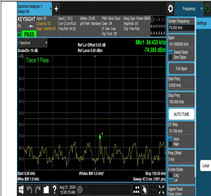
NTNV-N41-PC2-30-10-H-DFT-QPSK-Edge_1RB_Right-0.009-0.1 5-Ant1-PASS
