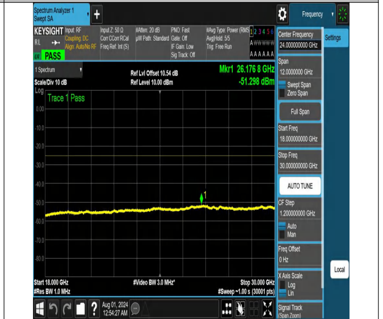
NTNV-N41-PC2-30-15-M-DFT-PI2BPSK-Edge_1RB_Right-18000-30000-Ant1-PASS
