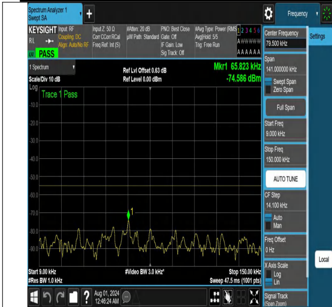
NTNV-N41-PC2-30-15-L-DFT-PI2BPSK-Edge_1RB_Left-0.009-0.15-Ant1-PASS
