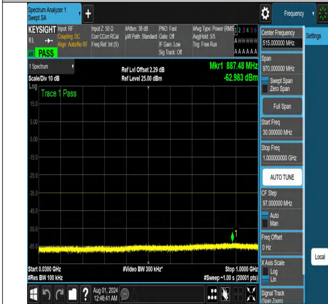
NTNV-N41-PC2-30-15-L-DFT-PI2BPSK-Edge_1RB_Left-30-1000-Ant1-PASS
