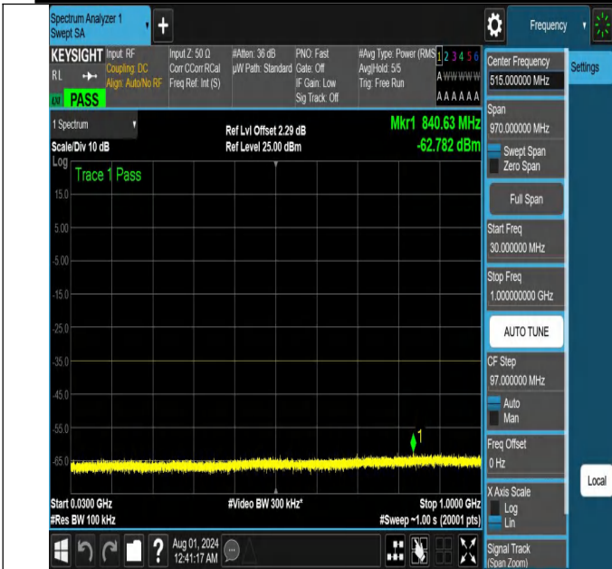
NTNV-N41-PC2-30-10-M-DFT-QPSK-Edge_1RB_Right-30-1000-Ant1-PASS
