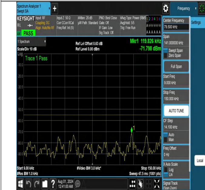
NTNV-N41-PC2-30-10-M-DFT-QPSK-Edge_1RB_Right-0.009-0. 15-Ant1-PASS
