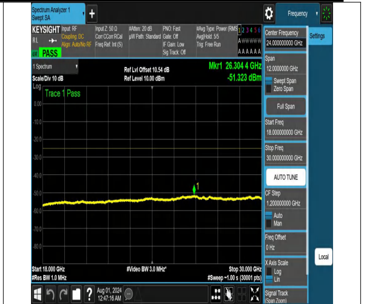
NTNV-N41-PC2-30-15-L-DFT-PI2BPSK-Edge_1RB_Left-18000-30000-Ant1-PASS
