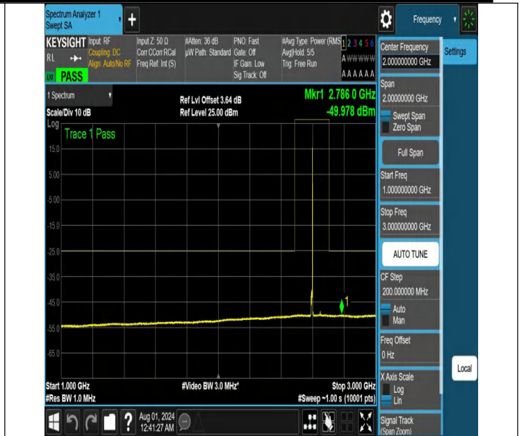
NTNV-N41-PC2-30-10-M-DFT-QPSK-Edge_1RB_Right-1000-300-Ant1-PASS
