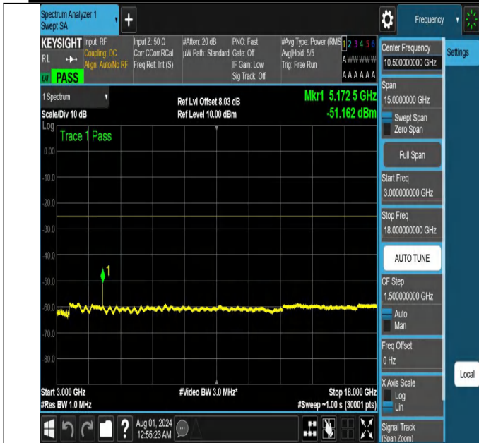
NTNV-N41-PC2-30-15-M-DFT-QPSK-Edge_1RB_Left-3000-1800 0-Ant1-PASS
