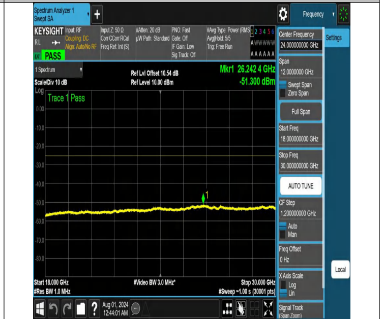
NTNV-N41-PC2-30-10-H-DFT-PI2BPSK-Edge_1RB_Right-18000- 30000-Ant1-PASS
