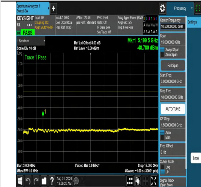
NTNV-N41-PC2-30-15-M-DFT-QPSK-Edge_1RB_Right-3000-18000-Ant1-PASS
