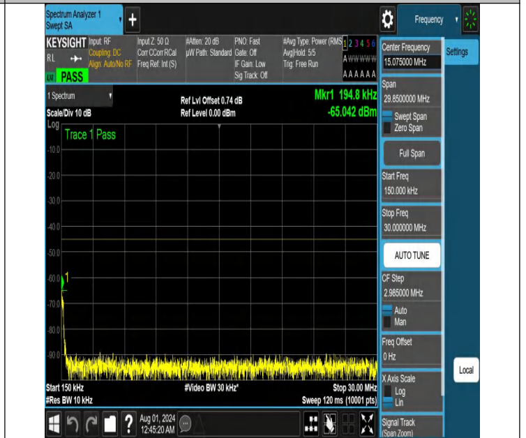
NTNV-N41-PC2-30-10-H-DFT-QPSK-Edge_1RB_Right-0.15-30-A nt1-PASS
