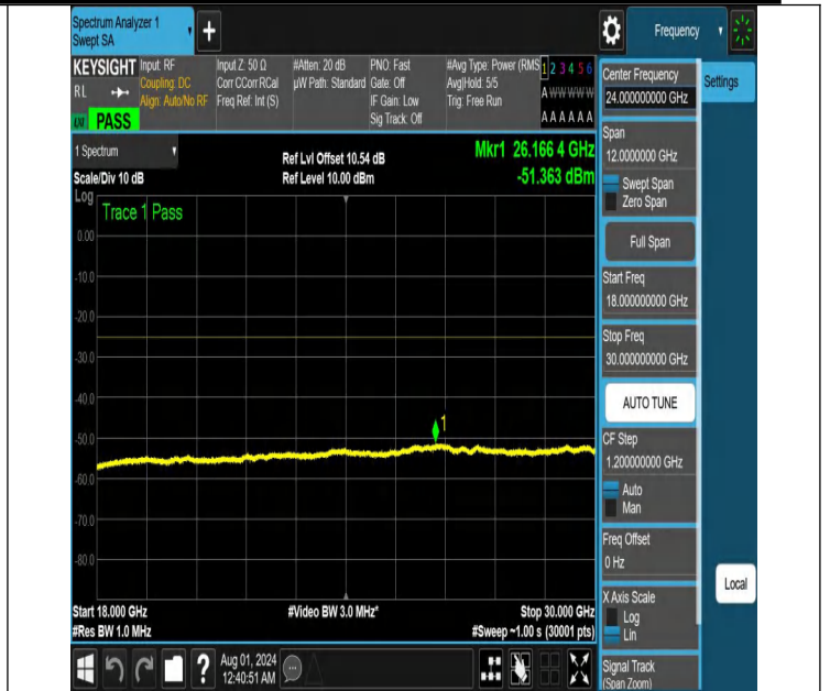
NTNV-N41-PC2-30-10-M-DFT-QPSK-Edge_1RB_Left-18000-300 00-Ant1-PASS
