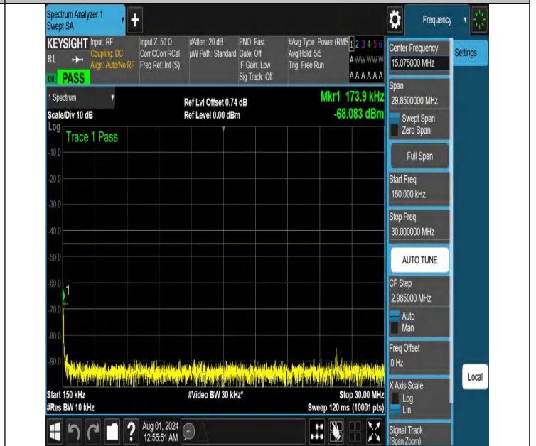
NTNV-N41-PC2-30-15-M-DFT-QPSK-Edge_1RB_Right-0.15-30-A nt1-PASS
