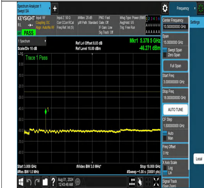
NTNV-N41-PC2-30-10-H-DFT-PI2BPSK-Edge_1RB_Right-3000- 18000-Ant1-PASS
