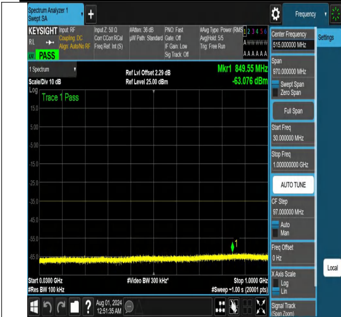
NTNV-N41-PC2-30-15-L-DFT-QPSK-Edge_1RB_Right-30-1000-Ant1-PASS
