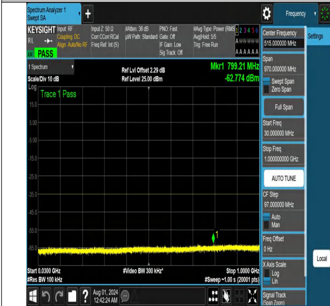
NTNV-N41-PC2-30-10-H-DFT-PI2BPSK-Edge_1RB_Left-30-1000-Ant1-PASS
