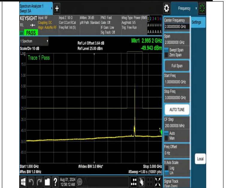
NTNV-N41-PC2-30-15-M-DFT-QPSK-Edge_1RB_Right-1000-300-0-Ant1-PASS
