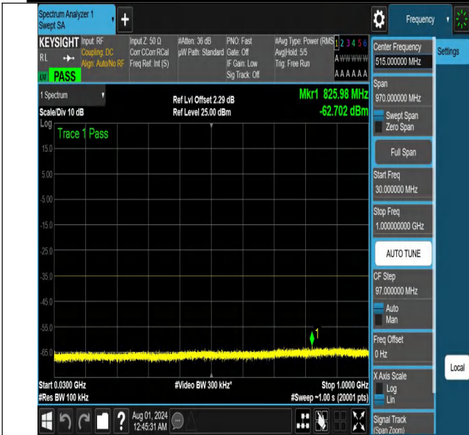
NTNV-N41-PC2-30-10-H-DFT-QPSK-Edge_1RB_Right-30-1000-Ant1-PASS
