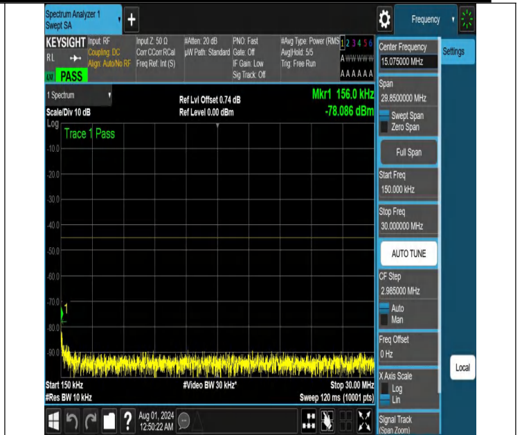
NTNV-N41-PC2-30-15-L-DFT-QPSK-Edge_1RB_Left-0.15-30-Ant1-PASS
