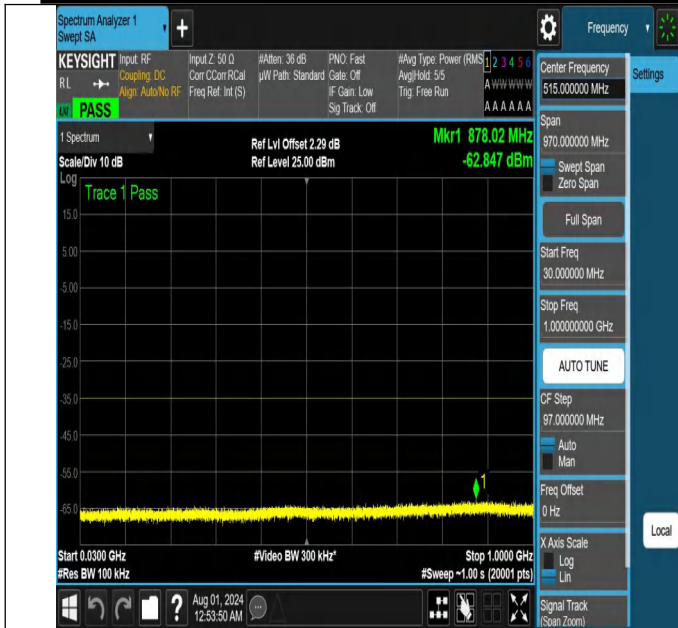
NTNV-N41-PC2-30-15-M-DFT-PI2BPSK-Edge_1RB_Right-30-1000-Ant1-PASS
