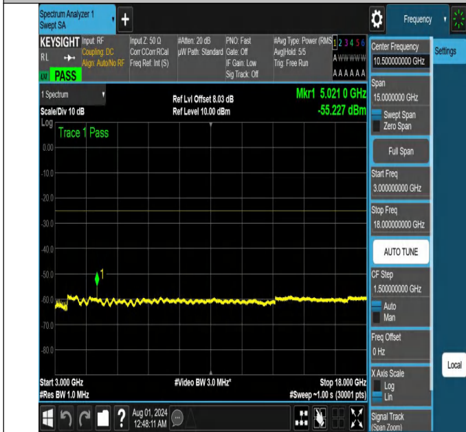
NTNV-N41-PC2-30-15-L-DFT-PI2BPSK-Edge_1RB_Right-3000-18000-Ant1-PASS
