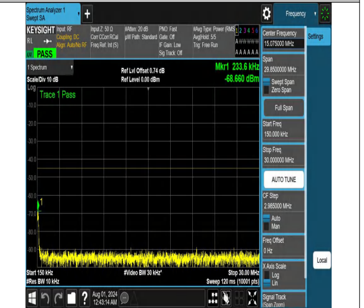
NTNV-N41-PC2-30-10-H-DFT-PI2BPSK-Edge_1RB_Right-0.15-3 0-Ant1-PASS
