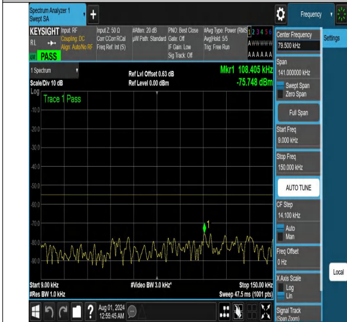
NTNV-N41-PC2-30-15-M-DFT-QPSK-Edge_1RB_Right-0.009-0. 15-Ant1-PASS
