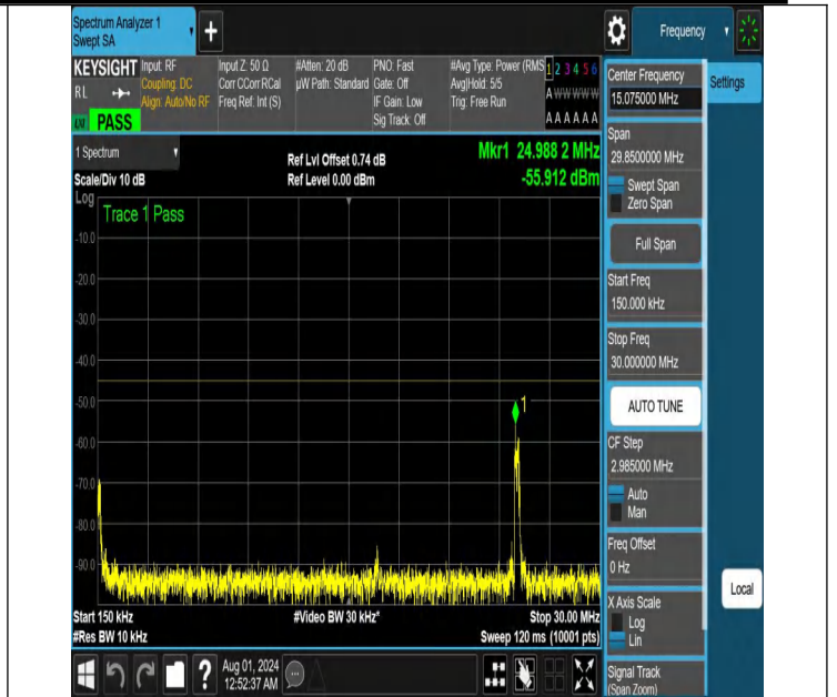
NTNV-N41-PC2-30-15-M-DFT-PI2BPSK-Edge_1RB_Left-0.15-30-Ant1-PASS
