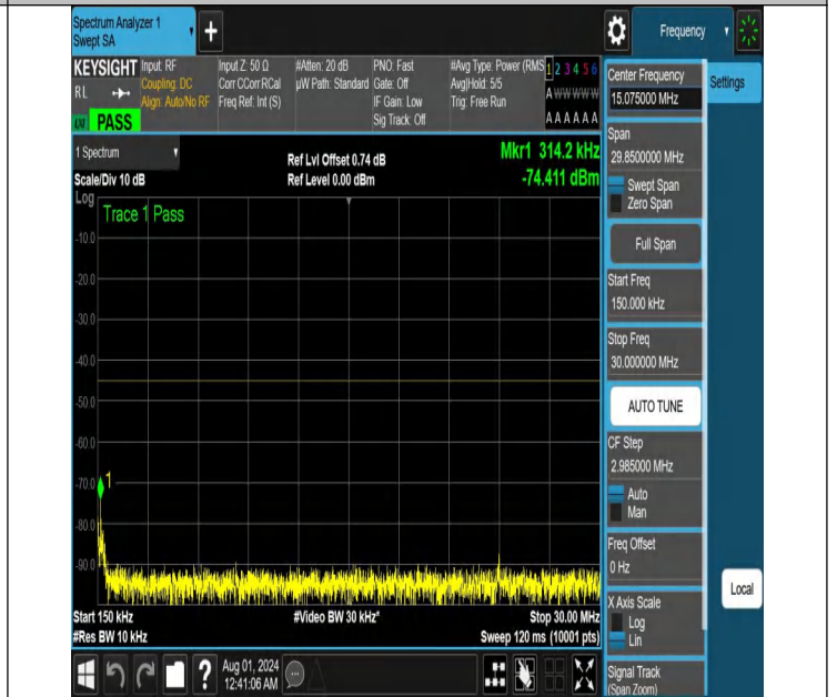
NTNV-N41-PC2-30-10-M-DFT-QPSK-Edge_1RB_Right-0.15-30-A nt1-PASS
