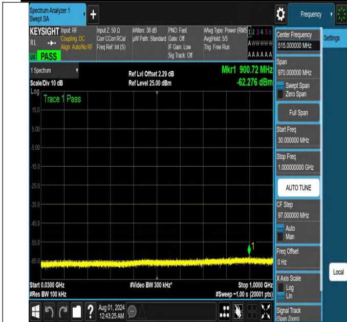
NTNV-N41-PC2-30-10-H-DFT-PI2BPSK-Edge_1RB_Right-30-10 00-Ant1-PASS
