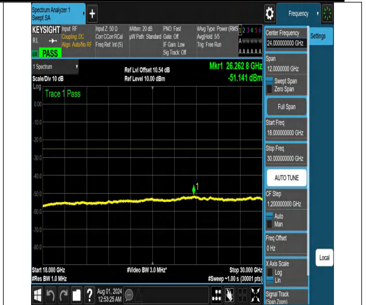
NTNV-N41-PC2-30-15-M-DFT-PI2BPSK-Edge_1RB_Left-18000-3 0000-Ant1-PASS
