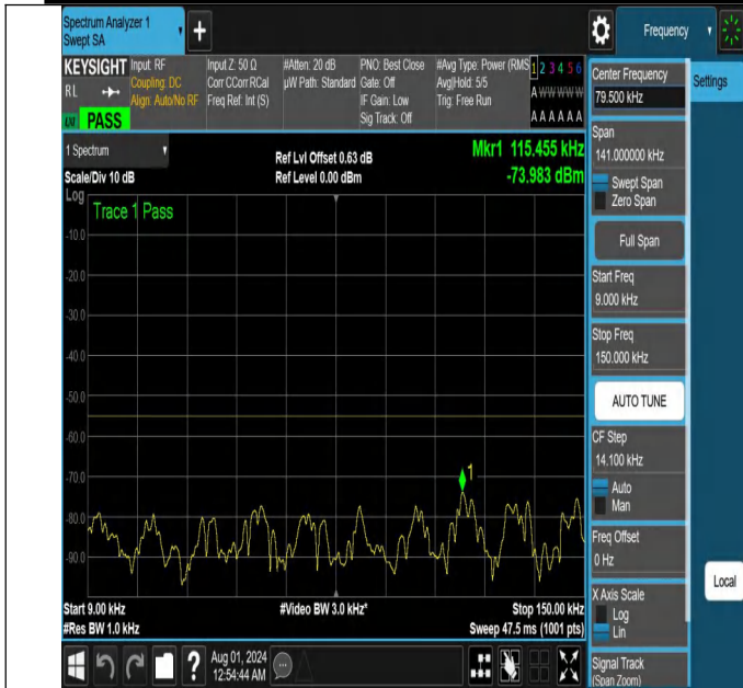
NTNV-N41-PC2-30-15-M-DFT-QPSK-Edge_1RB_Left-0.009-0.15 -Ant1-PASS
