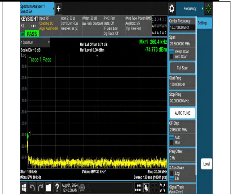
NTNV-N41-PC2-30-15-L-DFT-PI2BPSK-Edge_1RB_Left-0.15-30-Ant1-PASS
