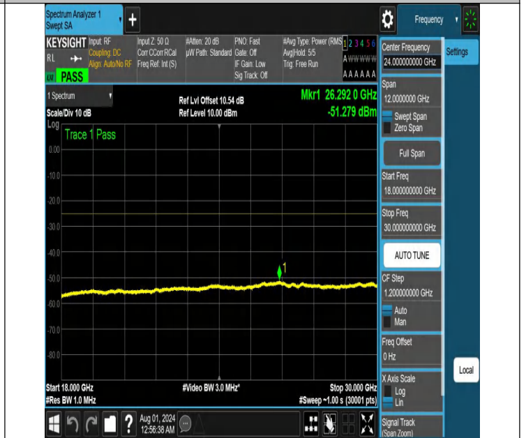
NTNV-N41-PC2-30-15-M-DFT-QPSK-Edge_1RB_Right-18000-30000-Ant1-PASS
