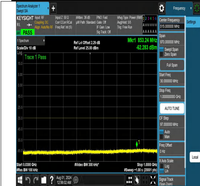
NTNV-N41-PC2-30-15-M-DFT-QPSK-Edge_1RB_Right-30-1000-Ant1-PASS
