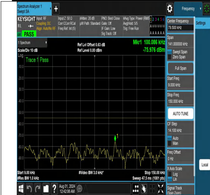
NTNV-N41-PC2-30-10-H-DFT-PI2BPSK-Edge_1RB_Left-0.009-0.15-Ant1-PASS
