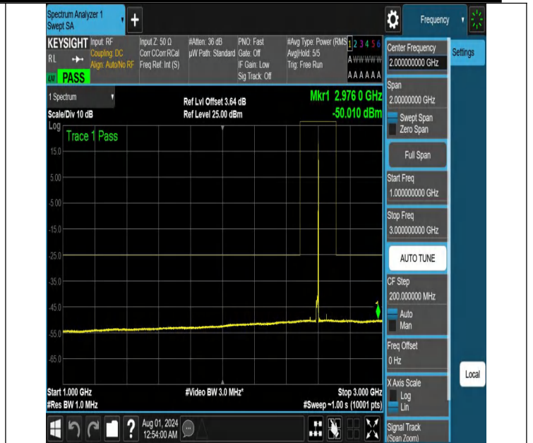
NTNV-N41-PC2-30-15-M-DFT-PI2BPSK-Edge_1RB_Right-1000-3000-Ant1-PASS
