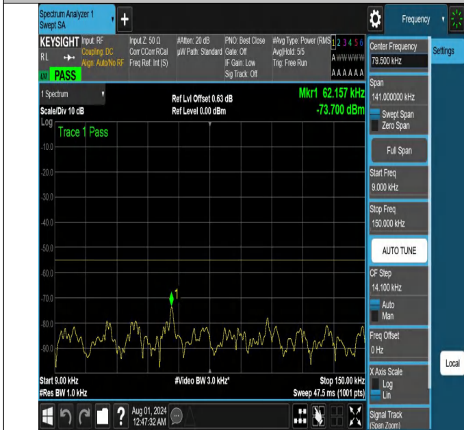
NTNV-N41-PC2-30-15-L-DFT-PI2BPSK-Edge_1RB_Right-0.009-150.000-Ant1-PASS
