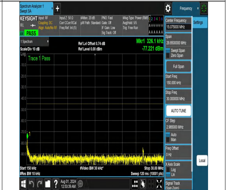
NTNV-N41-PC2-30-15-M-DFT-PI2BPSK-Edge_1RB_Right-0.15-3 0-Ant1-PASS
