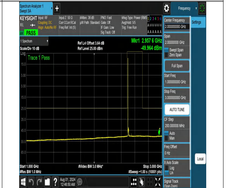
NTNV-N41-PC2-30-15-L-DFT-PI2BPSK-Edge_1RB_Left-1000-3000-Ant1-PASS
