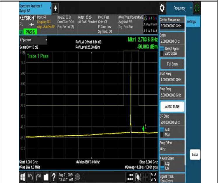
NTNV-N41-PC2-30-15-M-DFT-QPSK-Edge_1RB_Left-1000-3000-Ant1-PASS
