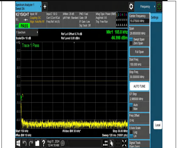
NTNV-N41-PC2-30-10-H-DFT-QPSK-Edge_1RB_Left-0.15-30-Ant 1-PASS
