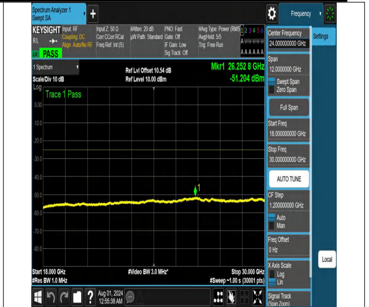
NTNV-N41-PC2-30-15-M-DFT-QPSK-Edge_1RB_Left-18000-300 00-Ant1-PASS
