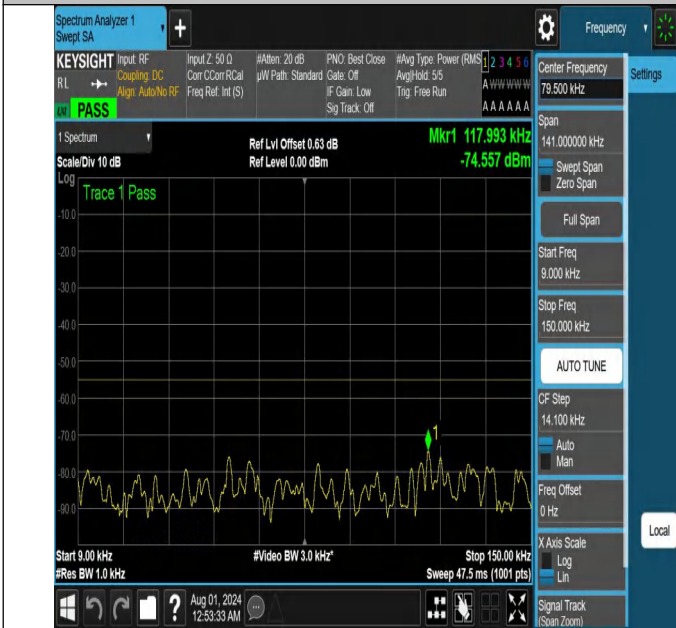
NTNV-N41-PC2-30-15-M-DFT-PI2BPSK-Edge_1RB_Right-0.009 -0.15-Ant1-PASS
