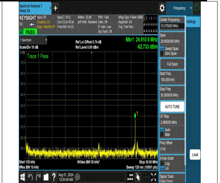
NTNV-N41-PC2-30-15-M-DFT-QPSK-Edge_1RB_Left-0.15-30-Ant 1-PASS
