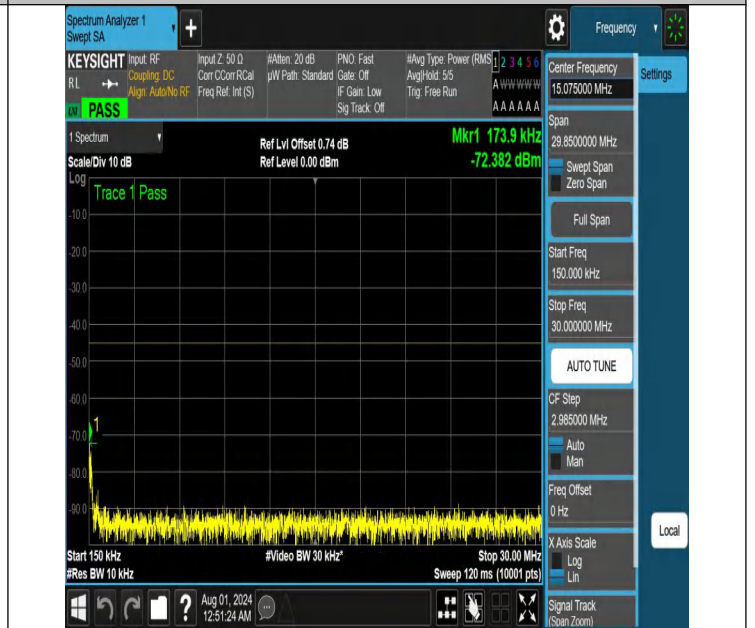
NTNV-N41-PC2-30-15-L-DFT-QPSK-Edge_1RB_Right-0.15-30-A nt1-PASS
