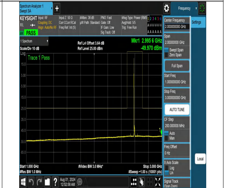
NTNV-N41-PC2-30-15-M-DFT-PI2BPSK-Edge_1RB_Left-1000-3000-Ant1-PASS
