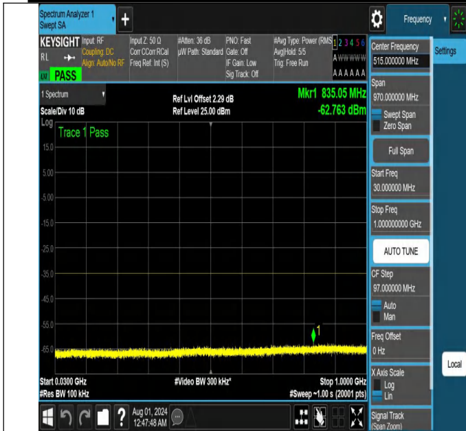
NTNV-N41-PC2-30-15-L-DFT-PI2BPSK-Edge_1RB_Right-30-1000-Ant1-PASS
