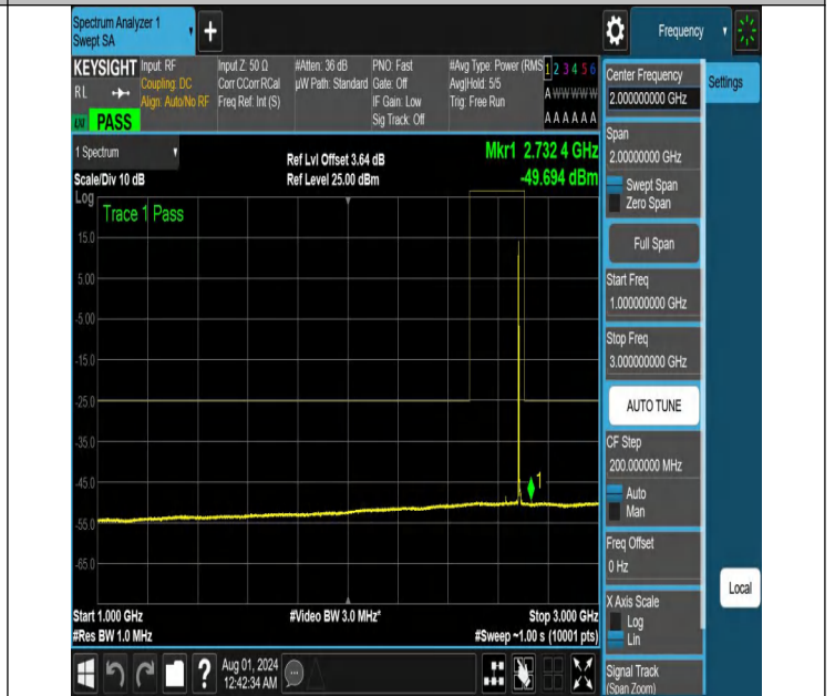
NTNV-N41-PC2-30-10-H-DFT-PI2BPSK-Edge_1RB_Left-1000-3000-Ant1-PASS
