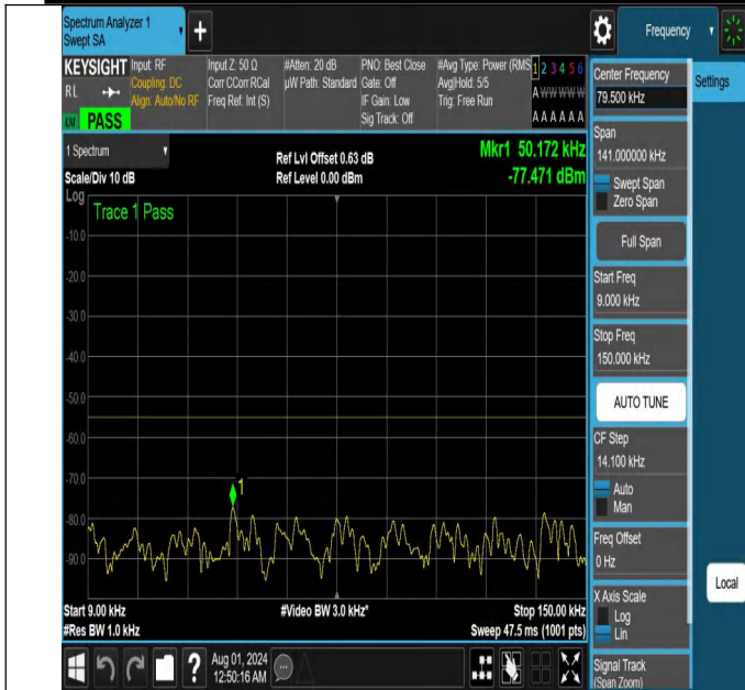
NTNV-N41-PC2-30-15-L-DFT-QPSK-Edge_1RB_Left-0.009-0.15-Ant1-PASS
