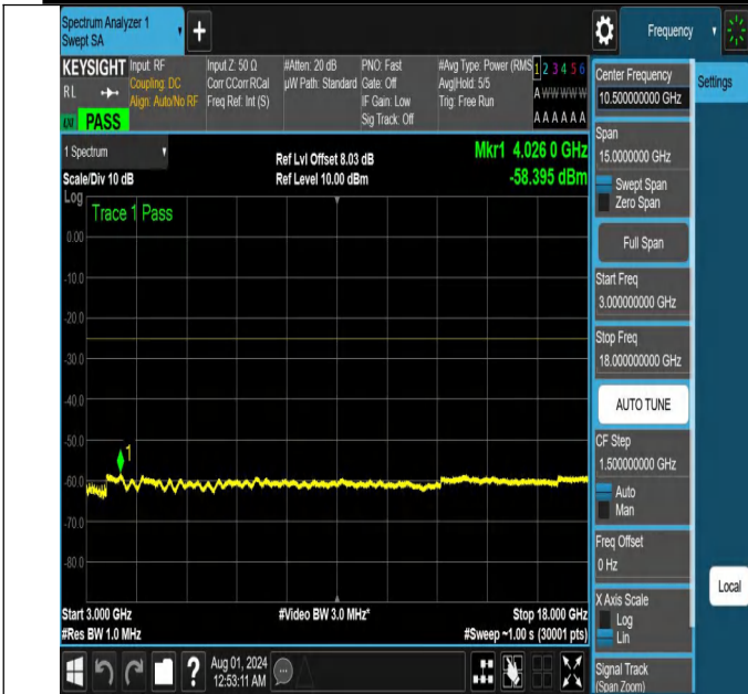
NTNV-N41-PC2-30-15-M-DFT-PI2BPSK-Edge_1RB_Left-3000-1 8000-Ant1-PASS
