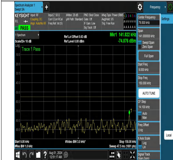
NTNV-N41-PC2-30-15-L-DFT-QPSK-Edge_1RB_Right-0.009-0.1 5-Ant1-PASS
