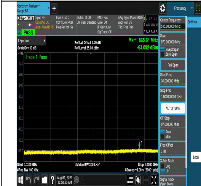
NTNV-N41-PC2-30-15-L-DFT-QPSK-Edge_1RB_Left-30-1000-Ant1-PASS
