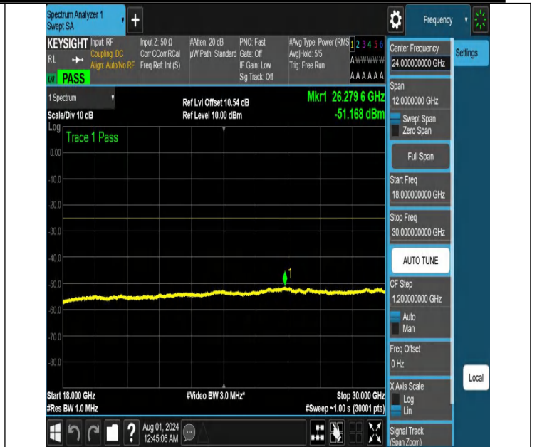
NTNV-N41-PC2-30-10-H-DFT-QPSK-Edge_1RB_Left-1800-3000 0-Ant1-PASS
