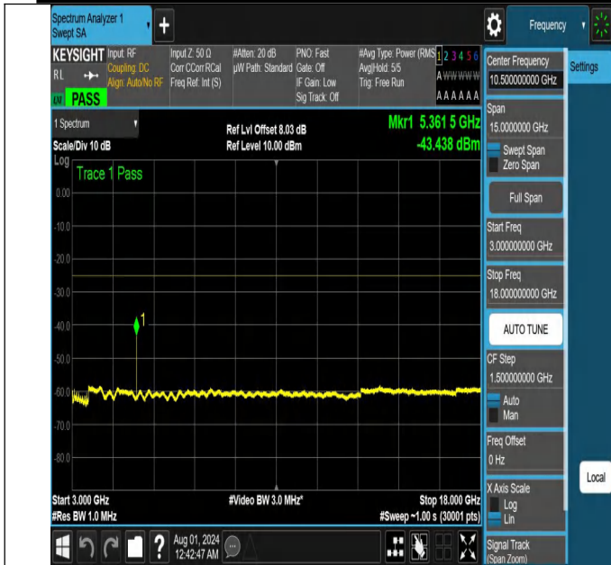
NTNV-N41-PC2-30-10-H-DFT-PI2BPSK-Edge_1RB_Left-3000-1 8000-Ant1-PASS
