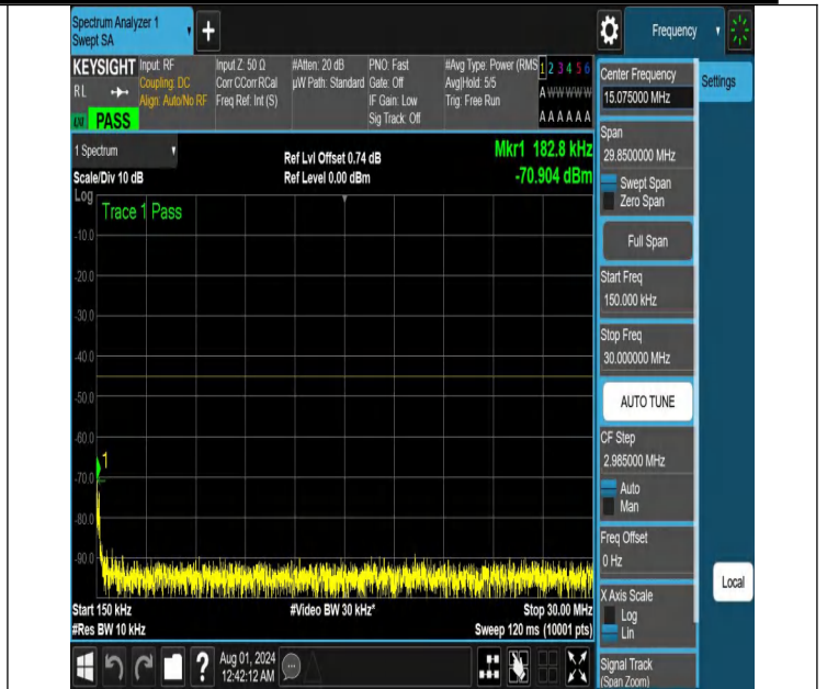
NTNV-N41-PC2-30-10-H-DFT-PI2BPSK-Edge_1RB_Left-0.15-30-Ant1-PASS
