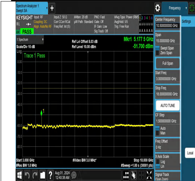
NTNV-N41-PC2-30-10-M-DFT-QPSK-Edge_1RB_Left-3000-1800 0-Ant1-PASS
