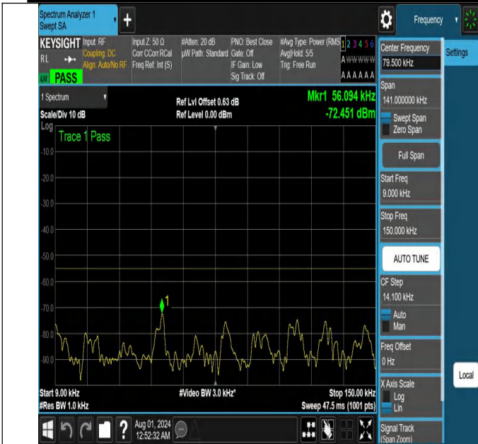
NTNV-N41-PC2-30-15-M-DFT-PI2BPSK-Edge_1RB_Left-0.009-0.15-Ant1-PASS
