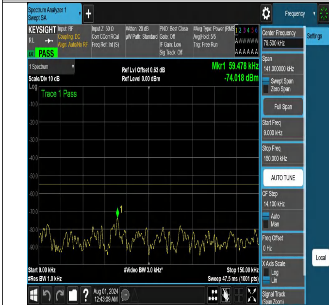
NTNV-N41-PC2-30-10-H-DFT-PI2BPSK-Edge_1RB_Right-0.009- 0.15-Ant1-PASS
