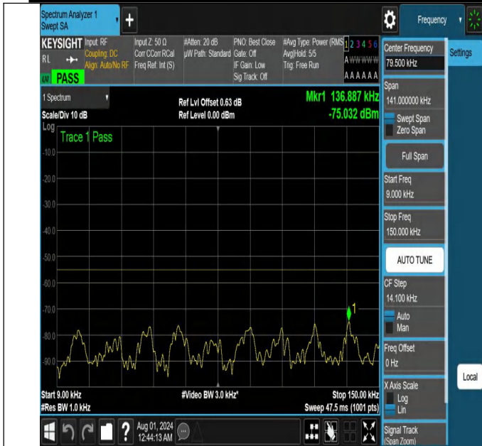
NTNV-N41-PC2-30-10-H-DFT-QPSK-Edge_1RB_Left-0.009-0.15 -Ant1-PASS
