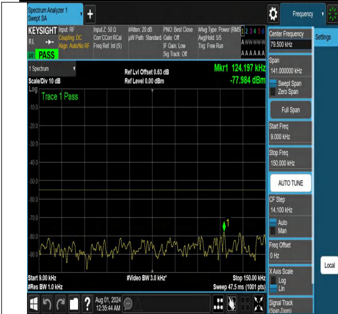
NTNV-N41-PC2-30-10-L-DFT-QPSK-Edge_1RB_Left-0.009-0.15-Ant1-PASS
