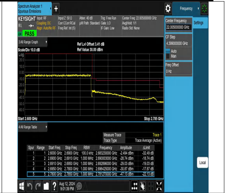
NTNV-N41-PC2-30-90-H-DFT-QPSK-Outer_Full-Ant1-PASS
