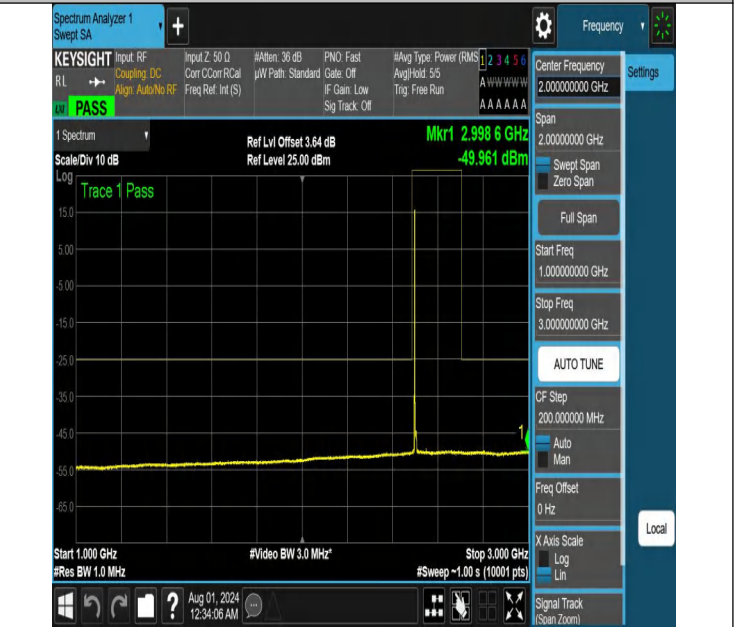
NTNV-N41-PC2-30-10-L-DFT-PI2BPSK-Edge_1RB_Left-1000-3000-Ant1-PASS
