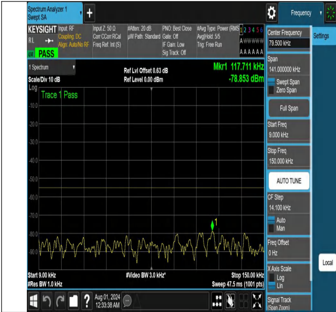
NTNV-N41-PC2-30-10-L-DFT-PI2BPSK-Edge_1RB_Left-0.009-0.15-Ant1-PASS
