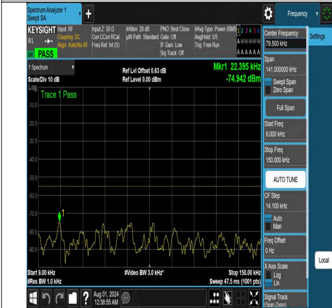
NTNV-N41-PC2-30-10-M-DFT-PI2BPSK-Edge_1RB_Right-0.009 -0.15-Ant1-PASS
