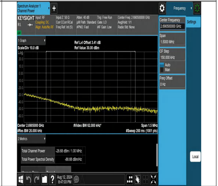
NTNV-N41-PC2-30-70-H-DFT-QPSK-Edge_1RB_Right-Ant1-PA SS
