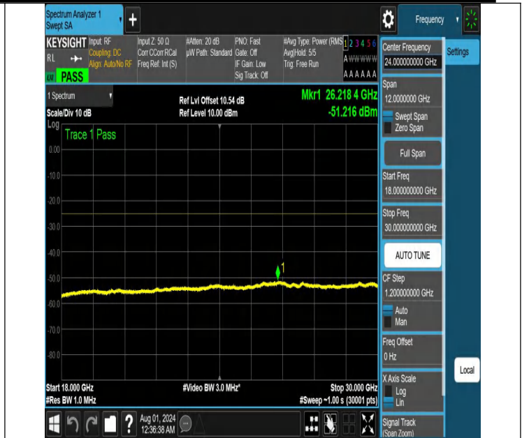
NTNV-N41-PC2-30-10-L-DFT-QPSK-Edge_1RB_Left-18000-3000 0-Ant1-PASS
