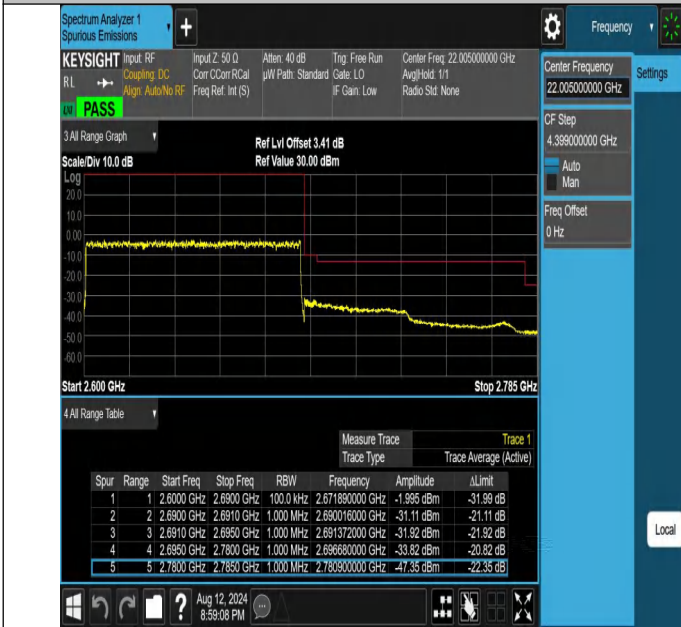
NTNV-N41-PC2-30-90-H-DFT-PI2BPSK-Outer_Full-Ant1-PASS
