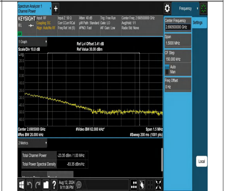
NTNV-N41-PC2-30-100-H-DFT-QPSK-Edge_1RB_Right-Ant1-PASS
