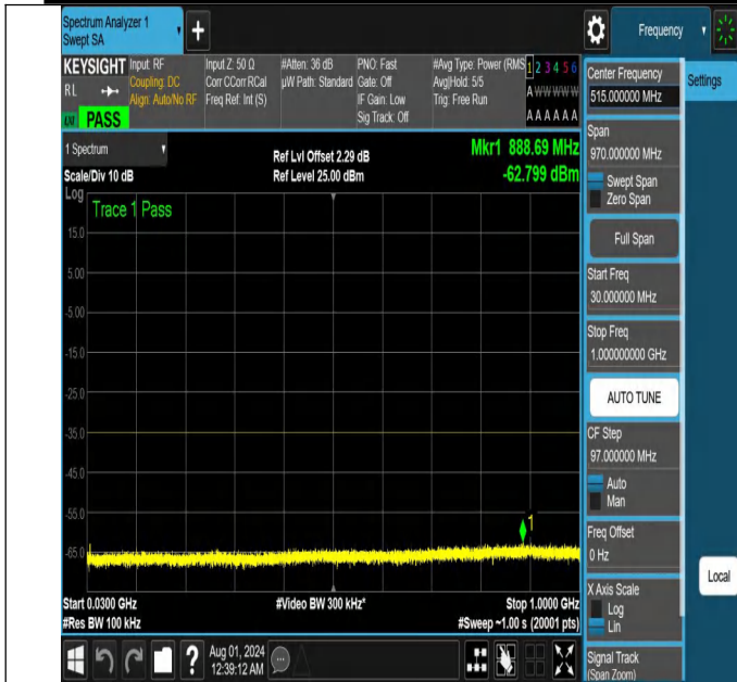
NTNV-N41-PC2-30-10-M-DFT-PI2BPSK-Edge_1RB_Right-30-10 00-Ant1-PASS
