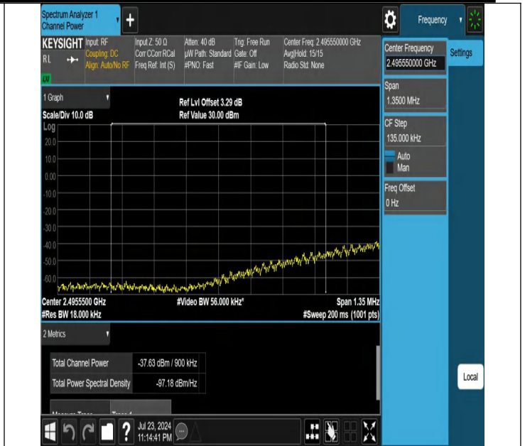
NTNV-N41-PC2-30-90-L-DFT-PI2BPSK-Edge_1RB_Left-Ant1-PA
