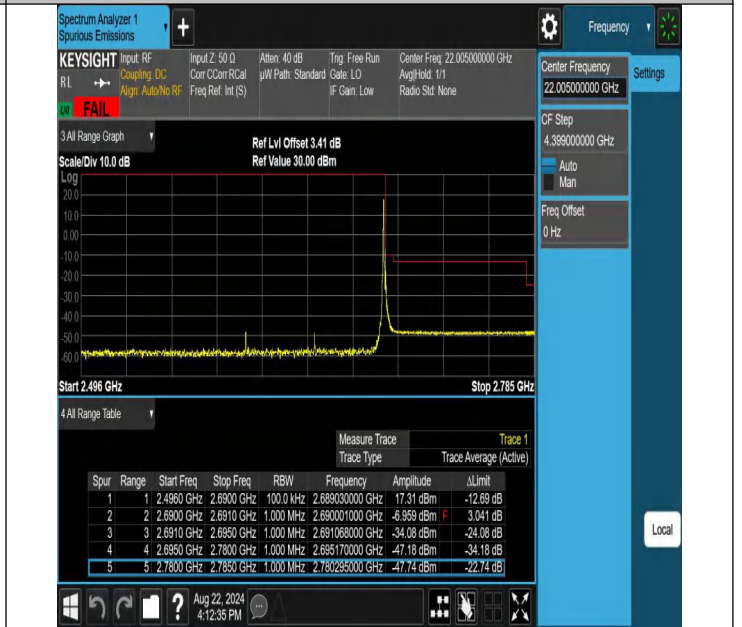
NTNV-N41-PC2-30-90-H-DFT-PI2BPSK-Edge_1RB_Right-Ant1-FAIL
