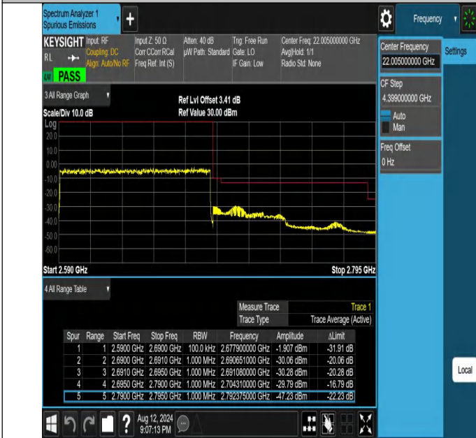
NTNV-N41-PC2-30-100-H-DFT-P12BPSK-Outer_Full-Ant1-PASS
