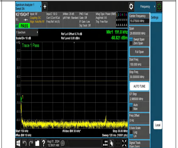
NTNV-N41-PC2-30-10-M-DFT-PI2BPSK-Edge_1RB_Right-0.15-3 0-Ant1-PASS
