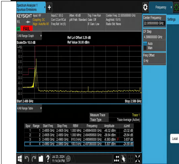
NTNV-N41-PC2-30-90-L-DFT-PI2BPSK-Edge_1RB_Left-Ant1-FAI
