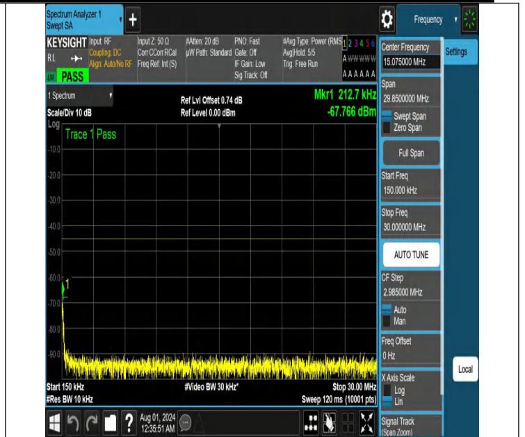
NTNV-N41-PC2-30-10-L-DFT-QPSK-Edge_1RB_Left-0.15-30-Ant 1-PASS
