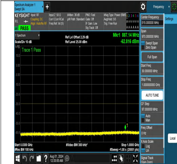
NTNV-N41-PC2-30-10-L-DFT-PI2BPSK-Edge_1RB_Left-30-1000-Ant1-PASS
