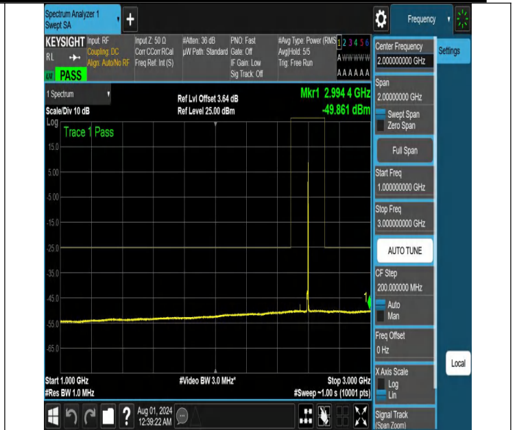
NTNV-N41-PC2-30-10-M-DFT-PI2BPSK-Edge_1RB_Right-1000-3 00-Ant1-PASS
