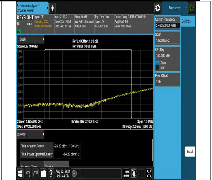
NTNV-N41-PC2-30-100-L-DFT-PI2BPSK-Edge_1RB_Left-Ant1-P
