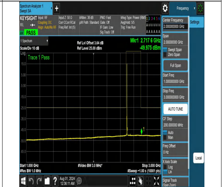
NTNV-N41-PC2-30-10-L-DFT-QPSK-Edge_1RB_Left-1000-3000-Ant1-PASS
