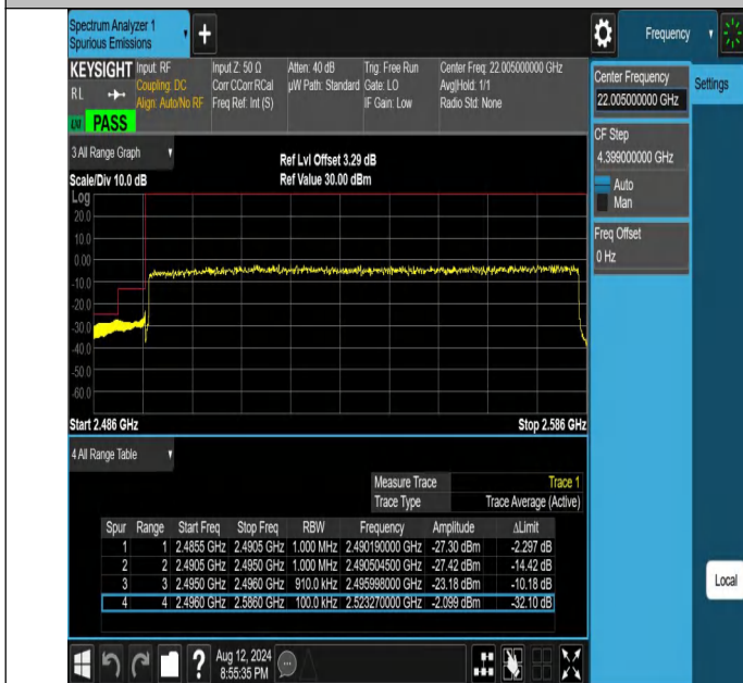
NTNV-N41-PC2-30-90-L-DFT-PI2BPSK-Outer_Full-Ant1-PASS
