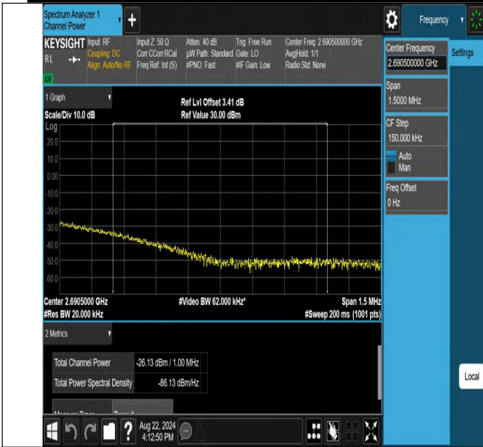
NTNV-N41-PC2-30-90-H-DFT-PI2BPSK-Edge_1RB_Right-Ant1-P ASS
