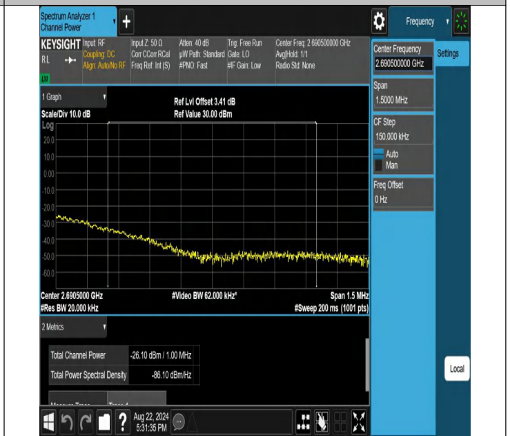
NTNV-N41-PC2-30-90-H-DFT-QPSK-Edge_1RB_Right-Ant1-PA SS
