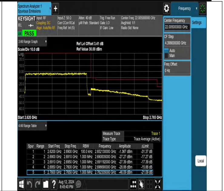
NTNV-N41-PC2-30-70-H-DFT-QPSK-Outer_Full-Ant1-PASS
