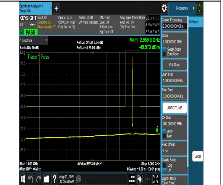
NTNV-N41-PC2-30-10-M-DFT-PI2BPSK-Edge_1RB_Left-1000-3000-Ant1-PASS
