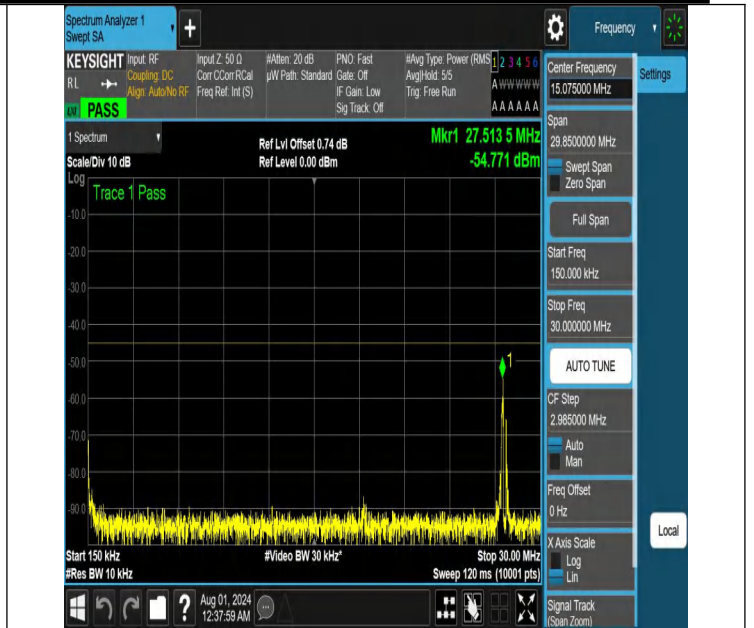
NTNV-N41-PC2-30-10-M-DFT-PI2BPSK-Edge_1RB_Left-0.15-30-Ant1-PASS
