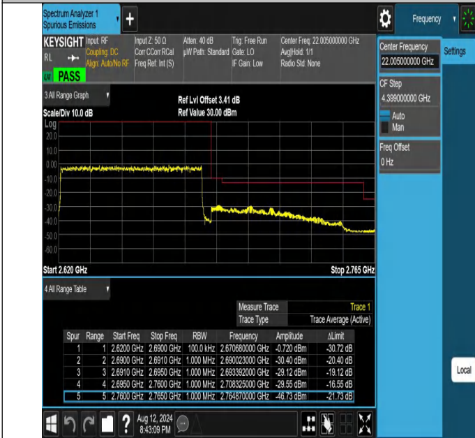
NTNV-N41-PC2-30-70-H-DFT-PI2BPSK-Outer_Full-Ant1-PASS
