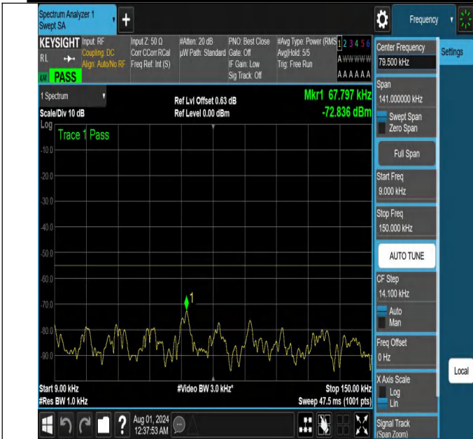
NTNV-N41-PC2-30-10-M-DFT-PI2BPSK-Edge_1RB_Left-0.009-0.15-Ant1-PASS
