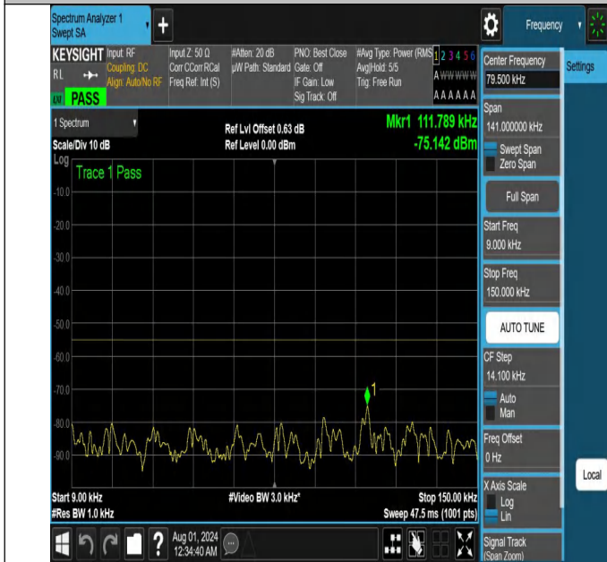
NTNV-N41-PC2-30-10-L-DFT-PI2BPSK-Edge_1RB_Right-0.009-0.15-Ant1-PASS
