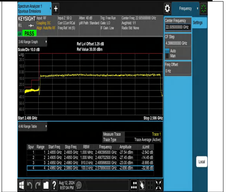
NTNV-N41-PC2-30-90-L-DFT-QPSK-Outer_Full-Ant1-PASS
