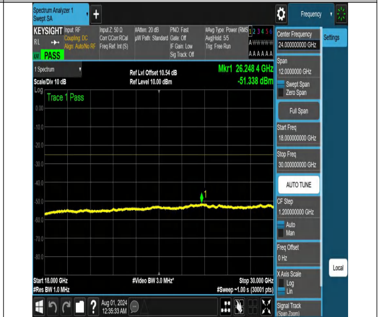
NTNV-N41-PC2-30-10-L-DFT-PI2BPSK-Edge_1RB_Right-18000- 30000-Ant1-PASS
