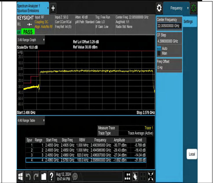
NTNV-N41-PC2-30-80-L-DFT-PI2BPSK-Outer_Full-Ant1-PASS
