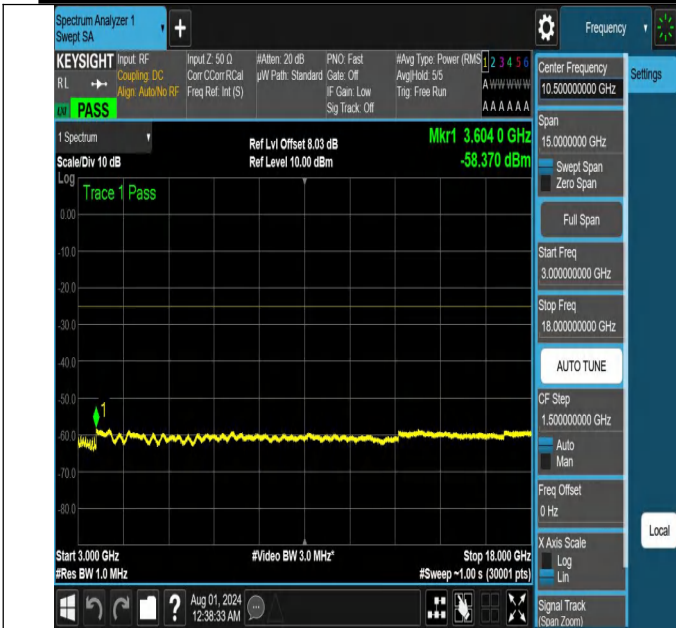
NTNV-N41-PC2-30-10-M-DFT-PI2BPSK-Edge_1RB_Left-3000-1 8000-Ant1-PASS
