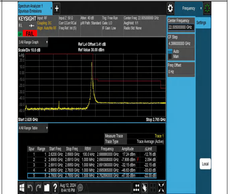
NTNV-N41-PC2-30-70-H-DFT-PI2BPSK-Edge_1RB_Right-Ant1-FAIL
