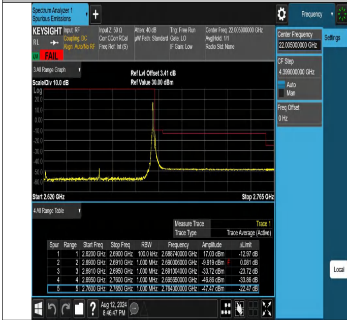
NTNV-N41-PC2-30-70-H-DFT-QPSK-Edge_1RB_Right-Ant1-FAIL
