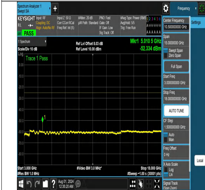
NTNV-N41-PC2-30-10-L-DFT-PI2BPSK-Edge_1RB_Right-3000- 18000-Ant1-PASS
