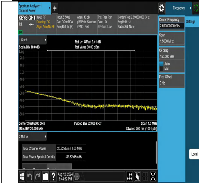
NTNV-N41-PC2-30-70-H-DFT-PI2BPSK-Edge_1RB_Right-Ant1-P ASS
