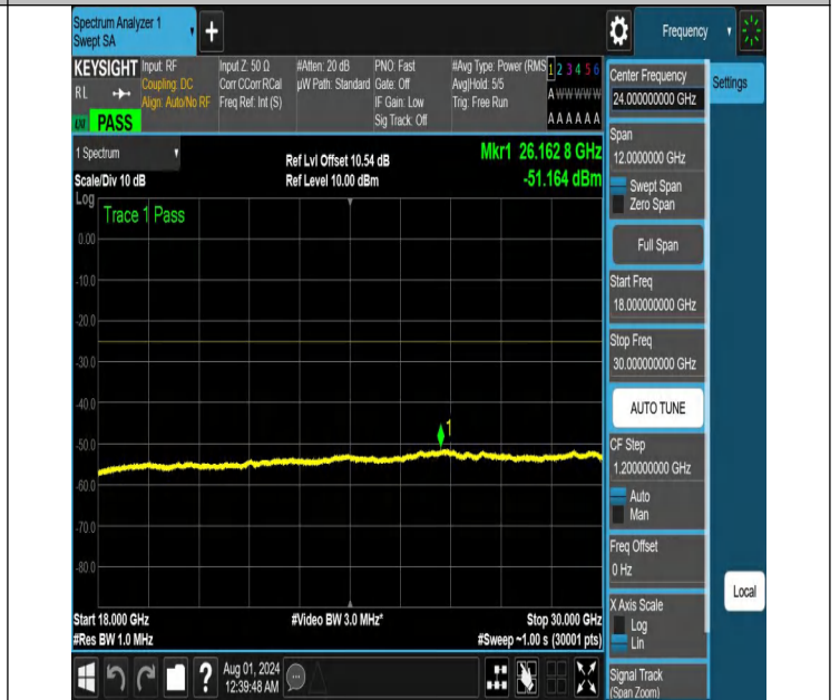
NTNV-N41-PC2-30-10-M-DFT-PI2BPSK-Edge_1RB_Right-18000- 30000-Ant1-PASS
