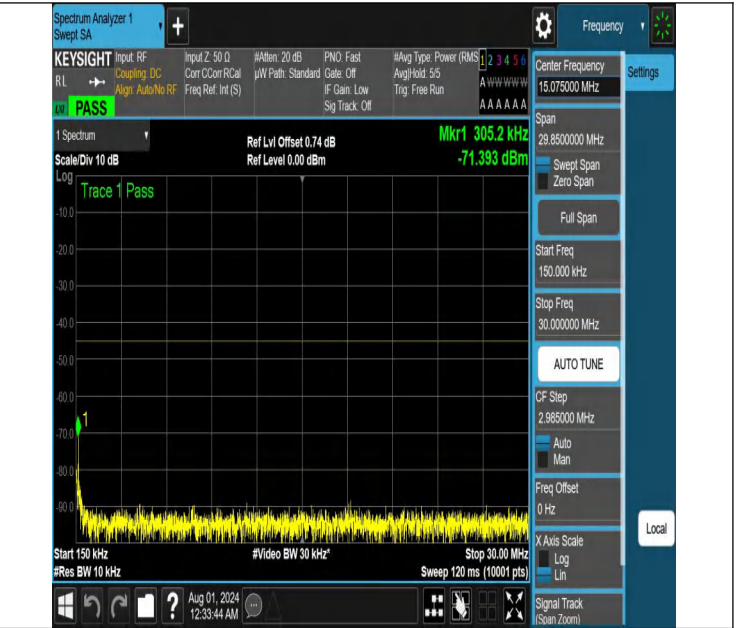
NTNV-N41-PC2-30-10-L-DFT-PI2BPSK-Edge_1RB_Left-0.15-30-Ant1-PASS
