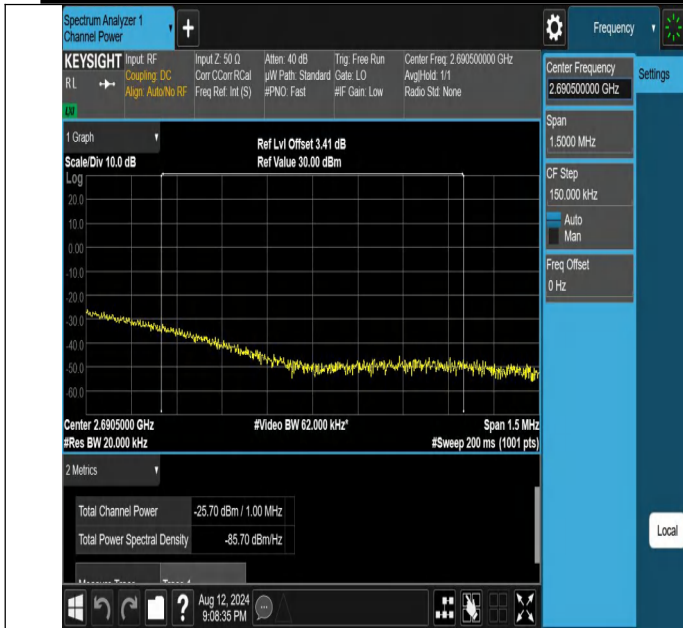
NTNV-N41-PC2-30-100-H-DFT-PI2BPSK-Edge_1RB_Right-Ant1-PASS
