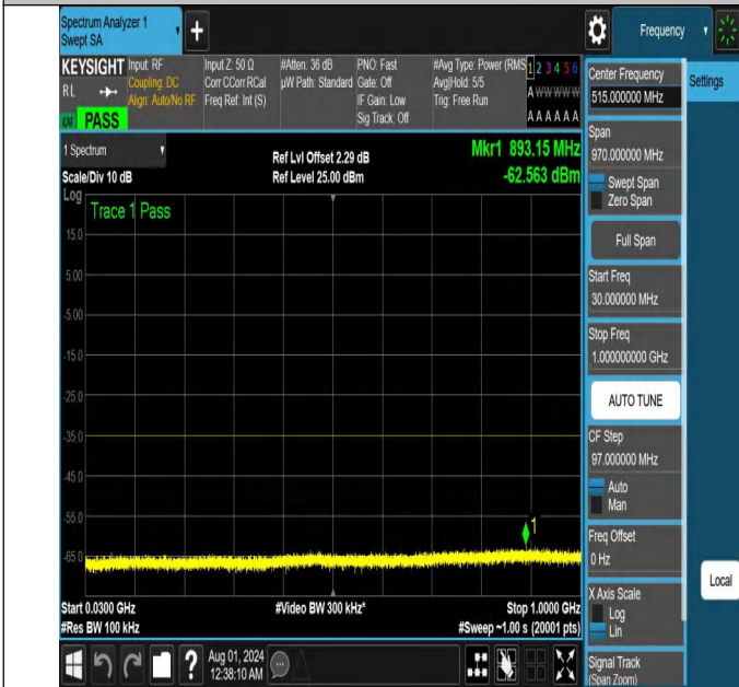
NTNV-N41-PC2-30-10-M-DFT-PI2BPSK-Edge_1RB_Left-30-1000-Ant1-PASS
