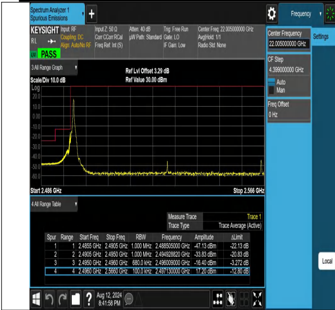
NTNV-N41-PC2-30-70-L-DFT-QPSK-Edge_1RB_Left-Ant1-PASS
