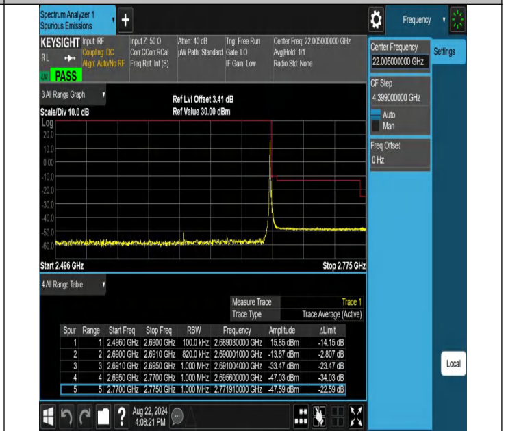
NTNV-N41-PC2-30-80-H-DFT-QPSK-Edge_1RB_Right-Ant1-PASS
