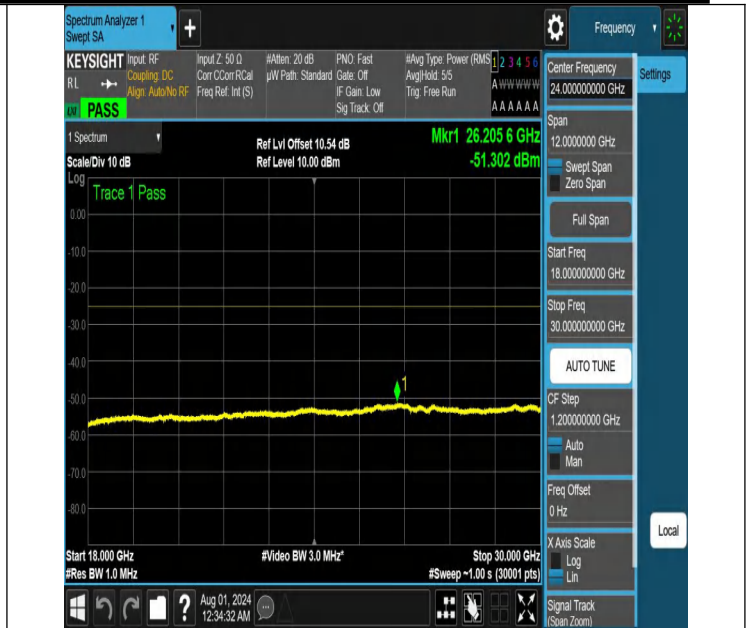
NTNV-N41-PC2-30-10-L-DFT-PI2BPSK-Edge_1RB_Left-18000-30000-Ant1-PASS
