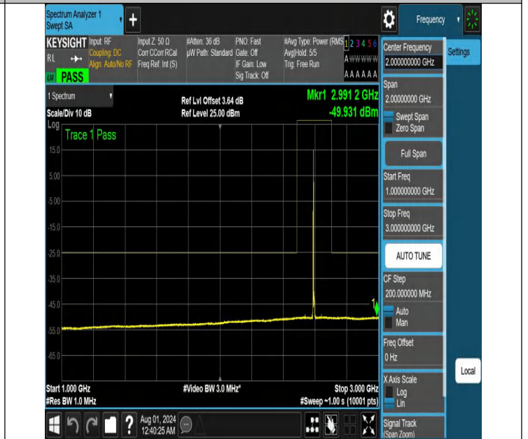
NTNV-N41-PC2-30-10-M-DFT-QPSK-Edge_1RB_Left-1000-3000-Ant1-PASS
