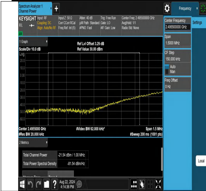
NTNV-N41-PC2-30-100-L-DFT-QPSK-Edge_1RB_Left-Ant1-PASS
