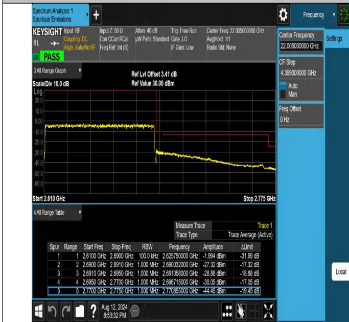
NTNV-N41-PC2-30-80-H-DFT-QPSK-Outer_Full-Ant1-PASS
