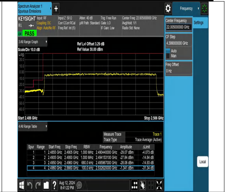
NTNV-N41-PC2-30-70-L-DFT-QPSK-Outer_Full-Ant1-PASS
