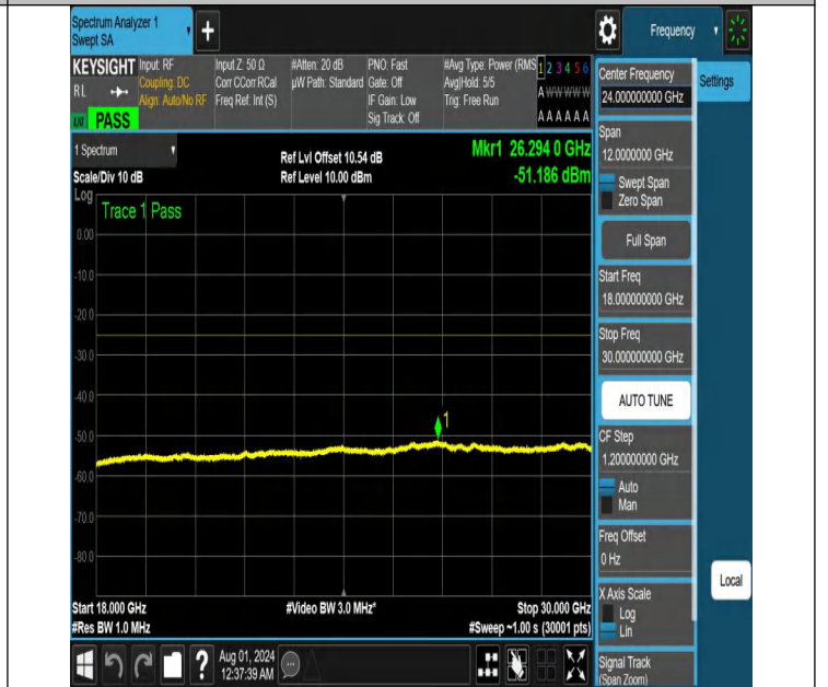
NTNV-N41-PC2-30-10-L-DFT-QPSK-Edge_1RB_Right-18000-30000-Ant1-PASS
