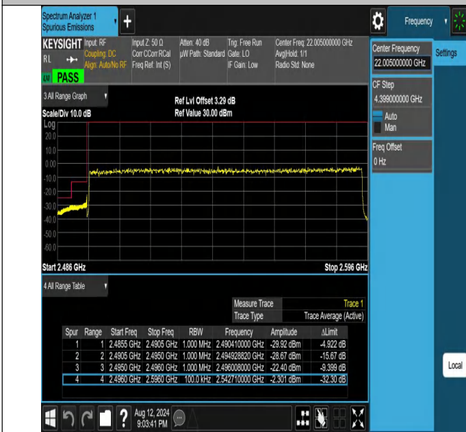
NTNV-N41-PC2-30-100-L-DFT-PI2BPSK-Outer_Full-Ant1-PASS
