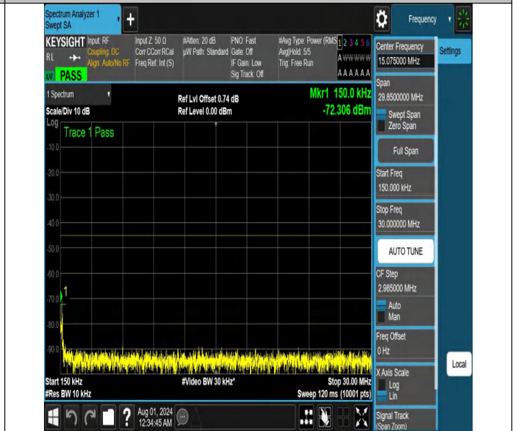
NTNV-N41-PC2-30-10-L-DFT-PI2BPSK-Edge_1RB_Right-0.15-30-Ant1-PASS
