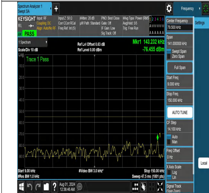
NTNV-N41-PC2-30-10-L-DFT-QPSK-Edge_1RB_Right-0.009-0.1 5-Ant1-PASS
