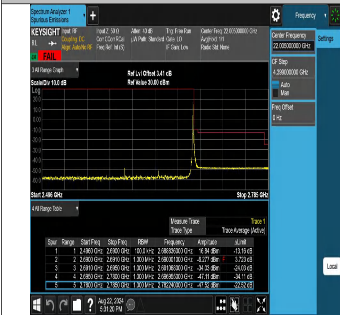
NTNV-N41-PC2-30-90-H-DFT-QPSK-Edge_1RB_Right-Ant1-FAIL
