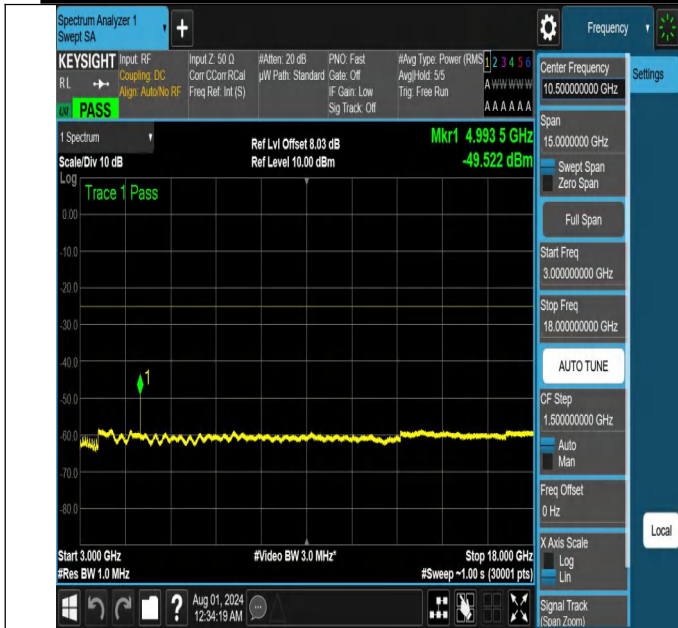
NTNV-N41-PC2-30-10-L-DFT-PI2BPSK-Edge_1RB_Left-3000-18000-Ant1-PASS
