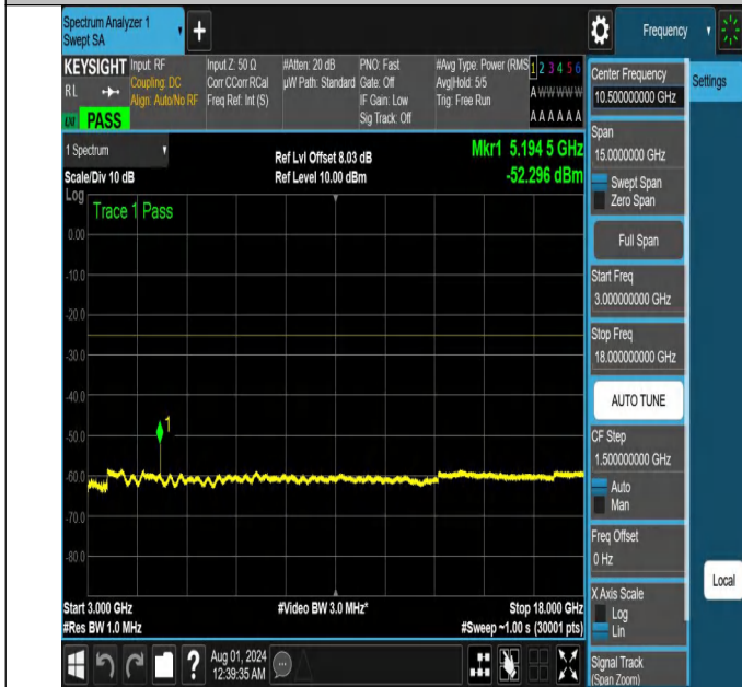
NTNV-N41-PC2-30-10-M-DFT-PI2BPSK-Edge_1RB_Right-3000- 18000-Ant1-PASS
