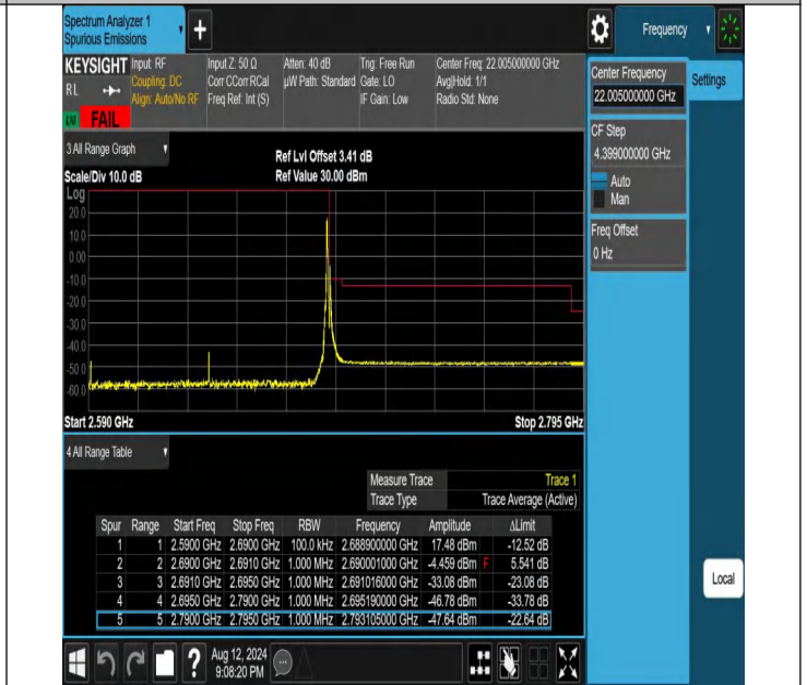
NTNV-N41-PC2-30-100-H-DFT-P12BPSK-Edge_1RB_Right-Ant1-FAIL
