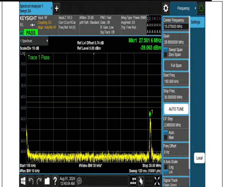
NTNV-N41-PC2-30-10-M-DFT-QPSK-Edge_1RB_Left-0.15-30-Ant 1-PASS
