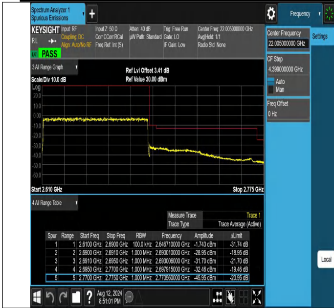
NTNV-N41-PC2-30-80-H-DFT-PI2BPSK-Outer_Full-Ant1-PASS
