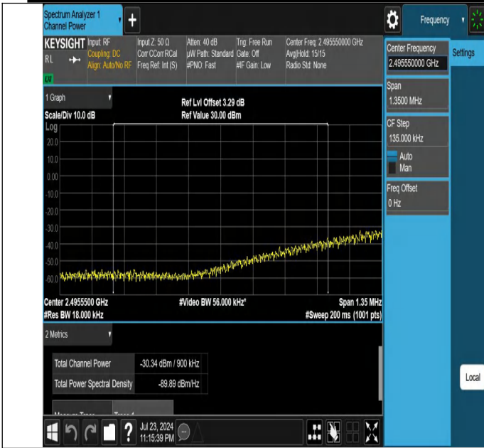
NTNV-N41-PC2-30-90-L-DFT-QPSK-Edge_1RB_Left-Ant1-PASS
