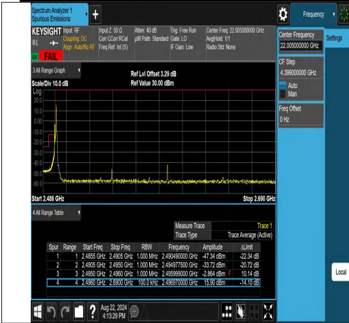
NTNV-N41-PC2-30-100-L-DFT-PI2BPSK-Edge_1RB_Left-Ant1-FA
