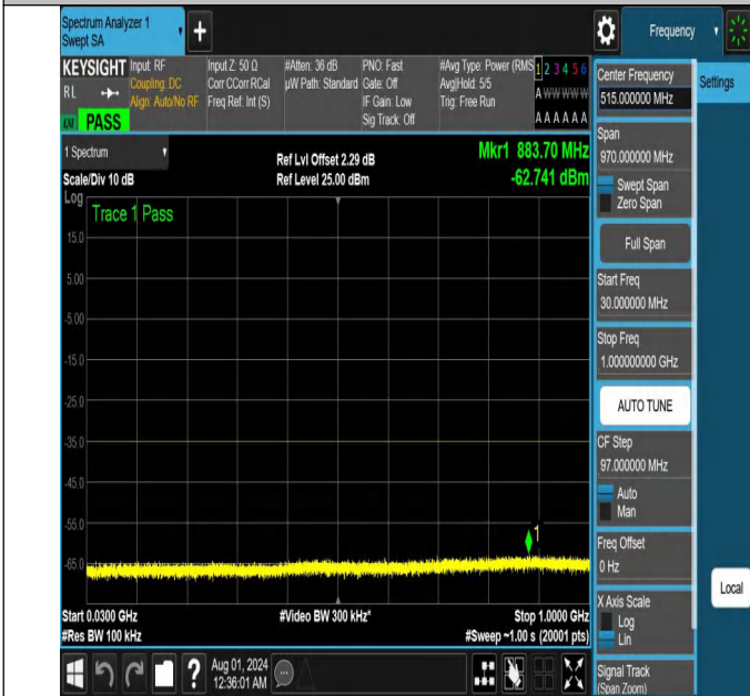
NTNV-N41-PC2-30-10-L-DFT-QPSK-Edge_1RB_Left-30-1000-Ant1-PASS
