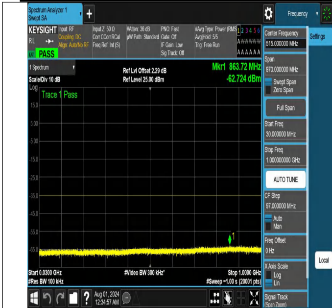
NTNV-N41-PC2-30-10-L-DFT-PI2BPSK-Edge_1RB_Right-30-10 00-Ant1-PASS
