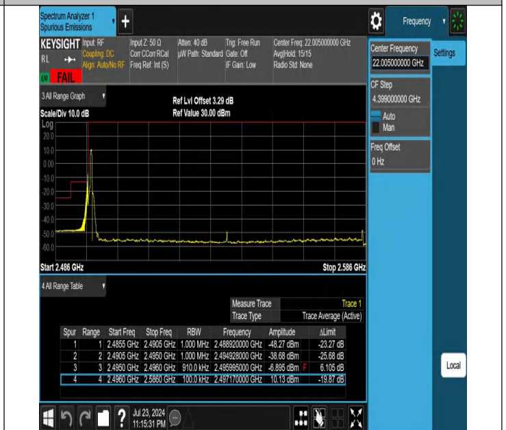
NTNV-N41-PC2-30-90-L-DFT-QPSK-Edge_1RB_Left-Ant1-FAIL
