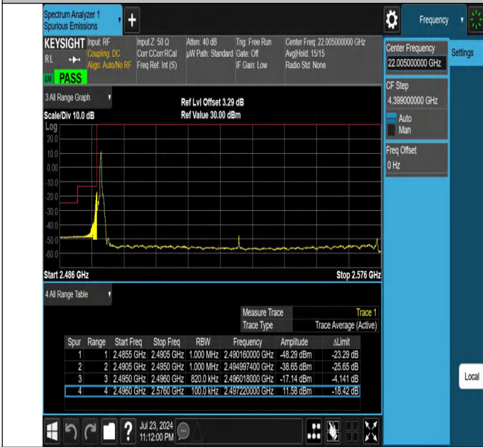
NTNV-N41-PC2-30-80-L-DFT-QPSK-Edge_1RB_Left-Ant1-PASS
