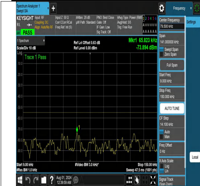
NTNV-N41-PC2-30-10-M-DFT-QPSK-Edge_1RB_Left-0.009-0.15 -Ant1-PASS
