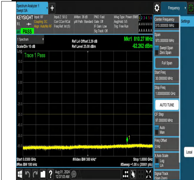
NTNV-N41-PC2-30-10-L-DFT-QPSK-Edge_1RB_Right-30-1000-Ant1-PASS
