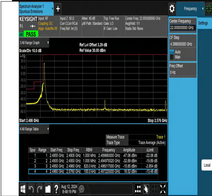
NTNV-N41-PC2-30-80-L-DFT-PI2BPSK-Edge_1RB_Left-Ant1-PA SS
