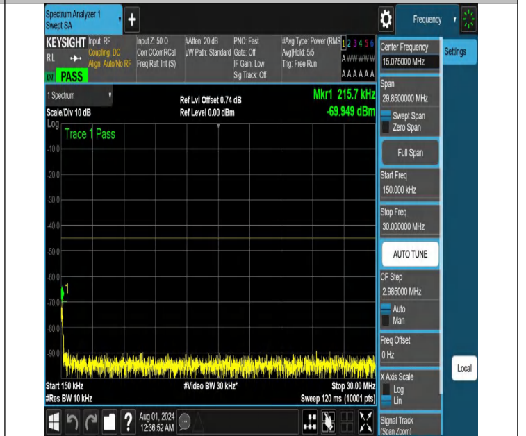
NTNV-N41-PC2-30-10-L-DFT-QPSK-Edge_1RB_Right-0.15-30-A nt1-PASS
