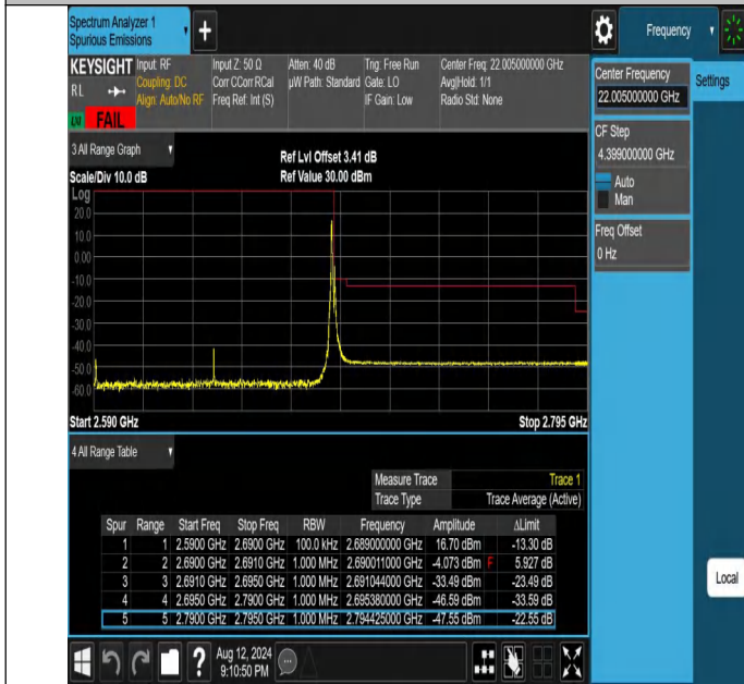
NTNV-N41-PC2-30-100-H-DFT-QPSK-Edge_1RB_Right-Ant1-FAIL
