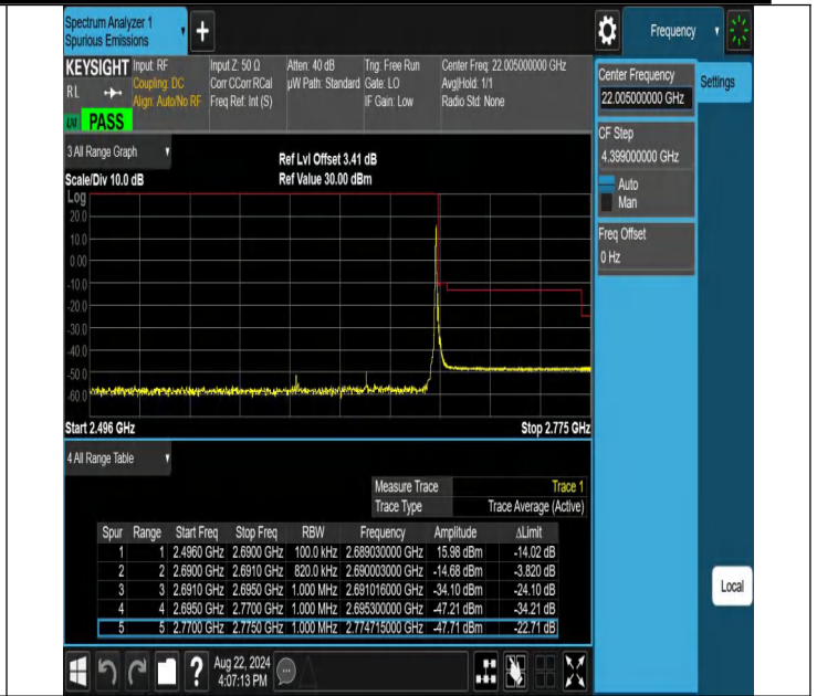
NTNV-N41-PC2-30-80-H-DFT-PI2BPSK-Edge_1RB_Right-Ant1-PASS
