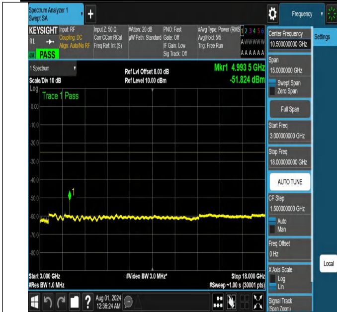
NTNV-N41-PC2-30-10-L-DFT-QPSK-Edge_1RB_Left-3000-1800 0-Ant1-PASS
