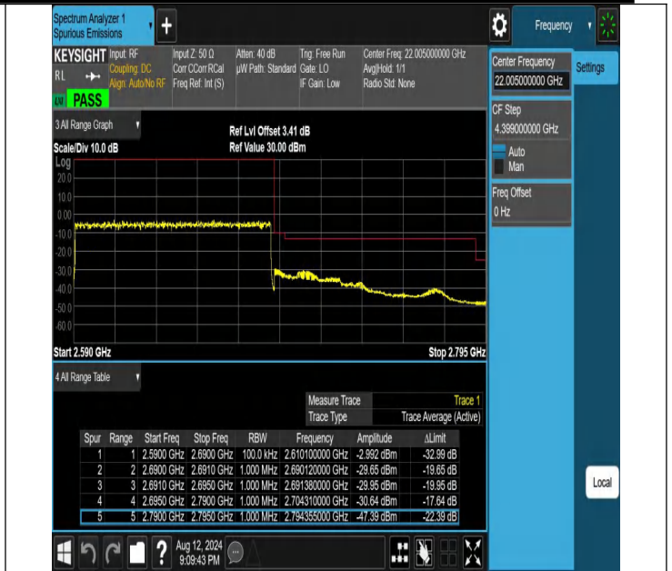
NTNV-N41-PC2-30-100-H-DFT-QPSK-Outer_Full-Ant1-PASS
