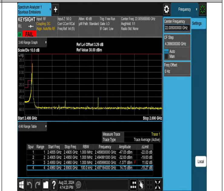
NTNV-N41-PC2-30-100-L-DFT-QPSK-Edge_1RB_Left-Ant1-FAIL
