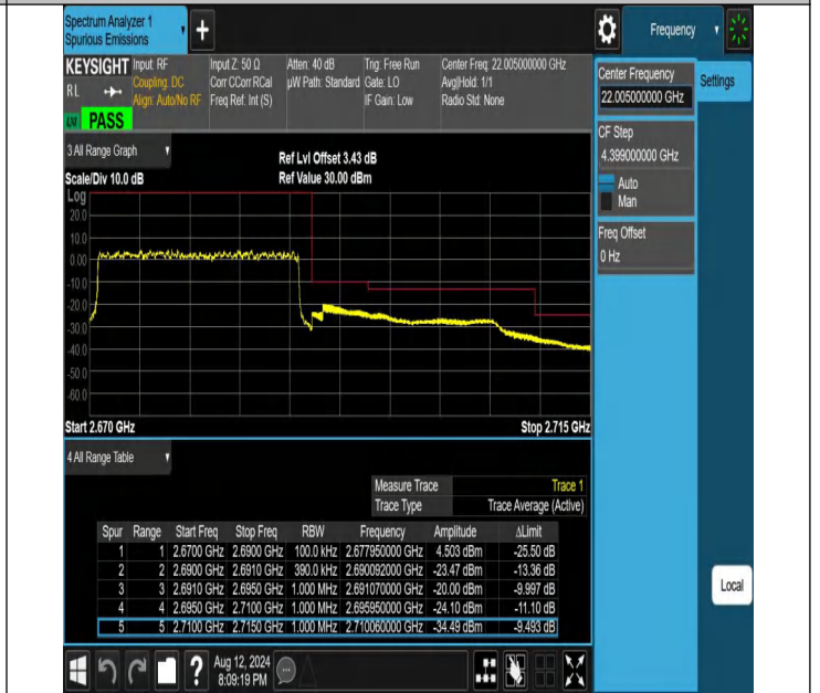
NTNV-N41-PC2-30-20-H-DFT-QPSK-Outter_Full-Ant1-PASS
