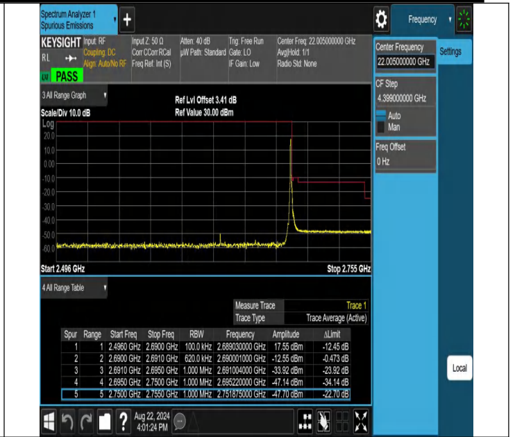
NTNV-N41-PC2-30-60-H-DFT-QPSK-Edge_1RB_Right-Ant1-PA SS
