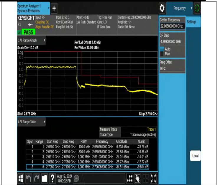
NTNV-N41-PC2-30-15-H-DFT-PI2BPSK-Outter_Full-Ant1-PASS
