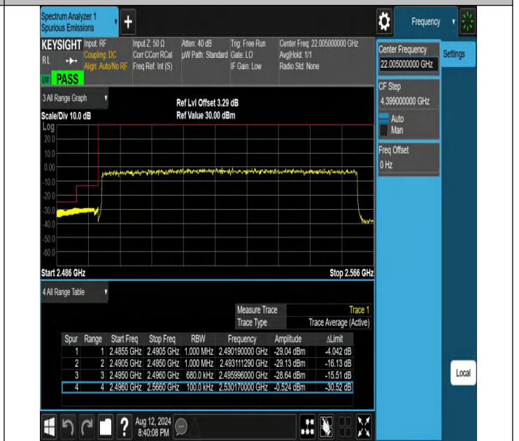
NTNV-N41-PC2-30-70-L-DFT-PI2BPSK-Outer_Full-Ant1-PASS
