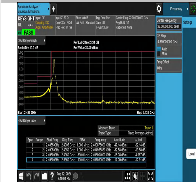
NTNV-N41-PC2-30-40-L-DFT-PI2BPSK-Edge_1RB_Left-Ant1-PASS
