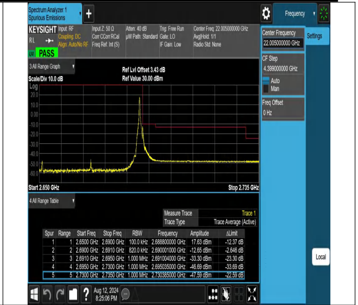
NTNV-N41-PC2-30-40-H-DFT-QPSK-Edge_1RB_Right-Ant1-PASS
