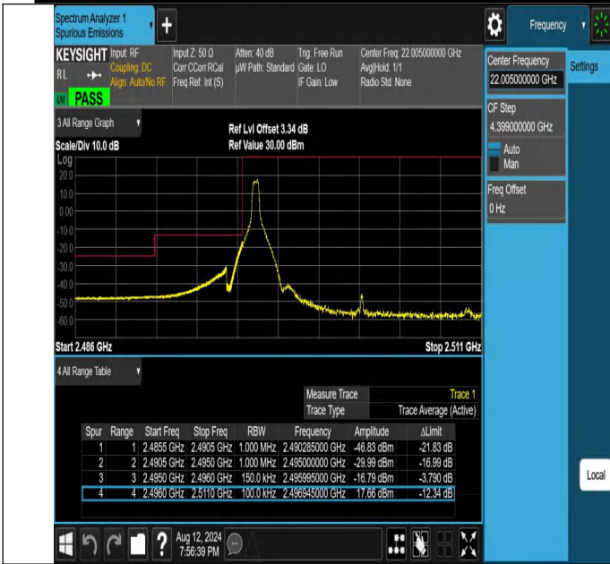
NTNV-N41-PC2-30-15-L-DFT-PI2BPSK-Edge_1RB_Left-Ant1-PA SS
