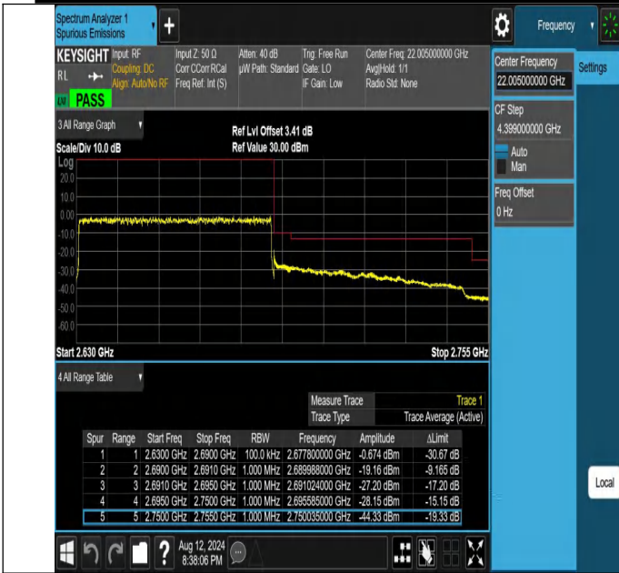
NTNV-N41-PC2-30-60-H-DFT-QPSK-Outer_Full-Ant1-PASS
