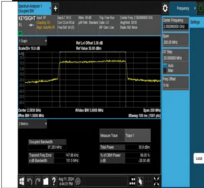
NTNV-N41-PC2-30-100-M-CP-QPSK-Outer_Full-Ant1-PASS
