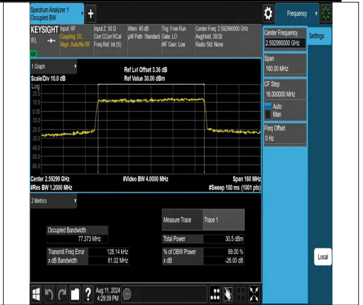
NTNV-N41-PC2-30-80-M-CP-16QAM-Outer_Full-Ant1-PASS
