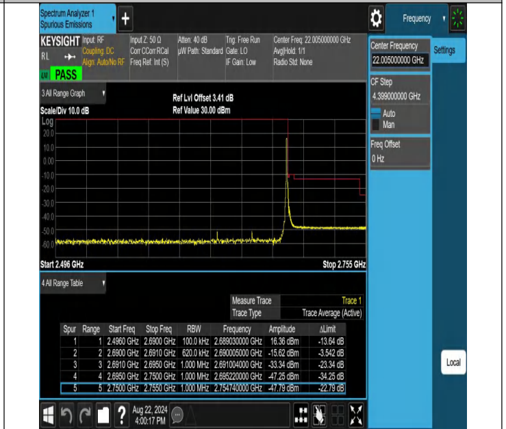
NTNV-N41-PC2-30-60-H-DFT-PI2BPSK-Edge_1RB_Right-Ant1-PASS
