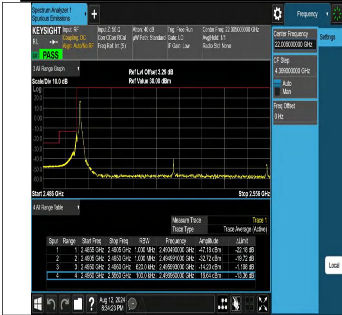
NTNV-N41-PC2-30-60-L-DFT-QPSK-Edge_1RB_Left-Ant1-PASS
