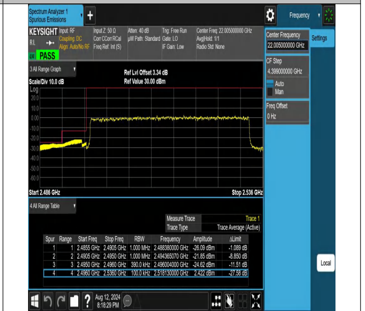
NTNV-N41-PC2-30-40-L-DFT-PI2BPSK-Outer_Full-Ant1-PASS
