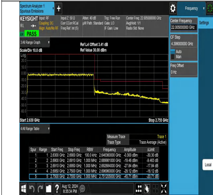
NTNV-N41-PC2-30-60-H-DFT-PI2BPSK-Outer_Full-Ant1-PASS
