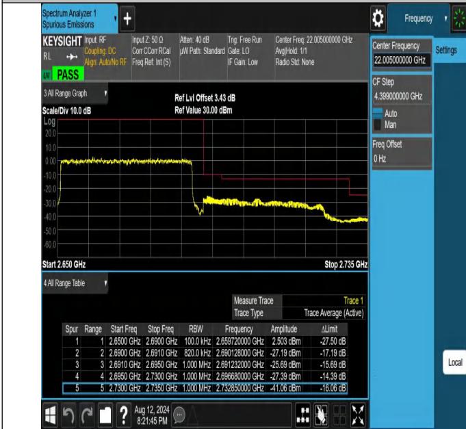
NTNV-N41-PC2-30-40-H-DFT-PI2BPSK-Outer_Full-Ant1-PASS
