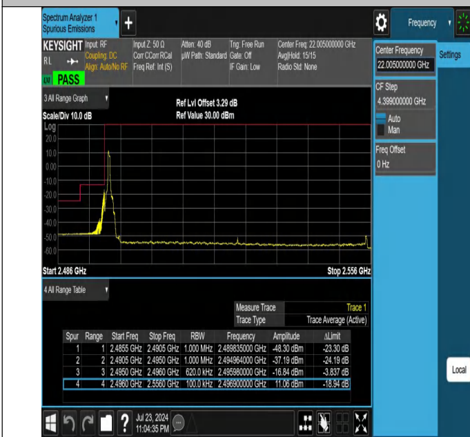
NTNV-N41-PC2-30-60-L-DFT-PI2BPSK-Edge_1RB_Left-Ant1-PASS
