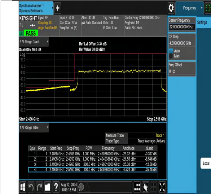
NTNV-N41-PC2-30-20-L-DFT-QPSK-Outter_Full-Ant1-PASS
