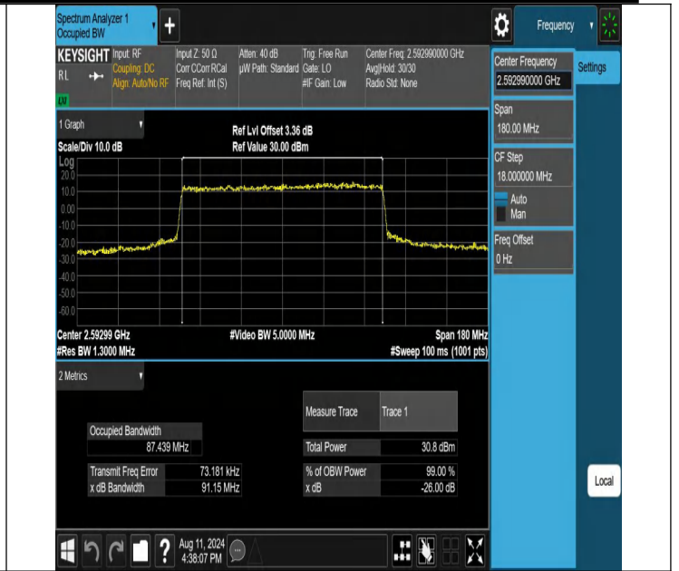
NTNV-N41-PC2-30-90-M-CP-16QAM-Outer_Full-Ant1-PASS
