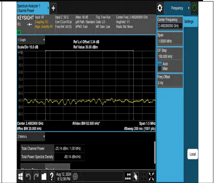
NTV-N41-PC2-30-30-L-DFT-QPSK-Outet_Full-Ant1-PASS
