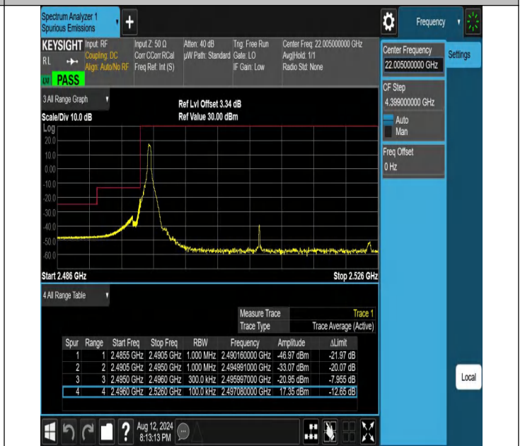
NTNV-N41-PC2-30-30-L-DFT-QPSK-Edge_1RB_Left-Ant1-PASS
