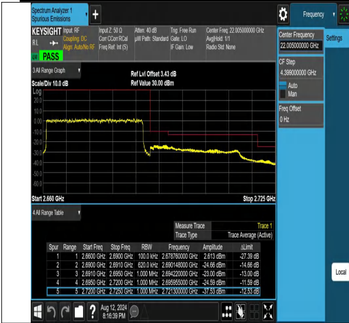
NTNV-N41-PC2-30-30-H-DFT-QPSK-Outer_Full-Ant1-PASS
