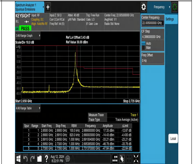
NTNV-N41-PC2-30-40-H-DFT-PI2BPSK-Edge_1RB_Right-Ant1-PASS
