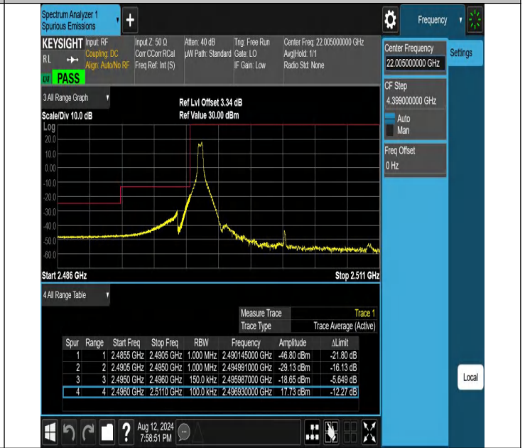
NTNV-N41-PC2-30-15-L-DFT-QPSK-Edge_1RB_Left-Ant1-PASS
