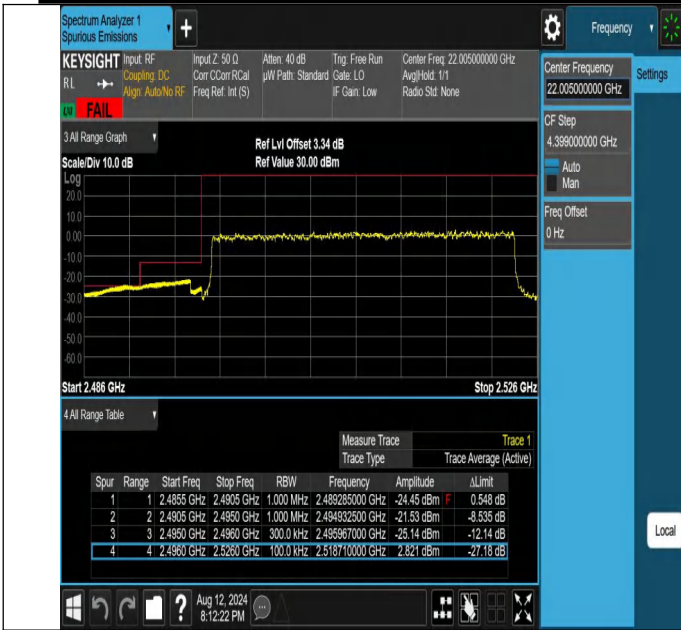
NTV-N41-PC2-30-30-L-DFT-QPSK-Outet_Full-Ant1-FAIL
