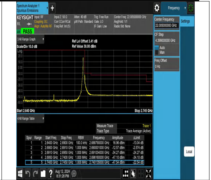
NTNV-N41-PC2-30-50-H-DFT-QPSK-Edge_1RB_Right-Ant1-PASS
