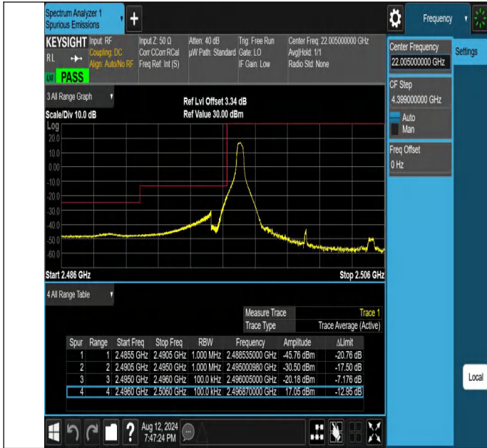
NTNV-N41-PC2-30-10-L-DFT-PI2BPSK-Edge_1RB_Left-Ant1-PA SS
