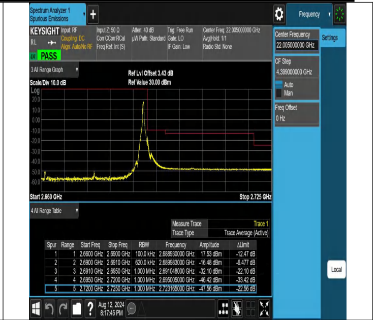
NTNV-N41-PC2-30-30-H-DFT-QPSK-Edge_1RB_Right-Ant1-PASS
