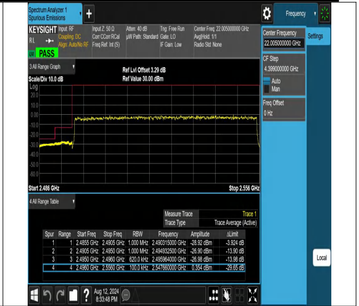
NTNV-N41-PC2-30-60-L-DFT-QPSK-Outer_Full-Ant1-PASS
