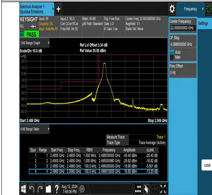
NTNV-N41-PC2-30-10-L-DFT-QPSK-Edge_1RB_Left-Ant1-PASS
