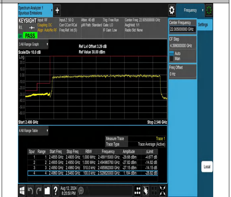
NTNV-N41-PC2-30-50-L-DFT-PI2BPSK-Outer_Full-Ant1-PASS
