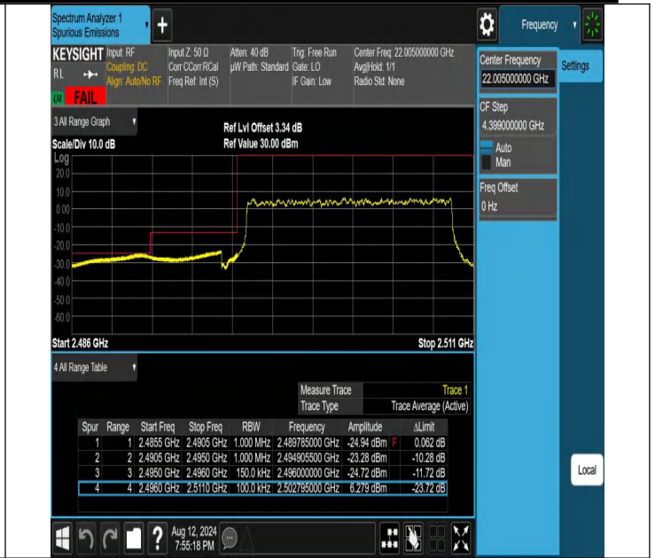
NTNV-N41-PC2-30-15-L-DFT-PI2BPSK-Outer_Full-Ant1-FAIL
