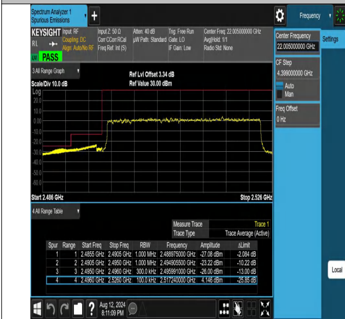
NTNV-N41-PC2-30-30-L-DFT-PI2BPSK-Outer_Full-Ant1-PASS
