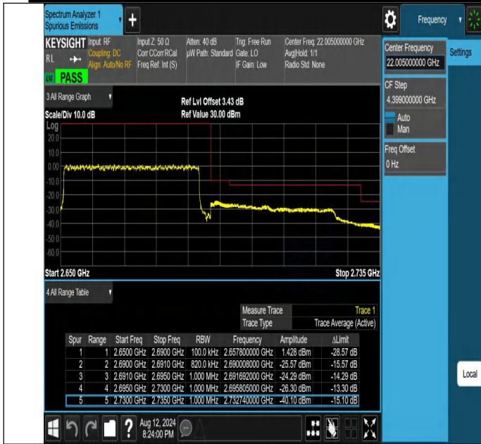
NTNV-N41-PC2-30-40-H-DFT-QPSK-Outer_Full-Ant1-PASS
