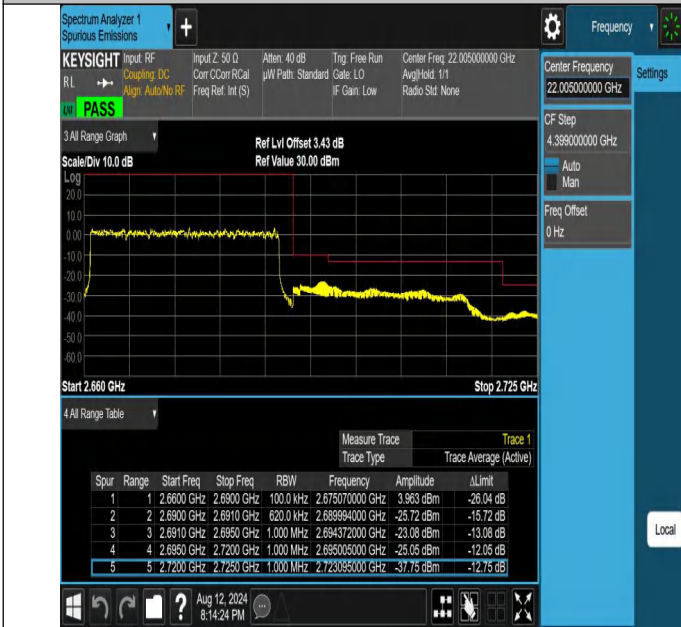
NTV-N41-PC2-30-30-H-DFT-PI2BPSK-Outet_Full-Ant1-PASS
