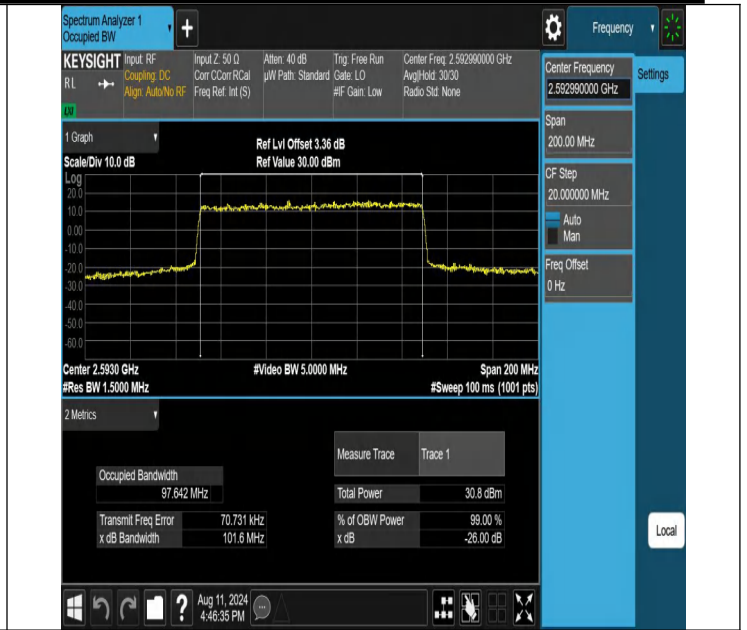
NTNV-N41-PC2-30-100-M-CP-16QAM-Outer_Full-Ant1-PASS
