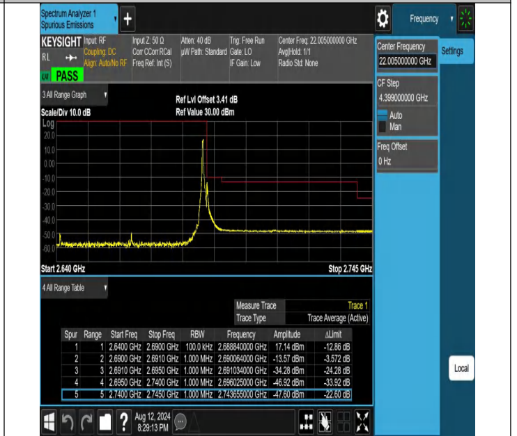
NTNV-N41-PC2-30-50-H-DFT-PI2BPSK-Edge_1RB_Right-Ant1-PASS
