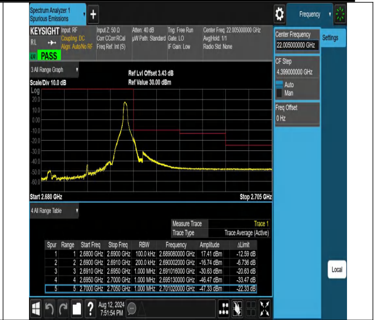
NTVN-N41-PC2-30-10-H-DFT-PI2BPSK-Edge_1RB_Right-Ant1-PASS
