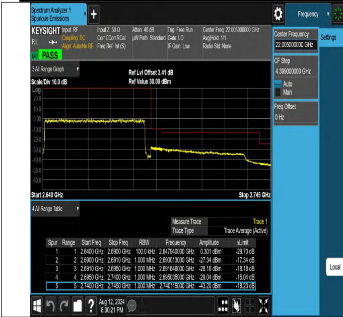
NTNV-N41-PC2-30-50-H-DFT-QPSK-Outer_Full-Ant1-PASS
