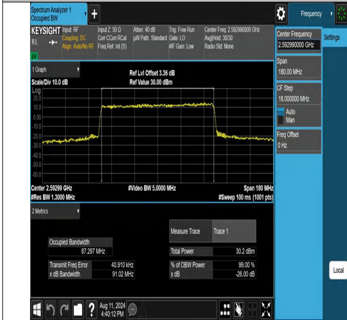
NTNV-N41-PC2-30-90-M-CP-64QAM-Outer_Full-Ant1-PASS
