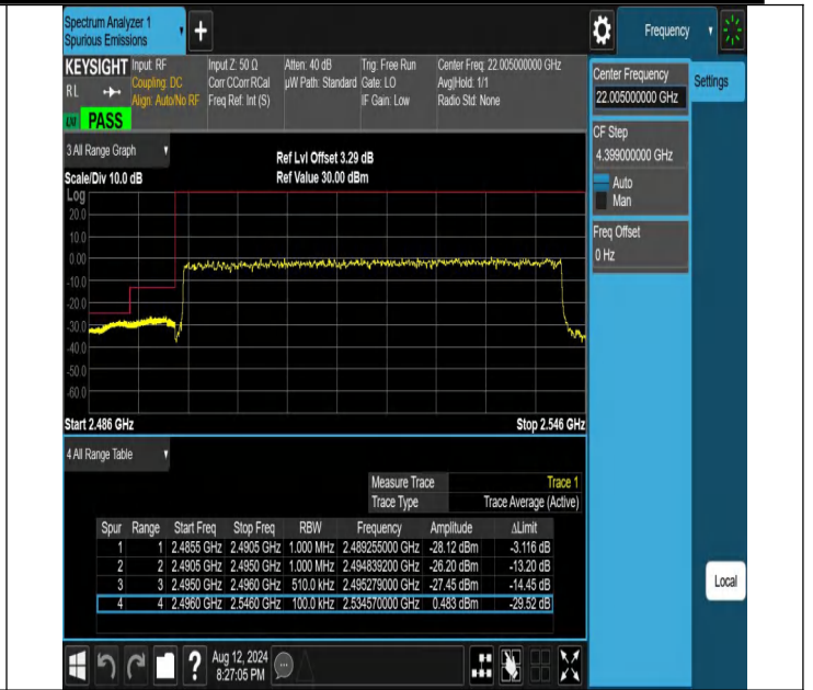
NTNV-N41-PC2-30-50-L-DFT-QPSK-Outer_Full-Ant1-PASS
