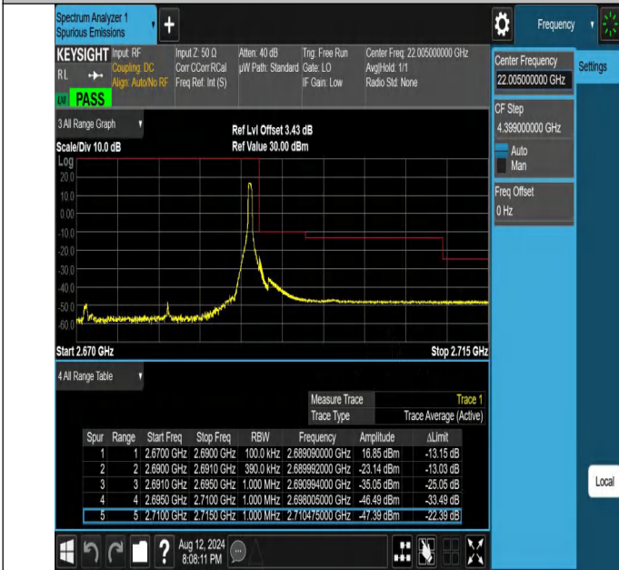
NTNV-N41-PC2-30-20-H-DFT-PI2BPSK-Edge_1RB_Right-Ant1-PASS
