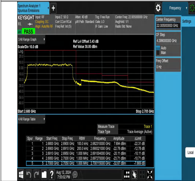
NTVN-N41-PC2-30-10-H-DFT-QPSK-Outer_Full-Ant1-PASS
