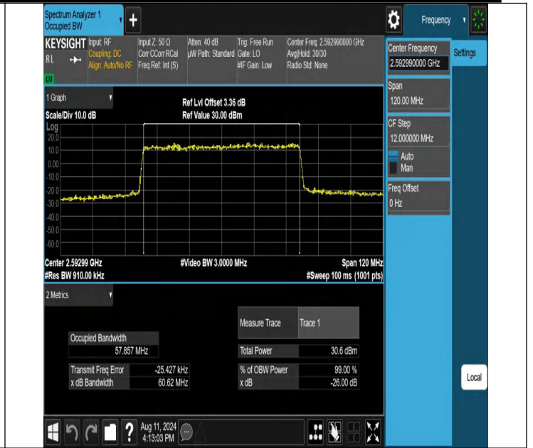
NTNV-N41-PC2-30-60-M-CP-16QAM-Outer_Full-Ant1-PASS
