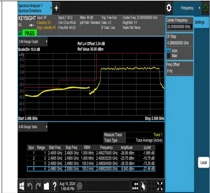
NTNV-N41-PC2-30-10-L-DFT-PI2BPSK-Outer_Full-Ant1-PASS
