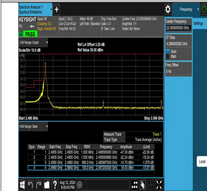
NTNV-N41-PC2-30-70-L-DFT-PI2BPSK-Edge_1RB_Left-Ant1-PA SS
