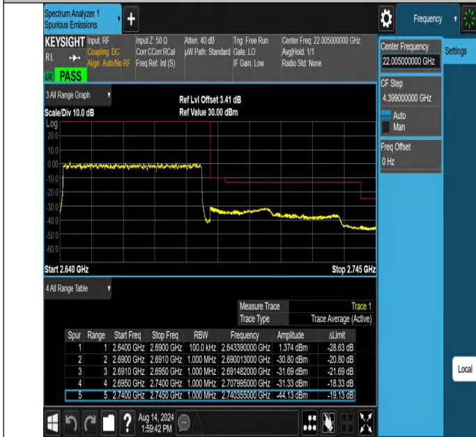
NTNV-N41-PC2-30-50-H-DFT-PI2BPSK-Outer_Full-Ant1-PASS
