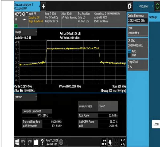
NTNV-N41-PC2-30-100-M-CP-64QAM-Outer_Full-Ant1-PASS
