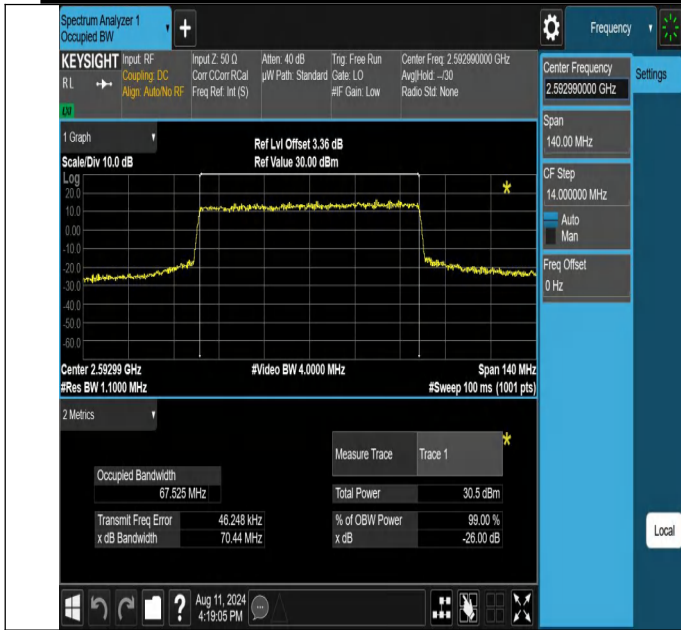
NTNV-N41-PC2-30-70-M-CP-QPSK-Outer_Full-Ant1-PASS
