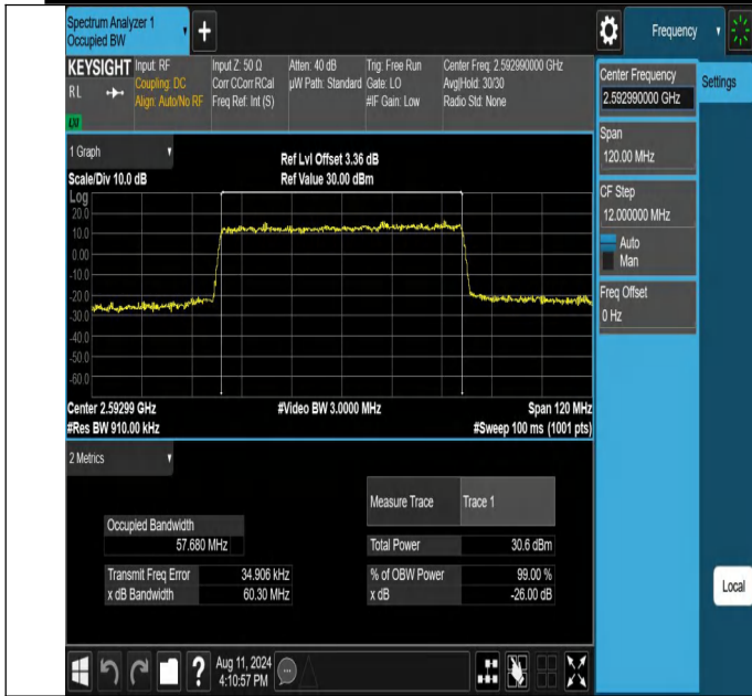
NTNV-N41-PC2-30-60-M-CP-QPSK-Outer_Full-Ant1-PASS
