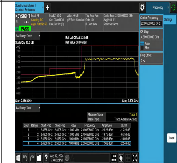
NTNV-N41-PC2-30-10-L-DFT-QPSK-Outer_Full-Ant1-PASS
