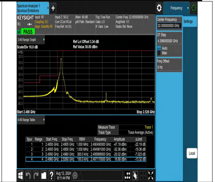
NTNV-N41-PC2-30-30-L-DFT-PI2BPSK-Edge_1RB_Left-Ant1-PA
