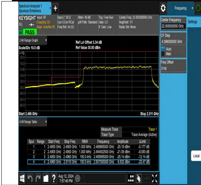
NTNV-N41-PC2-30-15-L-DFT-QPSK-Outter_Full-Ant1-PASS
