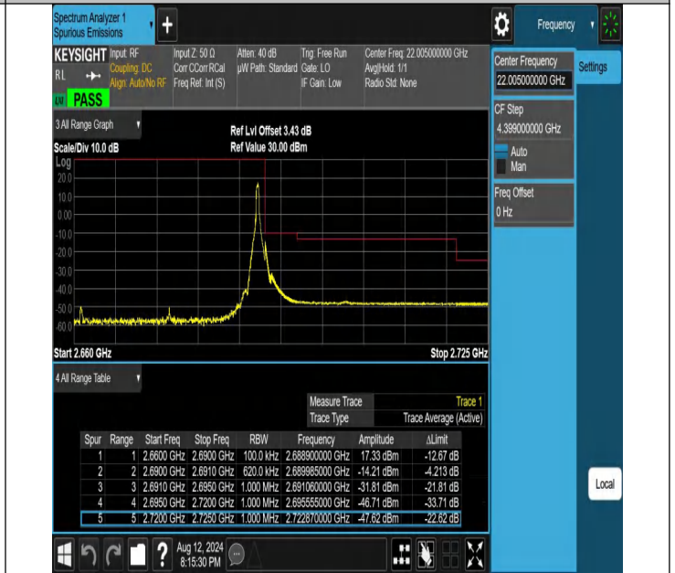
NTV-N41-PC2-30-30-H-DFT-PI2BPSK-Edge_1RB_Right-Ant1-PASS
