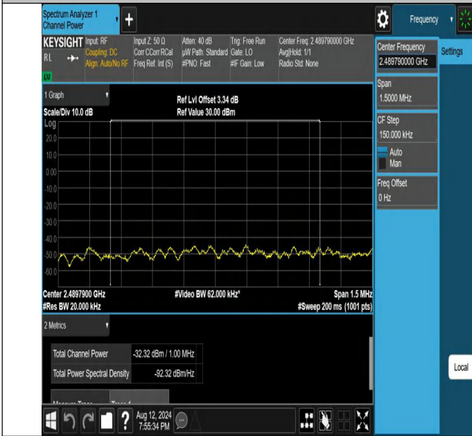
NTNV-N41-PC2-30-15-L-DFT-PI2BPSK-Outer_Full-Ant1-PASS
