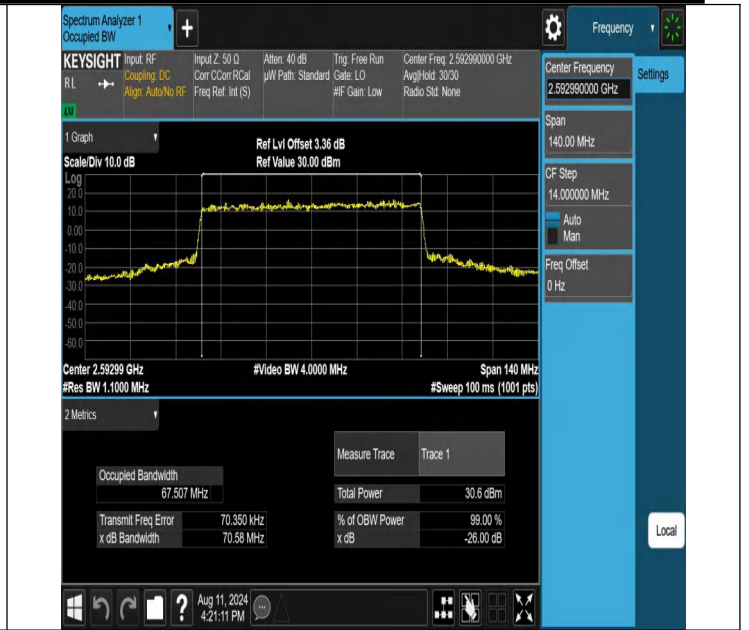
NTNV-N41-PC2-30-70-M-CP-16QAM-Outer_Full-Ant1-PASS
