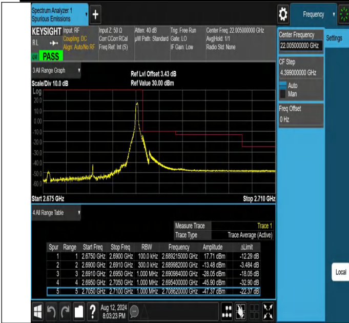
NTNV-N41-PC2-30-15-H-DFT-QPSK-Edge_1RB_Right-Ant1-PAS
