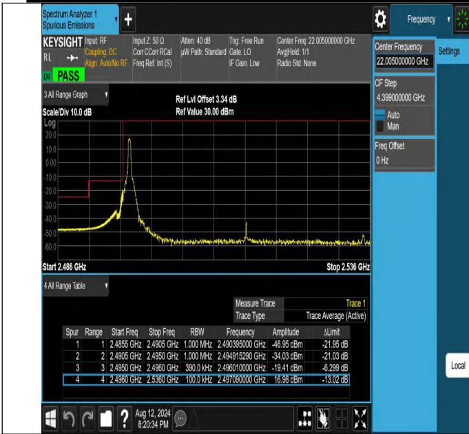
NTNV-N41-PC2-30-40-L-DFT-QPSK-Edge_1RB_Left-Ant1-PASS
