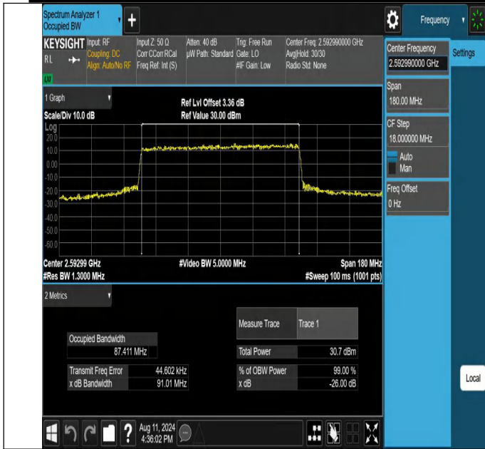
NTNV-N41-PC2-30-90-M-CP-QPSK-Outer_Full-Ant1-PASS
