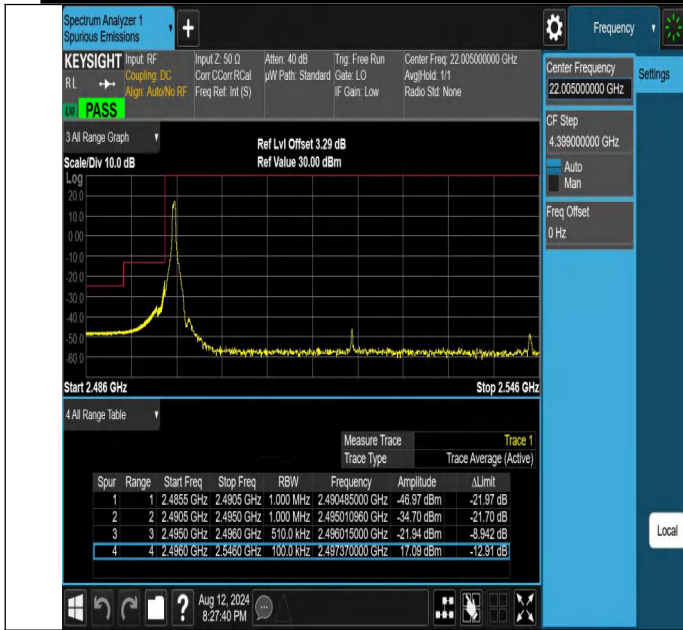
NTNV-N41-PC2-30-50-L-DFT-QPSK-Edge_1RB_Left-Ant1-PASS
