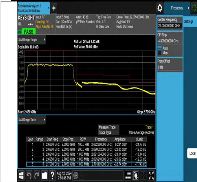
NTNV-N41-PC2-30-10-H-DFT-PI2BPSK-Outer_Full-Ant1-PASS
