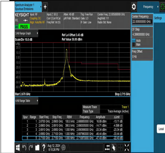
NTNV-N41-PC2-30-20-H-DFT-QPSK-Edge_1RB_Right-Ant1-PAS
