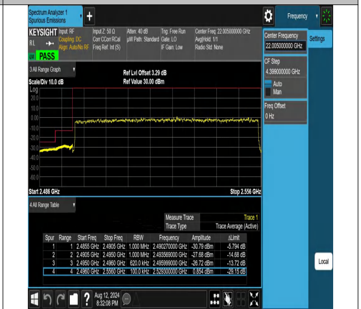
NTNV-N41-PC2-30-60-L-DFT-PI2BPSK-Outer_Full-Ant1-PASS
