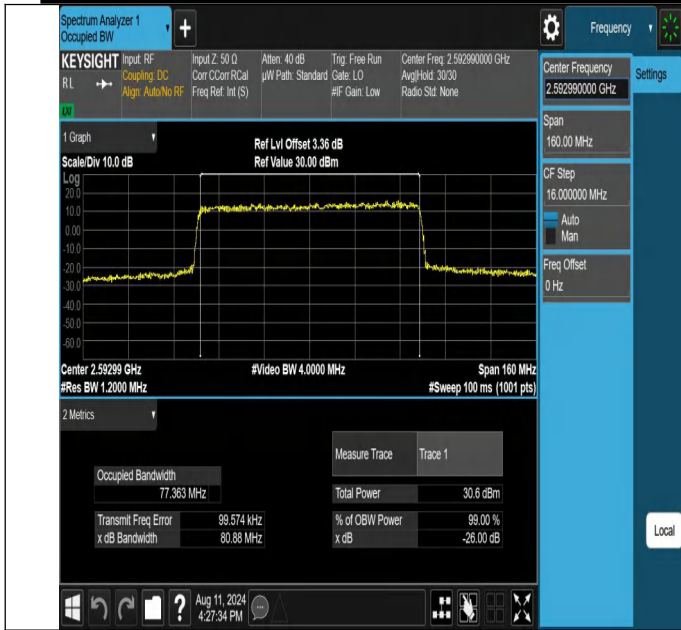
NTNV-N41-PC2-30-80-M-CP-QPSK-Outer_Full-Ant1-PASS
