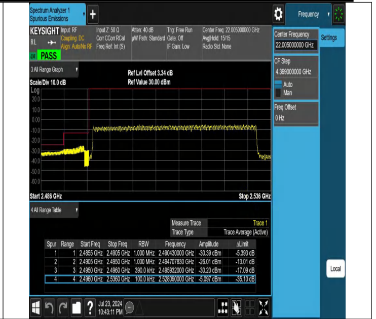
NTNV-N41-PC2-30-40-L-DFT-QPSK-Outer_Full-Ant1-PASS
