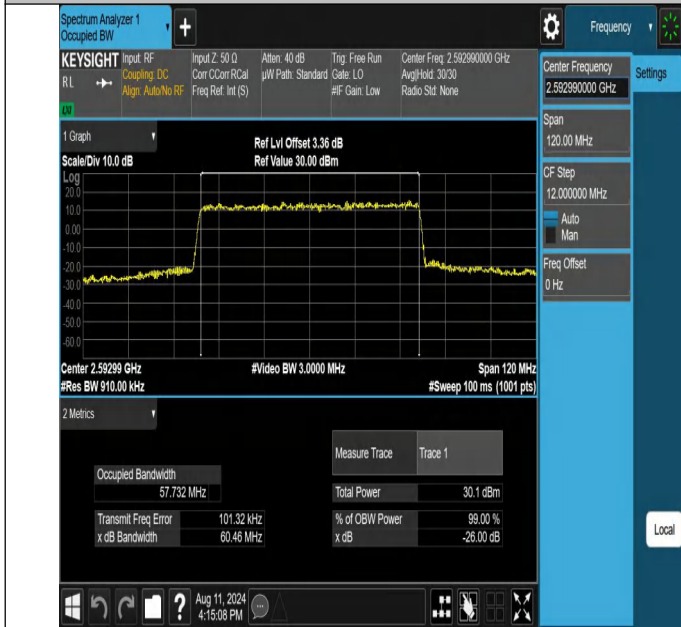
NTNV-N41-PC2-30-60-M-CP-64QAM-Outer_Full-Ant1-PASS
