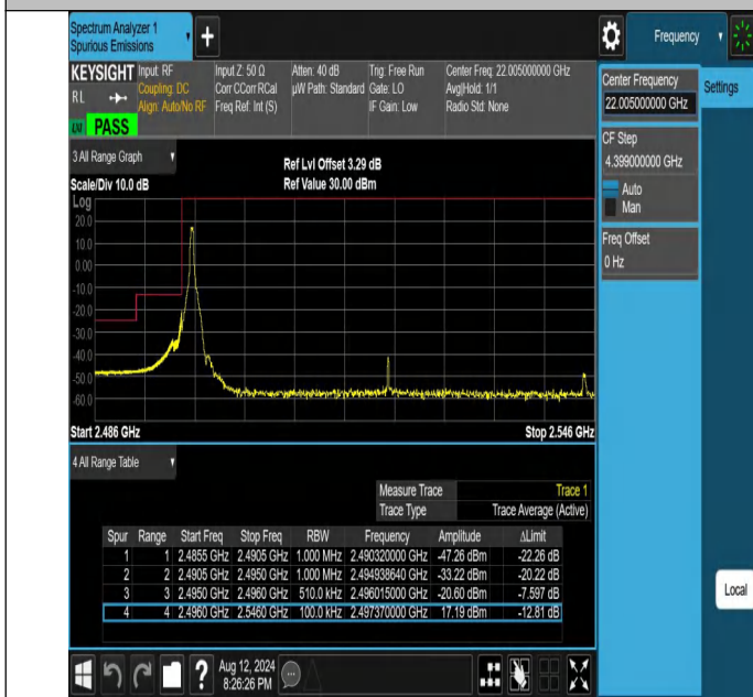
NTNV-N41-PC2-30-50-L-DFT-PI2BPSK-Edge_1RB_Left-Ant1-PASS
