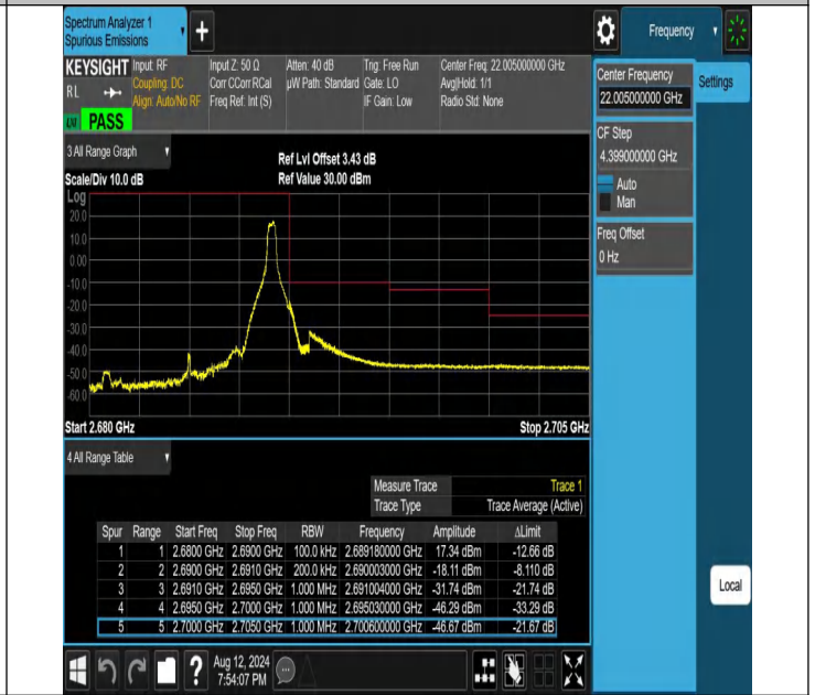
NTVN-N41-PC2-30-10-H-DFT-QPSK-Edge_1RB_Right-Ant1-PASS
