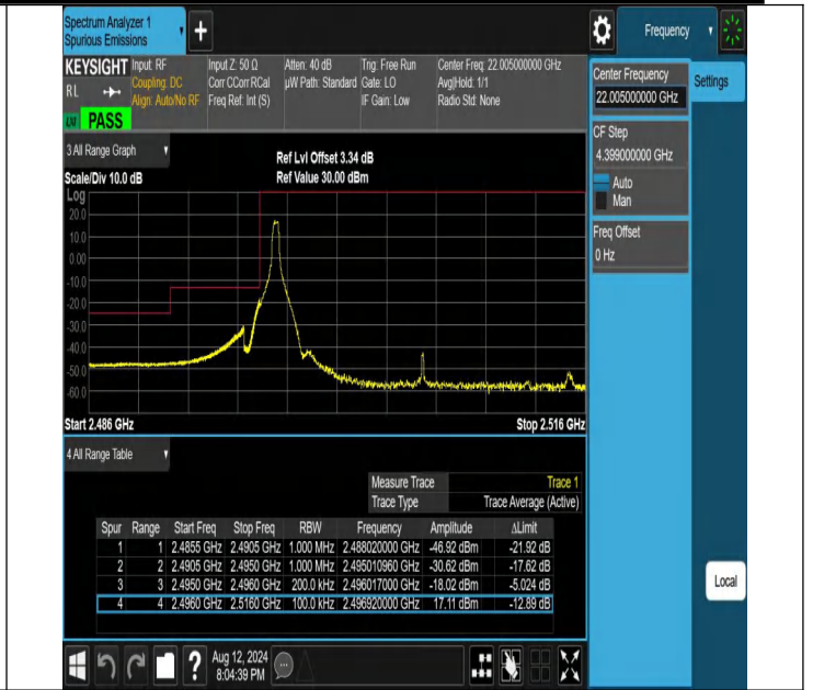
NTNV-N41-PC2-30-20-L-DFT-PI2BPSK-Edge_1RB_Left-Ant1-PAS
