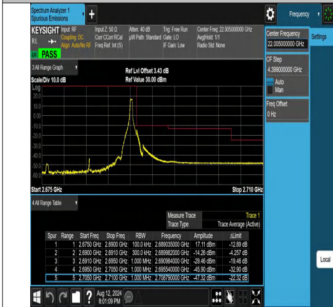
NTNV-N41-PC2-30-15-H-DFT-PI2BPSK-Edge_1RB_Right-Ant1-PASS
