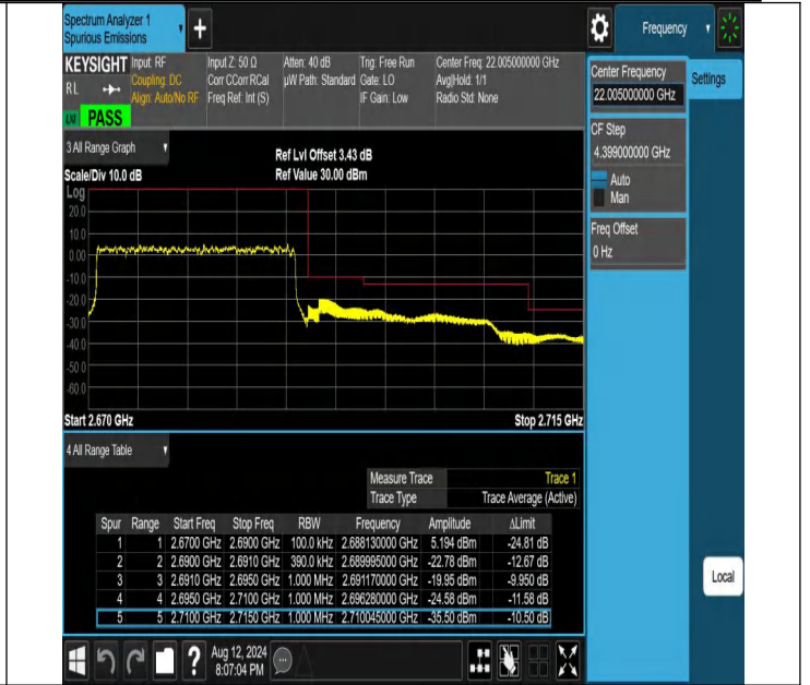
NTNV-N41-PC2-30-20-H-DFT-PI2BPSK-Outter_Full-Ant1-PASS
