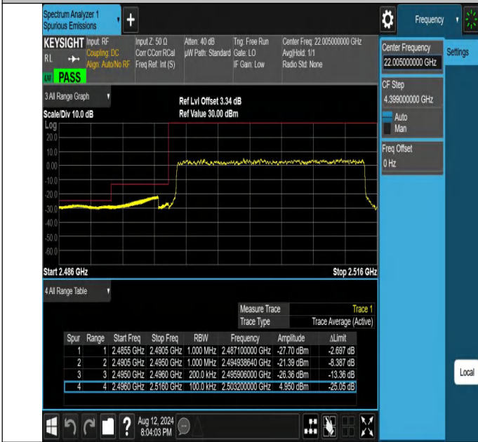
NTNV-N41-PC2-30-20-L-DFT-PI2BPSK-Outer_Full-Ant1-PASS
