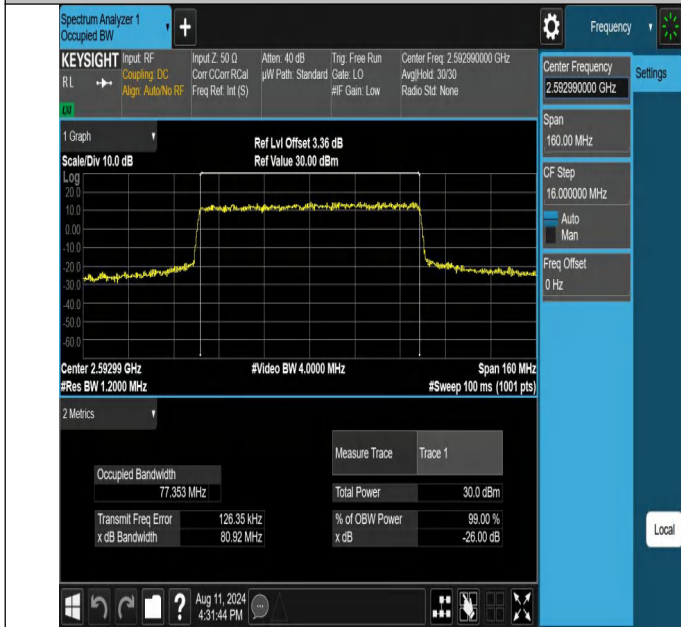
NTNV-N41-PC2-30-80-M-CP-64QAM-Outer_Full-Ant1-PASS
