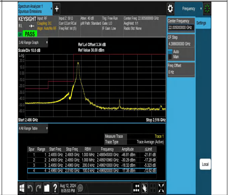
NTNV-N41-PC2-30-20-L-DFT-QPSK-Edge_1RB_Left-Ant1-PASS
