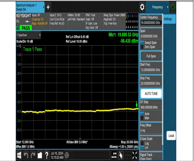
NTNV-DC_12A_n25A-PC3-15-5+25-M+H-N/A-N/A-DFT-PI2BPSK-E dge_1RB_Right-12000-20000-PASS
