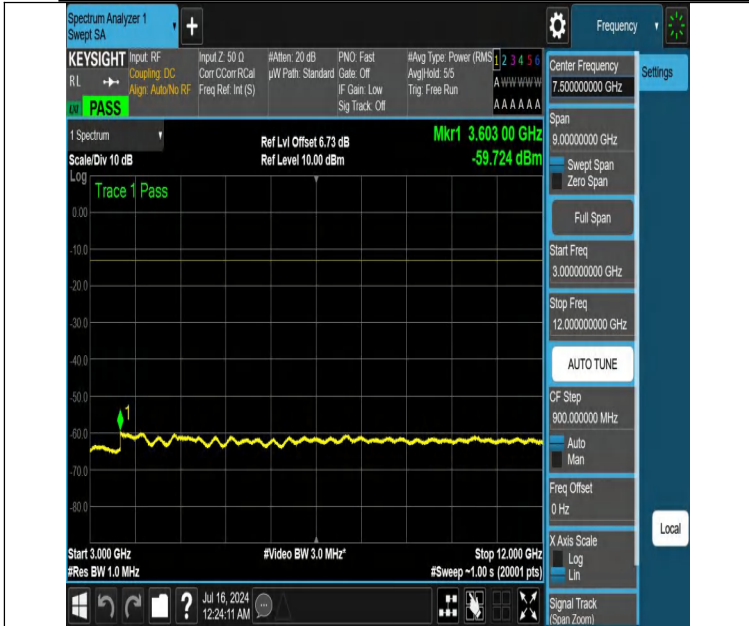
NTNV-DC_12A_n25A-PC3-15-5+30-M+M-N/A-N/A-DFT-PI2BPSK-Edge_1RB_Left-3000-12000-PASS
