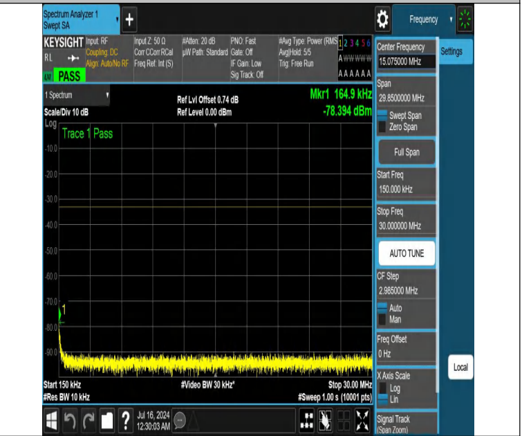
NTNV-DC_12A_n25A-PC3-15-5+30-M+H-N/A-N/A-DFT-PI2BPSK-E dge_1RB_Right-0.15-30-PASS
