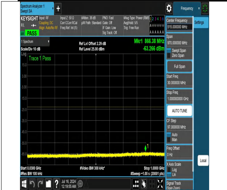
NTNV-DC_12A_n25A-PC3-15-5+30-M+L-N/A-N/A-DFT-PI2BPSK- Edge_1RB_Right-30-1000-PASS
