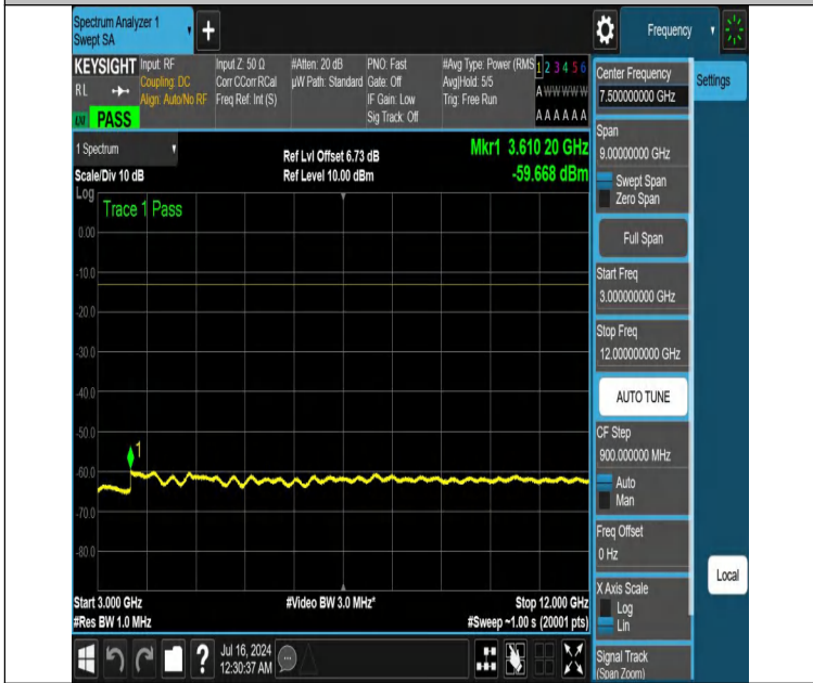
NTNV-DC_12A_n25A-PC3-15-5+30-M+H-N/A-N/A-DFT-PI2BPSK-Edge_1RB_Right-3000-12000-PASS
