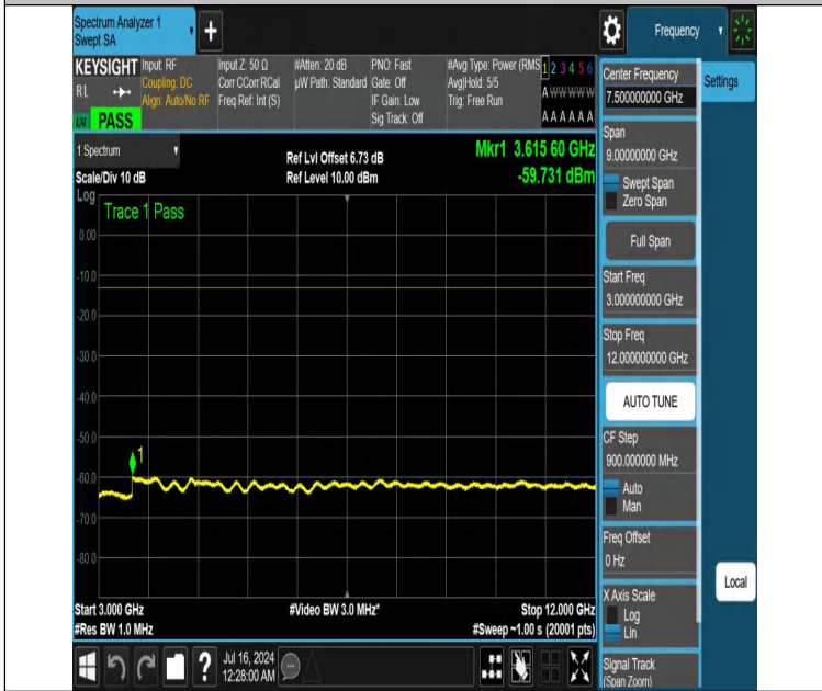
NTNV-DC_12A_n25A-PC3-15-5+30-M+M-N/A-N/A-DFT-QPSK-Edge_1RB_Right-3000-12000-PASS
