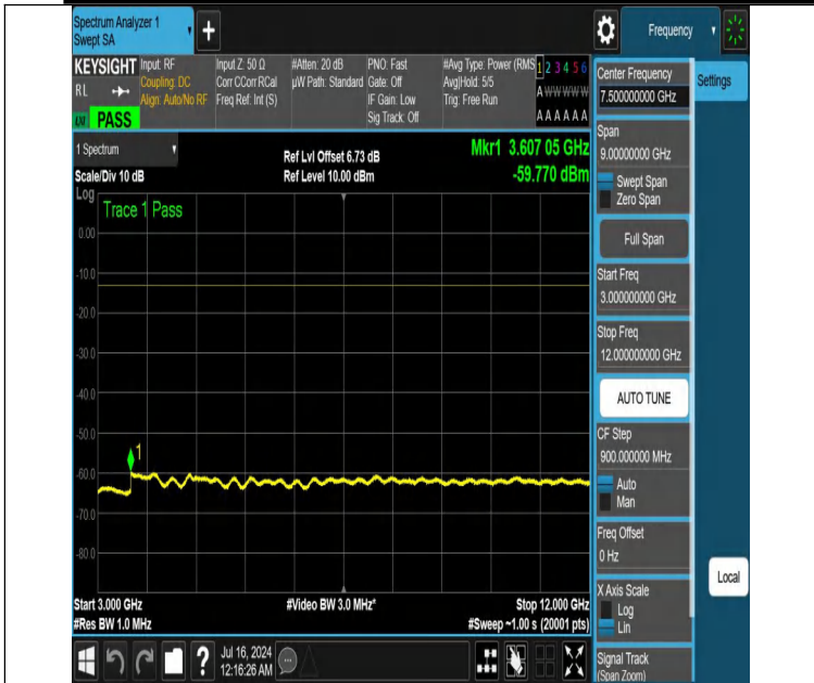
NTNV-DC_12A_n25A-PC3-15-5+25-M+H-N/A-N/A-DFT-QPSK-Edge e_1RB_Left-3000-12000-PASS
