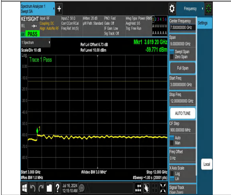
NTNV-DC_12A_n25A-PC3-15-5+25-M+H-N/A-N/A-DFT-PI2BPSK-Edge_1RB_Right-3000-12000-PASS
