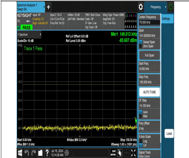
NTNV-DC_12A_n25A-PC3-15-5+25-M+H-N/A-N/A-DFT-PI2BPSK-Edge_1RB_Right-0.009-0.15-PASS
