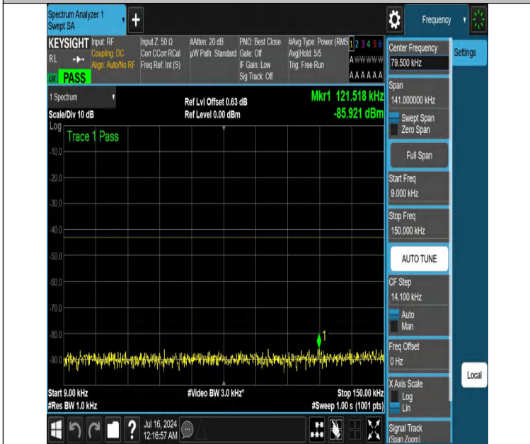
NTNV-DC_12A_n25A-PC3-15-5+25-M+H-N/A-N/A-DFT-QPSK-Edge e_1RB_Right-0.009-0.15-PASS
