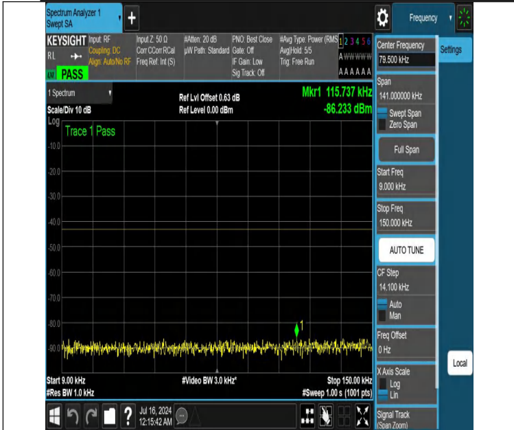
NTNV-DC_12A_n25A-PC3-15-5+25-M+H-N/A-N/A-DFT-QPSK-Edge e_1RB_Left-0.009-0.15-PASS
