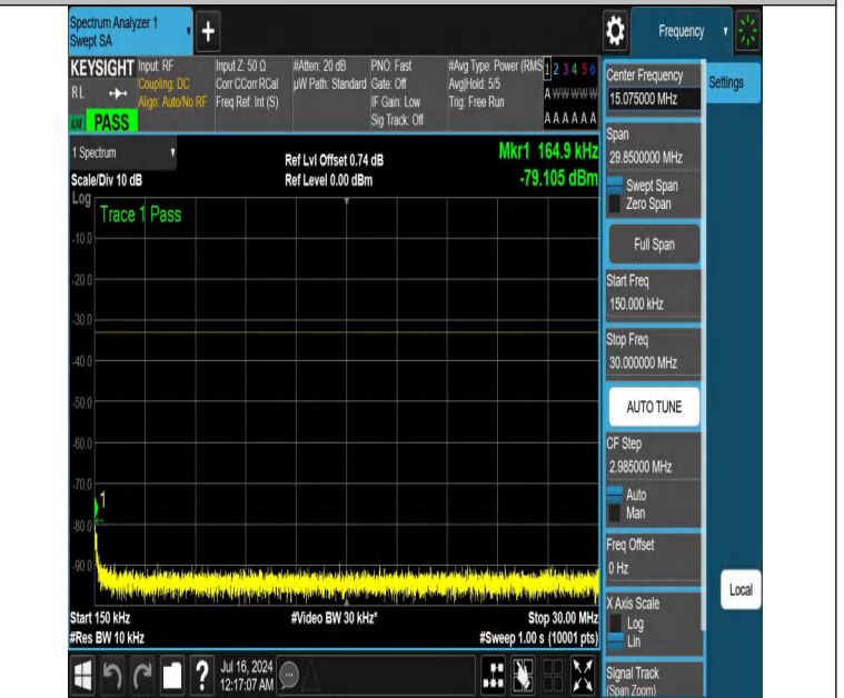
NTNV-DC_12A_n25A-PC3-15-5+25-M+H-N/A-N/A-DFT-QPSK-Edge e_1RB_Right-0.15-30-PASS
