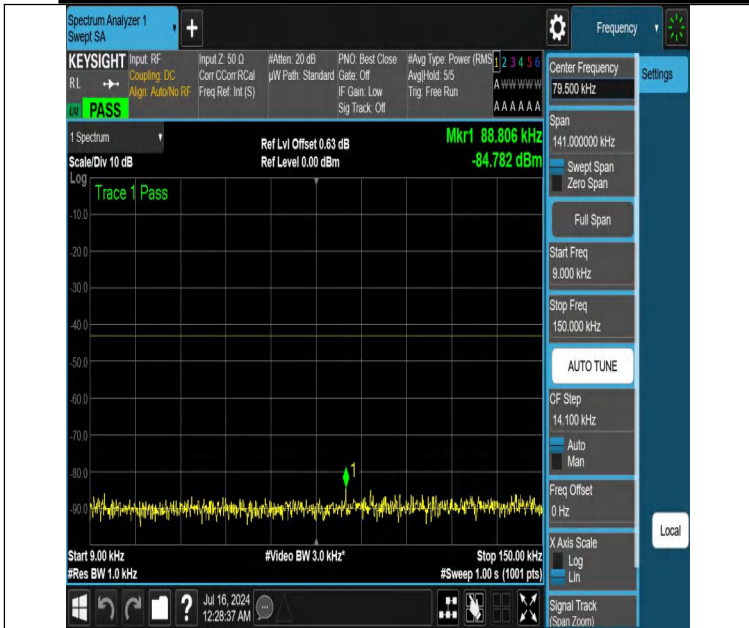
NTNV-DC_12A_n25A-PC3-15-5+30-M+H-N/A-N/A-DFT-PI2BPSK-Edge_1RB_Left-0.009-0.15-PASS
