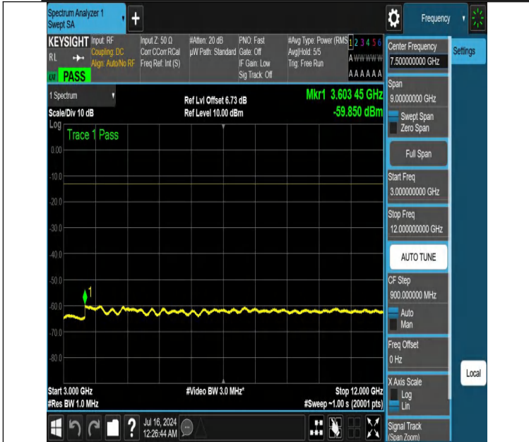
NTNV-DC_12A_n25A-PC3-15-5+30-M+M-N/A-N/A-DFT-QPSK-Edge_1RB_Left-3000-12000-PASS
