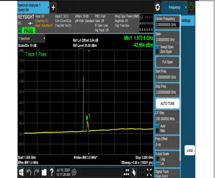
NTNV-DC_12A_n25A-PC3-15-5+25-M+H-N/A-N/A-DFT-QPSK-Edge e_1RB_Right-1000-3000-PASS
