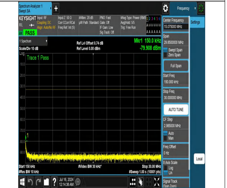
NTNV-DC_12A_n25A-PC3-15-5+25-M+H-N/A-N/A-DFT-PI2BPSK-E dge_1RB_Right-0.15-30-PASS
