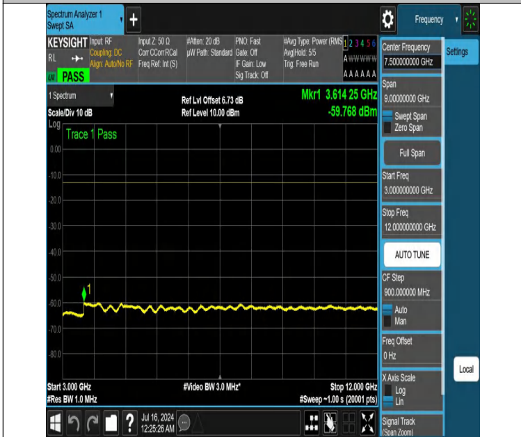
NTNV-DC_12A_n25A-PC3-15-5+30-M+M-N/A-N/A-DFT-PI2BPSK-Edge_1RB_Right-3000-12000-PASS
