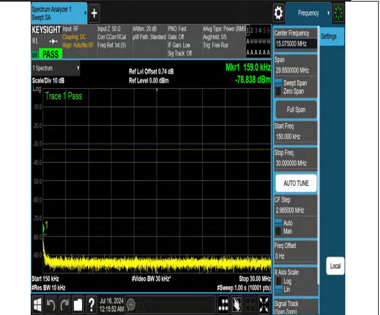
NTNV-DC_12A_n25A-PC3-15-5+25-M+H-N/A-N/A-DFT-QPSK-Edge e_1RB_Left-0.15-30-PASS
