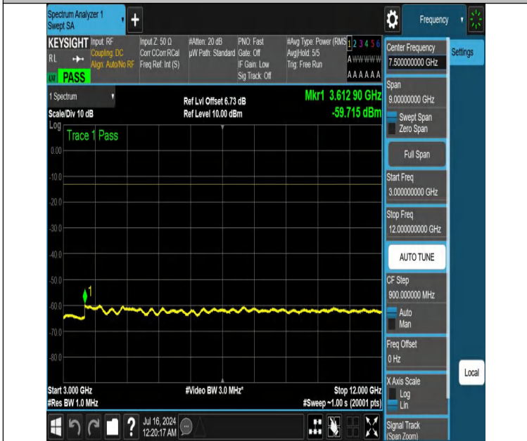
NTNV-DC_12A_n25A-PC3-15-5+30-M+L-N/A-N/A-DFT-PI2BPSK- Edge_1RB_Right-3000-12000-PASS
