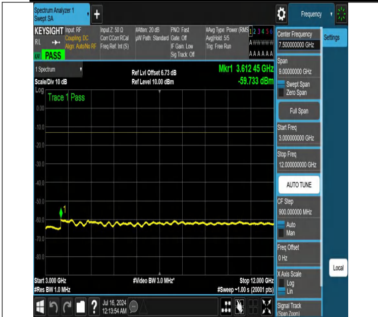
NTNV-DC_12A_n25A-PC3-15-5+25-M+H-N/A-N/A-DFT-PI2BPSK-Edge_1RB_Left-3000-12000-PASS
