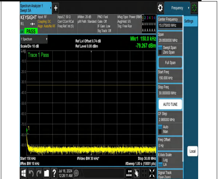
NTNV-DC_12A_n25A-PC3-15-5+30-M+M-N/A-N/A-DFT-QPSK-Edge_1RB_Left-0.15-30-PASS
