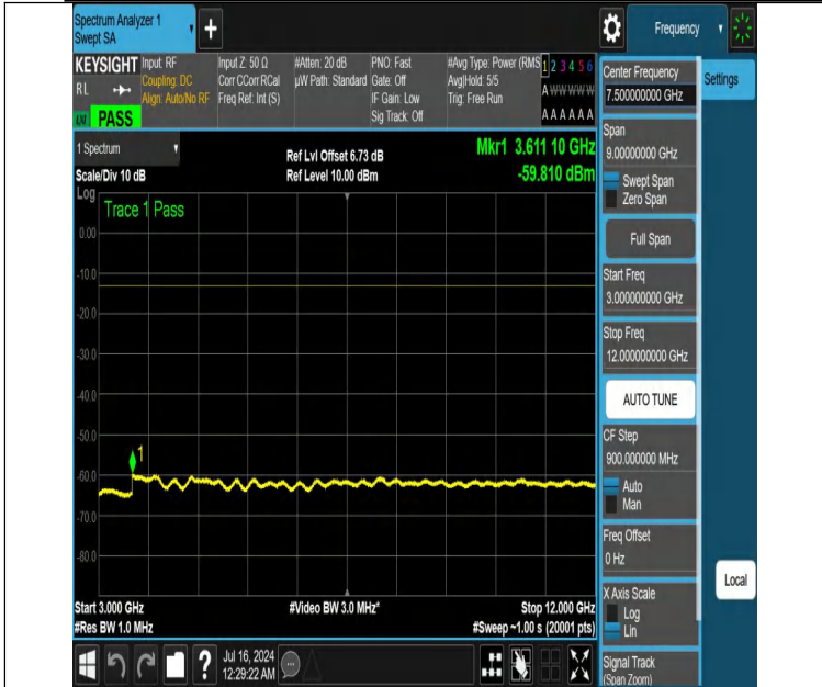
NTNV-DC_12A_n25A-PC3-15-5+30-M+H-N/A-N/A-DFT-PI2BPSK-Edge_1RB_Left-3000-12000-PASS
