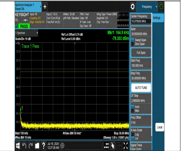
NTNV-DC_12A_n25A-PC3-15-5+30-M+M-N/A-N/A-DFT-QPSK-Edge_1RB_Right-0.15-30-PASS
