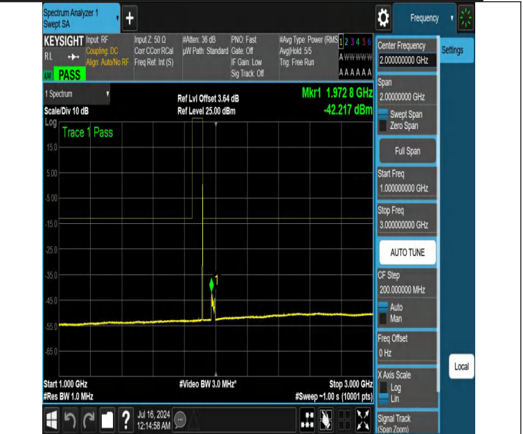
NTNV-DC_12A_n25A-PC3-15-5+25-M+H-N/A-N/A-DFT-PI2BPSK-E dge_1RB_Right-1000-3000-PASS
