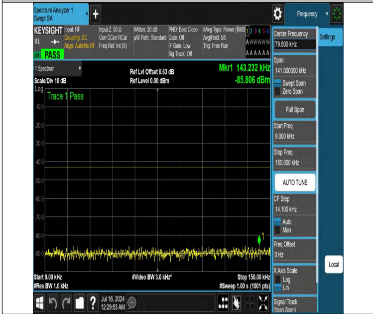
NTNV-DC_12A_n25A-PC3-15-5+30-M+H-N/A-N/A-DFT-PI2BPSK-Edge_1RB_Right-0.009-0.15-PASS
