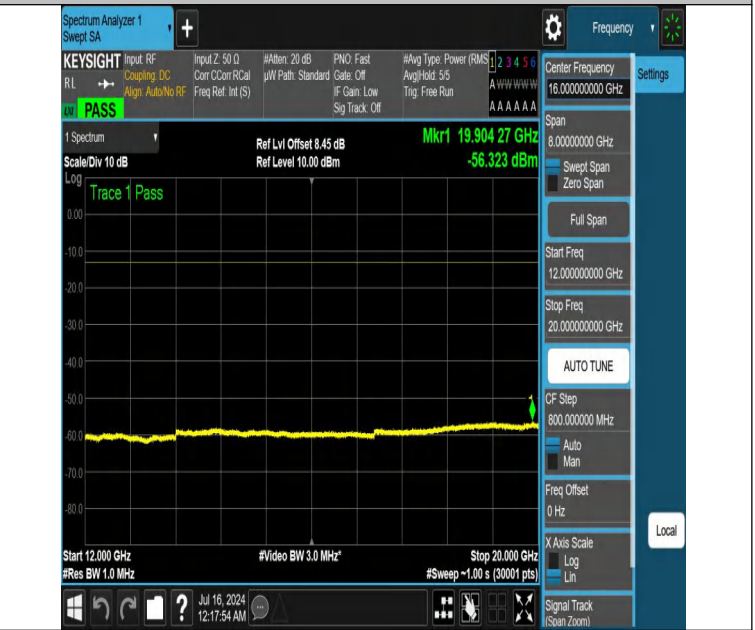
NTNV-DC_12A_n25A-PC3-15-5+25-M+H-N/A-N/A-DFT-QPSK-Edge e_1RB_Right-12000-20000-PASS
