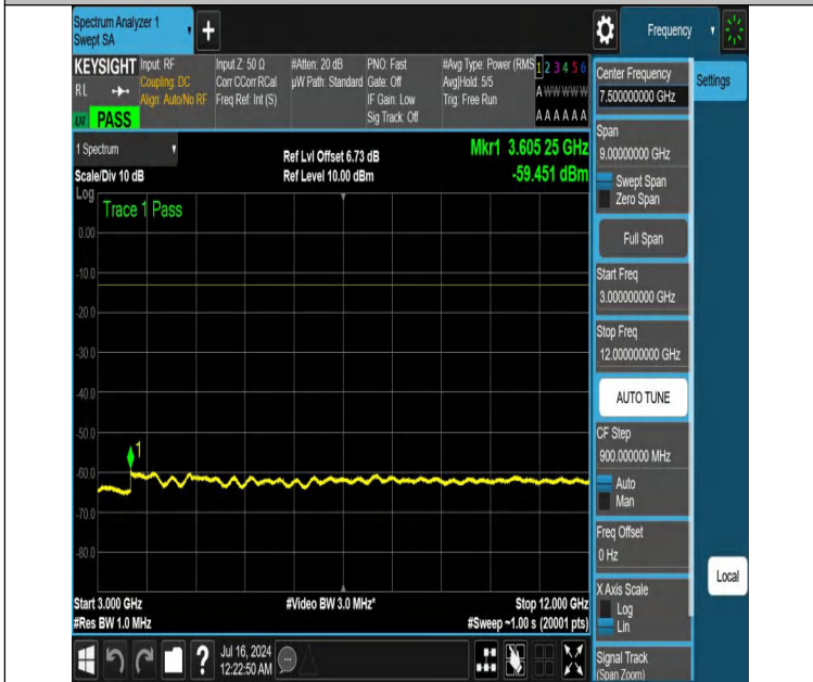
NTNV-DC_12A_n25A-PC3-15-5+30-M+L-N/A-N/A-DFT-QPSK-Edge e_1RB_Right-3000-12000-PASS
