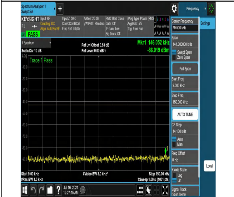
NTNV-DC_12A_n25A-PC3-15-5+30-M+M-N/A-N/A-DFT-QPSK-Edge_1RB_Right-0.009-0.15-PASS
