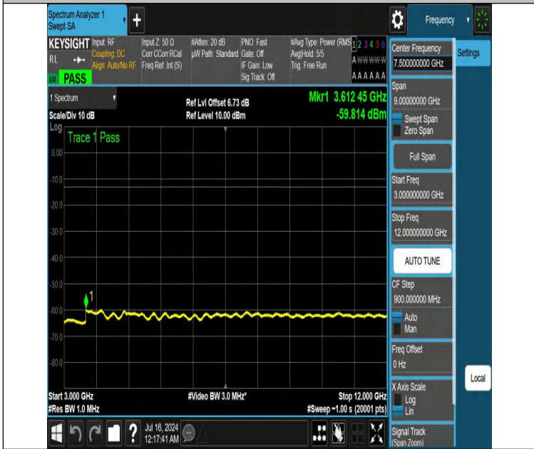
NTNV-DC_12A_n25A-PC3-15-5+25-M+H-N/A-N/A-DFT-QPSK-Edge e_1RB_Right-3000-12000-PASS
