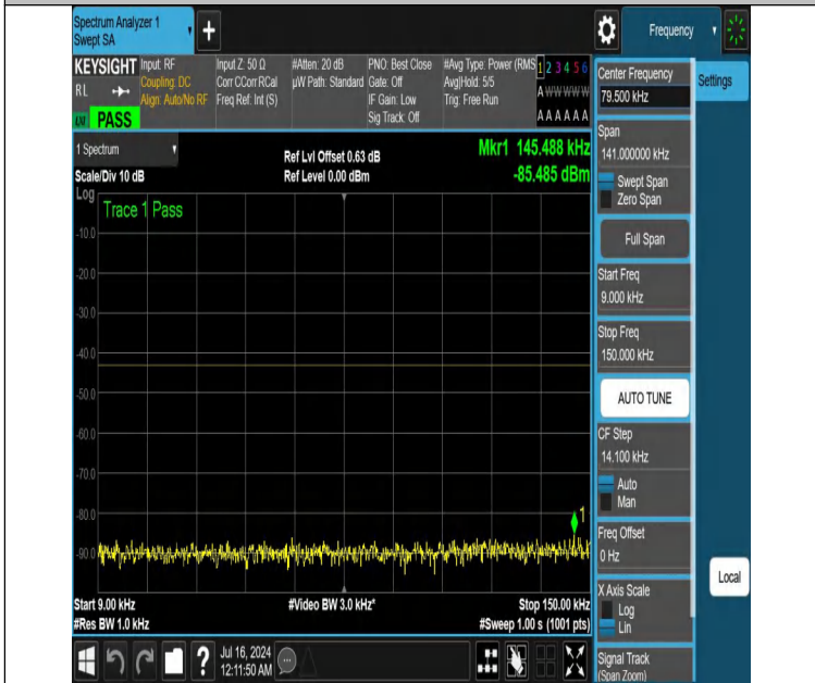
NTNV-DC_12A_n25A-PC3-15-5+25-M+M-N/A-N/A-DFT-QPSK-Edge_1RB_Right-0.009-0.15-PASS
