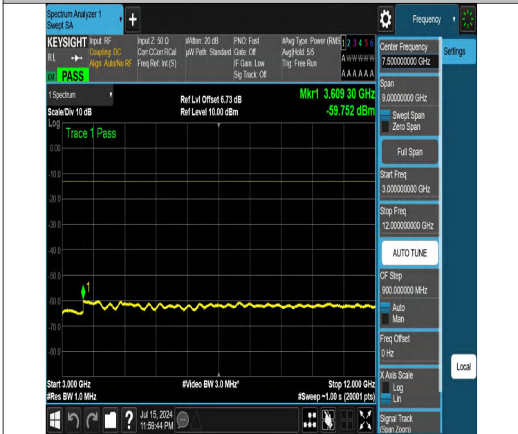
NTNV-DC_12A_n25A-PC3-15-5+20-M+H-N/A-N/A-DFT-PI2BPSK-Edge_1RB_Right-3000-12000-PASS
