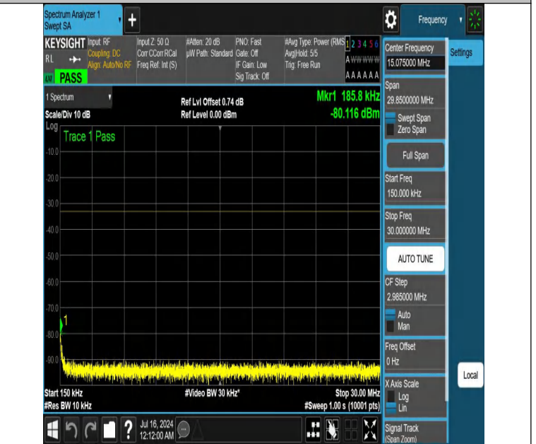
NTNV-DC_12A_n25A-PC3-15-5+25-M+M-N/A-N/A-DFT-QPSK-Edge_1RB_Right-0.15-30-PASS
