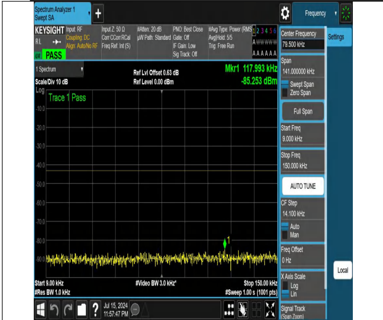
NTNV-DC_12A_n25A-PC3-15-5+20-M+H-N/A-N/A-DFT-PI2BPSK-Edge_1RB_Left-0.009-0.15-PASS
