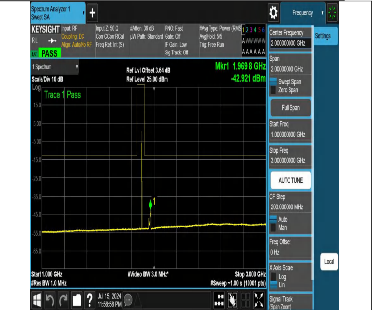
NTNV-DC_12A_n25A-PC3-15-5+20-M+M-N/A-N/A-DFT-QPSK-Edge_1RB_Right-1000-3000-PASS
