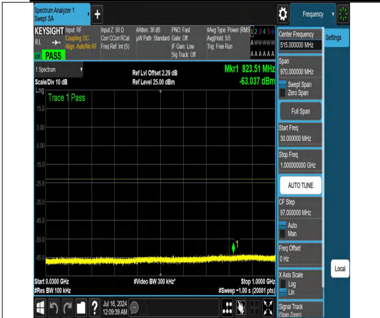
NTNV-DC_12A_n25A-PC3-15-5+25-M+M-N/A-N/A-DFT-PI2BPSK-Edge_1RB_Right-30-1000-PASS
