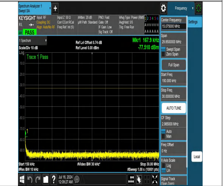
NTNV-DC_12A_n25A-PC3-15-5+25-M+M-N/A-N/A-DFT-PI2BPSK-E dge_1RB_Right-0.15-30-PASS
