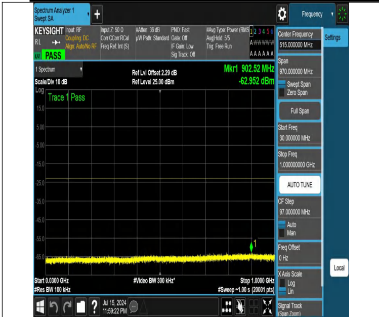
NTNV-DC_12A_n25A-PC3-15-5+20-M+H-N/A-N/A-DFT-PI2BPSK-Edge_1RB_Right-30-1000-PASS
