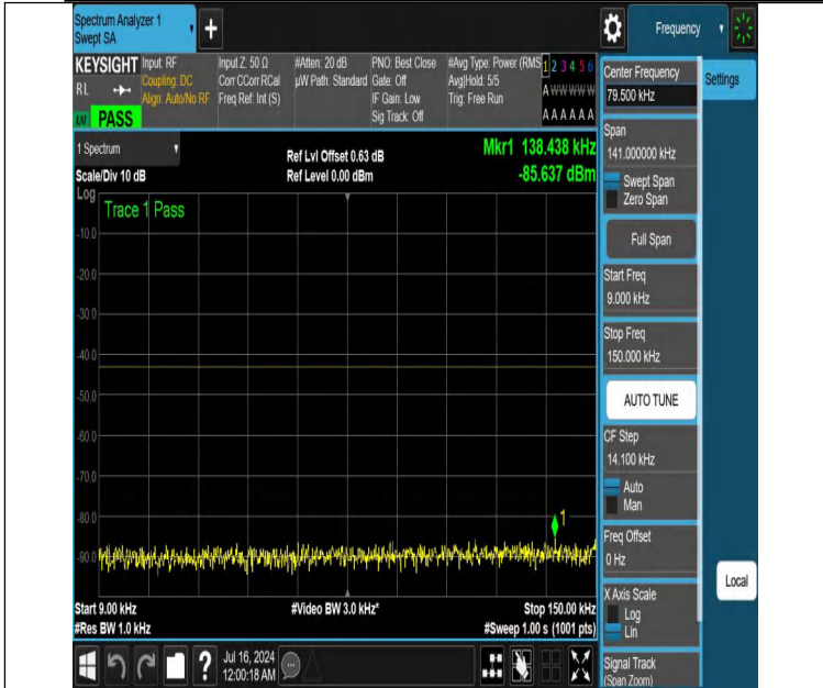
NTNV-DC_12A_n25A-PC3-15-5+20-M+H-N/A-N/A-DFT-QPSK-Edge e_1RB_Left-0.009-0.15-PASS
