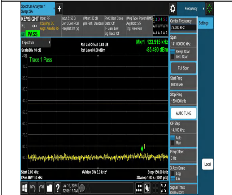
NTNV-DC_12A_n25A-PC3-15-5+25-M+M-N/A-N/A-DFT-PI2BPSK-Edge_1RB_Right-0.009-0.15-PASS
