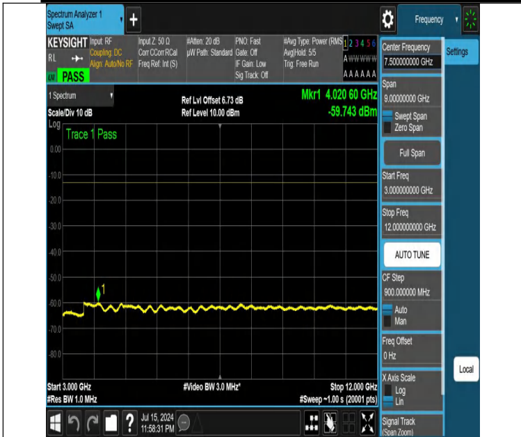
NTNV-DC_12A_n25A-PC3-15-5+20-M+H-N/A-N/A-DFT-PI2BPSK-Edge_1RB_Left-3000-12000-PASS
