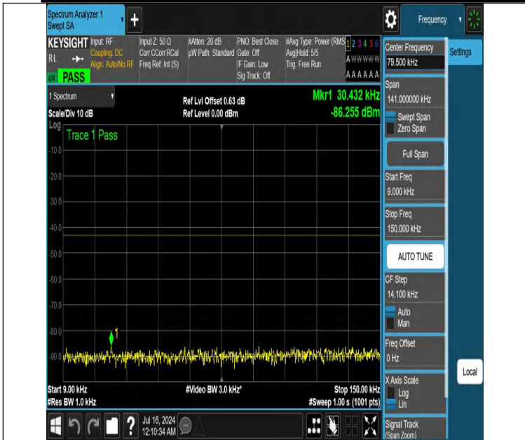
NTNV-DC_12A_n25A-PC3-15-5+25-M+M-N/A-N/A-DFT-QPSK-Edge_1RB_Left-0.009-0.15-PASS
