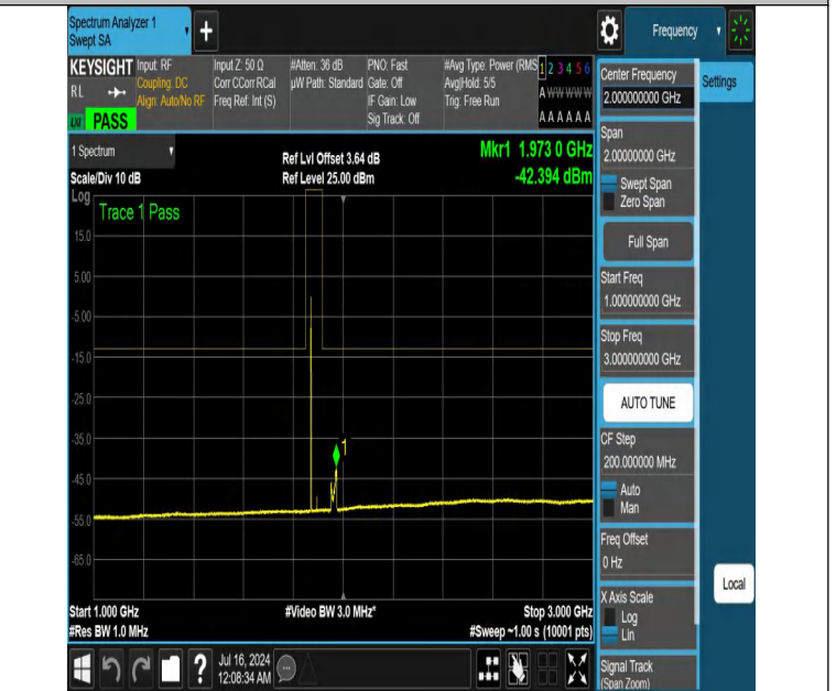
NTNV-DC_12A_n25A-PC3-15-5+25-M+M-N/A-N/A-DFT-PI2BPSK-E dge_1RB_Left-1000-3000-PASS
