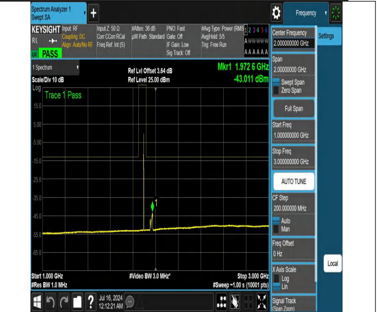
NTNV-DC_12A_n25A-PC3-15-5+25-M+M-N/A-N/A-DFT-QPSK-Edge_1RB_Right-1000-3000-PASS
