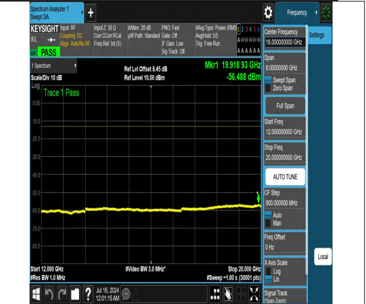
NTNV-DC_12A_n25A-PC3-15-5+20-M+H-N/A-N/A-DFT-QPSK-Edge e_1RB_Left-12000-20000-PASS
