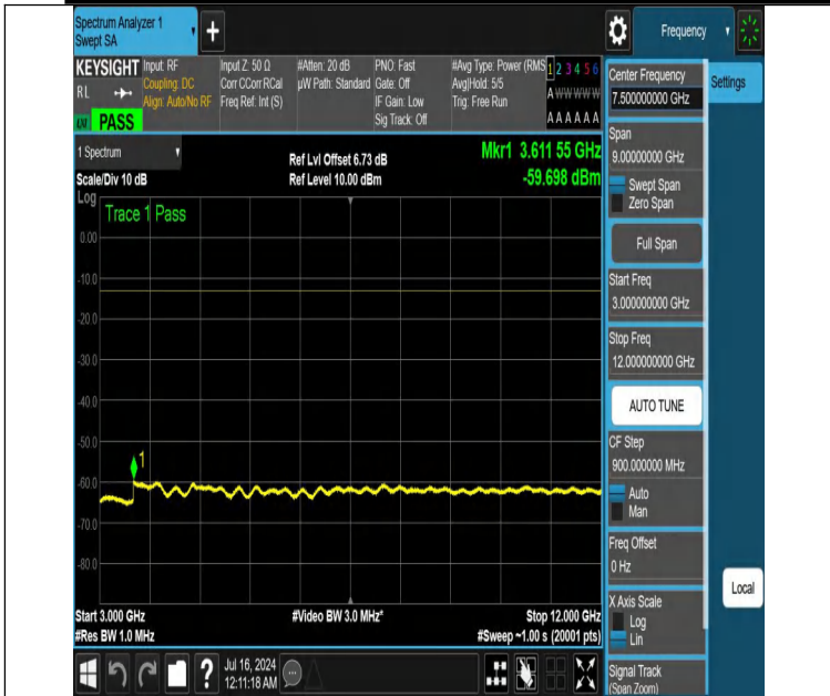
NTNV-DC_12A_n25A-PC3-15-5+25-M+M-N/A-N/A-DFT-QPSK-Edge_1RB_Left-3000-12000-PASS
