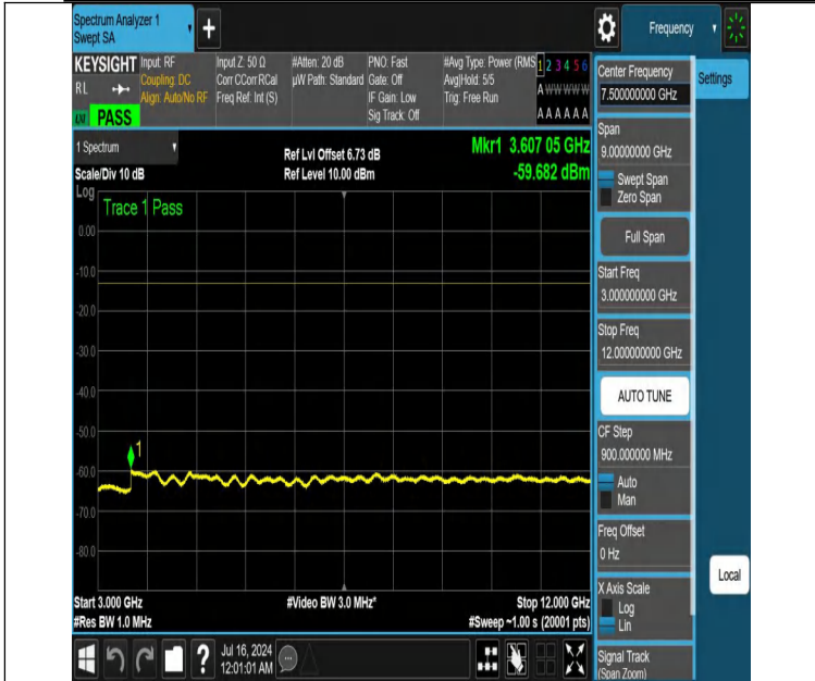
NTNV-DC_12A_n25A-PC3-15-5+20-M+H-N/A-N/A-DFT-QPSK-Edge e_1RB_Left-3000-12000-PASS
