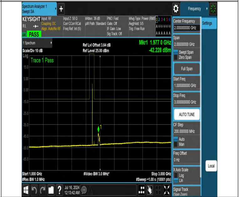
NTNV-DC_12A_n25A-PC3-15-5+25-M+H-N/A-N/A-DFT-PI2BPSK-E dge_1RB_Left-1000-3000-PASS
