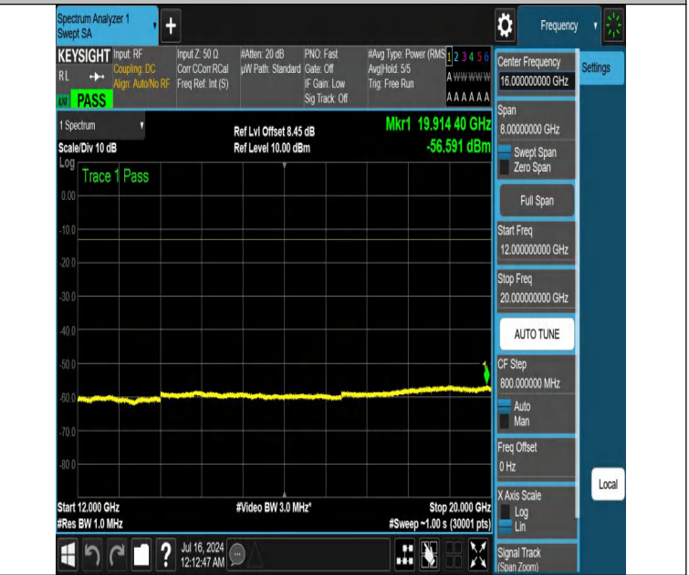
NTNV-DC_12A_n25A-PC3-15-5+25-M+M-N/A-N/A-DFT-QPSK-Edge_1RB_Right-12000-20000-PASS
