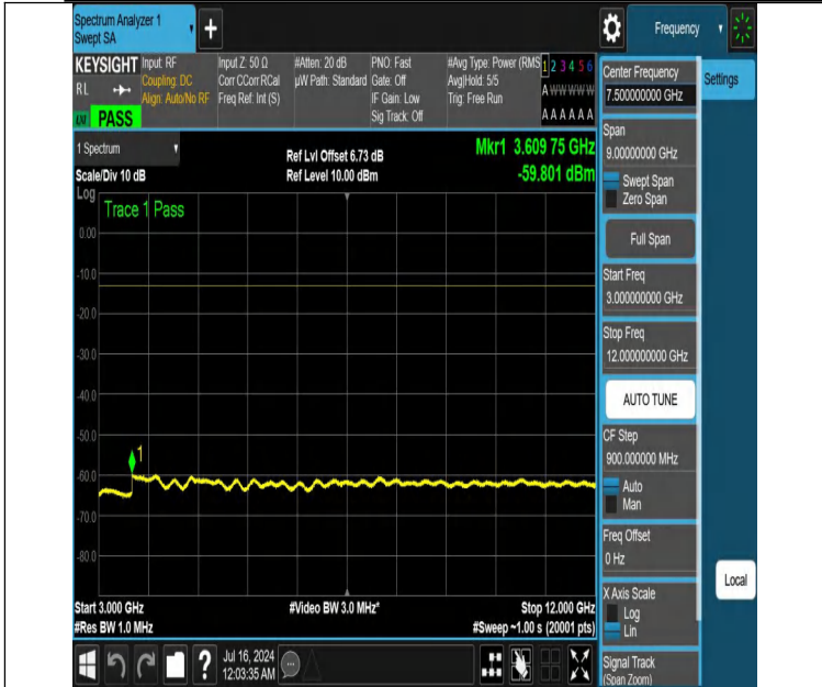
NTNV-DC_12A_n25A-PC3-15-5+25-M+L-N/A-N/A-DFT-PI2BPSK-Edge_1RB_Left-3000-12000-PASS
