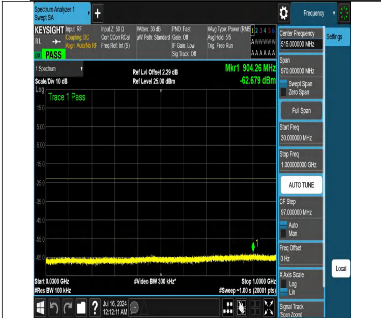
NTNV-DC_12A_n25A-PC3-15-5+25-M+M-N/A-N/A-DFT-QPSK-Edge_1RB_Right-30-1000-PASS
