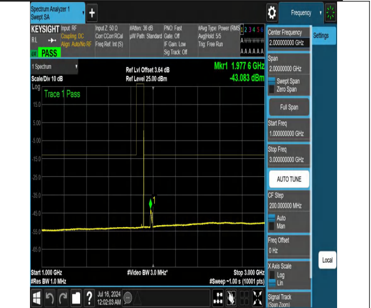
NTNV-DC_12A_n25A-PC3-15-5+20-M+H-N/A-N/A-DFT-QPSK-Edge e_1RB_Right-1000-3000-PASS
