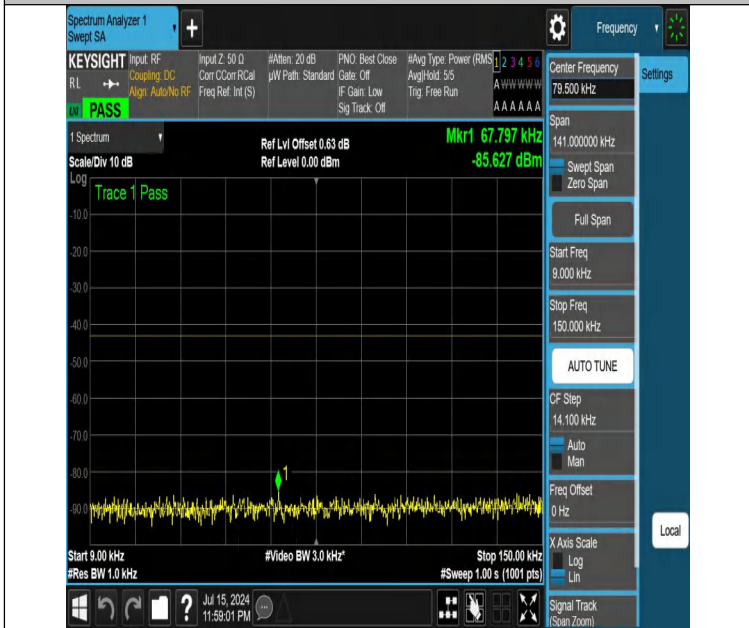
NTNV-DC_12A_n25A-PC3-15-5+20-M+H-N/A-N/A-DFT-PI2BPSK-Edge_1RB_Right-0.009-0.15-PASS
