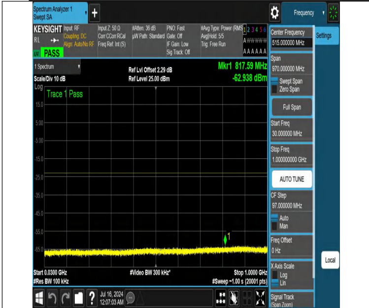
NTNV-DC_12A_n25A-PC3-15-5+25-M+L-N/A-N/A-DFT-QPSK-Edge e_1RB_Right-30-1000-PASS
