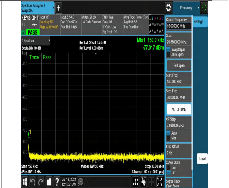
NTNV-DC_12A_n25A-PC3-15-5+25-M+H-N/A-N/A-DFT-PI2BPSK-E dge_1RB_Left-0.15-30-PASS
