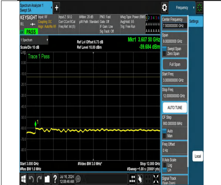
NTNV-DC_12A_n25A-PC3-15-5+25-M+M-N/A-N/A-DFT-PI2BPSK-Edge_1RB_Left-3000-12000-PASS
