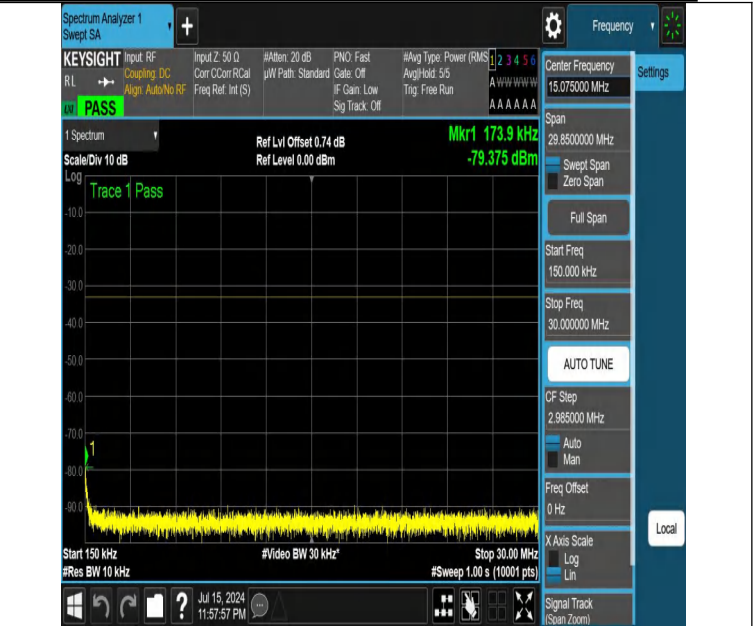
NTNV-DC_12A_n25A-PC3-15-5+20-M+H-N/A-N/A-DFT-PI2BPSK-E dge_1RB_Left-0.15-30-PASS
