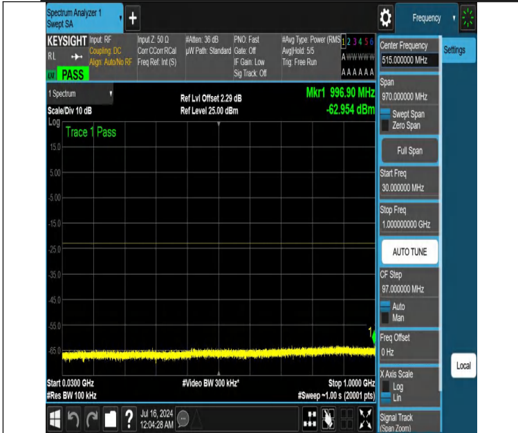
NTNV-DC_12A_n25A-PC3-15-5+25-M+L-N/A-N/A-DFT-PI2BPSK-Edge_1RB_Right-30-1000-PASS
