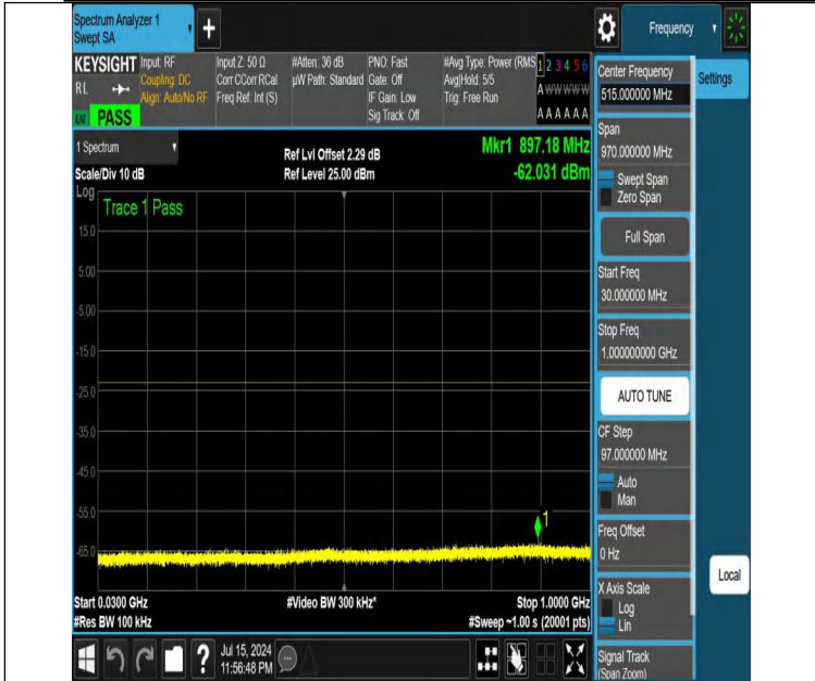
NTNV-DC_12A_n25A-PC3-15-5+20-M+M-N/A-N/A-DFT-QPSK-Edge_1RB_Right-30-1000-PASS
