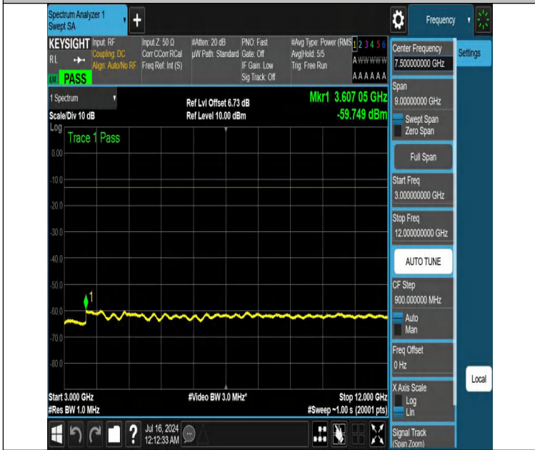
NTNV-DC_12A_n25A-PC3-15-5+25-M+M-N/A-N/A-DFT-QPSK-Edge_1RB_Right-3000-12000-PASS
