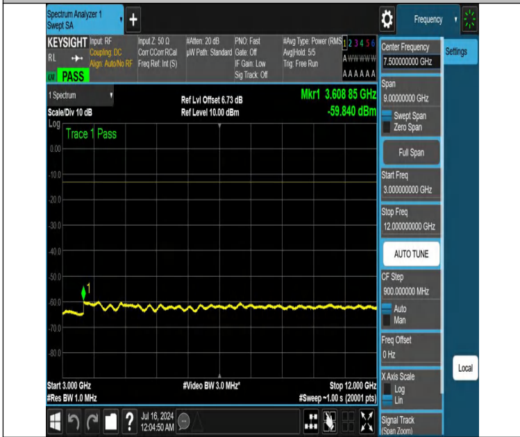
NTNV-DC_12A_n25A-PC3-15-5+25-M+L-N/A-N/A-DFT-PI2BPSK-Edge_1RB_Right-3000-12000-PASS
