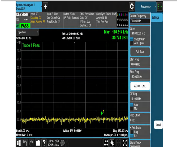
NTNV-DC_12A_n25A-PC3-15-5+25-M+L-N/A-N/A-DFT-QPSK-Edge e_1RB_Right-0.009-0.15-PASS
