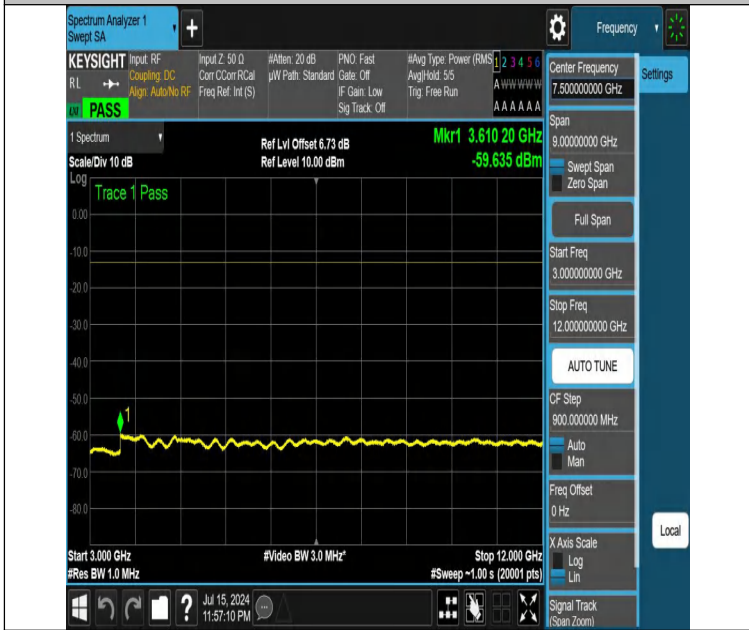
NTNV-DC_12A_n25A-PC3-15-5+20-M+M-N/A-N/A-DFT-QPSK-Edge_1RB_Right-3000-12000-PASS
