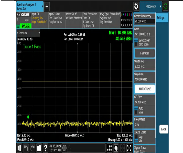
NTNV-DC_12A_n25A-PC3-15-5+25-M+H-N/A-N/A-DFT-PI2BPSK-Edge_1RB_Left-0.009-0.15-PASS
