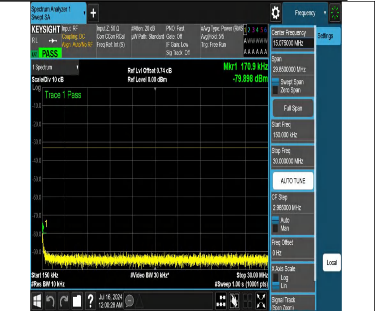
NTNV-DC_12A_n25A-PC3-15-5+20-M+H-N/A-N/A-DFT-QPSK-Edge e_1RB_Left-0.15-30-PASS
