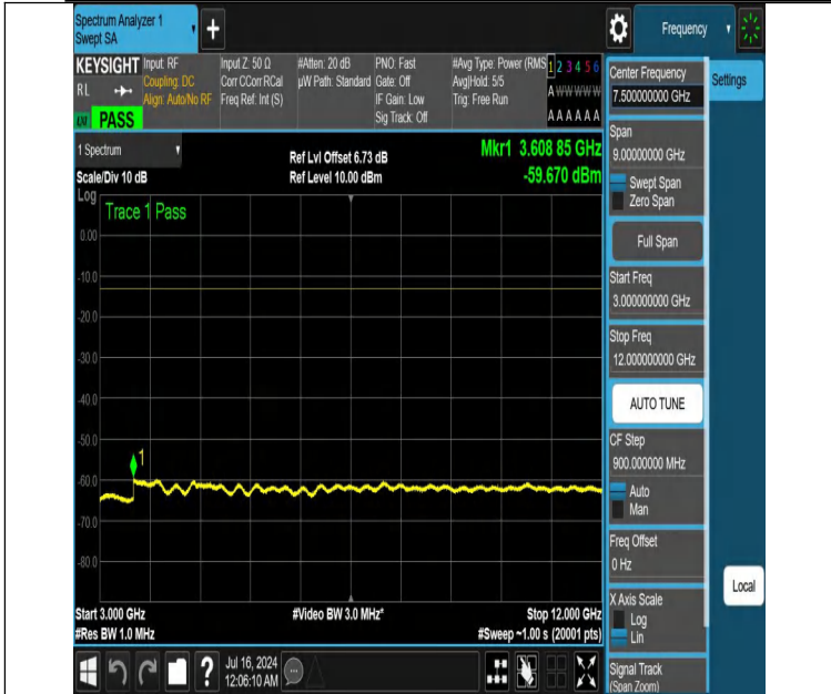
NTNV-DC_12A_n25A-PC3-15-5+25-M+L-N/A-N/A-DFT-QPSK-Edge e_1RB_Left-3000-12000-PASS
