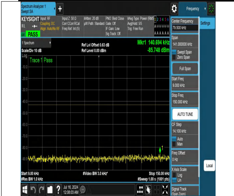
NTNV-DC_12A_n25A-PC3-15-5+25-M+M-N/A-N/A-DFT-PI2BPSK-Edge_1RB_Left-0.009-0.15-PASS
