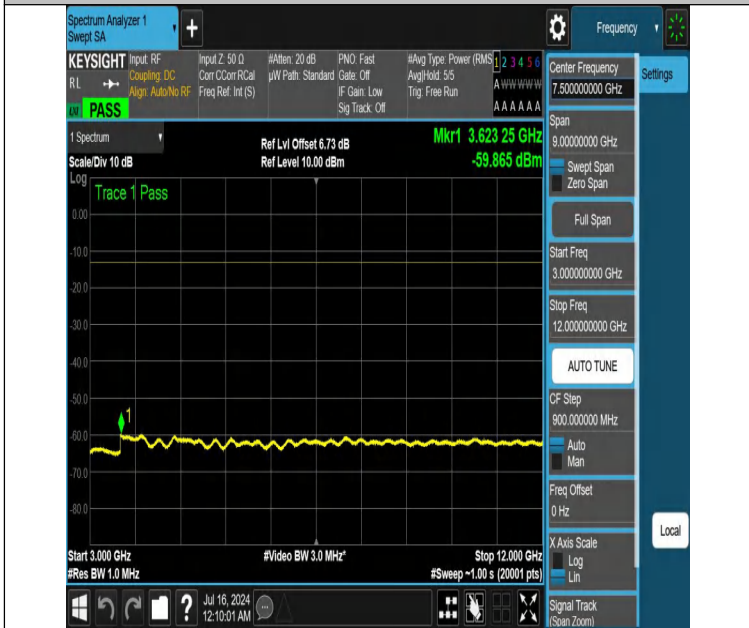
NTNV-DC_12A_n25A-PC3-15-5+25-M+M-N/A-N/A-DFT-PI2BPSK-Edge_1RB_Right-3000-12000-PASS
