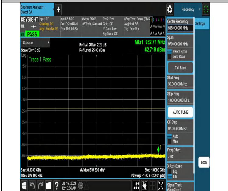
NTNV-DC_12A_n25A-PC3-15-5+25-M+M-N/A-N/A-DFT-QPSK-Edge_1RB_Left-30-1000-PASS
