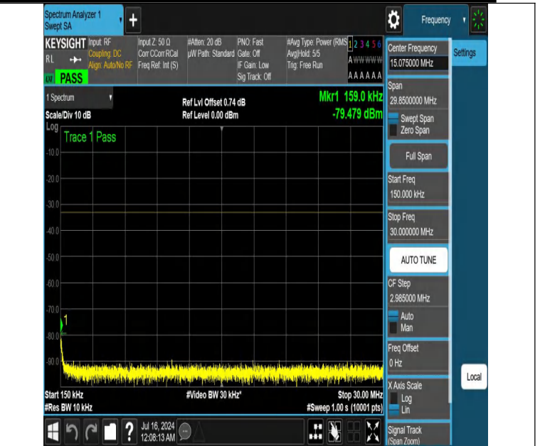
NTNV-DC_12A_n25A-PC3-15-5+25-M+M-N/A-N/A-DFT-PI2BPSK-E dge_1RB_Left-0.15-30-PASS
