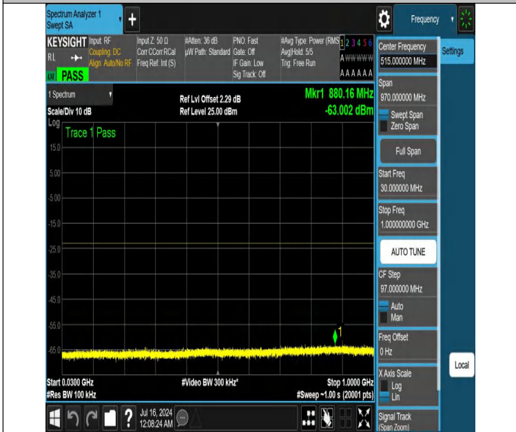
NTNV-DC_12A_n25A-PC3-15-5+25-M+M-N/A-N/A-DFT-PI2BPSK-Edge_1RB_Left-30-1000-PASS
