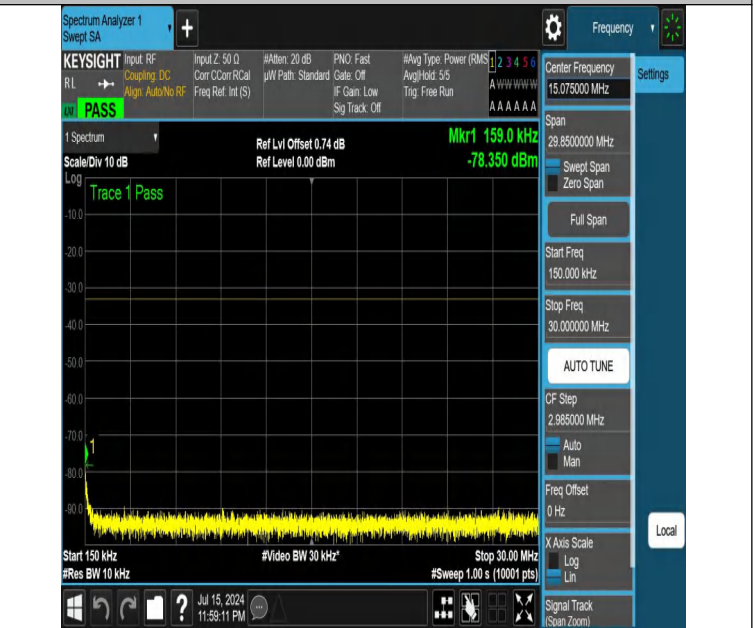
NTNV-DC_12A_n25A-PC3-15-5+20-M+H-N/A-N/A-DFT-PI2BPSK-E dge_1RB_Right-0.15-30-PASS
