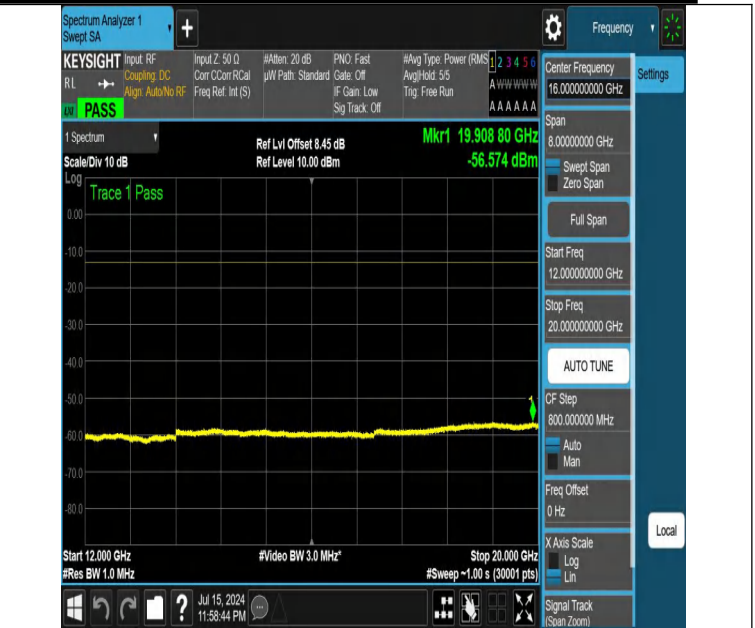
NTNV-DC_12A_n25A-PC3-15-5+20-M+H-N/A-N/A-DFT-PI2BPSK-E dge_1RB_Left-12000-20000-PASS
