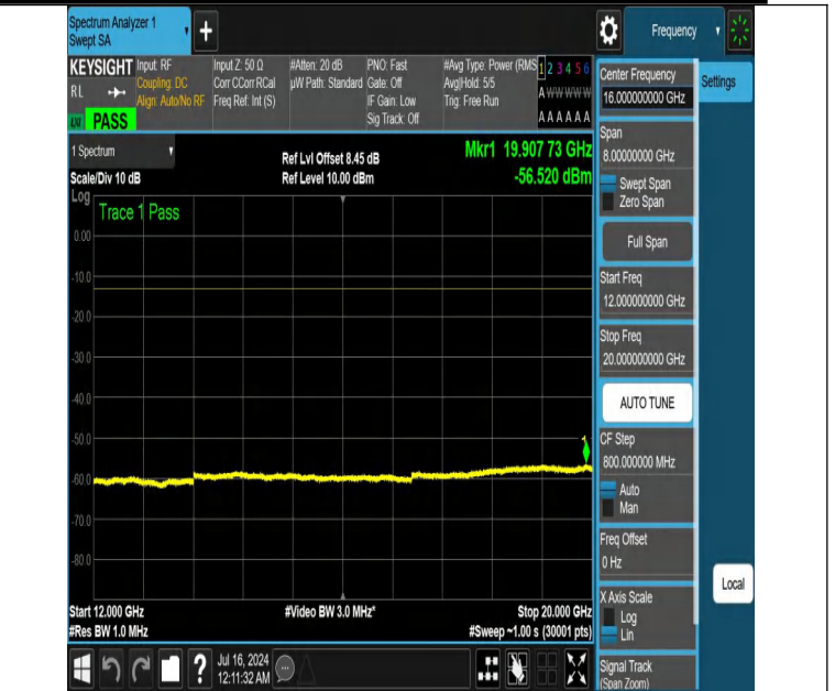
NTNV-DC_12A_n25A-PC3-15-5+25-M+M-N/A-N/A-DFT-QPSK-Edge_1RB_Left-12000-20000-PASS
