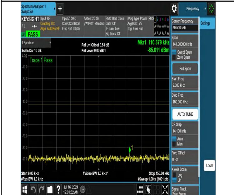
NTNV-DC_12A_n25A-PC3-15-5+20-M+H-N/A-N/A-DFT-QPSK-Edge e_1RB_Right-0.009-0.15-PASS
