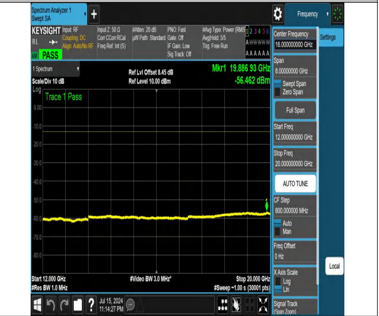
NTNV-DC_12A_n25A-PC3-15-5+5-M+H-N/A-N/A-DFT-PI2BPSK-Ed ge_1RB_Right-12000-20000-PASS
