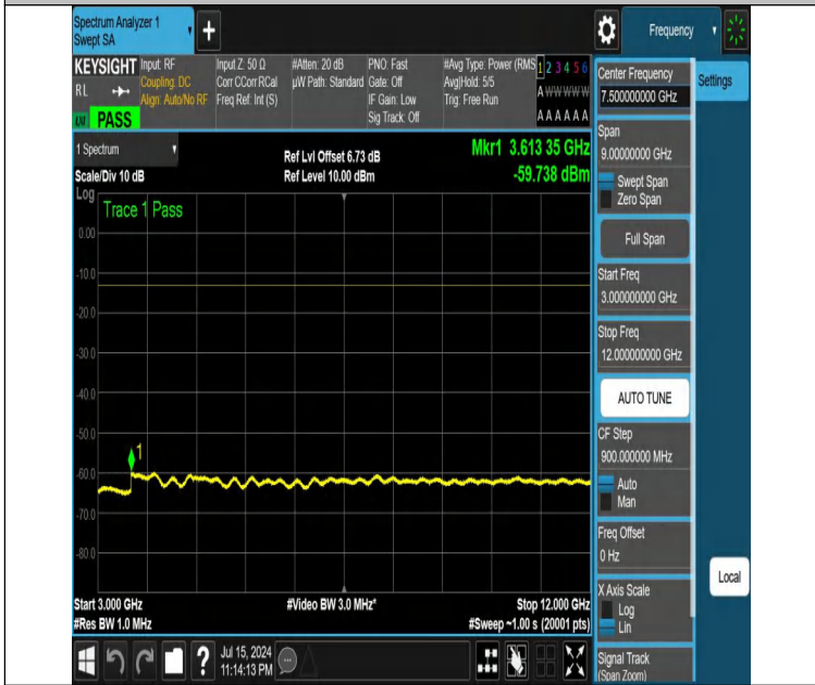
NTNV-DC_12A_n25A-PC3-15-5+5-M+H-N/A-N/A-DFT-PI2BPSK-E dge_1RB_Right-3000-12000-PASS
