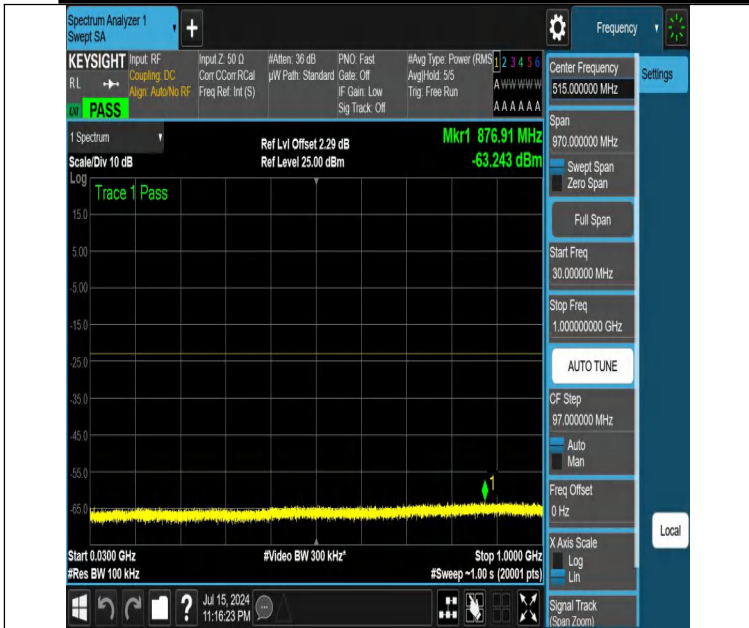
NTNV-DC_12A_n25A-PC3-15-5+5-M+H-N/A-N/A-DFT-QPSK-Edge _1RB_Right-30-1000-PASS
