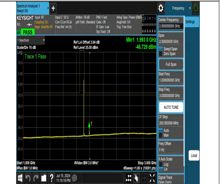
NTNV-DC_12A_n25A-PC3-15-5+5-M+H-N/A-N/A-DFT-QPSK-Edge_1RB_Left-1000-3000-PASS
