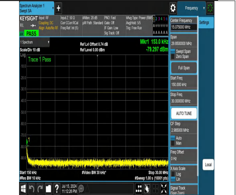
NTNV-DC_12A_n25A-PC3-15-5+5-M+H-N/A-N/A-DFT-PI2BPSK-Ed ge_1RB_Left-0.15-30-PASS
