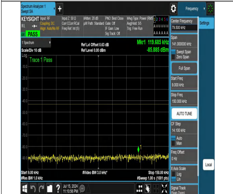
NTNV-DC_12A_n25A-PC3-15-5+5-M+M-N/A-N/A-DFT-QPSK-Edge e_1RB_Right-0.009-0.15-PASS
