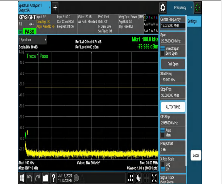
NTNV-DC_12A_n25A-PC3-15-5+5-M+H-N/A-N/A-DFT-QPSK-Edge _1RB_Right-0.15-30-PASS
