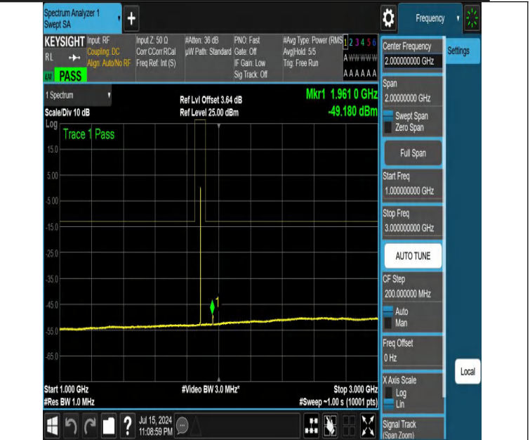
NTNV-DC_12A_n25A-PC3-15-5+5-M+M-N/A-N/A-DFT-PI2BPSK-Ed ge_1RB_Right-1000-3000-PASS
