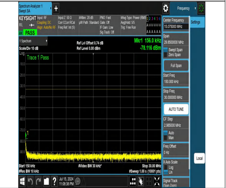
NTNV-DC_12A_n25A-PC3-15-5+5-M+M-N/A-N/A-DFT-PI2BPSK-Ed ge_1RB_Right-0.15-30-PASS
