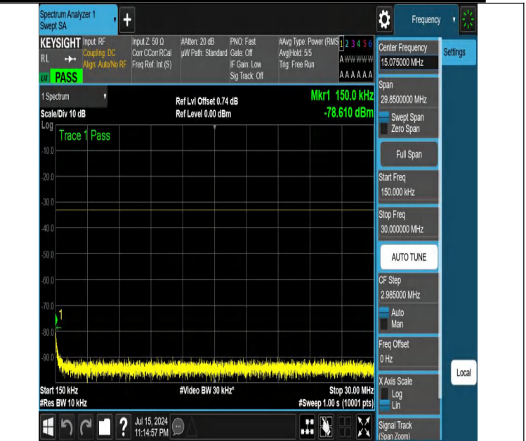
NTNV-DC_12A_n25A-PC3-15-5+5-M+H-N/A-N/A-DFT-QPSK-Edge_1RB_Left-0.15-30-PASS
