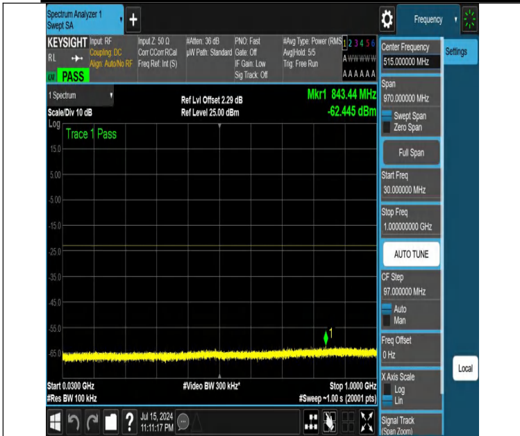
NTNV-DC_12A_n25A-PC3-15-5+5-M+M-N/A-N/A-DFT-QPSK-Edge e_1RB_Right-30-1000-PASS
