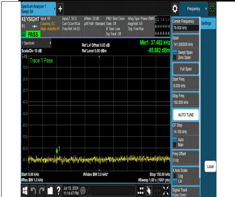
NTNV-DC_12A_n25A-PC3-15-5+5-M+H-N/A-N/A-DFT-QPSK-Edge_1RB_Left-0.009-0.15-PASS
