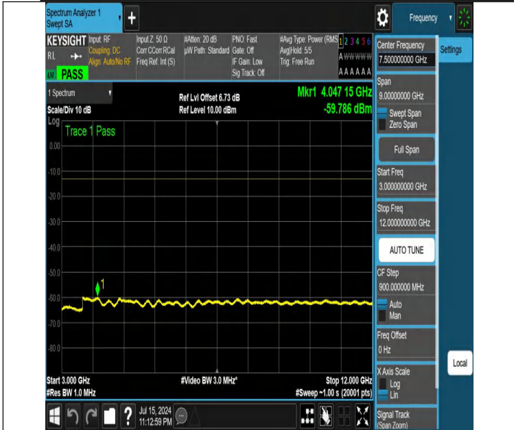
NTNV-DC_12A_n25A-PC3-15-5+5-M+H-N/A-N/A-DFT-PI2BPSK-E dge_1RB_Left-3000-12000-PASS
