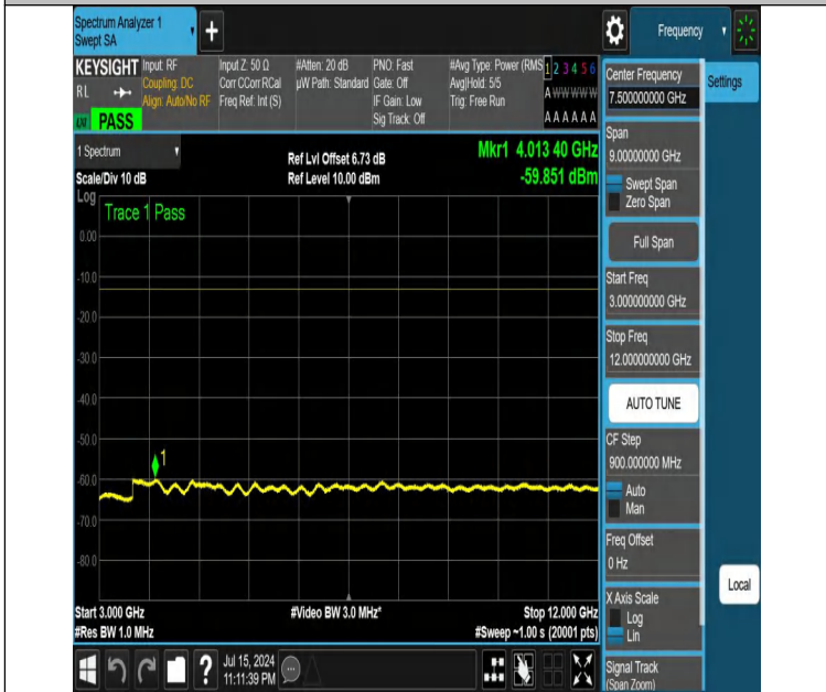
NTNV-DC_12A_n25A-PC3-15-5+5-M+M-N/A-N/A-DFT-QPSK-Edge e_1RB_Right-3000-12000-PASS
