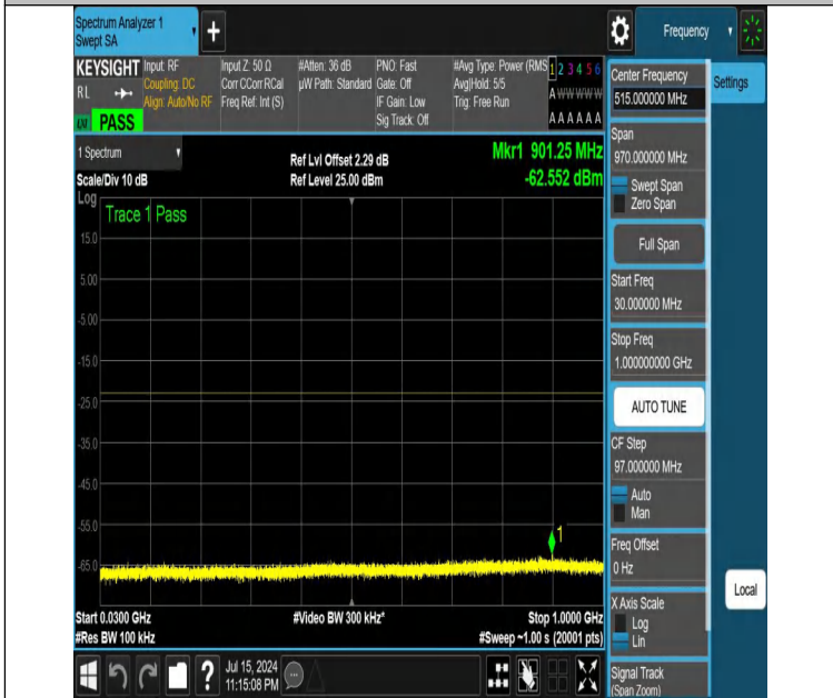
NTNV-DC_12A_n25A-PC3-15-5+5-M+H-N/A-N/A-DFT-QPSK-Edge_1RB_Left-30-1000-PASS
