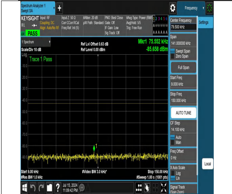
NTNV-DC_12A_n25A-PC3-15-5+5-M+M-N/A-N/A-DFT-QPSK-Edge e_1RB_Left-0.009-0.15-PASS
