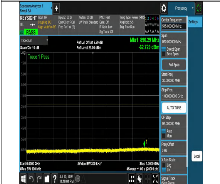
NTNV-DC_12A_n25A-PC3-15-5+5-M+M-N/A-N/A-DFT-QPSK-Edge e_1RB_Left-30-1000-PASS
