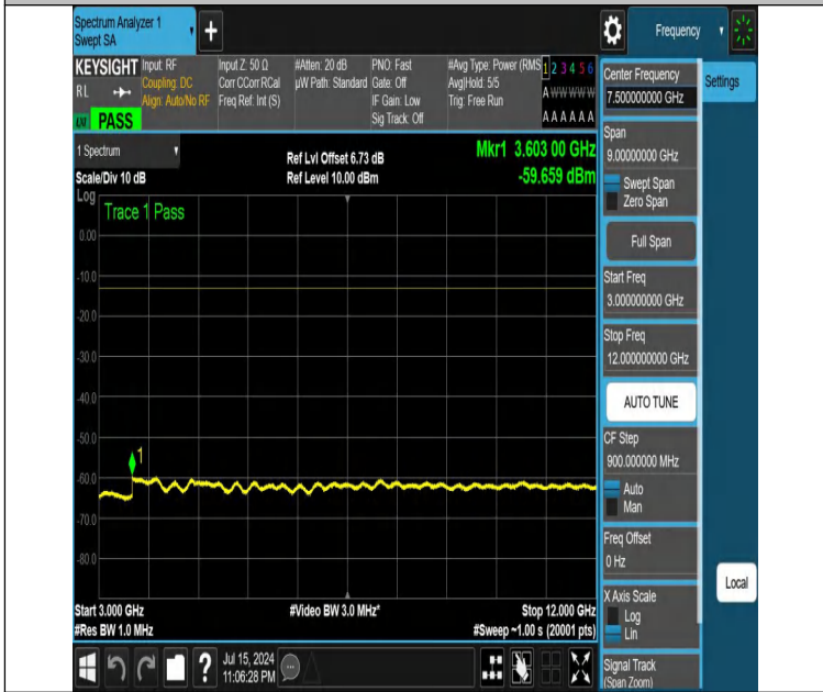
NTNV-DC_12A_n25A-PC3-15-5+5-M+L-N/A-N/A-DFT-QPSK-Edge_1RB_Right-3000-12000-PASS
