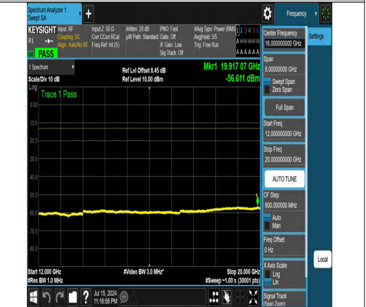
NTNV-DC_12A_n25A-PC3-15-5+5-M+H-N/A-N/A-DFT-QPSK-Edge _1RB_Right-12000-20000-PASS
