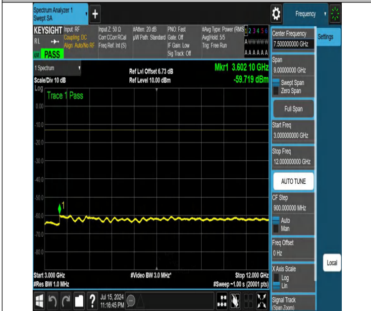
NTNV-DC_12A_n25A-PC3-15-5+5-M+H-N/A-N/A-DFT-QPSK-Edge _1RB_Right-3000-12000-PASS
