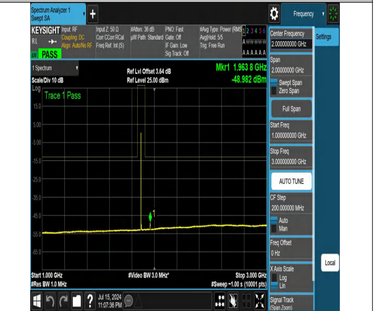
NTNV-DC_12A_n25A-PC3-15-5+5-M+M-N/A-N/A-DFT-PI2BPSK-Ed ge_1RB_Left-1000-3000-PASS
