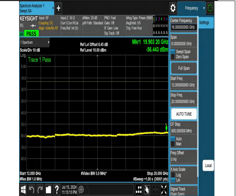
NTNV-DC_12A_n25A-PC3-15-5+5-M+H-N/A-N/A-DFT-PI2BPSK-Ed ge_1RB_Left-12000-20000-PASS
