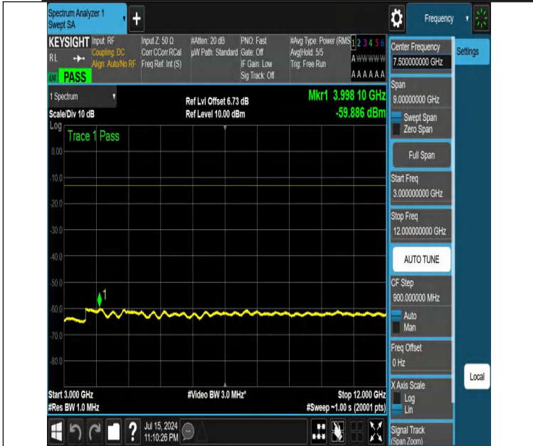
NTNV-DC_12A_n25A-PC3-15-5+5-M+M-N/A-N/A-DFT-QPSK-Edge e_1RB_Left-3000-12000-PASS
