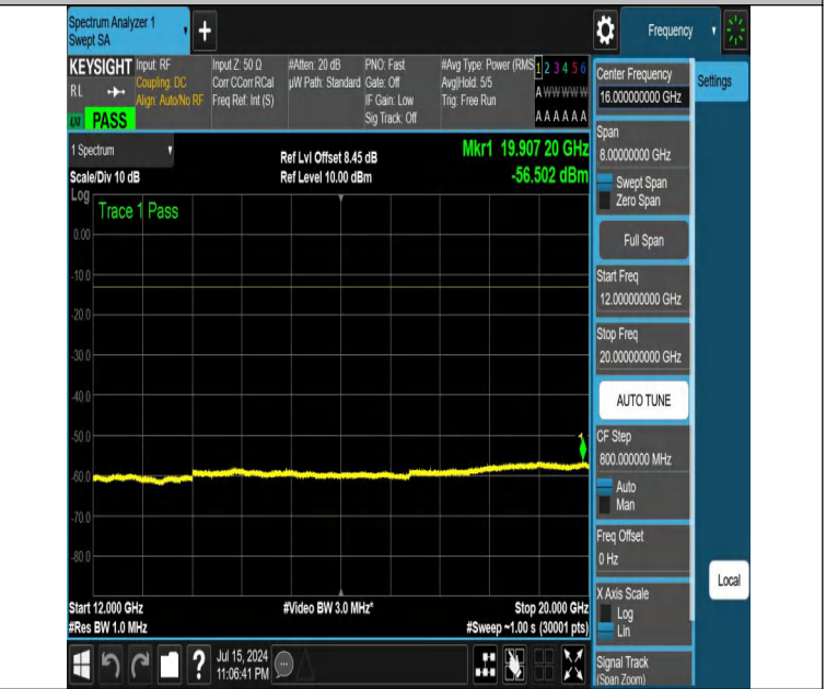
NTNV-DC_12A_n25A-PC3-15-5+5-M+L-N/A-N/A-DFT-QPSK-Edge_1RB_Right-12000-20000-PASS
