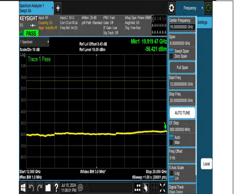
NTNV-DC_12A_n25A-PC3-15-5+5-M+M-N/A-N/A-DFT-PI2BPSK-Ed ge_1RB_Left-12000-20000-PASS
