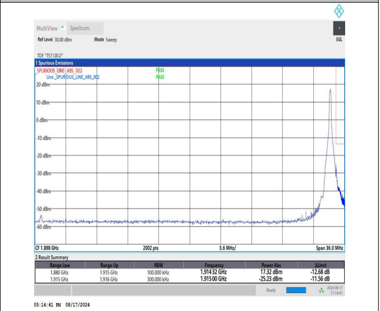
NTVN-DC_12A-n25A-PC3-15-5+35-M+H-QPSK-IDLE-DFT-QPSK-E dge_1RB_Right-PASS
