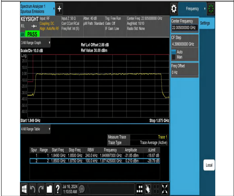
NTNV-DC_12A_n25A-PC3-15-5+25-M+L-N/A-N/A-DFT-PI2BPSK-Outer_Full-PASS
