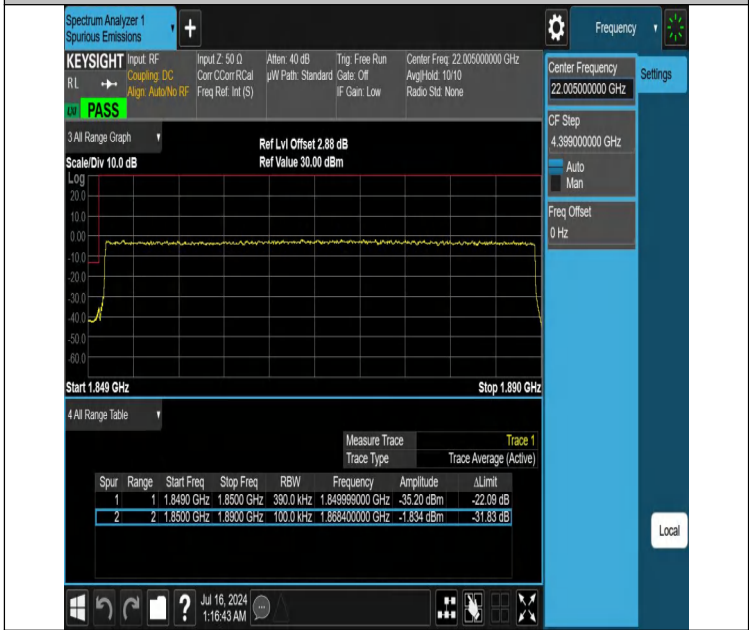
NTNV-DC_12A_n25A-PC3-15-5+40-M+L-N/A-N/A-DFT-PI2BPSK-Outer_Full-PASS
