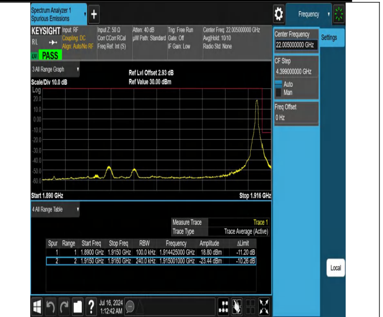
NTNV-DC_12A_n25A-PC3-15-5+25-M+H-N/A-N/A-DFT-QPSK-Edge_1RB_Right-PASS
