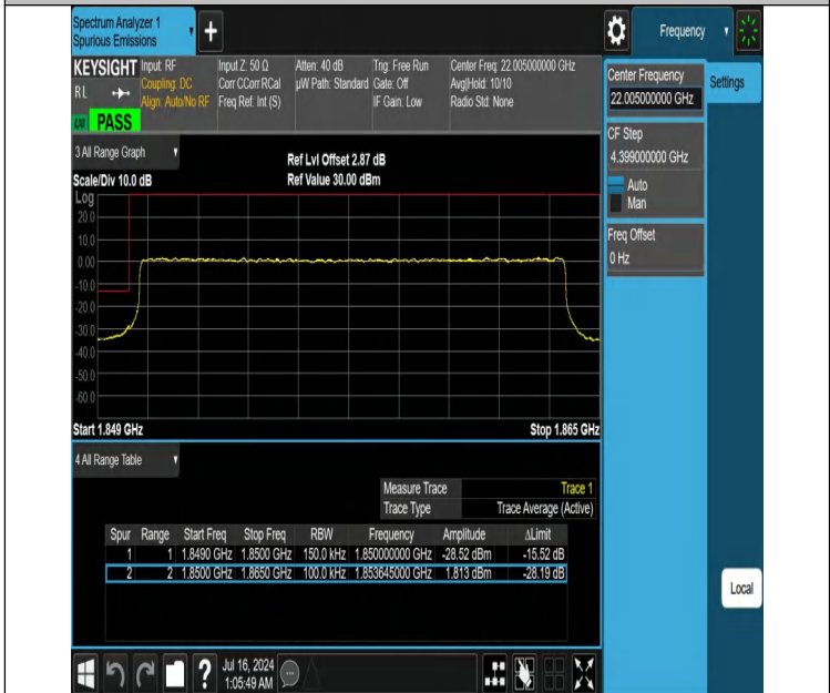
NTNV-DC_12A_n25A-PC3-15-5+15-M+L-N/A-N/A-DFT-QPSK-Outer_Full-PASS
