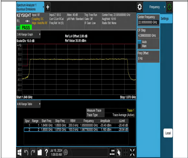
NTNV-DC_12A_n25A-PC3-15-5+20-M+L-N/A-N/A-DFT-PI2BPSK-Outer_Full-PASS
