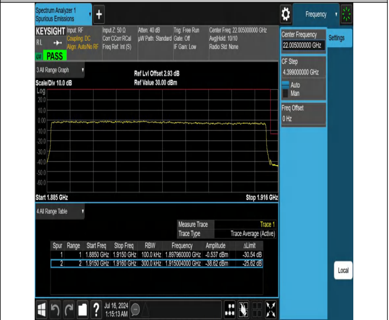
NTNV-DC_12A_n25A-PC3-15-5+30-M+H-N/A-N/A-DFT-PI2BPSK-O uter_Full-PASS
