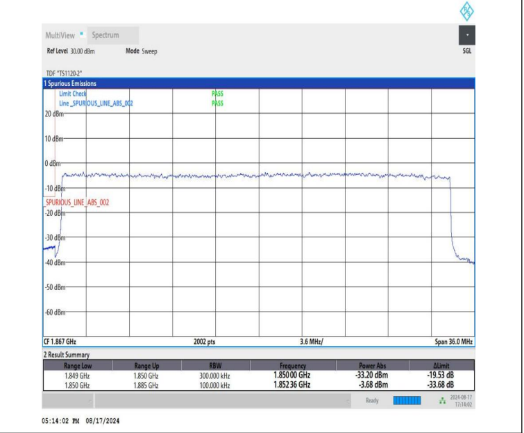
NTVN-DC_12A-n25A-PC3-15-5+35-M+L-QPSK-IDLE-DFT-QPSK-Outer_Full-PASS
