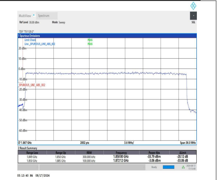
NTVN-DC_12A-n25A-PC3-15-5+35-M+L-QPSK-IDLE-DFT-BPSK-Outer_Full-PASS
