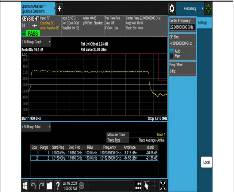
NTNV-DC_12A_n25A-PC3-15-5+15-M+H-N/A-N/A-DFT-PI2BPSK-O uter_Full-PASS
