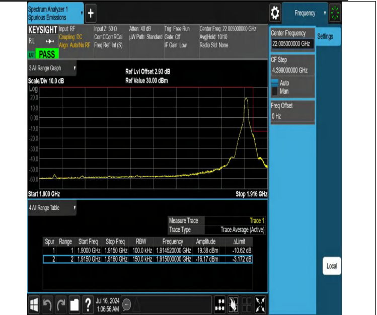
NTNV-DC_12A_n25A-PC3-15-5+15-M+H-N/A-N/A-DFT-QPSK-Edge_1RB_Right-PASS
