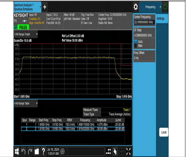
NTVN-DC_12A_n25A-PC3-15-5+10-M+H-N/A-N/A-DFT-PI2BPSK-O uter_Full-PASS
