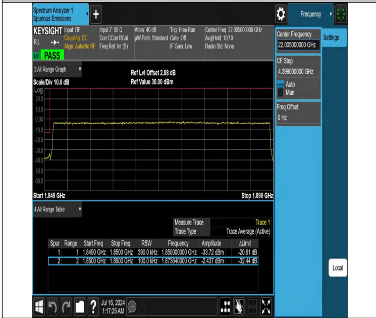
NTNV-DC_12A_n25A-PC3-15-5+40-M+L-N/A-N/A-DFT-QPSK-Outer_Full-PASS
