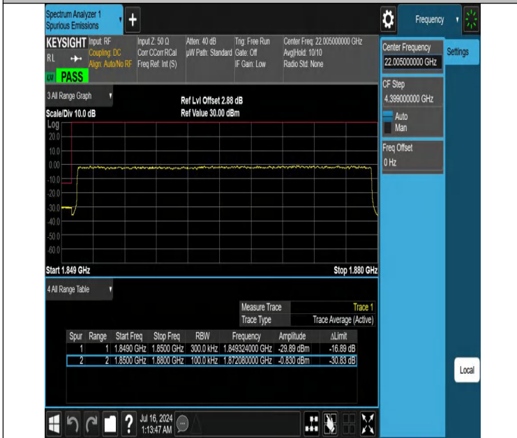
NTNV-DC_12A_n25A-PC3-15-5+30-M+L-N/A-N/A-DFT-PI2BPSK-Outer_Full-PASS
