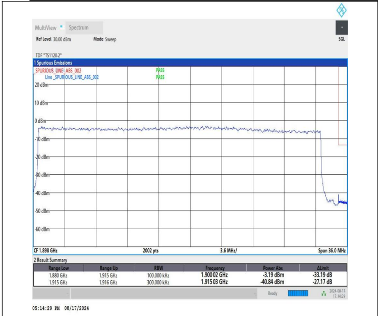
NTVN-DC_12A-n25A-PC3-15-5+35-M+H-QPSK-IDLE-DFT-BPSK-Outer_Full-PASS
