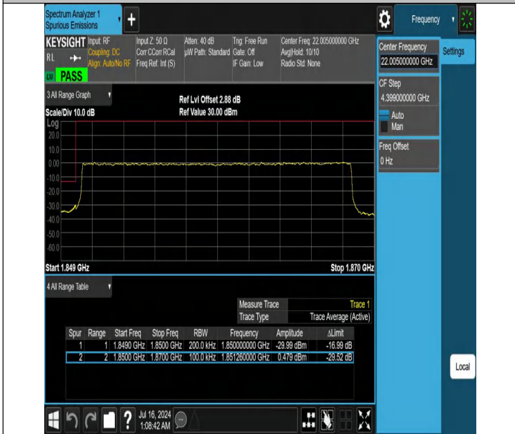
NTNV-DC_12A_n25A-PC3-15-5+20-M+L-N/A-N/A-DFT-QPSK-Outer_Full-PASS
