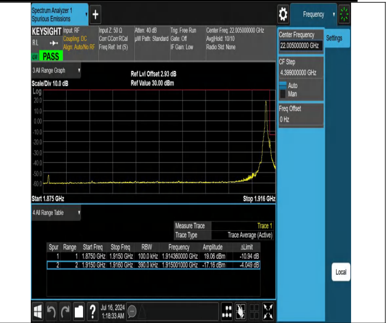
NTNV-DC_12A_n25A-PC3-15-5+40-M+H-N/A-N/A-DFT-QPSK-Edge_1RB_Right-PASS
