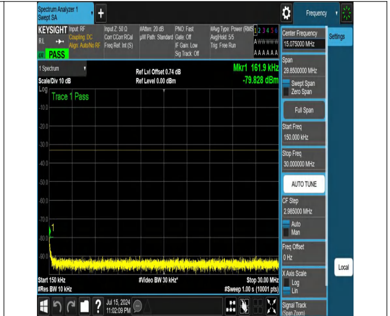
NTNV-DC_12A_n25A-PC3-15-5+5-M+L-N/A-N/A-DFT-PI2BPSK-Ed ge_1RB_Left-0.15-30-PASS
