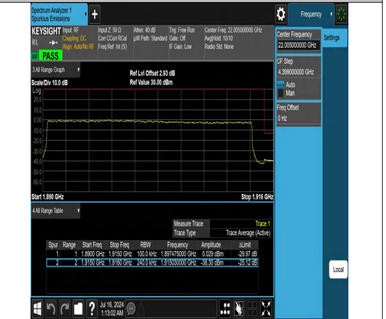
NTNV-DC_12A_n25A-PC3-15-5+25-M+H-N/A-N/A-DFT-QPSK-Outer_Full-PASS
