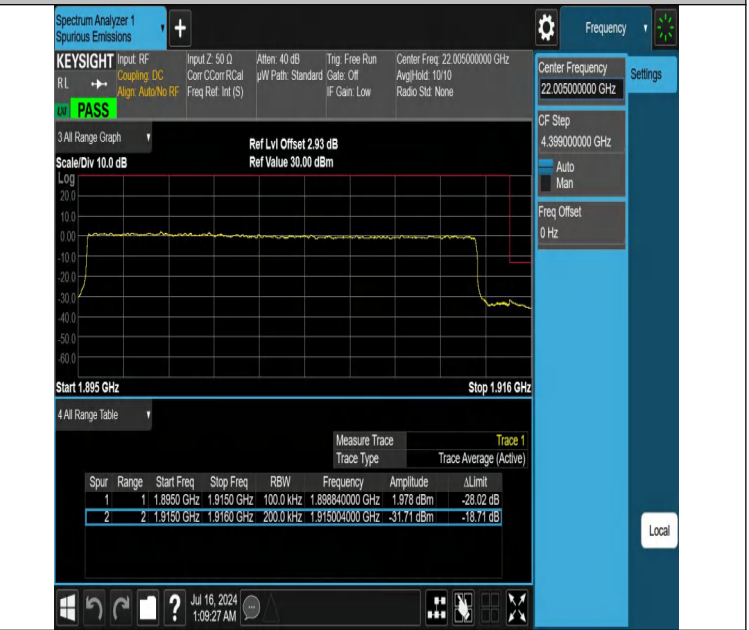
NTNV-DC_12A_n25A-PC3-15-5+20-M+H-N/A-N/A-DFT-PI2BPSK-O uter_Full-PASS
