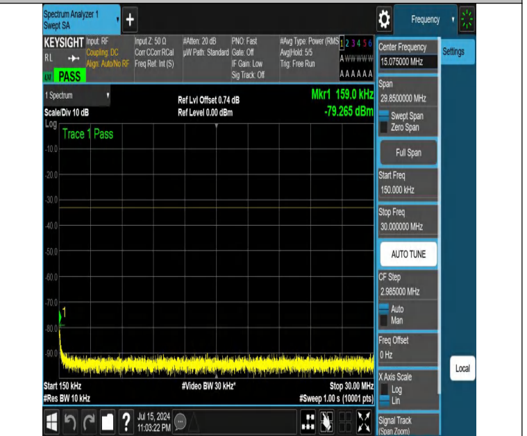
NTNV-DC_12A_n25A-PC3-15-5+5-M+L-N/A-N/A-DFT-PI2BPSK-Ed ge_1RB_Right-0.15-30-PASS
