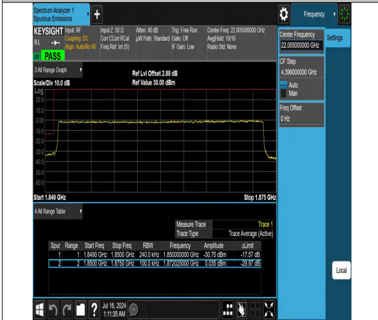
NTNV-DC_12A_n25A-PC3-15-5+25-M+L-N/A-N/A-DFT-QPSK-Outer_Full-PASS
