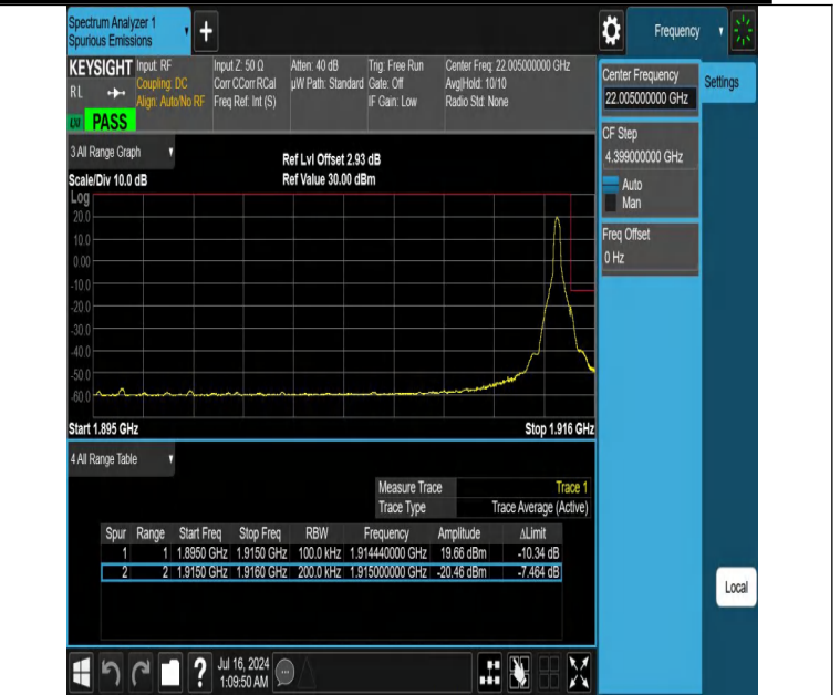
NTNV-DC_12A_n25A-PC3-15-5+20-M+H-N/A-N/A-DFT-QPSK-Edge_1RB_Right-PASS
