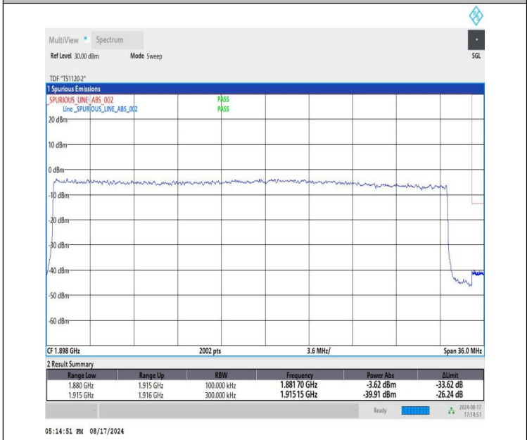
NTVN-DC_12A-n25A-PC3-15-5+35-M+H-QPSK-IDLE-DFT-QPSK-Outer_Full-PASS
