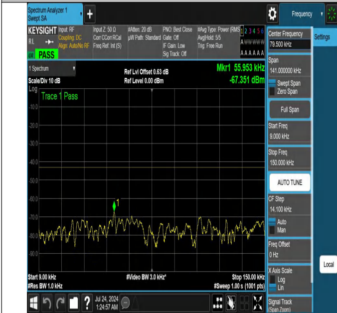
NTNV-N25-PC3-15-40-M-DFT-PI2BPSK-Edge_1RB_Right-0.009 -0.15-Ant1-PASS
