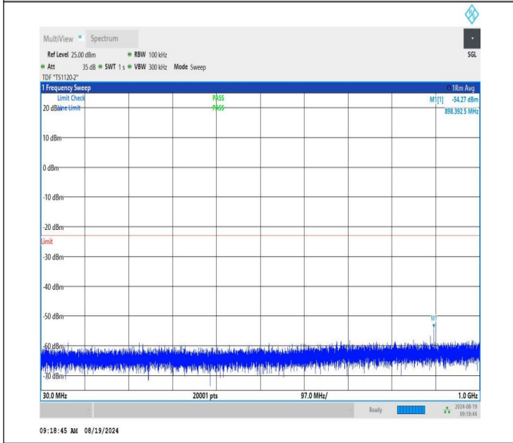
NTNV-n25-PC3-15-35-L-DFT-BPSK-Edge_1RB_Left-30-1000-PASS
