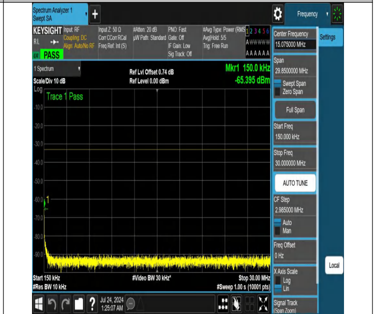
NTNV-N25-PC3-15-40-M-DFT-PI2BPSK-Edge_1RB_Right-0.15-3 0-Ant1-PASS
