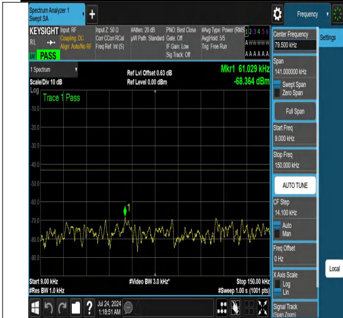
NTNV-N25-PC3-15-40-L-DFT-PI2BPSK-Edge_1RB_Left-0.009-0.15-Ant1-PASS
