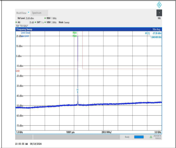
NTNV-n25-PC3-15-35-L-DFT-BPSK-Edge_1RB_Left-1000-3000-PASS
