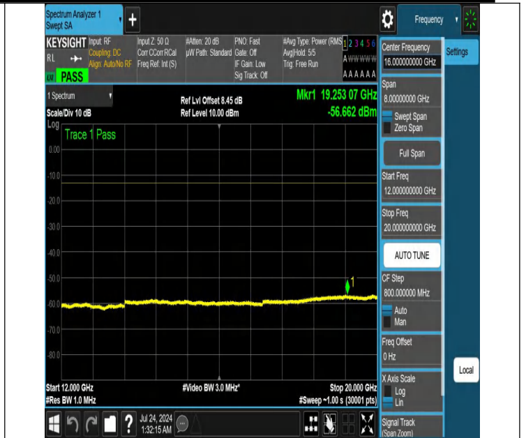
NTNV-N25-PC3-15-40-H-DFT-QPSK-Edge_1RB_Left-12000-2000 0-Ant1-PASS
