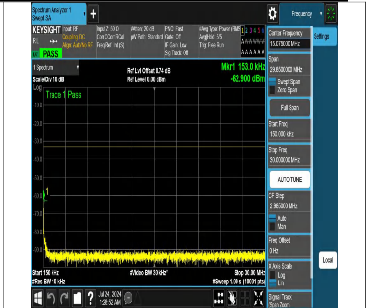
NTNV-N25-PC3-15-40-H-DFT-PI2BPSK-Edge_1RB_Left-0.15-30-Ant1-PASS
