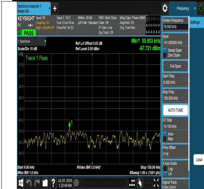
NTNV-N25-PC3-15-40-M-DFT-PI2BPSK-Edge_1RB_Left-0.009-0.15-Ant1-PASS
