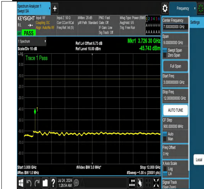
NTNV-N25-PC3-15-40-M-DFT-QPSK-Edge_1RB_Left-3000-1200 0-Ant1-PASS
