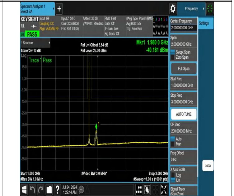
NTNV-N25-PC3-15-40-H-DFT-PI2BPSK-Edge_1RB_Left-1000-3000-Ant1-PASS
