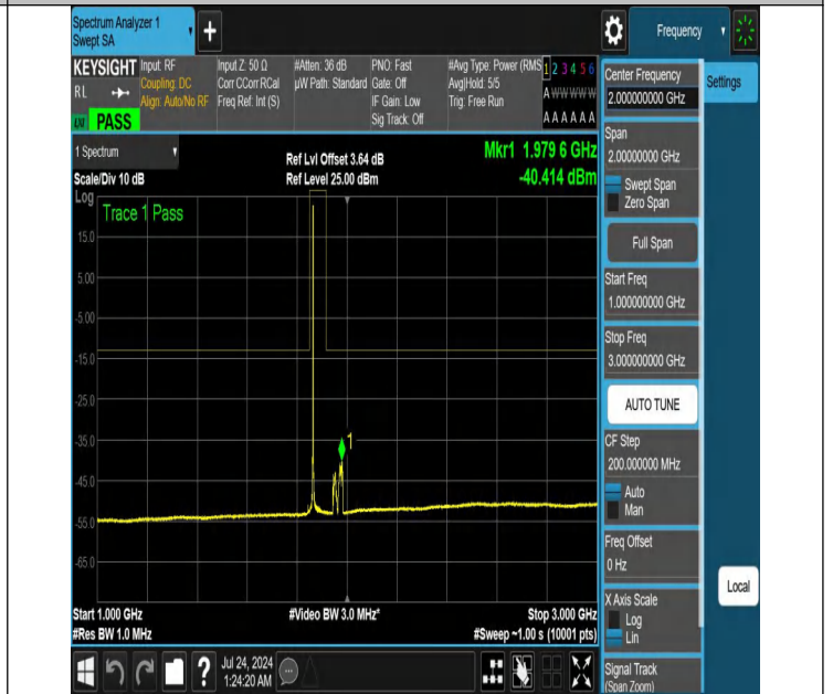
NTNV-N25-PC3-15-40-M-DFT-PI2BPSK-Edge_1RB_Left-1000-3000-Ant1-PASS
