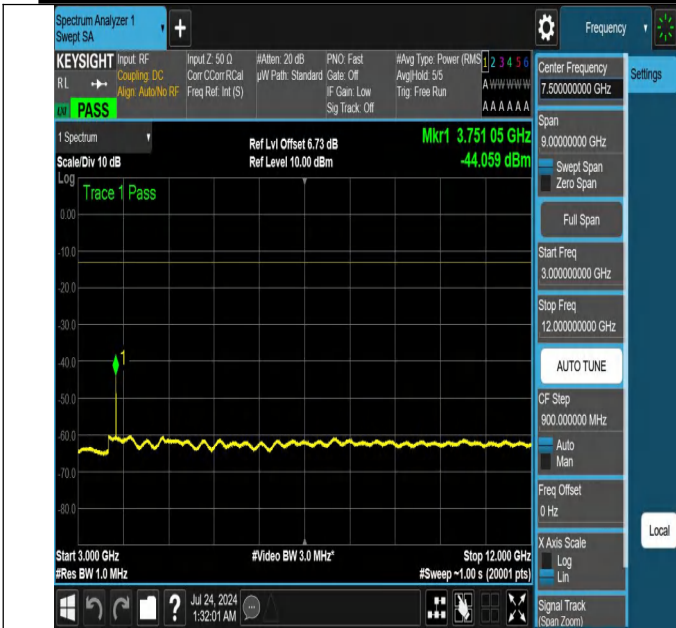
NTNV-N25-PC3-15-40-H-DFT-QPSK-Edge_1RB_Left-3000-1200 0-Ant1-PASS
