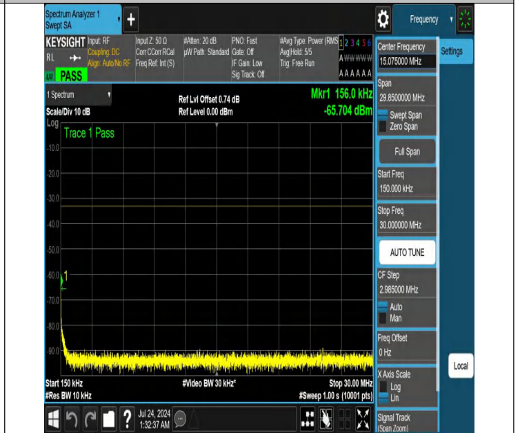
NTNV-N25-PC3-15-40-H-DFT-QPSK-Edge_1RB_Right-0.15-30-A nt1-PASS
