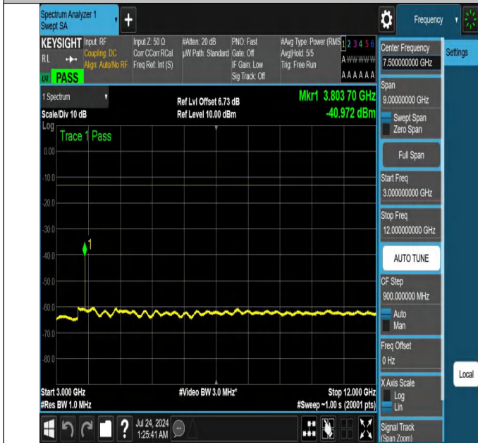
NTNV-N25-PC3-15-40-M-DFT-PI2BPSK-Edge_1RB_Right-3000-12000-Ant1-PASS
