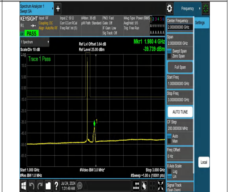
NTNV-N25-PC3-15-40-H-DFT-QPSK-Edge_1RB_Left-1000-3000- Ant1-PASS
