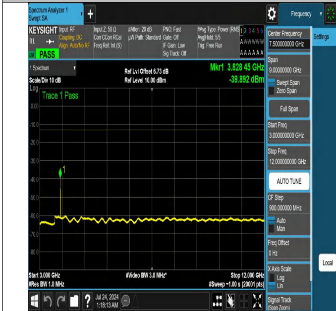
NTNV-N25-PC3-15-30-H-DFT-QPSK-Edge_1RB_Right-3000-120-00-Ant1-PASS
