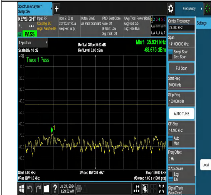
NTNV-N25-PC3-15-40-H-DFT-PI2BPSK-Edge_1RB_Right-0.009- 0.15-Ant1-PASS
