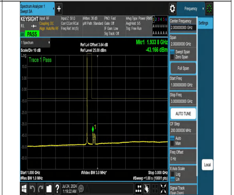
NTNV-N25-PC3-15-40-L-DFT-PI2BPSK-Edge_1RB_Left-1000-3000-Ant1-PASS
