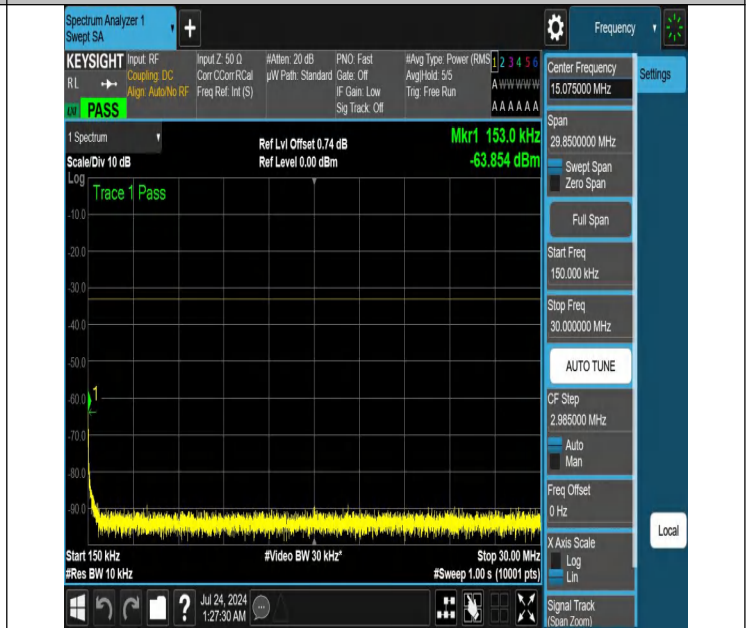
NTNV-N25-PC3-15-40-M-DFT-QPSK-Edge_1RB_Right-0.15-30-A nt1-PASS
