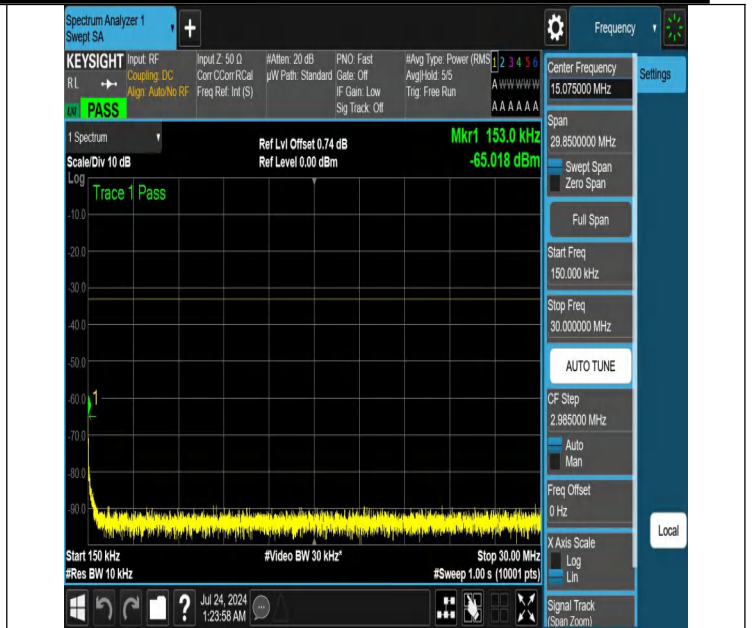
NTNV-N25-PC3-15-40-M-DFT-PI2BPSK-Edge_1RB_Left-0.15-30-Ant1-PASS
