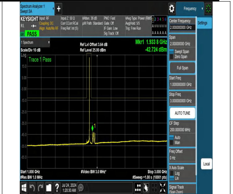
NTNV-N25-PC3-15-40-L-DFT-PI2BPSK-Edge_1RB_Right-1000-3000-Ant1-PASS
