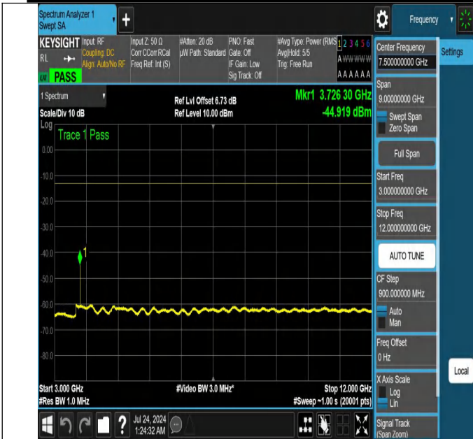
NTNV-N25-PC3-15-40-M-DFT-PI2BPSK-Edge_1RB_Left-3000-1 2000-Ant1-PASS
