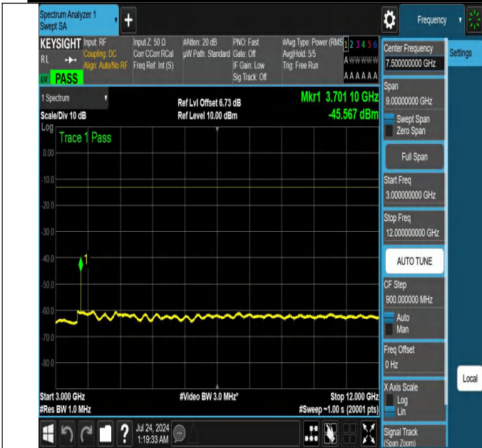
NTNV-N25-PC3-15-40-L-DFT-PI2BPSK-Edge_1RB_Left-3000-12000-Ant1-PASS
