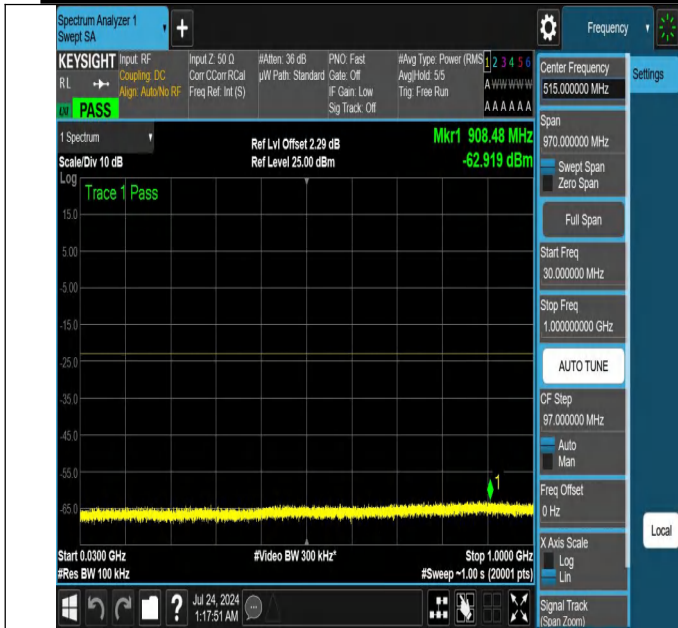
NTNV-N25-PC3-15-30-H-DFT-QPSK-Edge_1RB_Right-30-1000-Ant1-PASS
