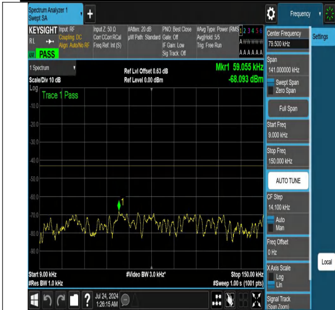
NTNV-N25-PC3-15-40-M-DFT-QPSK-Edge_1RB_Left-0.009-0.15 -Ant1-PASS
