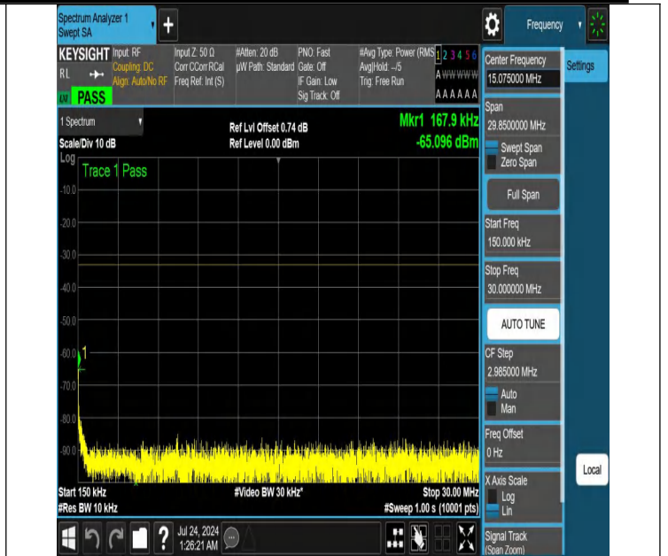
NTNV-N25-PC3-15-40-M-DFT-QPSK-Edge_1RB_Left-0.15-30-Ant 1-PASS
