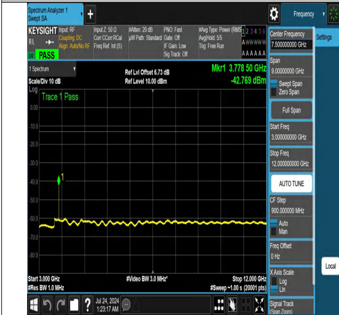
NTNV-N25-PC3-15-40-L-DFT-QPSK-Edge_1RB_Right-3000-12000-Ant1-PASS
