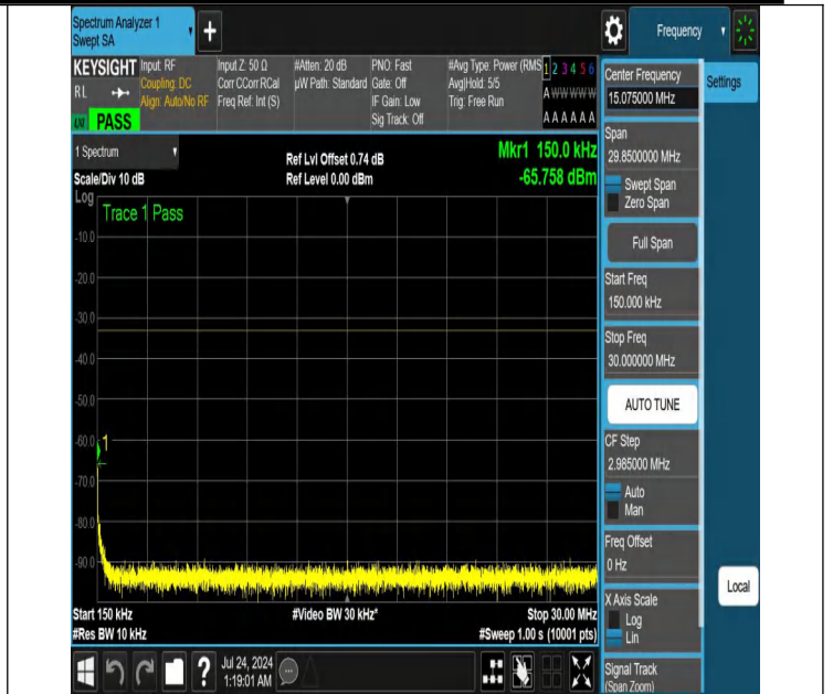
NTNV-N25-PC3-15-40-L-DFT-PI2BPSK-Edge_1RB_Left-0.15-30-Ant1-PASS
