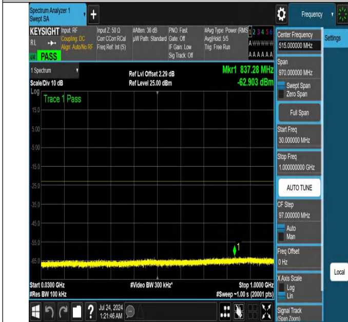
NTNV-N25-PC3-15-40-L-DFT-QPSK-Edge_1RB_Left-30-1000-Ant1-PASS
