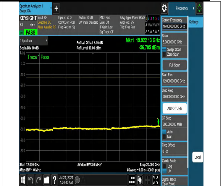
NTNV-N25-PC3-15-40-M-DFT-PI2BPSK-Edge_1RB_Left-12000-2 0000-Ant1-PASS
