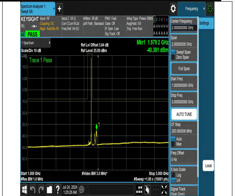
NTNV-N25-PC3-15-40-M-DFT-PI2BPSK-Edge_1RB_Right-1000-3000-Ant1-PASS
