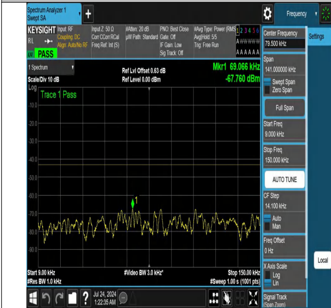
NTNV-N25-PC3-15-40-L-DFT-QPSK-Edge_1RB_Right-0.009-0.1 5-Ant1-PASS
