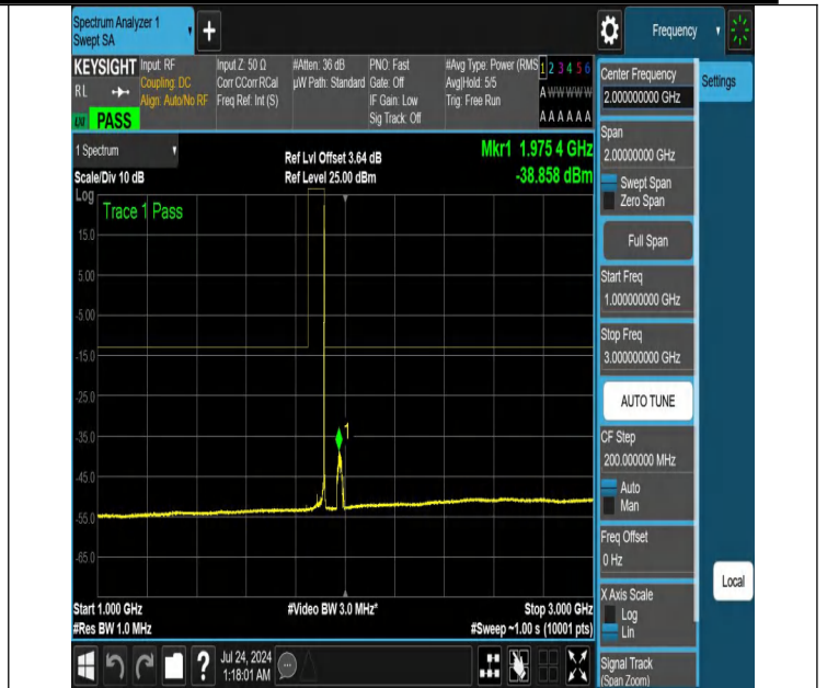
NTNV-N25-PC3-15-30-H-DFT-QPSK-Edge_1RB_Right-1000-300-0-Ant1-PASS
