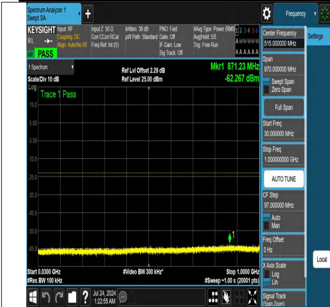
NTNV-N25-PC3-15-40-L-DFT-QPSK-Edge_1RB_Right-30-1000-Ant1-PASS
