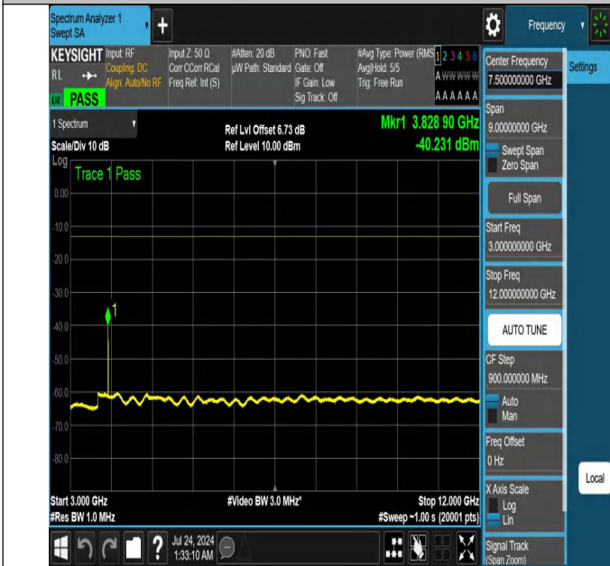
NTNV-N25-PC3-15-40-H-DFT-QPSK-Edge_1RB_Right-3000-12000-Ant1-PASS
