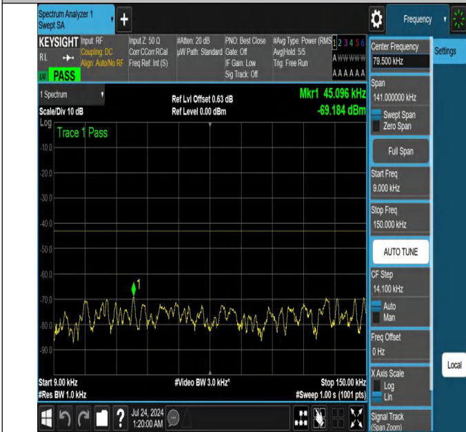
NTNV-N25-PC3-15-40-L-DFT-PI2BPSK-Edge_1RB_Right-0.009-150-Ant1-PASS
