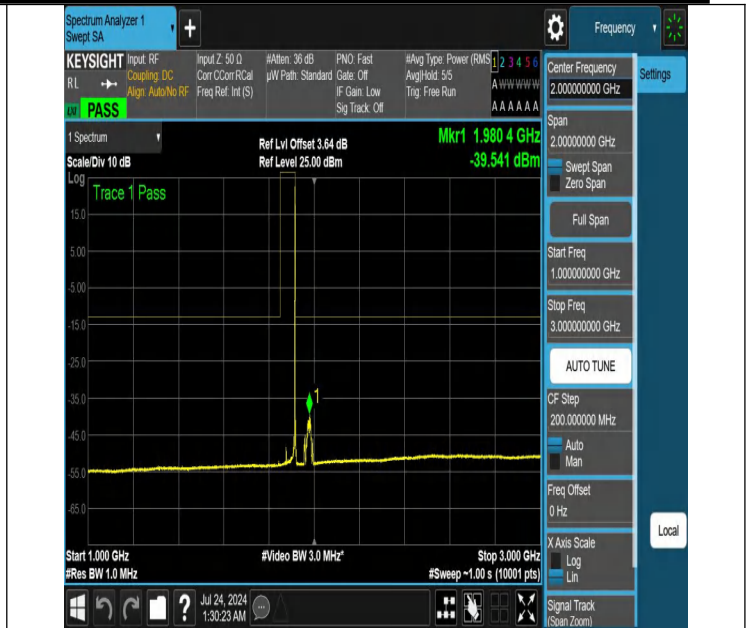
NTNV-N25-PC3-15-40-H-DFT-PI2BPSK-Edge_1RB_Right-1000-3000-Ant1-PASS
