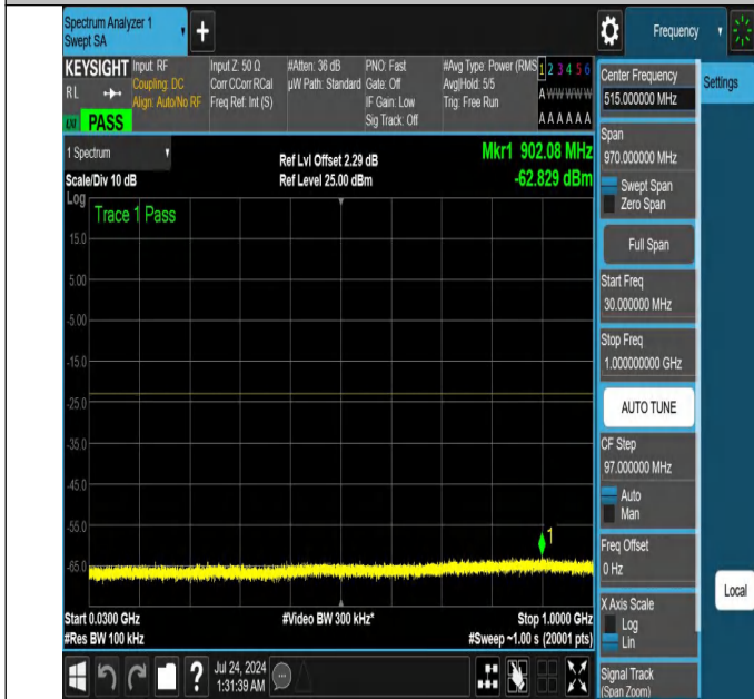
NTNV-N25-PC3-15-40-H-DFT-QPSK-Edge_1RB_Left-30-1000-A nt1-PASS
