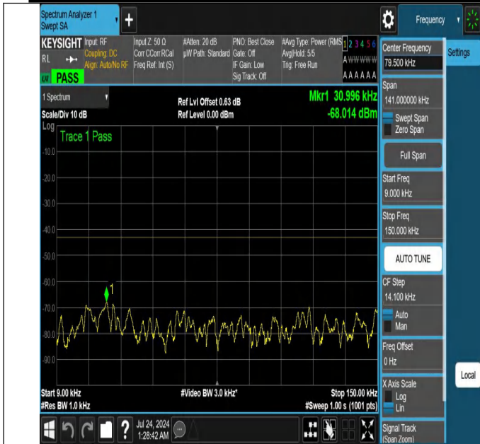
NTNV-N25-PC3-15-40-H-DFT-PI2BPSK-Edge_1RB_Left-0.009-0.15-Ant1-PASS
