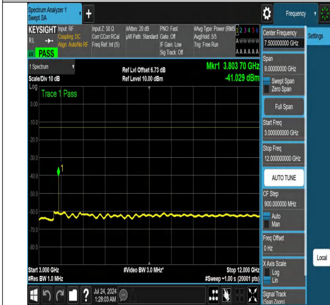
NTNV-N25-PC3-15-40-M-DFT-QPSK-Edge_1RB_Right-3000-12000-Ant1-PASS
