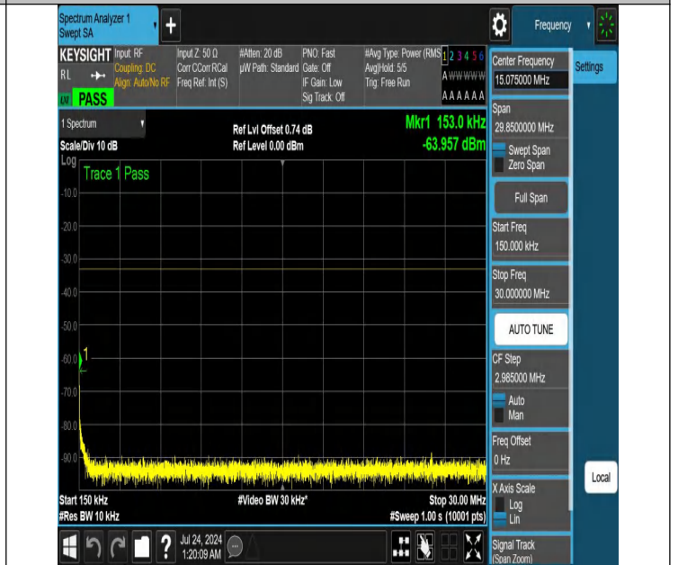
NTNV-N25-PC3-15-40-L-DFT-PI2BPSK-Edge_1RB_Right-0.15-30-Ant1-PASS
