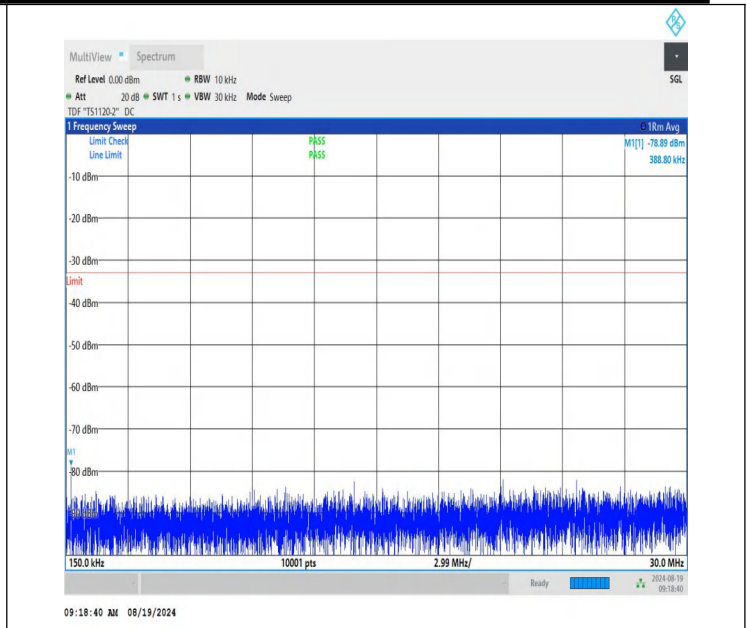
NTNV-n25-PC3-15-35-L-DFT-BPSK-Edge_1RB_Left-0.15-30-PASS
