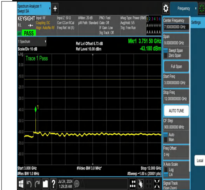
NTNV-N25-PC3-15-40-H-DFT-PI2BPSK-Edge_1RB_Left-3000-1 2000-Ant1-PASS
