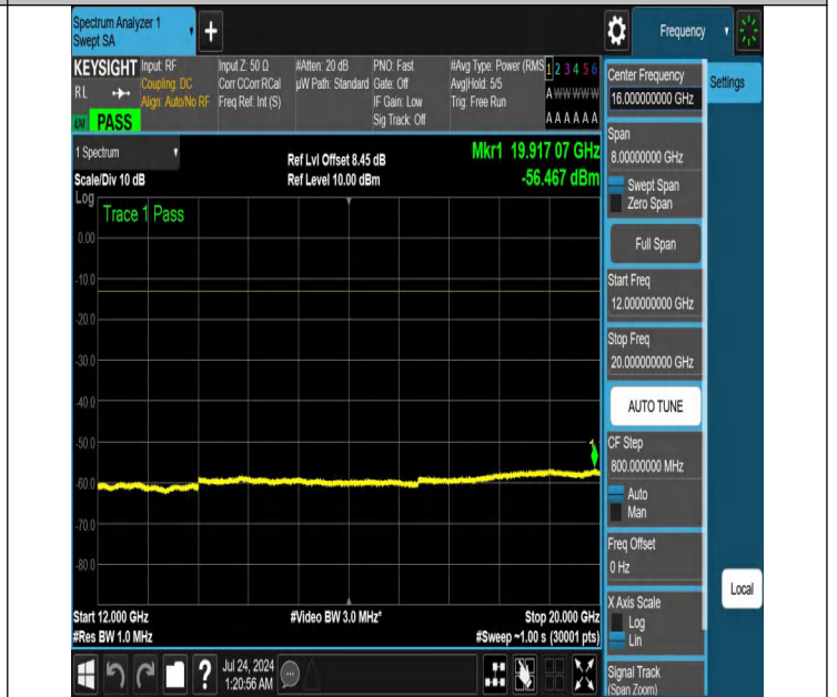
NTNV-N25-PC3-15-40-L-DFT-PI2BPSK-Edge_1RB_Right-12000-20000-Ant1-PASS
