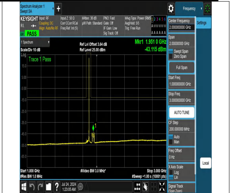
NTNV-N25-PC3-15-40-L-DFT-QPSK-Edge_1RB_Right-1000-3000-Ant1-PASS
