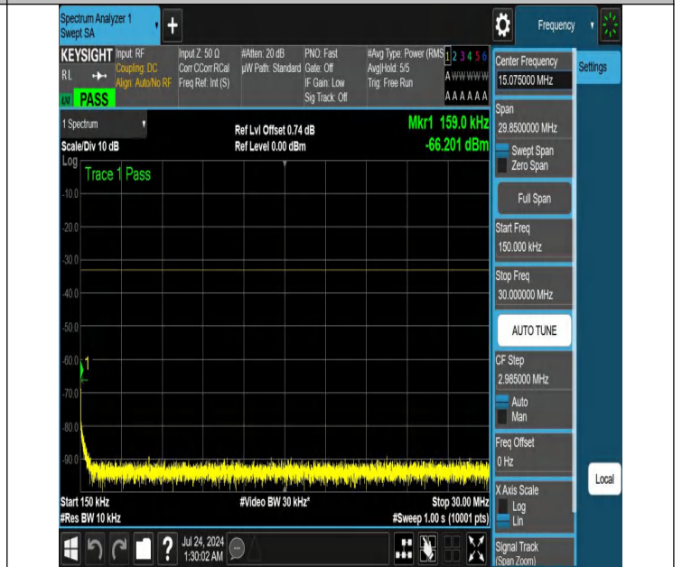
NTNV-N25-PC3-15-40-H-DFT-PI2BPSK-Edge_1RB_Right-0.15-3 0-Ant1-PASS
