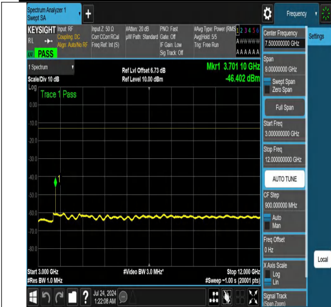
NTNV-N25-PC3-15-40-L-DFT-QPSK-Edge_1RB_Left-3000-1200 0-Ant1-PASS
