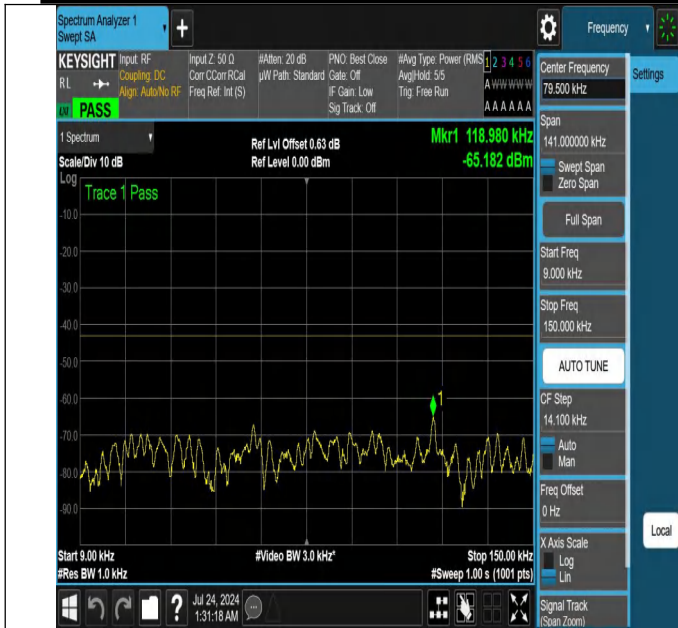
NTNV-N25-PC3-15-40-H-DFT-QPSK-Edge_1RB_Left-0.009-0.15 -Ant1-PASS
