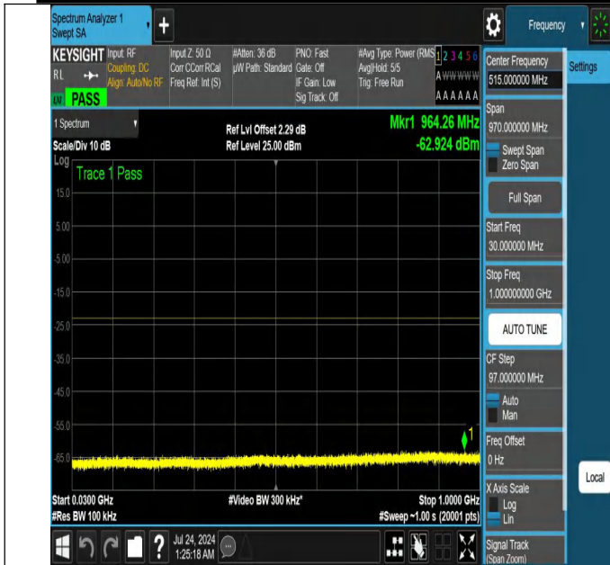
NTNV-N25-PC3-15-40-M-DFT-PI2BPSK-Edge_1RB_Right-30-1000-Ant1-PASS
