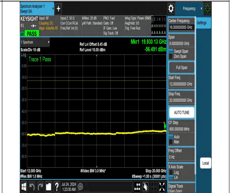
NTNV-N25-PC3-15-40-L-DFT-QPSK-Edge_1RB_Right-12000-20000-Ant1-PASS
