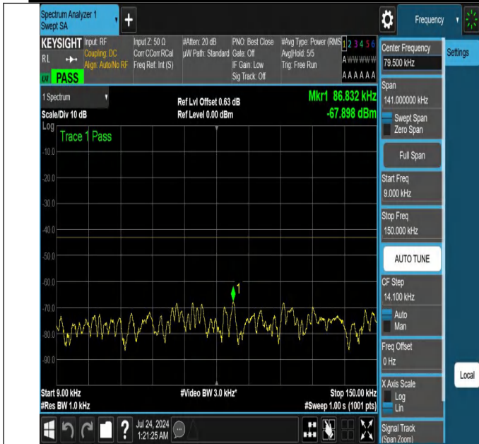
NTNV-N25-PC3-15-40-L-DFT-QPSK-Edge_1RB_Left-0.009-0.15-Ant1-PASS
