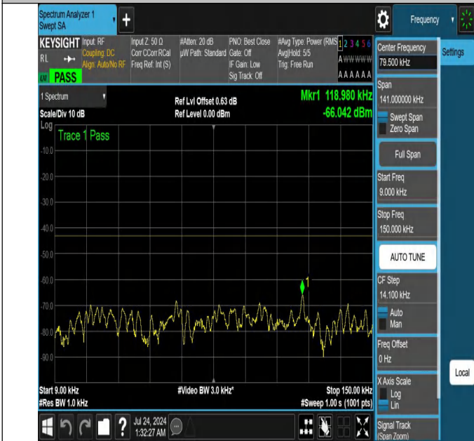
NTNV-N25-PC3-15-40-H-DFT-QPSK-Edge_1RB_Right-0.009-0.1 5-Ant1-PASS
