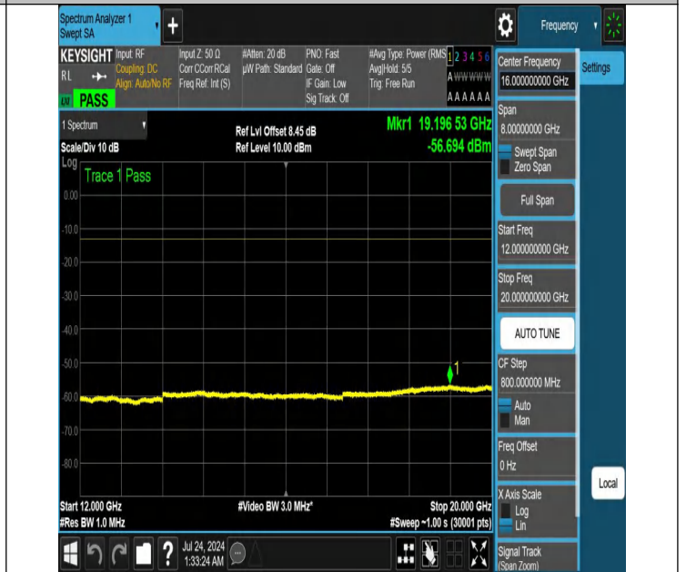
NTNV-N25-PC3-15-40-H-DFT-QPSK-Edge_1RB_Right-12000-20000-Ant1-PASS
