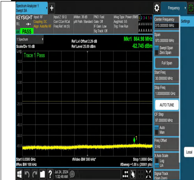
NTNV-N25-PC3-15-40-H-DFT-QPSK-Edge_1RB_Right-30-1000-Ant1-PASS
