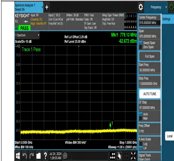
NTNV-N25-PC3-15-40-H-DFT-PI2BPSK-Edge_1RB_Left-30-1000-Ant1-PASS
