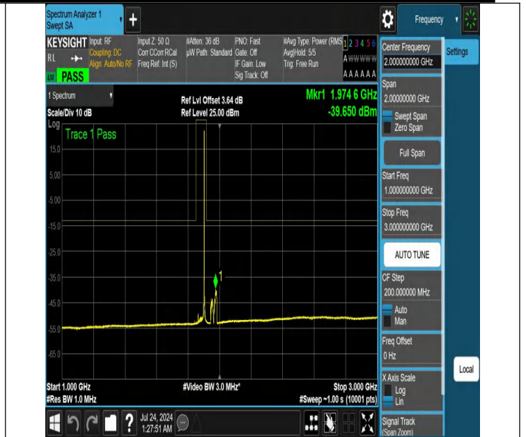
NTNV-N25-PC3-15-40-M-DFT-QPSK-Edge_1RB_Right-1000-300-0-Ant1-PASS
