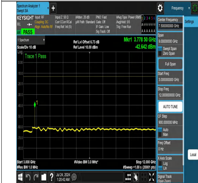
NTNV-N25-PC3-15-40-L-DFT-PI2BPSK-Edge_1RB_Right-3000-12000-Ant1-PASS
