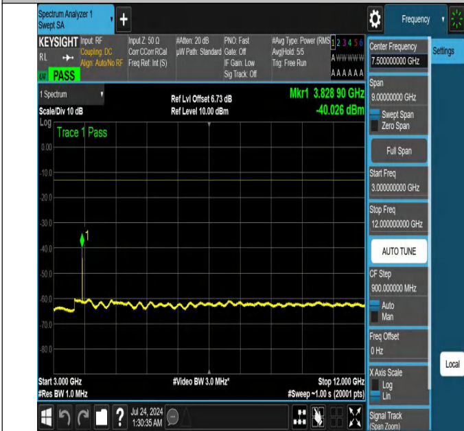
NTNV-N25-PC3-15-40-H-DFT-PI2BPSK-Edge_1RB_Right-3000-12000-Ant1-PASS
