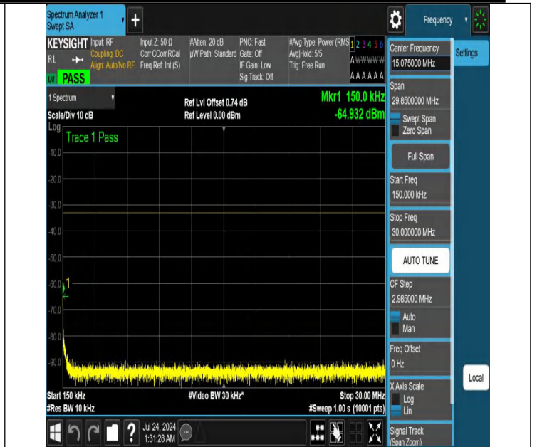
NTNV-N25-PC3-15-40-H-DFT-QPSK-Edge_1RB_Left-0.15-30-Ant 1-PASS
