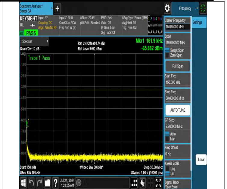
NTNV-N25-PC3-15-40-L-DFT-QPSK-Edge_1RB_Left-0.15-30-Ant 1-PASS
