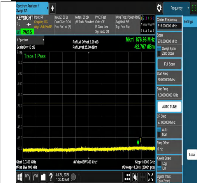
NTNV-N25-PC3-15-40-H-DFT-PI2BPSK-Edge_1RB_Right-30-1000-Ant1-PASS
