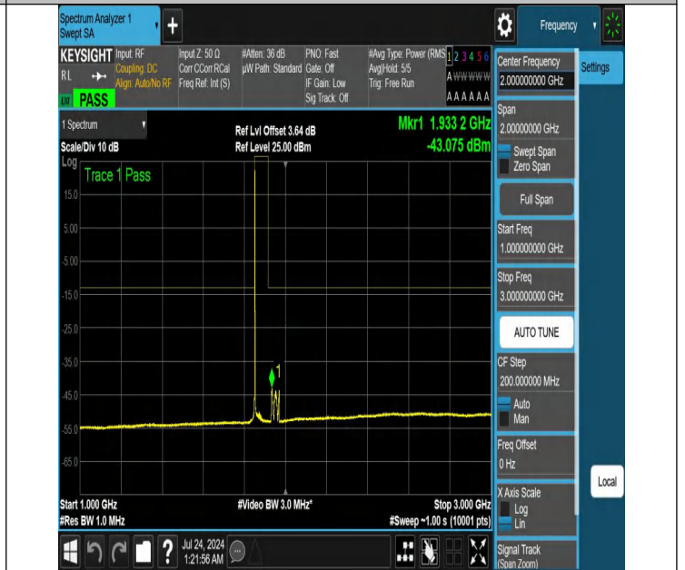
NTNV-N25-PC3-15-40-L-DFT-QPSK-Edge_1RB_Left-1000-3000-Ant1-PASS
