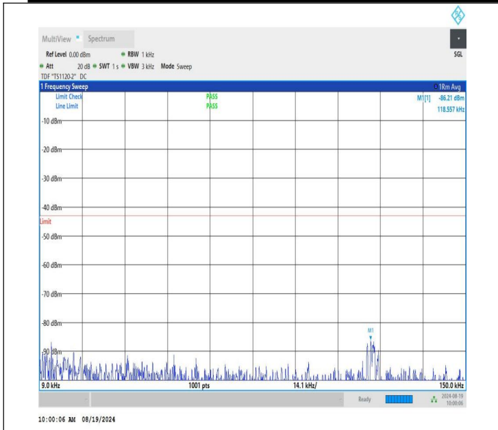
NTNV-n25-PC3-15-35-L-DFT-BPSK-Edge_1RB_Left-0.009-0.15-PASS
