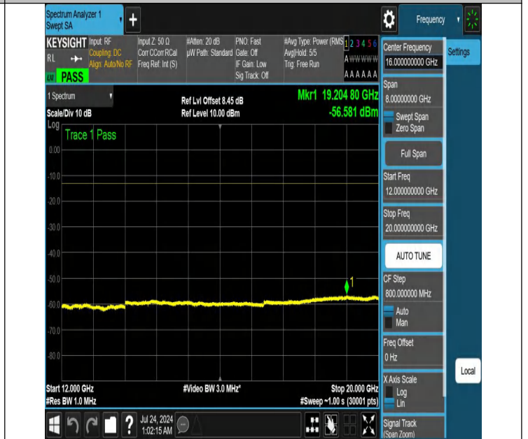
NTNV-N25-PC3-15-25-H-DFT-QPSK-Edge_1RB_Right-12000-20000-Ant1-PASS
