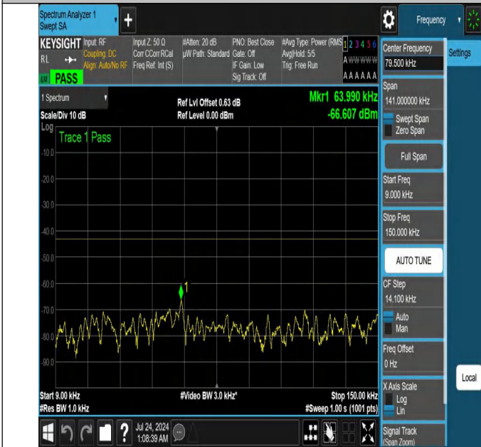
NTNV-N25-PC3-15-30-M-DFT-PI2BPSK-Edge_1RB_Right-0.009 -0.15-Ant1-PASS
