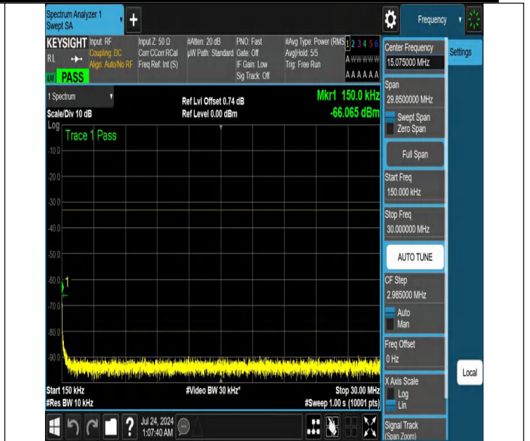
NTNV-N25-PC3-15-30-M-DFT-PI2BPSK-Edge_1RB_Left-0.15-30-Ant1-PASS
