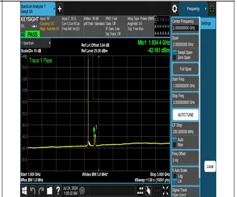
NTNV-N25-PC3-15-30-L-DFT-QPSK-Edge_1RB_Left-1000-3000-Ant1-PASS
