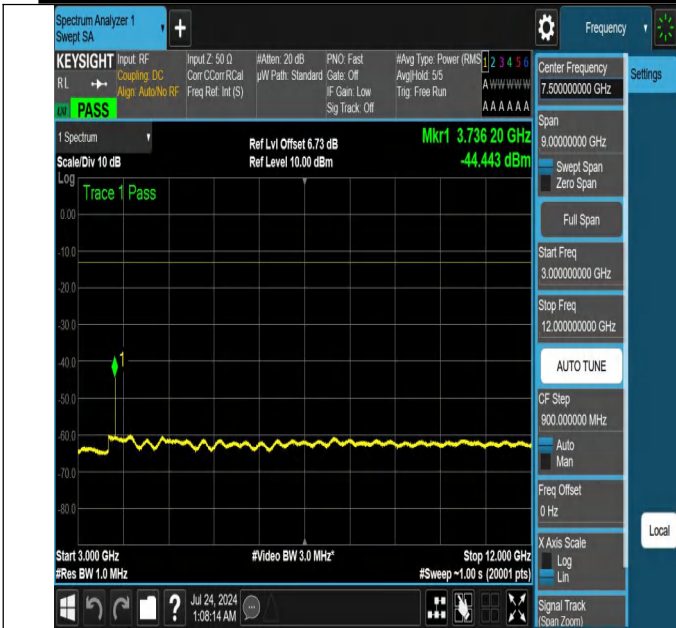
NTNV-N25-PC3-15-30-M-DFT-PI2BPSK-Edge_1RB_Left-3000-1 2000-Ant1-PASS
