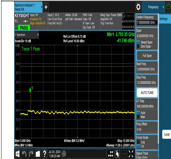
NTNV-N25-PC3-15-30-M-DFT-PI2BPSK-Edge_1RB_Right-3000-12000-Ant1-PASS
