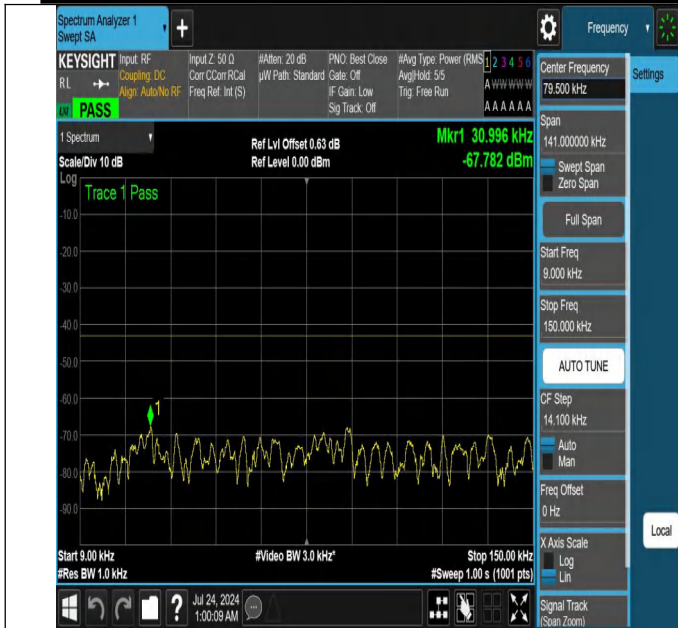
NTNV-N25-PC3-15-25-H-DFT-QPSK-Edge_1RB_Left-0.009-0.15 -Ant1-PASS
