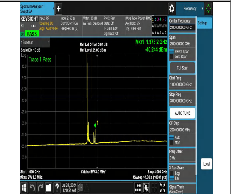
NTNV-N25-PC3-15-30-M-DFT-QPSK-Edge_1RB_Left-1000-3000-Ant1-PASS
