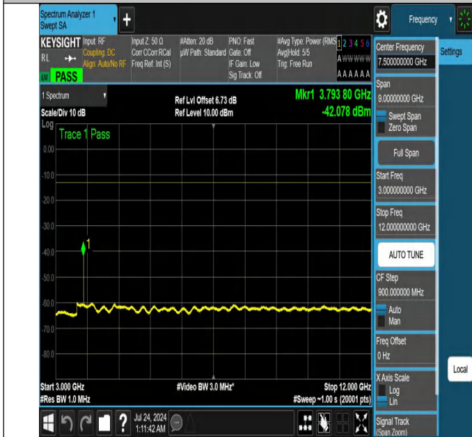
NTNV-N25-PC3-15-30-M-DFT-QPSK-Edge_1RB_Right-3000-12000-Ant1-PASS
