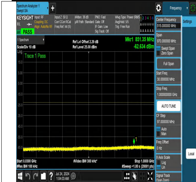
NTNV-N25-PC3-15-30-L-DFT-PI2BPSK-Edge_1RB_Right-30-1000-Ant1-PASS
