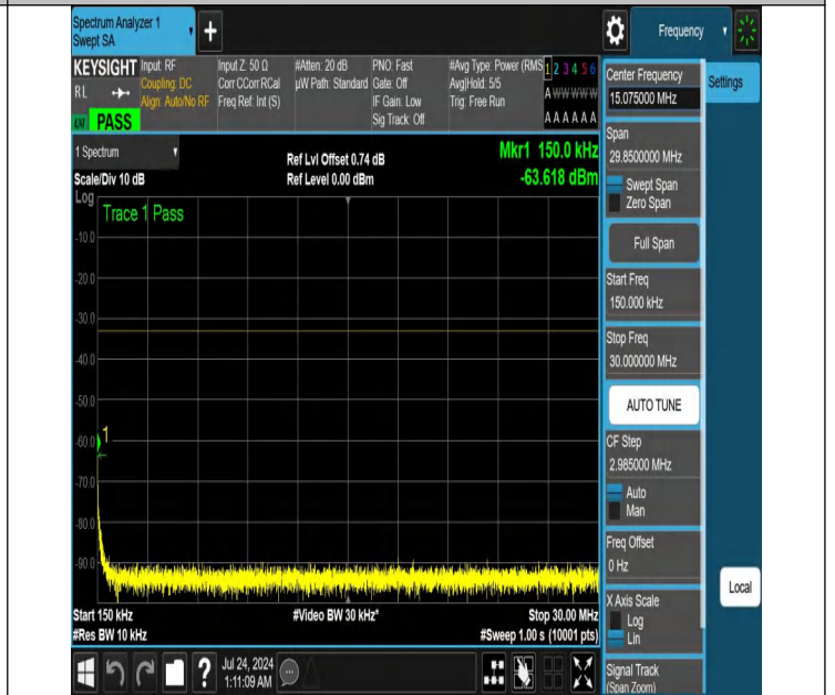
NTNV-N25-PC3-15-30-M-DFT-QPSK-Edge_1RB_Right-0.15-30-A nt1-PASS
