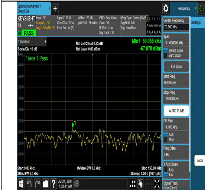
NTNV-N25-PC3-15-30-L-DFT-PI2BPSK-Edge_1RB_Right-0.009-150-Ant1-PASS
