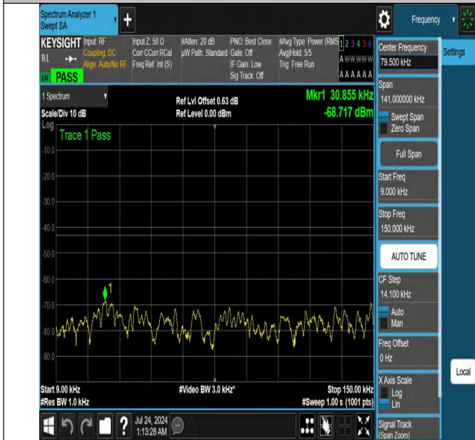
NTNV-N25-PC3-15-30-H-DFT-PI2BPSK-Edge_1RB_Right-0.009- 0.15-Ant1-PASS
