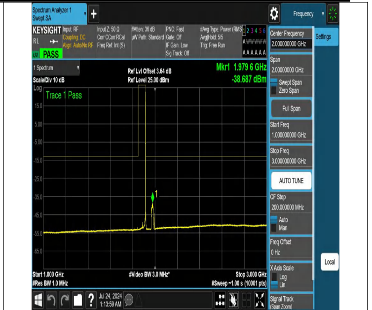
NTNV-N25-PC3-15-30-H-DFT-PI2BPSK-Edge_1RB_Right-1000-3000-Ant1-PASS
