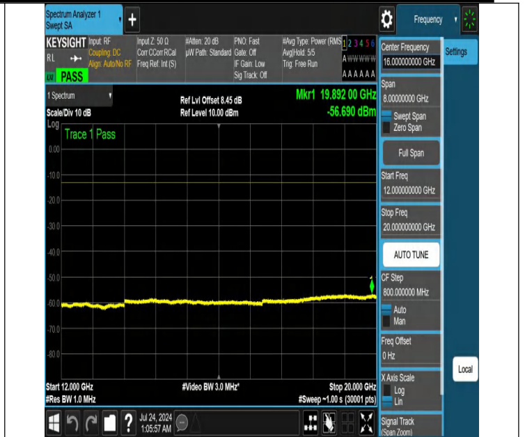
NTNV-N25-PC3-15-30-L-DFT-QPSK-Edge_1RB_Left-12000-2000 0-Ant1-PASS
