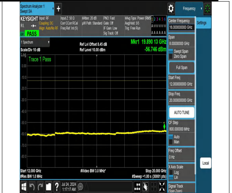
NTNV-N25-PC3-15-30-H-DFT-QPSK-Edge_1RB_Left-12000-2000 0-Ant1-PASS
