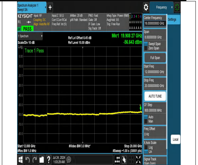
NTNV-N25-PC3-15-30-L-DFT-PI2BPSK-Edge_1RB_Left-12000-20000-Ant1-PASS
