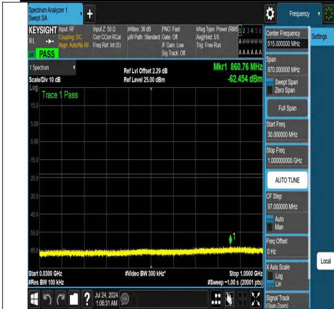
NTNV-N25-PC3-15-30-L-DFT-QPSK-Edge_1RB_Right-30-1000-Ant1-PASS
