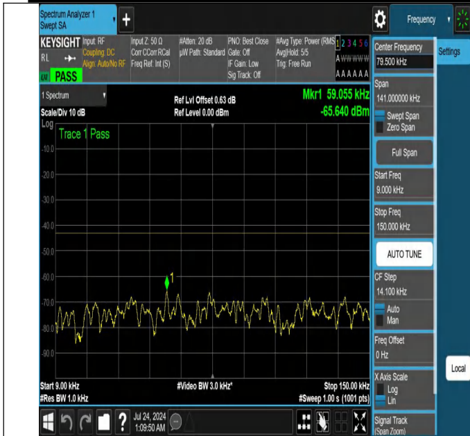
NTNV-N25-PC3-15-30-M-DFT-QPSK-Edge_1RB_Left-0.009-0.15 -Ant1-PASS
