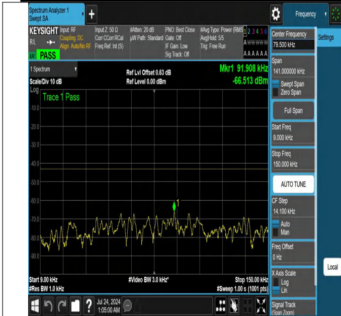
NTNV-N25-PC3-15-30-L-DFT-QPSK-Edge_1RB_Left-0.009-0.15-Ant1-PASS
