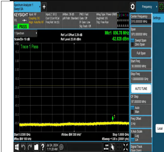
NTNV-N25-PC3-15-30-M-DFT-QPSK-Edge_1RB_Right-30-1000-Ant1-PASS
