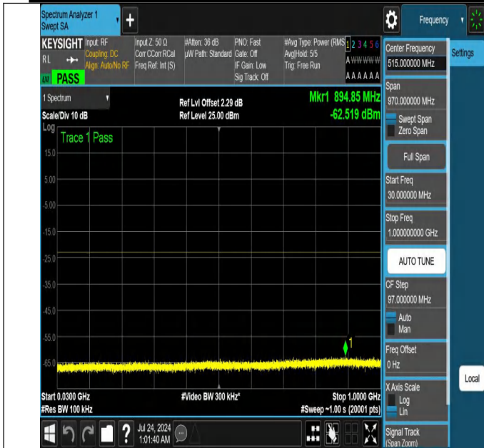
NTNV-N25-PC3-15-25-H-DFT-QPSK-Edge_1RB_Right-30-1000-Ant1-PASS
