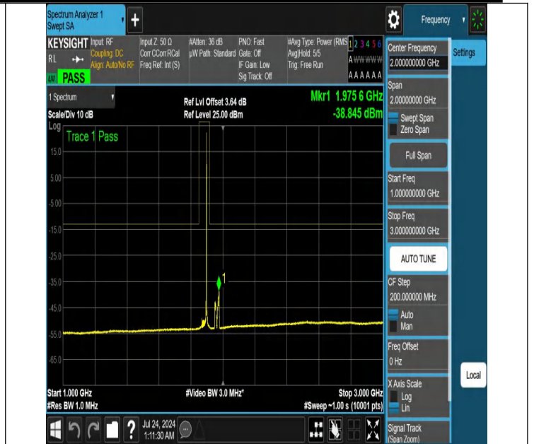
NTNV-N25-PC3-15-30-M-DFT-QPSK-Edge_1RB_Right-1000-300-0-Ant1-PASS
