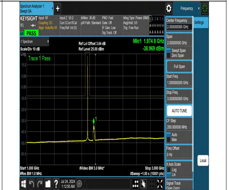
NTNV-N25-PC3-15-30-H-DFT-PI2BPSK-Edge_1RB_Left-1000-3000-Ant1-PASS
