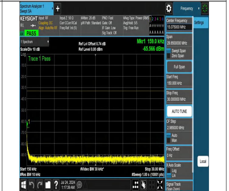
NTNV-N25-PC3-15-30-H-DFT-QPSK-Edge_1RB_Right-0.15-30-A nt1-PASS
