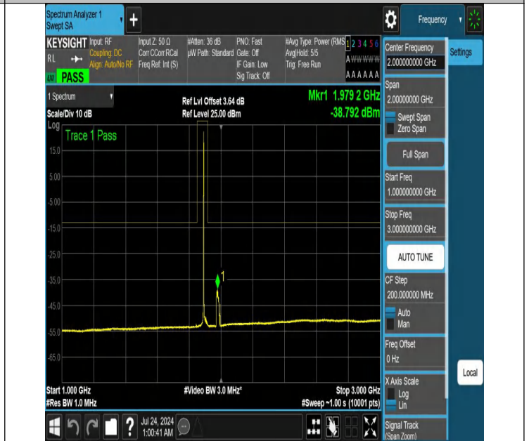
NTNV-N25-PC3-15-25-H-DFT-QPSK-Edge_1RB_Left-1000-3000- Ant1-PASS
