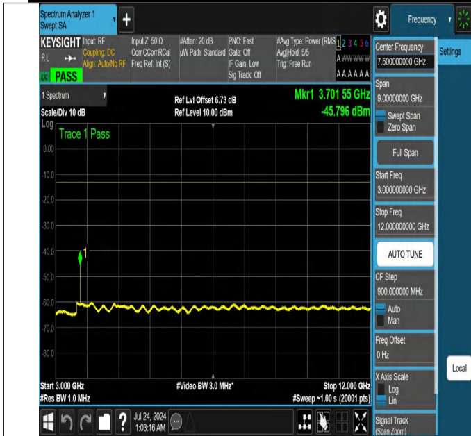
NTNV-N25-PC3-15-30-L-DFT-PI2BPSK-Edge_1RB_Left-3000-12000-Ant1-PASS
