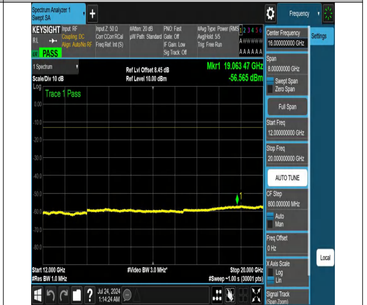
NTNV-N25-PC3-15-30-H-DFT-PI2BPSK-Edge_1RB_Right-12000-20000-Ant1-PASS
