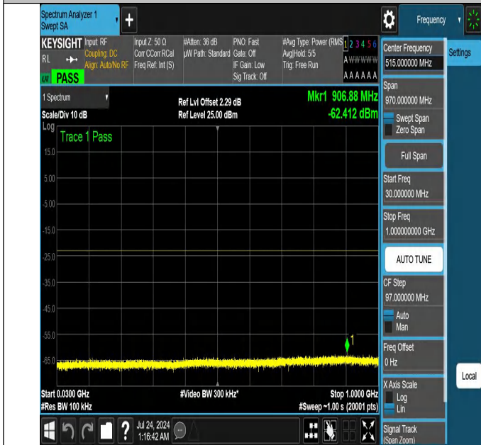
NTNV-N25-PC3-15-30-H-DFT-QPSK-Edge_1RB_Left-30-1000-A nt1-PASS
