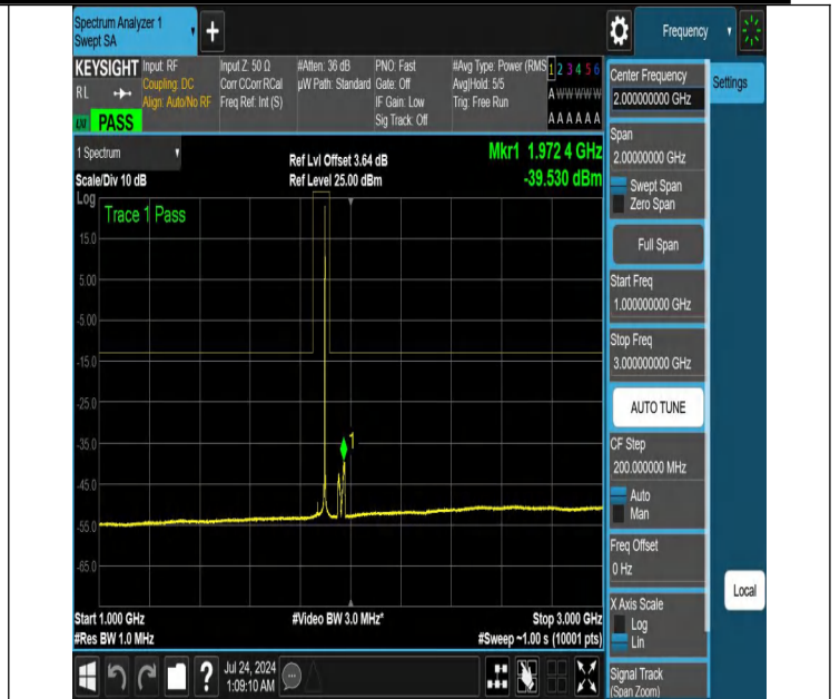
NTNV-N25-PC3-15-30-M-DFT-PI2BPSK-Edge_1RB_Right-1000-3000-Ant1-PASS
