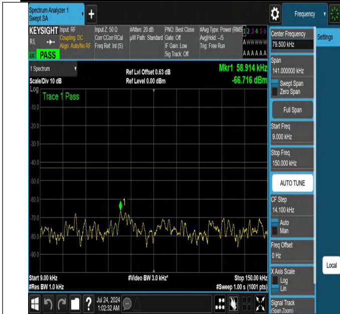
NTNV-N25-PC3-15-30-L-DFT-PI2BPSK-Edge_1RB_Left-0.009-0.15-Ant1-PASS
