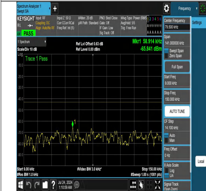
NTNV-N25-PC3-15-30-M-DFT-QPSK-Edge_1RB_Right-0.009-0. 15-Ant1-PASS
