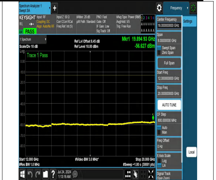
NTNV-N25-PC3-15-30-H-DFT-PI2BPSK-Edge_1RB_Left-12000-2 0000-Ant1-PASS
