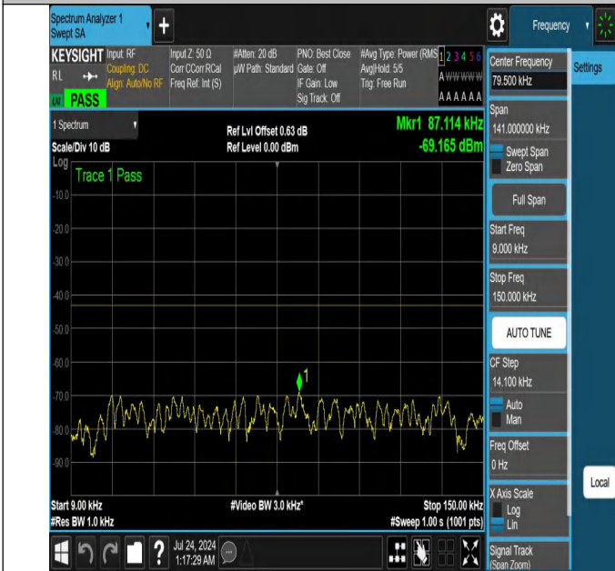
NTNV-N25-PC3-15-30-H-DFT-QPSK-Edge_1RB_Right-0.009-0.1 5-Ant1-PASS
