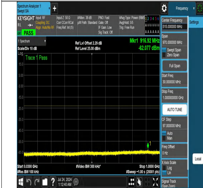
NTNV-N25-PC3-15-30-H-DFT-PI2BPSK-Edge_1RB_Left-30-1000-Ant1-PASS
