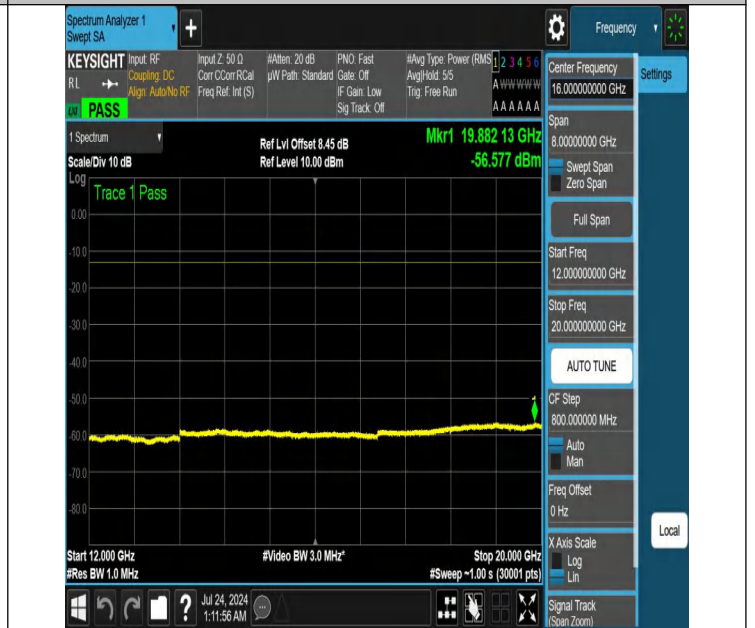
NTNV-N25-PC3-15-30-M-DFT-QPSK-Edge_1RB_Right-12000-20000-Ant1-PASS
