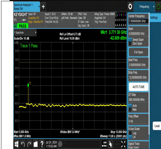
NTNV-N25-PC3-15-30-H-DFT-PI2BPSK-Edge_1RB_Left-3000-1 2000-Ant1-PASS
