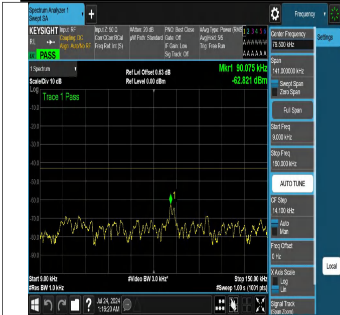
NTNV-N25-PC3-15-30-H-DFT-QPSK-Edge_1RB_Left-0.009-0.15 -Ant1-PASS
