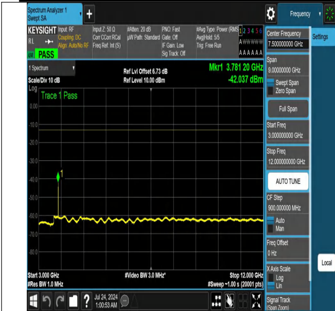
NTNV-N25-PC3-15-25-H-DFT-QPSK-Edge_1RB_Left-3000-1200 0-Ant1-PASS
