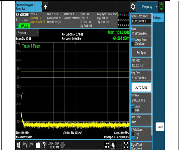
NTNV-N25-PC3-15-30-L-DFT-PI2BPSK-Edge_1RB_Left-0.15-30-Ant1-PASS
