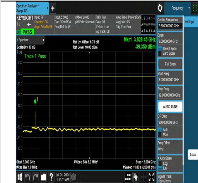
NTNV-N25-PC3-15-30-H-DFT-PI2BPSK-Edge_1RB_Right-3000-12000-Ant1-PASS
