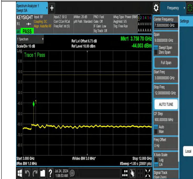
NTNV-N25-PC3-15-30-L-DFT-QPSK-Edge_1RB_Right-3000-12000-Ant1-PASS
