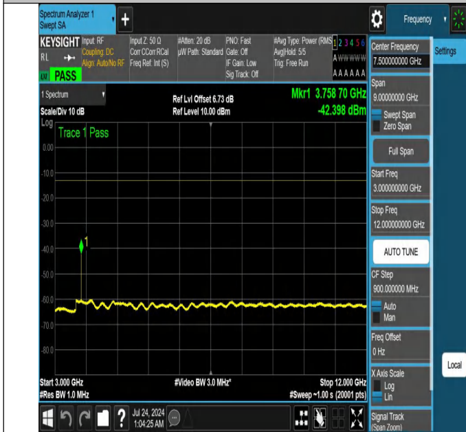
NTNV-N25-PC3-15-30-L-DFT-PI2BPSK-Edge_1RB_Right-3000-12000-Ant1-PASS
