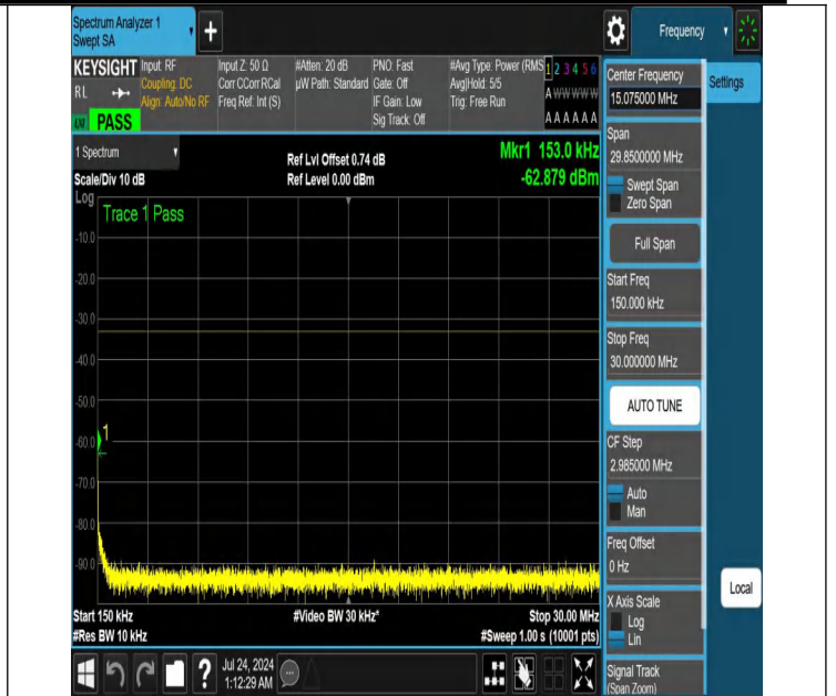
NTNV-N25-PC3-15-30-H-DFT-PI2BPSK-Edge_1RB_Left-0.15-30-Ant1-PASS
