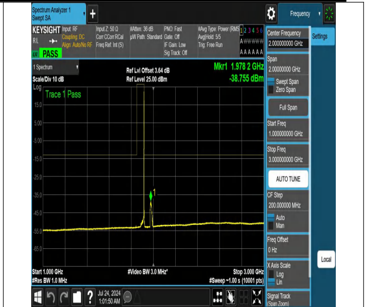
NTNV-N25-PC3-15-25-H-DFT-QPSK-Edge_1RB_Right-1000-300-0-Ant1-PASS
