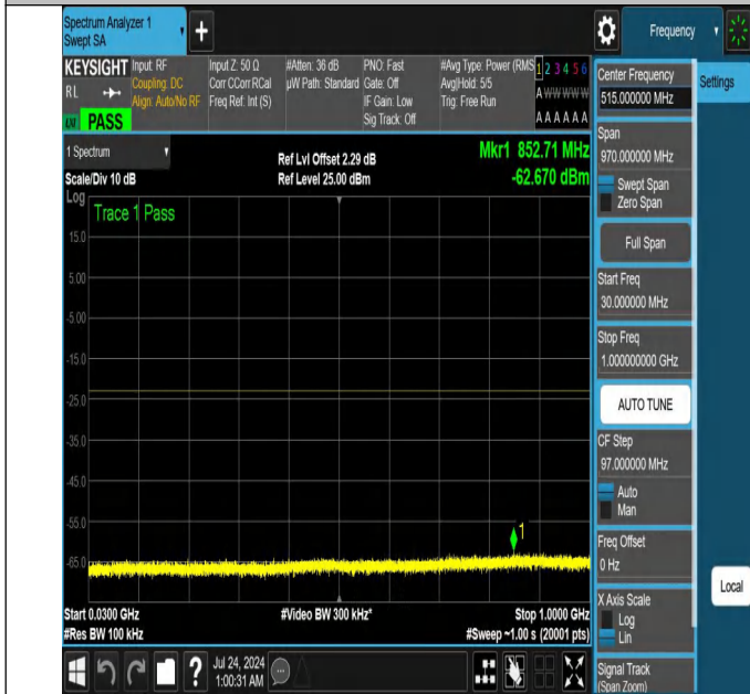
NTNV-N25-PC3-15-25-H-DFT-QPSK-Edge_1RB_Left-30-1000-A nt1-PASS
