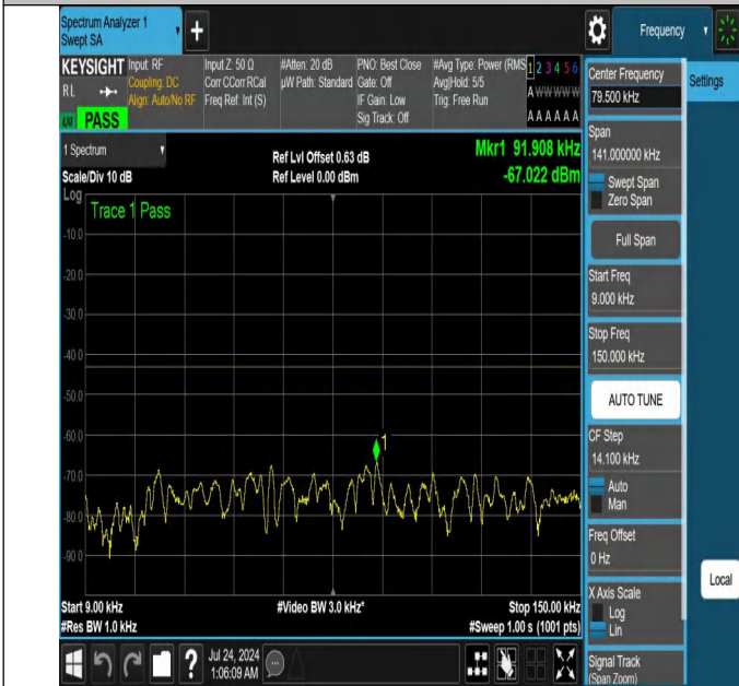
NTNV-N25-PC3-15-30-L-DFT-QPSK-Edge_1RB_Right-0.009-0.1 5-Ant1-PASS
