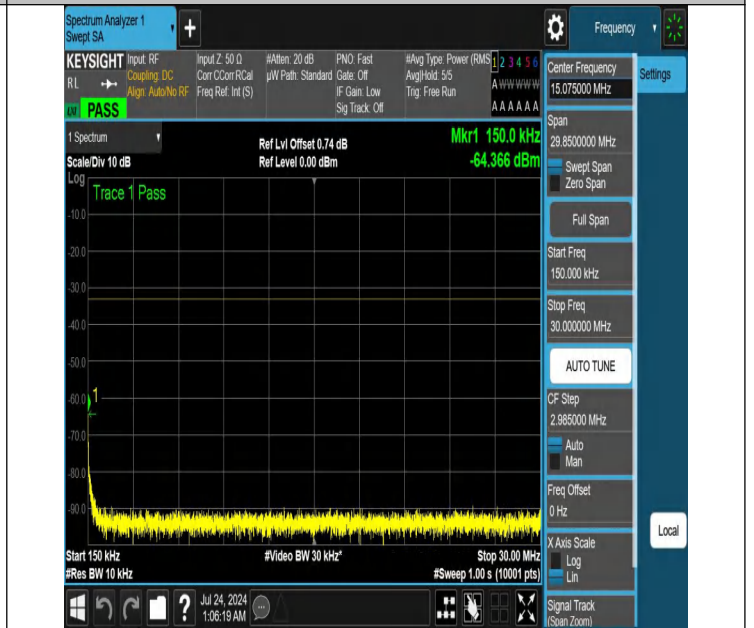
NTNV-N25-PC3-15-30-L-DFT-QPSK-Edge_1RB_Right-0.15-30-A nt1-PASS
