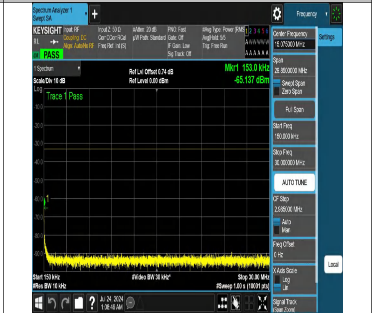
NTNV-N25-PC3-15-30-M-DFT-PI2BPSK-Edge_1RB_Right-0.15-3 0-Ant1-PASS
