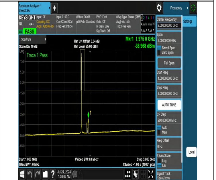
NTNV-N25-PC3-15-30-M-DFT-PI2BPSK-Edge_1RB_Left-1000-3000-Ant1-PASS
