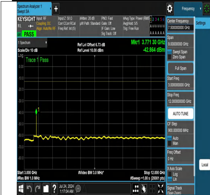
NTNV-N25-PC3-15-30-H-DFT-QPSK-Edge_1RB_Left-3000-1200 0-Ant1-PASS
