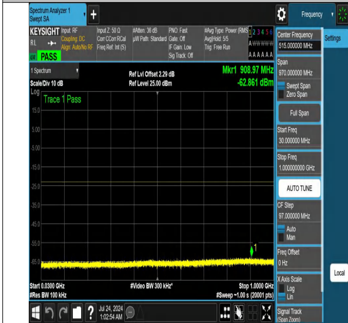
NTNV-N25-PC3-15-30-L-DFT-PI2BPSK-Edge_1RB_Left-30-1000-Ant1-PASS
