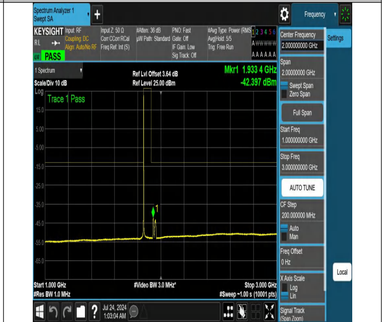
NTNV-N25-PC3-15-30-L-DFT-PI2BPSK-Edge_1RB_Left-1000-3000-Ant1-PASS
