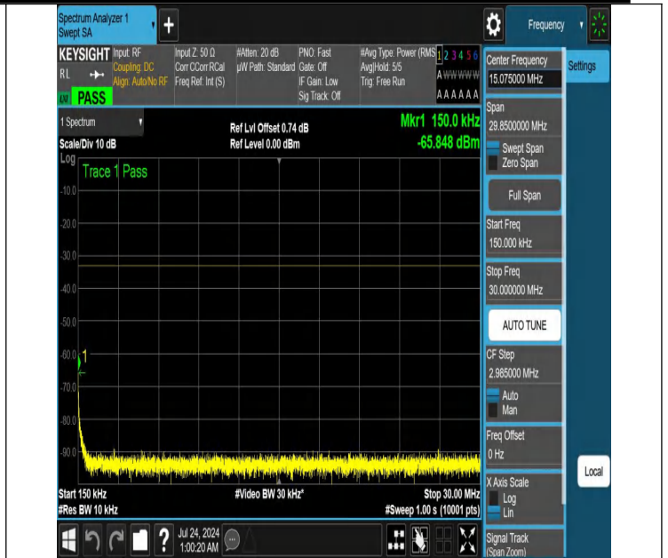
NTNV-N25-PC3-15-25-H-DFT-QPSK-Edge_1RB_Left-0.15-30-Ant 1-PASS
