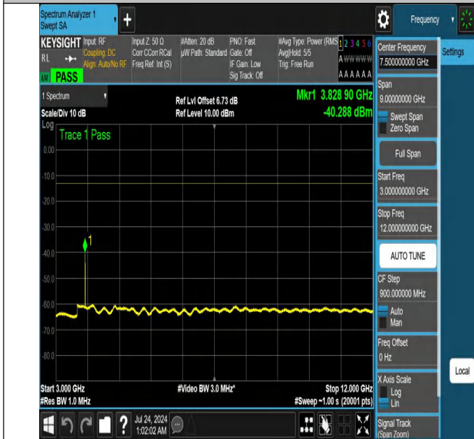
NTNV-N25-PC3-15-25-H-DFT-QPSK-Edge_1RB_Right-3000-12000-Ant1-PASS
