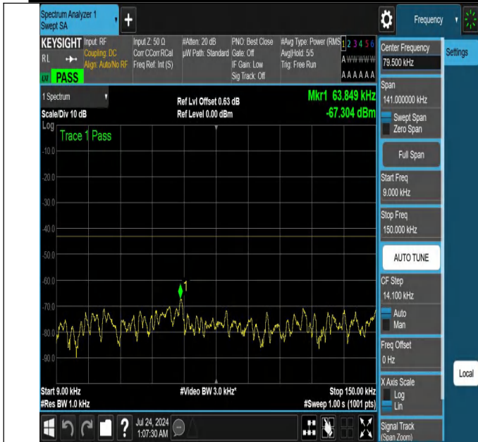
NTNV-N25-PC3-15-30-M-DFT-PI2BPSK-Edge_1RB_Left-0.009-0.15-Ant1-PASS
