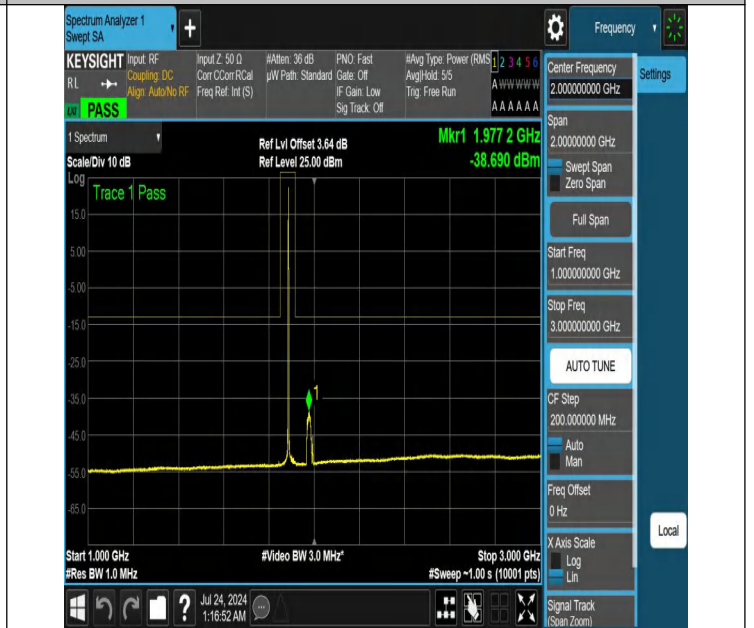
NTNV-N25-PC3-15-30-H-DFT-QPSK-Edge_1RB_Left-1000-3000-Ant1-PASS
