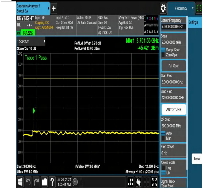
NTNV-N25-PC3-15-30-L-DFT-QPSK-Edge_1RB_Left-3000-1200 0-Ant1-PASS
