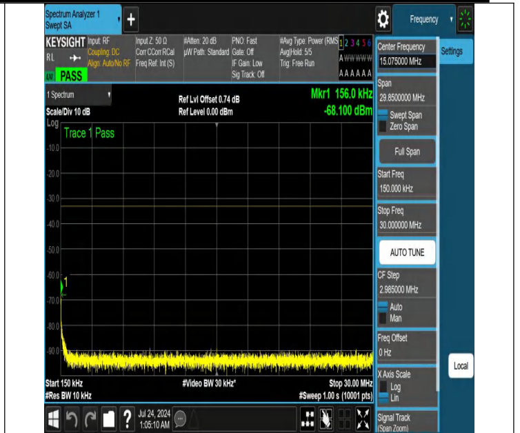
NTNV-N25-PC3-15-30-L-DFT-QPSK-Edge_1RB_Left-0.15-30-Ant 1-PASS
