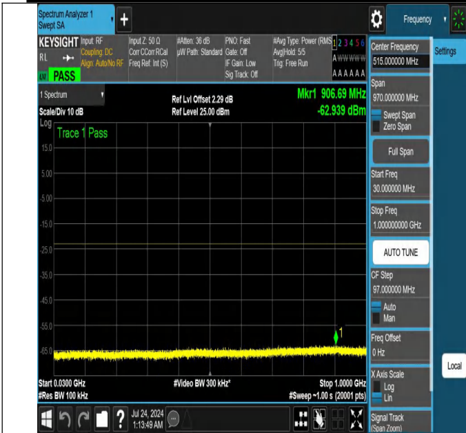
NTNV-N25-PC3-15-30-H-DFT-PI2BPSK-Edge_1RB_Right-30-1000-Ant1-PASS
