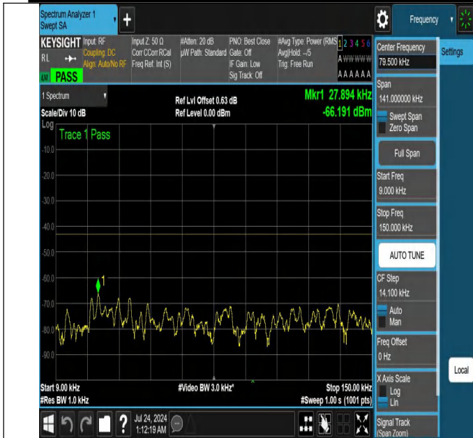
NTNV-N25-PC3-15-30-H-DFT-PI2BPSK-Edge_1RB_Left-0.009-0.15-Ant1-PASS
