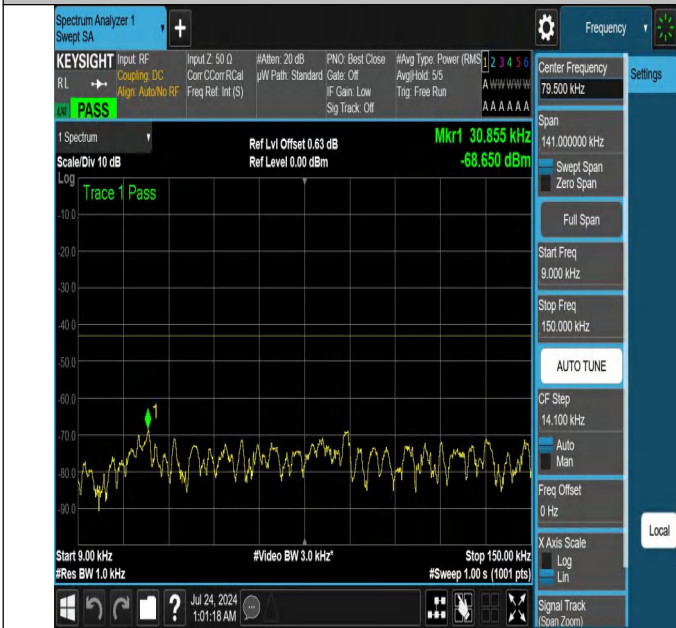
NTNV-N25-PC3-15-25-H-DFT-QPSK-Edge_1RB_Right-0.009-0.1 5-Ant1-PASS
