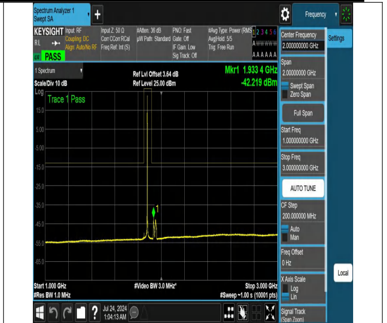
NTNV-N25-PC3-15-30-L-DFT-PI2BPSK-Edge_1RB_Right-1000-3000-Ant1-PASS
