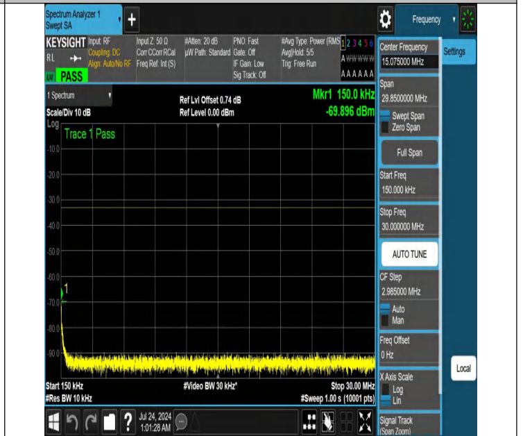
NTNV-N25-PC3-15-25-H-DFT-QPSK-Edge_1RB_Right-0.15-30-A nt1-PASS
