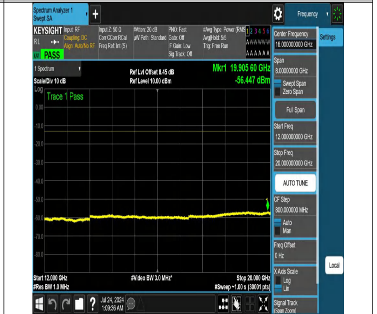
NTNV-N25-PC3-15-30-M-DFT-PI2BPSK-Edge_1RB_Right-12000-20000-Ant1-PASS
