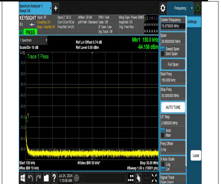
NTNV-N25-PC3-15-30-M-DFT-QPSK-Edge_1RB_Left-0.15-30-Ant 1-PASS
