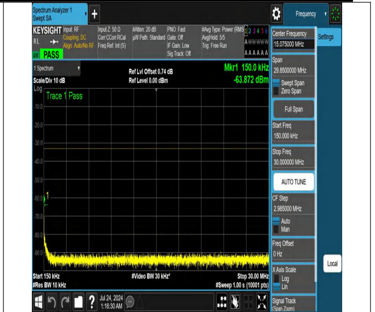
NTNV-N25-PC3-15-30-H-DFT-QPSK-Edge_1RB_Left-0.15-30-Ant 1-PASS
