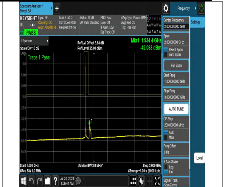
NTNV-N25-PC3-15-30-L-DFT-QPSK-Edge_1RB_Right-1000-3000-Ant1-PASS
