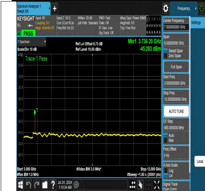
NTNV-N25-PC3-15-30-M-DFT-QPSK-Edge_1RB_Left-3000-1200 0-Ant1-PASS
