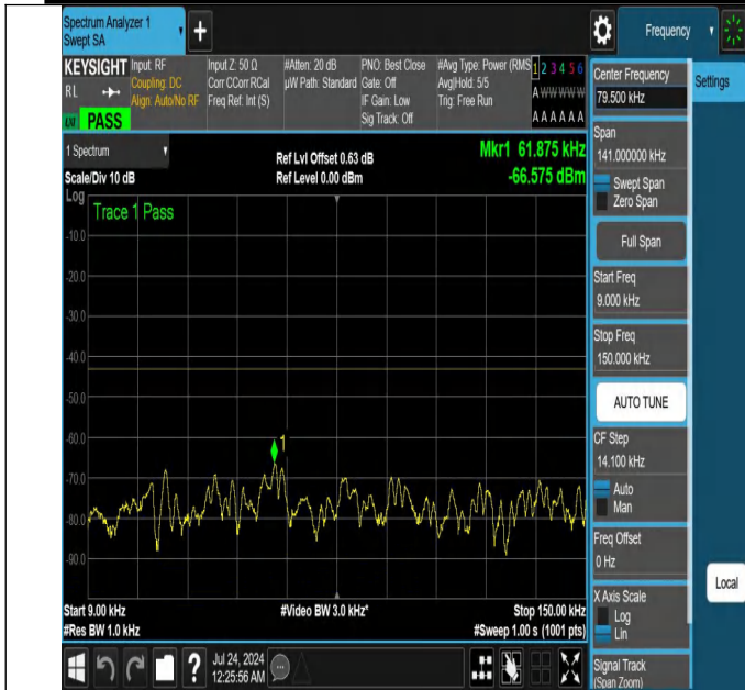
NTNV-N25-PC3-15-15-H-DFT-PI2BPSK-Edge_1RB_Left-0.009-0.15-Ant1-PASS
