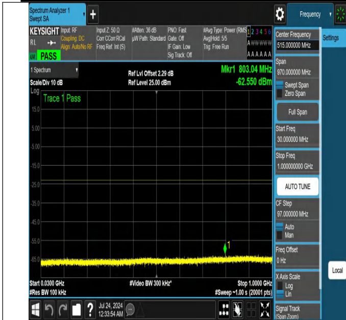
NTNV-N25-PC3-15-20-L-DFT-PI2BPSK-Edge_1RB_Right-30-1000-Ant1-PASS
