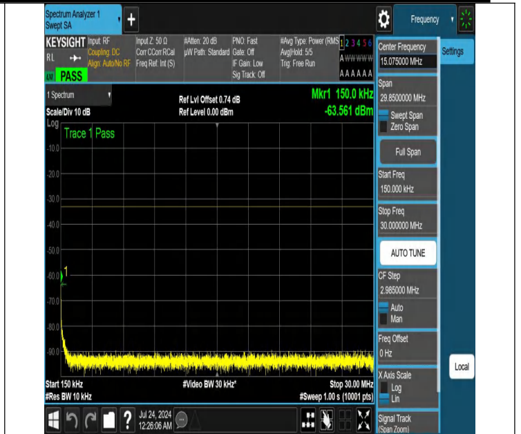
NTNV-N25-PC3-15-15-H-DFT-PI2BPSK-Edge_1RB_Left-0.15-30-Ant1-PASS
