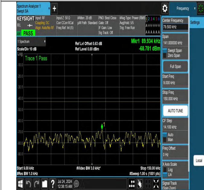
NTNV-N25-PC3-15-20-M-DFT-PI2BPSK-Edge_1RB_Right-0.009 -0.15-Ant1-PASS
