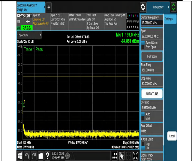
NTNV-N25-PC3-15-20-L-DFT-QPSK-Edge_1RB_Left-0.15-30-Ant 1-PASS
