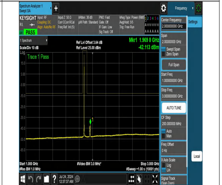
NTNV-N25-PC3-15-20-M-DFT-PI2BPSK-Edge_1RB_Left-1000-3000-Ant1-PASS
