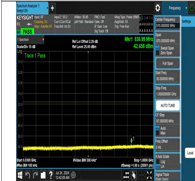
NTNV-N25-PC3-15-20-H-DFT-PI2BPSK-Edge_1RB_Left-30-1000-Ant1-PASS
