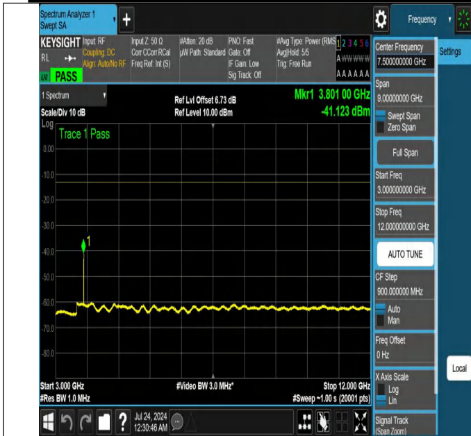
NTNV-N25-PC3-15-15-H-DFT-QPSK-Edge_1RB_Left-3000-1200 0-Ant1-PASS
