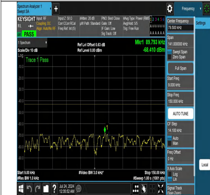
NTNV-N25-PC3-15-20-L-DFT-QPSK-Edge_1RB_Right-0.009-0.1 5-Ant1-PASS
