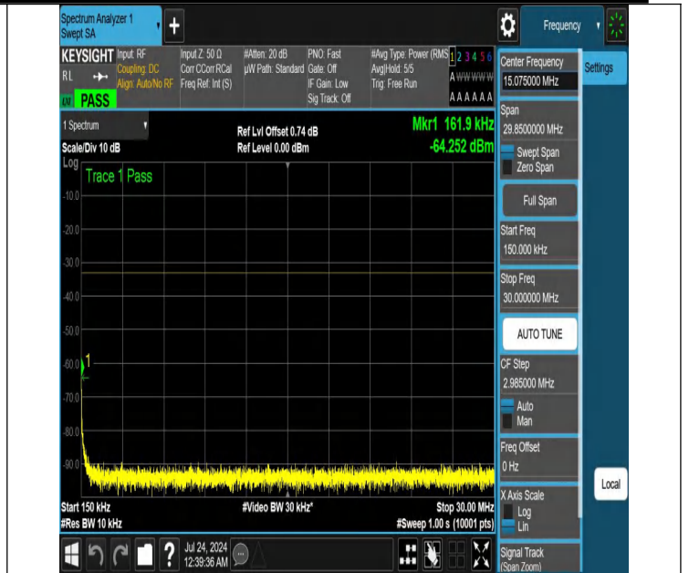
NTNV-N25-PC3-15-20-M-DFT-QPSK-Edge_1RB_Left-0.15-30-Ant 1-PASS
