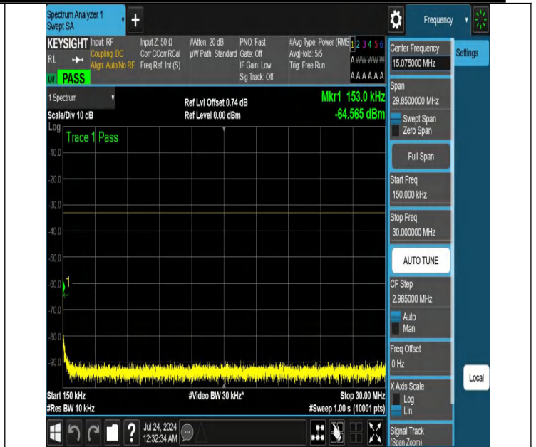
NTNV-N25-PC3-15-20-L-DFT-PI2BPSK-Edge_1RB_Left-0.15-30-Ant1-PASS
