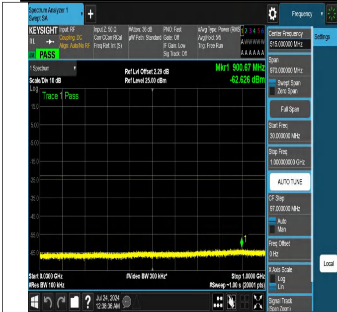
NTNV-N25-PC3-15-20-M-DFT-PI2BPSK-Edge_1RB_Right-30-1000-Ant1-PASS
