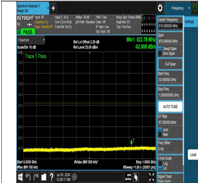
NTNV-N25-PC3-15-15-H-DFT-PI2BPSK-Edge_1RB_Left-30-1000-Ant1-PASS
