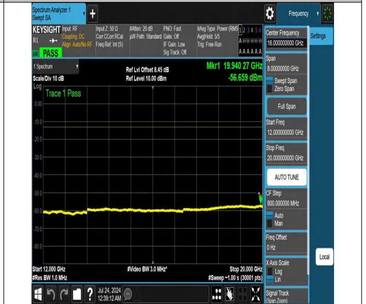
NTNV-N25-PC3-15-20-M-DFT-PI2BPSK-Edge_1RB_Right-12000-20000-Ant1-PASS
