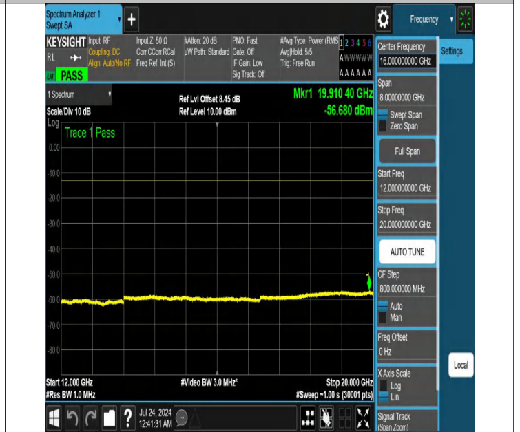
NTNV-N25-PC3-15-20-M-DFT-QPSK-Edge_1RB_Right-12000-20000-Ant1-PASS
