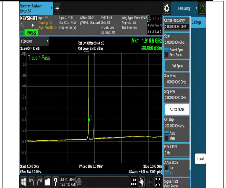
NTNV-N25-PC3-15-15-H-DFT-PI2BPSK-Edge_1RB_Right-1000-3000-Ant1-PASS
