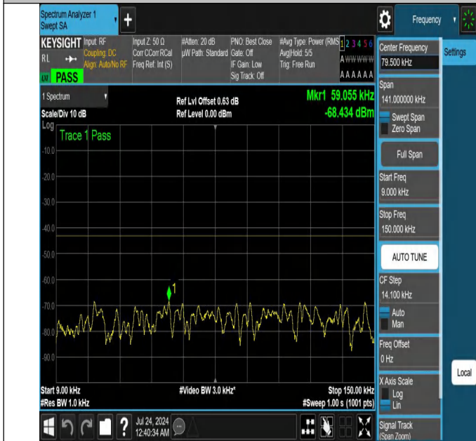
NTNV-N25-PC3-15-20-M-DFT-QPSK-Edge_1RB_Right-0.009-0. 15-Ant1-PASS
