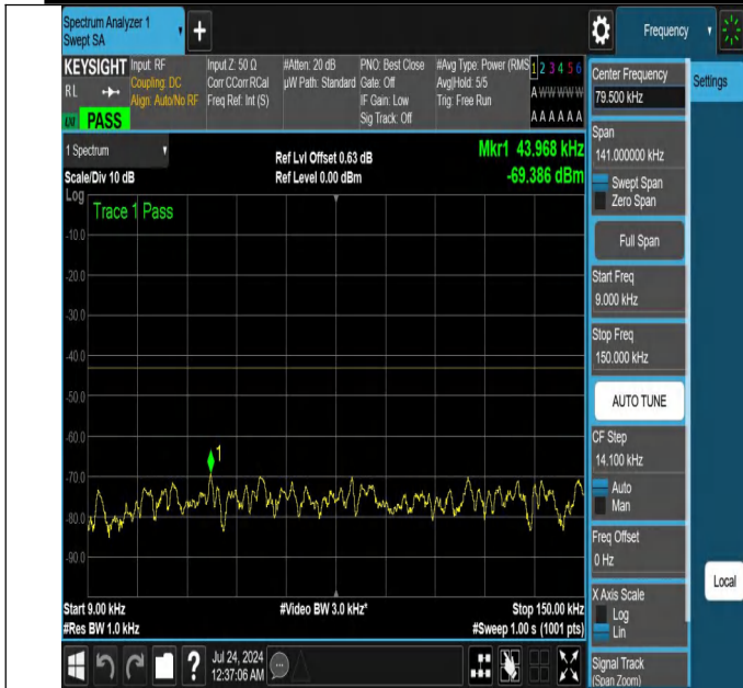
NTNV-N25-PC3-15-20-M-DFT-PI2BPSK-Edge_1RB_Left-0.009-0.15-Ant1-PASS
