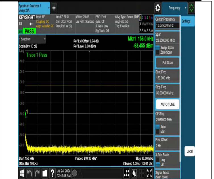
NTNV-N25-PC3-15-20-H-DFT-PI2BPSK-Edge_1RB_Left-0.15-30-Ant1-PASS
