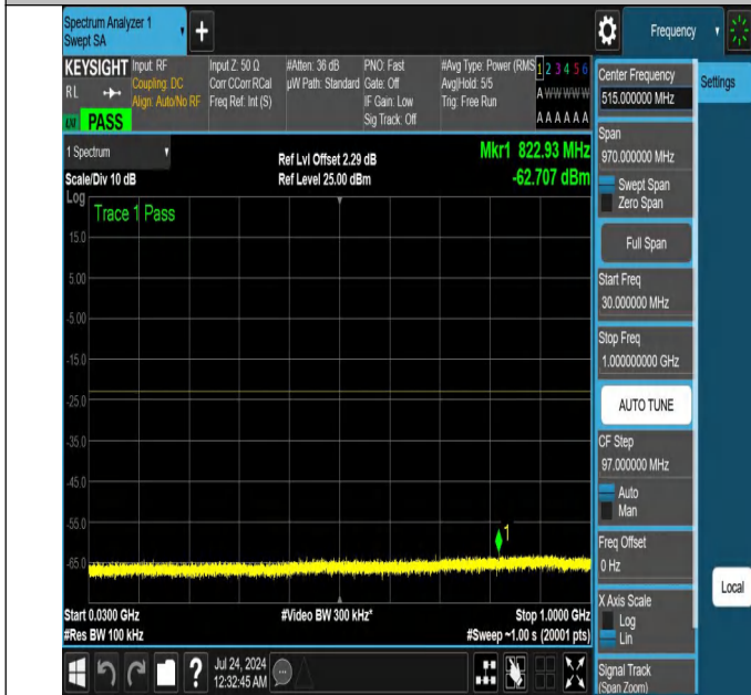
NTNV-N25-PC3-15-20-L-DFT-PI2BPSK-Edge_1RB_Left-30-1000-Ant1-PASS
