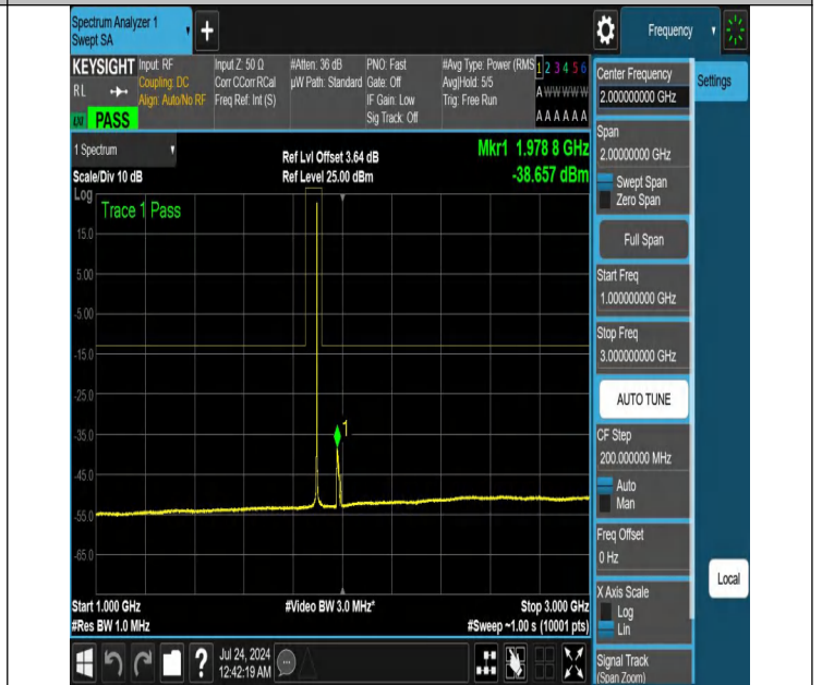
NTNV-N25-PC3-15-20-H-DFT-PI2BPSK-Edge_1RB_Left-1000-3000-Ant1-PASS
