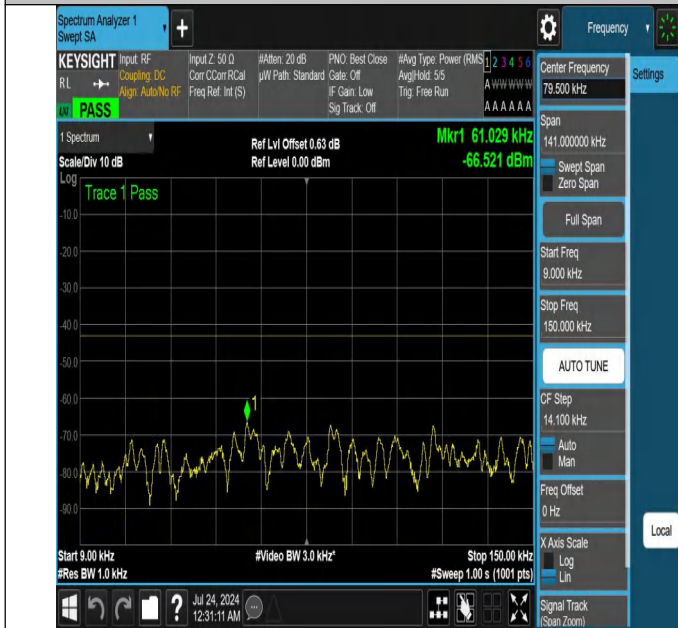
NTNV-N25-PC3-15-15-H-DFT-QPSK-Edge_1RB_Right-0.009-0.1 5-Ant1-PASS
