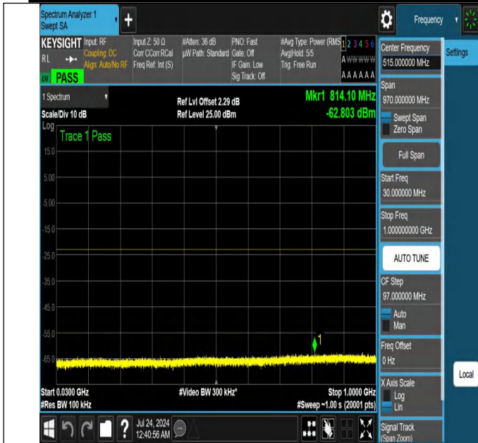
NTNV-N25-PC3-15-20-M-DFT-QPSK-Edge_1RB_Right-30-1000-Ant1-PASS
