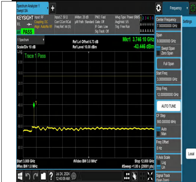
NTNV-N25-PC3-15-20-M-DFT-QPSK-Edge_1RB_Left-3000-1200 0-Ant1-PASS
