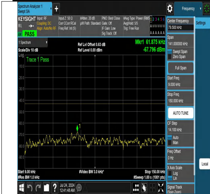
NTNV-N25-PC3-15-20-H-DFT-PI2BPSK-Edge_1RB_Left-0.009-0.15-Ant1-PASS
