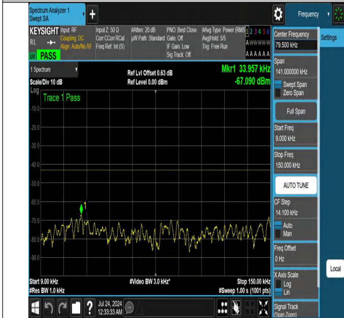
NTNV-N25-PC3-15-20-L-DFT-PI2BPSK-Edge_1RB_Right-0.009-0.15-Ant1-PASS
