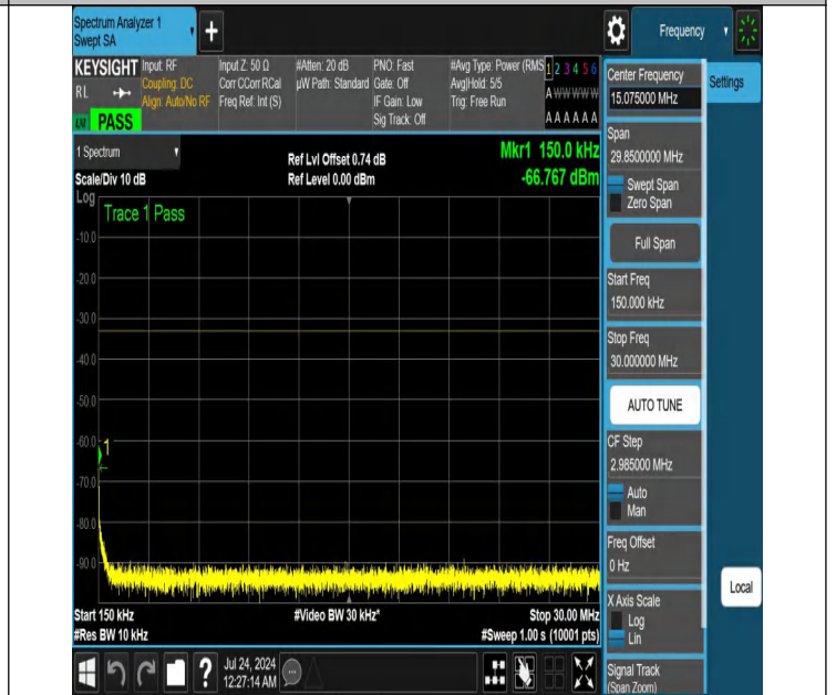
NTNV-N25-PC3-15-15-H-DFT-PI2BPSK-Edge_1RB_Right-0.15-3 0-Ant1-PASS
