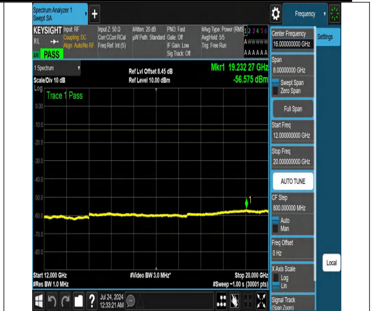
NTNV-N25-PC3-15-20-L-DFT-PI2BPSK-Edge_1RB_Left-12000-20000-Ant1-PASS
