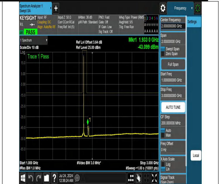
NTNV-N25-PC3-15-20-L-DFT-QPSK-Edge_1RB_Right-1000-3000-Ant1-PASS
