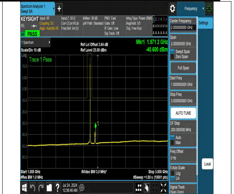
NTNV-N25-PC3-15-20-M-DFT-PI2BPSK-Edge_1RB_Right-1000-3000-Ant1-PASS
