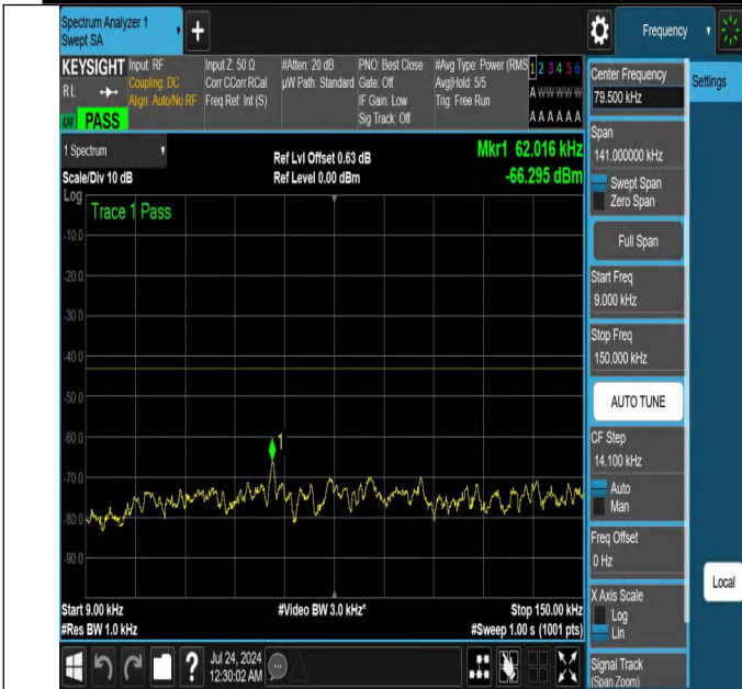
NTNV-N25-PC3-15-15-H-DFT-QPSK-Edge_1RB_Left-0.009-0.15 -Ant1-PASS
