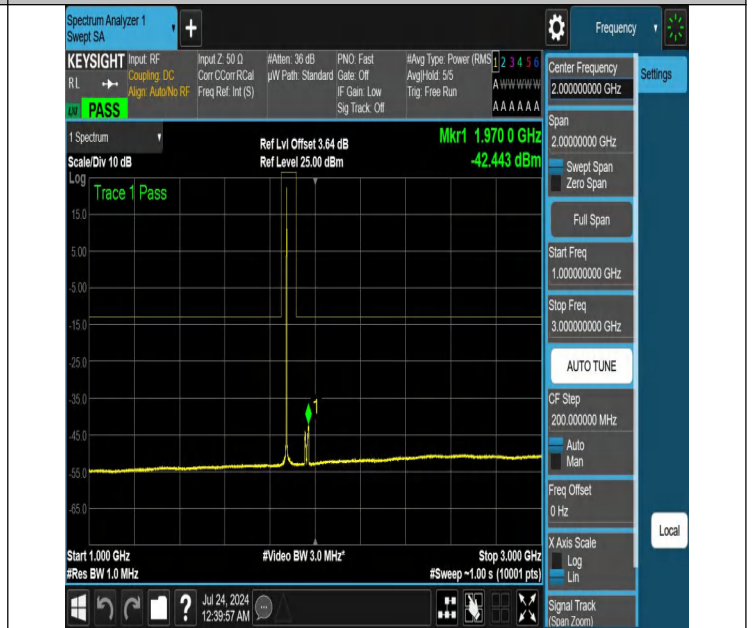
NTNV-N25-PC3-15-20-M-DFT-QPSK-Edge_1RB_Left-1000-3000-Ant1-PASS
