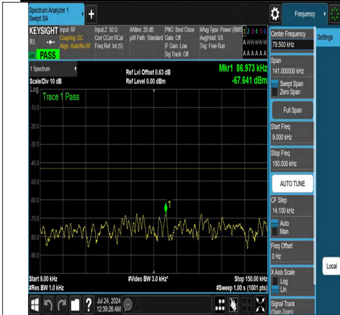
NTNV-N25-PC3-15-20-M-DFT-QPSK-Edge_1RB_Left-0.009-0.15 -Ant1-PASS
