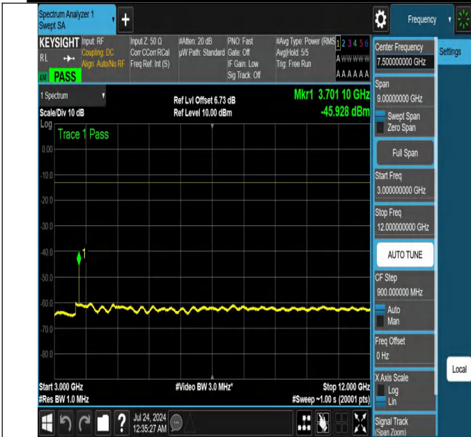
NTNV-N25-PC3-15-20-L-DFT-QPSK-Edge_1RB_Left-3000-1200 0-Ant1-PASS
