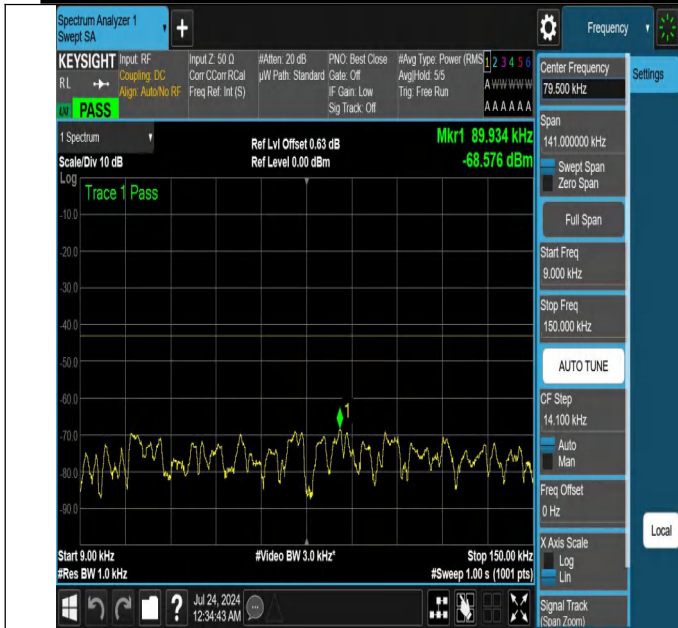
NTNV-N25-PC3-15-20-L-DFT-QPSK-Edge_1RB_Left-0.009-0.15-Ant1-PASS
