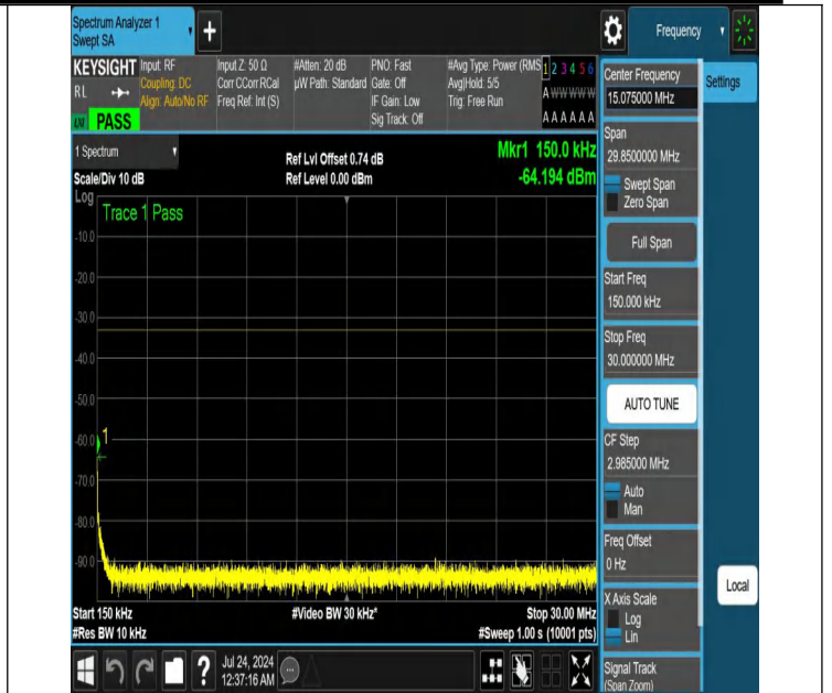
NTNV-N25-PC3-15-20-M-DFT-PI2BPSK-Edge_1RB_Left-0.15-30-Ant1-PASS
