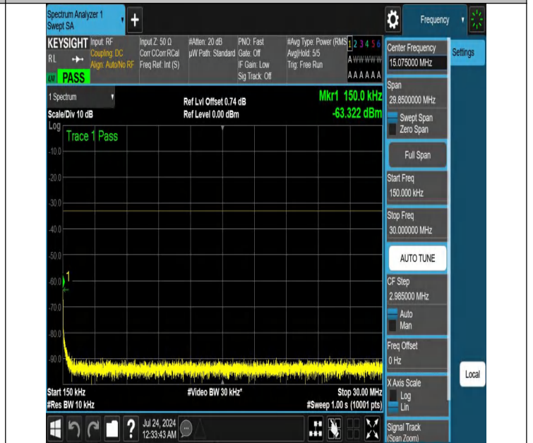
NTNV-N25-PC3-15-20-L-DFT-PI2BPSK-Edge_1RB_Right-0.15-30-Ant1-PASS
