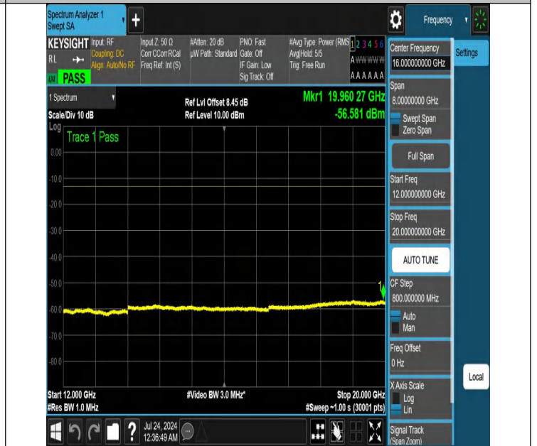
NTNV-N25-PC3-15-20-L-DFT-QPSK-Edge_1RB_Right-12000-20000-Ant1-PASS
