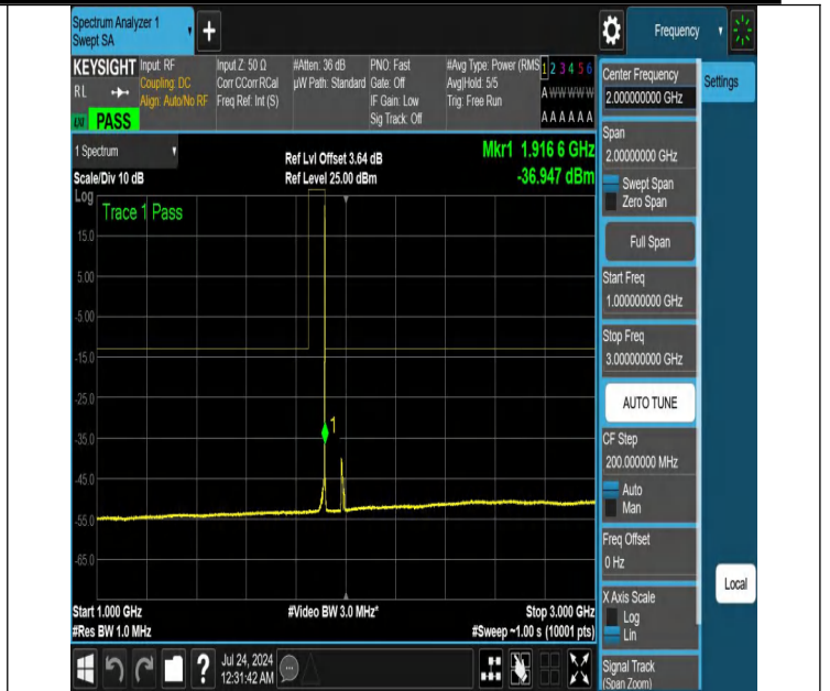
NTNV-N25-PC3-15-15-H-DFT-QPSK-Edge_1RB_Right-1000-300-0-Ant1-PASS
