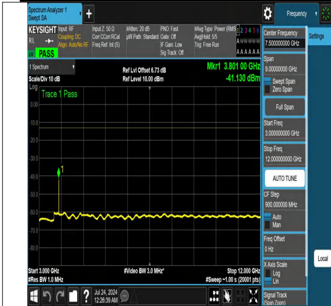
NTNV-N25-PC3-15-15-H-DFT-PI2BPSK-Edge_1RB_Left-3000-1 2000-Ant1-PASS
