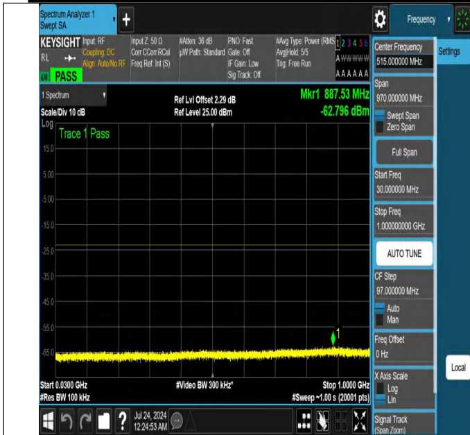
NTNV-N25-PC3-15-15-M-DFT-QPSK-Edge_1RB_Right-30-1000-Ant1-PASS
