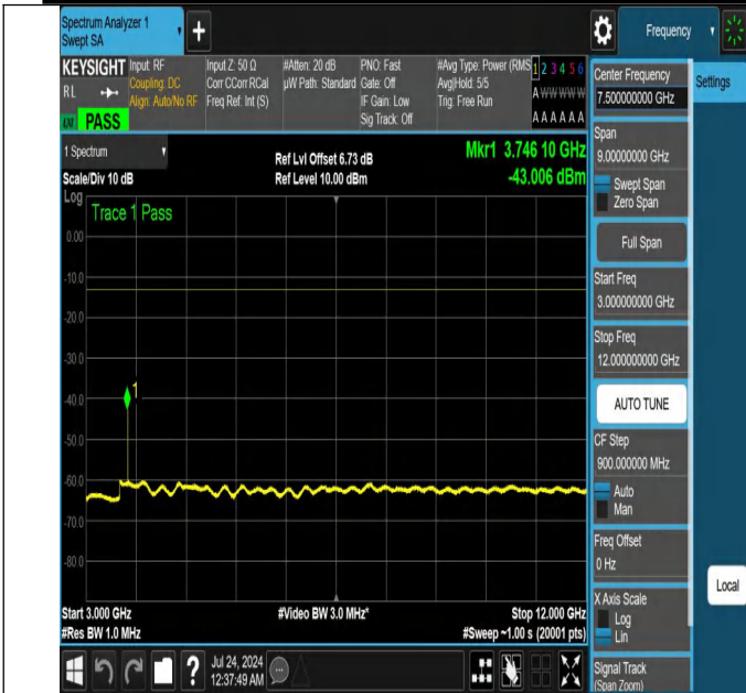
NTNV-N25-PC3-15-20-M-DFT-PI2BPSK-Edge_1RB_Left-3000-1 2000-Ant1-PASS
