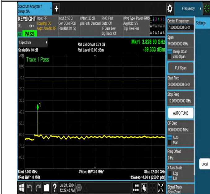
NTNV-N25-PC3-15-15-H-DFT-PI2BPSK-Edge_1RB_Right-3000-12000-Ant1-PASS
