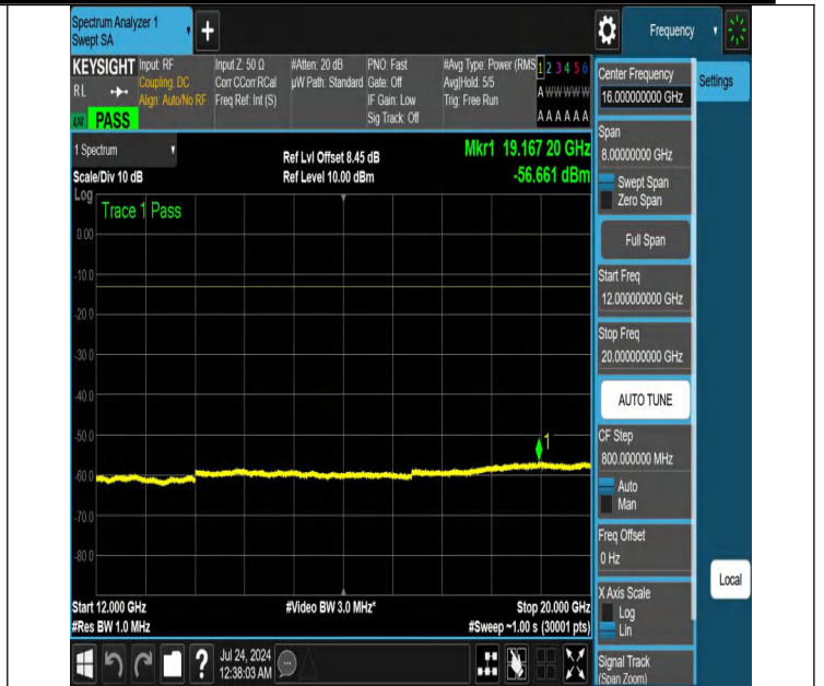
NTNV-N25-PC3-15-20-M-DFT-PI2BPSK-Edge_1RB_Left-12000-2 0000-Ant1-PASS
