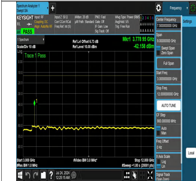
NTNV-N25-PC3-15-15-M-DFT-QPSK-Edge_1RB_Right-3000-12000-Ant1-PASS
