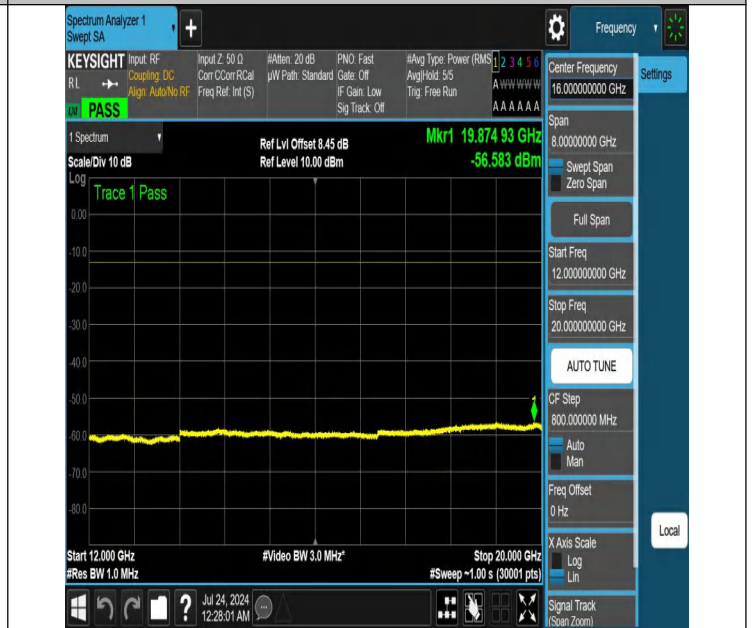
NTNV-N25-PC3-15-15-H-DFT-PI2BPSK-Edge_1RB_Right-12000-20000-Ant1-PASS
