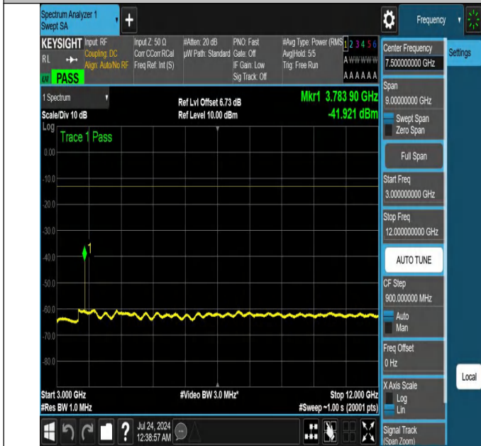
NTNV-N25-PC3-15-20-M-DFT-PI2BPSK-Edge_1RB_Right-3000-12000-Ant1-PASS
