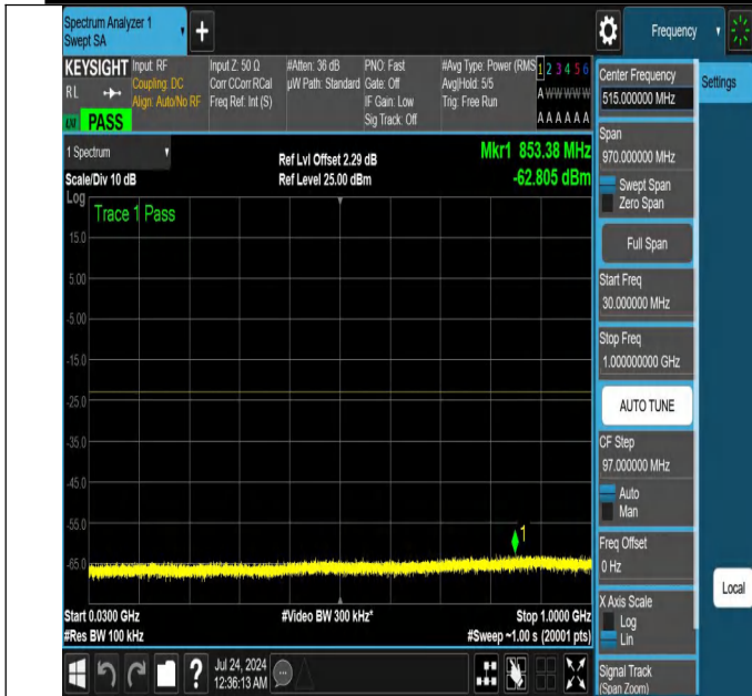
NTNV-N25-PC3-15-20-L-DFT-QPSK-Edge_1RB_Right-30-1000-Ant1-PASS
