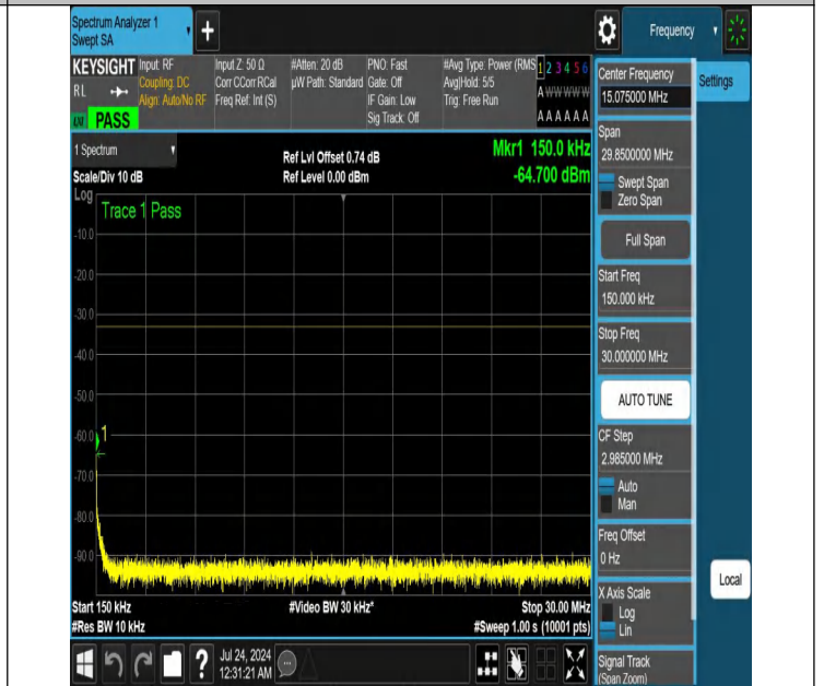
NTNV-N25-PC3-15-15-H-DFT-QPSK-Edge_1RB_Right-0.15-30-A nt1-PASS
