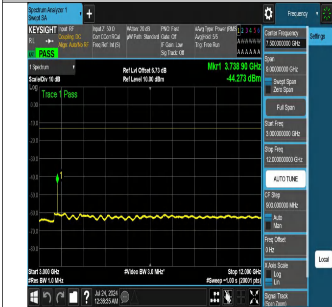
NTNV-N25-PC3-15-20-L-DFT-QPSK-Edge_1RB_Right-3000-12000-Ant1-PASS
