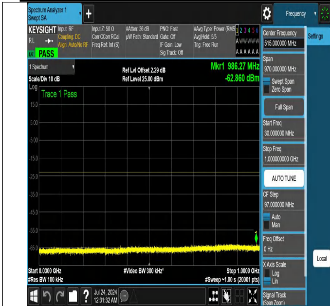
NTNV-N25-PC3-15-15-H-DFT-QPSK-Edge_1RB_Right-30-1000-Ant1-PASS
