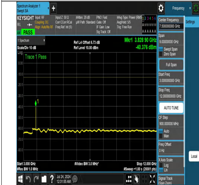
NTNV-N25-PC3-15-15-H-DFT-QPSK-Edge_1RB_Right-3000-120-00-Ant1-PASS
