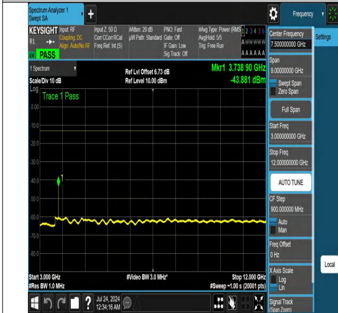
NTNV-N25-PC3-15-20-L-DFT-PI2BPSK-Edge_1RB_Right-3000-12000-Ant1-PASS
