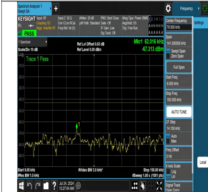
NTNV-N25-PC3-15-15-H-DFT-PI2BPSK-Edge_1RB_Right-0.009- 0.15-Ant1-PASS
