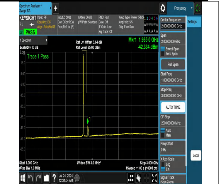
NTNV-N25-PC3-15-20-L-DFT-PI2BPSK-Edge_1RB_Right-1000-3000-Ant1-PASS
