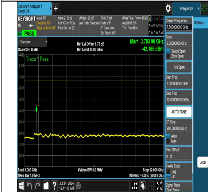
NTNV-N25-PC3-15-20-M-DFT-QPSK-Edge_1RB_Right-3000-12000-Ant1-PASS
