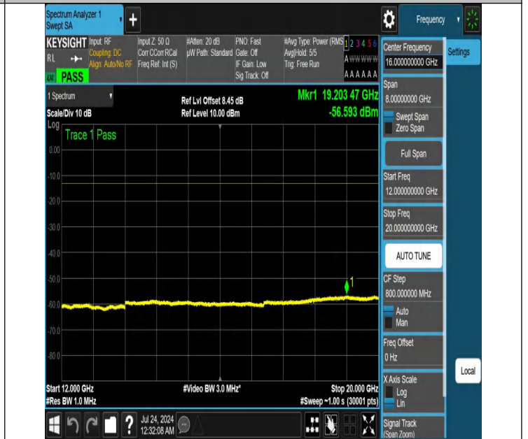
NTNV-N25-PC3-15-15-H-DFT-QPSK-Edge_1RB_Right-12000-20-000-Ant1-PASS
