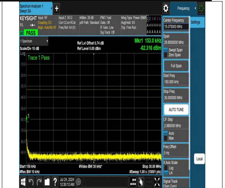
NTNV-N25-PC3-15-15-H-DFT-QPSK-Edge_1RB_Left-0.15-30-Ant 1-PASS
