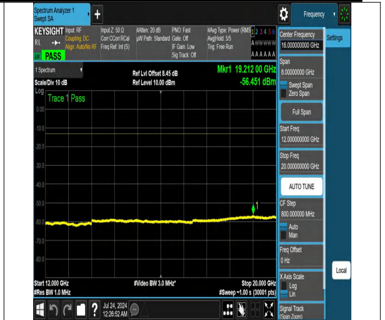
NTNV-N25-PC3-15-15-H-DFT-PI2BPSK-Edge_1RB_Left-12000-2 0000-Ant1-PASS
