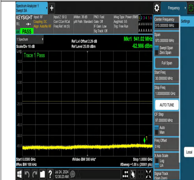
NTNV-N25-PC3-15-15-H-DFT-QPSK-Edge_1RB_Left-30-1000-A nt1-PASS
