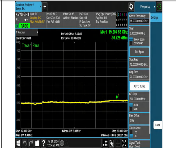
NTNV-N25-PC3-15-20-L-DFT-PI2BPSK-Edge_1RB_Right-12000-20000-Ant1-PASS
