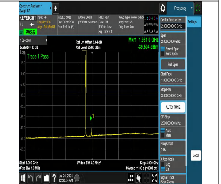
NTNV-N25-PC3-15-15-H-DFT-QPSK-Edge_1RB_Left-1000-3000- Ant1-PASS
