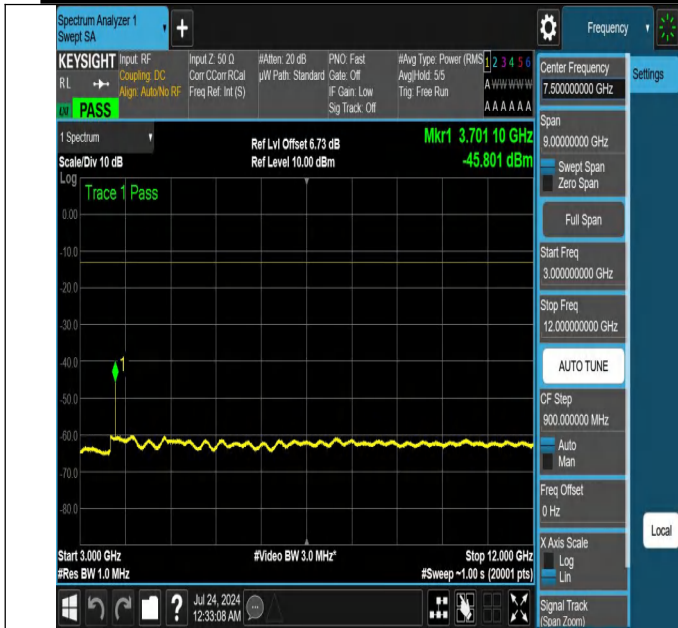
NTNV-N25-PC3-15-20-L-DFT-PI2BPSK-Edge_1RB_Left-3000-12000-Ant1-PASS
