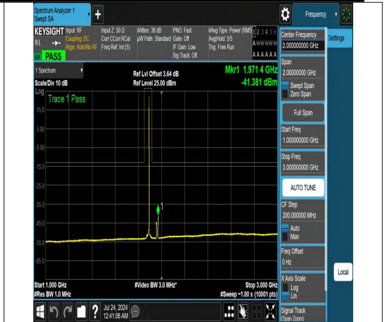
NTNV-N25-PC3-15-20-M-DFT-QPSK-Edge_1RB_Right-1000-300-0-Ant1-PASS
