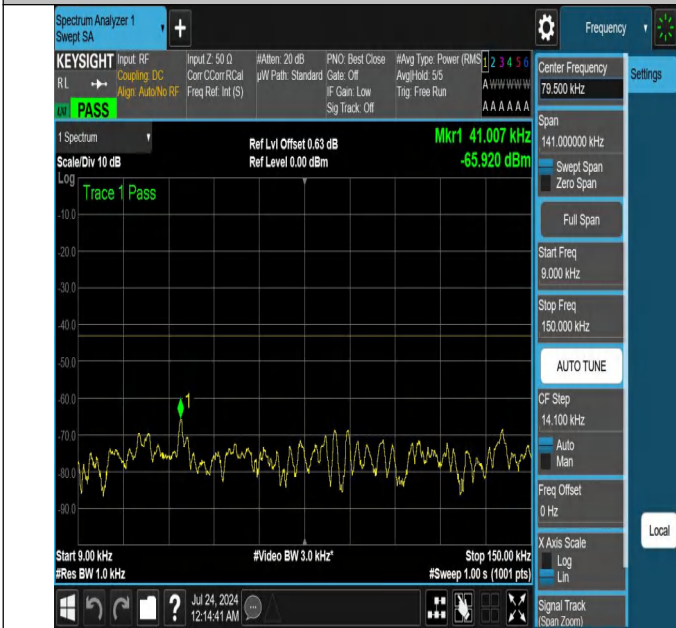
NTNV-N25-PC3-15-10-H-DFT-QPSK-Edge_1RB_Right-0.009-0.1 5-Ant1-PASS
