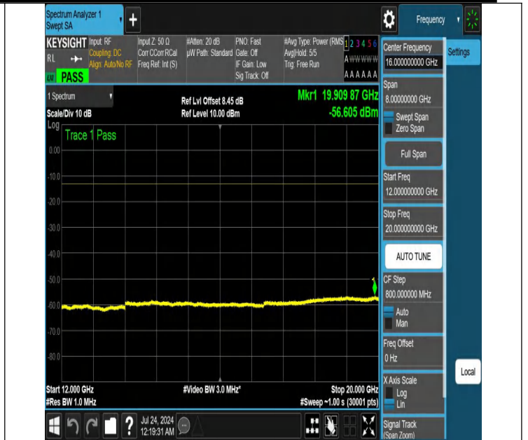
NTNV-N25-PC3-15-15-L-DFT-QPSK-Edge_1RB_Left-12000-2000 0-Ant1-PASS
