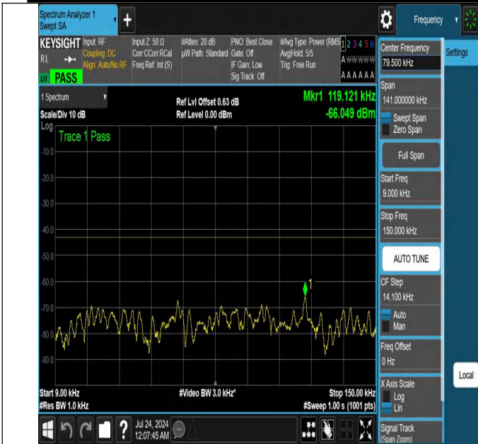
NTNV-N25-PC3-15-10-M-DFT-QPSK-Edge_1RB_Left-0.009-0.15 -Ant1-PASS
