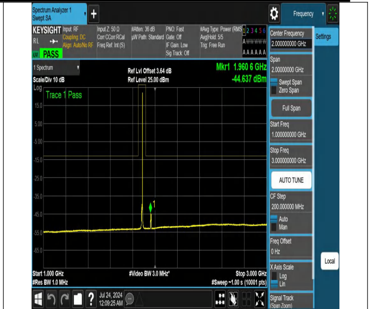
NTNV-N25-PC3-15-10-M-DFT-QPSK-Edge_1RB_Right-1000-300-0-Ant1-PASS
