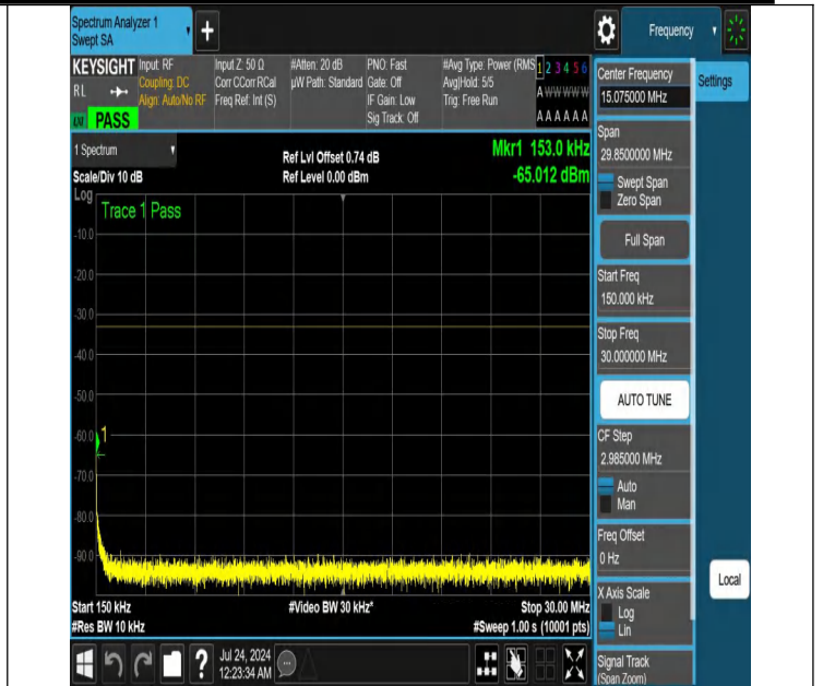
NTNV-N25-PC3-15-15-M-DFT-QPSK-Edge_1RB_Left-0.15-30-Ant 1-PASS
