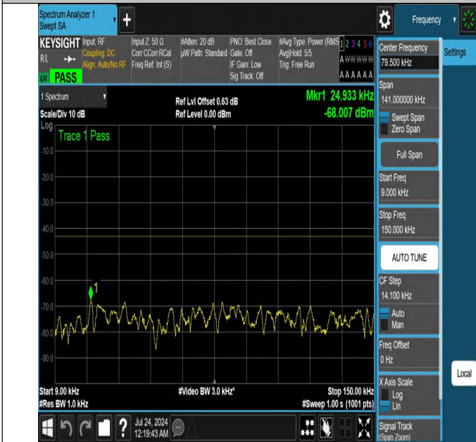
NTNV-N25-PC3-15-15-L-DFT-QPSK-Edge_1RB_Right-0.009-0.1 5-Ant1-PASS
