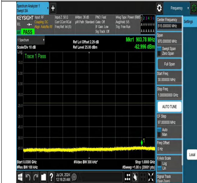
NTNV-N25-PC3-15-15-L-DFT-PI2BPSK-Edge_1RB_Left-30-1000-Ant1-PASS
