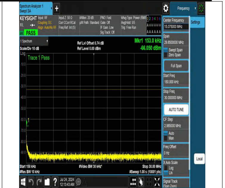
NTNV-N25-PC3-15-10-H-DFT-QPSK-Edge_1RB_Left-0.15-30-Ant 1-PASS
