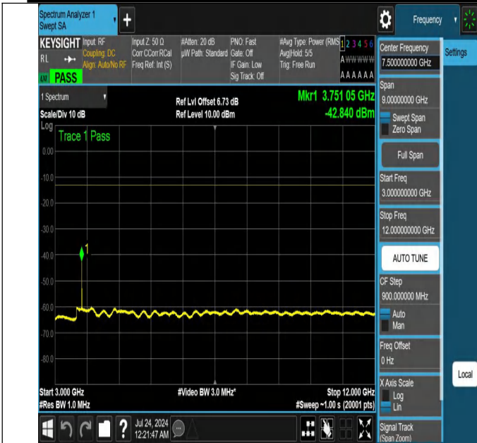
NTNV-N25-PC3-15-15-M-DFT-PI2BPSK-Edge_1RB_Left-3000-1 2000-Ant1-PASS
