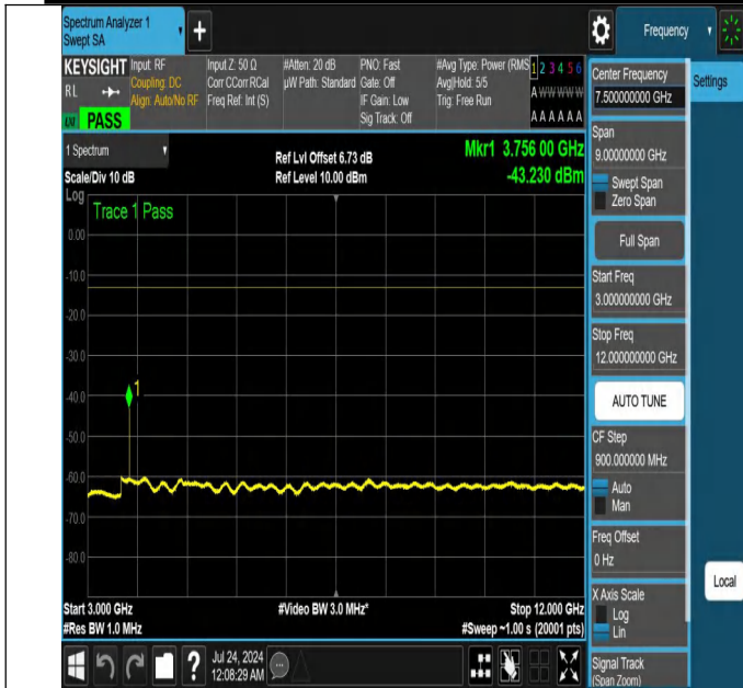
NTNV-N25-PC3-15-10-M-DFT-QPSK-Edge_1RB_Left-3000-1200 0-Ant1-PASS
