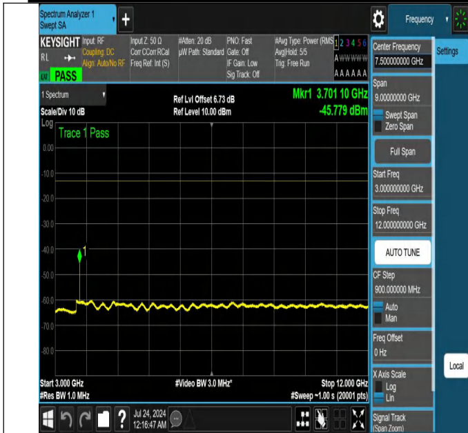
NTNV-N25-PC3-15-15-L-DFT-PI2BPSK-Edge_1RB_Left-3000-12000-Ant1-PASS
