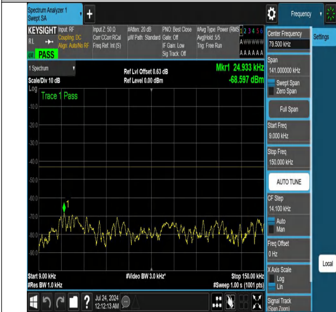
NTNV-N25-PC3-15-10-H-DFT-PI2BPSK-Edge_1RB_Right-0.009- 0.15-Ant1-PASS
