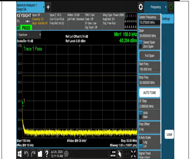
NTNV-N25-PC3-15-10-H-DFT-PI2BPSK-Edge_1RB_Left-0.15-30-Ant1-PASS
