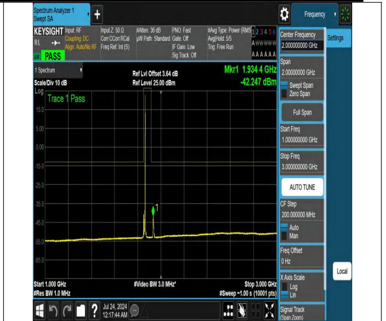
NTNV-N25-PC3-15-15-L-DFT-PI2BPSK-Edge_1RB_Right-1000-3000-Ant1-PASS
