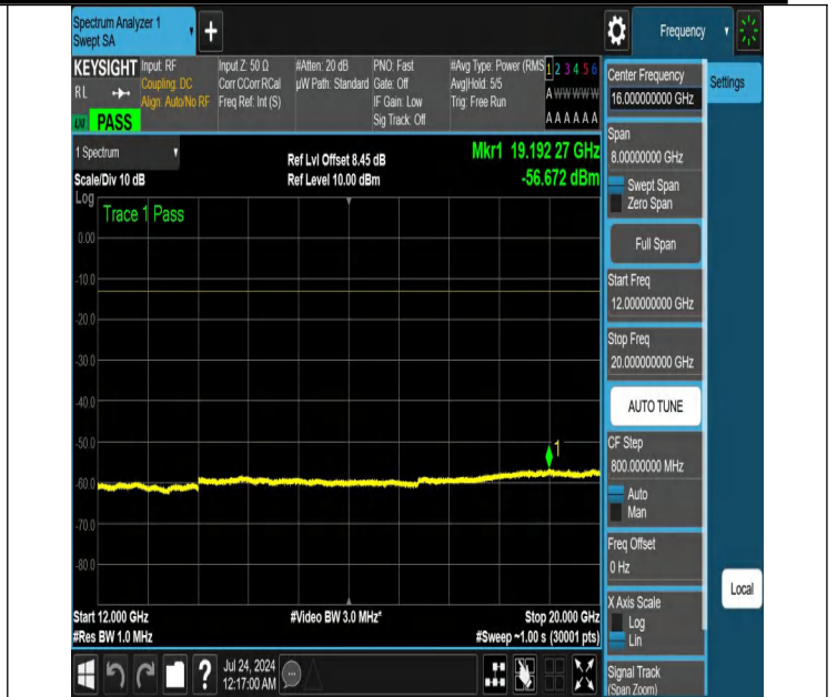
NTNV-N25-PC3-15-15-L-DFT-PI2BPSK-Edge_1RB_Left-12000-20000-Ant1-PASS
