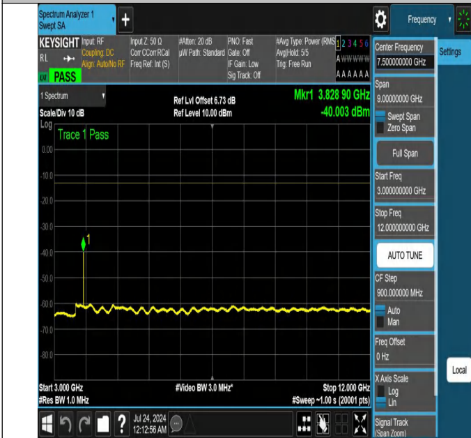
NTNV-N25-PC3-15-10-H-DFT-PI2BPSK-Edge_1RB_Right-3000-12000-Ant1-PASS
