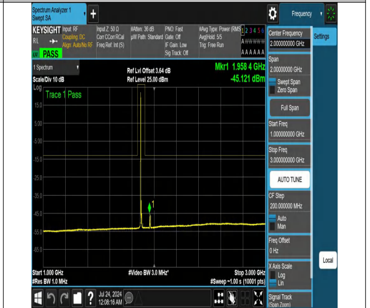
NTNV-N25-PC3-15-10-M-DFT-QPSK-Edge_1RB_Left-1000-3000-Ant1-PASS
