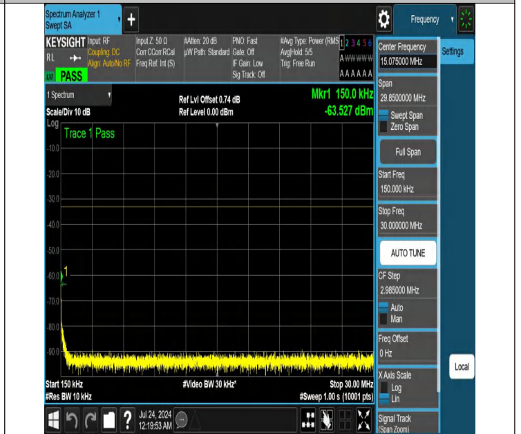
NTNV-N25-PC3-15-15-L-DFT-QPSK-Edge_1RB_Right-0.15-30-A nt1-PASS
