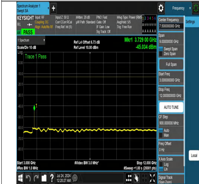
NTNV-N25-PC3-15-15-L-DFT-QPSK-Edge_1RB_Right-3000-12000-Ant1-PASS
