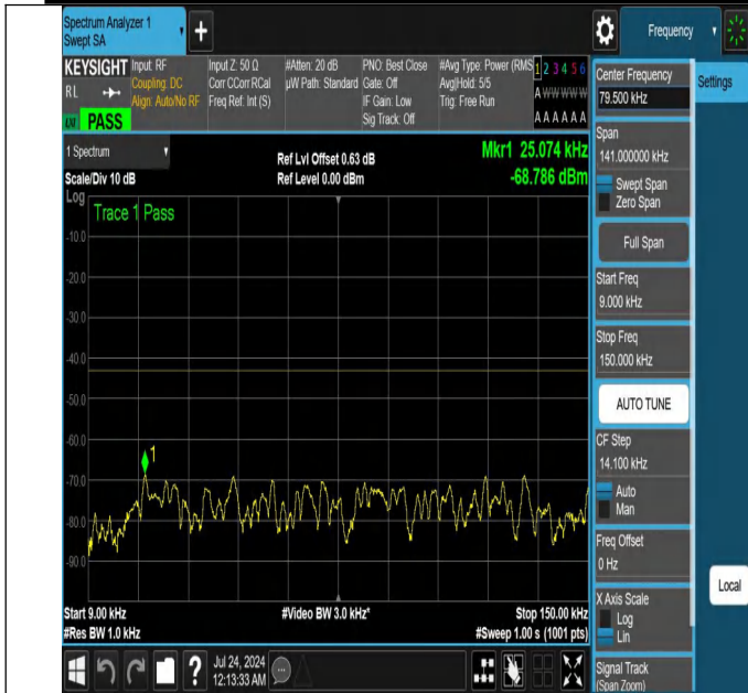
NTNV-N25-PC3-15-10-H-DFT-QPSK-Edge_1RB_Left-0.009-0.15 -Ant1-PASS
