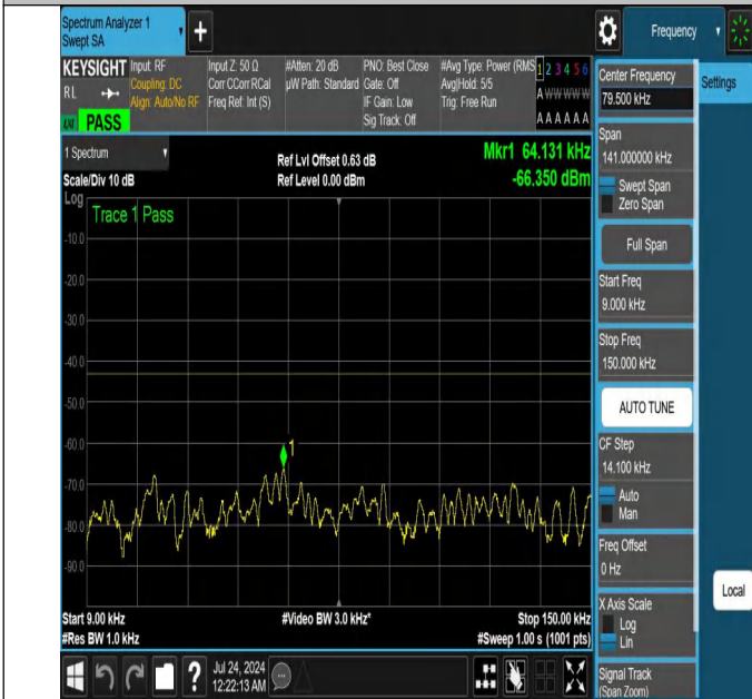
NTNV-N25-PC3-15-15-M-DFT-PI2BPSK-Edge_1RB_Right-0.009 -0.15-Ant1-PASS
