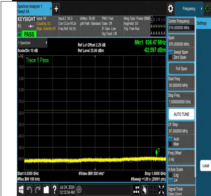
NTNV-N25-PC3-15-10-H-DFT-PI2BPSK-Edge_1RB_Right-30-1000-Ant1-PASS
