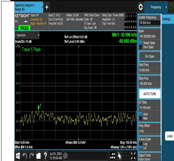
NTNV-N25-PC3-15-15-L-DFT-PI2BPSK-Edge_1RB_Left-0.009-0.15-Ant1-PASS
