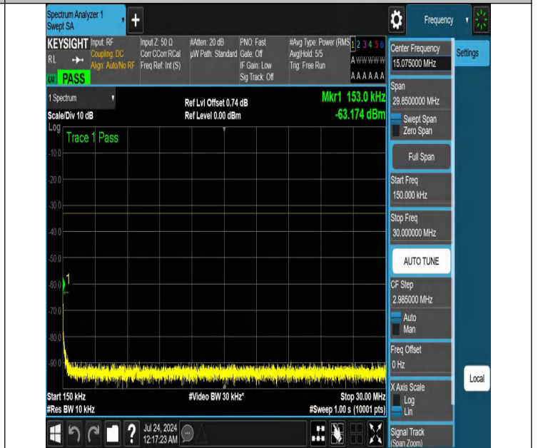
NTNV-N25-PC3-15-15-L-DFT-PI2BPSK-Edge_1RB_Right-0.15-30-Ant1-PASS
