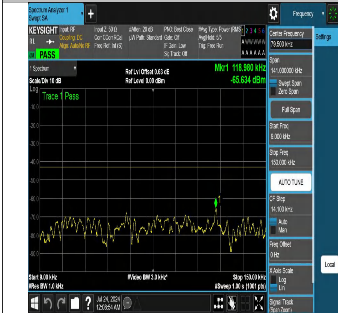
NTNV-N25-PC3-15-10-M-DFT-QPSK-Edge_1RB_Right-0.009-0. 15-Ant1-PASS
