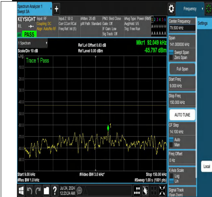
NTNV-N25-PC3-15-15-M-DFT-QPSK-Edge_1RB_Left-0.009-0.15 -Ant1-PASS
