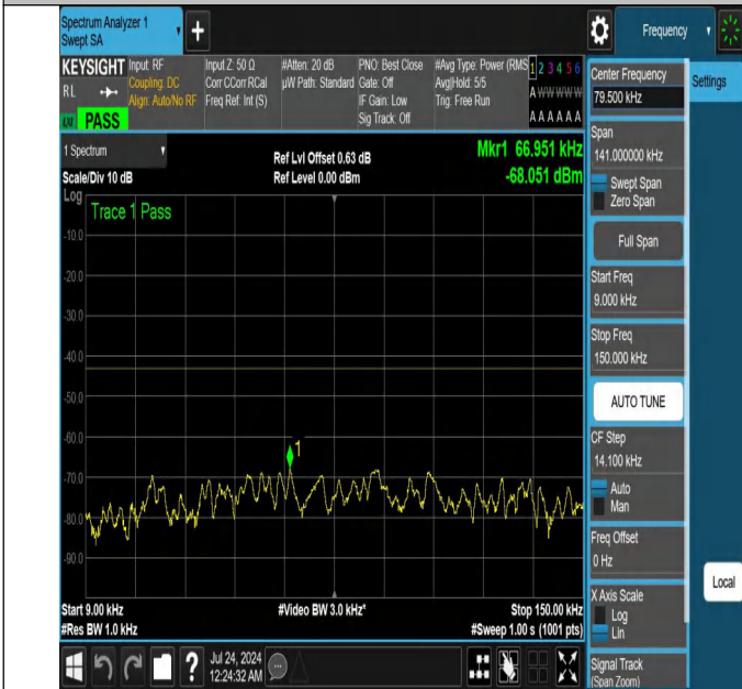
NTNV-N25-PC3-15-15-M-DFT-QPSK-Edge_1RB_Right-0.009-0. 15-Ant1-PASS
