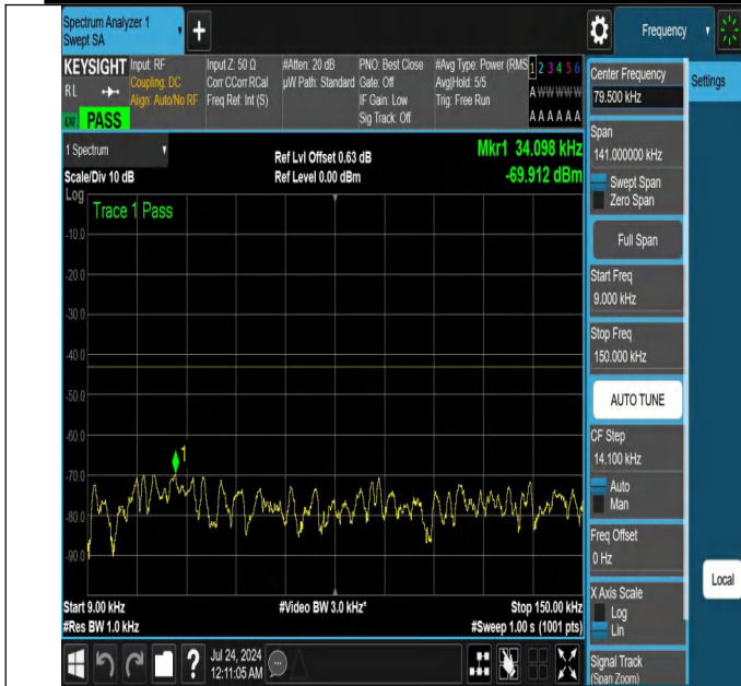
NTNV-N25-PC3-15-10-H-DFT-PI2BPSK-Edge_1RB_Left-0.009-0.15-Ant1-PASS
