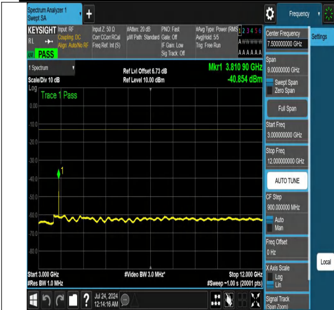
NTNV-N25-PC3-15-10-H-DFT-QPSK-Edge_1RB_Left-3000-1200 0-Ant1-PASS
