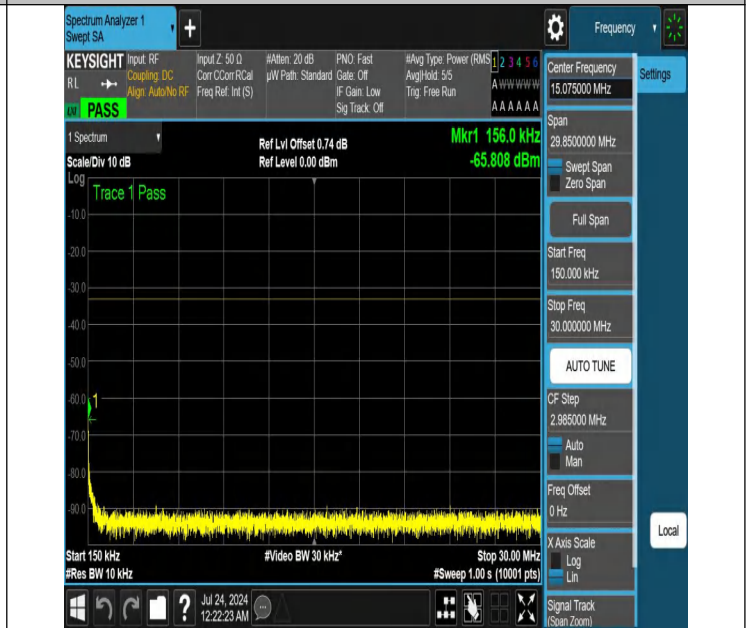
NTNV-N25-PC3-15-15-M-DFT-PI2BPSK-Edge_1RB_Right-0.15-3 0-Ant1-PASS
