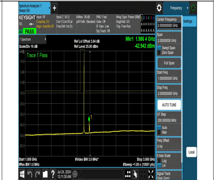
NTNV-N25-PC3-15-10-H-DFT-PI2BPSK-Edge_1RB_Left-1000-3000-Ant1-PASS
