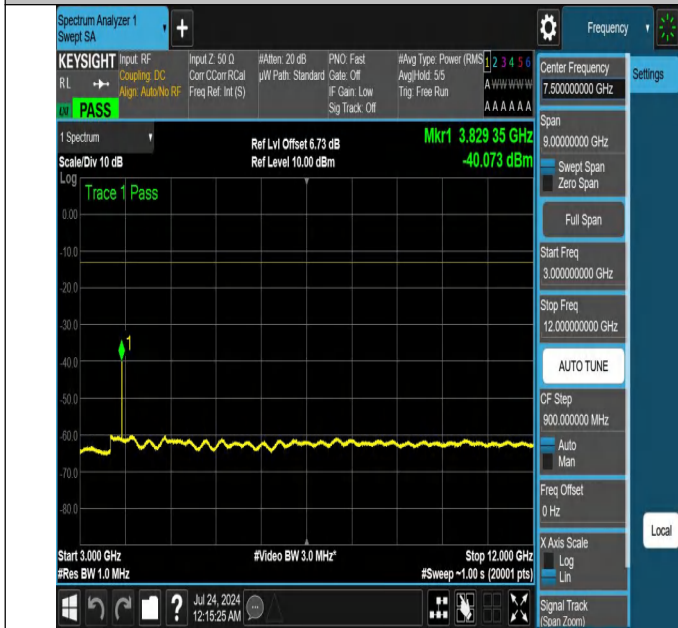
NTNV-N25-PC3-15-10-H-DFT-QPSK-Edge_1RB_Right-3000-12000-Ant1-PASS
