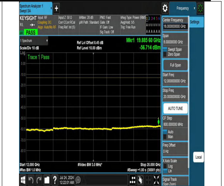
NTNV-N25-PC3-15-15-M-DFT-PI2BPSK-Edge_1RB_Left-12000-2 0000-Ant1-PASS
