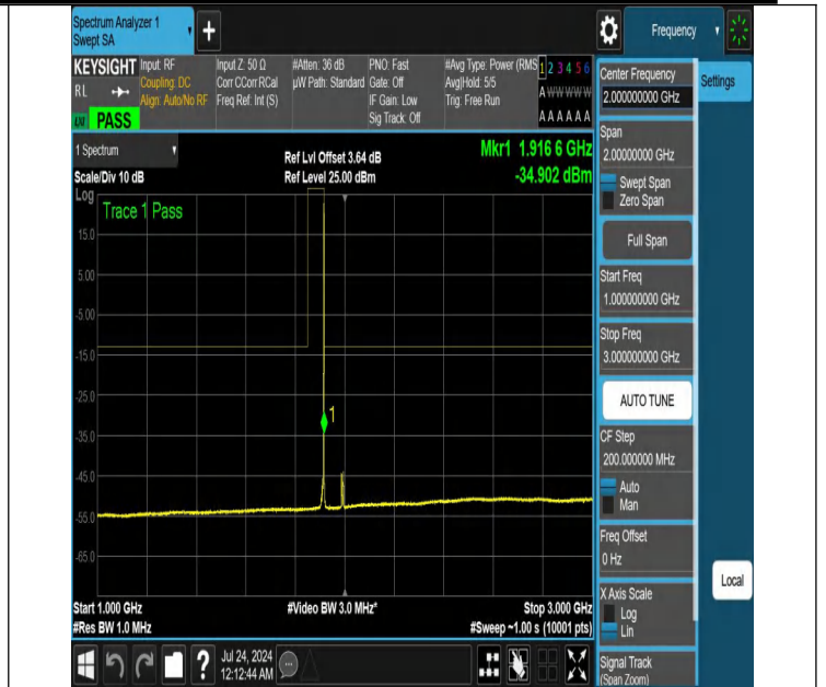
NTNV-N25-PC3-15-10-H-DFT-PI2BPSK-Edge_1RB_Right-1000-3000-Ant1-PASS
