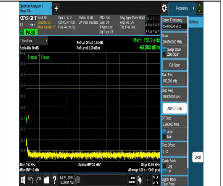
NTNV-N25-PC3-15-10-M-DFT-QPSK-Edge_1RB_Right-0.15-30-A nt1-PASS
