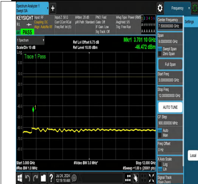
NTNV-N25-PC3-15-15-L-DFT-QPSK-Edge_1RB_Left-3000-1200 0-Ant1-PASS
