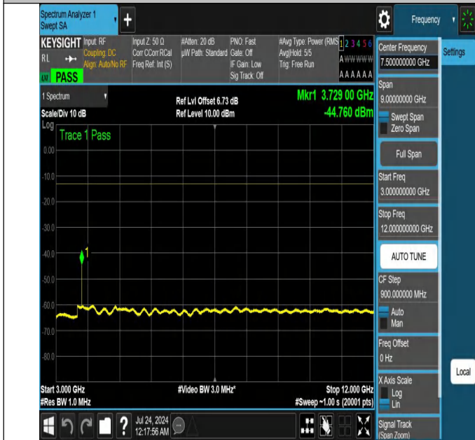
NTNV-N25-PC3-15-15-L-DFT-PI2BPSK-Edge_1RB_Right-3000-12000-Ant1-PASS
