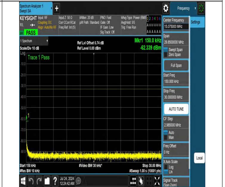
NTNV-N25-PC3-15-15-M-DFT-QPSK-Edge_1RB_Right-0.15-30-A nt1-PASS
