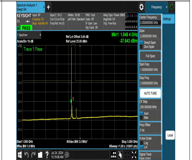
NTNV-N25-PC3-15-15-L-DFT-QPSK-Edge_1RB_Left-1000-3000-Ant1-PASS
