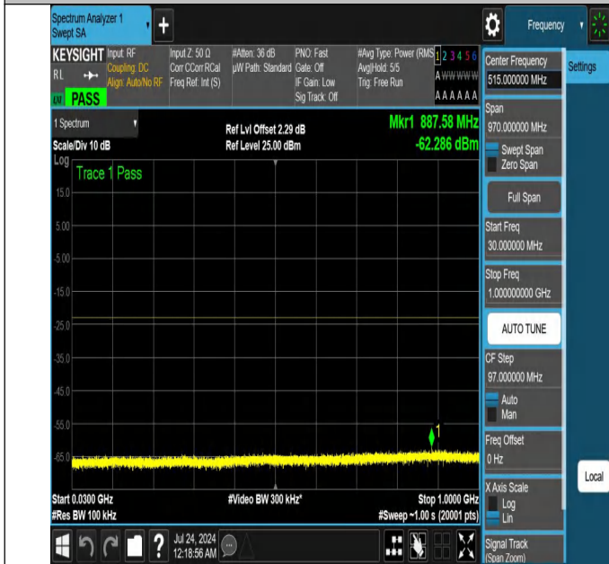
NTNV-N25-PC3-15-15-L-DFT-QPSK-Edge_1RB_Left-30-1000-Ant1-PASS
