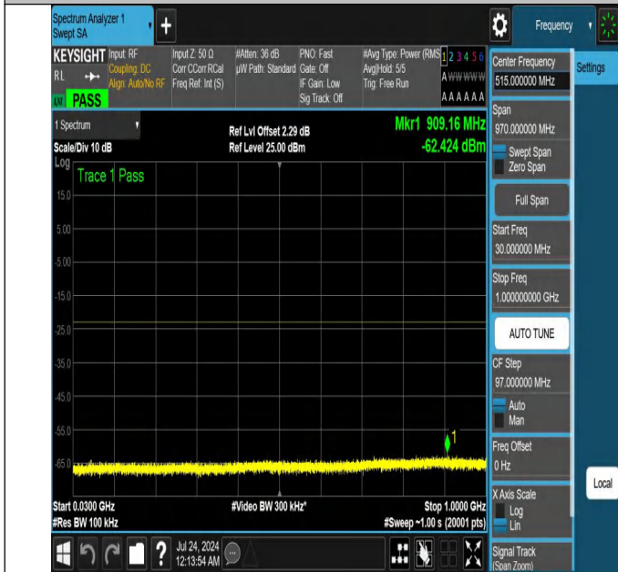
NTNV-N25-PC3-15-10-H-DFT-QPSK-Edge_1RB_Left-30-1000-A nt1-PASS
