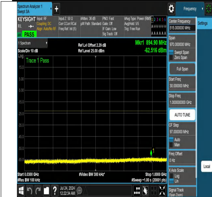
NTNV-N25-PC3-15-15-M-DFT-PI2BPSK-Edge_1RB_Right-30-1000-Ant1-PASS
