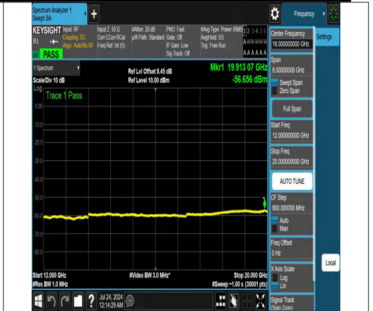
NTNV-N25-PC3-15-10-H-DFT-QPSK-Edge_1RB_Left-12000-2000 0-Ant1-PASS
