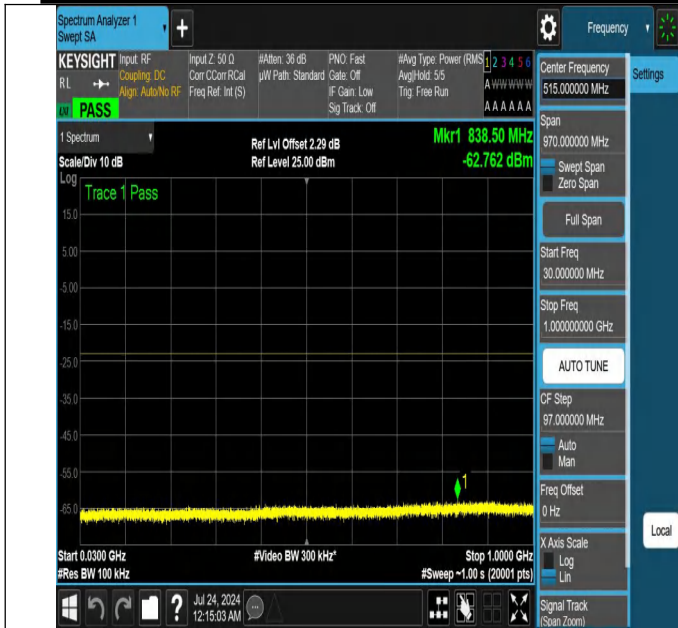
NTNV-N25-PC3-15-10-H-DFT-QPSK-Edge_1RB_Right-30-1000-Ant1-PASS
