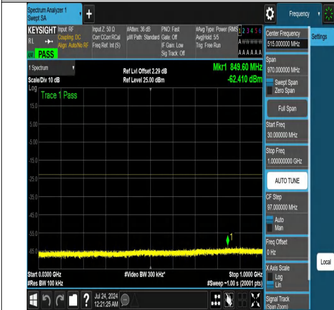
NTNV-N25-PC3-15-15-M-DFT-PI2BPSK-Edge_1RB_Left-30-1000-Ant1-PASS
