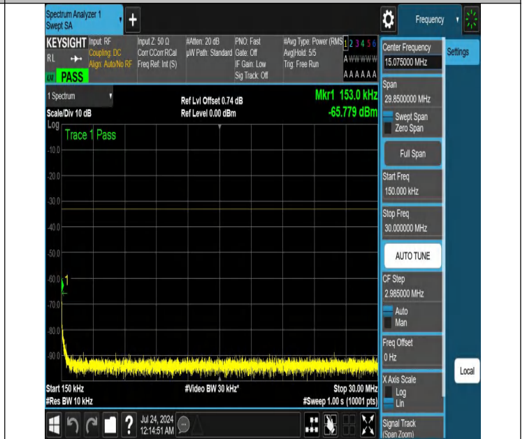
NTNV-N25-PC3-15-10-H-DFT-QPSK-Edge_1RB_Right-0.15-30-A nt1-PASS
