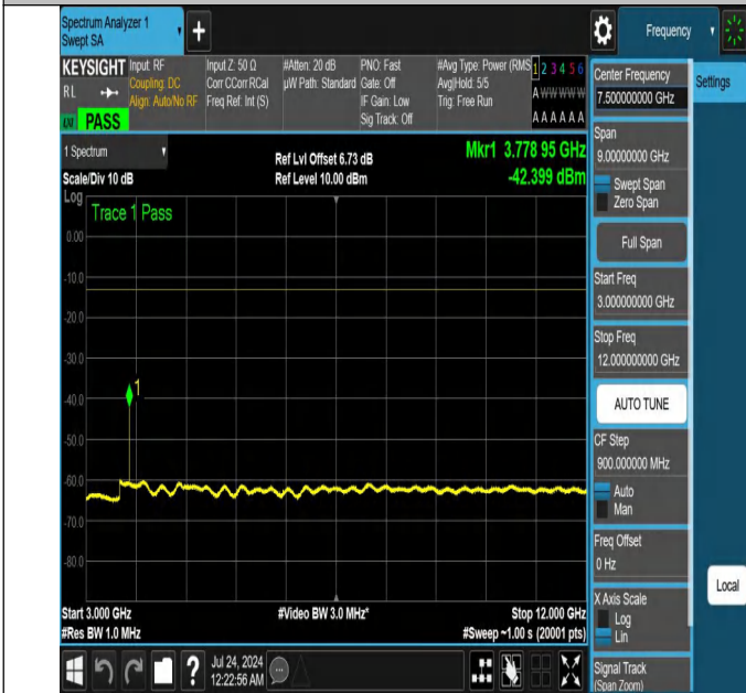
NTNV-N25-PC3-15-15-M-DFT-PI2BPSK-Edge_1RB_Right-3000-12000-Ant1-PASS
