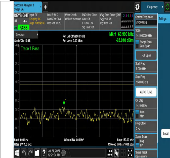
NTNV-N25-PC3-15-15-M-DFT-PI2BPSK-Edge_1RB_Left-0.009-0.15-Ant1-PASS
