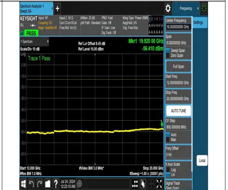
NTNV-N25-PC3-15-15-M-DFT-PI2BPSK-Edge_1RB_Right-12000-20000-Ant1-PASS
