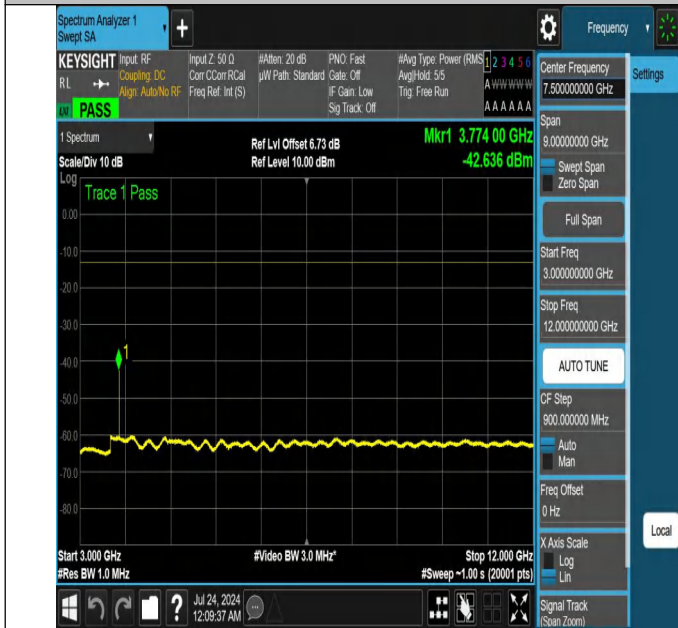
NTNV-N25-PC3-15-10-M-DFT-QPSK-Edge_1RB_Right-3000-12000-Ant1-PASS
