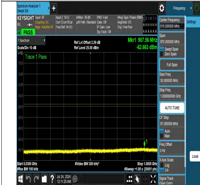
NTNV-N25-PC3-15-10-H-DFT-PI2BPSK-Edge_1RB_Left-30-1000-Ant1-PASS
