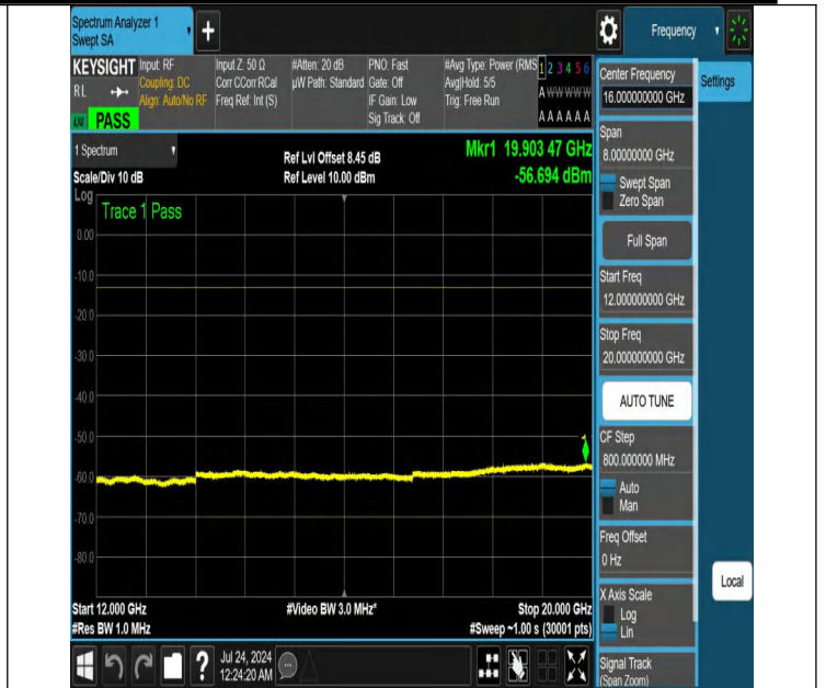
NTNV-N25-PC3-15-15-M-DFT-QPSK-Edge_1RB_Left-12000-200 00-Ant1-PASS
