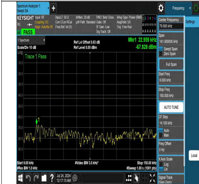
NTNV-N25-PC3-15-15-L-DFT-PI2BPSK-Edge_1RB_Right-0.009-0.15-Ant1-PASS
