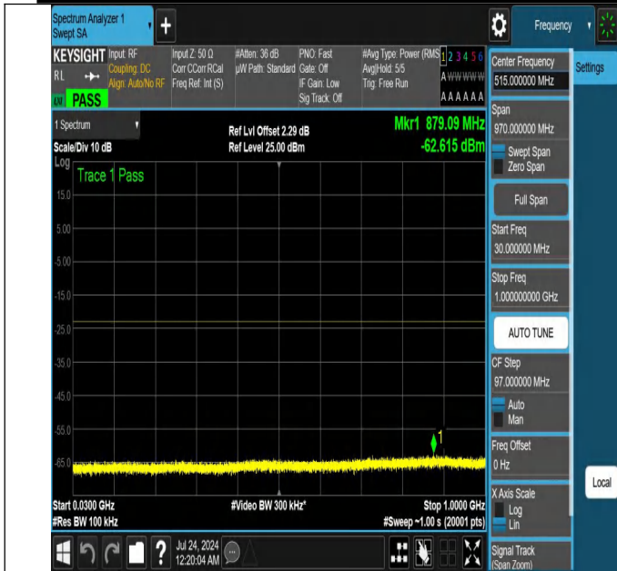
NTNV-N25-PC3-15-15-L-DFT-QPSK-Edge_1RB_Right-30-1000-Ant1-PASS
