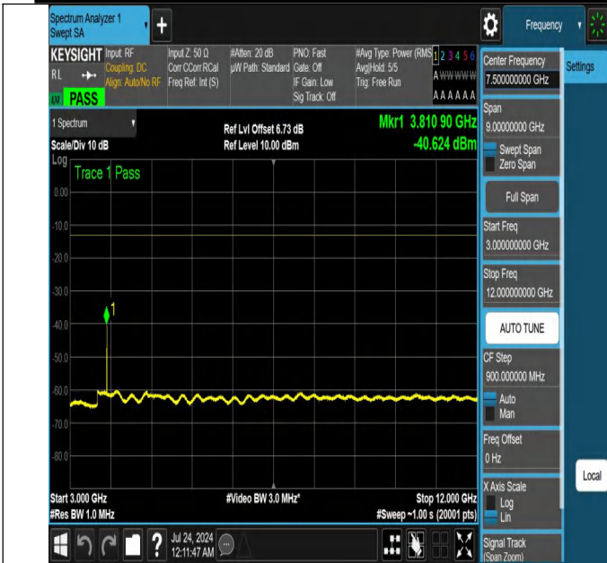
NTNV-N25-PC3-15-10-H-DFT-PI2BPSK-Edge_1RB_Left-3000-1 2000-Ant1-PASS
