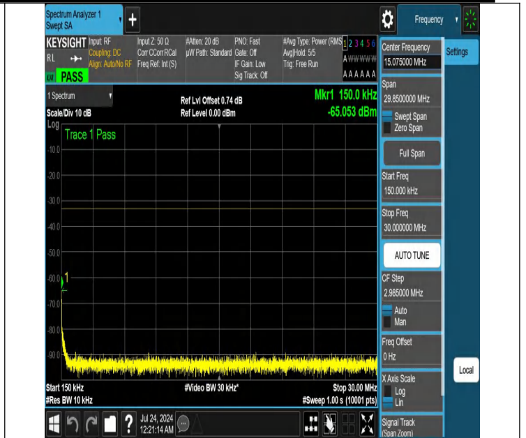
NTNV-N25-PC3-15-15-M-DFT-PI2BPSK-Edge_1RB_Left-0.15-30-Ant1-PASS
