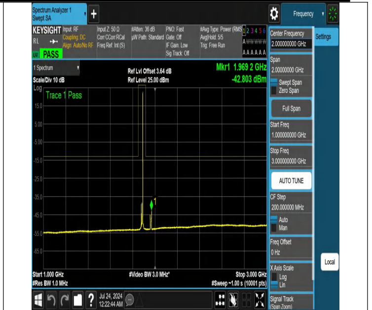
NTNV-N25-PC3-15-15-M-DFT-PI2BPSK-Edge_1RB_Right-1000-3000-Ant1-PASS
