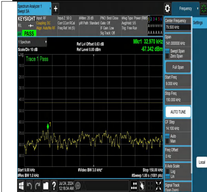
NTNV-N25-PC3-15-15-L-DFT-QPSK-Edge_1RB_Left-0.009-0.15-Ant1-PASS
