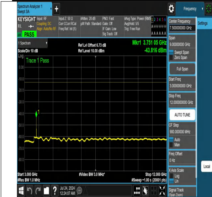
NTNV-N25-PC3-15-15-M-DFT-QPSK-Edge_1RB_Left-3000-1200 0-Ant1-PASS
