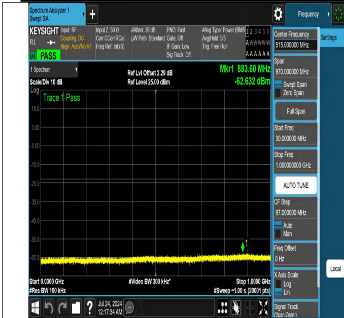
NTNV-N25-PC3-15-15-L-DFT-PI2BPSK-Edge_1RB_Right-30-1000-Ant1-PASS
