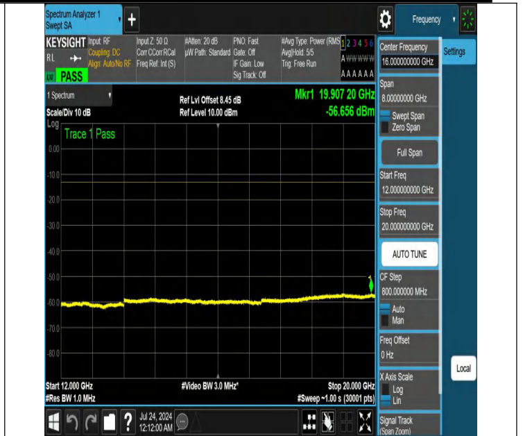
NTNV-N25-PC3-15-10-H-DFT-PI2BPSK-Edge_1RB_Left-12000-2 0000-Ant1-PASS
