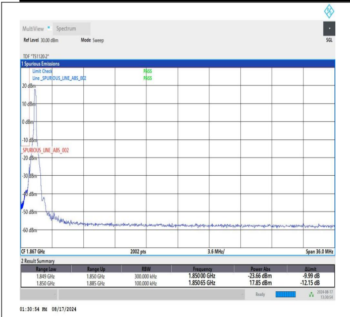
NTVN-n25-PC3-15-35-L-DFT-BPSK-Edge_1RB_Left-PASS
