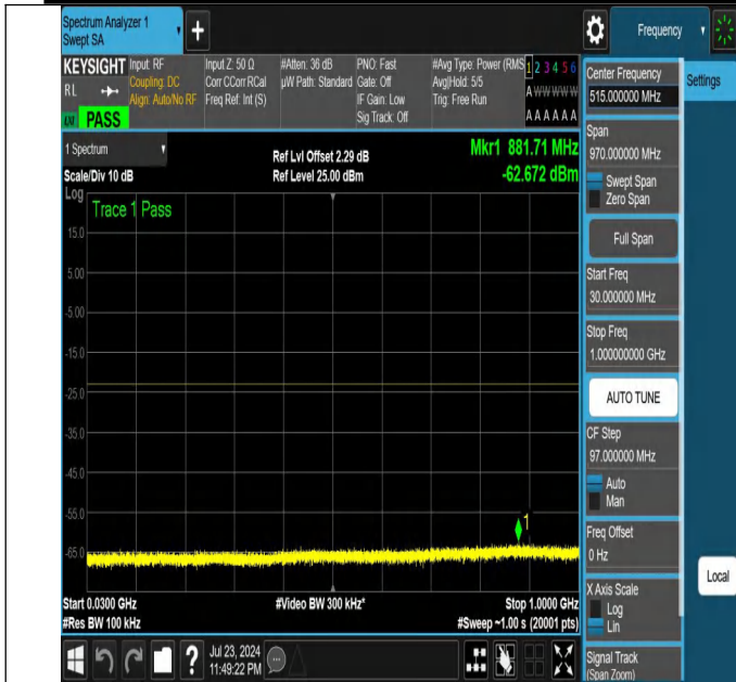
NTNV-N25-PC3-15-5-L-DFT-QPSK-Edge_1RB_Right-30-1000-A nt1-PASS
