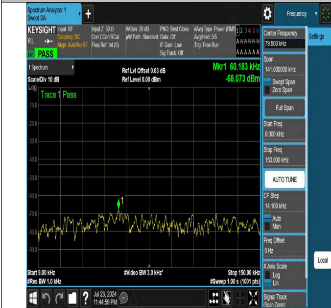
NTNV-N25-PC3-15-5-L-DFT-PI2BPSK-Edge_1RB_Right-0.009-150-Ant1-PASS
