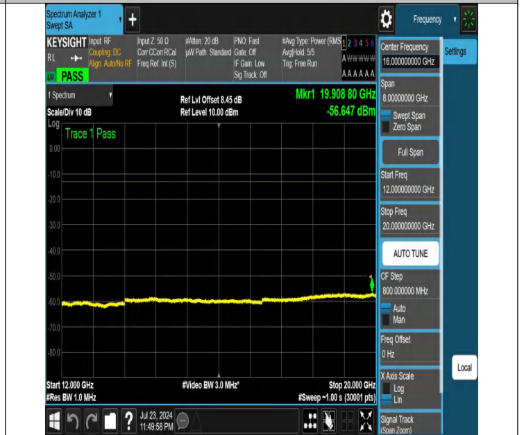
NTNV-N25-PC3-15-5-L-DFT-QPSK-Edge_1RB_Right-12000-2000 0-Ant1-PASS
