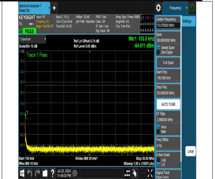
NTNV-N25-PC3-15-5-L-DFT-QPSK-Edge_1RB_Left-0.15-30-Ant1-PASS
