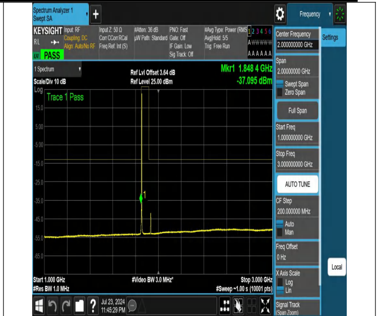
NTNV-N25-PC3-15-5-L-DFT-PI2BPSK-Edge_1RB_Right-1000-30 00-Ant1-PASS
