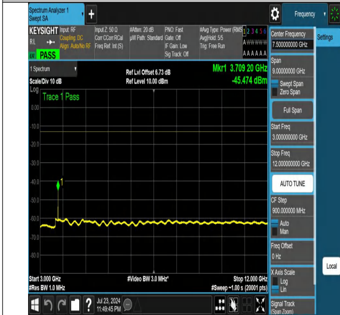
NTNV-N25-PC3-15-5-L-DFT-QPSK-Edge_1RB_Right-3000-1200 0-Ant1-PASS
