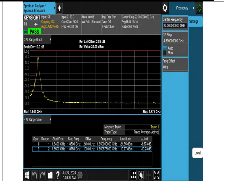
NTNV-N25-PC3-15-25-L-DFT-PI2BPSK-Edge_1RB_Left-Ant1-PASS
