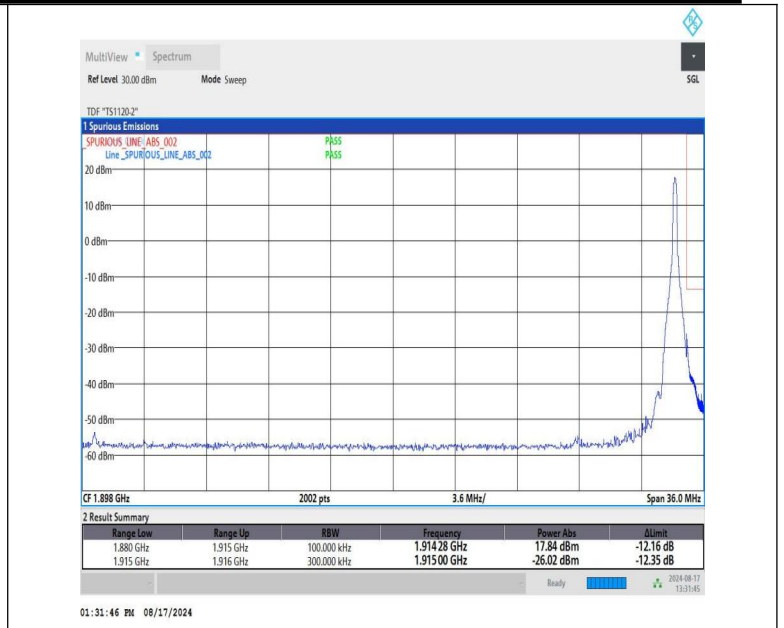
NTV-n25-PC3-15-35-H-DFT-BPSK-Edge_1RB_Right-PASS
