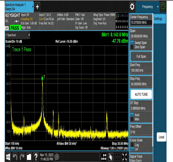
NTNV_N7_PC3_15_20_H_TID24_N/A_0.15_30_#1
