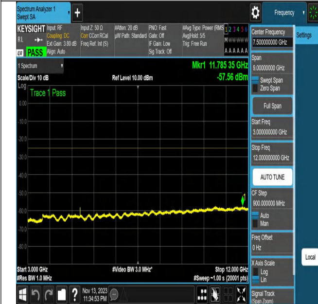
NTNV_N7_PC3_15_20_H_TID12_N/A_3000_12000_#1
