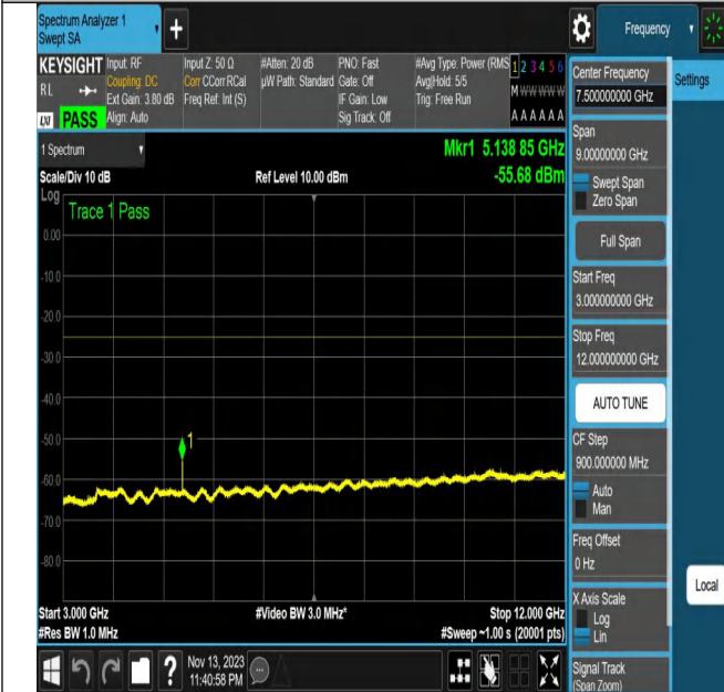
NTNV_N7_PC3_15_20_H_TID18_N/A_3000_12000_#1
