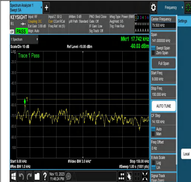
NTNV_N7_PC3_15_20_H_TID24_N/A_0.009_0.15_#1
