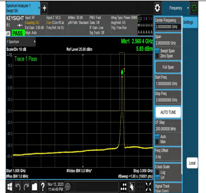
NTNV_N7_PC3_15_20_H_TID22_N/A_1000_3000_#1
