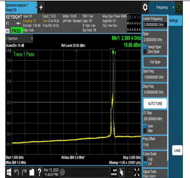
NTNV_N7_PC3_15_20_H_TID18_N/A_1000_3000_#1
