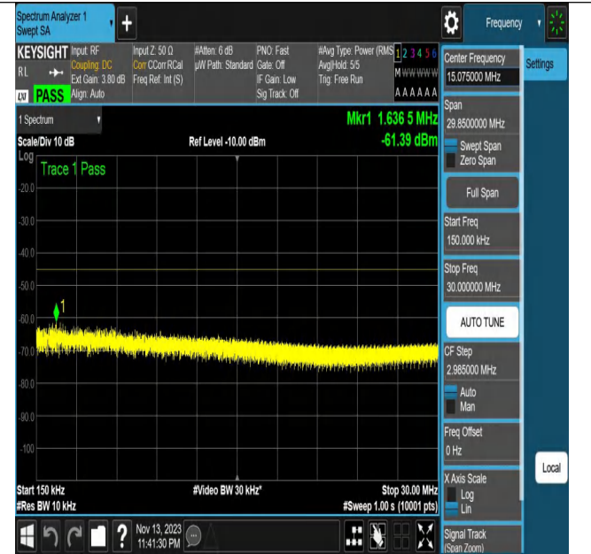
NTNV_N7_PC3_15_20_H_TID19_N/A_0.15_30_#1
