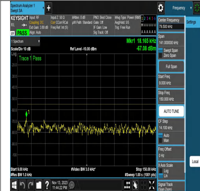
NTNV_N7_PC3_15_20_H_TID22_N/A_0.009_0.15_#1
