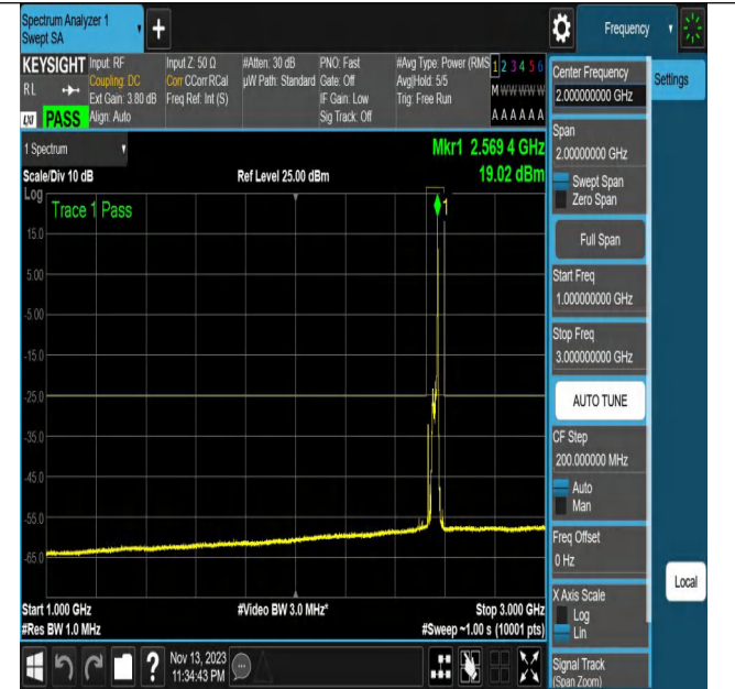
NTNV_N7_PC3_15_20_H_TID12_N/A_1000_3000_#1
