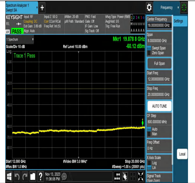
NTNV_N7_PC3_15_20_H_TID13_N/A_12000_20000_#1
