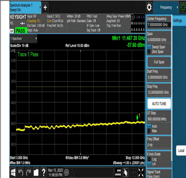
NTNV_N7_PC3_15_20_H_TID14_N/A_3000_12000_#1
