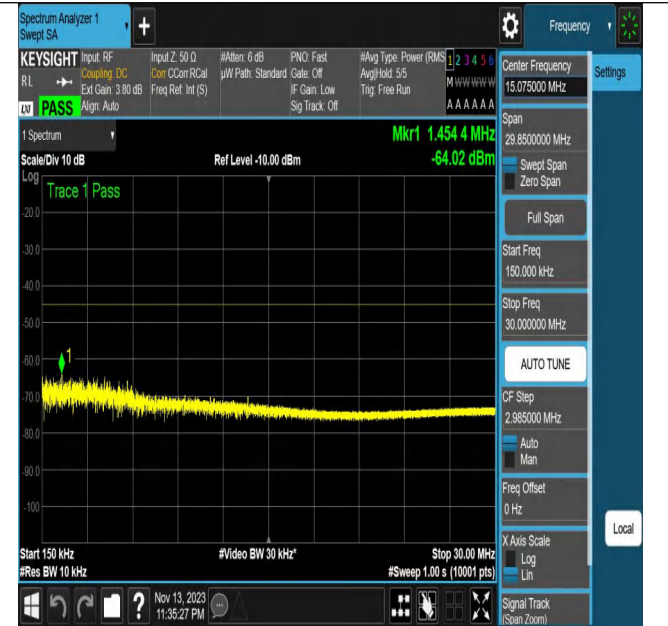
NTNV_N7_PC3_15_20_H_TID13_N/A_0.15_30_#1
