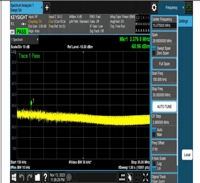
NTNV_N7_PC3_15_20_H_TID16_N/A_0.15_30_#1
