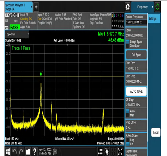
NTNV_N7_PC3_15_20_H_TID12_N/A_0.15_30_#1
