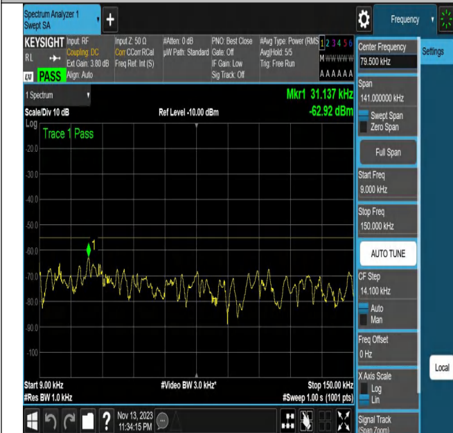
NTNV_N7_PC3_15_20_H_TID12_N/A_0.009_0.15_#1
