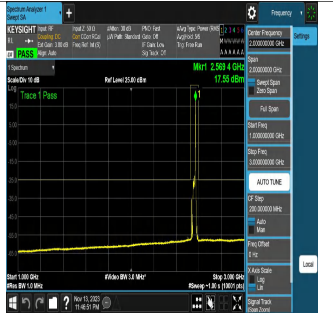
NTNV_N7_PC3_15_20_H_TID24_N/A_1000_3000_#1
