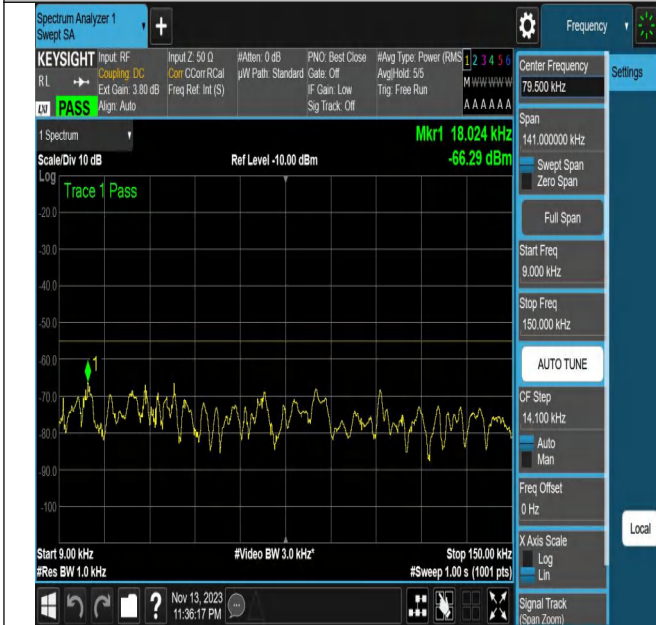
NTNV_N7_PC3_15_20_H_TID14_N/A_0.009_0.15_#1
