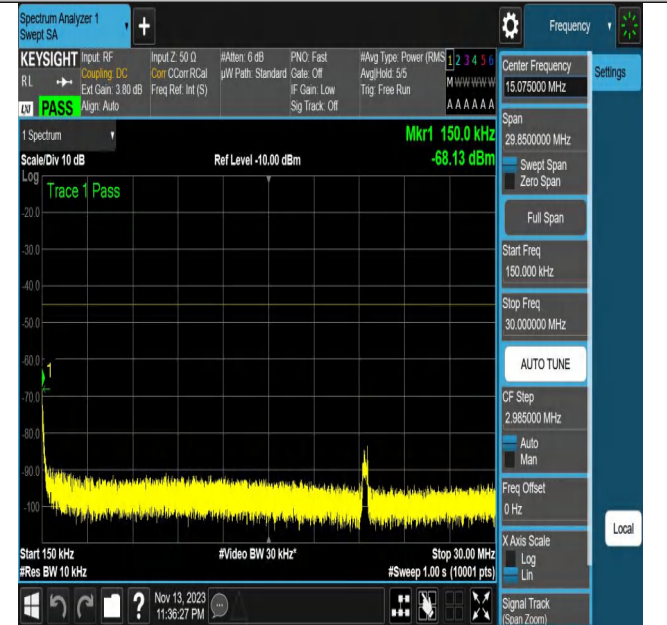
NTNV_N7_PC3_15_20_H_TID14_N/A_0.15_30_#1
