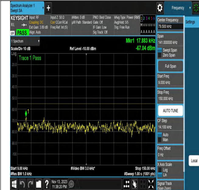
NTNV_N7_PC3_15_20_H_TID16_N/A_0.009_0.15_#1
