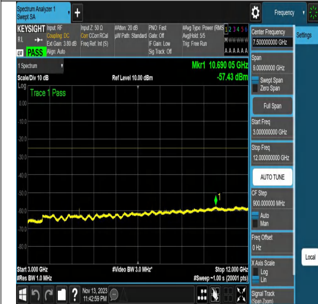
NTNV_N7_PC3_15_20_H_TID20_N/A_3000_12000_#1
