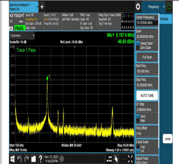
NTNV_N7_PC3_15_20_H_TID18_N/A_0.15_30_#1
