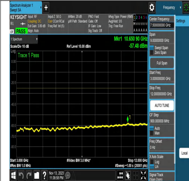
NTNV_N7_PC3_15_20_H_TID16_N/A_3000_12000_#1
