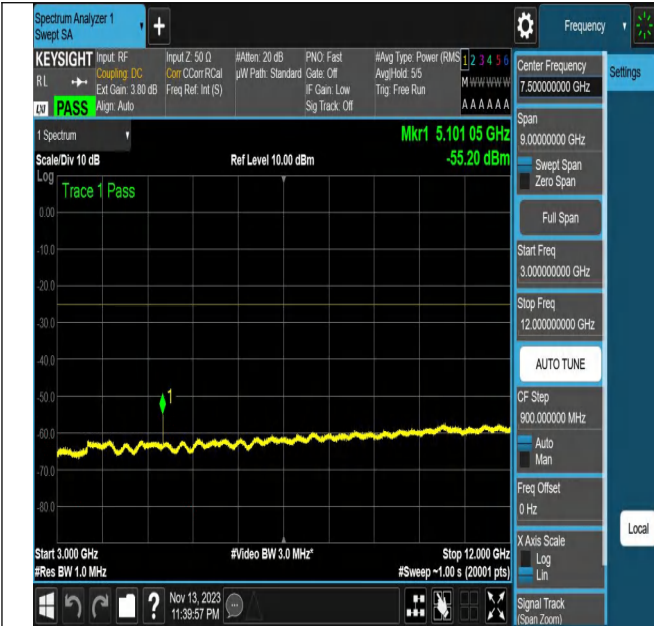
NTNV_N7_PC3_15_20_H_TID17_N/A_3000_12000_#1
