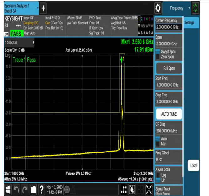
NTNV_N7_PC3_15_20_H_TID20_N/A_1000_3000_#1
