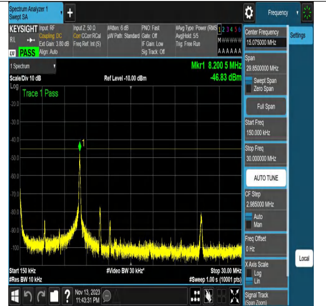
NTNV_N7_PC3_15_20_H_TID21_N/A_0.15_30_#1
