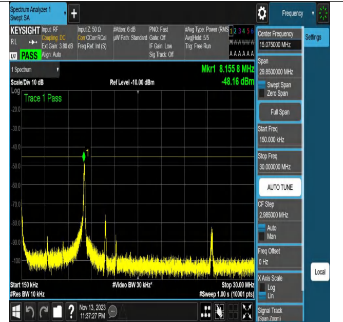
NTNV_N7_PC3_15_20_H_TID15_N/A_0.15_30_#1
