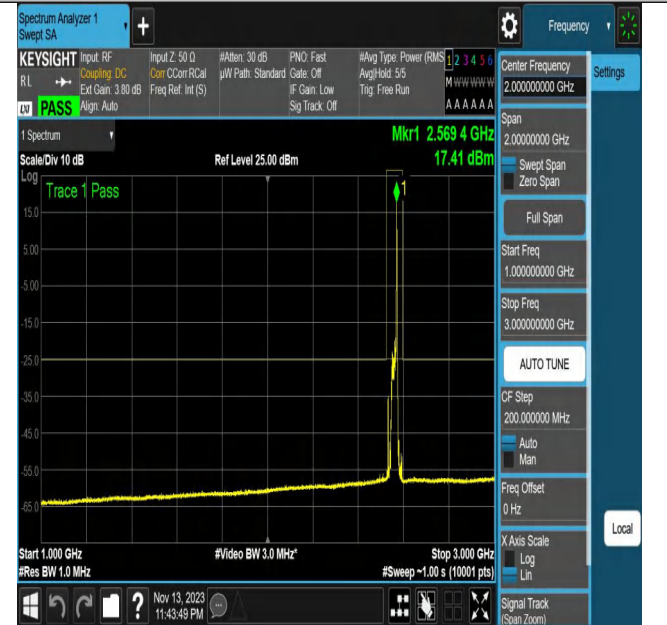
NTNV_N7_PC3_15_20_H_TID21_N/A_1000_3000_#1
