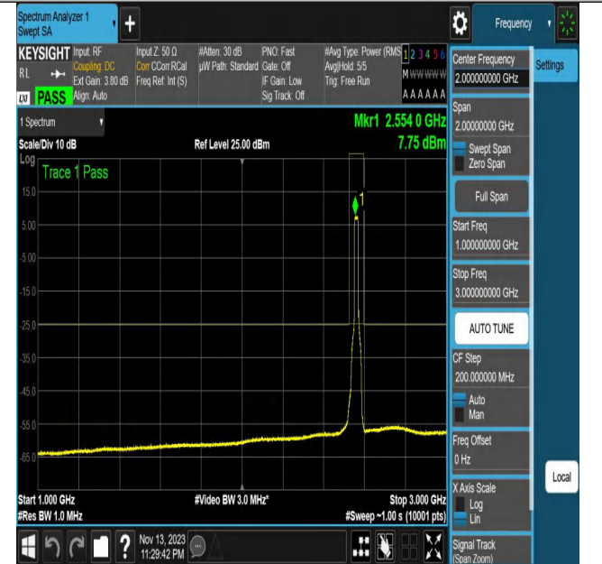
NTNV_N7_PC3_15_20_H_TID7_N/A_1000_3000_#1
