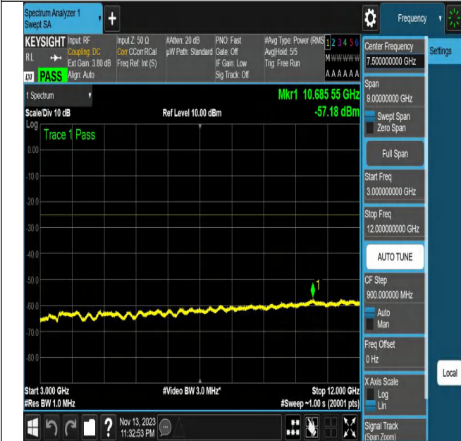
NTNV_N7_PC3_15_20_H_TID10_N/A_3000_12000_#1
