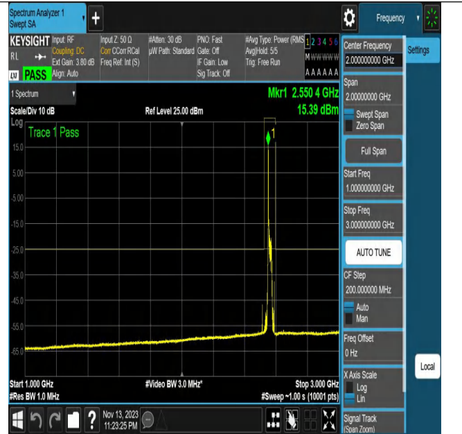
NTNV_N7_PC3_15_20_H_TID2_N/A_1000_3000_#1
