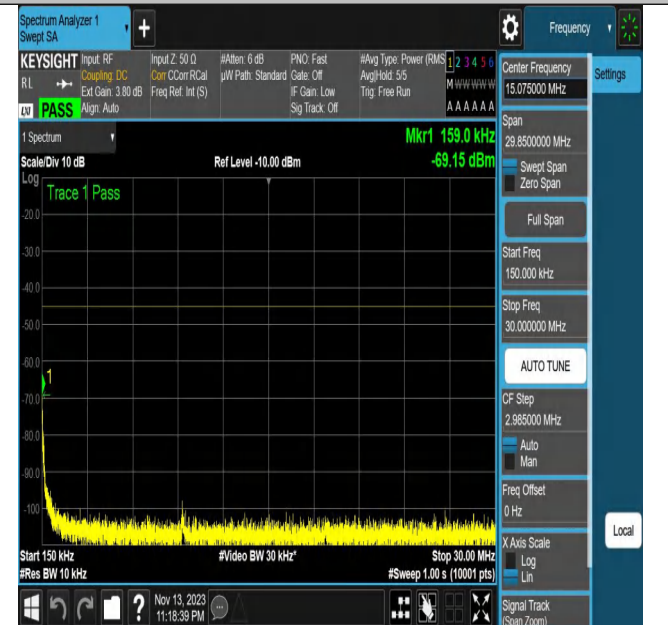
NTNV_N7_PC3_15_20_M_TID27_N/A_0.15_30_#1
