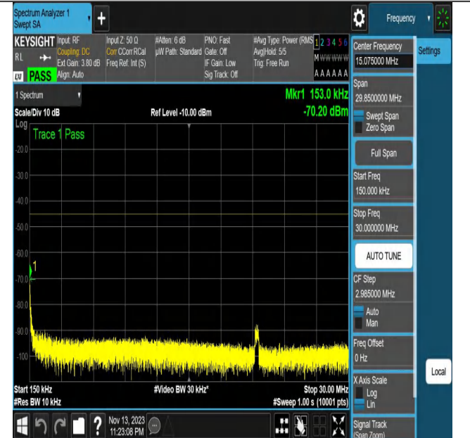
NTNV_N7_PC3_15_20_H_TID2_N/A_0.15_30_#1
