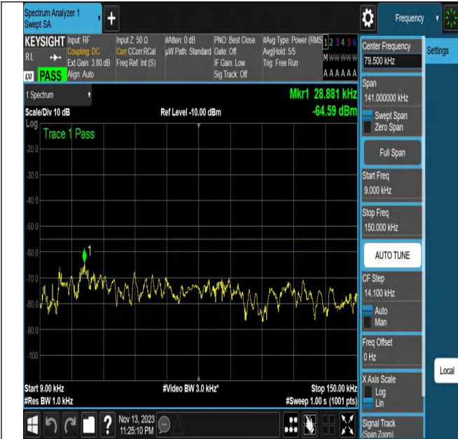
NTNV_N7_PC3_15_20_H_TID3_N/A_0.009_0.15_#1
