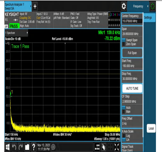
NTNV_N7_PC3_15_20_M_TID26_N/A_0.15_30_#1
