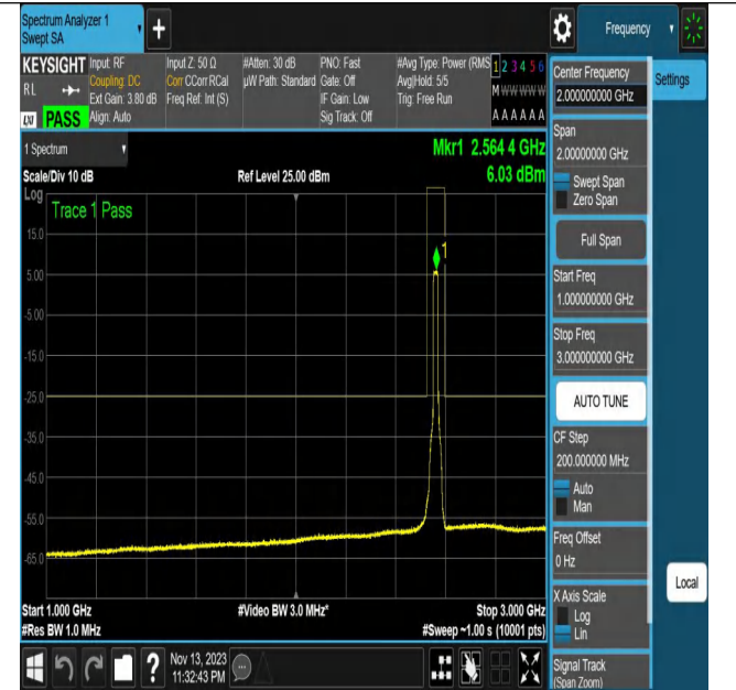
NTNV_N7_PC3_15_20_H_TID10_N/A_1000_3000_#1
