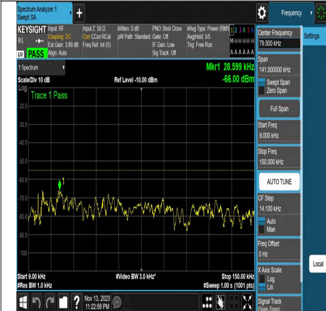
NTNV_N7_PC3_15_20_H_TID2_N/A_0.009_0.15_#1
