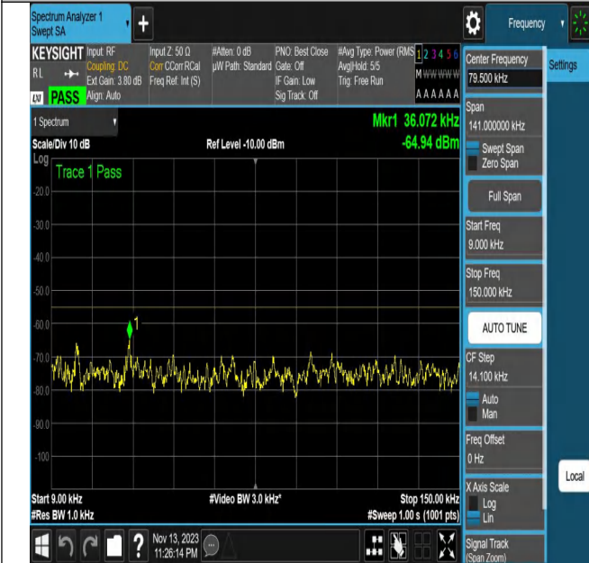
NTNV_N7_PC3_15_20_H_TID4_N/A_0.009_0.15_#1
