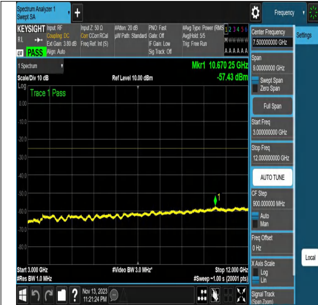
NTNV_N7_PC3_15_20_H_TID1_N/A_3000_12000_#1
