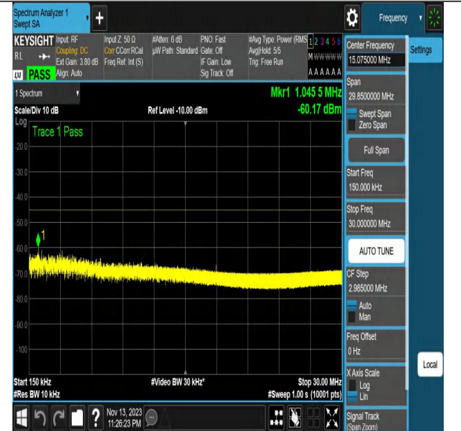
NTNV_N7_PC3_15_20_H_TID4_N/A_0.15_30_#1
