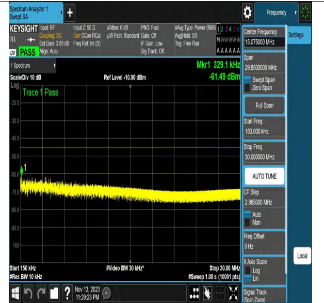
NTNV_N7_PC3_15_20_H_TID7_N/A_0.15_30_#1
