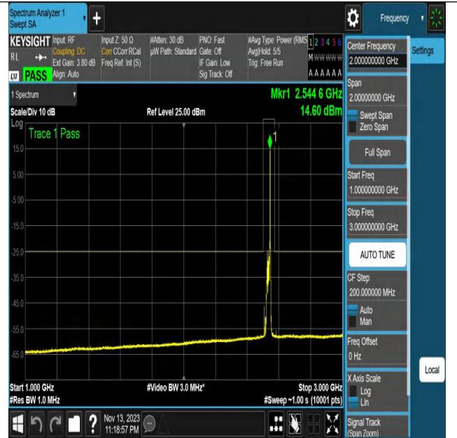
NTNV_N7_PC3_15_20_M_TID27_N/A_1000_3000_#1
