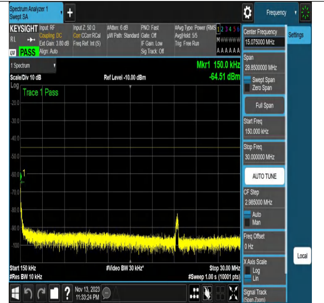
NTNV_N7_PC3_15_20_H_TID11_N/A_0.15_30_#1
