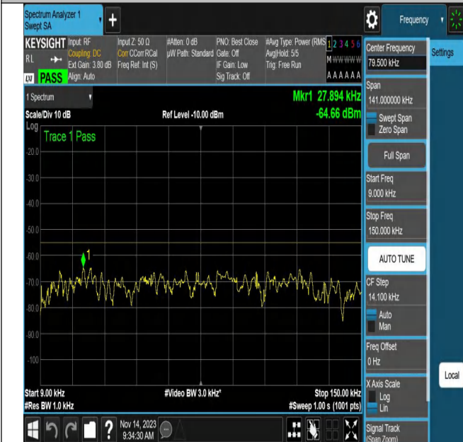
NTNV_N7_PC3_15_20_H_TID6_N/A_0.009_0.15_#1
