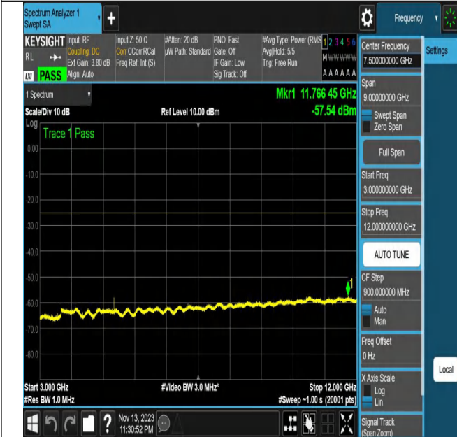
NTNV_N7_PC3_15_20_H_TID8_N/A_3000_12000_#1
