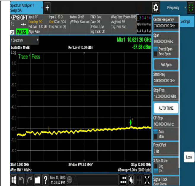
NTNV_N7_PC3_15_20_H_TID9_N/A_3000_12000_#1
