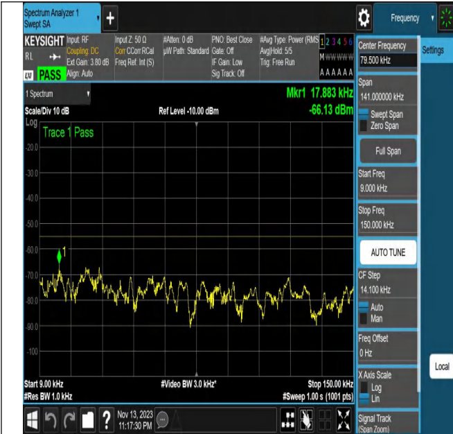
NTNV_N7_PC3_15_20_M_TID26_N/A_0.009_0.15_#1
