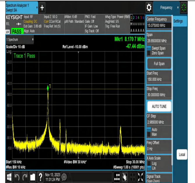
NTNV_N7_PC3_15_20_H_TID9_N/A_0.15_30_#1
