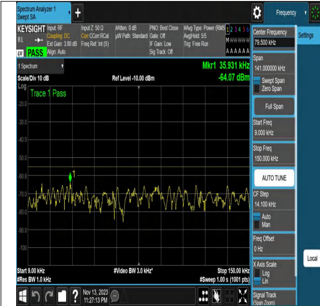
NTNV_N7_PC3_15_20_H_TID5_N/A_0.009_0.15_#1
