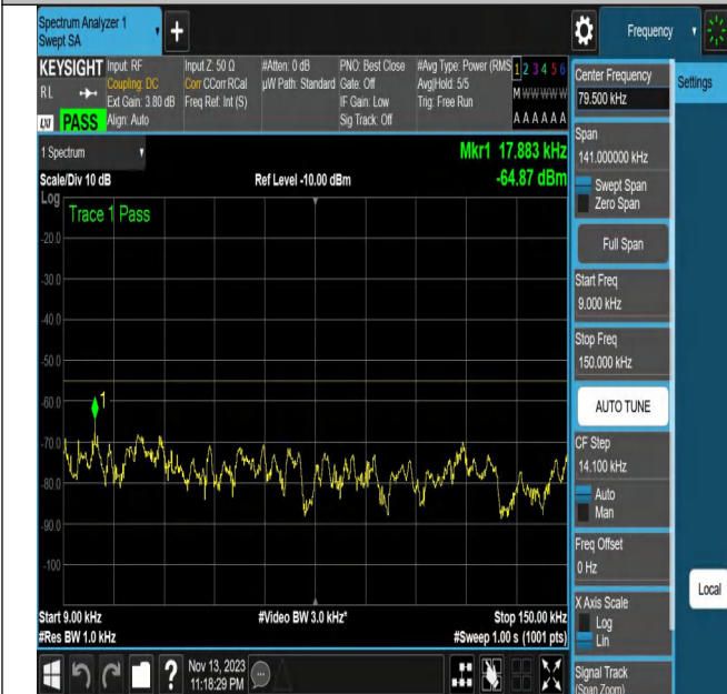
NTNV_N7_PC3_15_20_M_TID27_N/A_0.009_0.15_#1
