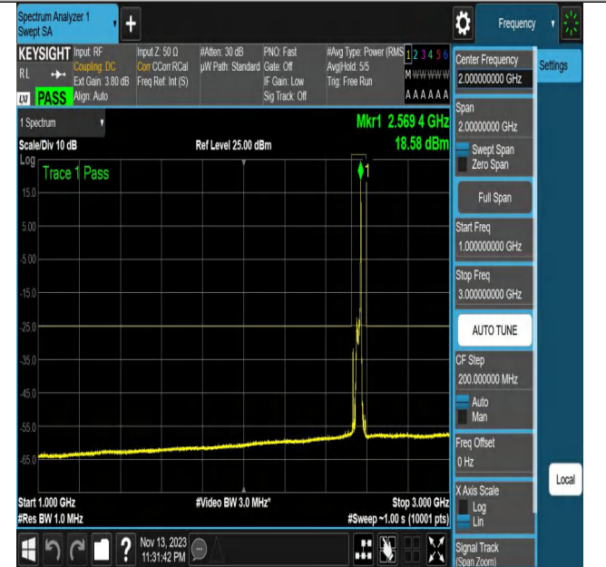
NTNV_N7_PC3_15_20_H_TID9_N/A_1000_3000_#1
