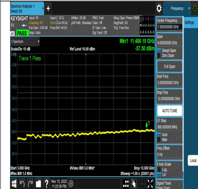
NTNV_N7_PC3_15_20_H_TID2_N/A_3000_12000_#1
