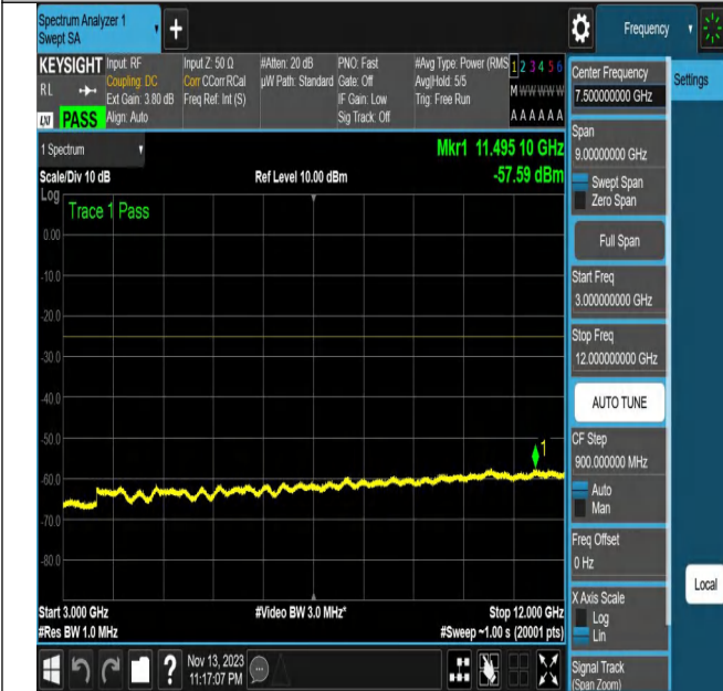
NTNV_N7_PC3_15_20_M_TID25_N/A_3000_12000_#1
