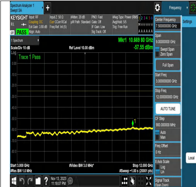
NTNV_N7_PC3_15_20_M_TID26_N/A_3000_12000_#1
