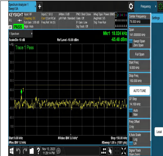
NTNV_N7_PC3_15_20_H_TID7_N/A_0.009_0.15_#1
