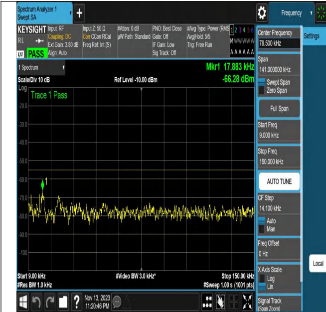
NTNV_N7_PC3_15_20_H_TID1_N/A_0.009_0.15_#1
