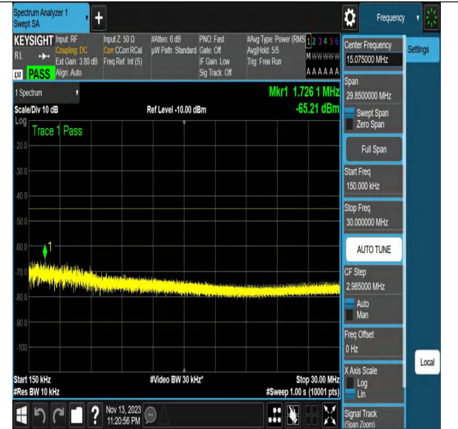
NTNV_N7_PC3_15_20_H_TID1_N/A_0.15_30_#1
