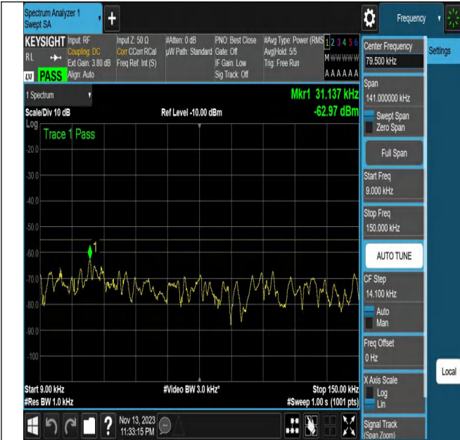
NTNV_N7_PC3_15_20_H_TID11_N/A_0.009_0.15_#1
