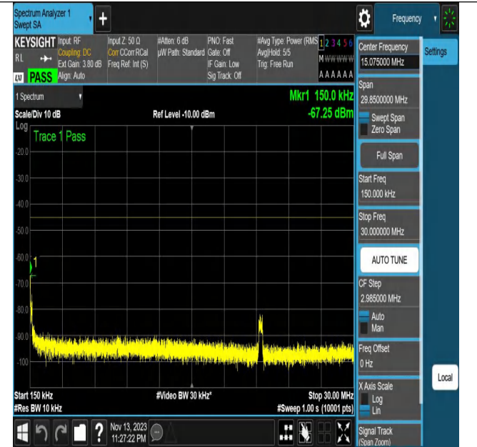
NTNV_N7_PC3_15_20_H_TID5_N/A_0.15_30_#1
