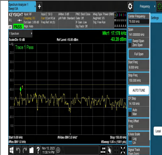
NTNV_N7_PC3_15_20_H_TID8_N/A_0.009_0.15_#1
