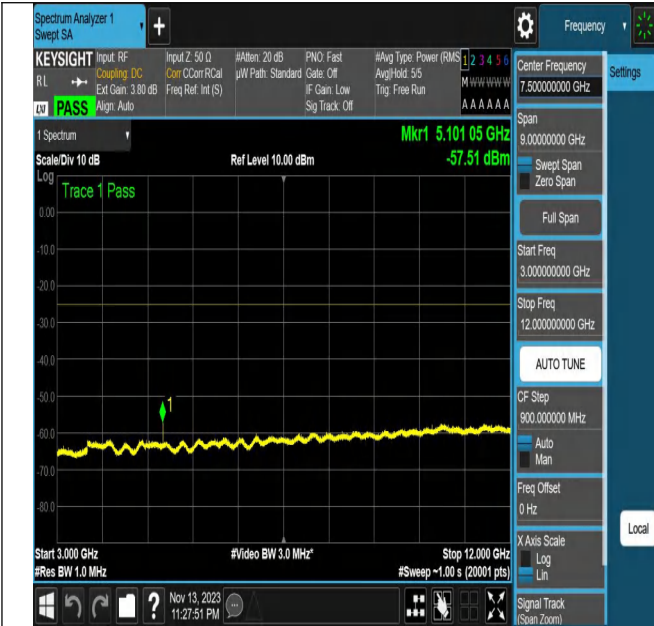
NTNV_N7_PC3_15_20_H_TID5_N/A_3000_12000_#1
