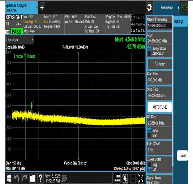
NTNV_N7_PC3_15_20_H_TID10_N/A_0.15_30_#1
