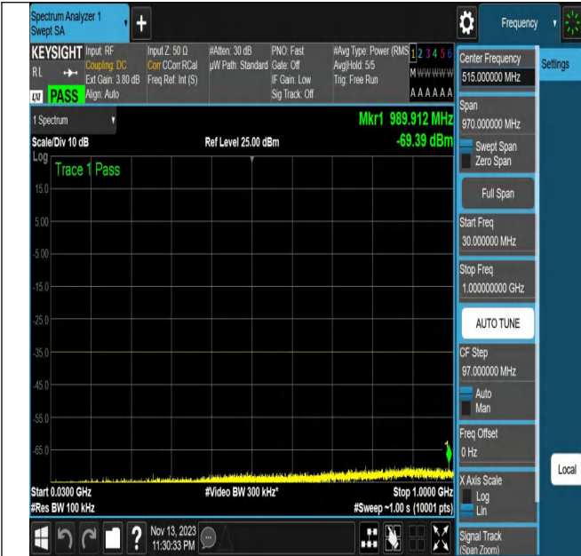
NTNV_N7_PC3_15_20_H_TID8_N/A_30_1000_#1
