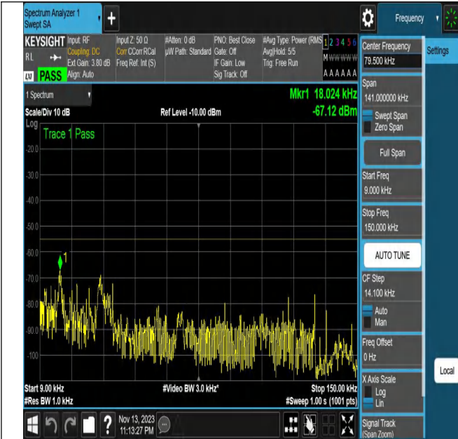
NTNV_N7_PC3_15_20_M_TID22_N/A_0.009_0.15_#1
