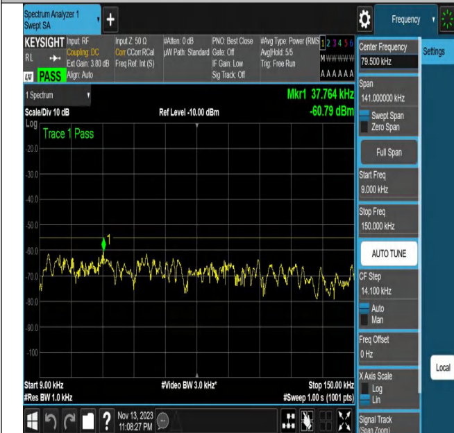
NTNV_N7_PC3_15_20_M_TID17_N/A_0.009_0.15_#1
