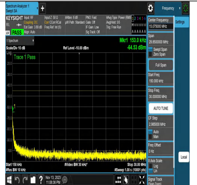
NTNV_N7_PC3_15_20_M_TID17_N/A_0.15_30_#1
