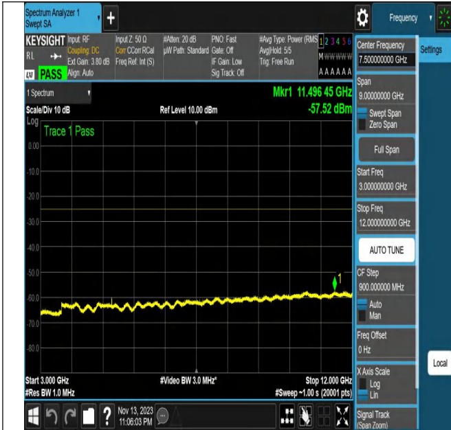
NTNV_N7_PC3_15_20_M_TID14_N/A_3000_12000_#1
