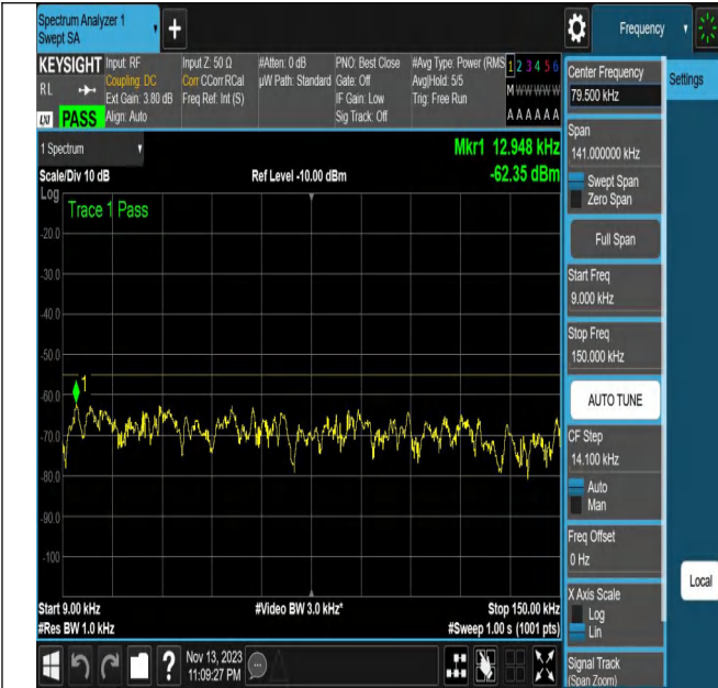
NTNV_N7_PC3_15_20_M_TID18_N/A_0.009_0.15_#1
