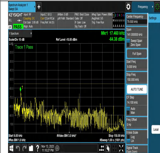
NTNV_N7_PC3_15_20_M_TID19_N/A_0.009_0.15_#1
