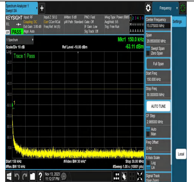
NTNV_N7_PC3_15_20_M_TID21_N/A_0.15_30_#1
