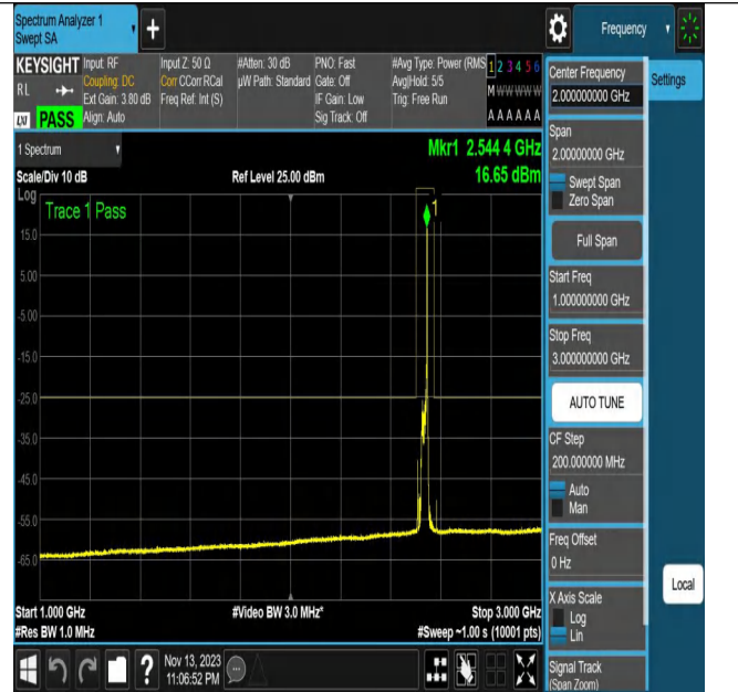
NTNV_N7_PC3_15_20_M_TID15_N/A_1000_3000_#1
