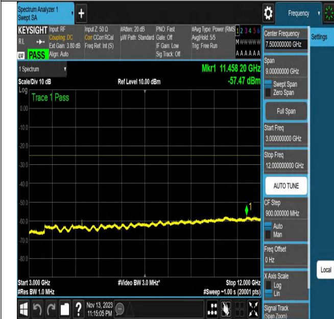
NTNV_N7_PC3_15_20_M_TID23_N/A_3000_12000_#1
