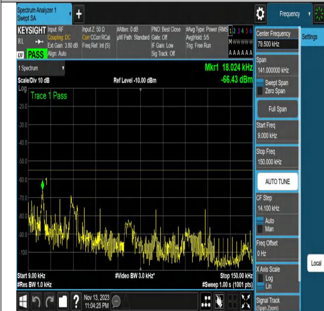
NTNV_N7_PC3_15_20_M_TID13_N/A_0.009_0.15_#1
