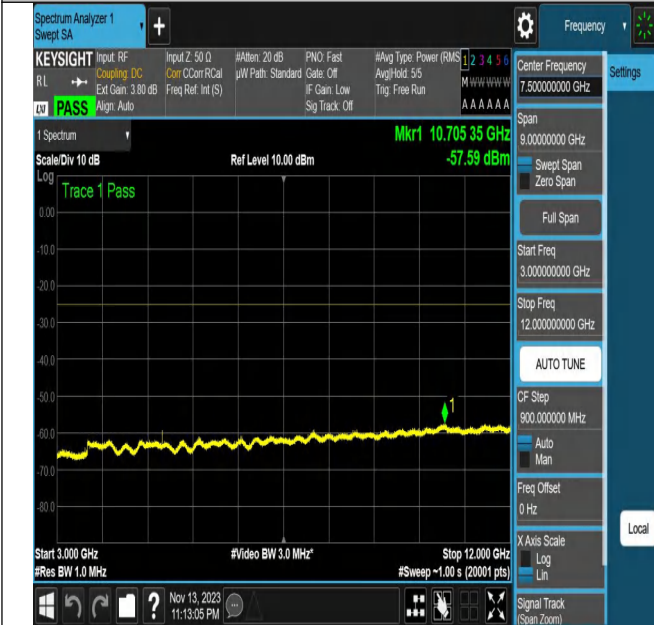
NTNV_N7_PC3_15_20_M_TID21_N/A_3000_12000_#1
