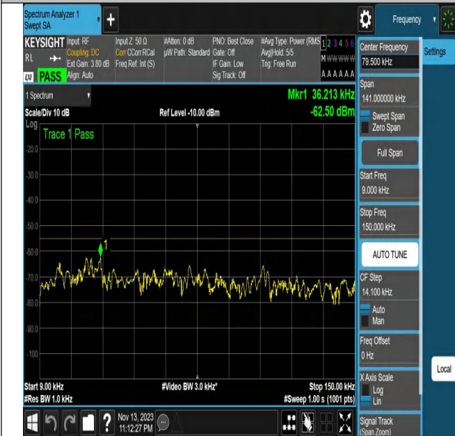
NTNV_N7_PC3_15_20_M_TID21_N/A_0.009_0.15_#1
