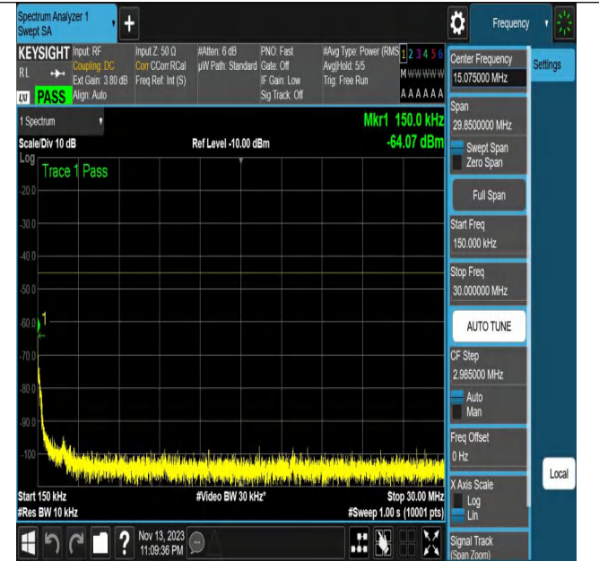
NTNV_N7_PC3_15_20_M_TID18_N/A_0.15_30_#1
