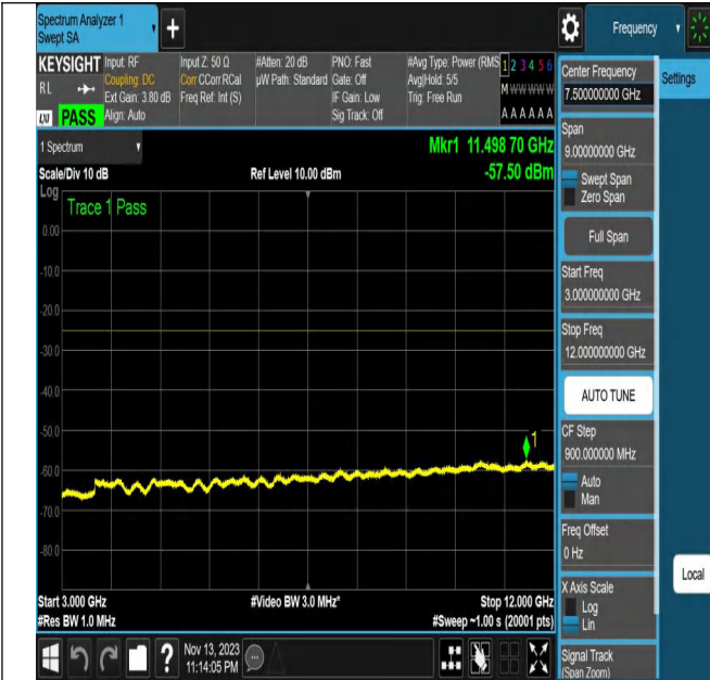
NTNV_N7_PC3_15_20_M_TID22_N/A_3000_12000_#1
