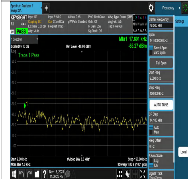
NTNV_N7_PC3_15_20_M_TID15_N/A_0.009_0.15_#1
