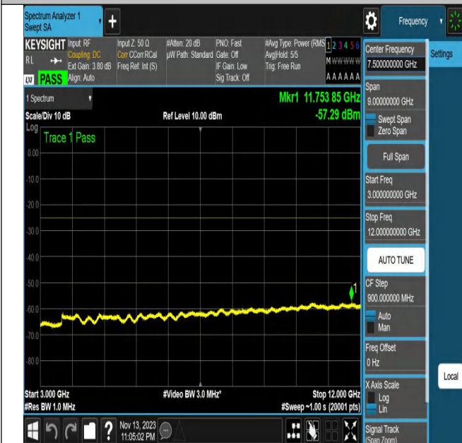
NTNV_N7_PC3_15_20_M_TID13_N/A_3000_12000_#1
