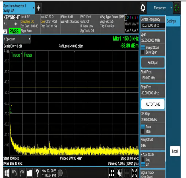
NTNV_N7_PC3_15_20_M_TID15_N/A_0.15_30_#1
