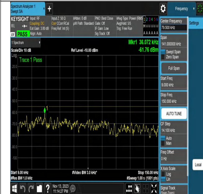
NTNV_N7_PC3_15_20_M_TID23_N/A_0.009_0.15_#1
