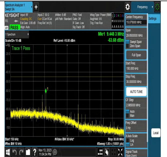
NTNV_N7_PC3_15_20_M_TID13_N/A_0.15_30_#1
