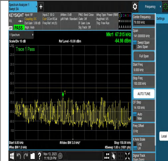
NTNV_N7_PC3_15_20_M_TID25_N/A_0.009_0.15_#1
