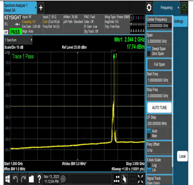
NTNV_N7_PC3_15_20_M_TID21_N/A_1000_3000_#1
