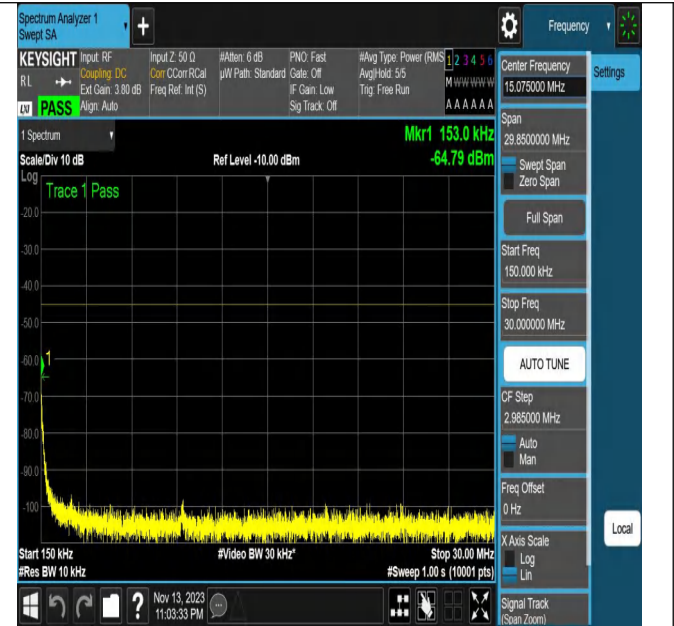
NTNV_N7_PC3_15_20_M_TID12_N/A_0.15_30_#1
