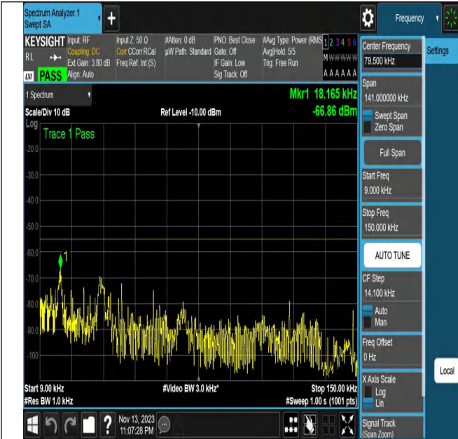
NTNV_N7_PC3_15_20_M_TID16_N/A_0.009_0.15_#1
