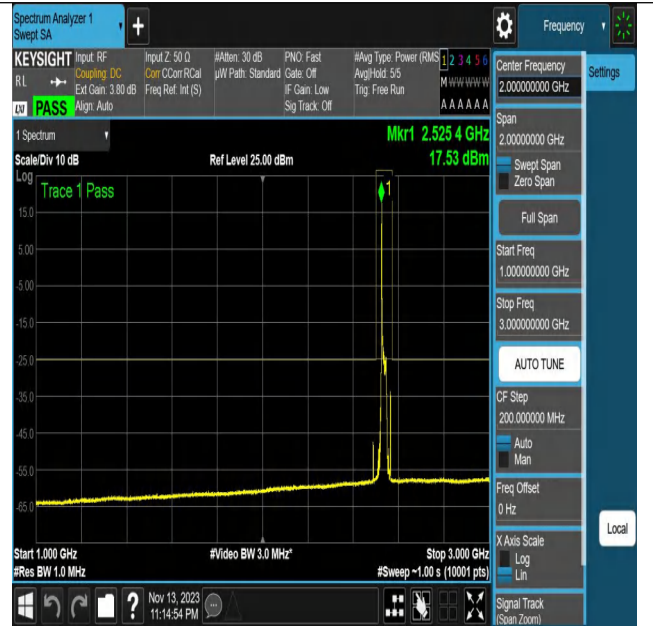
NTNV_N7_PC3_15_20_M_TID23_N/A_1000_3000_#1
