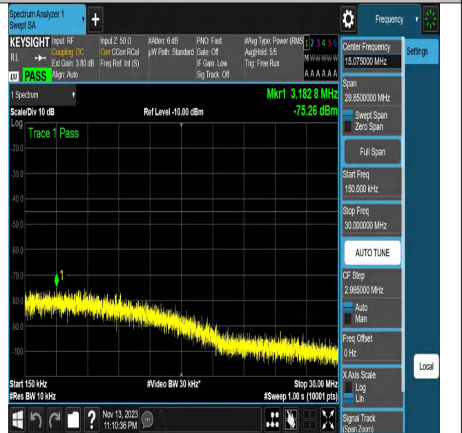
NTNV_N7_PC3_15_20_M_TID19_N/A_0.15_30_#1
