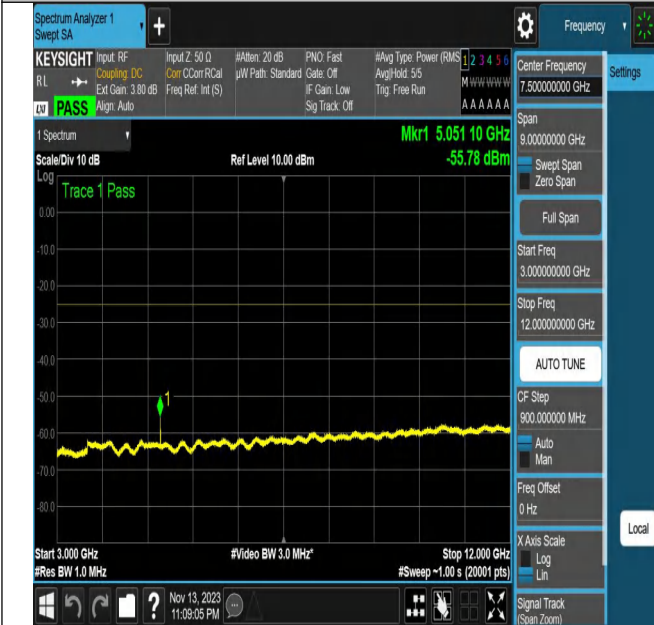
NTNV_N7_PC3_15_20_M_TID17_N/A_3000_12000_#1
