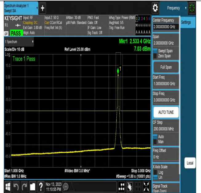
NTNV_N7_PC3_15_20_M_TID19_N/A_1000_3000_#1
