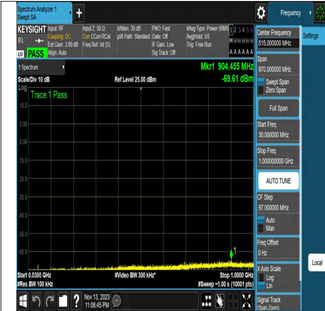
NTNV_N7_PC3_15_20_M_TID17_N/A_30_1000_#1
