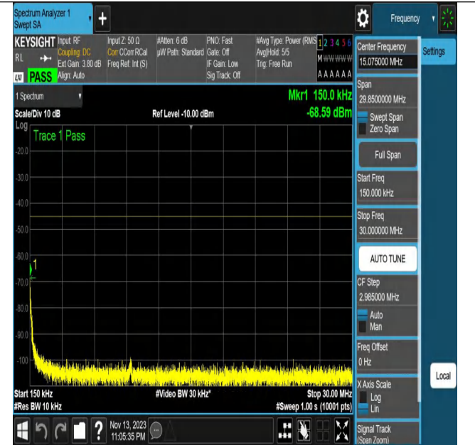
NTNV_N7_PC3_15_20_M_TID14_N/A_0.15_30_#1
