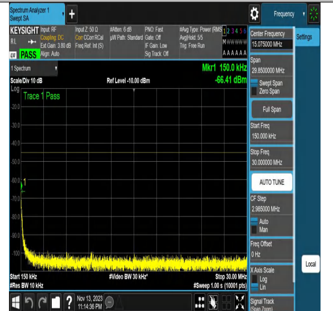
NTNV_N7_PC3_15_20_M_TID23_N/A_0.15_30_#1
