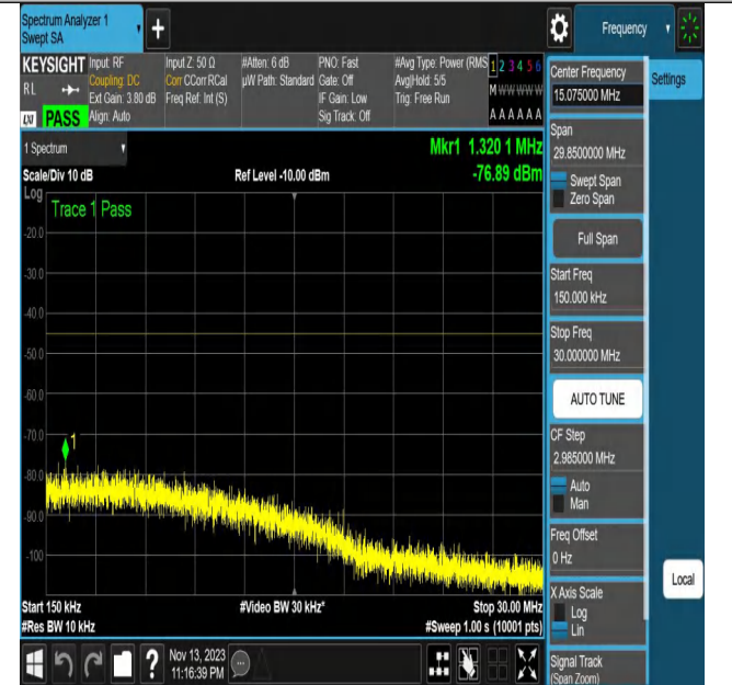
NTNV_N7_PC3_15_20_M_TID25_N/A_0.15_30_#1
