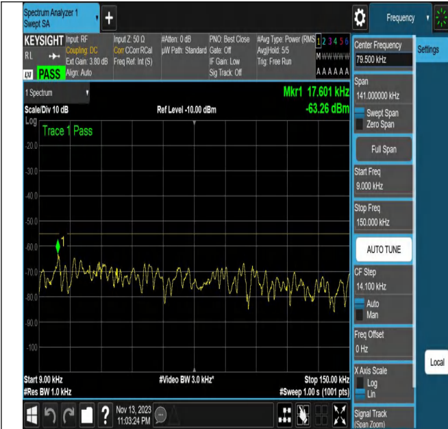
NTNV_N7_PC3_15_20_M_TID12_N/A_0.009_0.15_#1
