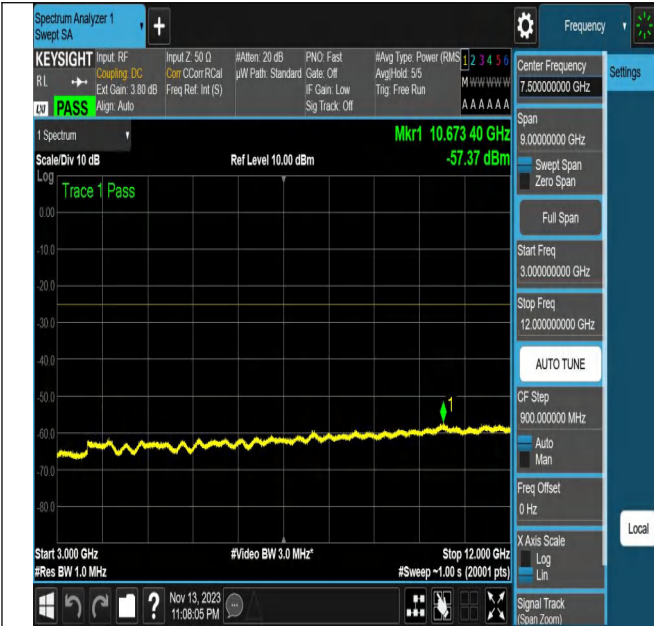
NTNV_N7_PC3_15_20_M_TID16_N/A_3000_12000_#1
