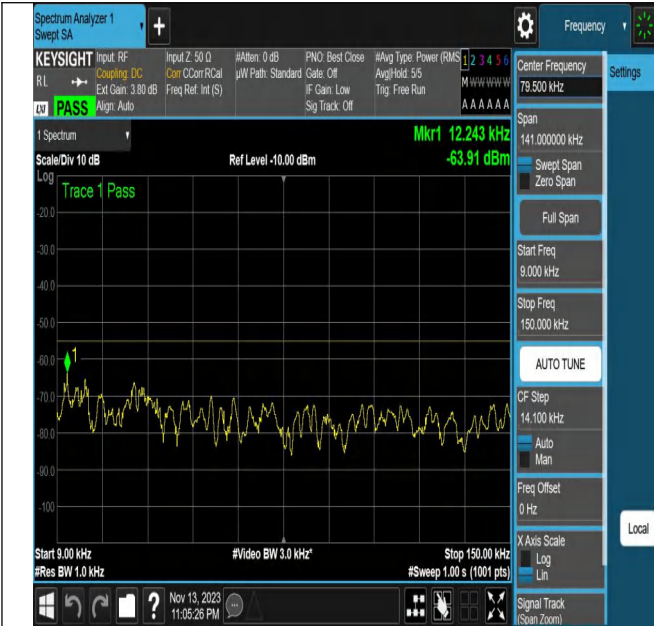
NTNV_N7_PC3_15_20_M_TID14_N/A_0.009_0.15_#1
