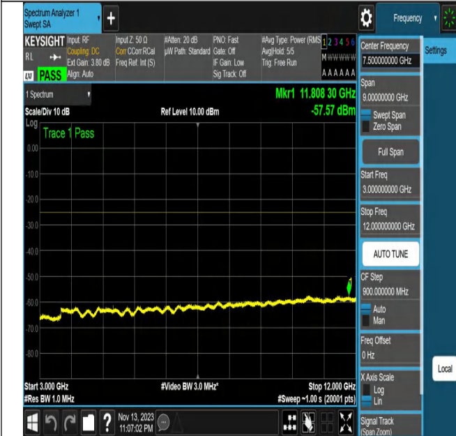
NTNV_N7_PC3_15_20_M_TID15_N/A_3000_12000_#1
