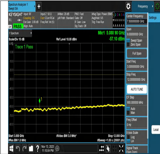
NTNV_N7_PC3_15_20_M_TID18_N/A_3000_12000_#1
