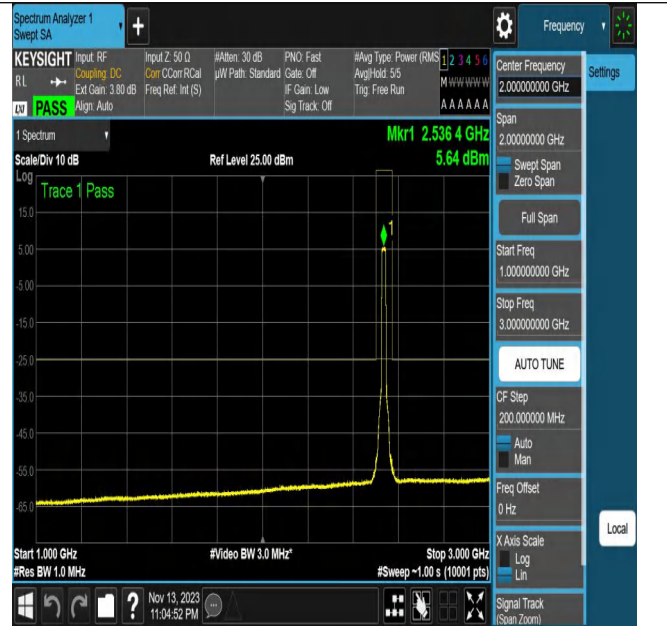
NTNV_N7_PC3_15_20_M_TID13_N/A_1000_3000_#1
