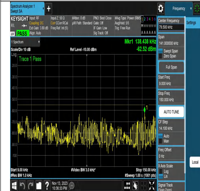
NTNV_N7_PC3_15_20_L_TID16_N/A_0.009_0.15_#1
