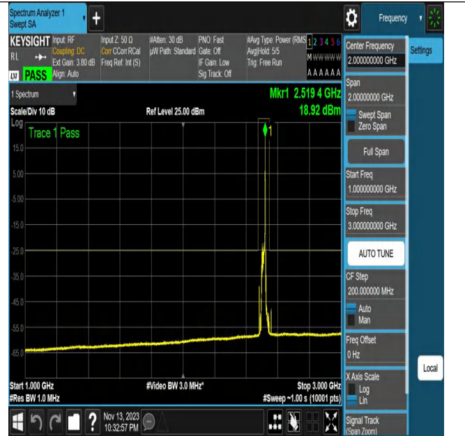
NTNV_N7_PC3_15_20_L_TID12_N/A_1000_3000_#1
