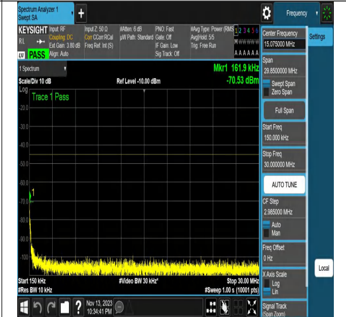
NTNV_N7_PC3_15_20_L_TID14_N/A_0.15_30_#1
