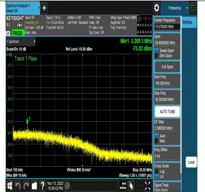
NTNV_N7_PC3_15_20_L_TID19_N/A_0.15_30_#1
