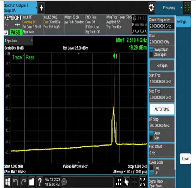
NTNV_N7_PC3_15_20_L_TID18_N/A_1000_3000_#1
