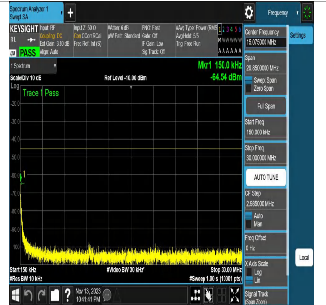
NTNV_N7_PC3_15_20_L_TID21_N/A_0.15_30_#1
