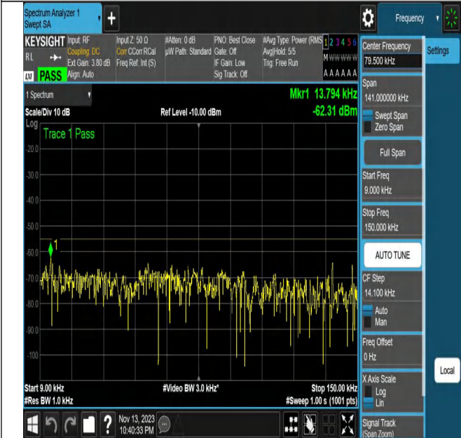
NTNV_N7_PC3_15_20_L_TID20_N/A_0.009_0.15_#1
