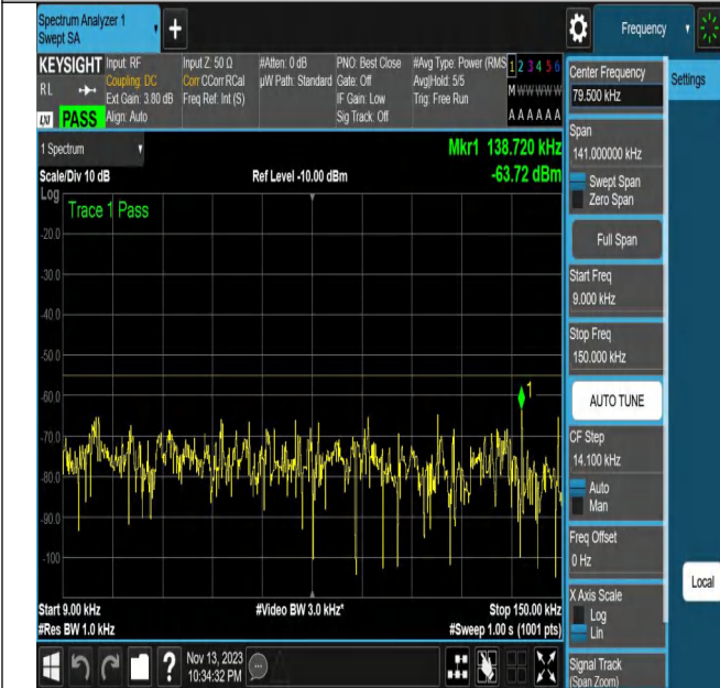
NTNV_N7_PC3_15_20_L_TID14_N/A_0.009_0.15_#1
