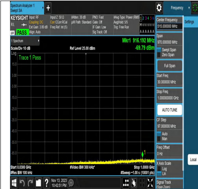
NTNV_N7_PC3_15_20_L_TID22_N/A_30_1000_#1
