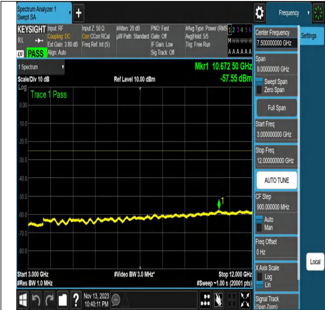
NTNV_N7_PC3_15_20_L_TID19_N/A_3000_12000_#1
