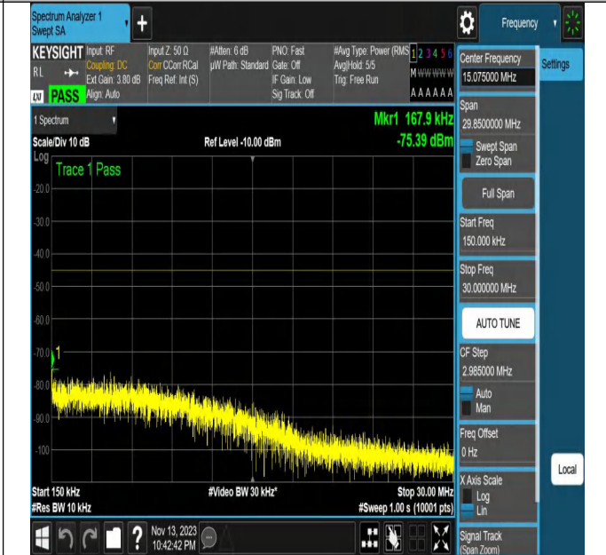
NTNV_N7_PC3_15_20_L_TID22_N/A_0.15_30_#1
