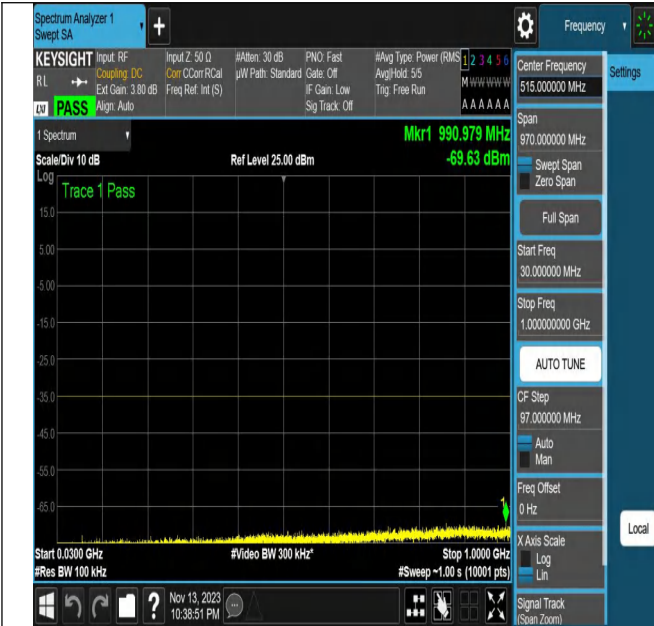
NTNV_N7_PC3_15_20_L_TID18_N/A_30_1000_#1
