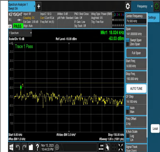
NTNV_N7_PC3_15_20_L_TID24_N/A_0.009_0.15_#1
