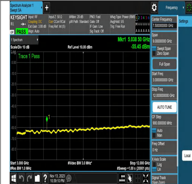
NTNV_N7_PC3_15_20_L_TID18_N/A_3000_12000_#1
