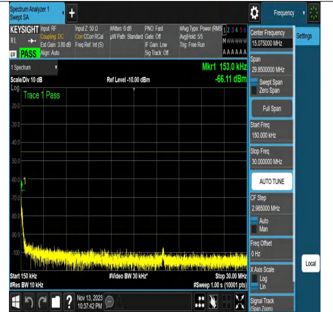
NTNV_N7_PC3_15_20_L_TID17_N/A_0.15_30_#1
