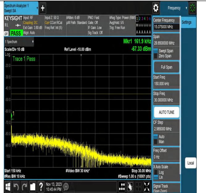
NTNV_N7_PC3_15_20_L_TID25_N/A_0.15_30_#1
