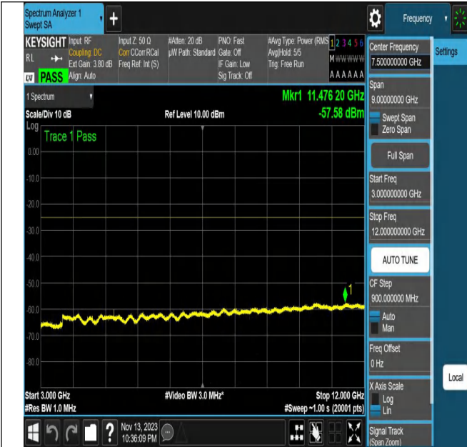
NTNV_N7_PC3_15_20_L_TID15_N/A_3000_12000_#1
