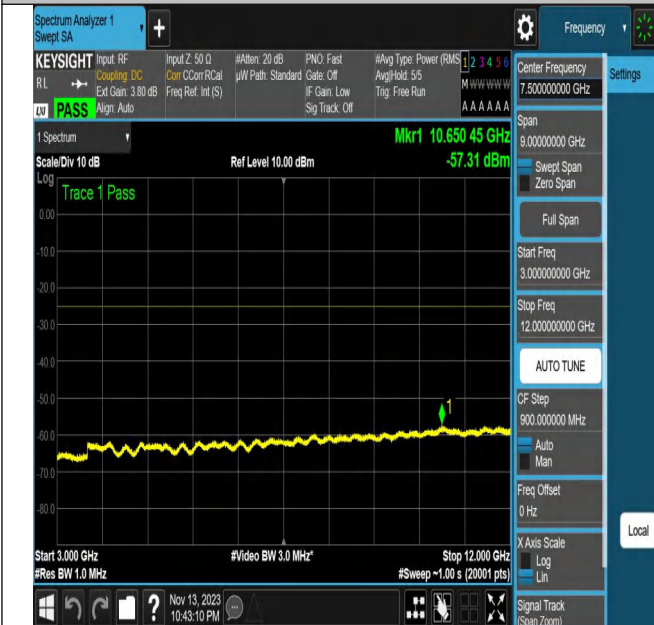
NTNV_N7_PC3_15_20_L_TID22_N/A_3000_12000_#1
