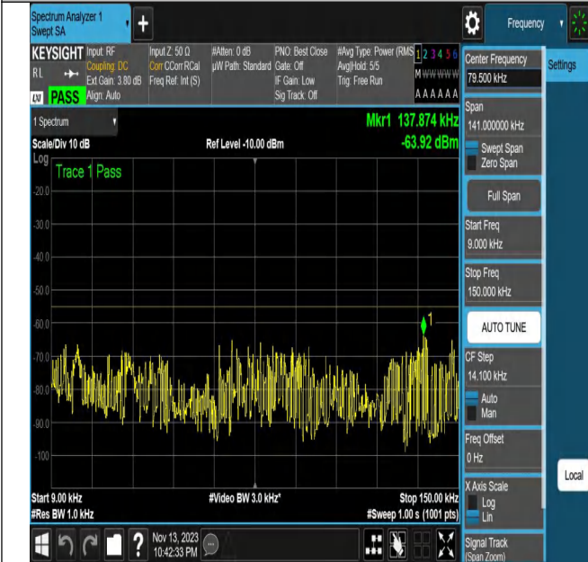
NTNV_N7_PC3_15_20_L_TID22_N/A_0.009_0.15_#1
