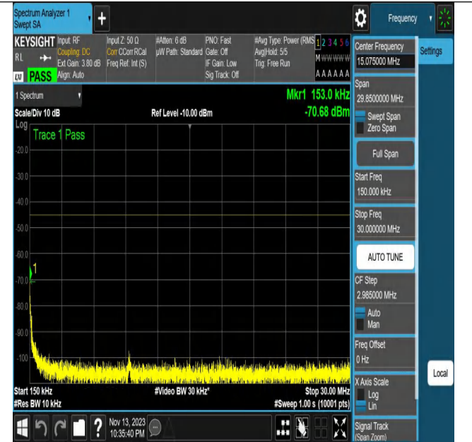
NTNV_N7_PC3_15_20_L_TID15_N/A_0.15_30_#1
