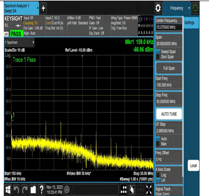
NTNV_N7_PC3_15_20_L_TID13_N/A_0.15_30_#1
