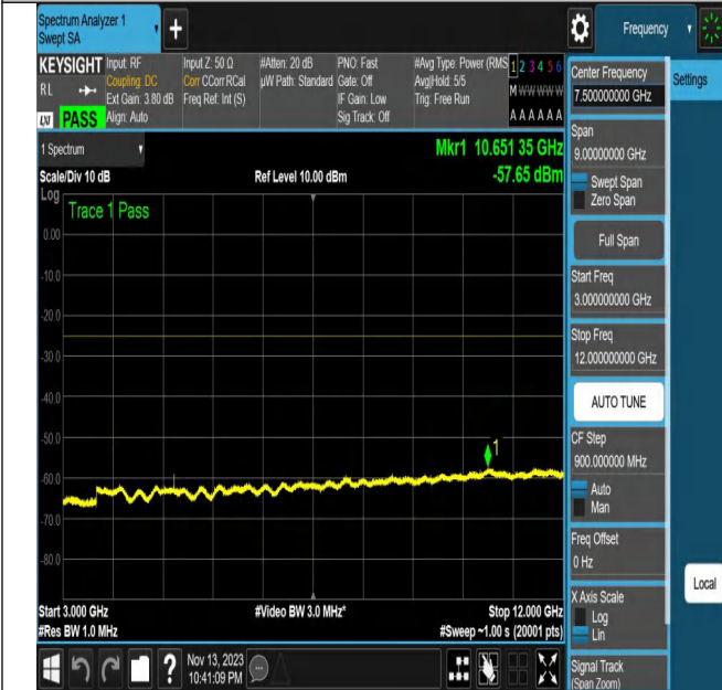
NTNV_N7_PC3_15_20_L_TID20_N/A_3000_12000_#1
