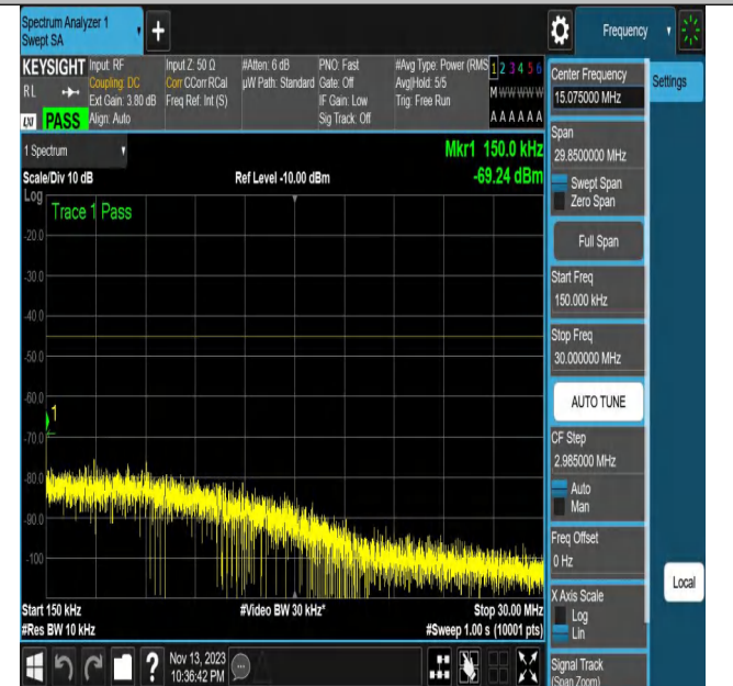
NTNV_N7_PC3_15_20_L_TID16_N/A_0.15_30_#1
