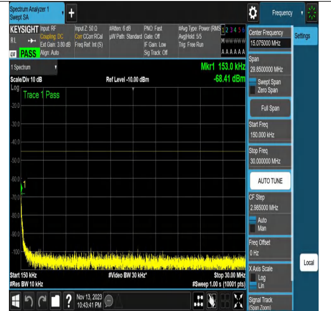
NTNV_N7_PC3_15_20_L_TID23_N/A_0.15_30_#1
