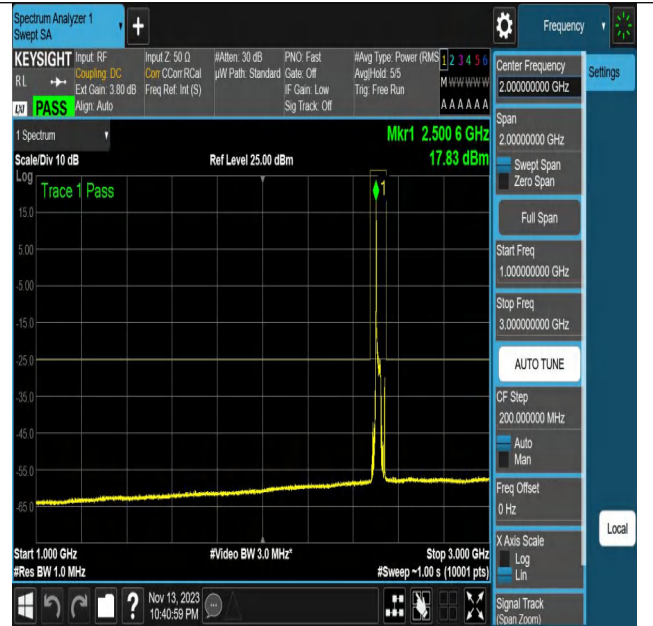
NTNV_N7_PC3_15_20_L_TID20_N/A_1000_3000_#1
