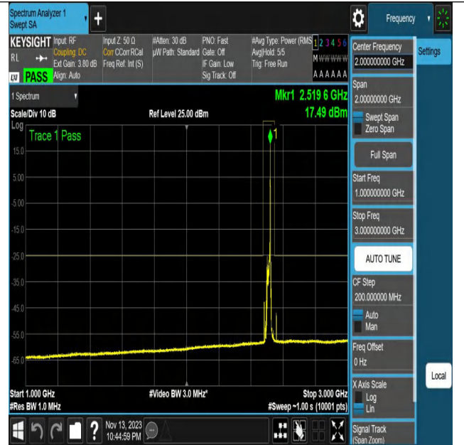
NTNV_N7_PC3_15_20_L_TID24_N/A_1000_3000_#1
