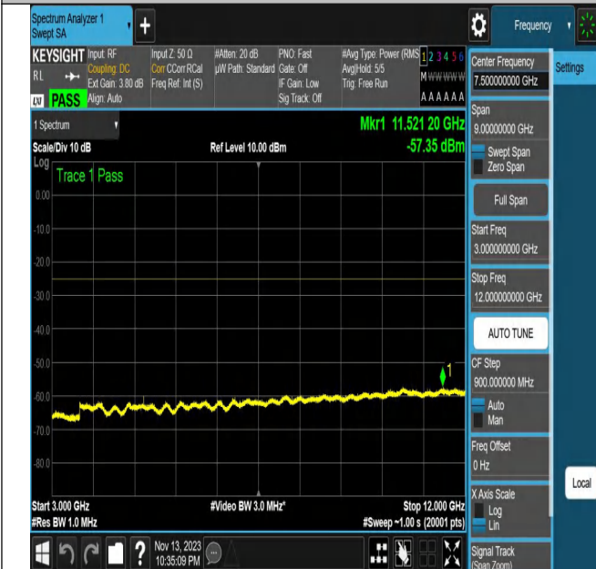
NTNV_N7_PC3_15_20_L_TID14_N/A_3000_12000_#1
