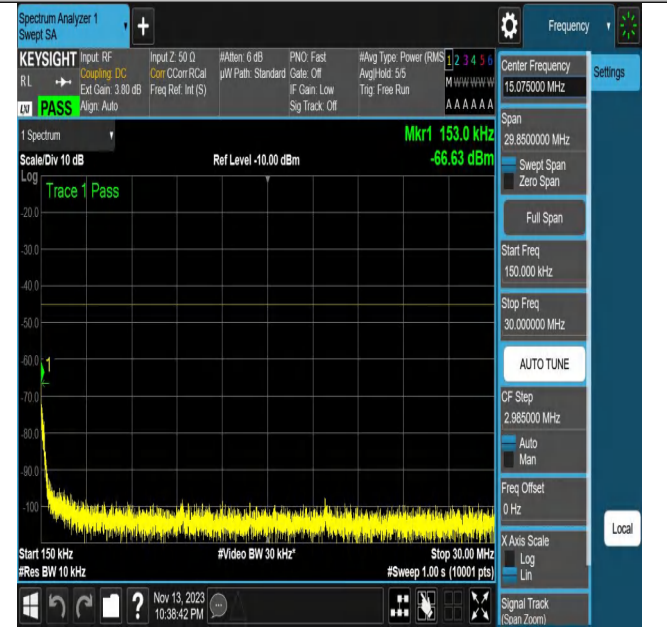
NTNV_N7_PC3_15_20_L_TID18_N/A_0.15_30_#1
