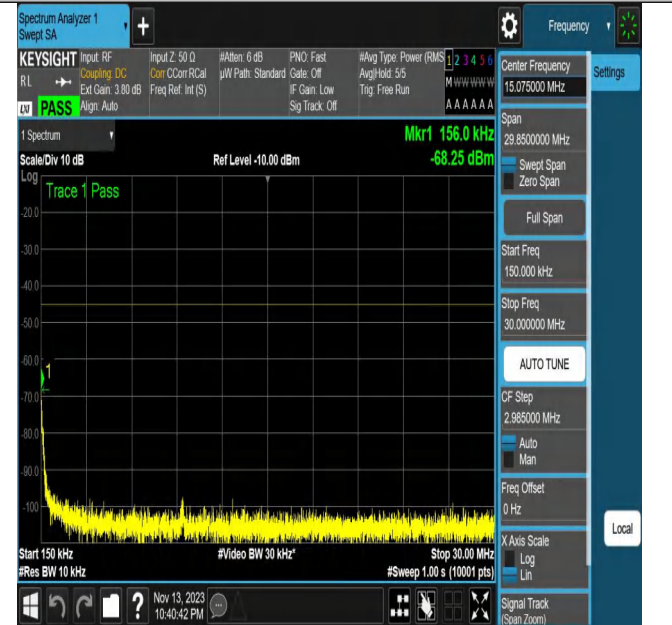
NTNV_N7_PC3_15_20_L_TID20_N/A_0.15_30_#1
