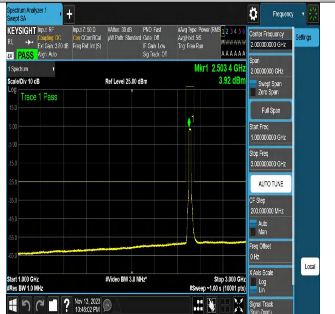
NTNV_N7_PC3_15_20_L_TID25_N/A_1000_3000_#1
