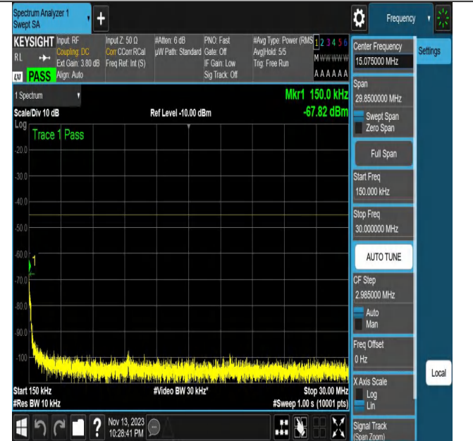
NTNV_N7_PC3_15_20_L_TID8_N/A_0.15_30_#1
