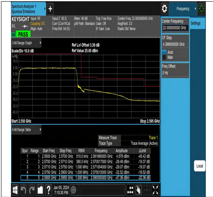
NTVN_N7_PC3_15_20_H_TID10_#1
