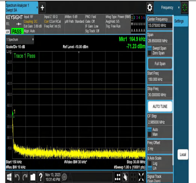
NTNV_N7_PC3_15_20_L_TID11_N/A_0.15_30_#1
