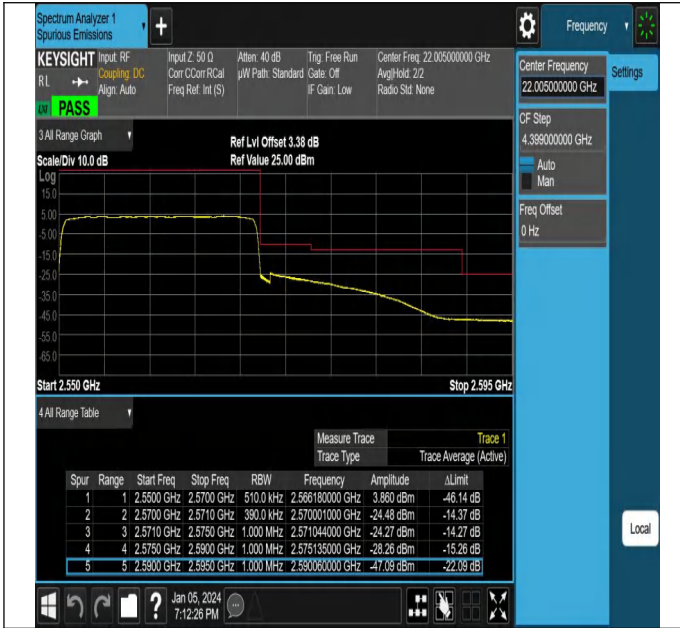
NTVN_N7_PC3_15_20_H_TID22_#1
