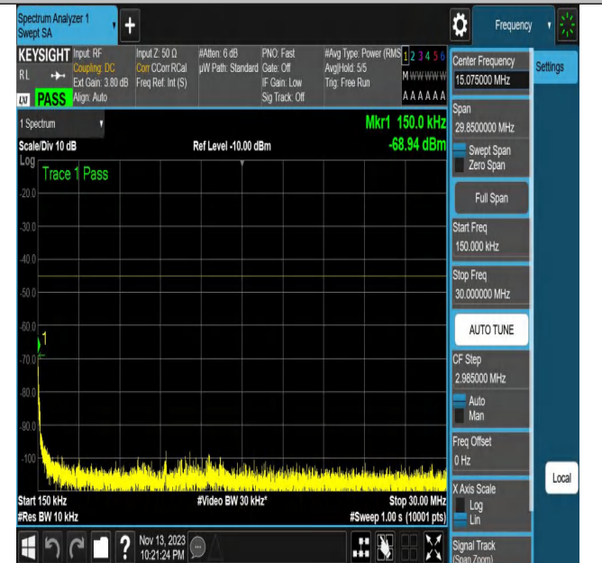
NTNV_N7_PC3_15_20_L_TID2_N/A_0.15_30_#1
