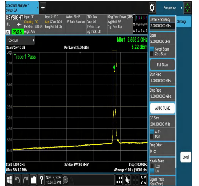
NTNV_N7_PC3_15_20_L_TID4_N/A_1000_3000_#1
