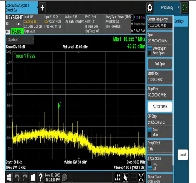
NTNV_N7_PC3_15_20_L_TID4_N/A_0.15_30_#1
