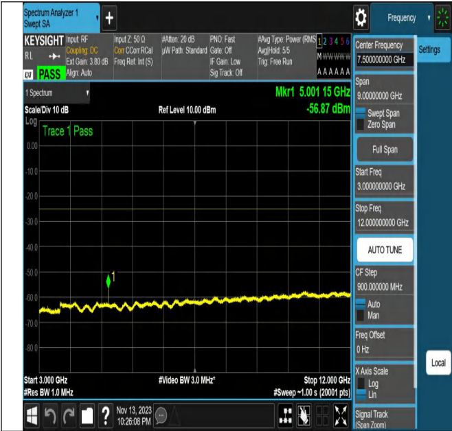
NTNV_N7_PC3_15_20_L_TID5_N/A_3000_12000_#1
