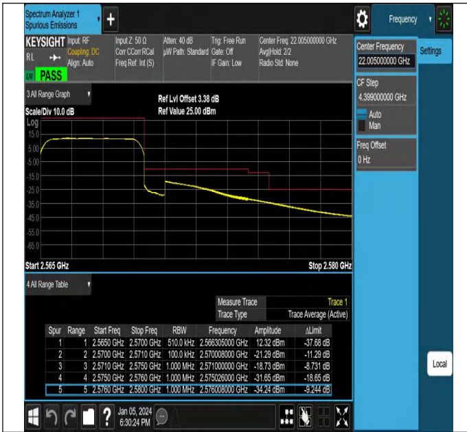
NTNV_N7_PC3_15_5_H_TID4_#1
