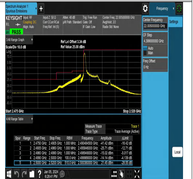
NTNV_N7_PC3_15_5_L_TID23_#1
