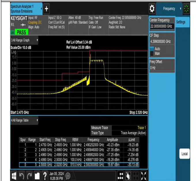
NTNV_N7_PC3_15_5_L_TID10_#1
