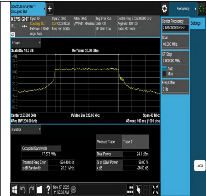
NTNV_N7_PC3_15_20_M_TID1_Ant1#1
