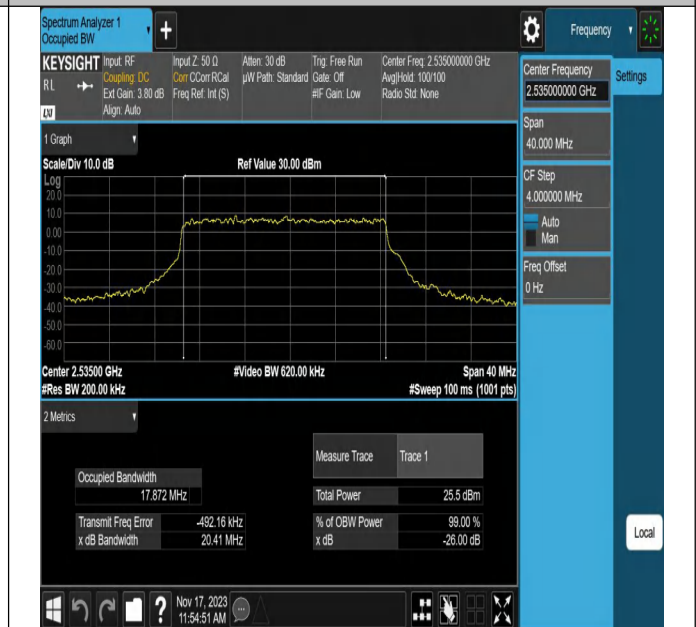
NTNV_N7_PC3_15_20_M_TID4_Ant1#1
