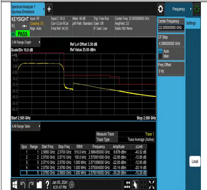
NTNV_N7_PC3_15_5_H_TID13_#1
