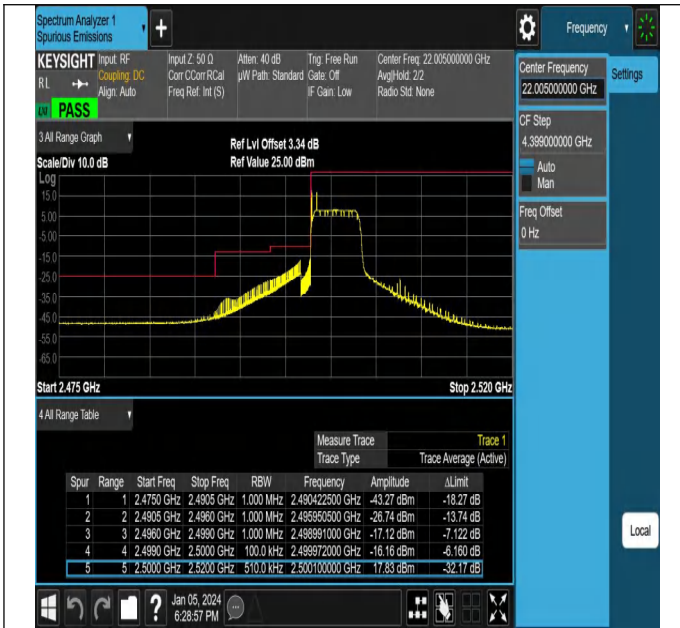
NTNV_N7_PC3_15_5_L_TID25_#1
