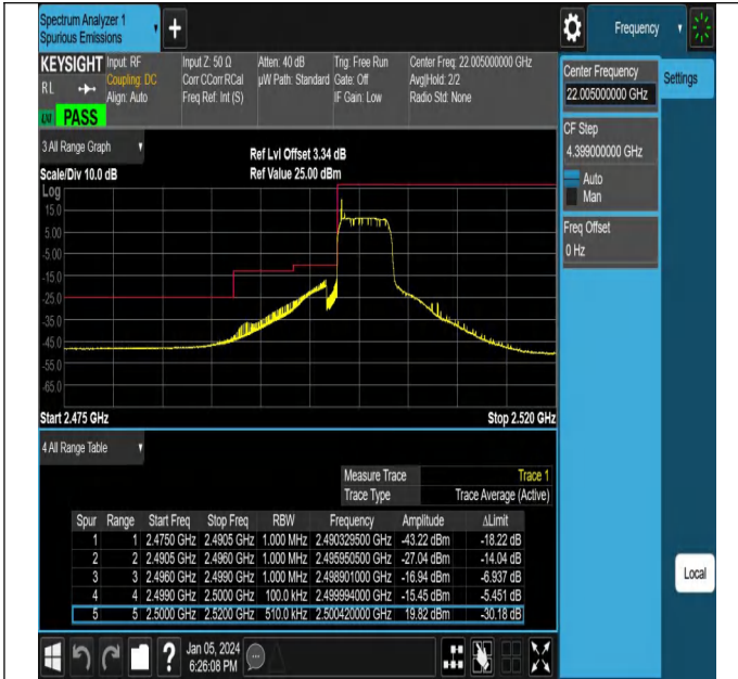
NTNV_N7_PC3_15_5_L_TID7_#1
