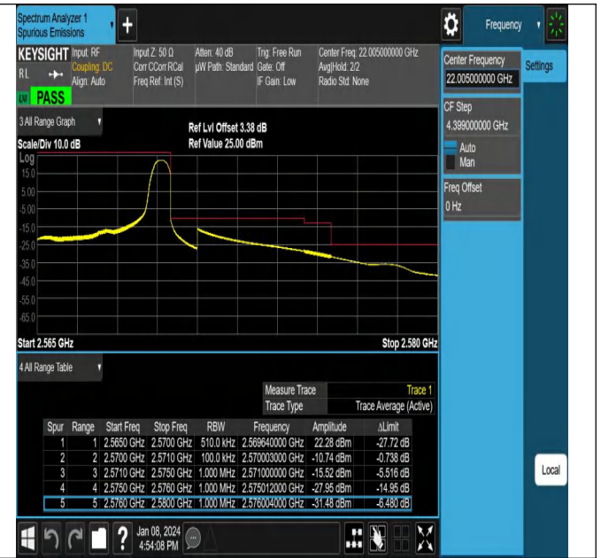
NTNV_N7_PC3_15_5_H_TID6_#1
