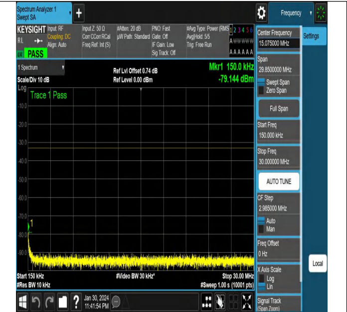
NTNV-N78-3450-3550-PC2-30-100-M-CP-64QAM-Edge_1RB _Right-Ant2-PASS
