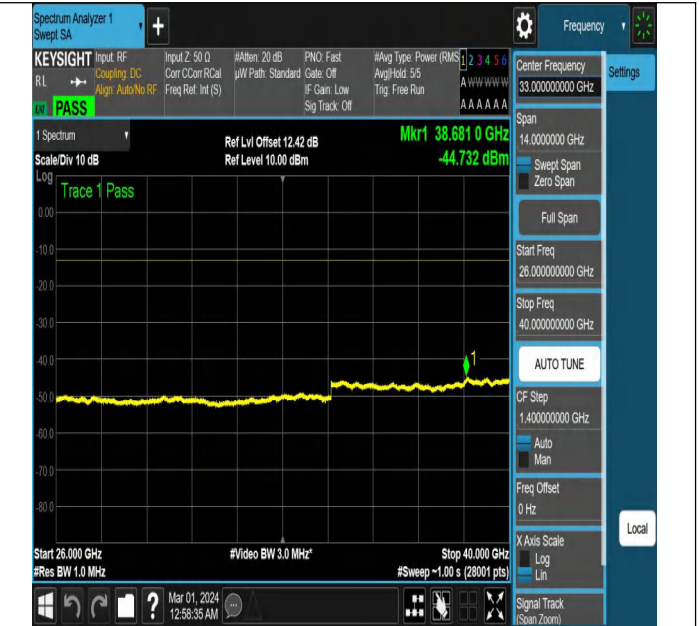
NTNV-N78-3450-3550-PC2-30-100-M-CP-16QAM-Edge_1RB _Right-Ant2-PASS
