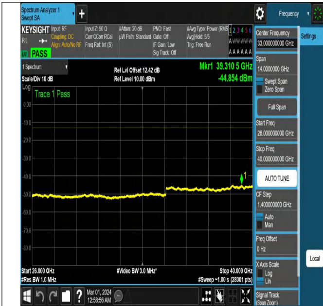
NTVN-N78-3450-3550-PC2-30-100-M-CP-64QAM-Outer_Full-Ant2-PASS
