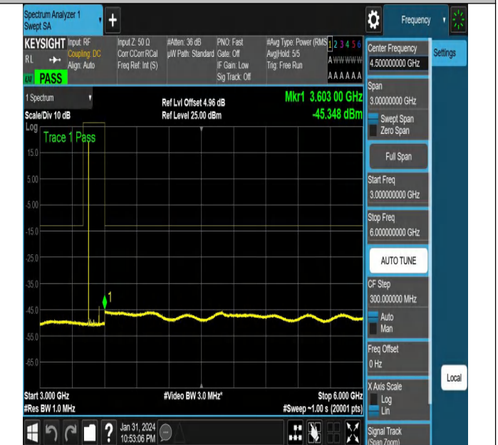
NTNV-N78-3450-3550-PC2-30-100-H-CP-QPSK-Edge_1RB_L
