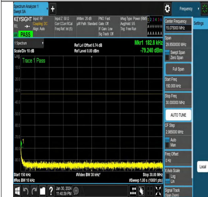
NTVN-N78-3450-3550-PC2-30-100-M-CP-64QAM-Edge_1RB_Left-Ant2-PASS
