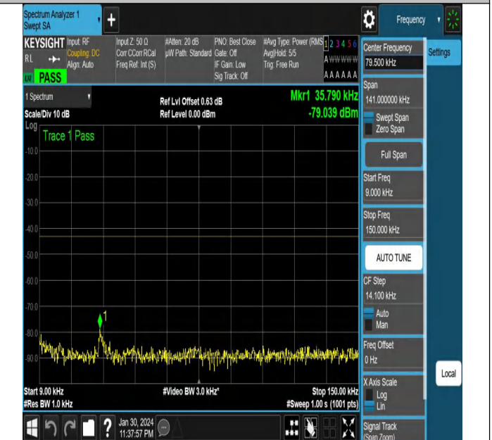
NTNV-N78-3450-3550-PC2-30-100-M-CP-16QAM-Edge_1RB _Right-Ant2-PASS
