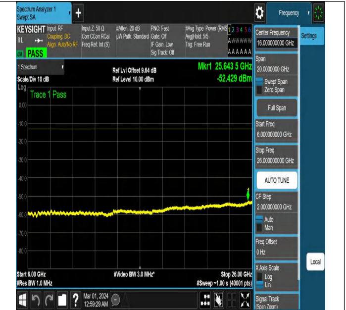
NTNV-N78-3450-3550-PC2-30-100-M-CP-64QAM-Edge_1RB _Right-Ant2-PASS
