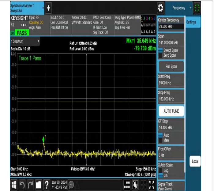
NTNV-N78-3450-3550-PC2-30-100-M-CP-256QAM-Edge_1R B_Right-Ant2-PASS
