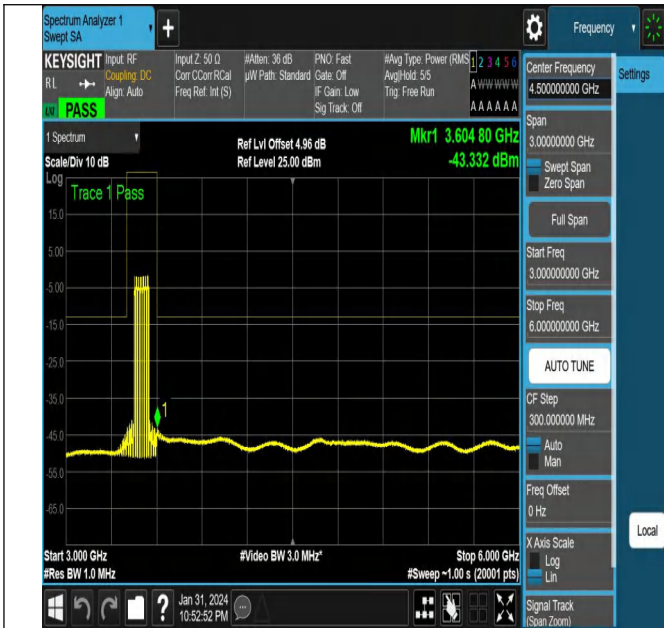
NTNV-N78-3450-3550-PC2-30-100-H-CP-QPSK-Outter_Full-A nt2-PASS
