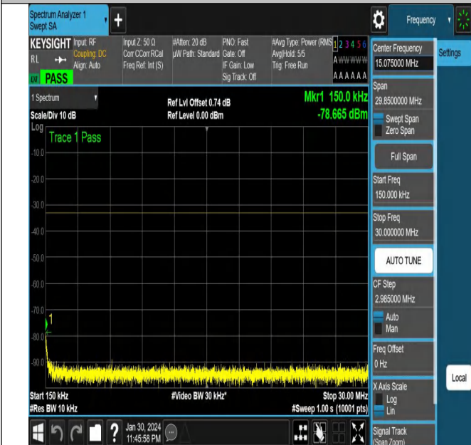
NTNV-N78-3450-3550-PC2-30-100-M-CP-256QAM-Edge_1R B_Right-Ant2-PASS
