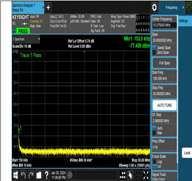
NTNV-N78-3450-3550-PC2-30-100-M-CP-16QAM-Edge_1RB _Right-Ant2-PASS
