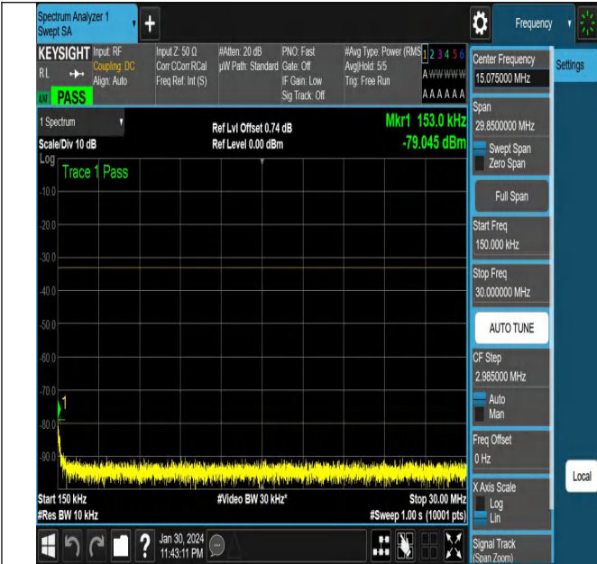
NTNV-N78-3450-3550-PC2-30-100-M-CP-256QAM-Outer_Full -Ant2-PASS
