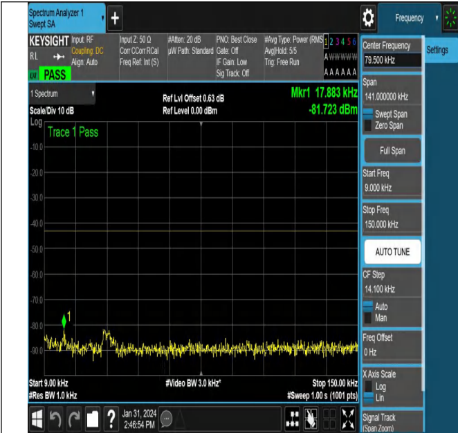
NTNV-N78-3450-3550-PC2-30-100-H-CP-QPSK-Outer_Full-A nt2-PASS
