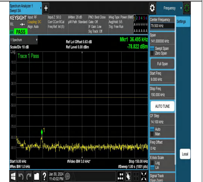
NTNV-N78-3450-3550-PC2-30-100-M-CP-256QAM-Outer_Full -Ant2-PASS
