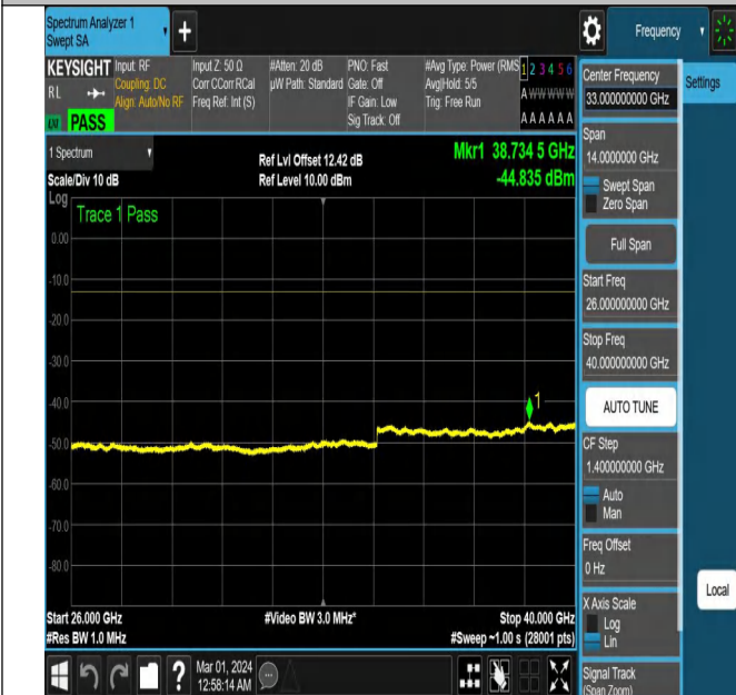
NTNV-N78-3450-3550-PC2-30-100-M-CP-16QAM-Edge_1RB _Left-Ant2-PASS
