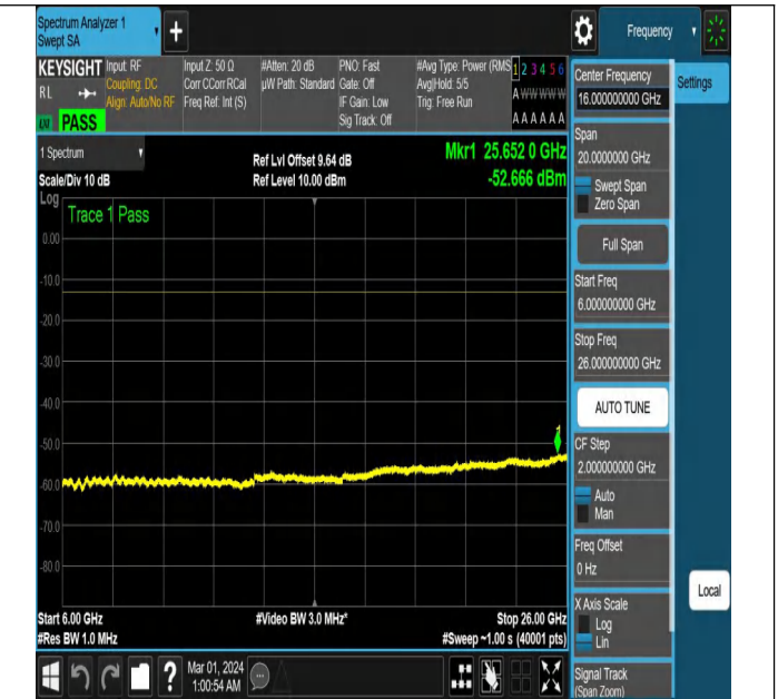
NTNV-N78-3450-3550-PC2-30-100-H-CP-QPSK-Outter_Full-A nt2-PASS
