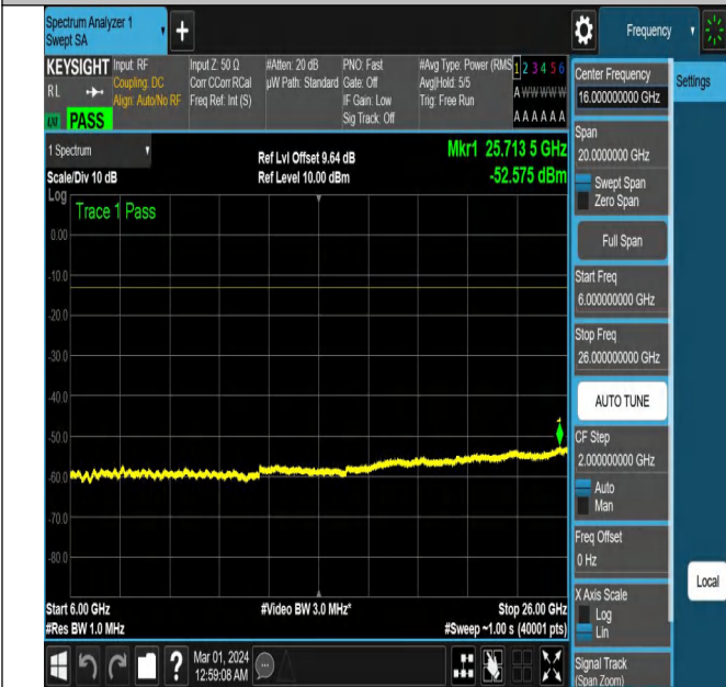
NTNV-N78-3450-3550-PC2-30-100-M-CP-64QAM-Edge_1RB _Left-Ant2-PASS
