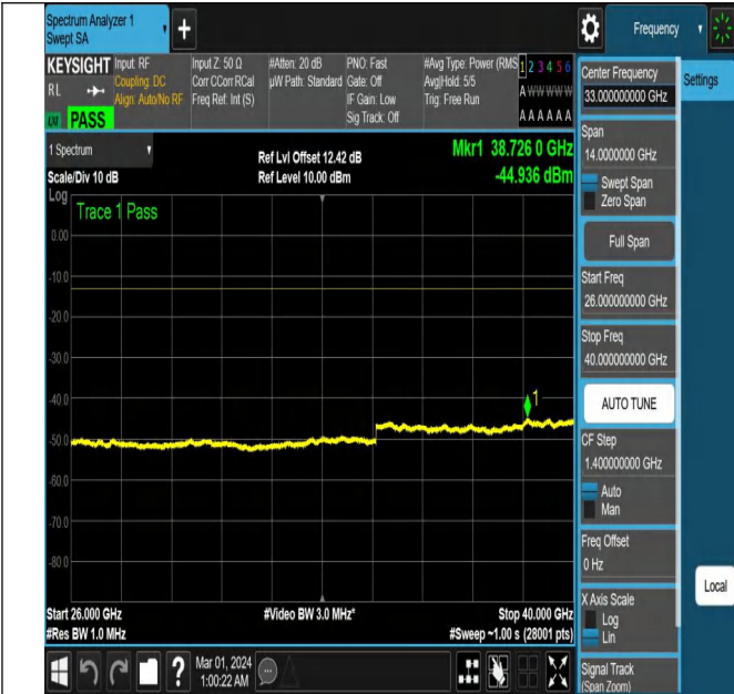
NTNV-N78-3450-3550-PC2-30-100-M-CP-256QAM-Edge_1R B_Left-Ant2-PASS
