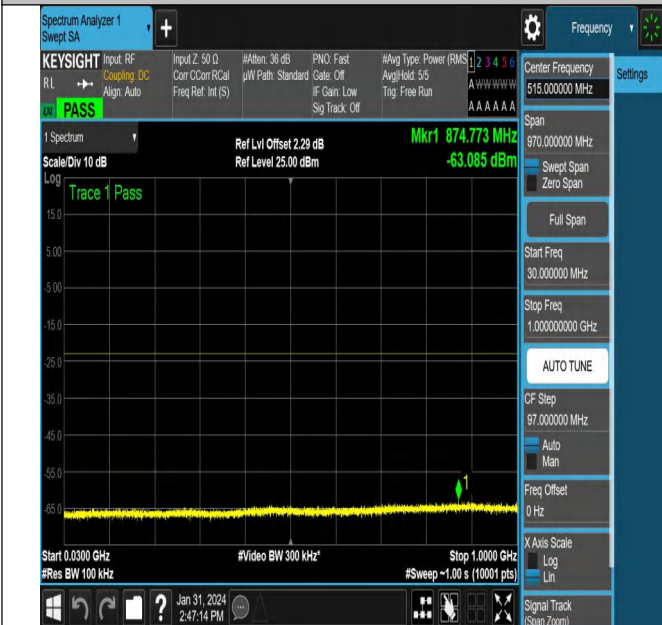
NTNV-N78-3450-3550-PC2-30-100-H-CP-QPSK-Outer_Full-A nt2-PASS
