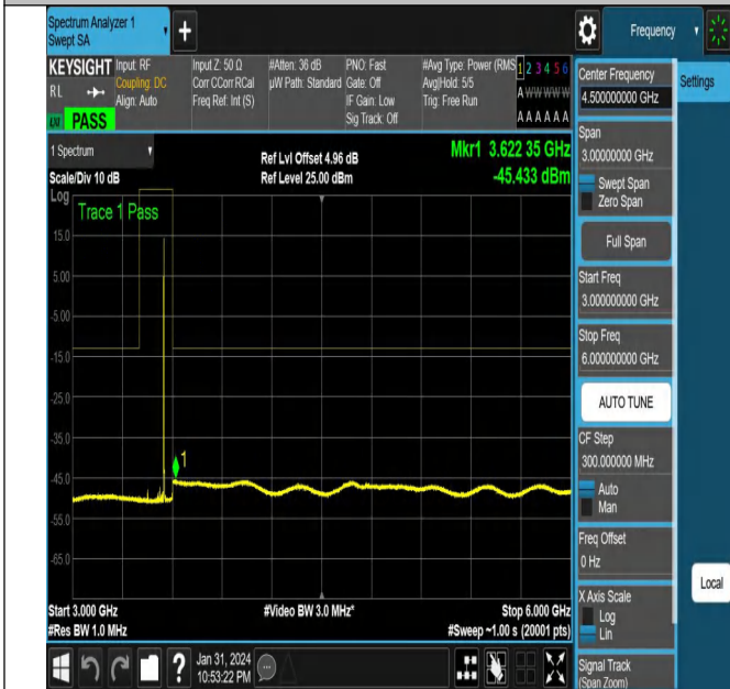
NTNV-N78-3450-3550-PC2-30-100-H-CP-QPSK-Edge_1RB_ Right-Ant2-PASS
