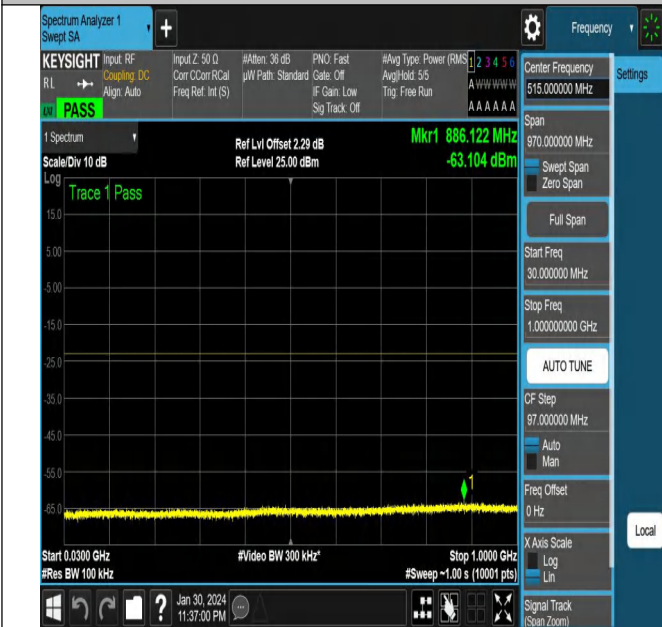
NTNV-N78-3450-3550-PC2-30-100-M-CP-16QAM-Edge_1RB _Left-Ant2-PASS
