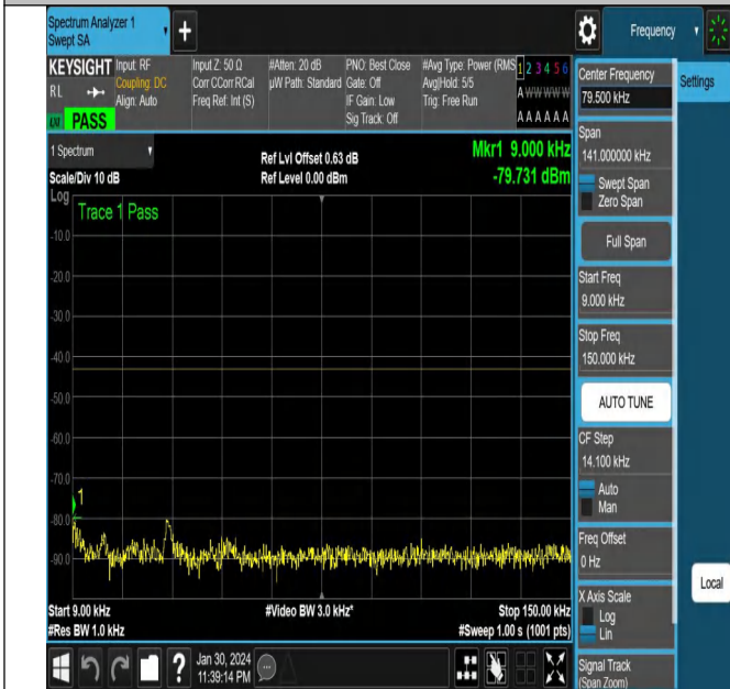
NTNV-N78-3450-3550-PC2-30-100-M-CP-64QAM-Outer_Full- Ant2-PASS
