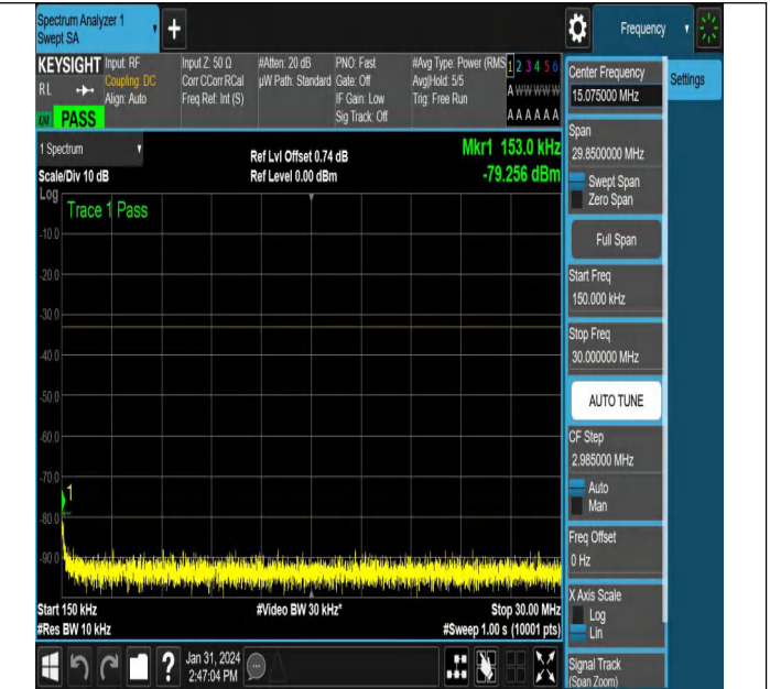
NTNV-N78-3450-3550-PC2-30-100-H-CP-QPSK-Outer_Full-A nt2-PASS
