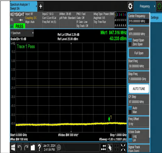
NTNV-N78-3450-3550-PC2-30-100-L-CP-QPSK-Edge_1RB_R
