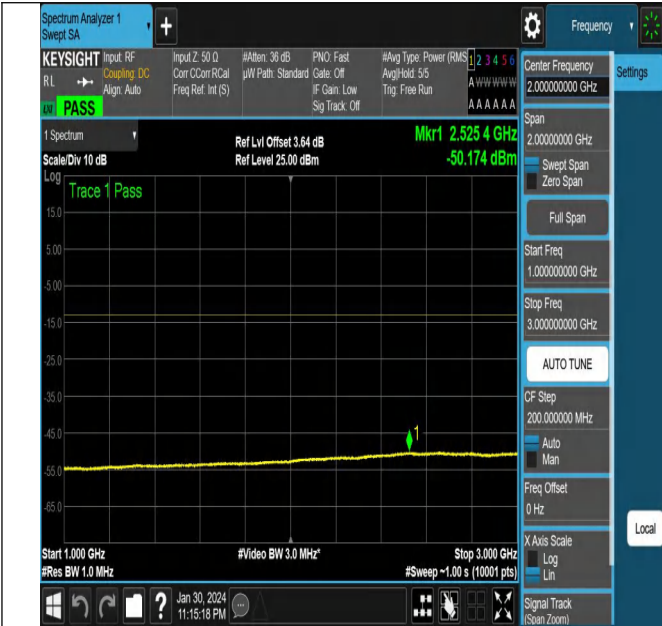
NTNV-N78-3450-3550-PC2-30-100-H-CP-256QAM-Edge_1RB _Right-Ant1-PASS
