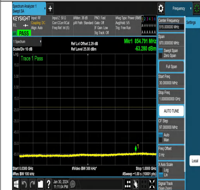
NTNV-N78-3450-3550-PC2-30-100-H-CP-64QAM-Edge_1RB_
