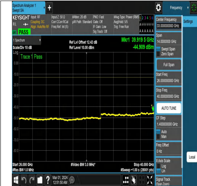
NTVN-N78-3450-3550-PC2-30-100-H-CP-256QAM-Edge_1RB _Left-Ant1-PASS
