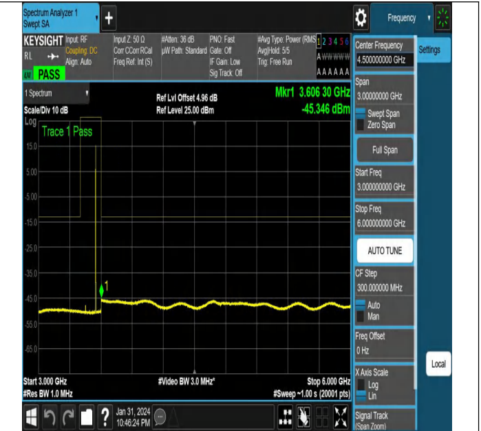
NTNV-N78-3450-3550-PC2-30-100-H-CP-256QAM-Edge_1RB _Right-Ant1-PASS
