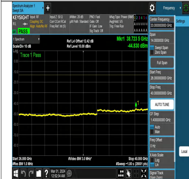
NTVN-N78-3450-3550-PC2-30-100-L-CP-QPSK-Outer_Full-An t2-PASS
