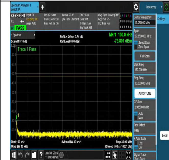
NTNV-N78-3450-3550-PC2-30-100-H-CP-64QAM-Edge_1RB_Left-Ant1-PASS
