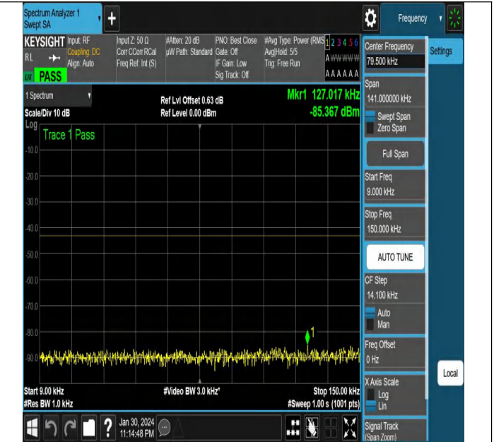
NTVN-N78-3450-3550-PC2-30-100-H-CP-256QAM-Edge_1RB _Right-Ant1-PASS
