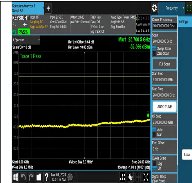
NTVN-N78-3450-3550-PC2-30-100-H-CP-256QAM-Outer_Full -Ant1-PASS
