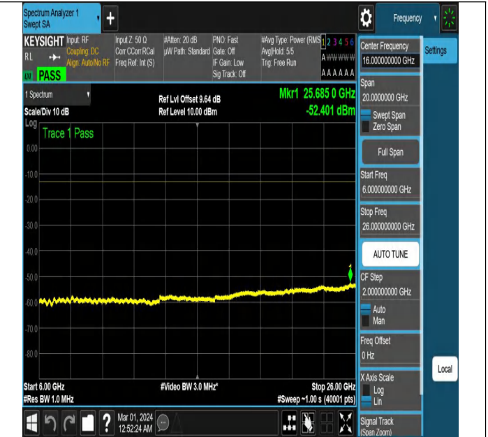
NTVN-N78-3450-3550-PC2-30-100-L-CP-QPSK-Outer_Full-An t2-PASS
