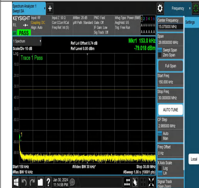
NTVN-N78-3450-3550-PC2-30-100-H-CP-256QAM-Edge_1RB _Right-Ant1-PASS
