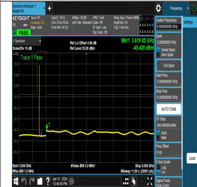
NTNV-N78-3450-3550-PC2-30-100-H-CP-256QAM-Edge_1RB _Left-Ant1-PASS
