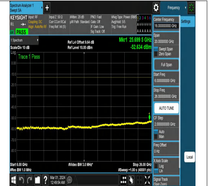
NTNV-N78-3450-3550-PC2-30-100-H-CP-16QAM-Edge_1RB_
