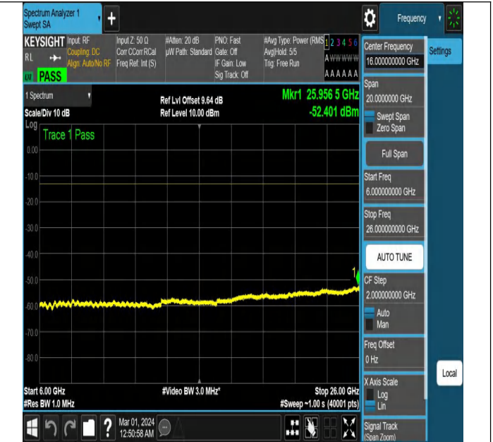
NTVN-N78-3450-3550-PC2-30-100-H-CP-64QAM-Edge_1RB_
