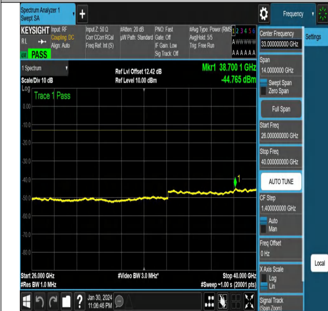
NTNV-N78-3450-3550-PC2-30-100-H-CP-16QAM-Edge_1RB_
