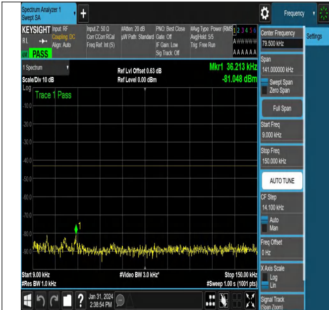
NTNV-N78-3450-3550-PC2-30-100-L-CP-QPSK-Outer_Full-An t2-PASS
