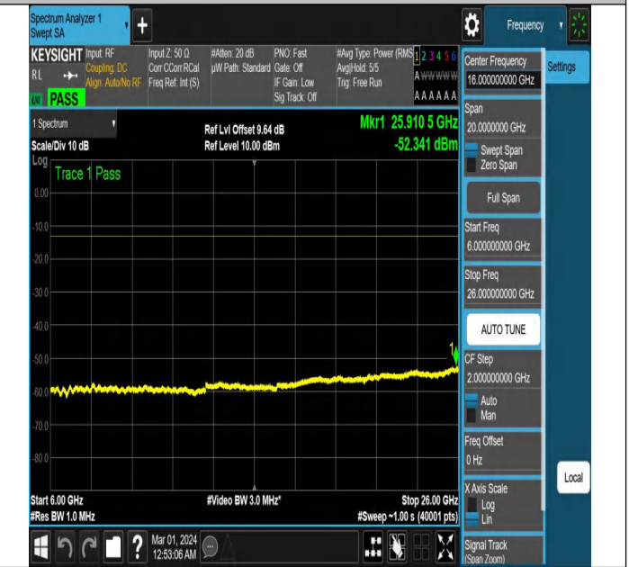
NTNV-N78-3450-3550-PC2-30-100-L-CP-QPSK-Edge_1RB_R
