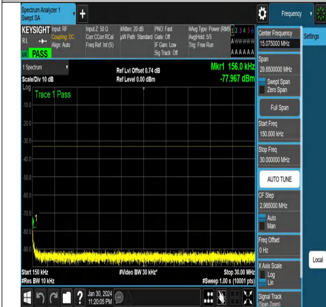
NTVN-N78-3450-3550-PC2-30-100-L-CP-16QAM-Outer_Full-A nt2-PASS
