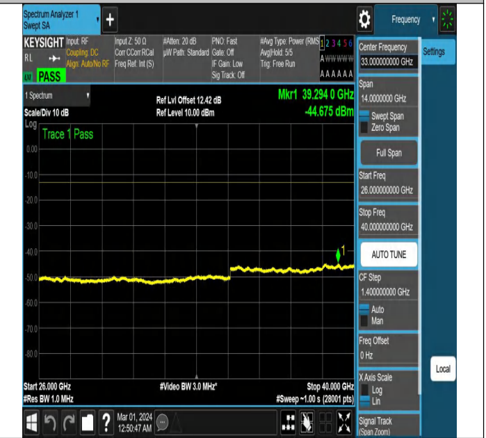
NTNV-N78-3450-3550-PC2-30-100-H-CP-64QAM-Edge_1RB_
