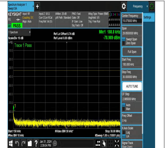
NTNV-N78-3450-3550-PC2-30-100-L-CP-QPSK-Outer_Full-An t2-PASS
