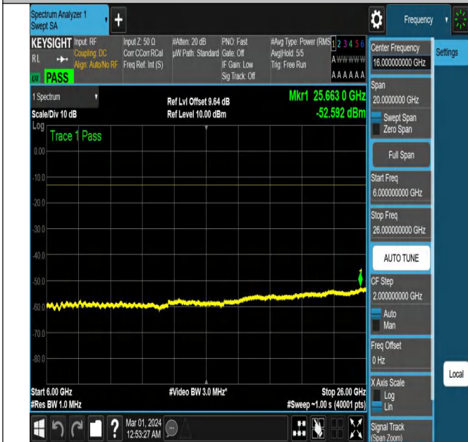
NTNV-N78-3450-3550-PC2-30-100-L-CP-16QAM-Outer_Full-A
