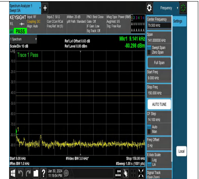
NTVN-N78-3450-3550-PC2-30-100-L-CP-16QAM-Outer_Full-A nt2-PASS
