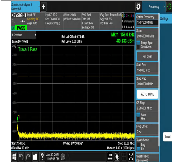
NTNV-N78-3450-3550-PC2-30-100-H-CP-16QAM-Edge_1RB_ Right-Ant1-PASS
