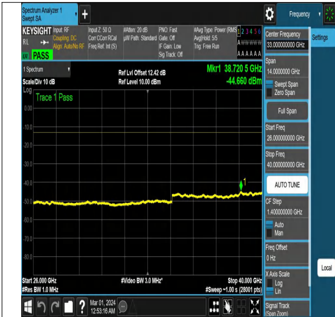
NTVN-N78-3450-3550-PC2-30-100-L-CP-QPSK-Edge_1RB_R ight-Ant2-PASS
