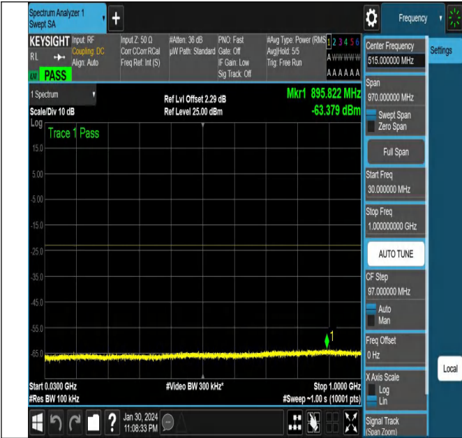
NTNV-N78-3450-3550-PC2-30-100-H-CP-64QAM-Outer_Full
