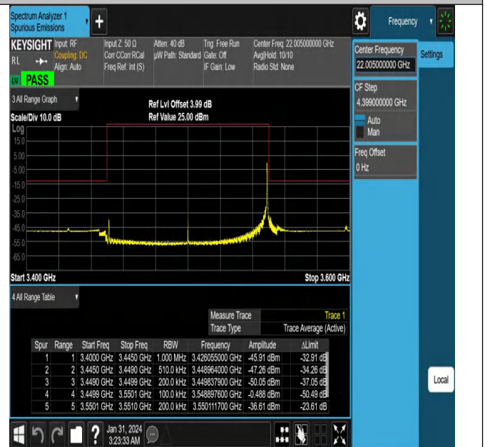
NTNV_N78-3450-3550_PC2_30_100_H_TID12_#1
