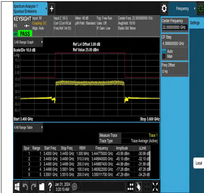
NTNV_N78-3450-3550_PC2_30_100_H_TID7_#1
