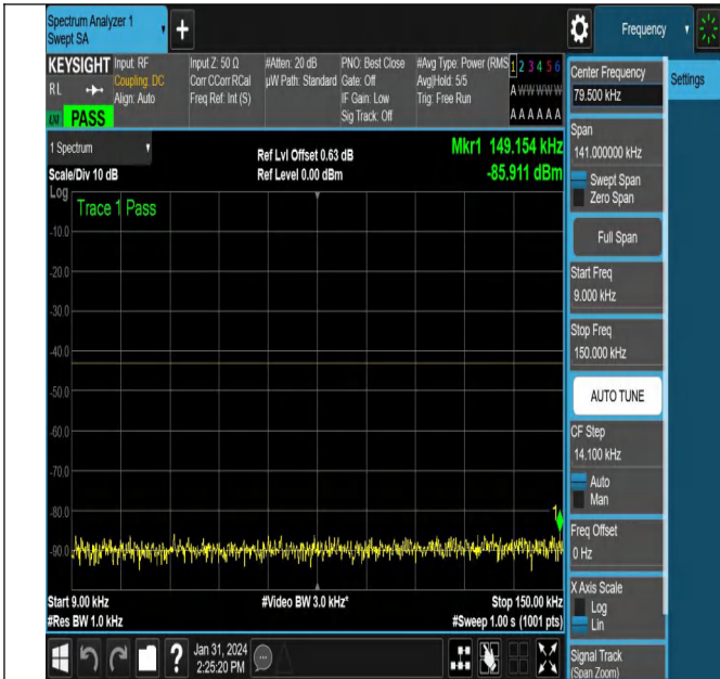
NTNV-N78-3450-3550-PC2-30-100-L-CP-QPSK-Outer_Full-An t1-PASS
