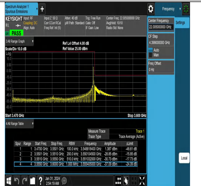
NTNV_N78-3450-3550_PC2_30_80_H_TID6_#1
