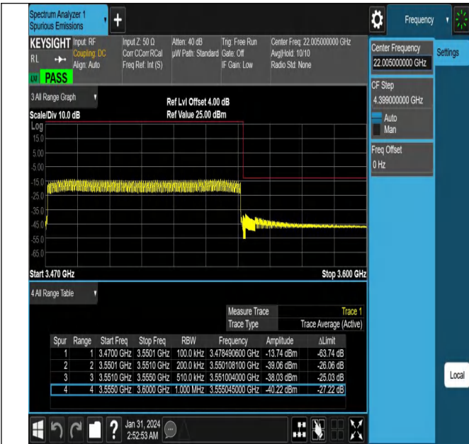
NTNV_N78-3450-3550_PC2_30_80_H_TID1_#1
