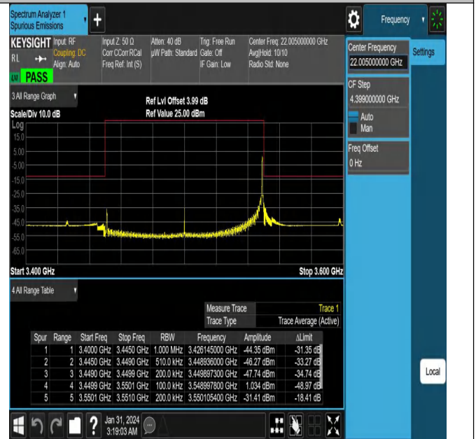
NTNV_N78-3450-3550_PC2_30_100_H_TID6_#1
