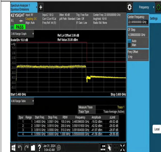
NTNV_N78-3450-3550_PC2_30_90_H_TID10_#1
