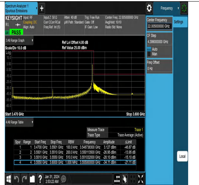
NTNV_N78-3450-3550_PC2_30_80_H_TID3_#1
