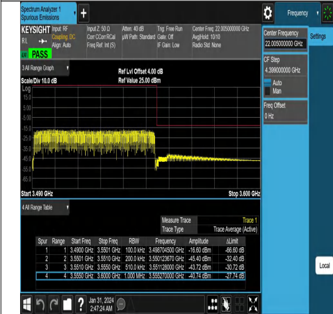
NTNV_N78-3450-3550_PC2_30_60_H_TID10_#1
