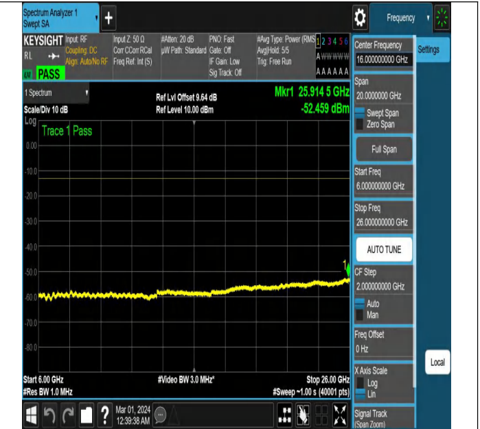
NTNV-N78-3450-3550-PC2-30-100-L-CP-QPSK-Outer_Full-An t1-PASS
