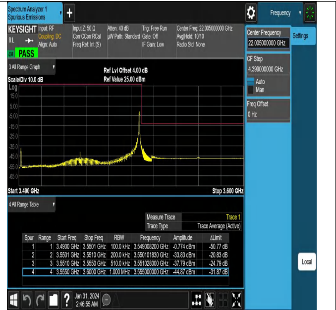
NTNV_N78-3450-3550_PC2_30_60_H_TID9_#1
