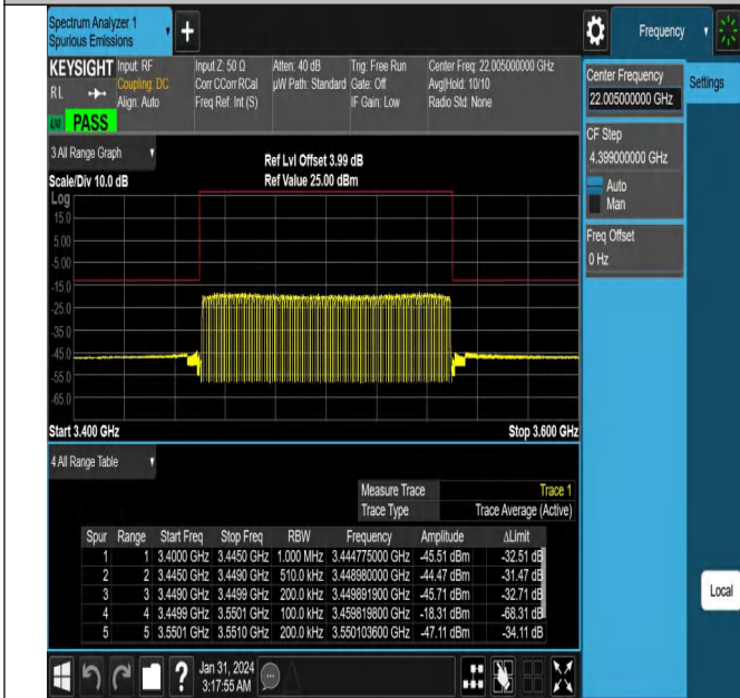
NTNV_N78-3450-3550_PC2_30_100_H_TID4_#1
