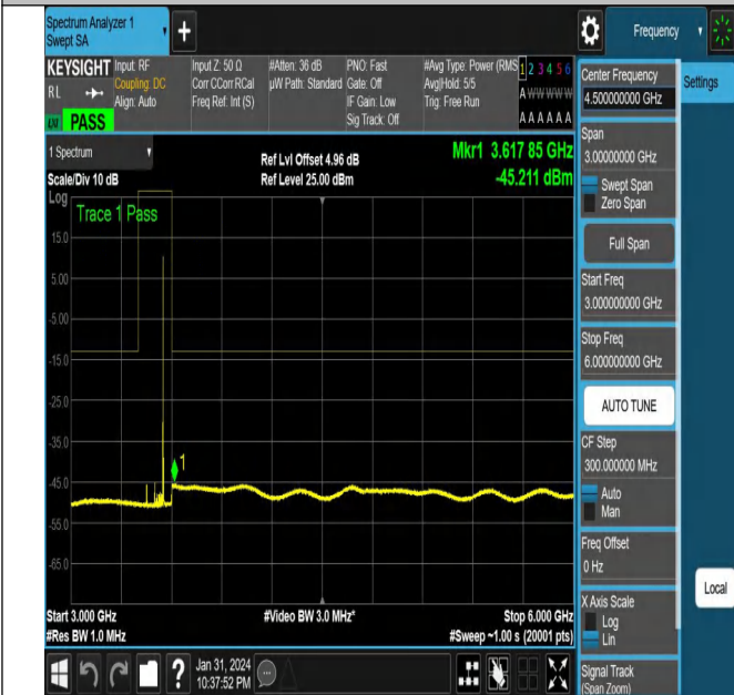
NTNV-N78-3450-3550-PC2-30-100-L-CP-QPSK-Edge_1RB_R ight-Ant1-PASS
