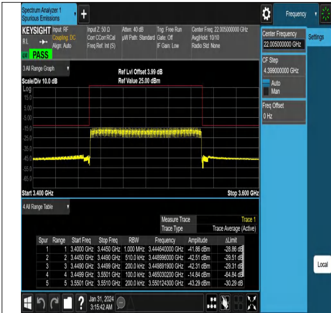
NTNV_N78-3450-3550_PC2_30_100_H_TID1_#1
