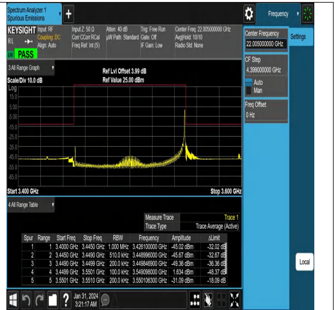
NTNV_N78-3450-3550_PC2_30_100_H_TID9_#1
