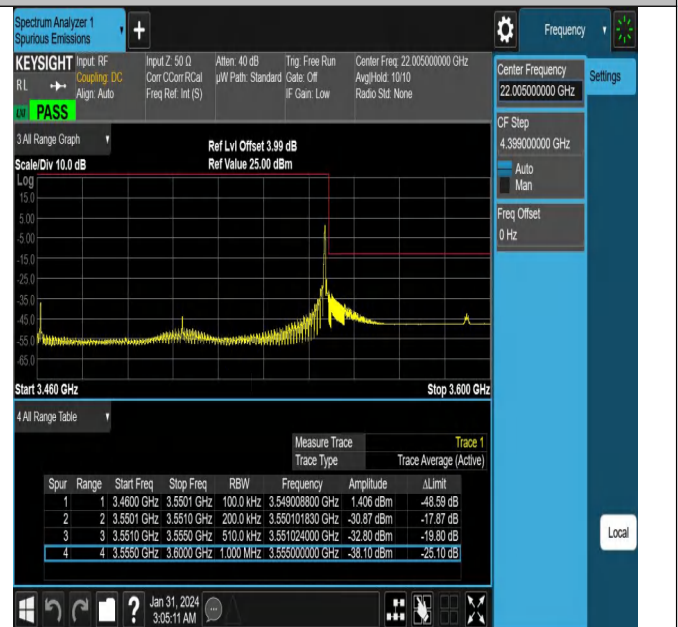
NTNV_N78-3450-3550_PC2_30_90_H_TID12_#1
