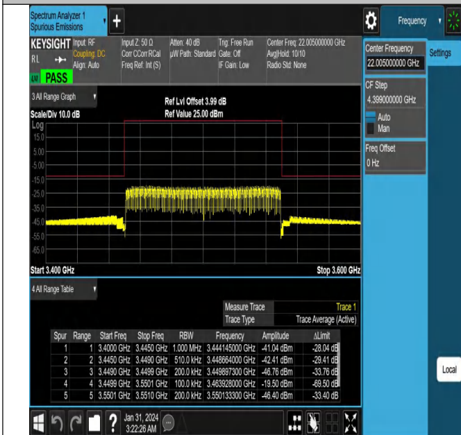
NTNV_N78-3450-3550_PC2_30_100_H_TID10_#1
