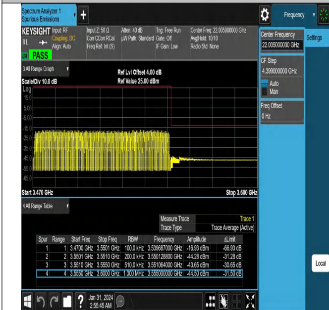
NTNV_N78-3450-3550_PC2_30_80_H_TID10_#1
