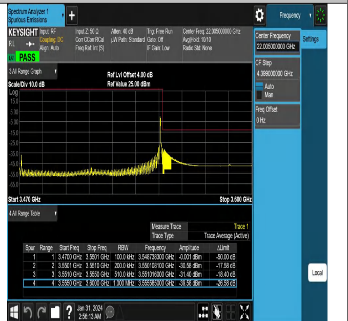
NTNV_N78-3450-3550_PC2_30_80_H_TID12_#1
