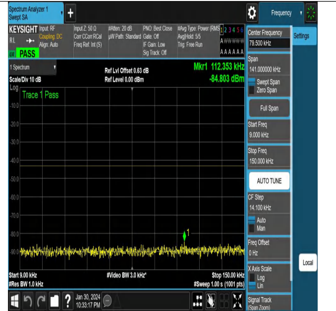
NTVN-N78-3450-3550-PC2-30-100-L-CP-16QAM-Outer_Full-A nt1-PASS
