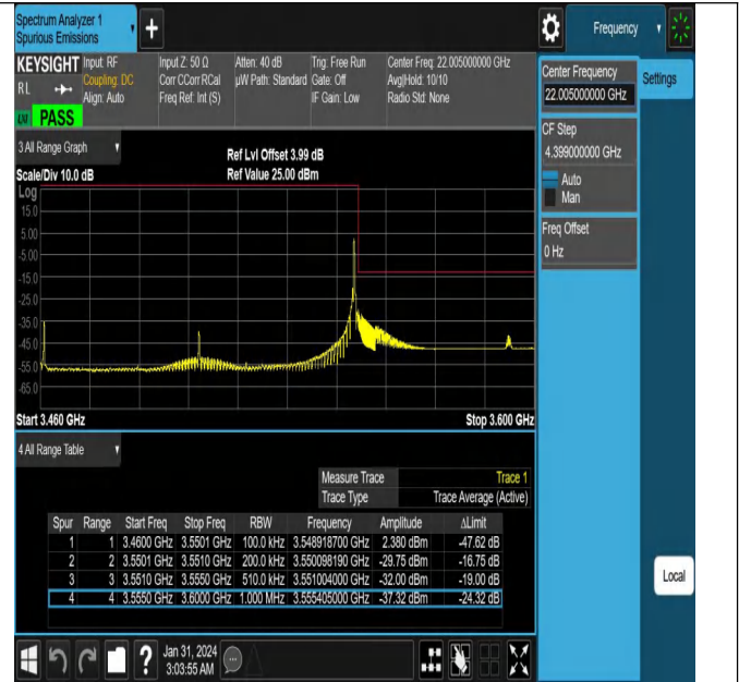
NTNV_N78-3450-3550_PC2_30_90_H_TID9_#1
