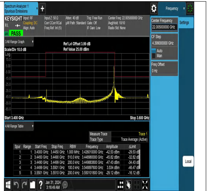
NTNV_N78-3450-3550_PC2_30_100_H_TID3_#1
