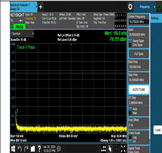
NTVN-N78-3450-3550-PC2-30-100-L-CP-16QAM-Outer_Full-A nt1-PASS
