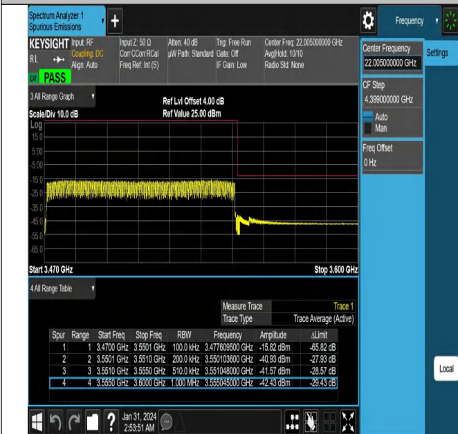
NTNV_N78-3450-3550_PC2_30_80_H_TID4_#1
